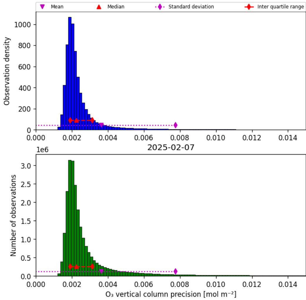
Figure 30: Histogram of "O 3 vertical column precision" for 2025-02-07 to 2025-02-08
