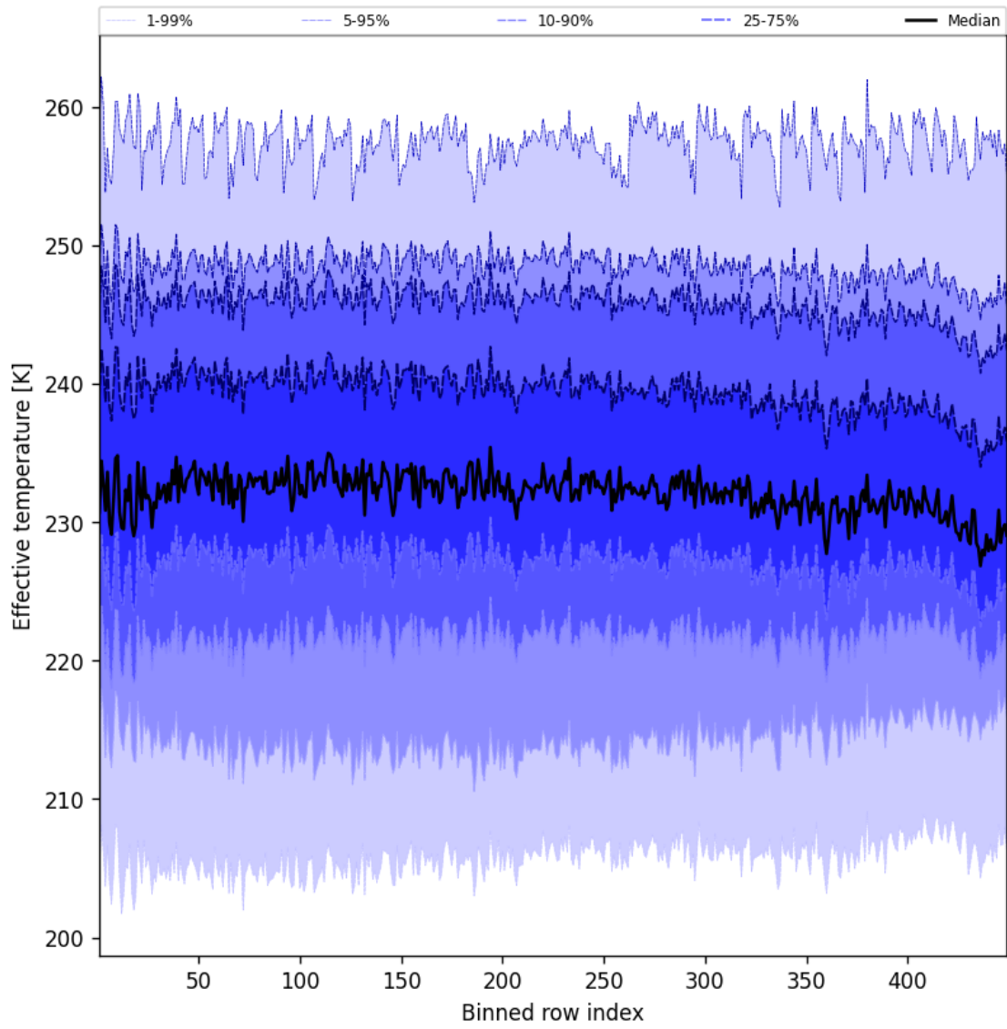
Figure 50: Along track statistics of “Effective temperature” for 2025-02-07 to 2025-02-08
