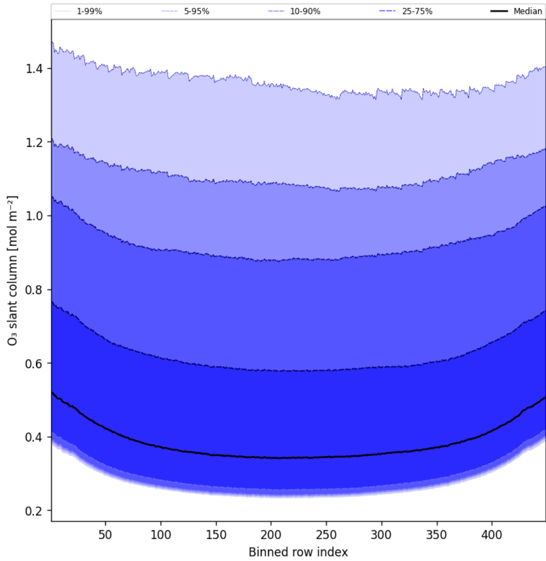
Figure 43: Along track statistics of “O 3 slant column” for 2025-02-07 to 2025-02-08
