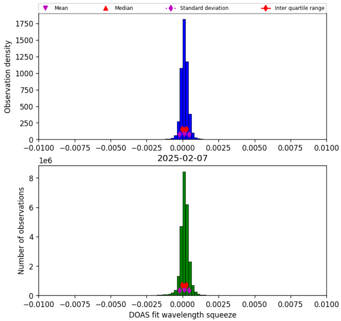
Figure 36: Histogram of “DOAS fit wavelength squeeze” for 2025-02-07 to 2025-02-08
