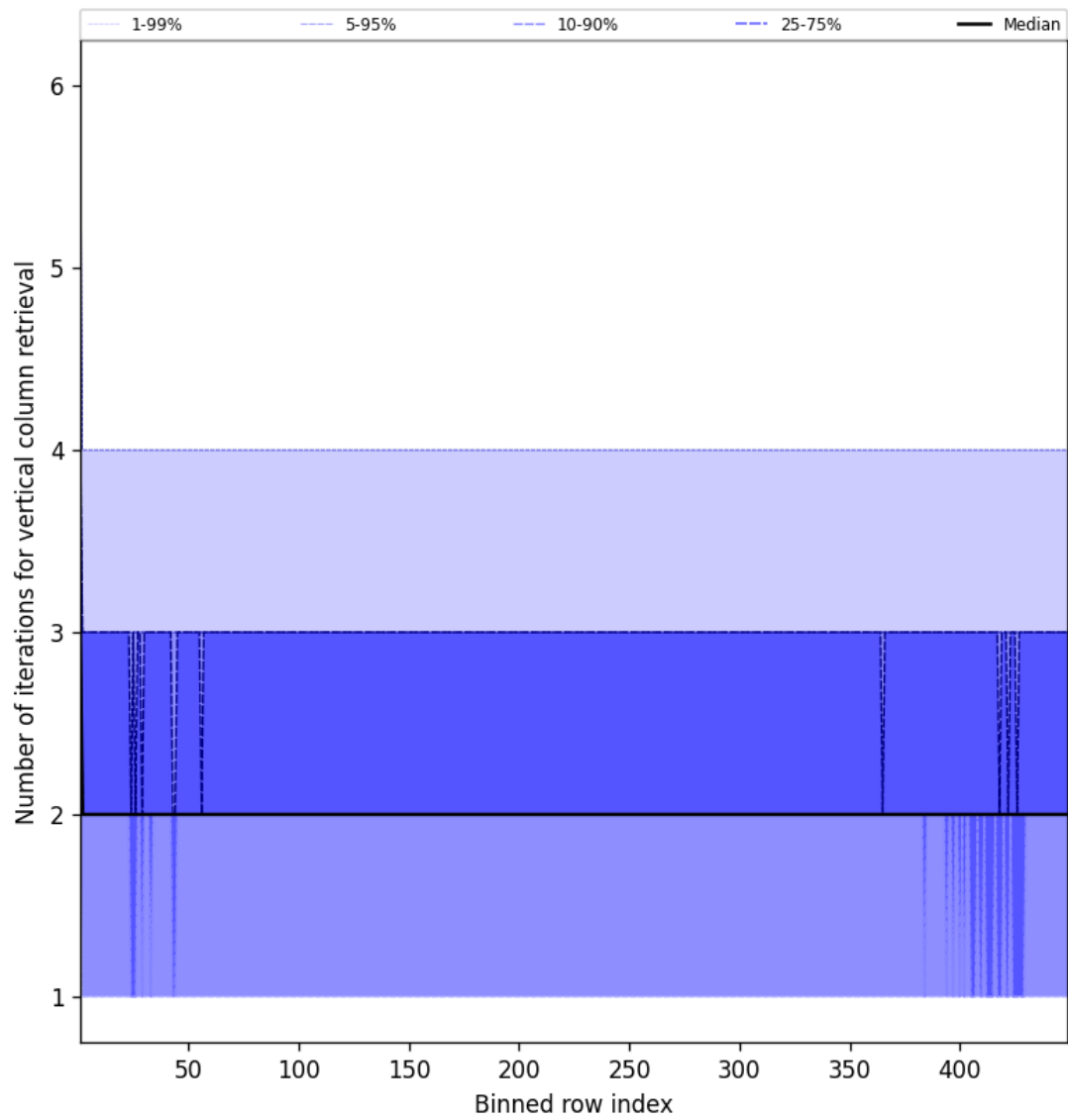
Figure 51: Along track statistics of “Number of iterations for vertical column retrieval” for 2025-02-07 to 2025-02-08
