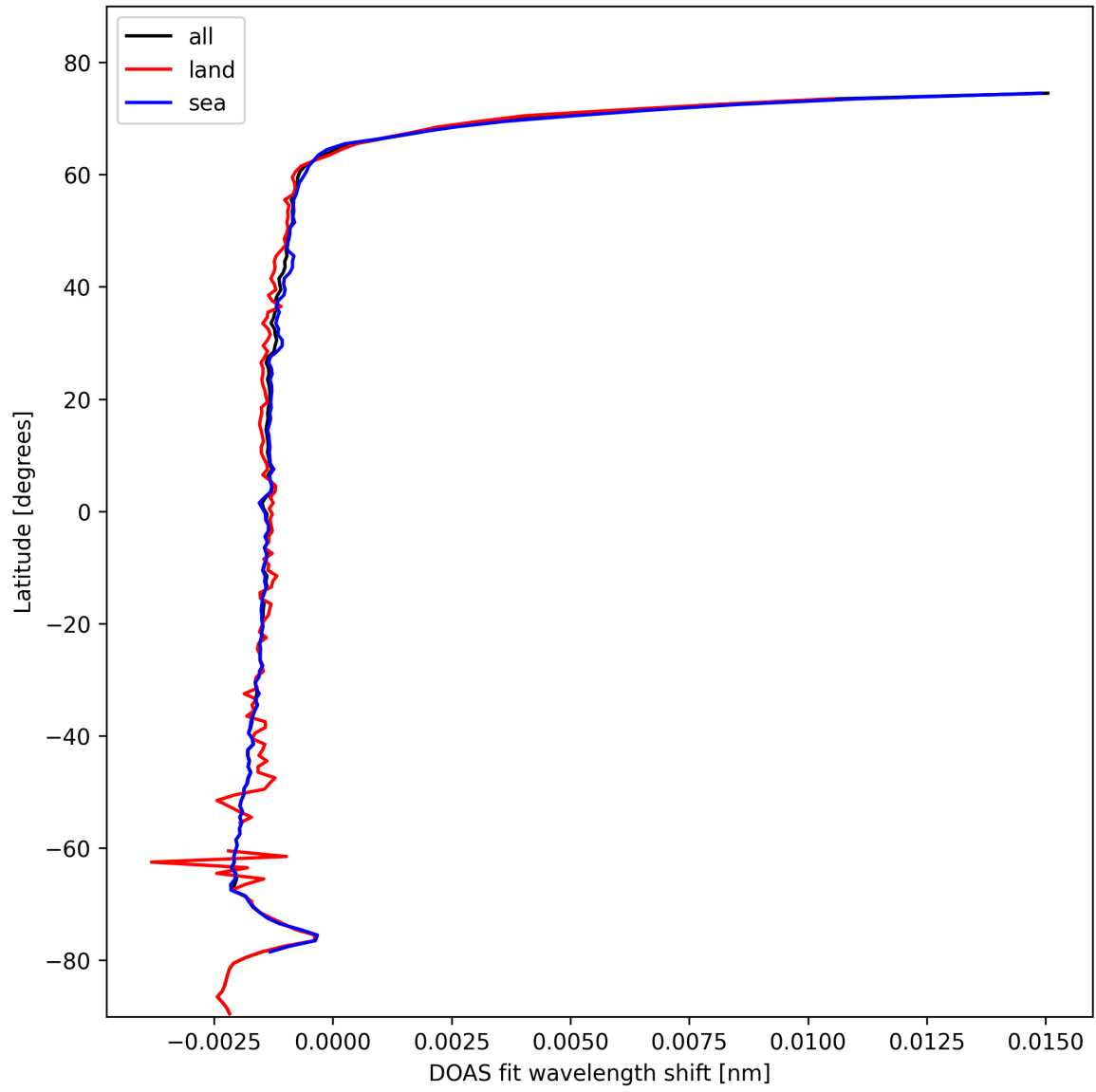
Figure 23: Zonal average of “DOAS fit wavelength shift” for 2025-02-07 to 2025-02-08.
