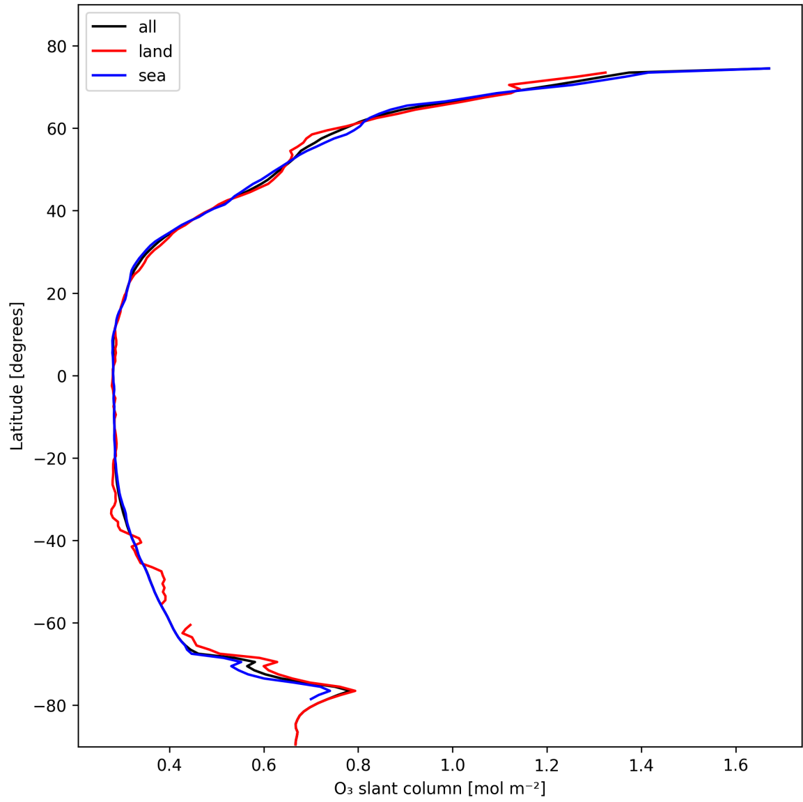
Figure 19: Zonal average of “O 3 slant column” for 2025-02-07 to 2025-02-08.
