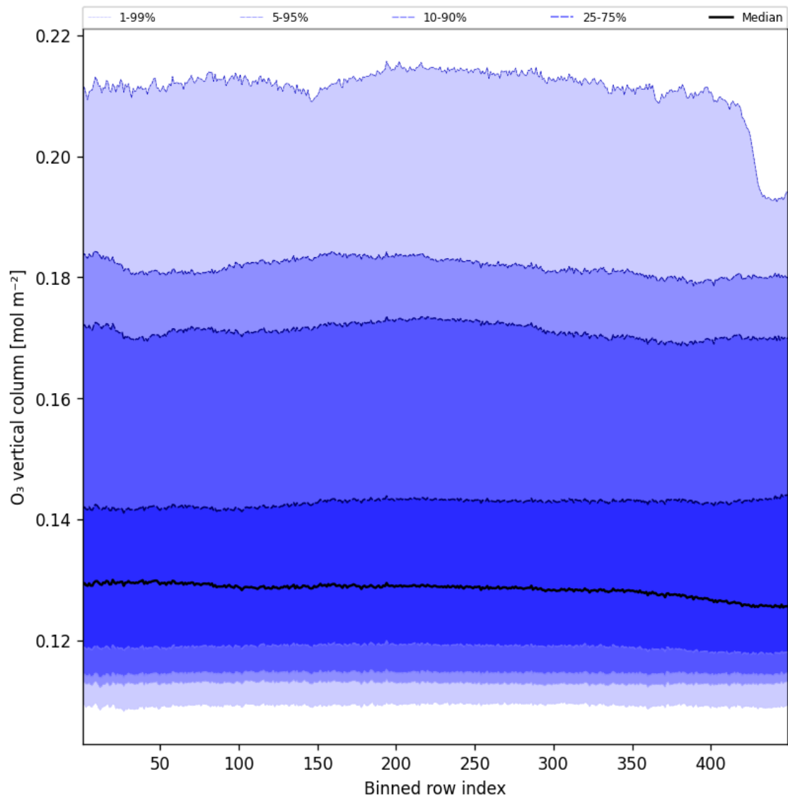
Figure 41: Along track statistics of “ \text{O}_3 vertical column” for 2025-02-07 to 2025-02-08
