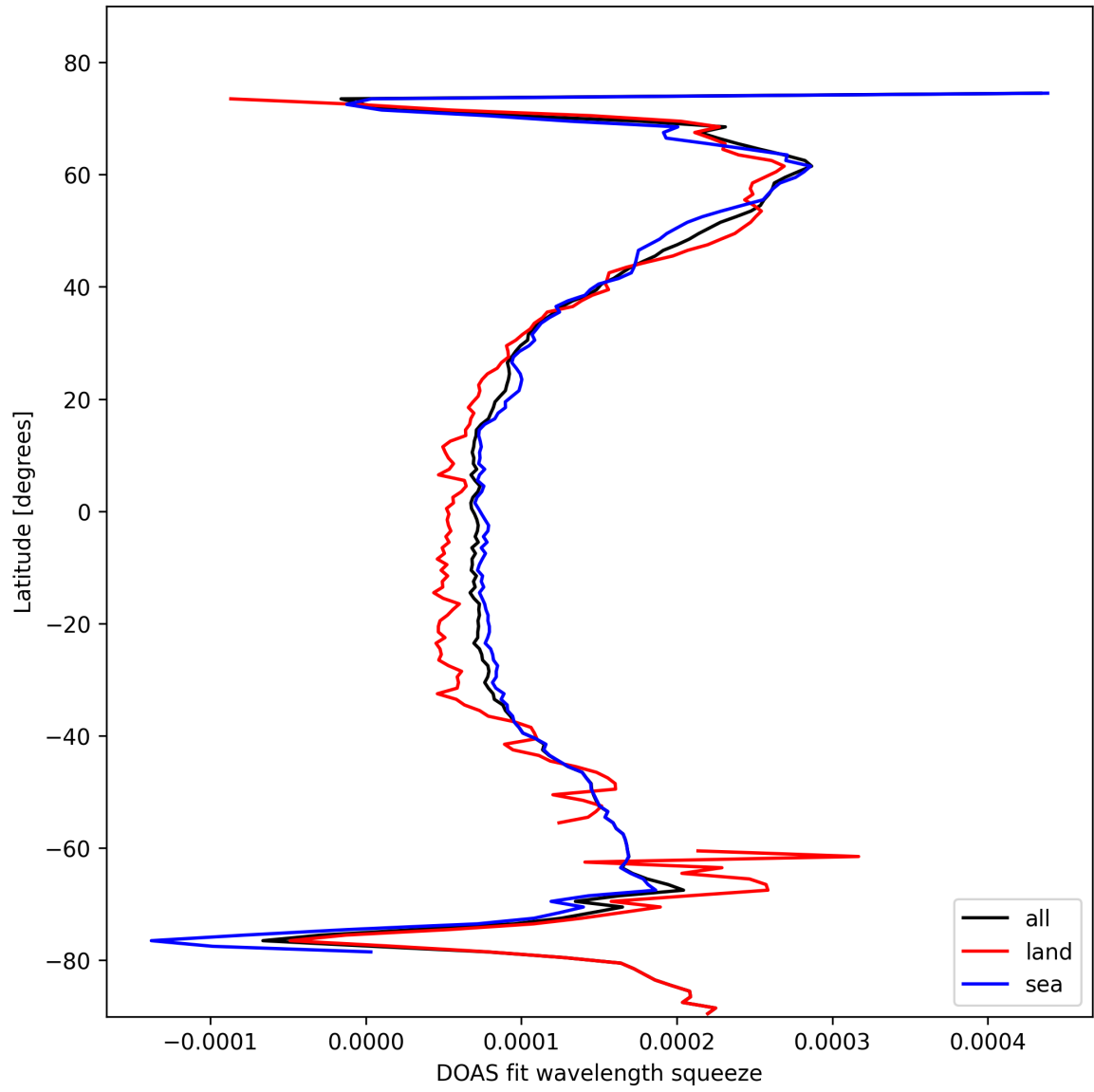
Figure 24: Zonal average of “DOAS fit wavelength squeeze” for 2025-02-07 to 2025-02-08.
