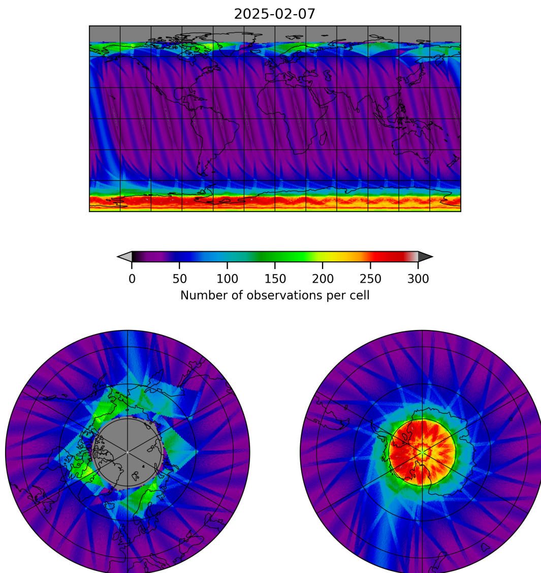
Figure 15: Map of the number of observations for 2025-02-07 to 2025-02-08
