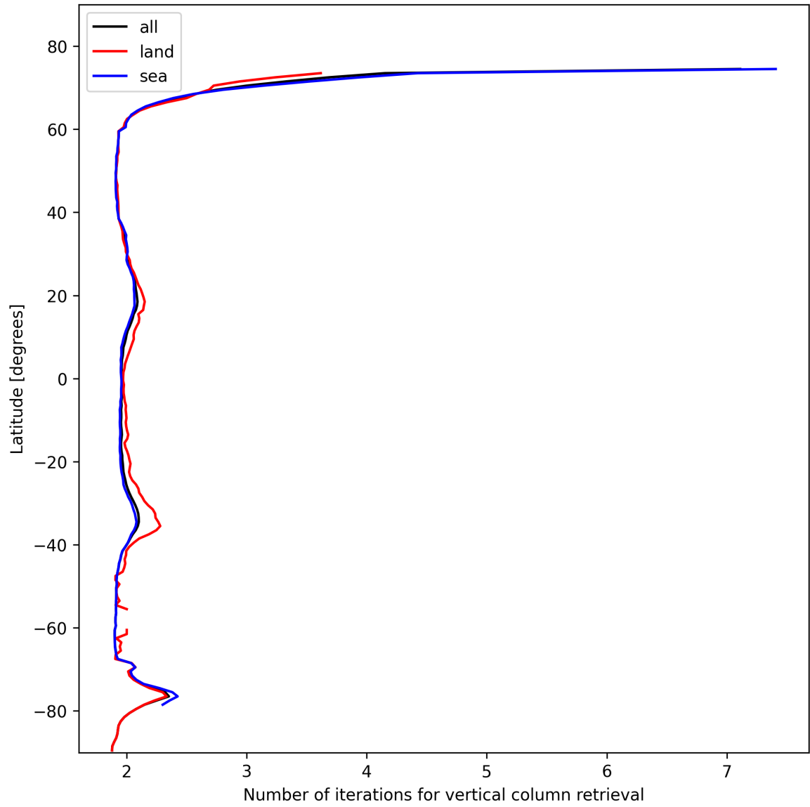
Figure 27: Zonal average of “Number of iterations for vertical column retrieval” for 2025-02-07 to 2025-02-08.
