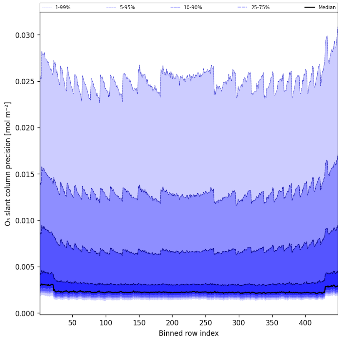
Figure 44: Along track statistics of “O 3 slant column precision” for 2025-02-07 to 2025-02-08
