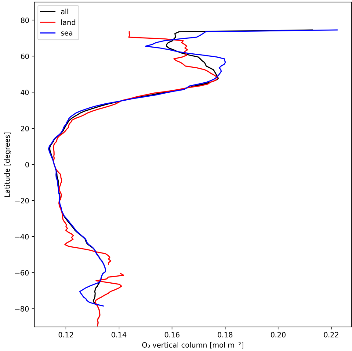
Figure 17: Zonal average of “O 3 vertical column” for 2025-02-07 to 2025-02-08.
