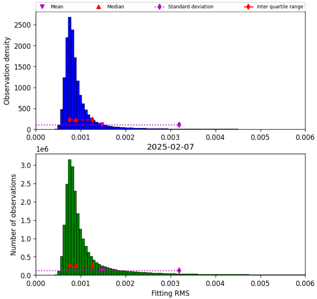
Figure 34: Histogram of “Fitting RMS” for 2025-02-07 to 2025-02-08
