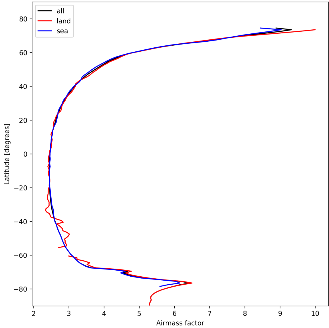
Figure 25: Zonal average of “Airmass factor” for 2025-02-07 to 2025-02-08.
