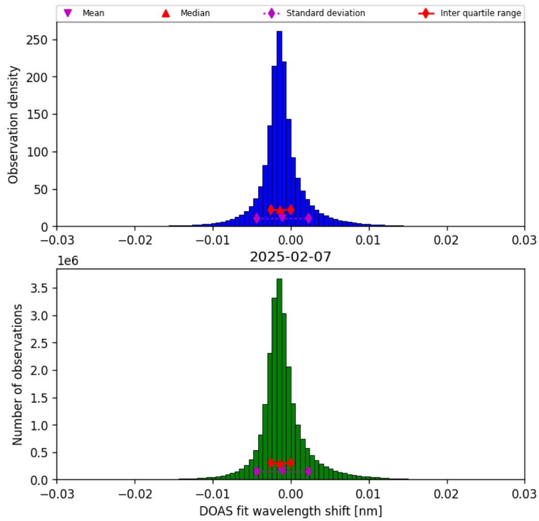
Figure 35: Histogram of “DOAS fit wavelength shift” for 2025-02-07 to 2025-02-08
