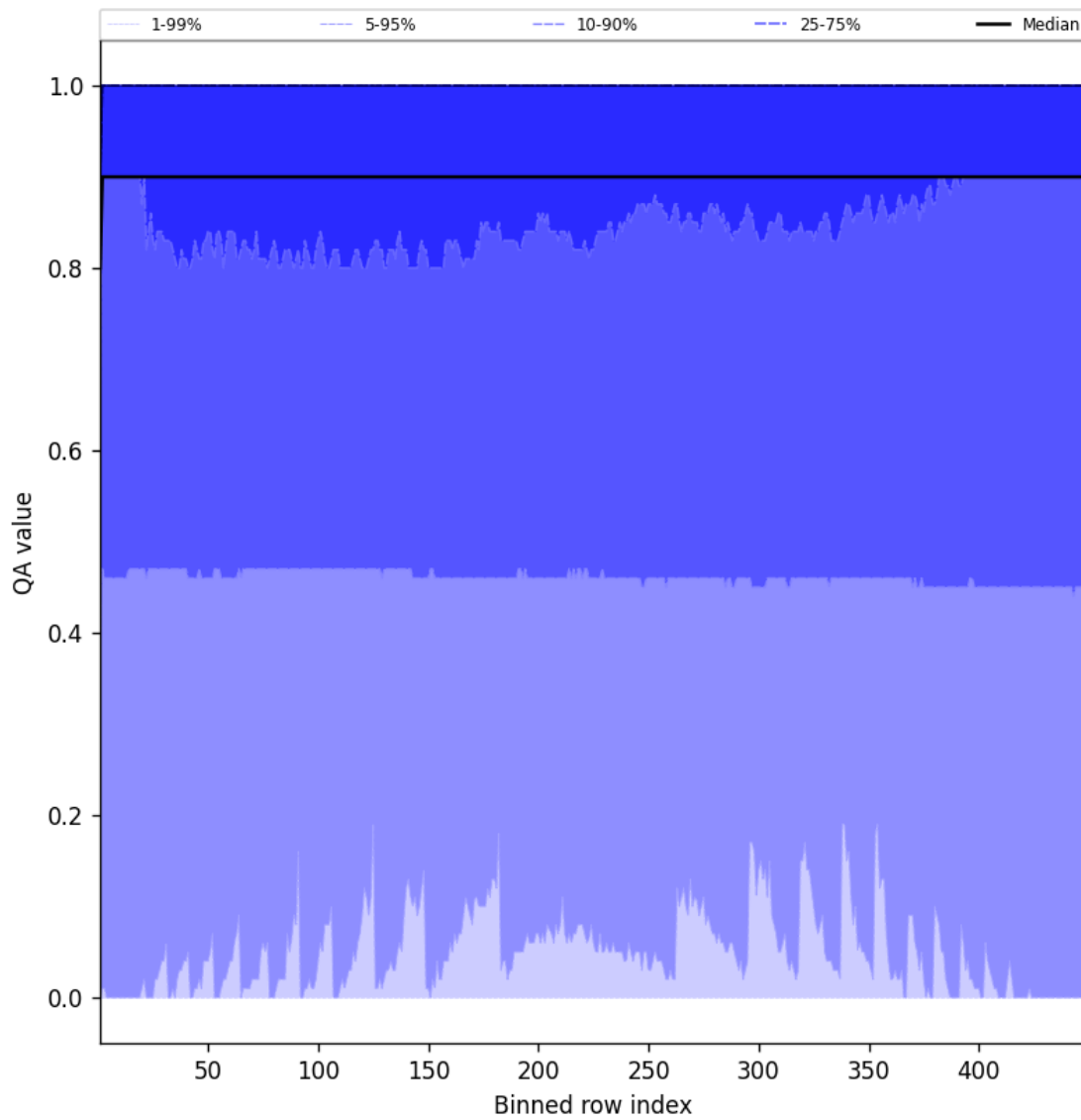
Figure 40: Along track statistics of “QA value” for 2025-02-07 to 2025-02-08
