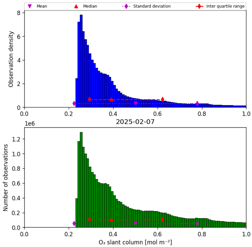
Figure 31: Histogram of “O 3 slant column” for 2025-02-07 to 2025-02-08
