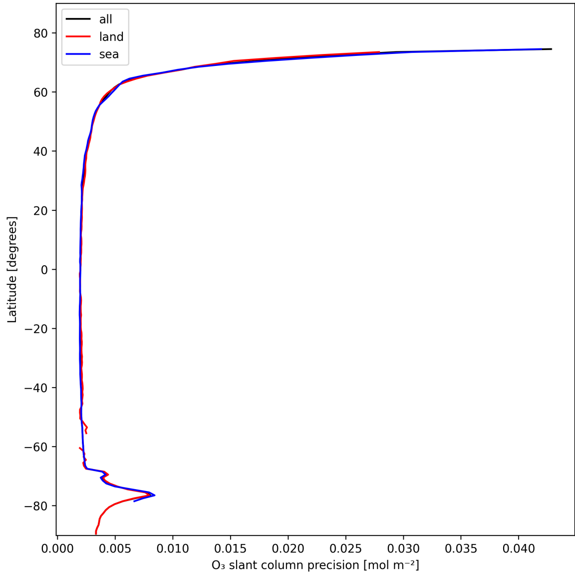
Figure 20: Zonal average of “O 3 slant column precision” for 2025-02-07 to 2025-02-08.
