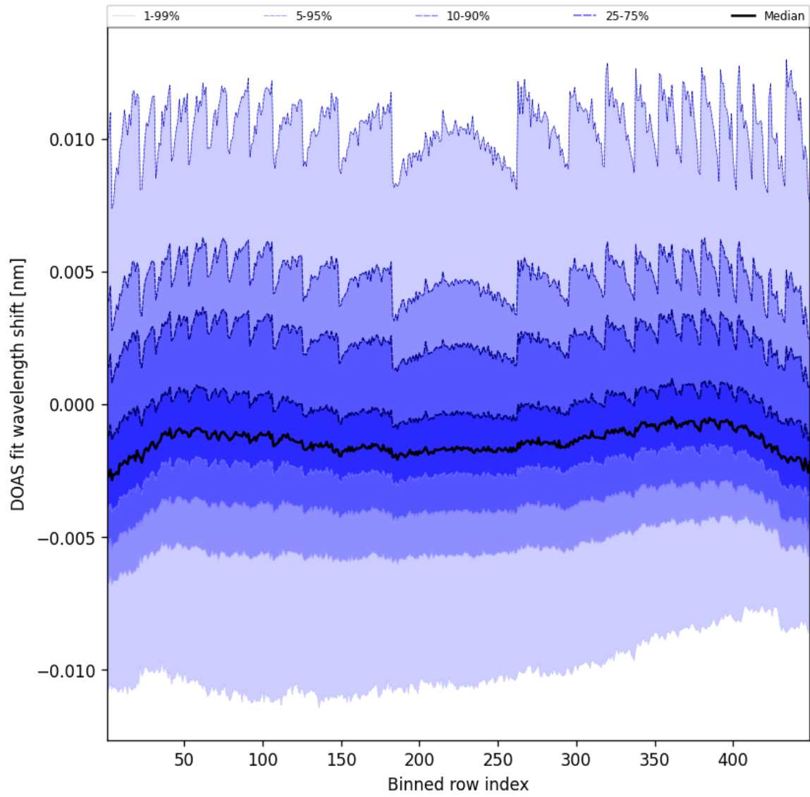
Figure 47: Along track statistics of “DOAS fit wavelength shift” for 2025-02-07 to 2025-02-08
