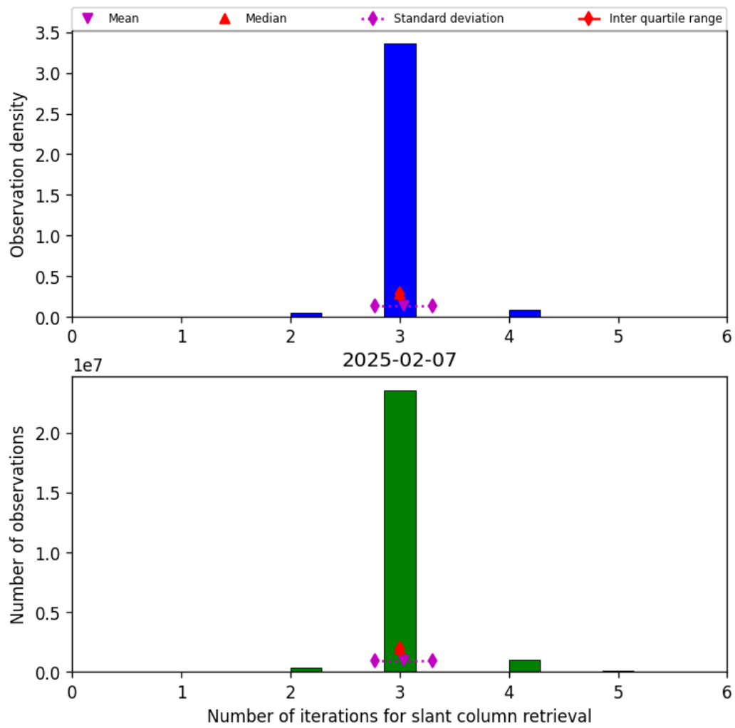
Figure 33: Histogram of “Number of iterations for slant column retrieval” for 2025-02-07 to 2025-02-08
