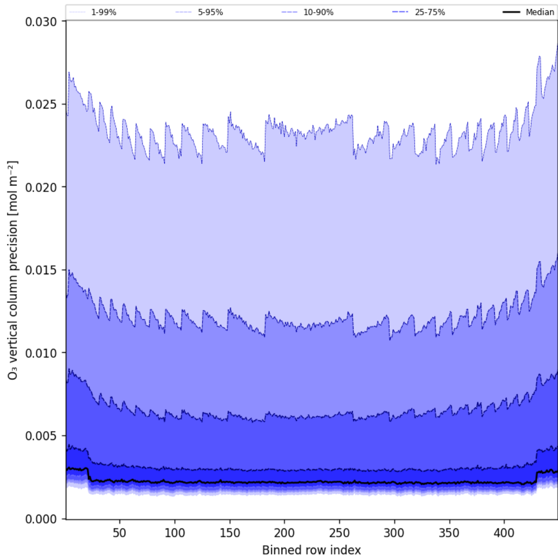
Figure 42: Along track statistics of “O 3 vertical column precision” for 2025-02-07 to 2025-02-08
