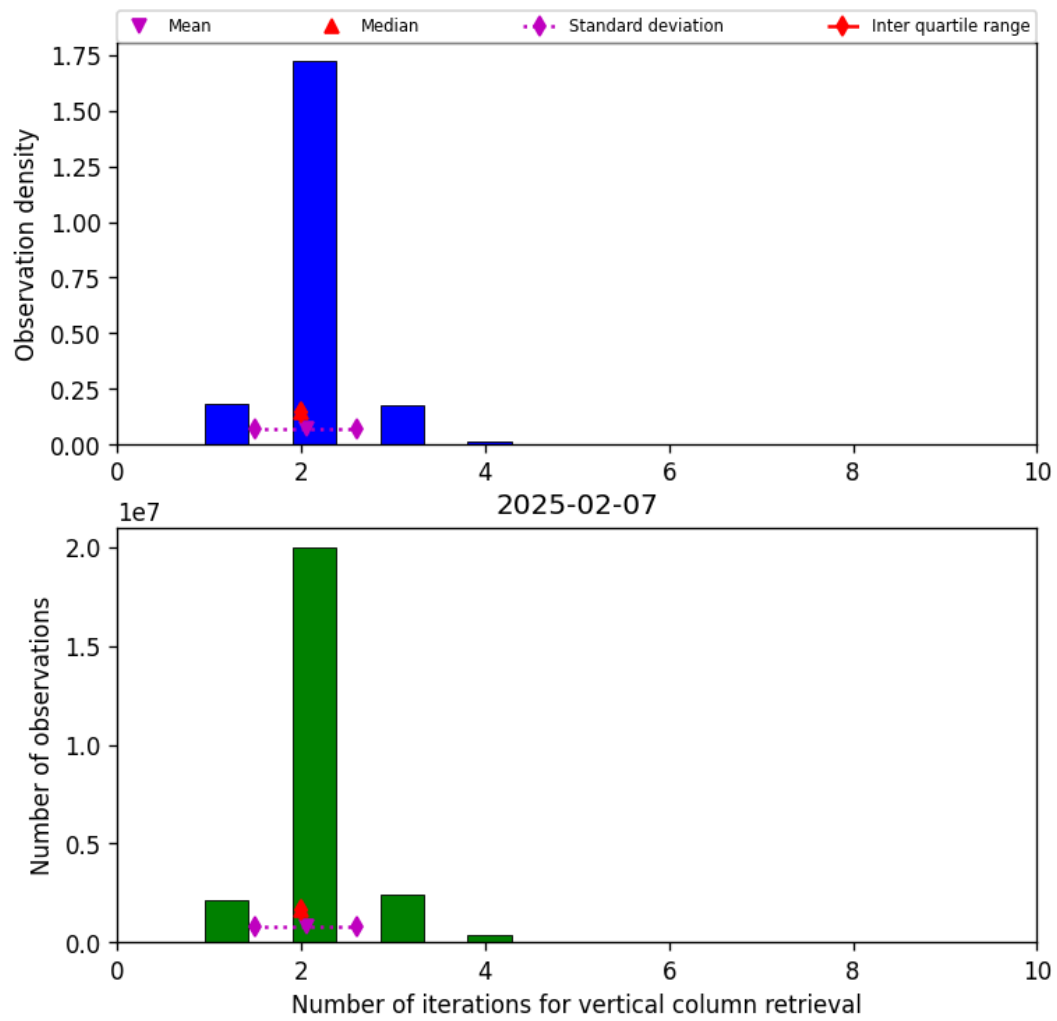
Figure 39: Histogram of “Number of iterations for vertical column retrieval” for 2025-02-07 to 2025-02-08
