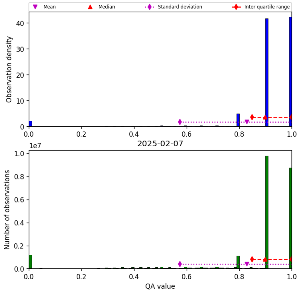
Figure 28: Histogram of “QA value” for 2025-02-07 to 2025-02-08
