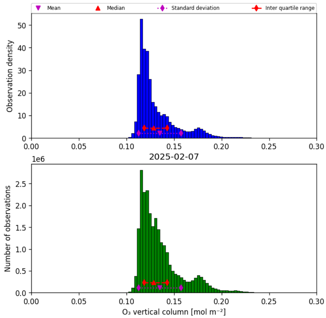
Figure 29: Histogram of “O 3 vertical column” for 2025-02-07 to 2025-02-08
