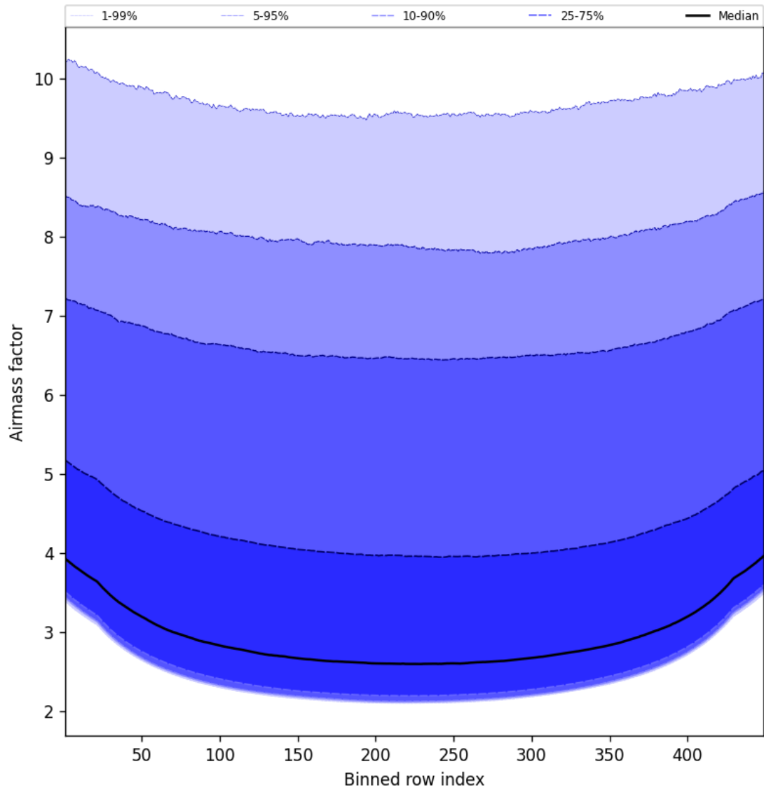
Figure 49: Along track statistics of “Airmass factor” for 2025-02-07 to 2025-02-08
