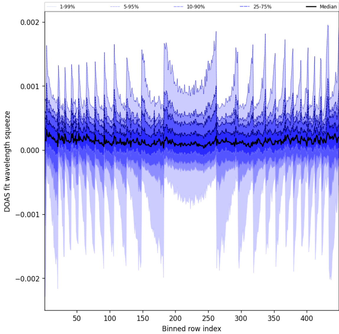
Figure 48: Along track statistics of “DOAS fit wavelength squeeze” for 2025-02-07 to 2025-02-08
