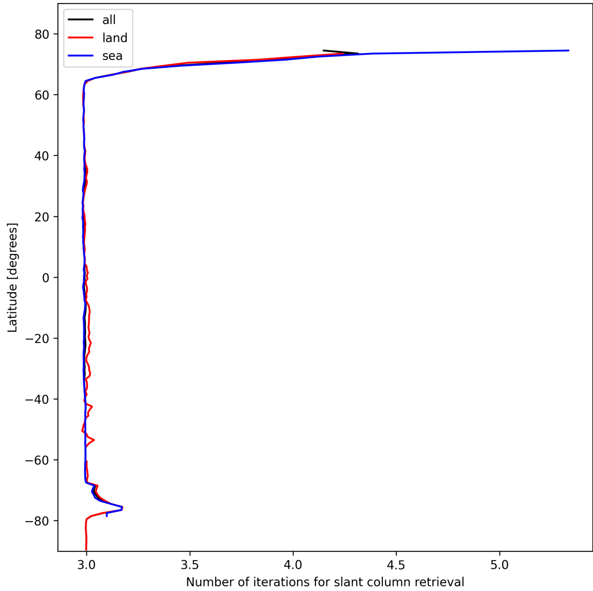
Figure 21: Zonal average of “Number of iterations for slant column retrieval” for 2025-02-07 to 2025-02-08.
