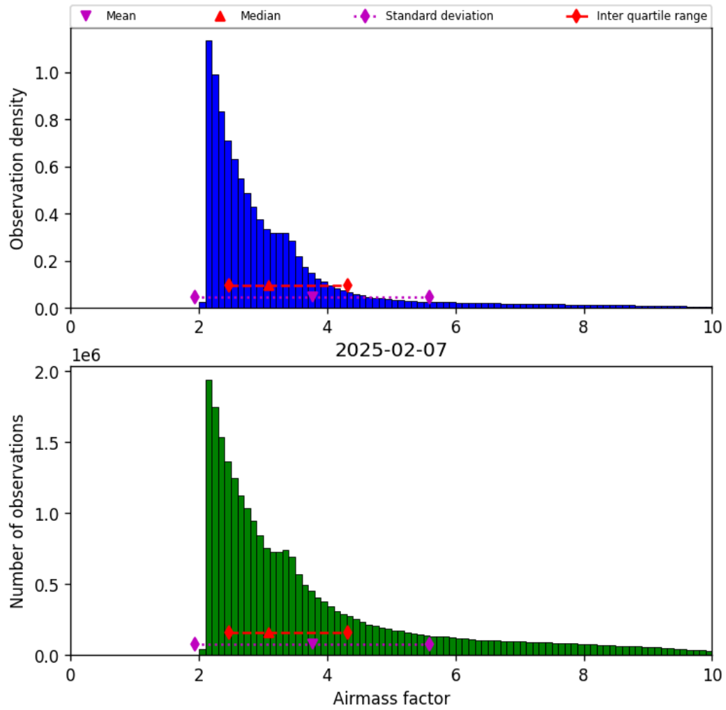
Figure 37: Histogram of “Airmass factor” for 2025-02-07 to 2025-02-08
