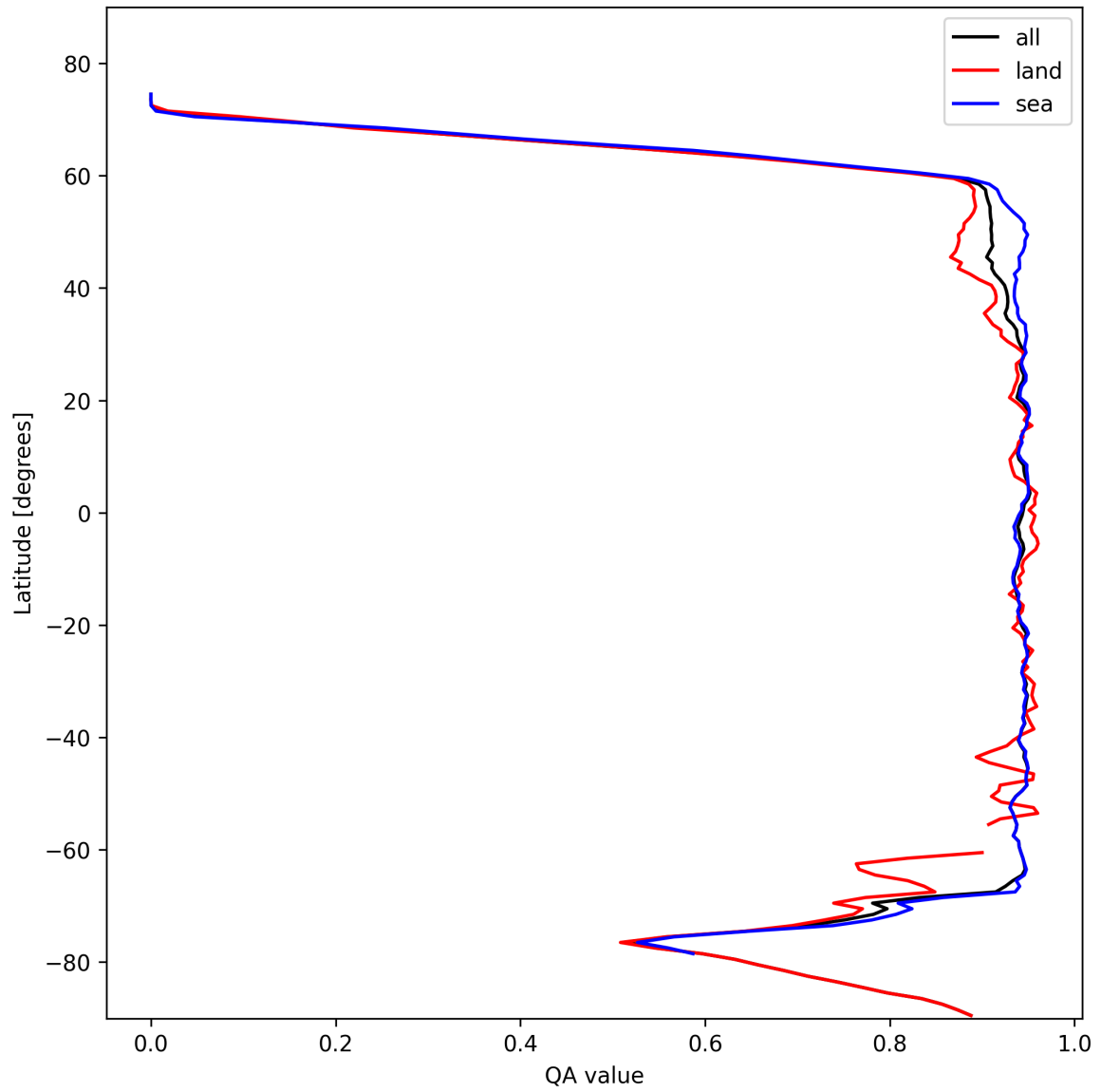
Figure 16: Zonal average of “QA value” for 2025-02-07 to 2025-02-08.
