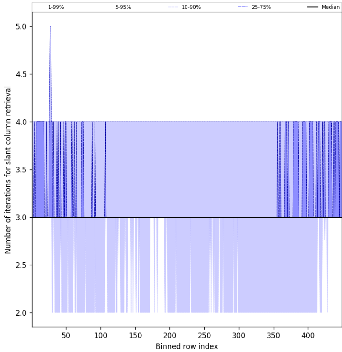
Figure 45: Along track statistics of “Number of iterations for slant column retrieval” for 2025-02-07 to 2025-02-08
