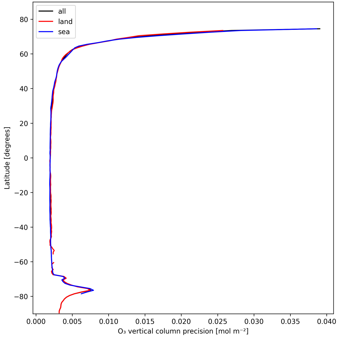
Figure 18: Zonal average of “O 3 vertical column precision” for 2025-02-07 to 2025-02-08.
