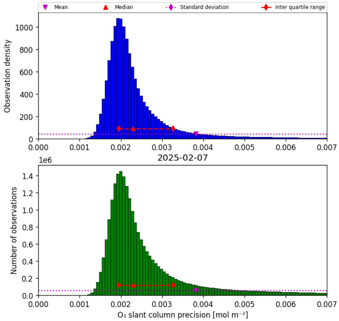
Figure 32: Histogram of “O 3 slant column precision” for 2025-02-07 to 2025-02-08
