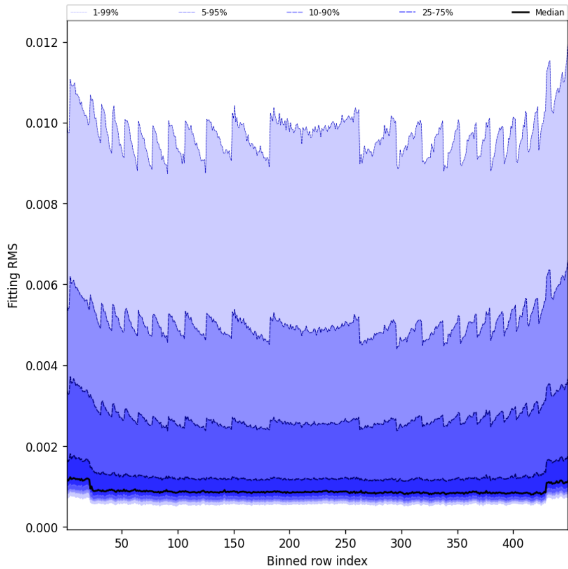
Figure 46: Along track statistics of “Fitting RMS” for 2025-02-07 to 2025-02-08
