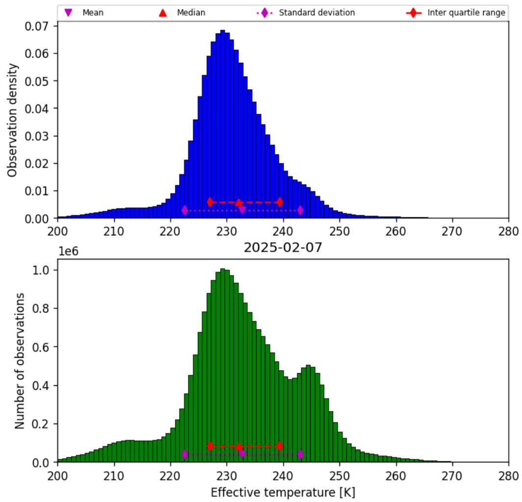
Figure 38: Histogram of “Effective temperature” for 2025-02-07 to 2025-02-08
