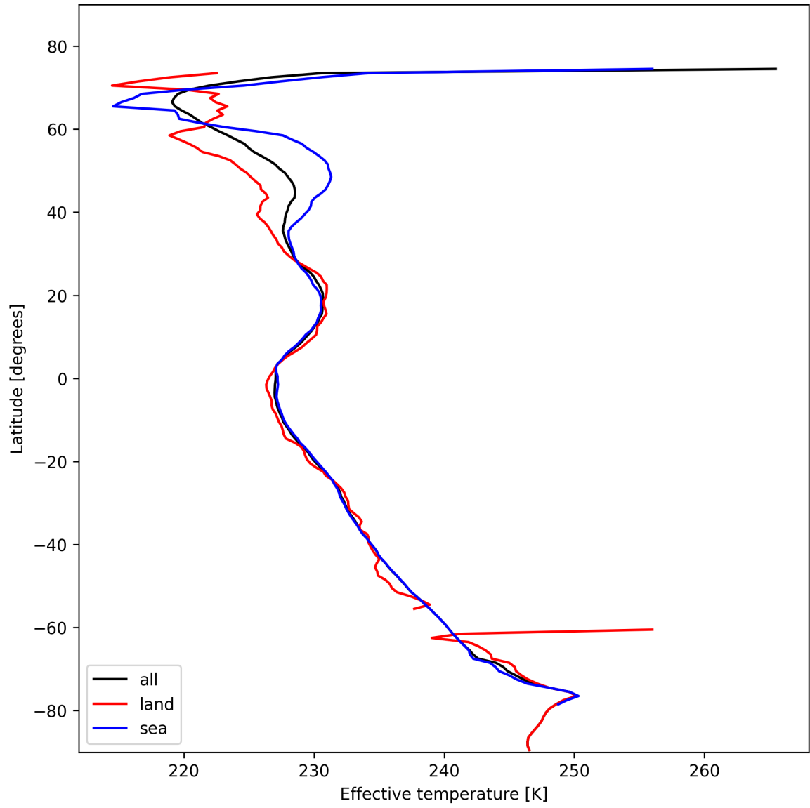
Figure 26: Zonal average of “Effective temperature” for 2025-02-07 to 2025-02-08.
