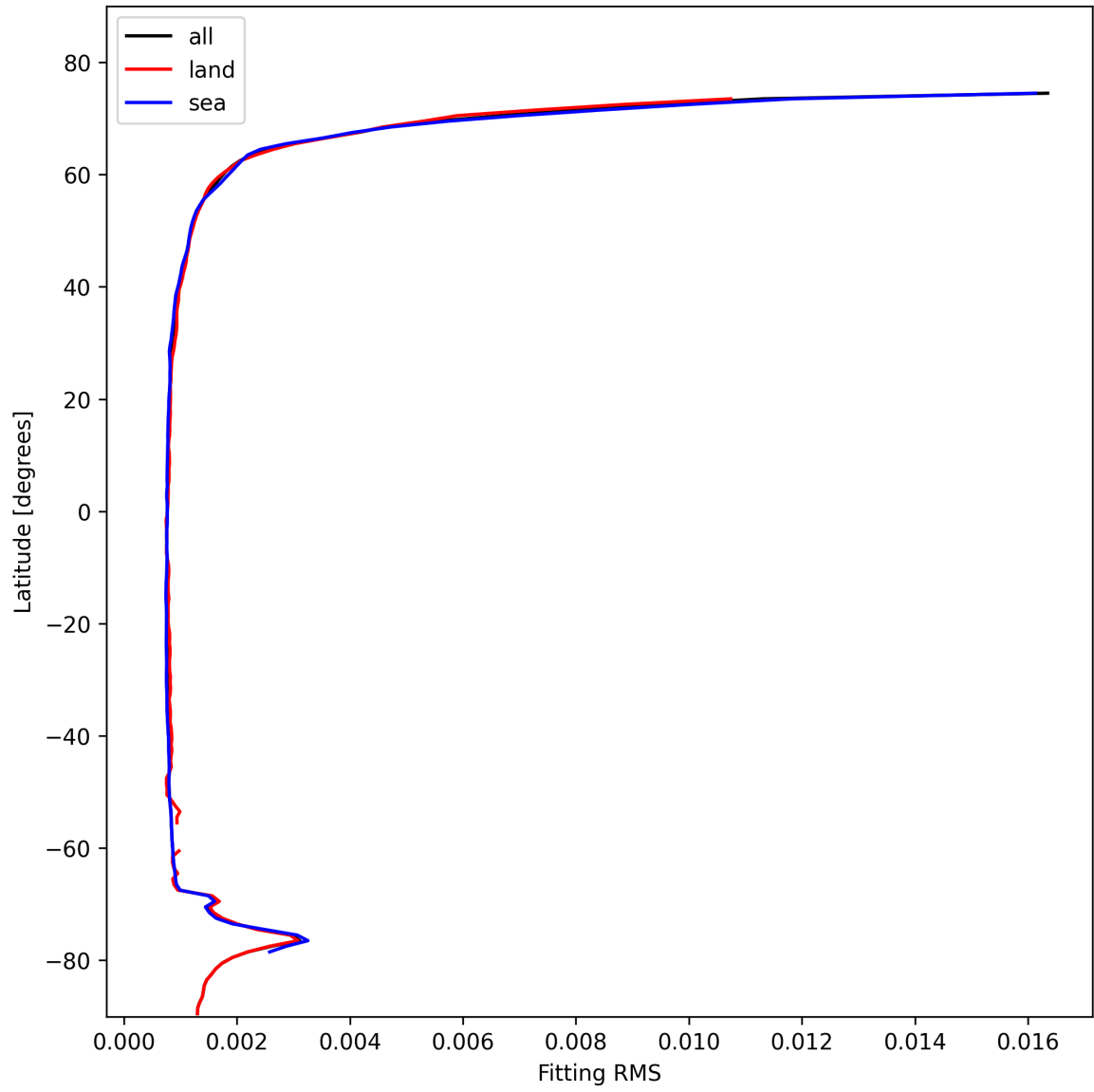
Figure 22: Zonal average of “Fitting RMS” for 2025-02-07 to 2025-02-08.
