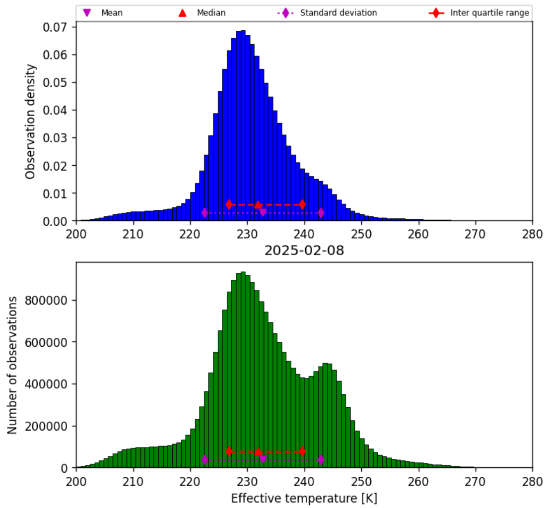
Figure 38: Histogram of “Effective temperature” for 2025-02-08 to 2025-02-09
