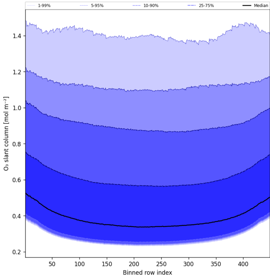
Figure 43: Along track statistics of “O 3 slant column” for 2025-02-08 to 2025-02-09
