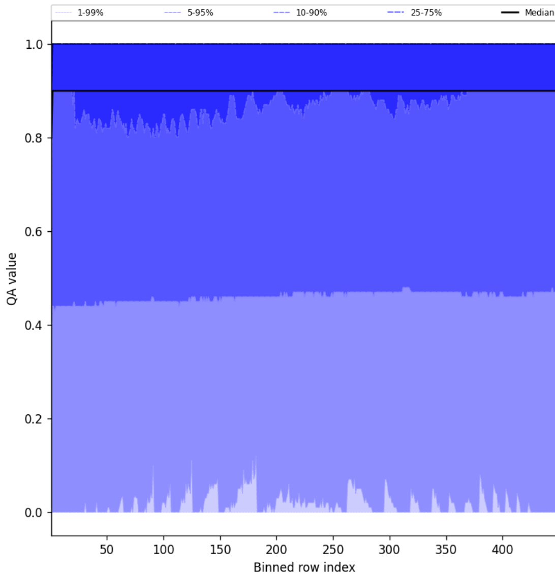
Figure 40: Along track statistics of “QA value” for 2025-02-08 to 2025-02-09
