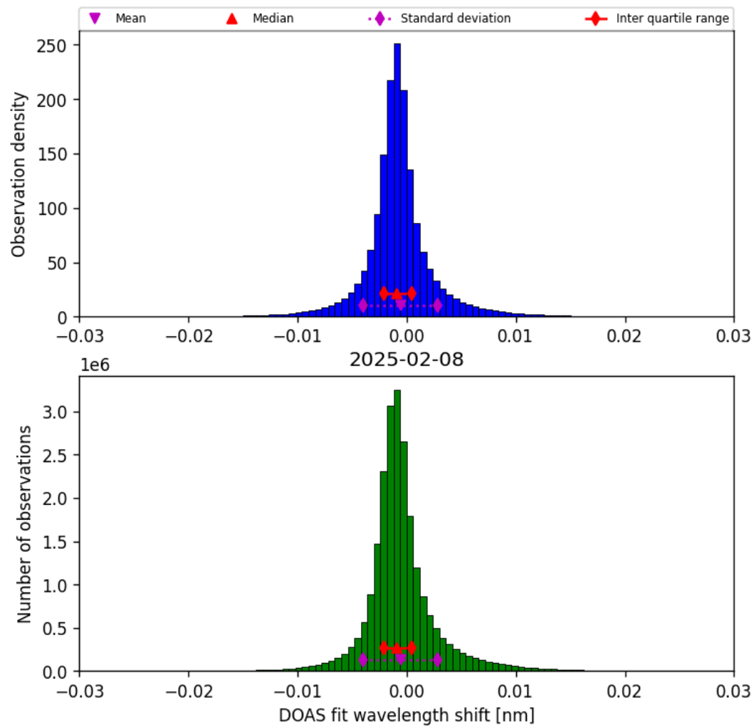
Figure 35: Histogram of “DOAS fit wavelength shift” for 2025-02-08 to 2025-02-09
