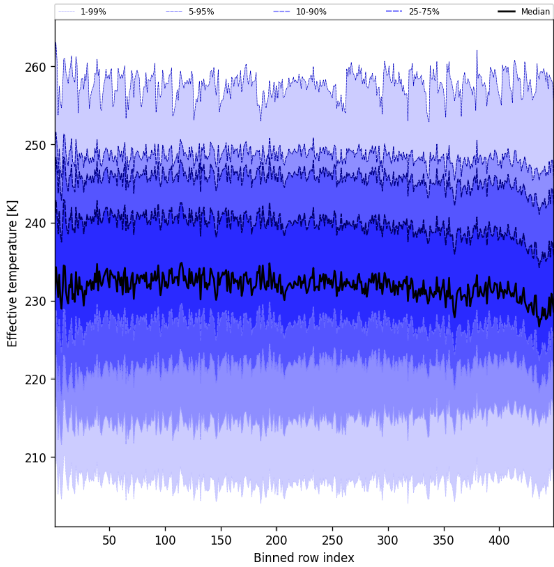
Figure 50: Along track statistics of “Effective temperature” for 2025-02-08 to 2025-02-09
