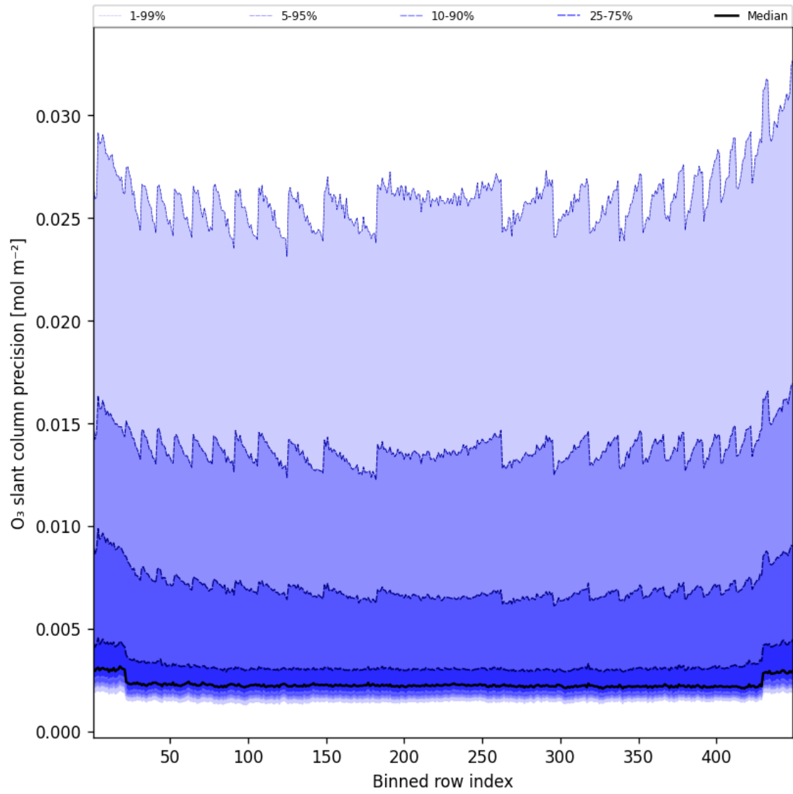
Figure 44: Along track statistics of “O 3 slant column precision” for 2025-02-08 to 2025-02-09
