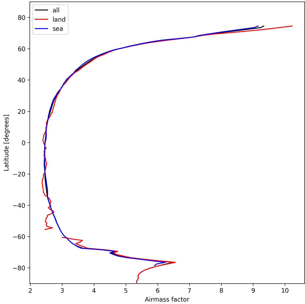
Figure 25: Zonal average of “Airmass factor” for 2025-02-08 to 2025-02-09.
