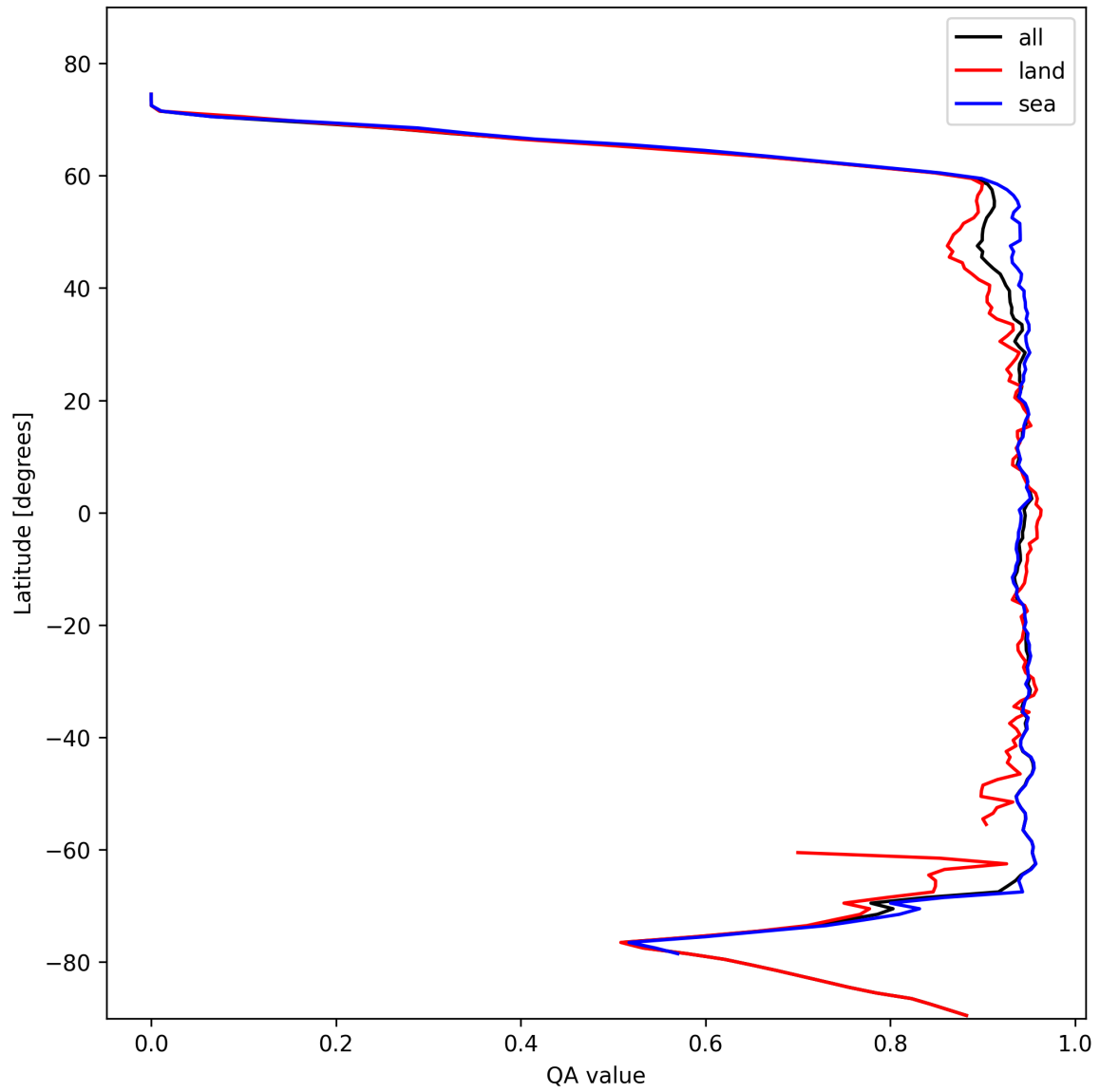
Figure 16: Zonal average of “QA value” for 2025-02-08 to 2025-02-09.
