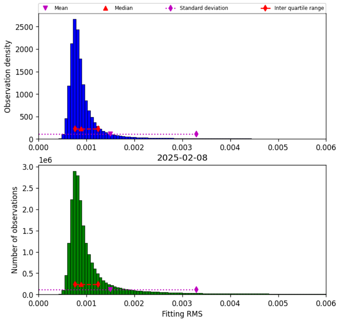
Figure 34: Histogram of “Fitting RMS” for 2025-02-08 to 2025-02-09
