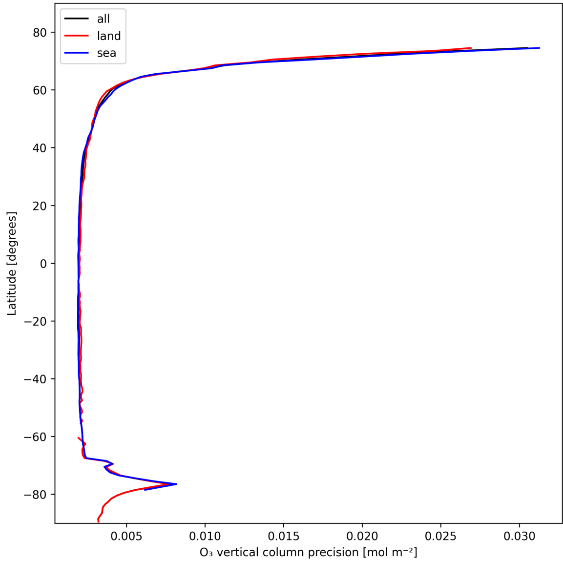
Figure 18: Zonal average of “O 3 vertical column precision” for 2025-02-08 to 2025-02-09.
