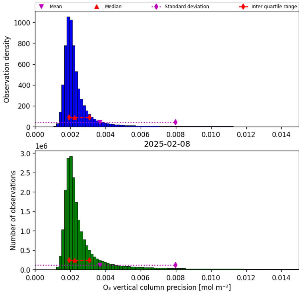
Figure 30: Histogram of “O 3 vertical column precision” for 2025-02-08 to 2025-02-09
