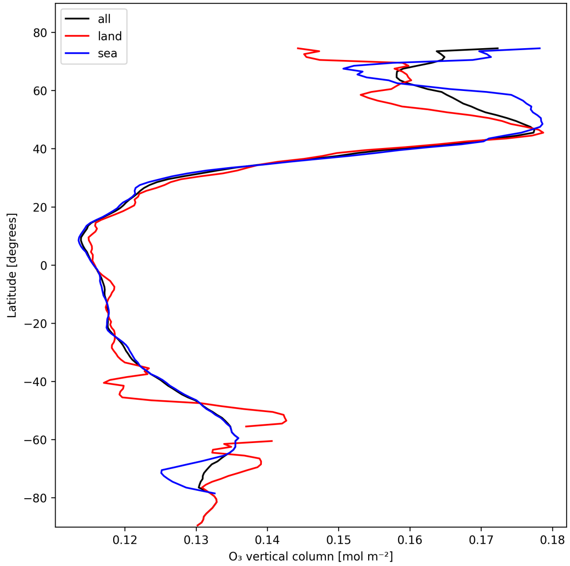
Figure 17: Zonal average of “O 3 vertical column” for 2025-02-08 to 2025-02-09.
