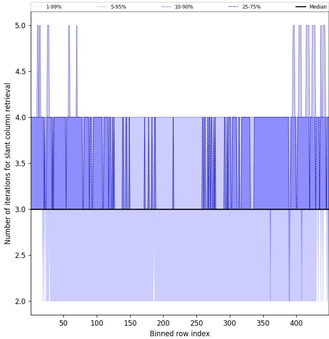
Figure 45: Along track statistics of “Number of iterations for slant column retrieval” for 2025-02-08 to 2025-02-09
