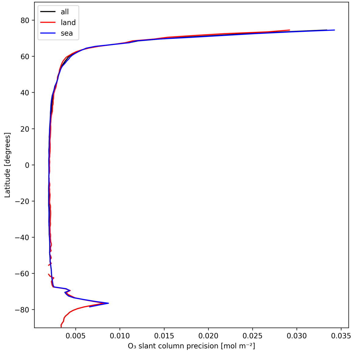
Figure 20: Zonal average of "O 3 slant column precision" for 2025-02-08 to 2025-02-09.
