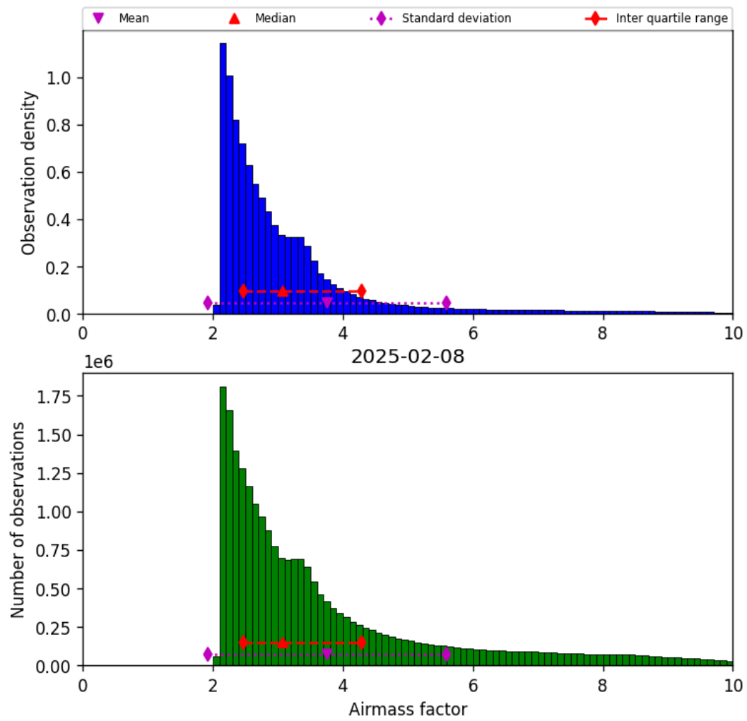
Figure 37: Histogram of “Airmass factor” for 2025-02-08 to 2025-02-09
