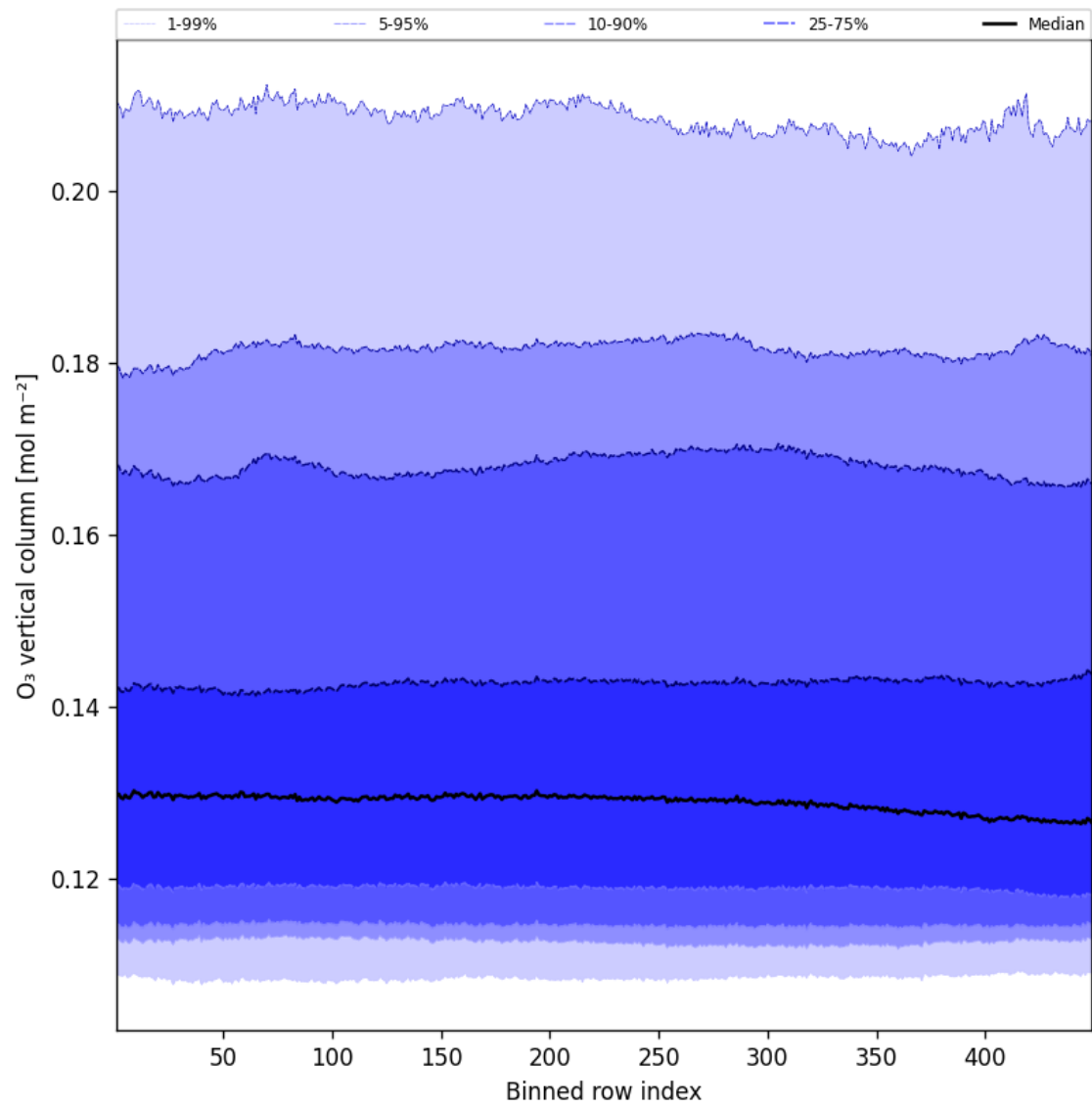
Figure 41: Along track statistics of “O 3 vertical column” for 2025-02-08 to 2025-02-09
