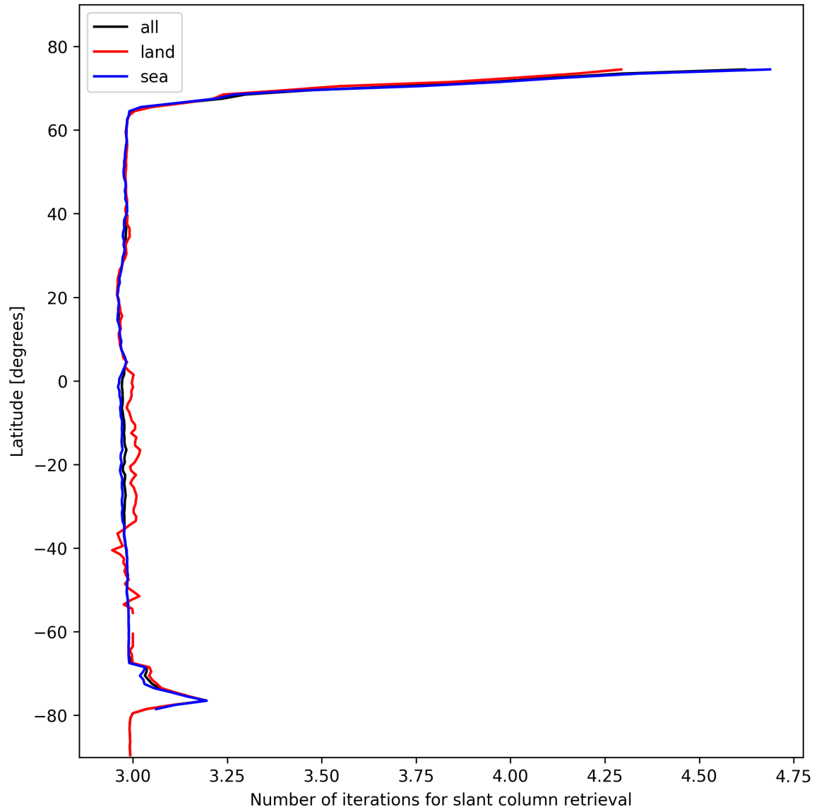
Figure 21: Zonal average of “Number of iterations for slant column retrieval” for 2025-02-08 to 2025-02-09.
