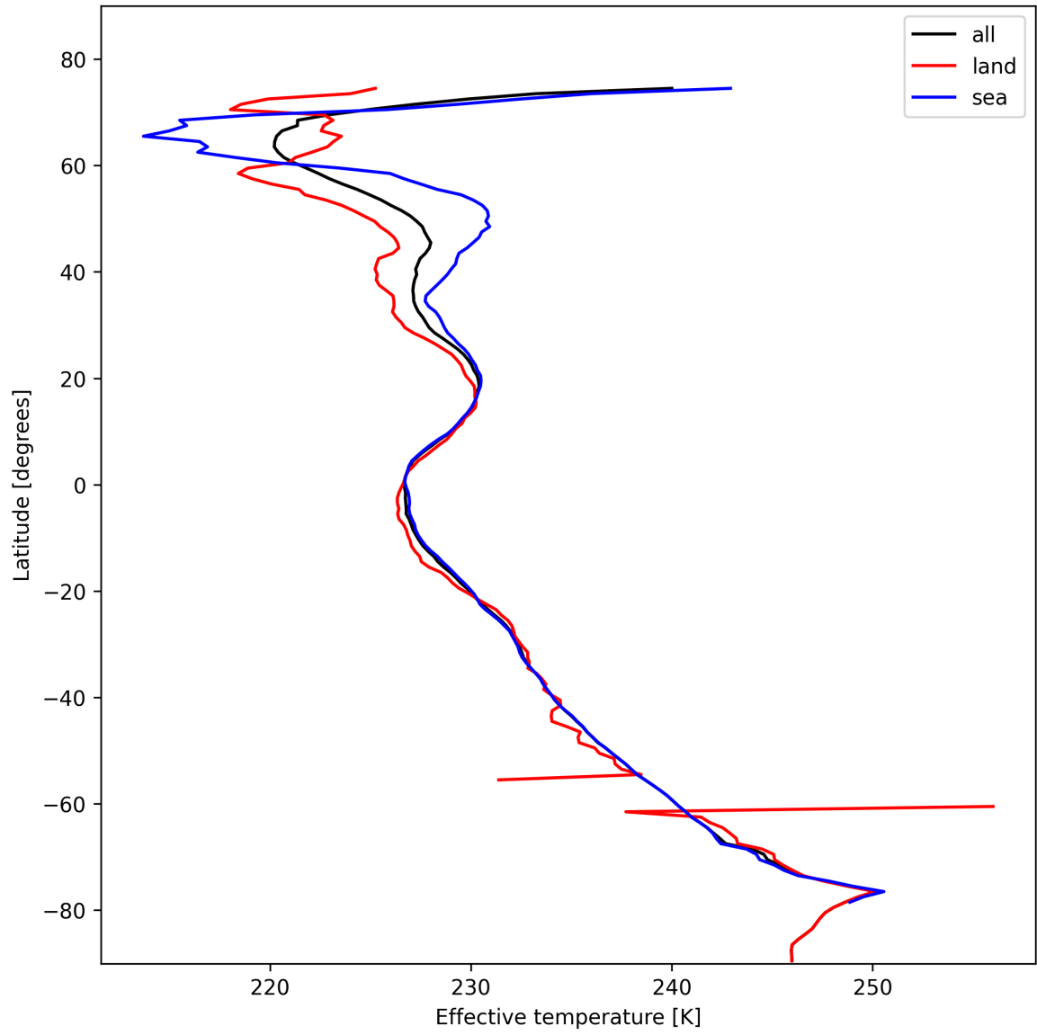
Figure 26: Zonal average of “Effective temperature” for 2025-02-08 to 2025-02-09.
