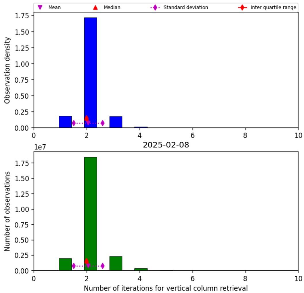
Figure 39: Histogram of “Number of iterations for vertical column retrieval” for 2025-02-08 to 2025-02-09
