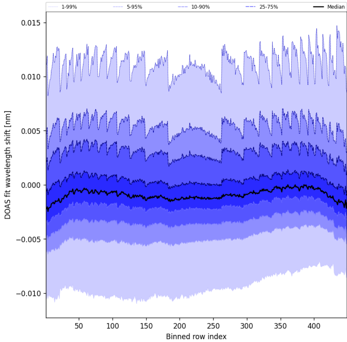
Figure 47: Along track statistics of “DOAS fit wavelength shift” for 2025-02-08 to 2025-02-09
