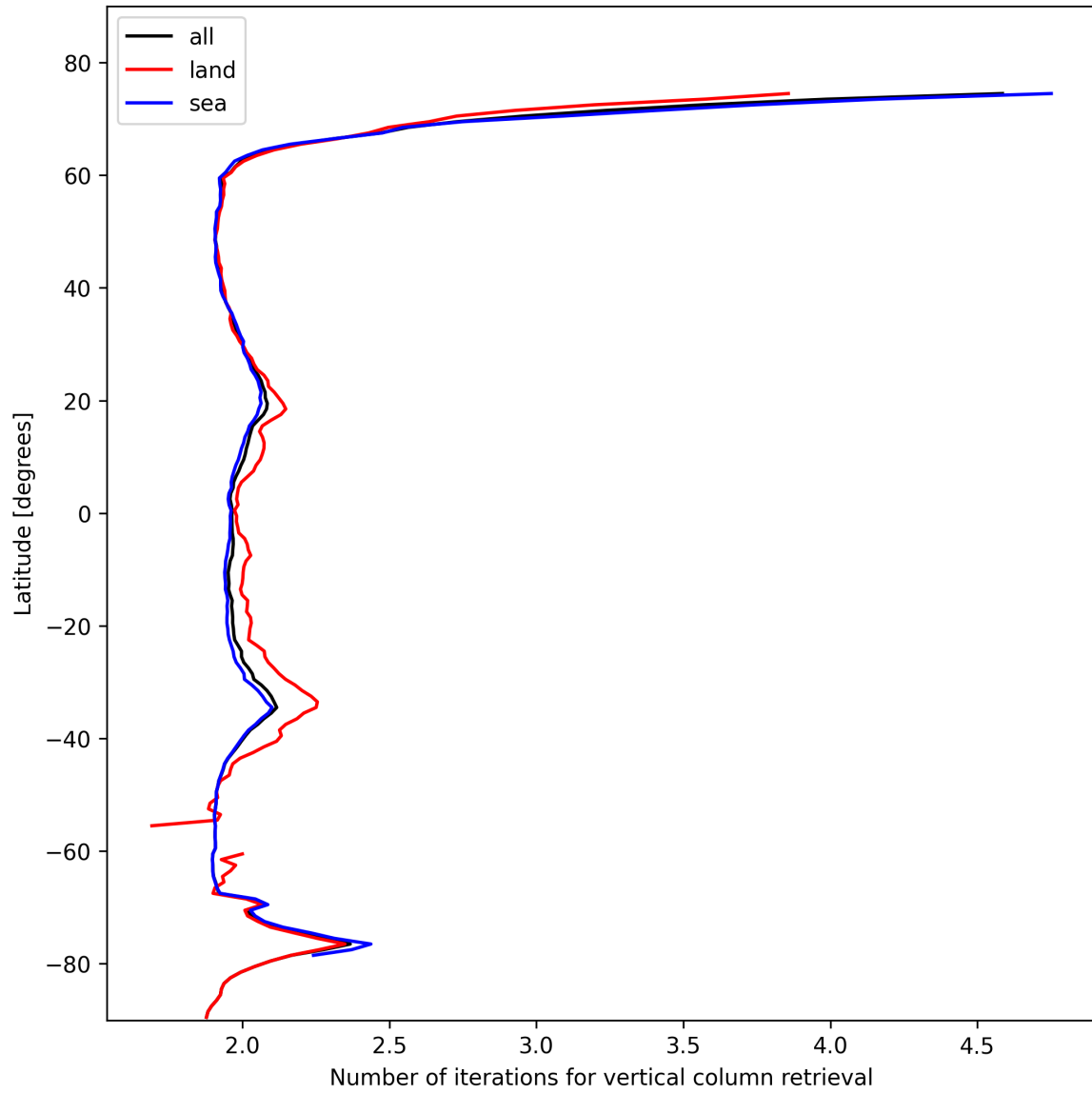
Figure 27: Zonal average of “Number of iterations for vertical column retrieval” for 2025-02-08 to 2025-02-09.
