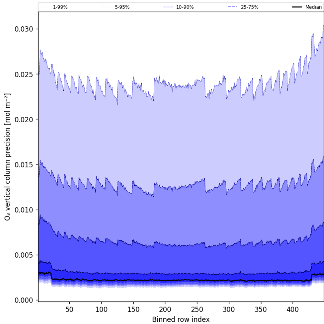
Figure 42: Along track statistics of “O 3 vertical column precision” for 2025-02-08 to 2025-02-09
