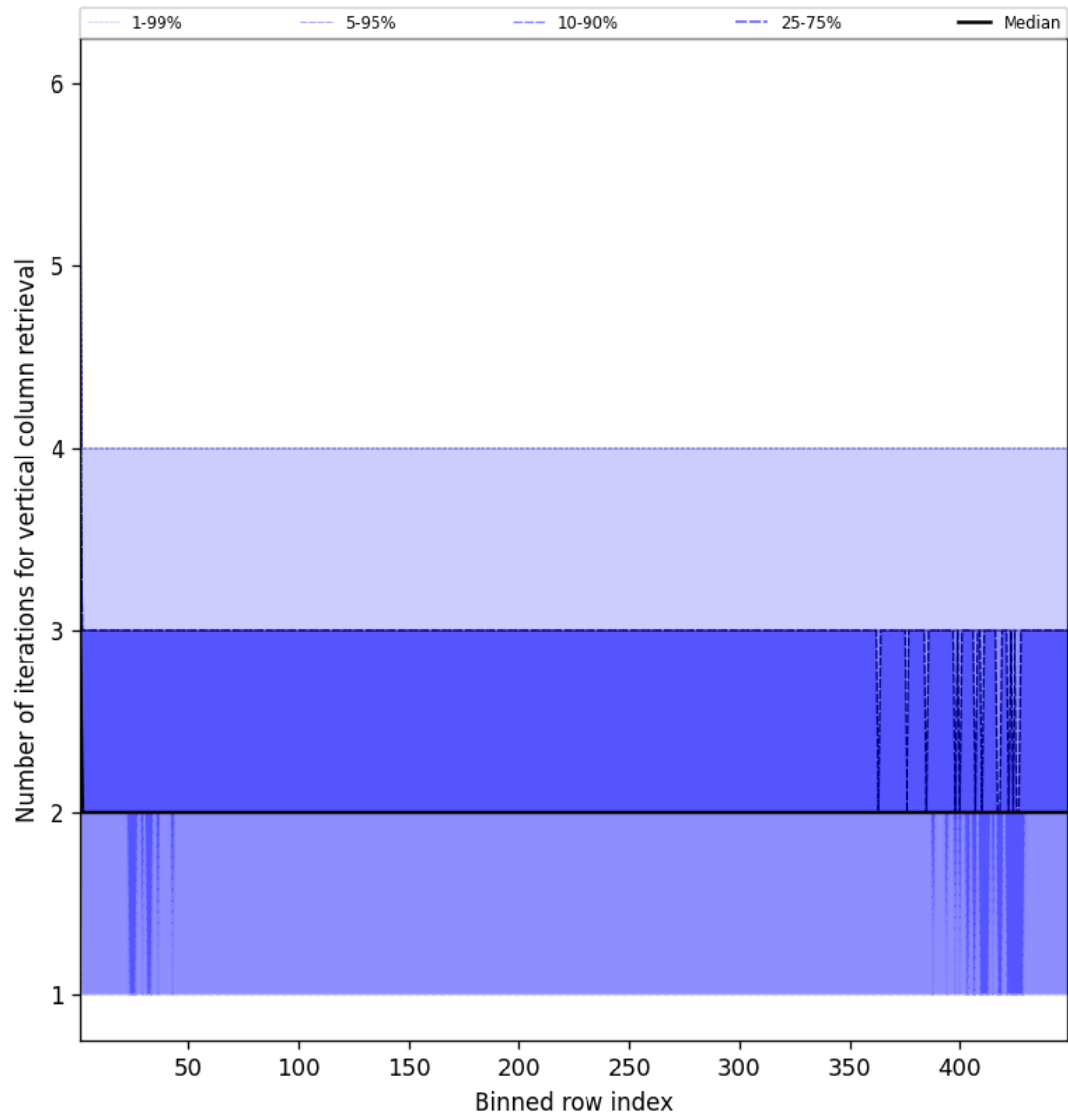
Figure 51: Along track statistics of “Number of iterations for vertical column retrieval” for 2025-02-08 to 2025-02-09
