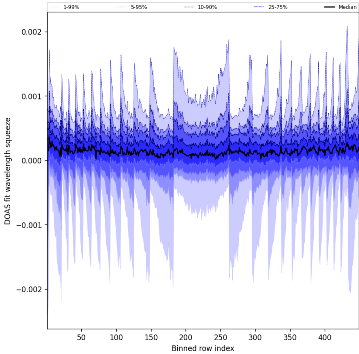
Figure 48: Along track statistics of “DOAS fit wavelength squeeze” for 2025-02-08 to 2025-02-09
