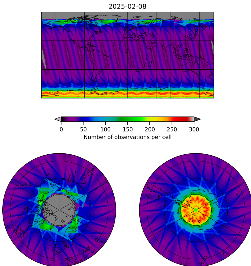
Figure 15: Map of the number of observations for 2025-02-08 to 2025-02-09
