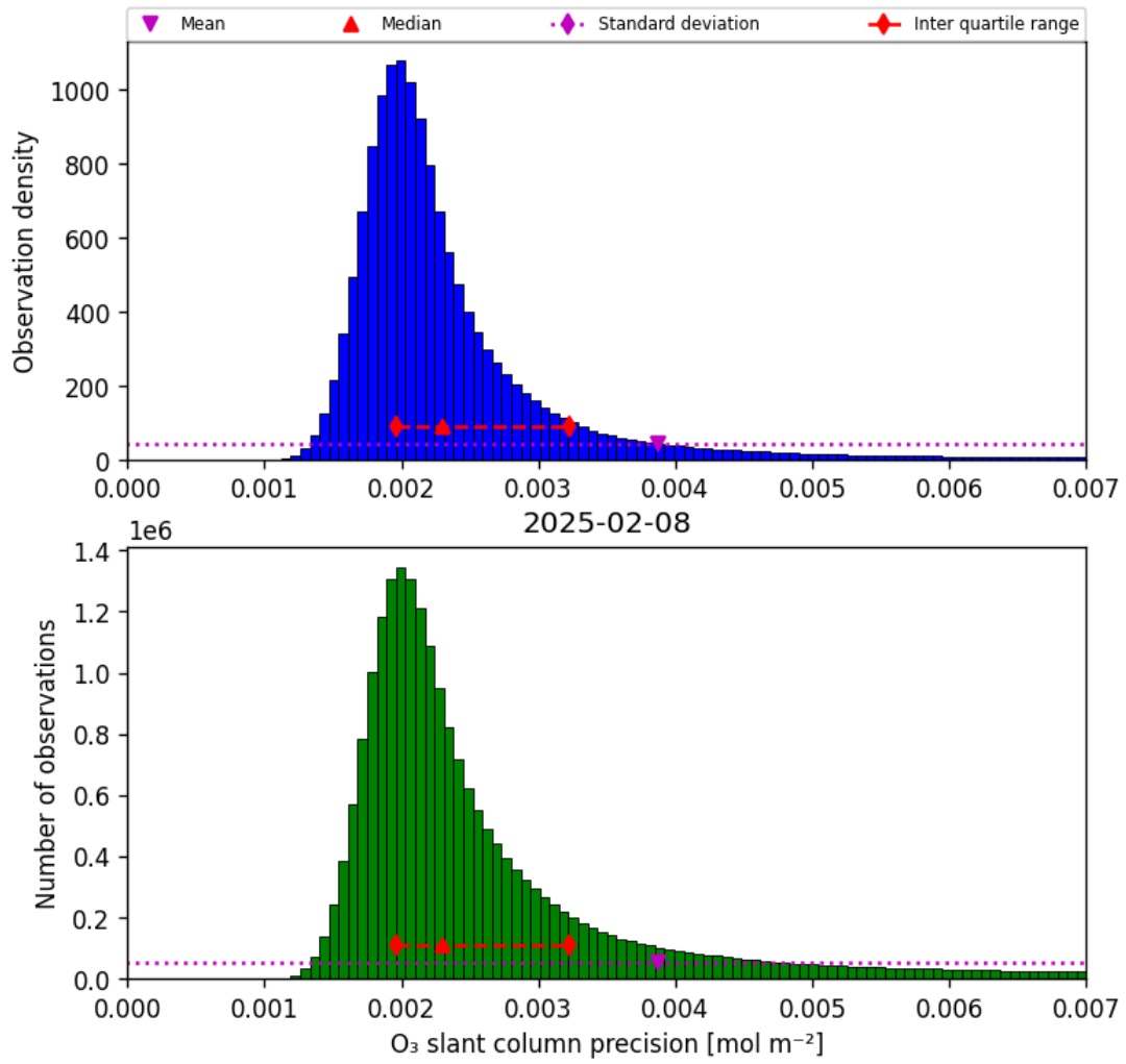
Figure 32: Histogram of “O 3 slant column precision” for 2025-02-08 to 2025-02-09
