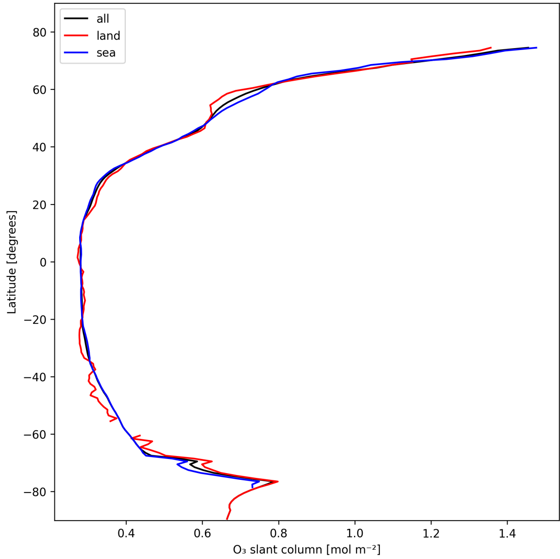
Figure 19: Zonal average of “O 3 slant column” for 2025-02-08 to 2025-02-09.
