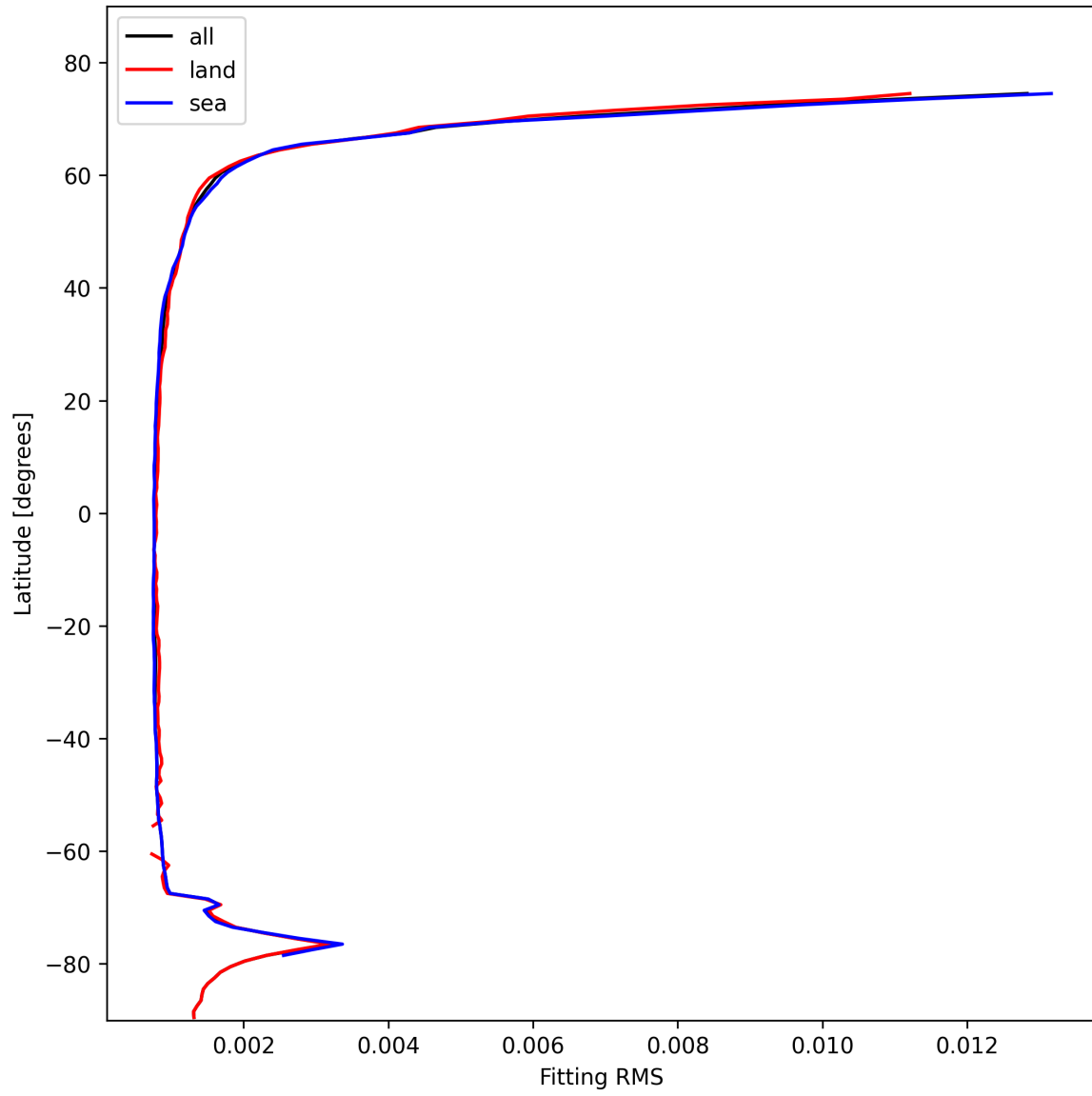
Figure 22: Zonal average of “Fitting RMS” for 2025-02-08 to 2025-02-09.
