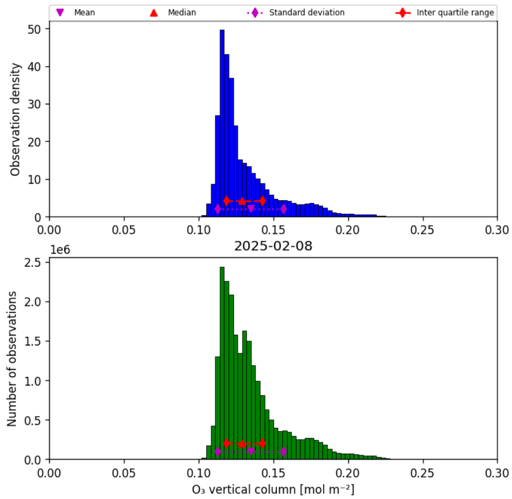
Figure 29: Histogram of “O 3 vertical column” for 2025-02-08 to 2025-02-09
