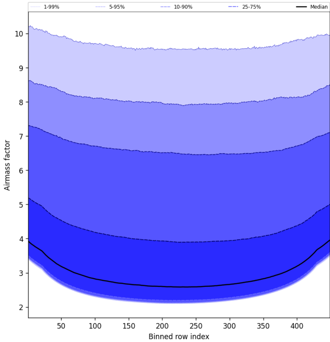
Figure 49: Along track statistics of “Airmass factor” for 2025-02-08 to 2025-02-09
