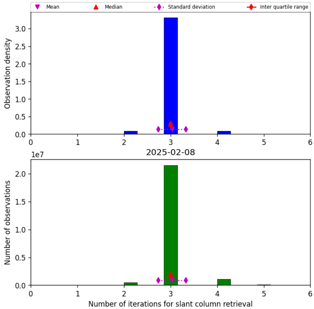
Figure 33: Histogram of "Number of iterations for slant column retrieval" for 2025-02-08 to 2025-02-09
