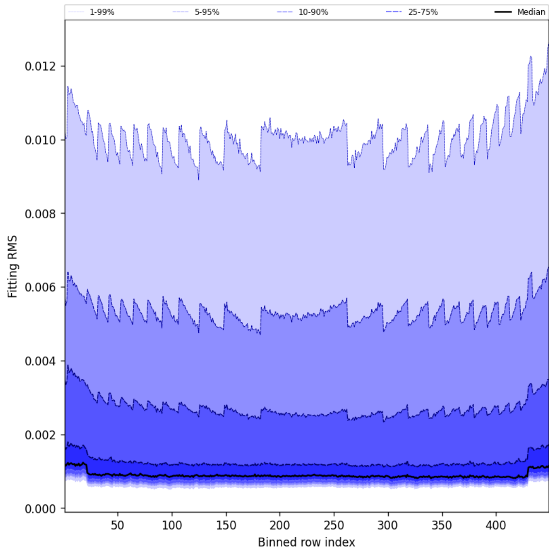
Figure 46: Along track statistics of “Fitting RMS” for 2025-02-08 to 2025-02-09
