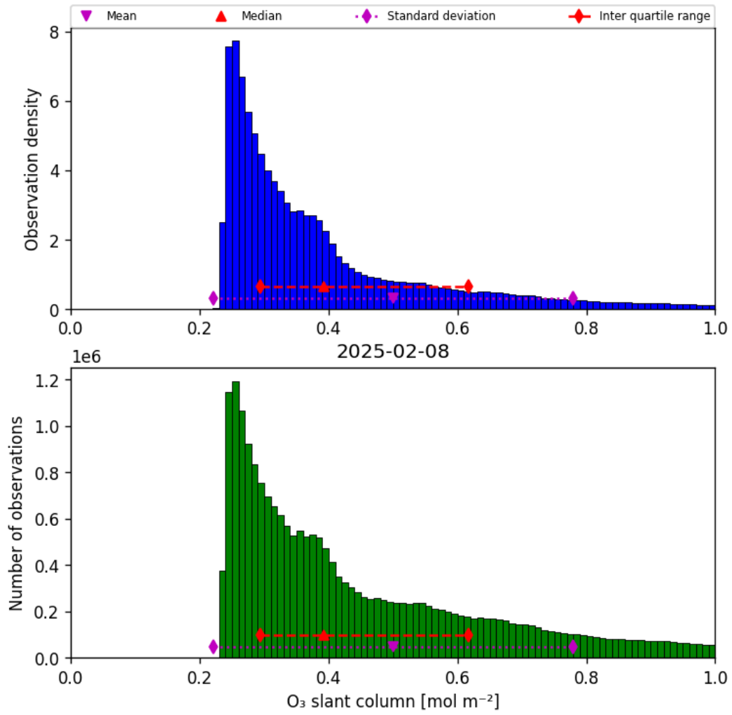
Figure 31: Histogram of “O 3 slant column” for 2025-02-08 to 2025-02-09
