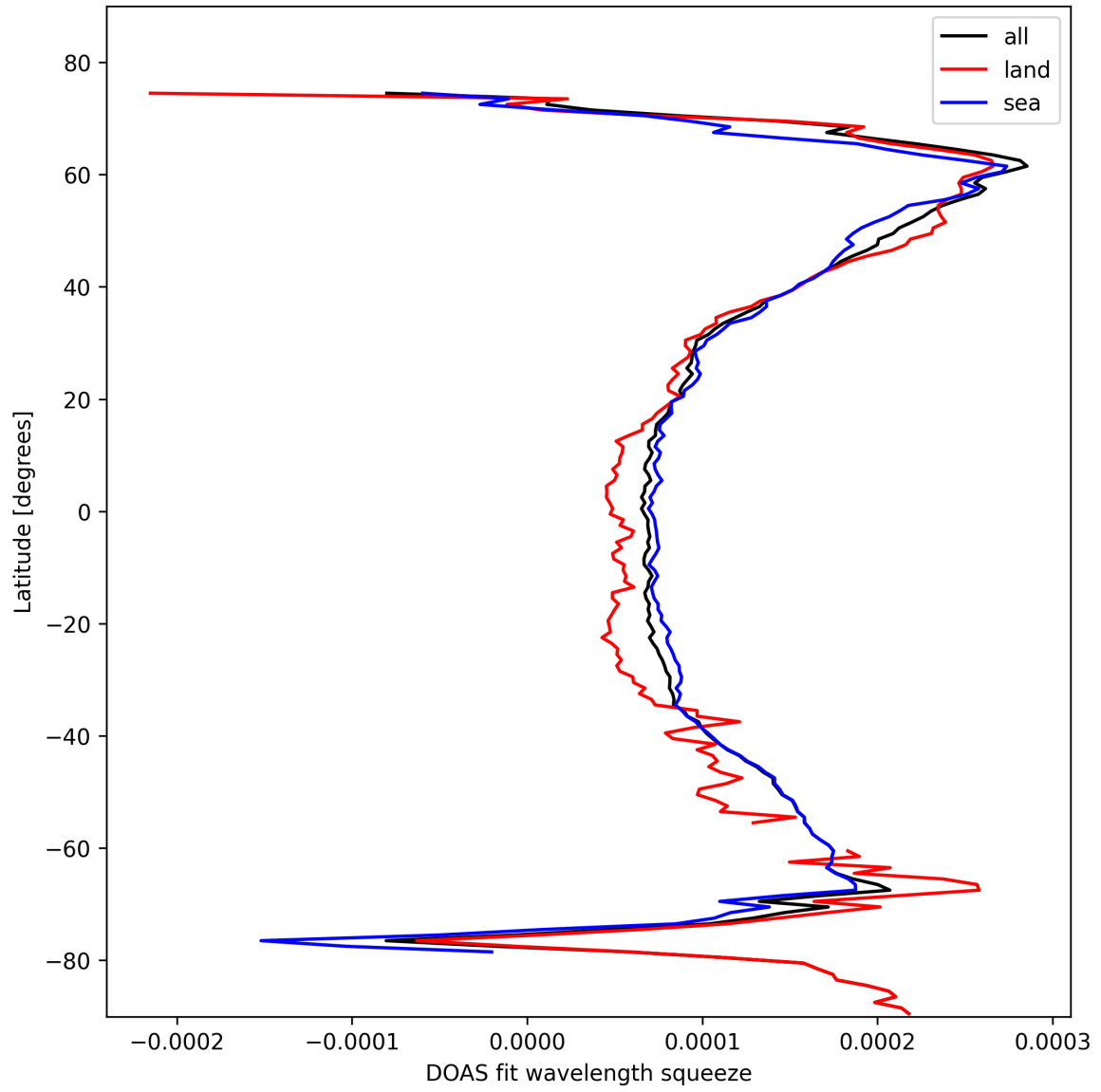
Figure 24: Zonal average of “DOAS fit wavelength squeeze” for 2025-02-08 to 2025-02-09.
