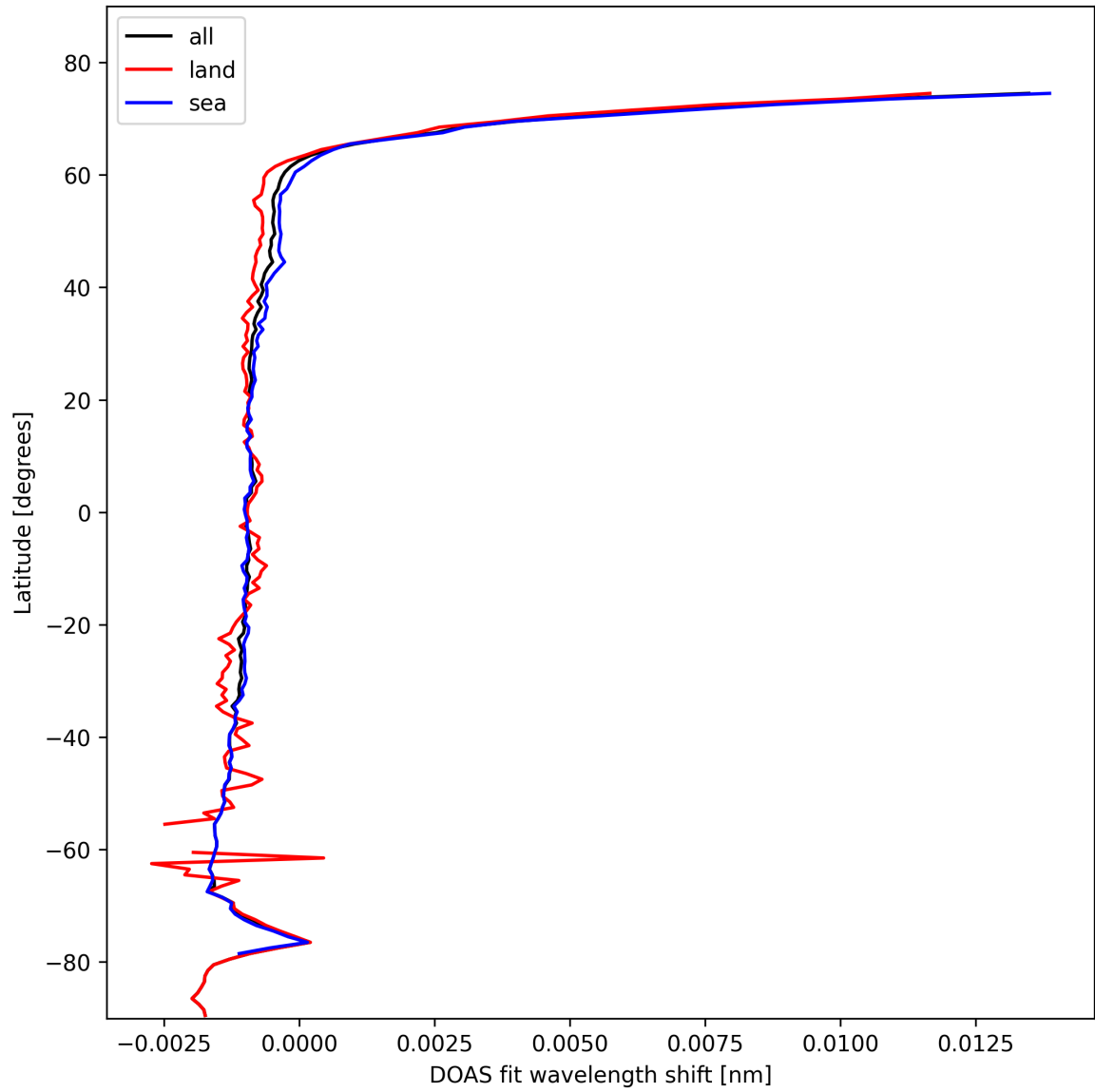
Figure 23: Zonal average of "DOAS fit wavelength shift" for 2025-02-08 to 2025-02-09.
