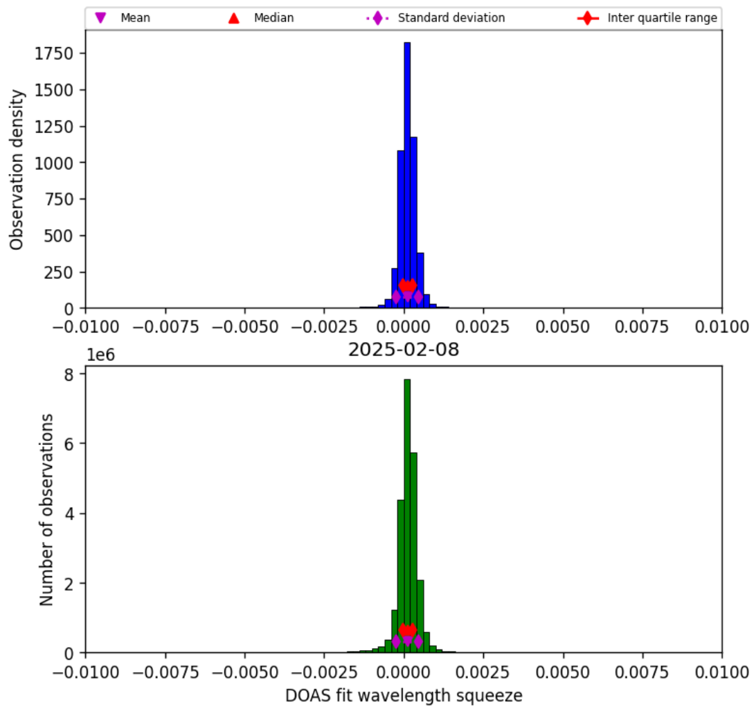
Figure 36: Histogram of “DOAS fit wavelength squeeze” for 2025-02-08 to 2025-02-09
