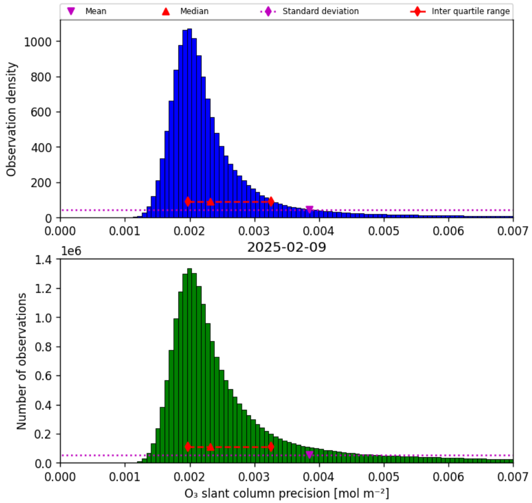
Figure 32: Histogram of “O 3 slant column precision” for 2025-02-09 to 2025-02-10
