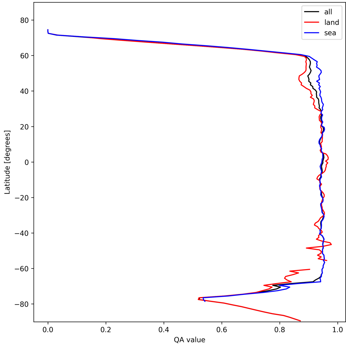
Figure 16: Zonal average of “QA value” for 2025-02-09 to 2025-02-10.
