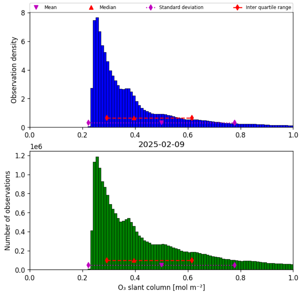
Figure 31: Histogram of “O 3 slant column” for 2025-02-09 to 2025-02-10
