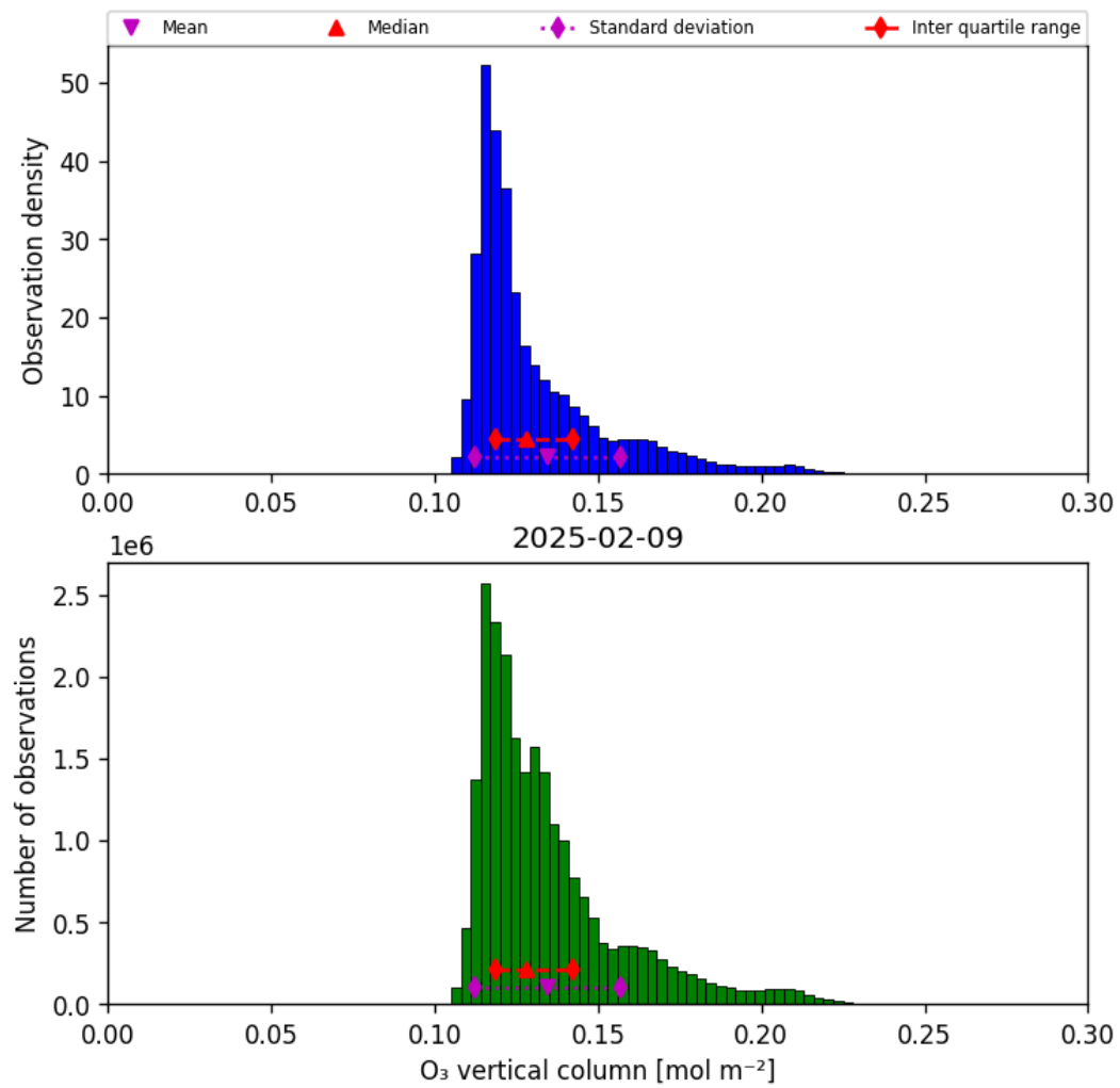
Figure 29: Histogram of “O 3 vertical column” for 2025-02-09 to 2025-02-10
