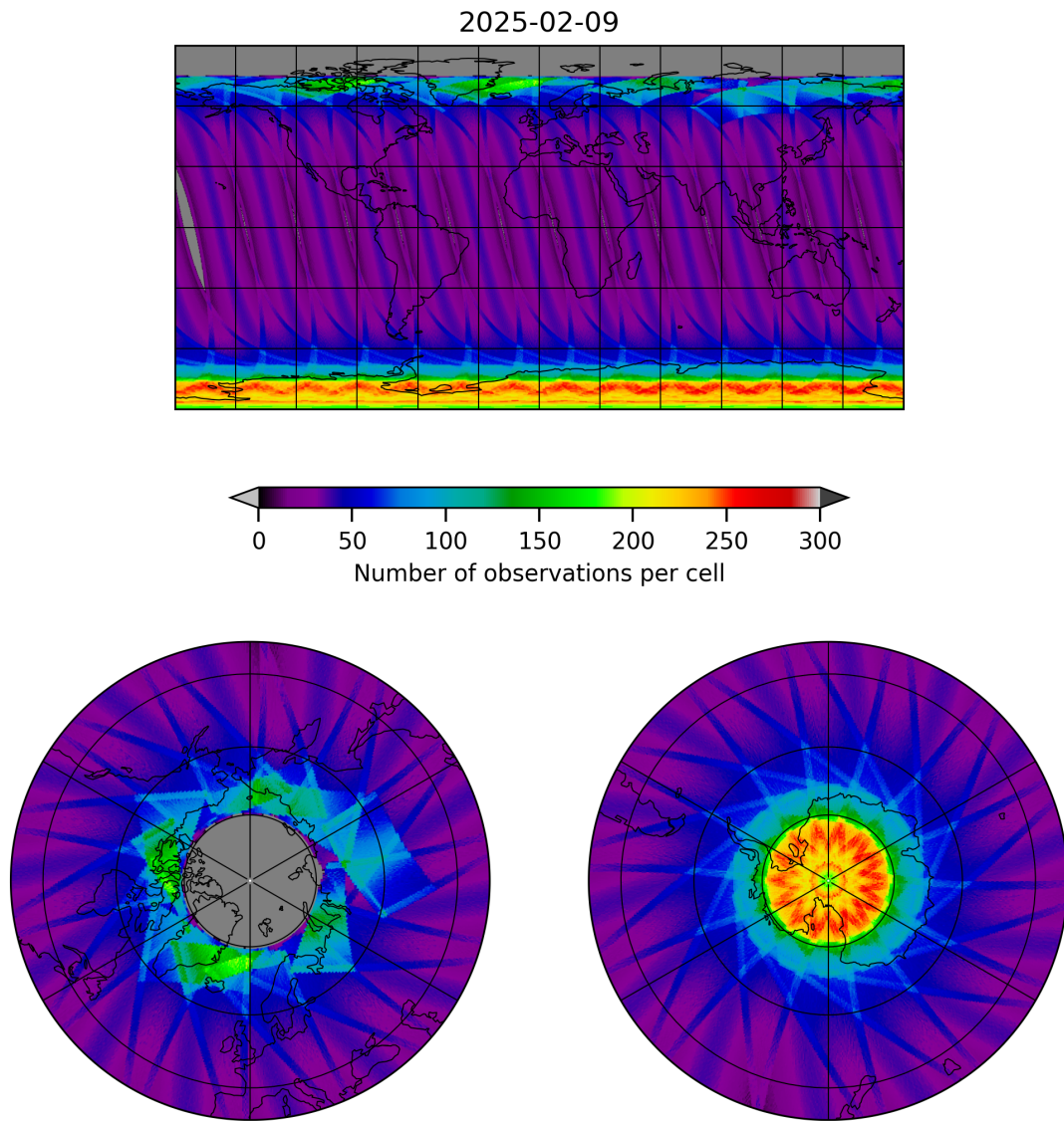
Figure 15: Map of the number of observations for 2025-02-09 to 2025-02-10
