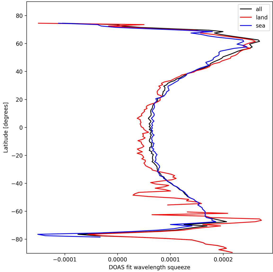
Figure 24: Zonal average of “DOAS fit wavelength squeeze” for 2025-02-09 to 2025-02-10.
