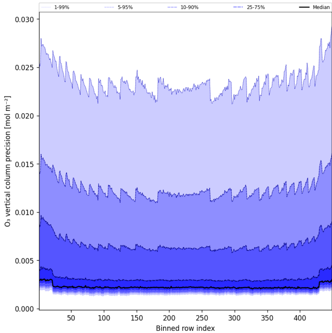
Figure 42: Along track statistics of “O 3 vertical column precision” for 2025-02-09 to 2025-02-10
