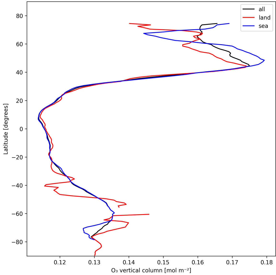
Figure 17: Zonal average of “O 3 vertical column” for 2025-02-09 to 2025-02-10.
