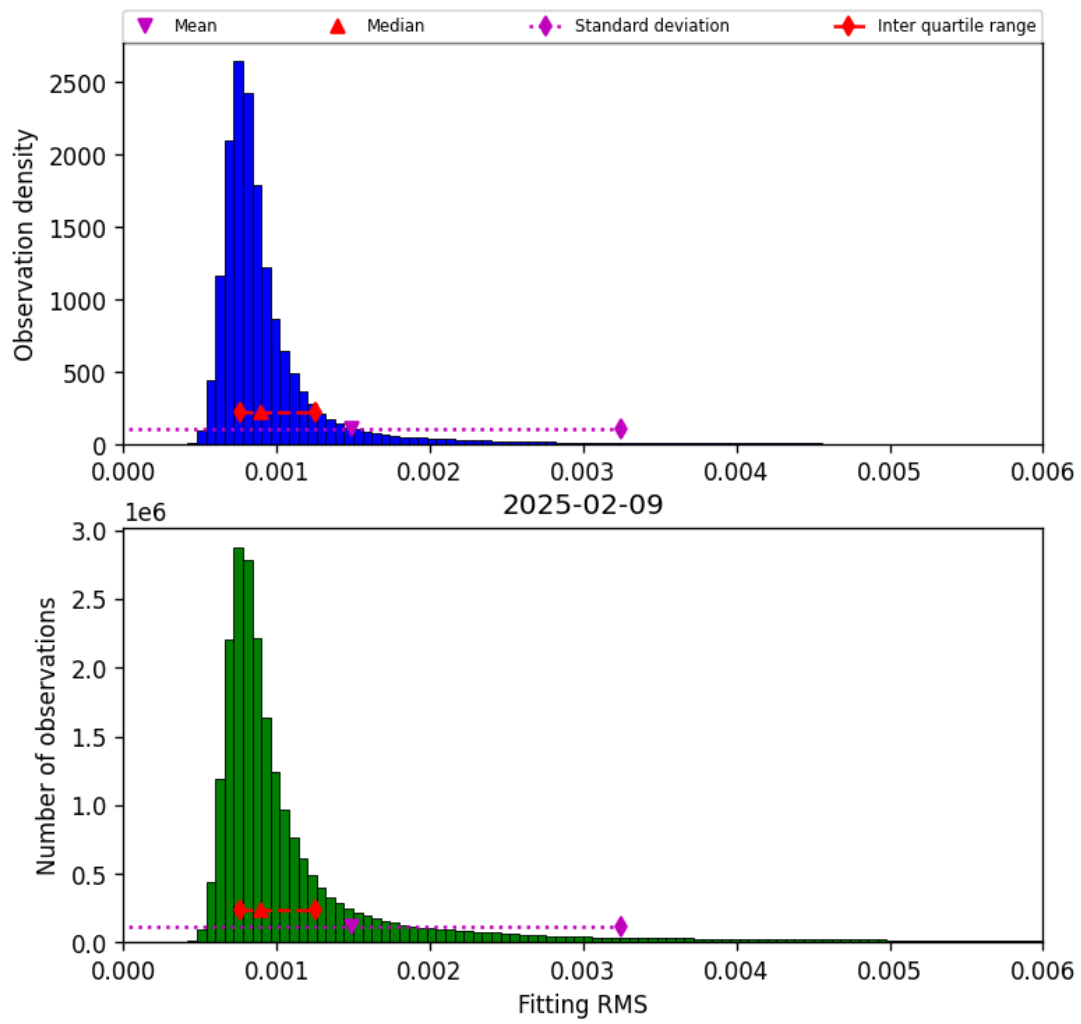
Figure 34: Histogram of “Fitting RMS” for 2025-02-09 to 2025-02-10
