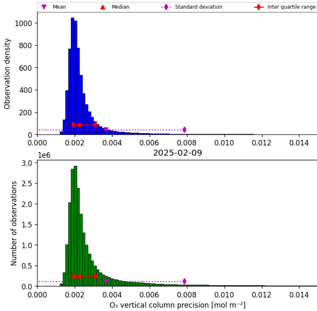
Figure 30: Histogram of “O 3 vertical column precision” for 2025-02-09 to 2025-02-10
