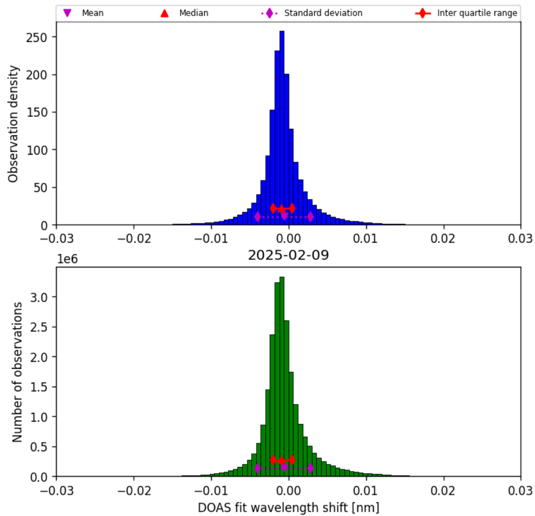
Figure 35: Histogram of “DOAS fit wavelength shift” for 2025-02-09 to 2025-02-10
