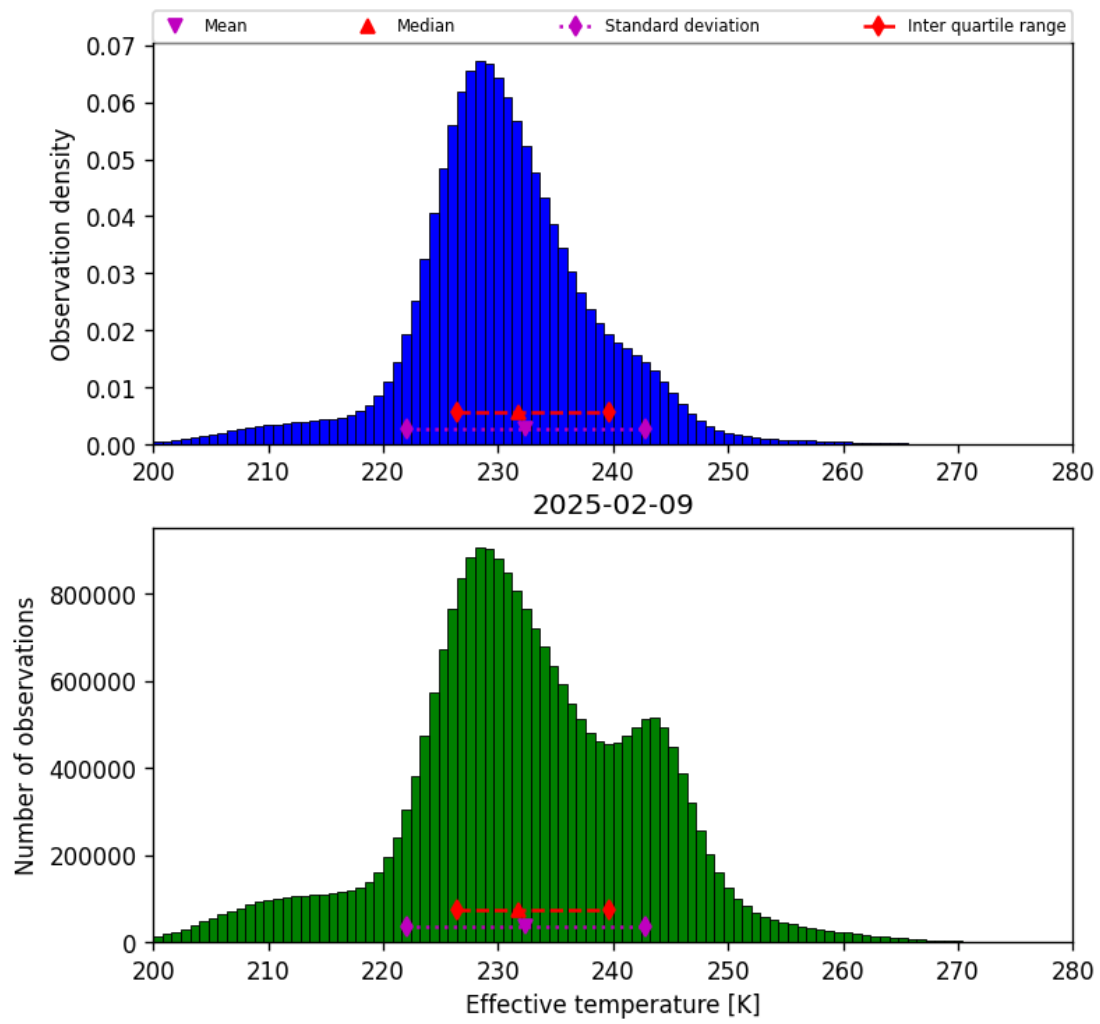
Figure 38: Histogram of “Effective temperature” for 2025-02-09 to 2025-02-10
