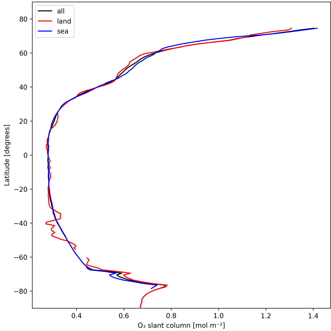
Figure 19: Zonal average of “O 3 slant column” for 2025-02-09 to 2025-02-10.
