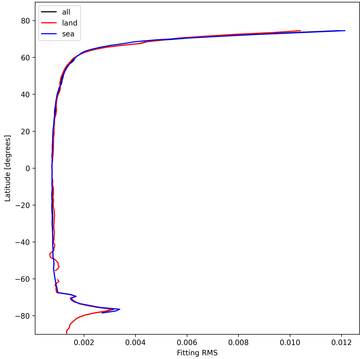
Figure 22: Zonal average of “Fitting RMS” for 2025-02-09 to 2025-02-10.
