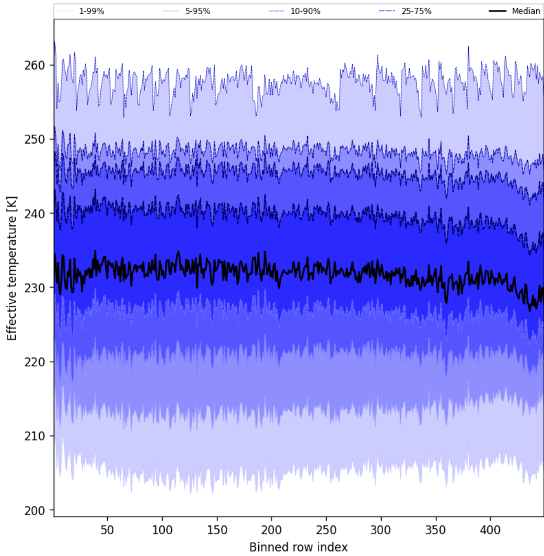
Figure 50: Along track statistics of “Effective temperature” for 2025-02-09 to 2025-02-10
