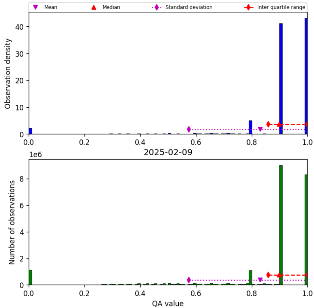
Figure 28: Histogram of “QA value” for 2025-02-09 to 2025-02-10
