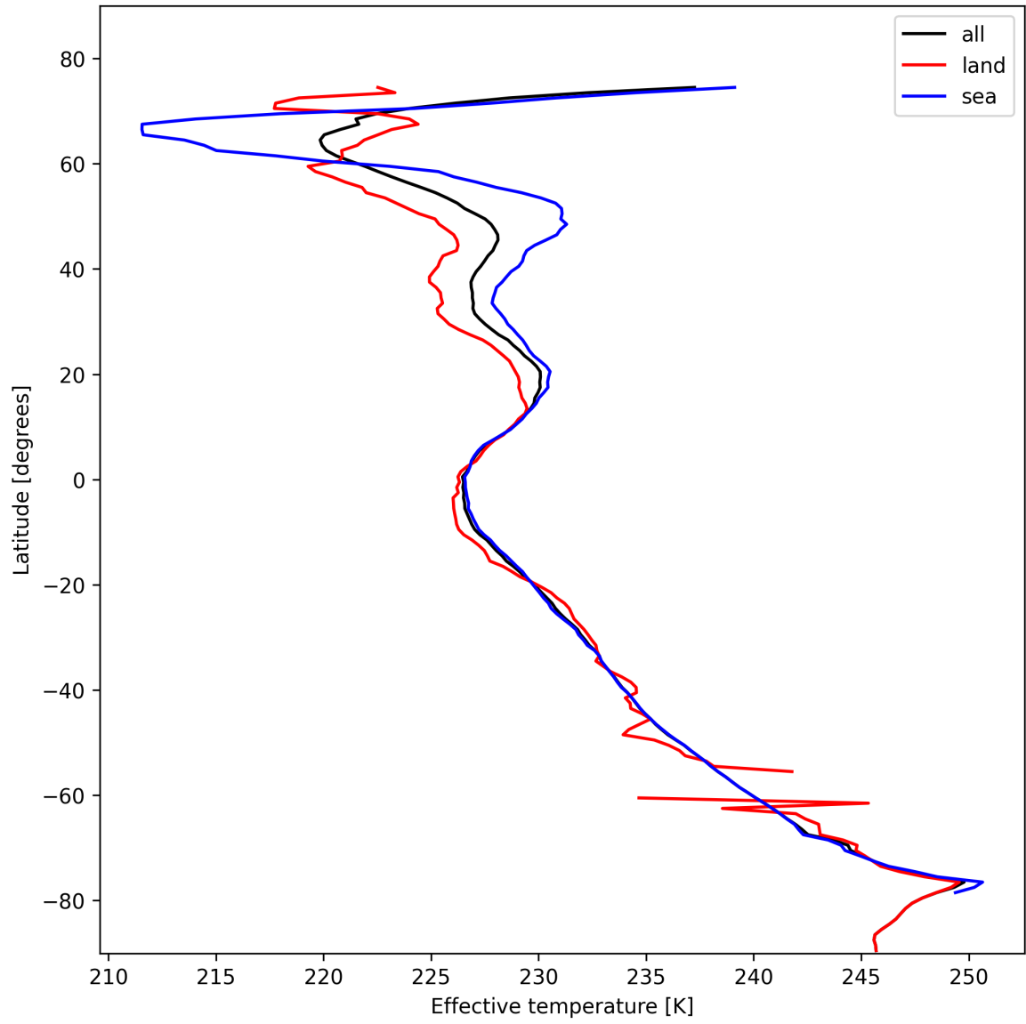
Figure 26: Zonal average of "Effective temperature" for 2025-02-09 to 2025-02-10.
