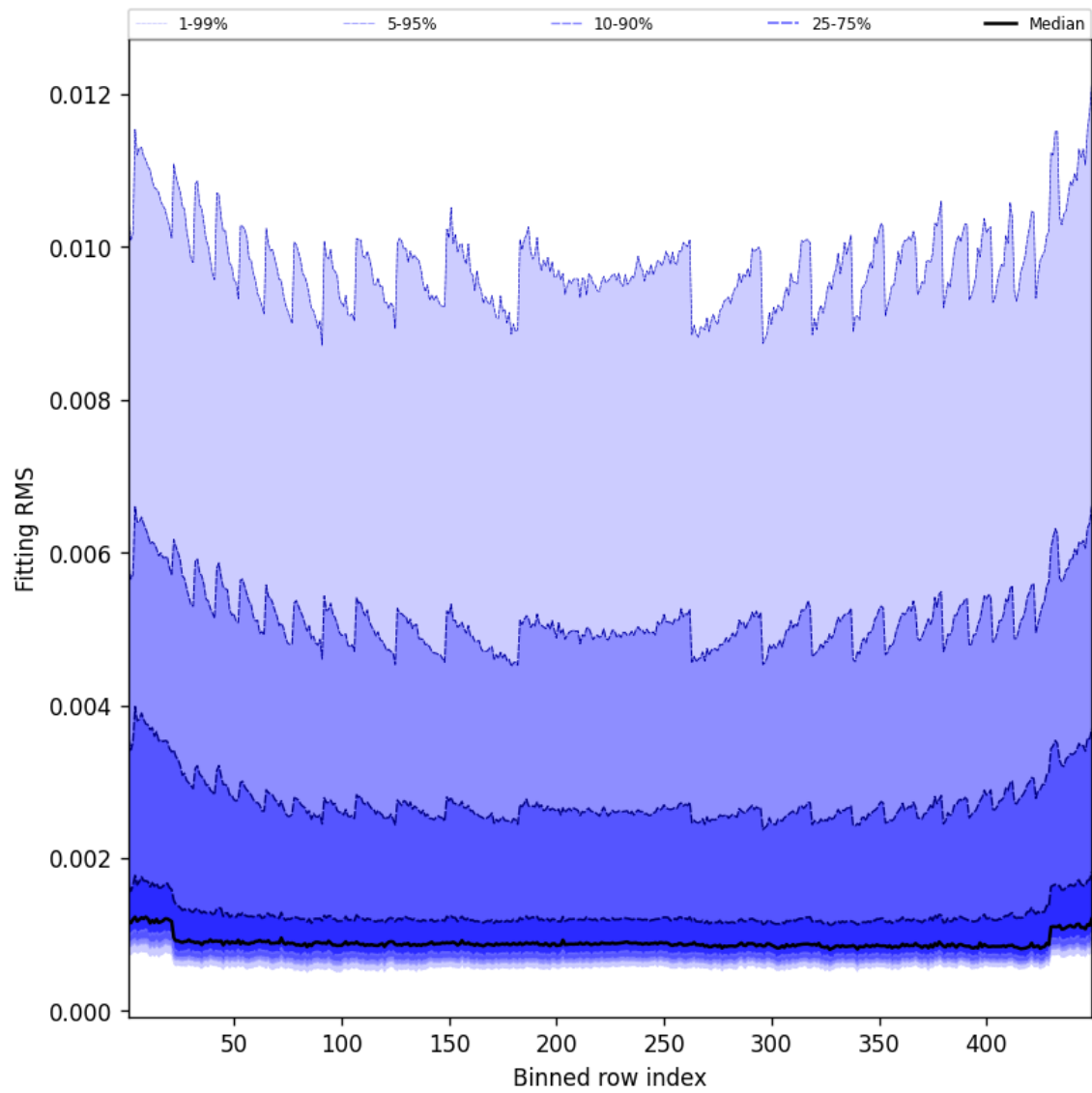
Figure 46: Along track statistics of “Fitting RMS” for 2025-02-09 to 2025-02-10
