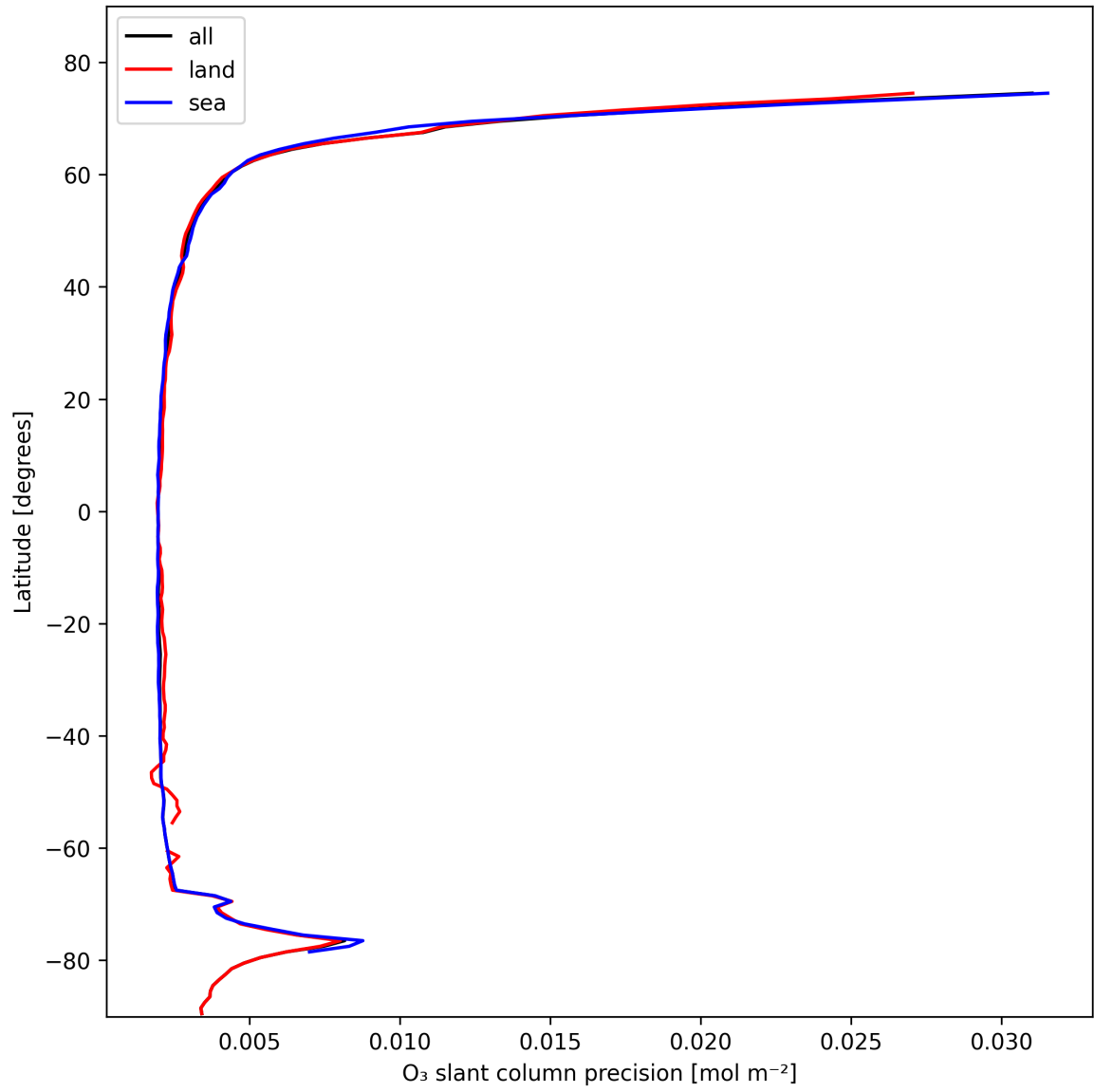
Figure 20: Zonal average of “O 3 slant column precision” for 2025-02-09 to 2025-02-10.
