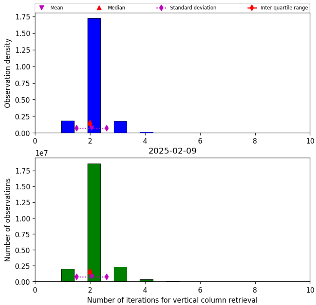
Figure 39: Histogram of “Number of iterations for vertical column retrieval” for 2025-02-09 to 2025-02-10
