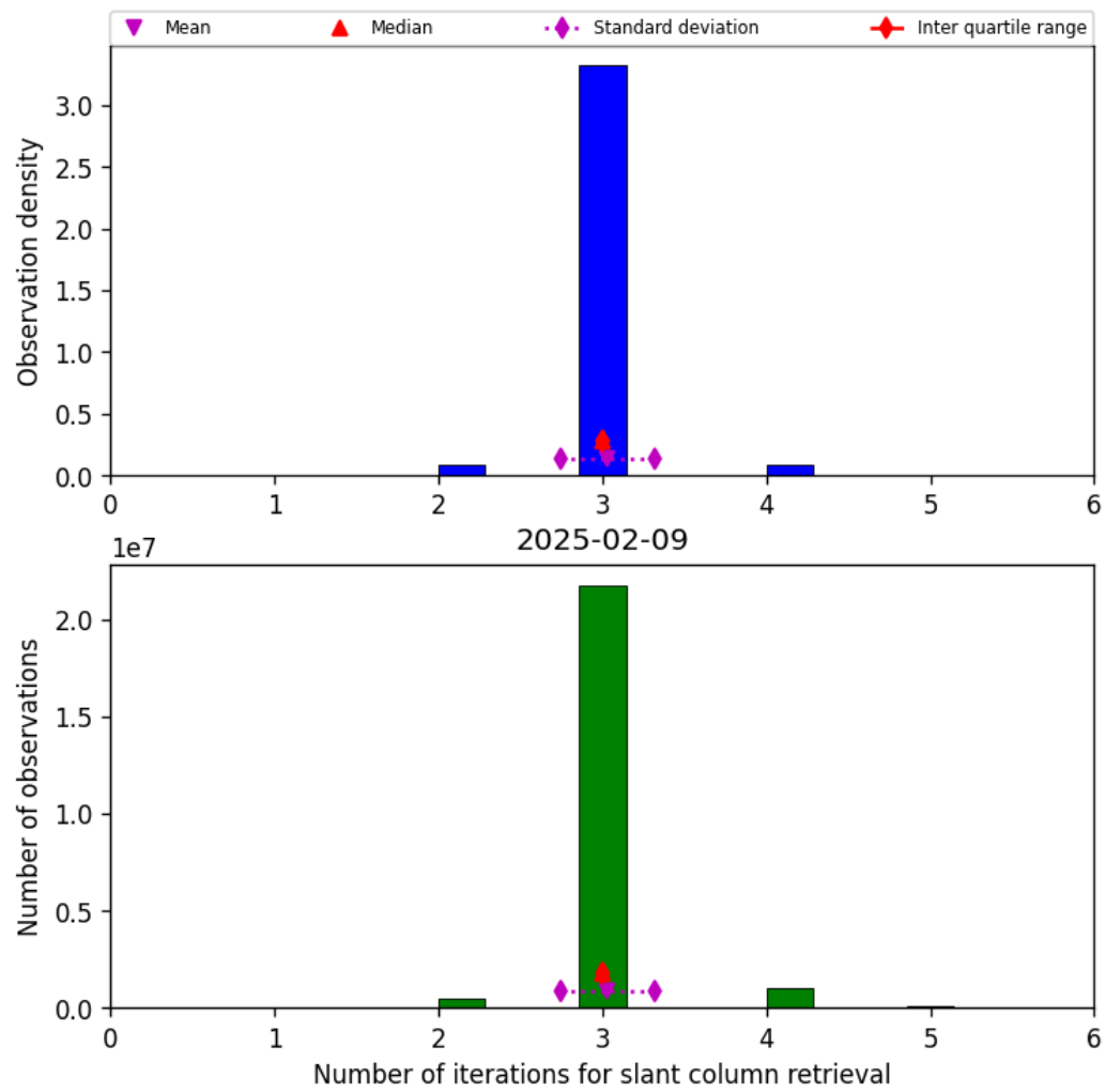
Figure 33: Histogram of "Number of iterations for slant column retrieval" for 2025-02-09 to 2025-02-10
