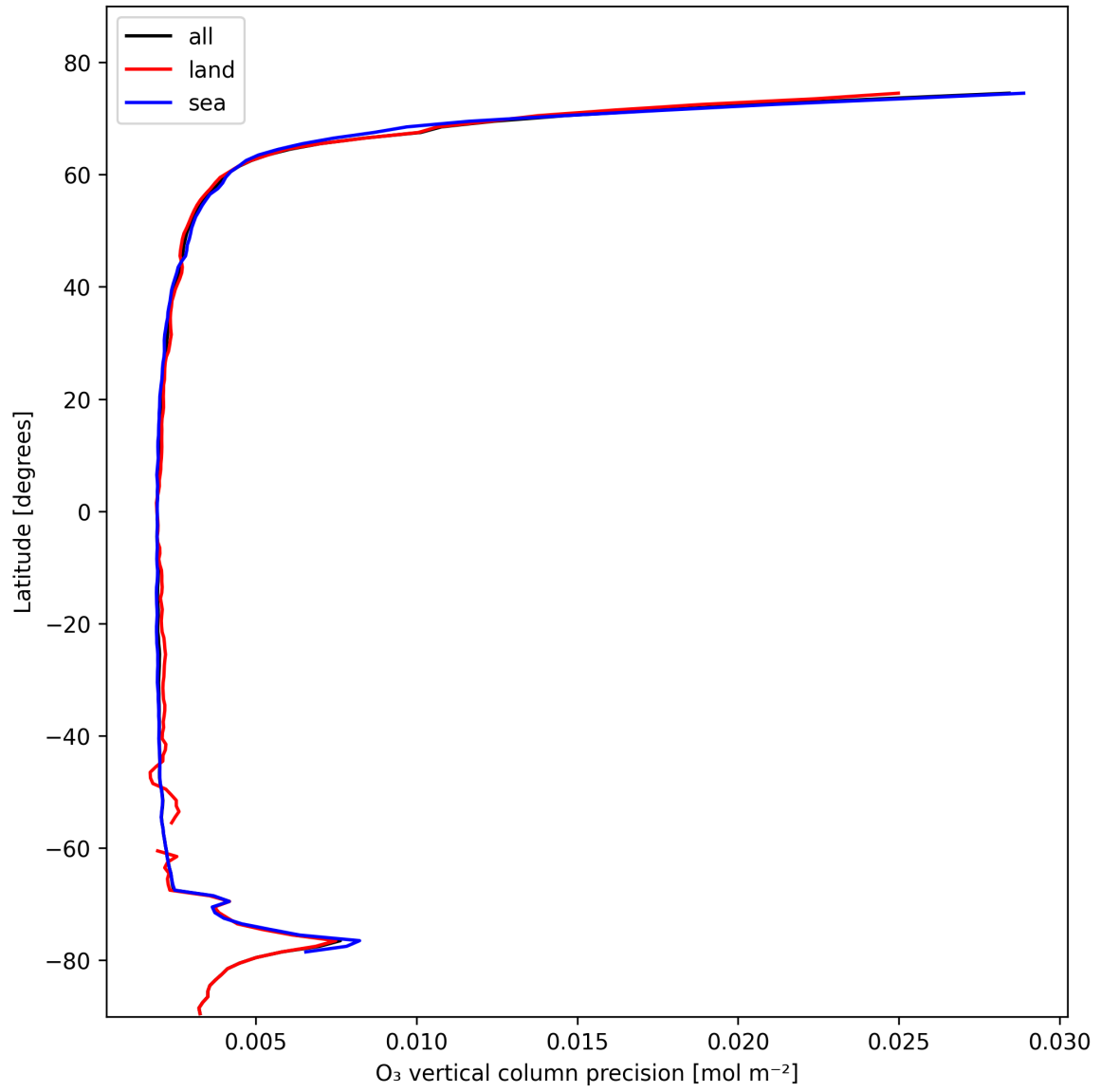
Figure 18: Zonal average of "O 3 vertical column precision" for 2025-02-09 to 2025-02-10.
