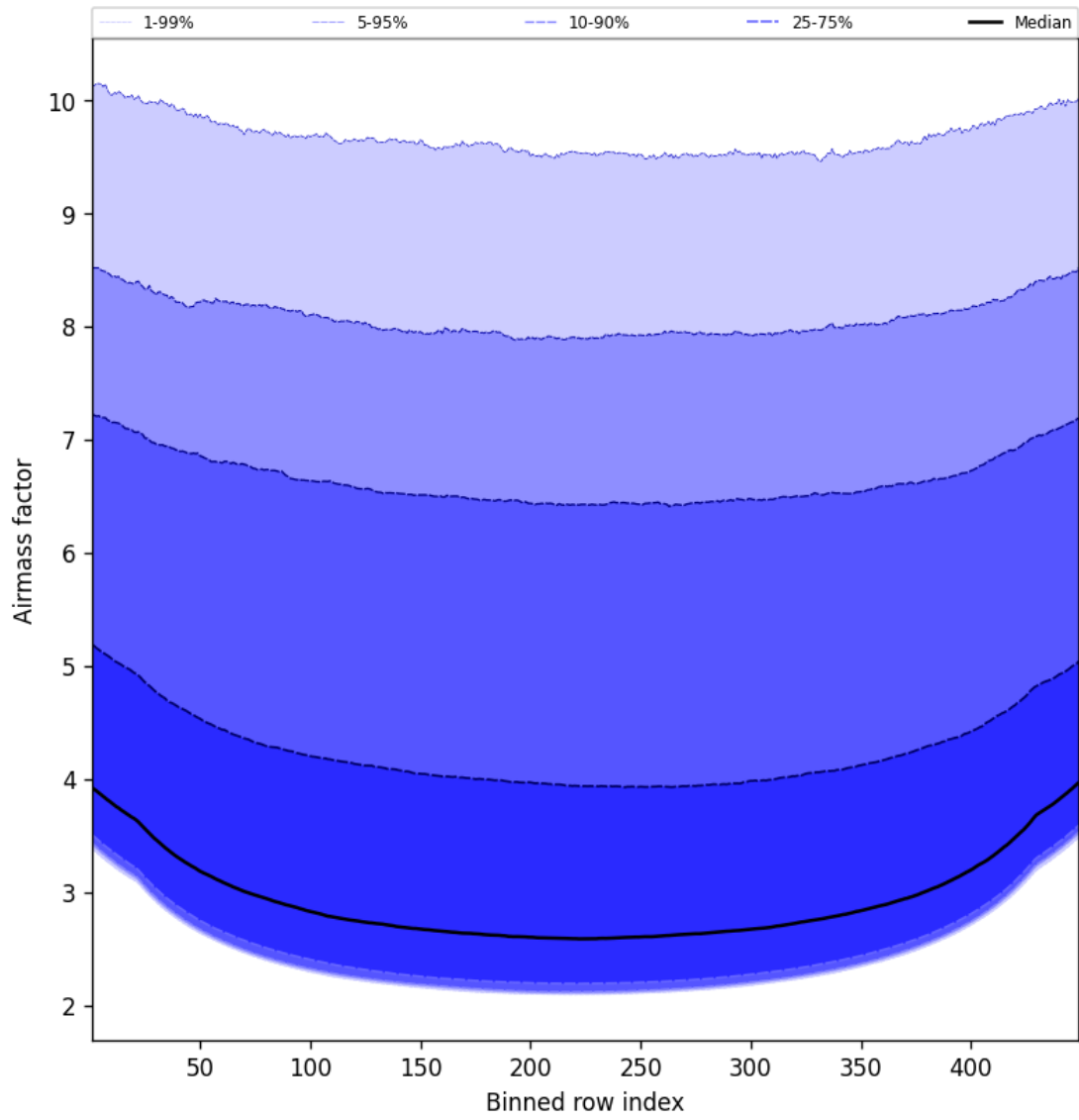
Figure 49: Along track statistics of “Airmass factor” for 2025-02-09 to 2025-02-10
