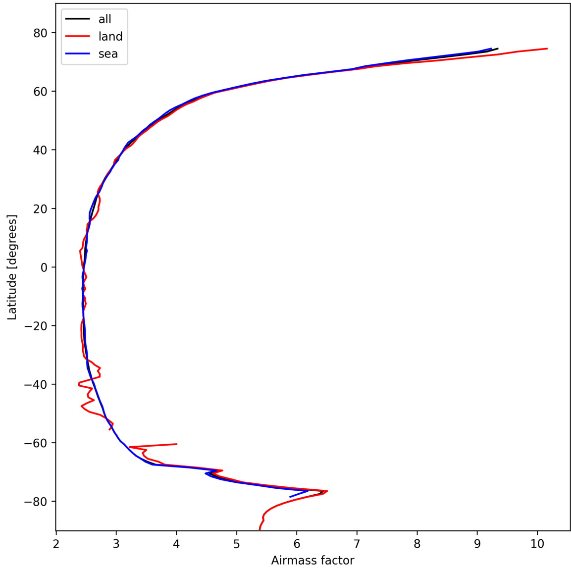
Figure 25: Zonal average of “Airmass factor” for 2025-02-09 to 2025-02-10.
