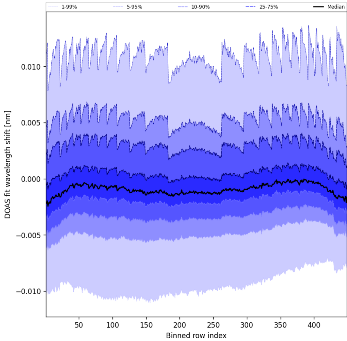
Figure 47: Along track statistics of “DOAS fit wavelength shift” for 2025-02-09 to 2025-02-10
