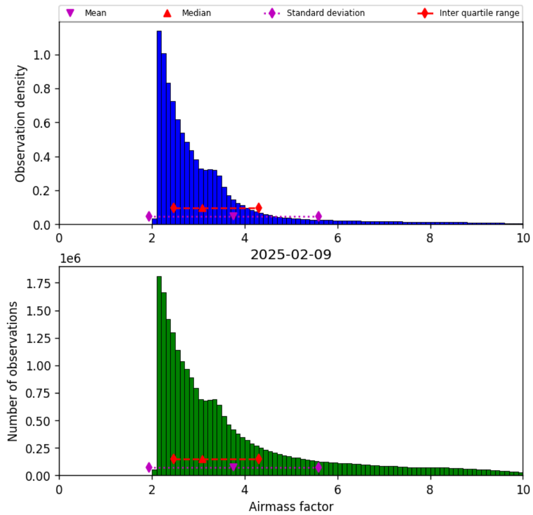
Figure 37: Histogram of “Airmass factor” for 2025-02-09 to 2025-02-10
