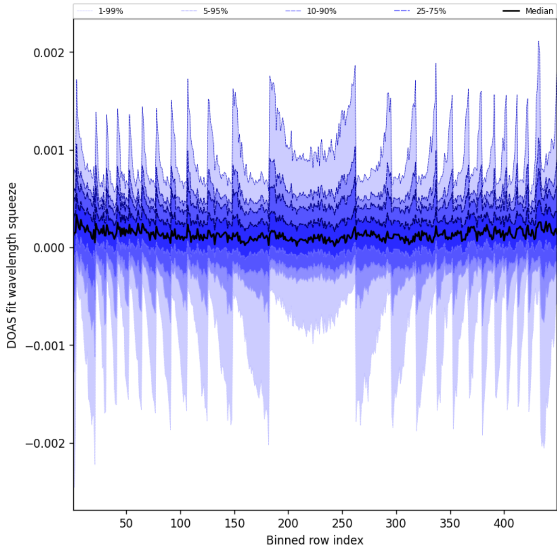
Figure 48: Along track statistics of “DOAS fit wavelength squeeze” for 2025-02-09 to 2025-02-10
