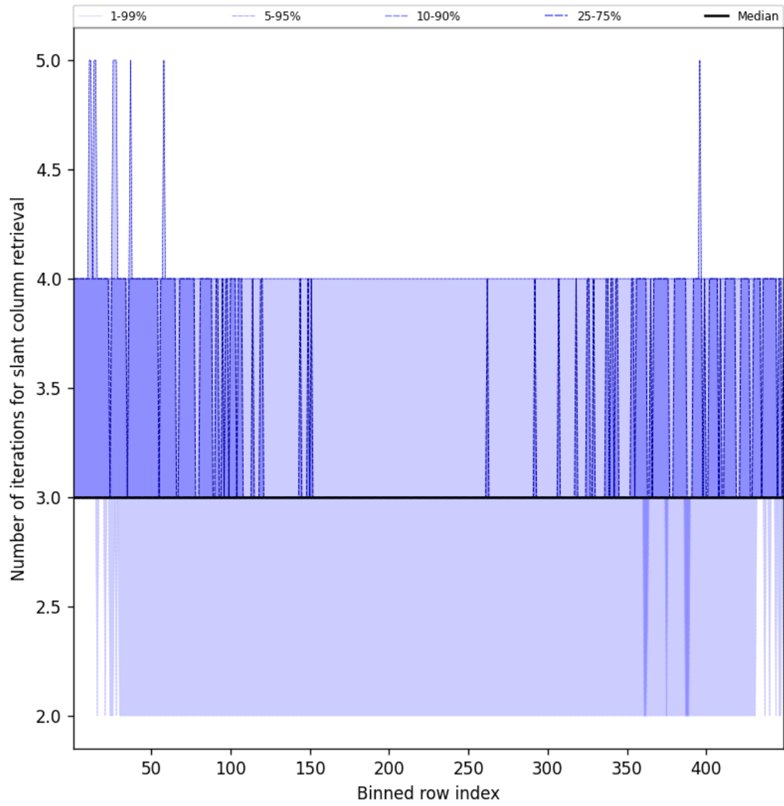
Figure 45: Along track statistics of “Number of iterations for slant column retrieval” for 2025-02-09 to 2025-02-10
