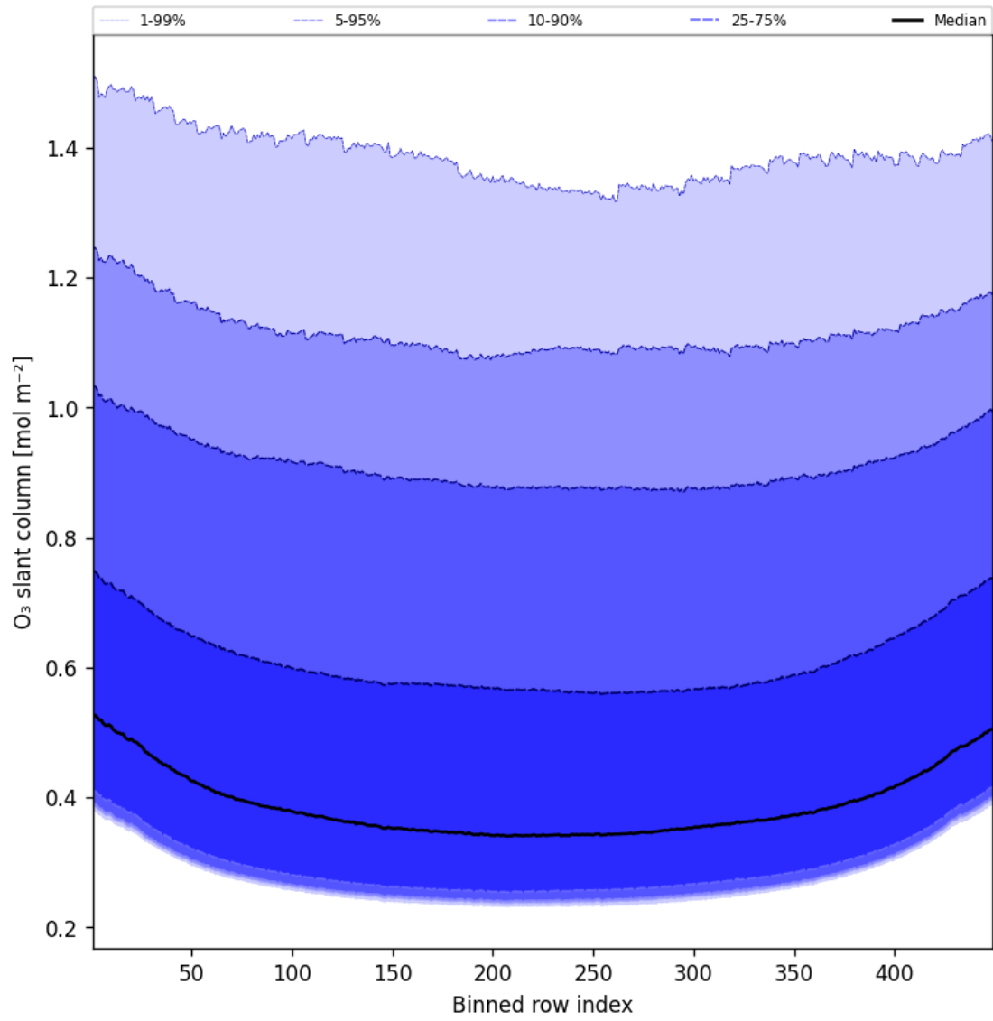
Figure 43: Along track statistics of “O 3 slant column” for 2025-02-09 to 2025-02-10
