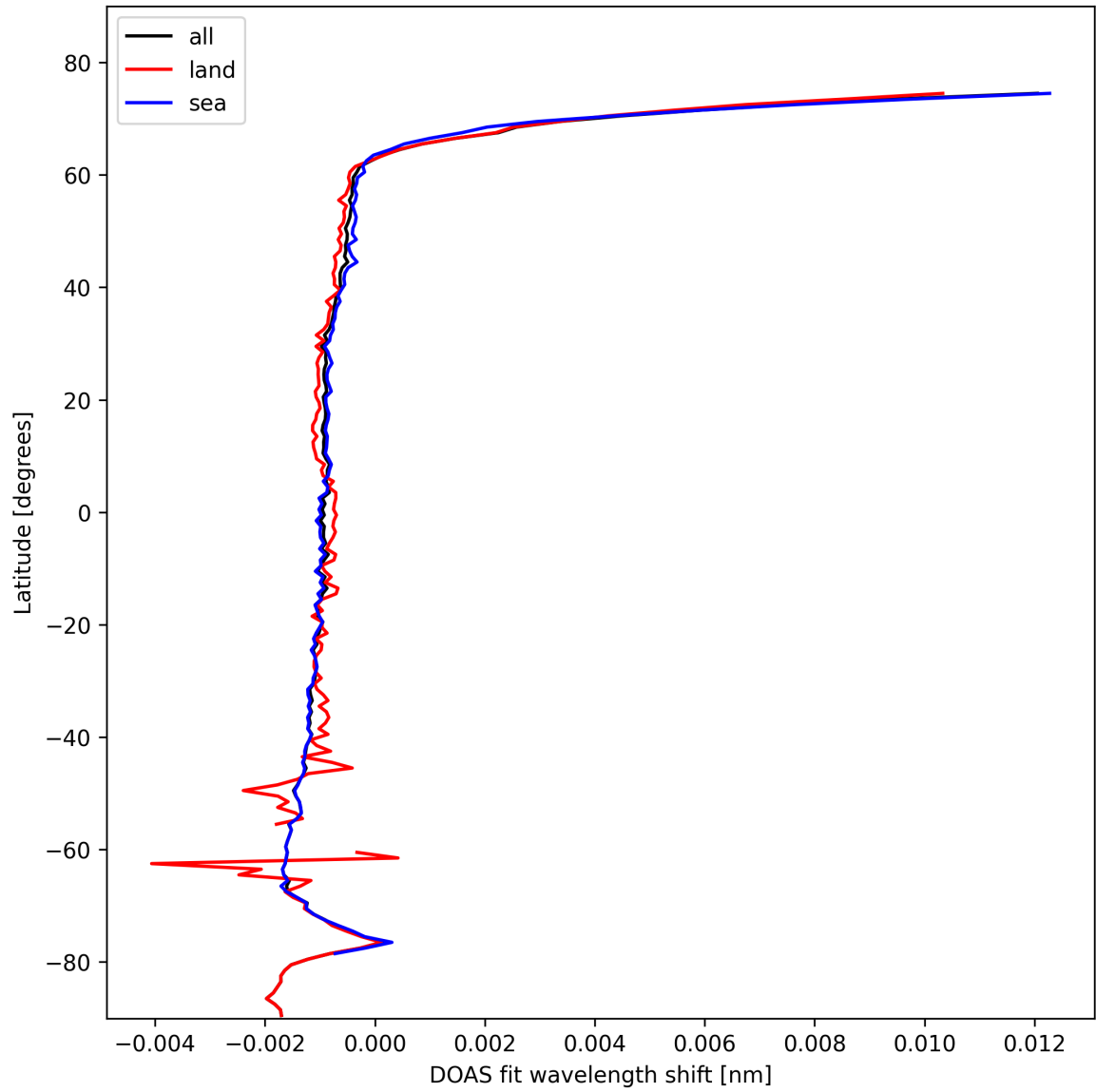
Figure 23: Zonal average of “DOAS fit wavelength shift” for 2025-02-09 to 2025-02-10.
