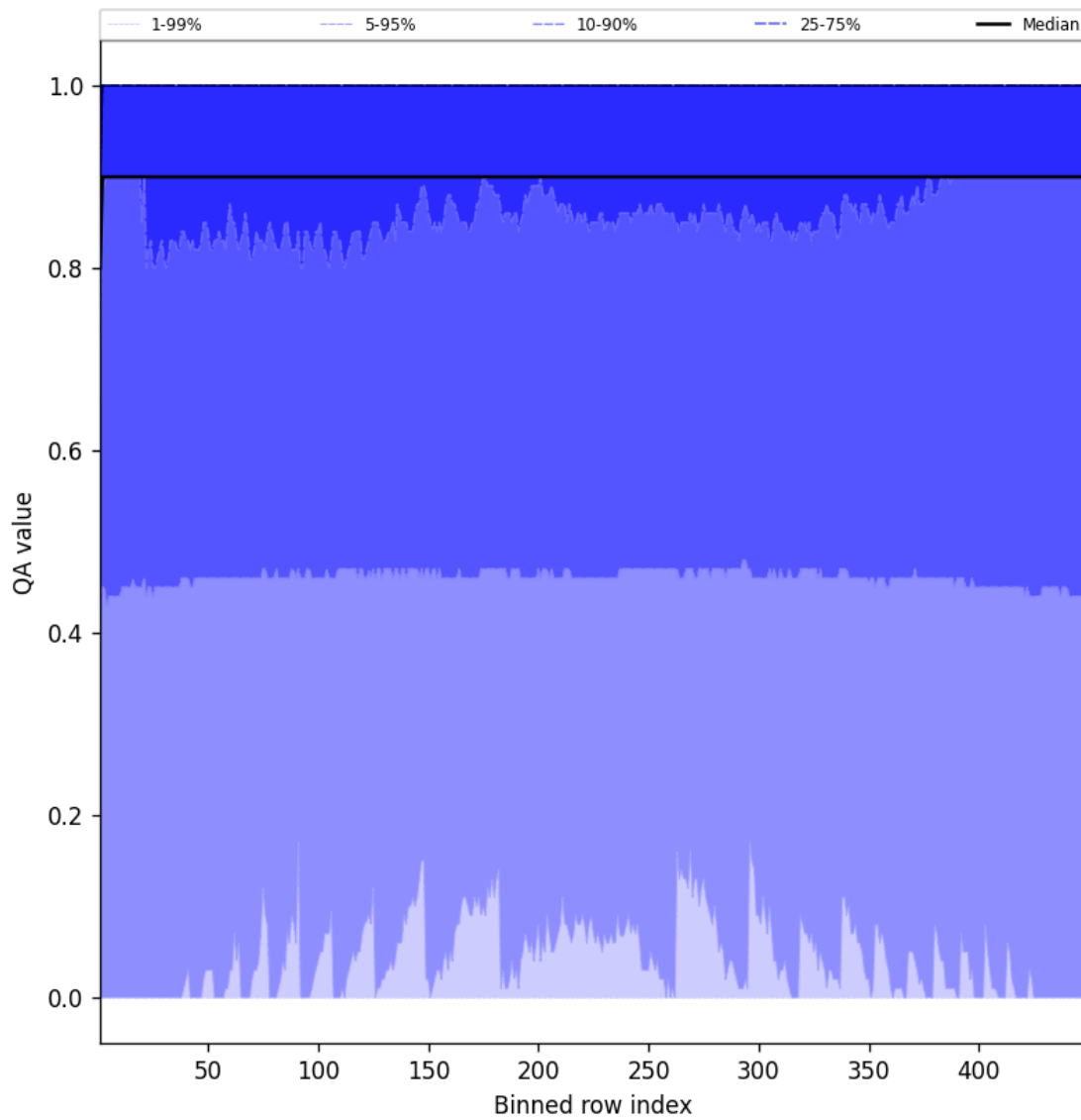
Figure 40: Along track statistics of “QA value” for 2025-02-09 to 2025-02-10
