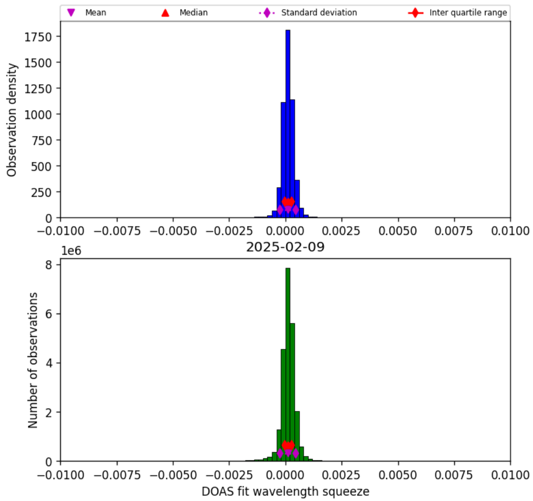
Figure 36: Histogram of “DOAS fit wavelength squeeze” for 2025-02-09 to 2025-02-10
