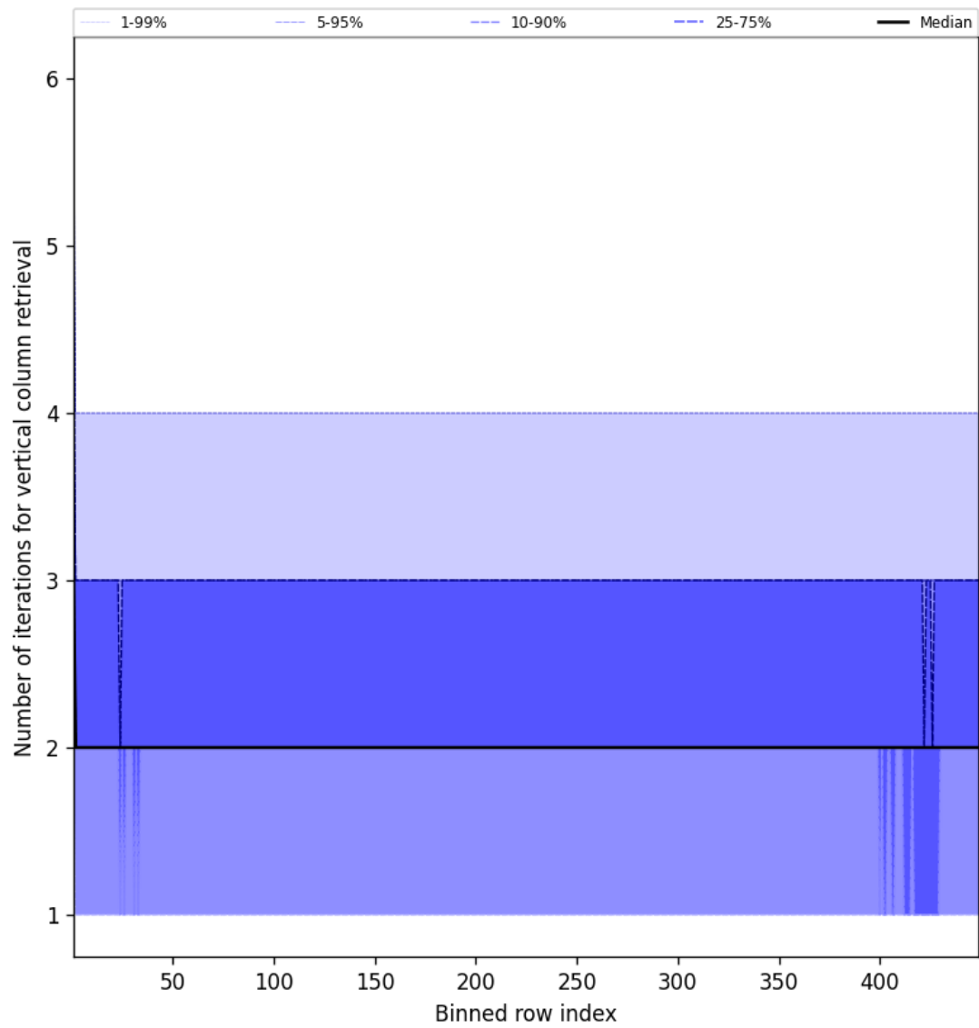
Figure 51: Along track statistics of “Number of iterations for vertical column retrieval” for 2025-02-09 to 2025-02-10
