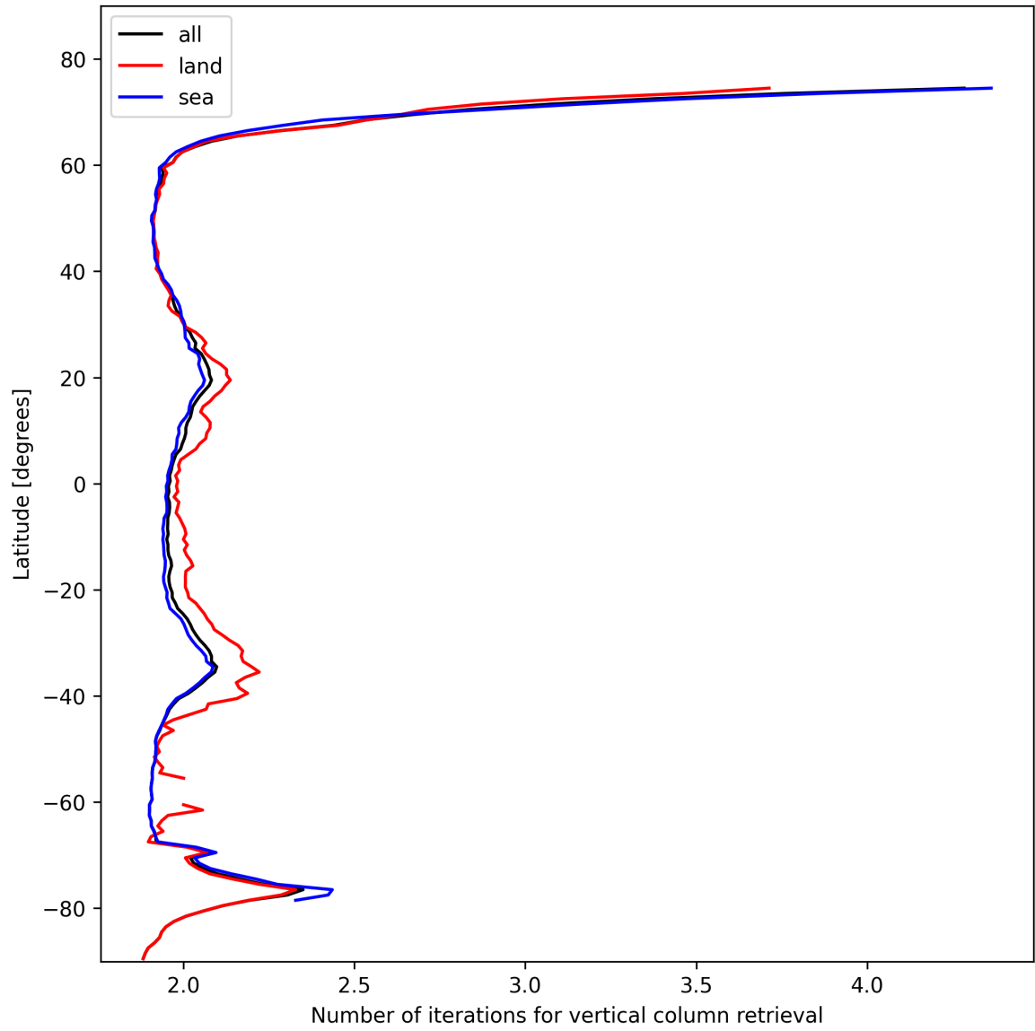
Figure 27: Zonal average of “Number of iterations for vertical column retrieval” for 2025-02-09 to 2025-02-10.
