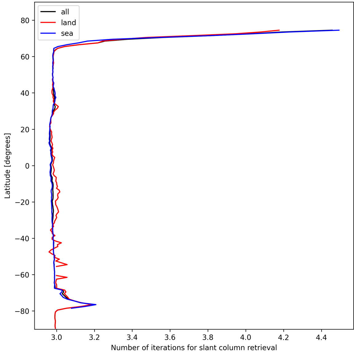
Figure 21: Zonal average of “Number of iterations for slant column retrieval” for 2025-02-09 to 2025-02-10.
