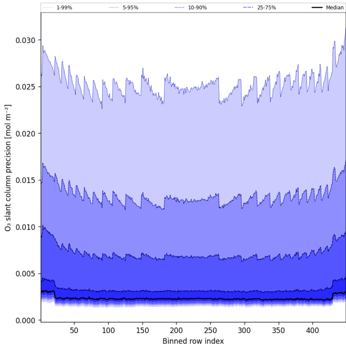
Figure 44: Along track statistics of “O 3 slant column precision” for 2025-02-09 to 2025-02-10
