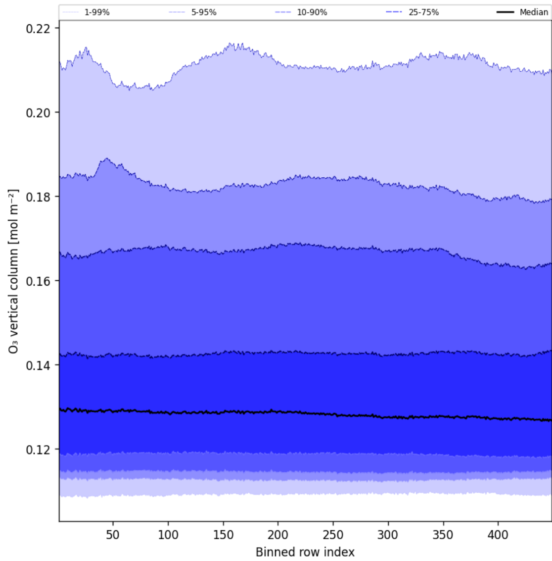
Figure 41: Along track statistics of “O 3 vertical column” for 2025-02-09 to 2025-02-10
