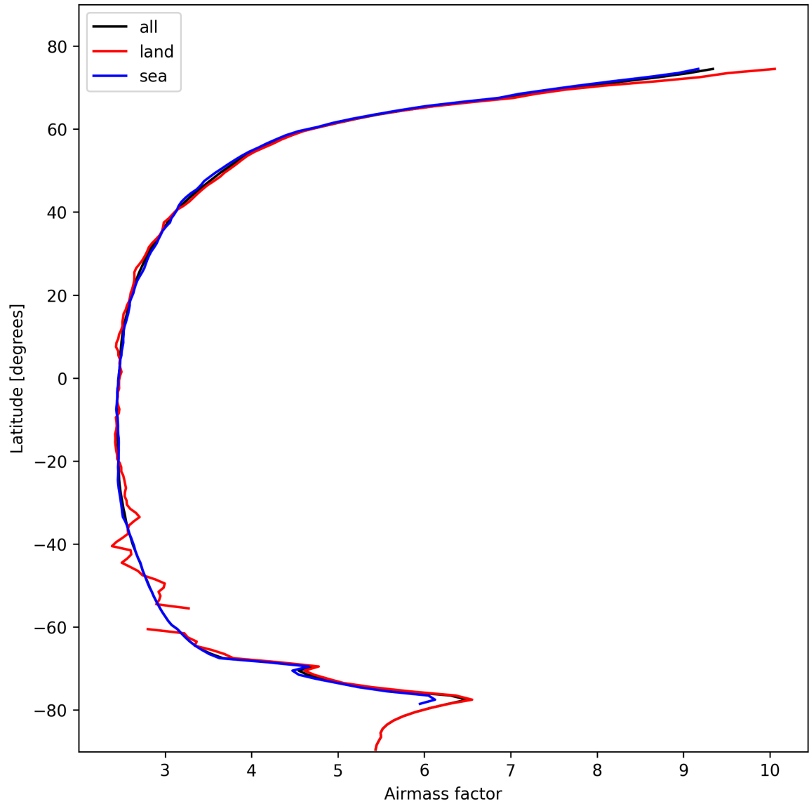
Figure 25: Zonal average of “Airmass factor” for 2025-02-10 to 2025-02-11.
