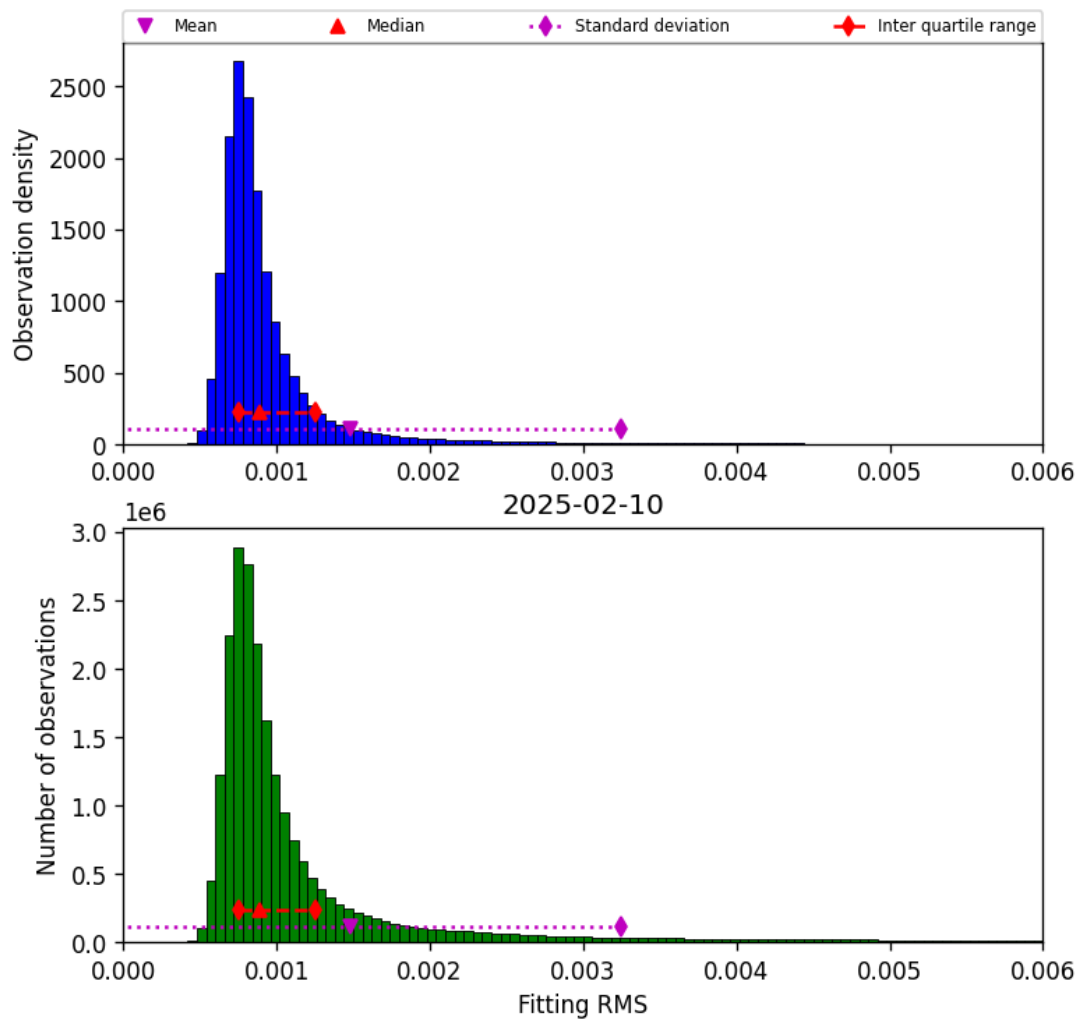
Figure 34: Histogram of “Fitting RMS” for 2025-02-10 to 2025-02-11
