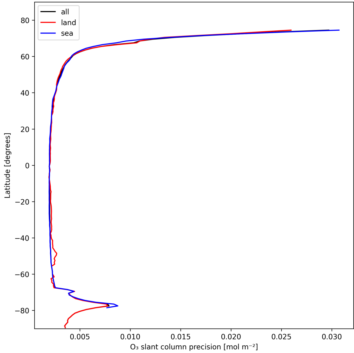
Figure 20: Zonal average of “O 3 slant column precision” for 2025-02-10 to 2025-02-11.
