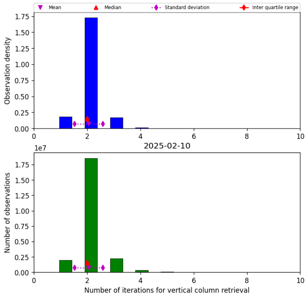
Figure 39: Histogram of “Number of iterations for vertical column retrieval” for 2025-02-10 to 2025-02-11
