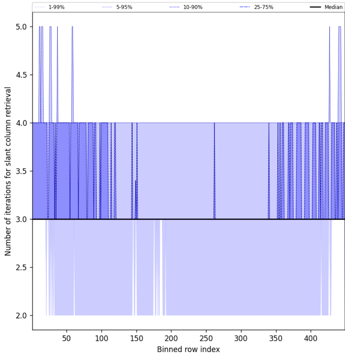
Figure 45: Along track statistics of “Number of iterations for slant column retrieval” for 2025-02-10 to 2025-02-11
