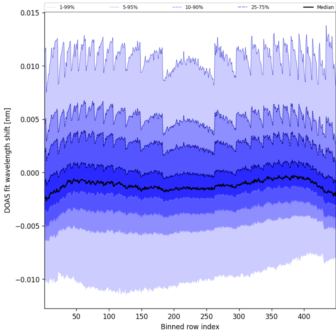
Figure 47: Along track statistics of “DOAS fit wavelength shift” for 2025-02-10 to 2025-02-11
