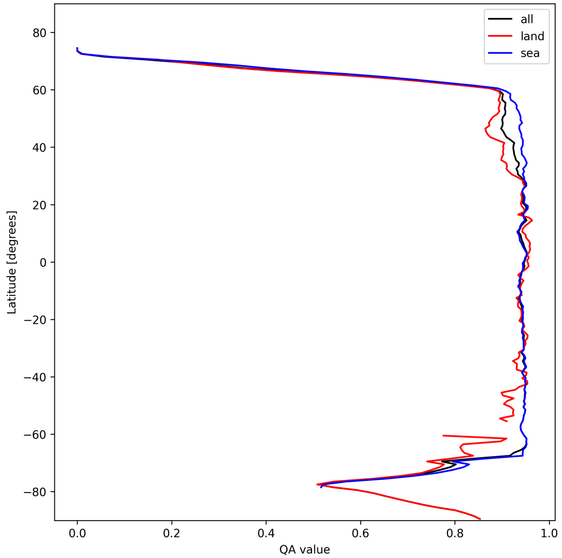
Figure 16: Zonal average of “QA value” for 2025-02-10 to 2025-02-11.
