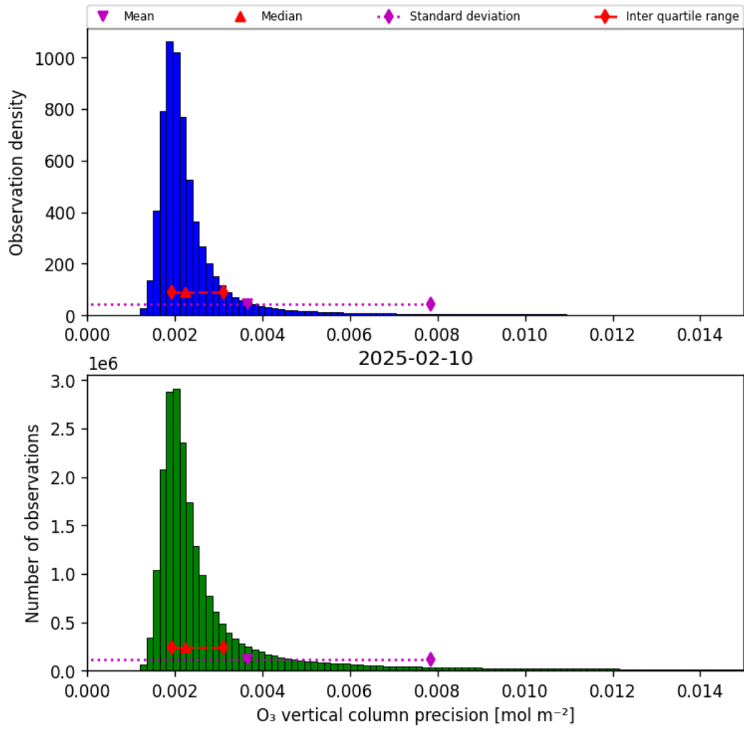
Figure 30: Histogram of "O 3 vertical column precision" for 2025-02-10 to 2025-02-11
