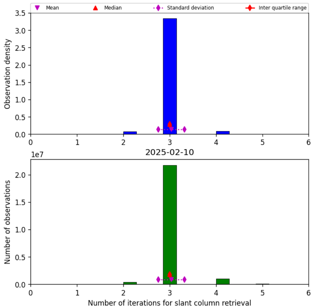
Figure 33: Histogram of “Number of iterations for slant column retrieval” for 2025-02-10 to 2025-02-11
