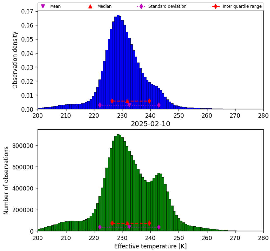
Figure 38: Histogram of “Effective temperature” for 2025-02-10 to 2025-02-11
