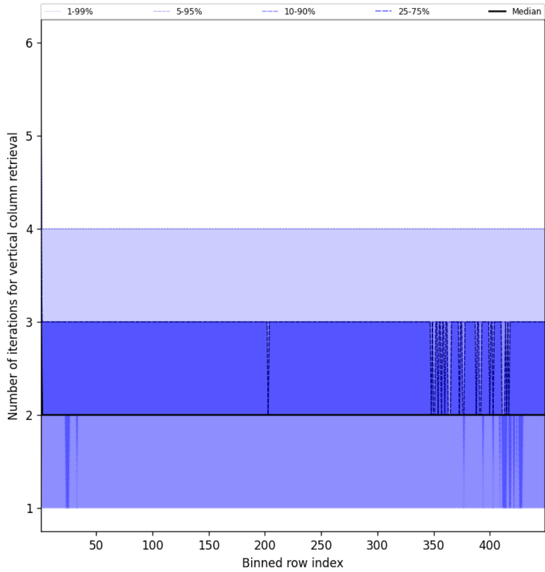
Figure 51: Along track statistics of “Number of iterations for vertical column retrieval” for 2025-02-10 to 2025-02-11
