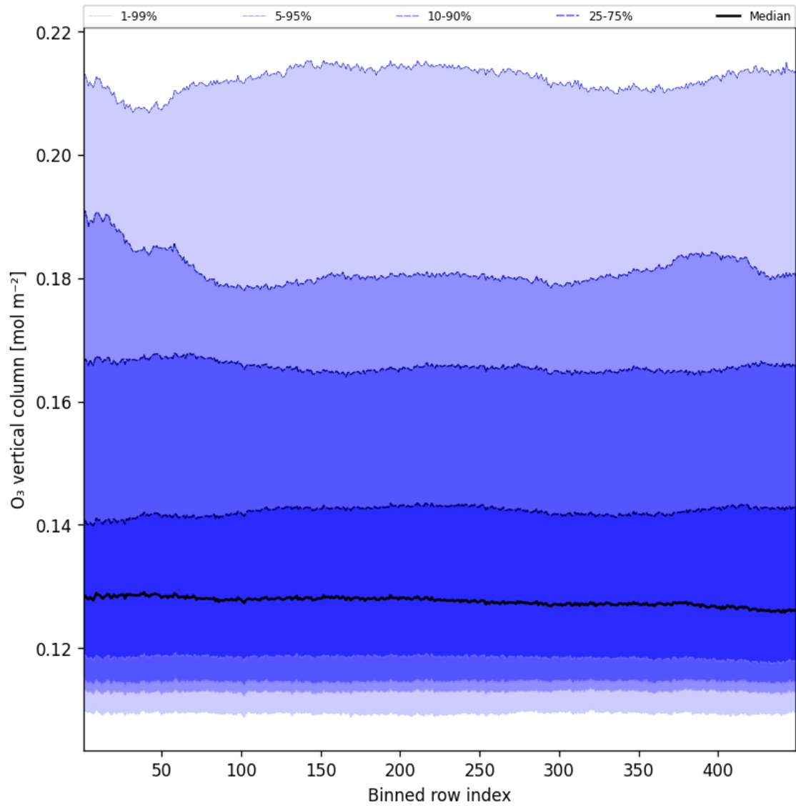
Figure 41: Along track statistics of “O 3 vertical column” for 2025-02-10 to 2025-02-11
