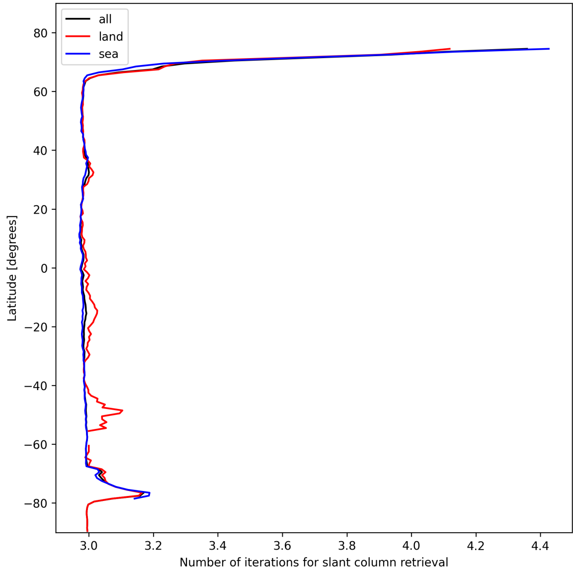
Figure 21: Zonal average of “Number of iterations for slant column retrieval” for 2025-02-10 to 2025-02-11.
