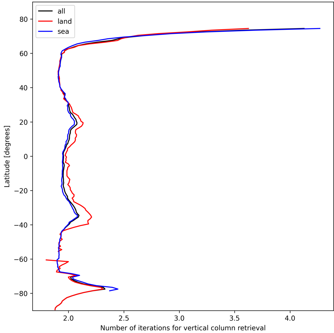
Figure 27: Zonal average of “Number of iterations for vertical column retrieval” for 2025-02-10 to 2025-02-11.
