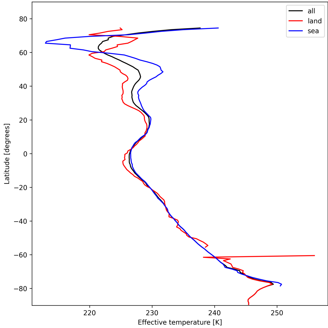
Figure 26: Zonal average of “Effective temperature” for 2025-02-10 to 2025-02-11.
