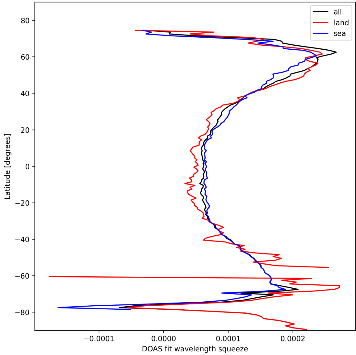
Figure 24: Zonal average of "DOAS fit wavelength squeeze" for 2025-02-10 to 2025-02-11.
