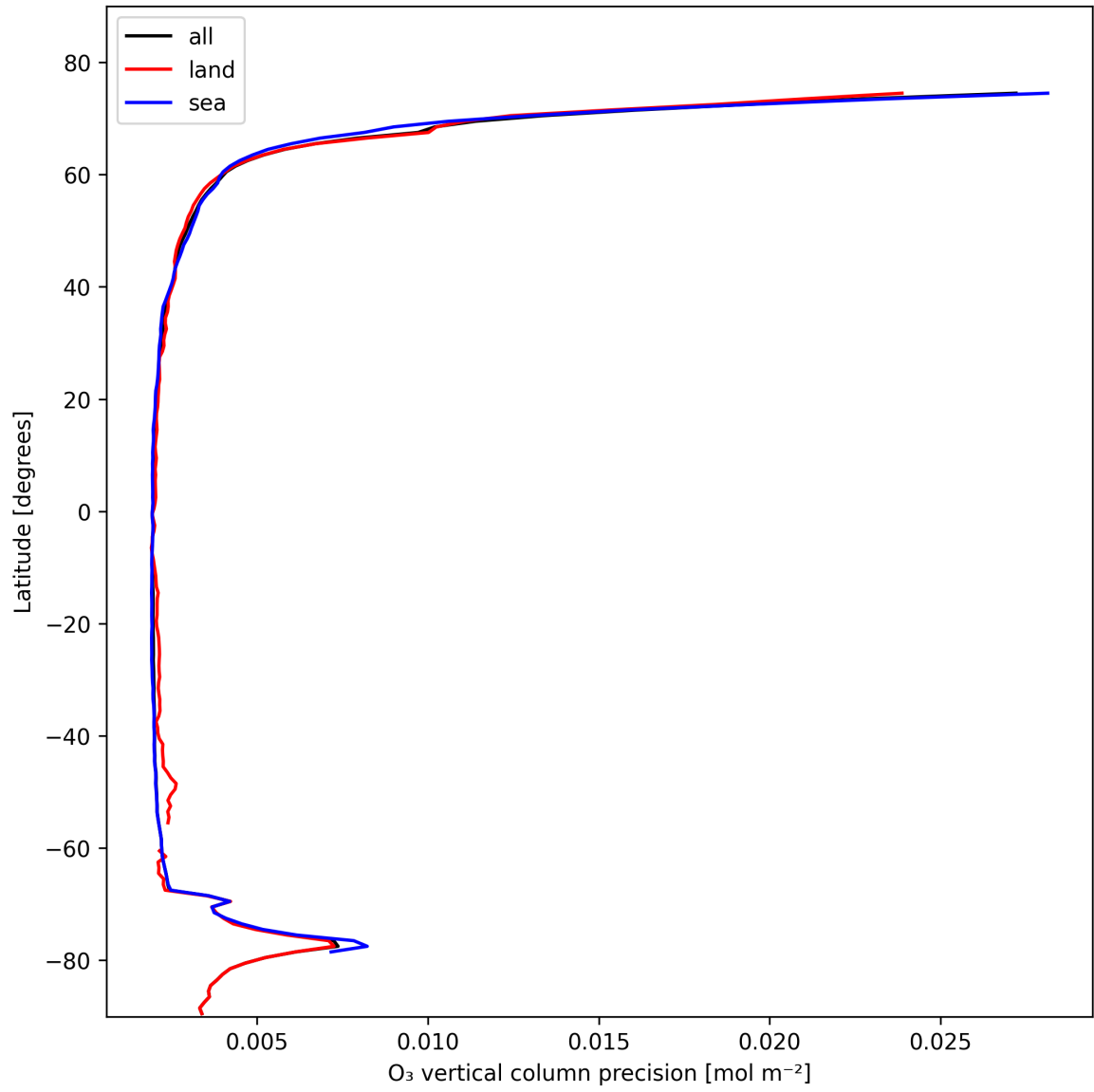
Figure 18: Zonal average of “O 3 vertical column precision” for 2025-02-10 to 2025-02-11.
