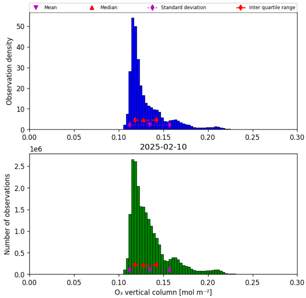
Figure 29: Histogram of “O 3 vertical column” for 2025-02-10 to 2025-02-11
