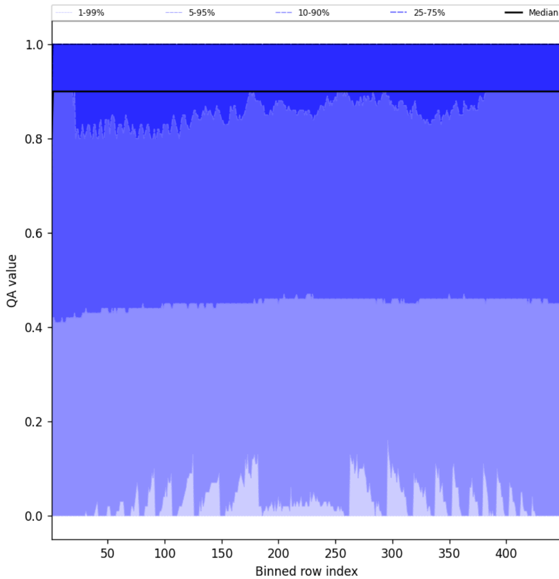
Figure 40: Along track statistics of “QA value” for 2025-02-10 to 2025-02-11
