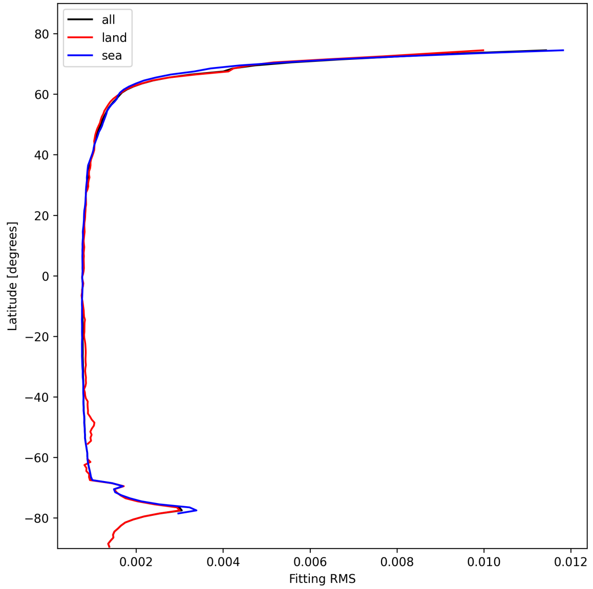
Figure 22: Zonal average of “Fitting RMS” for 2025-02-10 to 2025-02-11.
