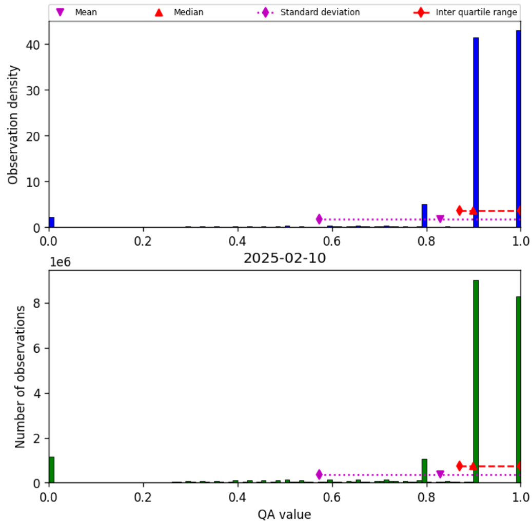
Figure 28: Histogram of “QA value” for 2025-02-10 to 2025-02-11
