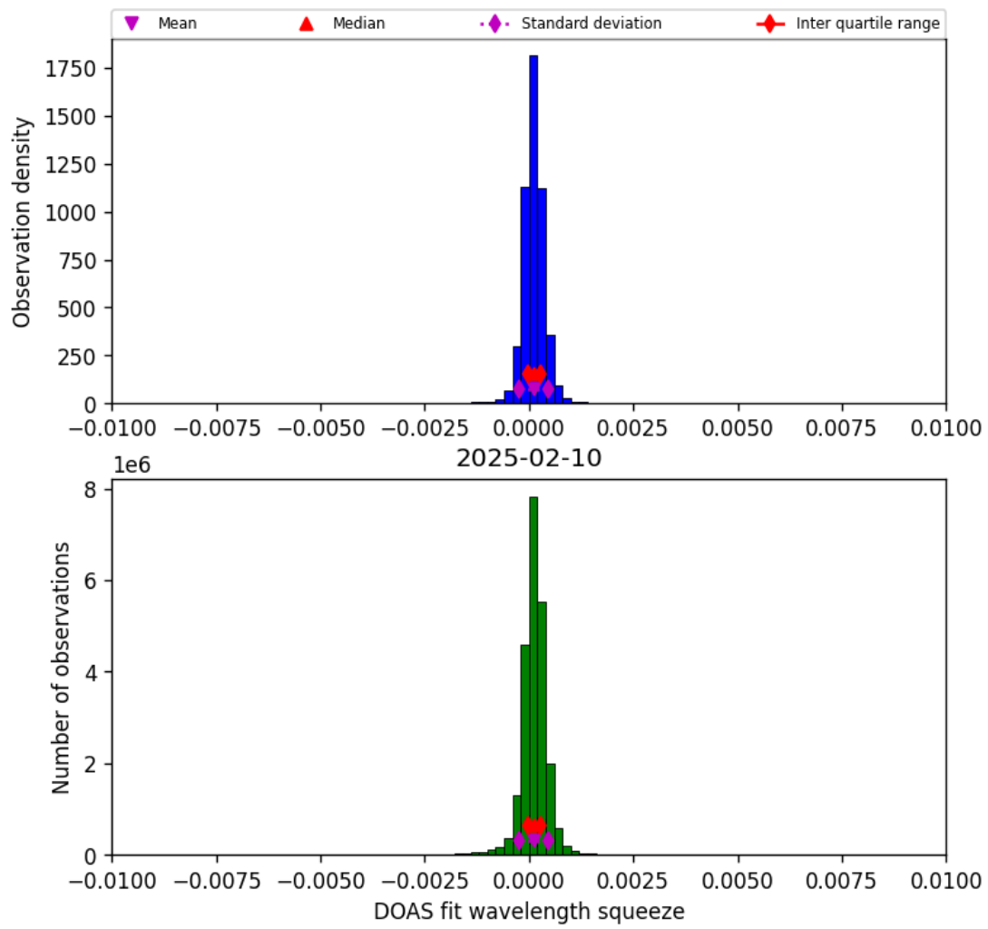
Figure 36: Histogram of “DOAS fit wavelength squeeze” for 2025-02-10 to 2025-02-11
