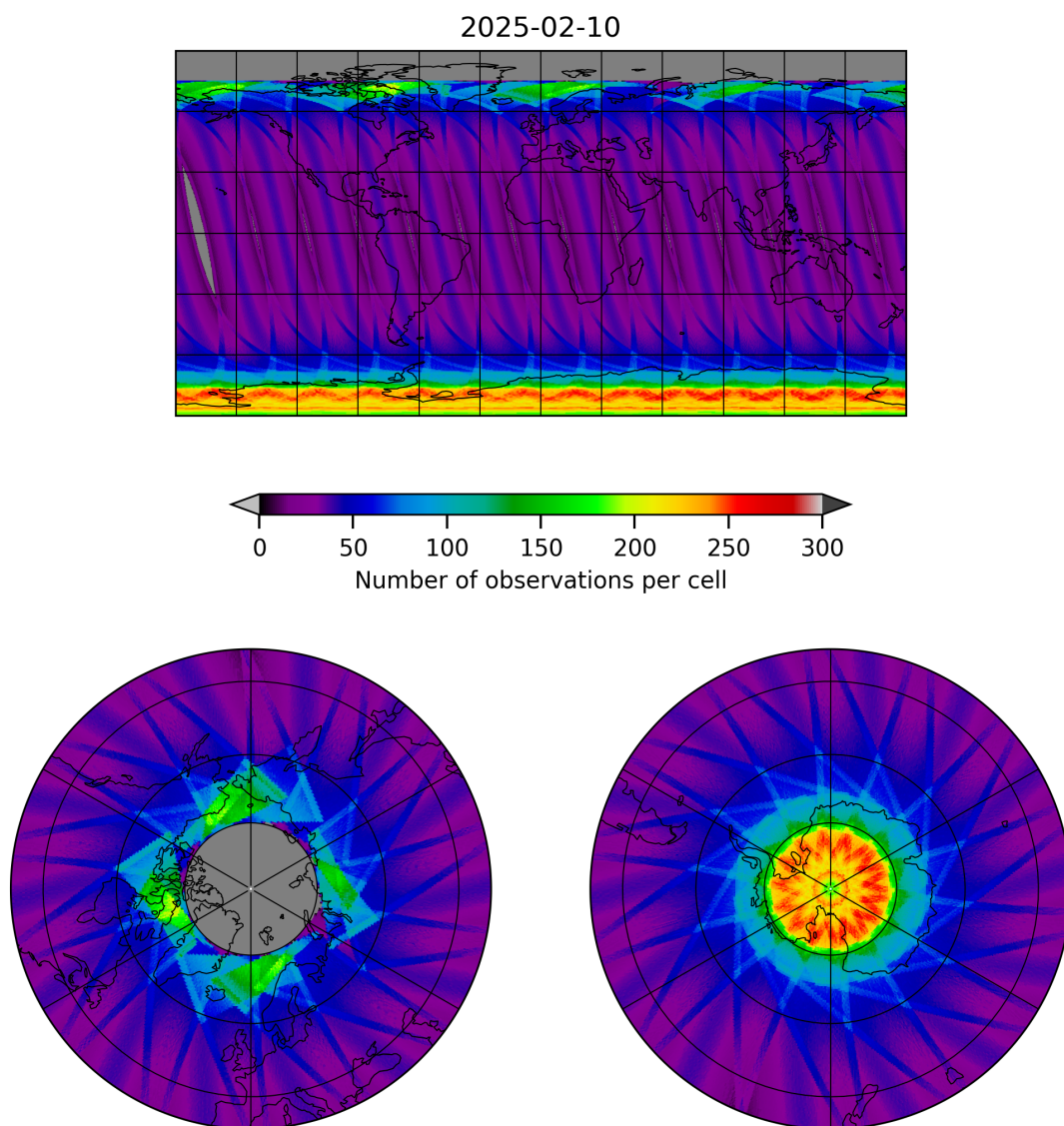
Figure 15: Map of the number of observations for 2025-02-10 to 2025-02-11
