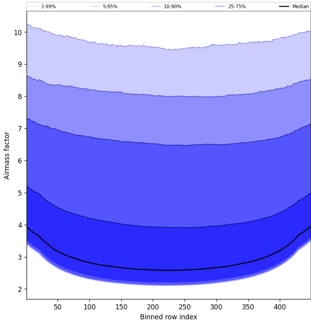
Figure 49: Along track statistics of “Airmass factor” for 2025-02-10 to 2025-02-11
