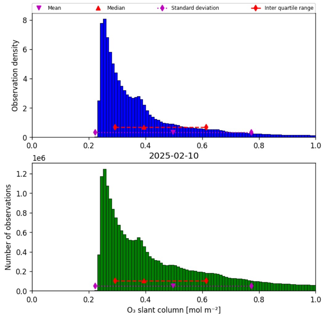
Figure 31: Histogram of “O 3 slant column” for 2025-02-10 to 2025-02-11
