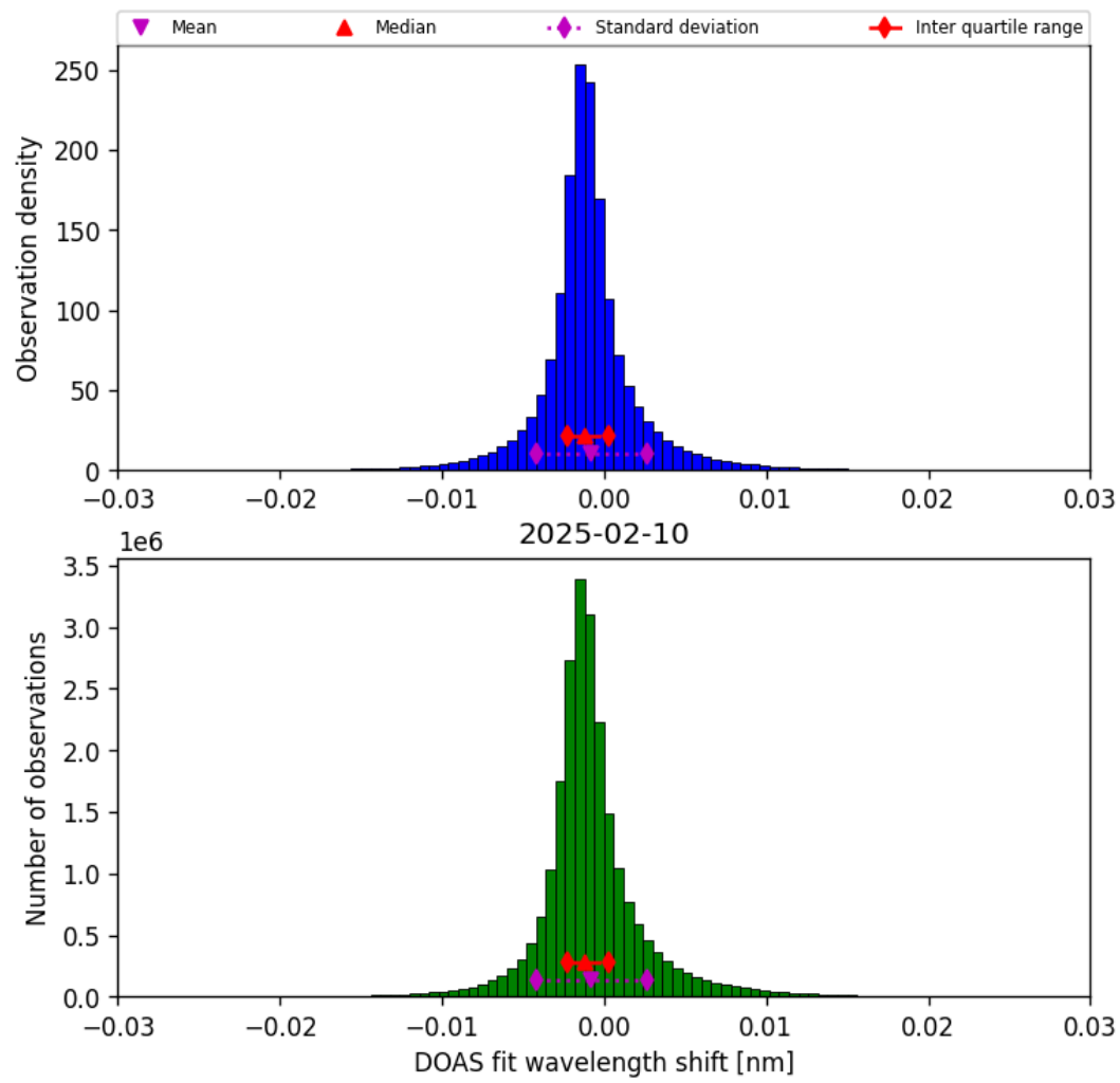
Figure 35: Histogram of “DOAS fit wavelength shift” for 2025-02-10 to 2025-02-11
