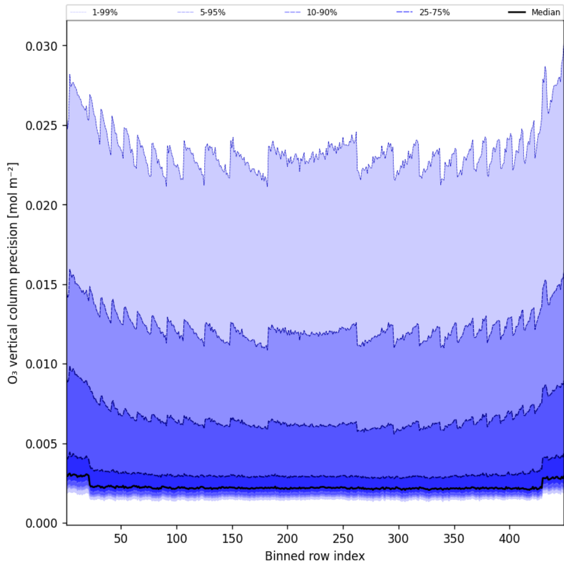
Figure 42: Along track statistics of “O 3 vertical column precision” for 2025-02-10 to 2025-02-11
