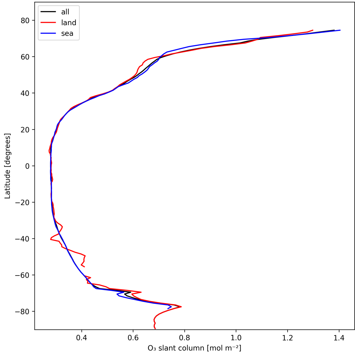
Figure 19: Zonal average of “O 3 slant column” for 2025-02-10 to 2025-02-11.
