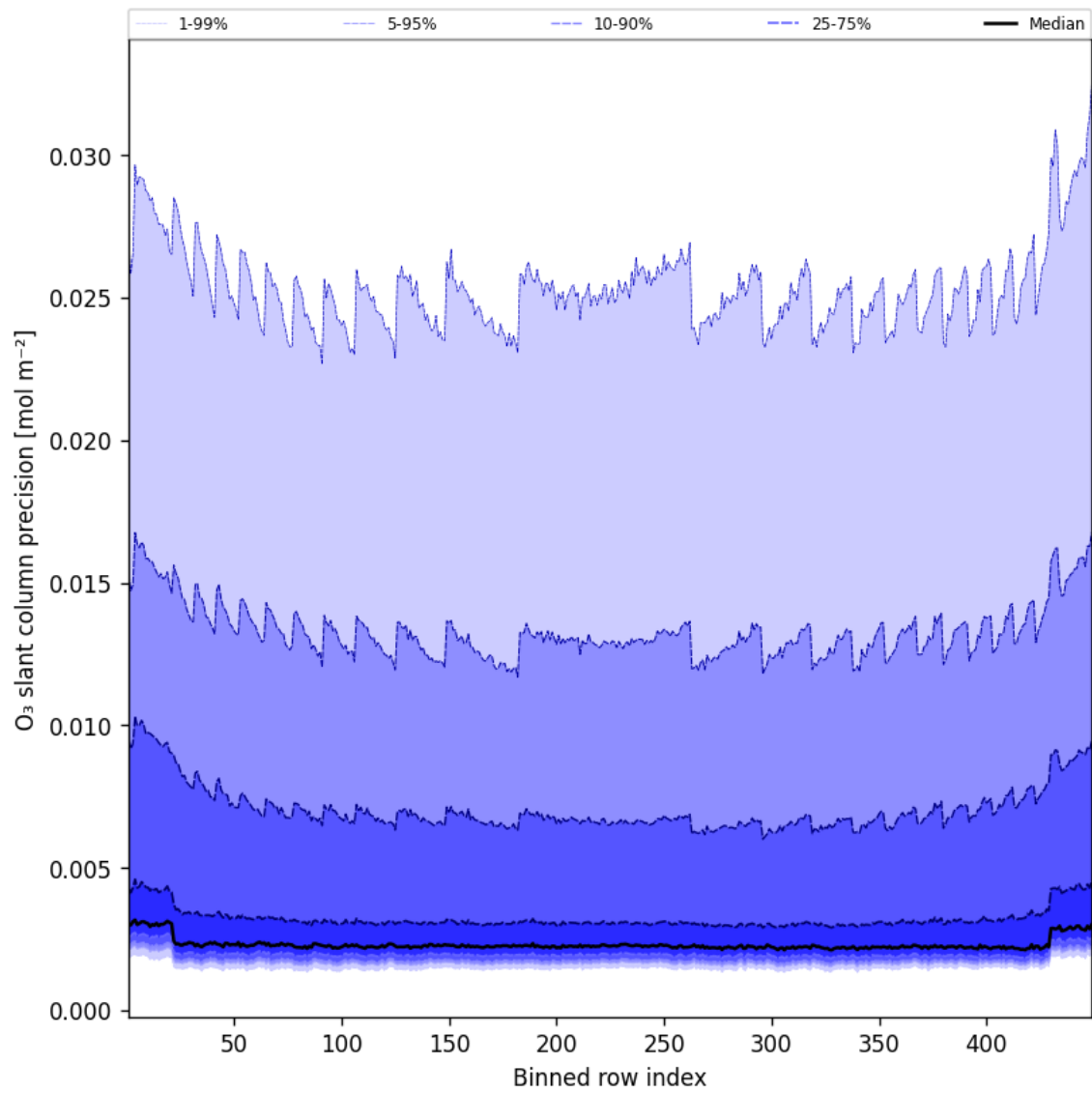
Figure 44: Along track statistics of “O 3 slant column precision” for 2025-02-10 to 2025-02-11
