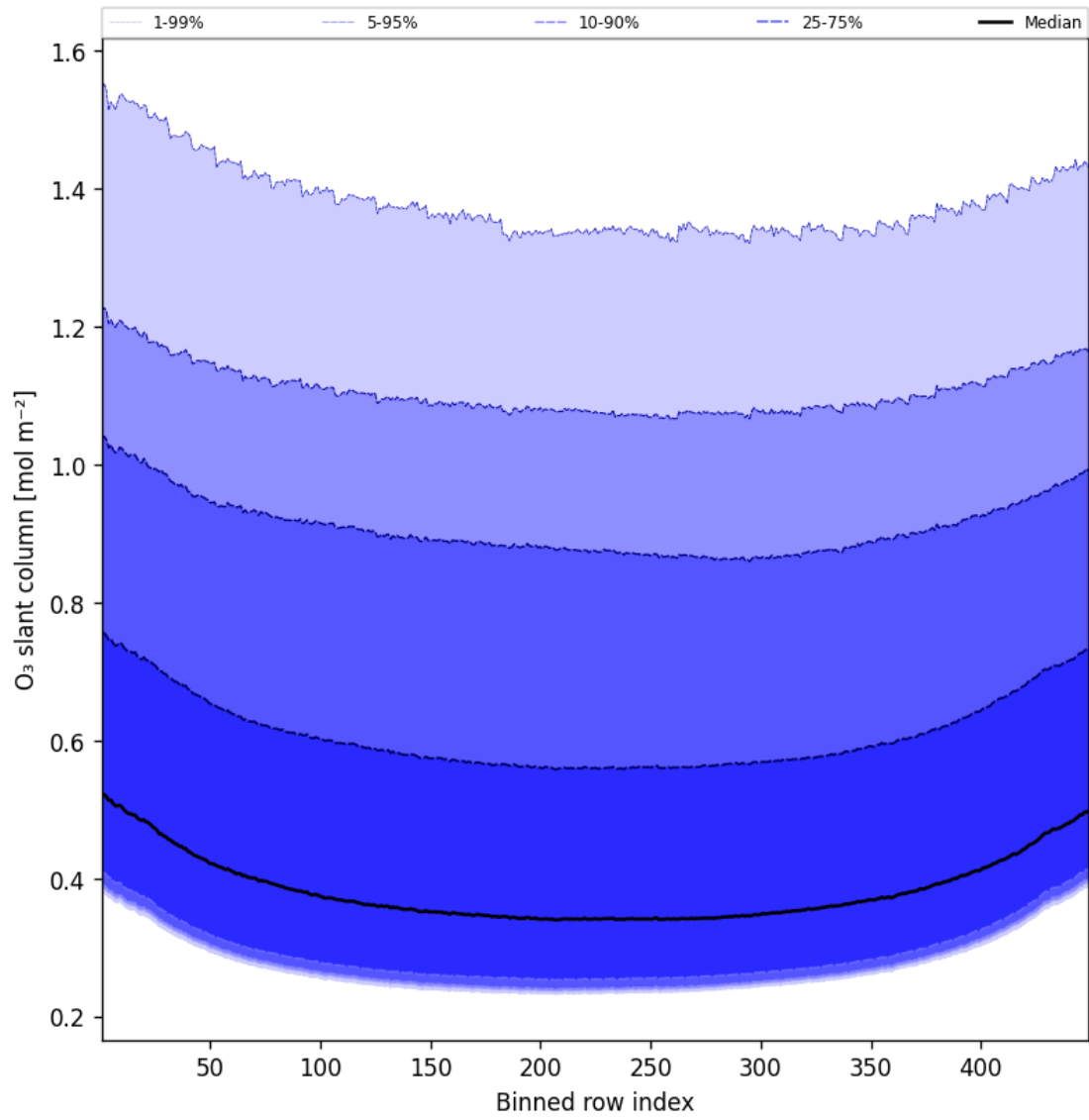
Figure 43: Along track statistics of “O 3 slant column” for 2025-02-10 to 2025-02-11
