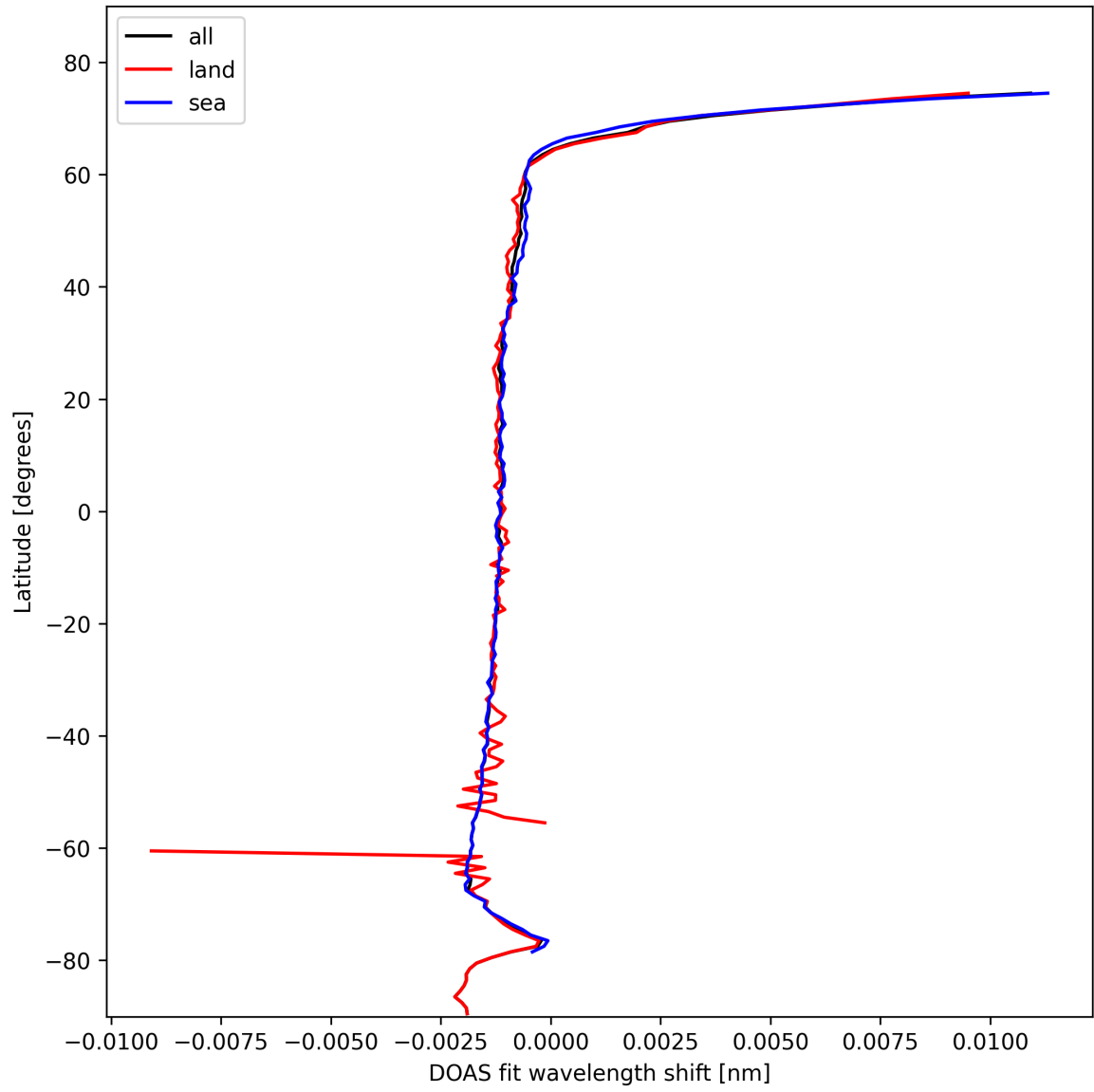
Figure 23: Zonal average of “DOAS fit wavelength shift” for 2025-02-10 to 2025-02-11.
