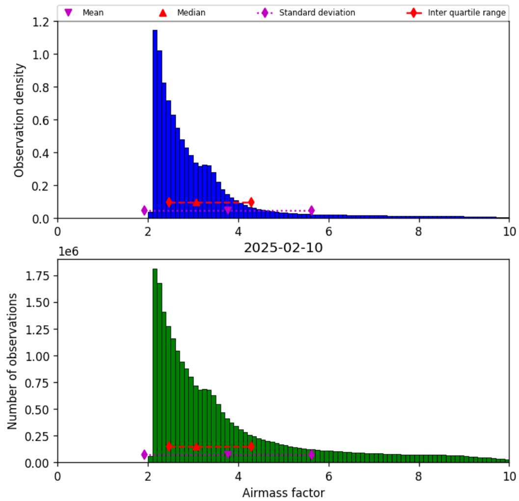
Figure 37: Histogram of “Airmass factor” for 2025-02-10 to 2025-02-11
