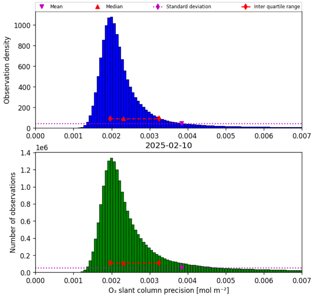
Figure 32: Histogram of “O 3 slant column precision” for 2025-02-10 to 2025-02-11
