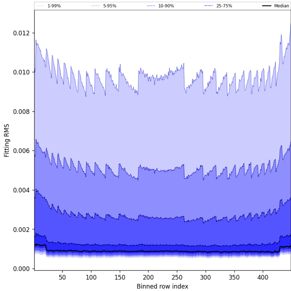
Figure 46: Along track statistics of “Fitting RMS” for 2025-02-10 to 2025-02-11
