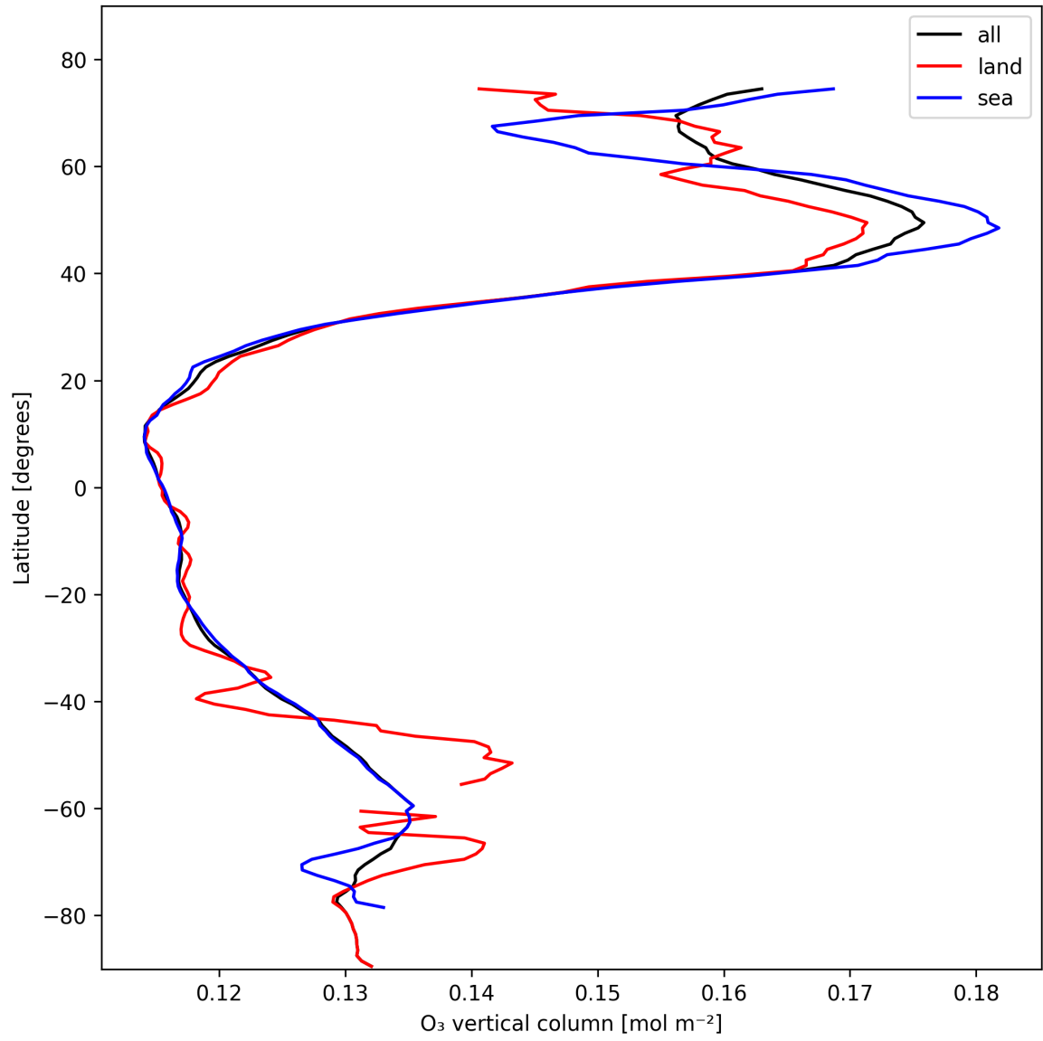
Figure 17: Zonal average of “O 3 vertical column” for 2025-02-10 to 2025-02-11.
