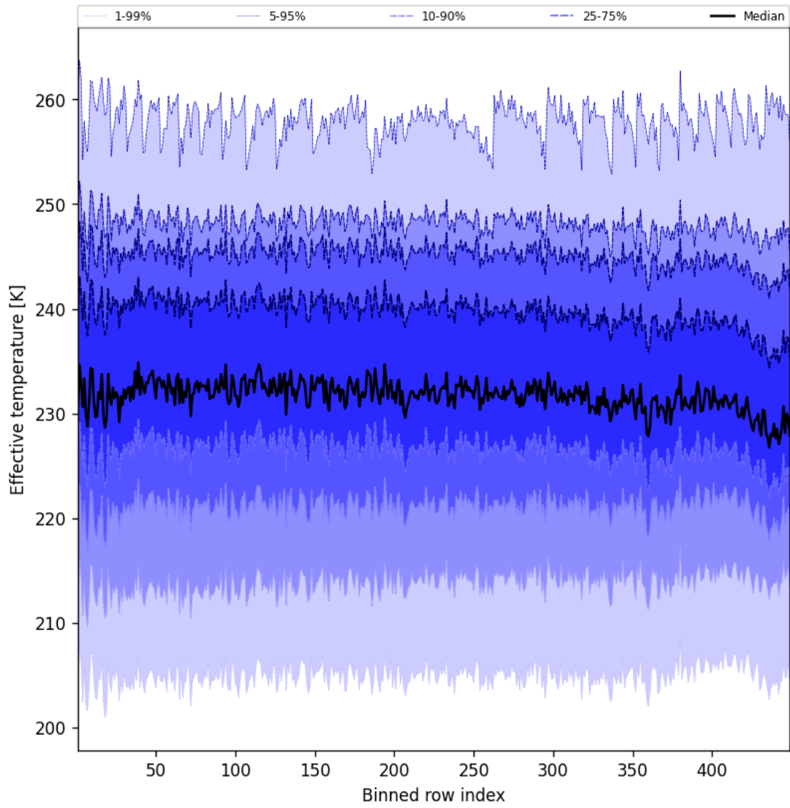
Figure 50: Along track statistics of “Effective temperature” for 2025-02-10 to 2025-02-11
