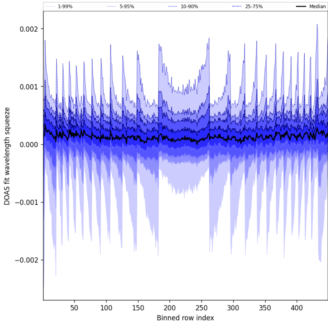
Figure 48: Along track statistics of “DOAS fit wavelength squeeze” for 2025-02-10 to 2025-02-11
