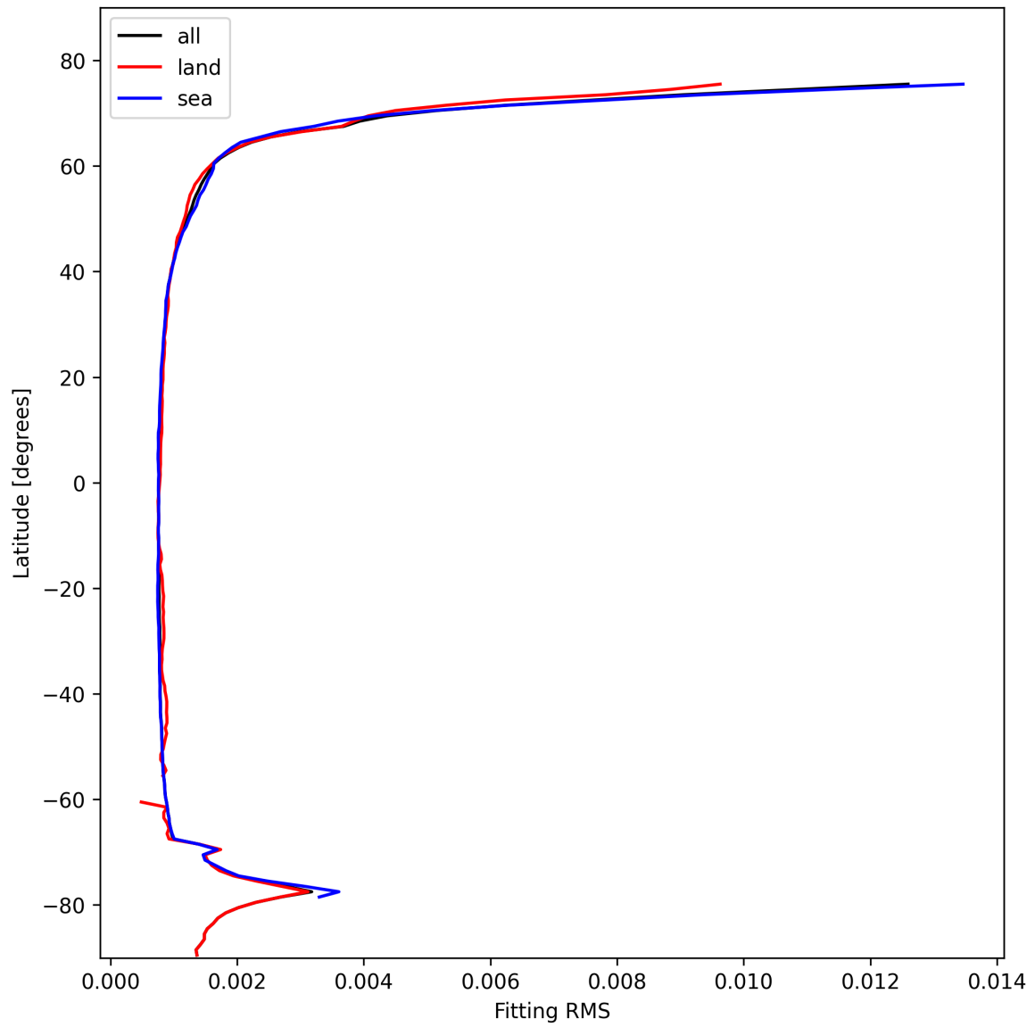
Figure 22: Zonal average of “Fitting RMS” for 2025-02-11 to 2025-02-11.
