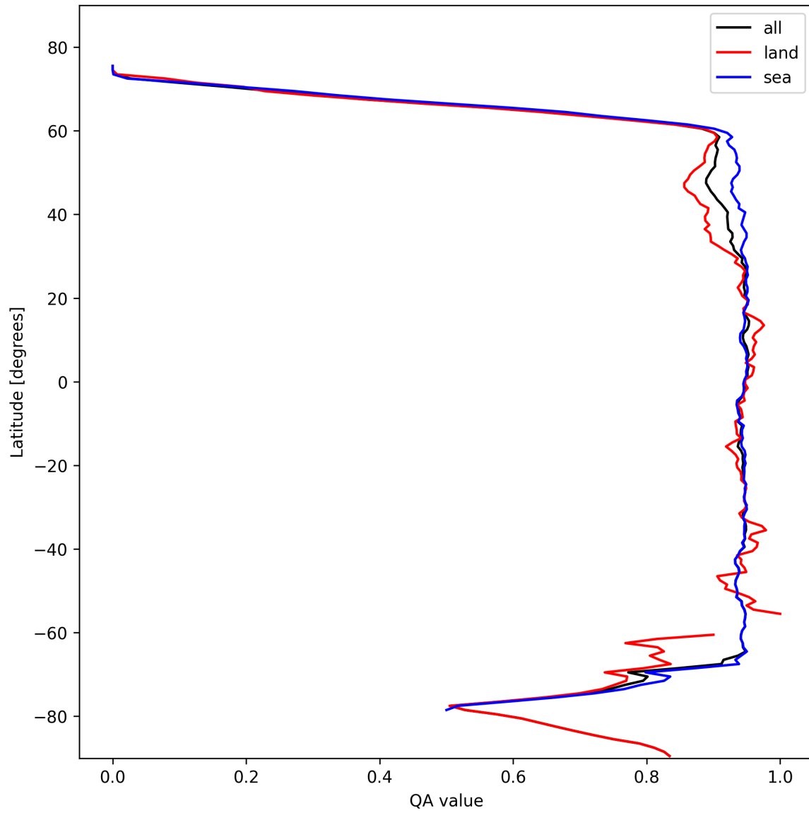
Figure 16: Zonal average of “QA value” for 2025-02-11 to 2025-02-11.
