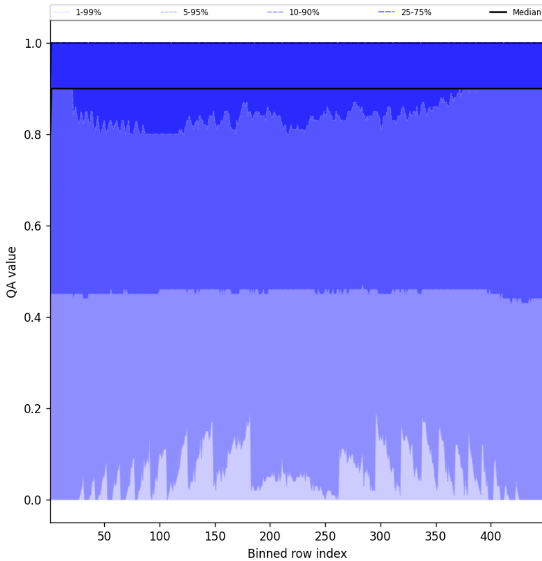
Figure 40: Along track statistics of “QA value” for 2025-02-11 to 2025-02-11
