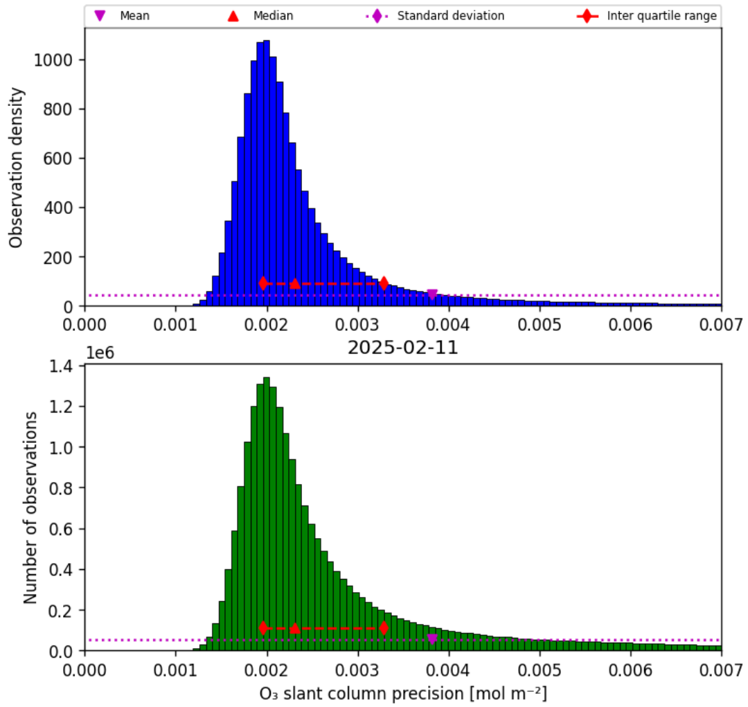
Figure 32: Histogram of “O 3 slant column precision” for 2025-02-11 to 2025-02-11
