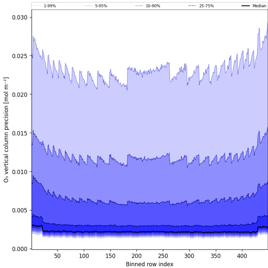
Figure 42: Along track statistics of “O 3 vertical column precision” for 2025-02-11 to 2025-02-11
