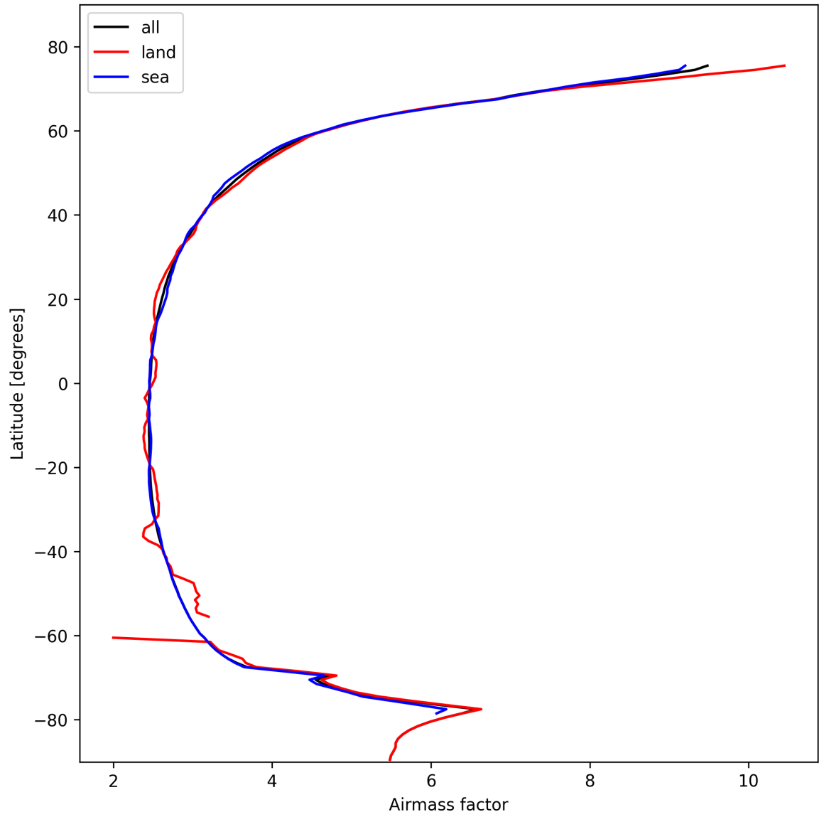
Figure 25: Zonal average of “Airmass factor” for 2025-02-11 to 2025-02-11.
