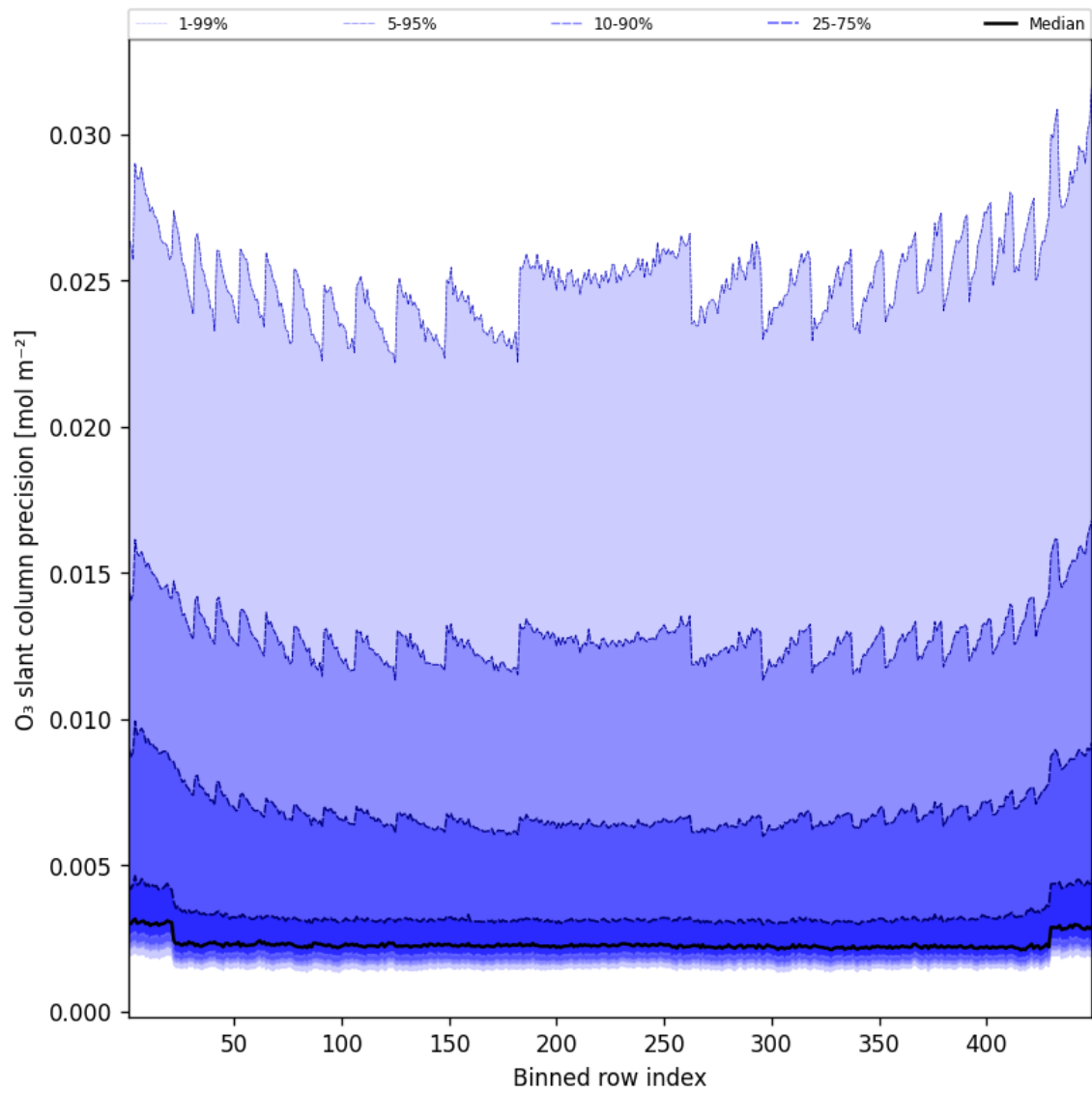
Figure 44: Along track statistics of “O 3 slant column precision” for 2025-02-11 to 2025-02-11
