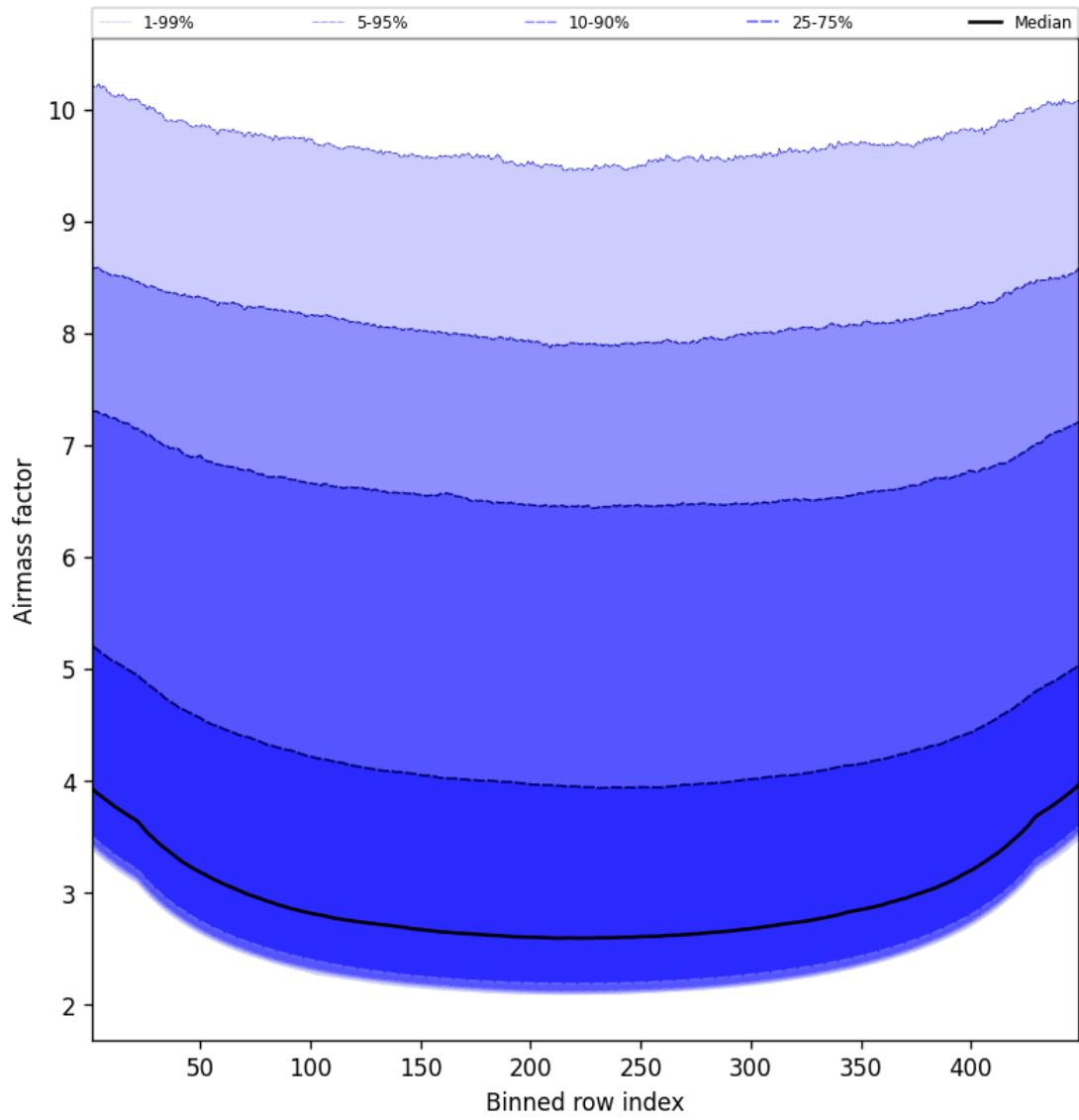
Figure 49: Along track statistics of “Airmass factor” for 2025-02-11 to 2025-02-11
