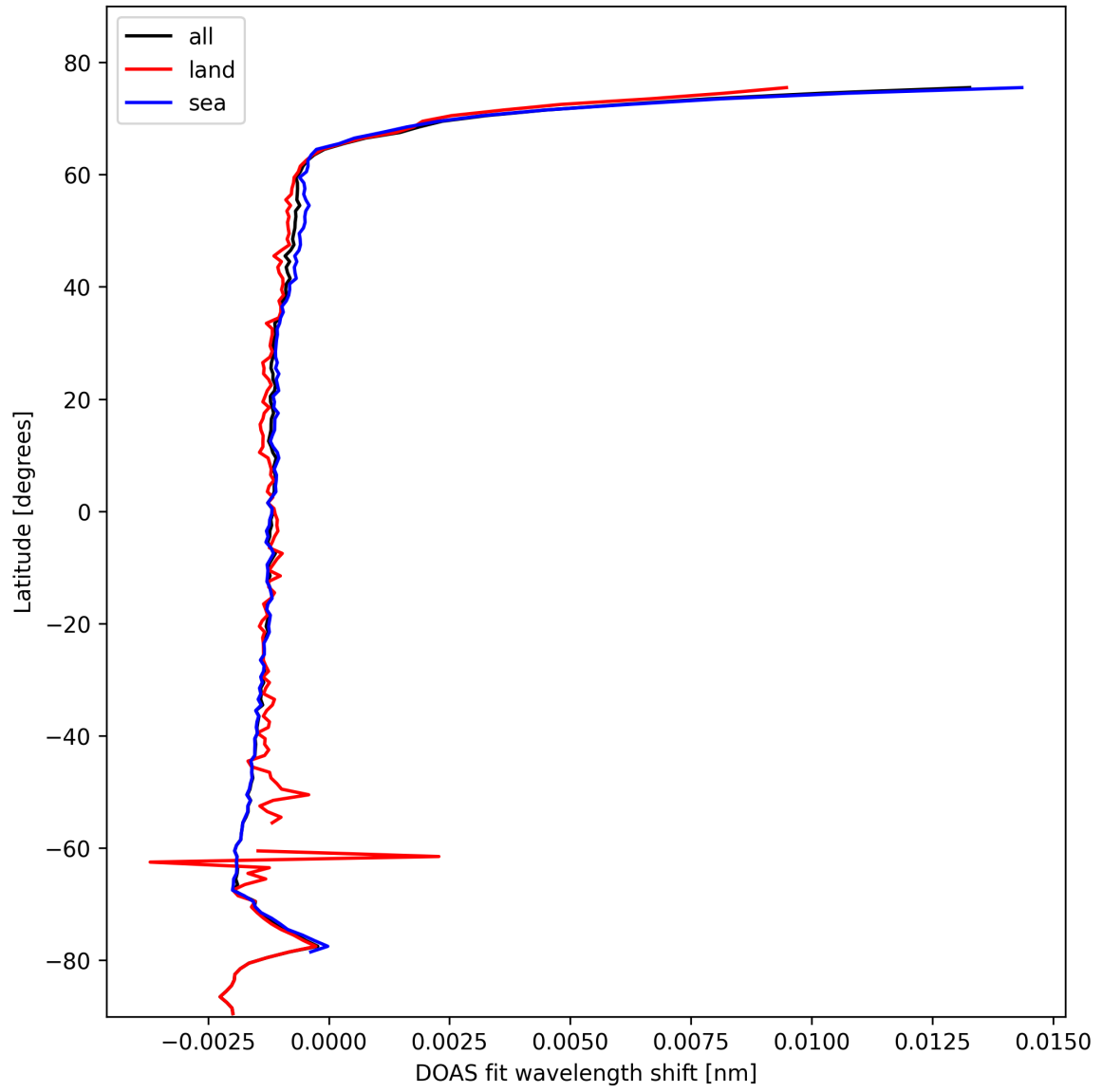
Figure 23: Zonal average of “DOAS fit wavelength shift” for 2025-02-11 to 2025-02-11.
