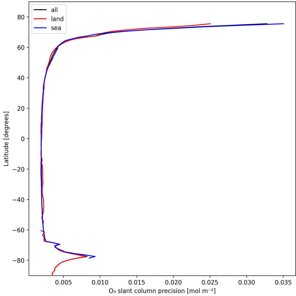
Figure 20: Zonal average of “O 3 slant column precision” for 2025-02-11 to 2025-02-11.
