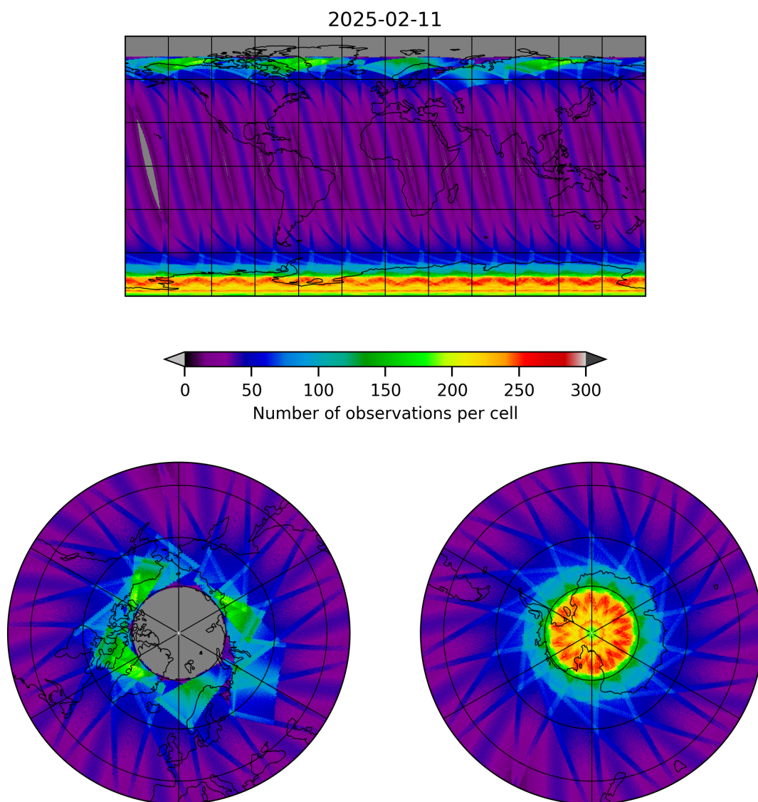
Figure 15: Map of the number of observations for 2025-02-11 to 2025-02-11
