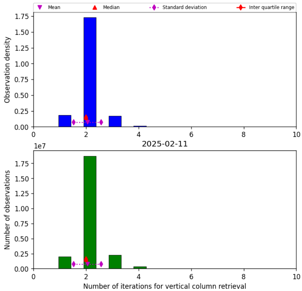
Figure 39: Histogram of “Number of iterations for vertical column retrieval” for 2025-02-11 to 2025-02-11
