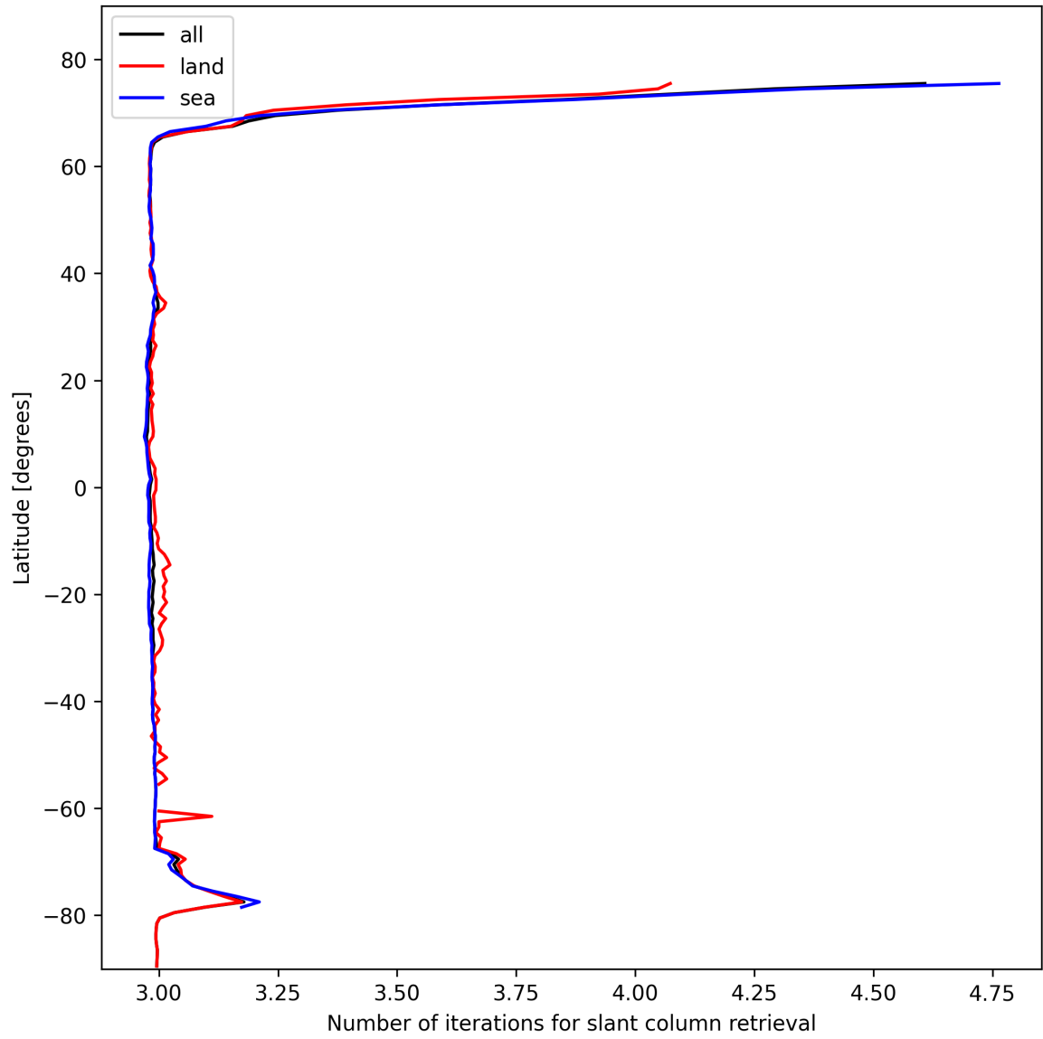
Figure 21: Zonal average of “Number of iterations for slant column retrieval” for 2025-02-11 to 2025-02-11.
