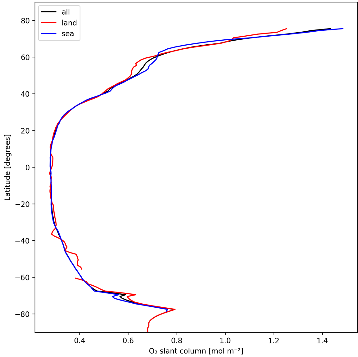
Figure 19: Zonal average of “O 3 slant column” for 2025-02-11 to 2025-02-11.
