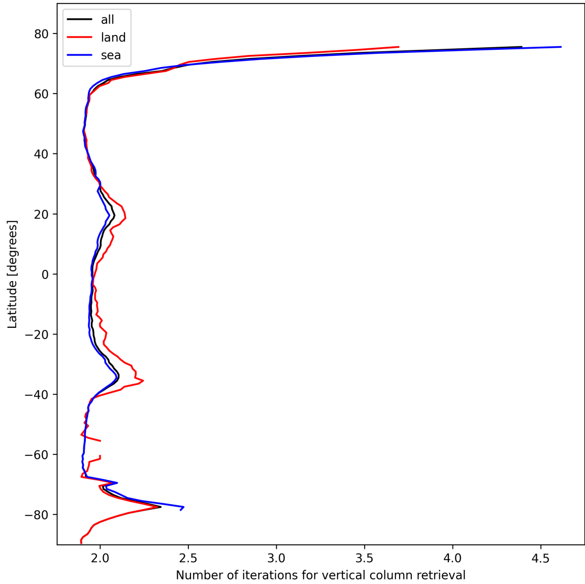
Figure 27: Zonal average of “Number of iterations for vertical column retrieval” for 2025-02-11 to 2025-02-11.
