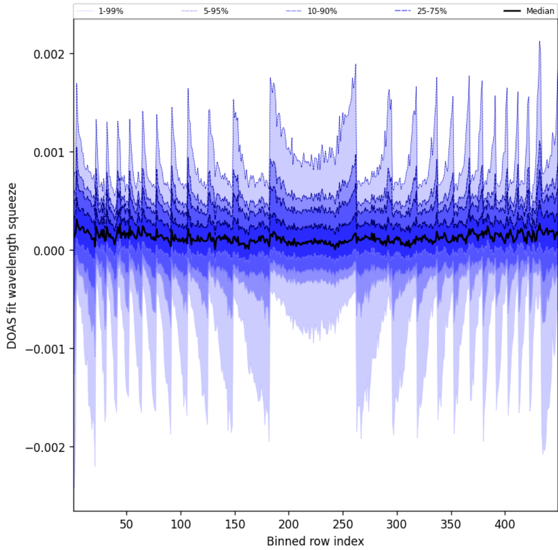
Figure 48: Along track statistics of “DOAS fit wavelength squeeze” for 2025-02-11 to 2025-02-11
