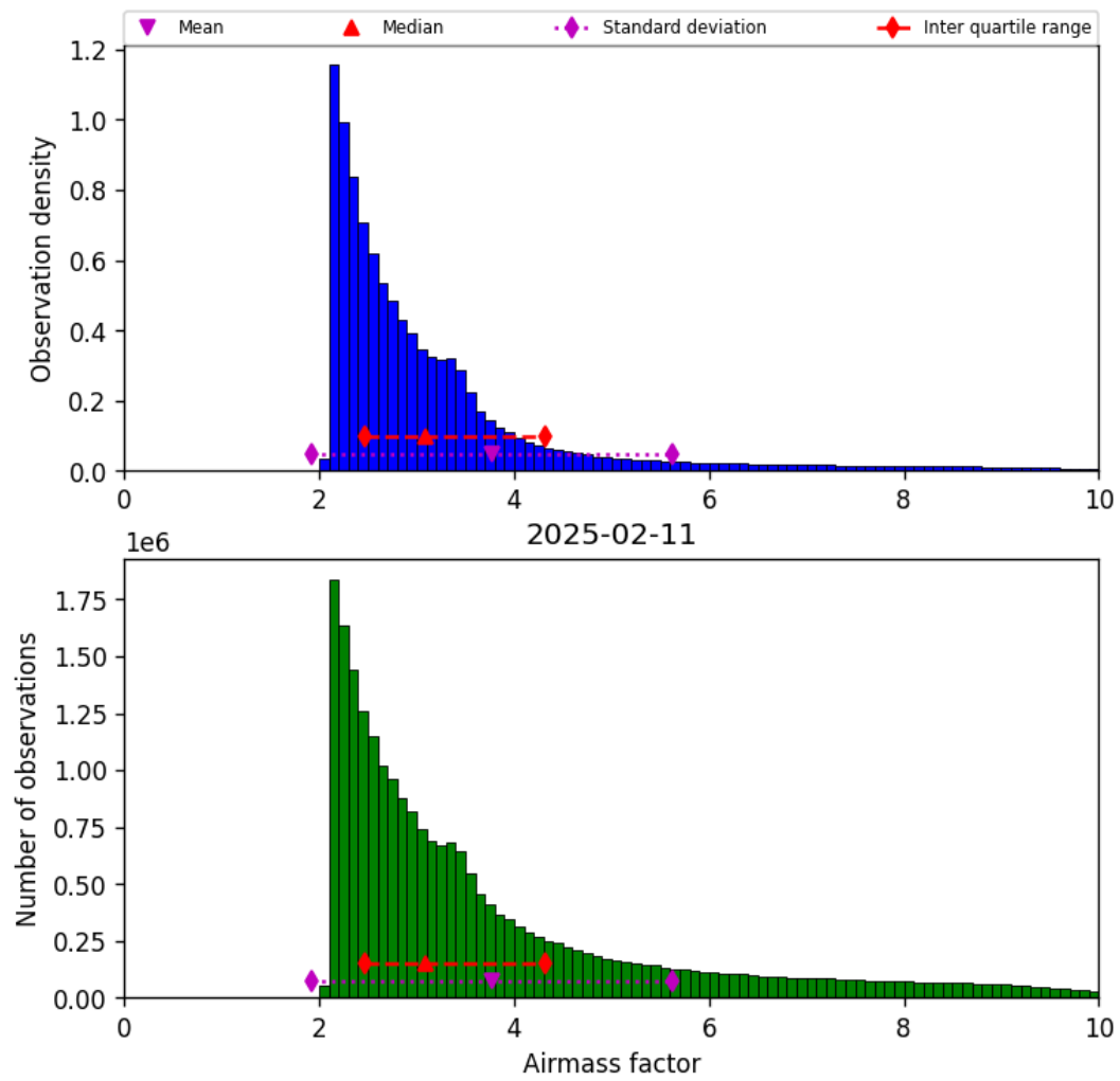
Figure 37: Histogram of “Airmass factor” for 2025-02-11 to 2025-02-11
