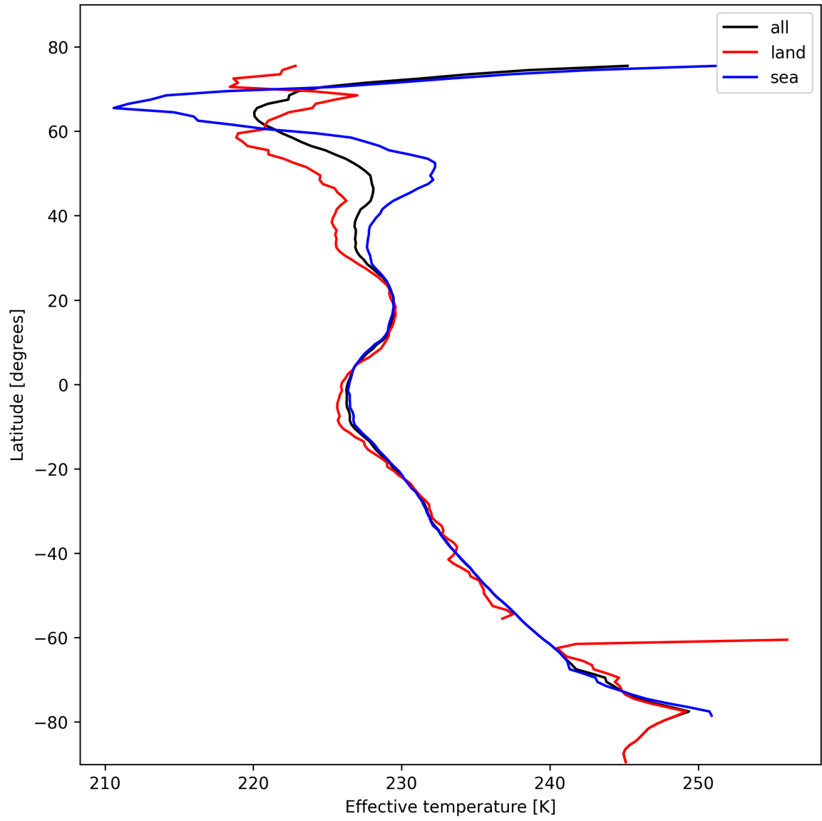
Figure 26: Zonal average of “Effective temperature” for 2025-02-11 to 2025-02-11.
