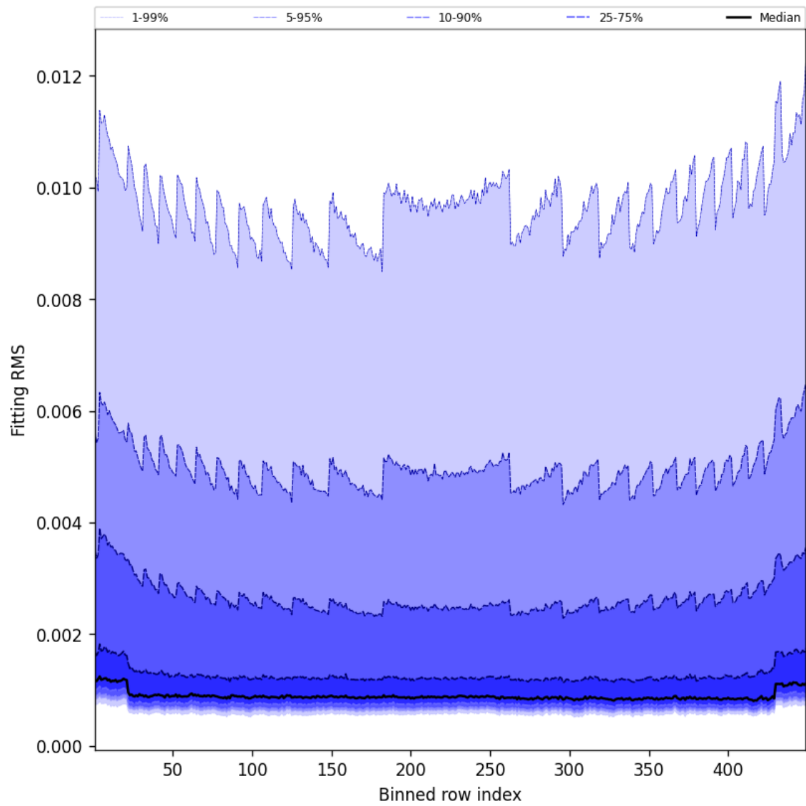
Figure 46: Along track statistics of “Fitting RMS” for 2025-02-11 to 2025-02-11
