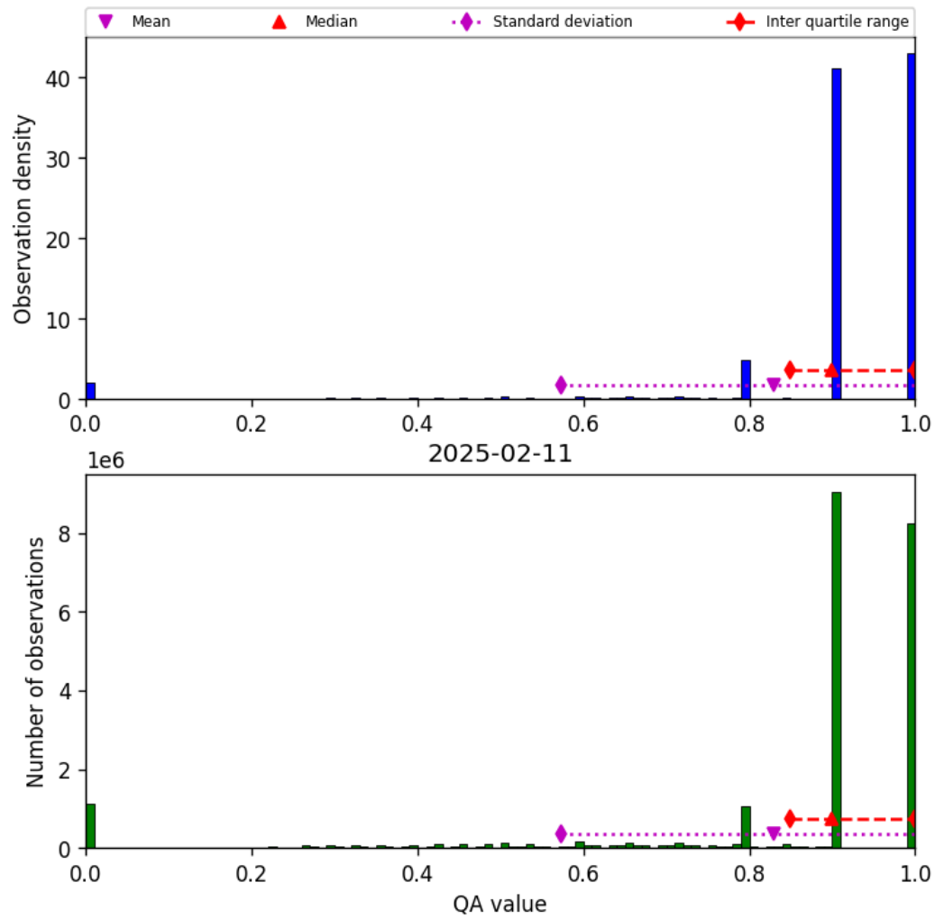
Figure 28: Histogram of “QA value” for 2025-02-11 to 2025-02-11
