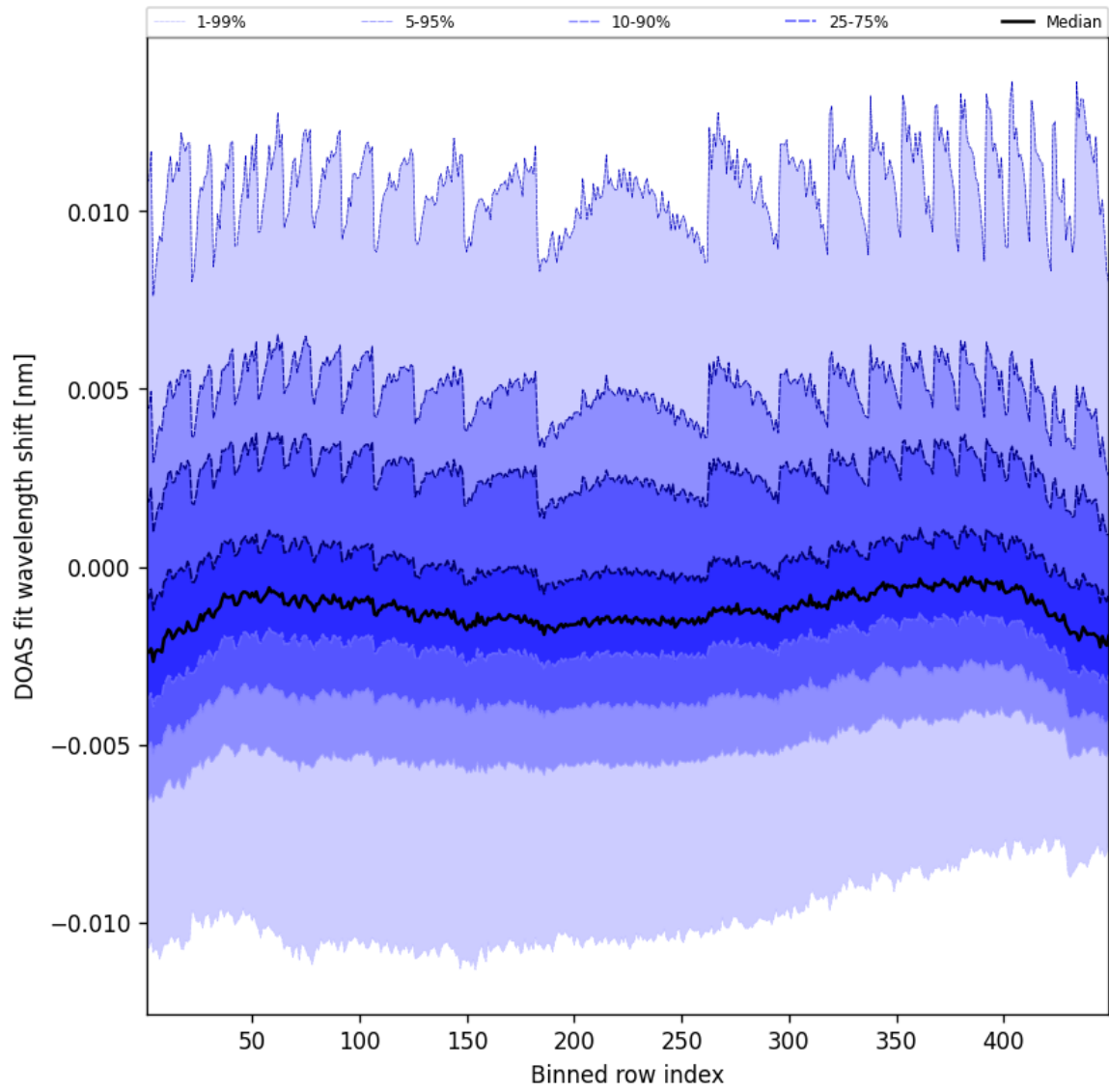
Figure 47: Along track statistics of “DOAS fit wavelength shift” for 2025-02-11 to 2025-02-11
