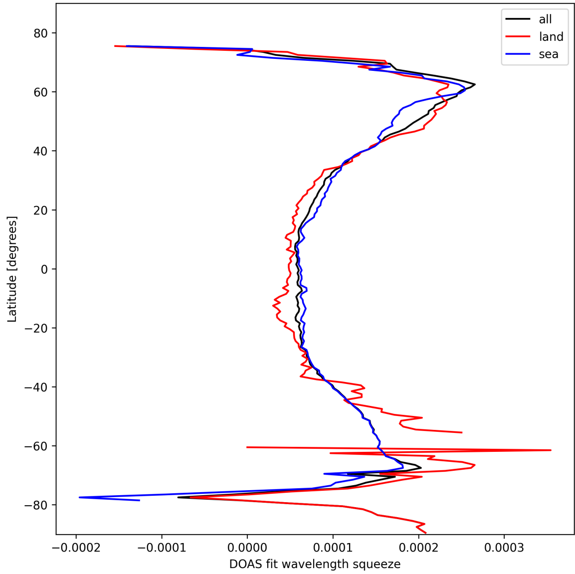
Figure 24: Zonal average of “DOAS fit wavelength squeeze” for 2025-02-11 to 2025-02-11.
