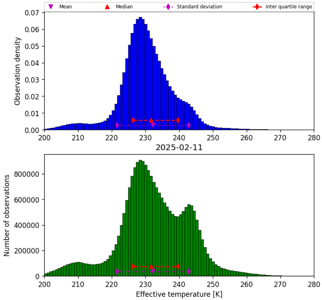
Figure 38: Histogram of “Effective temperature” for 2025-02-11 to 2025-02-11
