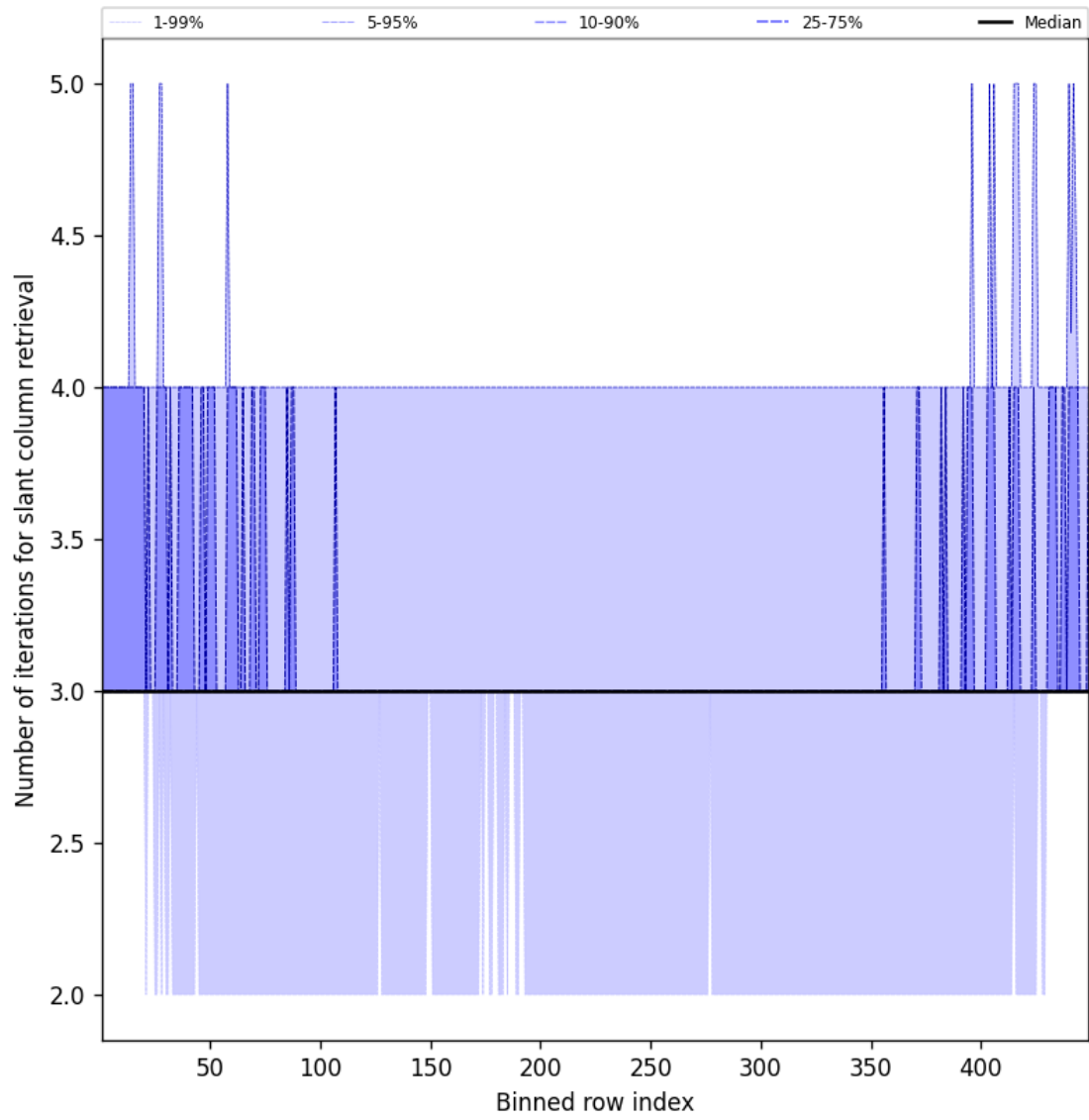
Figure 45: Along track statistics of “Number of iterations for slant column retrieval” for 2025-02-11 to 2025-02-11
