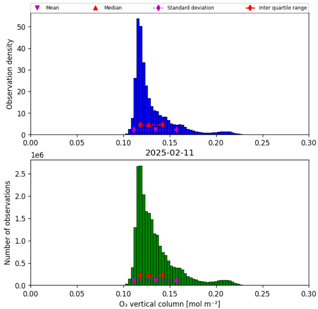
Figure 29: Histogram of “O 3 vertical column” for 2025-02-11 to 2025-02-11
