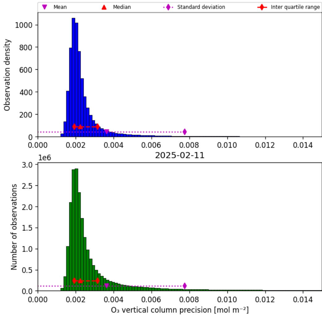
Figure 30: Histogram of “O 3 vertical column precision” for 2025-02-11 to 2025-02-11
