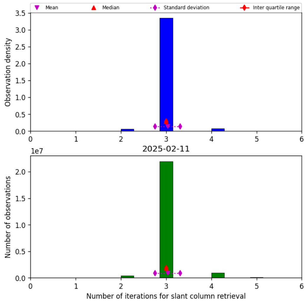
Figure 33: Histogram of “Number of iterations for slant column retrieval” for 2025-02-11 to 2025-02-11
