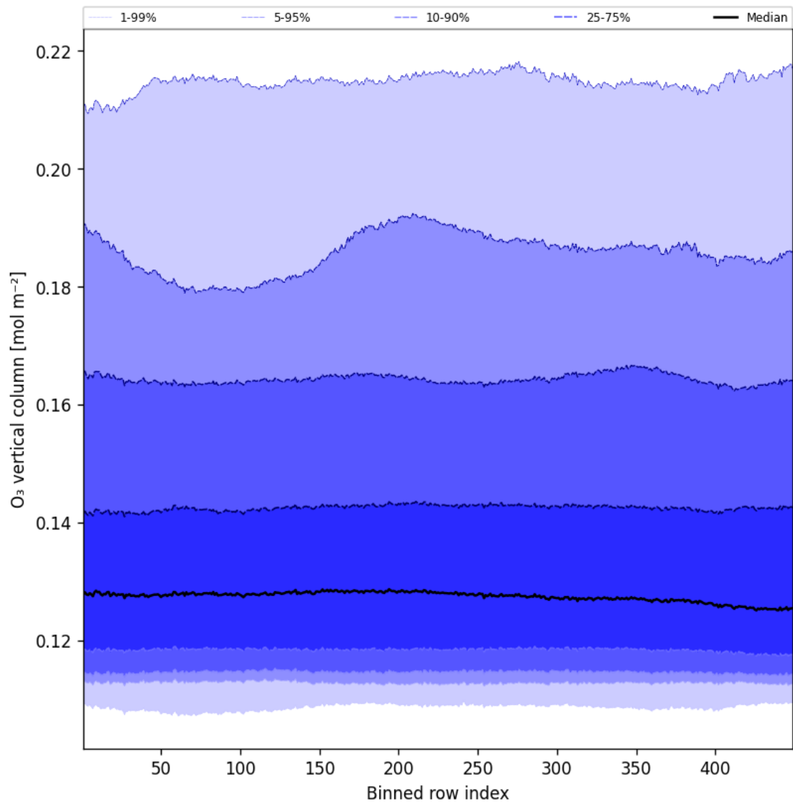
Figure 41: Along track statistics of “O 3 vertical column” for 2025-02-11 to 2025-02-11
