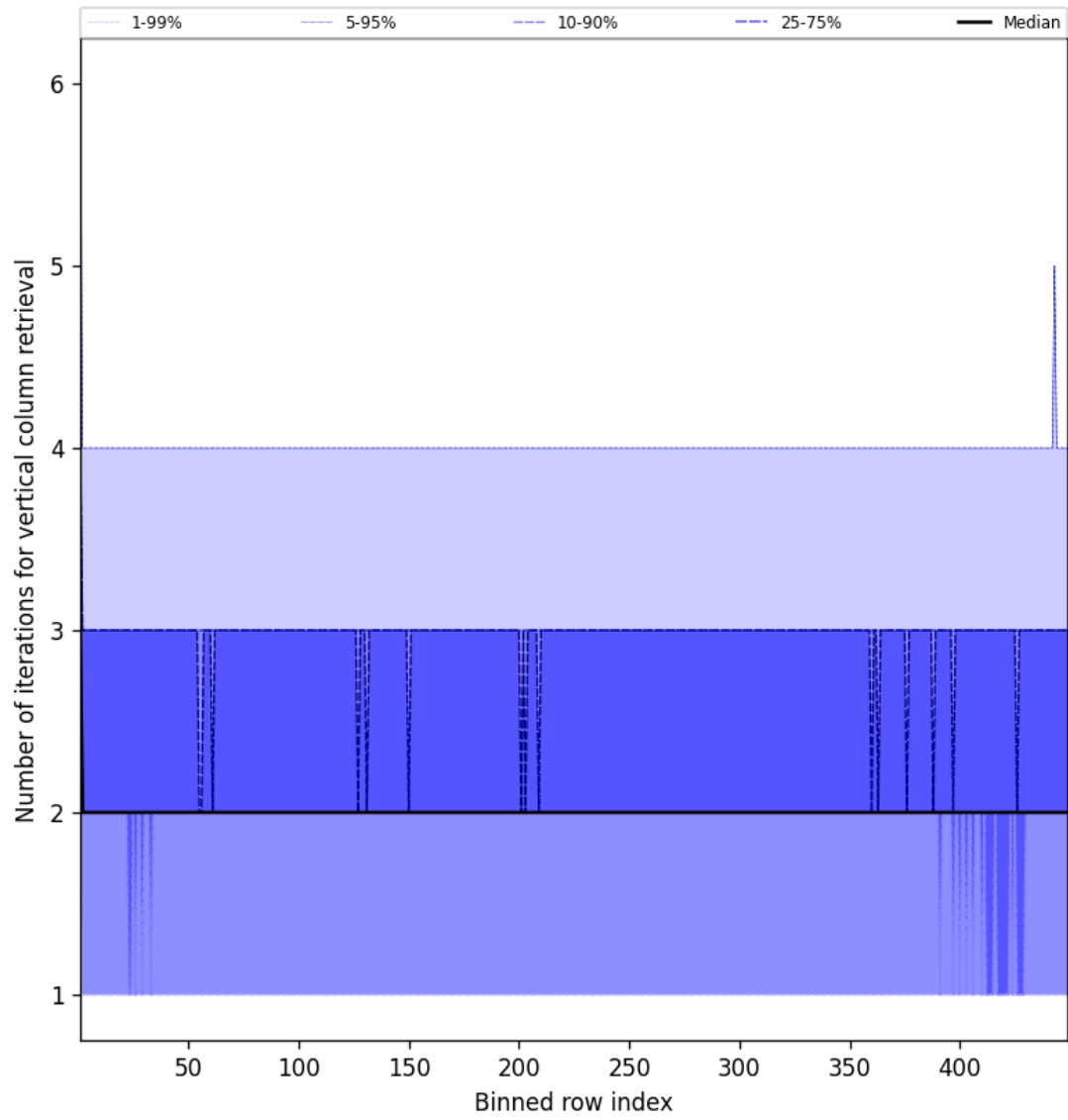
Figure 51: Along track statistics of “Number of iterations for vertical column retrieval” for 2025-02-11 to 2025-02-11
