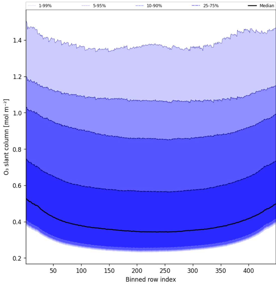
Figure 43: Along track statistics of “O 3 slant column” for 2025-02-11 to 2025-02-11
