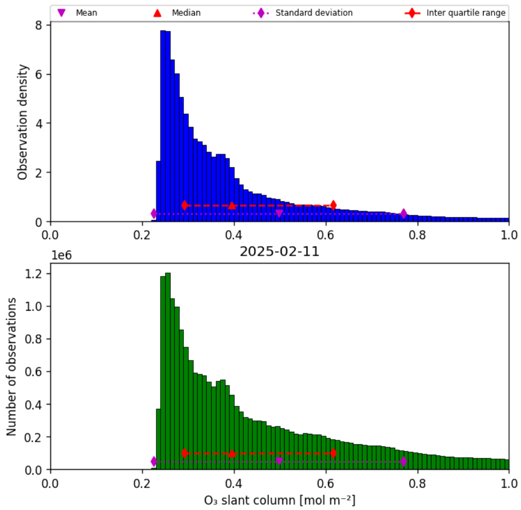
Figure 31: Histogram of “O 3 slant column” for 2025-02-11 to 2025-02-11
