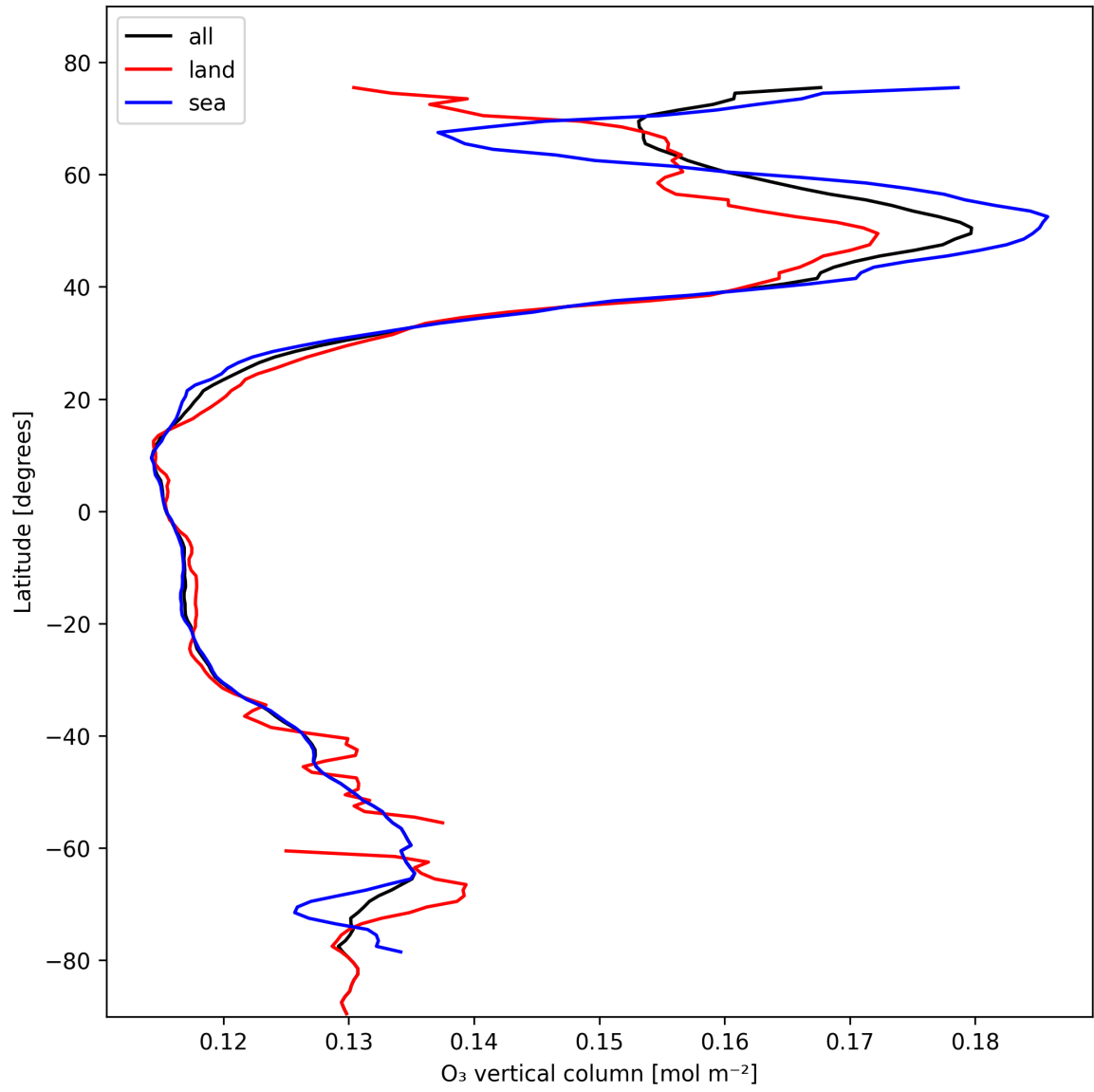
Figure 17: Zonal average of “O 3 vertical column” for 2025-02-11 to 2025-02-11.
