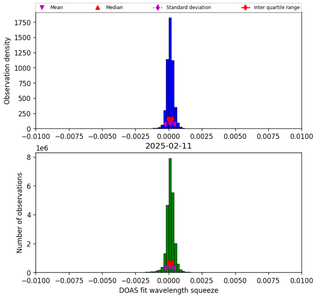
Figure 36: Histogram of “DOAS fit wavelength squeeze” for 2025-02-11 to 2025-02-11
