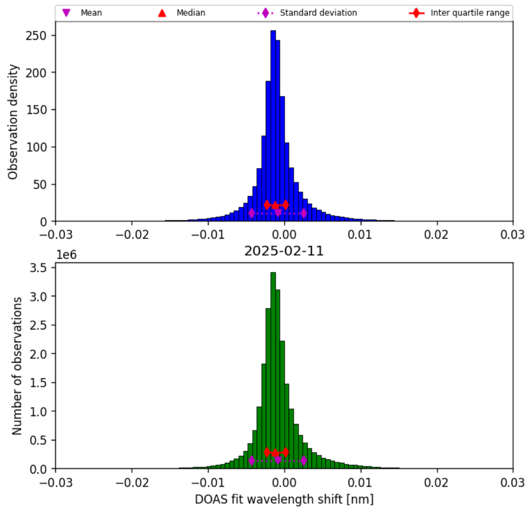
Figure 35: Histogram of “DOAS fit wavelength shift” for 2025-02-11 to 2025-02-11
