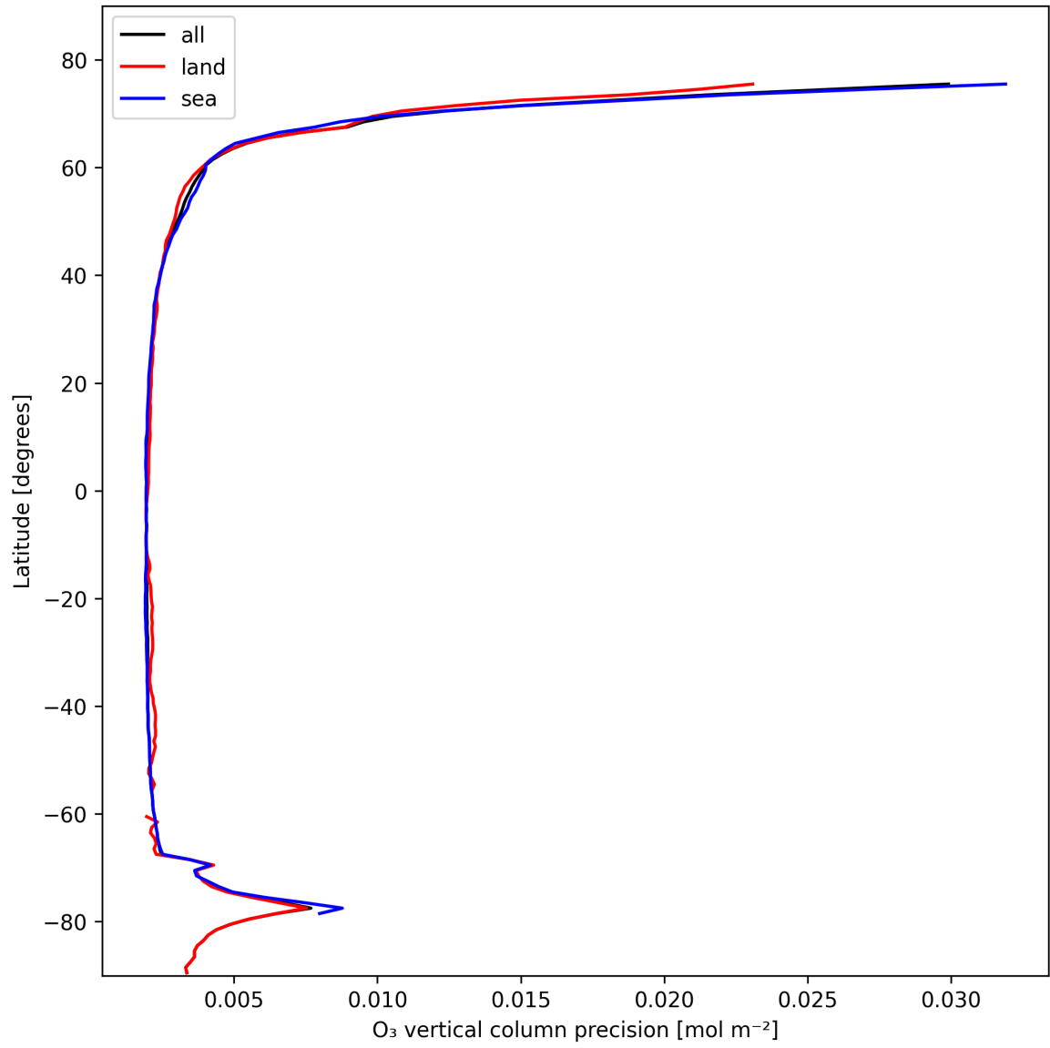
Figure 18: Zonal average of “O 3 vertical column precision” for 2025-02-11 to 2025-02-11.
