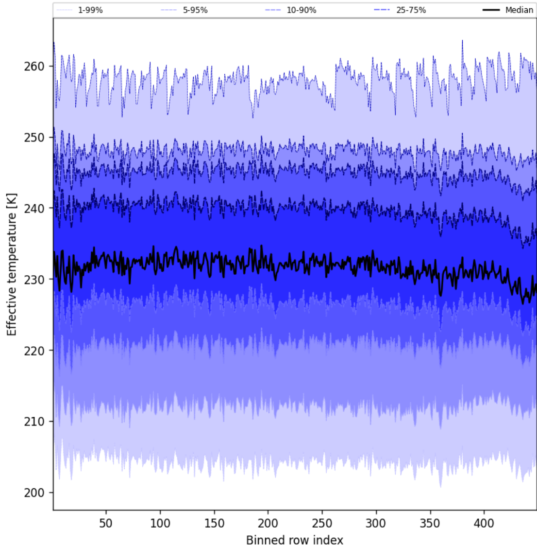
Figure 50: Along track statistics of “Effective temperature” for 2025-02-11 to 2025-02-11
