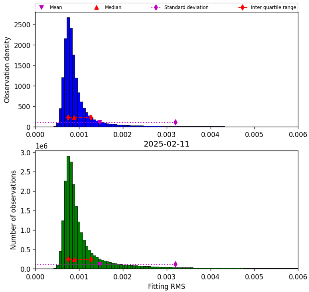
Figure 34: Histogram of “Fitting RMS” for 2025-02-11 to 2025-02-11
