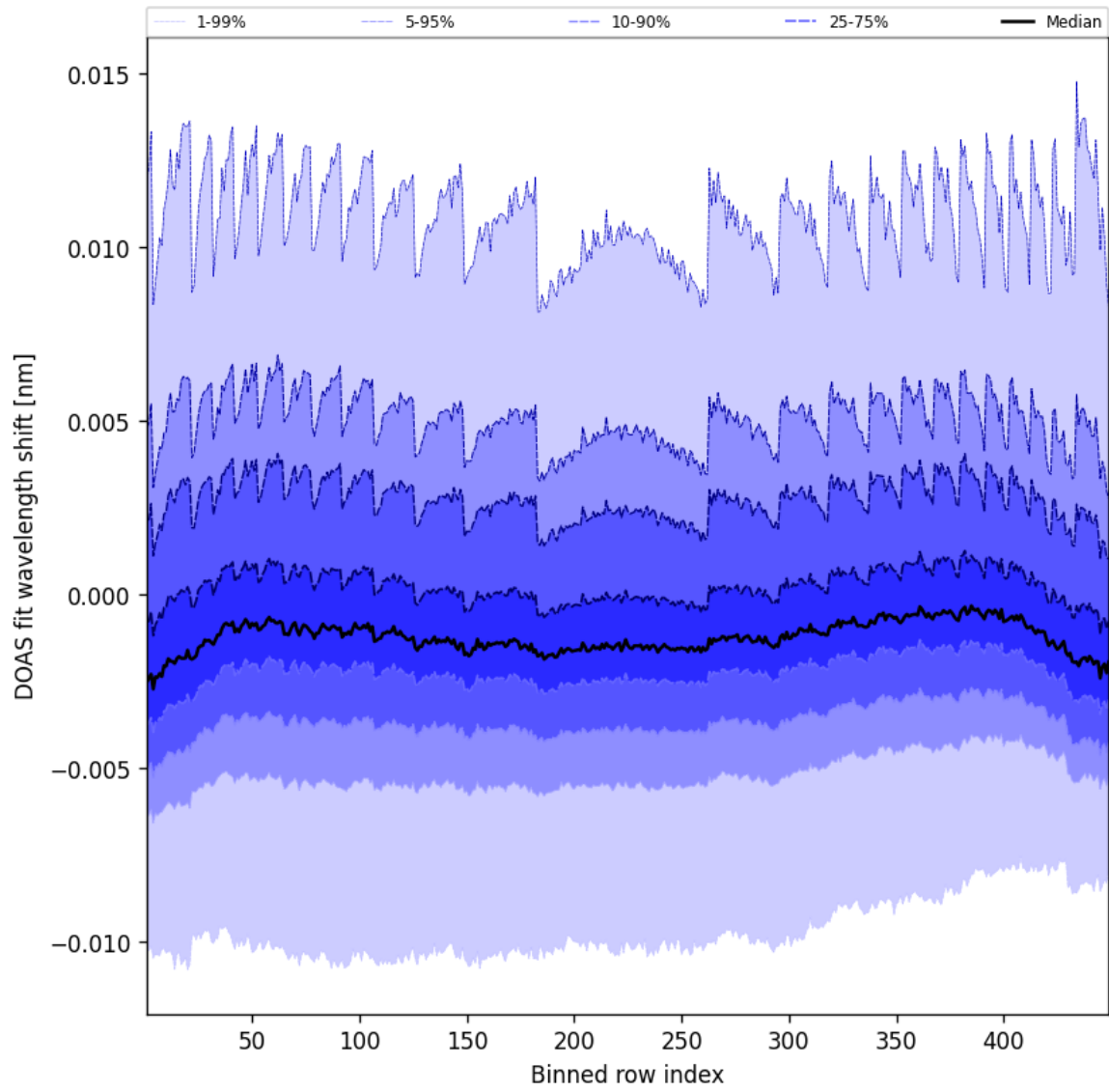
Figure 47: Along track statistics of “DOAS fit wavelength shift” for 2025-02-13 to 2025-02-14
