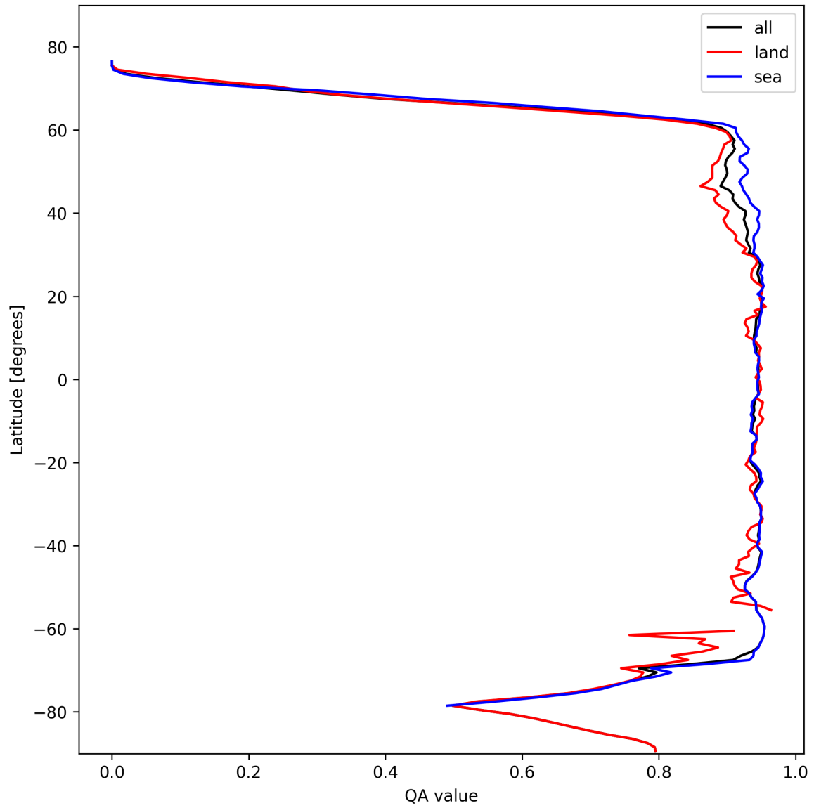
Figure 16: Zonal average of “QA value” for 2025-02-13 to 2025-02-14.
