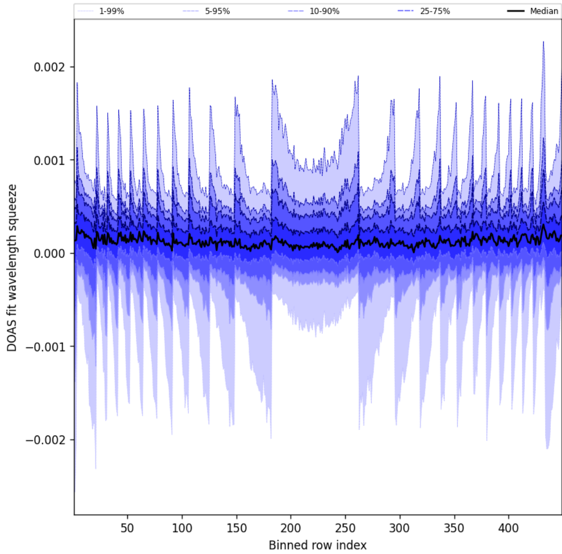
Figure 48: Along track statistics of “DOAS fit wavelength squeeze” for 2025-02-13 to 2025-02-14
