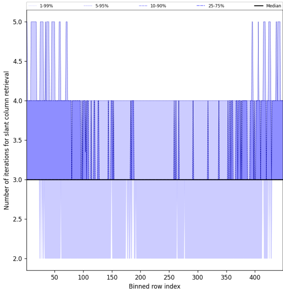
Figure 45: Along track statistics of “Number of iterations for slant column retrieval” for 2025-02-13 to 2025-02-14
