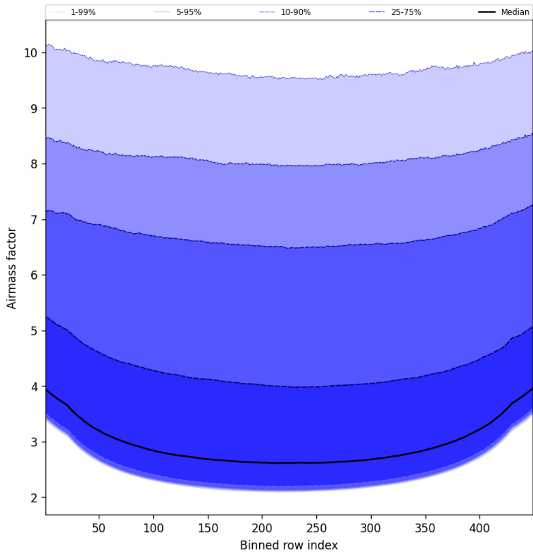
Figure 49: Along track statistics of “Airmass factor” for 2025-02-13 to 2025-02-14
