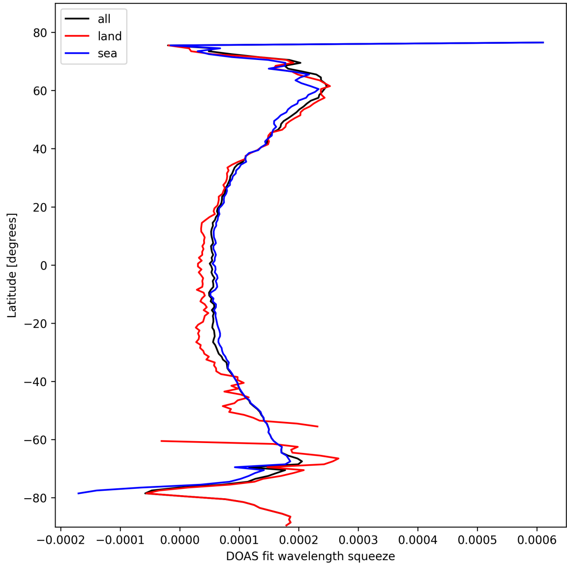
Figure 24: Zonal average of “DOAS fit wavelength squeeze” for 2025-02-13 to 2025-02-14.
