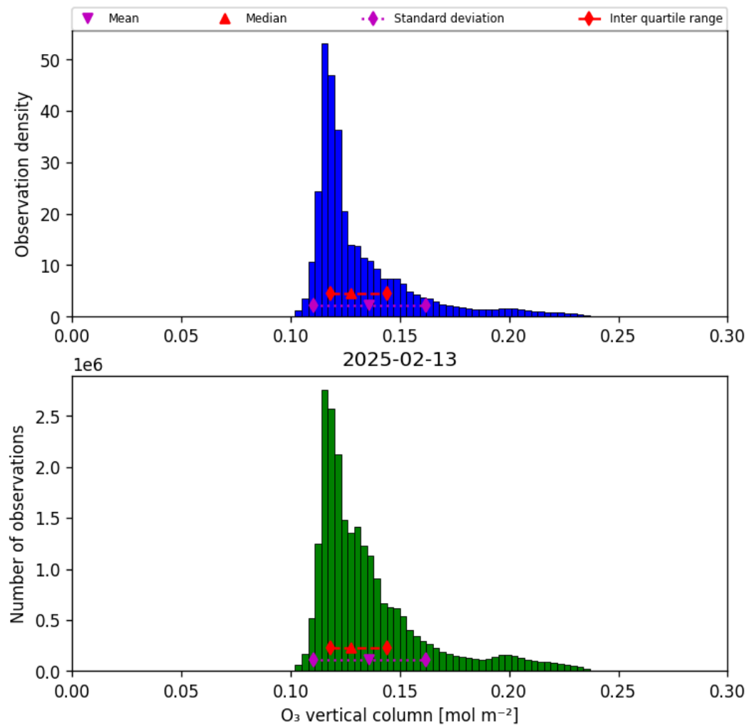
Figure 29: Histogram of “O 3 vertical column” for 2025-02-13 to 2025-02-14
