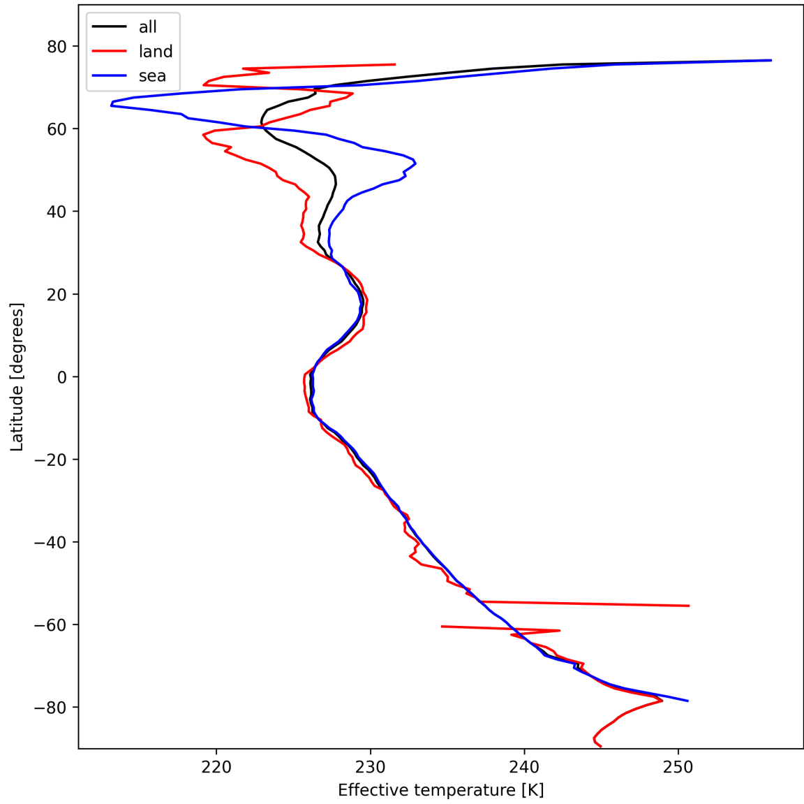
Figure 26: Zonal average of “Effective temperature” for 2025-02-13 to 2025-02-14.
