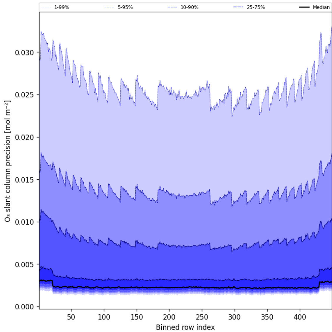
Figure 44: Along track statistics of “O 3 slant column precision” for 2025-02-13 to 2025-02-14
