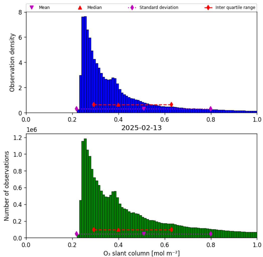
Figure 31: Histogram of “O 3 slant column” for 2025-02-13 to 2025-02-14
