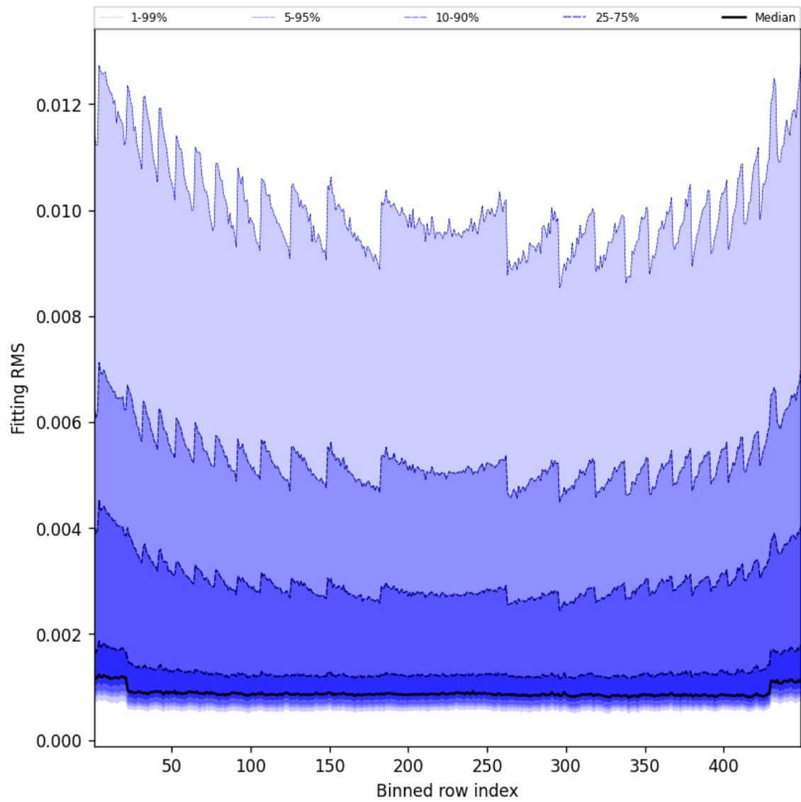
Figure 46: Along track statistics of “Fitting RMS” for 2025-02-13 to 2025-02-14
