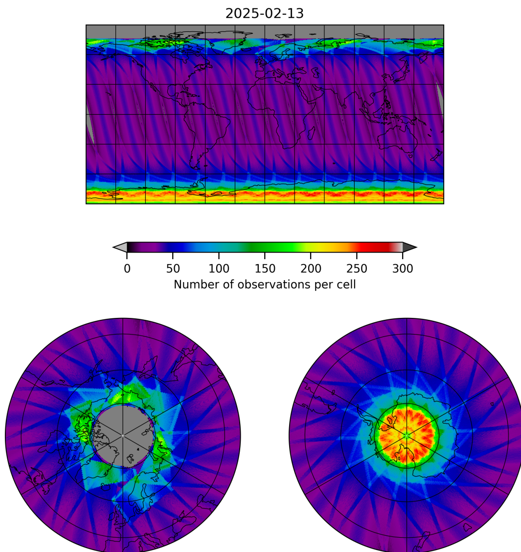
Figure 15: Map of the number of observations for 2025-02-13 to 2025-02-14
