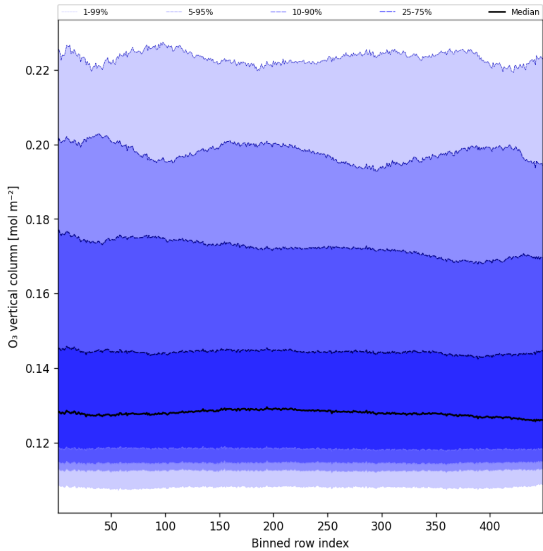
Figure 41: Along track statistics of “ \text{O}_3 vertical column” for 2025-02-13 to 2025-02-14
