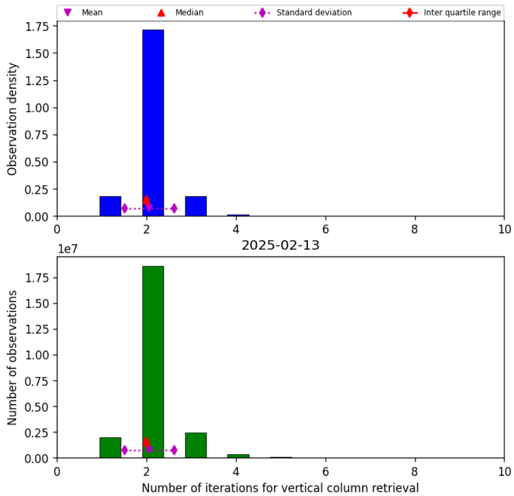
Figure 39: Histogram of “Number of iterations for vertical column retrieval” for 2025-02-13 to 2025-02-14
