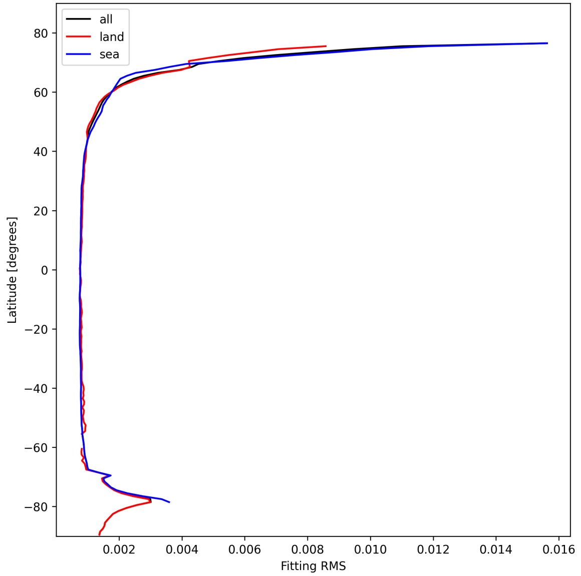
Figure 22: Zonal average of “Fitting RMS” for 2025-02-13 to 2025-02-14.
