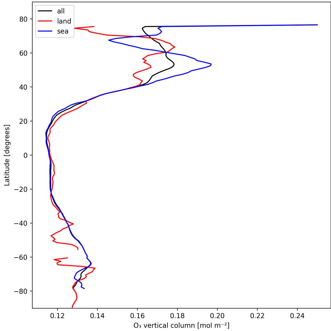
Figure 17: Zonal average of “O 3 vertical column” for 2025-02-13 to 2025-02-14.
