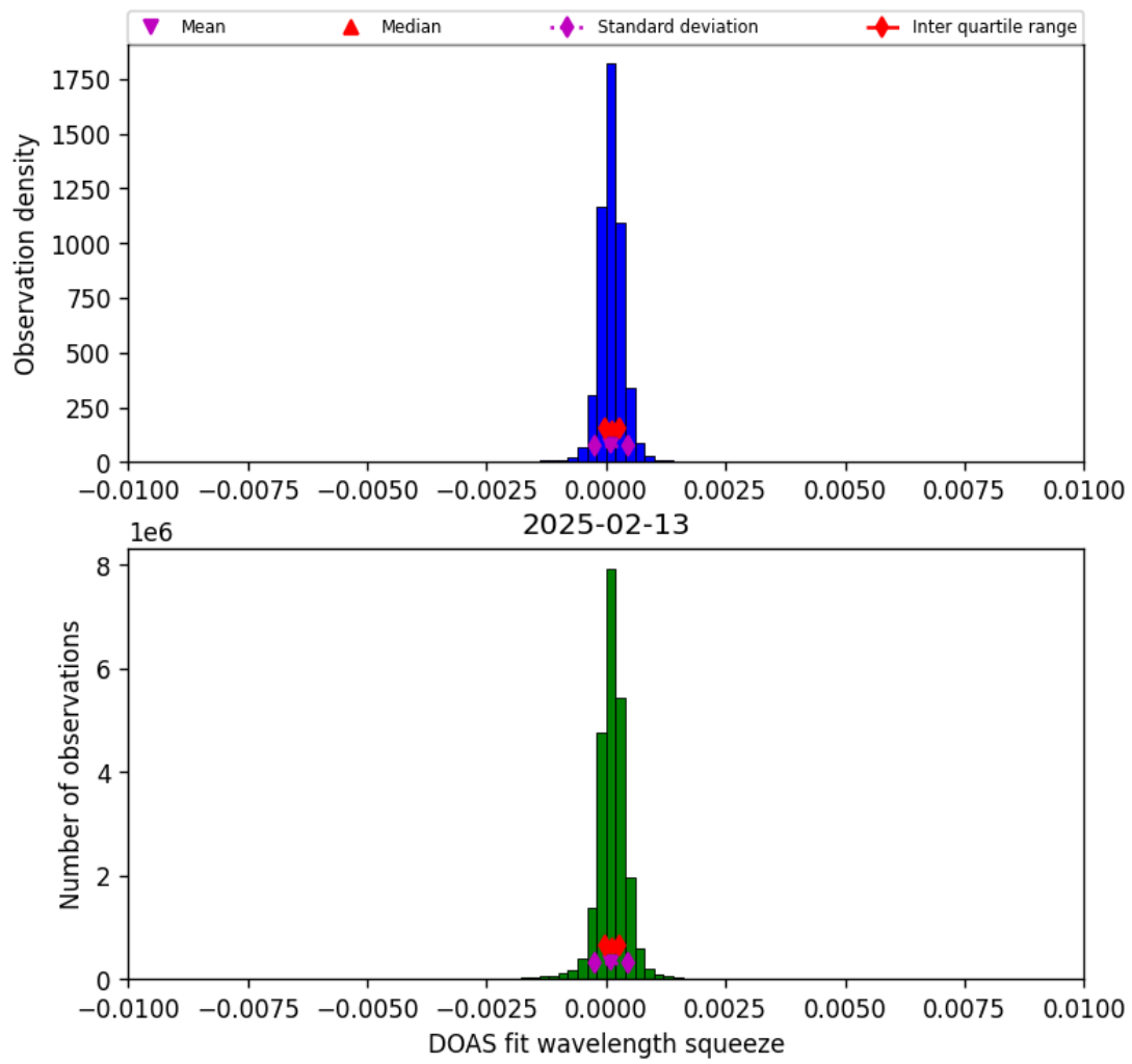
Figure 36: Histogram of “DOAS fit wavelength squeeze” for 2025-02-13 to 2025-02-14
