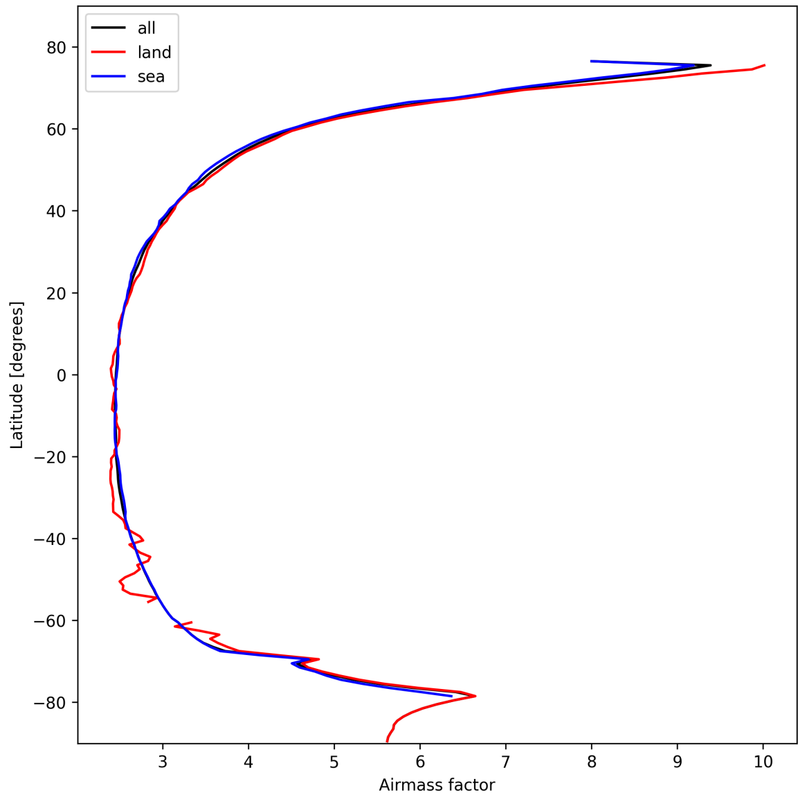
Figure 25: Zonal average of “Airmass factor” for 2025-02-13 to 2025-02-14.
