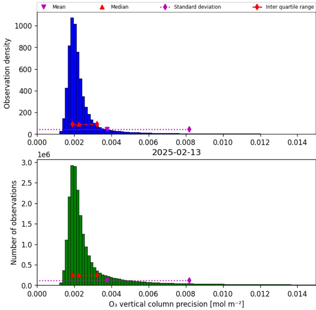
Figure 30: Histogram of “O 3 vertical column precision” for 2025-02-13 to 2025-02-14
