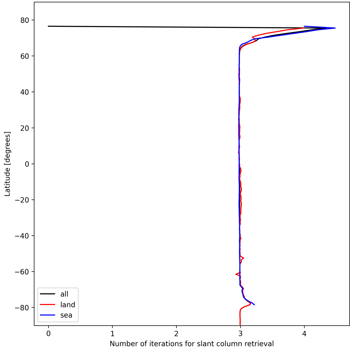
Figure 21: Zonal average of “Number of iterations for slant column retrieval” for 2025-02-13 to 2025-02-14.
