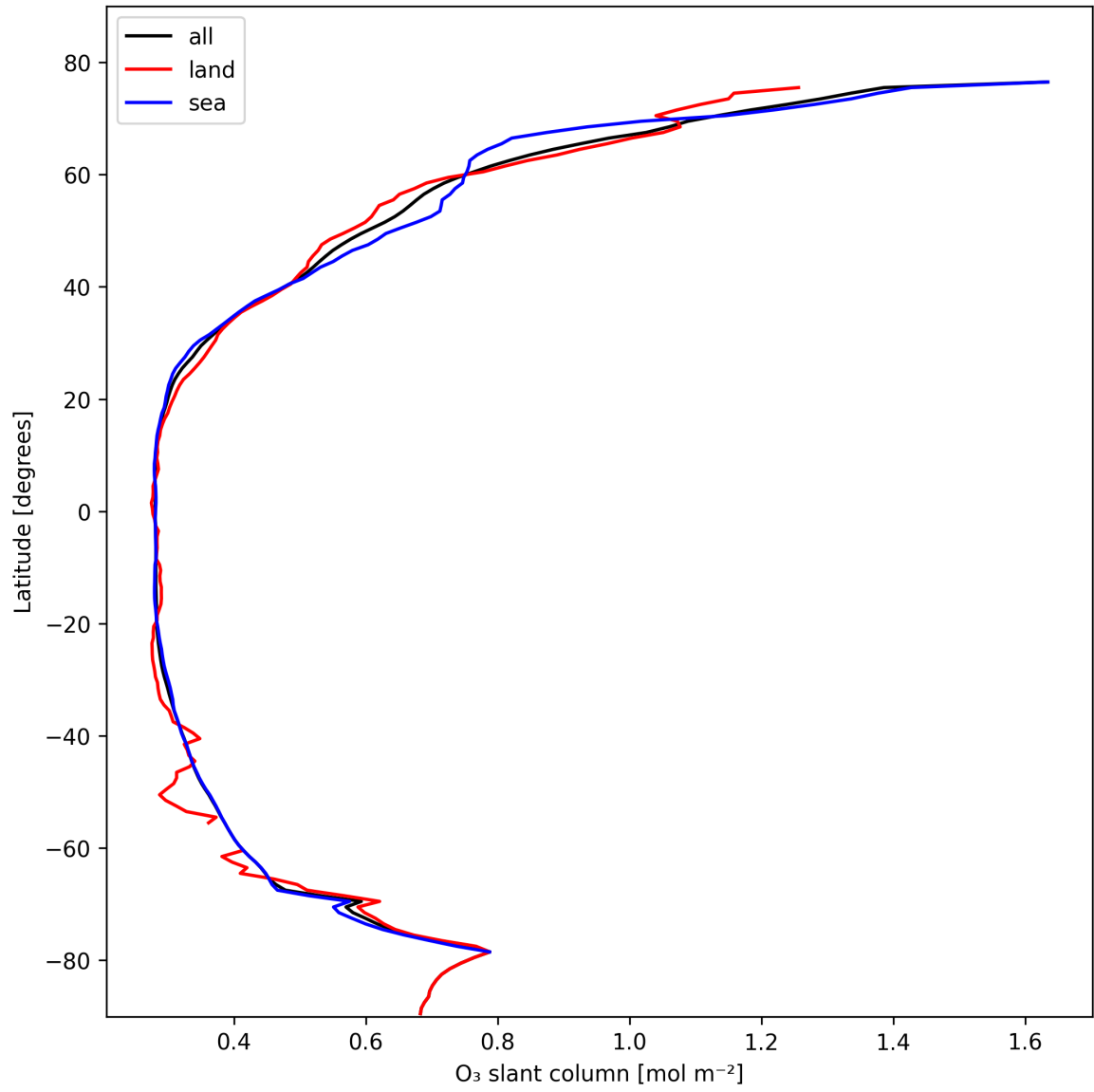
Figure 19: Zonal average of “O 3 slant column” for 2025-02-13 to 2025-02-14.
