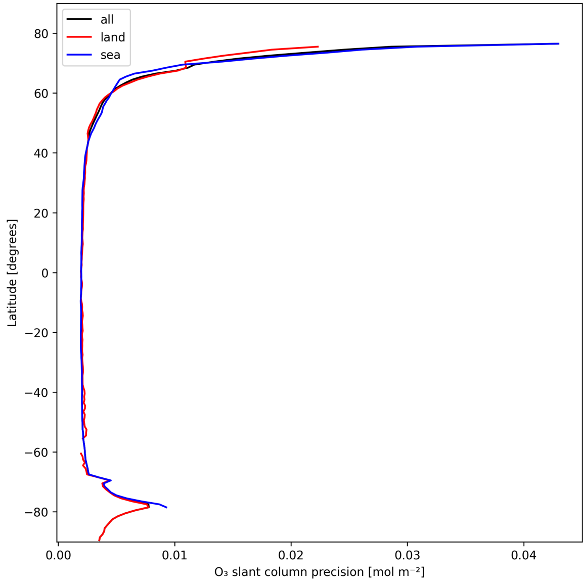
Figure 20: Zonal average of "O 3 slant column precision" for 2025-02-13 to 2025-02-14.
