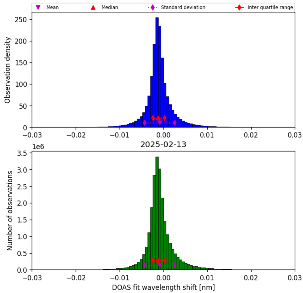
Figure 35: Histogram of “DOAS fit wavelength shift” for 2025-02-13 to 2025-02-14
