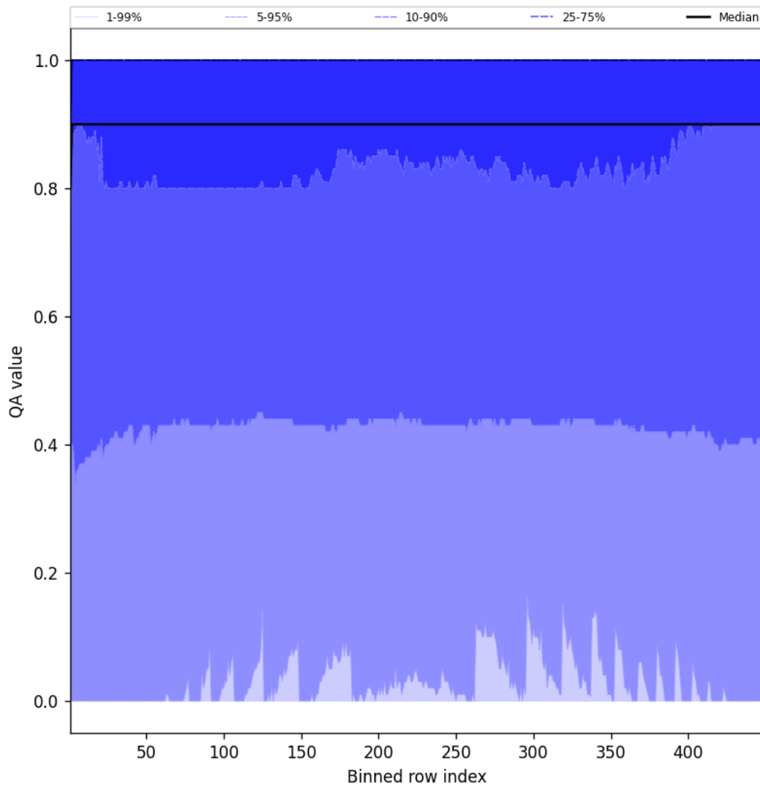
Figure 40: Along track statistics of “QA value” for 2025-02-13 to 2025-02-14
