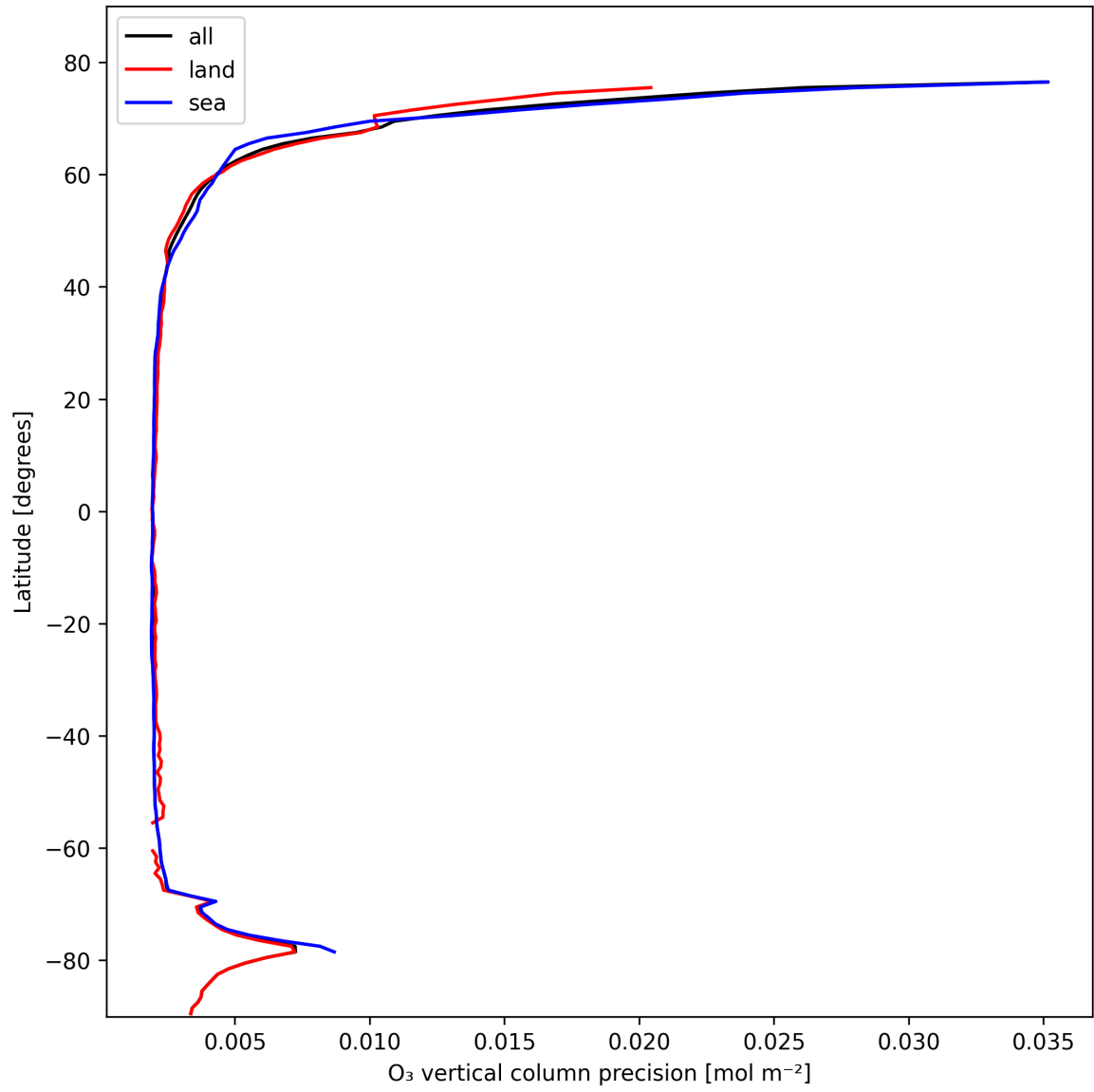
Figure 18: Zonal average of "O 3 vertical column precision" for 2025-02-13 to 2025-02-14.
