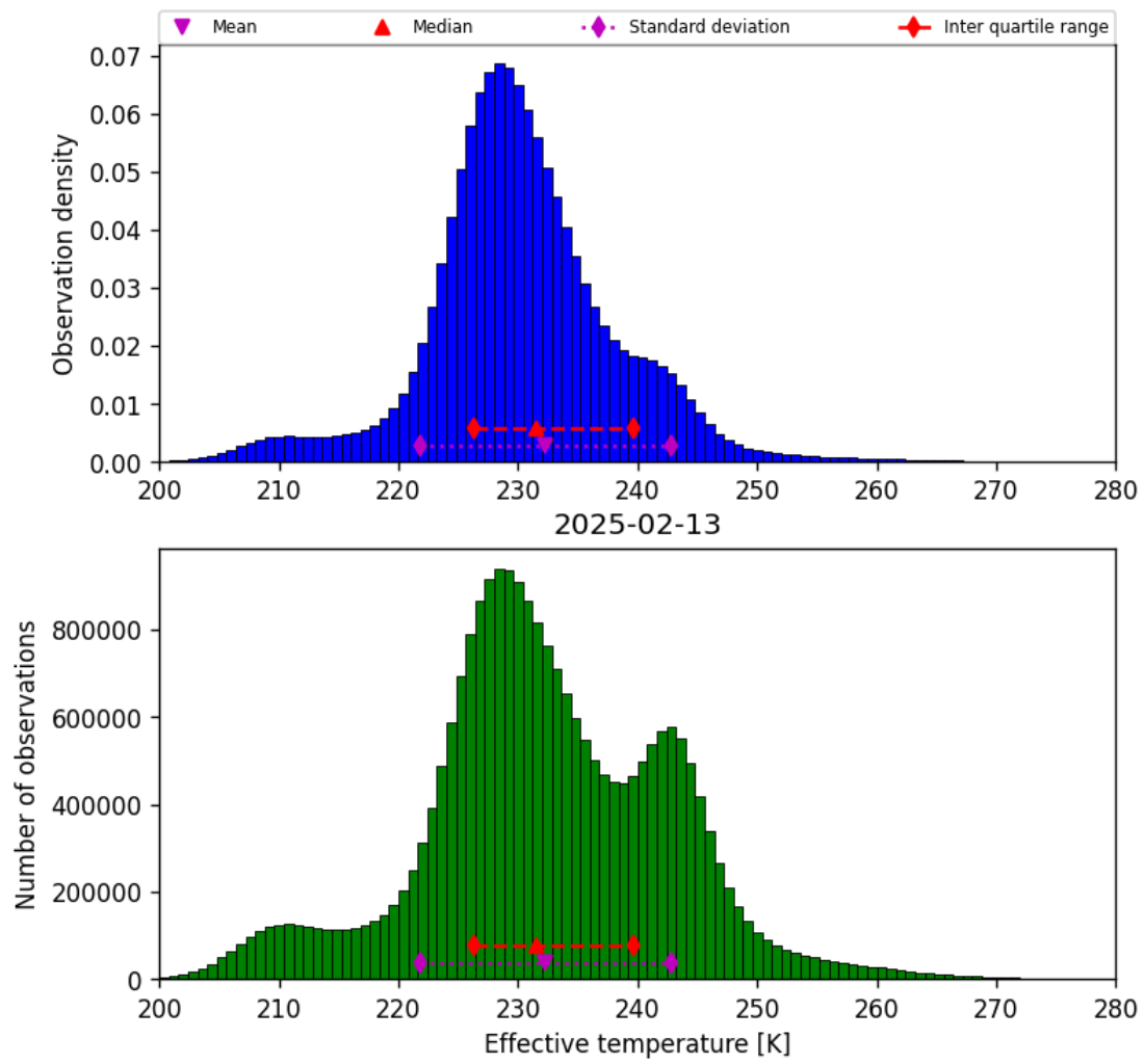
Figure 38: Histogram of “Effective temperature” for 2025-02-13 to 2025-02-14
