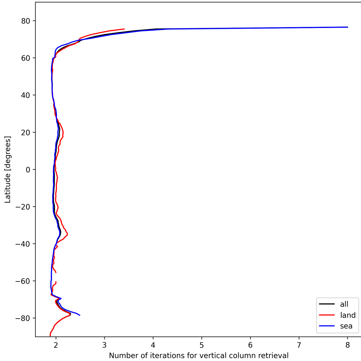
Figure 27: Zonal average of “Number of iterations for vertical column retrieval” for 2025-02-13 to 2025-02-14.
