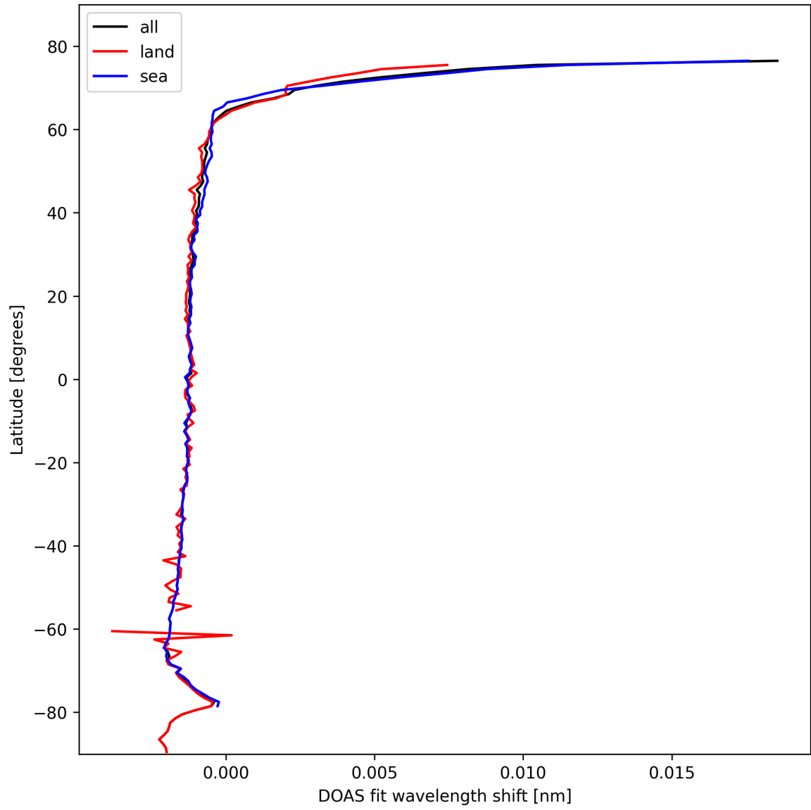
Figure 23: Zonal average of “DOAS fit wavelength shift” for 2025-02-13 to 2025-02-14.
