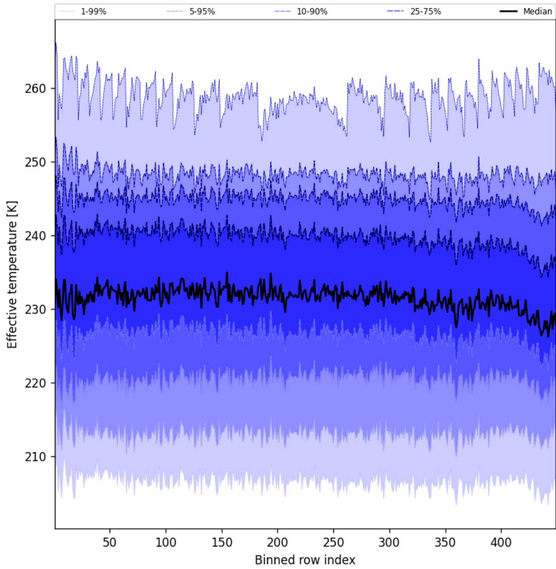
Figure 50: Along track statistics of “Effective temperature” for 2025-02-13 to 2025-02-14
