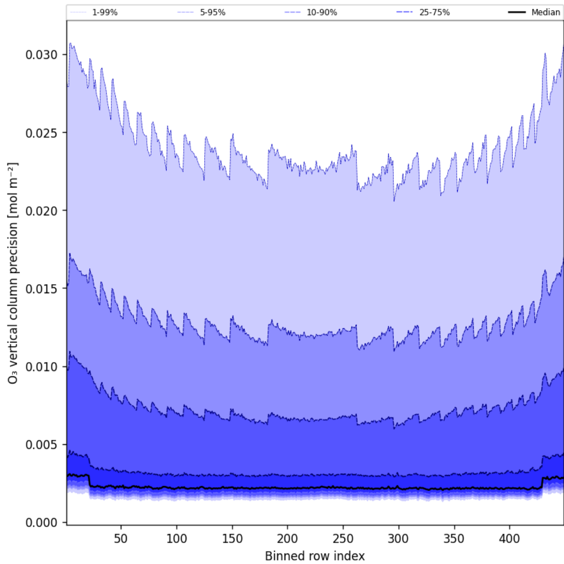
Figure 42: Along track statistics of “O 3 vertical column precision” for 2025-02-13 to 2025-02-14
