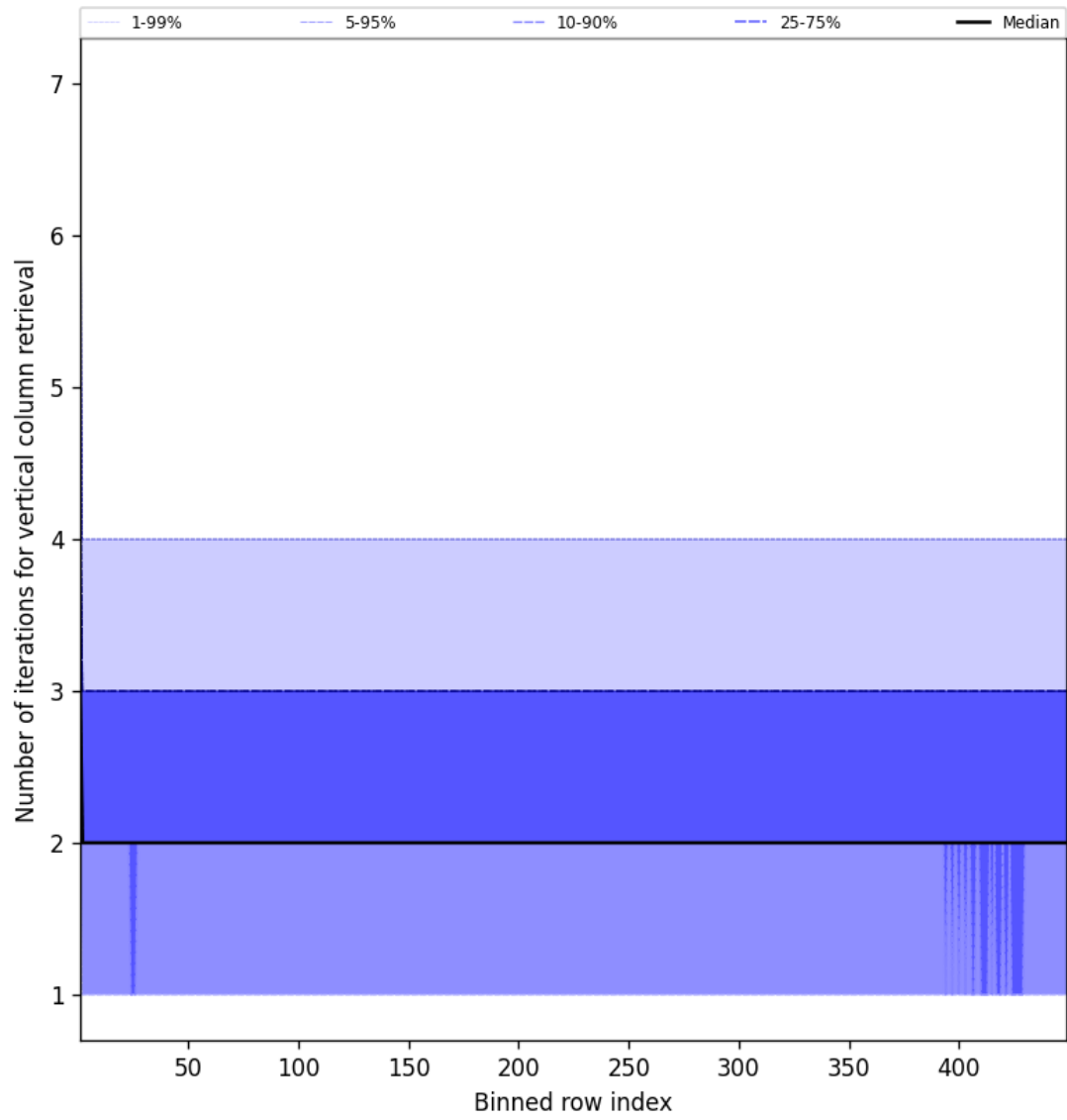
Figure 51: Along track statistics of “Number of iterations for vertical column retrieval” for 2025-02-13 to 2025-02-14
