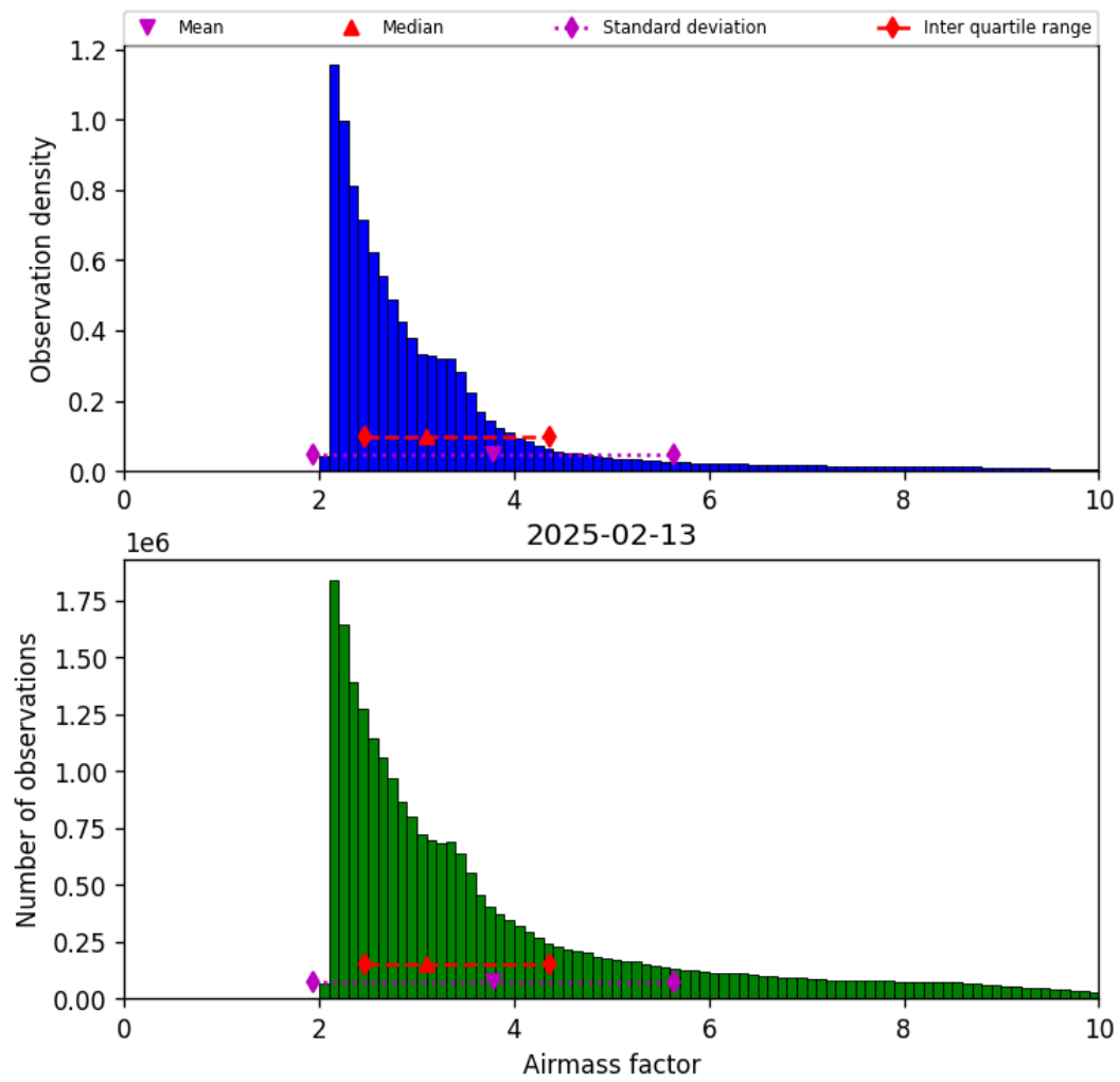
Figure 37: Histogram of “Airmass factor” for 2025-02-13 to 2025-02-14
