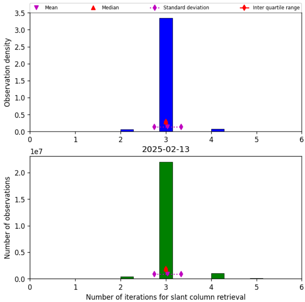
Figure 33: Histogram of “Number of iterations for slant column retrieval” for 2025-02-13 to 2025-02-14
