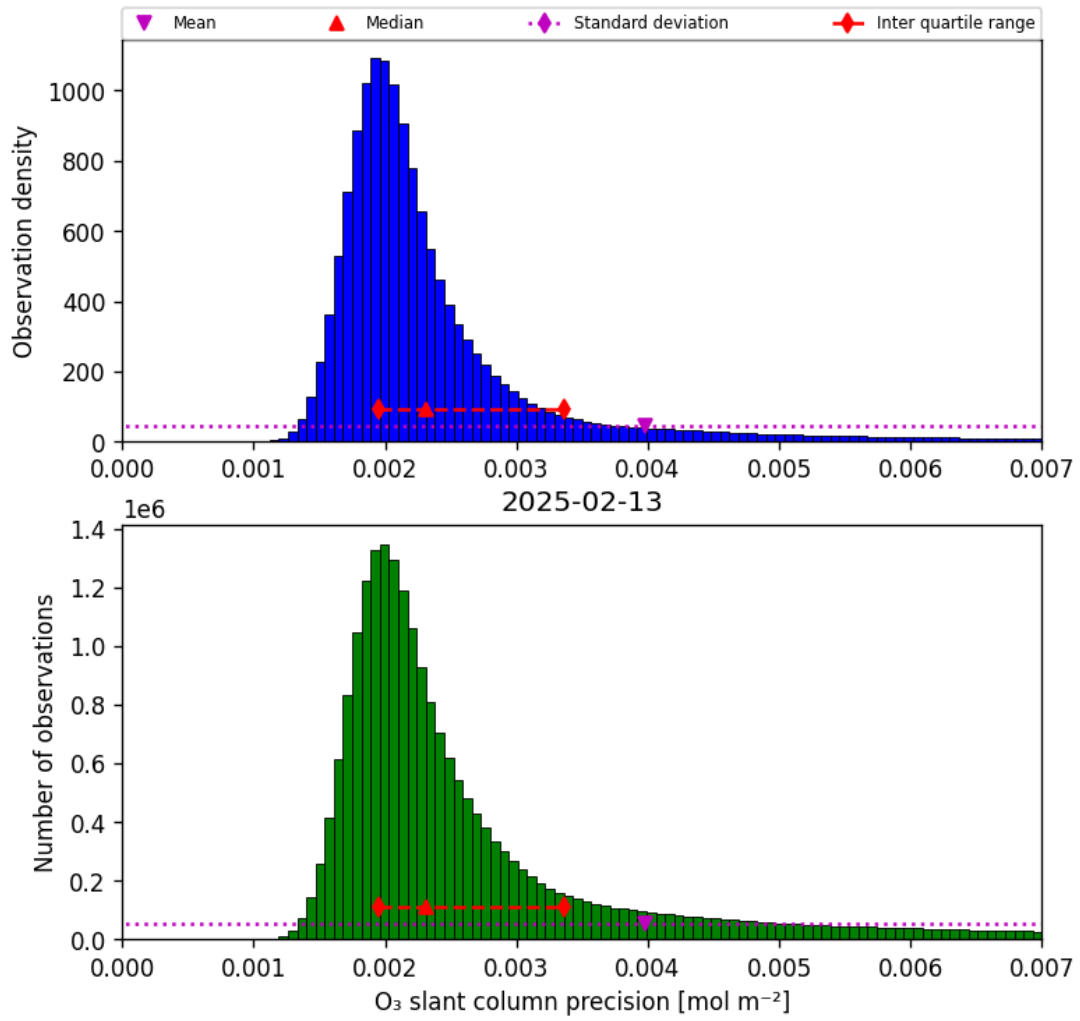
Figure 32: Histogram of “O 3 slant column precision” for 2025-02-13 to 2025-02-14
