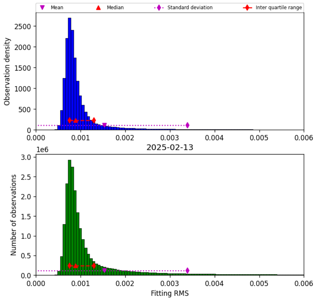
Figure 34: Histogram of “Fitting RMS” for 2025-02-13 to 2025-02-14
