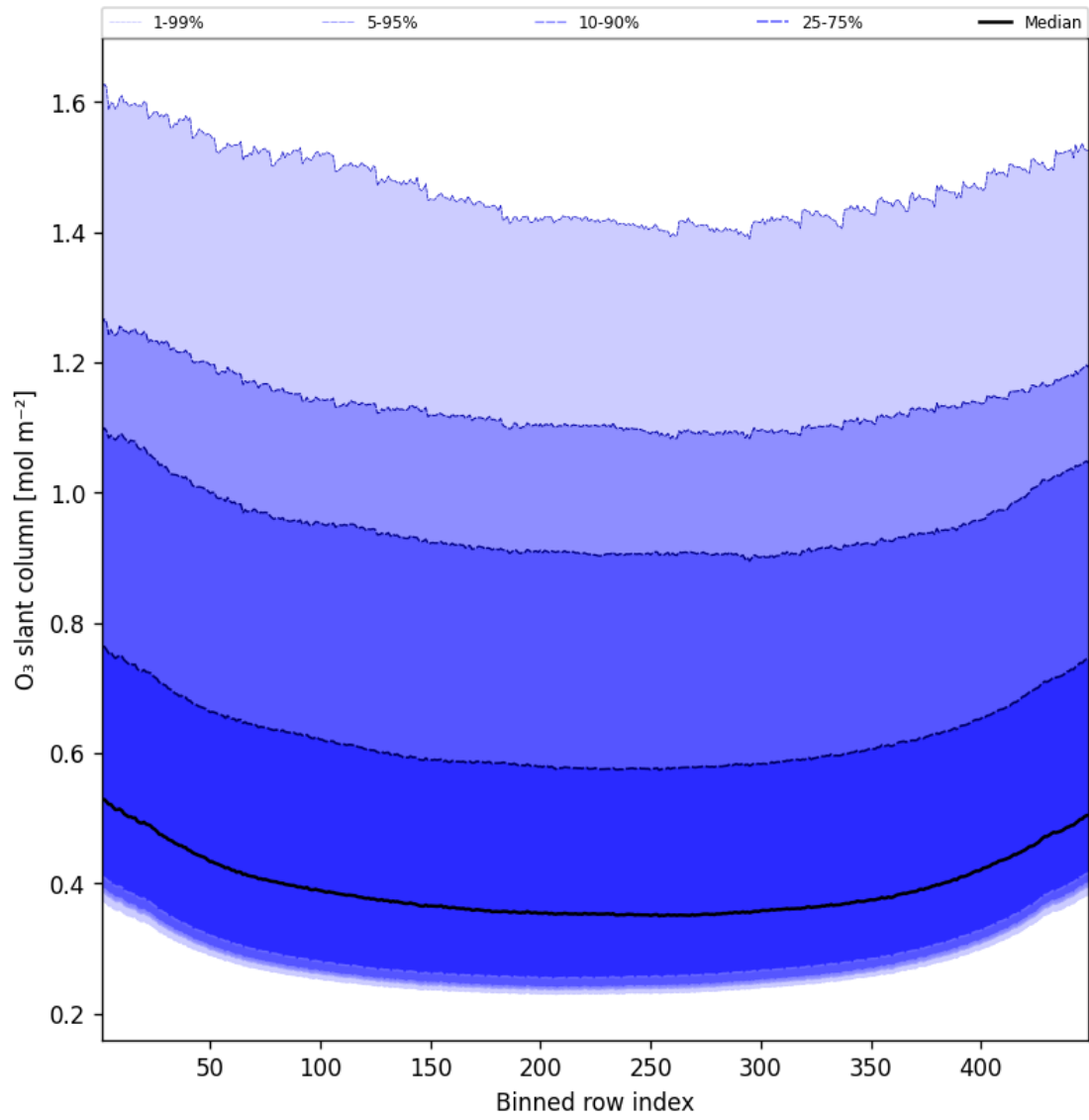
Figure 43: Along track statistics of “O 3 slant column” for 2025-02-13 to 2025-02-14
