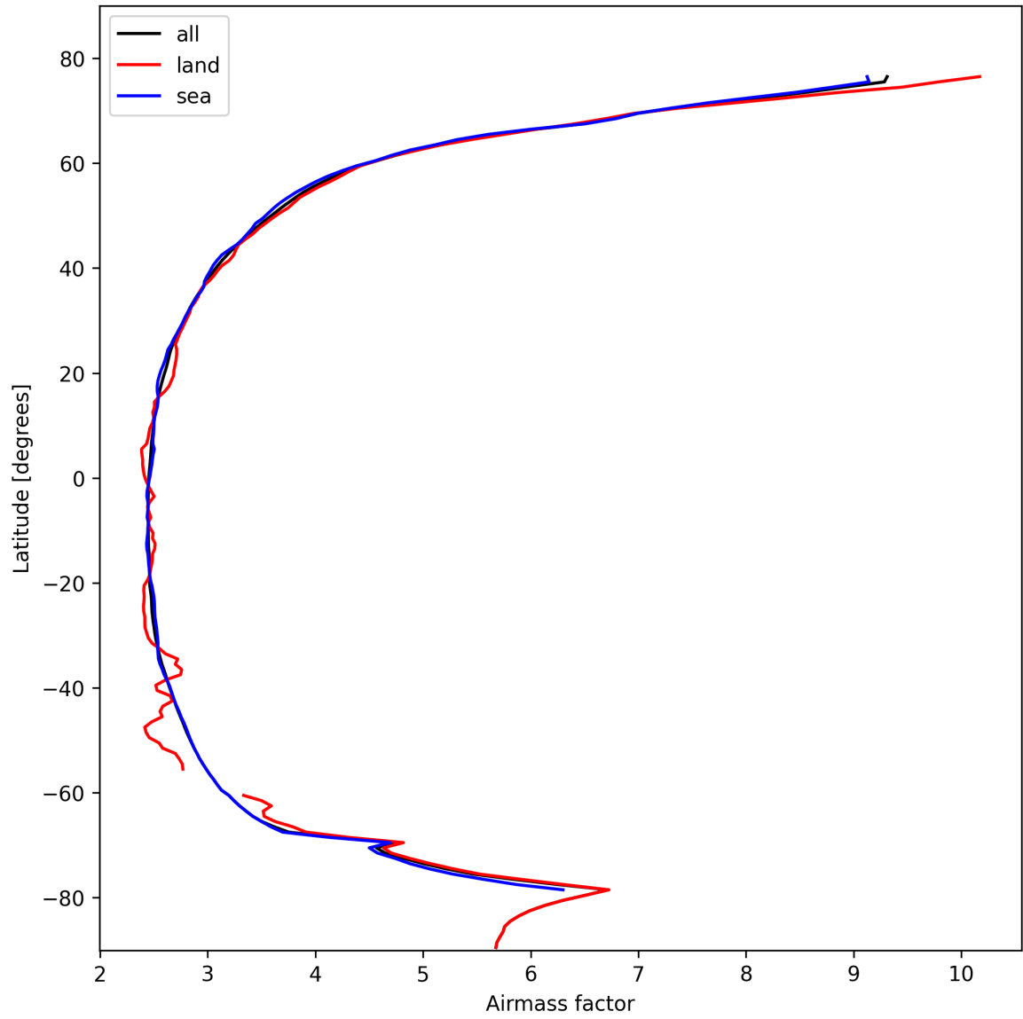
Figure 25: Zonal average of “Airmass factor” for 2025-02-14 to 2025-02-15.
