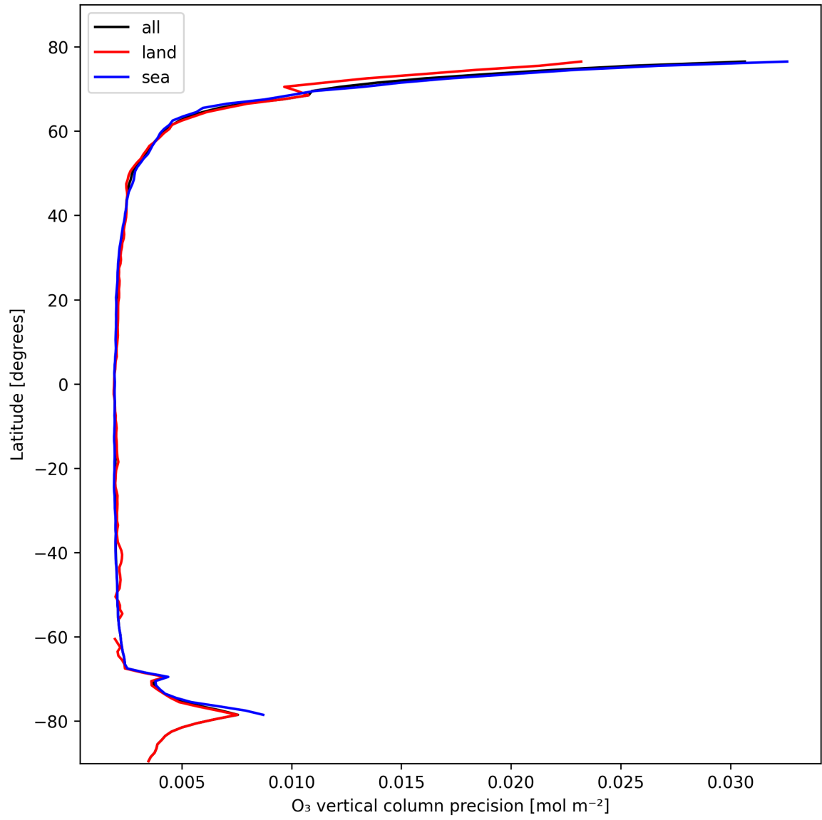
Figure 18: Zonal average of “O 3 vertical column precision” for 2025-02-14 to 2025-02-15.
