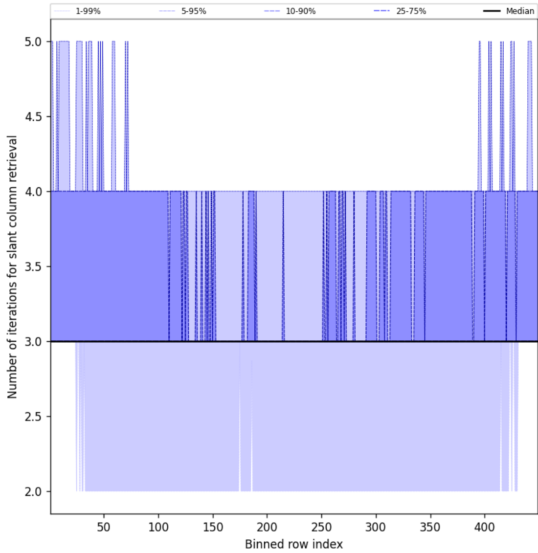
Figure 45: Along track statistics of “Number of iterations for slant column retrieval” for 2025-02-14 to 2025-02-15
