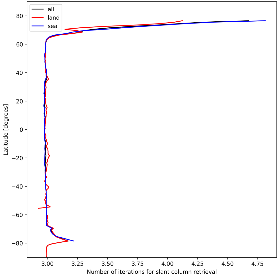
Figure 21: Zonal average of “Number of iterations for slant column retrieval” for 2025-02-14 to 2025-02-15.
