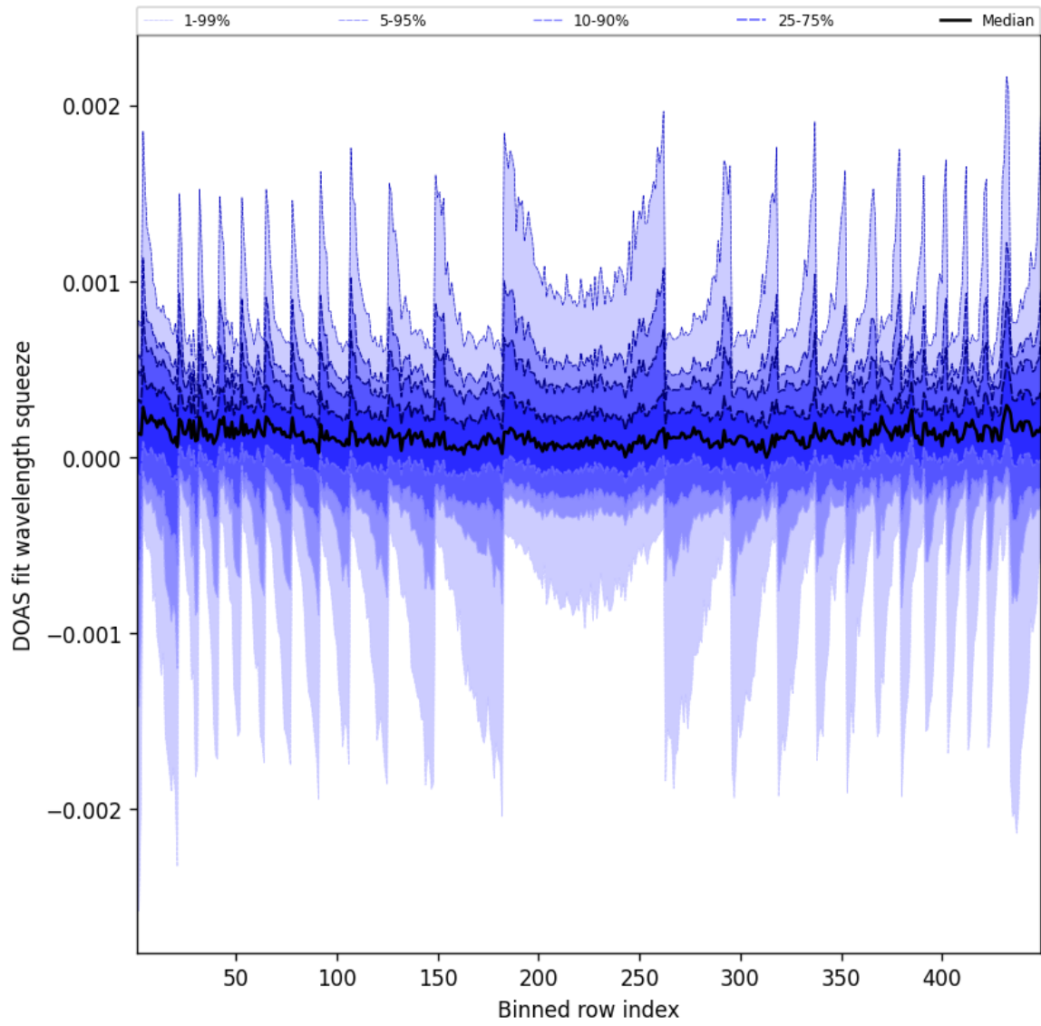
Figure 48: Along track statistics of “DOAS fit wavelength squeeze” for 2025-02-14 to 2025-02-15
