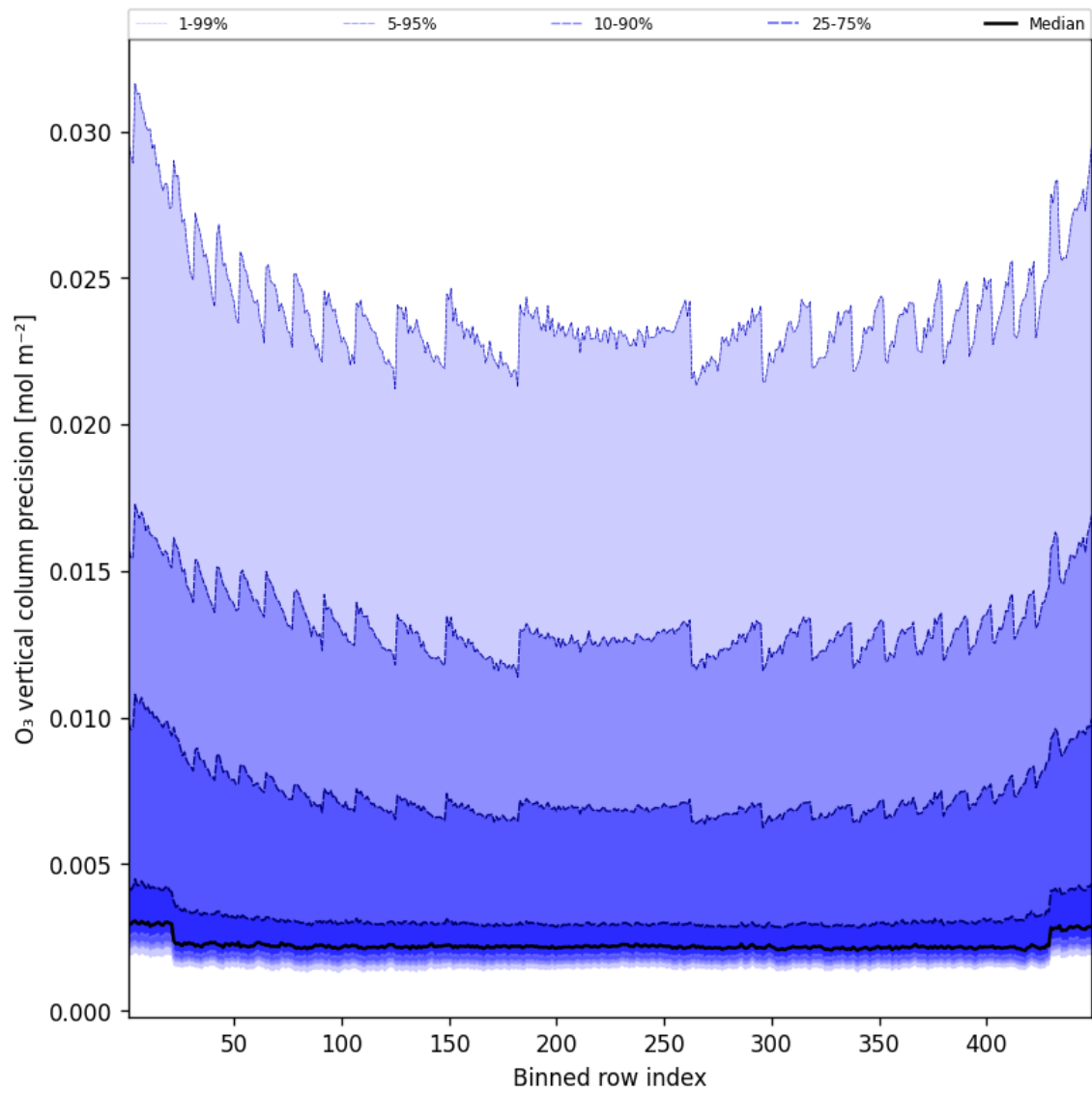
Figure 42: Along track statistics of “O 3 vertical column precision” for 2025-02-14 to 2025-02-15
