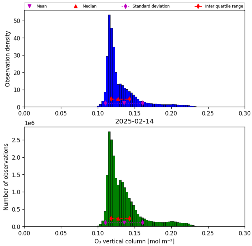
Figure 29: Histogram of “O 3 vertical column” for 2025-02-14 to 2025-02-15
