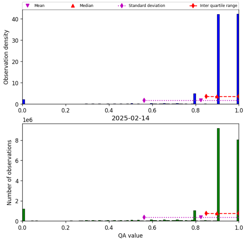
Figure 28: Histogram of “QA value” for 2025-02-14 to 2025-02-15
