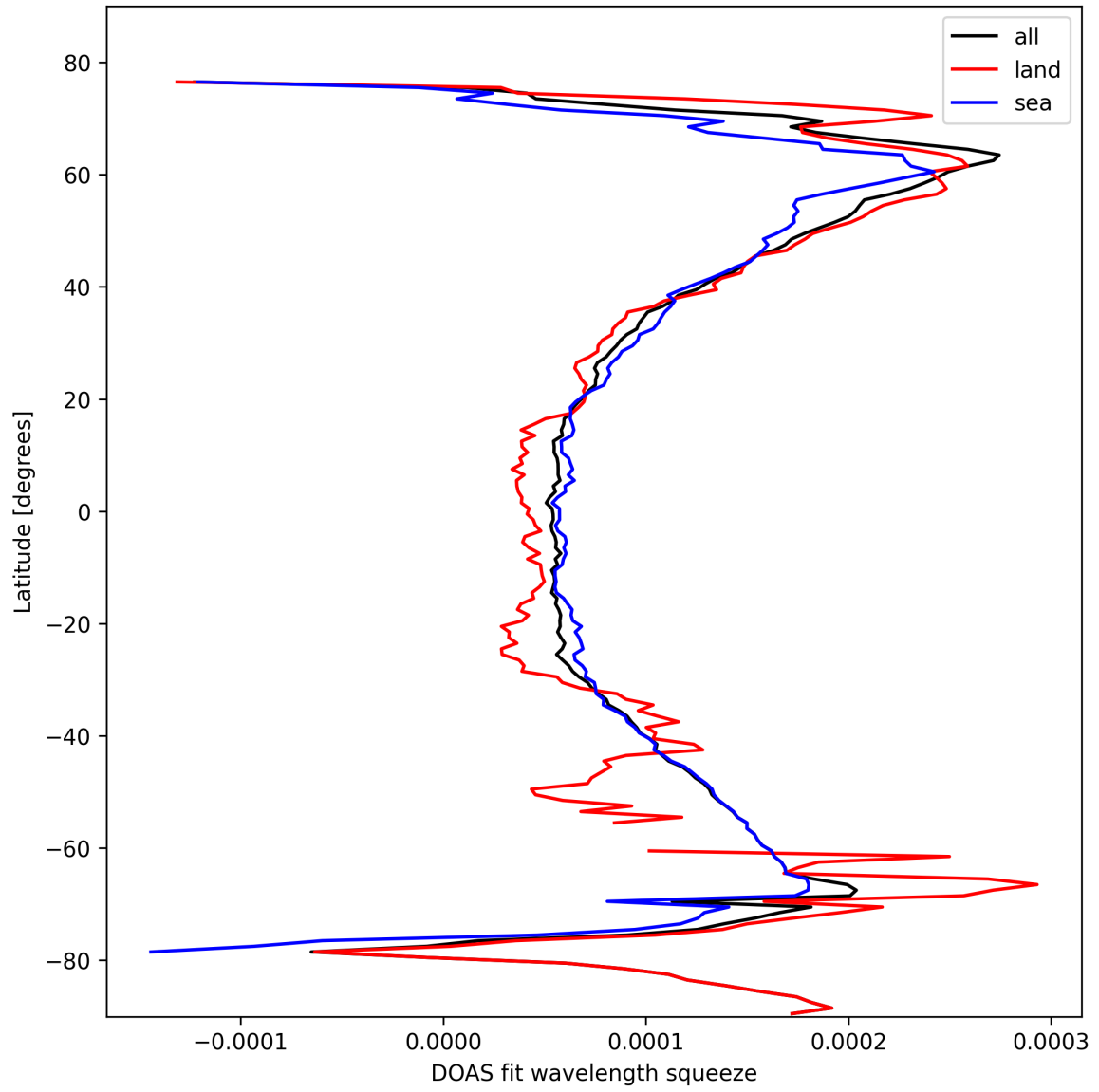
Figure 24: Zonal average of “DOAS fit wavelength squeeze” for 2025-02-14 to 2025-02-15.
