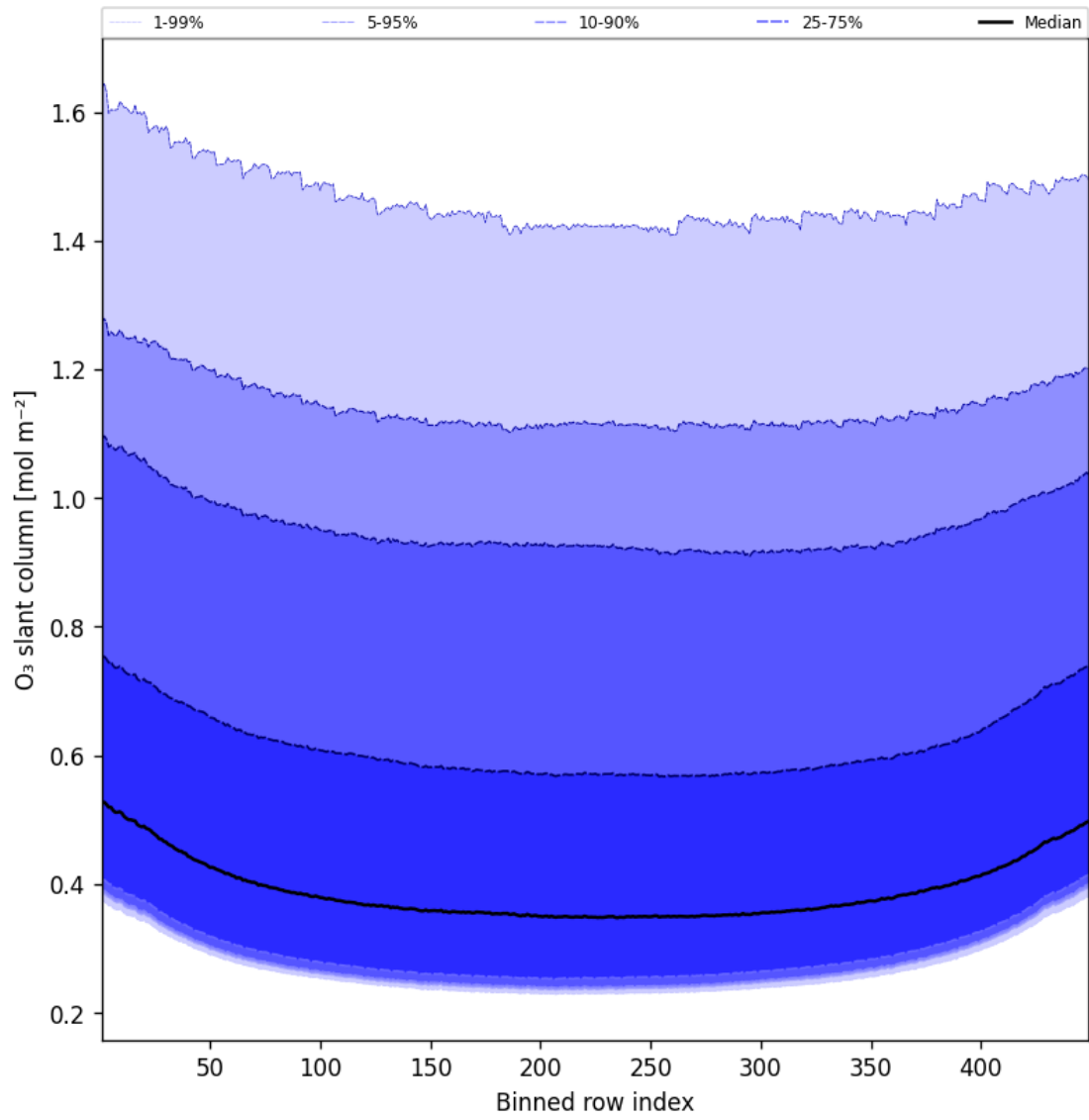
Figure 43: Along track statistics of “O 3 slant column” for 2025-02-14 to 2025-02-15
