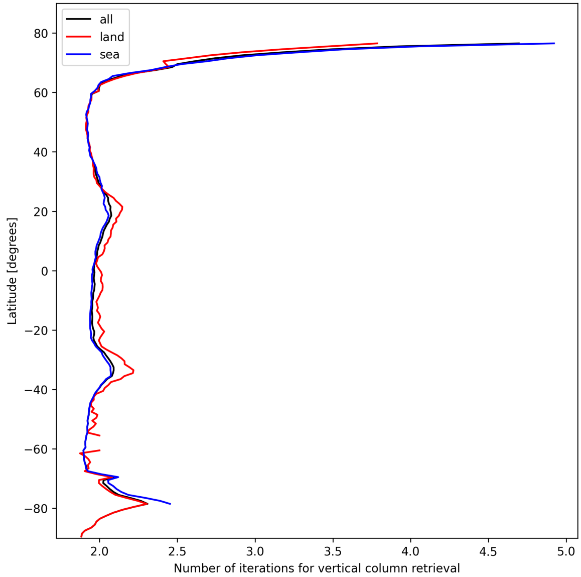
Figure 27: Zonal average of “Number of iterations for vertical column retrieval” for 2025-02-14 to 2025-02-15.
