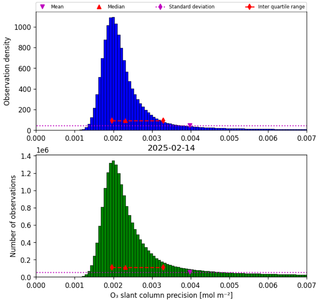
Figure 32: Histogram of “O 3 slant column precision” for 2025-02-14 to 2025-02-15
