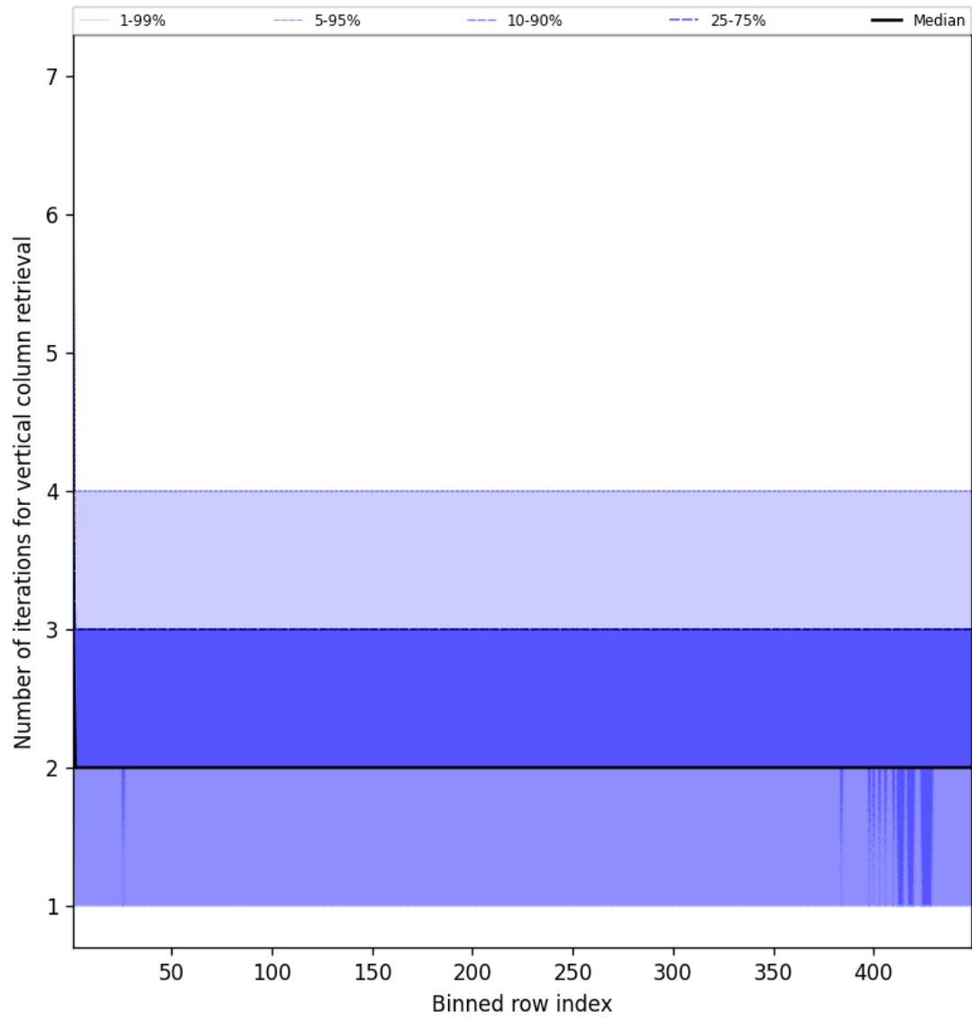
Figure 51: Along track statistics of “Number of iterations for vertical column retrieval” for 2025-02-14 to 2025-02-15
