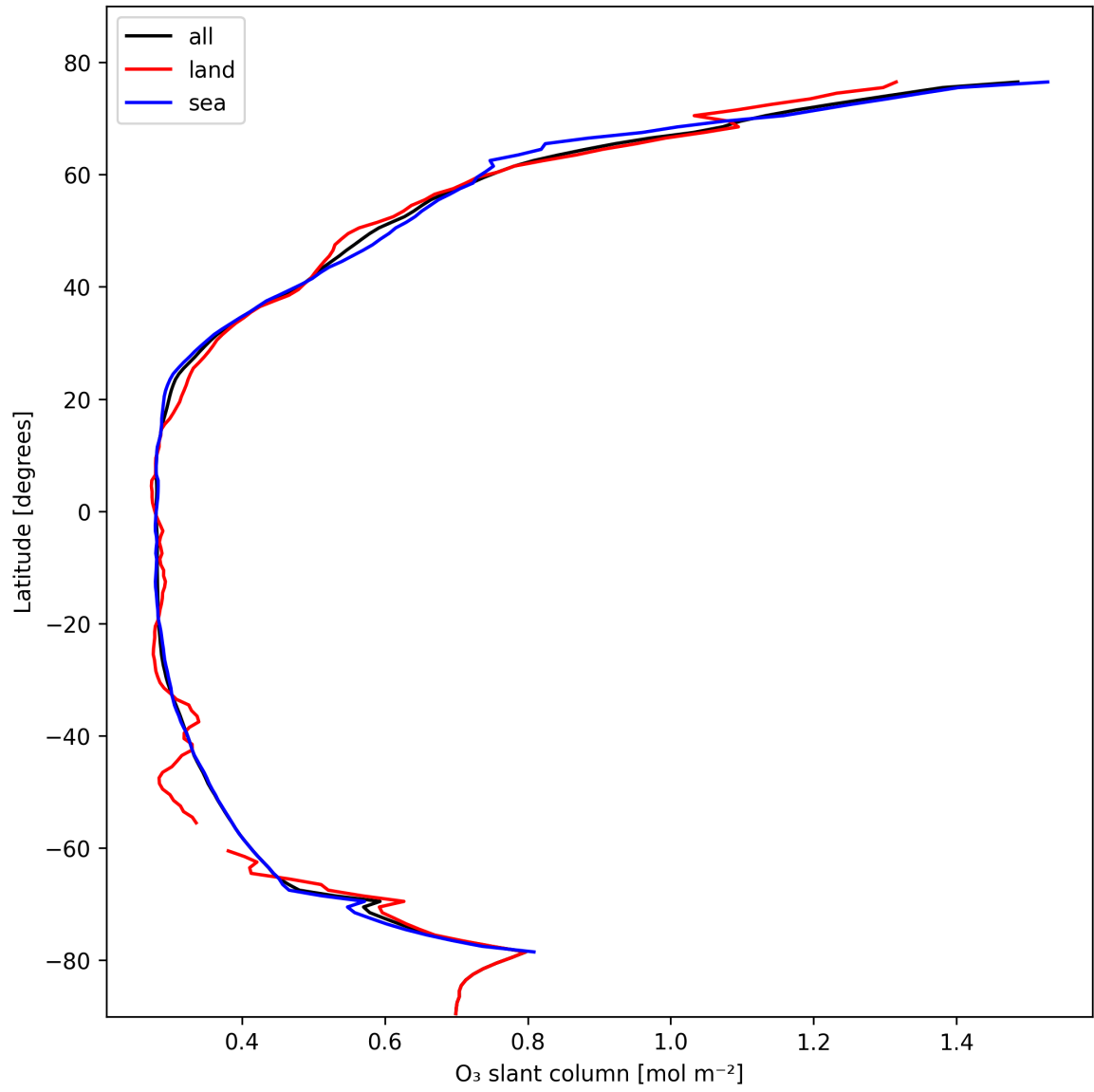
Figure 19: Zonal average of “O 3 slant column” for 2025-02-14 to 2025-02-15.
