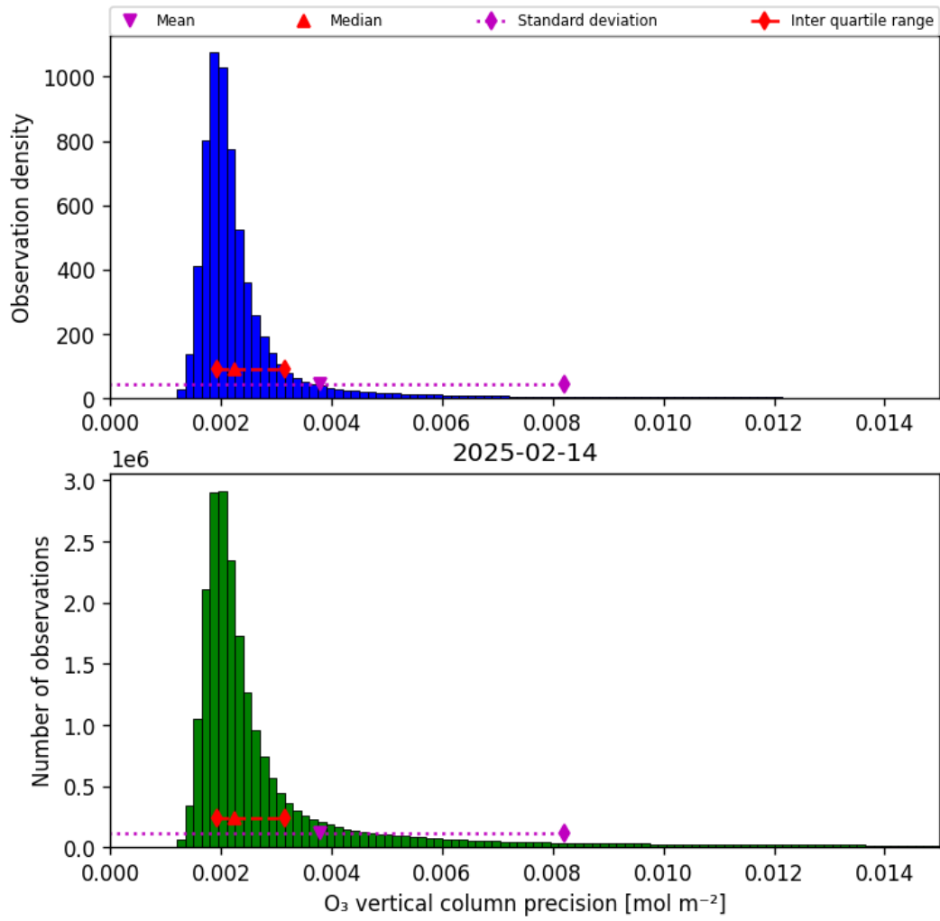
Figure 30: Histogram of “O 3 vertical column precision” for 2025-02-14 to 2025-02-15
