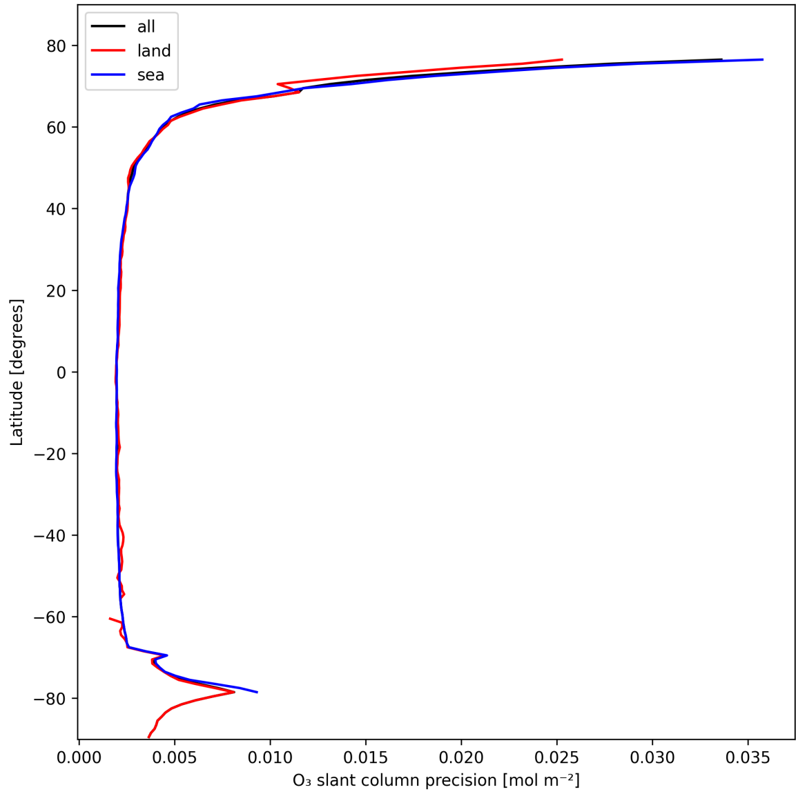
Figure 20: Zonal average of "O 3 slant column precision" for 2025-02-14 to 2025-02-15.
