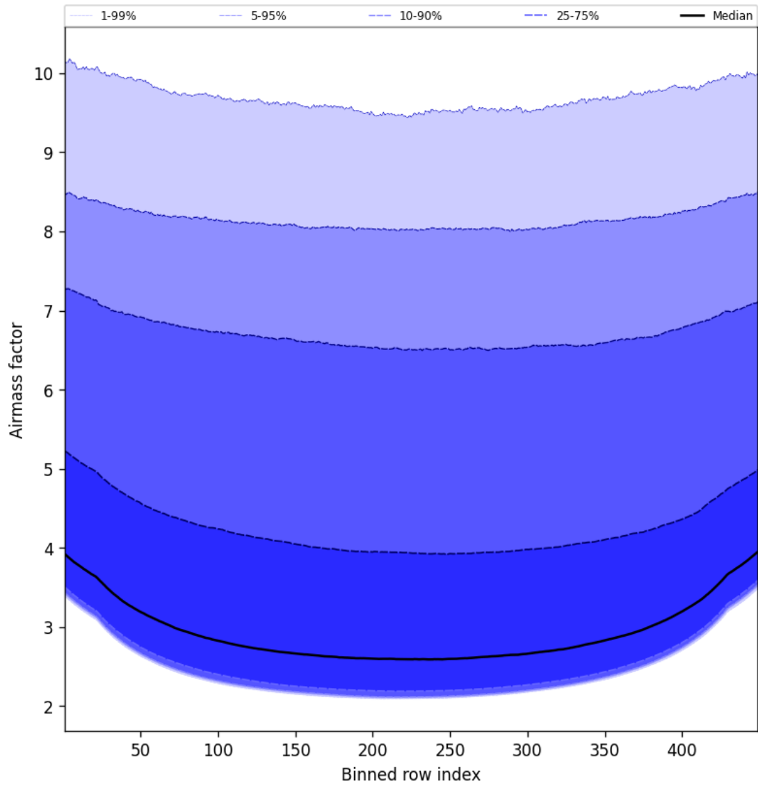
Figure 49: Along track statistics of “Airmass factor” for 2025-02-14 to 2025-02-15
