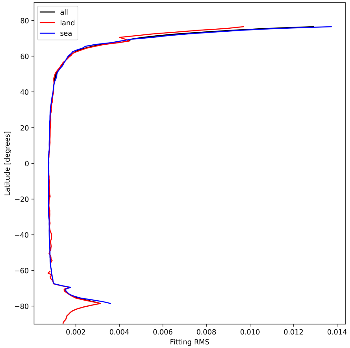
Figure 22: Zonal average of “Fitting RMS” for 2025-02-14 to 2025-02-15.
