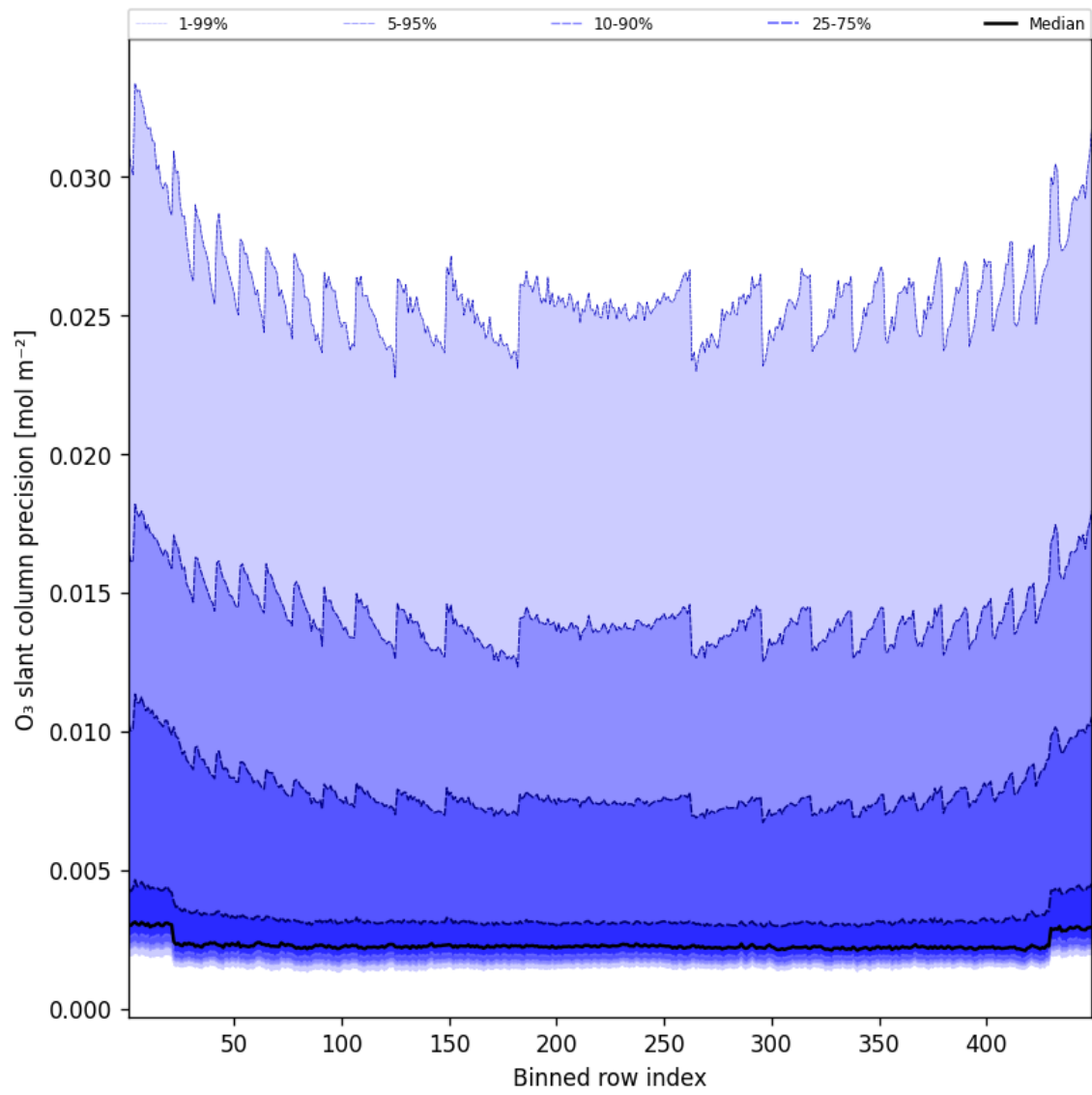
Figure 44: Along track statistics of "O 3 slant column precision" for 2025-02-14 to 2025-02-15
