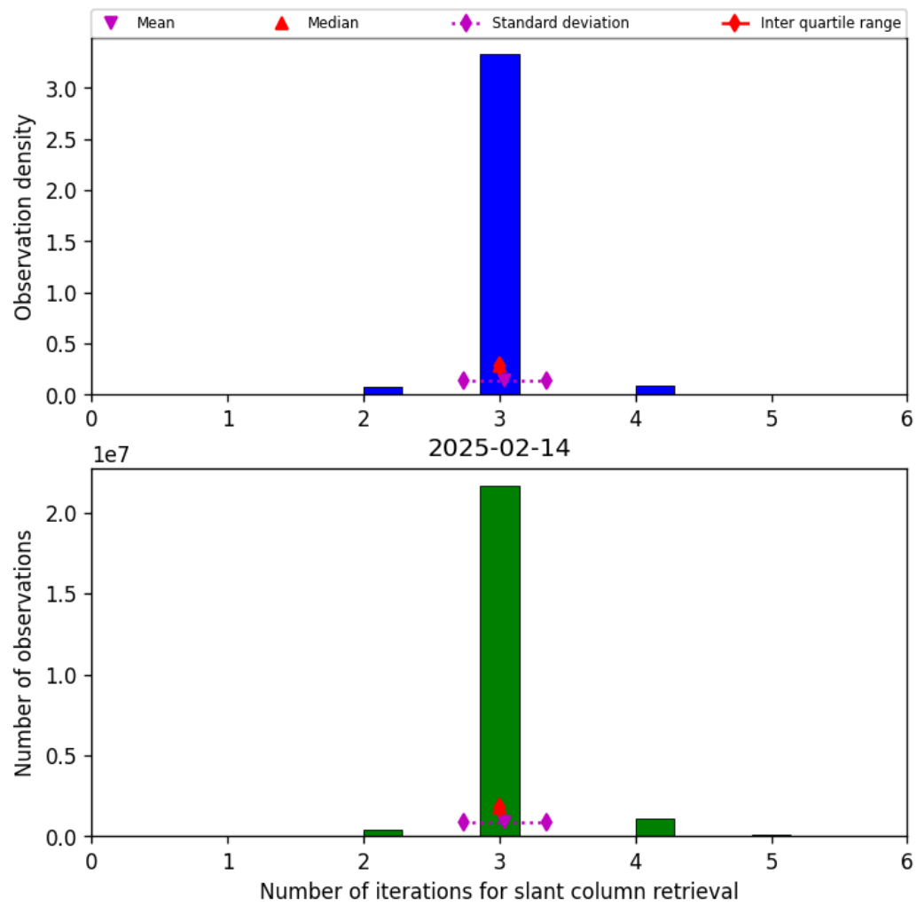
Figure 33: Histogram of “Number of iterations for slant column retrieval” for 2025-02-14 to 2025-02-15
