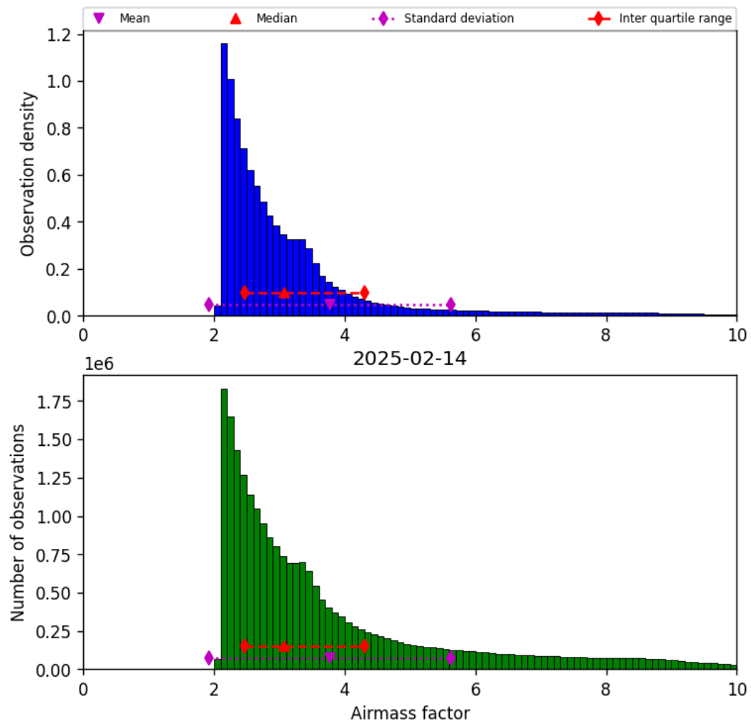
Figure 37: Histogram of “Airmass factor” for 2025-02-14 to 2025-02-15
