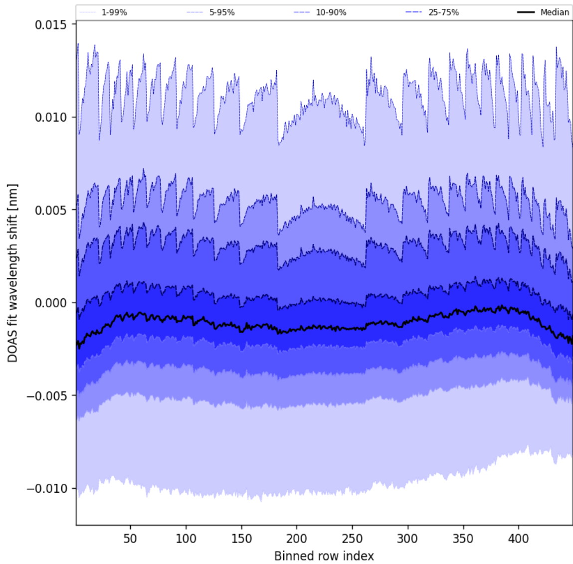
Figure 47: Along track statistics of “DOAS fit wavelength shift” for 2025-02-14 to 2025-02-15
