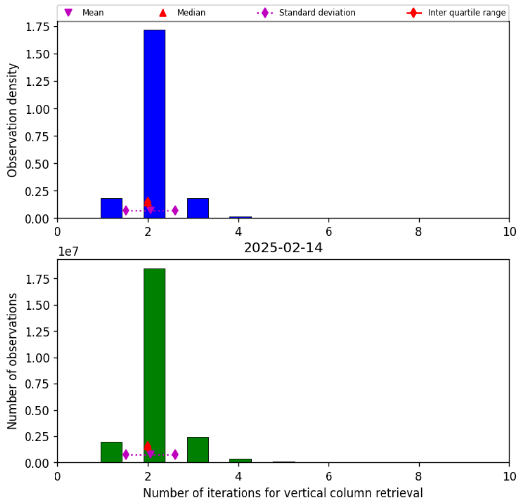
Figure 39: Histogram of “Number of iterations for vertical column retrieval” for 2025-02-14 to 2025-02-15
