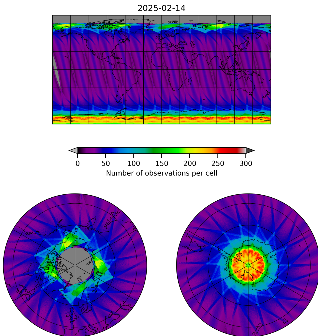
Figure 15: Map of the number of observations for 2025-02-14 to 2025-02-15
