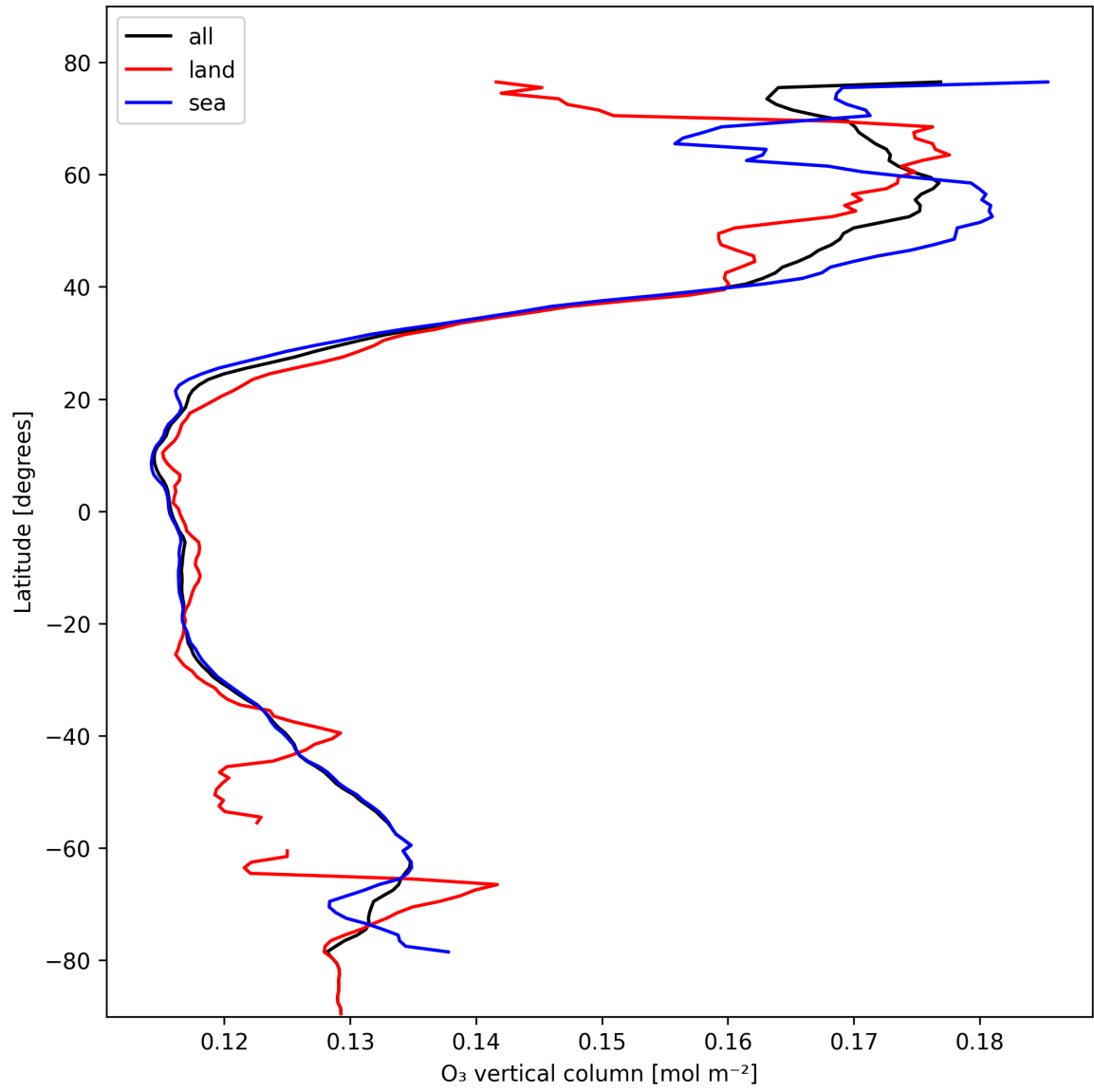
Figure 17: Zonal average of “O 3 vertical column” for 2025-02-14 to 2025-02-15.
