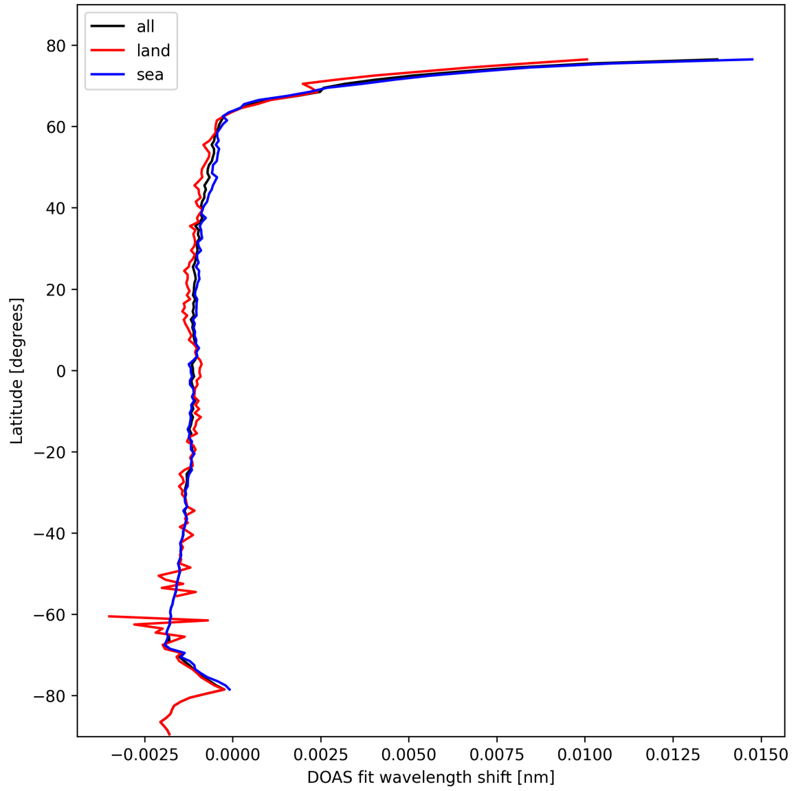
Figure 23: Zonal average of “DOAS fit wavelength shift” for 2025-02-14 to 2025-02-15.
