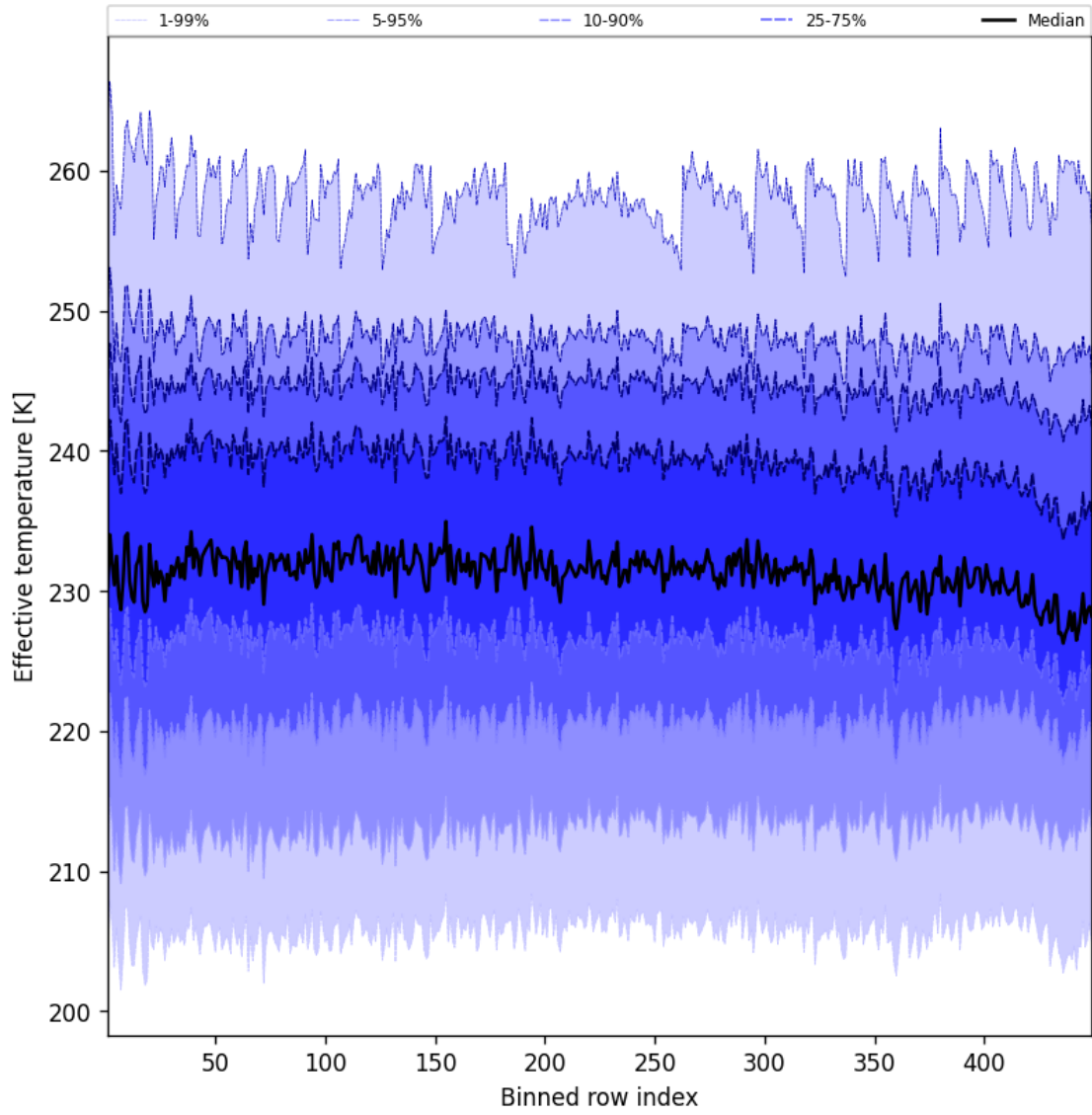
Figure 50: Along track statistics of “Effective temperature” for 2025-02-14 to 2025-02-15
