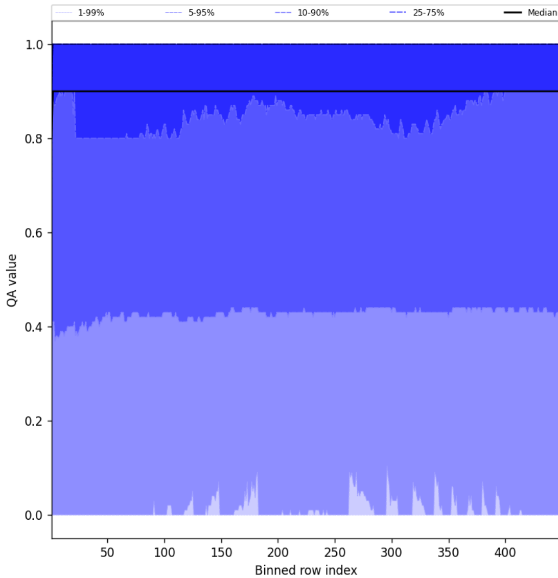
Figure 40: Along track statistics of “QA value” for 2025-02-14 to 2025-02-15
