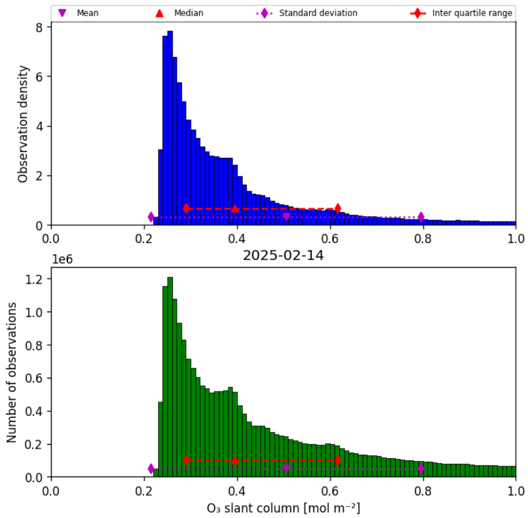
Figure 31: Histogram of “O 3 slant column” for 2025-02-14 to 2025-02-15
