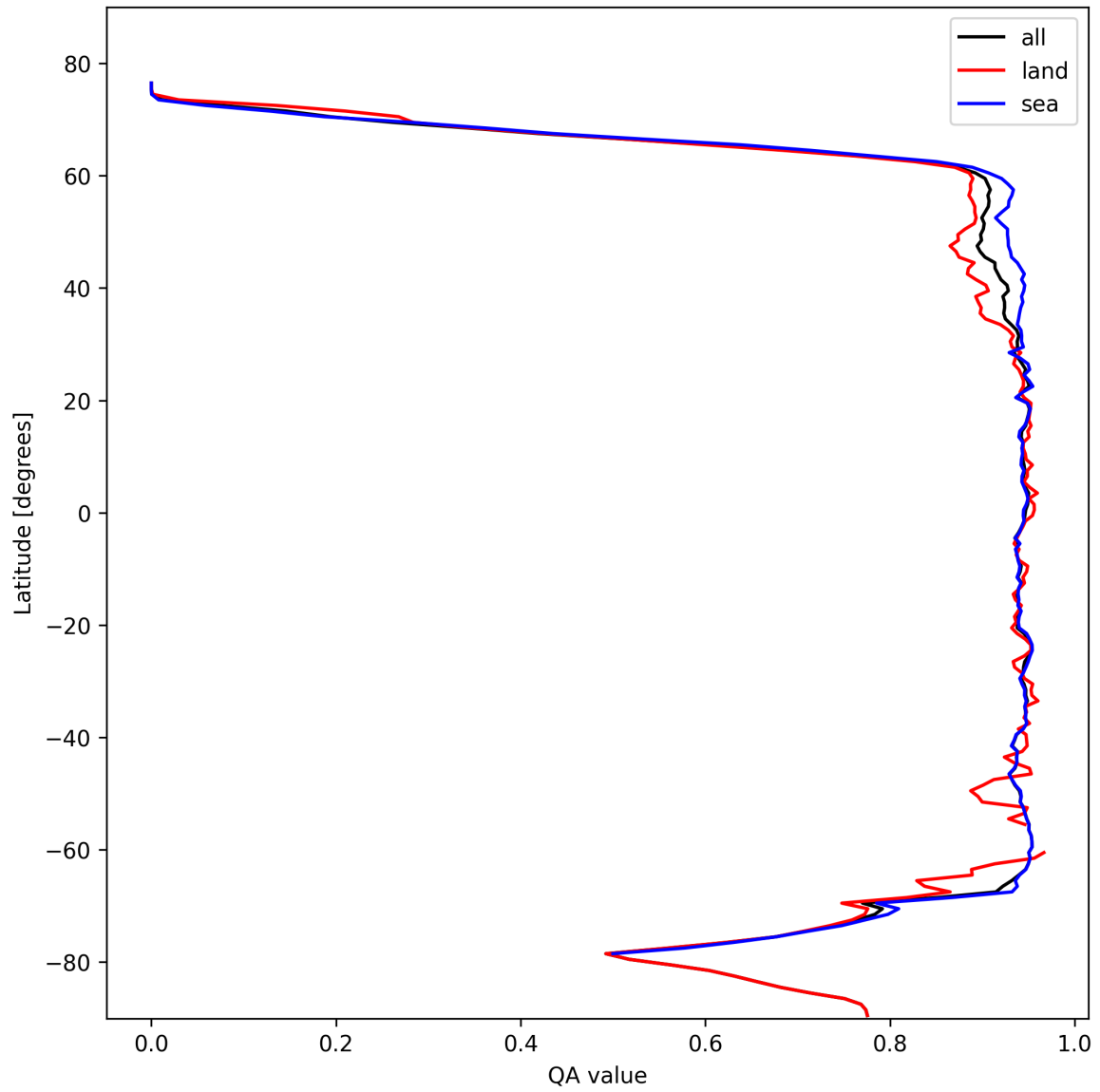
Figure 16: Zonal average of “QA value” for 2025-02-14 to 2025-02-15.
