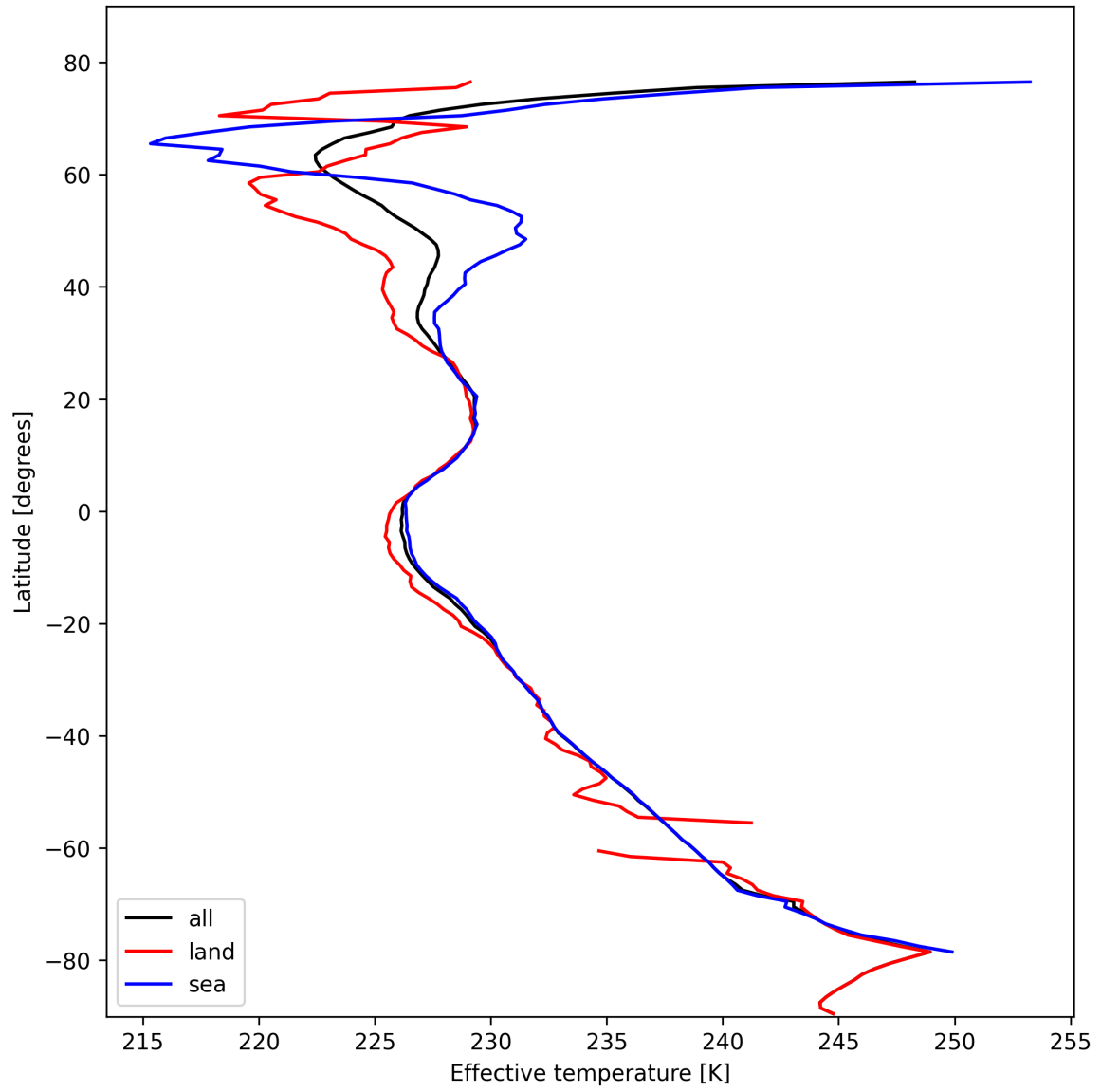
Figure 26: Zonal average of “Effective temperature” for 2025-02-14 to 2025-02-15.
