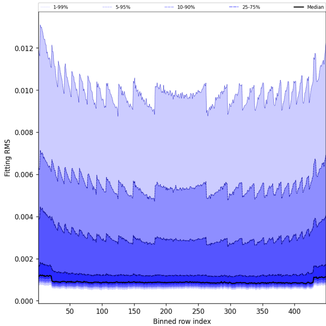
Figure 46: Along track statistics of “Fitting RMS” for 2025-02-14 to 2025-02-15
