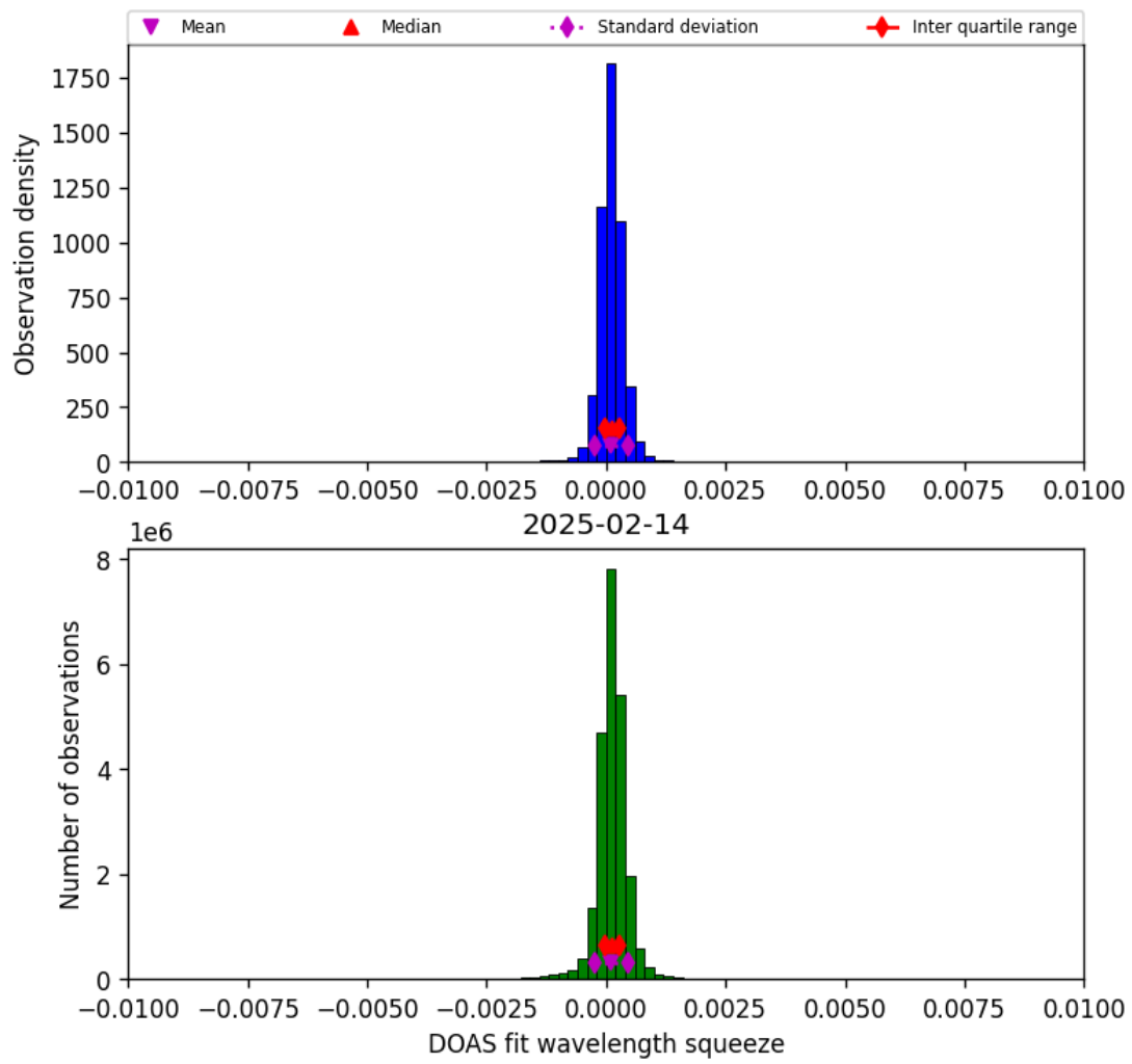
Figure 36: Histogram of “DOAS fit wavelength squeeze” for 2025-02-14 to 2025-02-15
