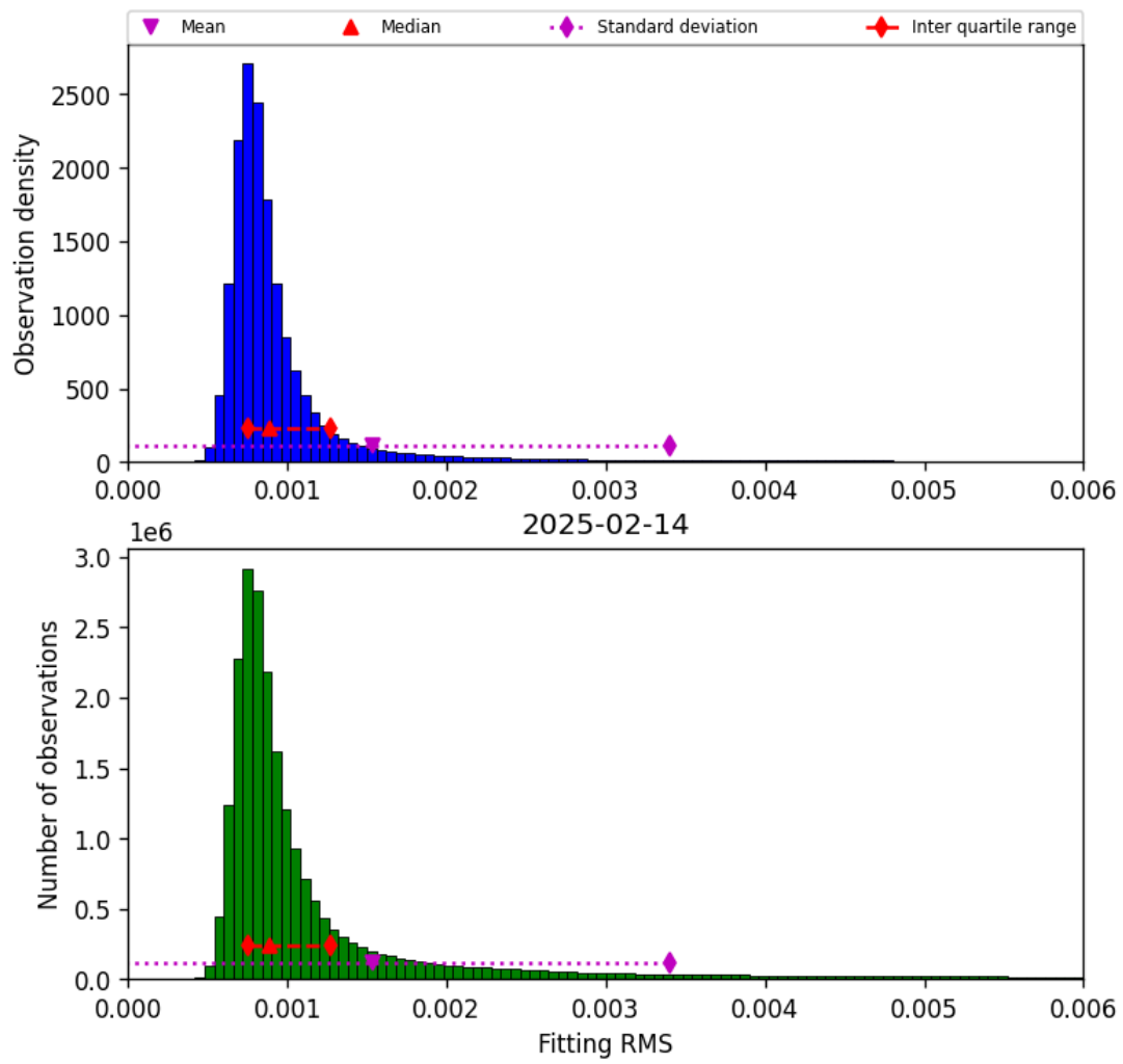
Figure 34: Histogram of “Fitting RMS” for 2025-02-14 to 2025-02-15
