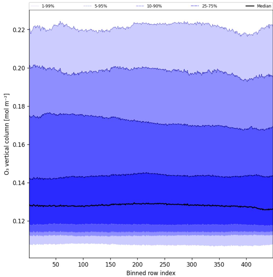
Figure 41: Along track statistics of “O 3 vertical column” for 2025-02-14 to 2025-02-15
