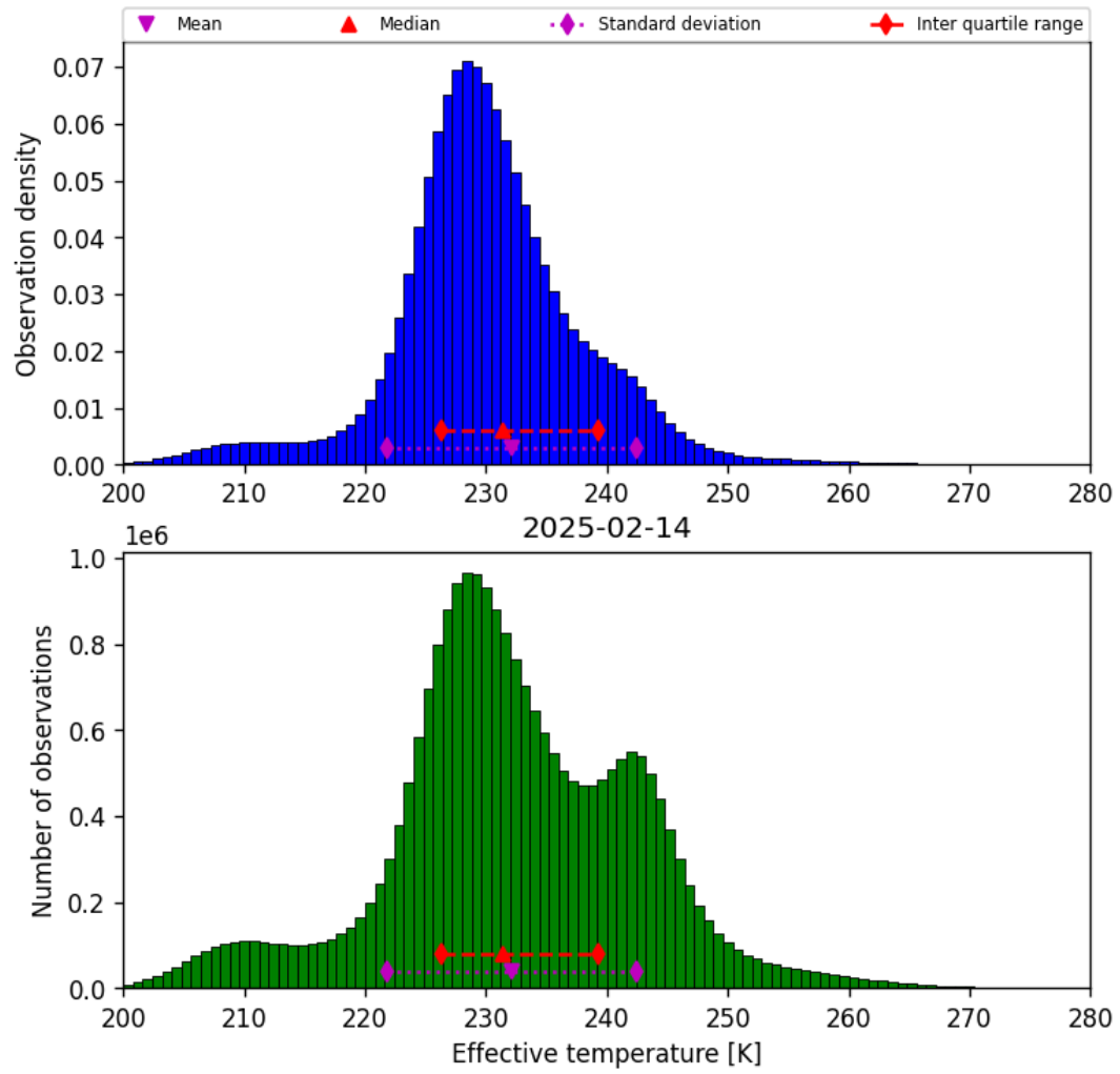
Figure 38: Histogram of “Effective temperature” for 2025-02-14 to 2025-02-15
