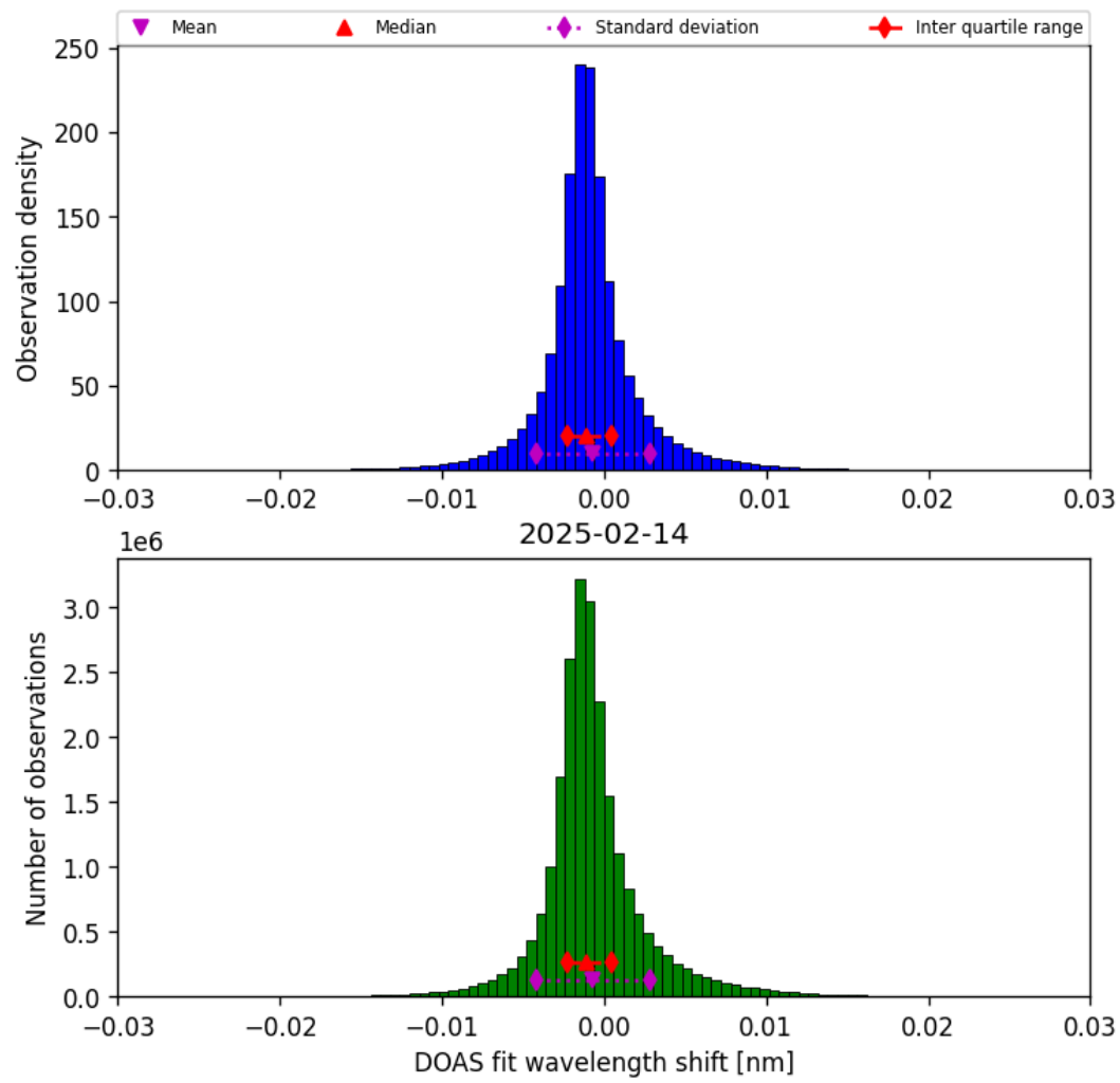
Figure 35: Histogram of “DOAS fit wavelength shift” for 2025-02-14 to 2025-02-15
