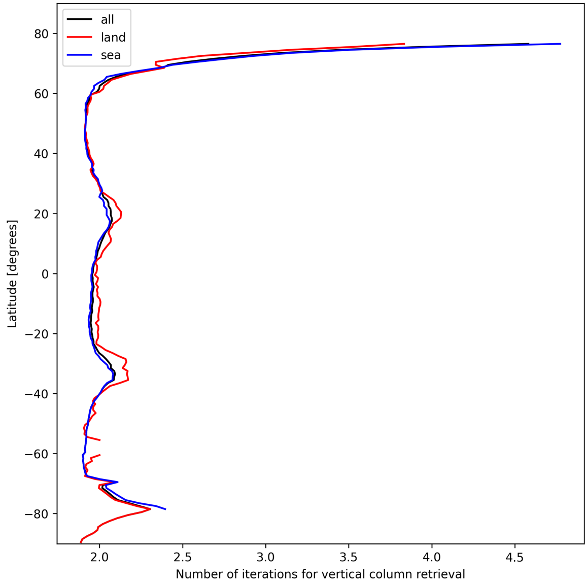
Figure 27: Zonal average of “Number of iterations for vertical column retrieval” for 2025-02-15 to 2025-02-16.
