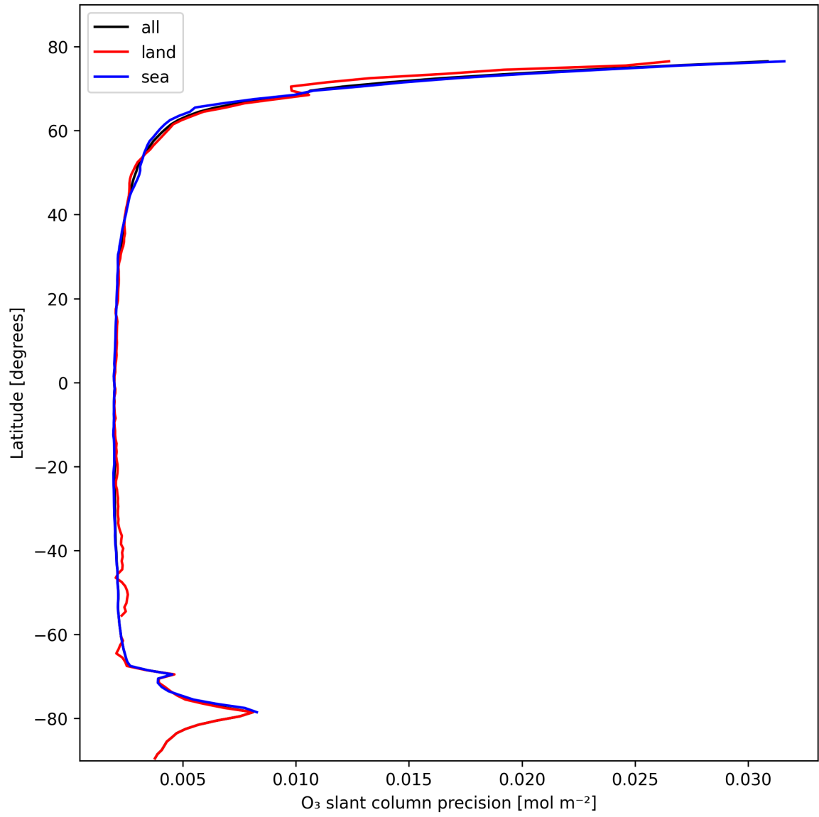
Figure 20: Zonal average of “O 3 slant column precision” for 2025-02-15 to 2025-02-16.
