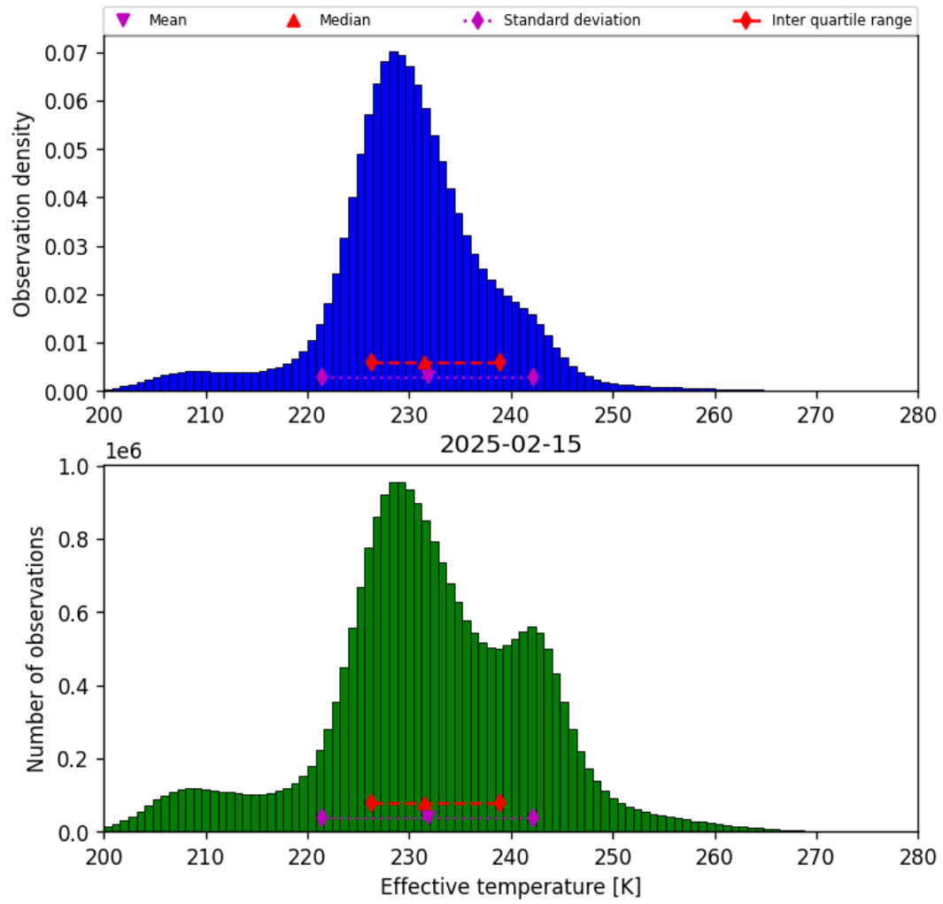
Figure 38: Histogram of “Effective temperature” for 2025-02-15 to 2025-02-16
