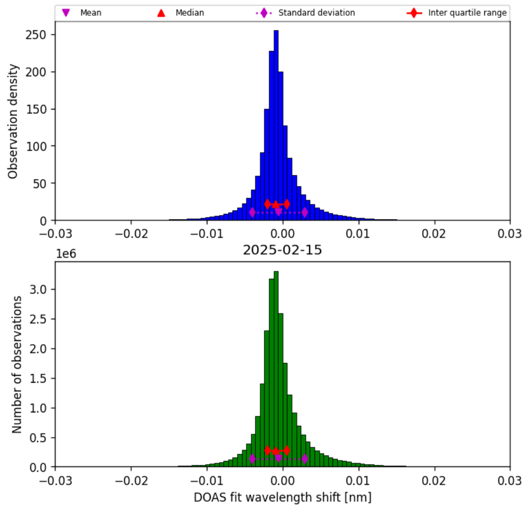
Figure 35: Histogram of “DOAS fit wavelength shift” for 2025-02-15 to 2025-02-16
