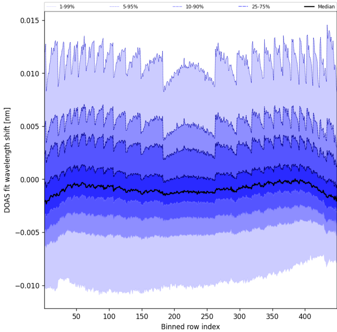
Figure 47: Along track statistics of “DOAS fit wavelength shift” for 2025-02-15 to 2025-02-16
