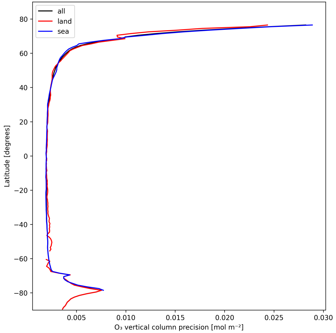
Figure 18: Zonal average of "O 3 vertical column precision" for 2025-02-15 to 2025-02-16.
