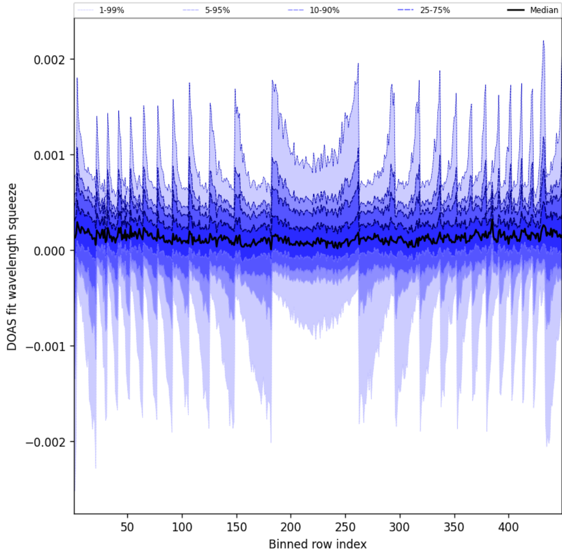
Figure 48: Along track statistics of “DOAS fit wavelength squeeze” for 2025-02-15 to 2025-02-16
