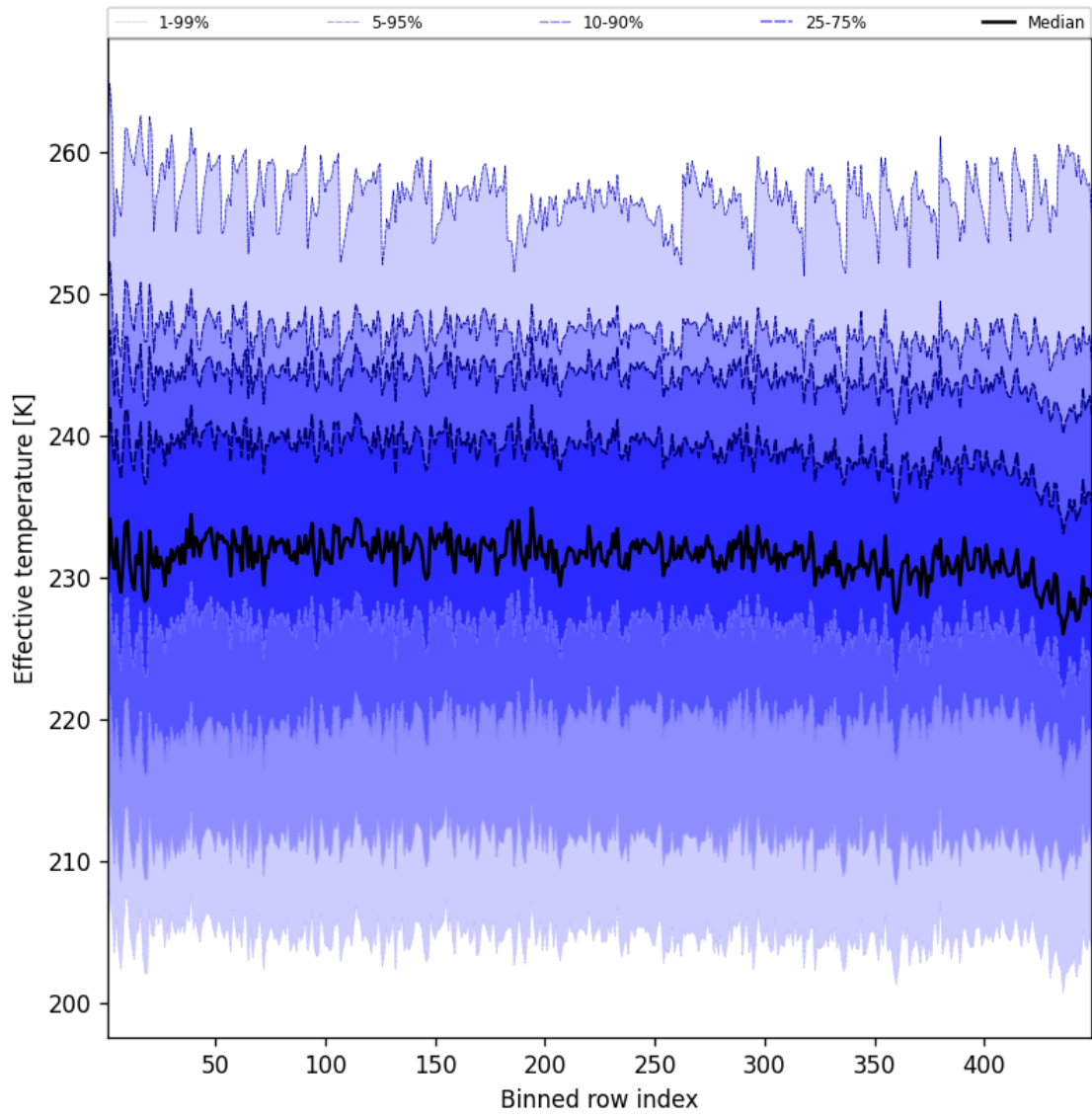
Figure 50: Along track statistics of “Effective temperature” for 2025-02-15 to 2025-02-16
