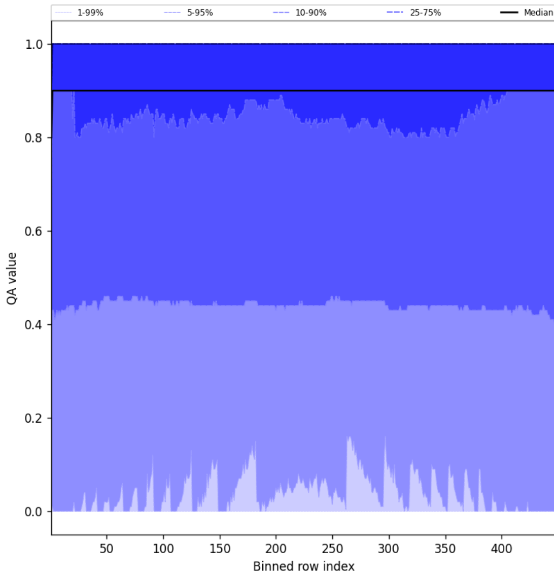
Figure 40: Along track statistics of “QA value” for 2025-02-15 to 2025-02-16
