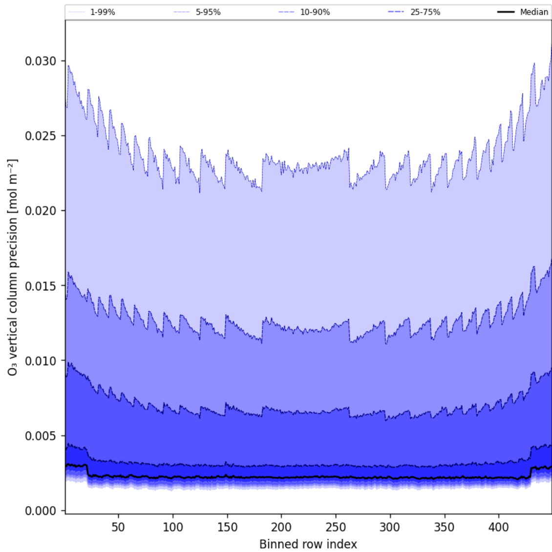
Figure 42: Along track statistics of “O 3 vertical column precision” for 2025-02-15 to 2025-02-16
