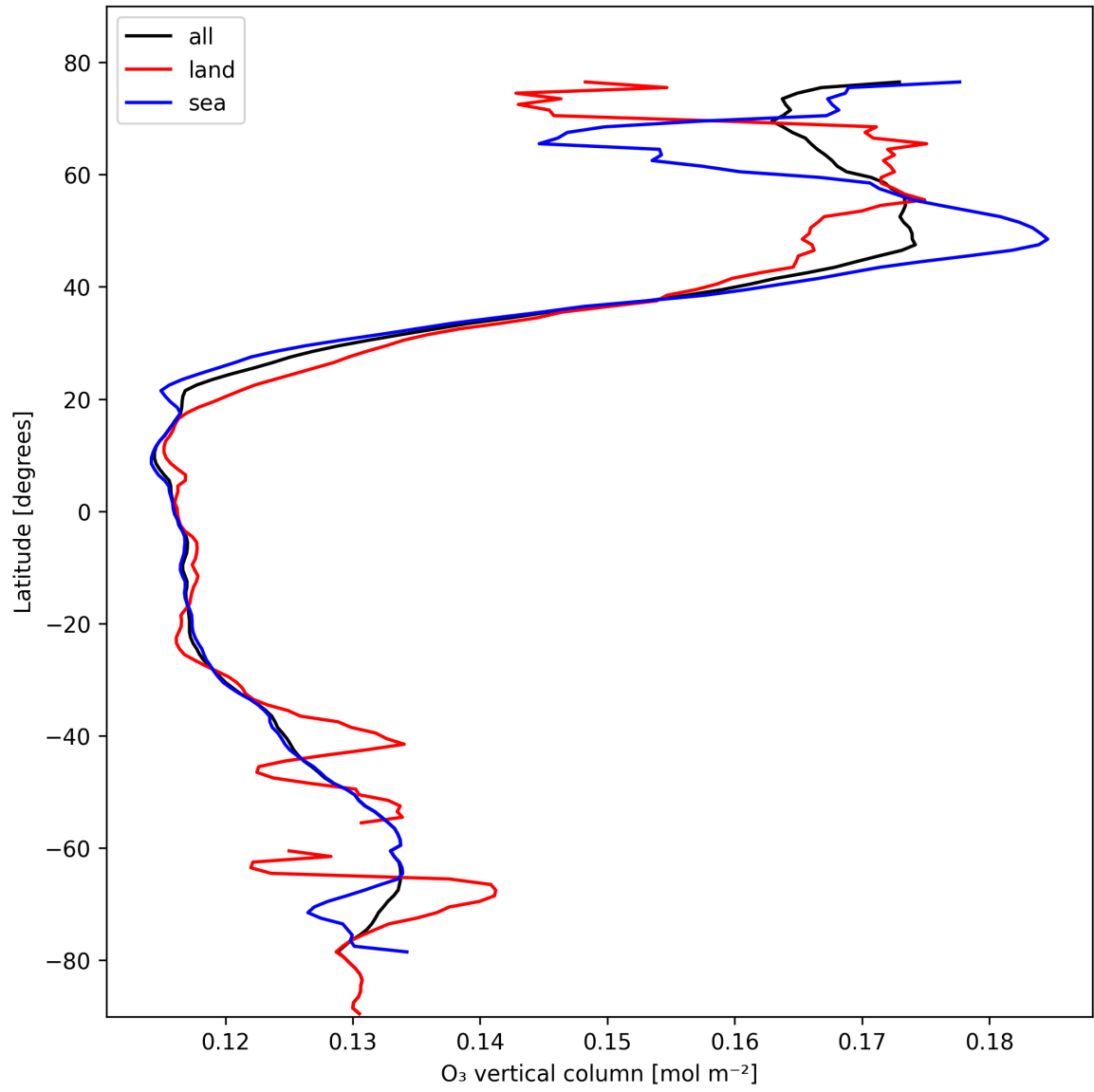
Figure 17: Zonal average of “O 3 vertical column” for 2025-02-15 to 2025-02-16.
