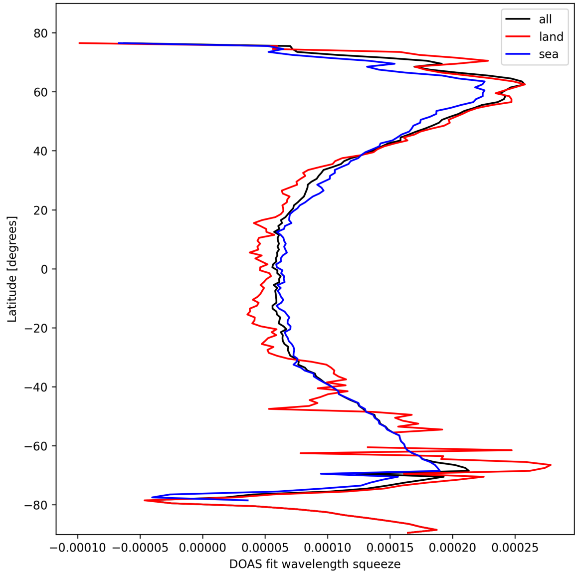
Figure 24: Zonal average of “DOAS fit wavelength squeeze” for 2025-02-15 to 2025-02-16.
