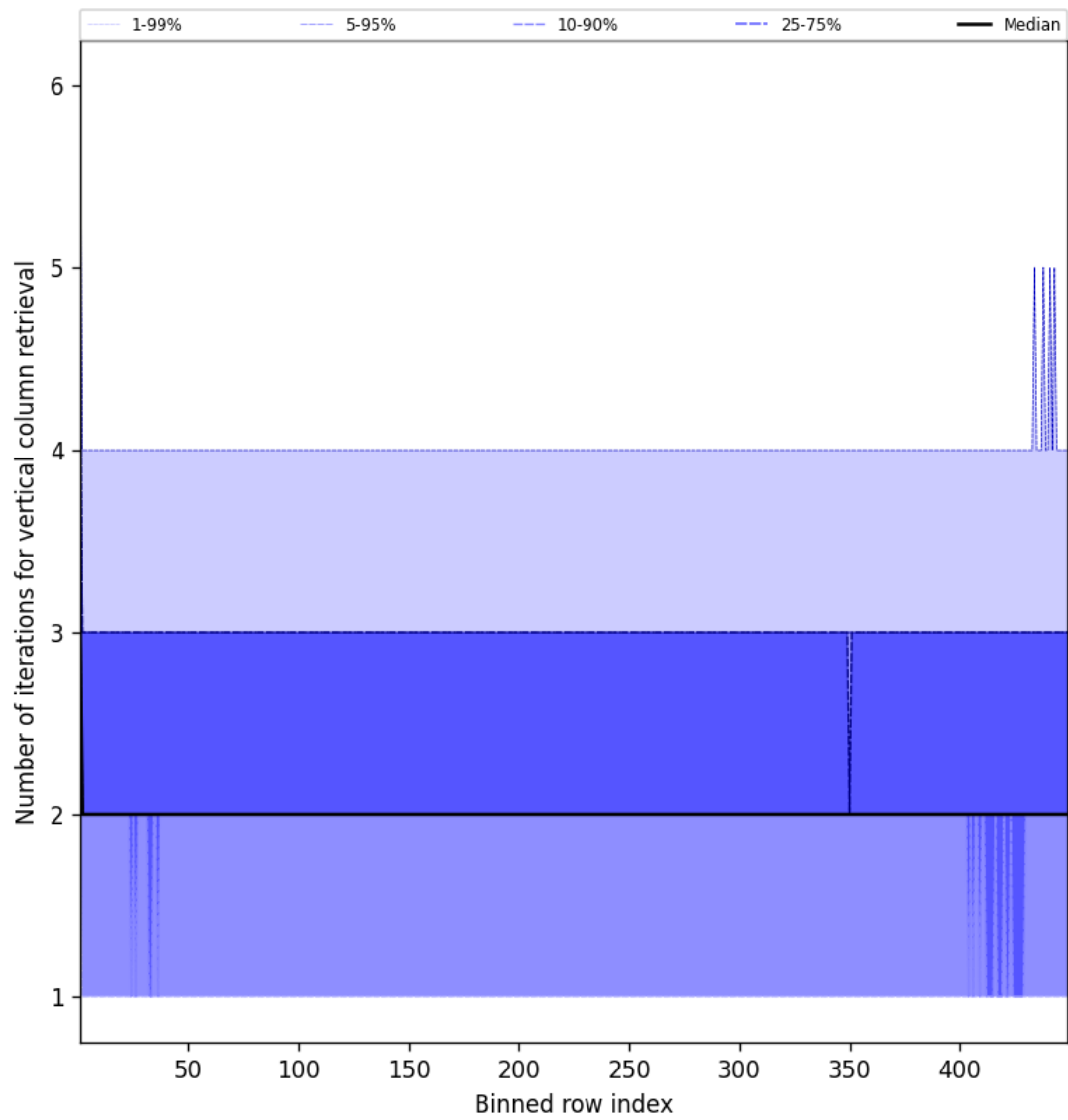
Figure 51: Along track statistics of “Number of iterations for vertical column retrieval” for 2025-02-15 to 2025-02-16
