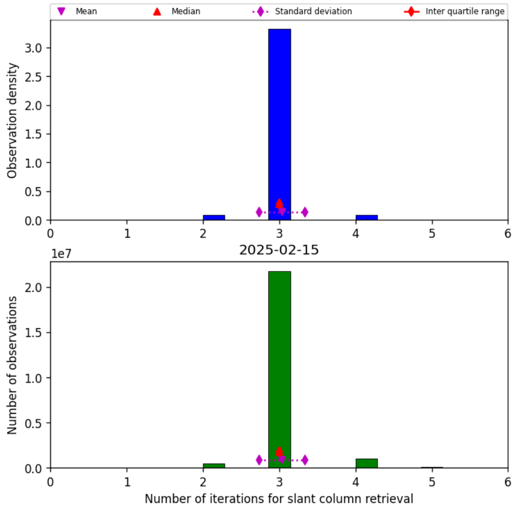
Figure 33: Histogram of “Number of iterations for slant column retrieval” for 2025-02-15 to 2025-02-16
