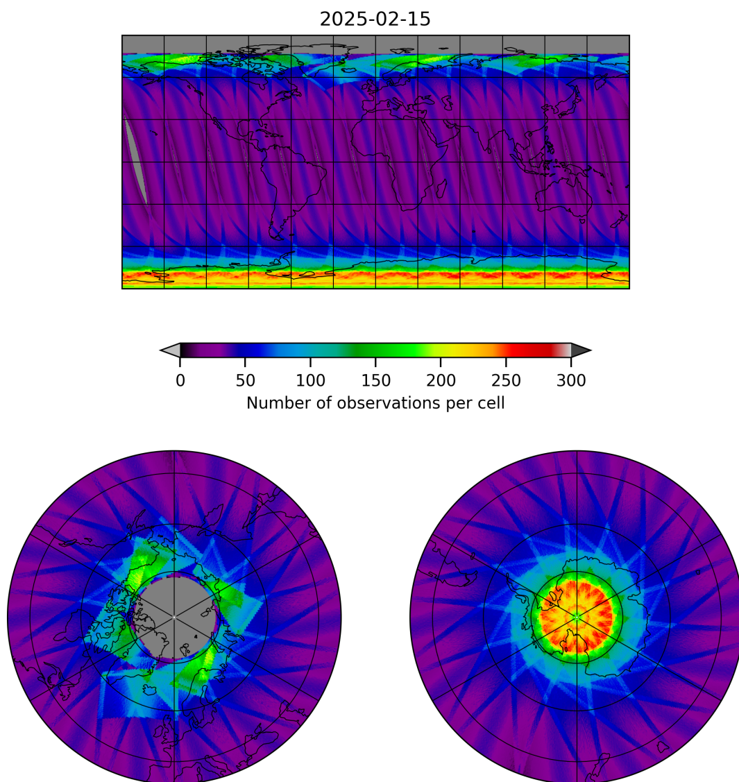
Figure 15: Map of the number of observations for 2025-02-15 to 2025-02-16
