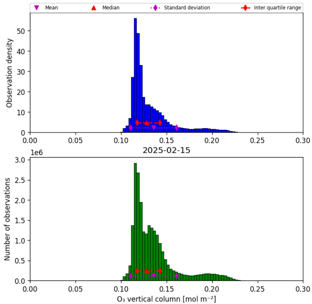
Figure 29: Histogram of “O 3 vertical column” for 2025-02-15 to 2025-02-16
