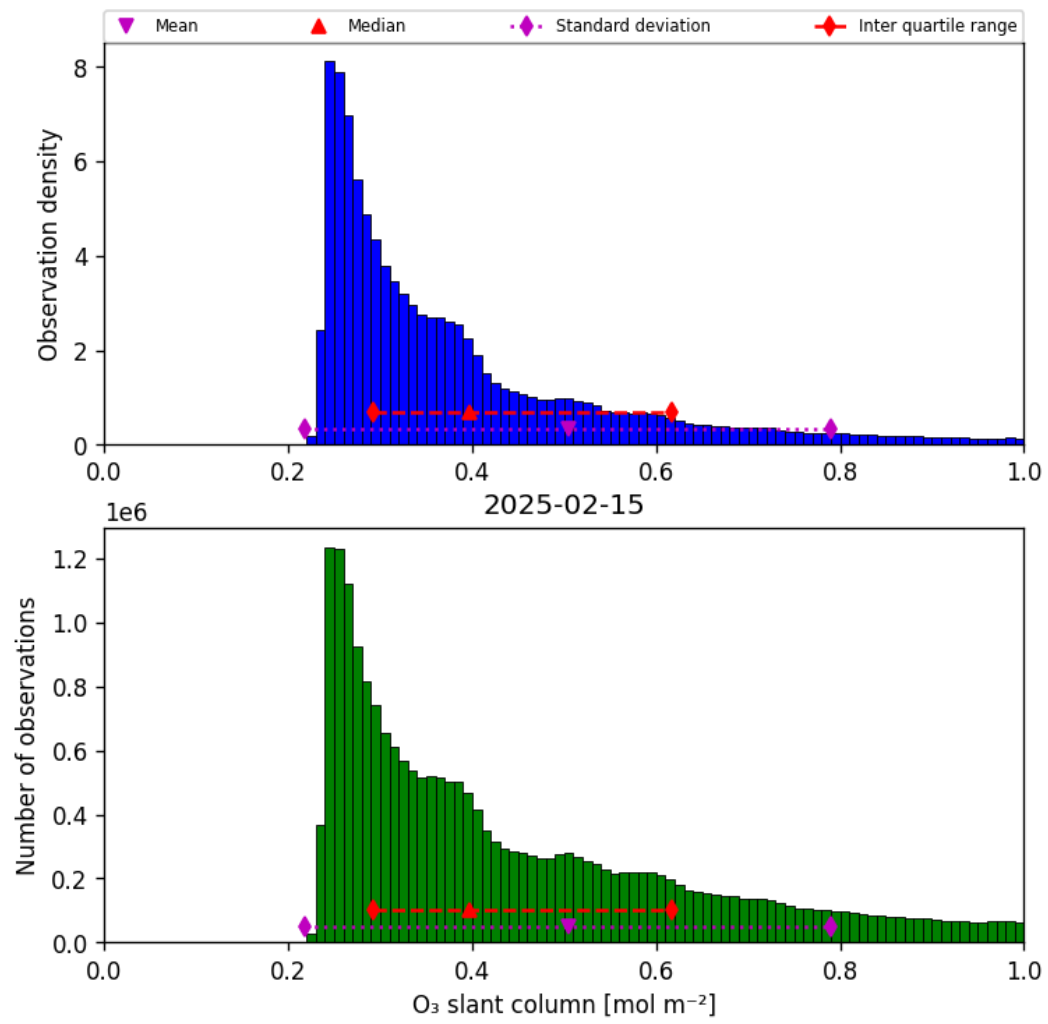
Figure 31: Histogram of “O 3 slant column” for 2025-02-15 to 2025-02-16
