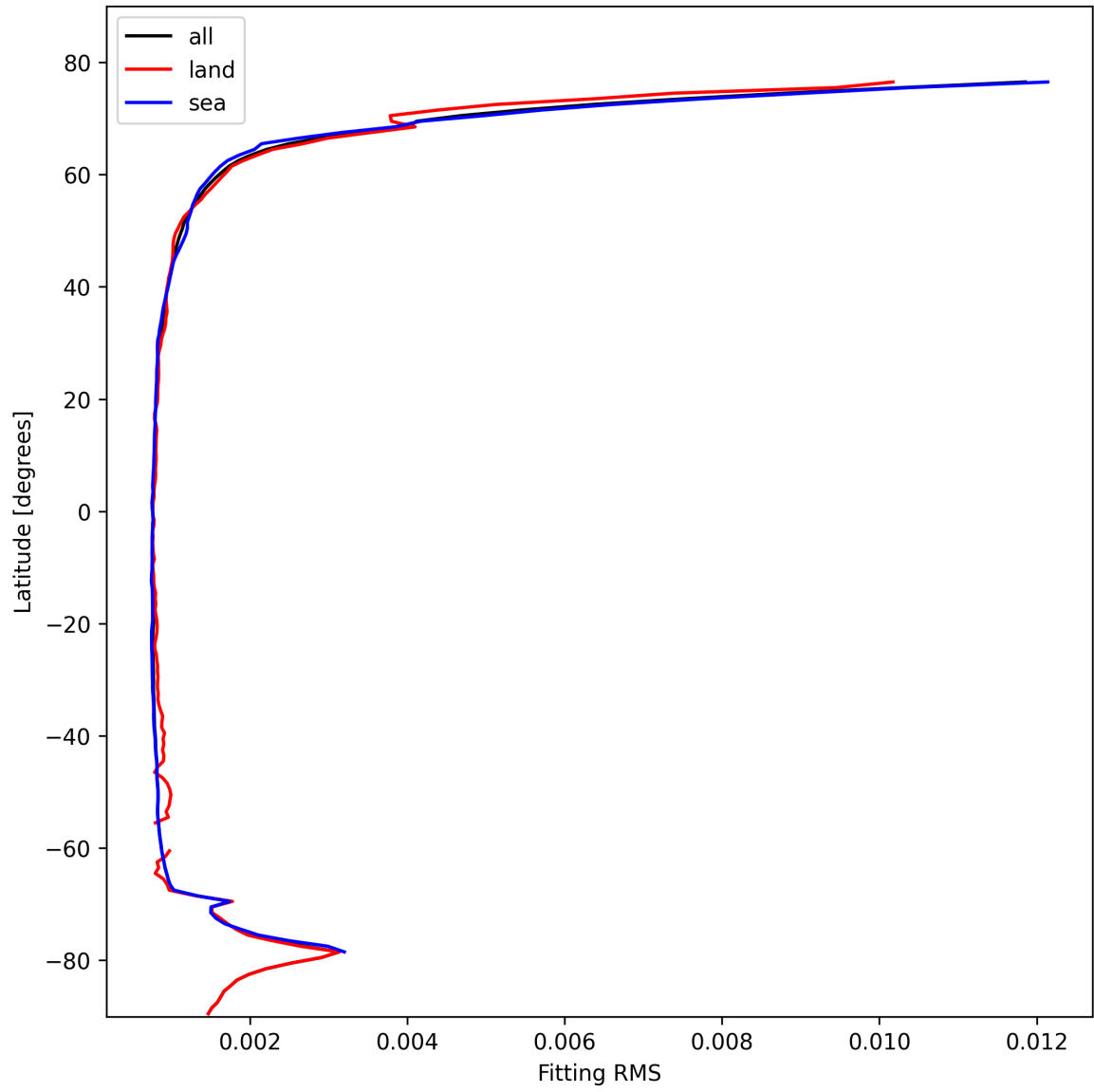
Figure 22: Zonal average of “Fitting RMS” for 2025-02-15 to 2025-02-16.
