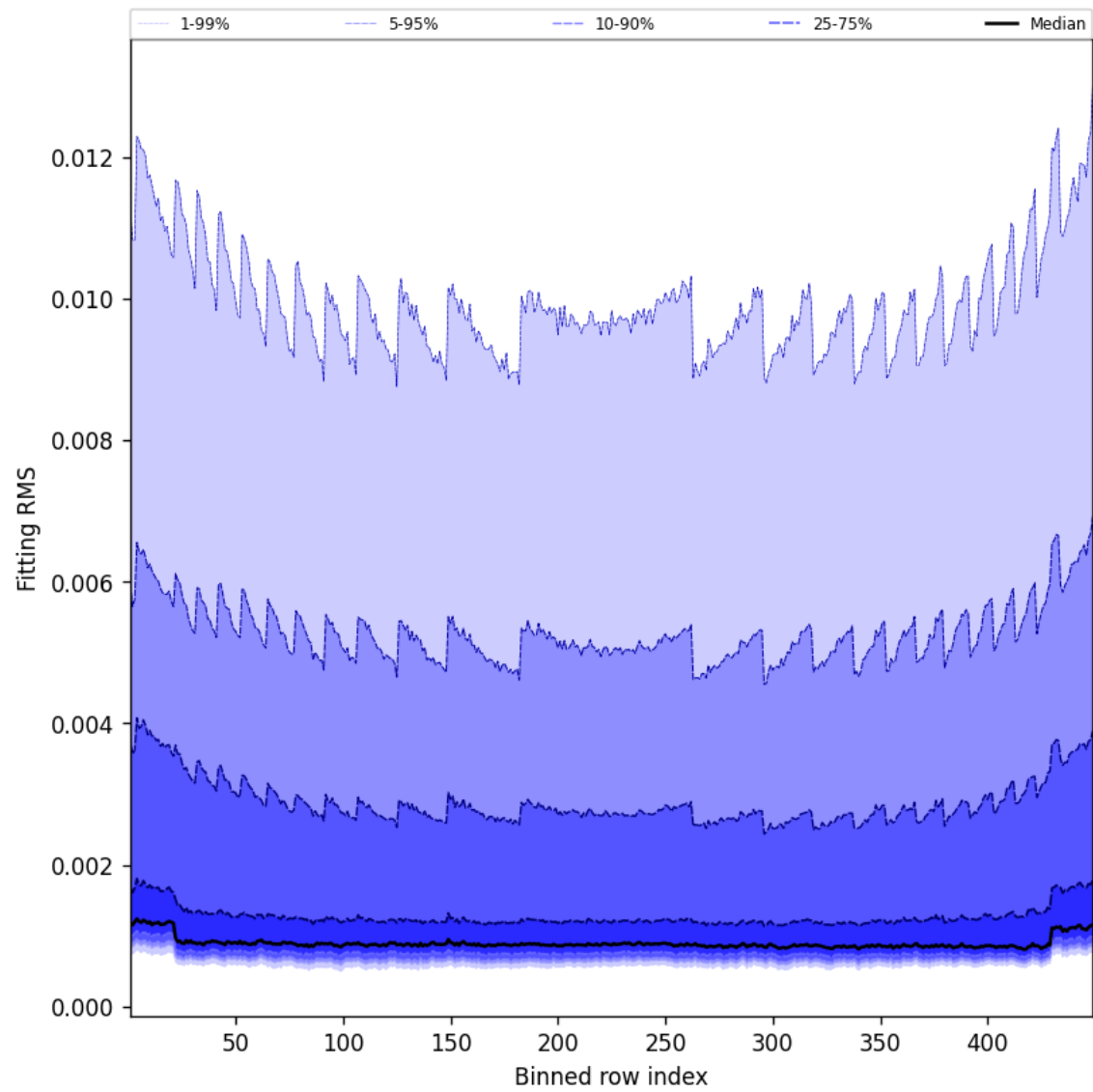
Figure 46: Along track statistics of “Fitting RMS” for 2025-02-15 to 2025-02-16
