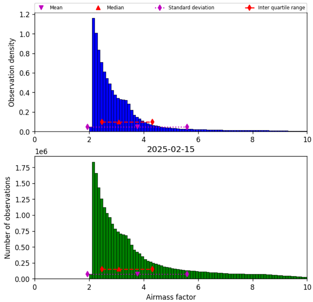
Figure 37: Histogram of “Airmass factor” for 2025-02-15 to 2025-02-16
