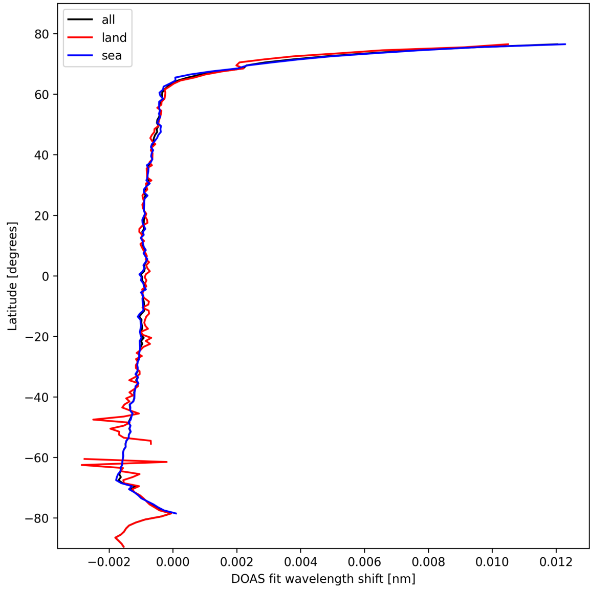
Figure 23: Zonal average of “DOAS fit wavelength shift” for 2025-02-15 to 2025-02-16.
