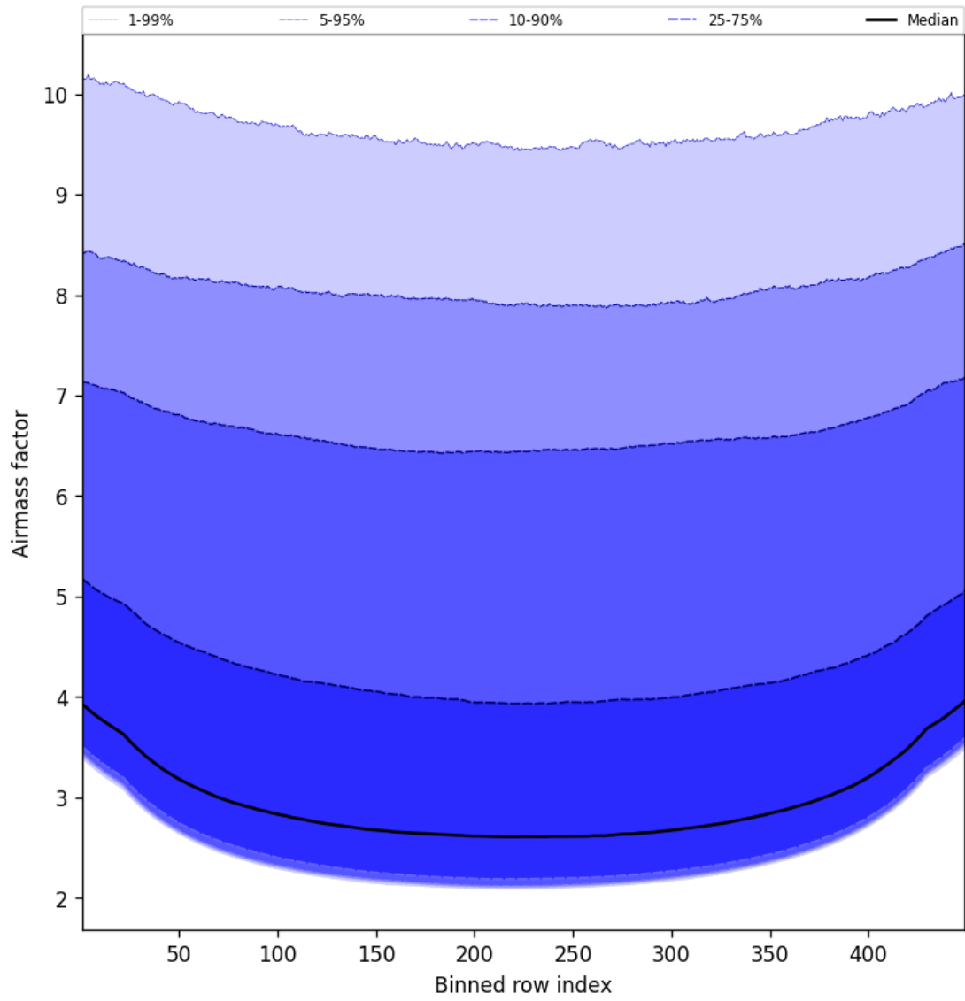
Figure 49: Along track statistics of “Airmass factor” for 2025-02-15 to 2025-02-16
