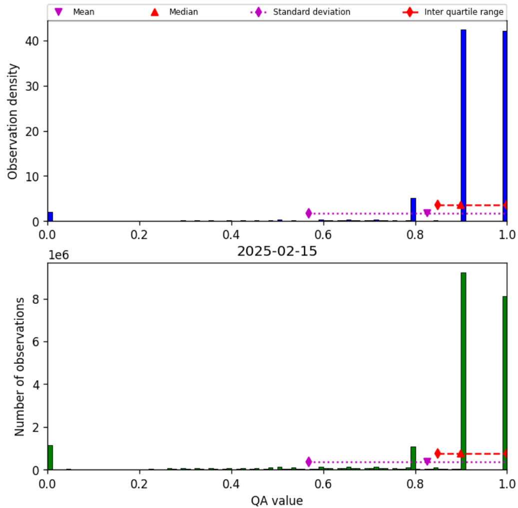
Figure 28: Histogram of “QA value” for 2025-02-15 to 2025-02-16
