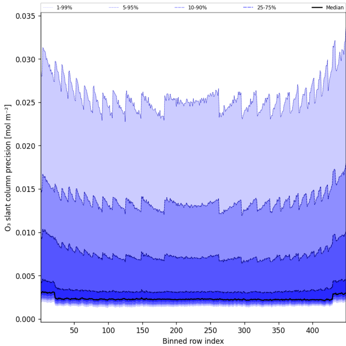
Figure 44: Along track statistics of “O 3 slant column precision” for 2025-02-15 to 2025-02-16
