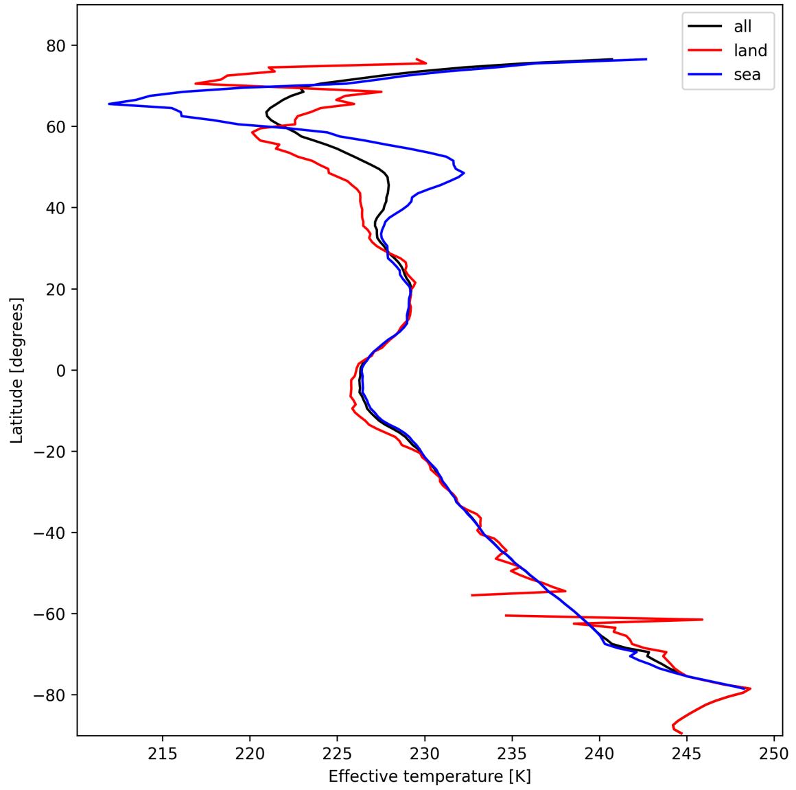
Figure 26: Zonal average of “Effective temperature” for 2025-02-15 to 2025-02-16.
