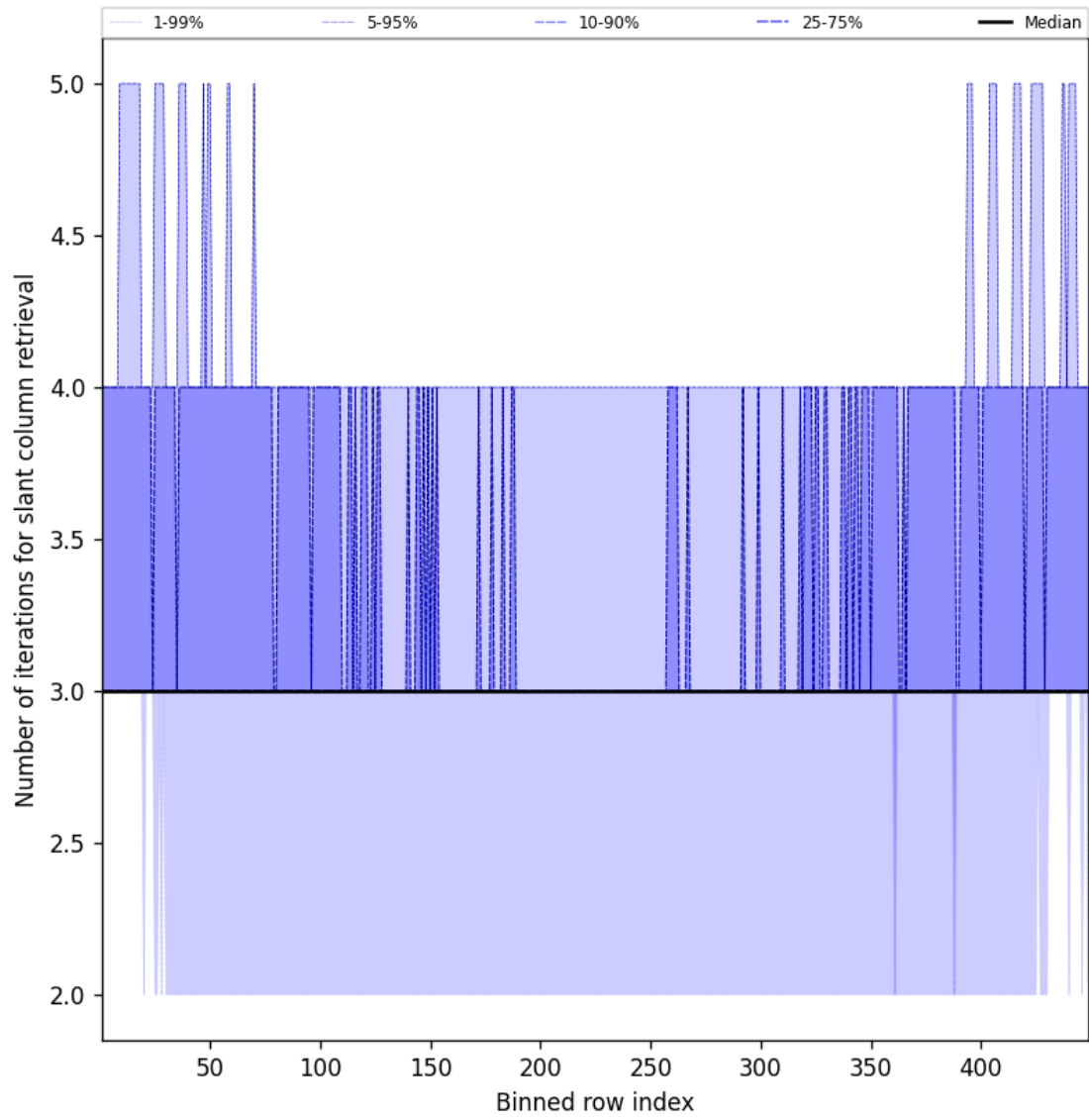
Figure 45: Along track statistics of “Number of iterations for slant column retrieval” for 2025-02-15 to 2025-02-16
