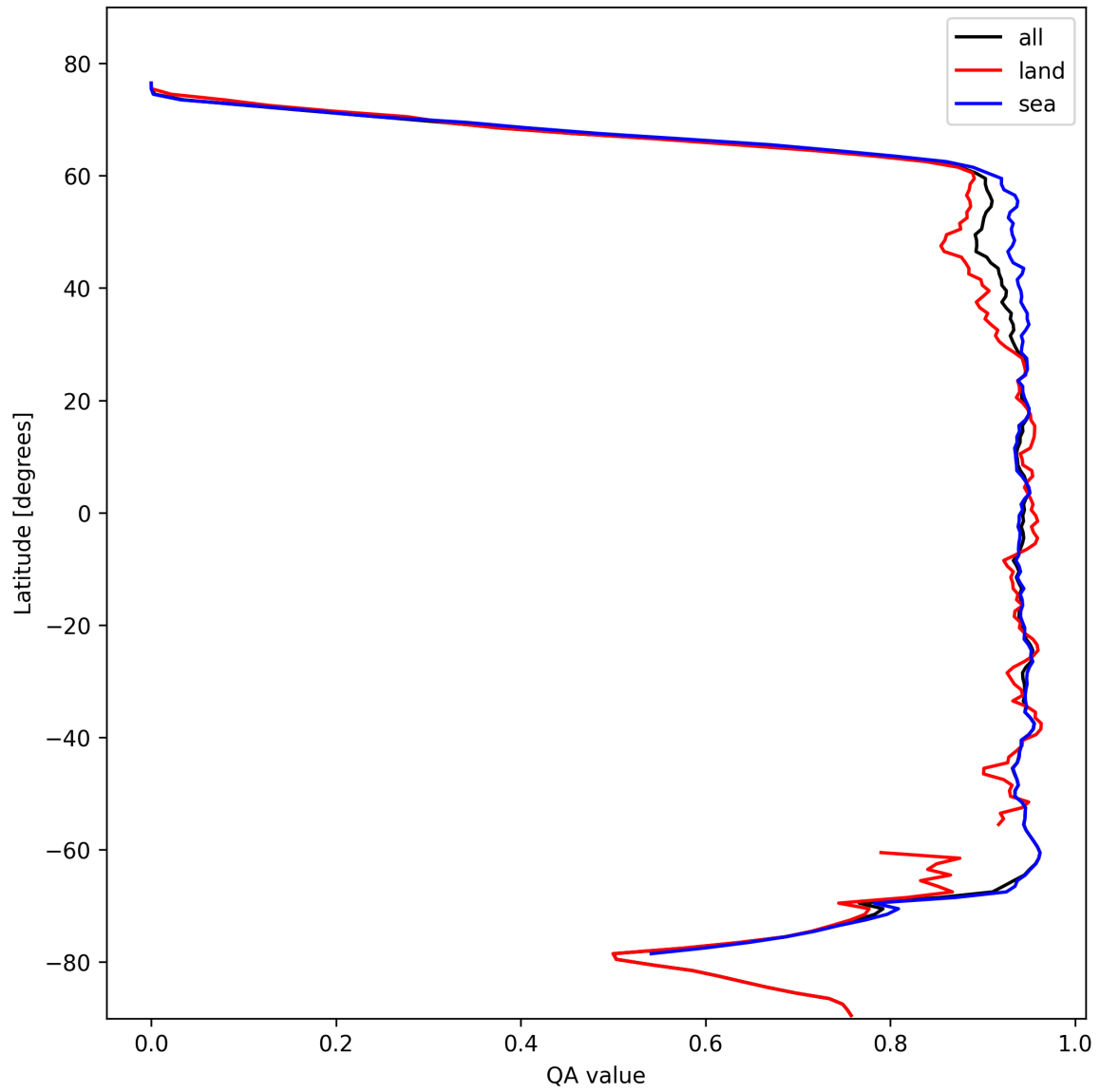
Figure 16: Zonal average of “QA value” for 2025-02-15 to 2025-02-16.
