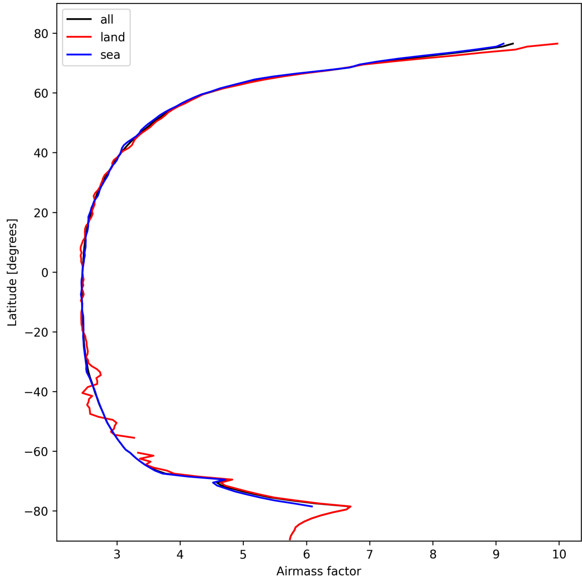
Figure 25: Zonal average of “Airmass factor” for 2025-02-15 to 2025-02-16.
