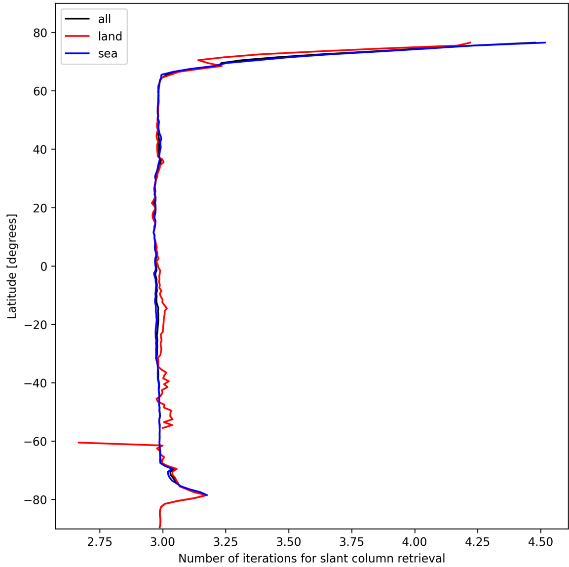
Figure 21: Zonal average of “Number of iterations for slant column retrieval” for 2025-02-15 to 2025-02-16.
