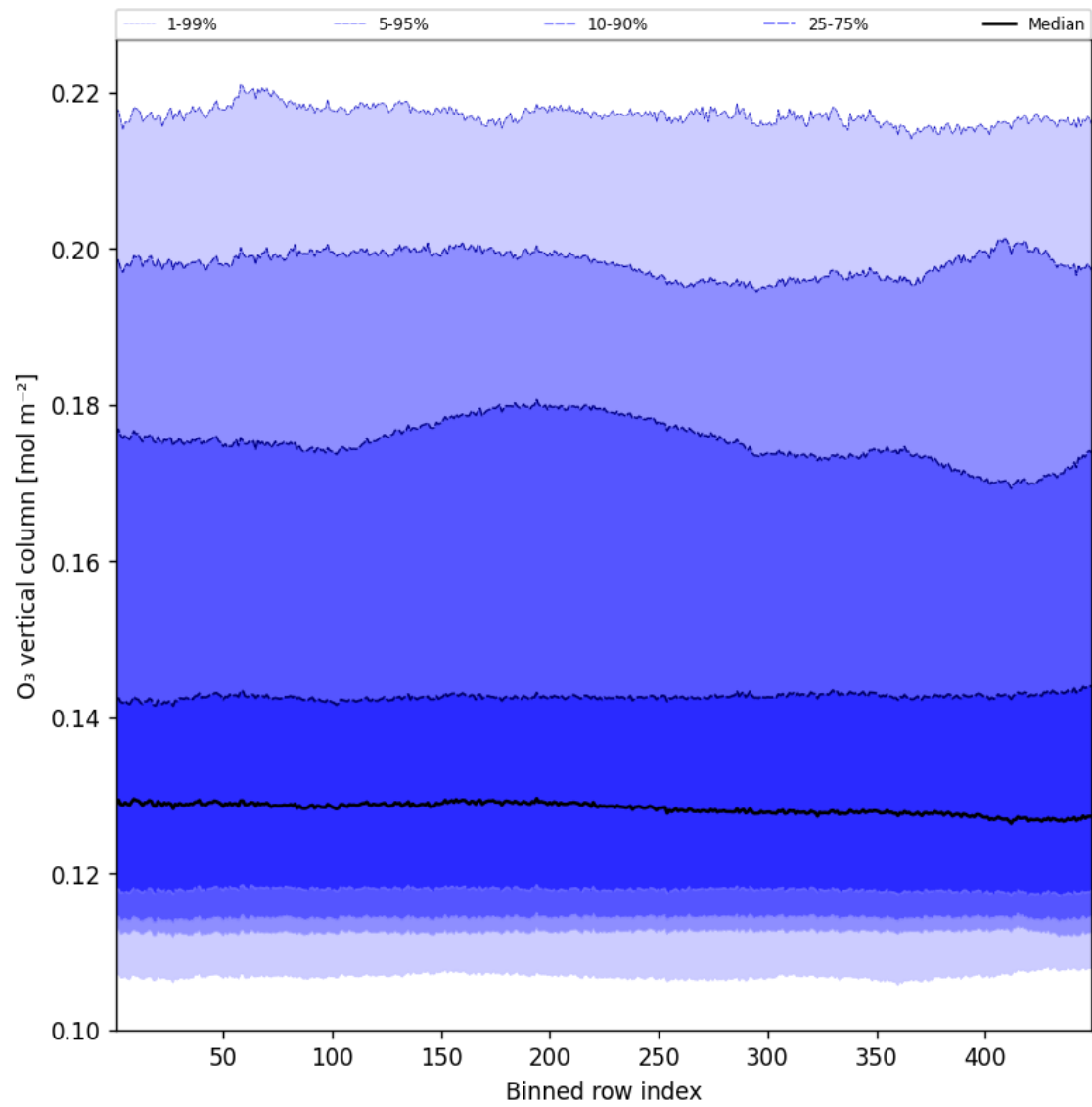
Figure 41: Along track statistics of “O 3 vertical column” for 2025-02-15 to 2025-02-16
