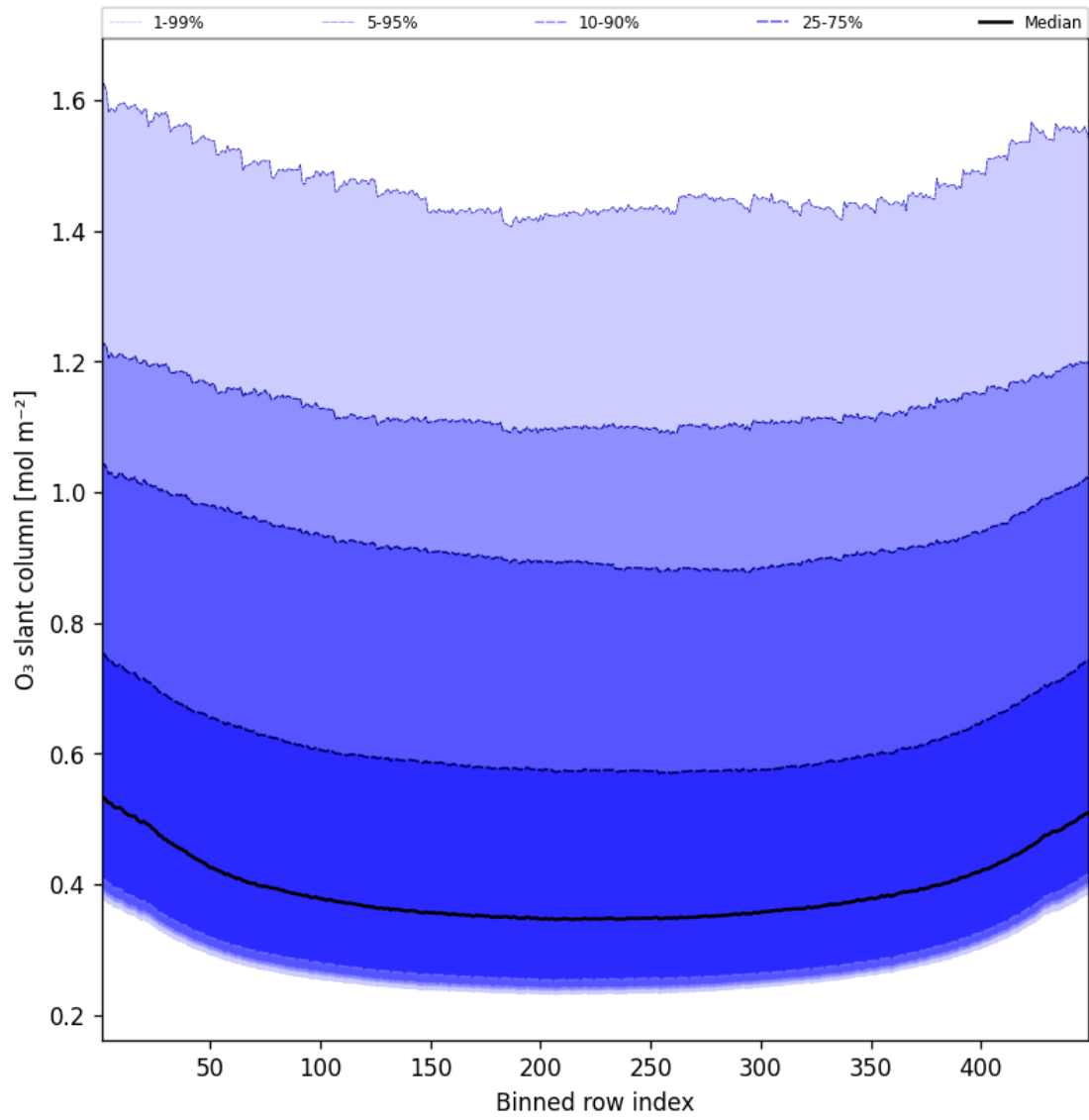
Figure 43: Along track statistics of “O 3 slant column” for 2025-02-15 to 2025-02-16
