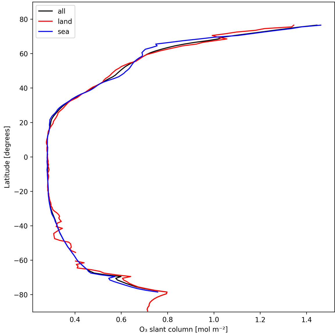
Figure 19: Zonal average of “O 3 slant column” for 2025-02-15 to 2025-02-16.
