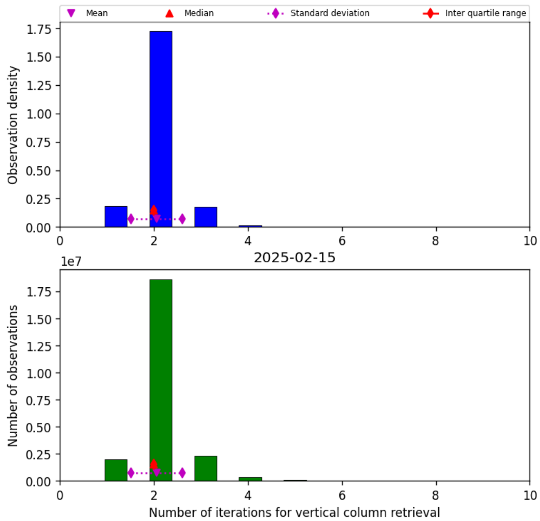
Figure 39: Histogram of “Number of iterations for vertical column retrieval” for 2025-02-15 to 2025-02-16
