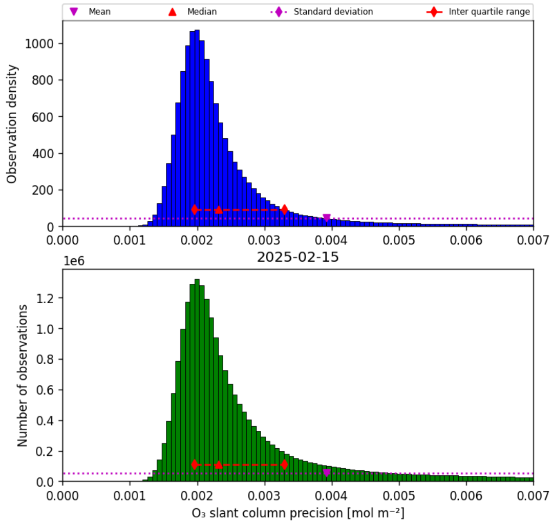
Figure 32: Histogram of “O 3 slant column precision” for 2025-02-15 to 2025-02-16
