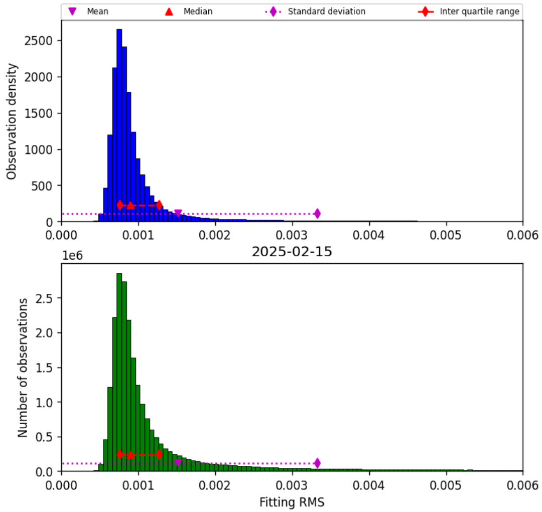
Figure 34: Histogram of “Fitting RMS” for 2025-02-15 to 2025-02-16
