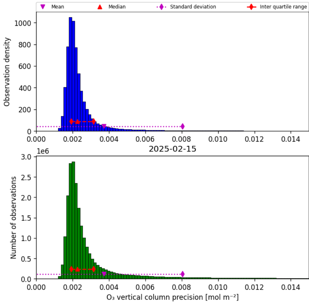
Figure 30: Histogram of “O 3 vertical column precision” for 2025-02-15 to 2025-02-16
