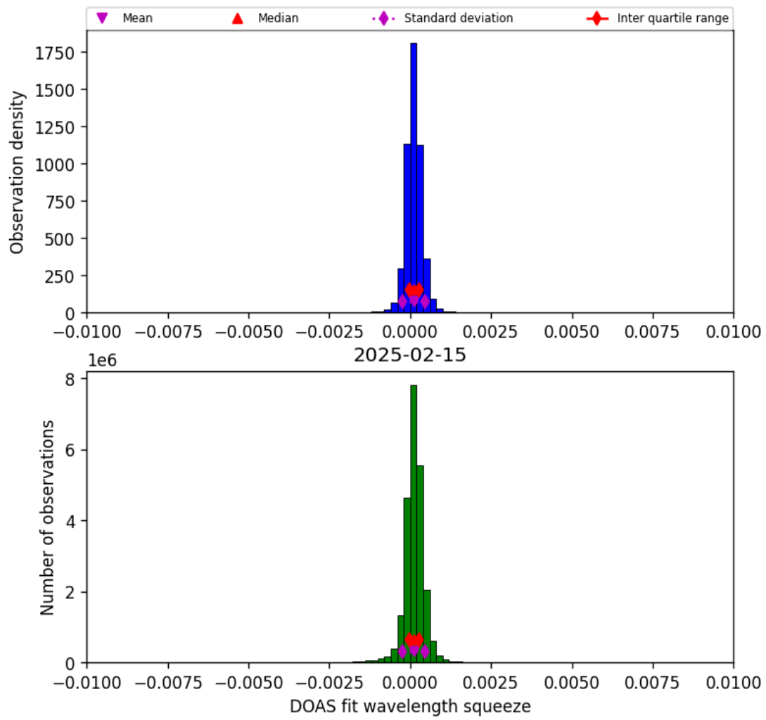
Figure 36: Histogram of “DOAS fit wavelength squeeze” for 2025-02-15 to 2025-02-16
