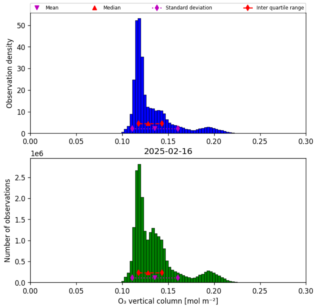
Figure 29: Histogram of “O 3 vertical column” for 2025-02-16 to 2025-02-16
