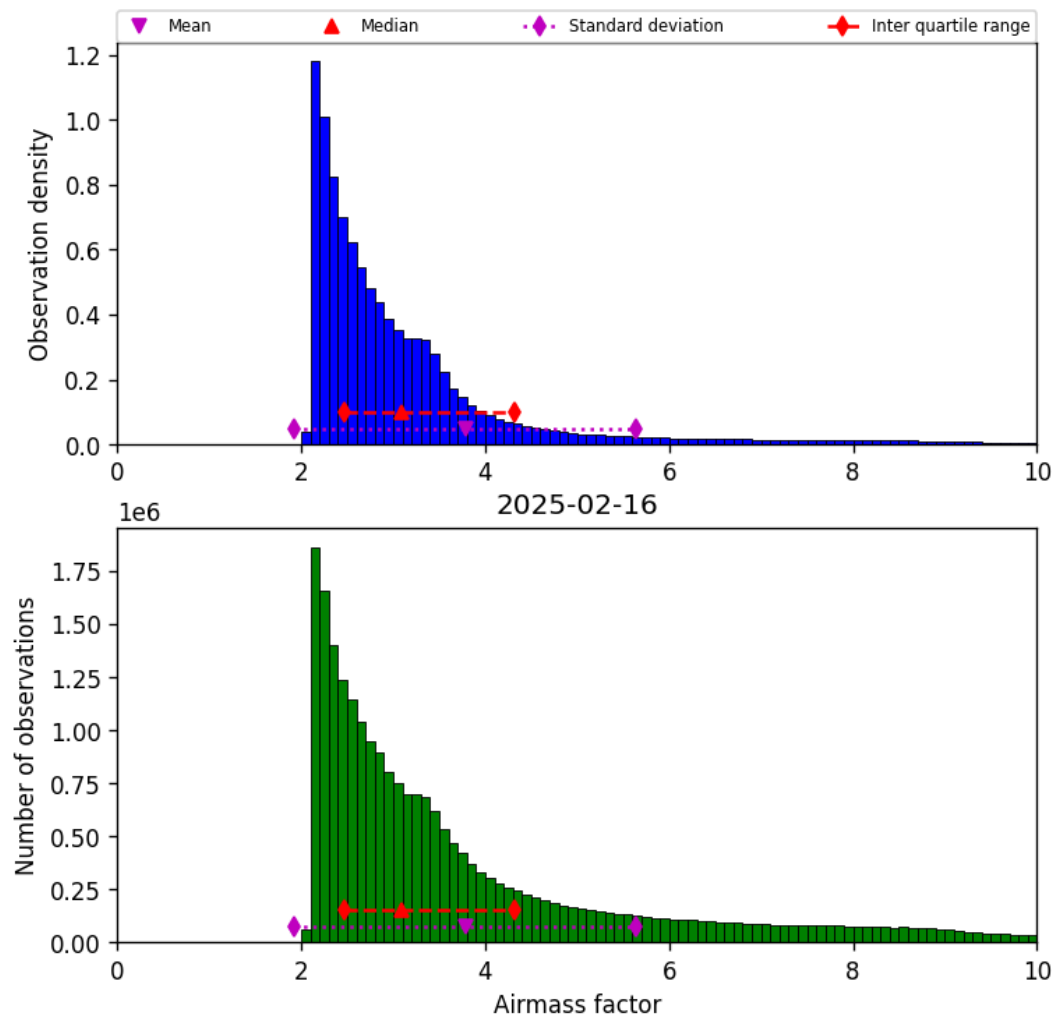
Figure 37: Histogram of “Airmass factor” for 2025-02-16 to 2025-02-16
