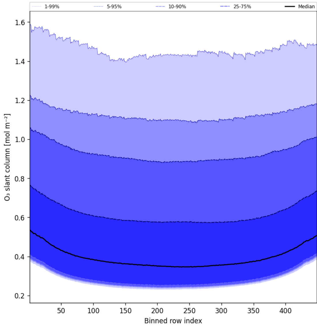
Figure 43: Along track statistics of "O 3 slant column" for 2025-02-16 to 2025-02-16
