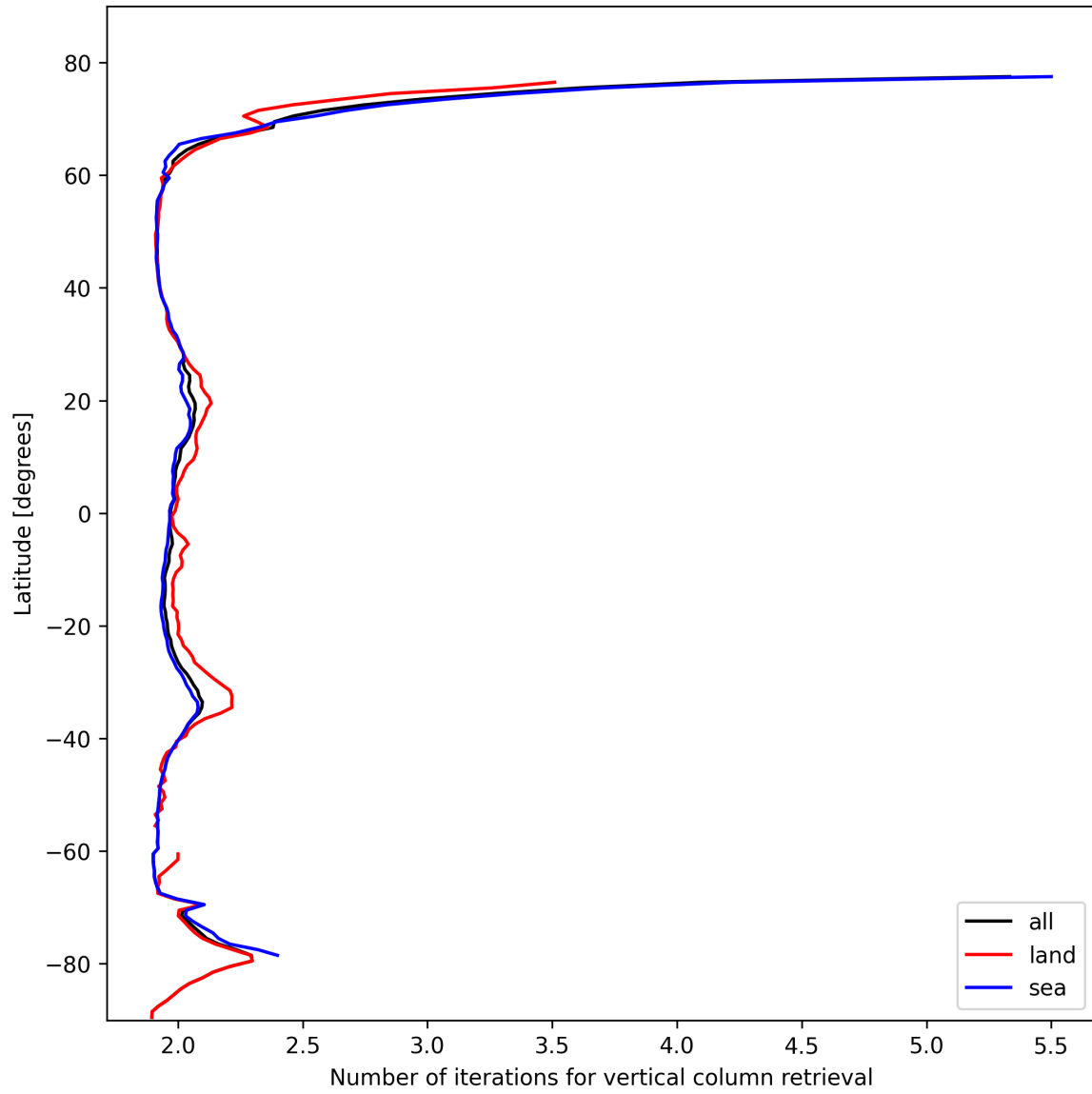
Figure 27: Zonal average of “Number of iterations for vertical column retrieval” for 2025-02-16 to 2025-02-16.
