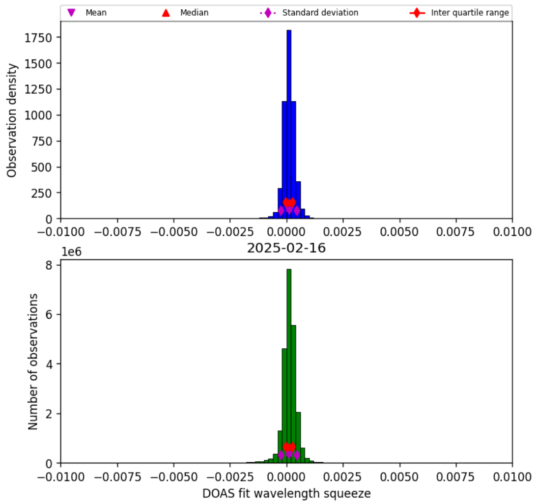
Figure 36: Histogram of “DOAS fit wavelength squeeze” for 2025-02-16 to 2025-02-16
