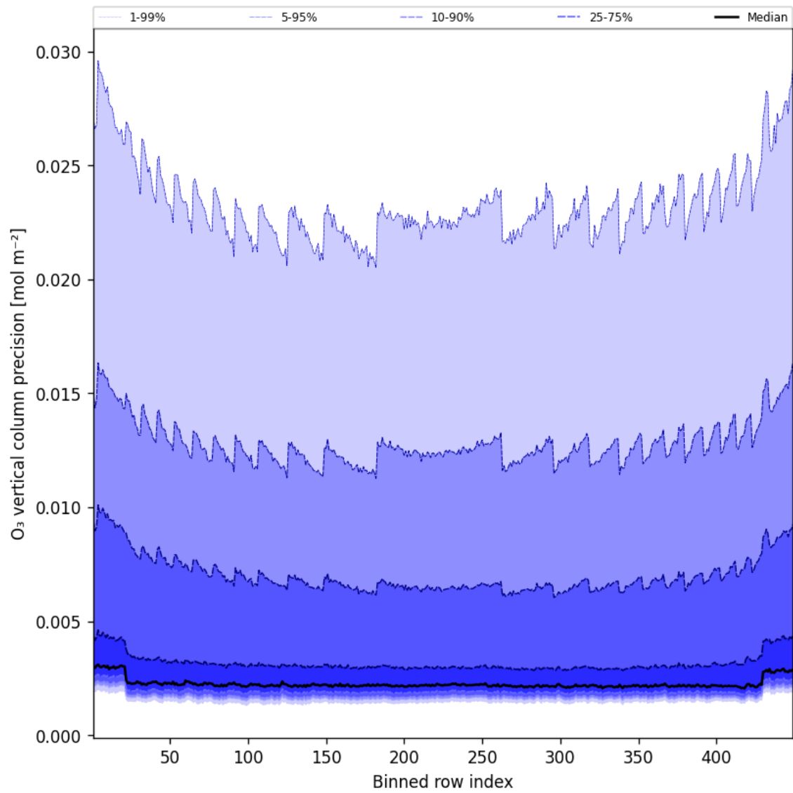
Figure 42: Along track statistics of “O 3 vertical column precision” for 2025-02-16 to 2025-02-16
