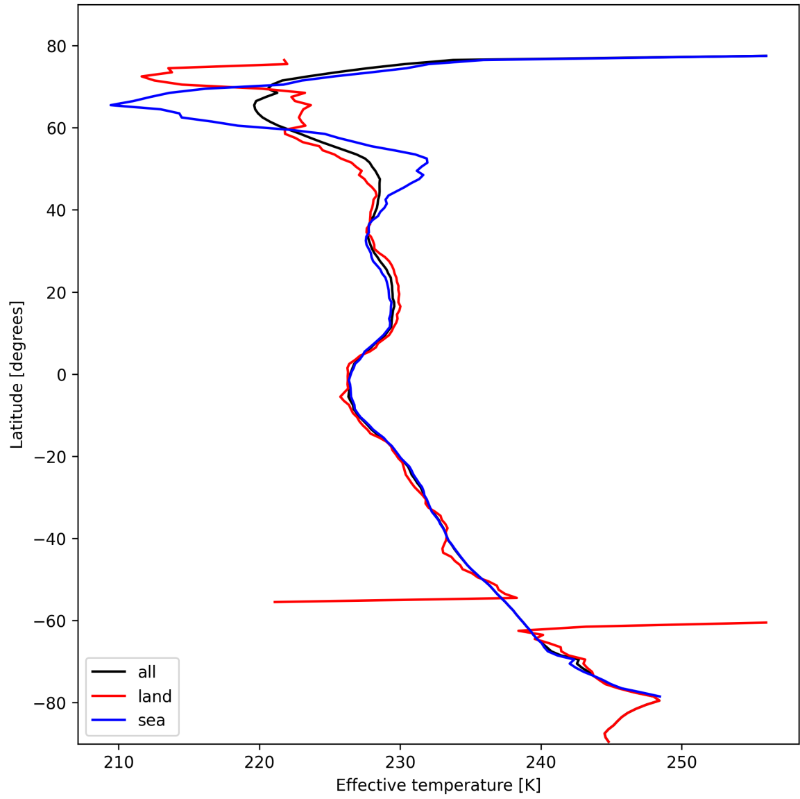
Figure 26: Zonal average of “Effective temperature” for 2025-02-16 to 2025-02-16.
