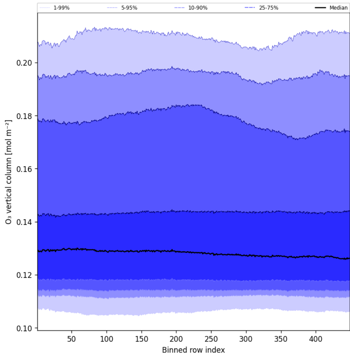
Figure 41: Along track statistics of “O 3 vertical column” for 2025-02-16 to 2025-02-16
