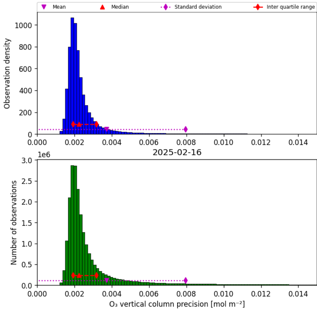
Figure 30: Histogram of “O 3 vertical column precision” for 2025-02-16 to 2025-02-16
