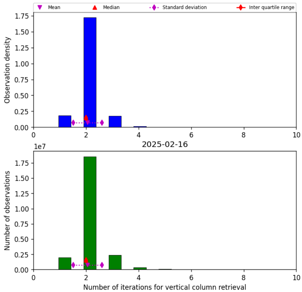
Figure 39: Histogram of “Number of iterations for vertical column retrieval” for 2025-02-16 to 2025-02-16
