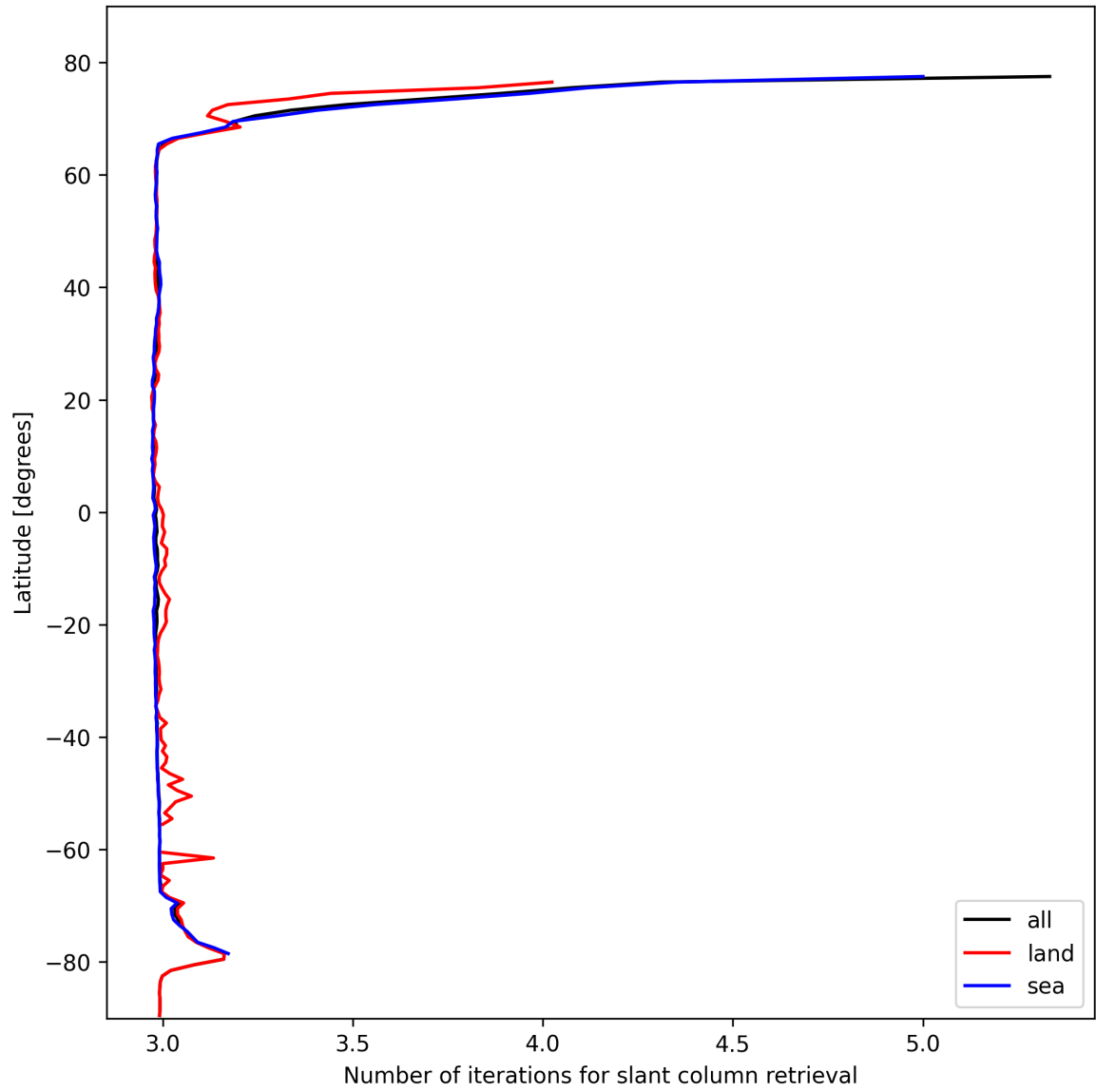
Figure 21: Zonal average of “Number of iterations for slant column retrieval” for 2025-02-16 to 2025-02-16.
