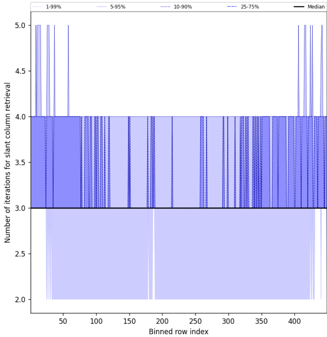
Figure 45: Along track statistics of “Number of iterations for slant column retrieval” for 2025-02-16 to 2025-02-16
