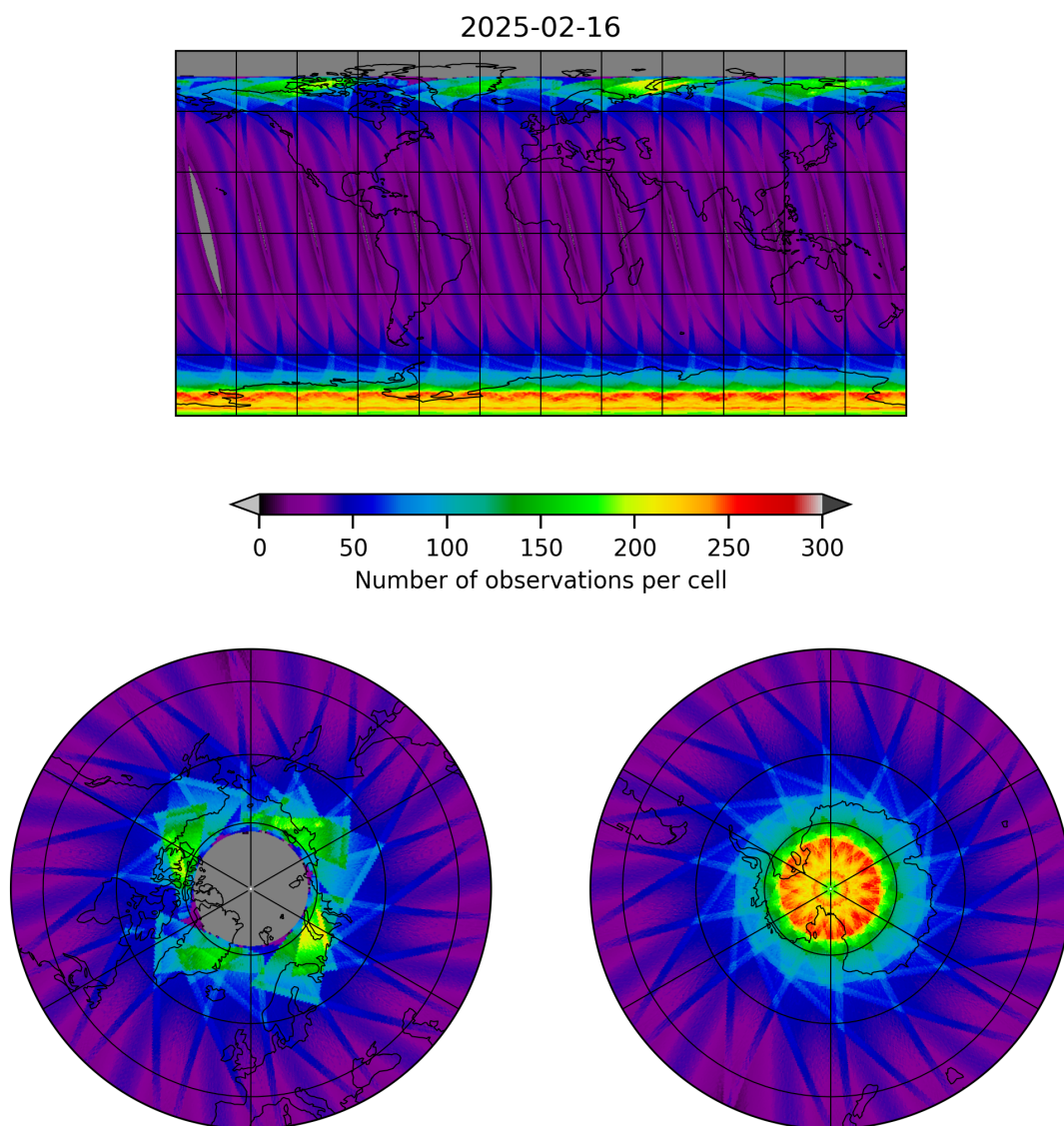
Figure 15: Map of the number of observations for 2025-02-16 to 2025-02-16
