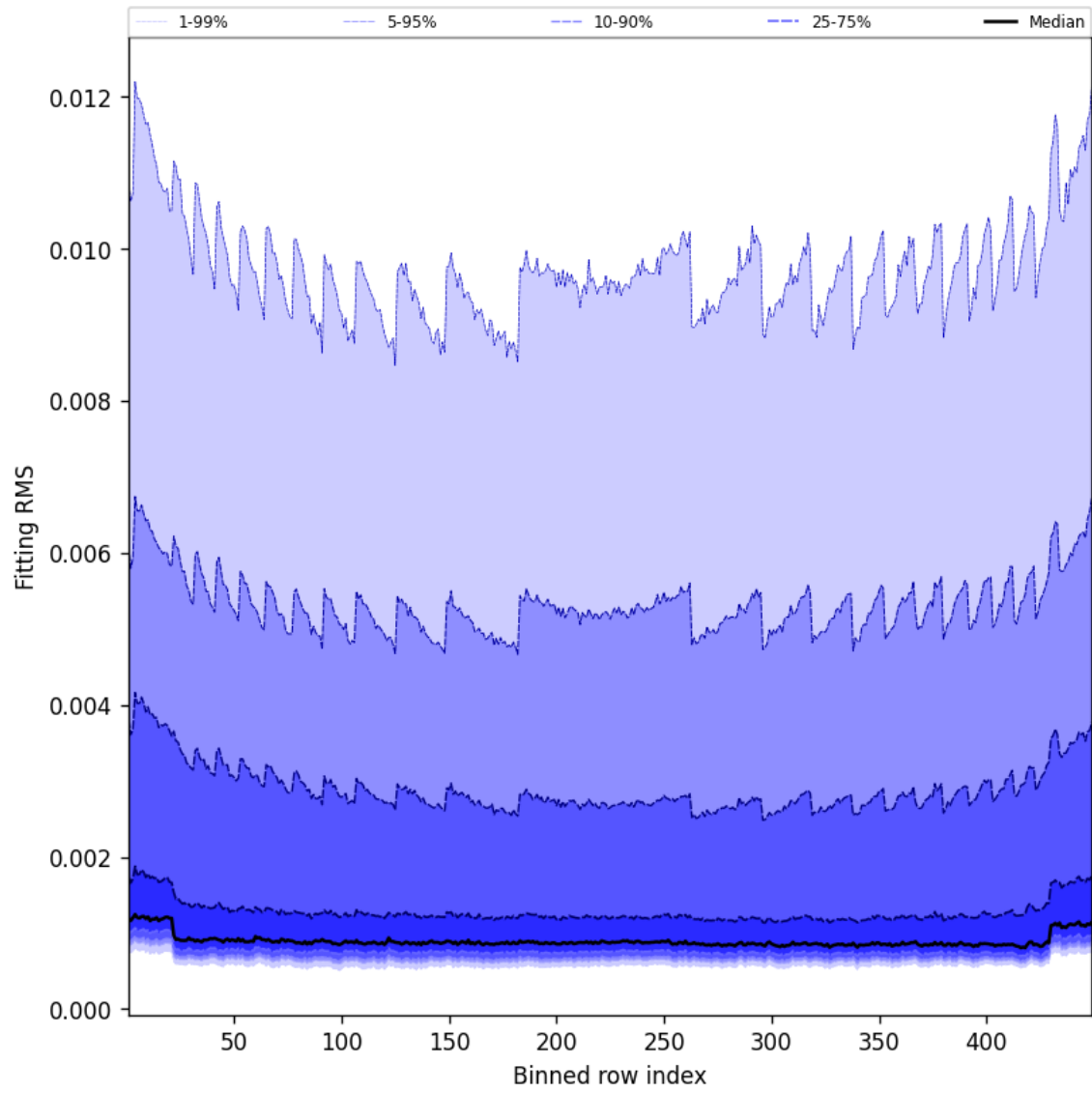
Figure 46: Along track statistics of “Fitting RMS” for 2025-02-16 to 2025-02-16
