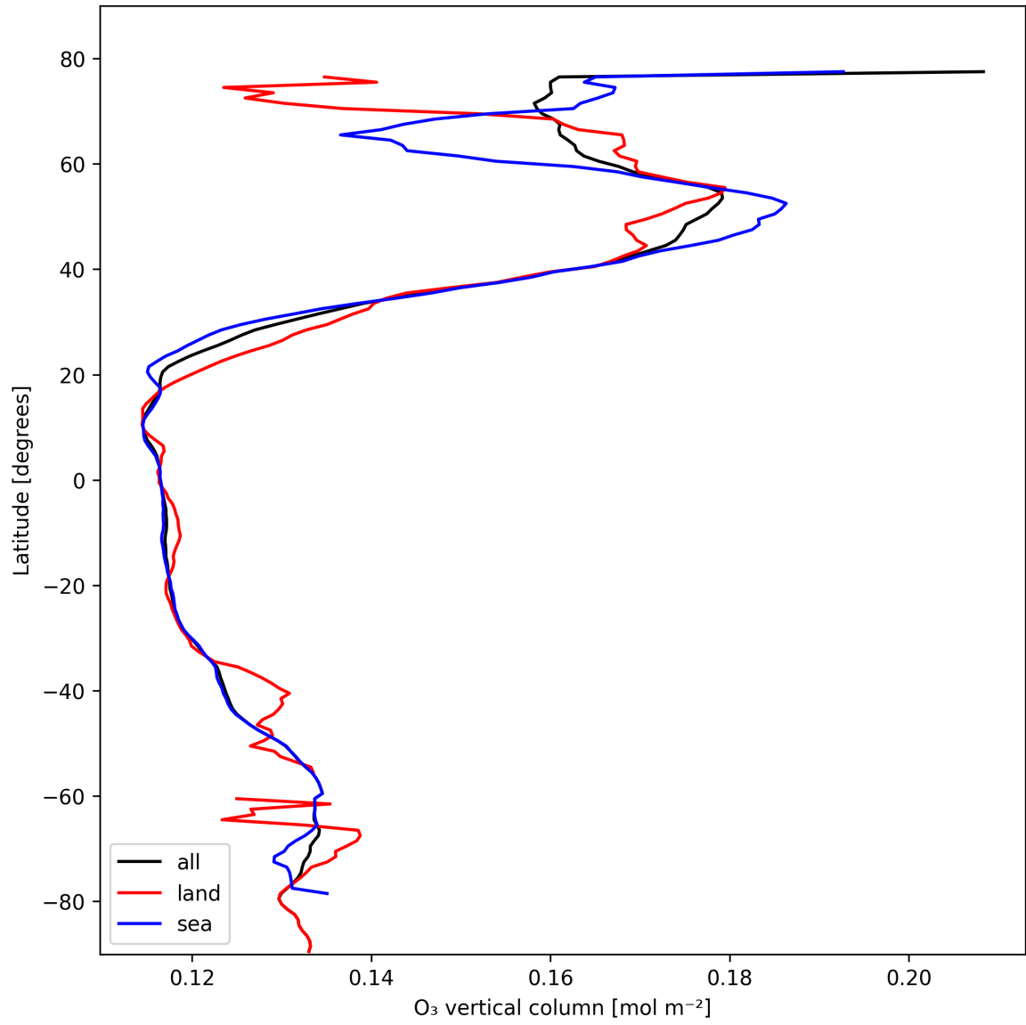
Figure 17: Zonal average of “O 3 vertical column” for 2025-02-16 to 2025-02-16.
