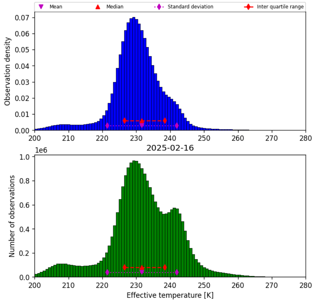
Figure 38: Histogram of “Effective temperature” for 2025-02-16 to 2025-02-16
