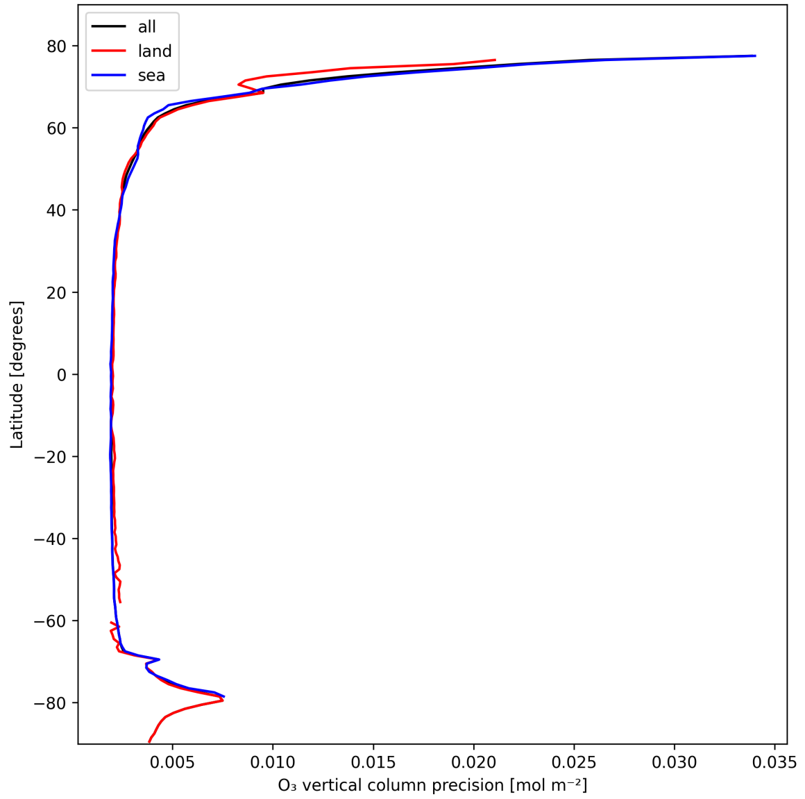
Figure 18: Zonal average of “O 3 vertical column precision” for 2025-02-16 to 2025-02-16.
