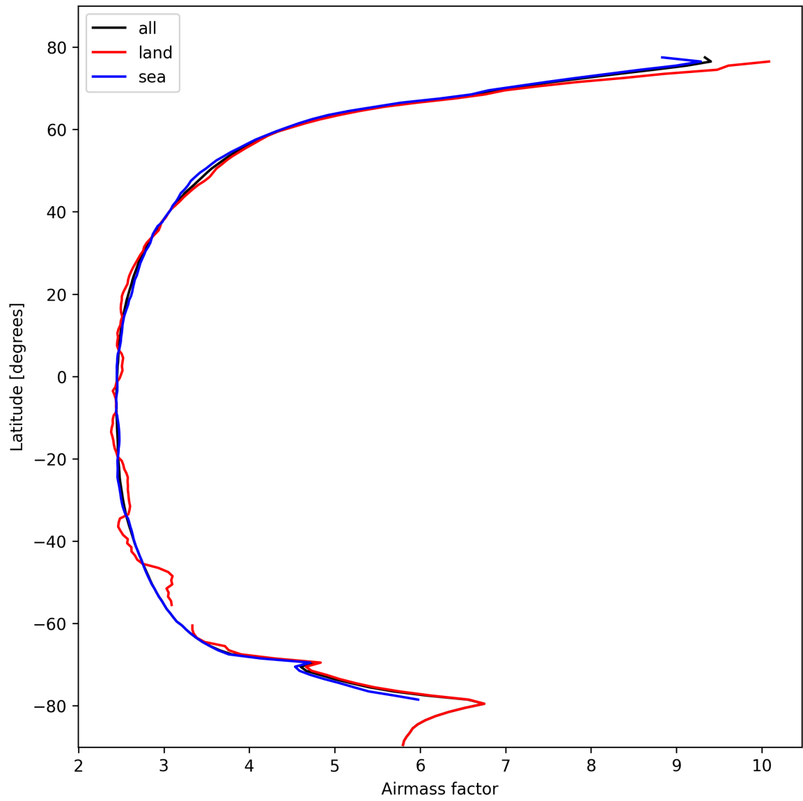
Figure 25: Zonal average of “Airmass factor” for 2025-02-16 to 2025-02-16.
