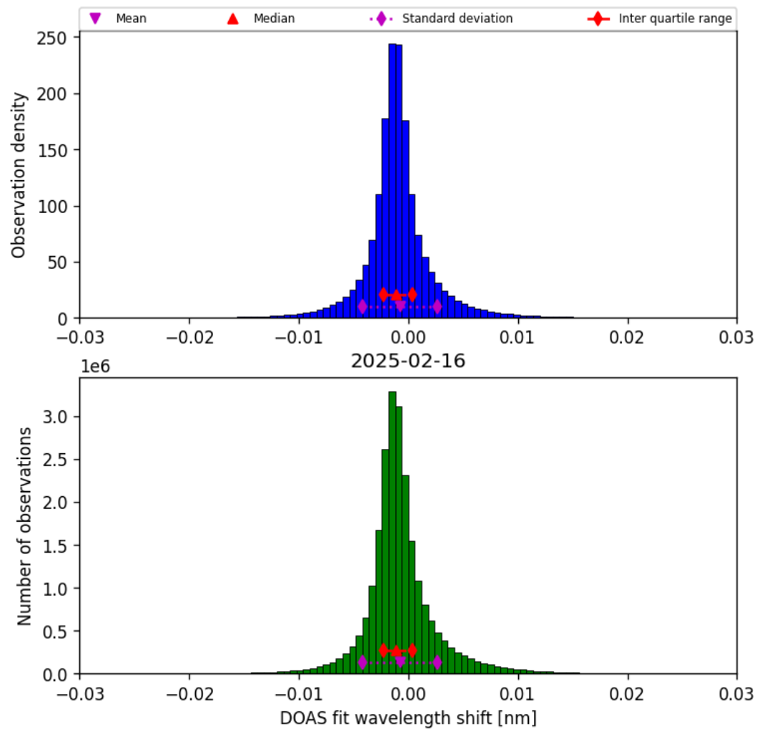
Figure 35: Histogram of “DOAS fit wavelength shift” for 2025-02-16 to 2025-02-16
