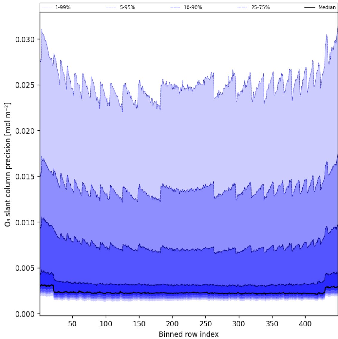
Figure 44: Along track statistics of “O 3 slant column precision” for 2025-02-16 to 2025-02-16
