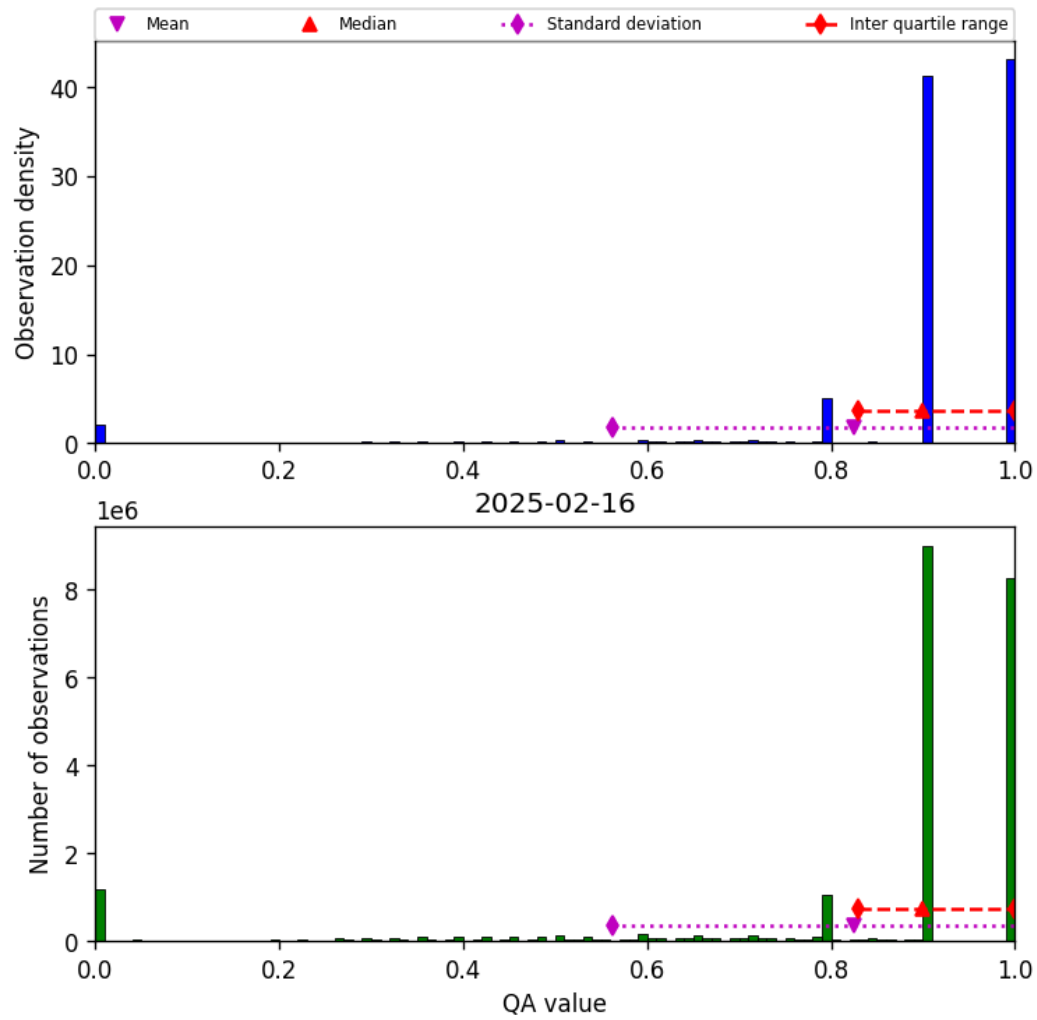
Figure 28: Histogram of “QA value” for 2025-02-16 to 2025-02-16
