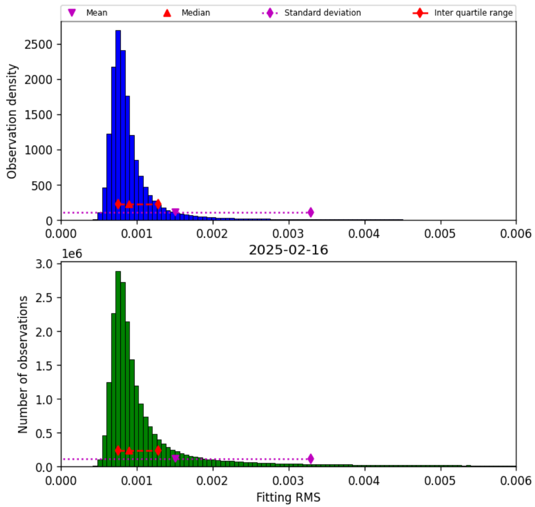
Figure 34: Histogram of “Fitting RMS” for 2025-02-16 to 2025-02-16
