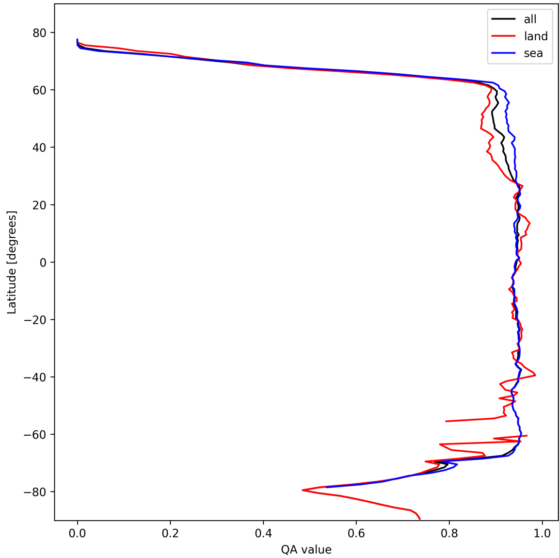
Figure 16: Zonal average of “QA value” for 2025-02-16 to 2025-02-16.
