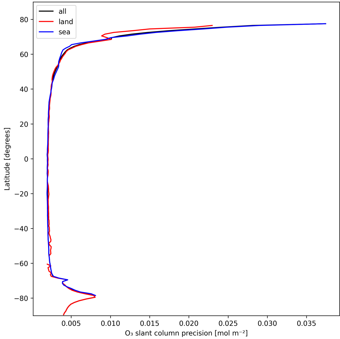
Figure 20: Zonal average of “O 3 slant column precision” for 2025-02-16 to 2025-02-16.
