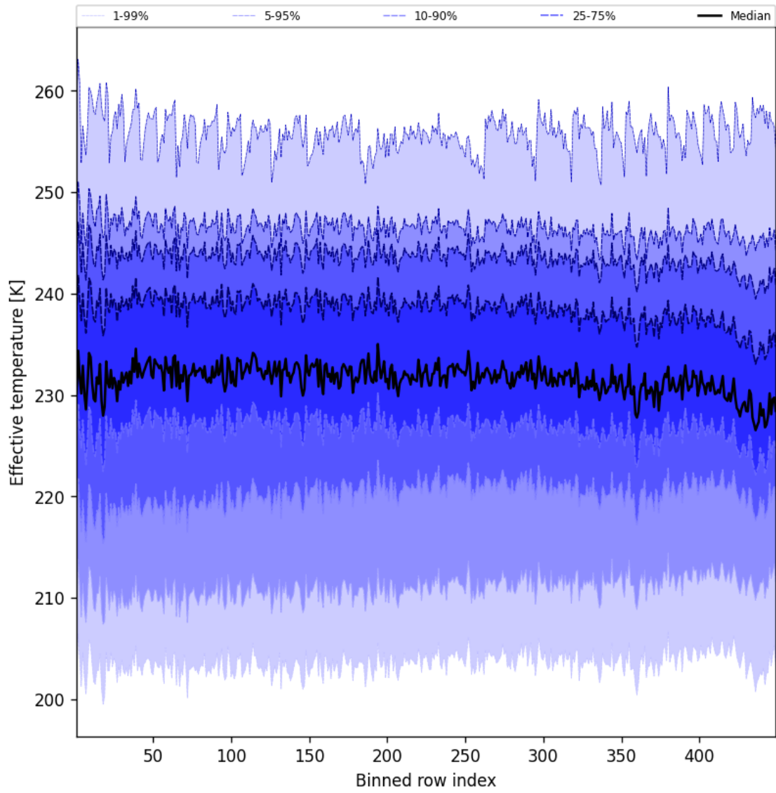
Figure 50: Along track statistics of “Effective temperature” for 2025-02-16 to 2025-02-16
