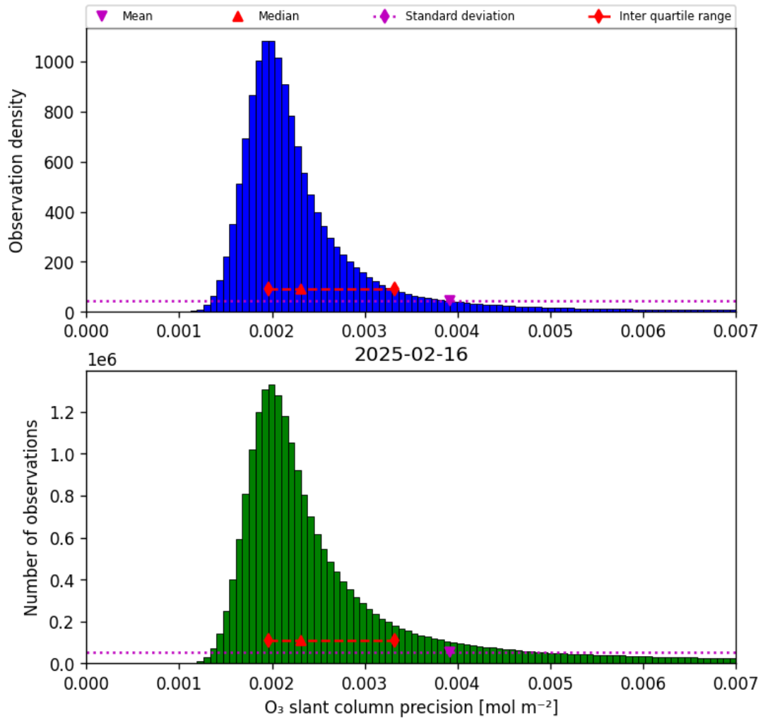
Figure 32: Histogram of “O 3 slant column precision” for 2025-02-16 to 2025-02-16
