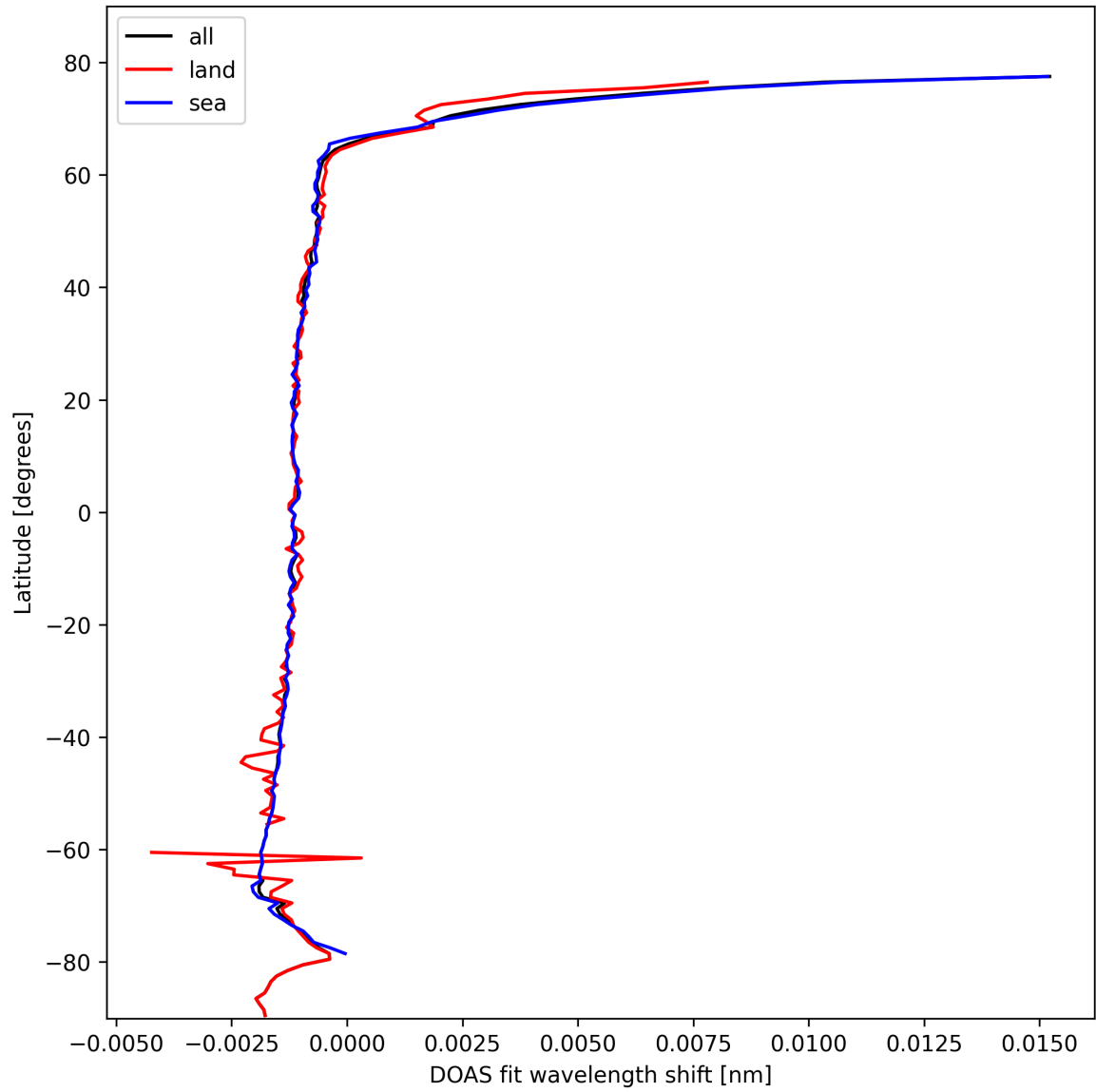
Figure 23: Zonal average of “DOAS fit wavelength shift” for 2025-02-16 to 2025-02-16.
