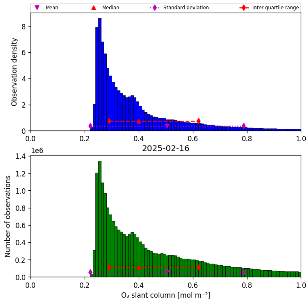
Figure 31: Histogram of “O 3 slant column” for 2025-02-16 to 2025-02-16
