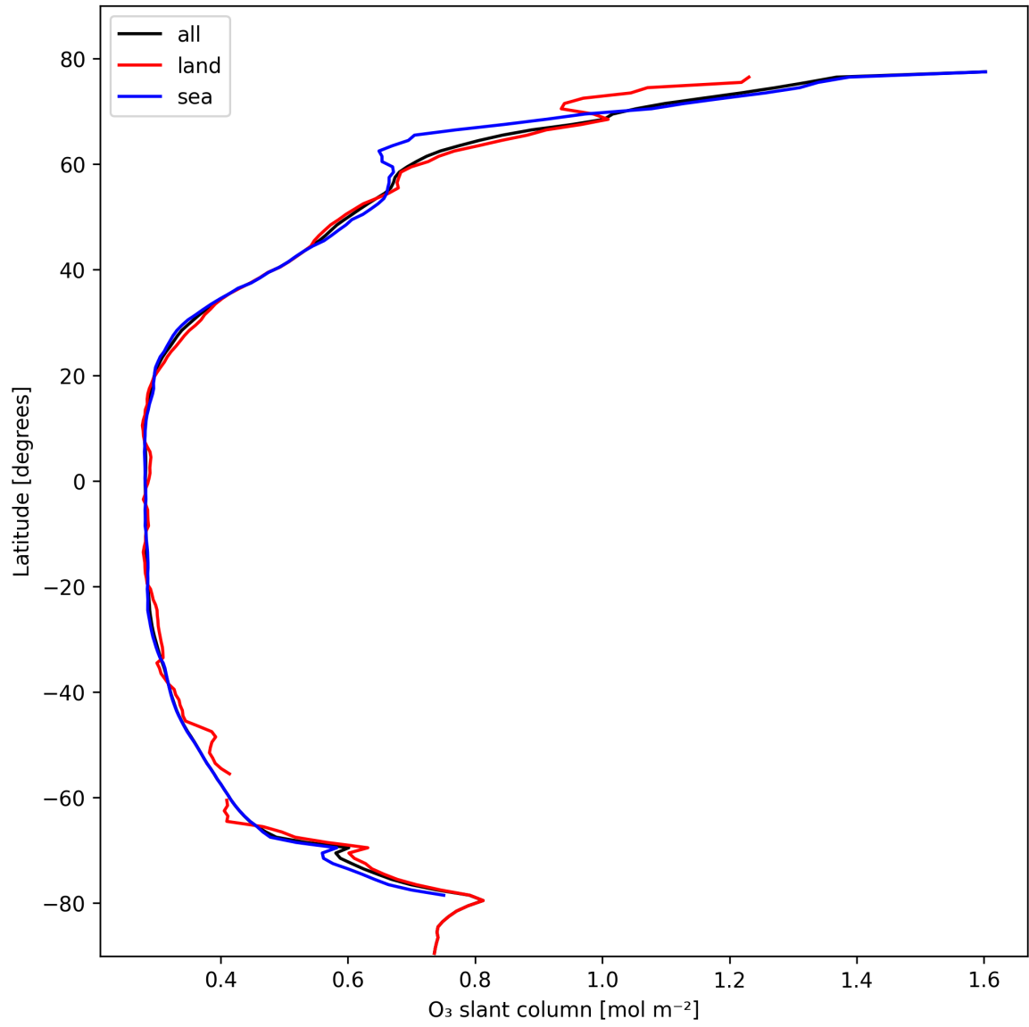
Figure 19: Zonal average of “O 3 slant column” for 2025-02-16 to 2025-02-16.
