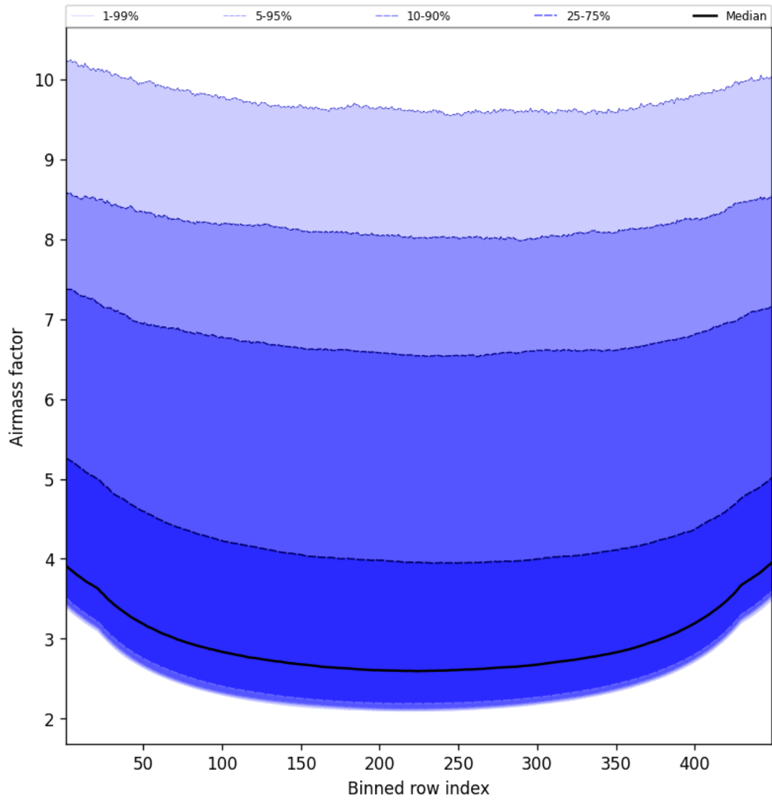
Figure 49: Along track statistics of “Airmass factor” for 2025-02-16 to 2025-02-16
