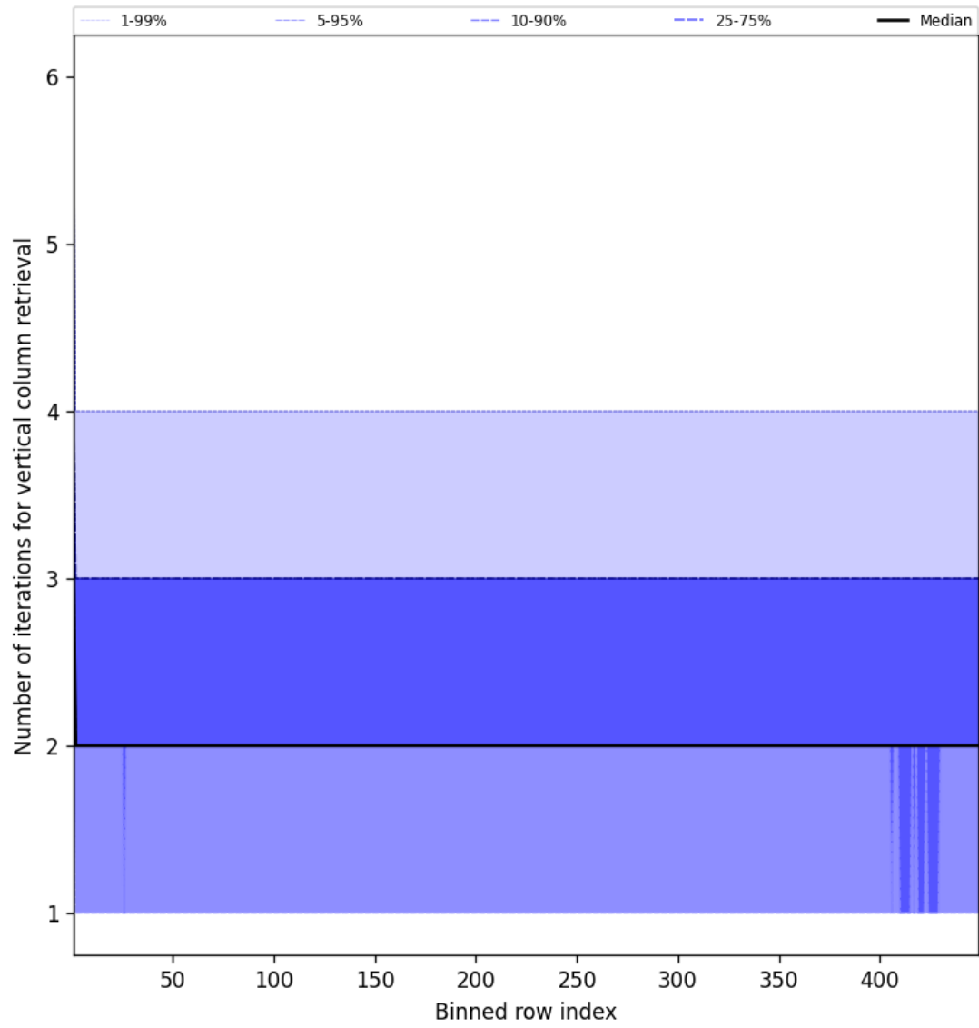
Figure 51: Along track statistics of “Number of iterations for vertical column retrieval” for 2025-02-16 to 2025-02-16
