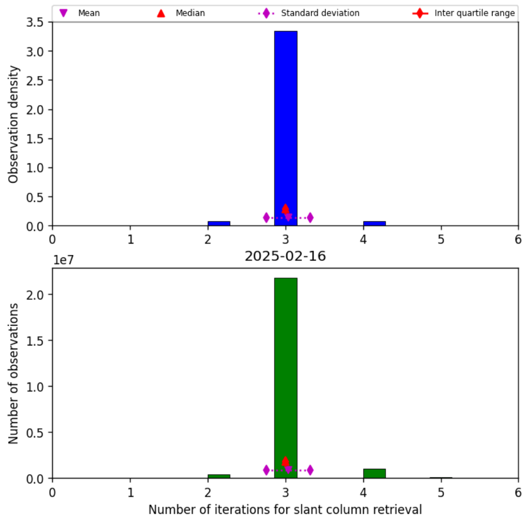
Figure 33: Histogram of “Number of iterations for slant column retrieval” for 2025-02-16 to 2025-02-16
