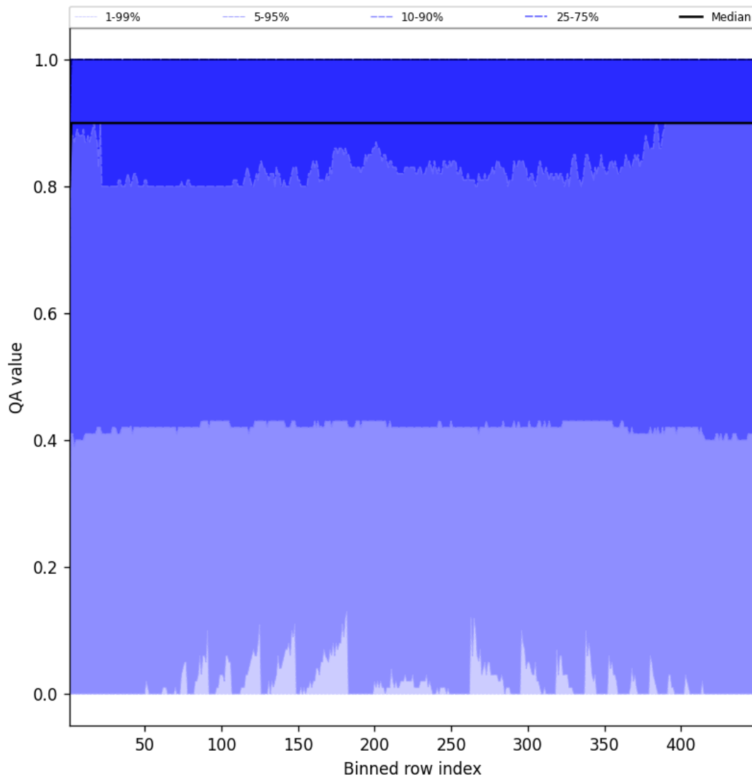
Figure 40: Along track statistics of “QA value” for 2025-02-16 to 2025-02-16
