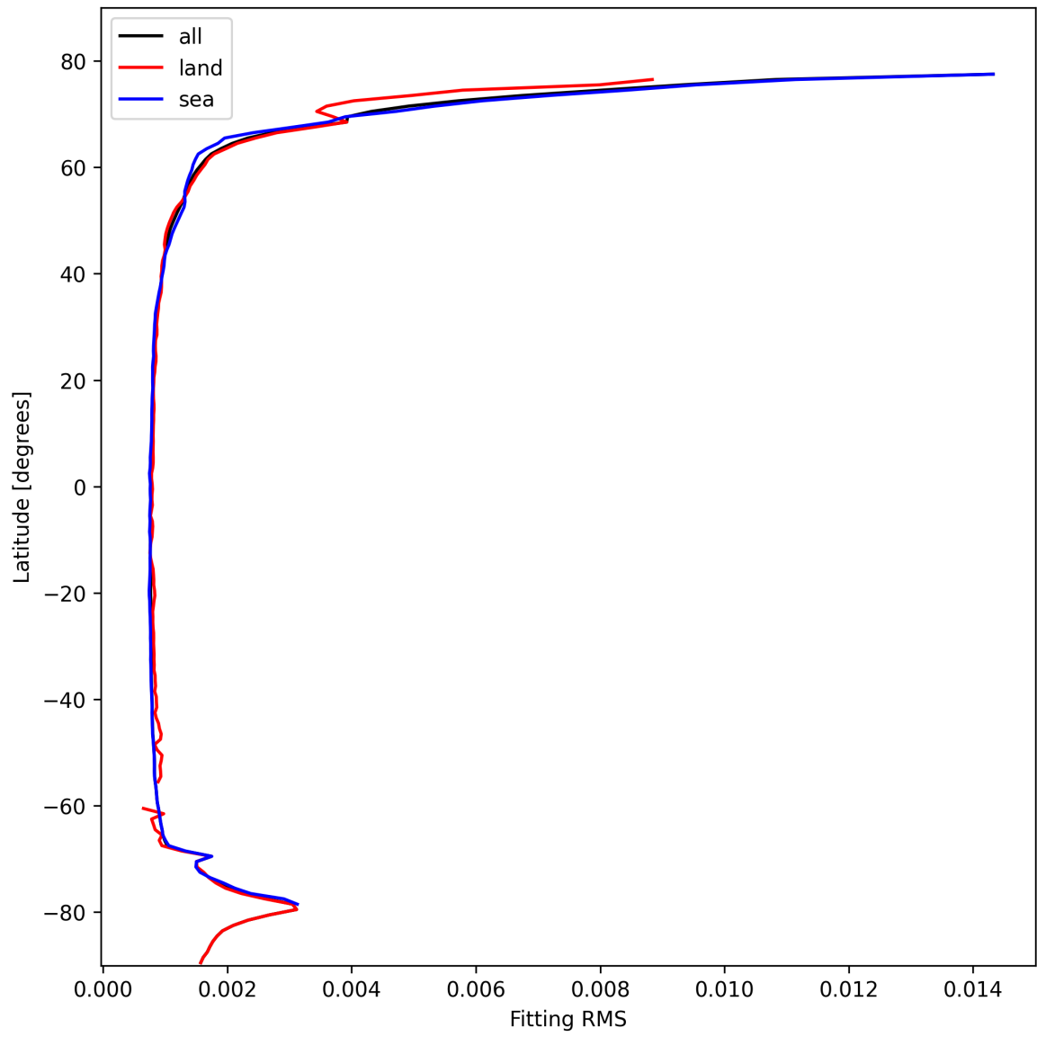
Figure 22: Zonal average of “Fitting RMS” for 2025-02-16 to 2025-02-16.
