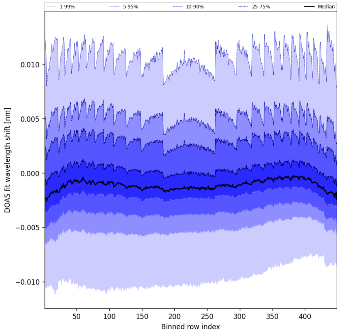
Figure 47: Along track statistics of “DOAS fit wavelength shift” for 2025-02-16 to 2025-02-16
