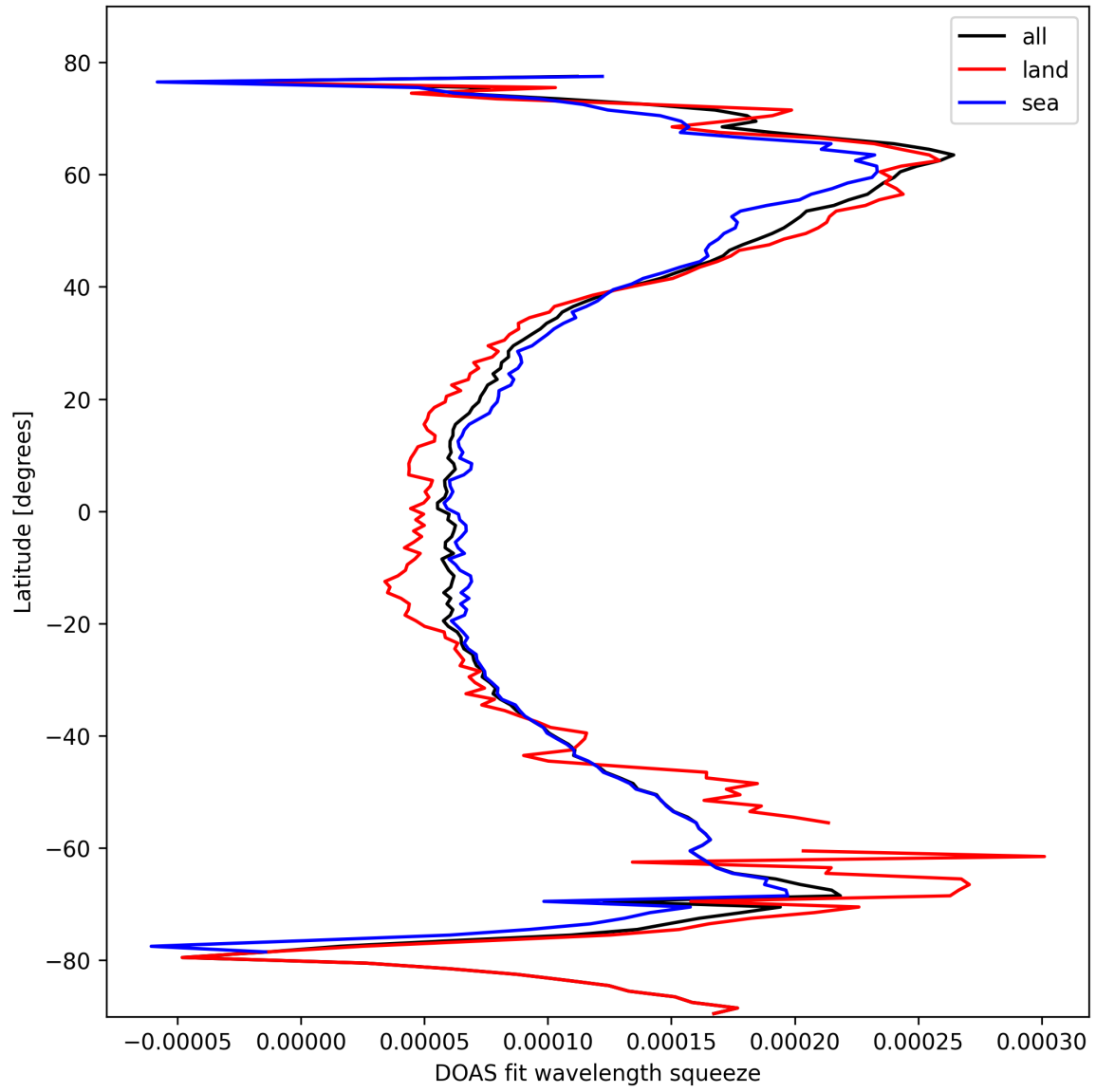
Figure 24: Zonal average of “DOAS fit wavelength squeeze” for 2025-02-16 to 2025-02-16.
