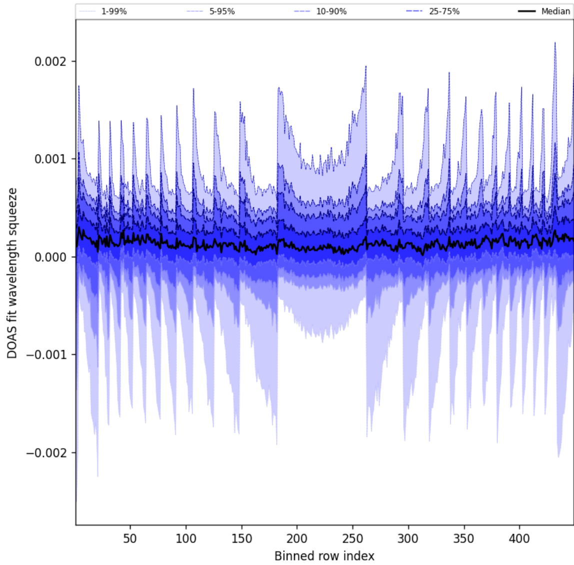
Figure 48: Along track statistics of “DOAS fit wavelength squeeze” for 2025-02-16 to 2025-02-16
