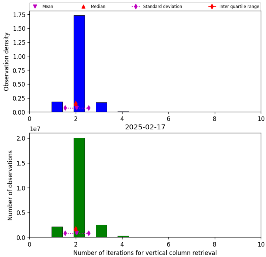
Figure 39: Histogram of “Number of iterations for vertical column retrieval” for 2025-02-17 to 2025-02-18
