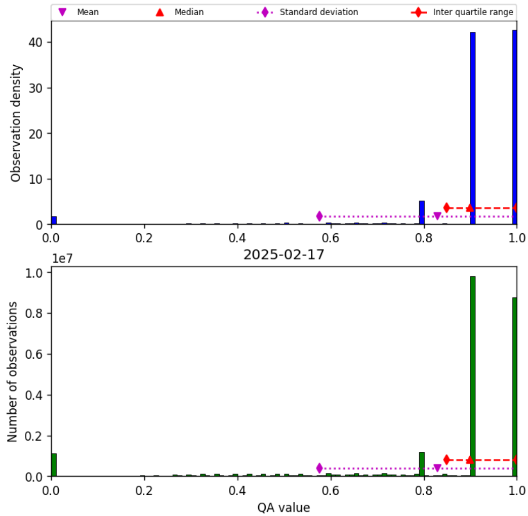
Figure 28: Histogram of “QA value” for 2025-02-17 to 2025-02-18
