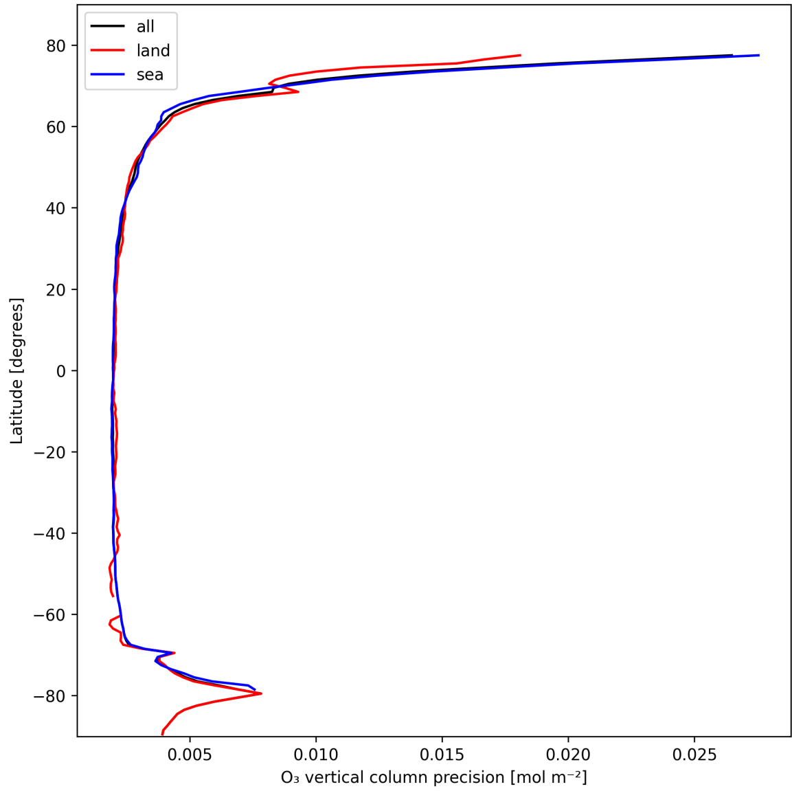
Figure 18: Zonal average of “O 3 vertical column precision” for 2025-02-17 to 2025-02-18.
