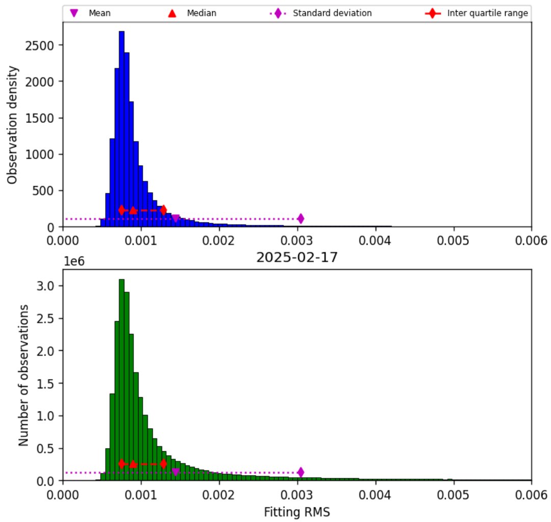
Figure 34: Histogram of “Fitting RMS” for 2025-02-17 to 2025-02-18
