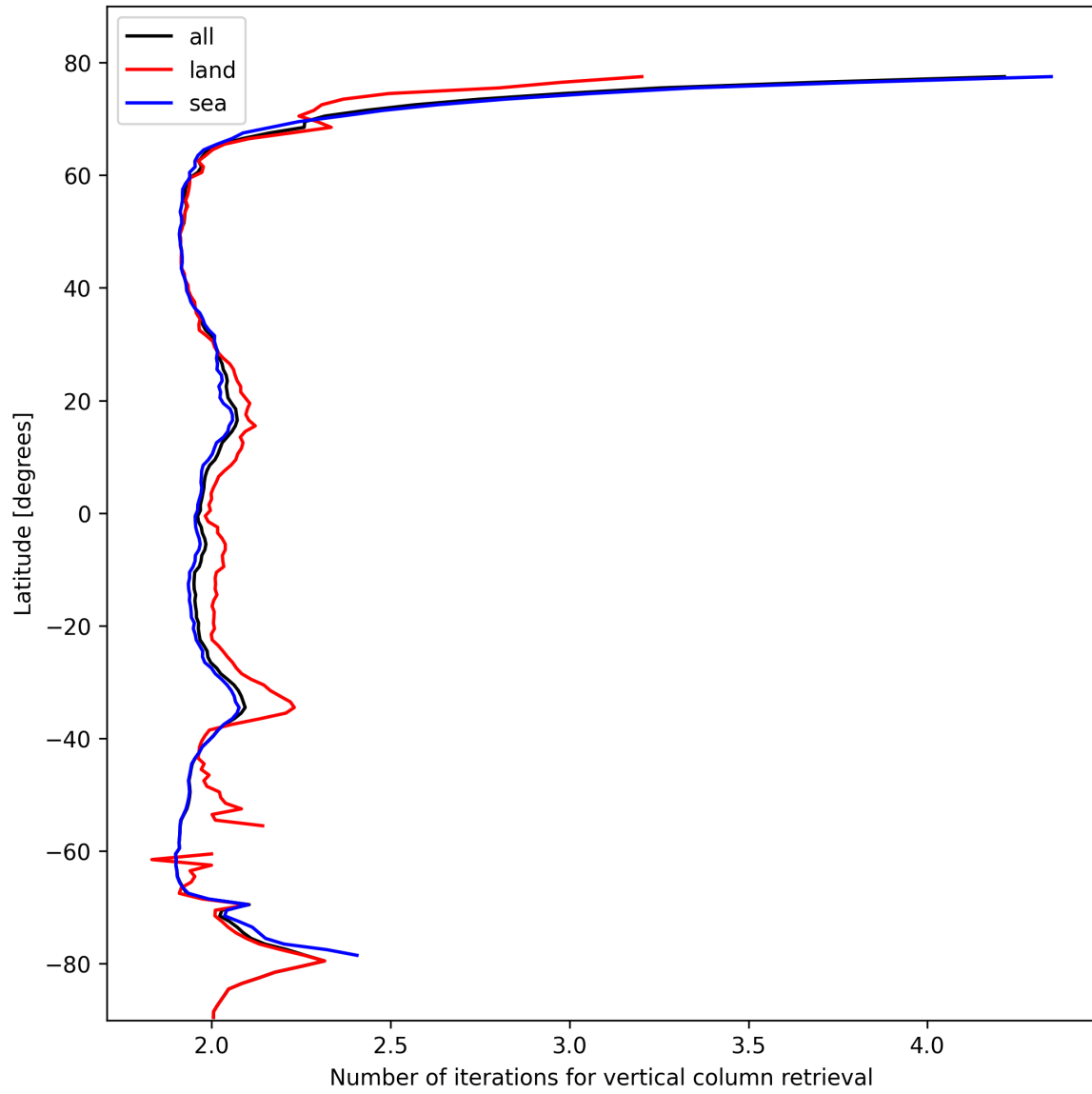
Figure 27: Zonal average of “Number of iterations for vertical column retrieval” for 2025-02-17 to 2025-02-18.
