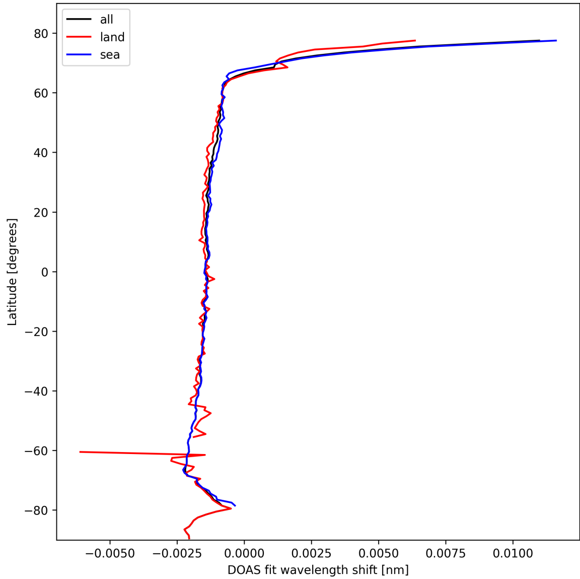
Figure 23: Zonal average of “DOAS fit wavelength shift” for 2025-02-17 to 2025-02-18.
