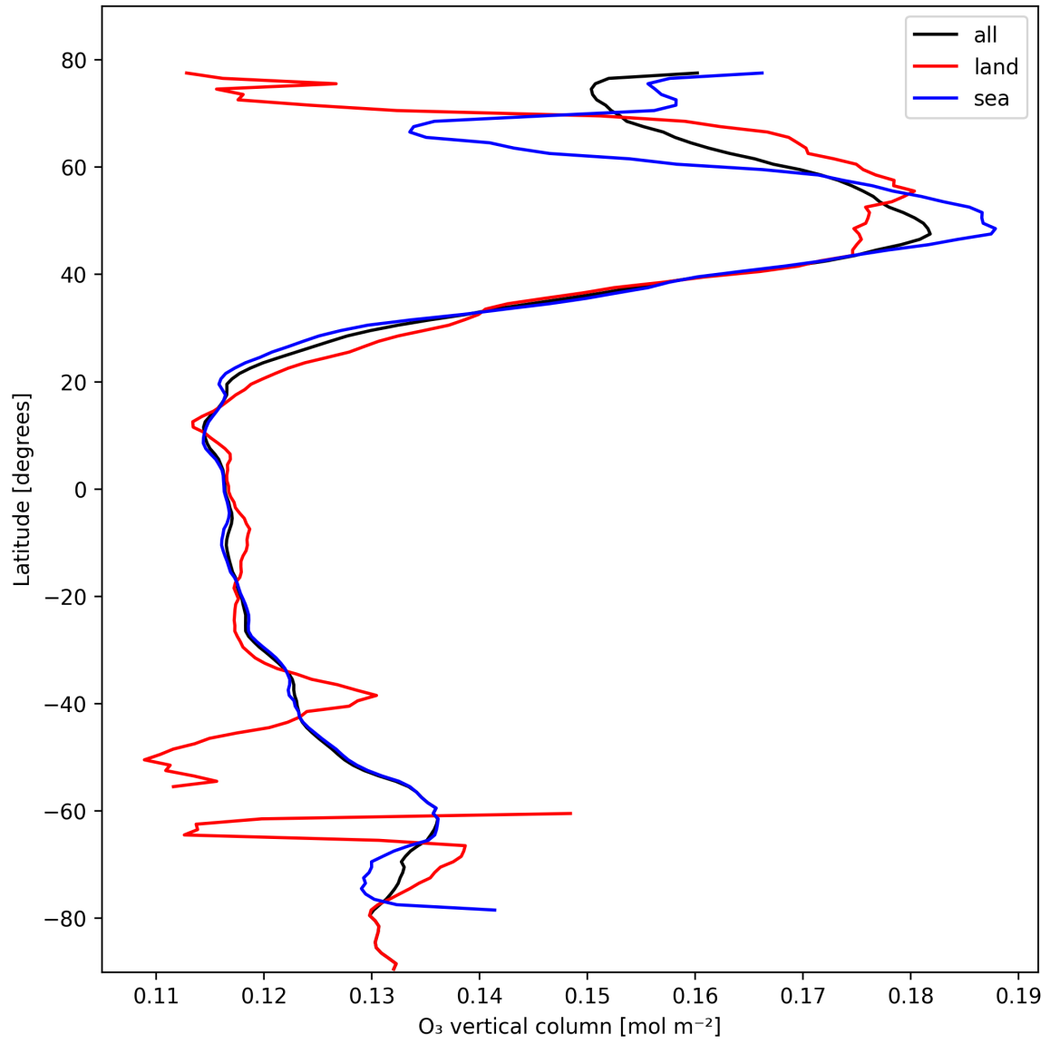
Figure 17: Zonal average of “O 3 vertical column” for 2025-02-17 to 2025-02-18.
