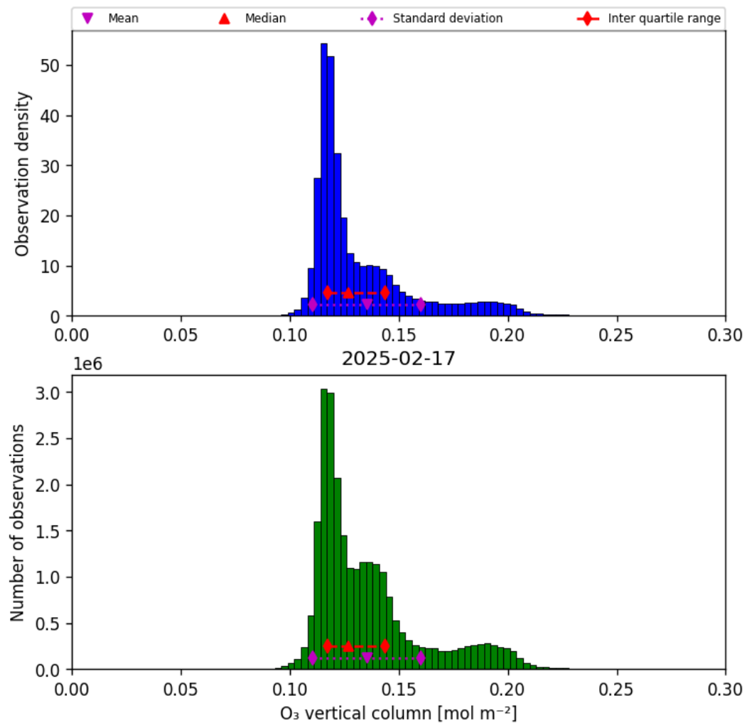
Figure 29: Histogram of “O 3 vertical column” for 2025-02-17 to 2025-02-18
