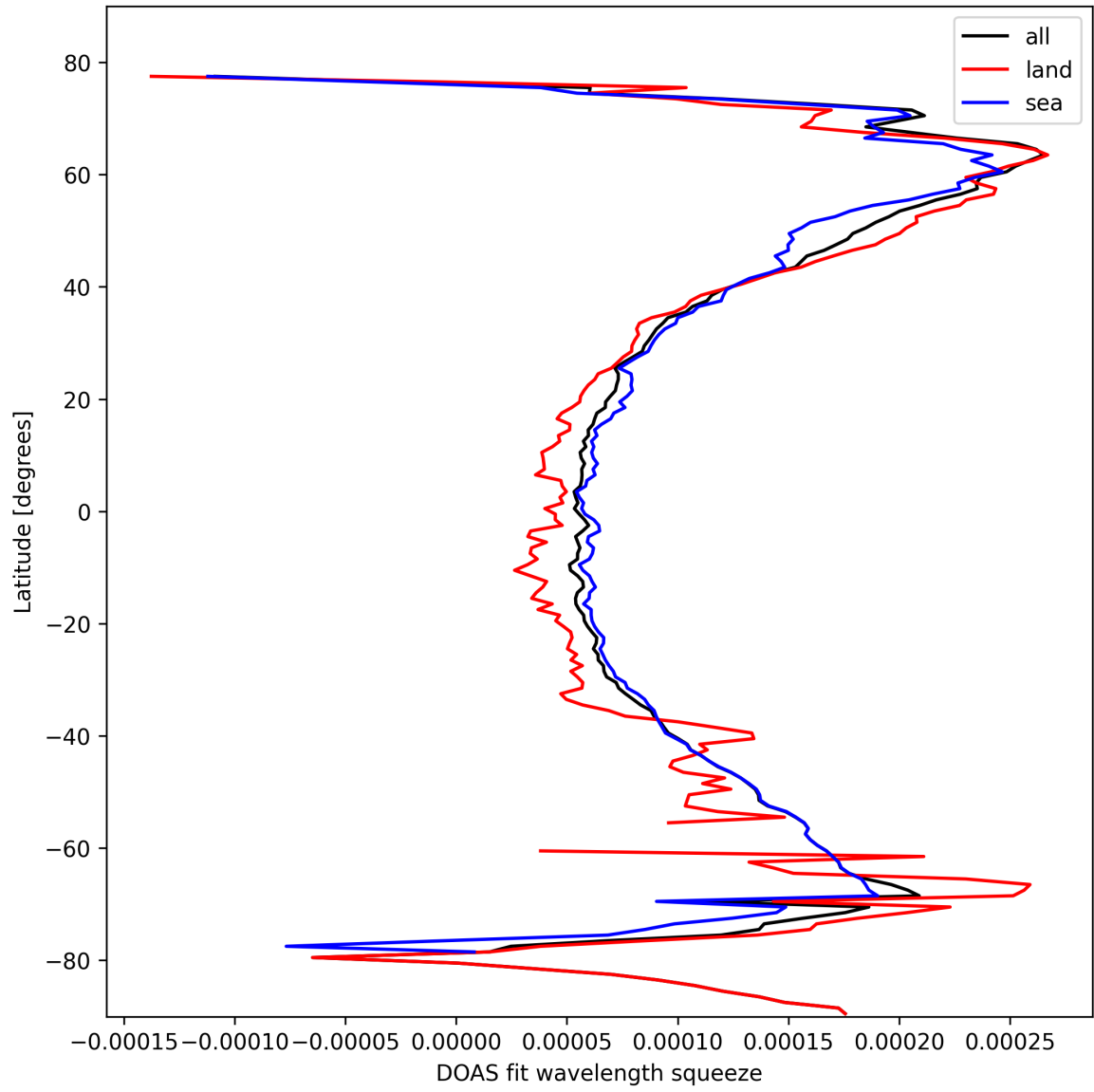
Figure 24: Zonal average of “DOAS fit wavelength squeeze” for 2025-02-17 to 2025-02-18.
