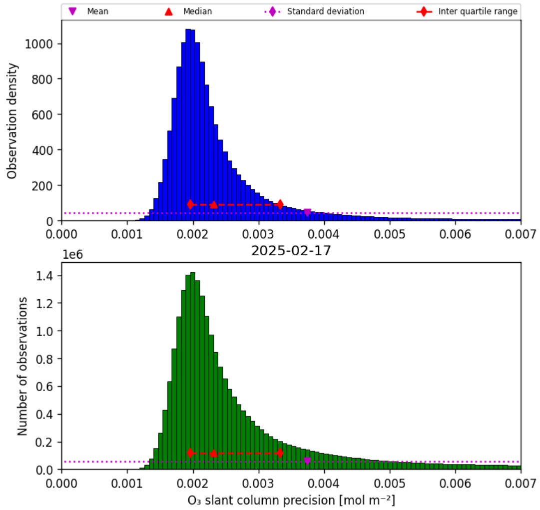
Figure 32: Histogram of “O 3 slant column precision” for 2025-02-17 to 2025-02-18
