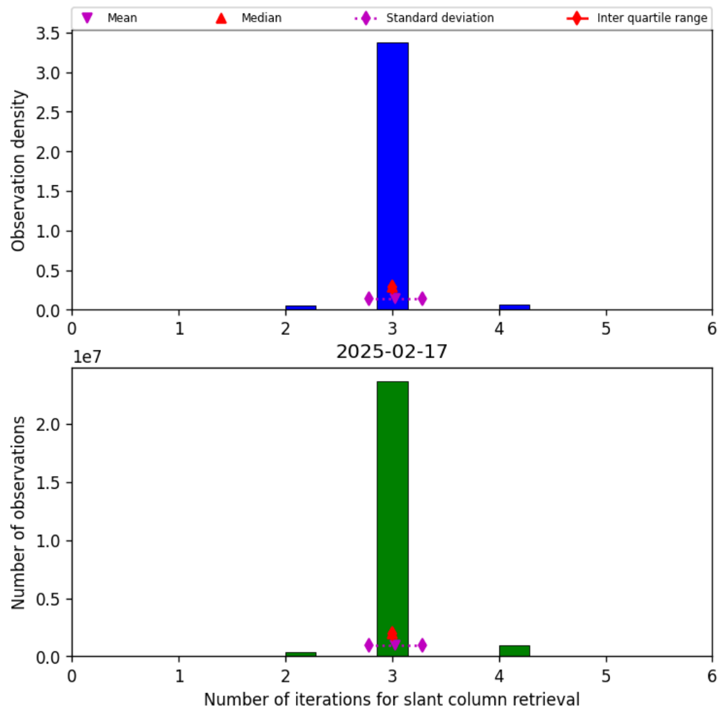
Figure 33: Histogram of “Number of iterations for slant column retrieval” for 2025-02-17 to 2025-02-18
