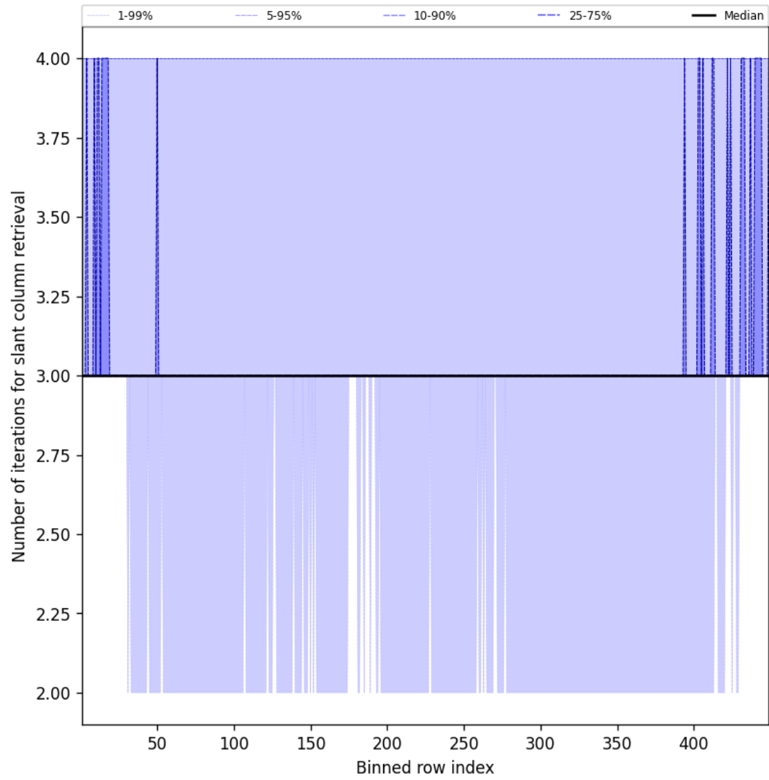
Figure 45: Along track statistics of “Number of iterations for slant column retrieval” for 2025-02-17 to 2025-02-18
