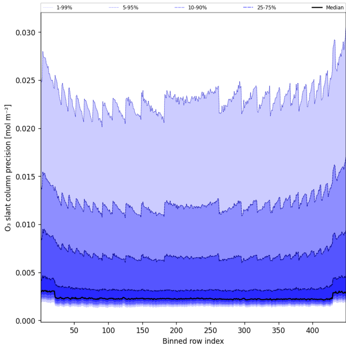
Figure 44: Along track statistics of “O 3 slant column precision” for 2025-02-17 to 2025-02-18
