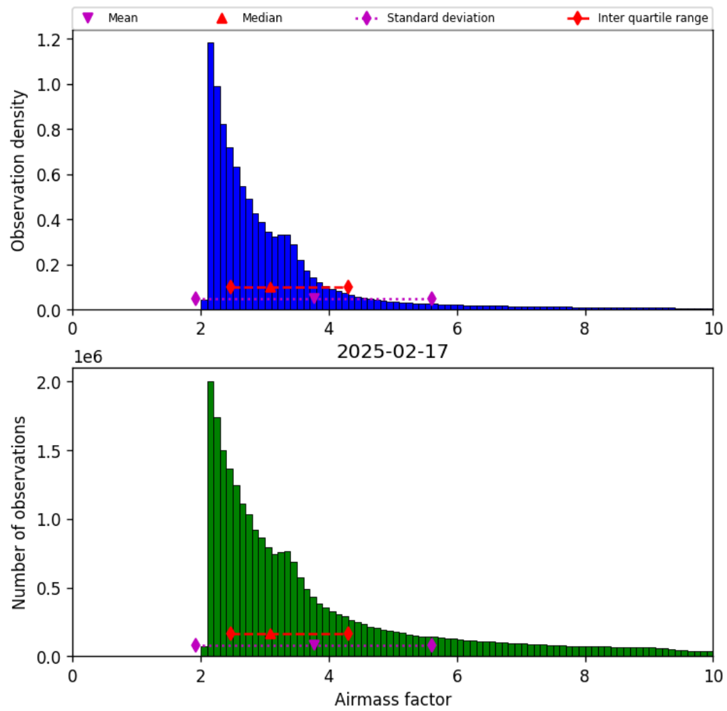
Figure 37: Histogram of “Airmass factor” for 2025-02-17 to 2025-02-18
