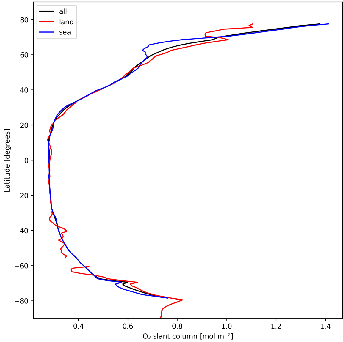
Figure 19: Zonal average of “O 3 slant column” for 2025-02-17 to 2025-02-18.
