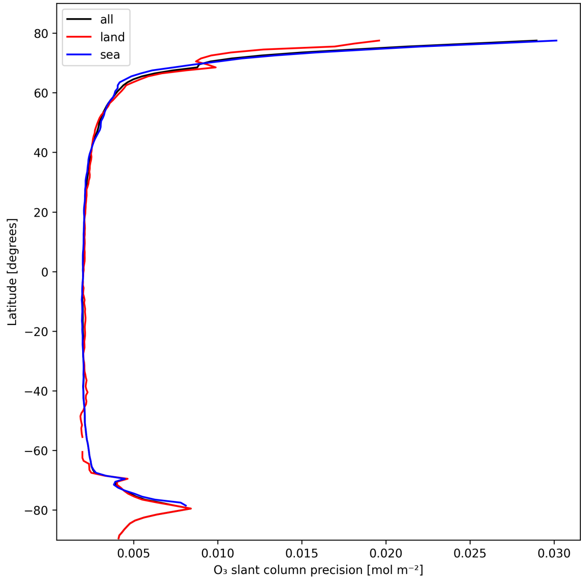
Figure 20: Zonal average of "O 3 slant column precision" for 2025-02-17 to 2025-02-18.
