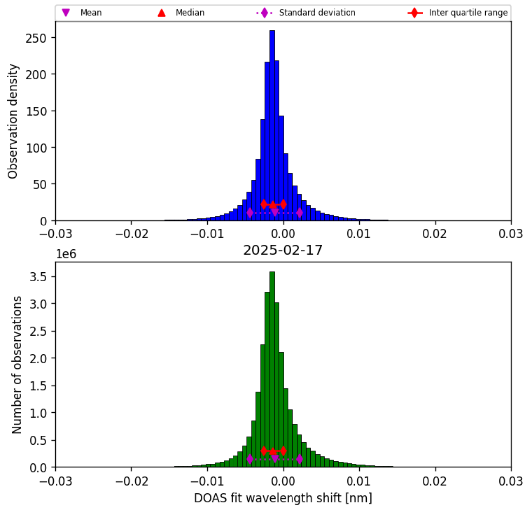
Figure 35: Histogram of “DOAS fit wavelength shift” for 2025-02-17 to 2025-02-18
