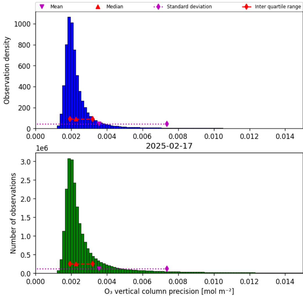
Figure 30: Histogram of “O 3 vertical column precision” for 2025-02-17 to 2025-02-18
