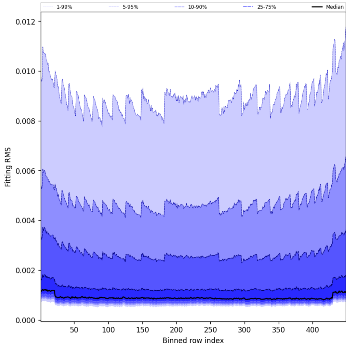
Figure 46: Along track statistics of “Fitting RMS” for 2025-02-17 to 2025-02-18
