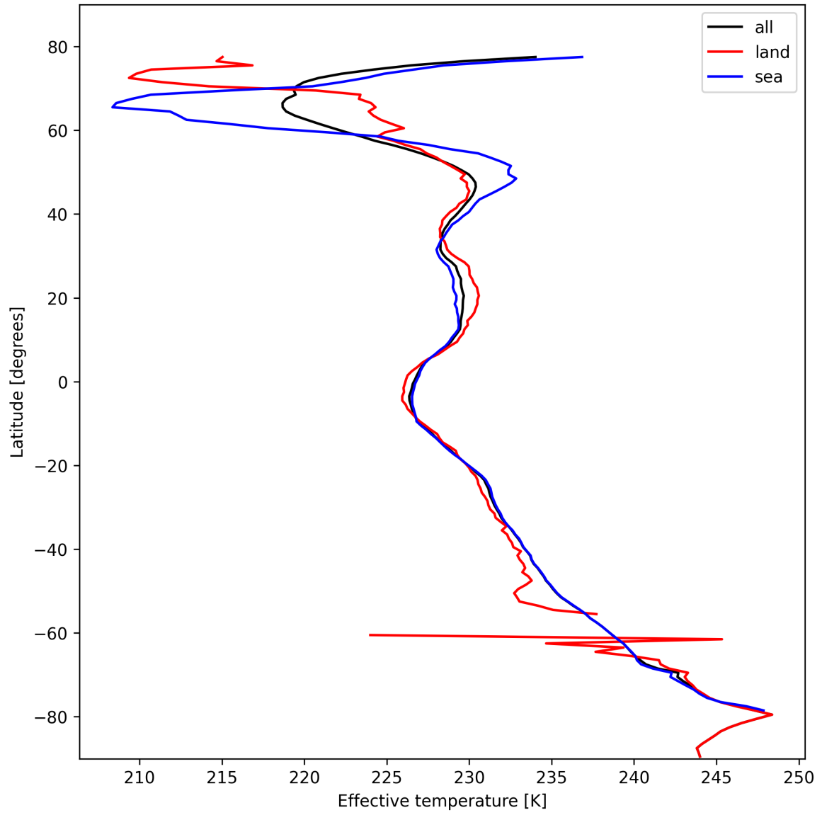
Figure 26: Zonal average of “Effective temperature” for 2025-02-17 to 2025-02-18.
