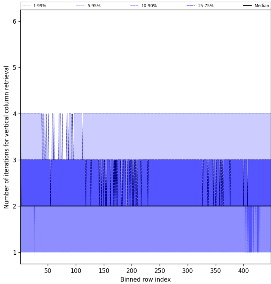
Figure 51: Along track statistics of “Number of iterations for vertical column retrieval” for 2025-02-17 to 2025-02-18
