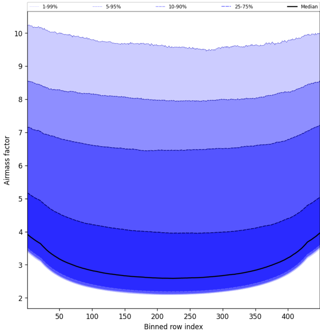
Figure 49: Along track statistics of “Airmass factor” for 2025-02-17 to 2025-02-18
