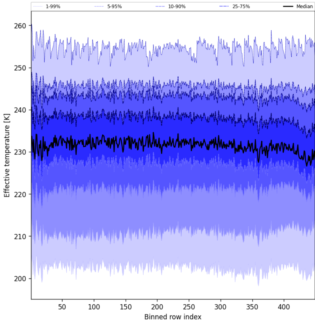
Figure 50: Along track statistics of “Effective temperature” for 2025-02-17 to 2025-02-18
