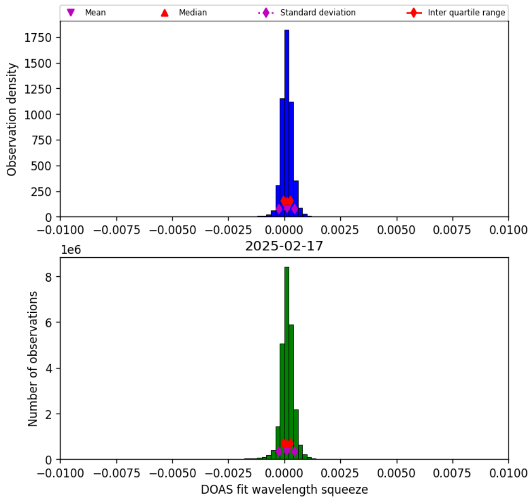
Figure 36: Histogram of “DOAS fit wavelength squeeze” for 2025-02-17 to 2025-02-18
