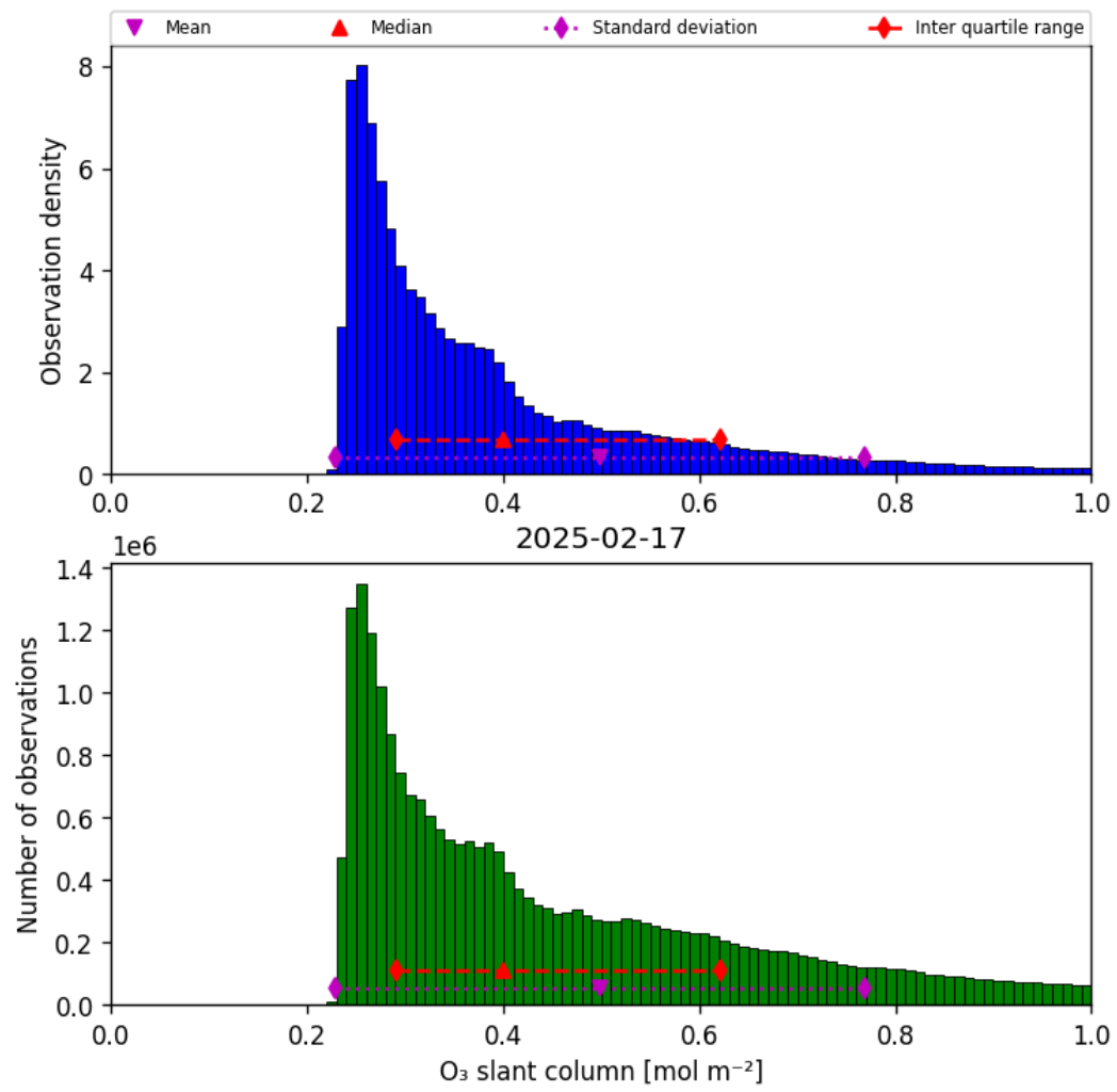
Figure 31: Histogram of “O 3 slant column” for 2025-02-17 to 2025-02-18
