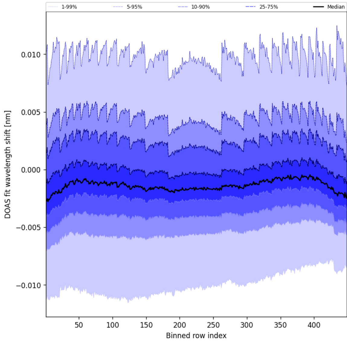
Figure 47: Along track statistics of “DOAS fit wavelength shift” for 2025-02-17 to 2025-02-18
