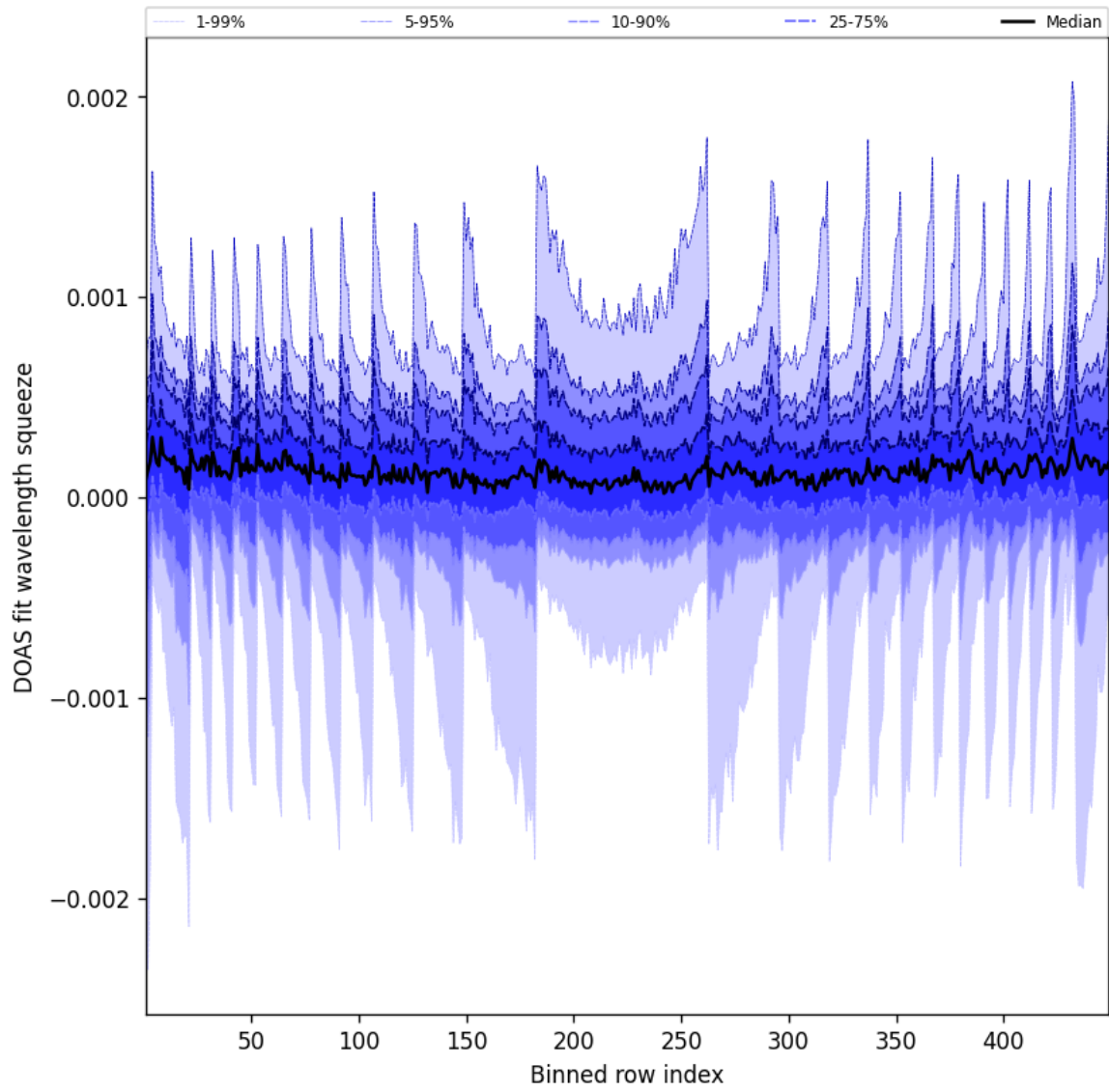
Figure 48: Along track statistics of “DOAS fit wavelength squeeze” for 2025-02-17 to 2025-02-18
