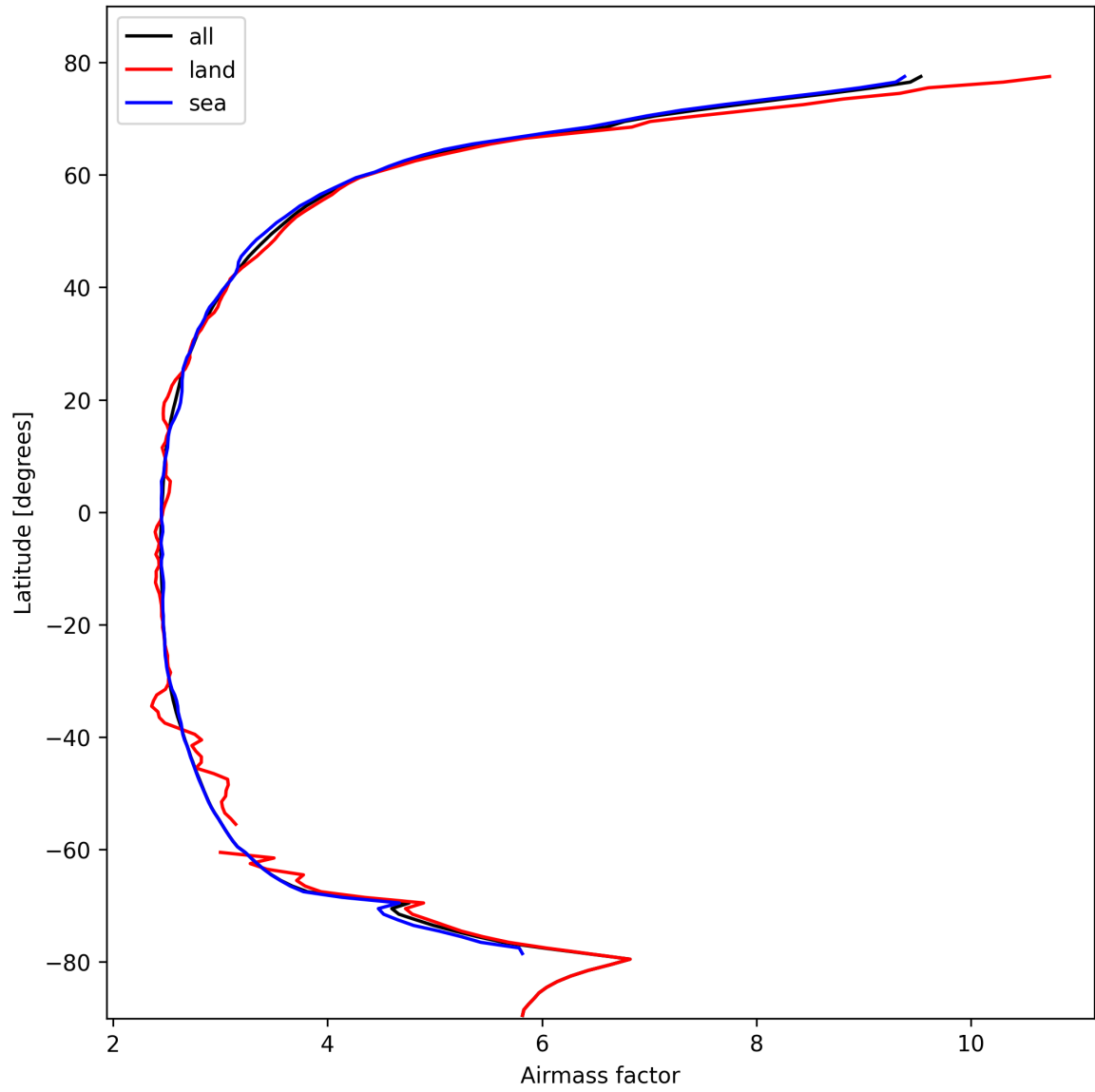
Figure 25: Zonal average of “Airmass factor” for 2025-02-17 to 2025-02-18.
