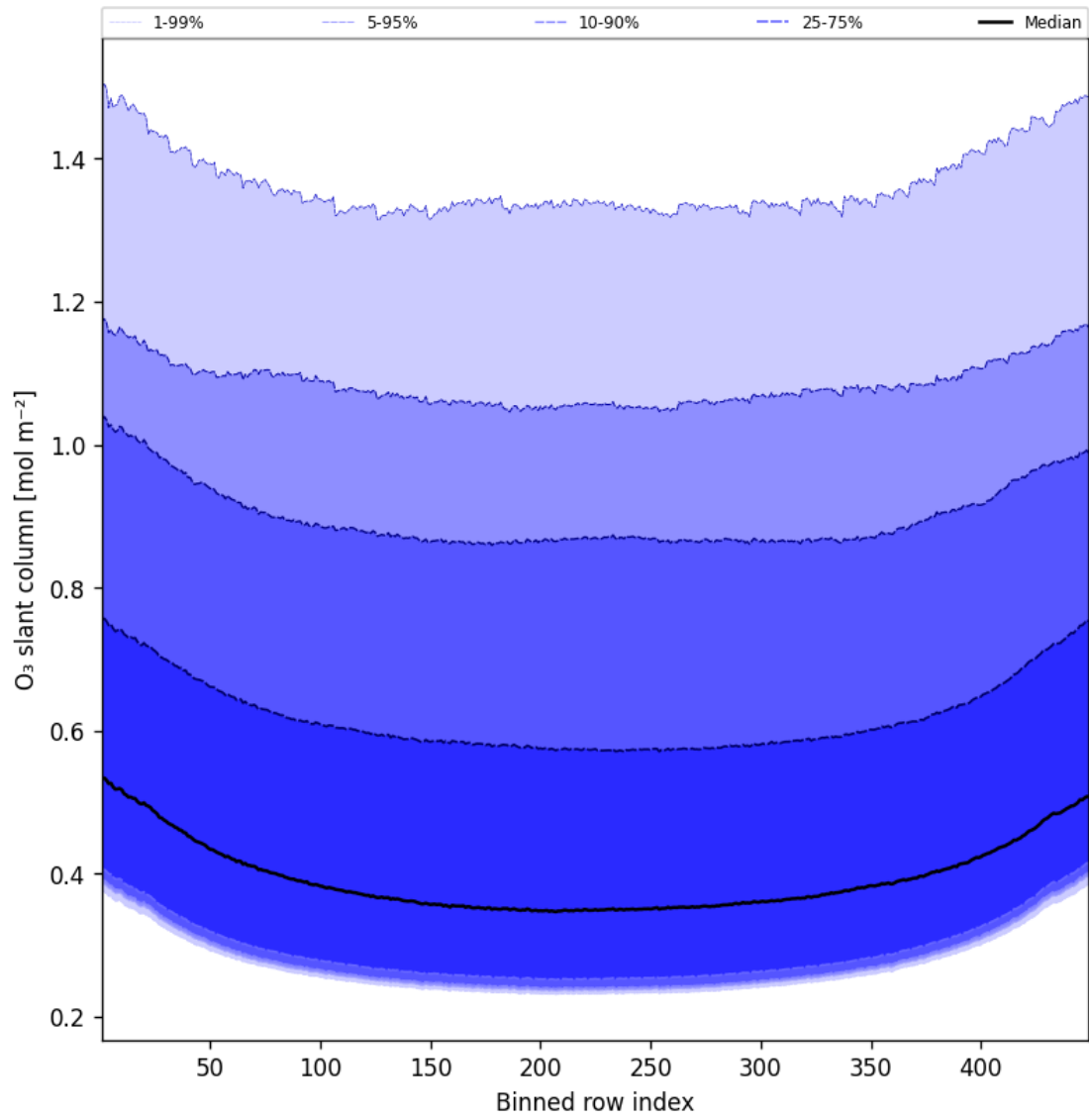
Figure 43: Along track statistics of “O 3 slant column” for 2025-02-17 to 2025-02-18
