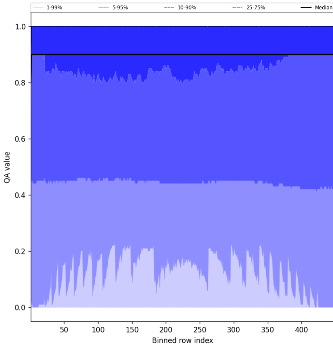
Figure 40: Along track statistics of “QA value” for 2025-02-17 to 2025-02-18
