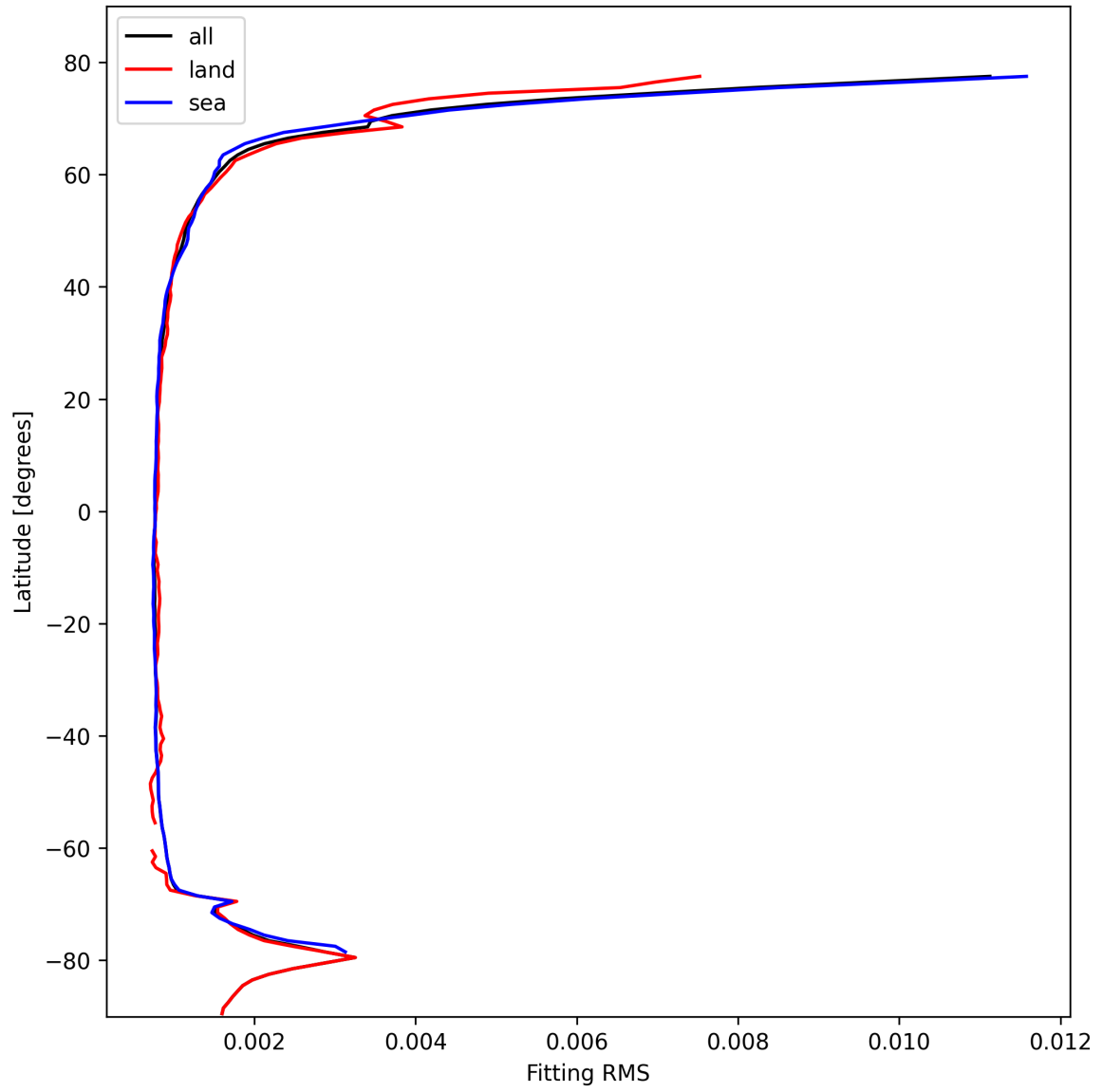
Figure 22: Zonal average of “Fitting RMS” for 2025-02-17 to 2025-02-18.
