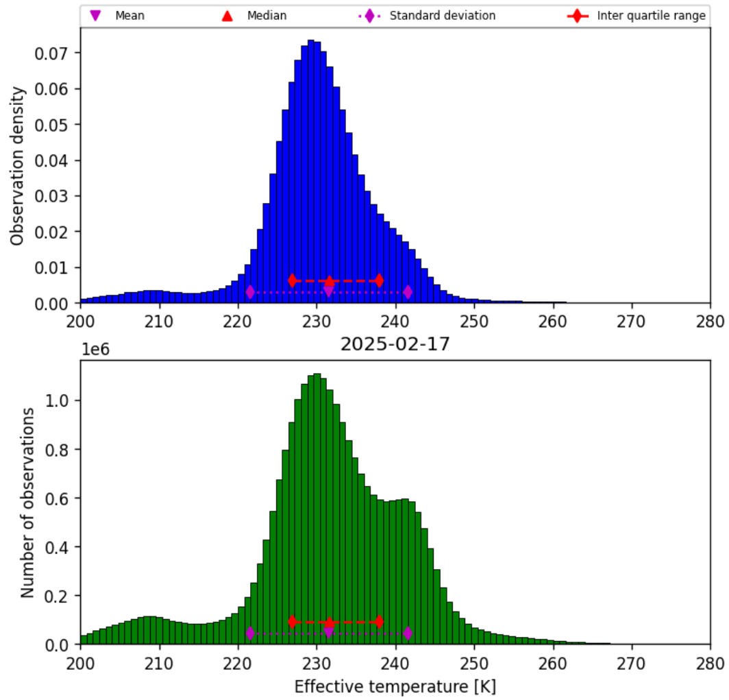
Figure 38: Histogram of “Effective temperature” for 2025-02-17 to 2025-02-18
