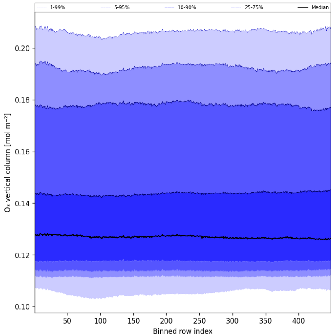
Figure 41: Along track statistics of “O 3 vertical column” for 2025-02-17 to 2025-02-18
