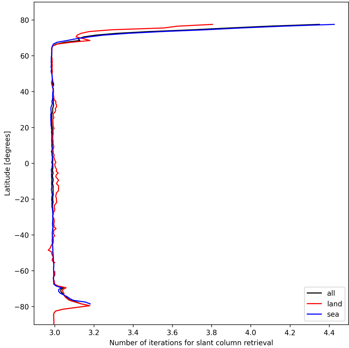
Figure 21: Zonal average of “Number of iterations for slant column retrieval” for 2025-02-17 to 2025-02-18.
