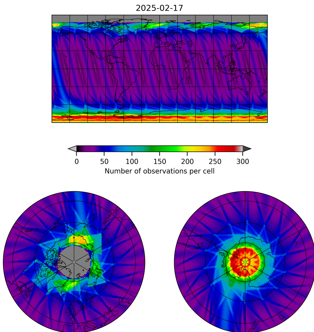
Figure 15: Map of the number of observations for 2025-02-17 to 2025-02-18
