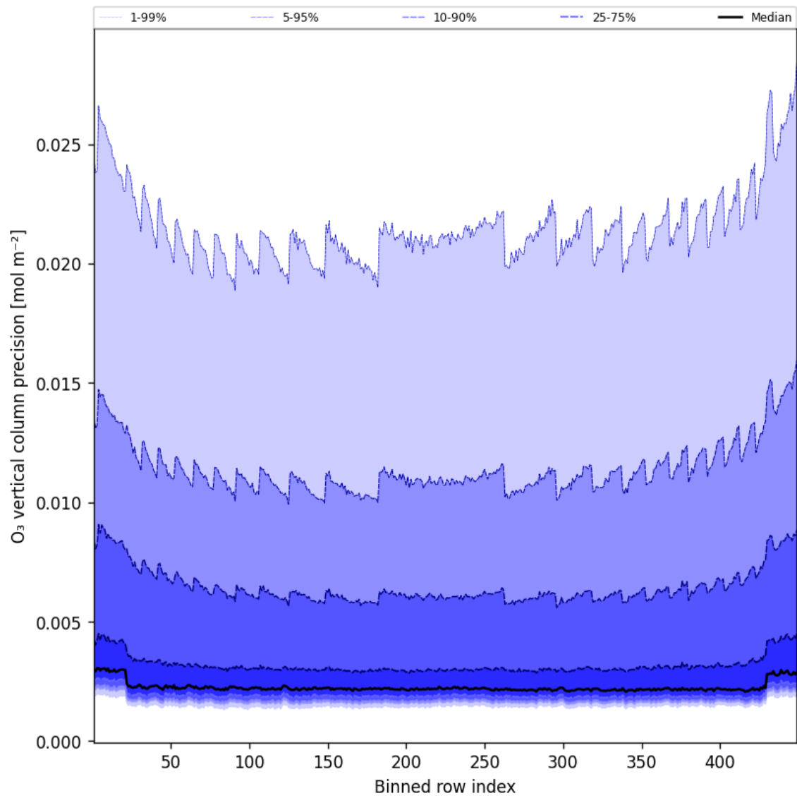
Figure 42: Along track statistics of “O 3 vertical column precision” for 2025-02-17 to 2025-02-18
