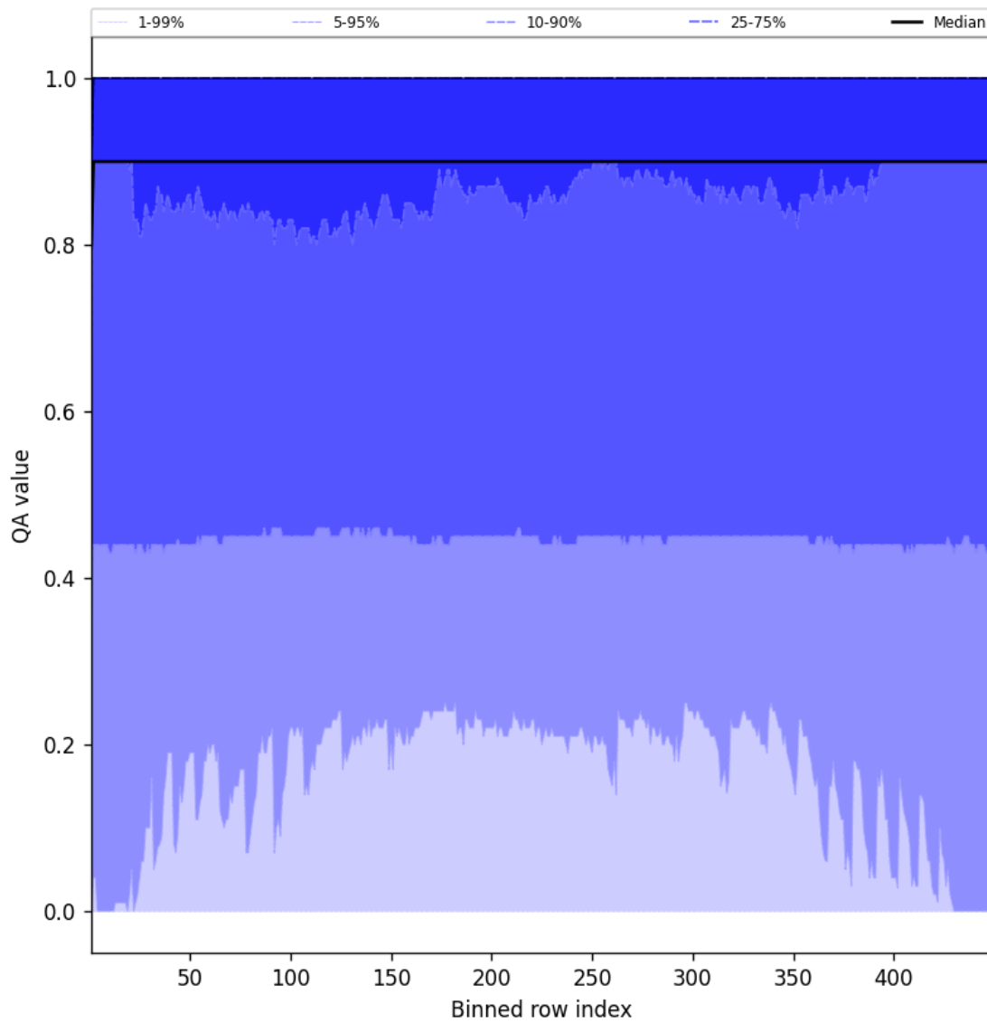
Figure 40: Along track statistics of “QA value” for 2025-02-18 to 2025-02-19
