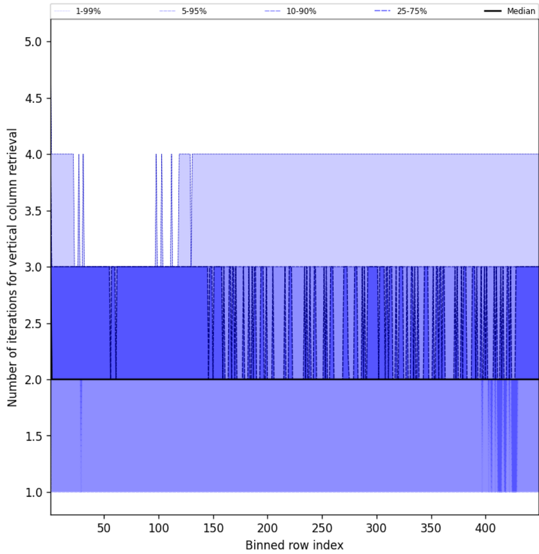
Figure 51: Along track statistics of “Number of iterations for vertical column retrieval” for 2025-02-18 to 2025-02-19
