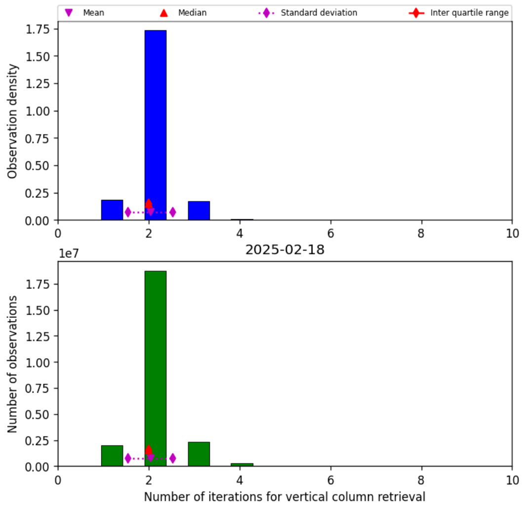
Figure 39: Histogram of “Number of iterations for vertical column retrieval” for 2025-02-18 to 2025-02-19
