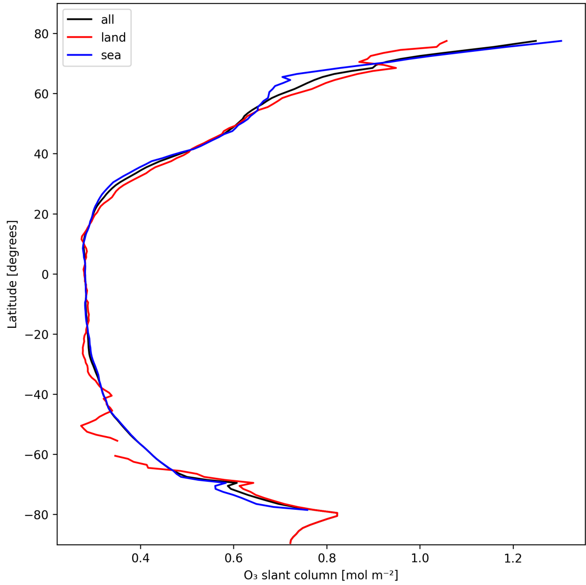
Figure 19: Zonal average of “O 3 slant column” for 2025-02-18 to 2025-02-19.
