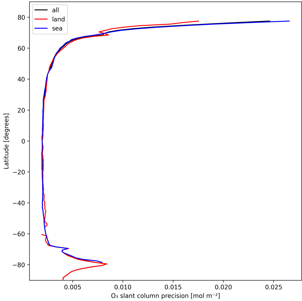
Figure 20: Zonal average of “O 3 slant column precision” for 2025-02-18 to 2025-02-19.
