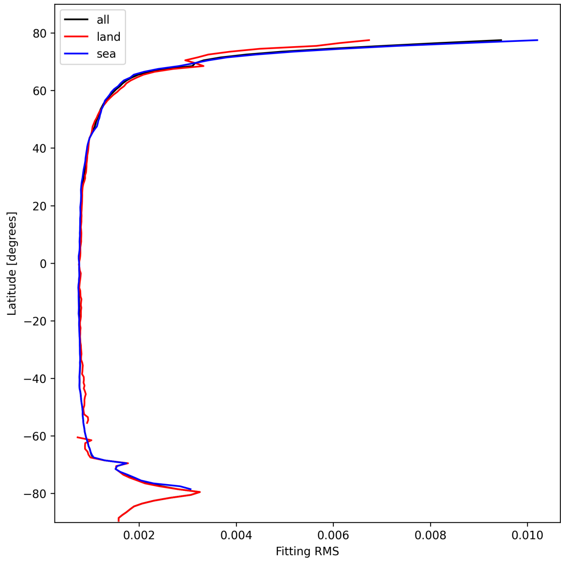
Figure 22: Zonal average of “Fitting RMS” for 2025-02-18 to 2025-02-19.
