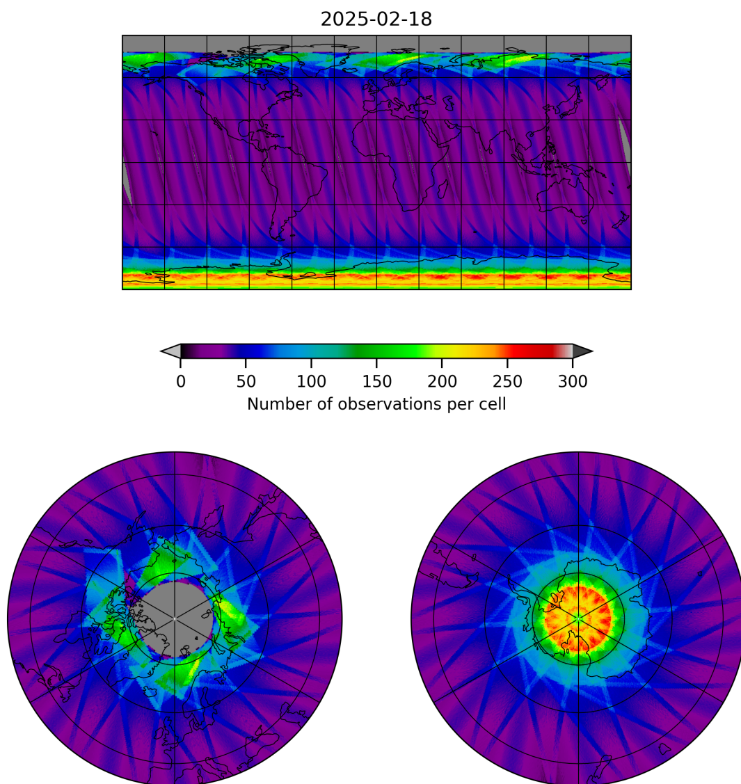
Figure 15: Map of the number of observations for 2025-02-18 to 2025-02-19
