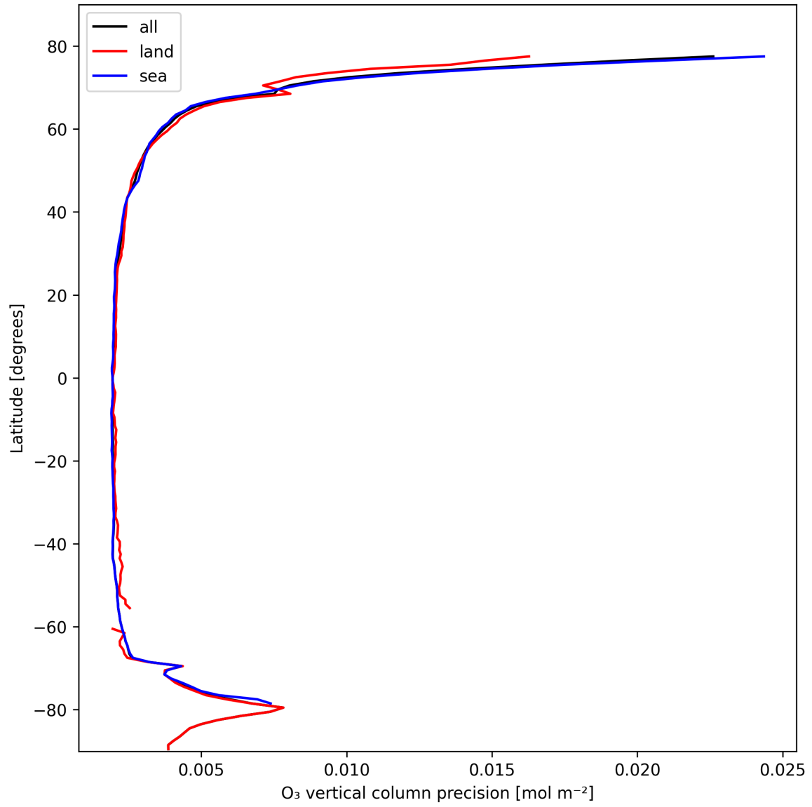
Figure 18: Zonal average of “O 3 vertical column precision” for 2025-02-18 to 2025-02-19.
