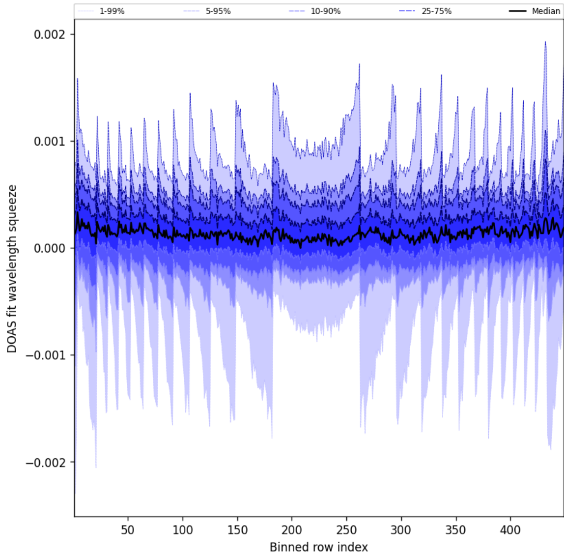
Figure 48: Along track statistics of “DOAS fit wavelength squeeze” for 2025-02-18 to 2025-02-19
