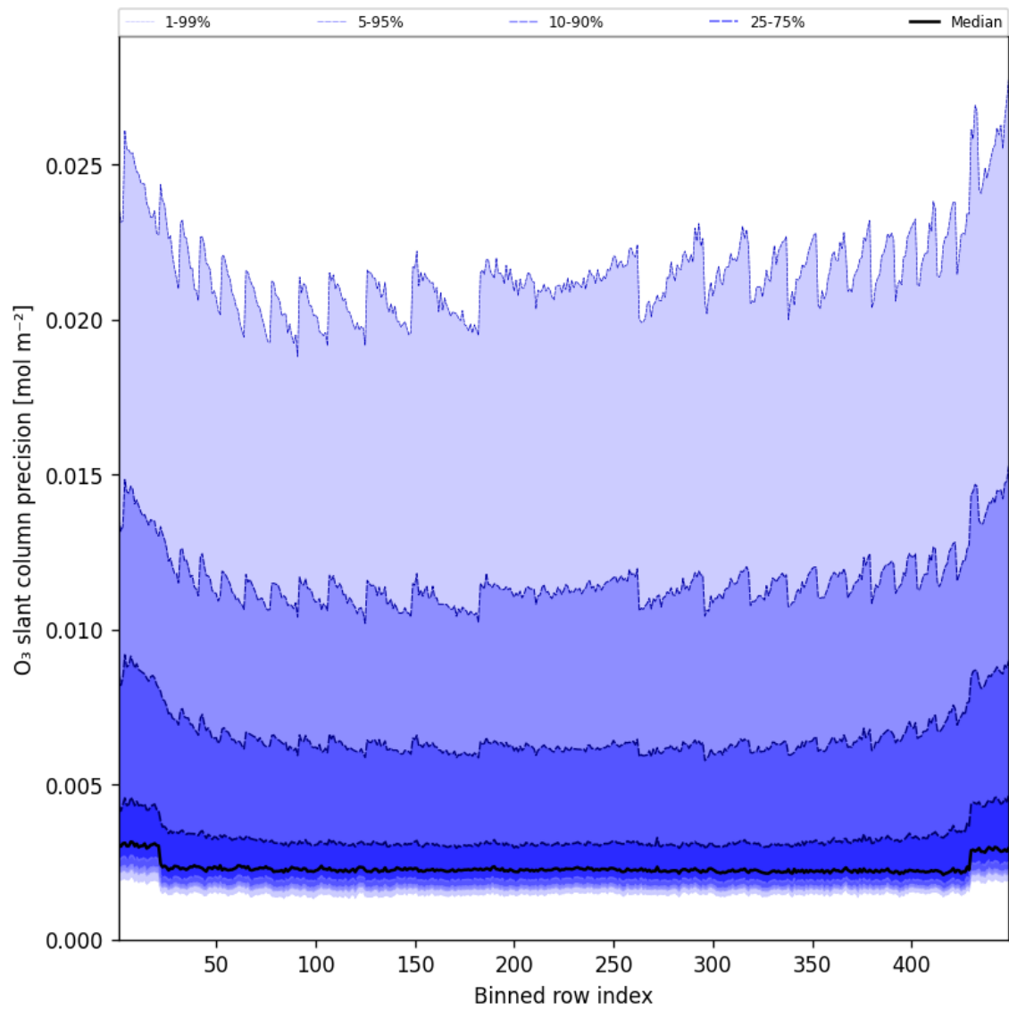
Figure 44: Along track statistics of “O 3 slant column precision” for 2025-02-18 to 2025-02-19
