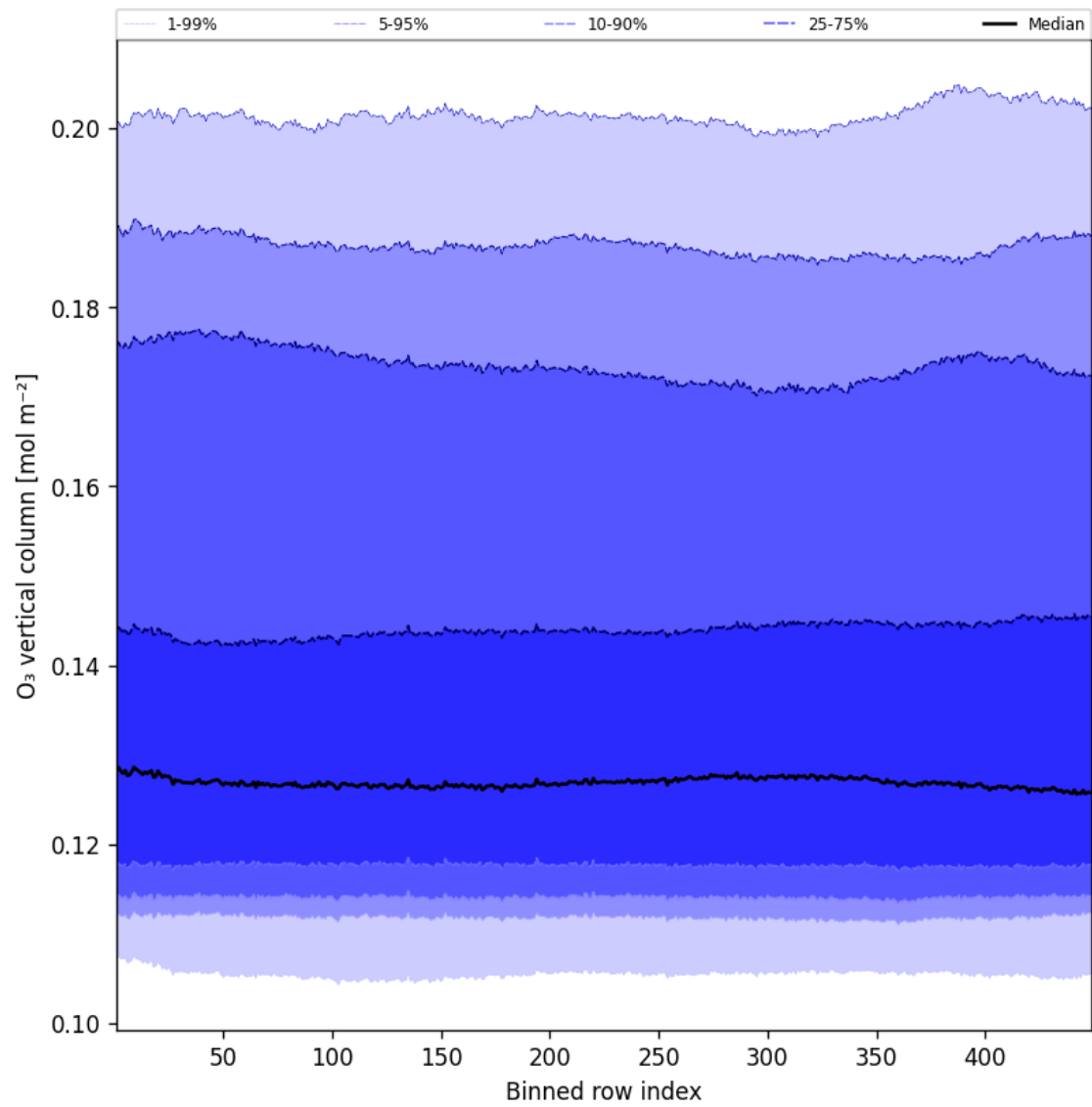
Figure 41: Along track statistics of “O 3 vertical column” for 2025-02-18 to 2025-02-19
