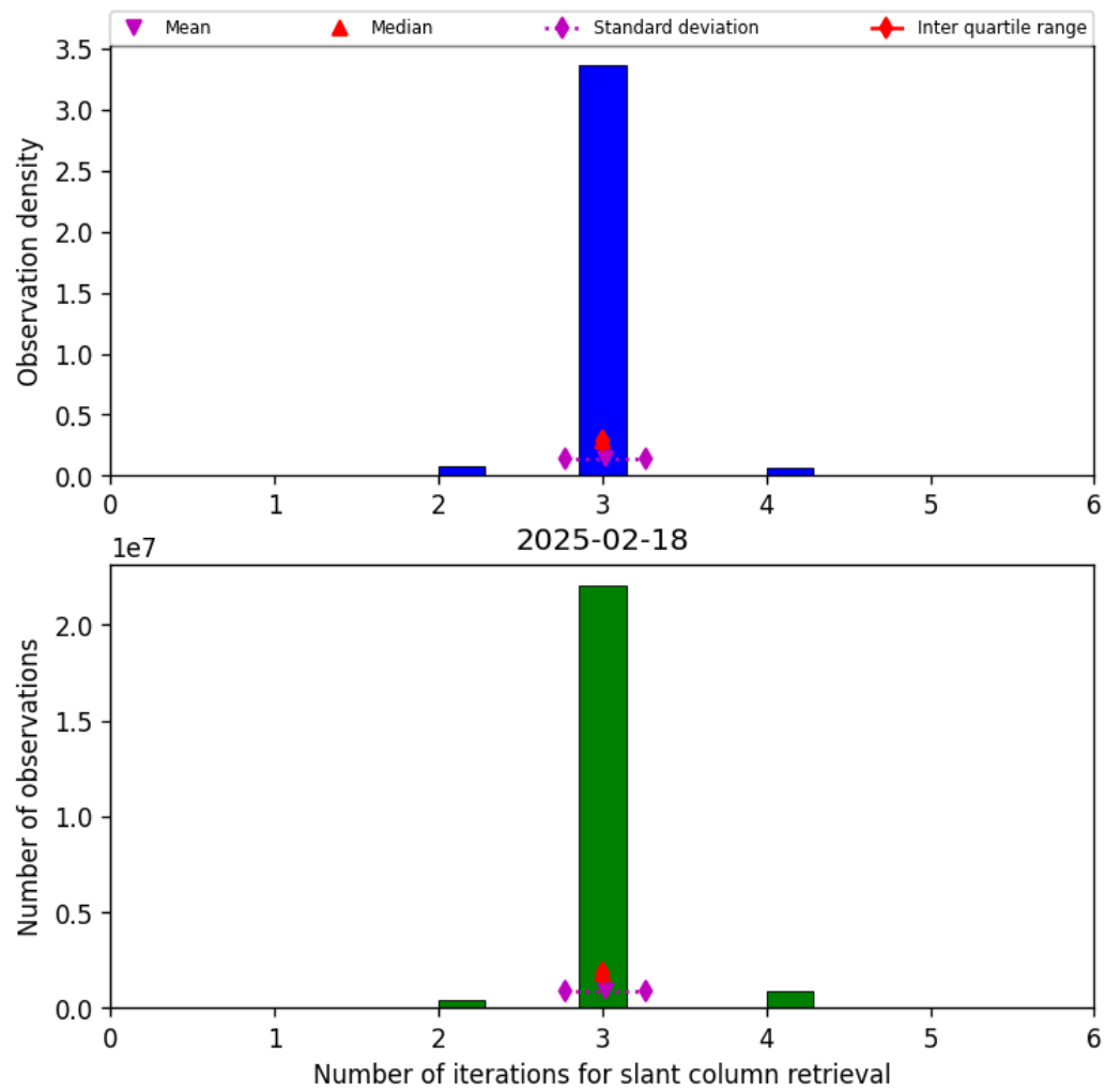
Figure 33: Histogram of “Number of iterations for slant column retrieval” for 2025-02-18 to 2025-02-19
