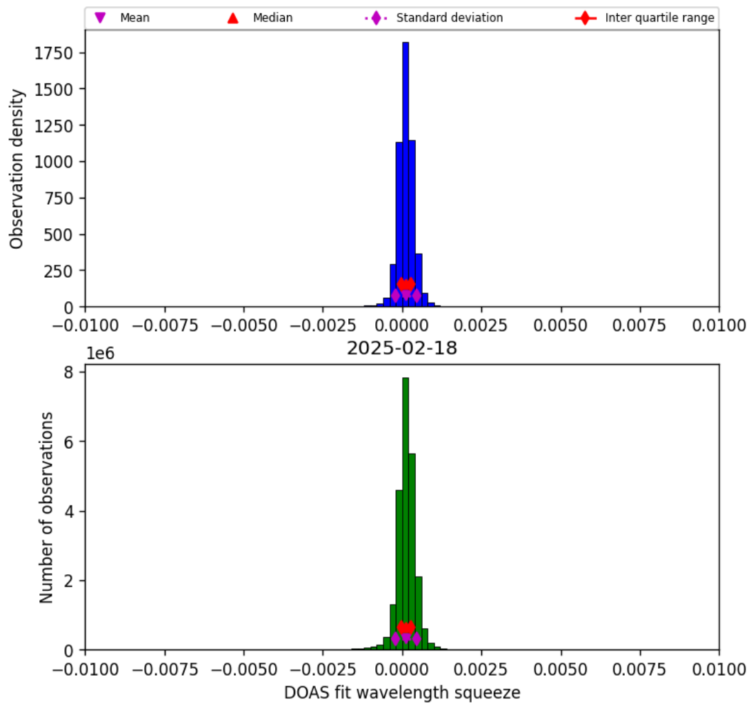
Figure 36: Histogram of “DOAS fit wavelength squeeze” for 2025-02-18 to 2025-02-19
