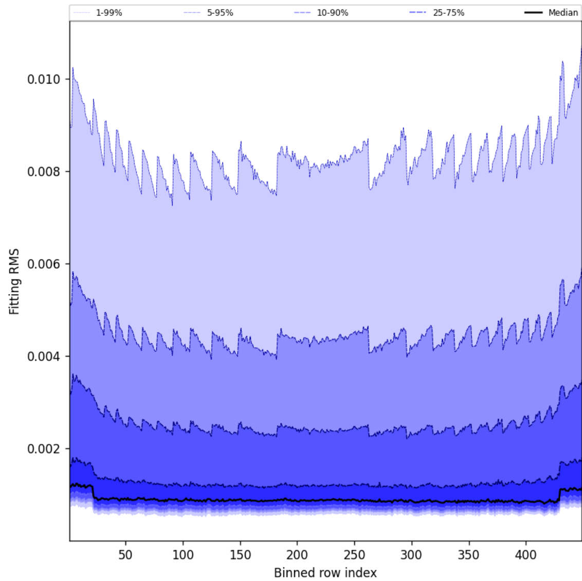
Figure 46: Along track statistics of “Fitting RMS” for 2025-02-18 to 2025-02-19
