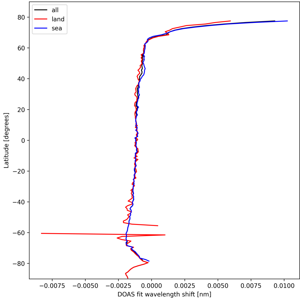
Figure 23: Zonal average of “DOAS fit wavelength shift” for 2025-02-18 to 2025-02-19.
