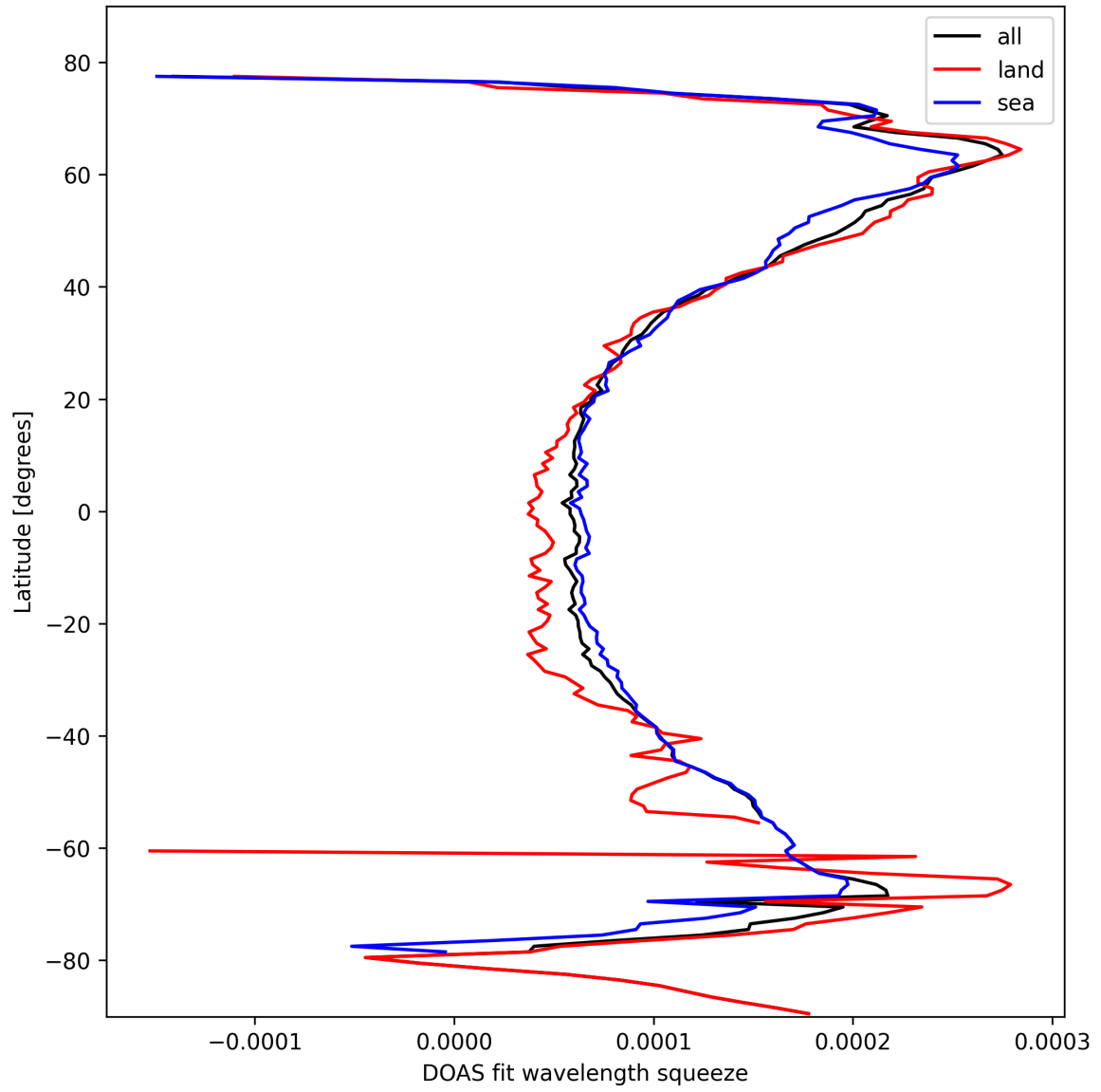
Figure 24: Zonal average of “DOAS fit wavelength squeeze” for 2025-02-18 to 2025-02-19.
