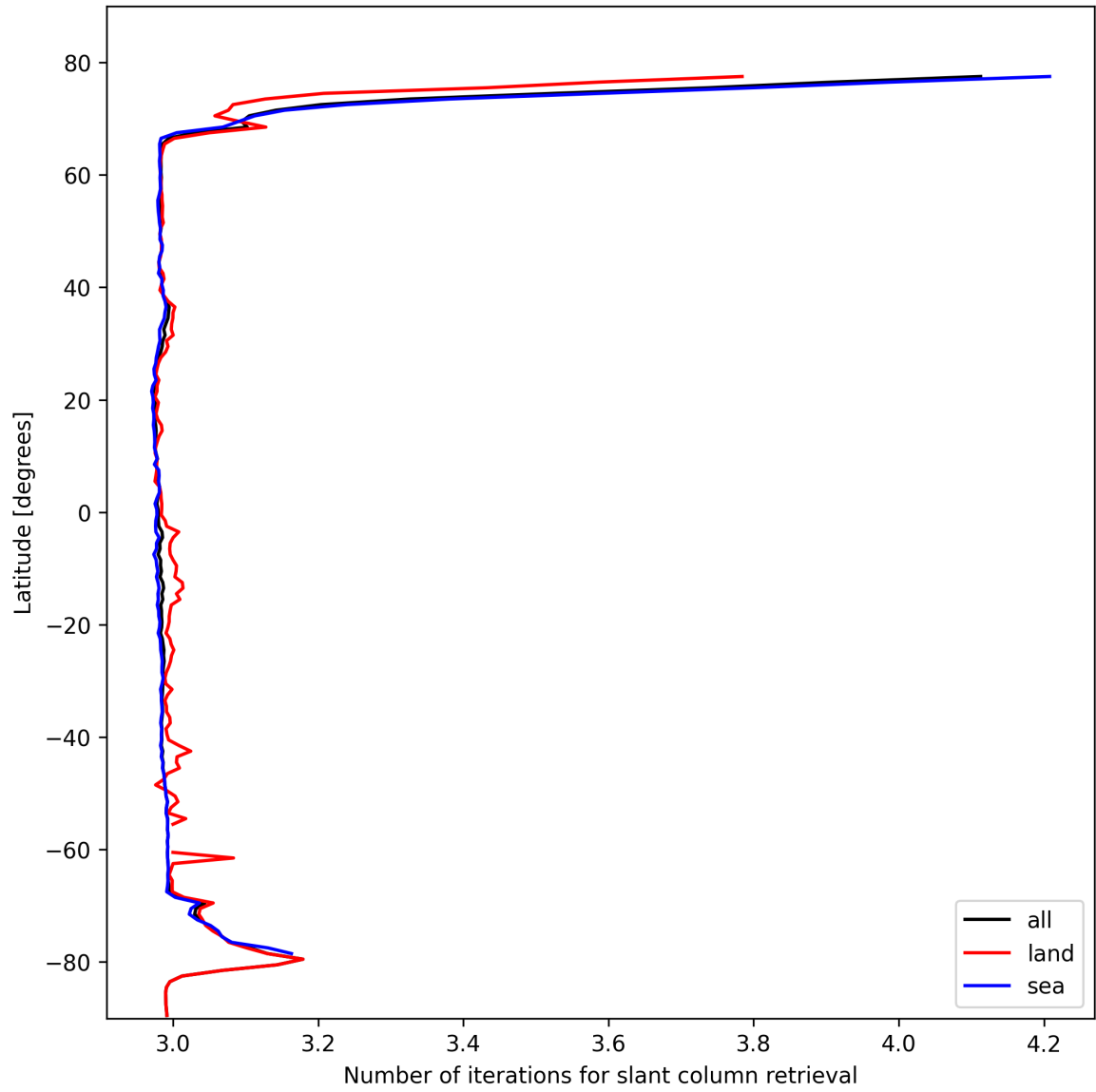
Figure 21: Zonal average of “Number of iterations for slant column retrieval” for 2025-02-18 to 2025-02-19.
