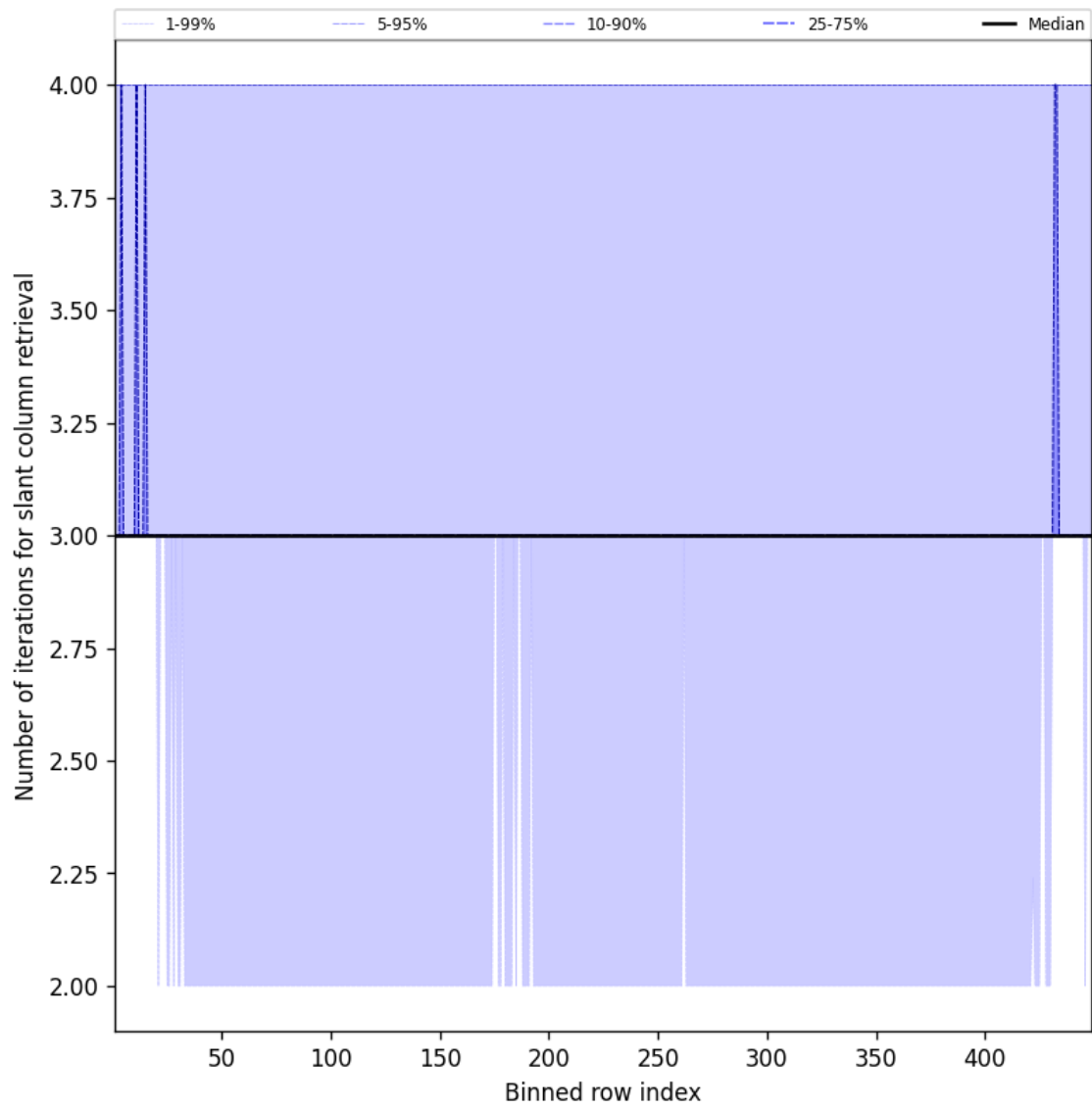
Figure 45: Along track statistics of “Number of iterations for slant column retrieval” for 2025-02-18 to 2025-02-19
