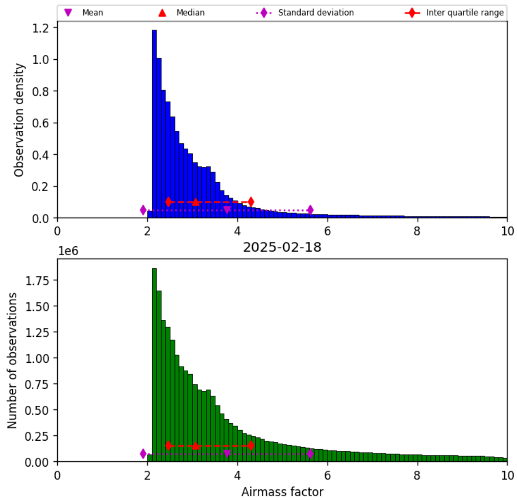
Figure 37: Histogram of “Airmass factor” for 2025-02-18 to 2025-02-19
