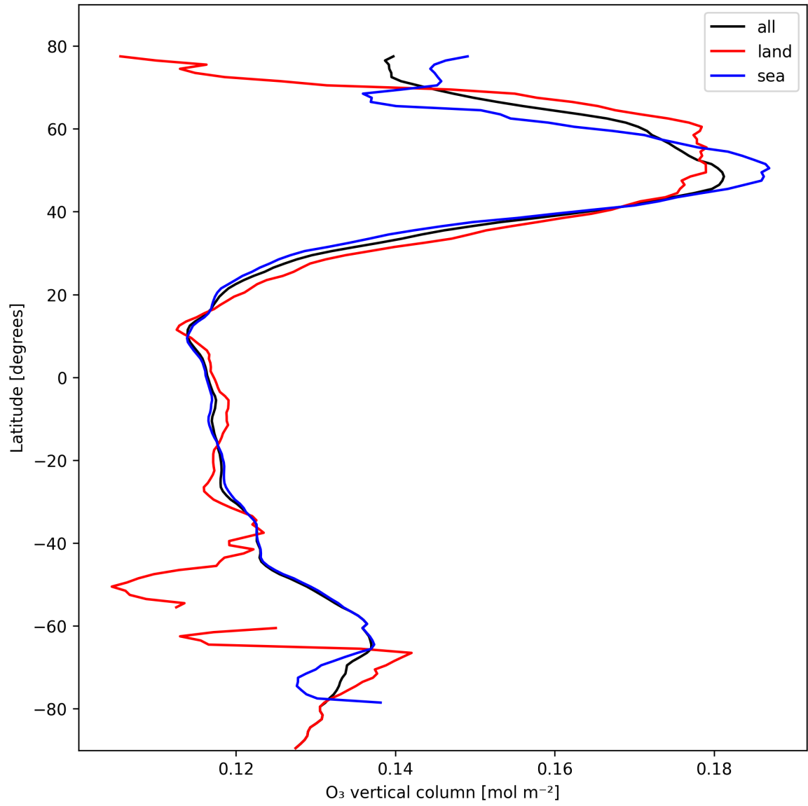
Figure 17: Zonal average of “O 3 vertical column” for 2025-02-18 to 2025-02-19.
