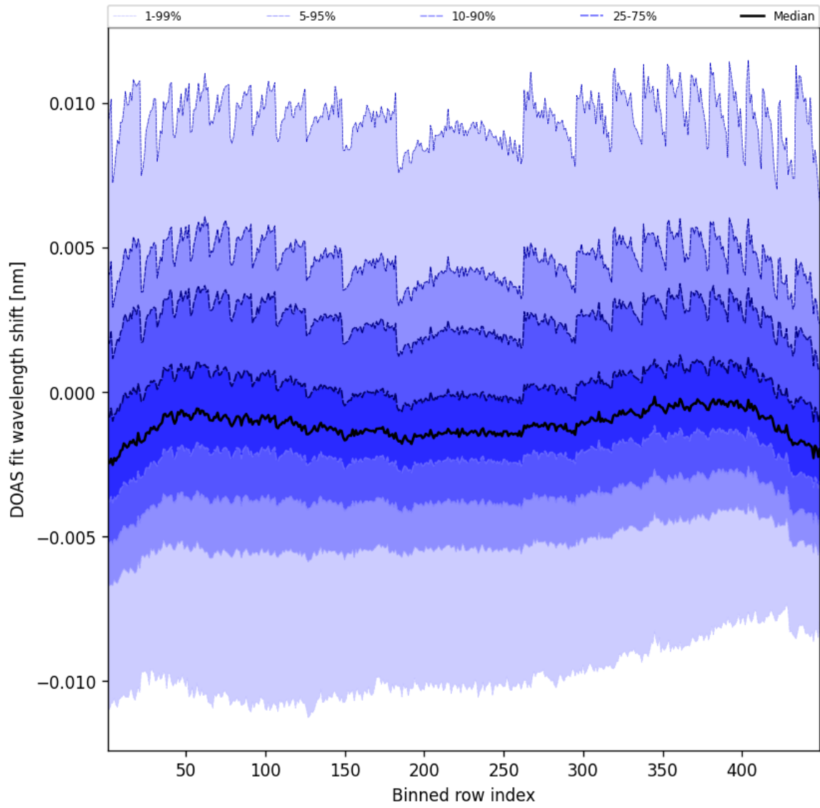
Figure 47: Along track statistics of “DOAS fit wavelength shift” for 2025-02-18 to 2025-02-19
