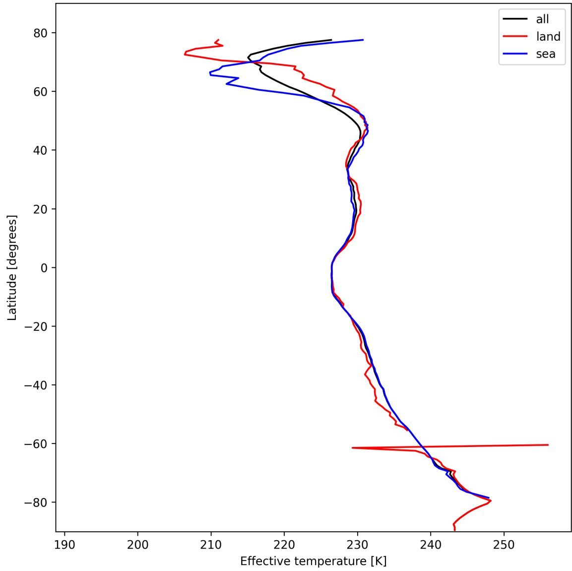
Figure 26: Zonal average of "Effective temperature" for 2025-02-18 to 2025-02-19.
