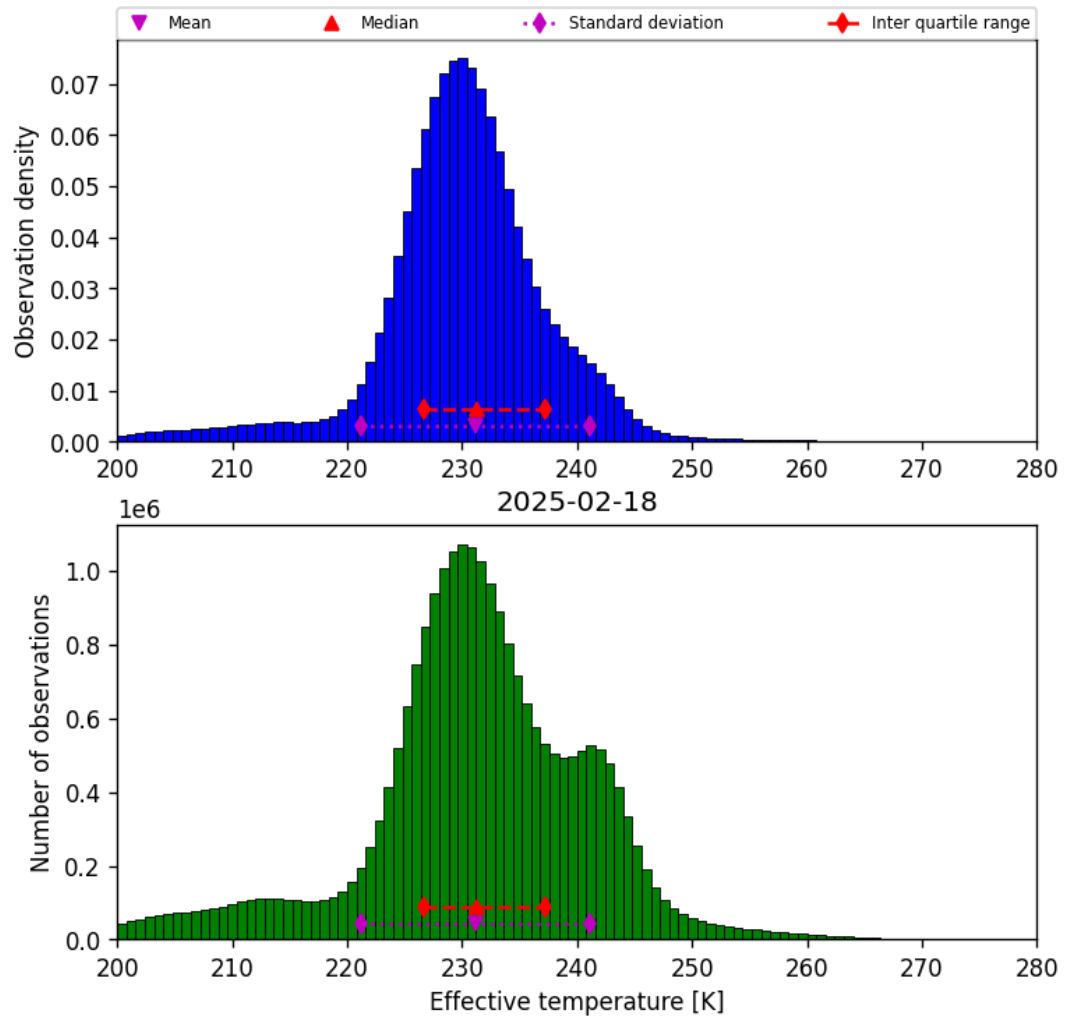
Figure 38: Histogram of “Effective temperature” for 2025-02-18 to 2025-02-19
