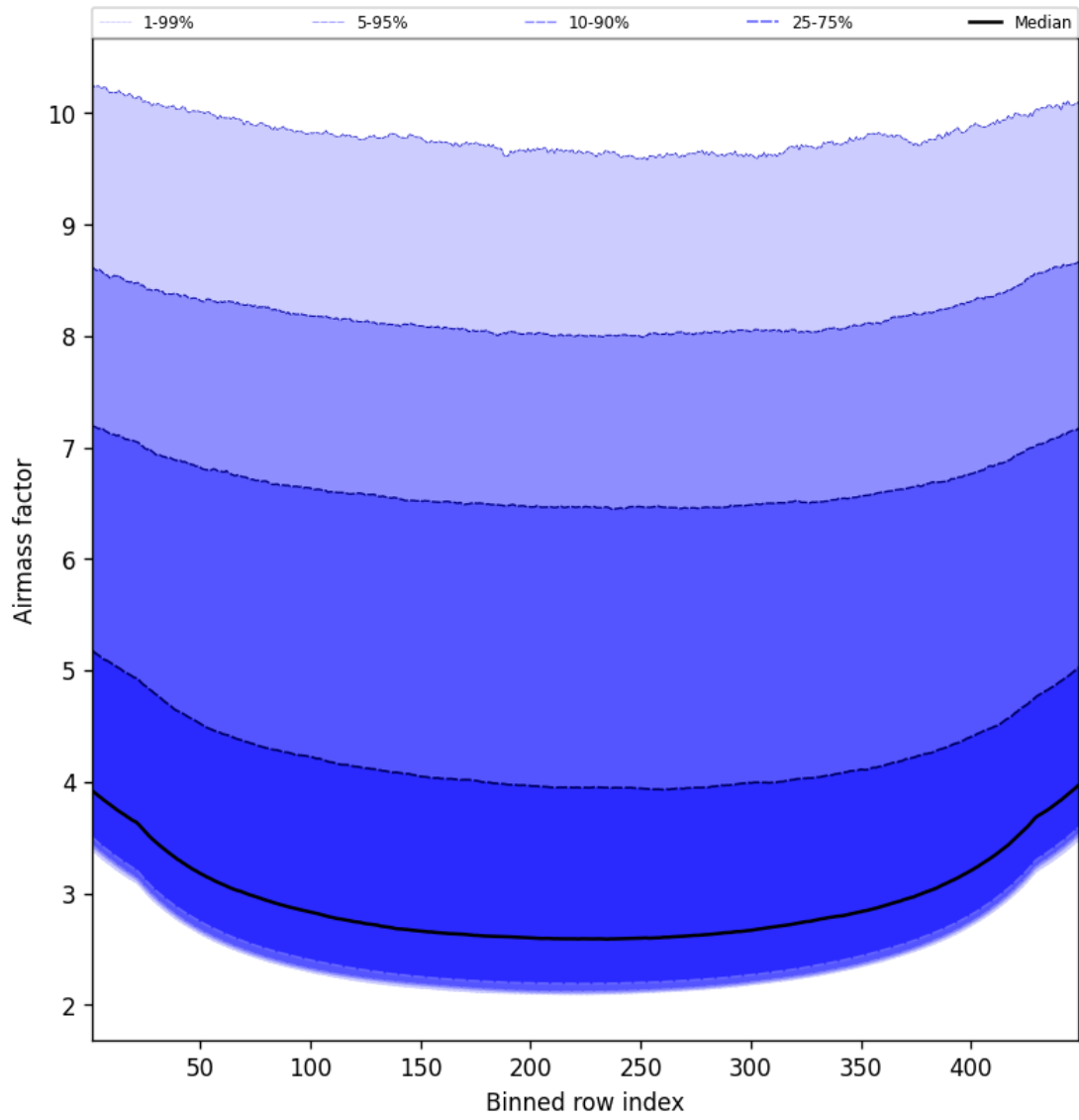
Figure 49: Along track statistics of “Airmass factor” for 2025-02-18 to 2025-02-19
