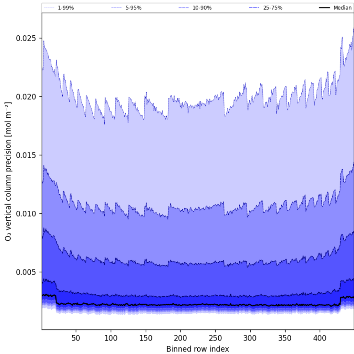
Figure 42: Along track statistics of “O 3 vertical column precision” for 2025-02-18 to 2025-02-19
