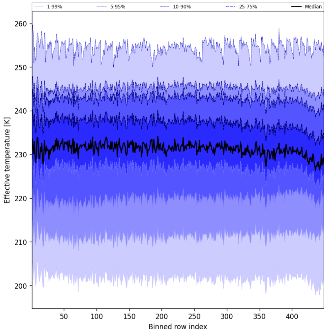
Figure 50: Along track statistics of “Effective temperature” for 2025-02-18 to 2025-02-19
