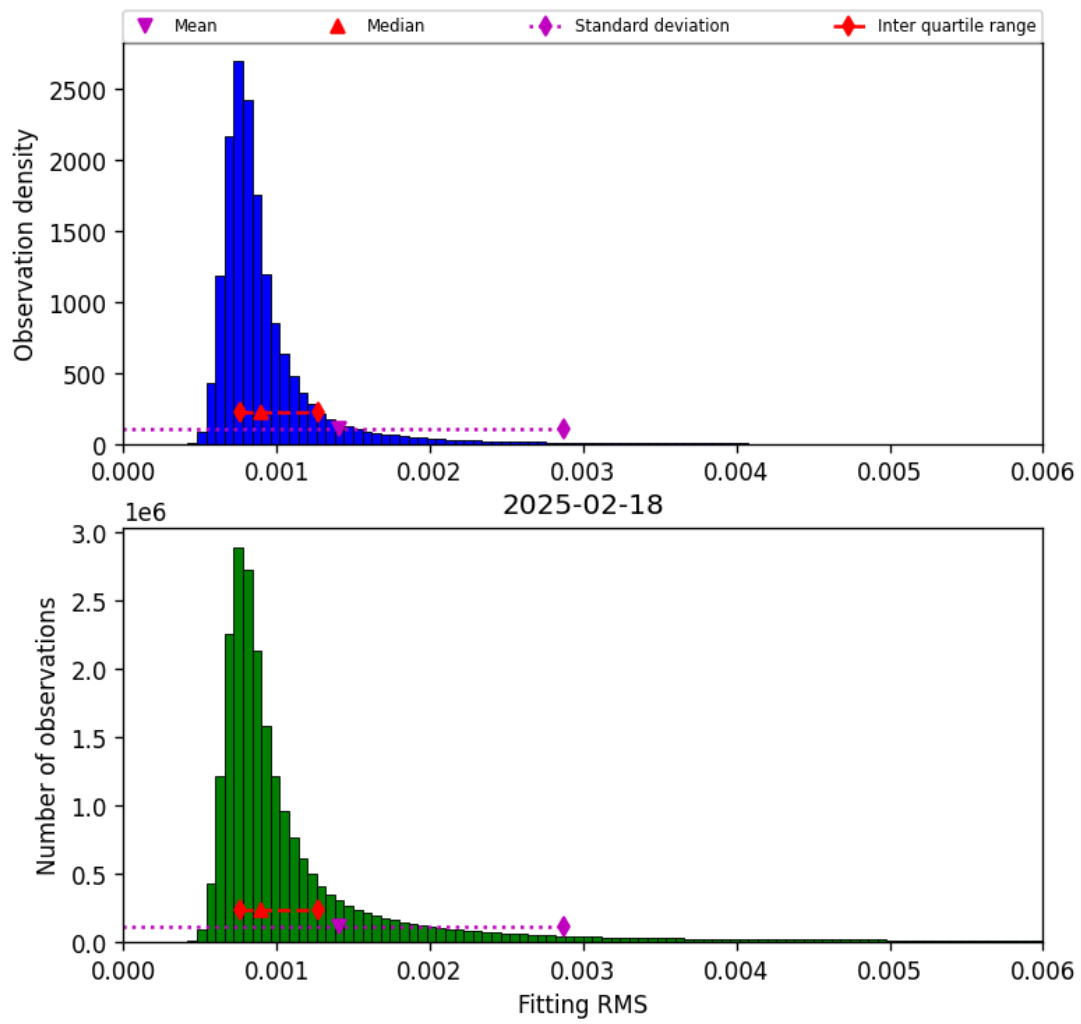
Figure 34: Histogram of “Fitting RMS” for 2025-02-18 to 2025-02-19
