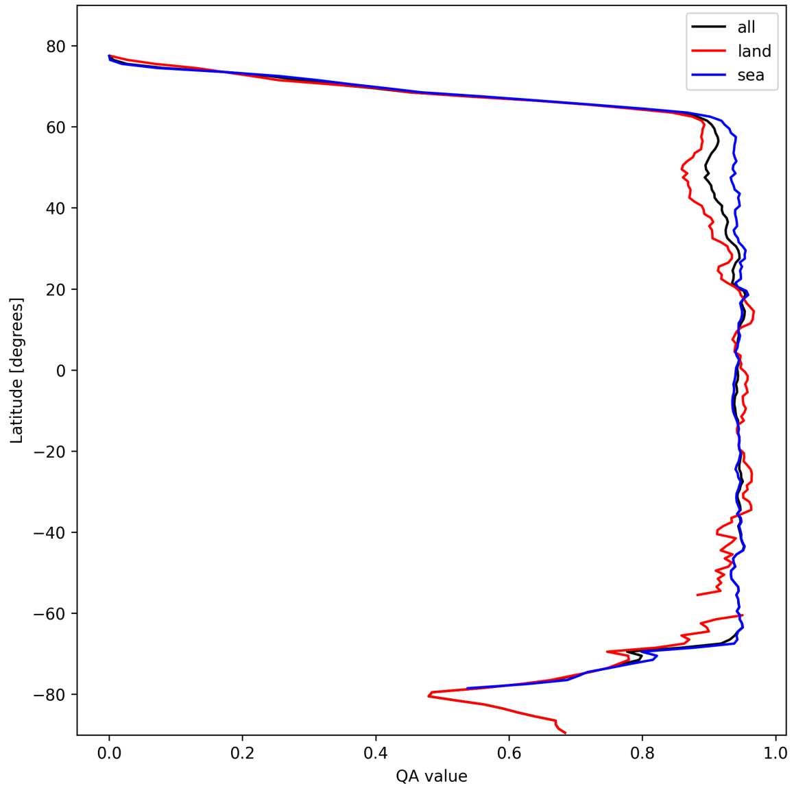
Figure 16: Zonal average of “QA value” for 2025-02-18 to 2025-02-19.
