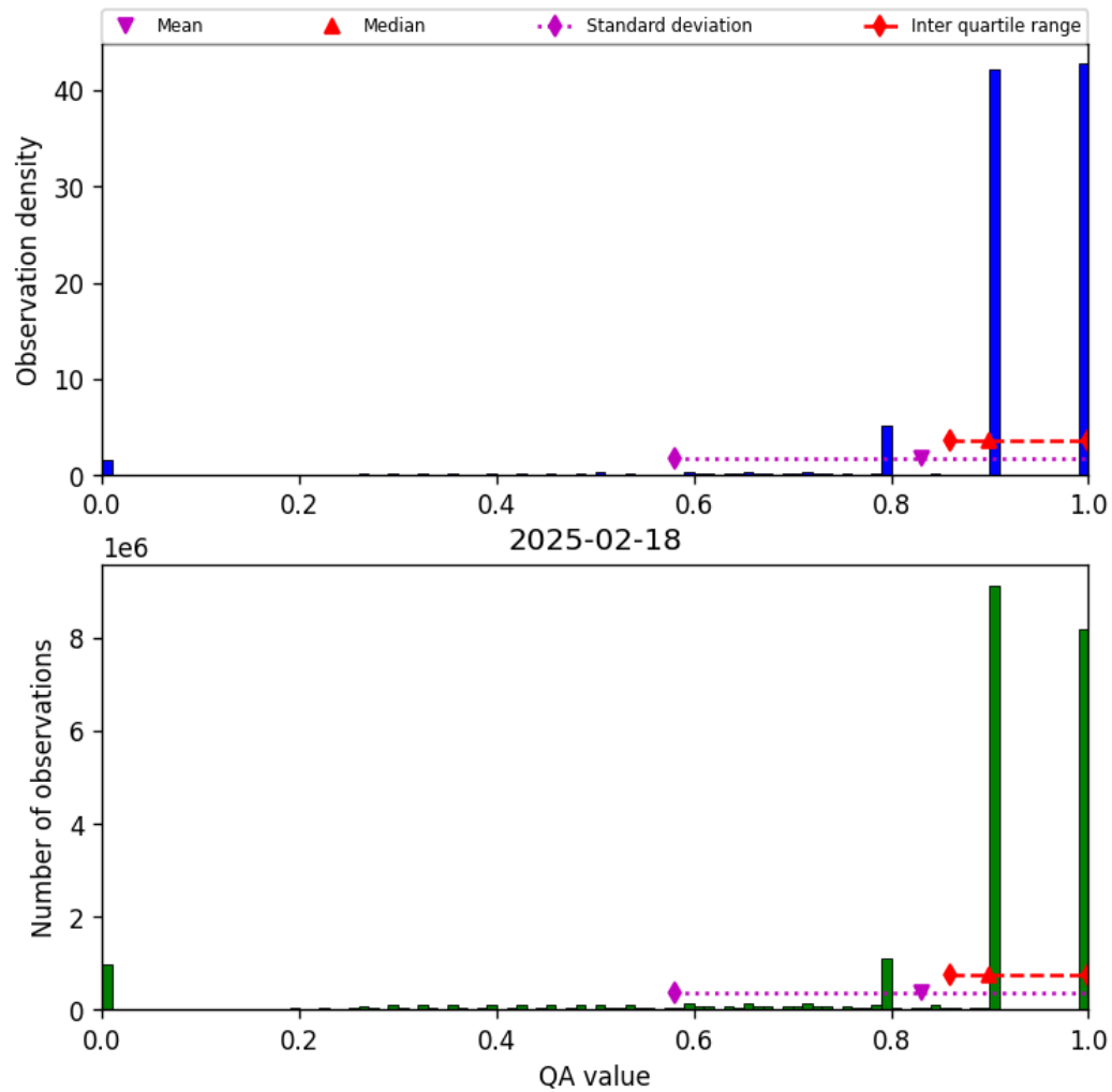
Figure 28: Histogram of “QA value” for 2025-02-18 to 2025-02-19
