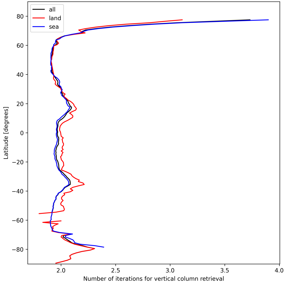
Figure 27: Zonal average of “Number of iterations for vertical column retrieval” for 2025-02-18 to 2025-02-19.
