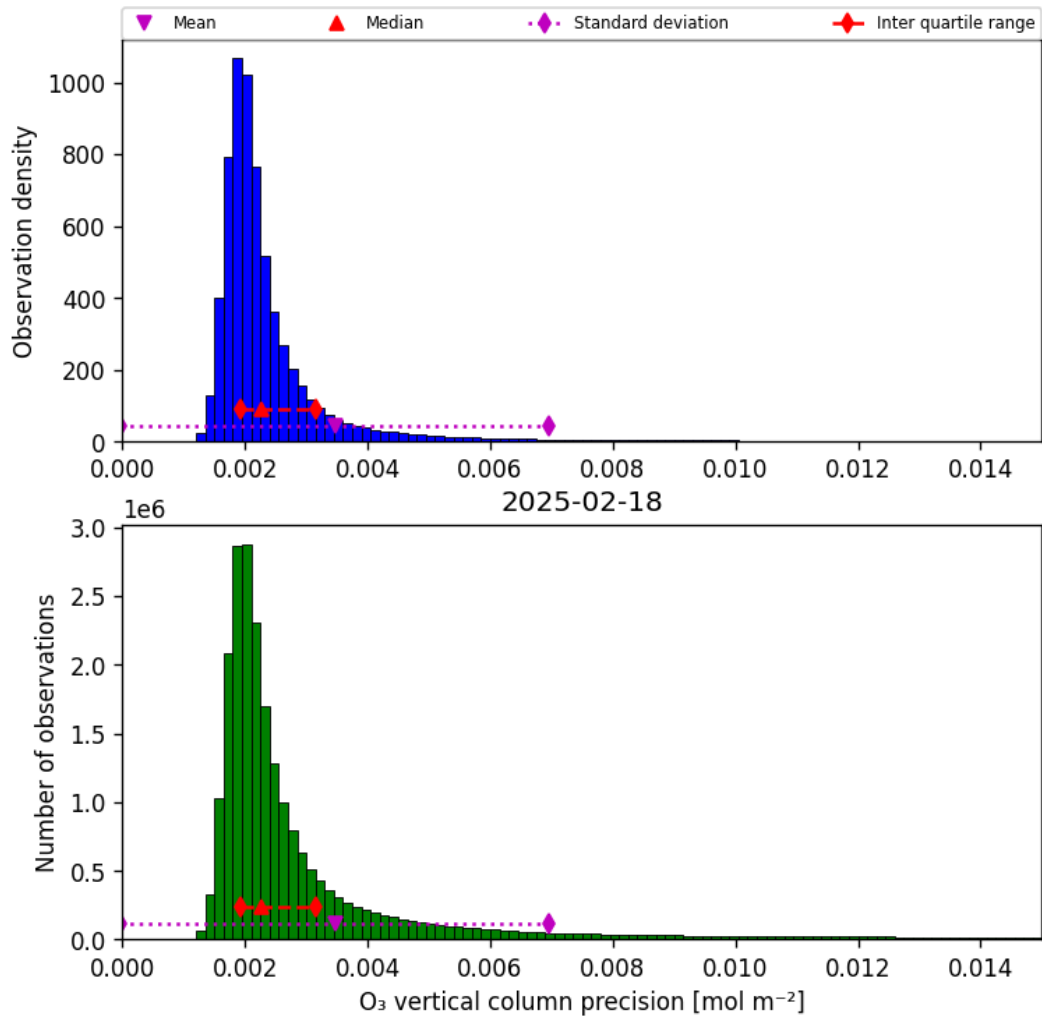
Figure 30: Histogram of “O 3 vertical column precision” for 2025-02-18 to 2025-02-19
