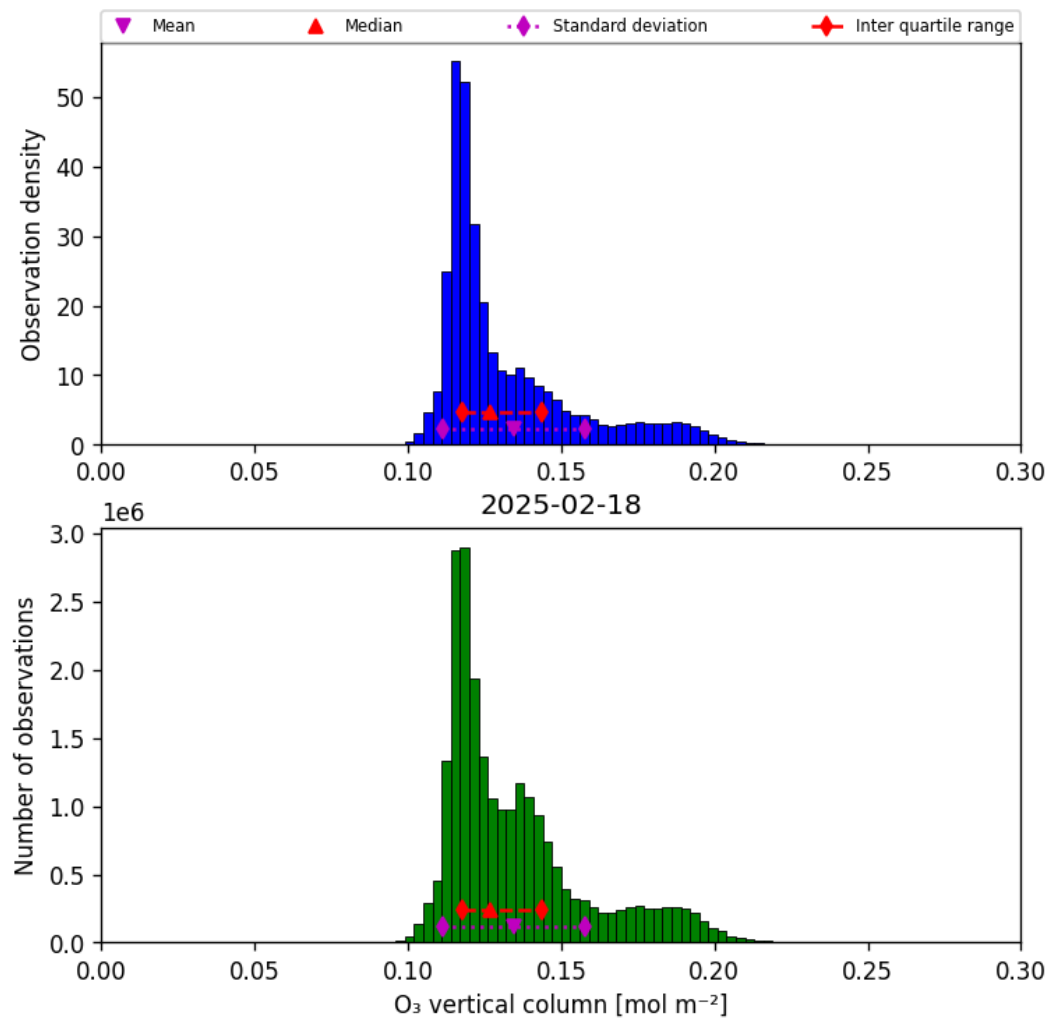
Figure 29: Histogram of “O 3 vertical column” for 2025-02-18 to 2025-02-19
