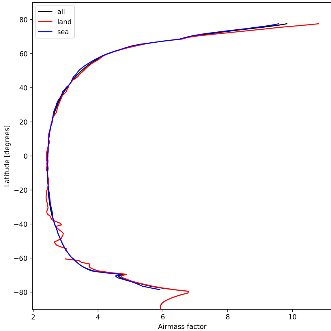
Figure 25: Zonal average of “Airmass factor” for 2025-02-18 to 2025-02-19.
