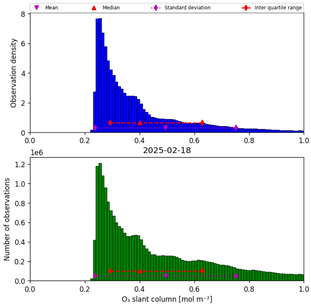
Figure 31: Histogram of “O 3 slant column” for 2025-02-18 to 2025-02-19
