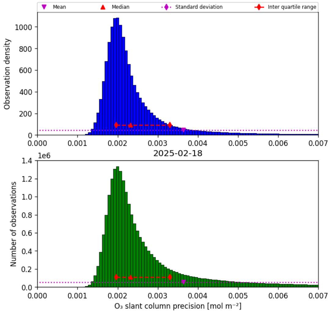
Figure 32: Histogram of "O 3 slant column precision" for 2025-02-18 to 2025-02-19
