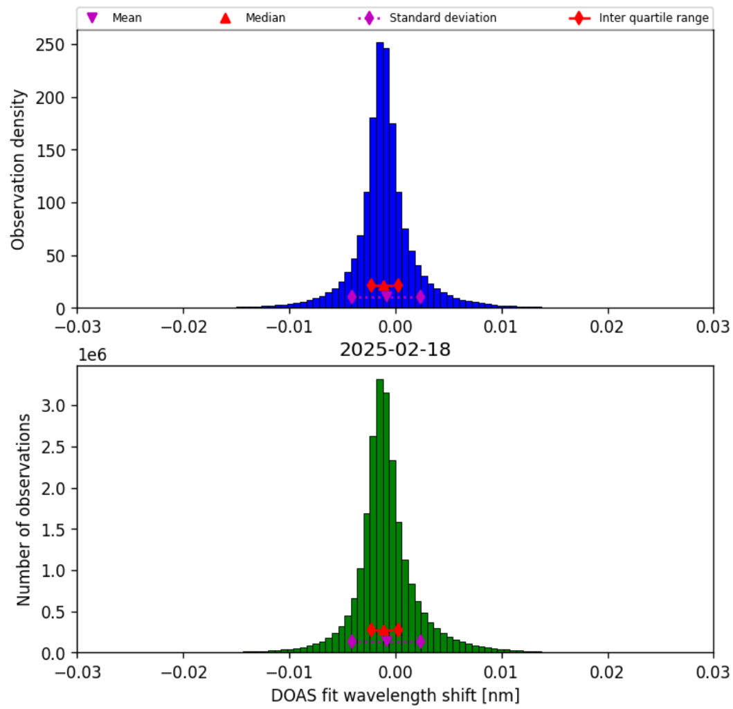
Figure 35: Histogram of “DOAS fit wavelength shift” for 2025-02-18 to 2025-02-19
