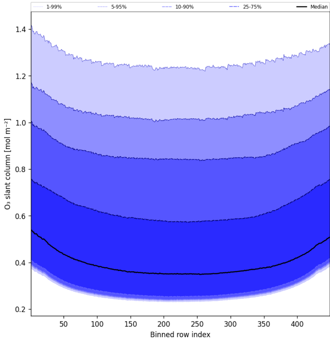
Figure 43: Along track statistics of “O 3 slant column” for 2025-02-18 to 2025-02-19
