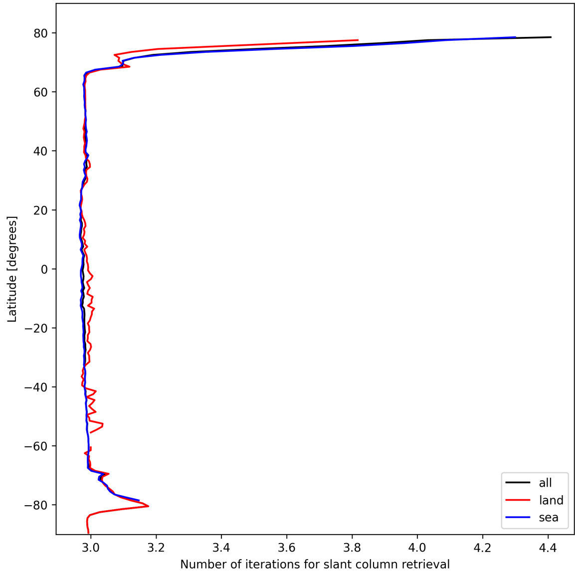
Figure 21: Zonal average of “Number of iterations for slant column retrieval” for 2025-02-19 to 2025-02-20.
