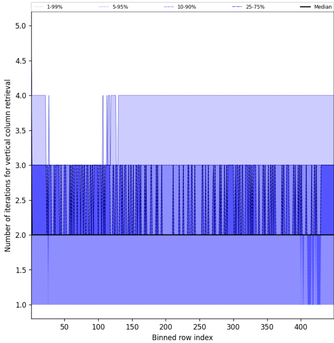
Figure 51: Along track statistics of “Number of iterations for vertical column retrieval” for 2025-02-19 to 2025-02-20
