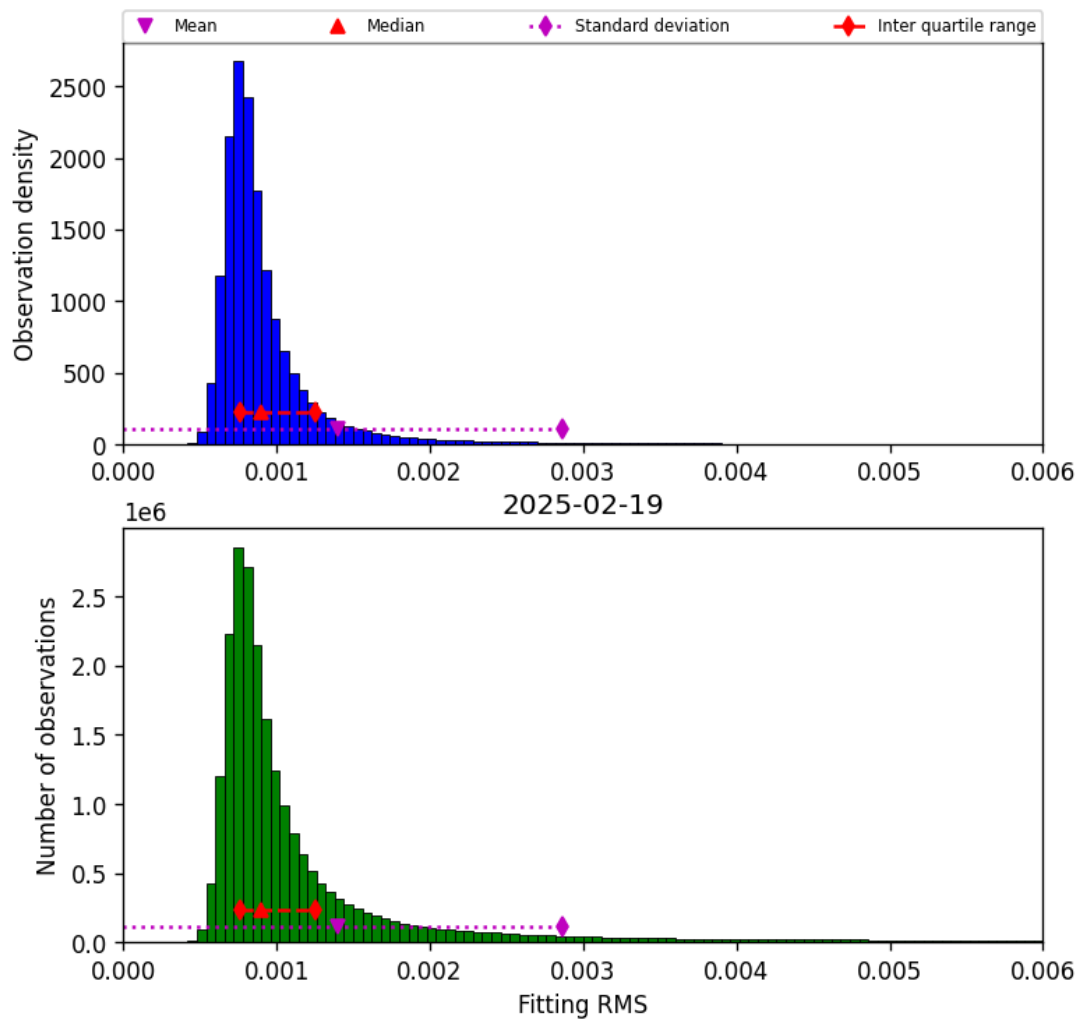
Figure 34: Histogram of “Fitting RMS” for 2025-02-19 to 2025-02-20
