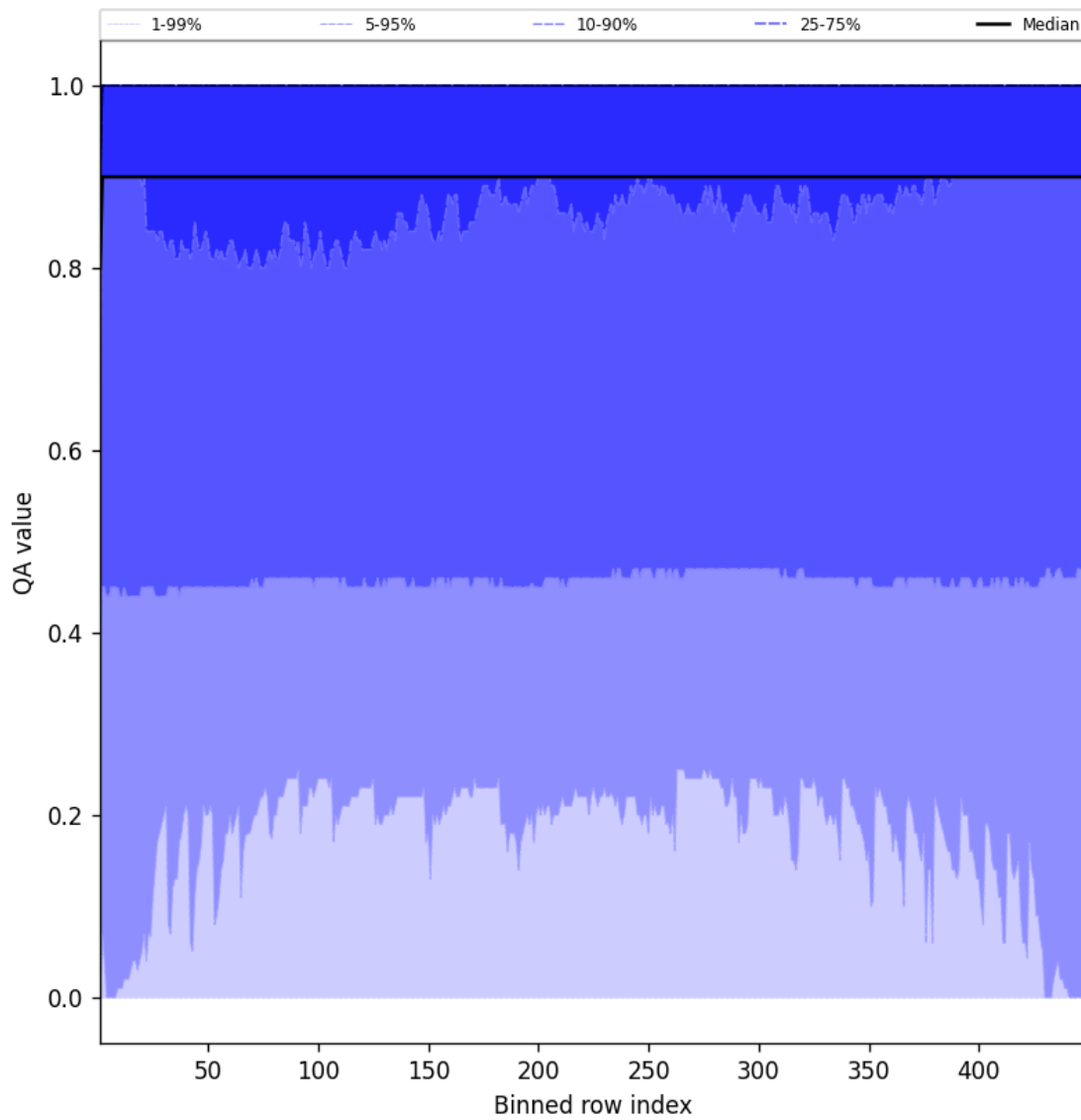
Figure 40: Along track statistics of “QA value” for 2025-02-19 to 2025-02-20
