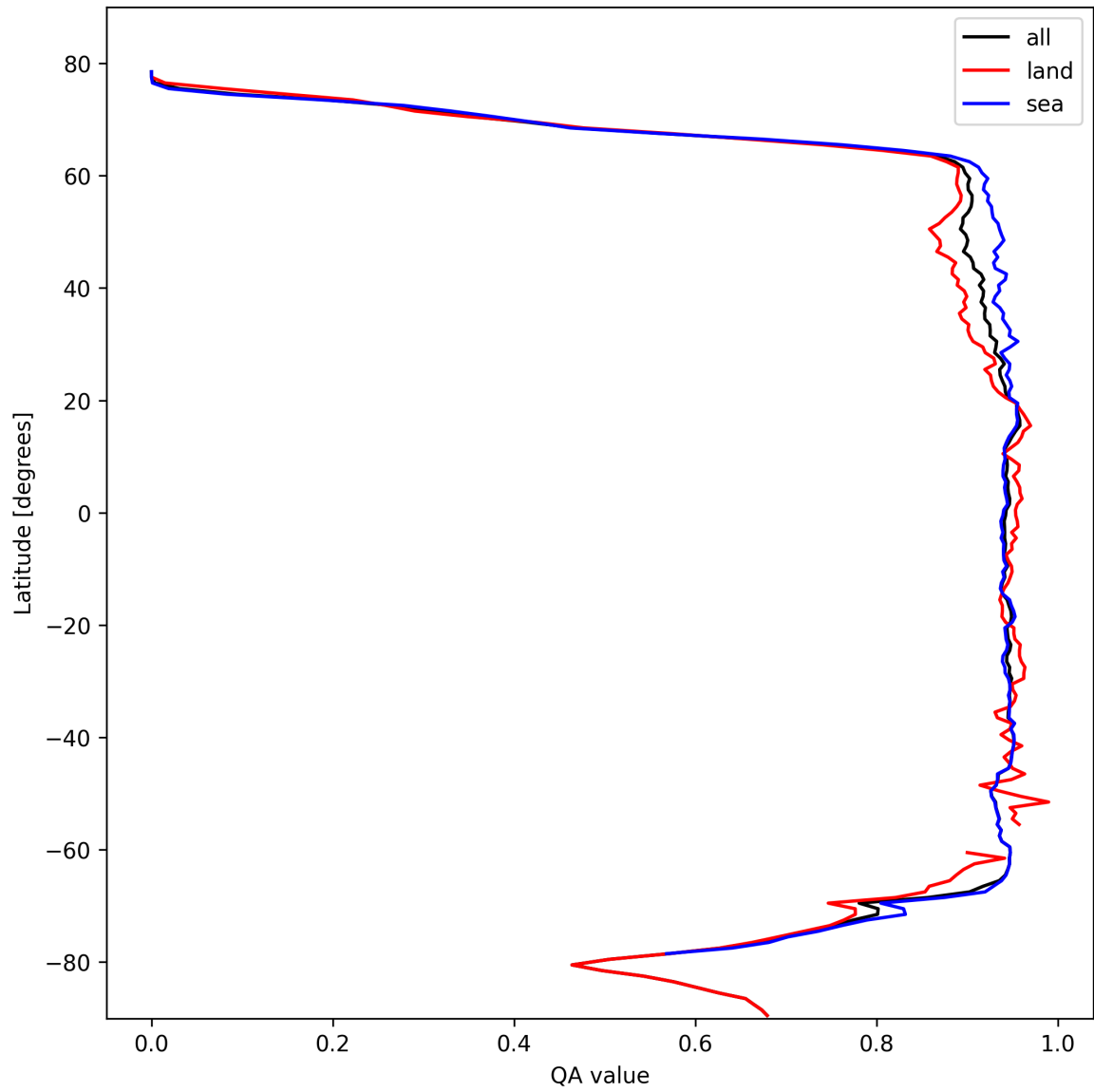
Figure 16: Zonal average of “QA value” for 2025-02-19 to 2025-02-20.
