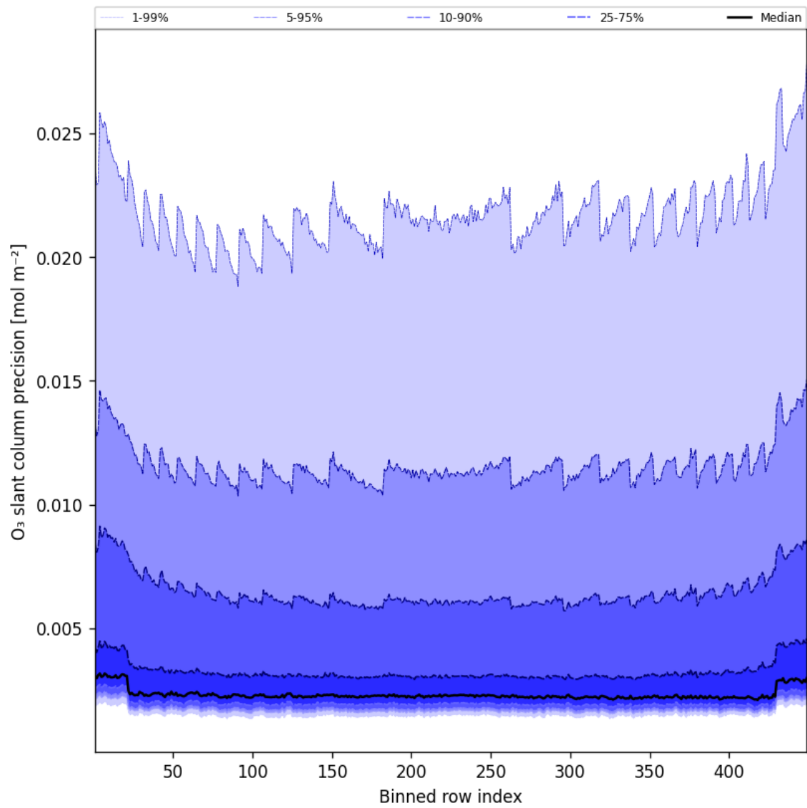
Figure 44: Along track statistics of “O 3 slant column precision” for 2025-02-19 to 2025-02-20
