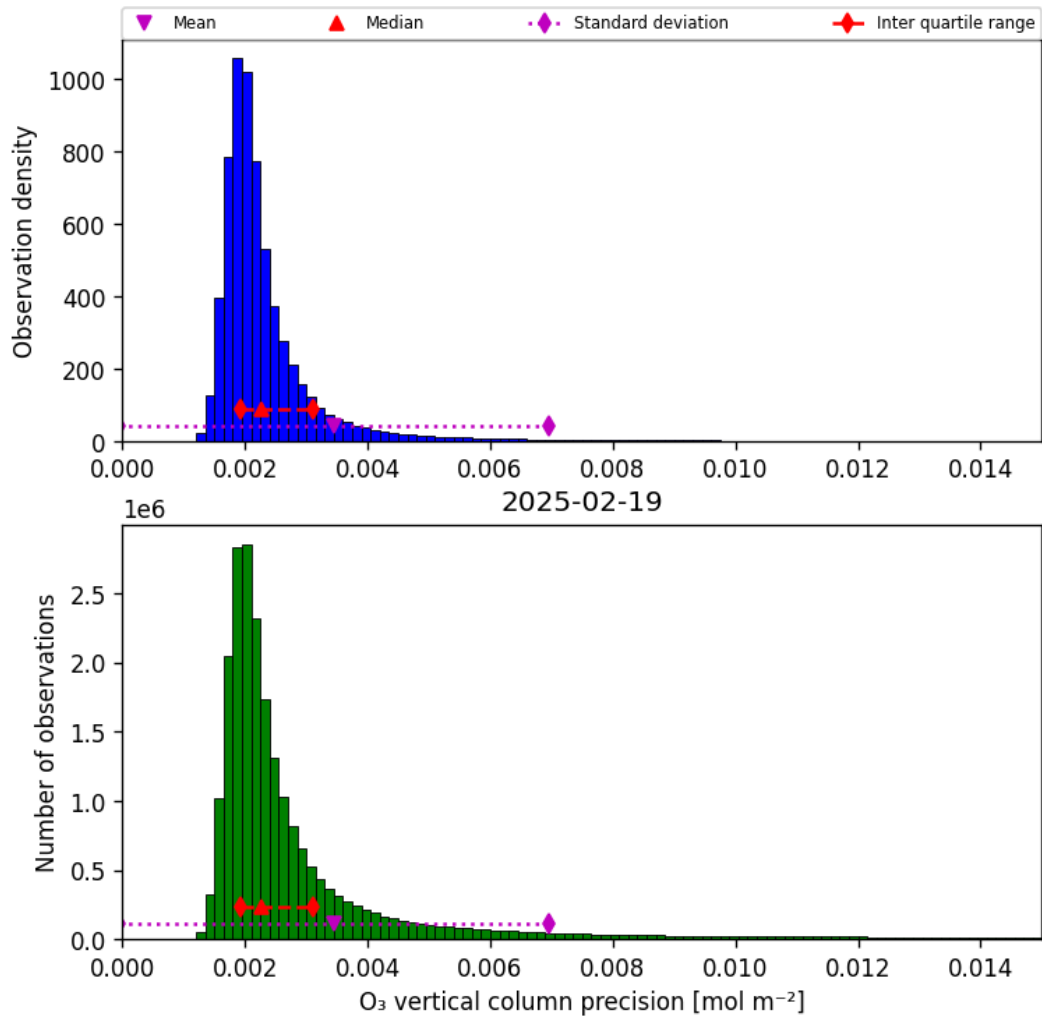
Figure 30: Histogram of “O 3 vertical column precision” for 2025-02-19 to 2025-02-20
