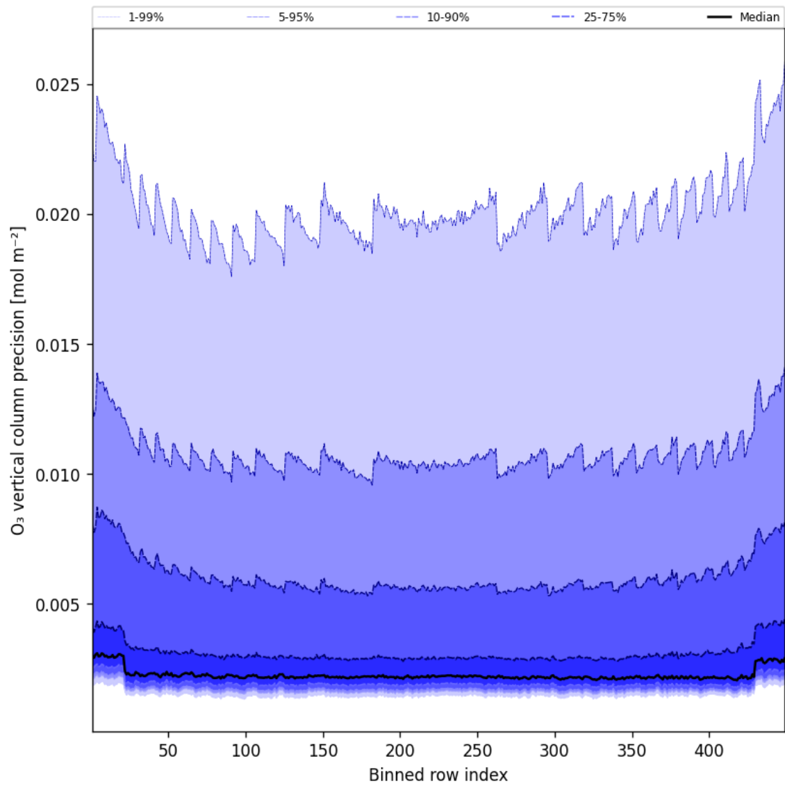
Figure 42: Along track statistics of “O 3 vertical column precision” for 2025-02-19 to 2025-02-20
