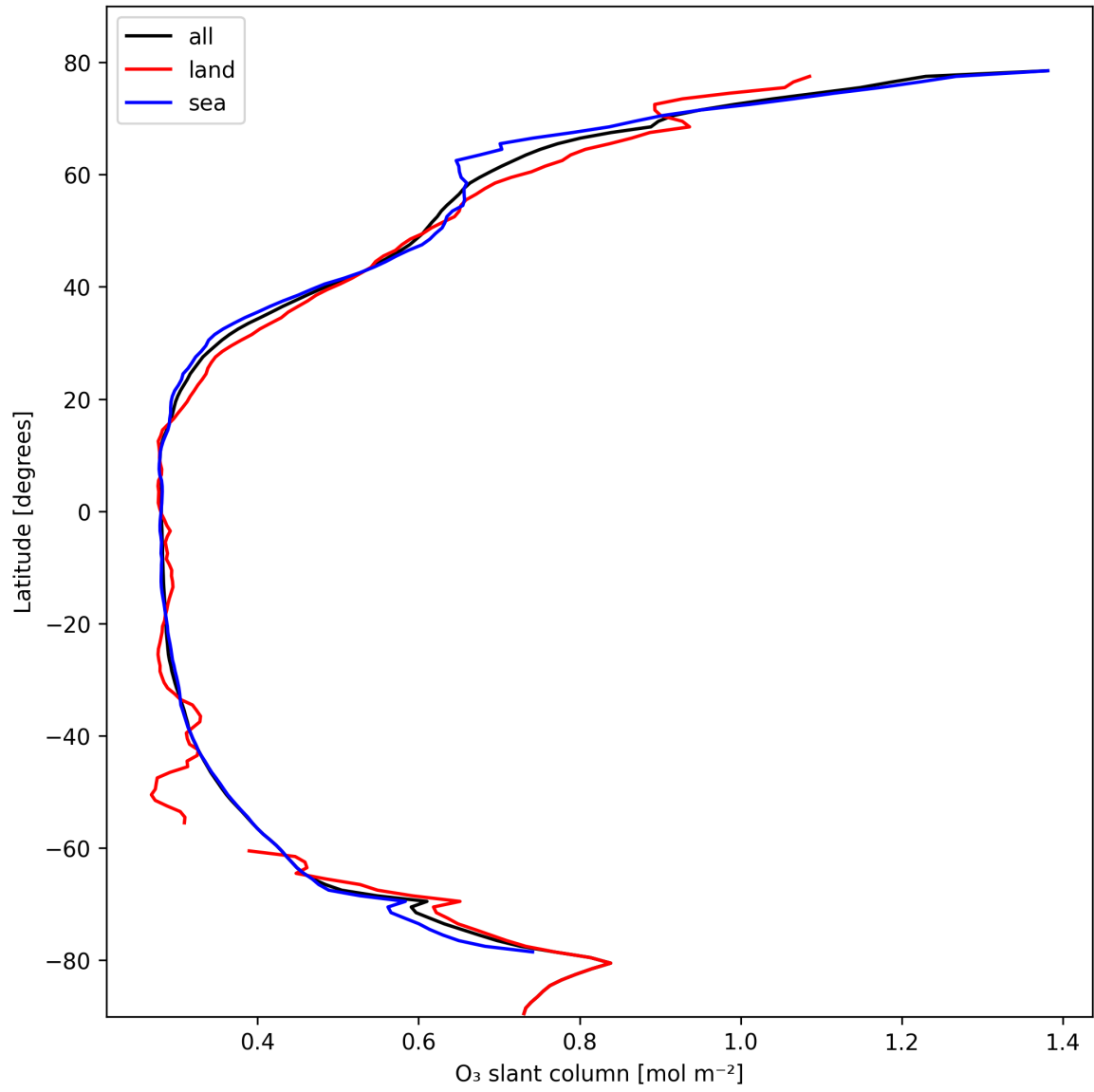
Figure 19: Zonal average of “O 3 slant column” for 2025-02-19 to 2025-02-20.
