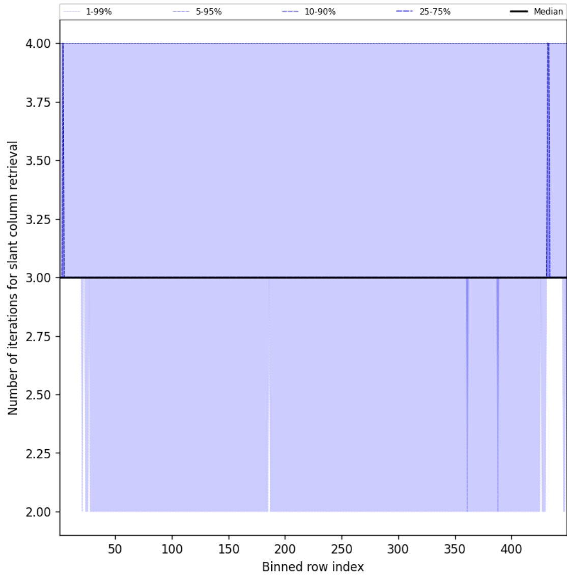
Figure 45: Along track statistics of “Number of iterations for slant column retrieval” for 2025-02-19 to 2025-02-20
