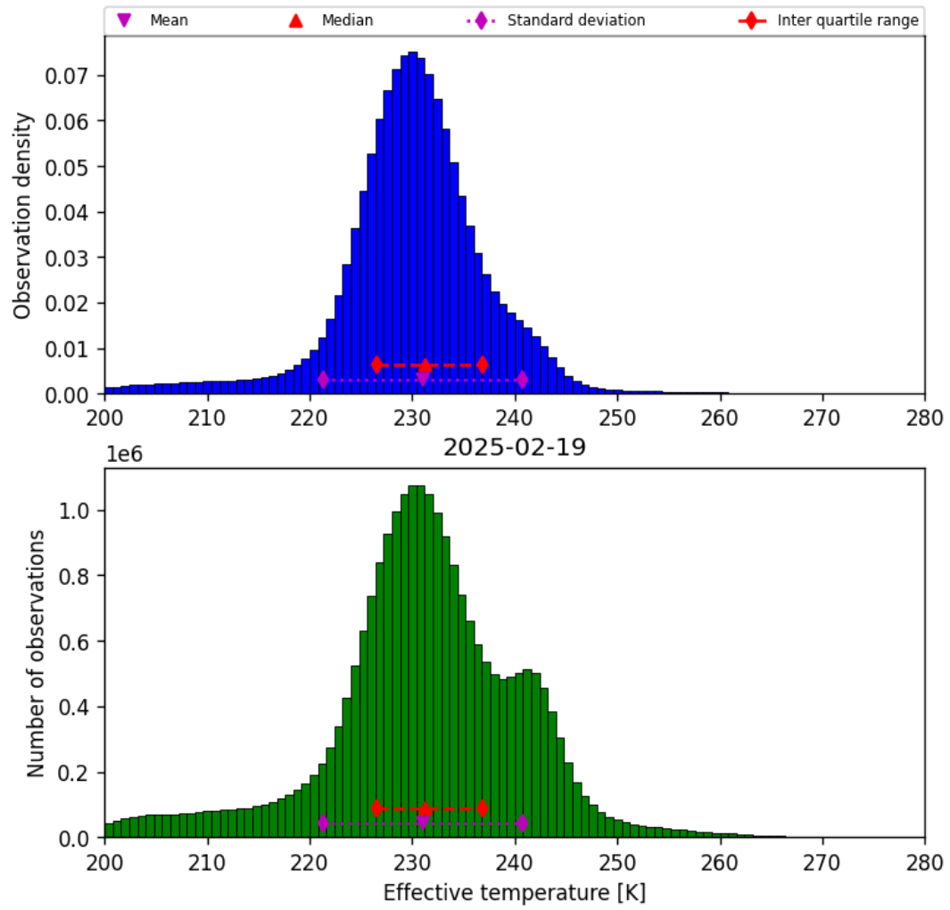
Figure 38: Histogram of “Effective temperature” for 2025-02-19 to 2025-02-20
