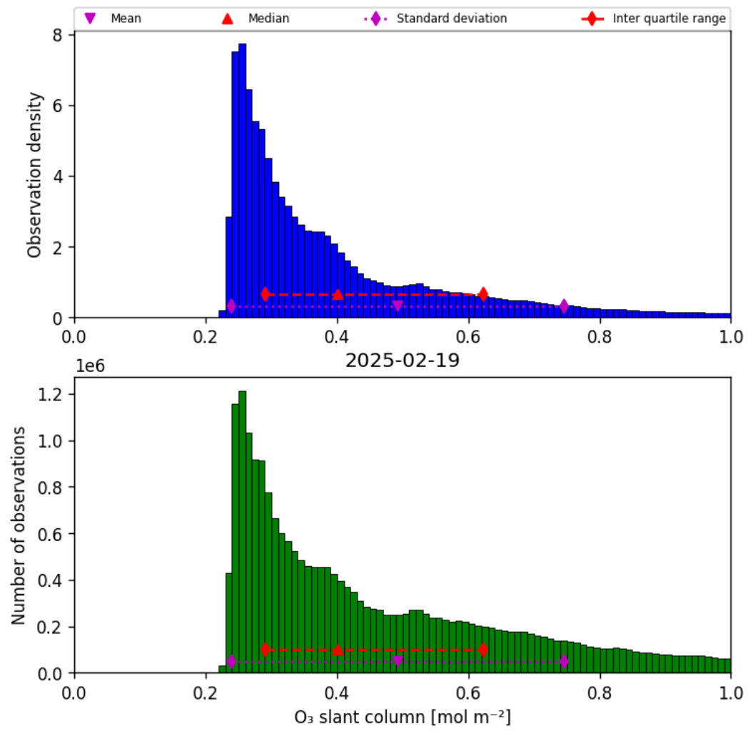
Figure 31: Histogram of “O 3 slant column” for 2025-02-19 to 2025-02-20
