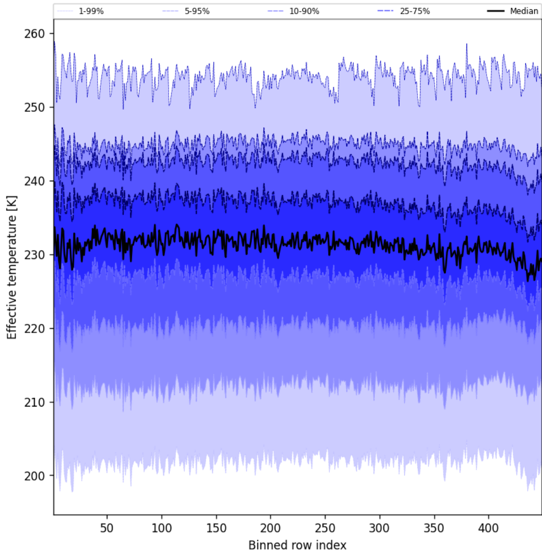
Figure 50: Along track statistics of “Effective temperature” for 2025-02-19 to 2025-02-20
