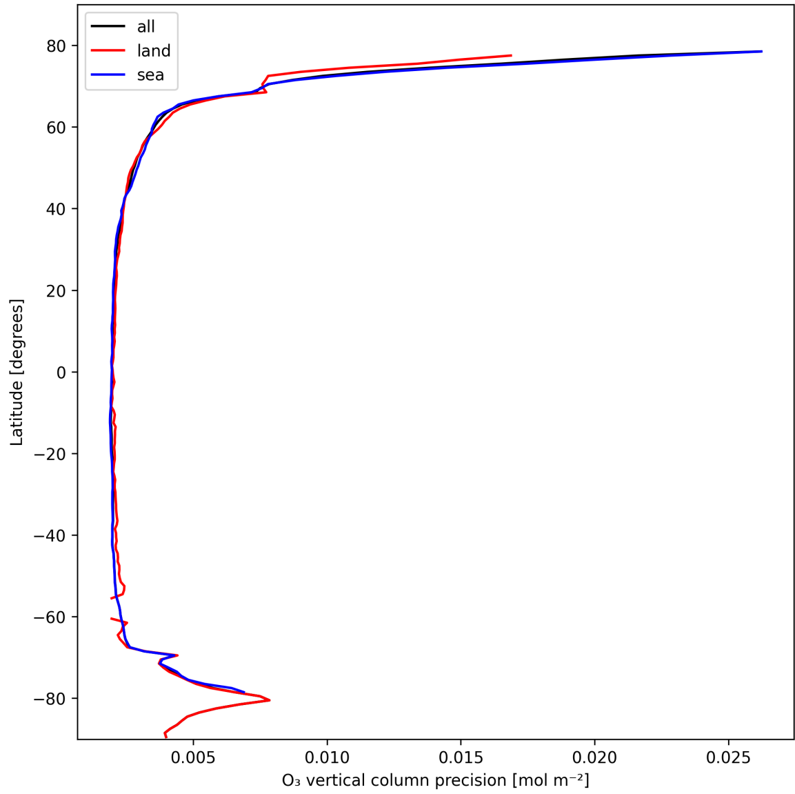
Figure 18: Zonal average of “O 3 vertical column precision” for 2025-02-19 to 2025-02-20.
