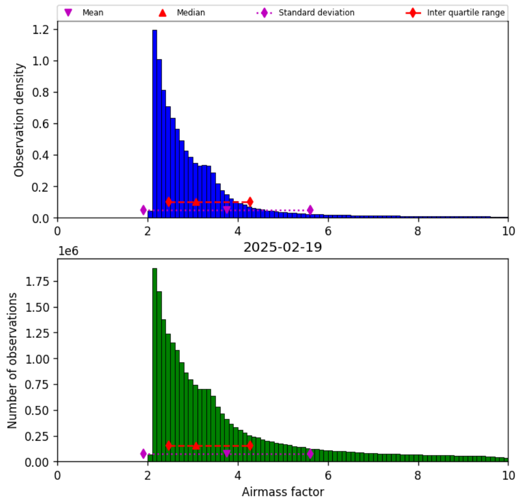
Figure 37: Histogram of “Airmass factor” for 2025-02-19 to 2025-02-20
