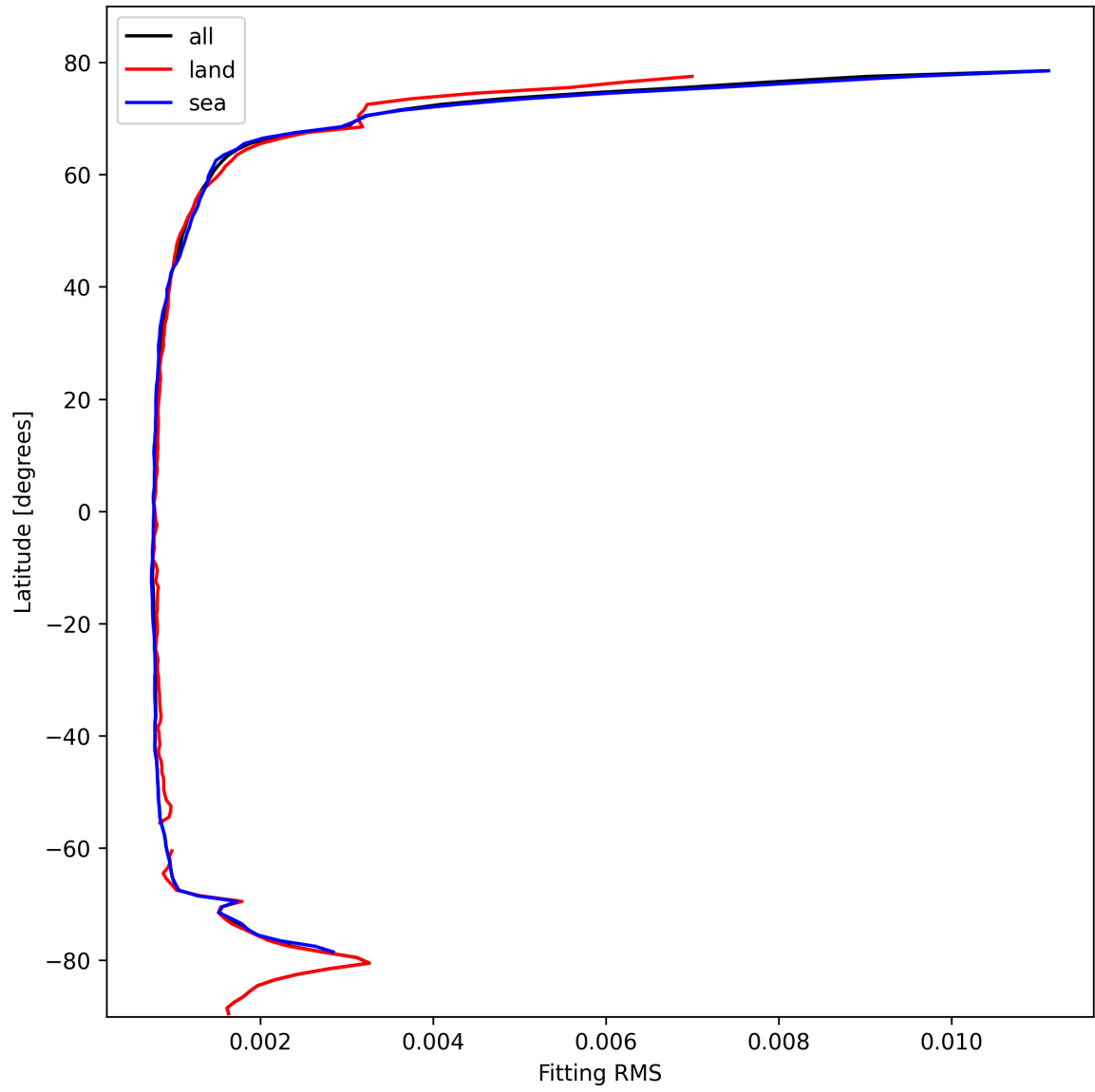
Figure 22: Zonal average of “Fitting RMS” for 2025-02-19 to 2025-02-20.
