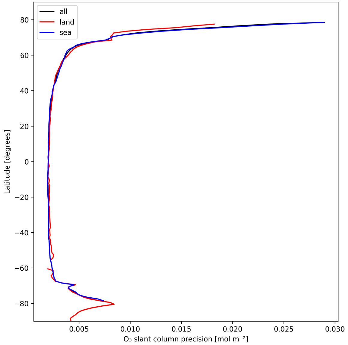
Figure 20: Zonal average of “O 3 slant column precision” for 2025-02-19 to 2025-02-20.
