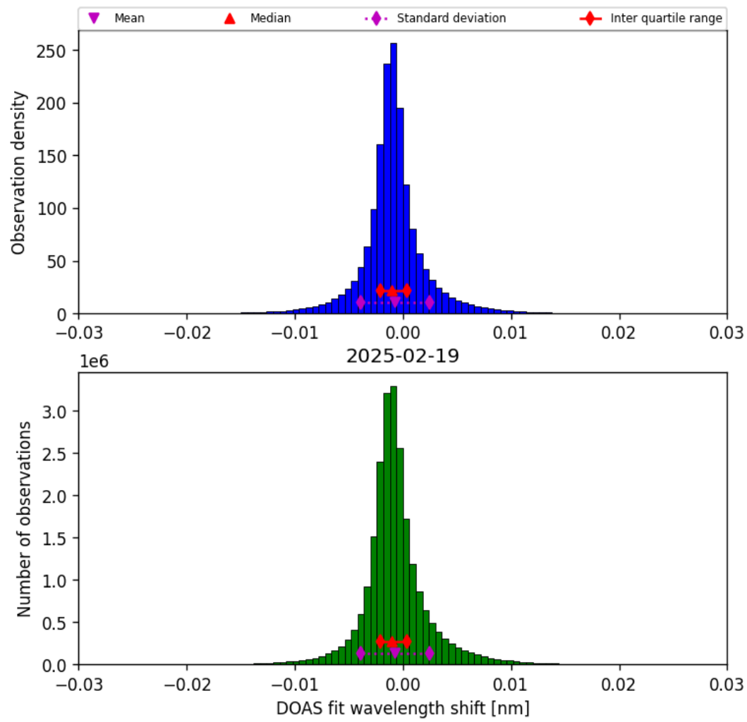
Figure 35: Histogram of “DOAS fit wavelength shift” for 2025-02-19 to 2025-02-20
