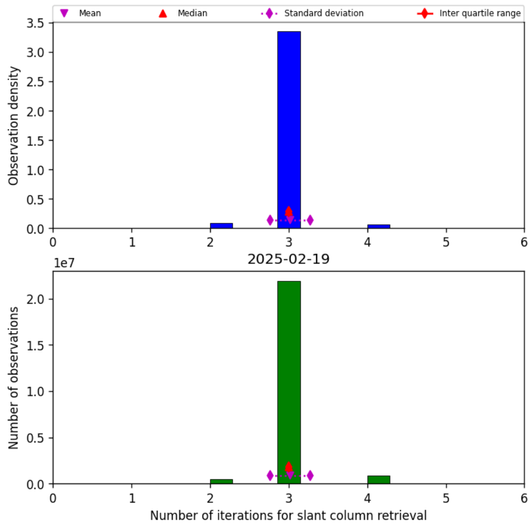
Figure 33: Histogram of “Number of iterations for slant column retrieval” for 2025-02-19 to 2025-02-20
