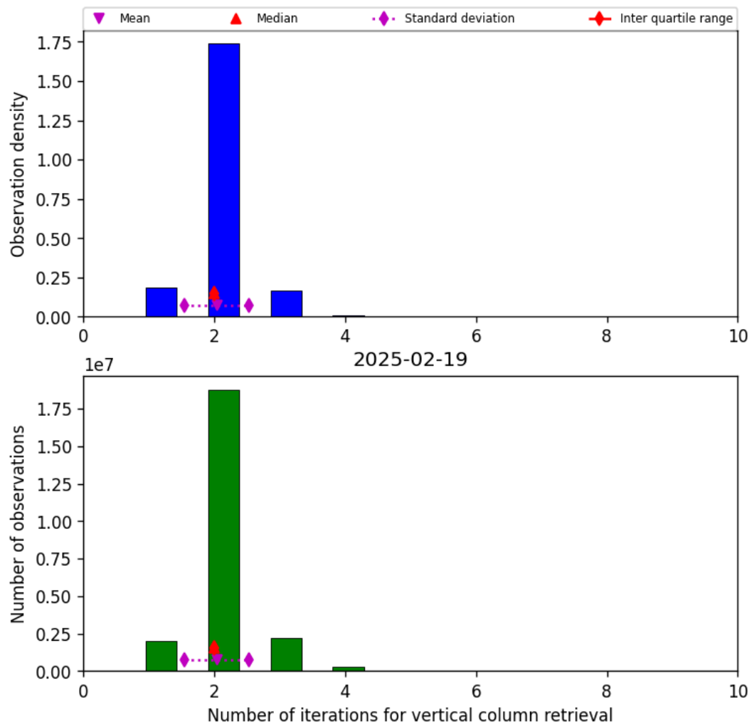
Figure 39: Histogram of “Number of iterations for vertical column retrieval” for 2025-02-19 to 2025-02-20
