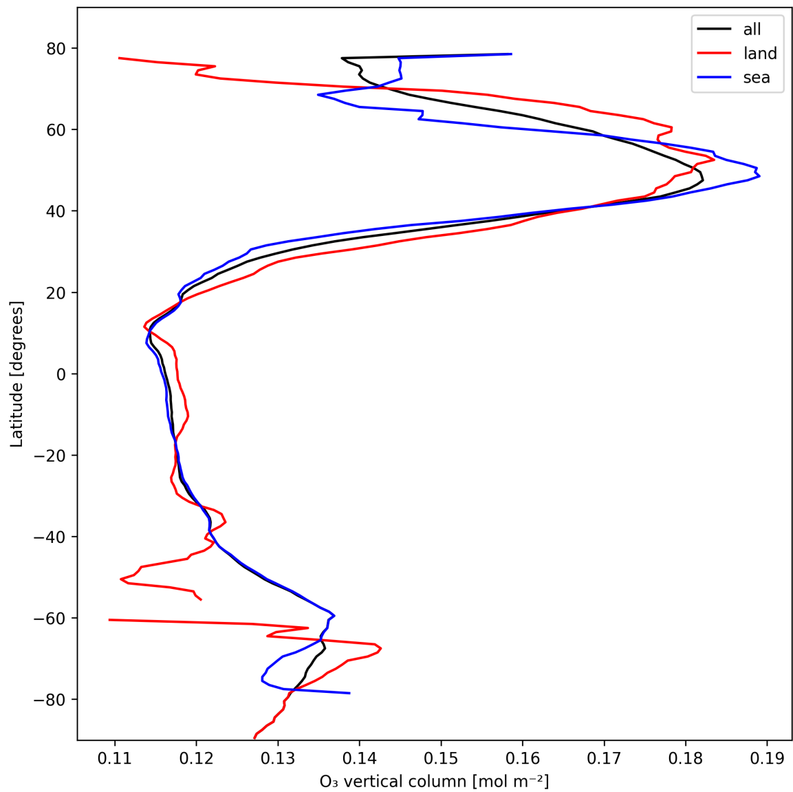
Figure 17: Zonal average of “O 3 vertical column” for 2025-02-19 to 2025-02-20.
