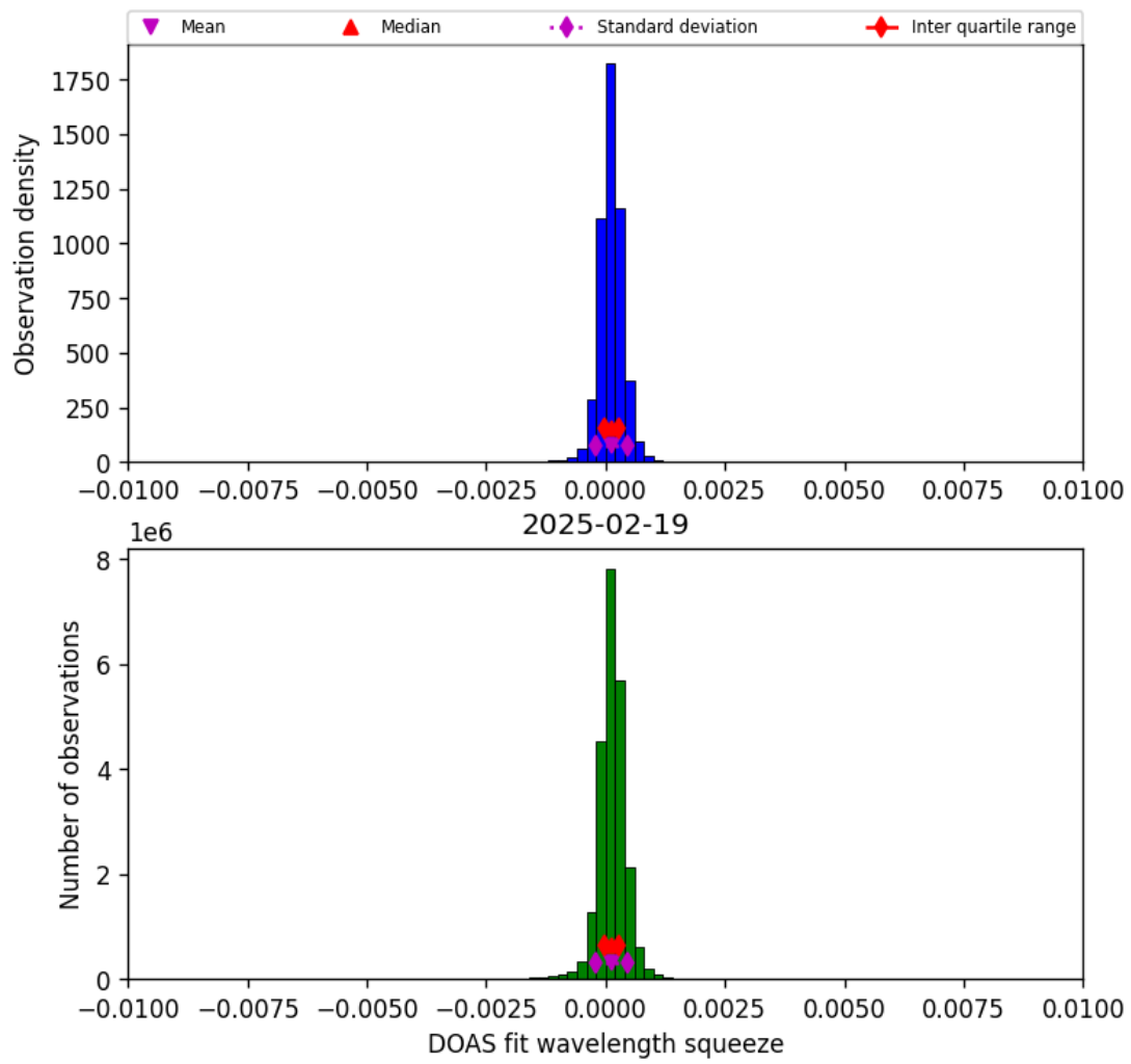
Figure 36: Histogram of “DOAS fit wavelength squeeze” for 2025-02-19 to 2025-02-20
