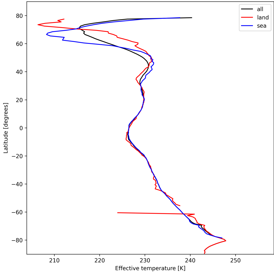
Figure 26: Zonal average of “Effective temperature” for 2025-02-19 to 2025-02-20.
