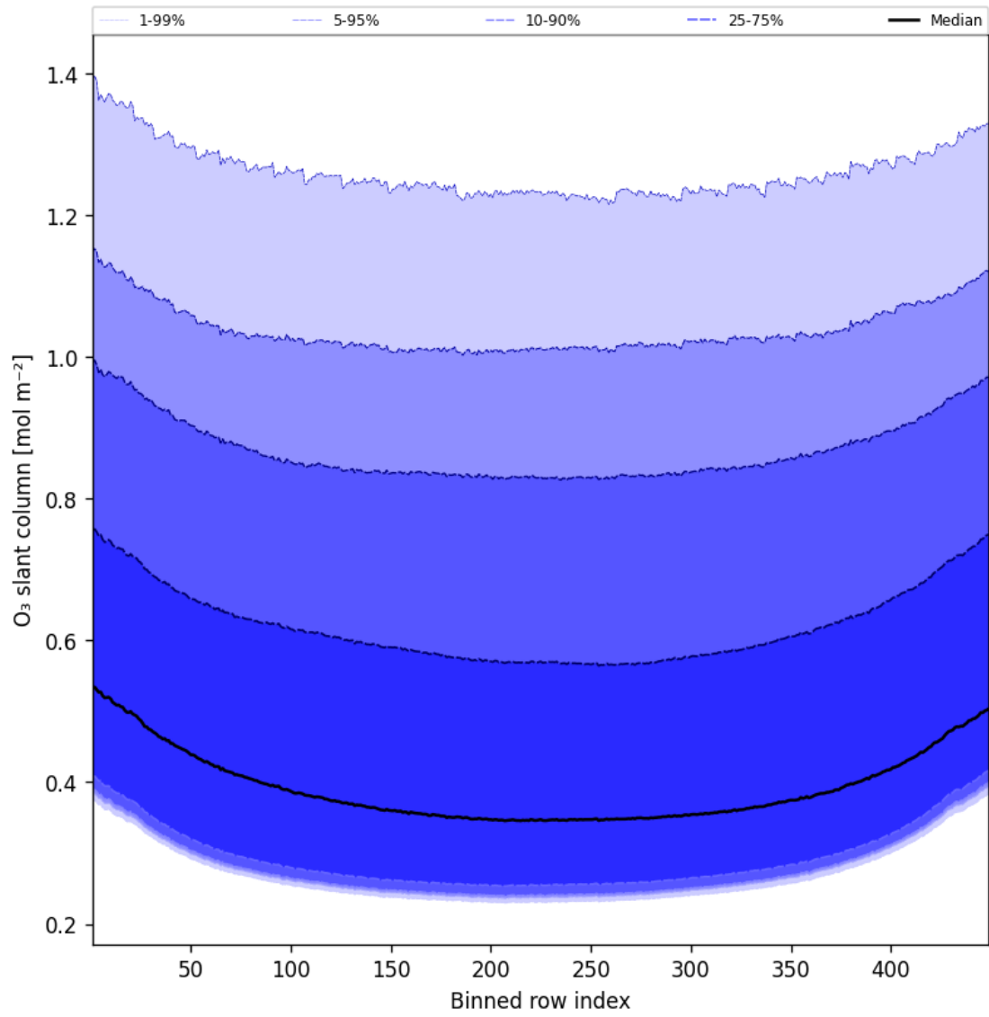
Figure 43: Along track statistics of “O 3 slant column” for 2025-02-19 to 2025-02-20
