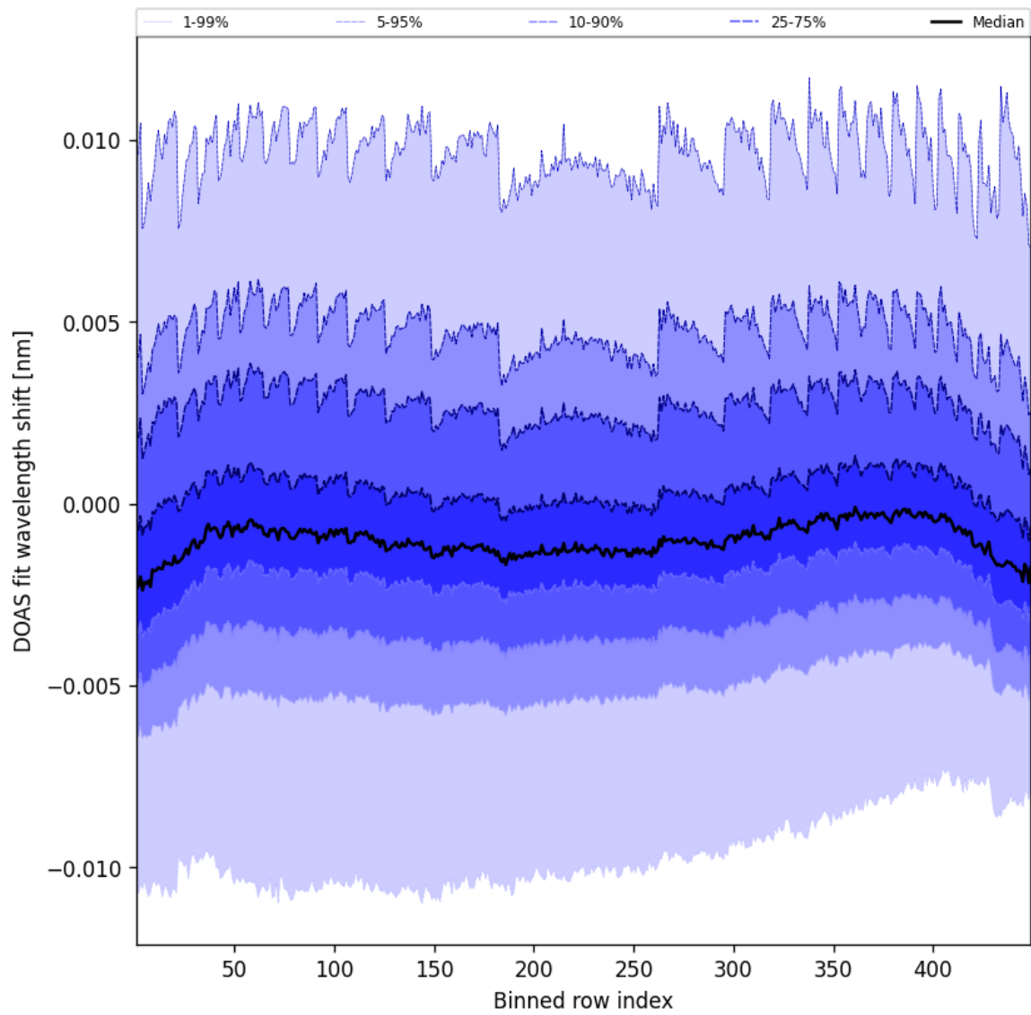
Figure 47: Along track statistics of “DOAS fit wavelength shift” for 2025-02-19 to 2025-02-20
