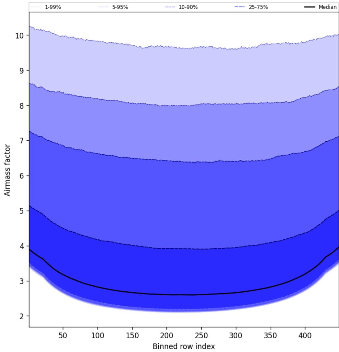
Figure 49: Along track statistics of “Airmass factor” for 2025-02-19 to 2025-02-20
