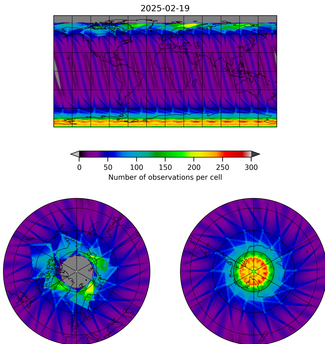
Figure 15: Map of the number of observations for 2025-02-19 to 2025-02-20
