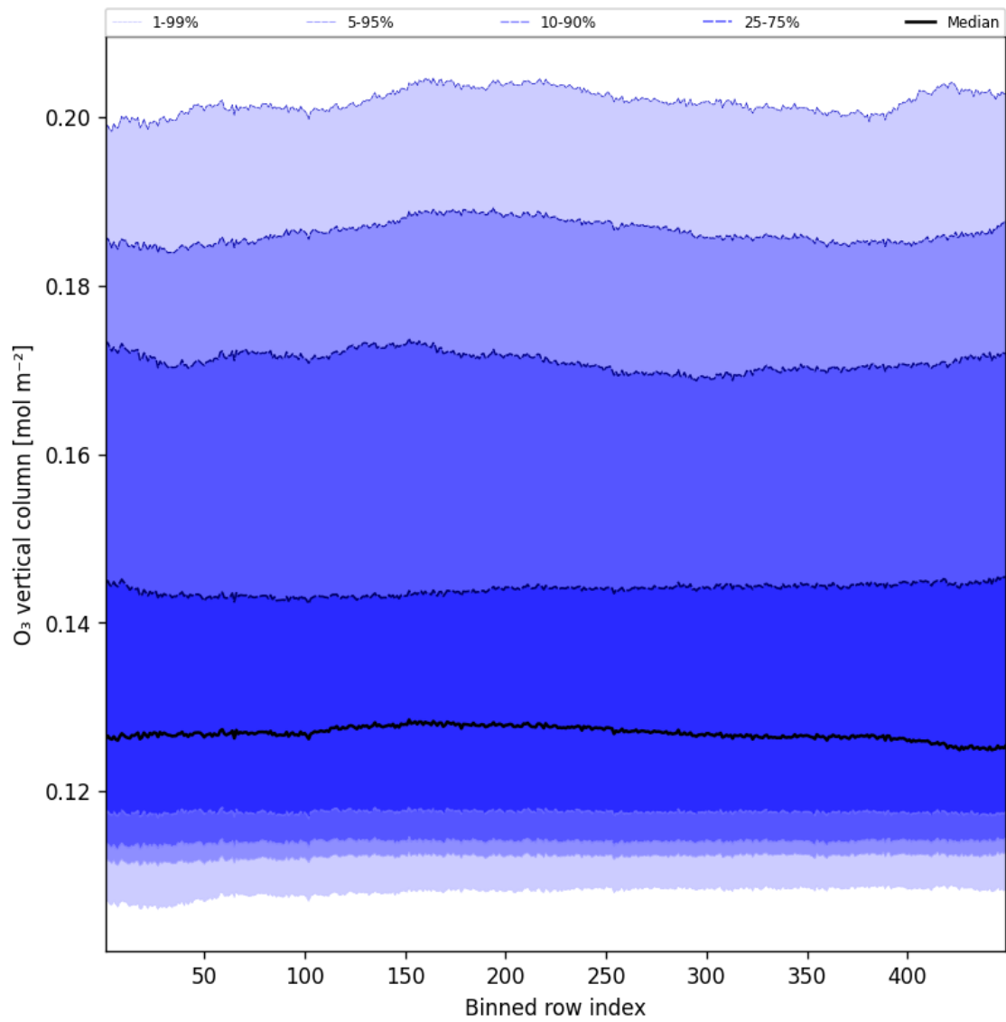
Figure 41: Along track statistics of “O 3 vertical column” for 2025-02-19 to 2025-02-20
