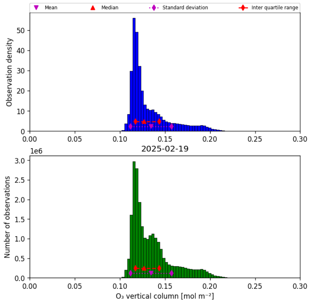
Figure 29: Histogram of “O 3 vertical column” for 2025-02-19 to 2025-02-20
