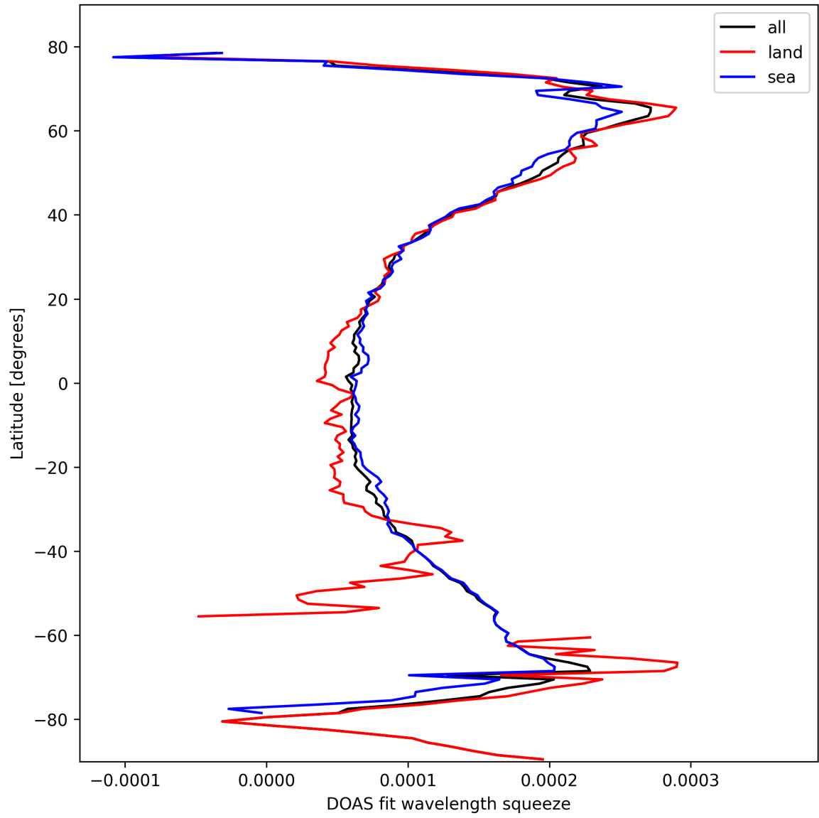
Figure 24: Zonal average of “DOAS fit wavelength squeeze” for 2025-02-19 to 2025-02-20.
