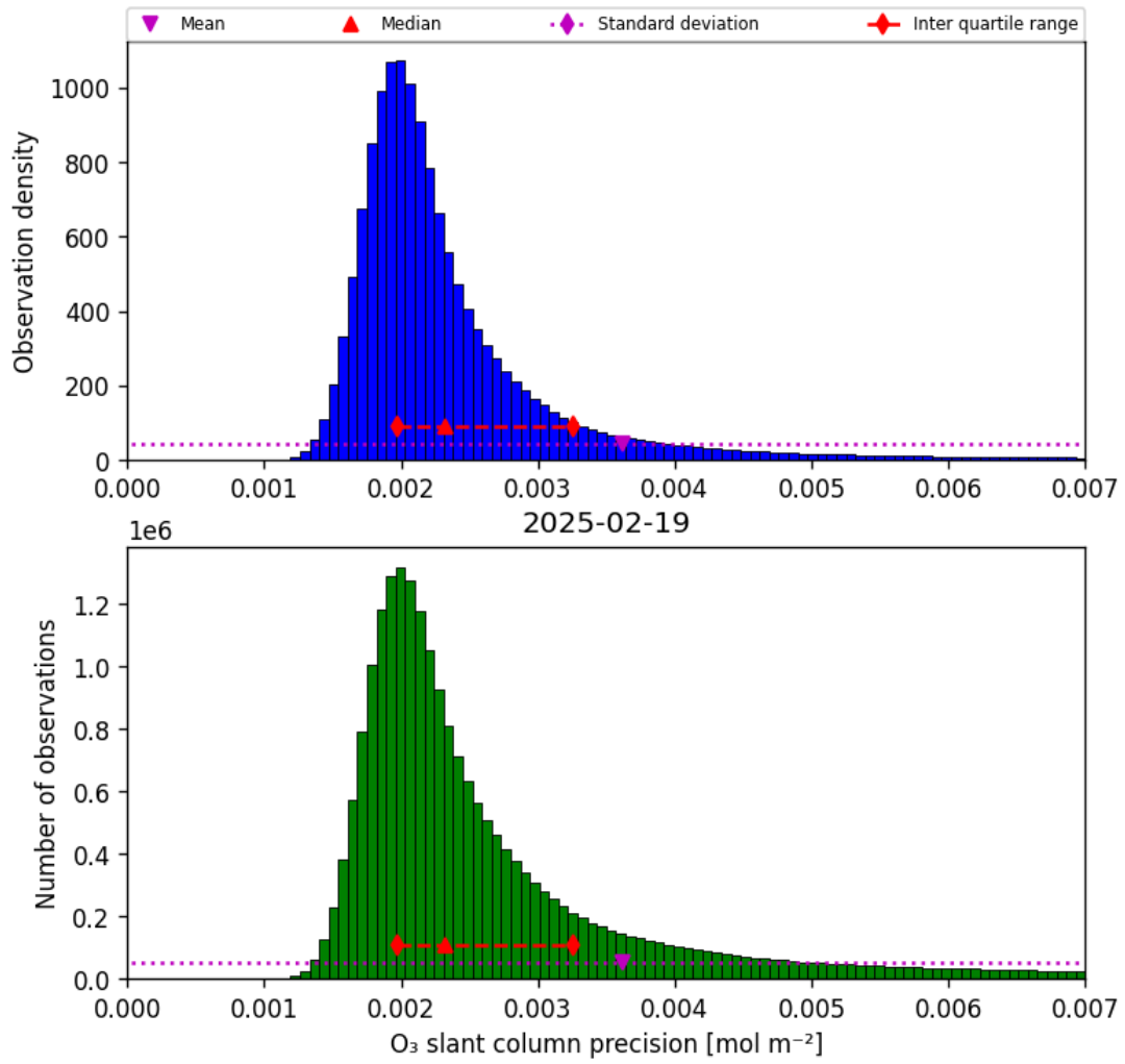
Figure 32: Histogram of “O 3 slant column precision” for 2025-02-19 to 2025-02-20
