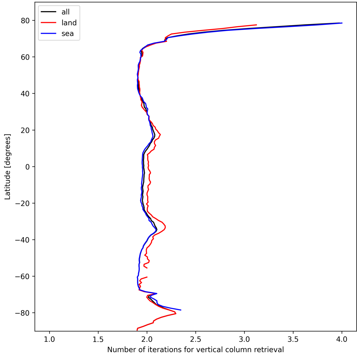
Figure 27: Zonal average of “Number of iterations for vertical column retrieval” for 2025-02-19 to 2025-02-20.
