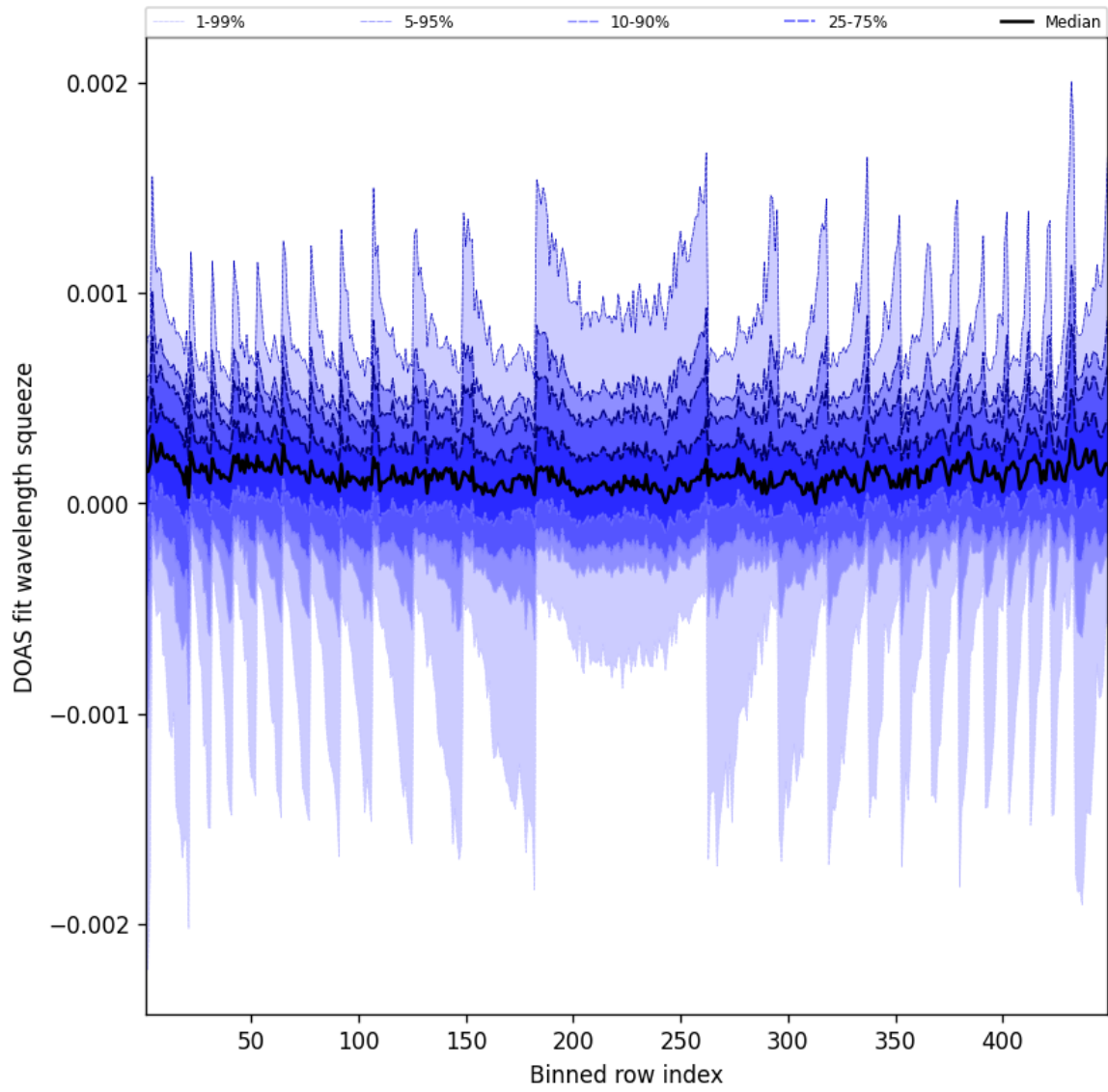
Figure 48: Along track statistics of “DOAS fit wavelength squeeze” for 2025-02-19 to 2025-02-20
