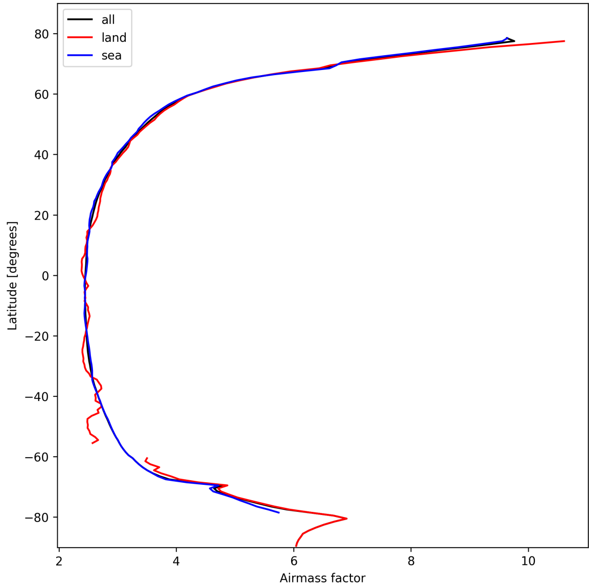
Figure 25: Zonal average of “Airmass factor” for 2025-02-19 to 2025-02-20.
