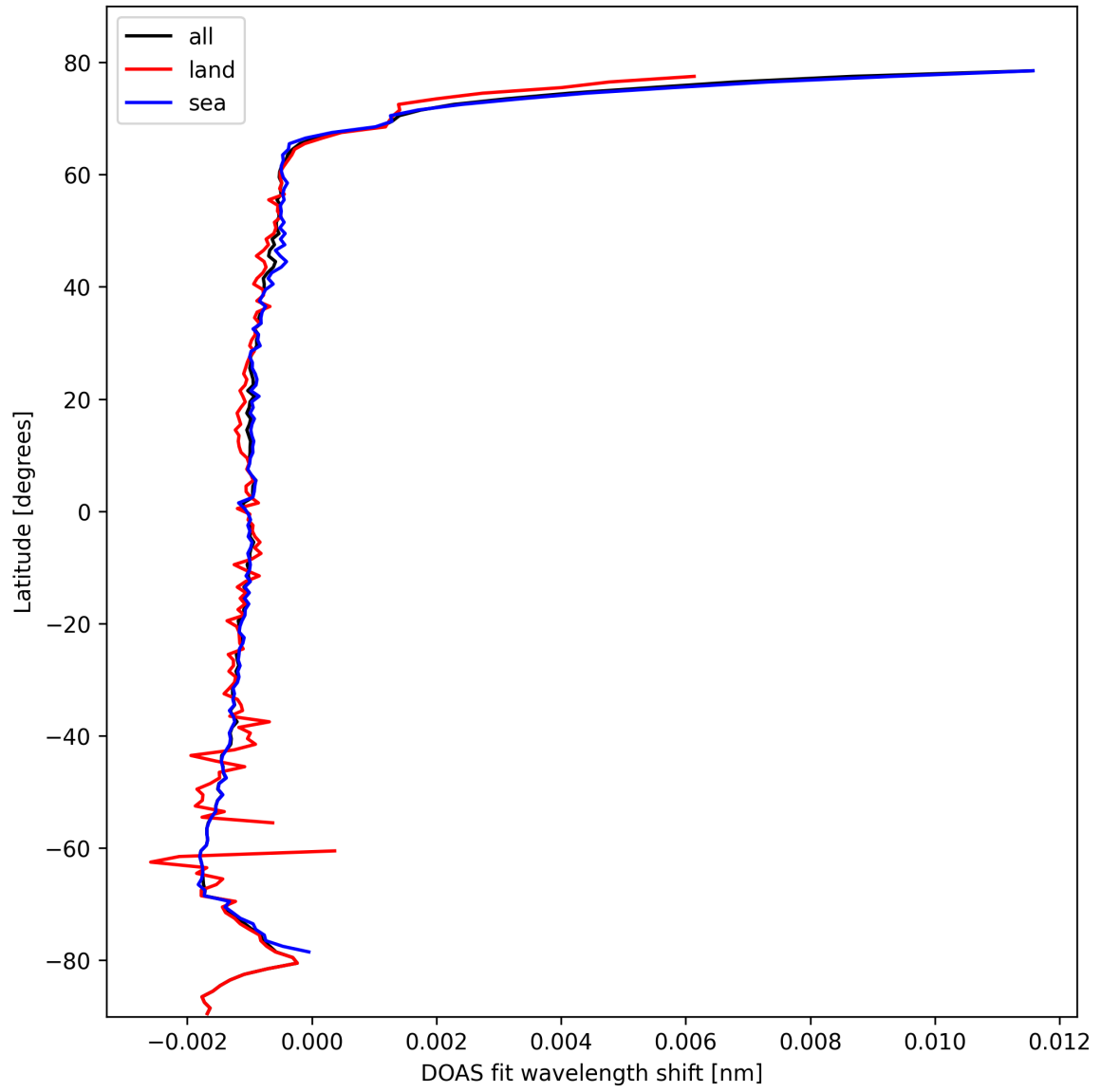
Figure 23: Zonal average of “DOAS fit wavelength shift” for 2025-02-19 to 2025-02-20.
