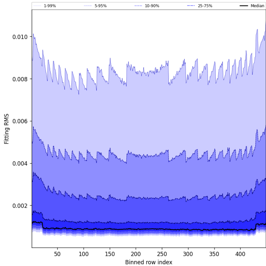
Figure 46: Along track statistics of “Fitting RMS” for 2025-02-19 to 2025-02-20
