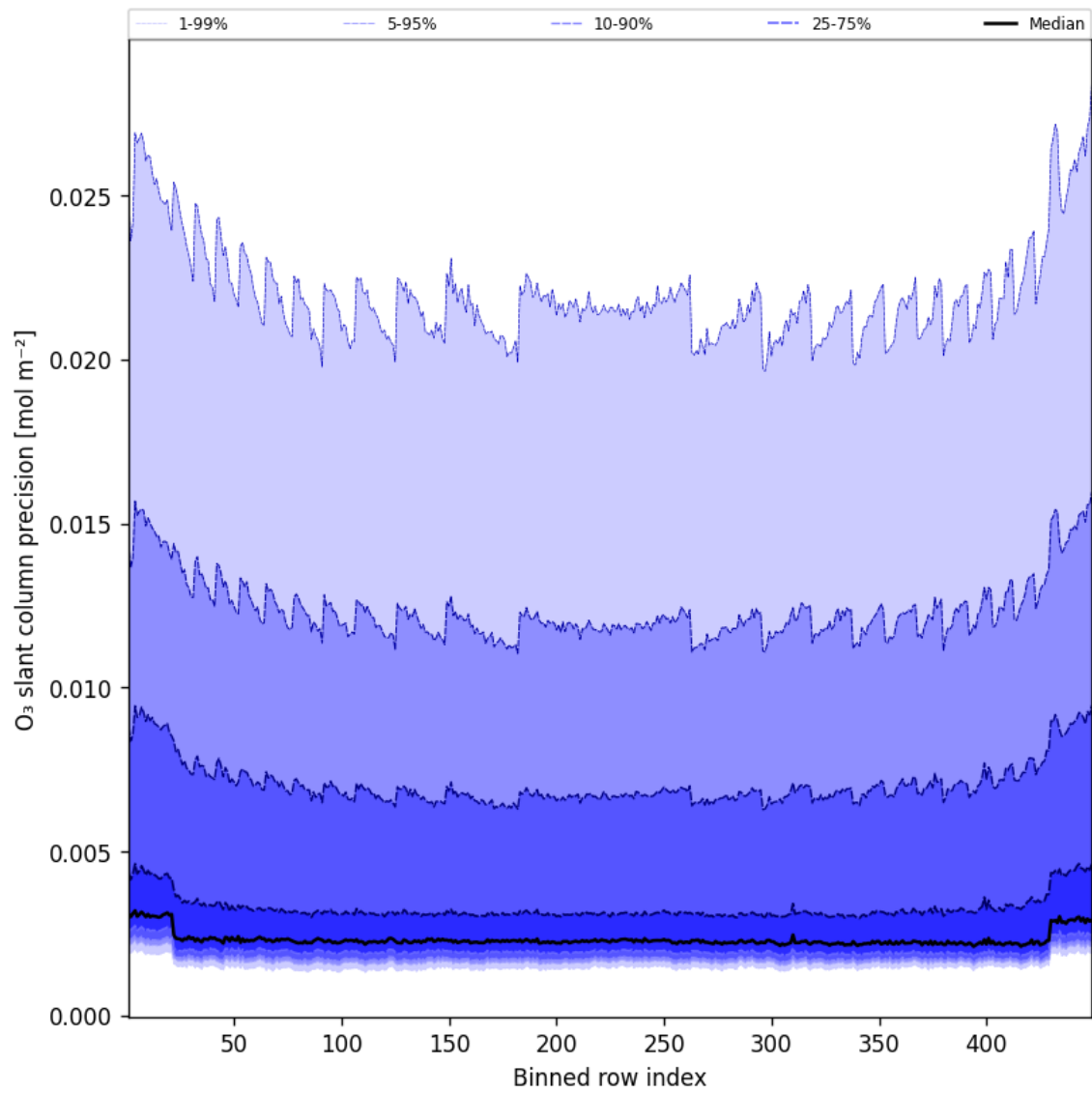
Figure 44: Along track statistics of “O 3 slant column precision” for 2025-02-21 to 2025-02-22
