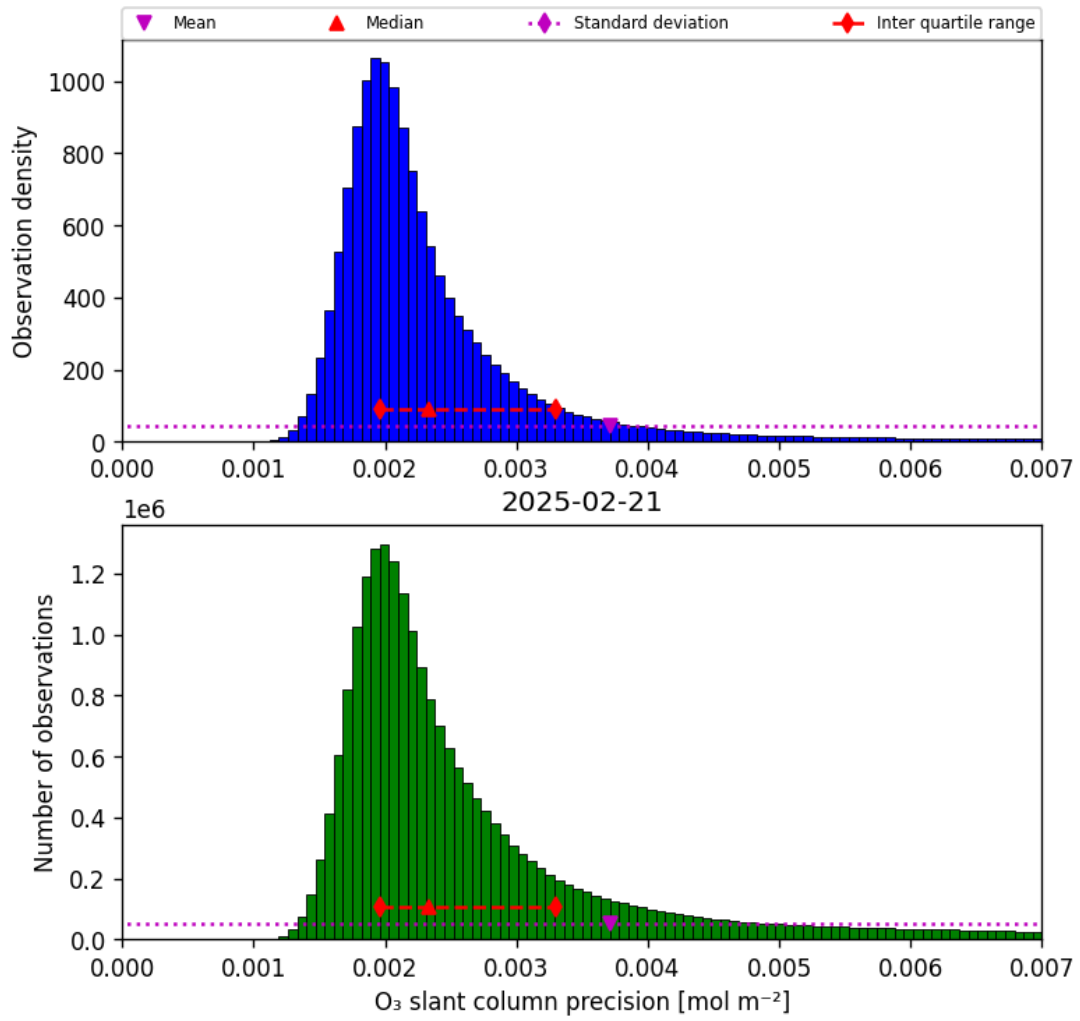
Figure 32: Histogram of “O 3 slant column precision” for 2025-02-21 to 2025-02-22
