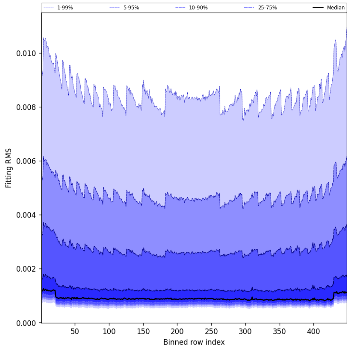
Figure 46: Along track statistics of “Fitting RMS” for 2025-02-21 to 2025-02-22
