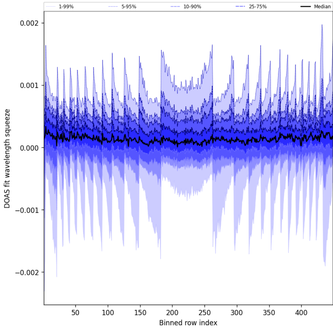
Figure 48: Along track statistics of “DOAS fit wavelength squeeze” for 2025-02-21 to 2025-02-22
