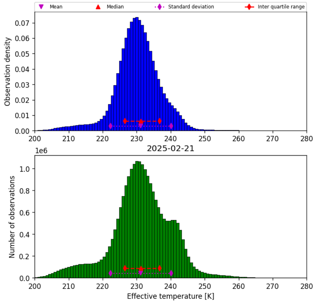
Figure 38: Histogram of “Effective temperature” for 2025-02-21 to 2025-02-22
