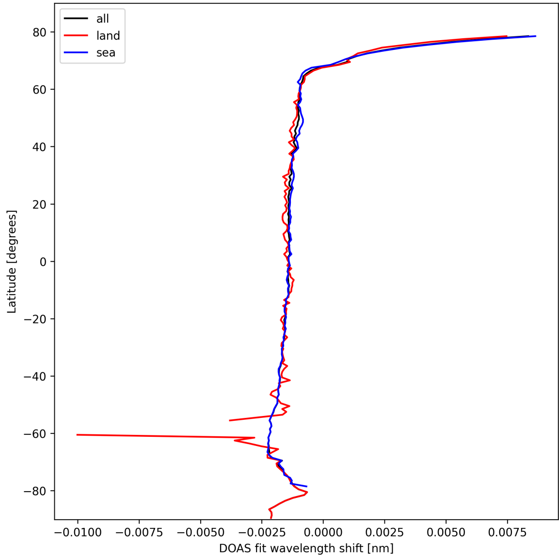
Figure 23: Zonal average of “DOAS fit wavelength shift” for 2025-02-21 to 2025-02-22.
