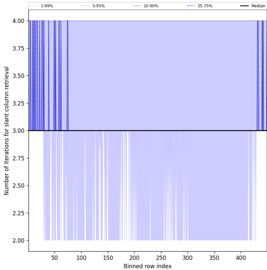
Figure 45: Along track statistics of “Number of iterations for slant column retrieval” for 2025-02-21 to 2025-02-22
