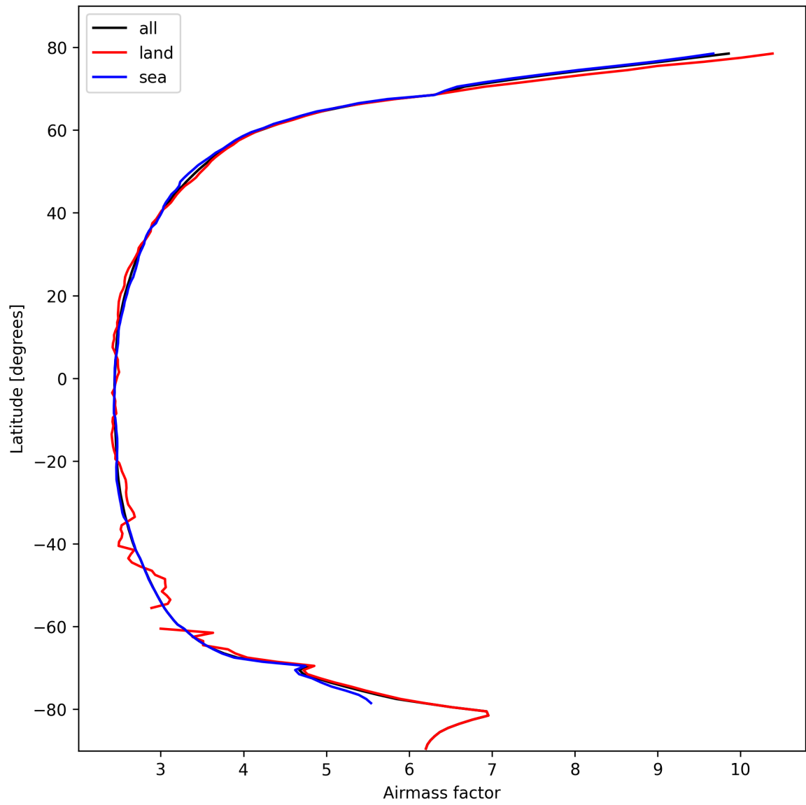
Figure 25: Zonal average of “Airmass factor” for 2025-02-21 to 2025-02-22.
