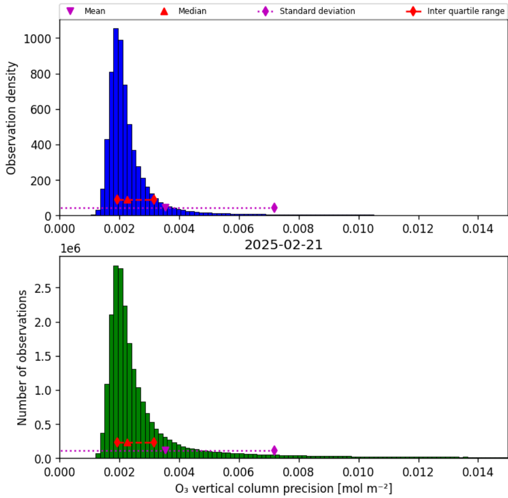
Figure 30: Histogram of “O 3 vertical column precision” for 2025-02-21 to 2025-02-22
