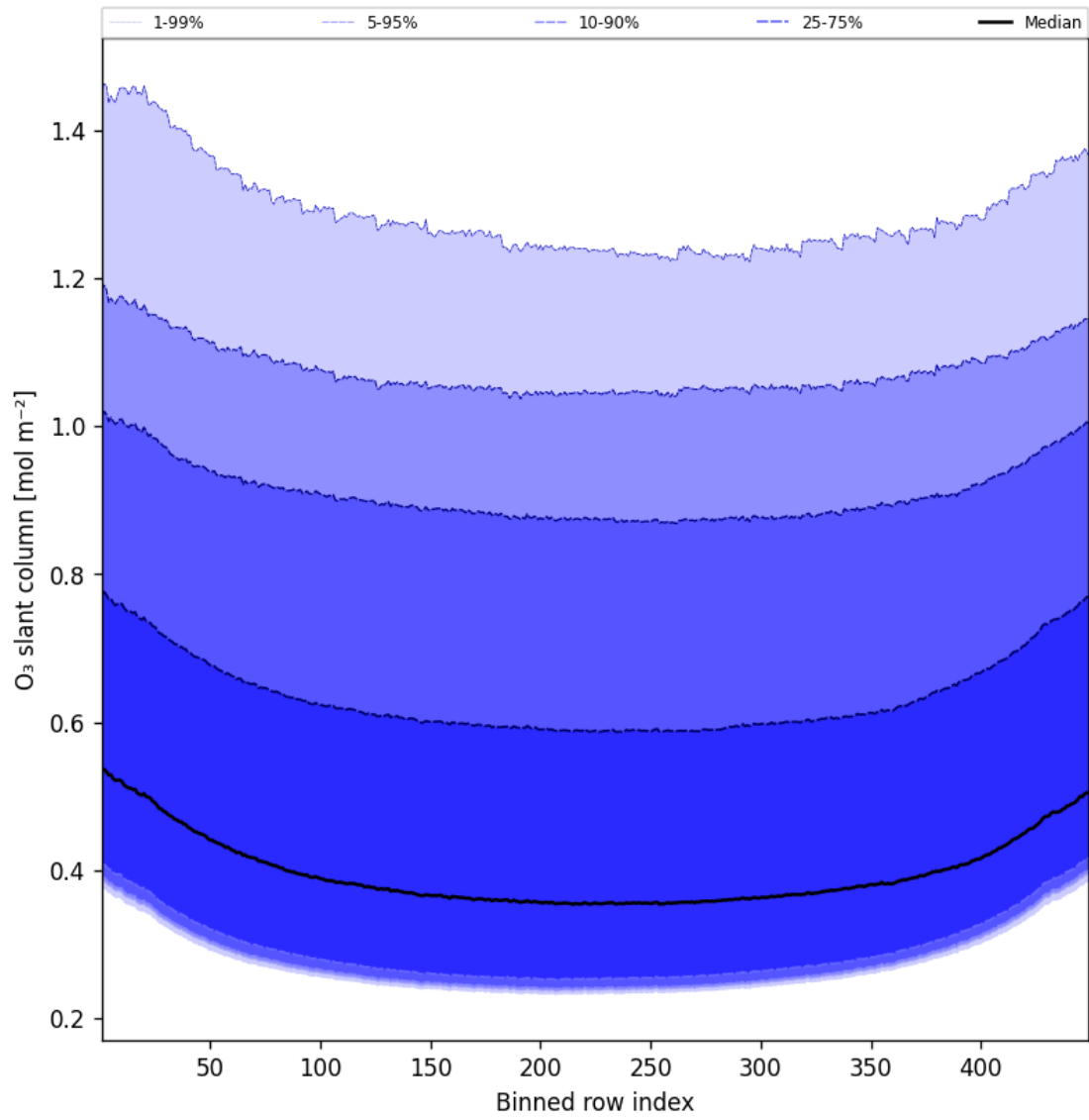
Figure 43: Along track statistics of “O 3 slant column” for 2025-02-21 to 2025-02-22
