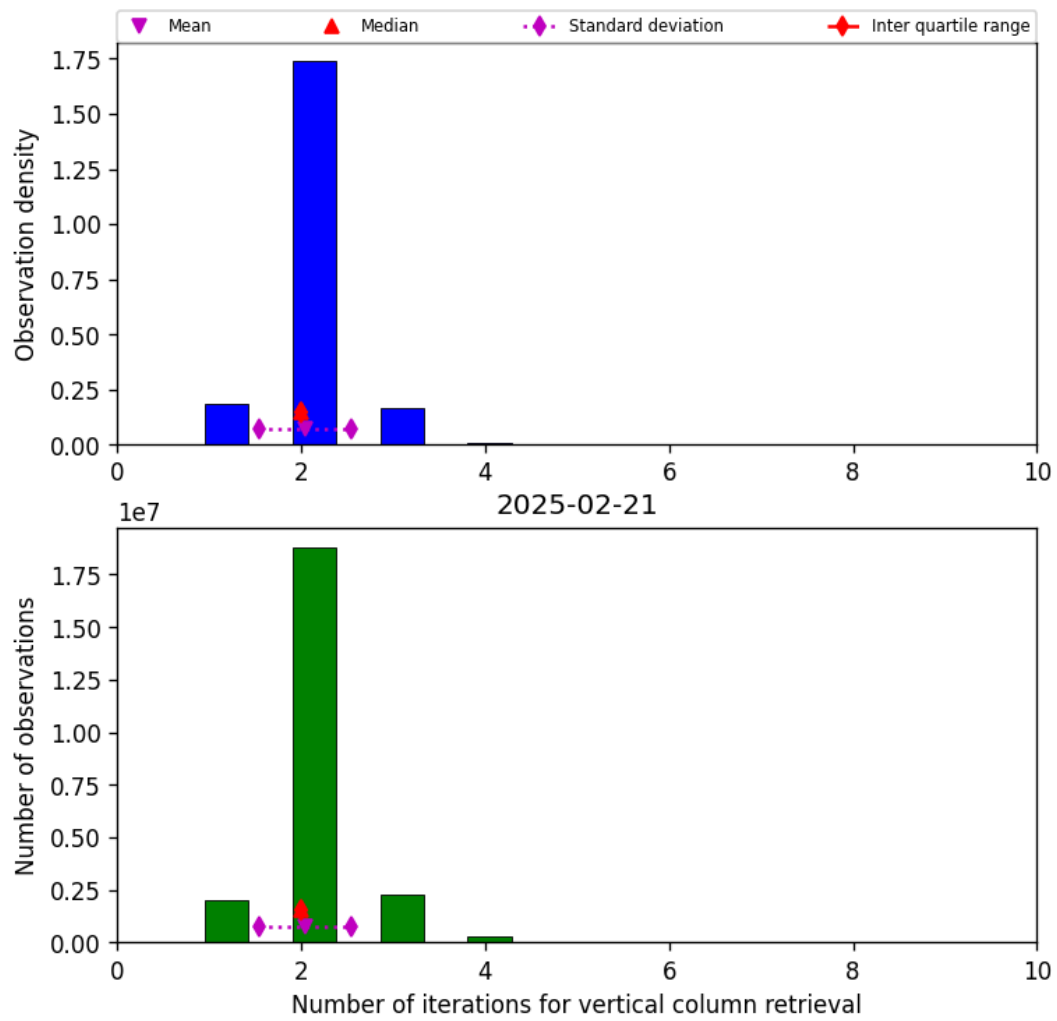
Figure 39: Histogram of “Number of iterations for vertical column retrieval” for 2025-02-21 to 2025-02-22
