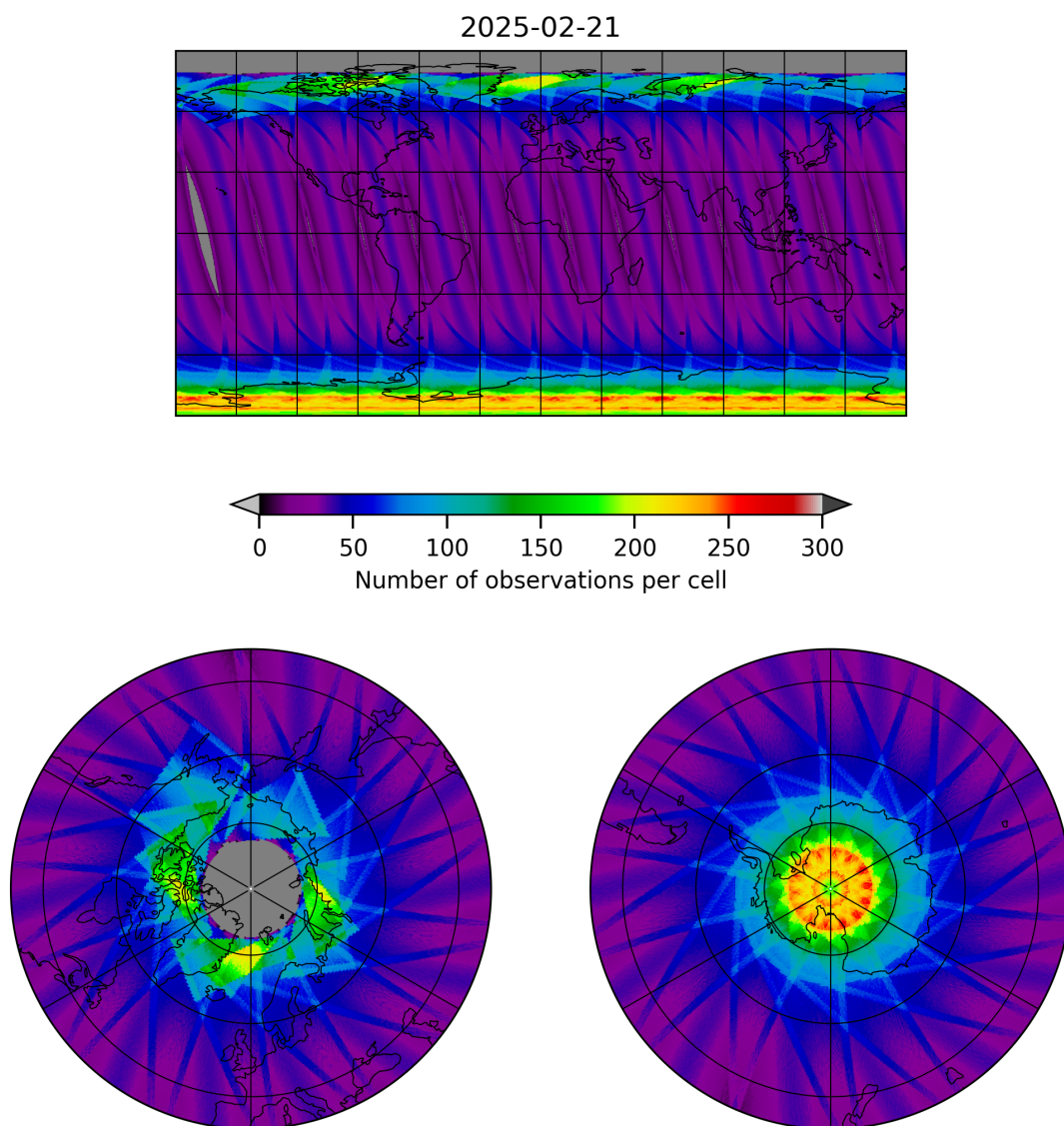
Figure 15: Map of the number of observations for 2025-02-21 to 2025-02-22
