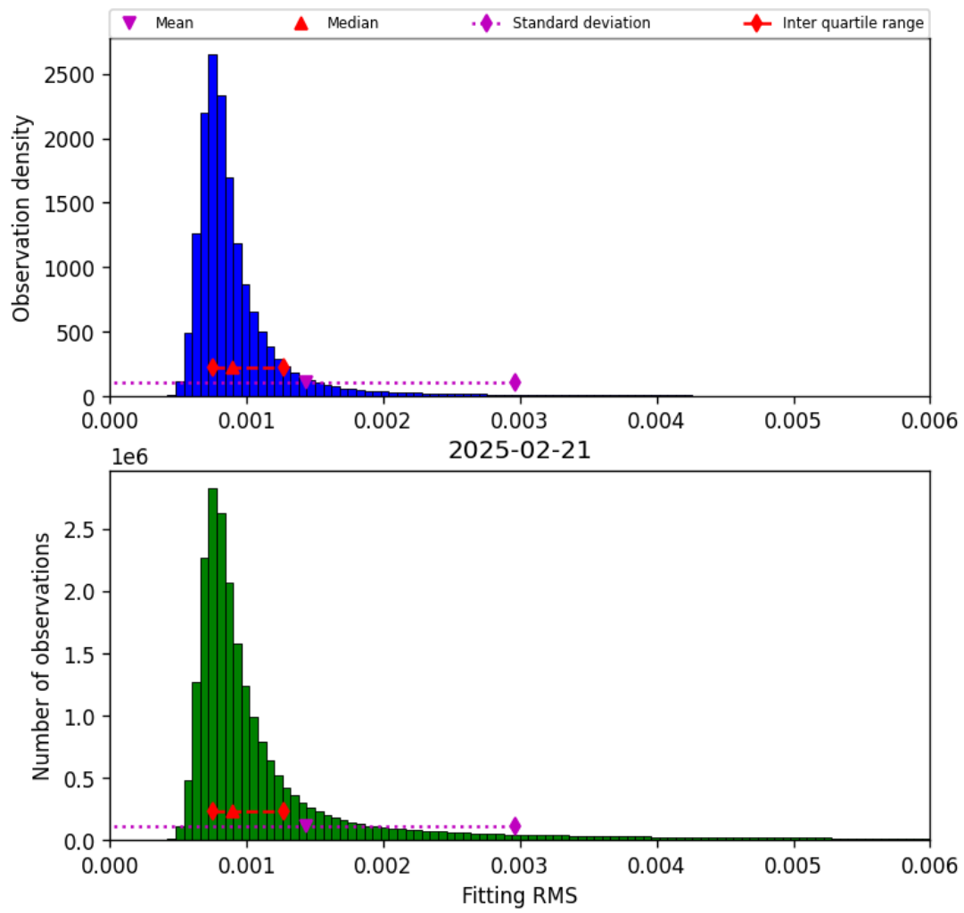
Figure 34: Histogram of “Fitting RMS” for 2025-02-21 to 2025-02-22
