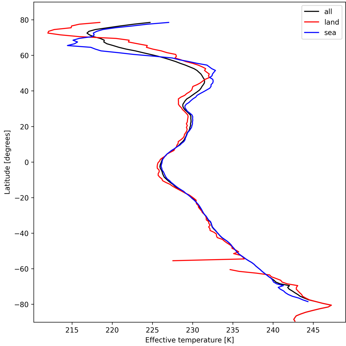
Figure 26: Zonal average of “Effective temperature” for 2025-02-21 to 2025-02-22.
