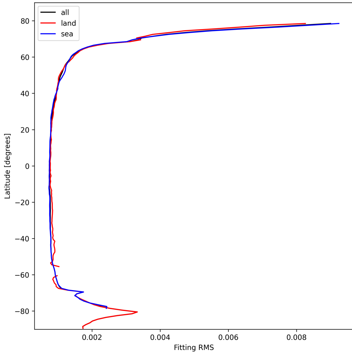
Figure 22: Zonal average of “Fitting RMS” for 2025-02-21 to 2025-02-22.
