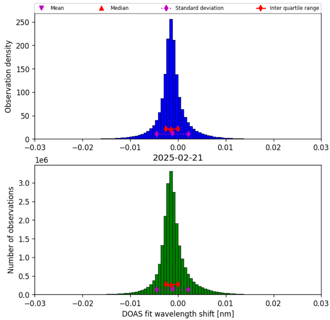
Figure 35: Histogram of “DOAS fit wavelength shift” for 2025-02-21 to 2025-02-22
