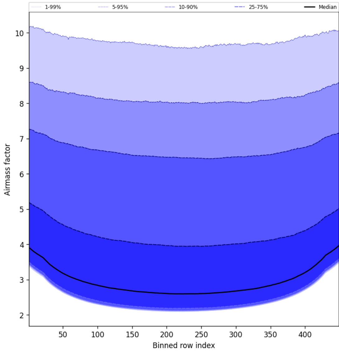
Figure 49: Along track statistics of “Airmass factor” for 2025-02-21 to 2025-02-22
