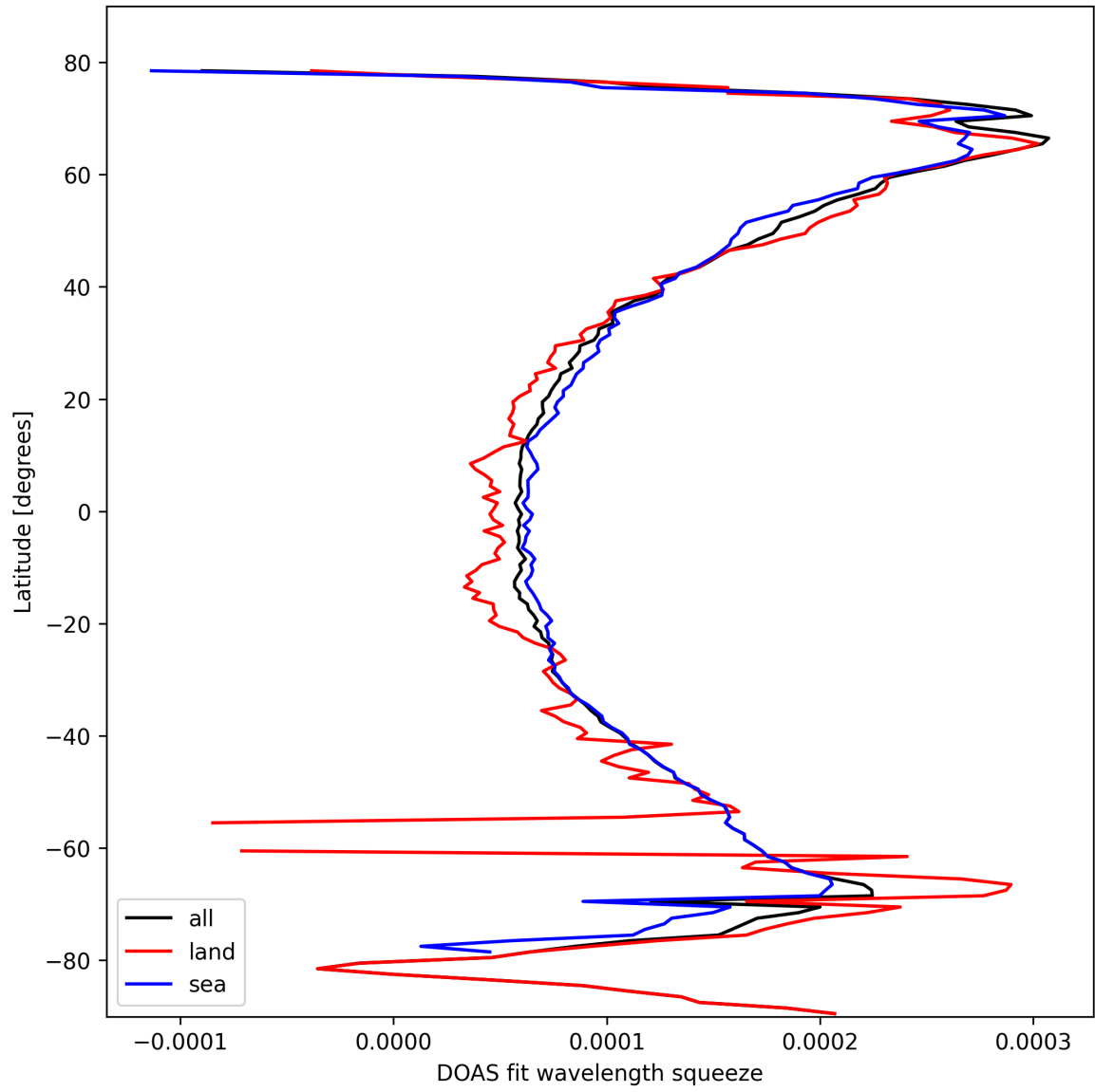
Figure 24: Zonal average of “DOAS fit wavelength squeeze” for 2025-02-21 to 2025-02-22.
