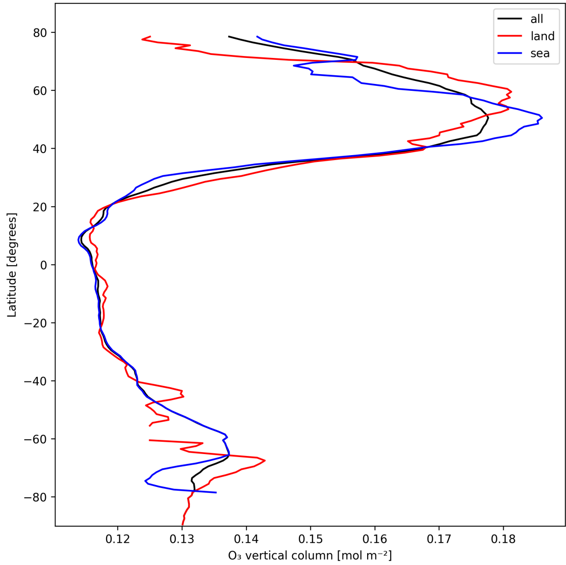
Figure 17: Zonal average of “O 3 vertical column” for 2025-02-21 to 2025-02-22.
