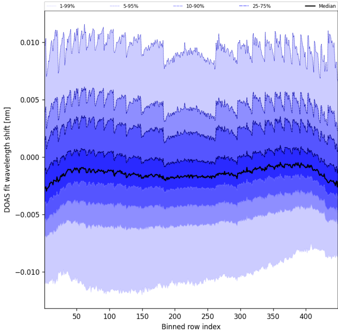
Figure 47: Along track statistics of "DOAS fit wavelength shift" for 2025-02-21 to 2025-02-22
