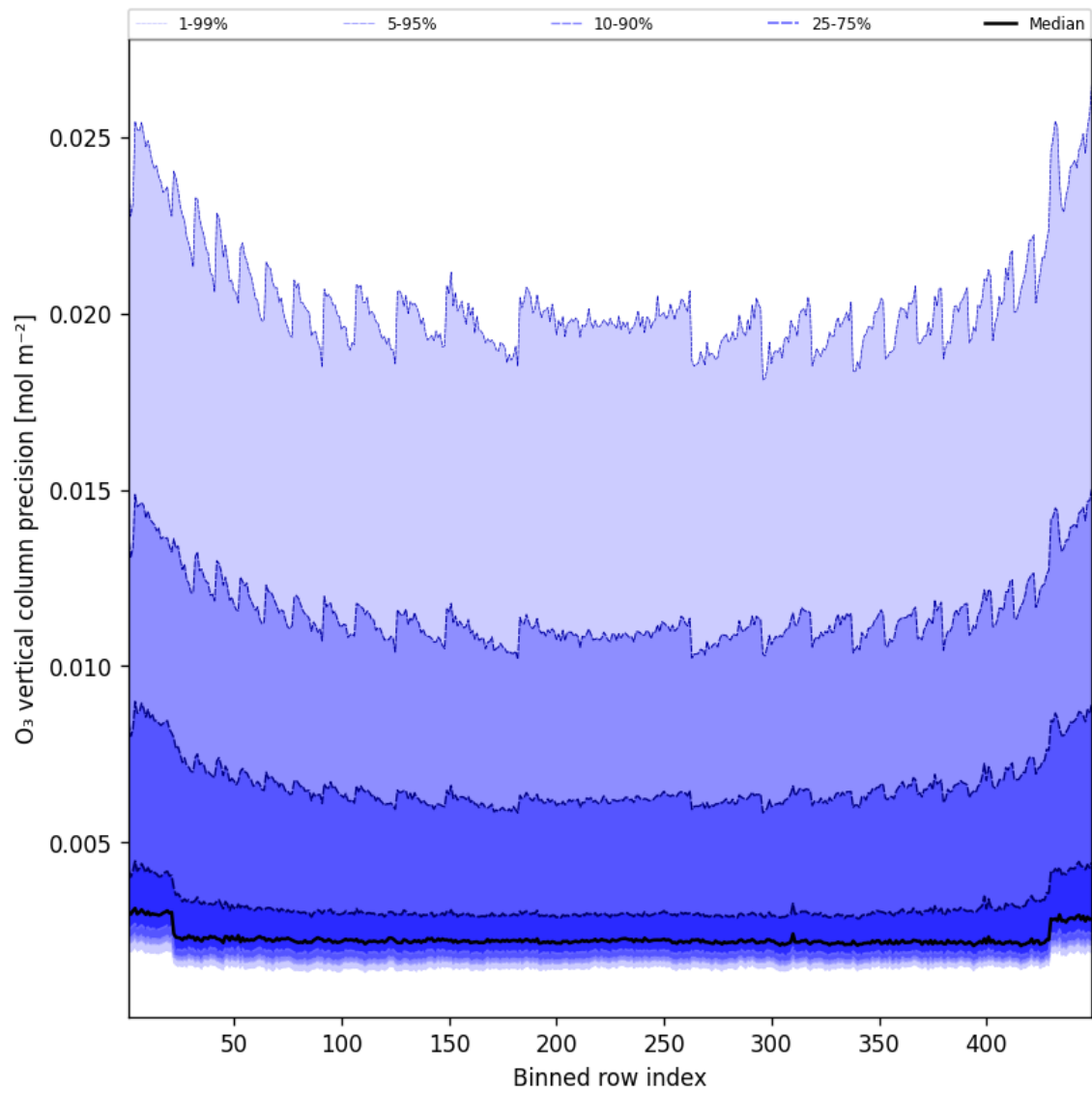
Figure 42: Along track statistics of “O 3 vertical column precision” for 2025-02-21 to 2025-02-22
