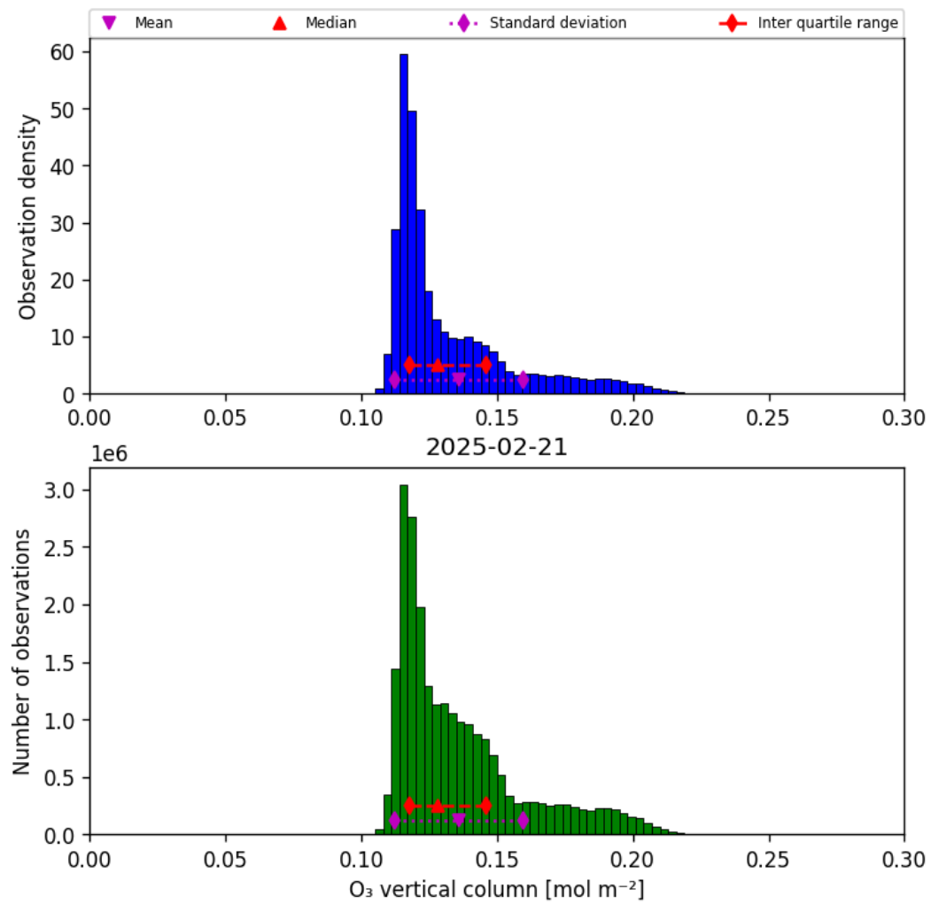
Figure 29: Histogram of “O 3 vertical column” for 2025-02-21 to 2025-02-22
