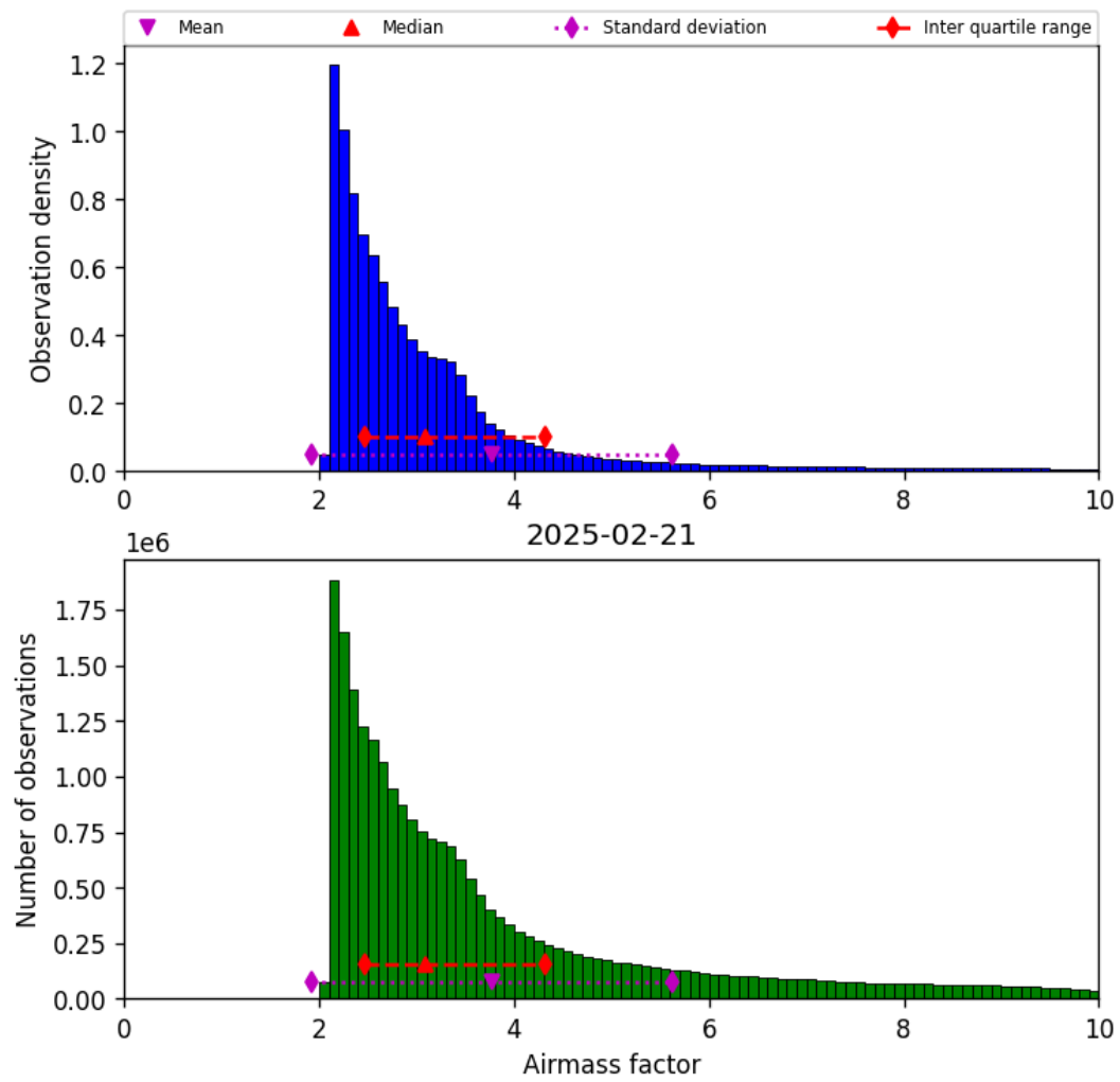
Figure 37: Histogram of “Airmass factor” for 2025-02-21 to 2025-02-22
