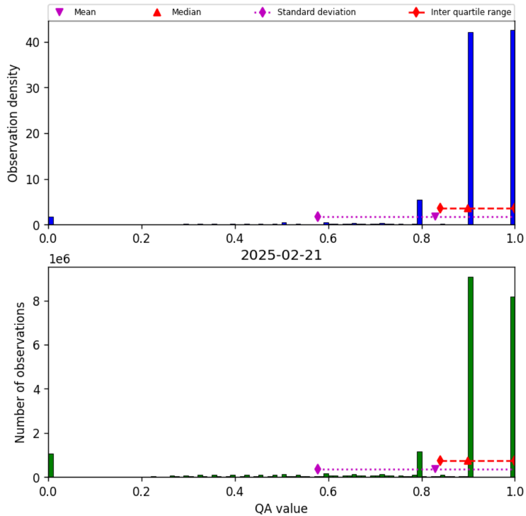
Figure 28: Histogram of “QA value” for 2025-02-21 to 2025-02-22
