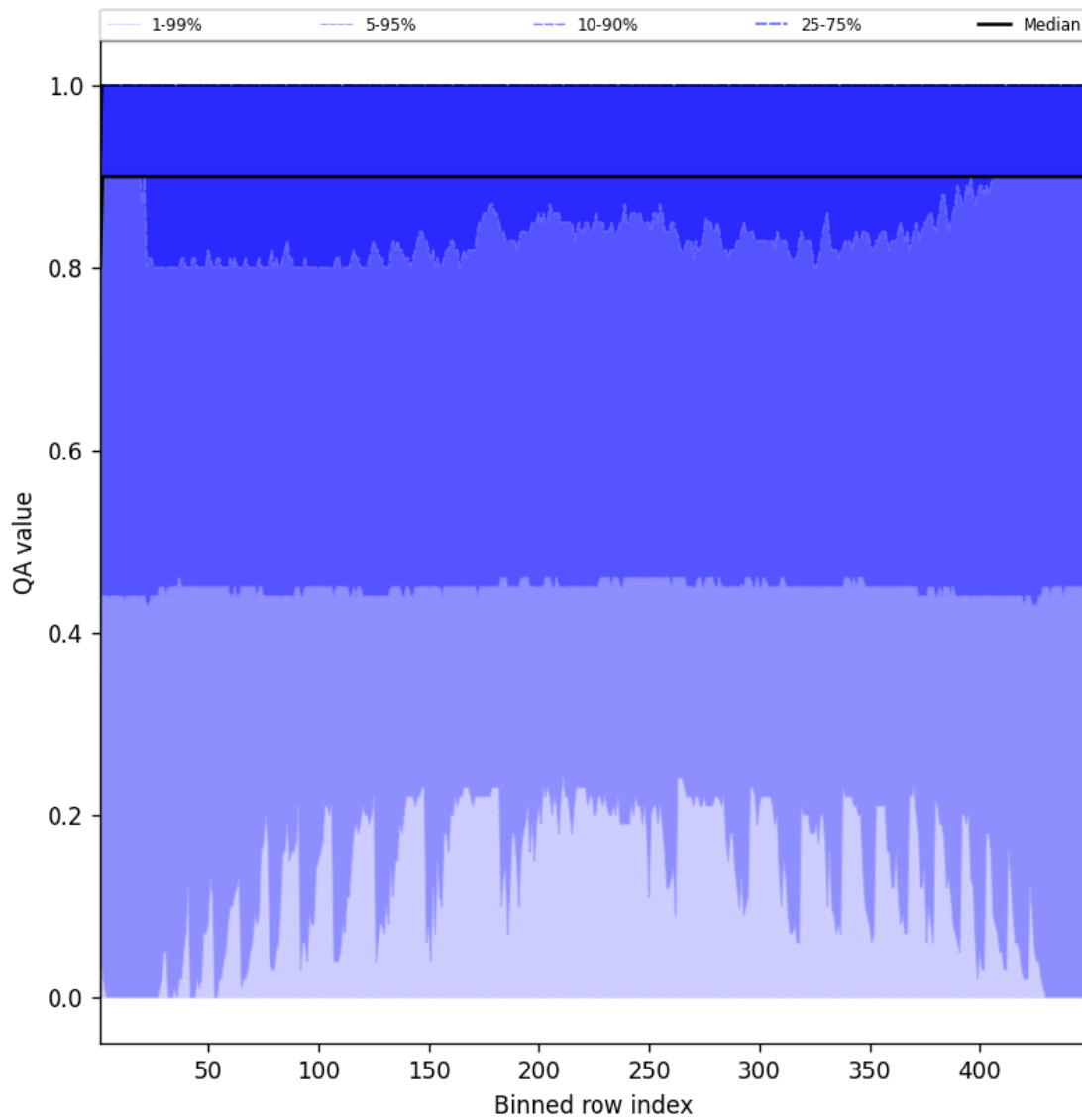
Figure 40: Along track statistics of “QA value” for 2025-02-21 to 2025-02-22
