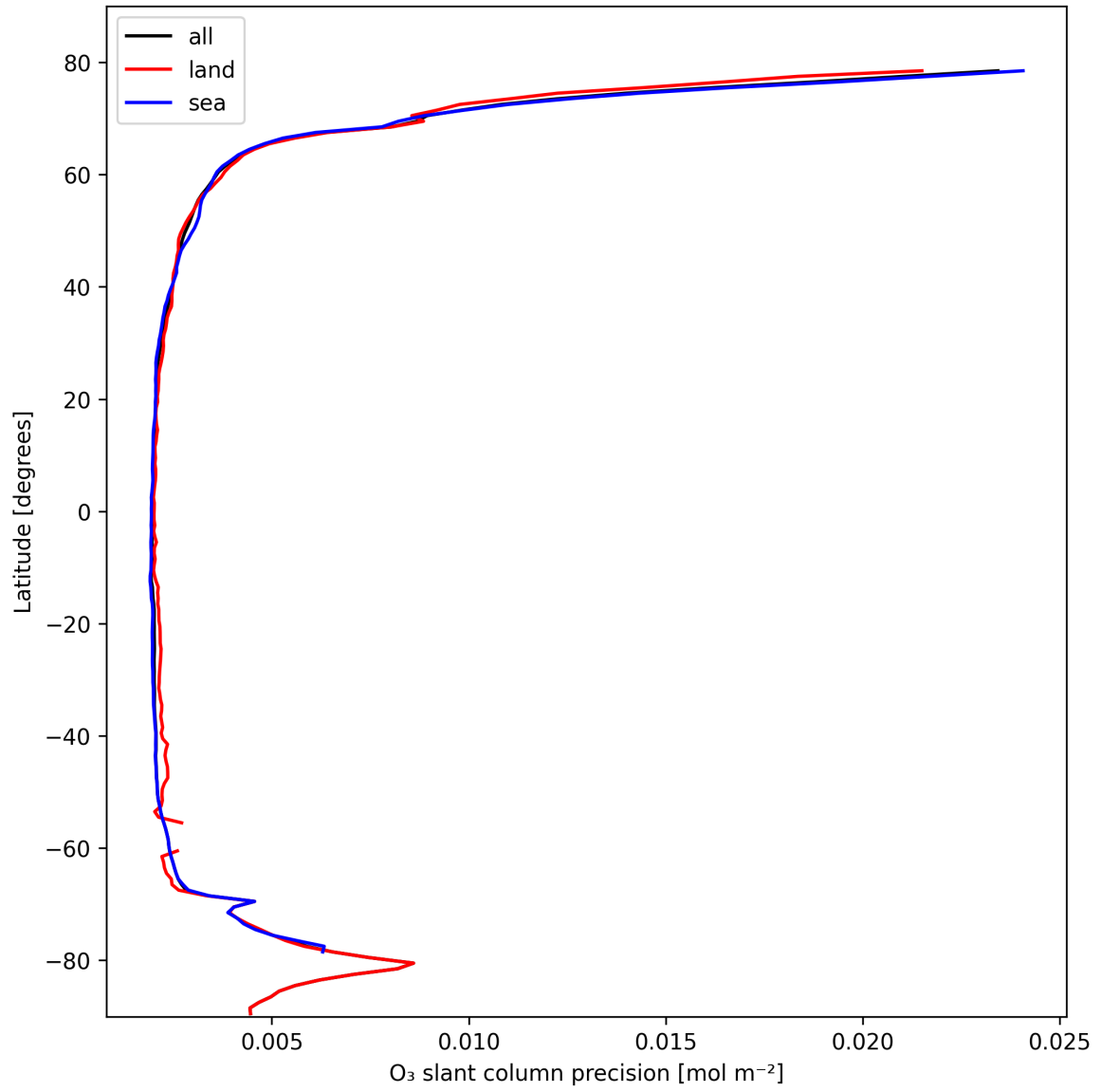
Figure 20: Zonal average of “O 3 slant column precision” for 2025-02-21 to 2025-02-22.
