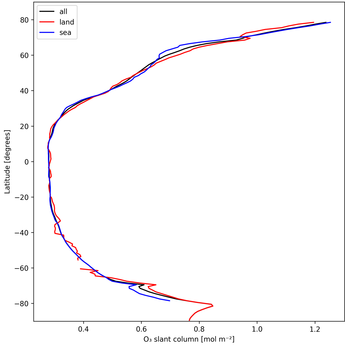
Figure 19: Zonal average of “O 3 slant column” for 2025-02-21 to 2025-02-22.
