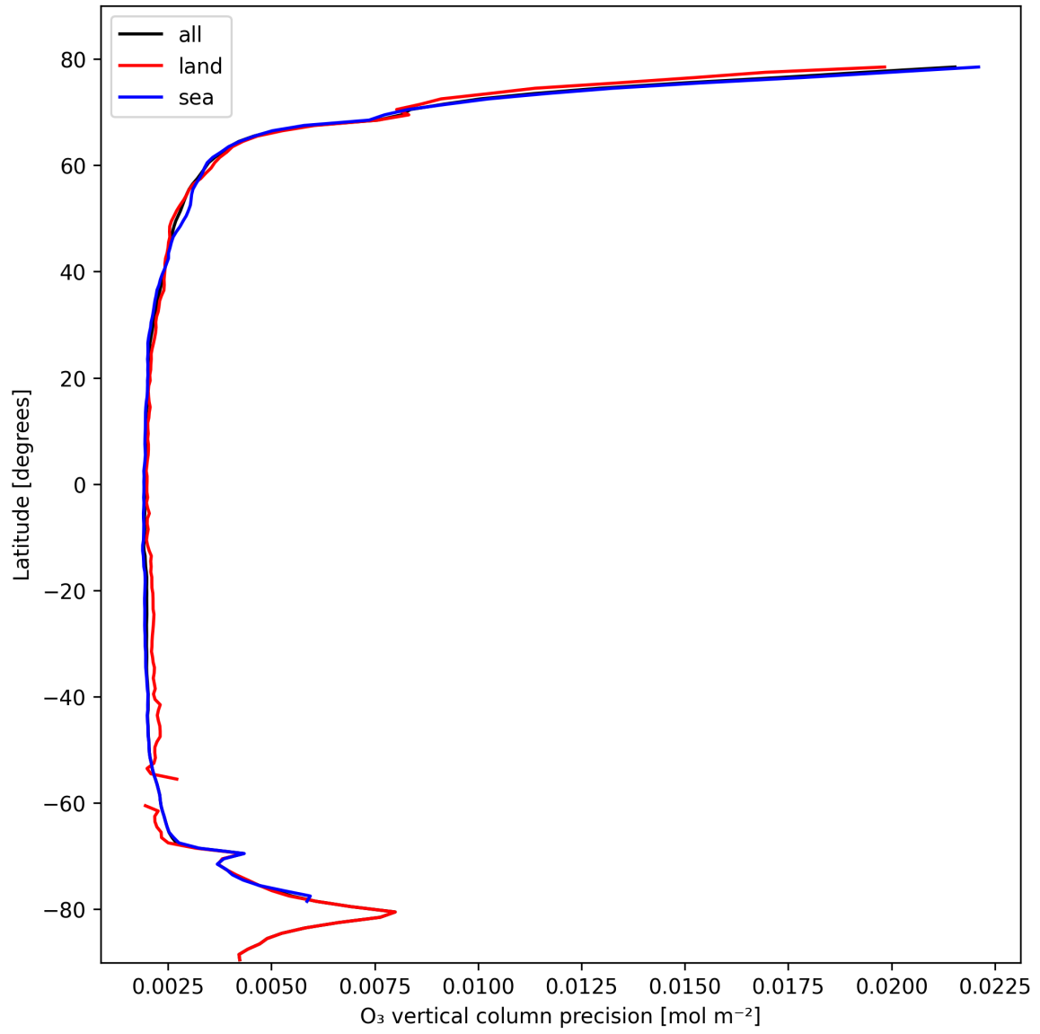
Figure 18: Zonal average of “O 3 vertical column precision” for 2025-02-21 to 2025-02-22.
