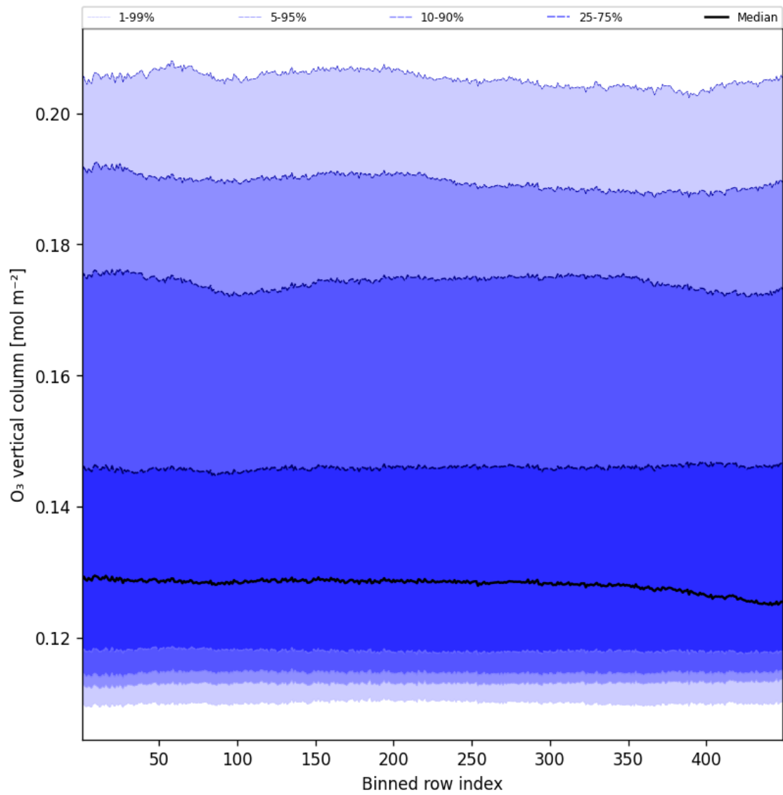
Figure 41: Along track statistics of “O 3 vertical column” for 2025-02-21 to 2025-02-22
