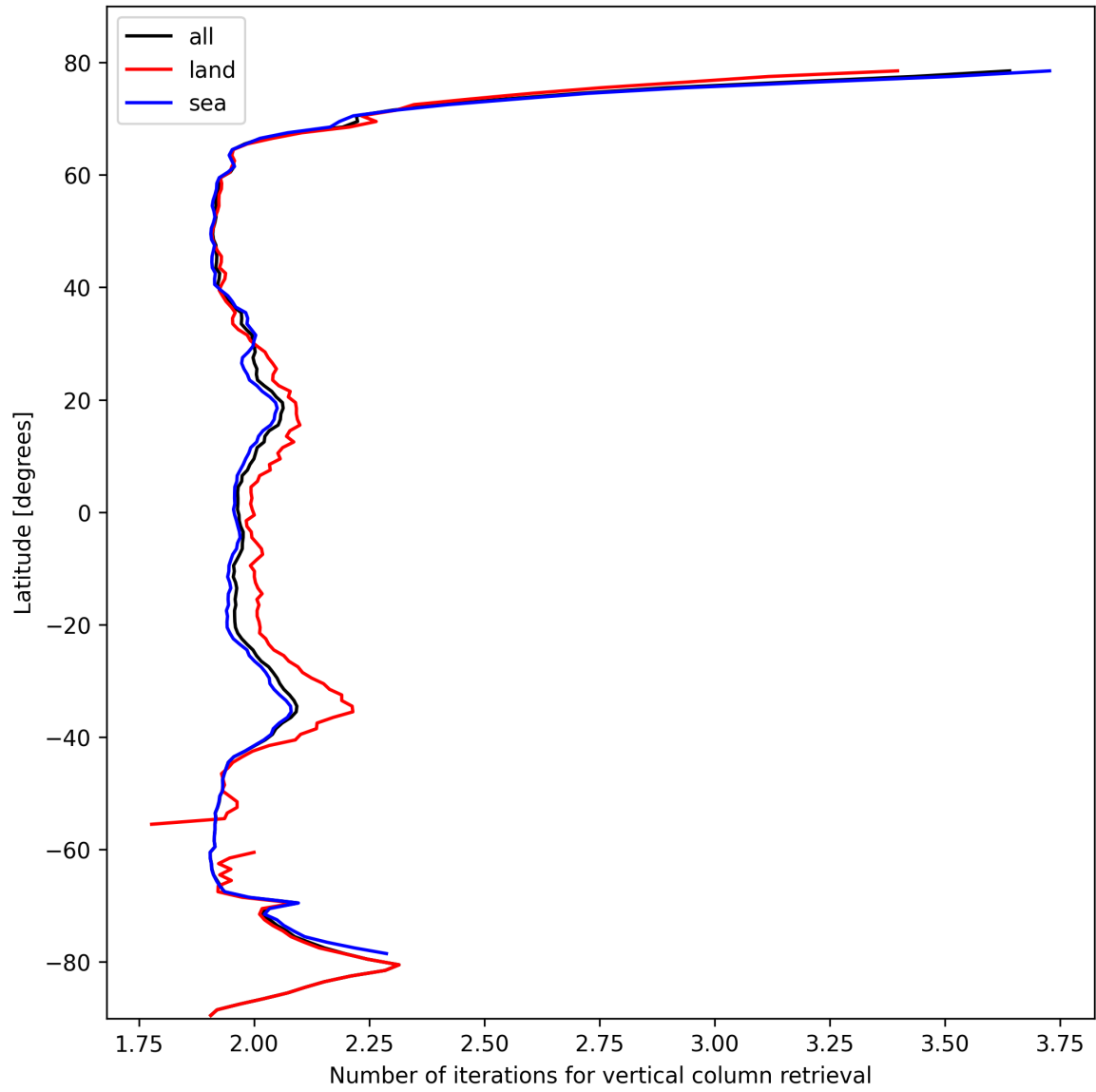
Figure 27: Zonal average of “Number of iterations for vertical column retrieval” for 2025-02-21 to 2025-02-22.
