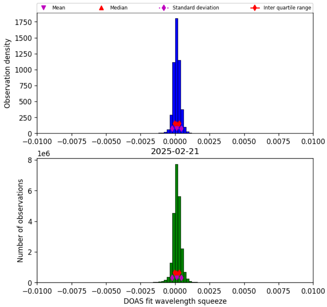
Figure 36: Histogram of “DOAS fit wavelength squeeze” for 2025-02-21 to 2025-02-22
