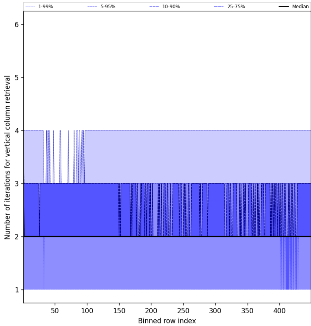
Figure 51: Along track statistics of “Number of iterations for vertical column retrieval” for 2025-02-21 to 2025-02-22
