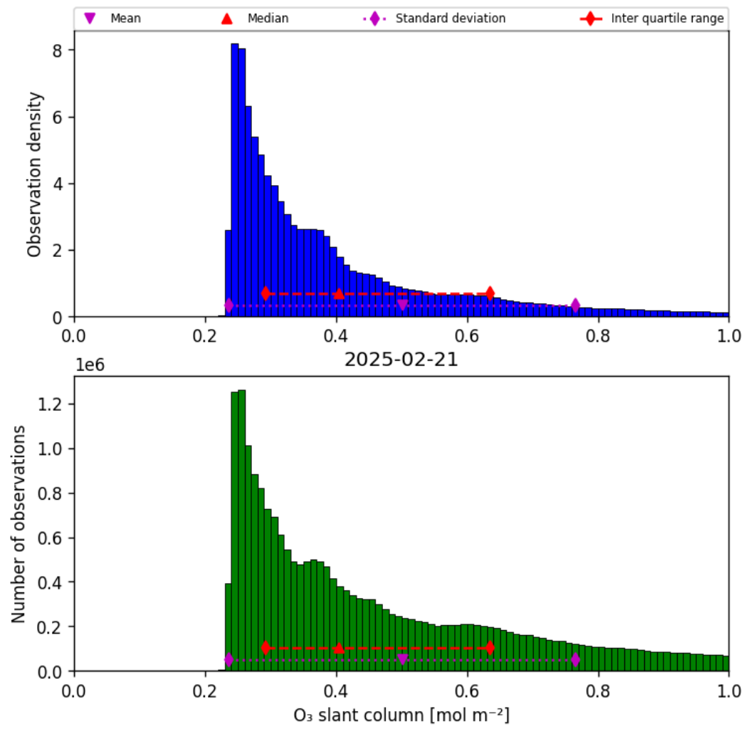
Figure 31: Histogram of “O 3 slant column” for 2025-02-21 to 2025-02-22
