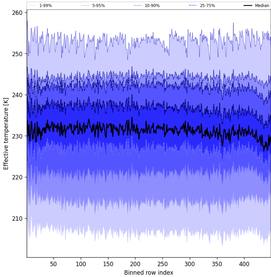
Figure 50: Along track statistics of “Effective temperature” for 2025-02-21 to 2025-02-22
