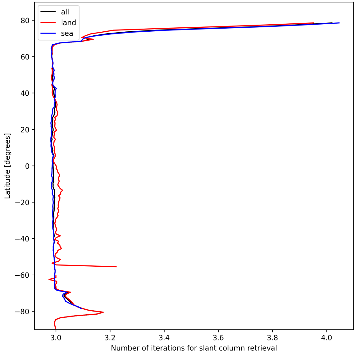
Figure 21: Zonal average of “Number of iterations for slant column retrieval” for 2025-02-21 to 2025-02-22.
