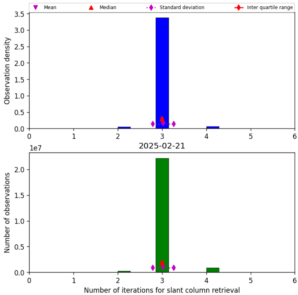
Figure 33: Histogram of “Number of iterations for slant column retrieval” for 2025-02-21 to 2025-02-22
