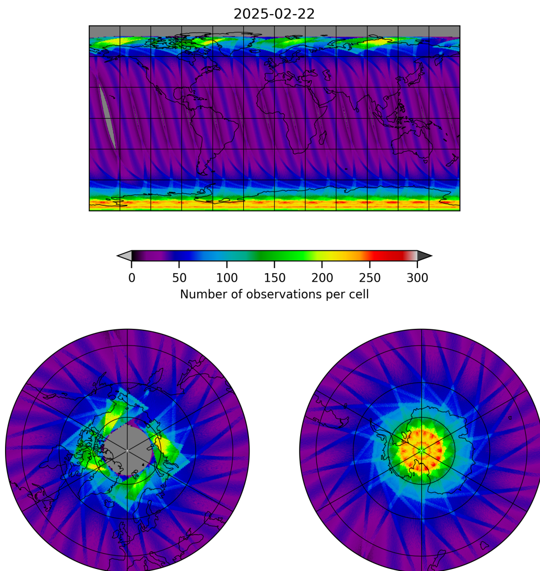
Figure 15: Map of the number of observations for 2025-02-22 to 2025-02-22
