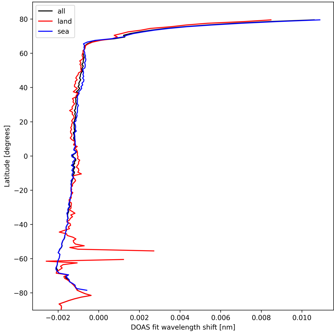
Figure 23: Zonal average of “DOAS fit wavelength shift” for 2025-02-22 to 2025-02-22.
