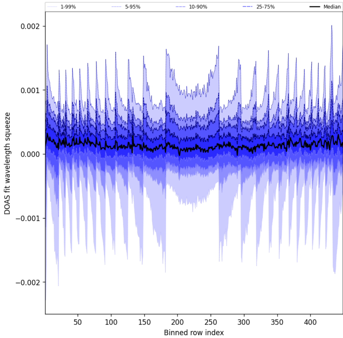
Figure 48: Along track statistics of “DOAS fit wavelength squeeze” for 2025-02-22 to 2025-02-22
