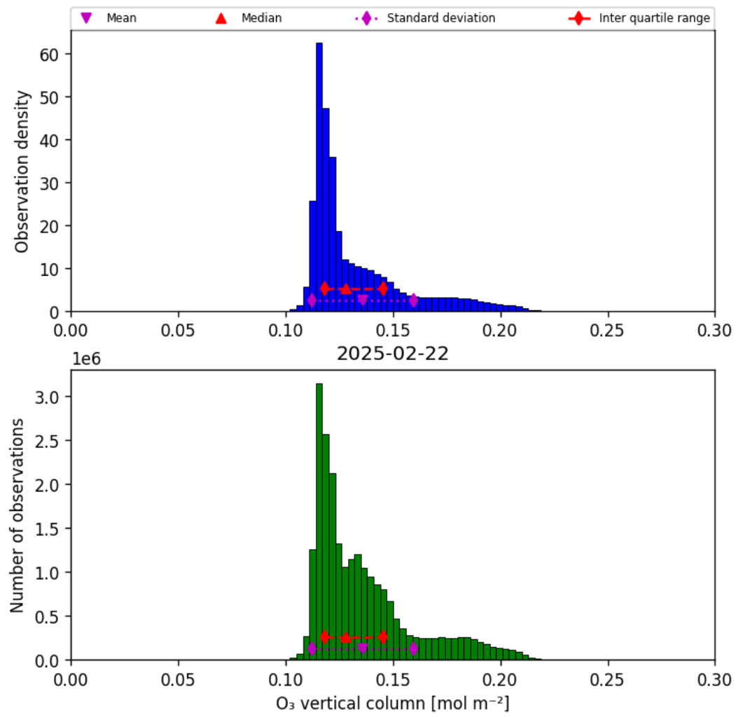
Figure 29: Histogram of “O 3 vertical column” for 2025-02-22 to 2025-02-22
