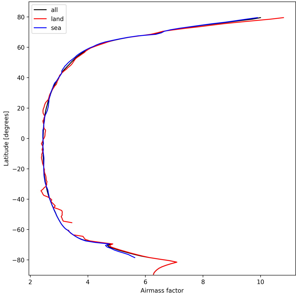
Figure 25: Zonal average of “Airmass factor” for 2025-02-22 to 2025-02-22.
