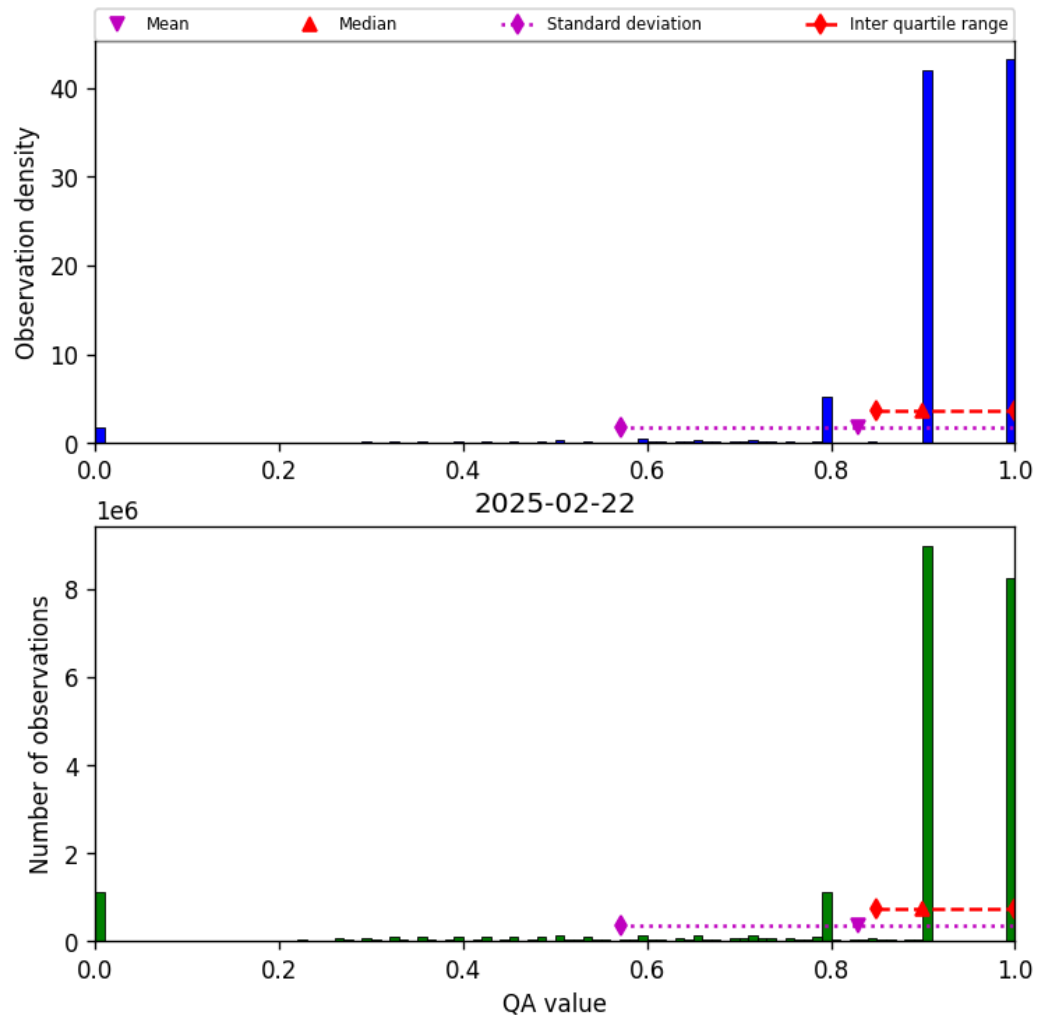
Figure 28: Histogram of “QA value” for 2025-02-22 to 2025-02-22
