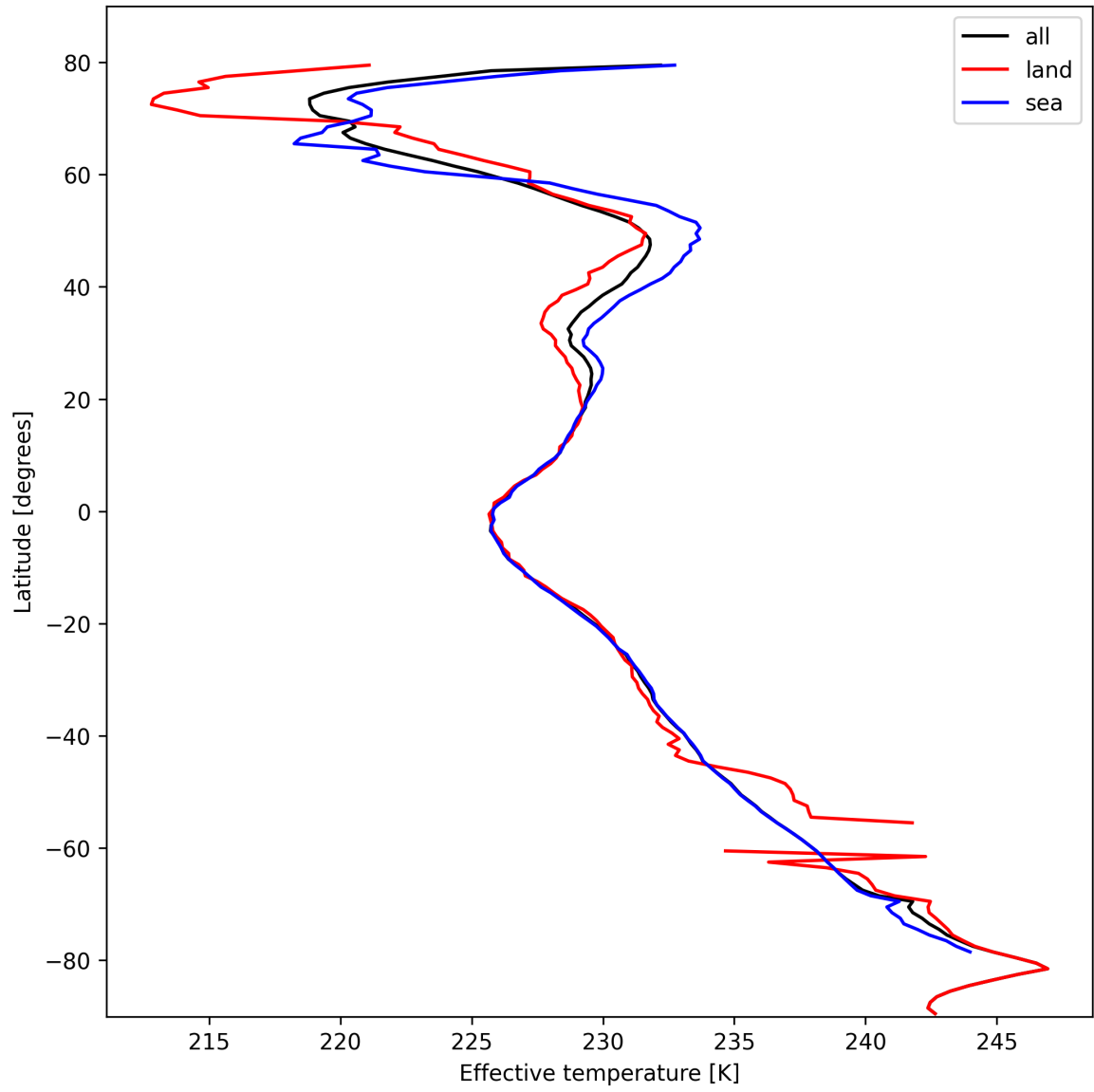
Figure 26: Zonal average of “Effective temperature” for 2025-02-22 to 2025-02-22.
