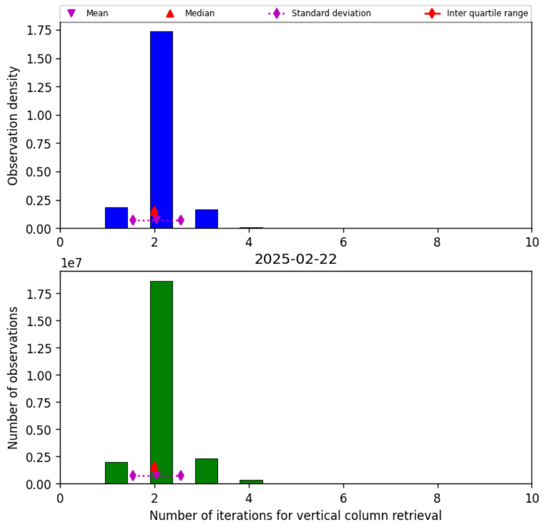
Figure 39: Histogram of “Number of iterations for vertical column retrieval” for 2025-02-22 to 2025-02-22
