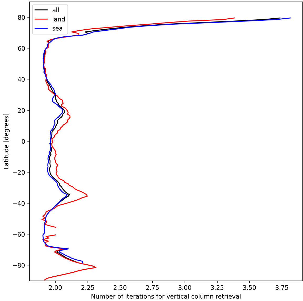
Figure 27: Zonal average of “Number of iterations for vertical column retrieval” for 2025-02-22 to 2025-02-22.
