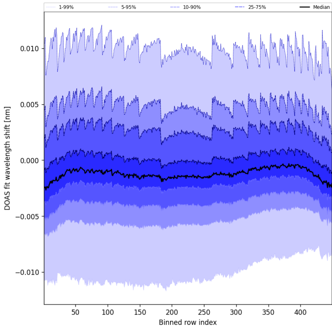
Figure 47: Along track statistics of “DOAS fit wavelength shift” for 2025-02-22 to 2025-02-22
