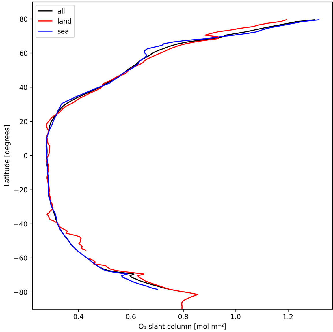
Figure 19: Zonal average of “O 3 slant column” for 2025-02-22 to 2025-02-22.
