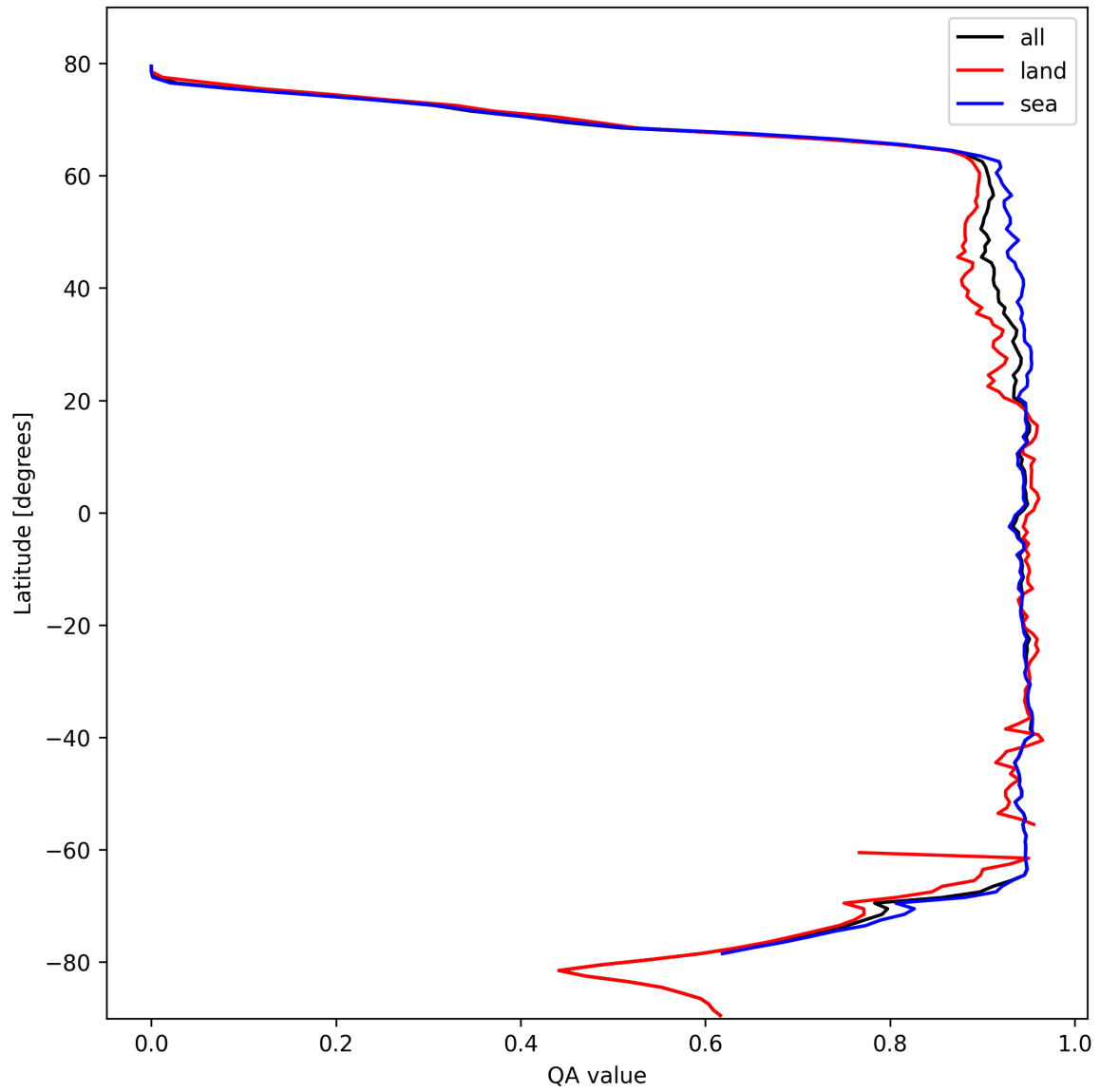
Figure 16: Zonal average of “QA value” for 2025-02-22 to 2025-02-22.
