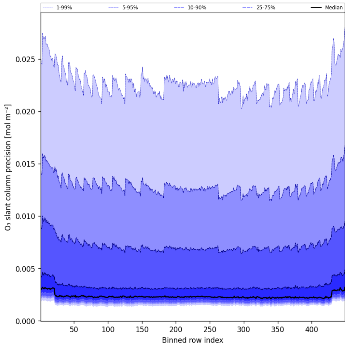
Figure 44: Along track statistics of “O 3 slant column precision” for 2025-02-22 to 2025-02-22
