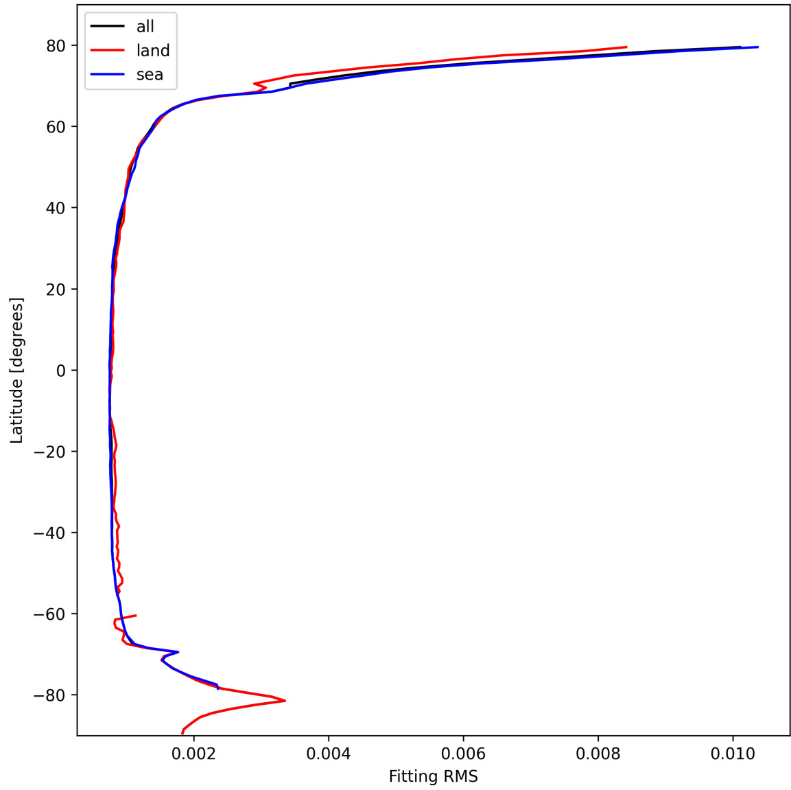
Figure 22: Zonal average of “Fitting RMS” for 2025-02-22 to 2025-02-22.
