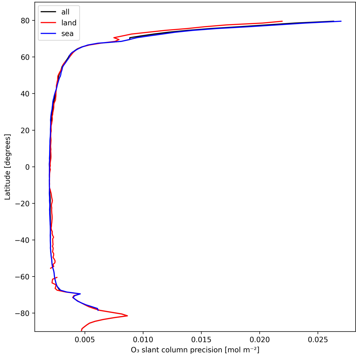
Figure 20: Zonal average of “O 3 slant column precision” for 2025-02-22 to 2025-02-22.
