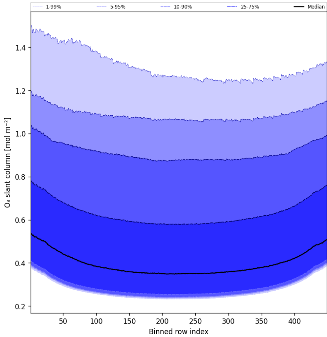
Figure 43: Along track statistics of “O 3 slant column” for 2025-02-22 to 2025-02-22
