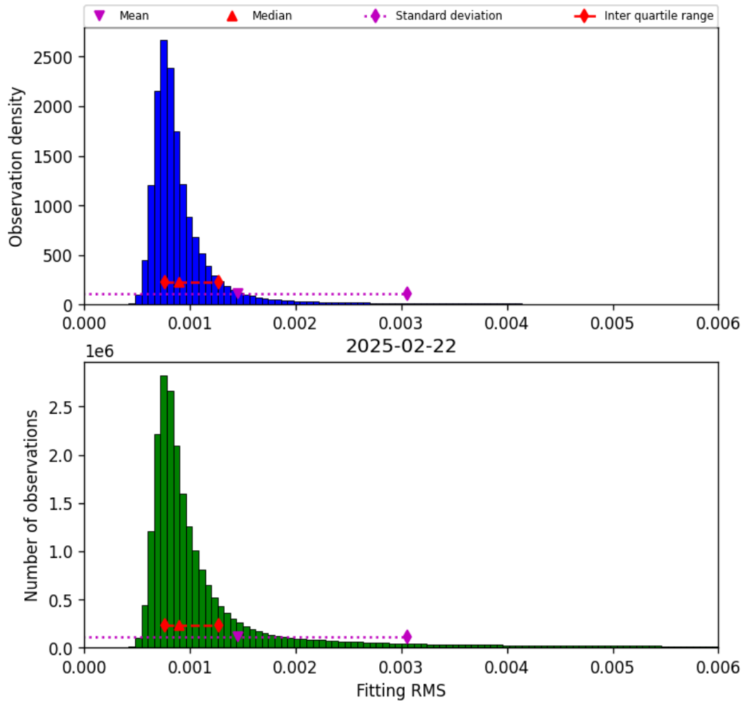
Figure 34: Histogram of “Fitting RMS” for 2025-02-22 to 2025-02-22
