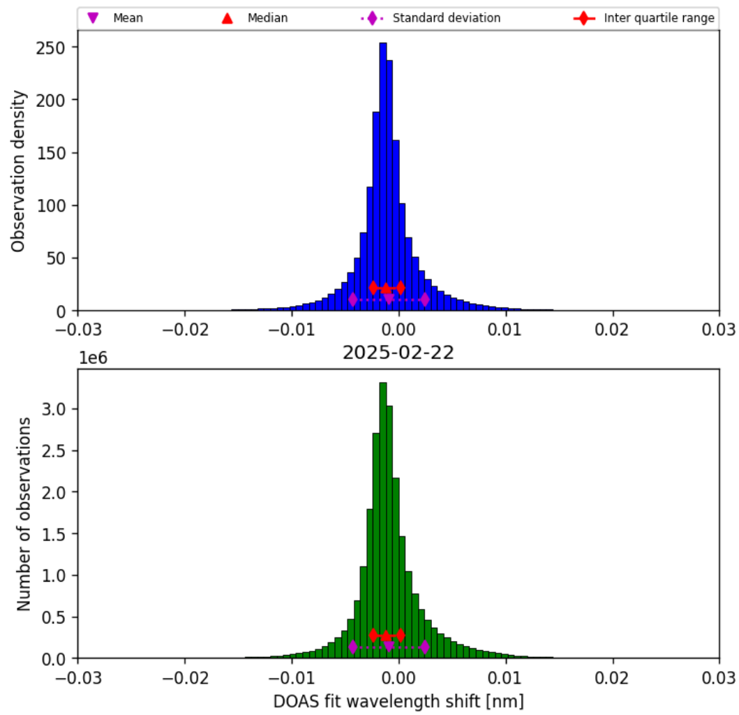
Figure 35: Histogram of “DOAS fit wavelength shift” for 2025-02-22 to 2025-02-22
