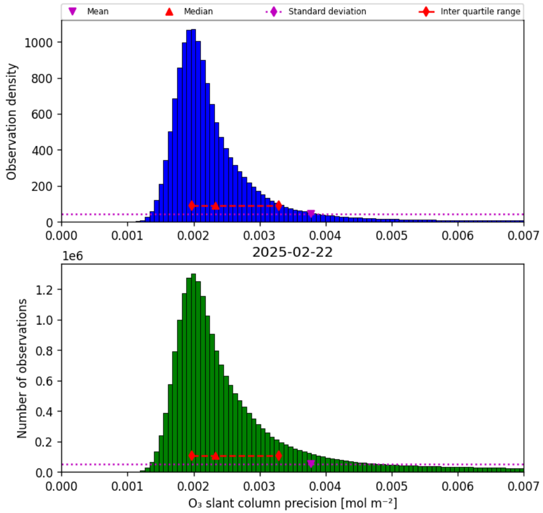
Figure 32: Histogram of “O 3 slant column precision” for 2025-02-22 to 2025-02-22
