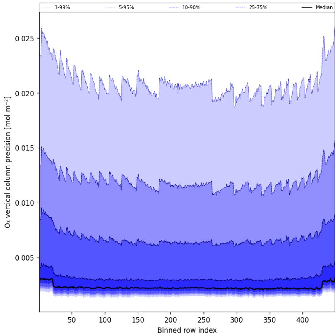
Figure 42: Along track statistics of “O 3 vertical column precision” for 2025-02-22 to 2025-02-22
