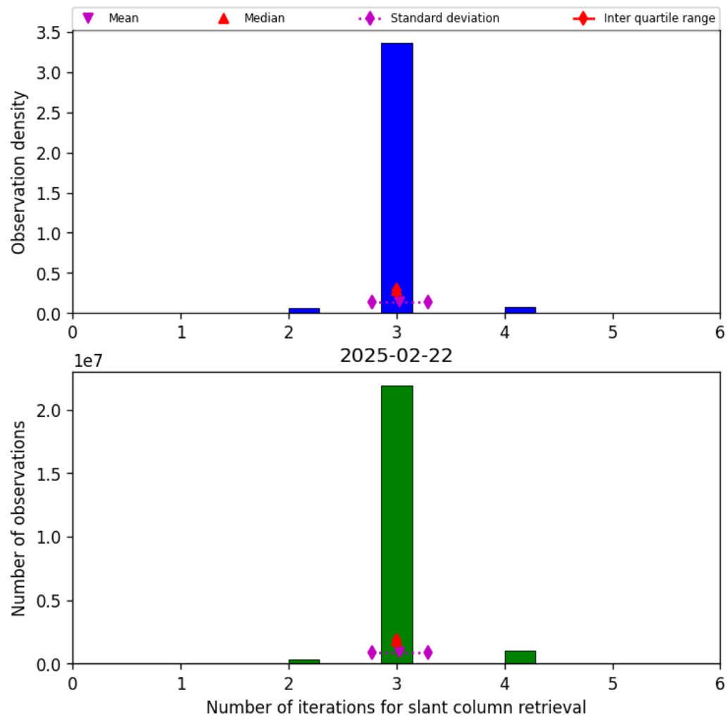
Figure 33: Histogram of “Number of iterations for slant column retrieval” for 2025-02-22 to 2025-02-22
