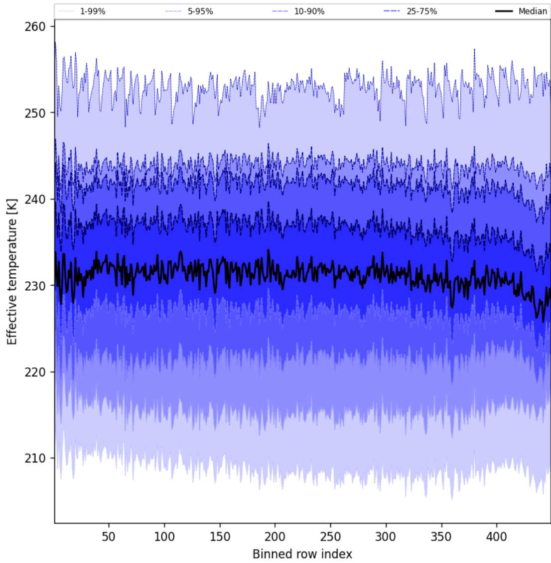
Figure 50: Along track statistics of “Effective temperature” for 2025-02-22 to 2025-02-22
