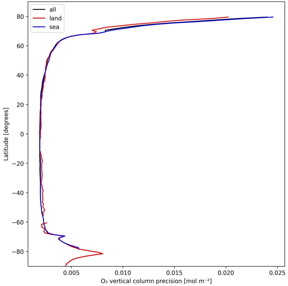
Figure 18: Zonal average of “O 3 vertical column precision” for 2025-02-22 to 2025-02-22.
