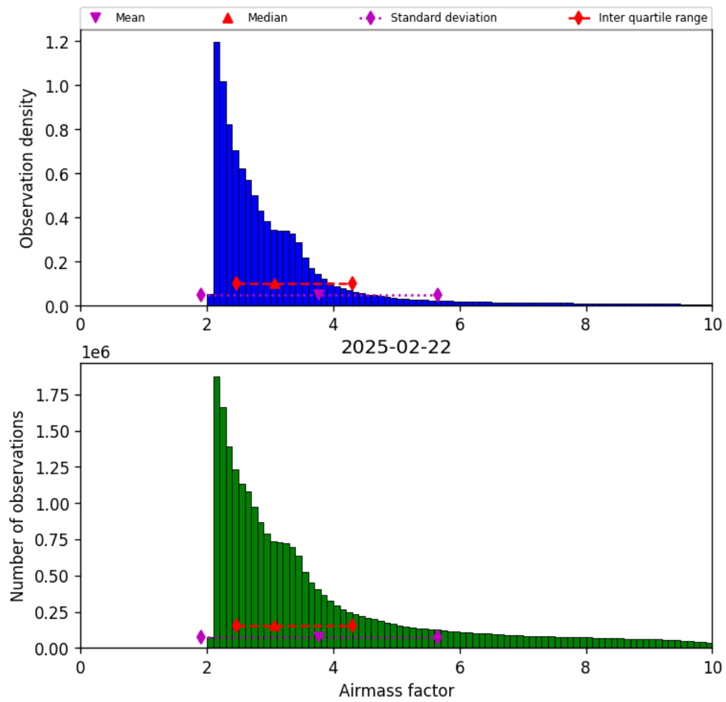
Figure 37: Histogram of “Airmass factor” for 2025-02-22 to 2025-02-22
