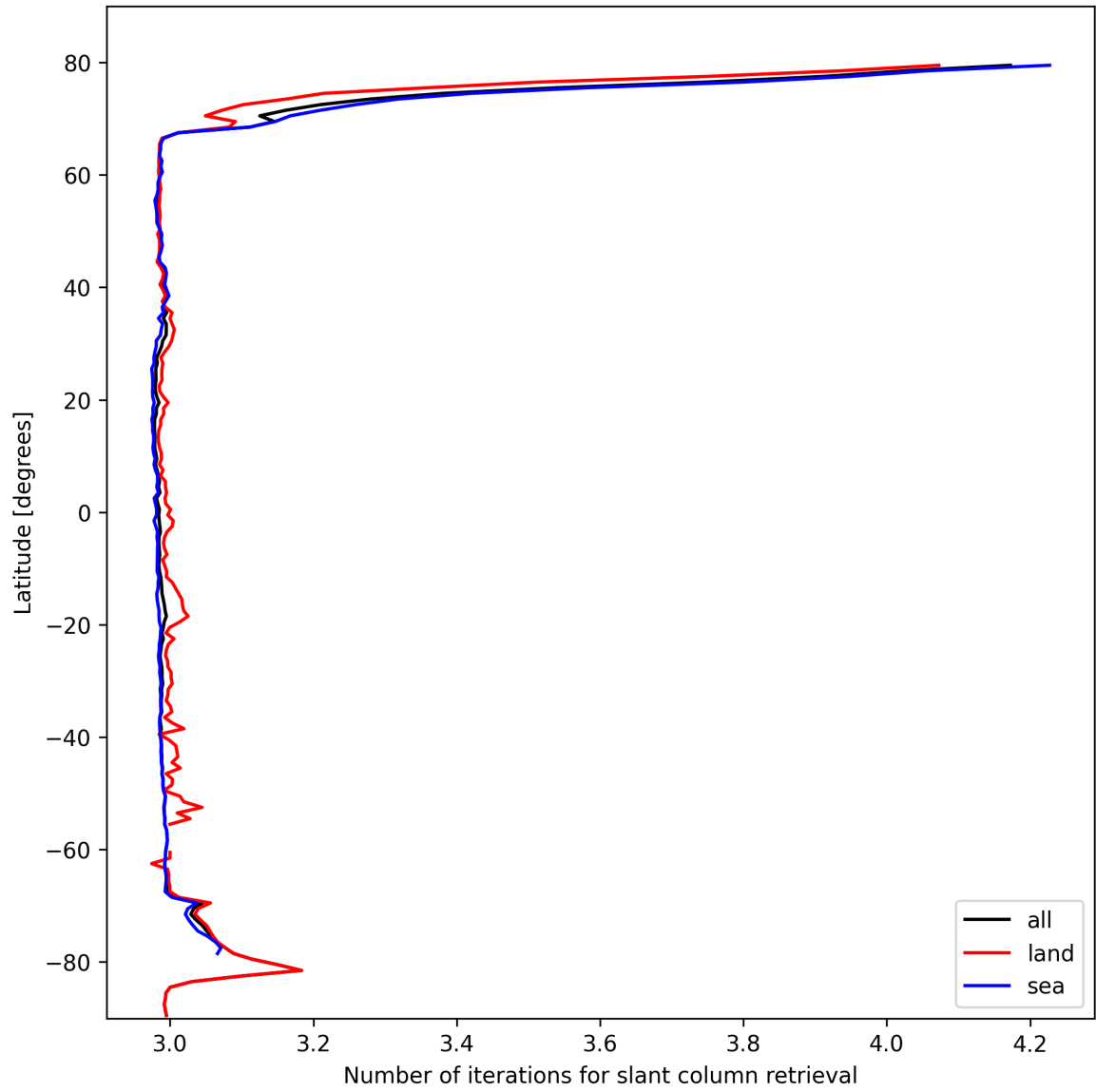
Figure 21: Zonal average of “Number of iterations for slant column retrieval” for 2025-02-22 to 2025-02-22.
