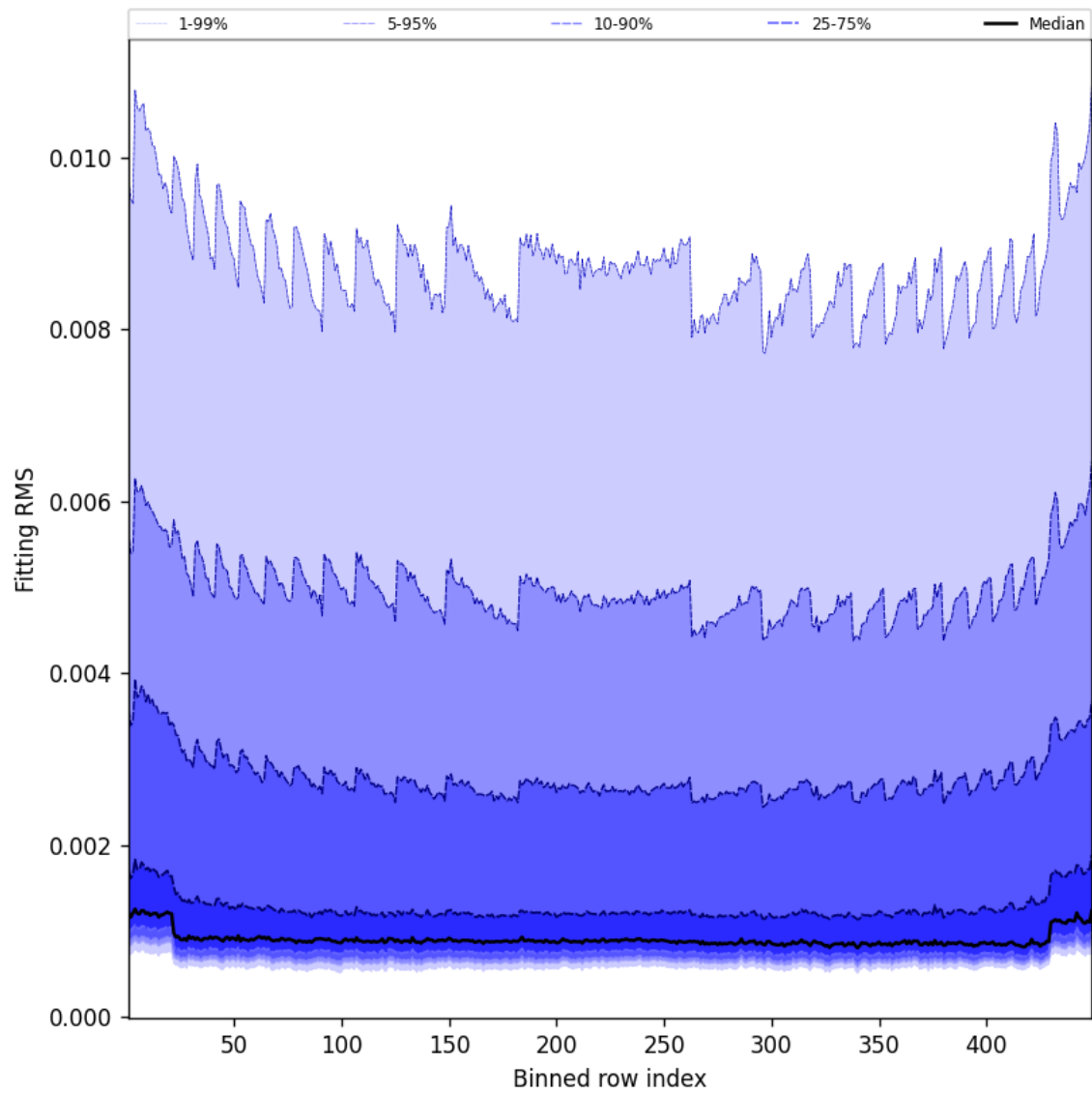
Figure 46: Along track statistics of “Fitting RMS” for 2025-02-22 to 2025-02-22
