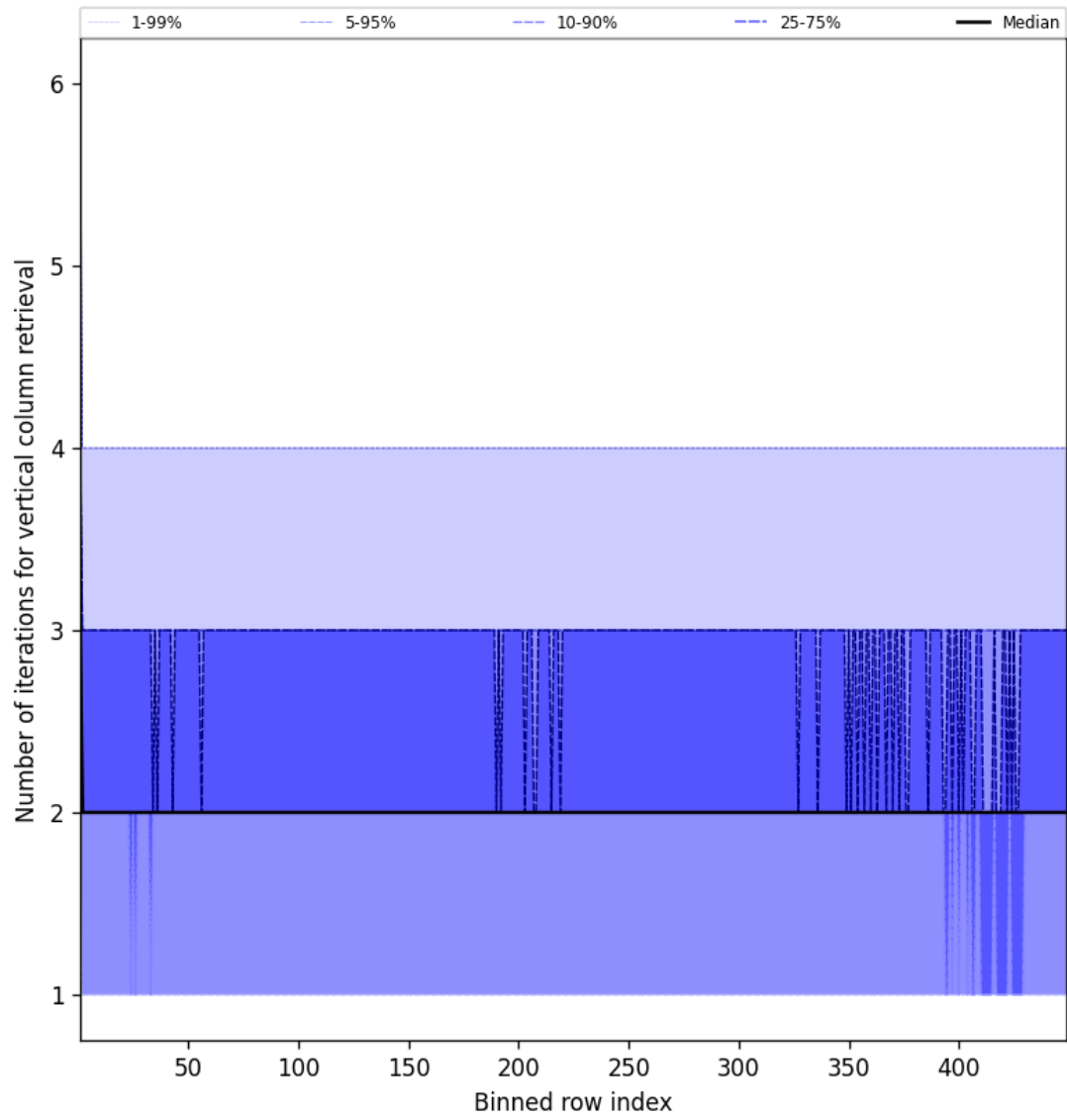
Figure 51: Along track statistics of “Number of iterations for vertical column retrieval” for 2025-02-22 to 2025-02-22
