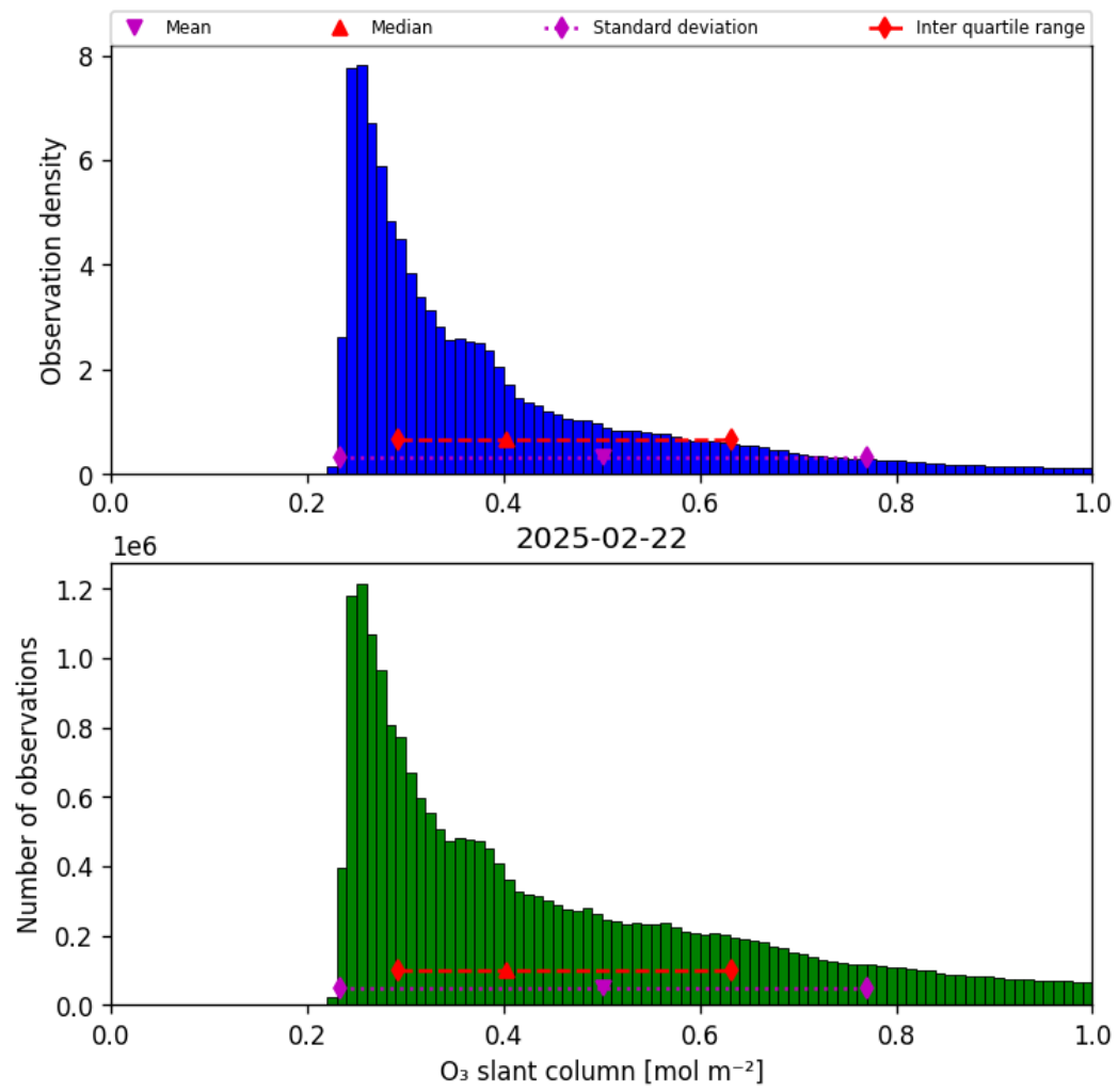
Figure 31: Histogram of “O 3 slant column” for 2025-02-22 to 2025-02-22
