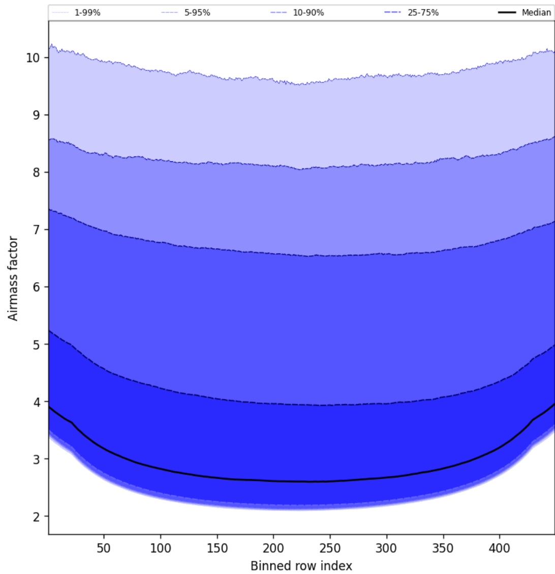
Figure 49: Along track statistics of “Airmass factor” for 2025-02-22 to 2025-02-22
