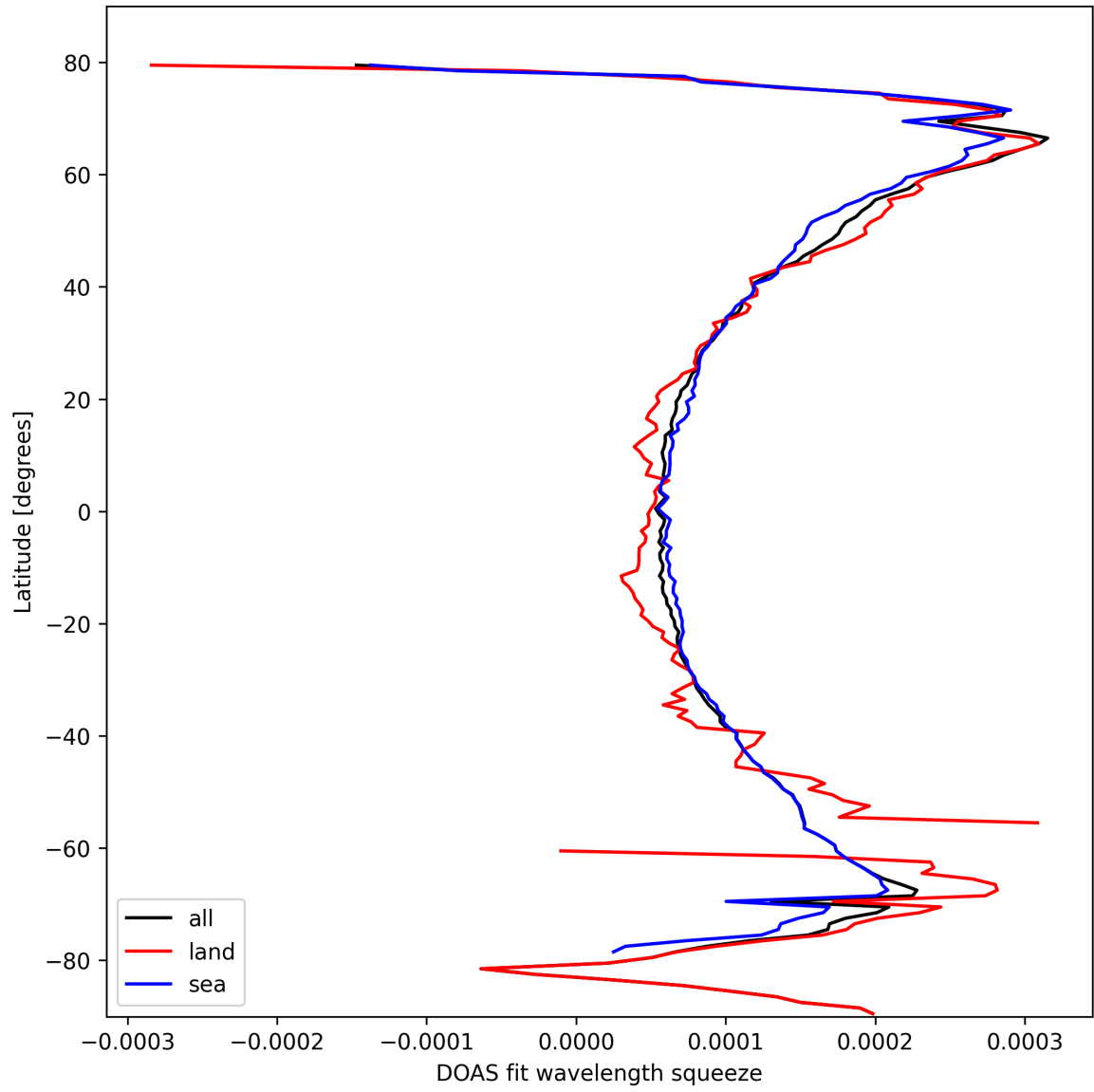
Figure 24: Zonal average of “DOAS fit wavelength squeeze” for 2025-02-22 to 2025-02-22.
