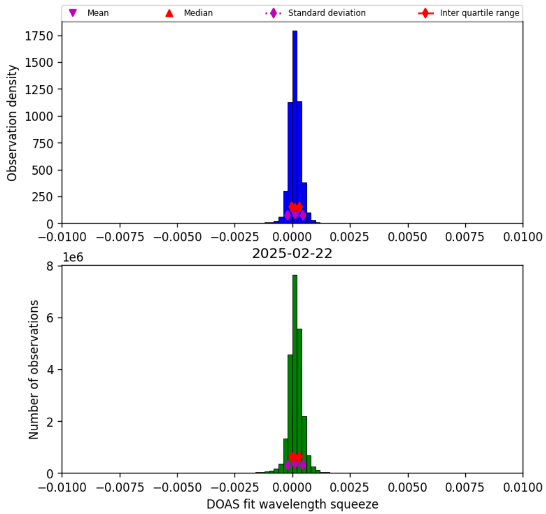
Figure 36: Histogram of “DOAS fit wavelength squeeze” for 2025-02-22 to 2025-02-22
