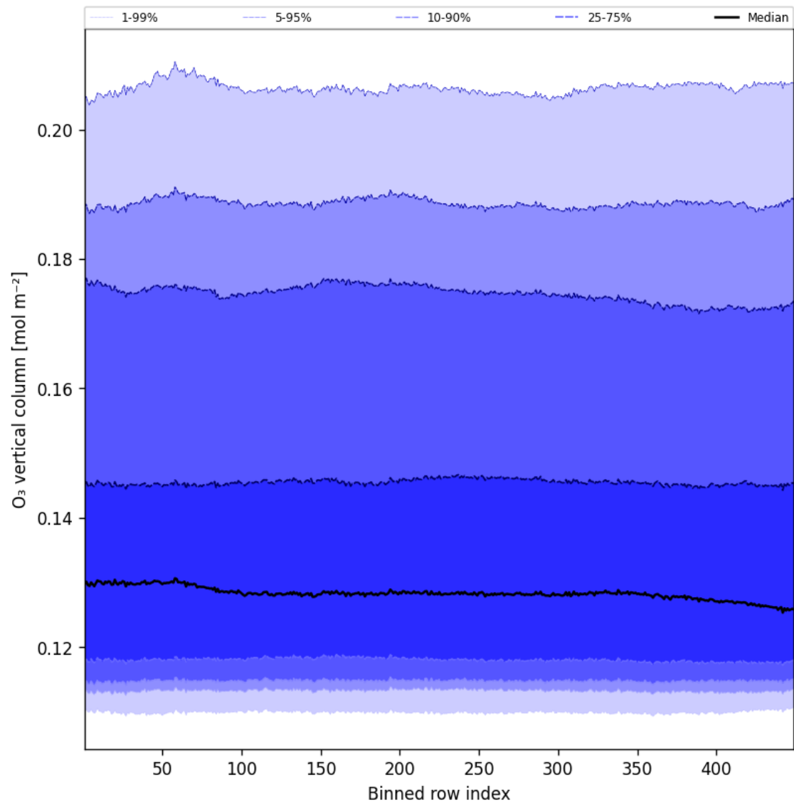
Figure 41: Along track statistics of “O 3 vertical column” for 2025-02-22 to 2025-02-22
