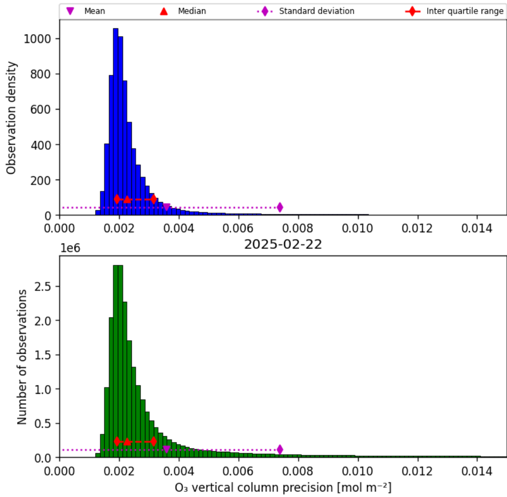
Figure 30: Histogram of “O 3 vertical column precision” for 2025-02-22 to 2025-02-22
