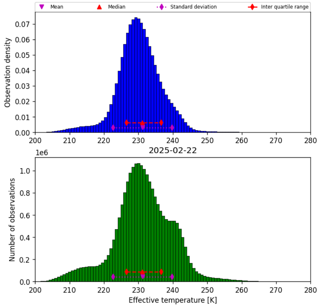
Figure 38: Histogram of “Effective temperature” for 2025-02-22 to 2025-02-22
