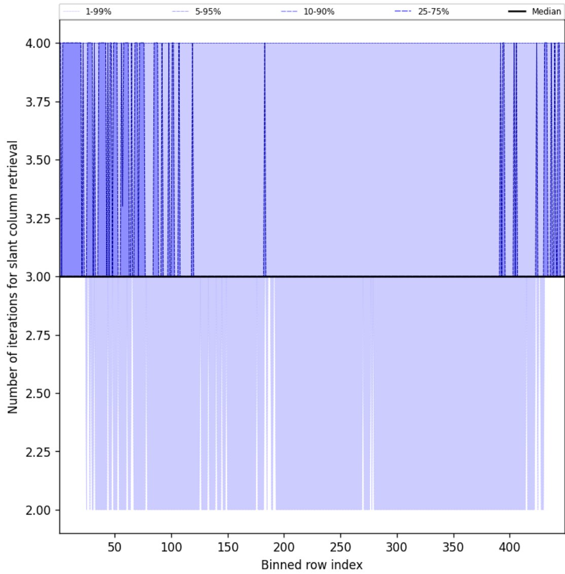
Figure 45: Along track statistics of “Number of iterations for slant column retrieval” for 2025-02-22 to 2025-02-22
