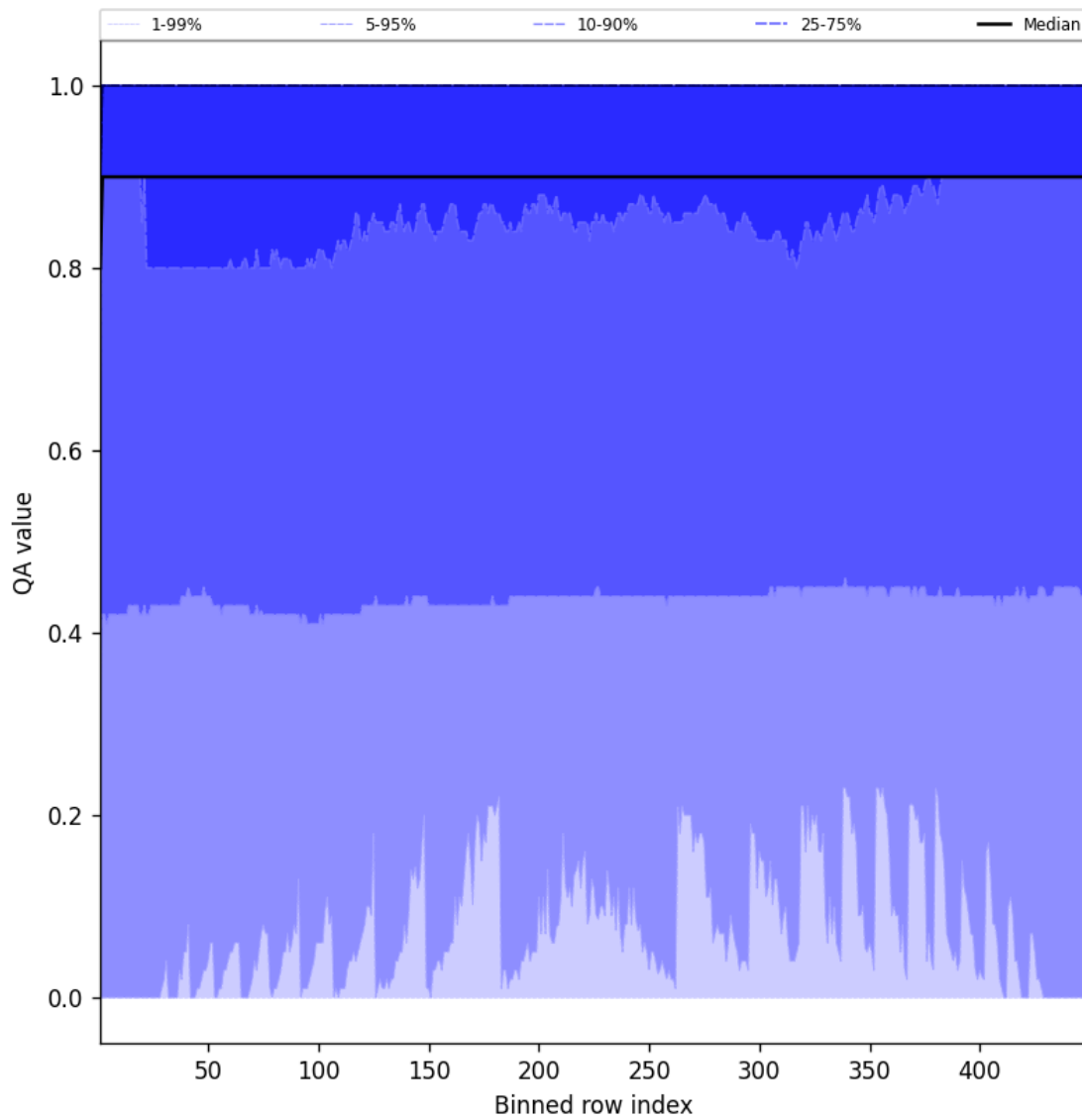
Figure 40: Along track statistics of “QA value” for 2025-02-22 to 2025-02-22
