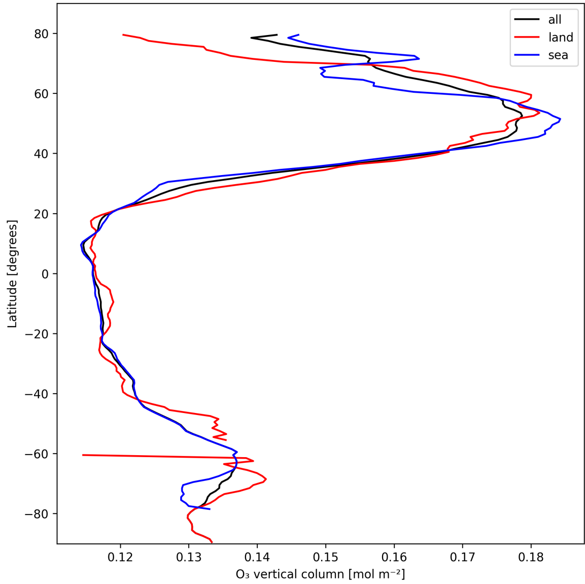
Figure 17: Zonal average of “O 3 vertical column” for 2025-02-22 to 2025-02-22.
