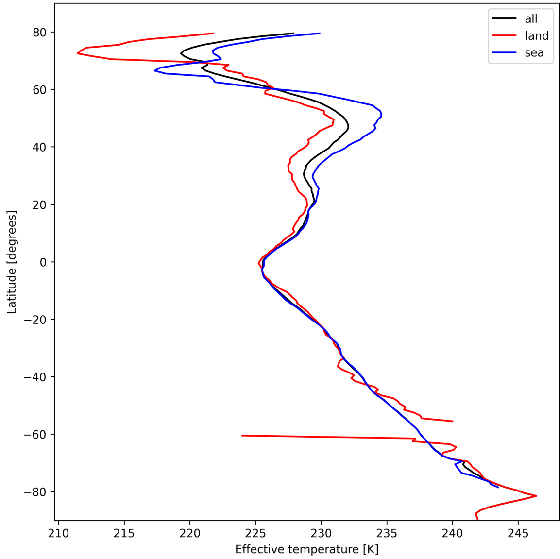
Figure 26: Zonal average of “Effective temperature” for 2025-02-23 to 2025-02-24.
