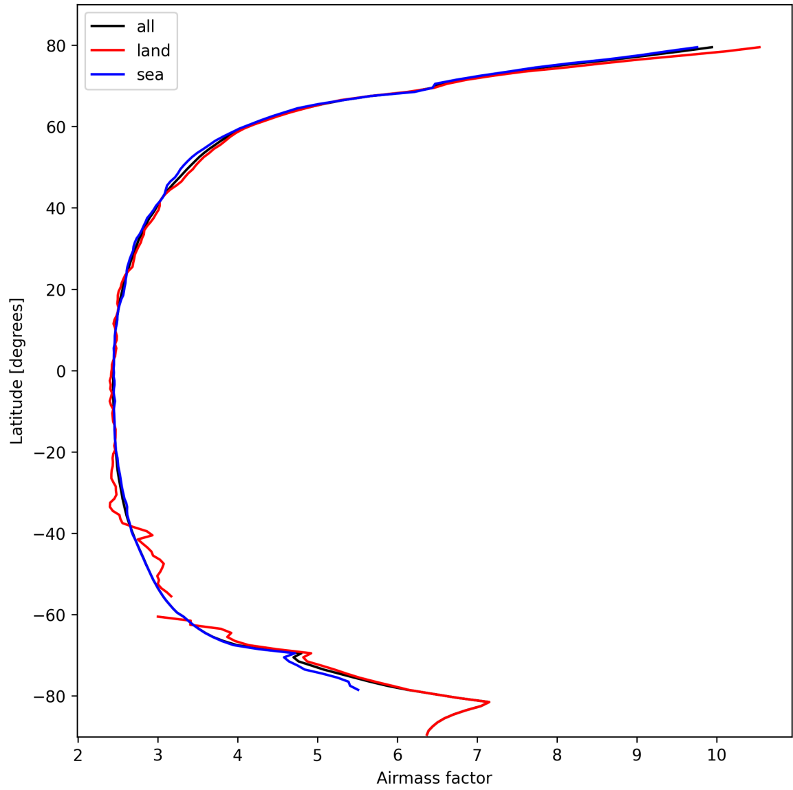
Figure 25: Zonal average of “Airmass factor” for 2025-02-23 to 2025-02-24.
