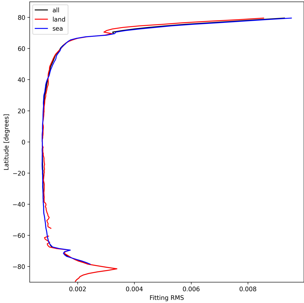
Figure 22: Zonal average of “Fitting RMS” for 2025-02-23 to 2025-02-24.
