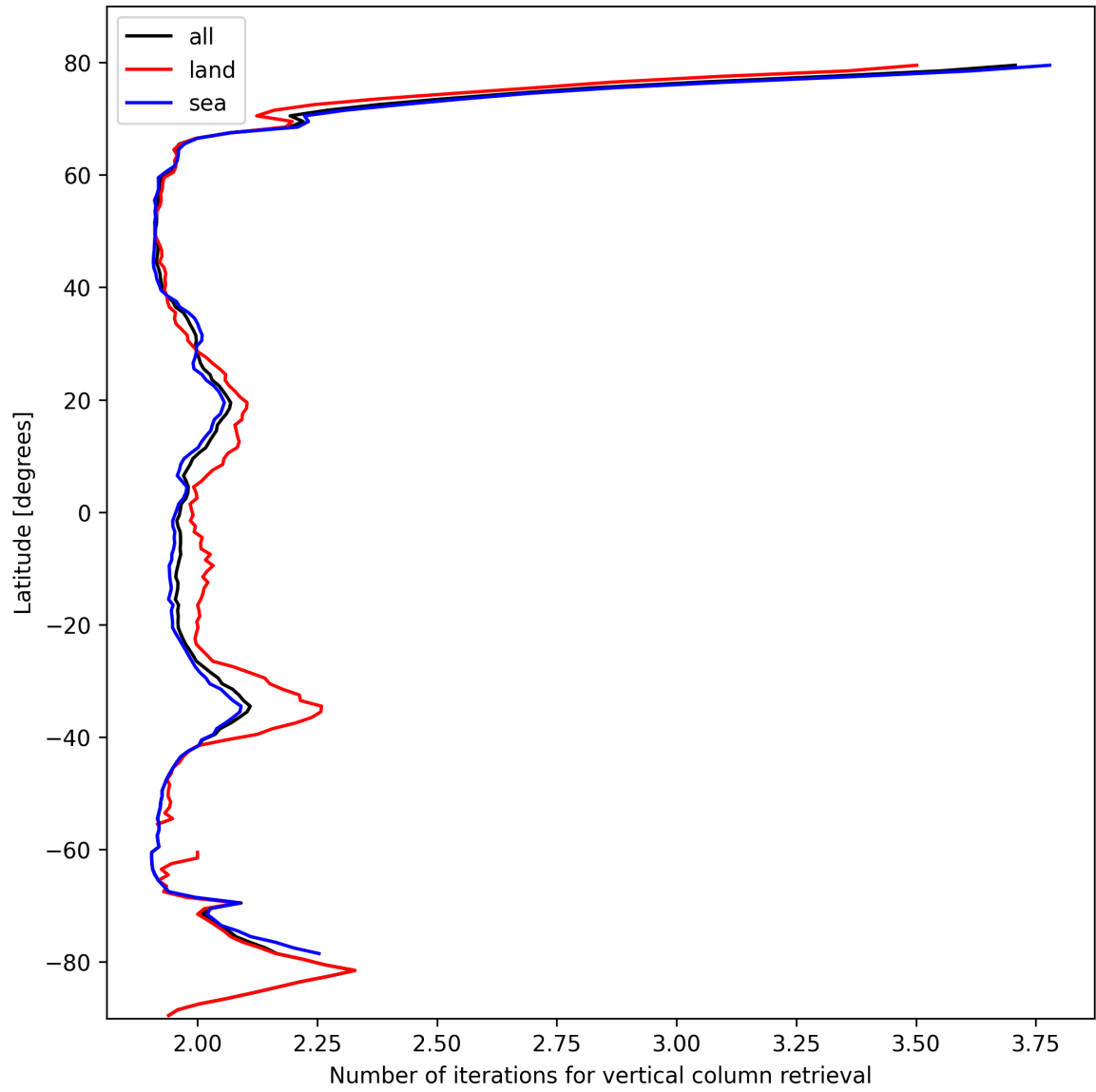
Figure 27: Zonal average of “Number of iterations for vertical column retrieval” for 2025-02-23 to 2025-02-24.
