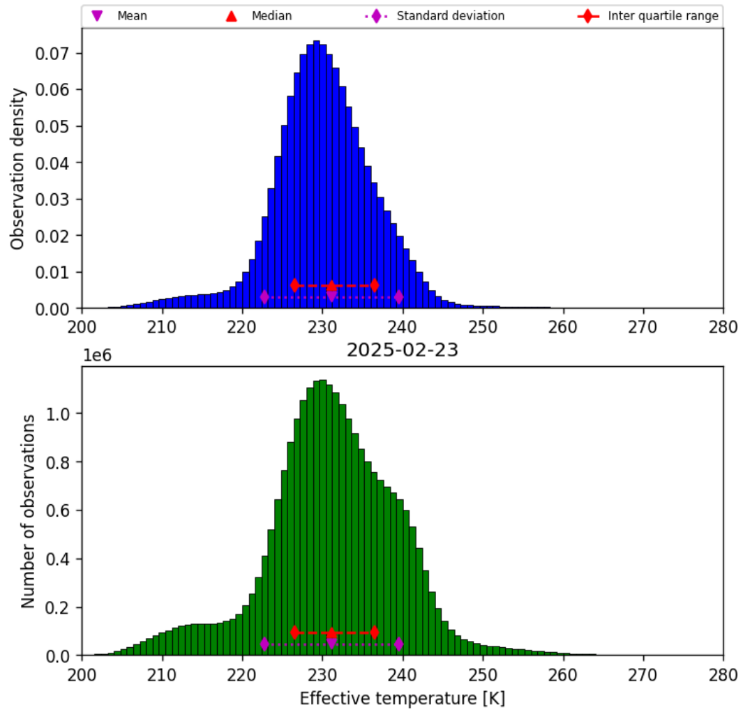
Figure 38: Histogram of “Effective temperature” for 2025-02-23 to 2025-02-24
