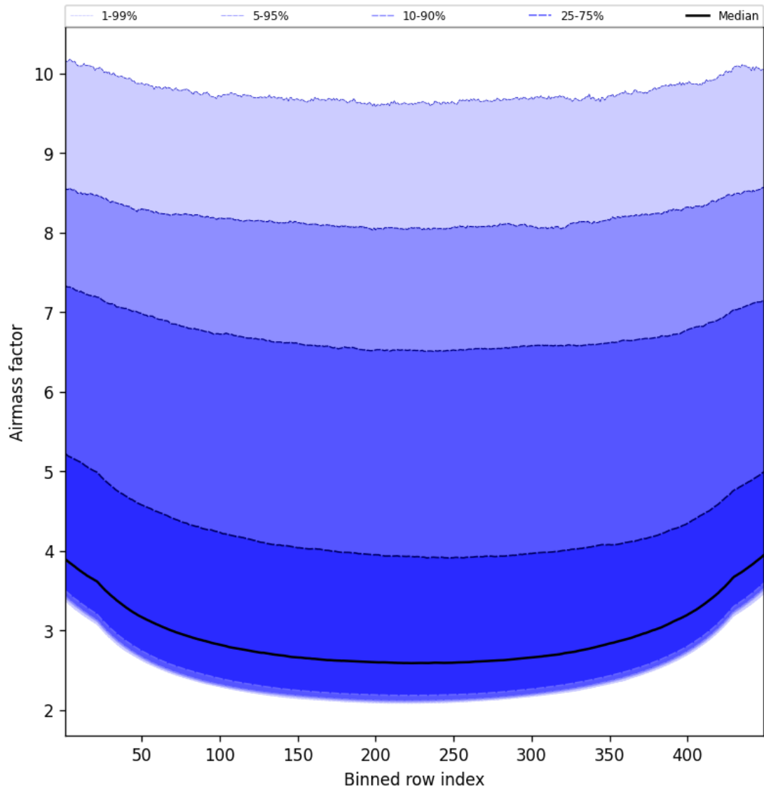
Figure 49: Along track statistics of “Airmass factor” for 2025-02-23 to 2025-02-24
