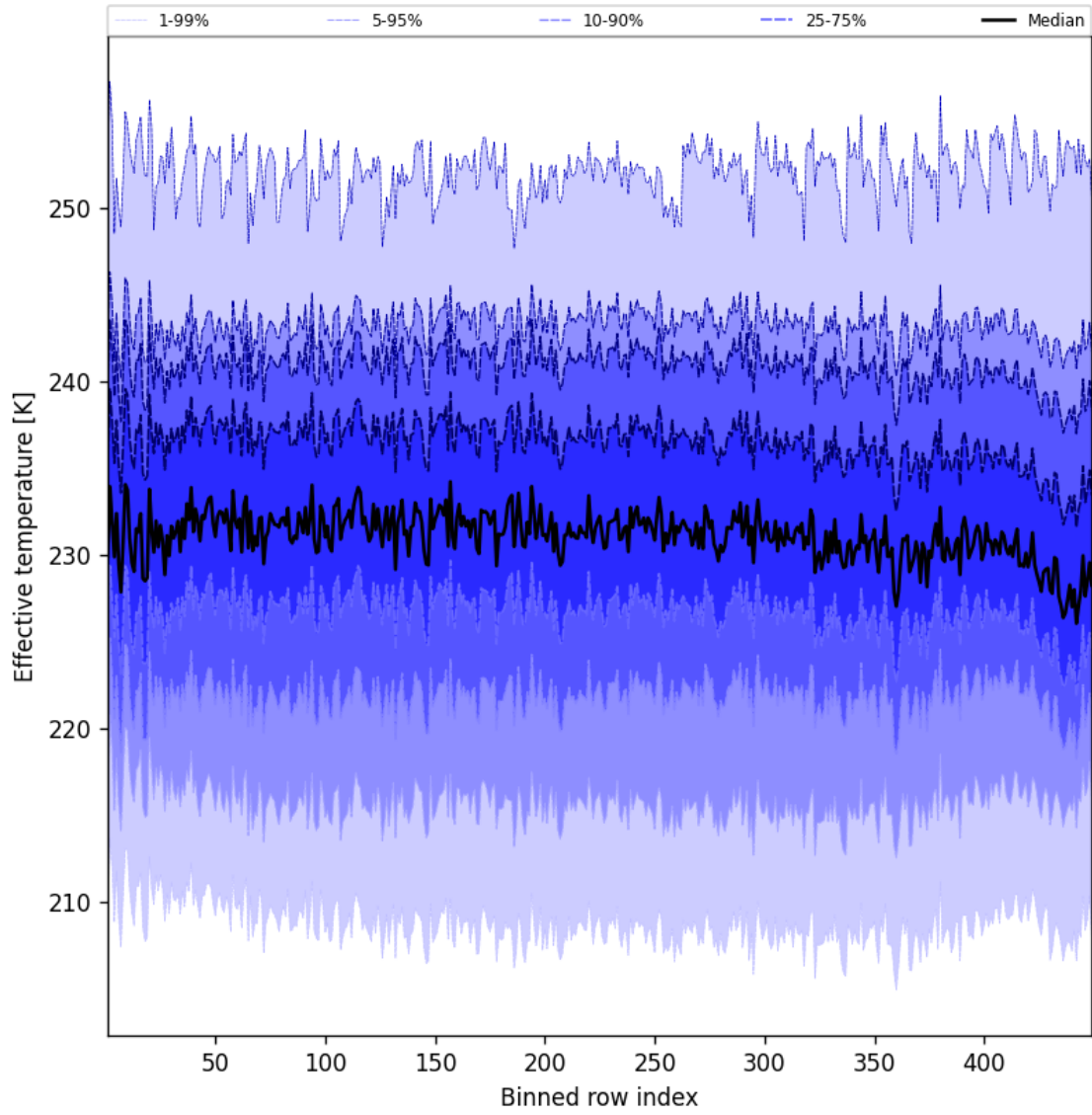
Figure 50: Along track statistics of “Effective temperature” for 2025-02-23 to 2025-02-24
