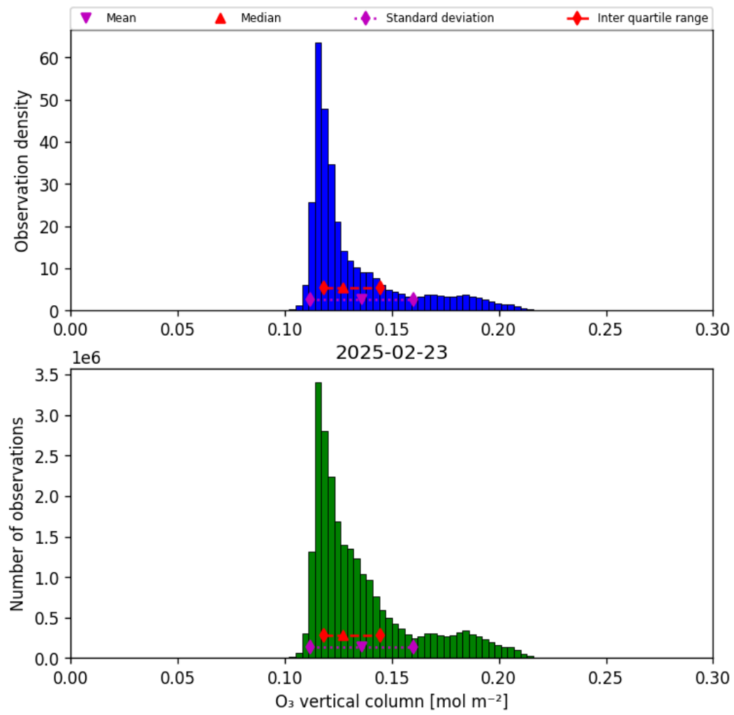
Figure 29: Histogram of “O 3 vertical column” for 2025-02-23 to 2025-02-24
