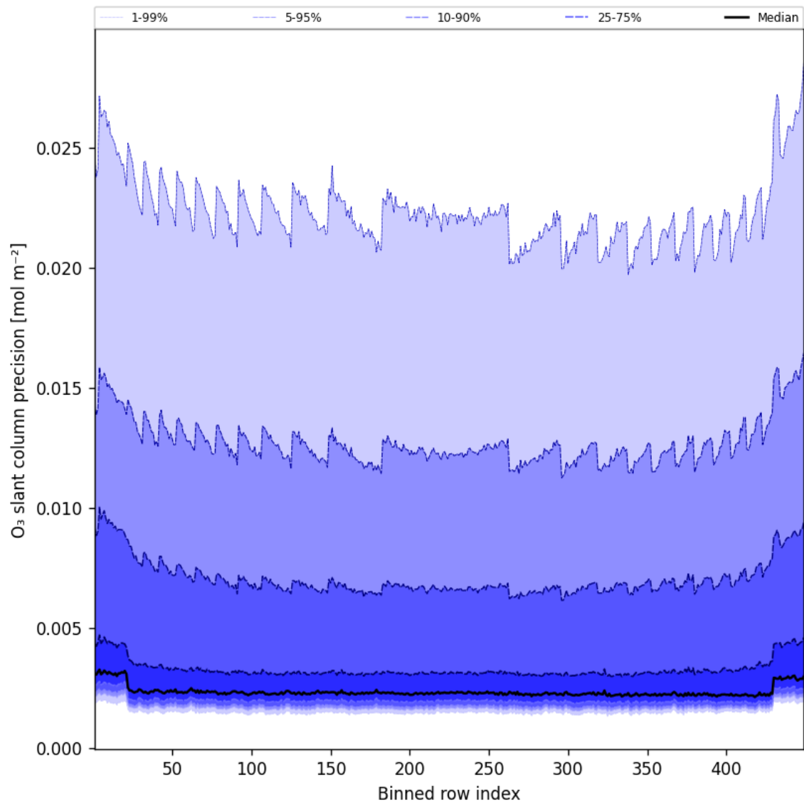
Figure 44: Along track statistics of “O 3 slant column precision” for 2025-02-23 to 2025-02-24
