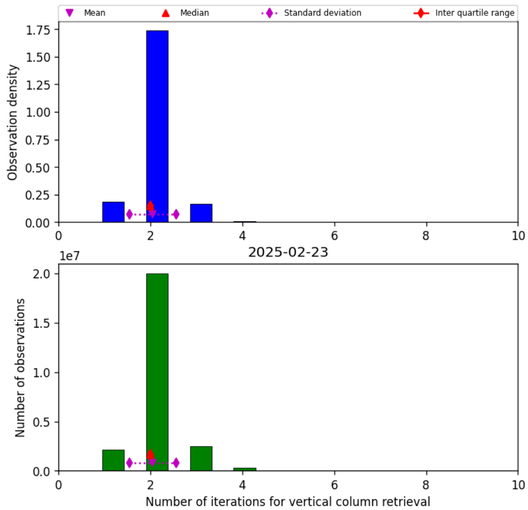
Figure 39: Histogram of “Number of iterations for vertical column retrieval” for 2025-02-23 to 2025-02-24
