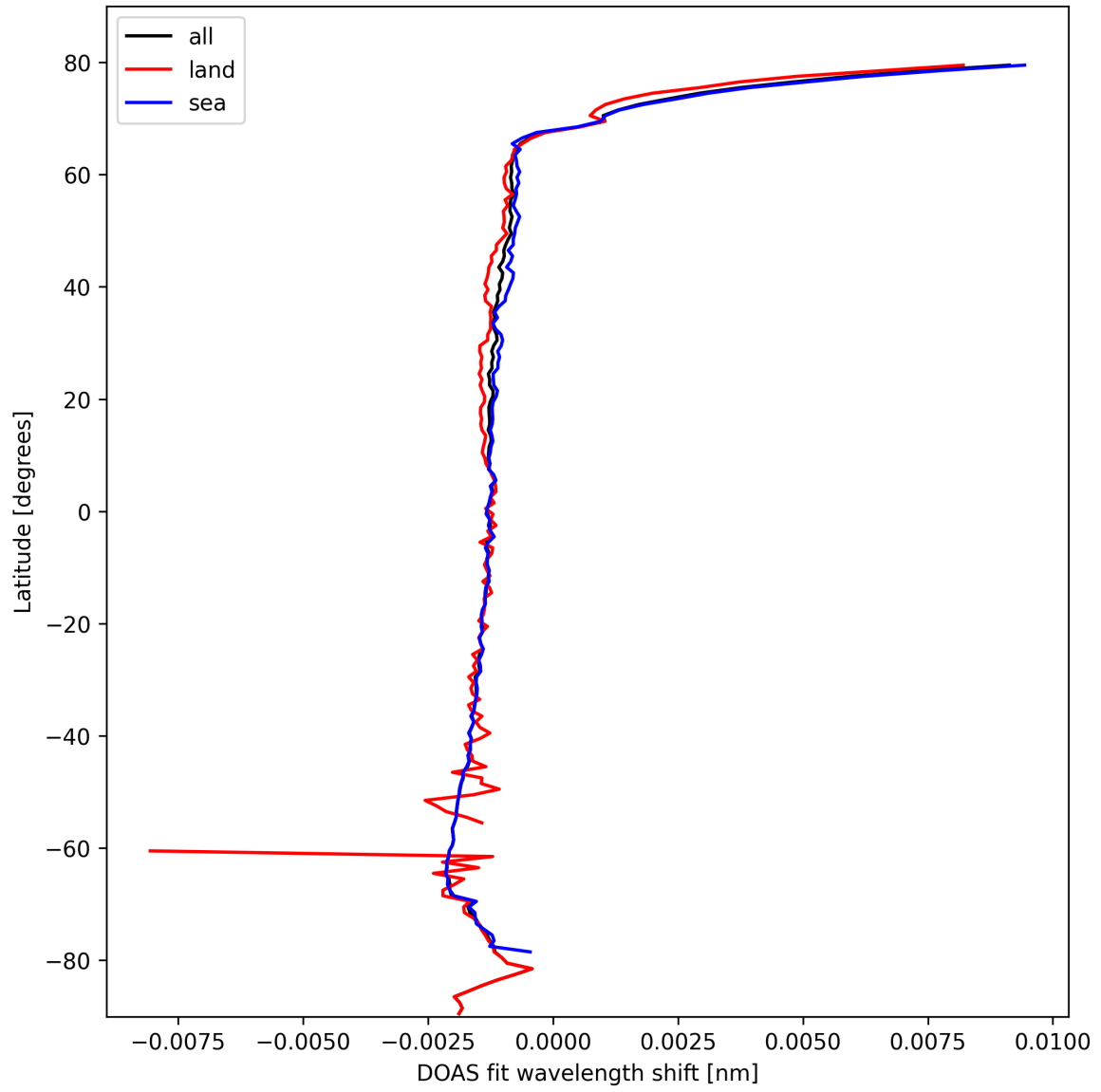
Figure 23: Zonal average of “DOAS fit wavelength shift” for 2025-02-23 to 2025-02-24.
