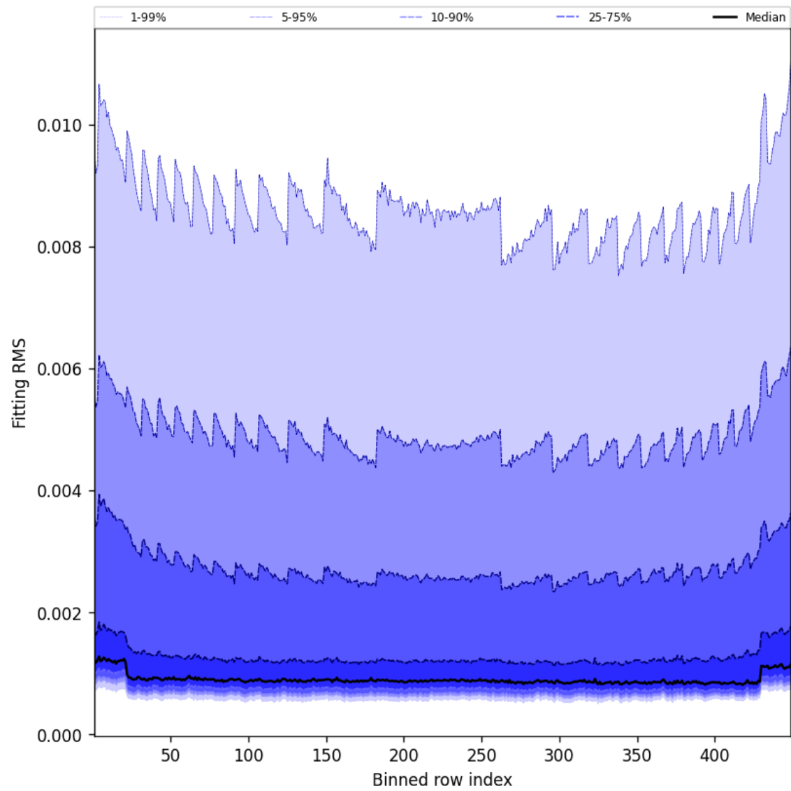
Figure 46: Along track statistics of “Fitting RMS” for 2025-02-23 to 2025-02-24
