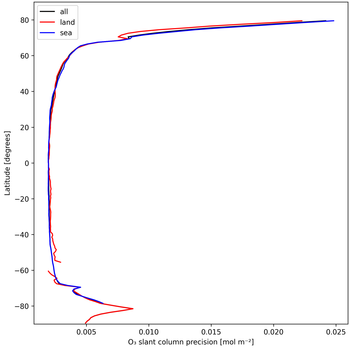
Figure 20: Zonal average of "O 3 slant column precision" for 2025-02-23 to 2025-02-24.
