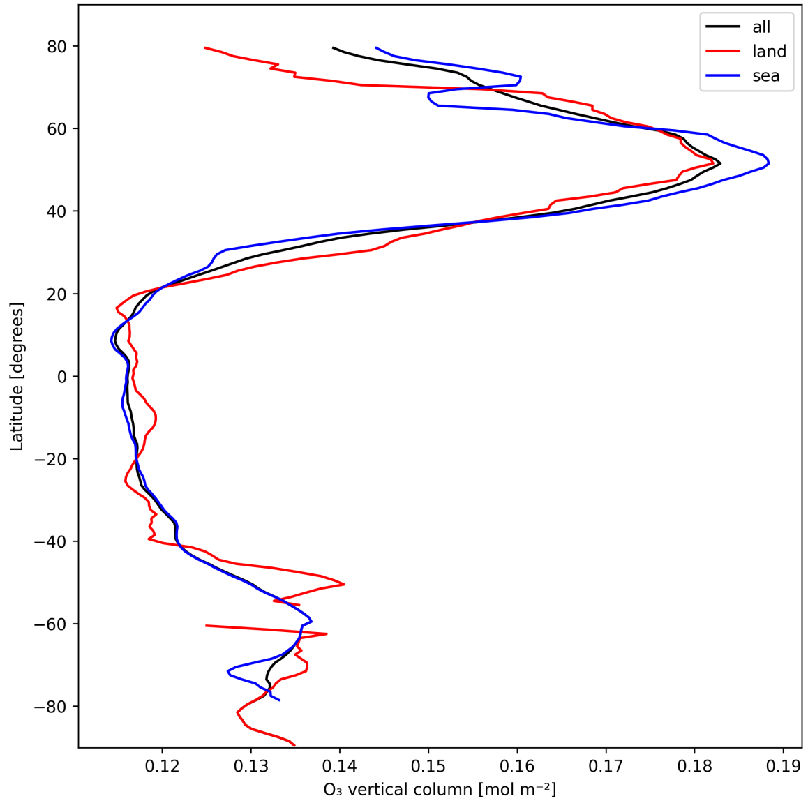
Figure 17: Zonal average of “O 3 vertical column” for 2025-02-23 to 2025-02-24.
