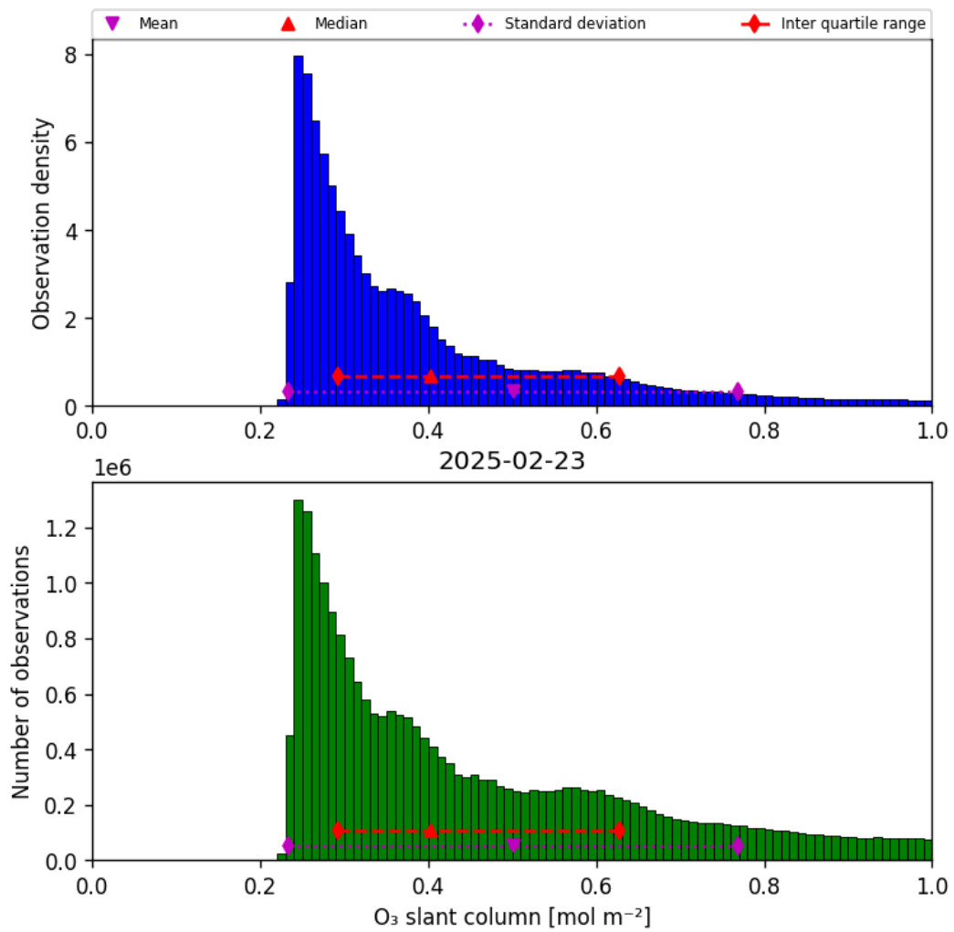
Figure 31: Histogram of “O 3 slant column” for 2025-02-23 to 2025-02-24
