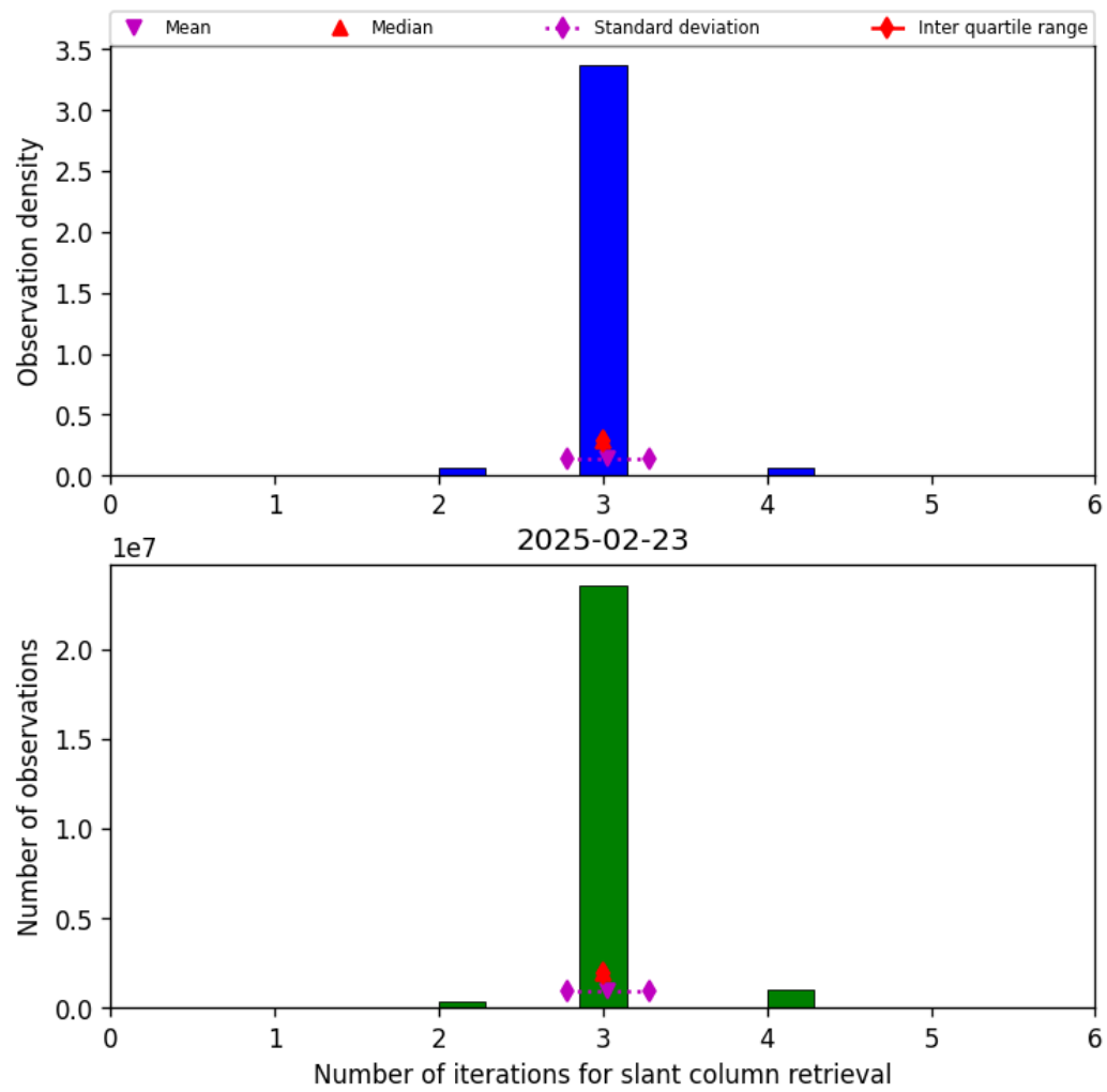
Figure 33: Histogram of “Number of iterations for slant column retrieval” for 2025-02-23 to 2025-02-24
