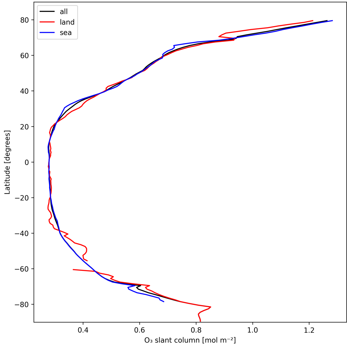
Figure 19: Zonal average of “O 3 slant column” for 2025-02-23 to 2025-02-24.
