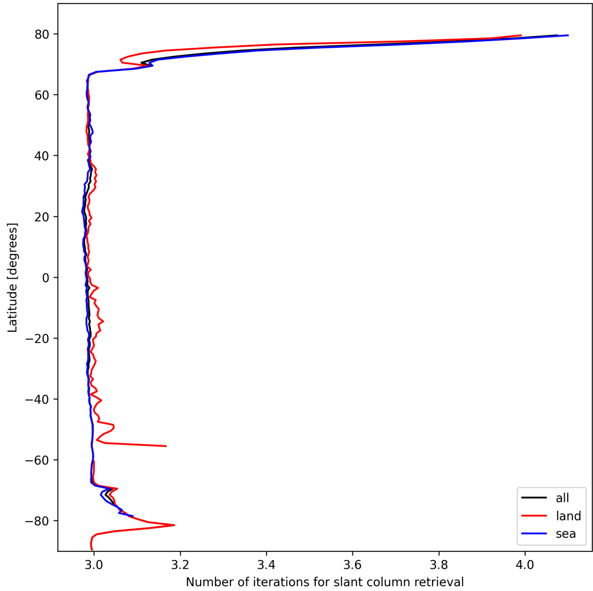
Figure 21: Zonal average of “Number of iterations for slant column retrieval” for 2025-02-23 to 2025-02-24.
