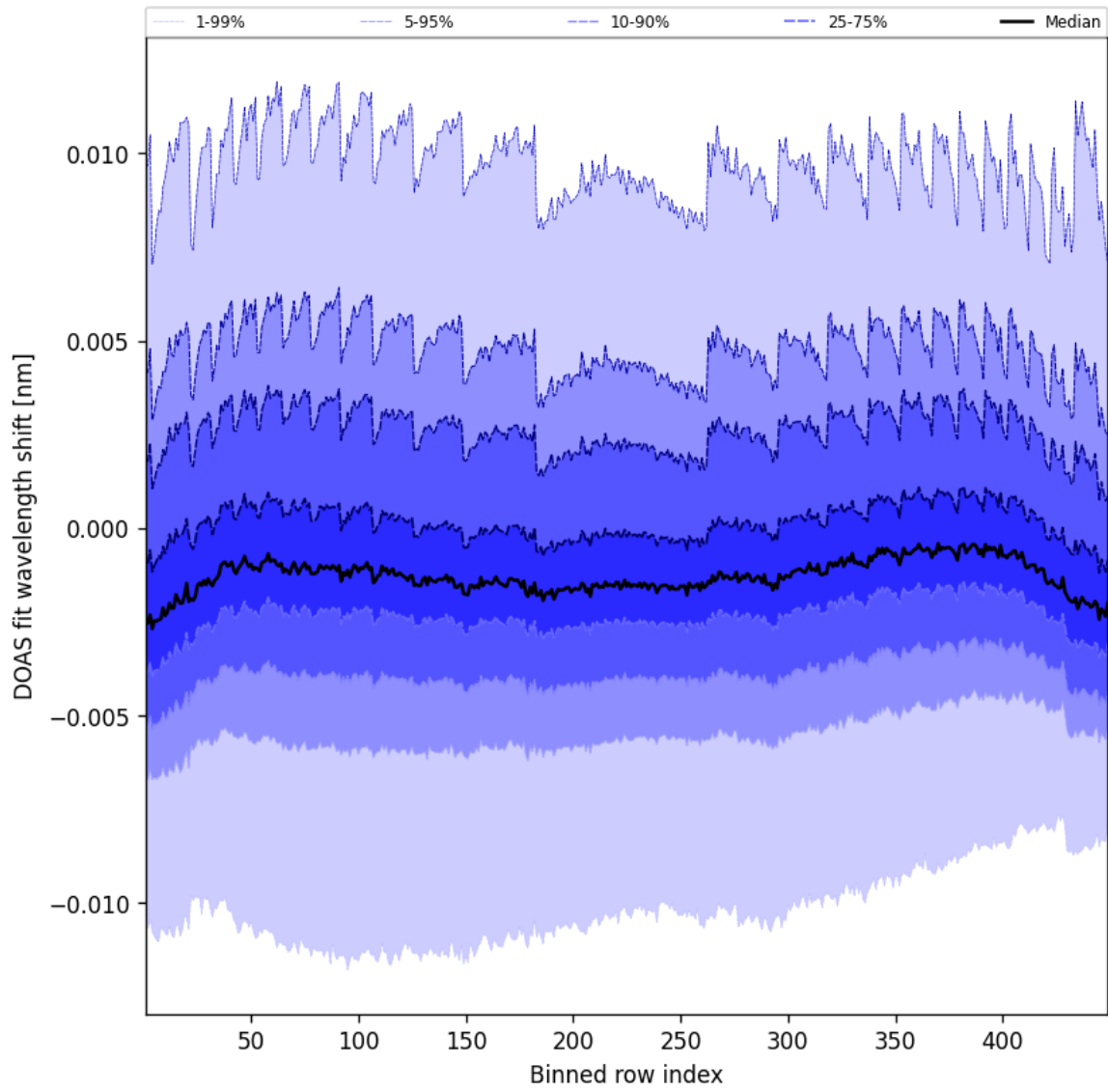
Figure 47: Along track statistics of “DOAS fit wavelength shift” for 2025-02-23 to 2025-02-24
