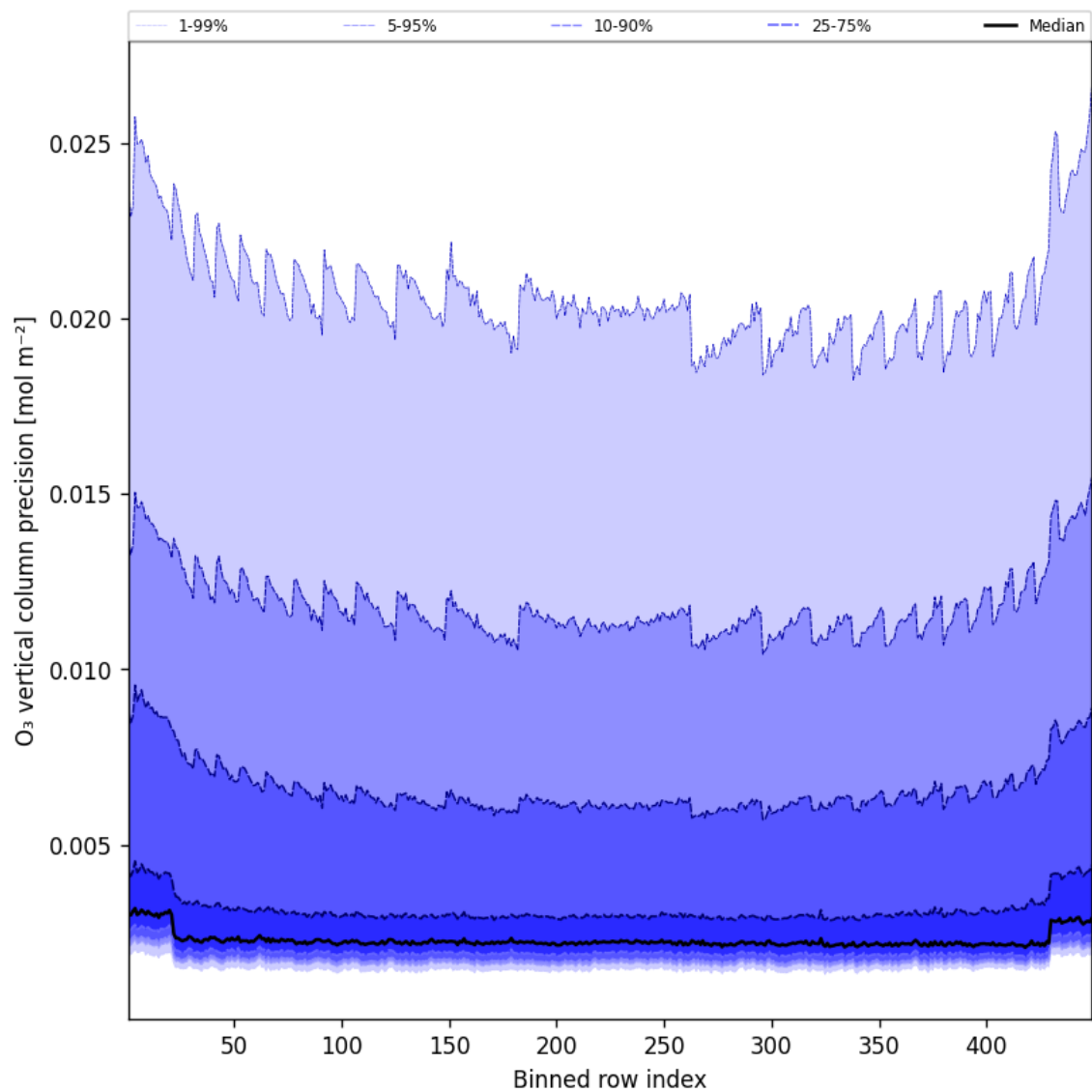
Figure 42: Along track statistics of “O 3 vertical column precision” for 2025-02-23 to 2025-02-24
