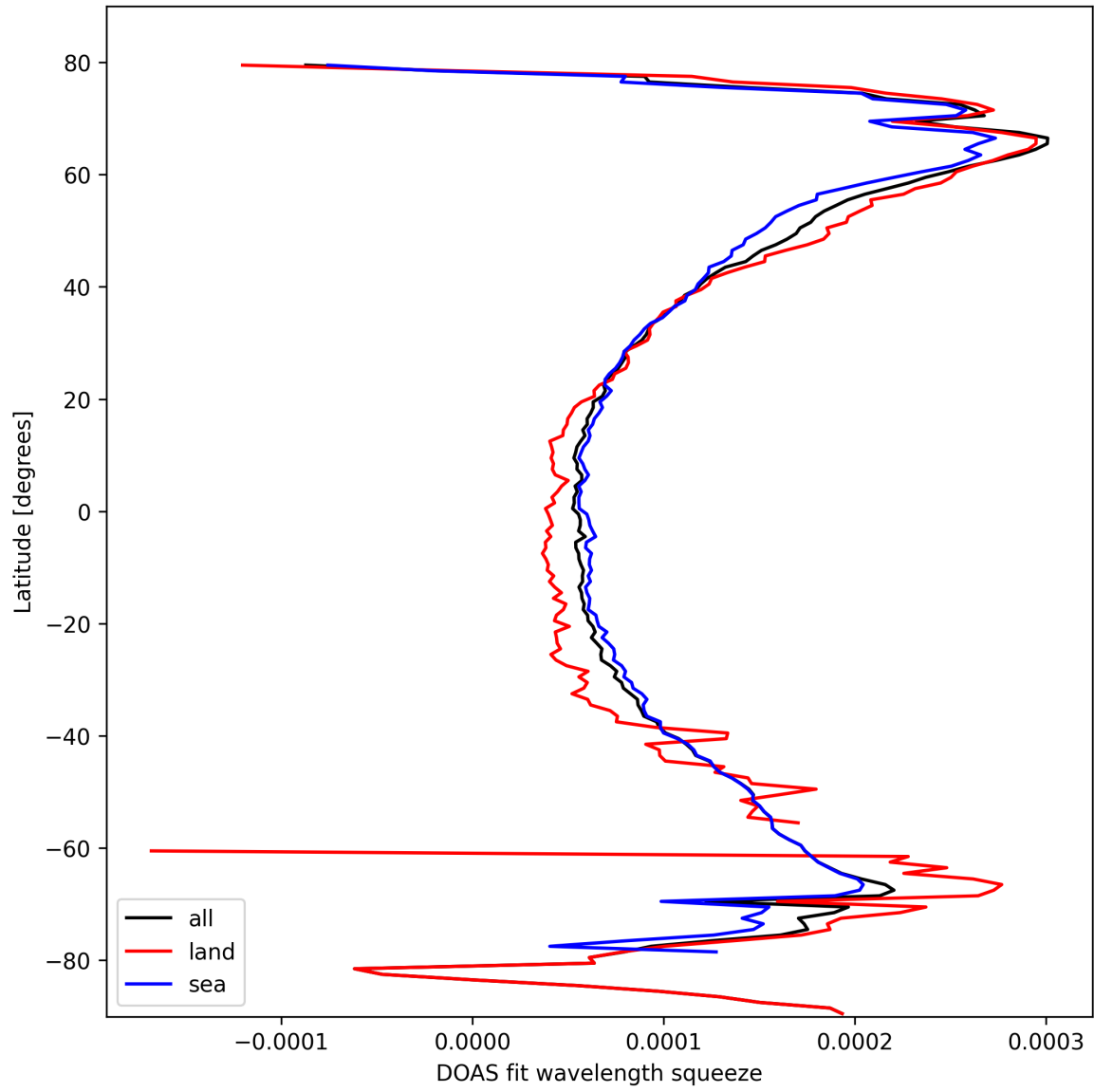
Figure 24: Zonal average of “DOAS fit wavelength squeeze” for 2025-02-23 to 2025-02-24.
