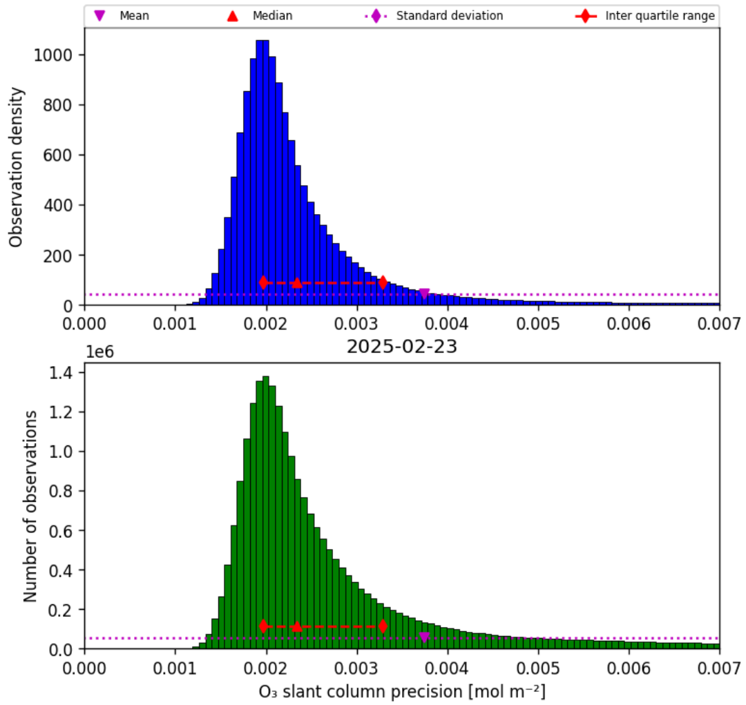
Figure 32: Histogram of “O 3 slant column precision” for 2025-02-23 to 2025-02-24
