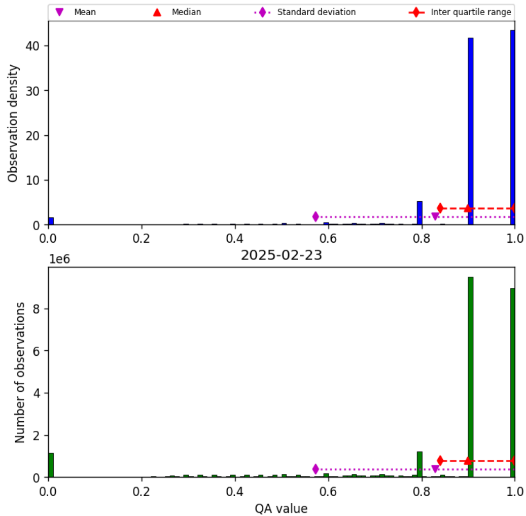
Figure 28: Histogram of “QA value” for 2025-02-23 to 2025-02-24
