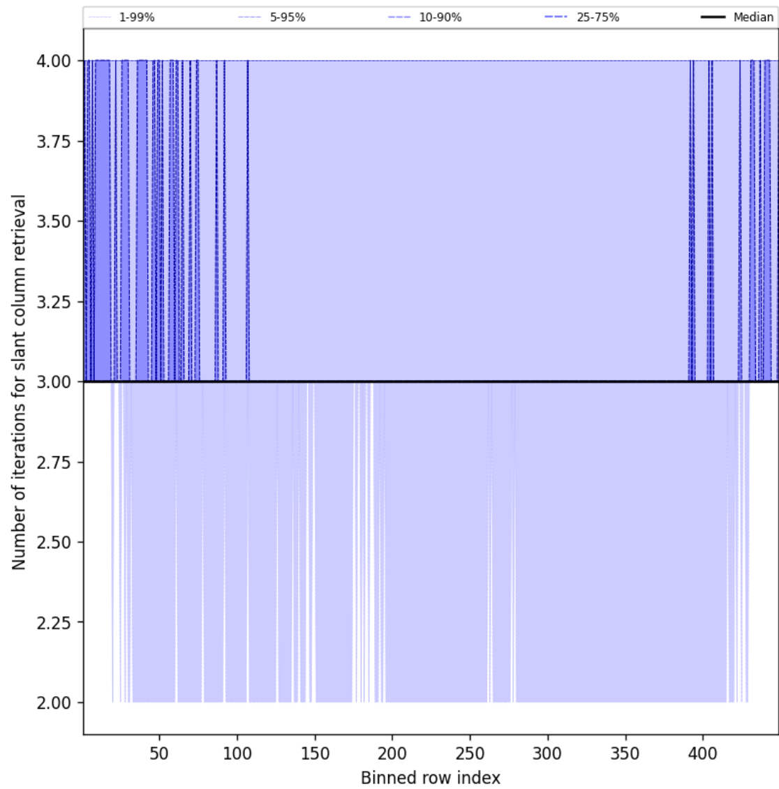
Figure 45: Along track statistics of “Number of iterations for slant column retrieval” for 2025-02-23 to 2025-02-24
