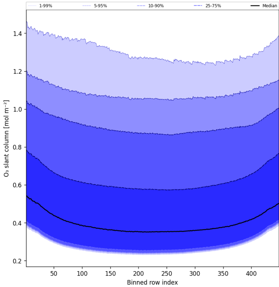
Figure 43: Along track statistics of “O 3 slant column” for 2025-02-23 to 2025-02-24
