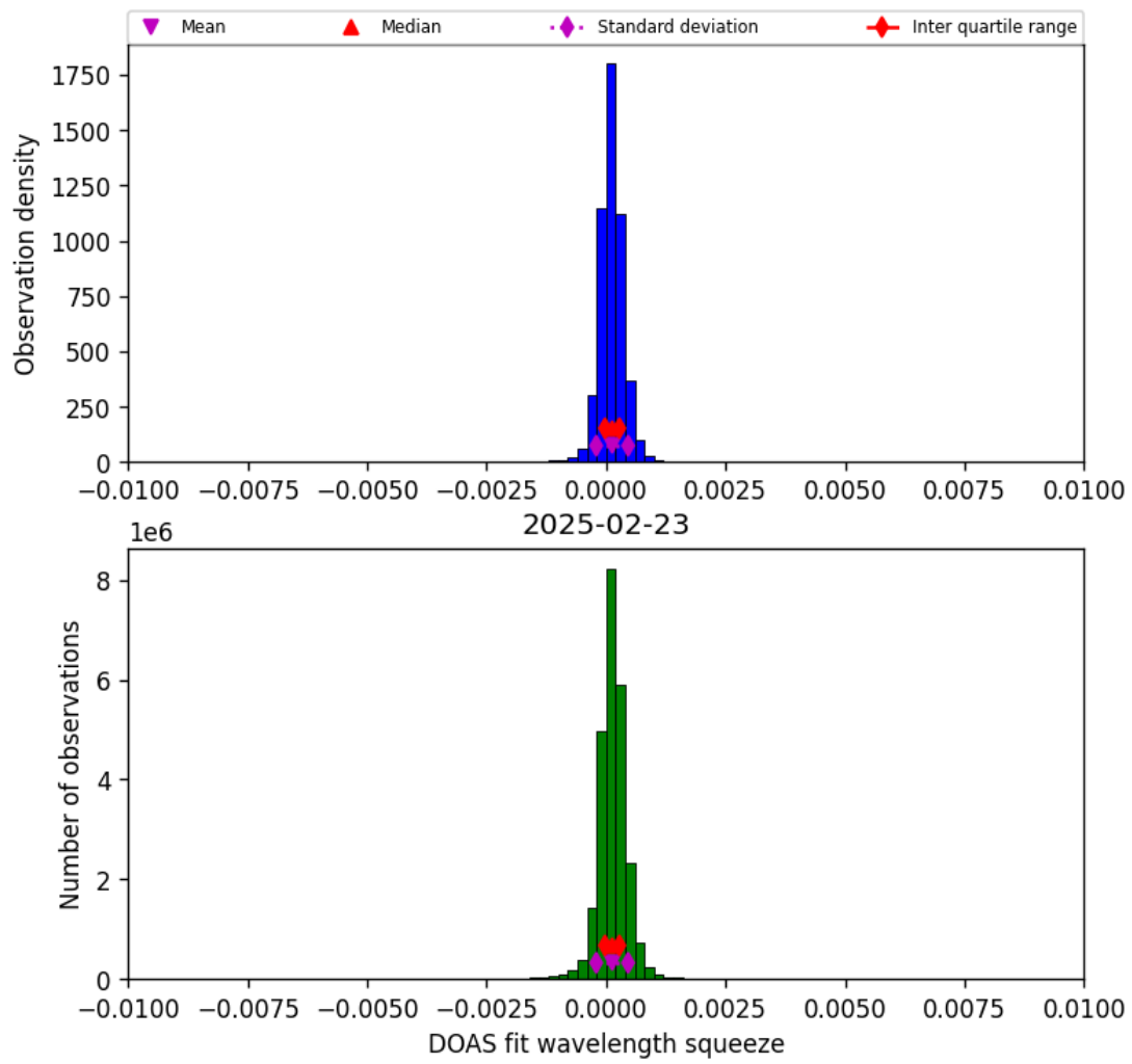
Figure 36: Histogram of “DOAS fit wavelength squeeze” for 2025-02-23 to 2025-02-24
