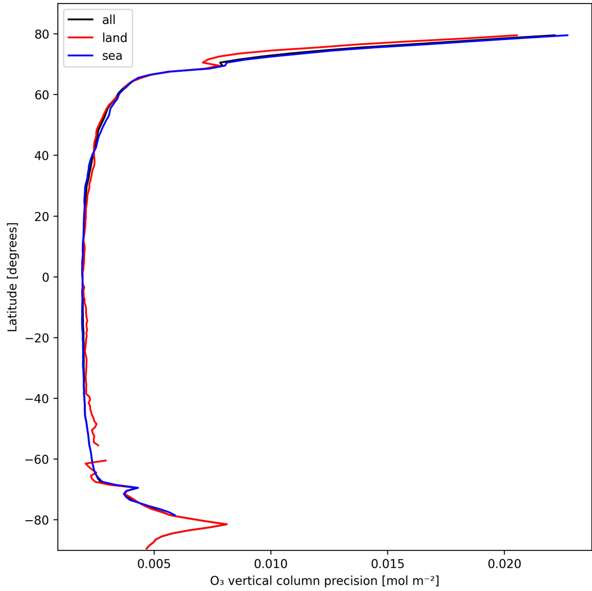
Figure 18: Zonal average of “O 3 vertical column precision” for 2025-02-23 to 2025-02-24.
