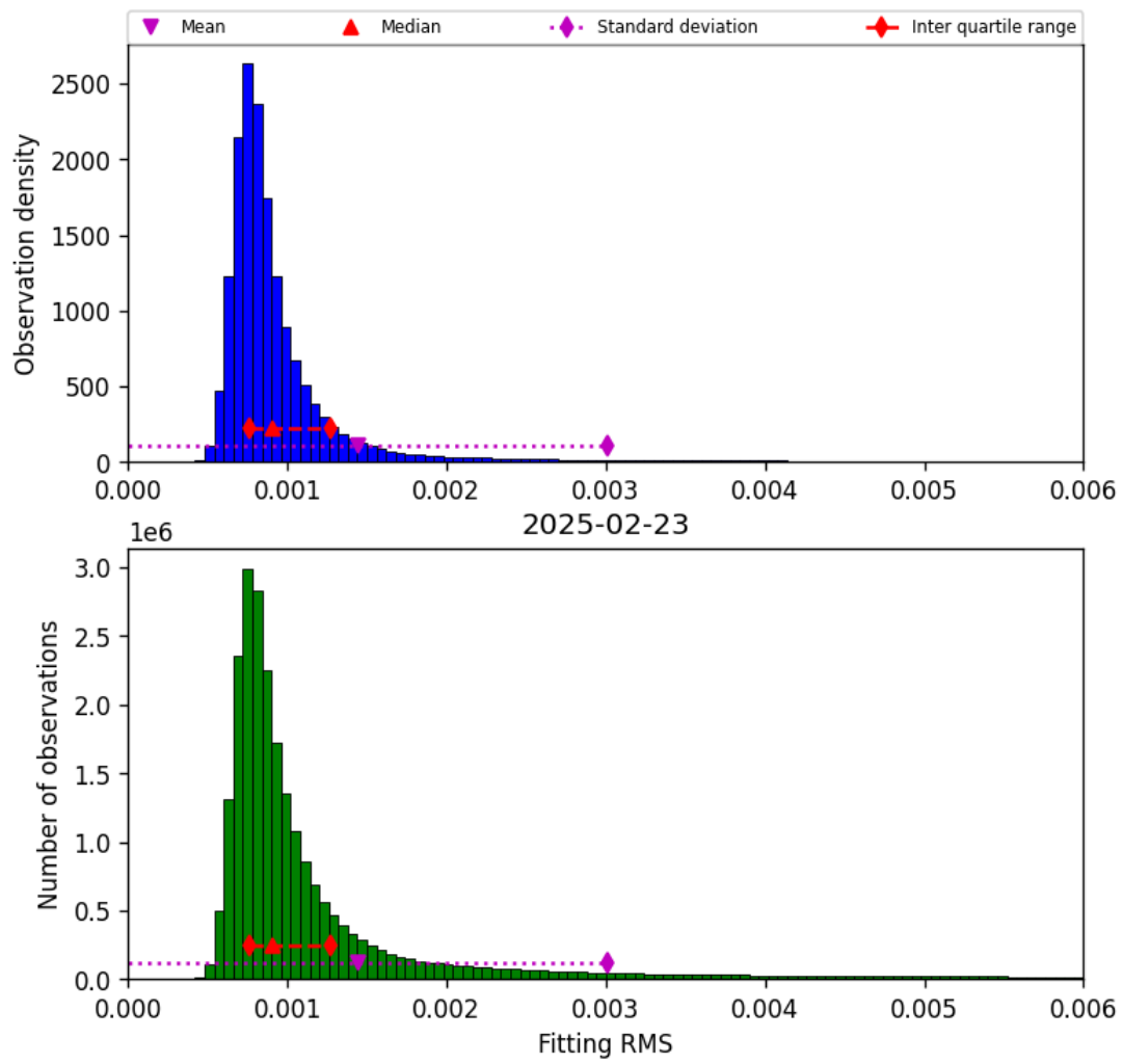
Figure 34: Histogram of “Fitting RMS” for 2025-02-23 to 2025-02-24
