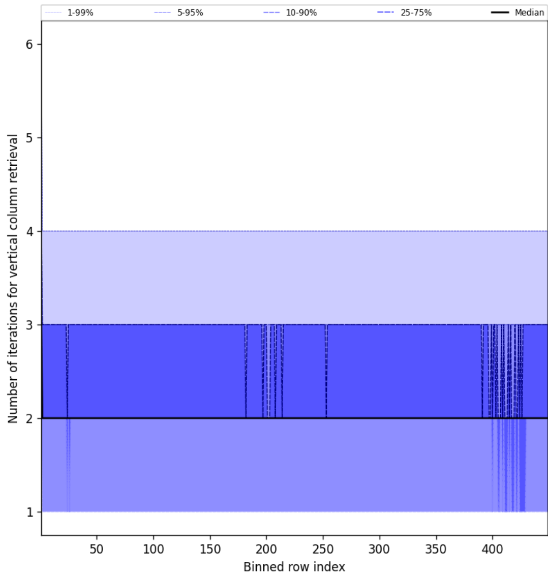
Figure 51: Along track statistics of “Number of iterations for vertical column retrieval” for 2025-02-23 to 2025-02-24
