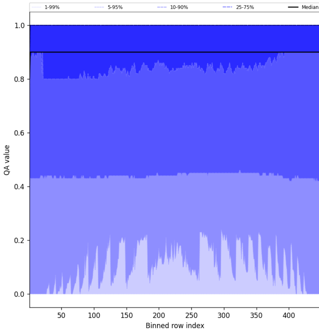
Figure 40: Along track statistics of “QA value” for 2025-02-23 to 2025-02-24
