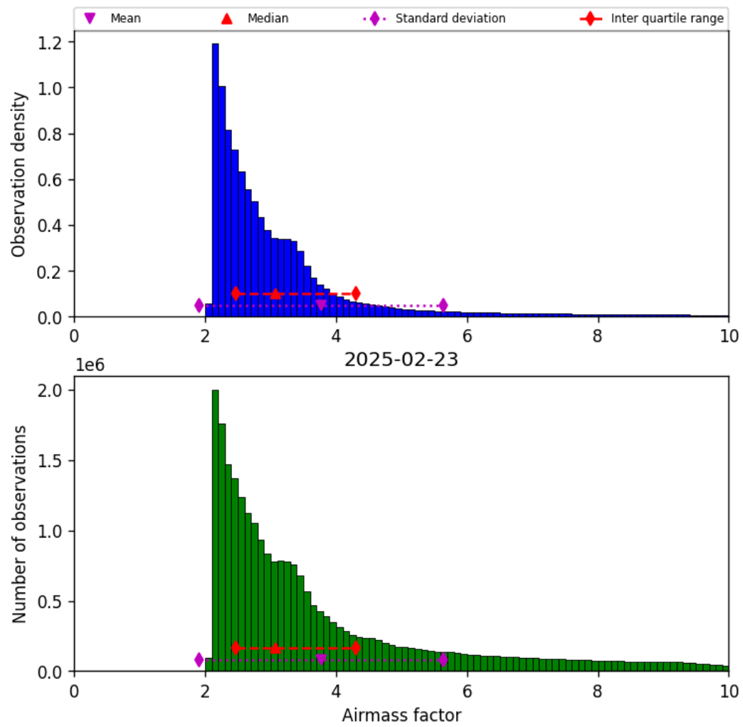
Figure 37: Histogram of “Airmass factor” for 2025-02-23 to 2025-02-24
