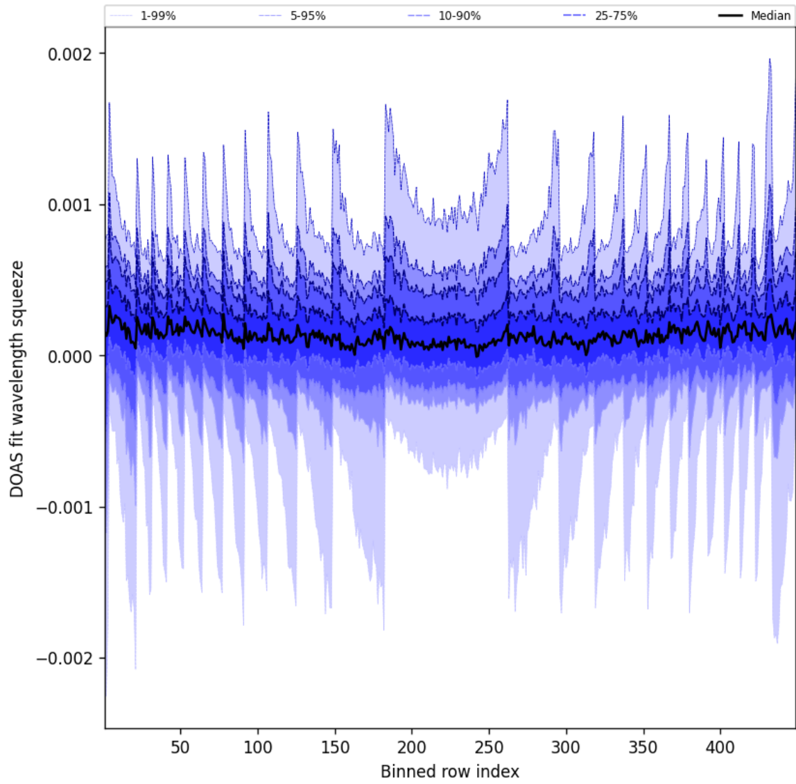
Figure 48: Along track statistics of “DOAS fit wavelength squeeze” for 2025-02-23 to 2025-02-24
