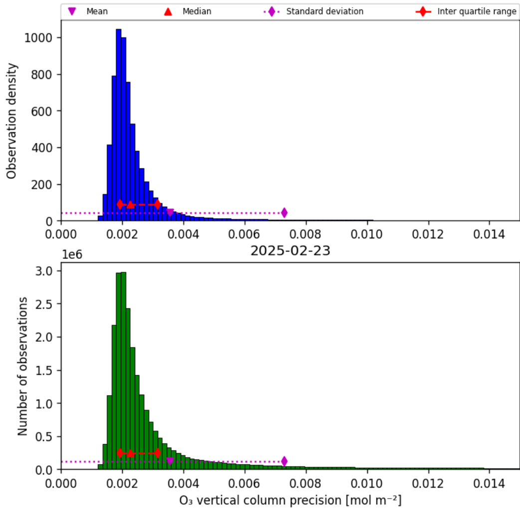
Figure 30: Histogram of “O 3 vertical column precision” for 2025-02-23 to 2025-02-24
