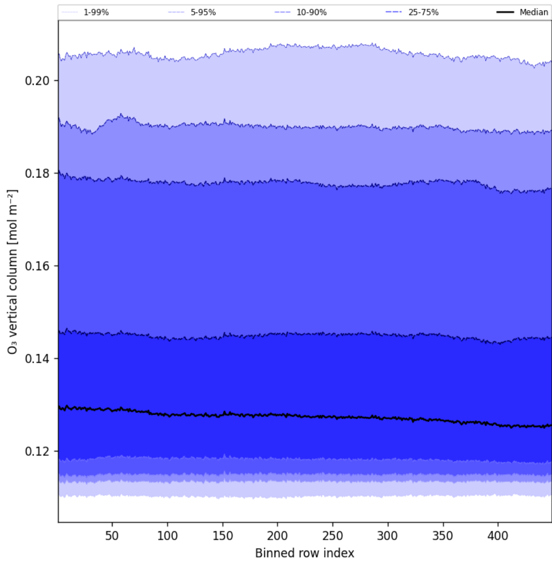
Figure 41: Along track statistics of “O 3 vertical column” for 2025-02-23 to 2025-02-24
