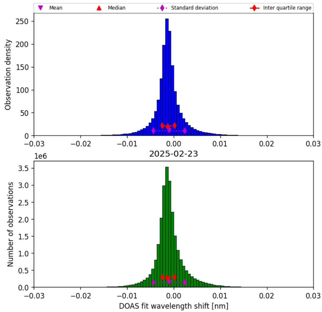
Figure 35: Histogram of “DOAS fit wavelength shift” for 2025-02-23 to 2025-02-24
