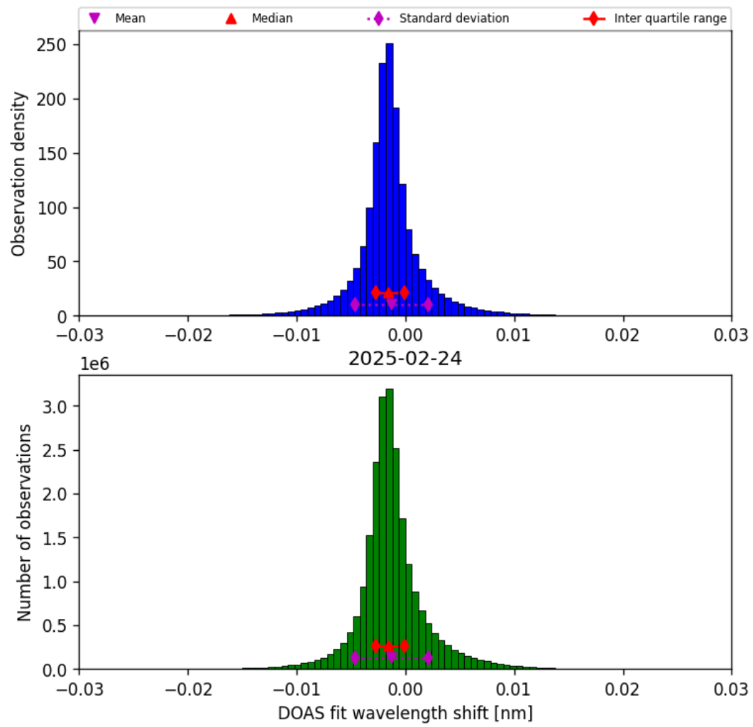
Figure 35: Histogram of “DOAS fit wavelength shift” for 2025-02-24 to 2025-02-25
