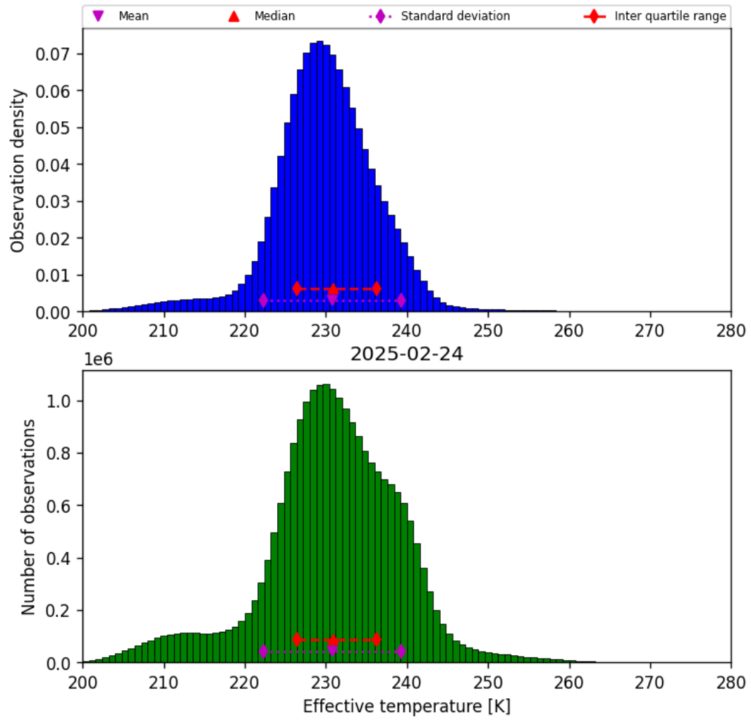
Figure 38: Histogram of “Effective temperature” for 2025-02-24 to 2025-02-25
