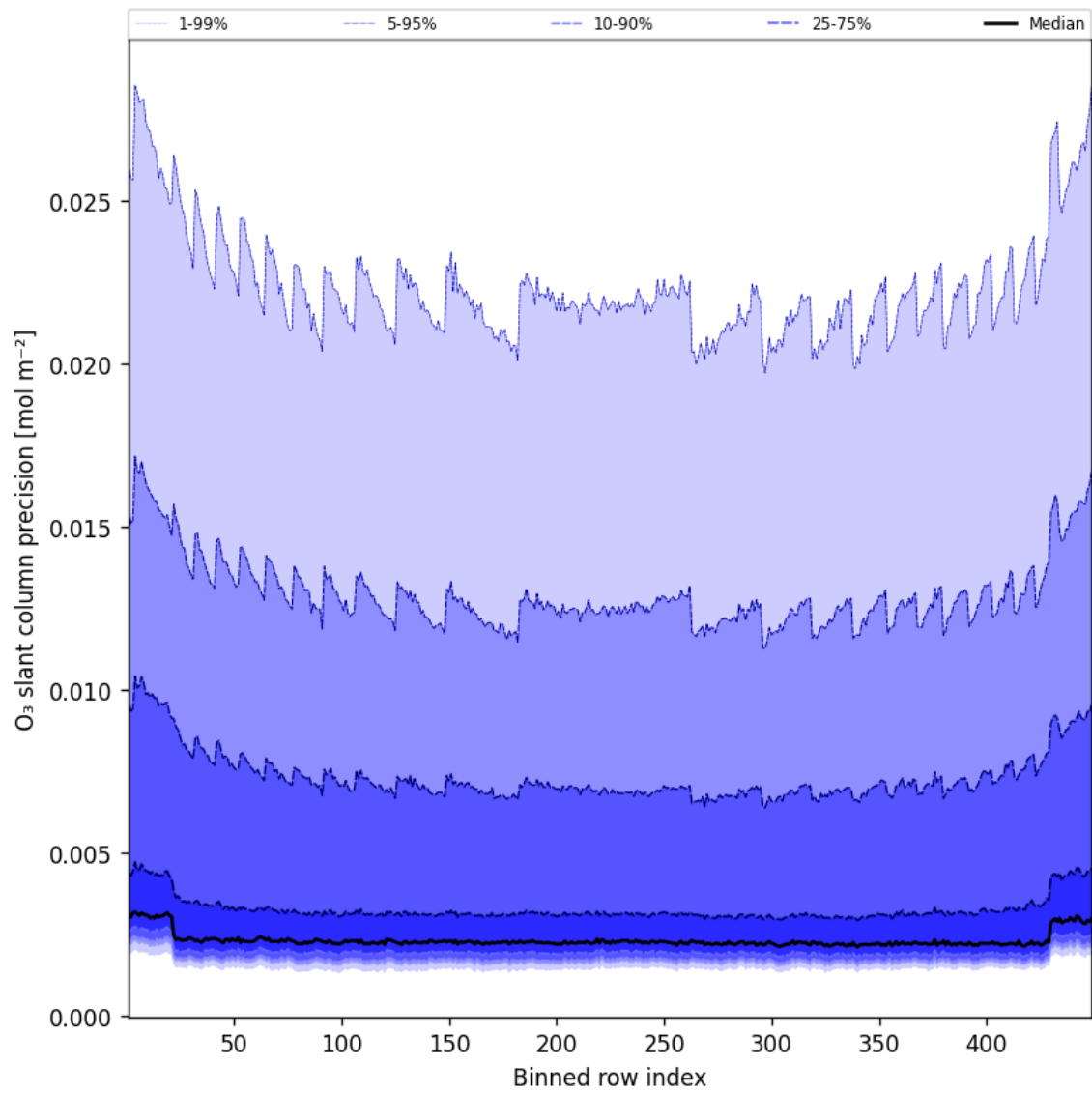
Figure 44: Along track statistics of “O 3 slant column precision” for 2025-02-24 to 2025-02-25
