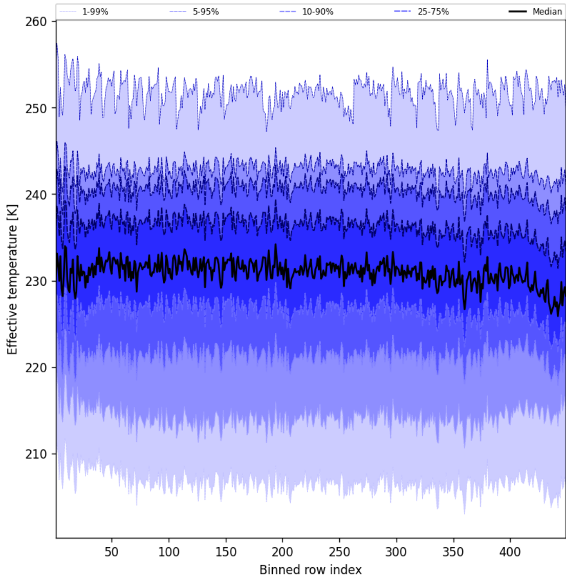
Figure 50: Along track statistics of “Effective temperature” for 2025-02-24 to 2025-02-25
