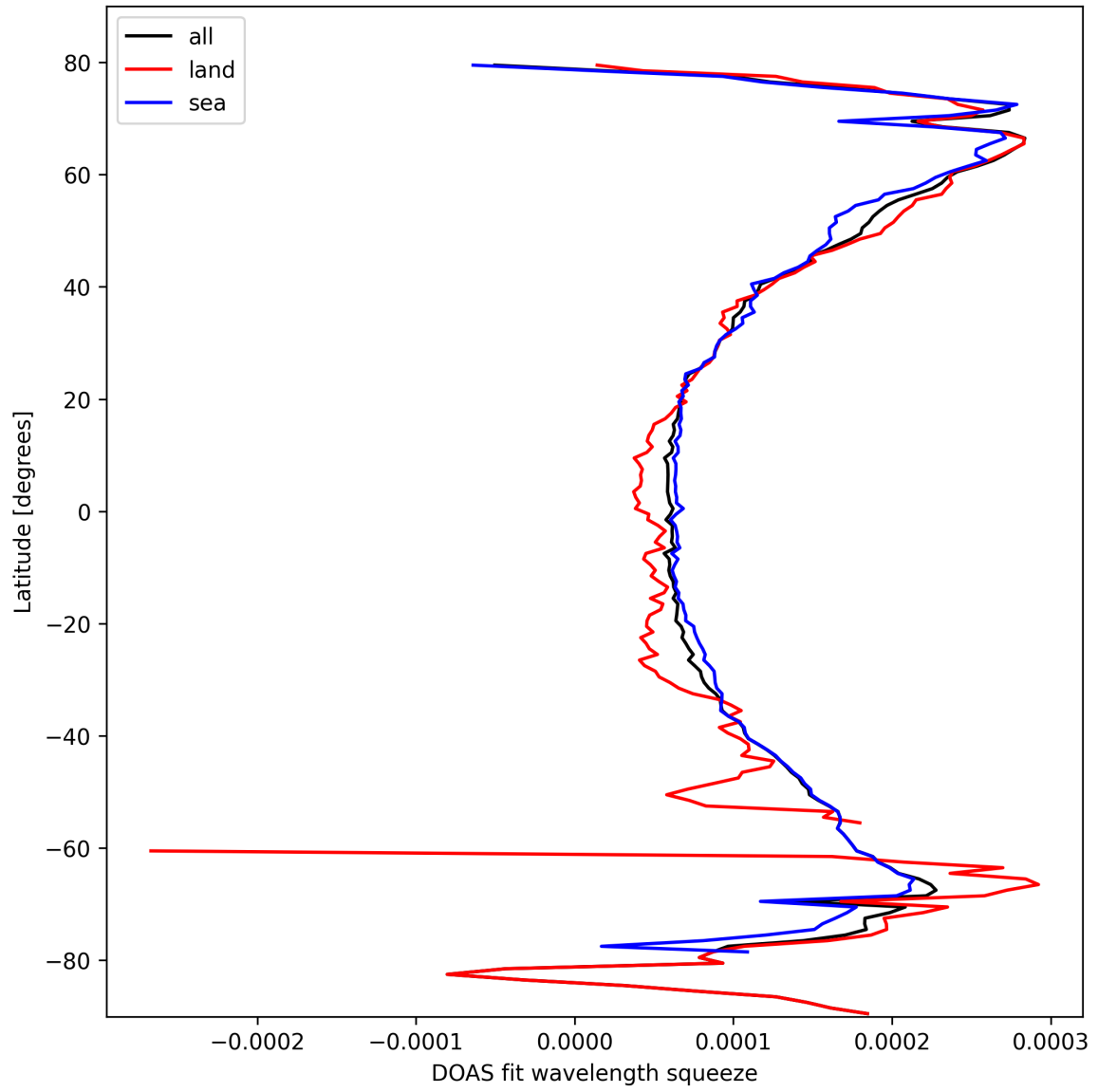
Figure 24: Zonal average of "DOAS fit wavelength squeeze" for 2025-02-24 to 2025-02-25.
