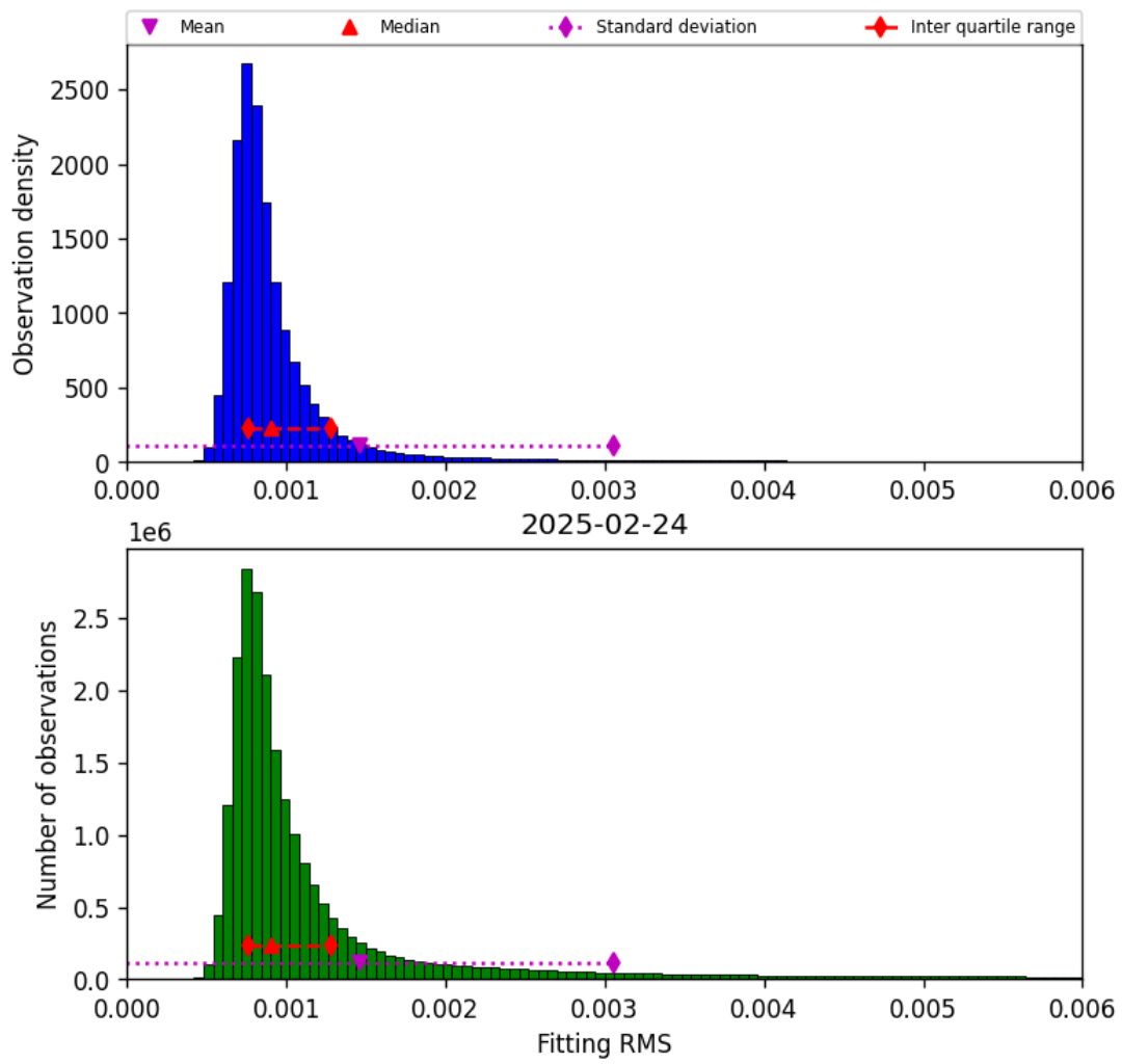
Figure 34: Histogram of “Fitting RMS” for 2025-02-24 to 2025-02-25
