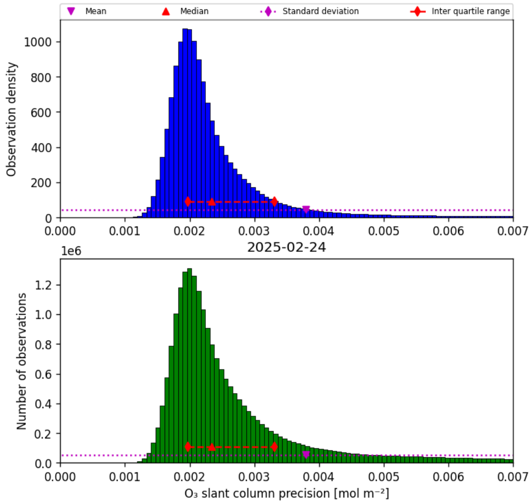
Figure 32: Histogram of “O 3 slant column precision” for 2025-02-24 to 2025-02-25
