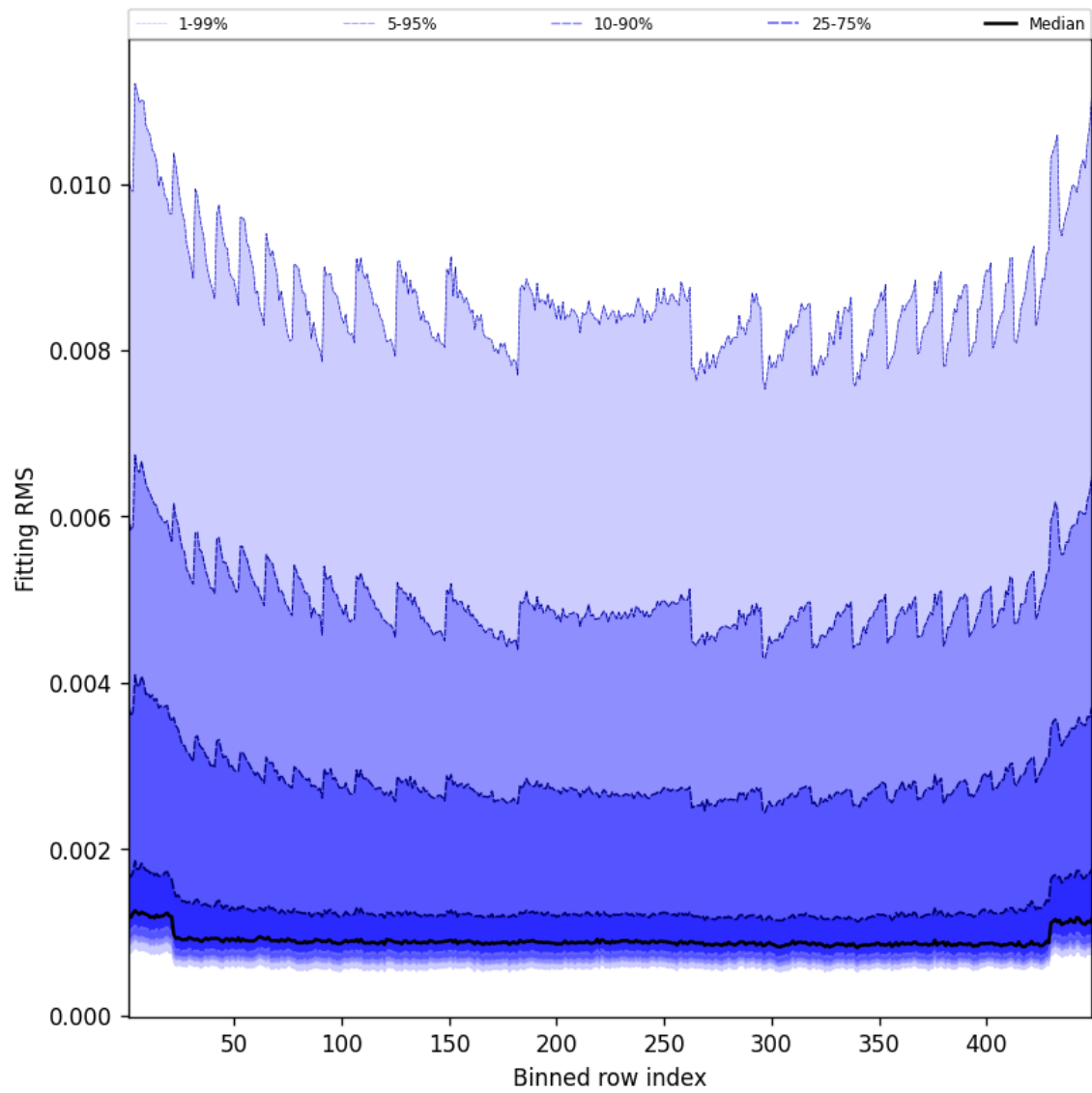
Figure 46: Along track statistics of “Fitting RMS” for 2025-02-24 to 2025-02-25
