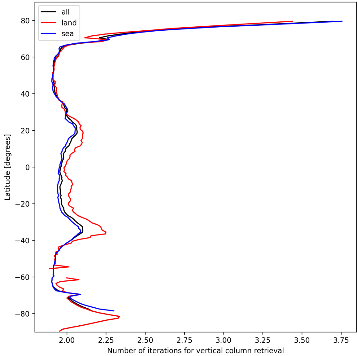
Figure 27: Zonal average of “Number of iterations for vertical column retrieval” for 2025-02-24 to 2025-02-25.
