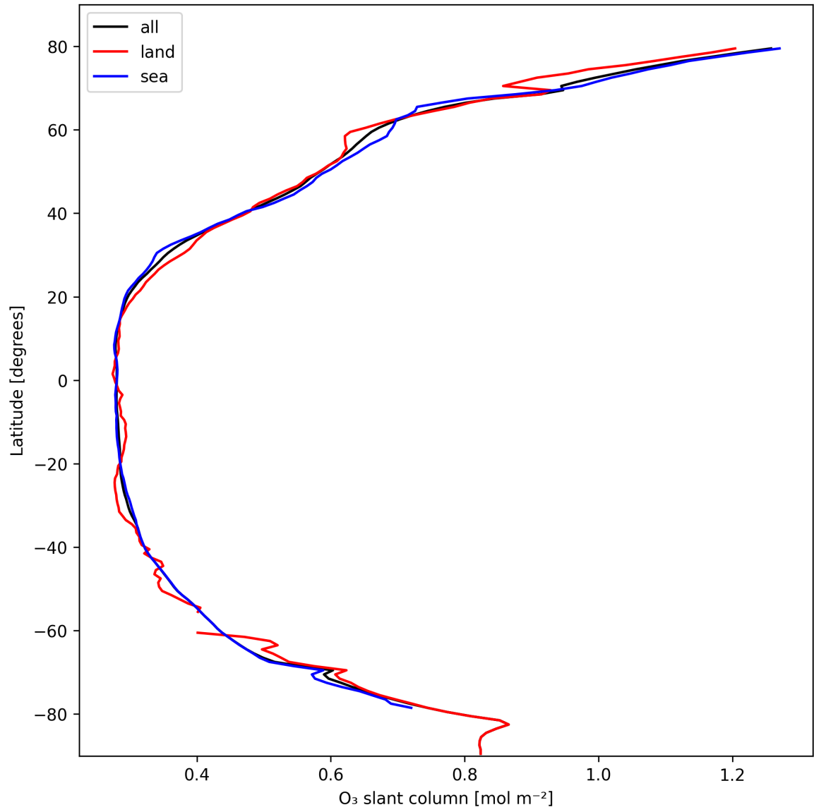
Figure 19: Zonal average of “O 3 slant column” for 2025-02-24 to 2025-02-25.
