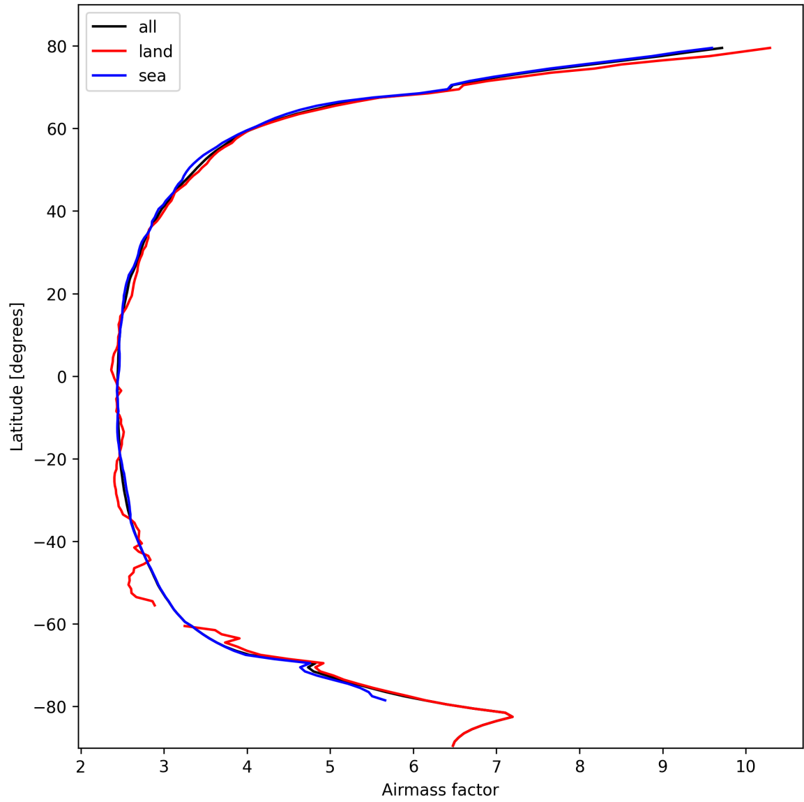
Figure 25: Zonal average of “Airmass factor” for 2025-02-24 to 2025-02-25.
