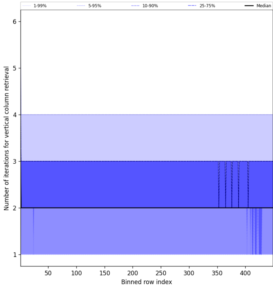
Figure 51: Along track statistics of “Number of iterations for vertical column retrieval” for 2025-02-24 to 2025-02-25
