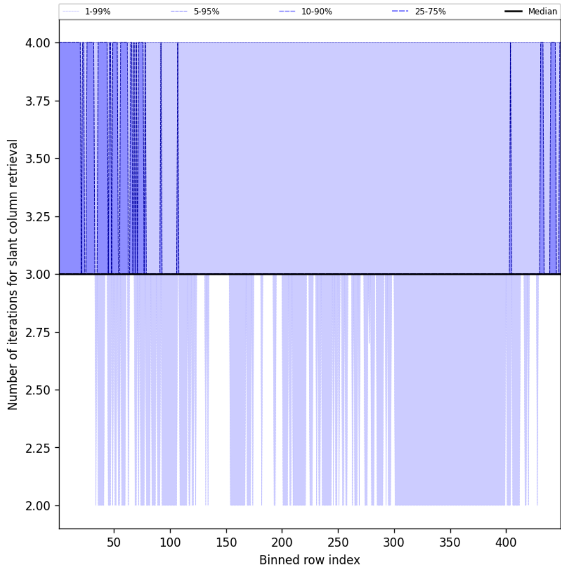
Figure 45: Along track statistics of “Number of iterations for slant column retrieval” for 2025-02-24 to 2025-02-25
