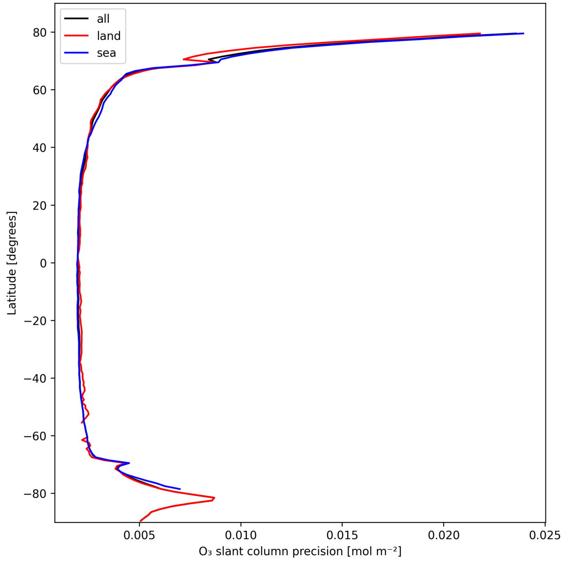
Figure 20: Zonal average of “O 3 slant column precision” for 2025-02-24 to 2025-02-25.
