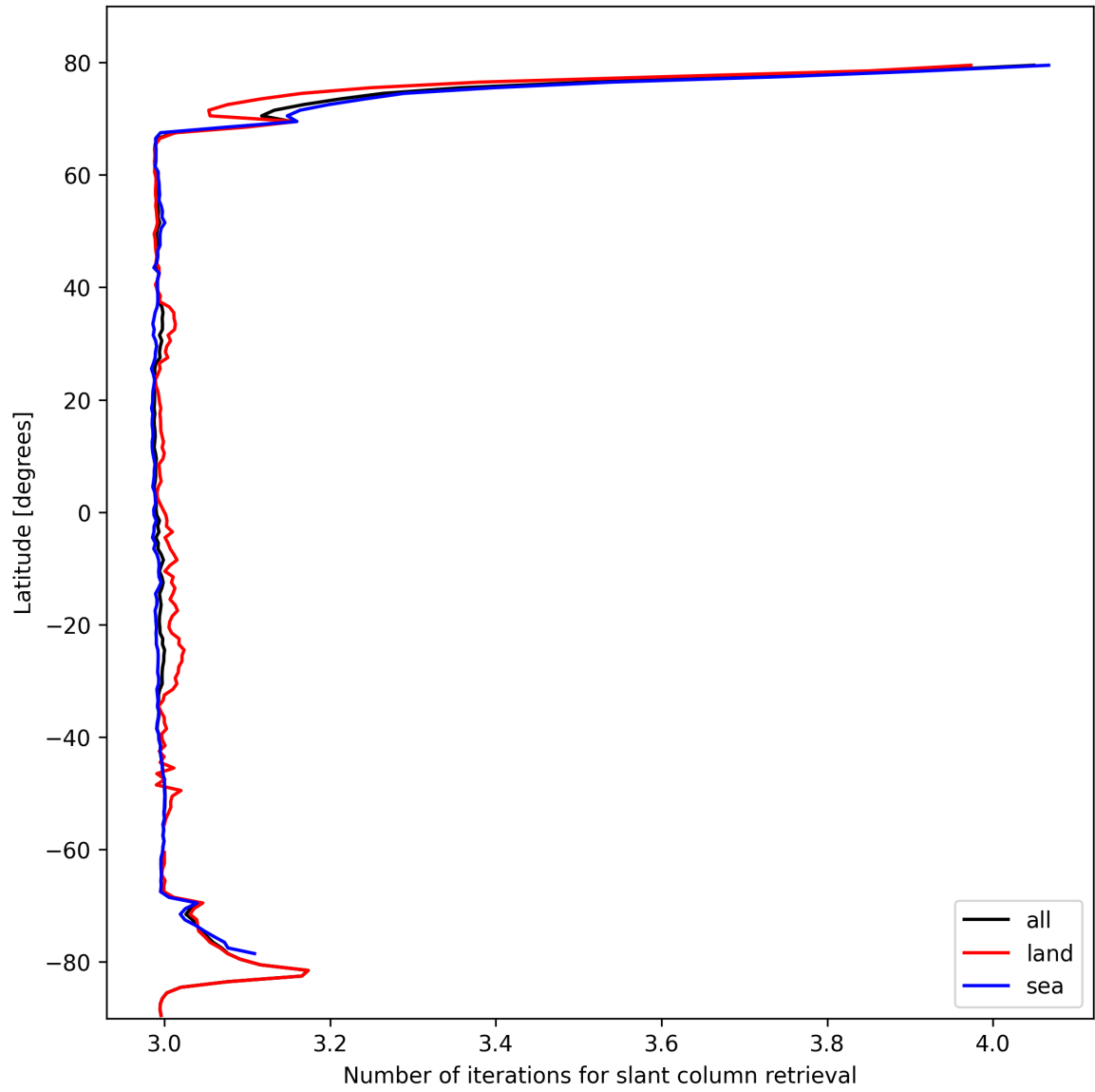
Figure 21: Zonal average of “Number of iterations for slant column retrieval” for 2025-02-24 to 2025-02-25.
