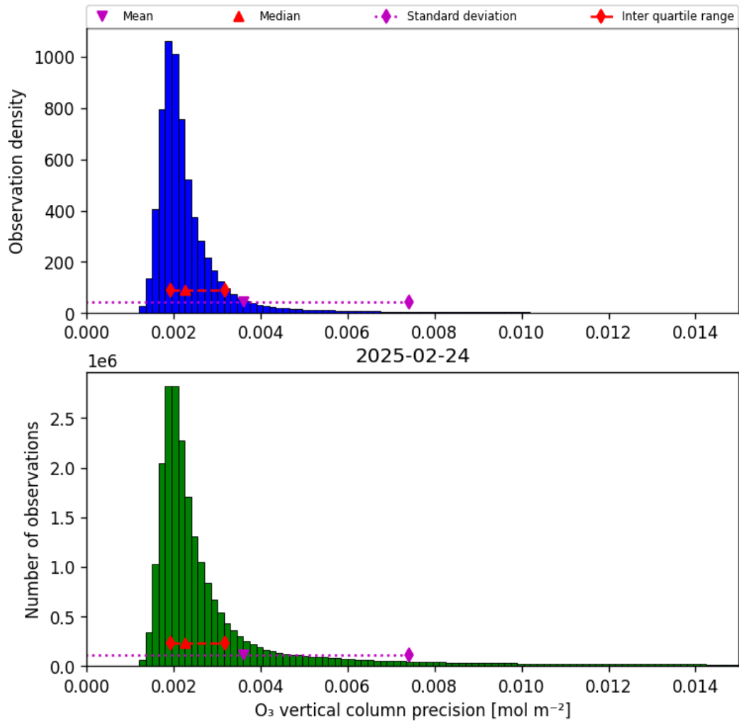
Figure 30: Histogram of “O 3 vertical column precision” for 2025-02-24 to 2025-02-25
