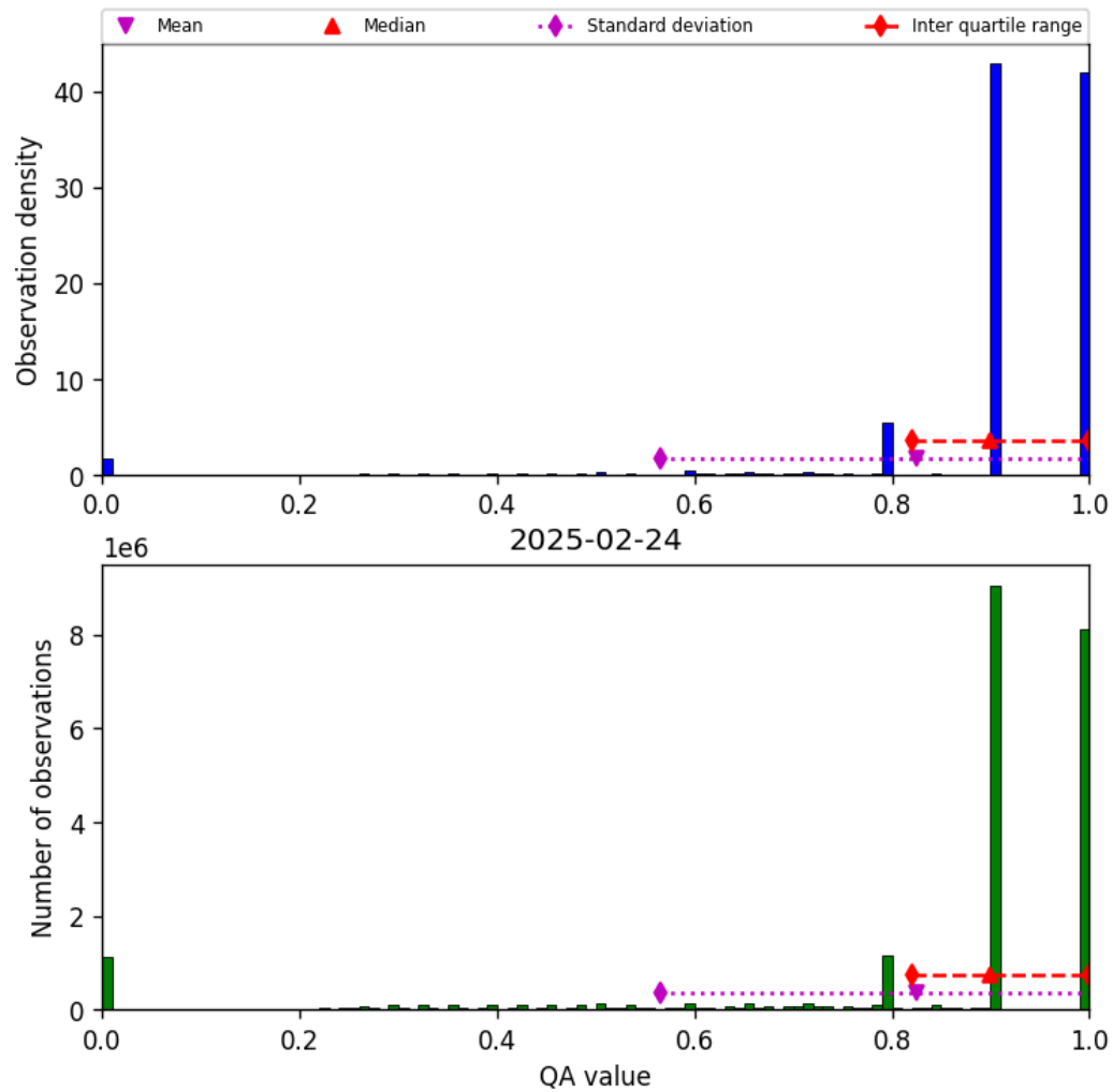
Figure 28: Histogram of “QA value” for 2025-02-24 to 2025-02-25
