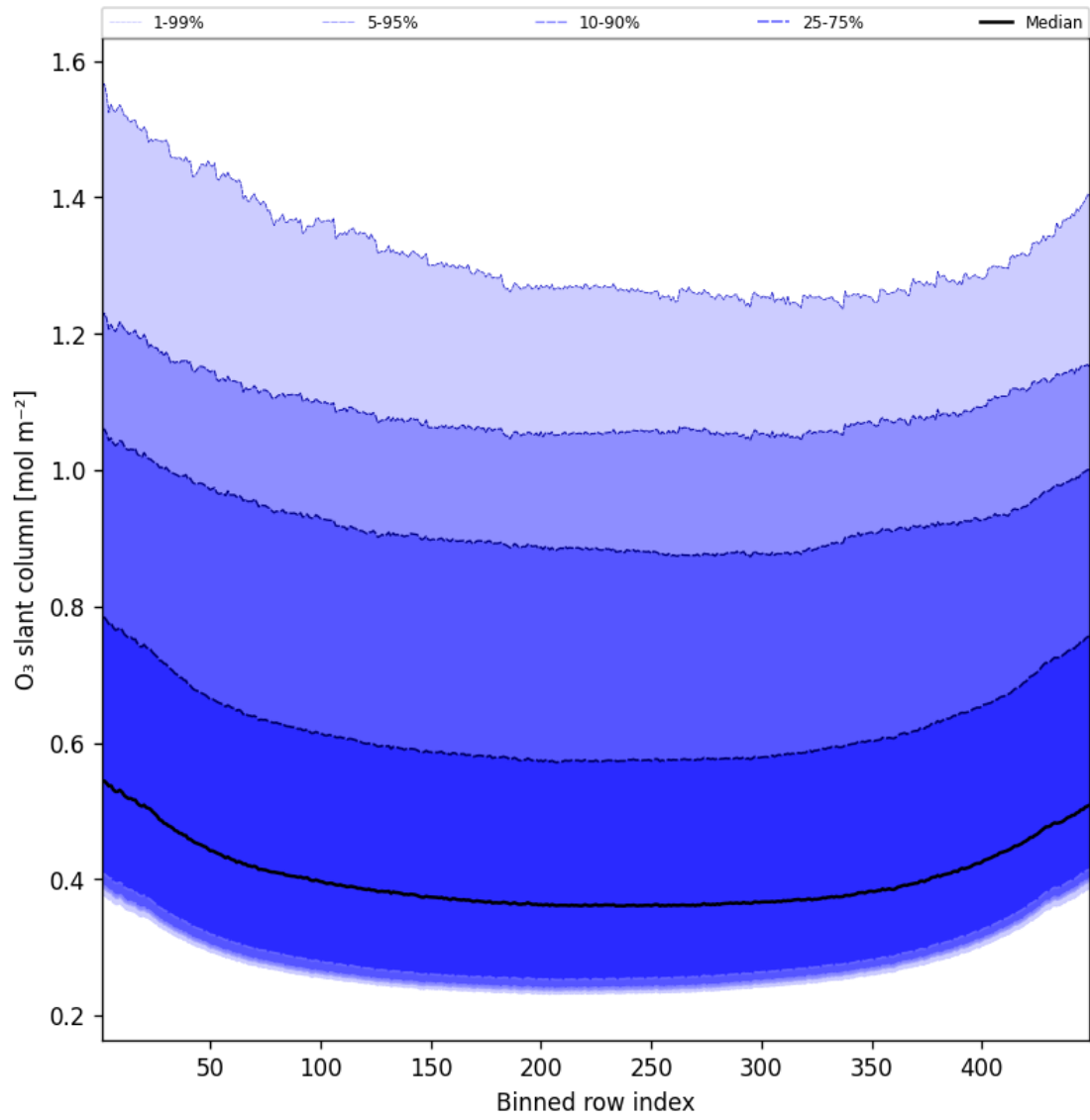
Figure 43: Along track statistics of “O 3 slant column” for 2025-02-24 to 2025-02-25
