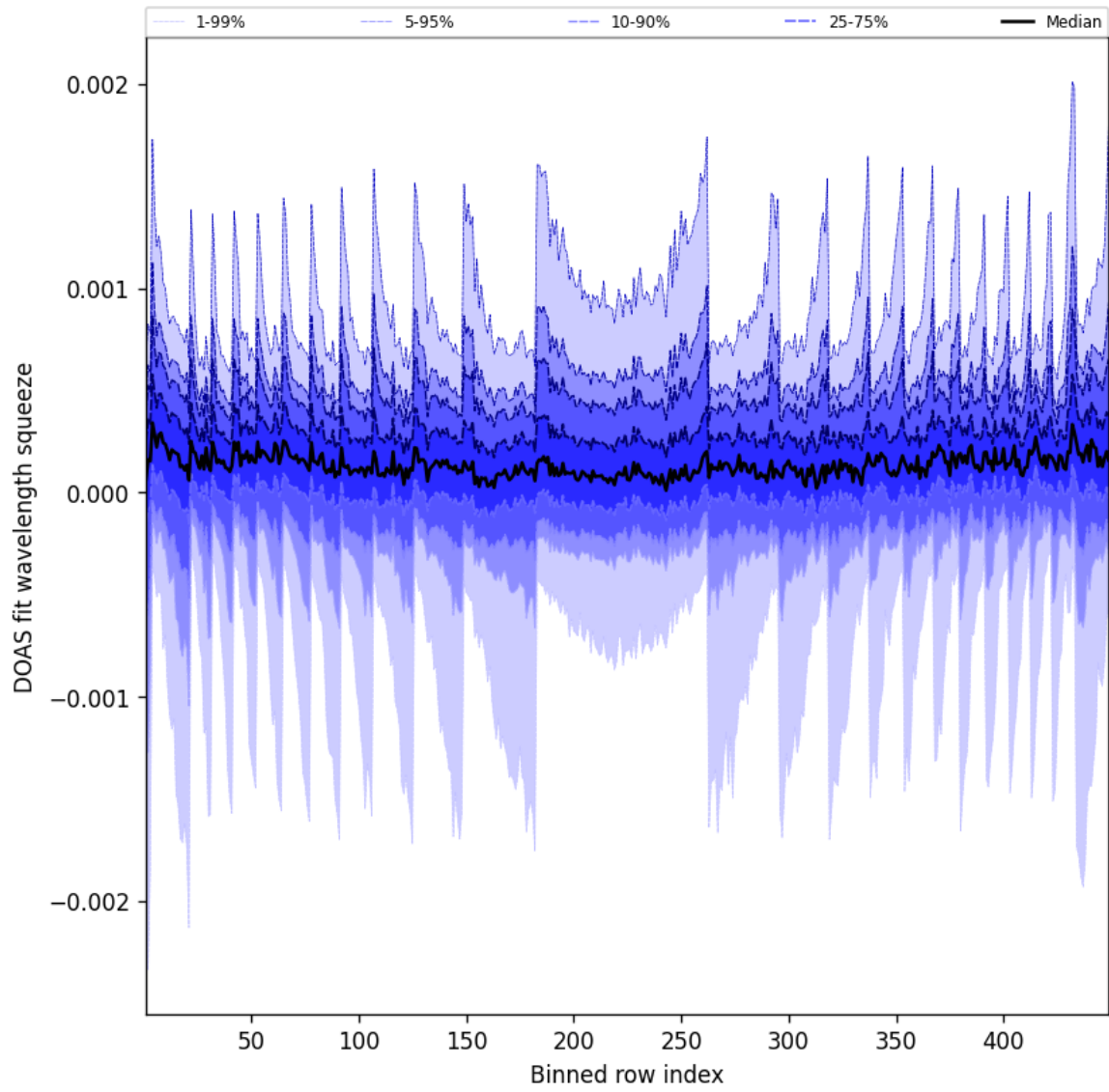
Figure 48: Along track statistics of “DOAS fit wavelength squeeze” for 2025-02-24 to 2025-02-25
