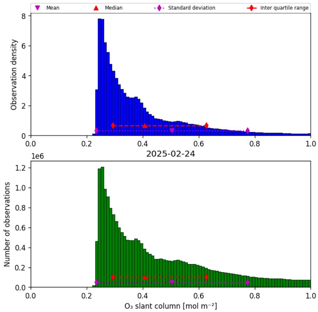
Figure 31: Histogram of “O 3 slant column” for 2025-02-24 to 2025-02-25
