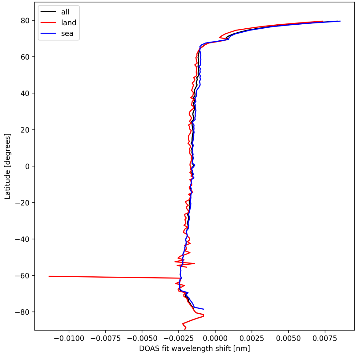
Figure 23: Zonal average of “DOAS fit wavelength shift” for 2025-02-24 to 2025-02-25.
