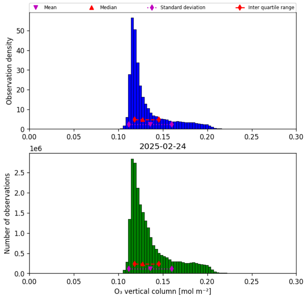
Figure 29: Histogram of “O 3 vertical column” for 2025-02-24 to 2025-02-25
