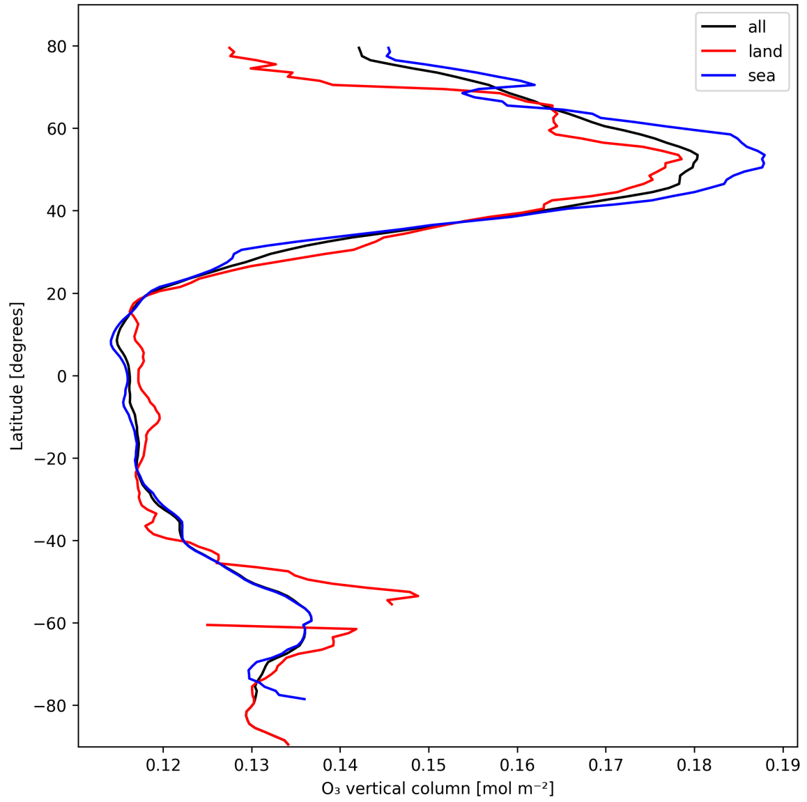
Figure 17: Zonal average of “O 3 vertical column” for 2025-02-24 to 2025-02-25.
