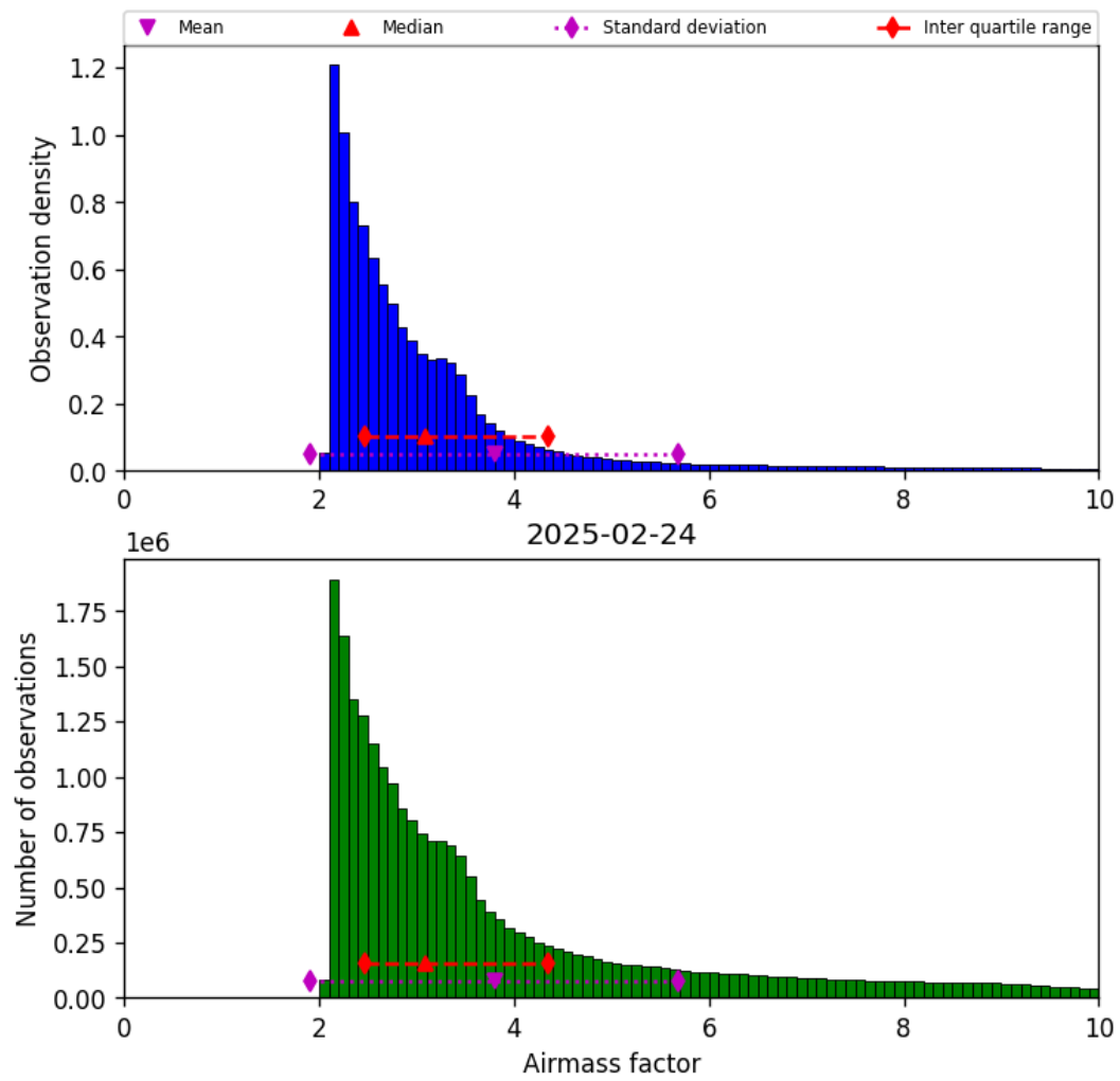
Figure 37: Histogram of “Airmass factor” for 2025-02-24 to 2025-02-25
