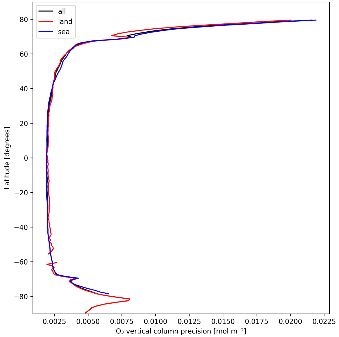
Figure 18: Zonal average of “O 3 vertical column precision” for 2025-02-24 to 2025-02-25.
