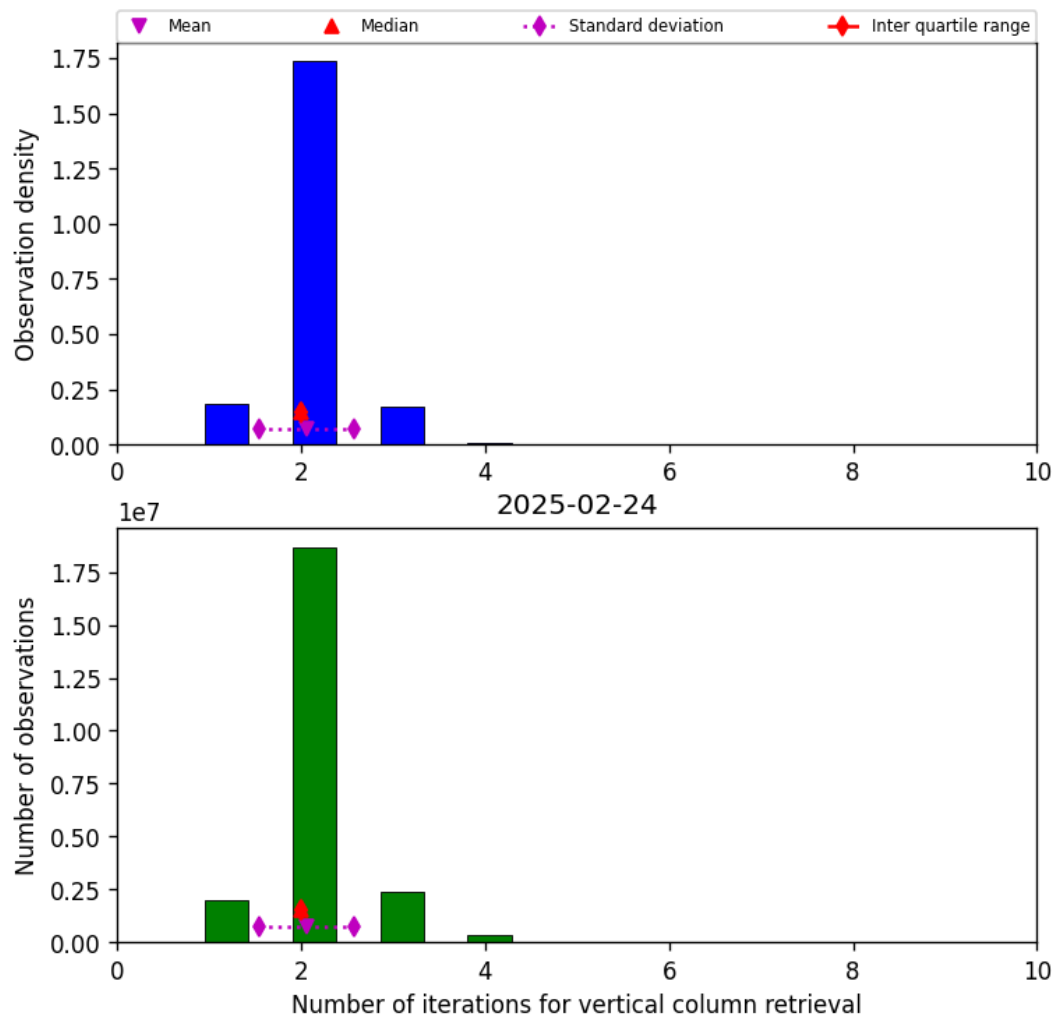
Figure 39: Histogram of “Number of iterations for vertical column retrieval” for 2025-02-24 to 2025-02-25
