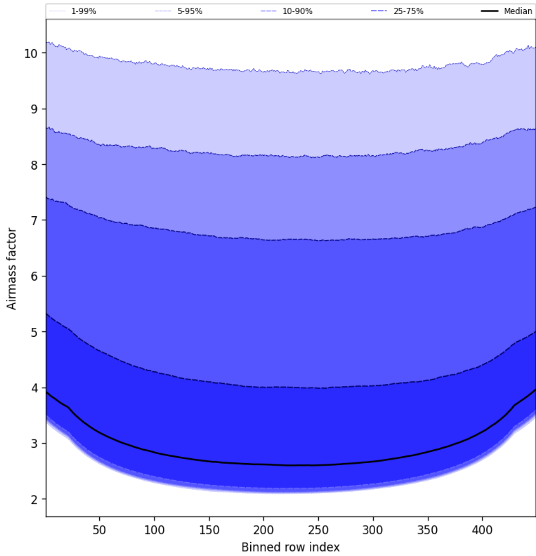
Figure 49: Along track statistics of “Airmass factor” for 2025-02-24 to 2025-02-25
