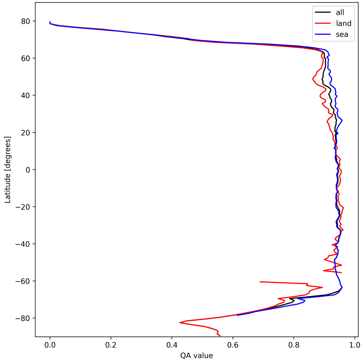
Figure 16: Zonal average of “QA value” for 2025-02-24 to 2025-02-25.
