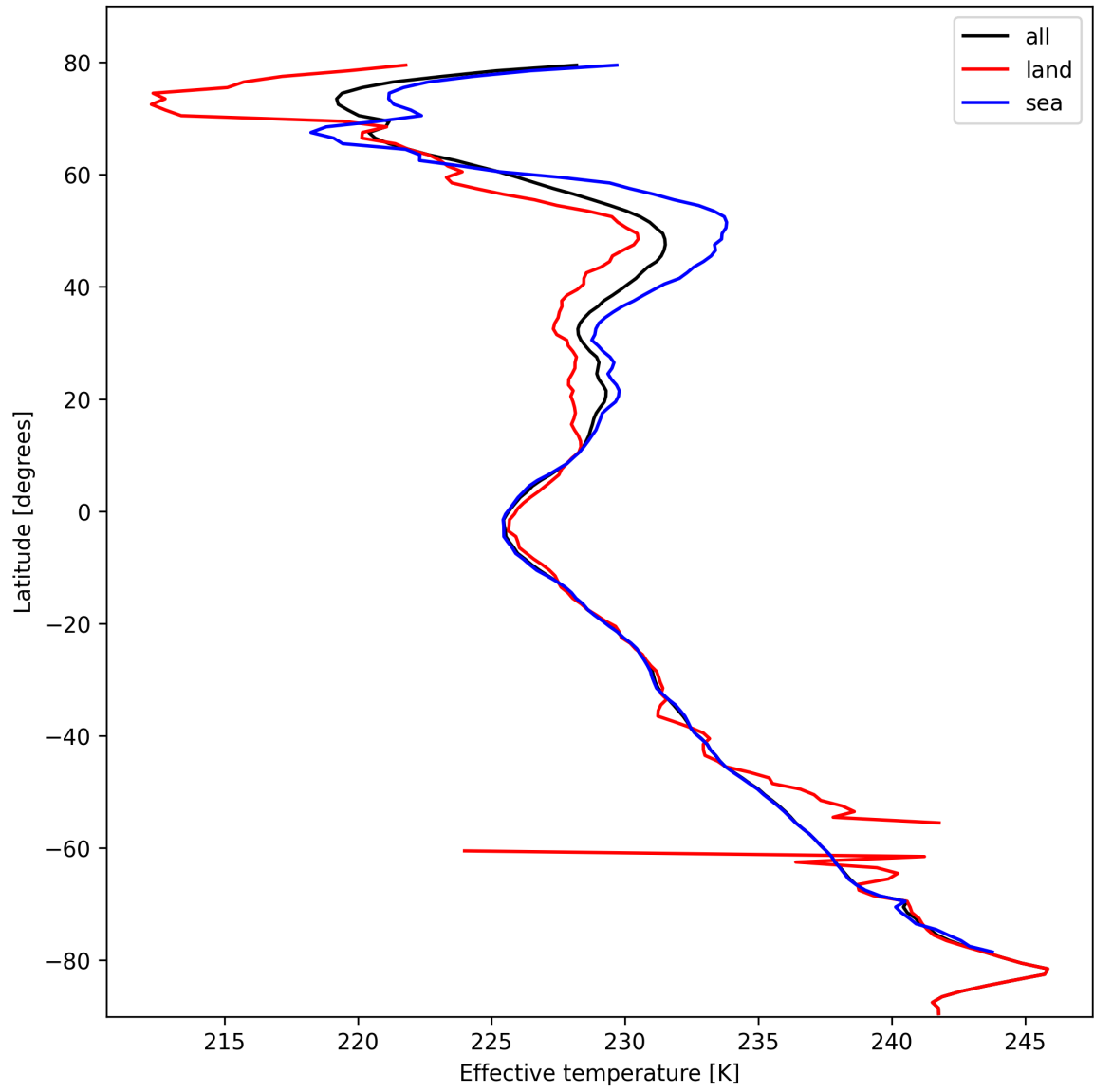
Figure 26: Zonal average of “Effective temperature” for 2025-02-24 to 2025-02-25.
