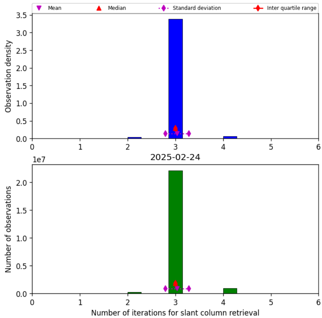
Figure 33: Histogram of “Number of iterations for slant column retrieval” for 2025-02-24 to 2025-02-25
