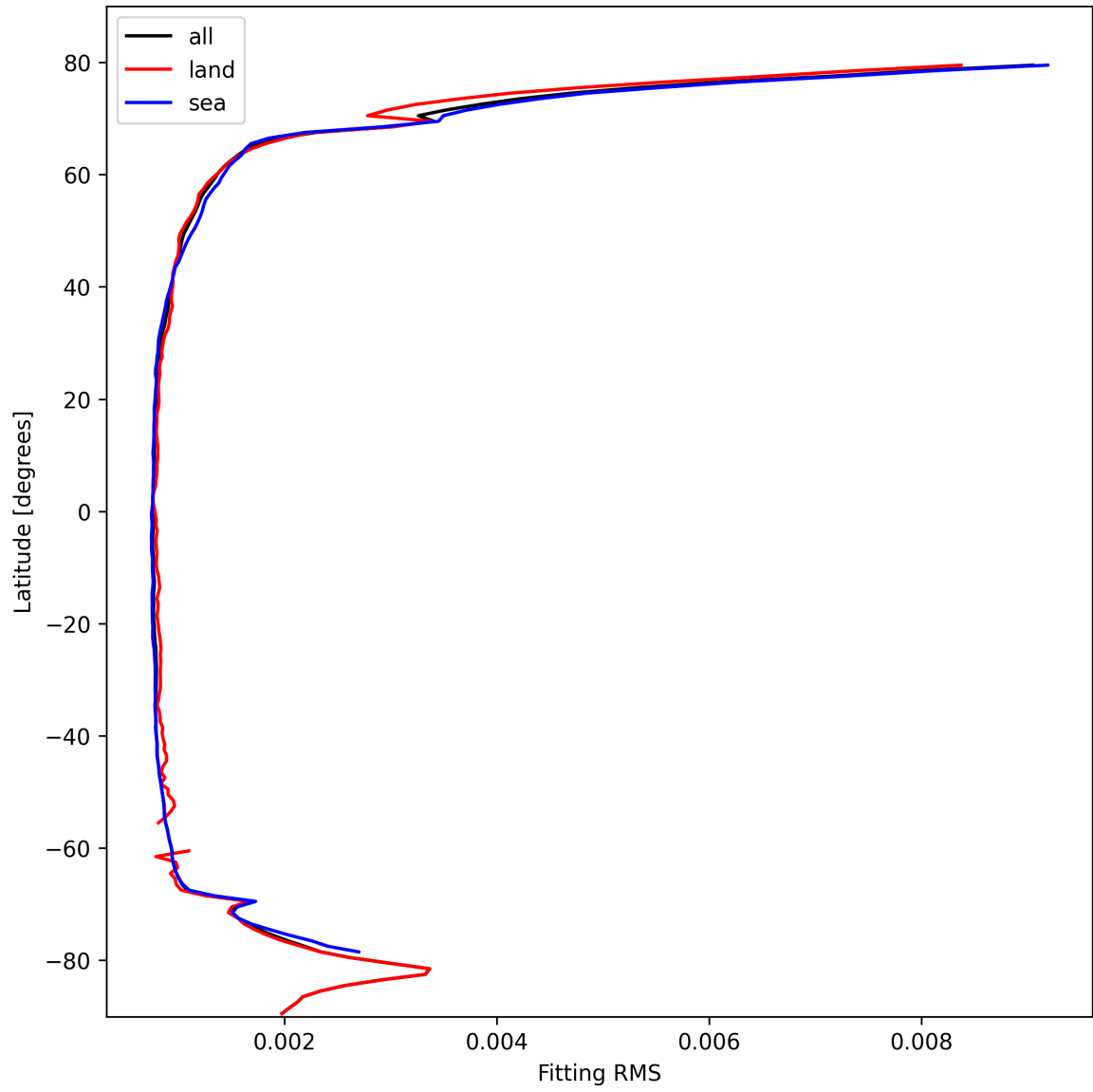
Figure 22: Zonal average of “Fitting RMS” for 2025-02-24 to 2025-02-25.
