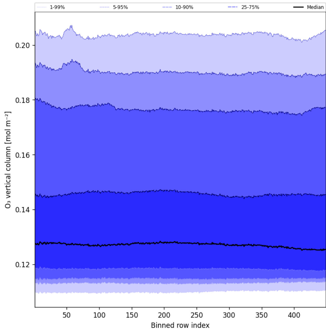
Figure 41: Along track statistics of “ \text{O}_3 vertical column” for 2025-02-24 to 2025-02-25
