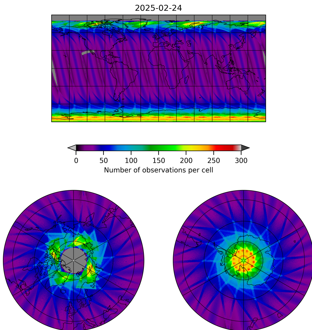
Figure 15: Map of the number of observations for 2025-02-24 to 2025-02-25
