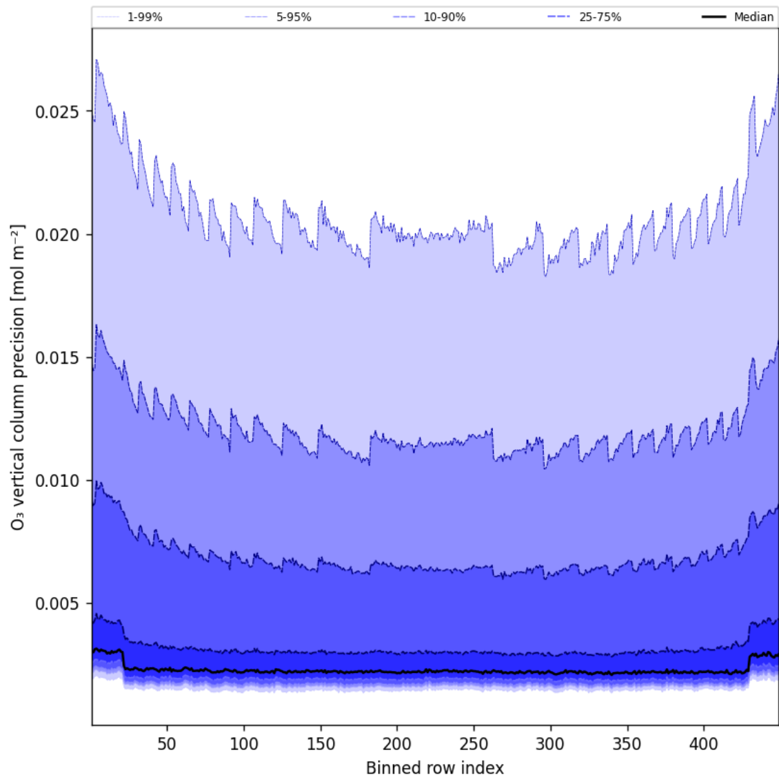
Figure 42: Along track statistics of “O 3 vertical column precision” for 2025-02-24 to 2025-02-25
