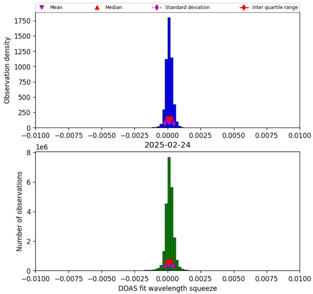
Figure 36: Histogram of “DOAS fit wavelength squeeze” for 2025-02-24 to 2025-02-25
