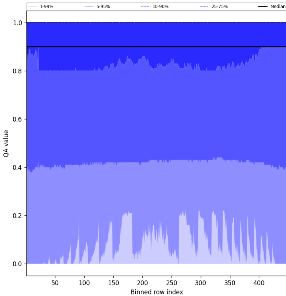
Figure 40: Along track statistics of “QA value” for 2025-02-24 to 2025-02-25
