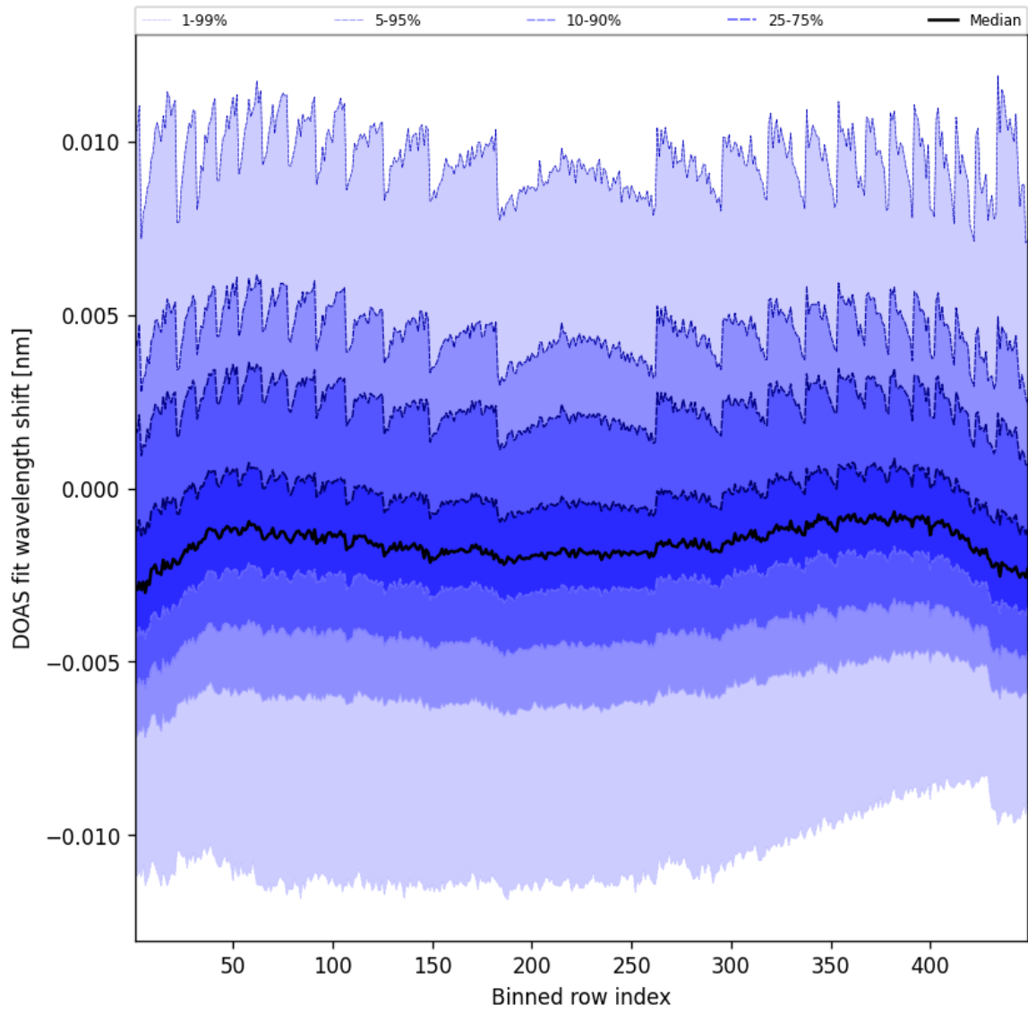
Figure 47: Along track statistics of “DOAS fit wavelength shift” for 2025-02-24 to 2025-02-25
