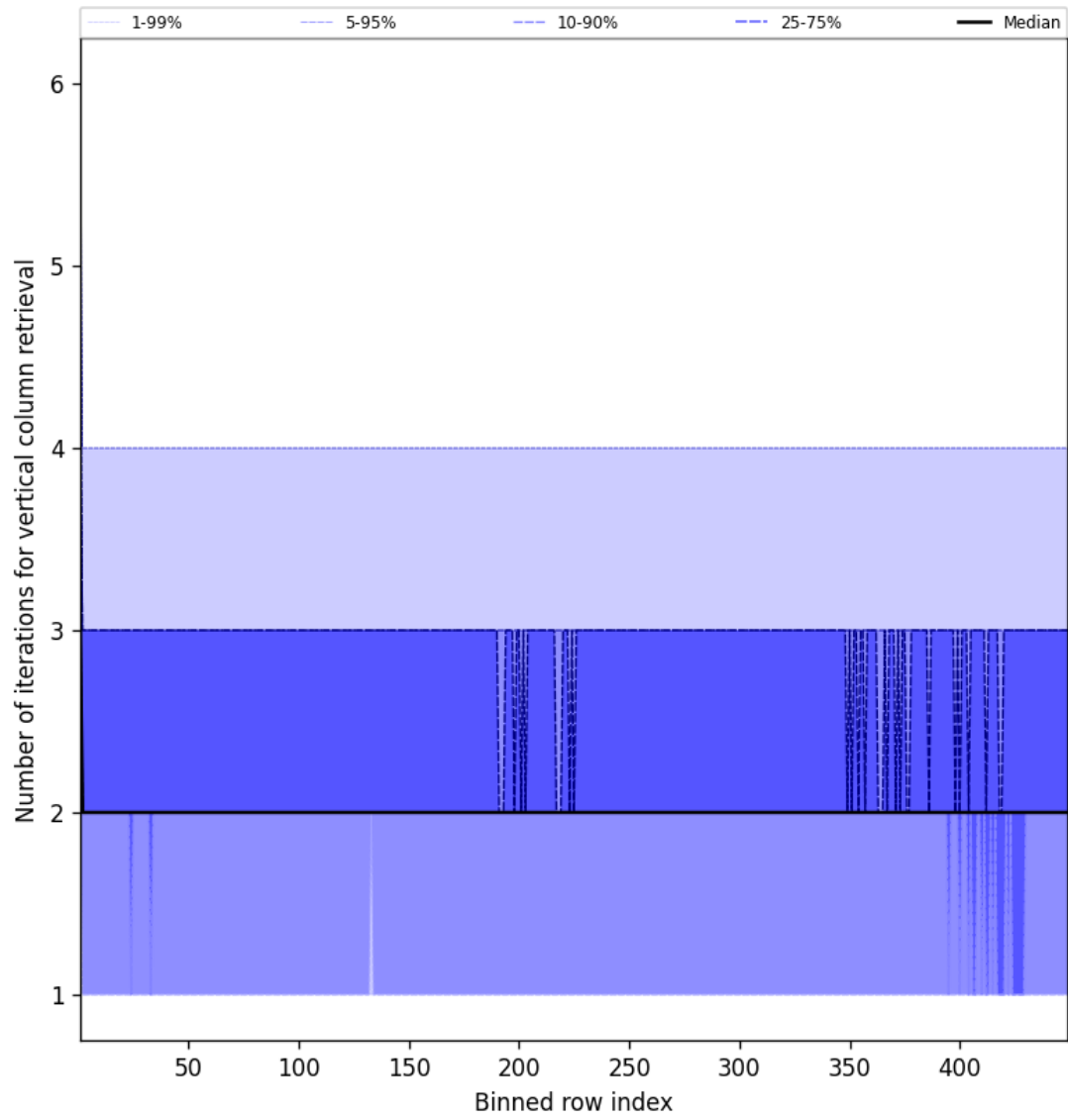
Figure 51: Along track statistics of “Number of iterations for vertical column retrieval” for 2025-02-25 to 2025-02-26
