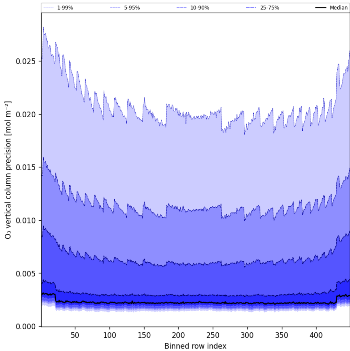
Figure 42: Along track statistics of “O 3 vertical column precision” for 2025-02-25 to 2025-02-26
