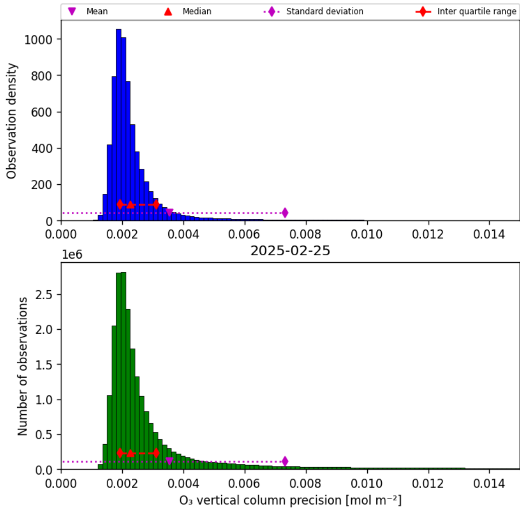
Figure 30: Histogram of “O 3 vertical column precision” for 2025-02-25 to 2025-02-26
