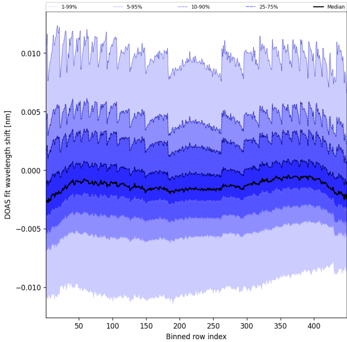
Figure 47: Along track statistics of “DOAS fit wavelength shift” for 2025-02-25 to 2025-02-26
