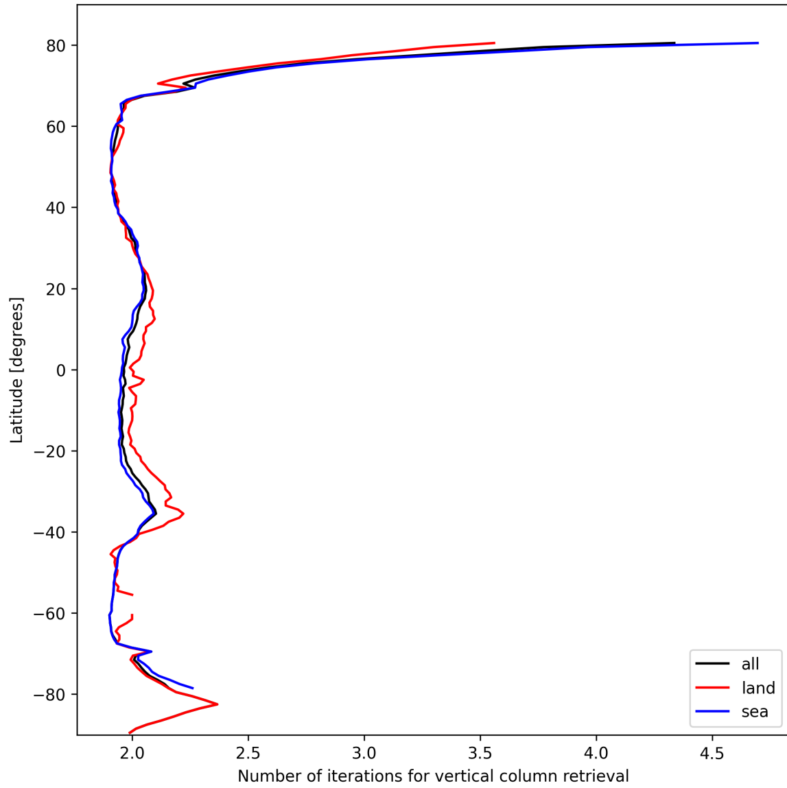
Figure 27: Zonal average of “Number of iterations for vertical column retrieval” for 2025-02-25 to 2025-02-26.
