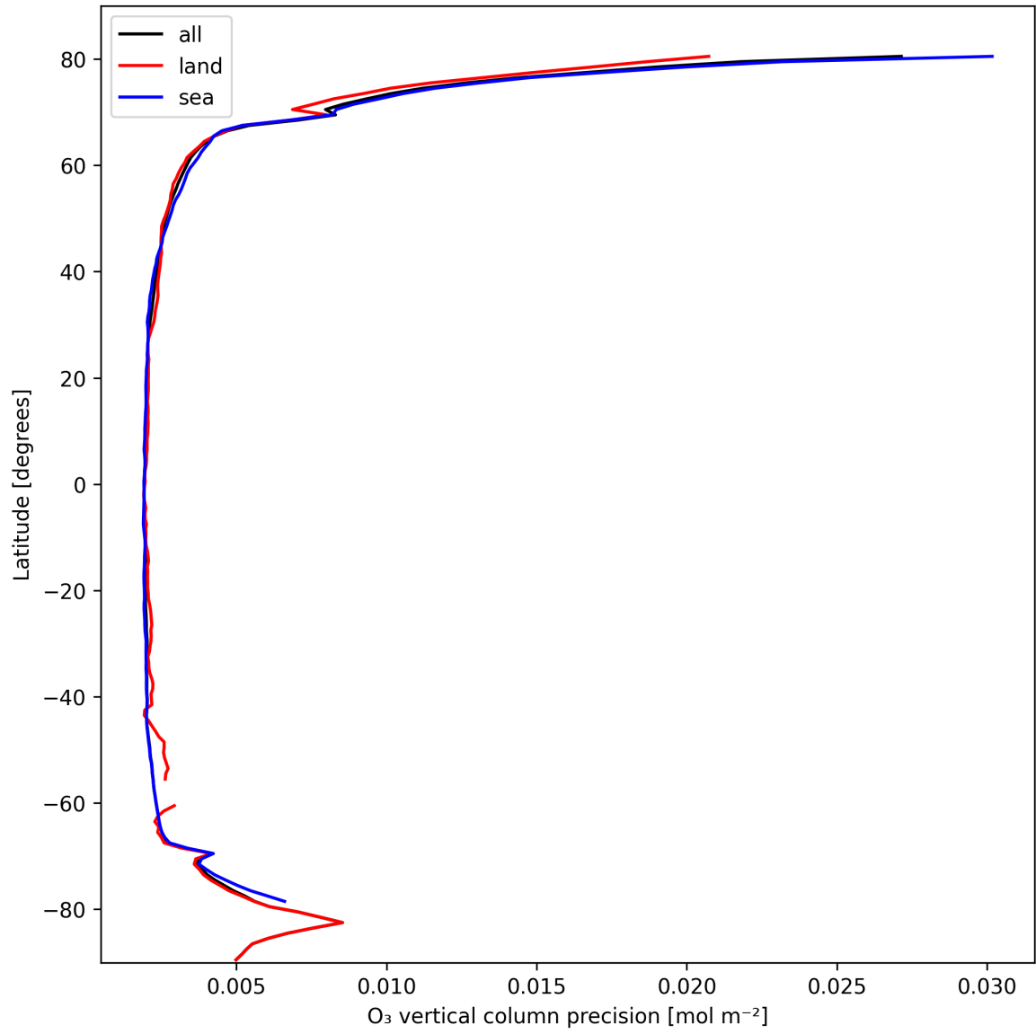
Figure 18: Zonal average of “O 3 vertical column precision” for 2025-02-25 to 2025-02-26.
