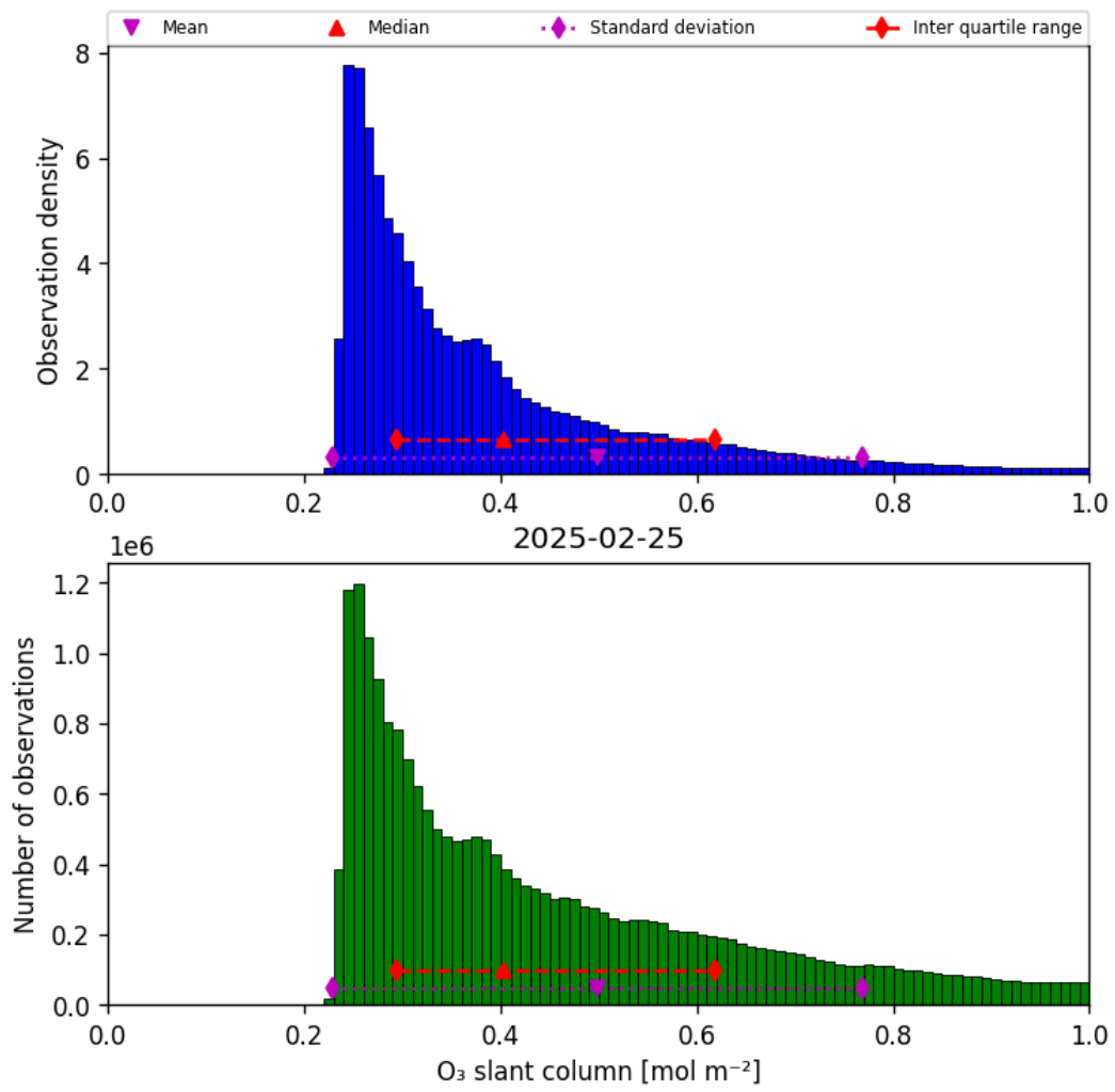
Figure 31: Histogram of “O 3 slant column” for 2025-02-25 to 2025-02-26
