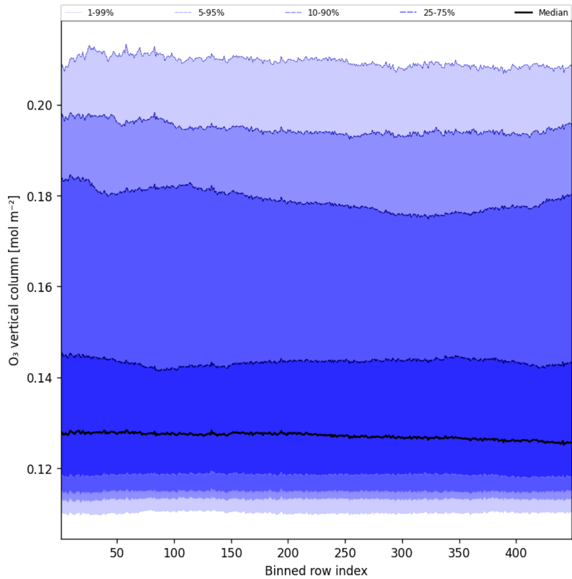
Figure 41: Along track statistics of “O 3 vertical column” for 2025-02-25 to 2025-02-26
