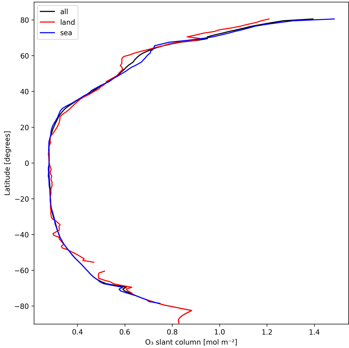
Figure 19: Zonal average of “O 3 slant column” for 2025-02-25 to 2025-02-26.
