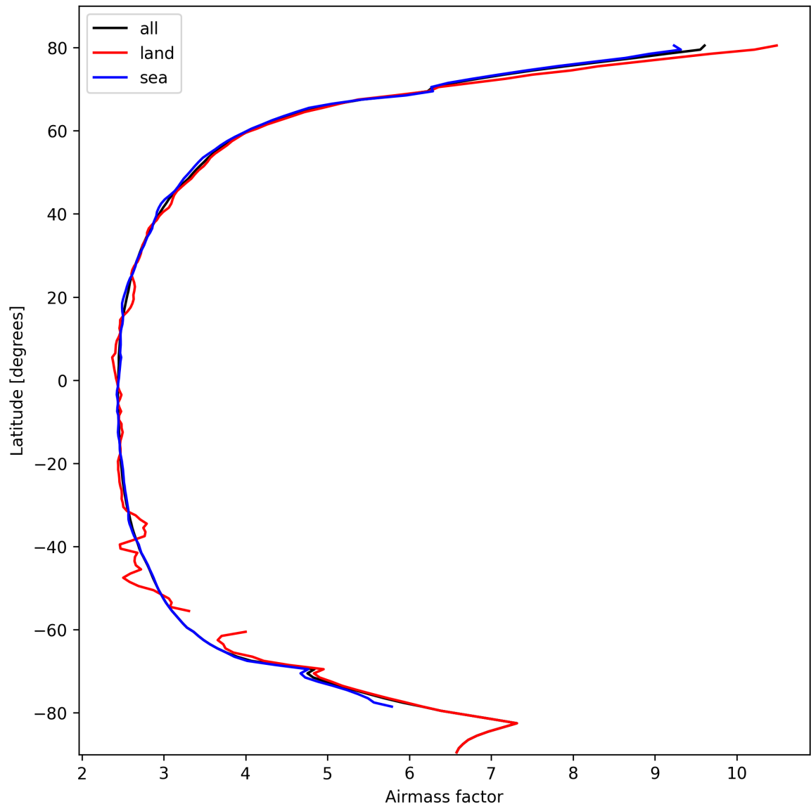
Figure 25: Zonal average of “Airmass factor” for 2025-02-25 to 2025-02-26.
