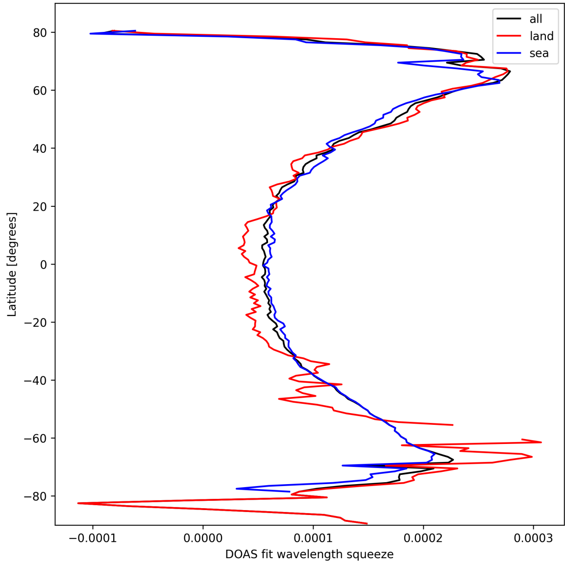
Figure 24: Zonal average of “DOAS fit wavelength squeeze” for 2025-02-25 to 2025-02-26.
