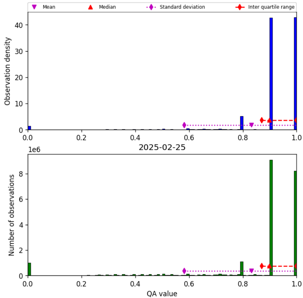
Figure 28: Histogram of “QA value” for 2025-02-25 to 2025-02-26
