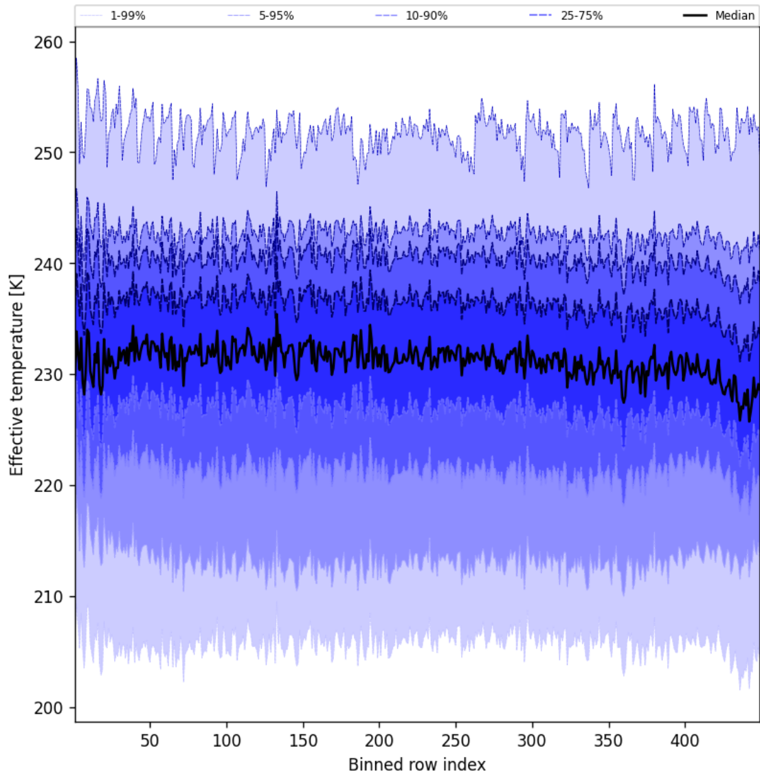
Figure 50: Along track statistics of “Effective temperature” for 2025-02-25 to 2025-02-26
