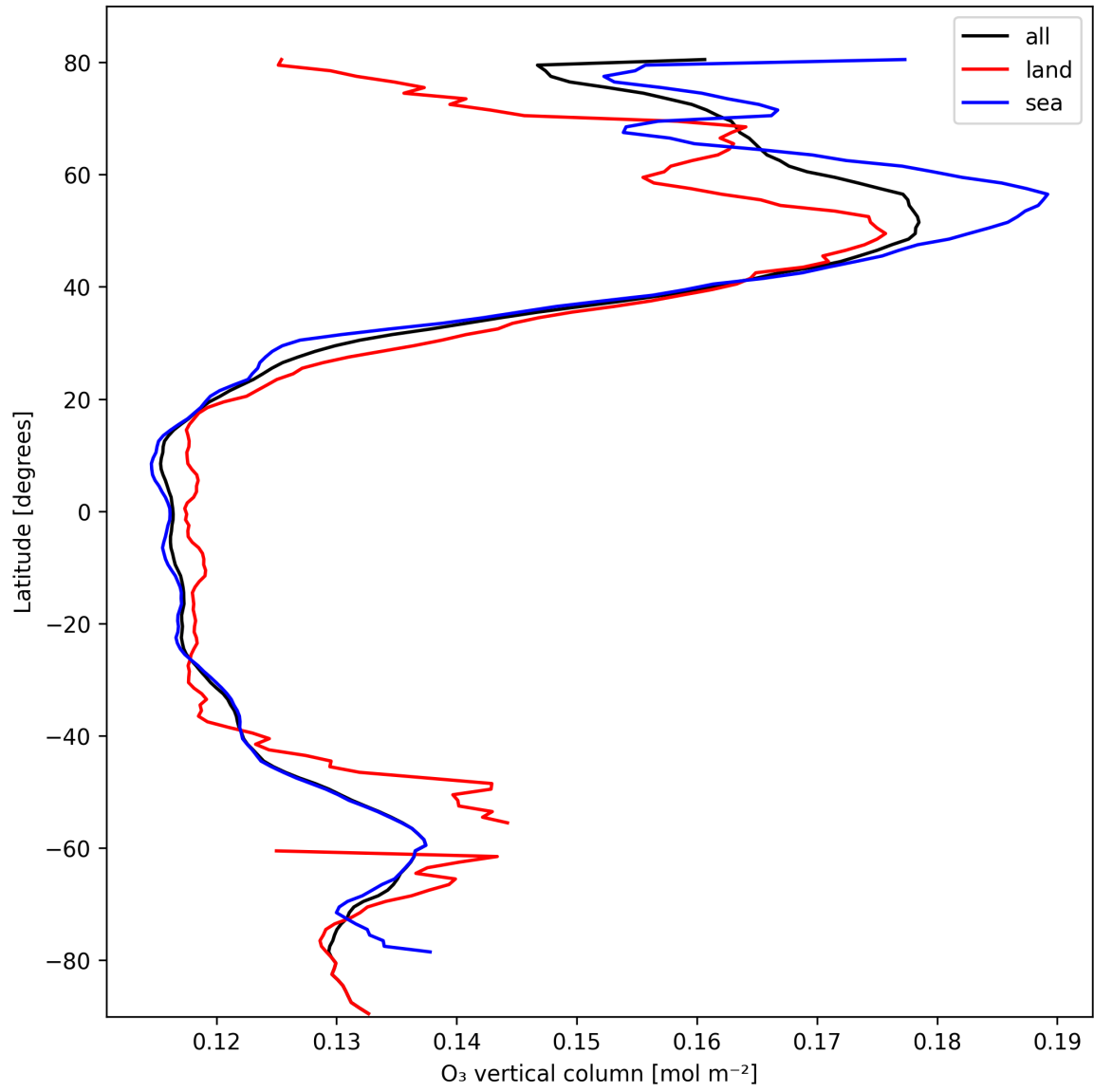
Figure 17: Zonal average of “O 3 vertical column” for 2025-02-25 to 2025-02-26.
