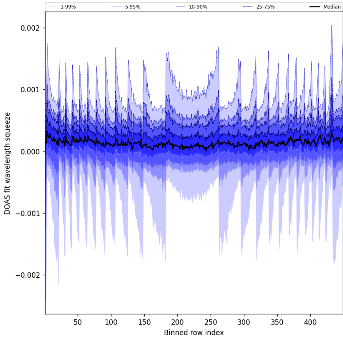
Figure 48: Along track statistics of “DOAS fit wavelength squeeze” for 2025-02-25 to 2025-02-26
