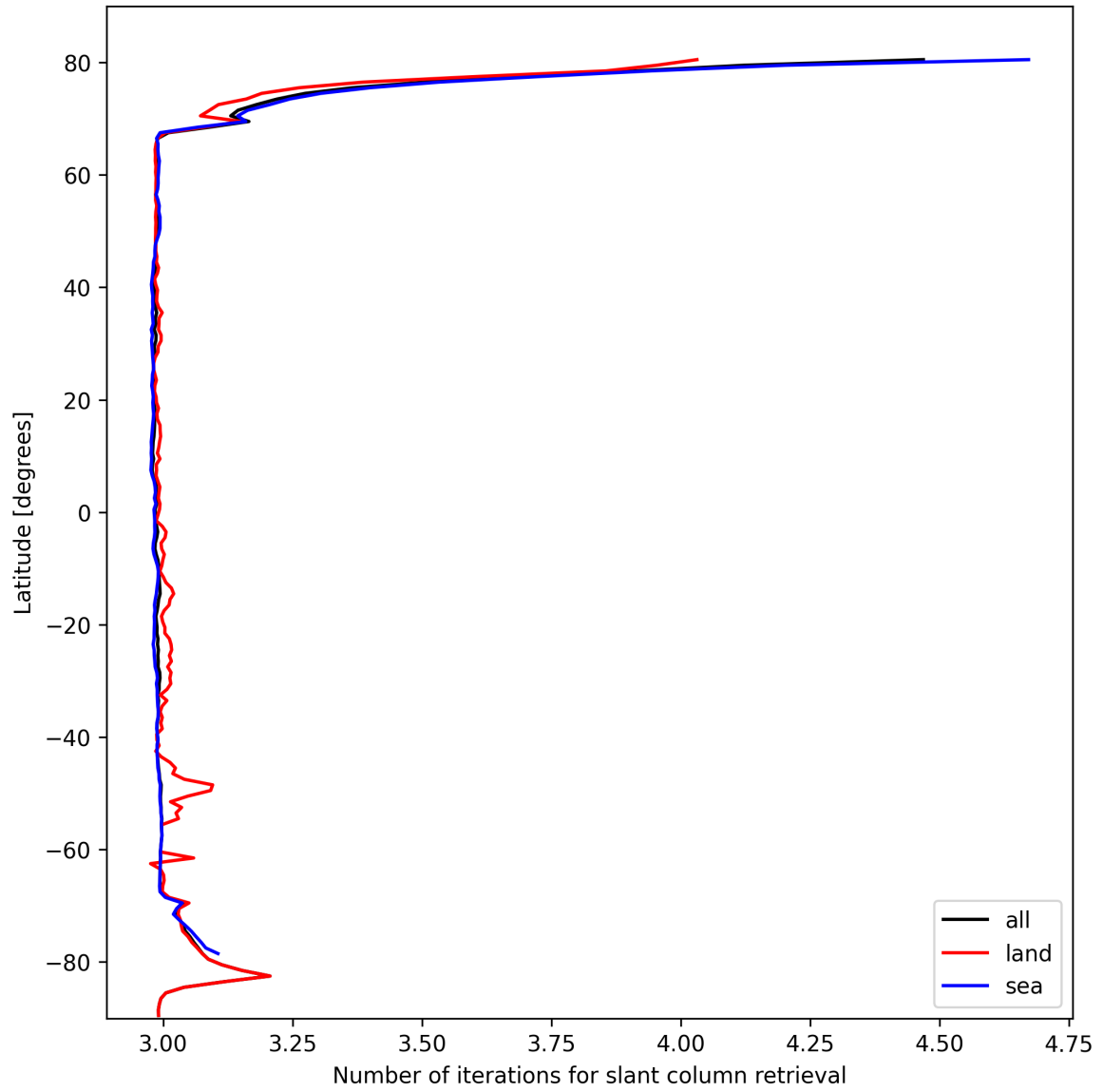
Figure 21: Zonal average of “Number of iterations for slant column retrieval” for 2025-02-25 to 2025-02-26.
