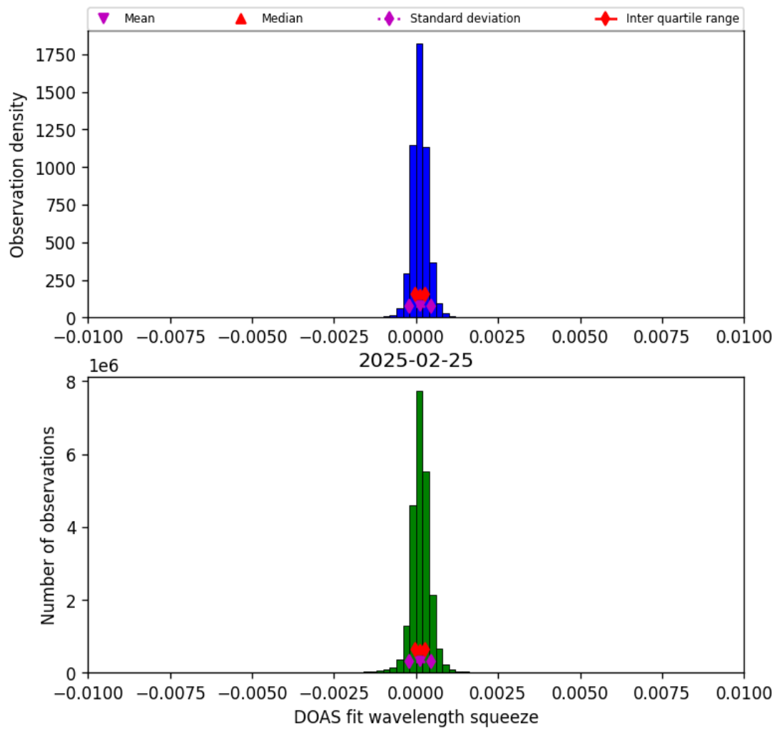
Figure 36: Histogram of “DOAS fit wavelength squeeze” for 2025-02-25 to 2025-02-26
