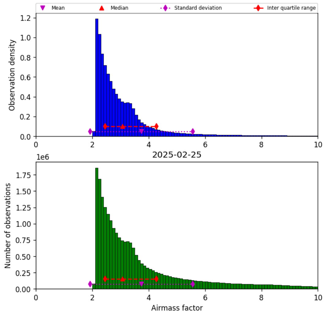
Figure 37: Histogram of “Airmass factor” for 2025-02-25 to 2025-02-26
