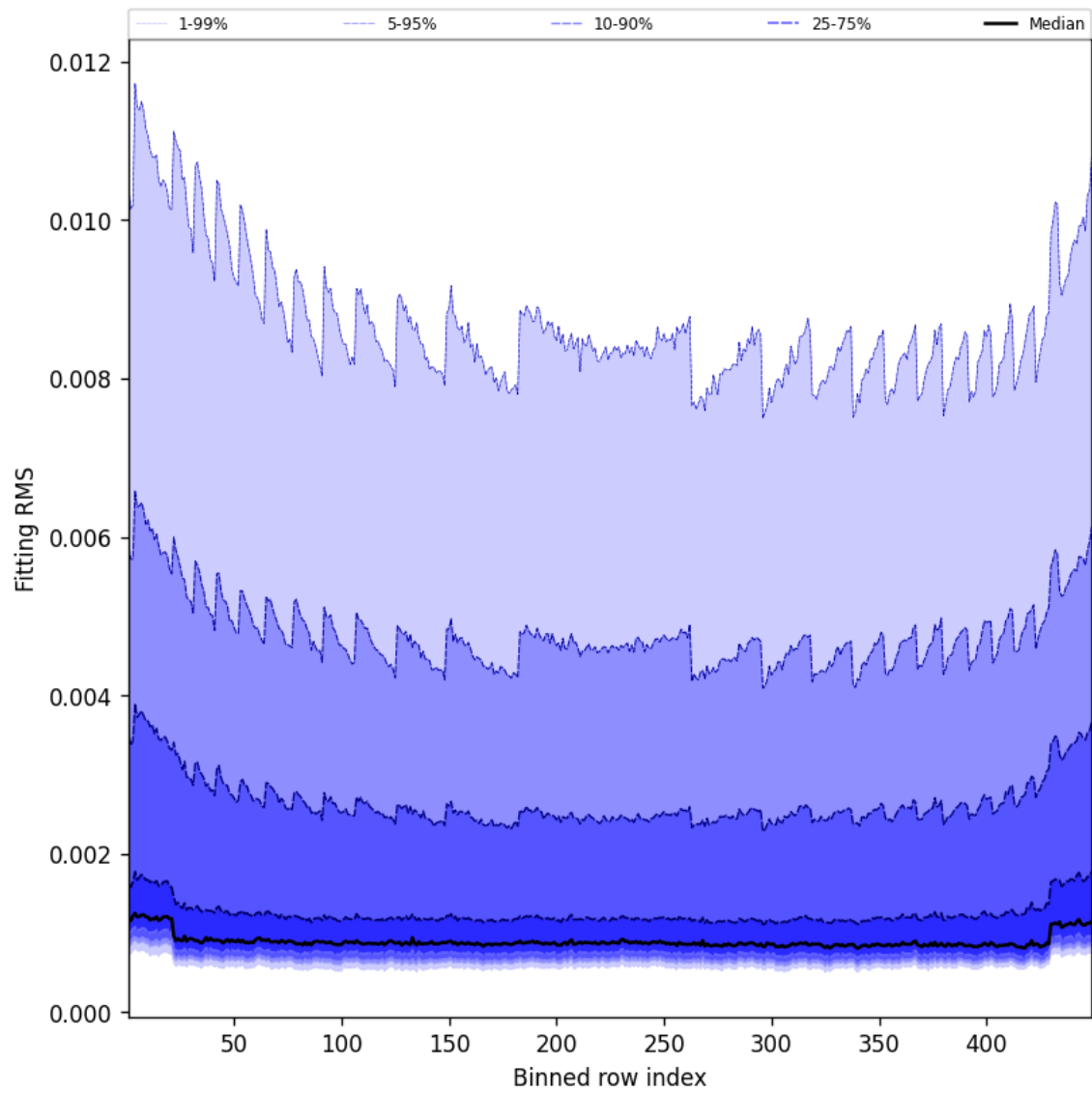
Figure 46: Along track statistics of “Fitting RMS” for 2025-02-25 to 2025-02-26
