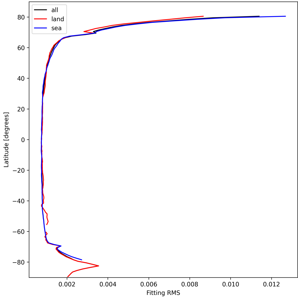
Figure 22: Zonal average of “Fitting RMS” for 2025-02-25 to 2025-02-26.
