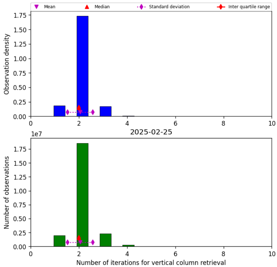
Figure 39: Histogram of “Number of iterations for vertical column retrieval” for 2025-02-25 to 2025-02-26
