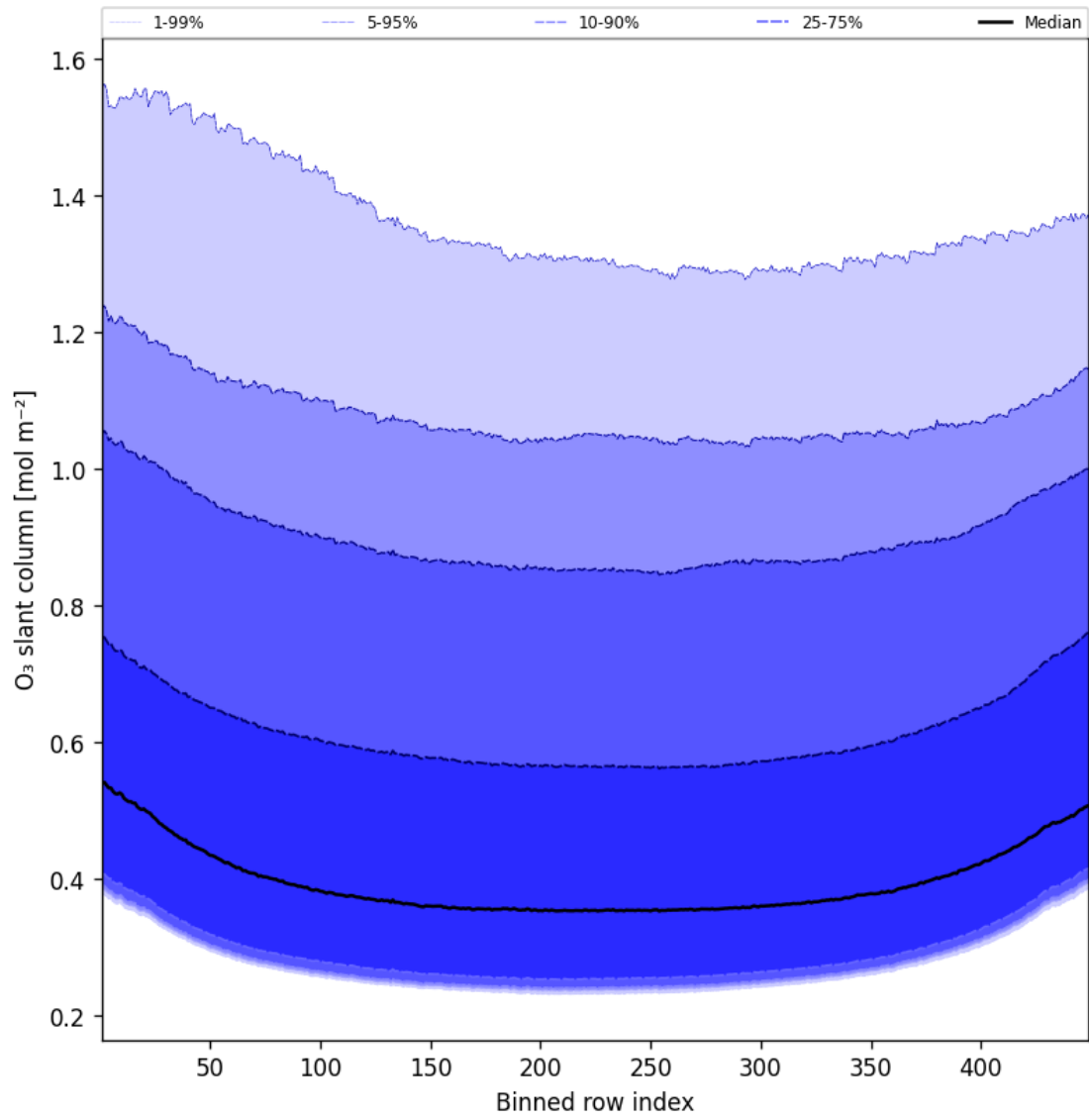
Figure 43: Along track statistics of “O 3 slant column” for 2025-02-25 to 2025-02-26
