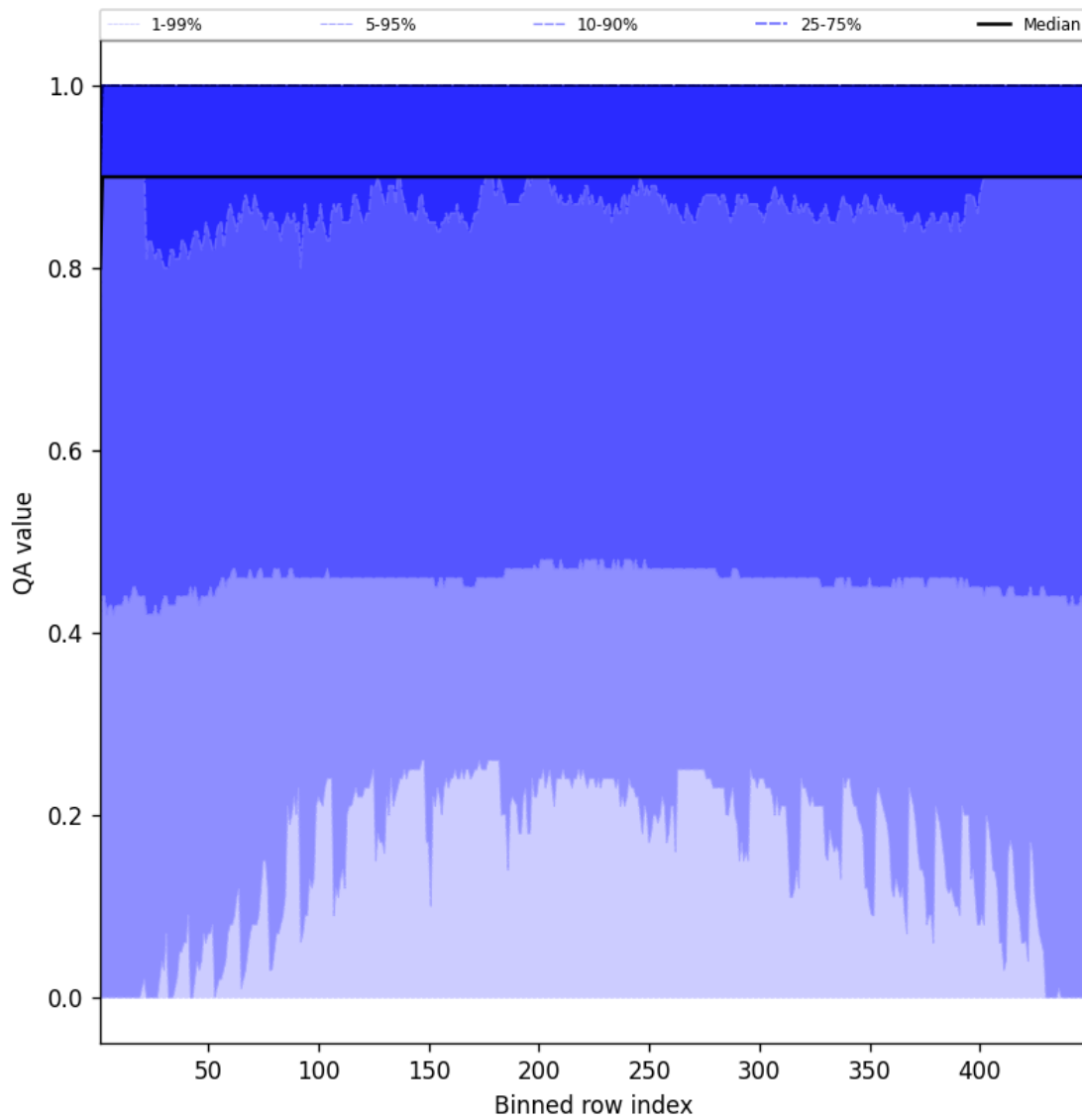
Figure 40: Along track statistics of “QA value” for 2025-02-25 to 2025-02-26
