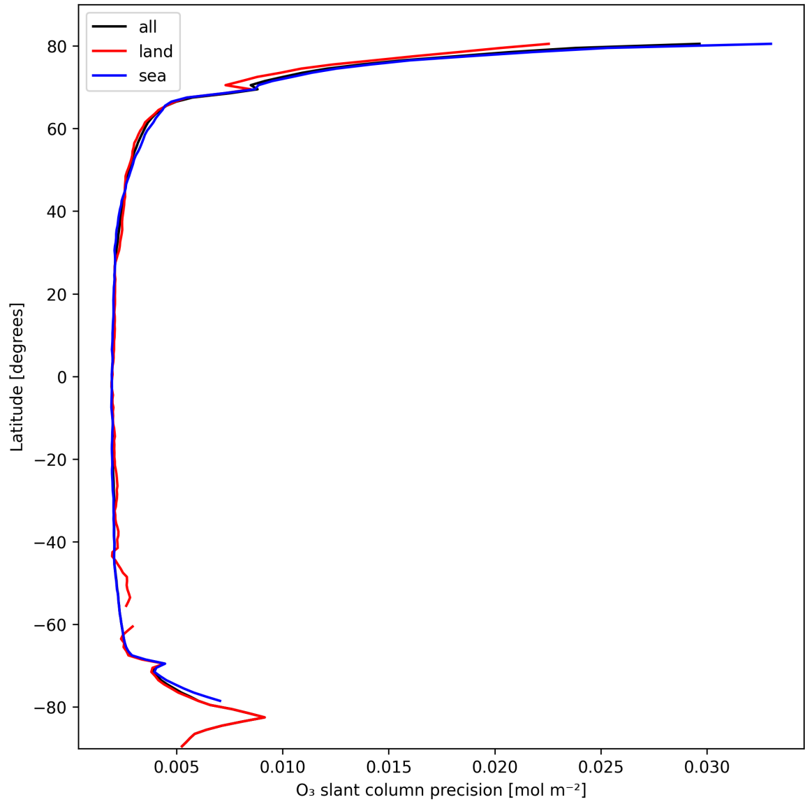
Figure 20: Zonal average of “O 3 slant column precision” for 2025-02-25 to 2025-02-26.
