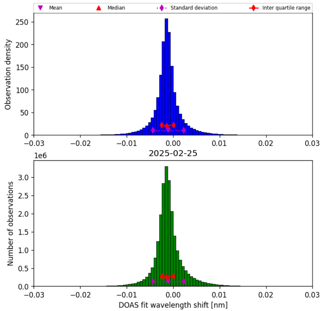
Figure 35: Histogram of “DOAS fit wavelength shift” for 2025-02-25 to 2025-02-26
