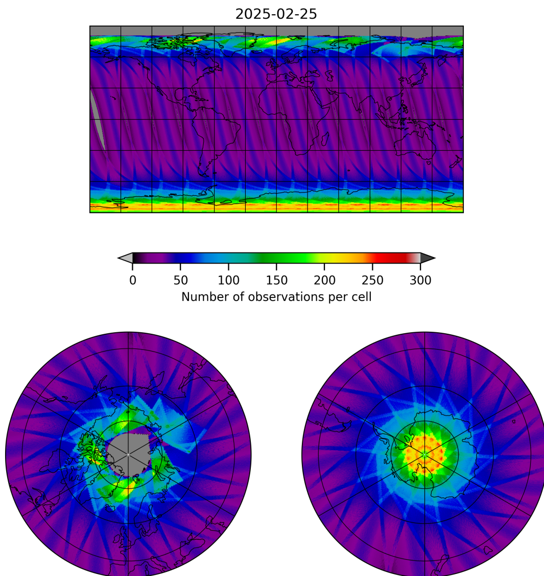
Figure 15: Map of the number of observations for 2025-02-25 to 2025-02-26
