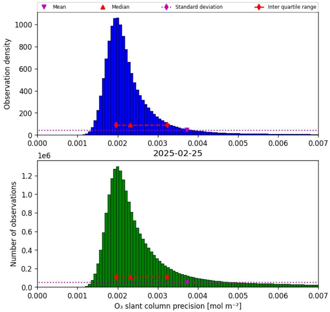
Figure 32: Histogram of “O 3 slant column precision” for 2025-02-25 to 2025-02-26
