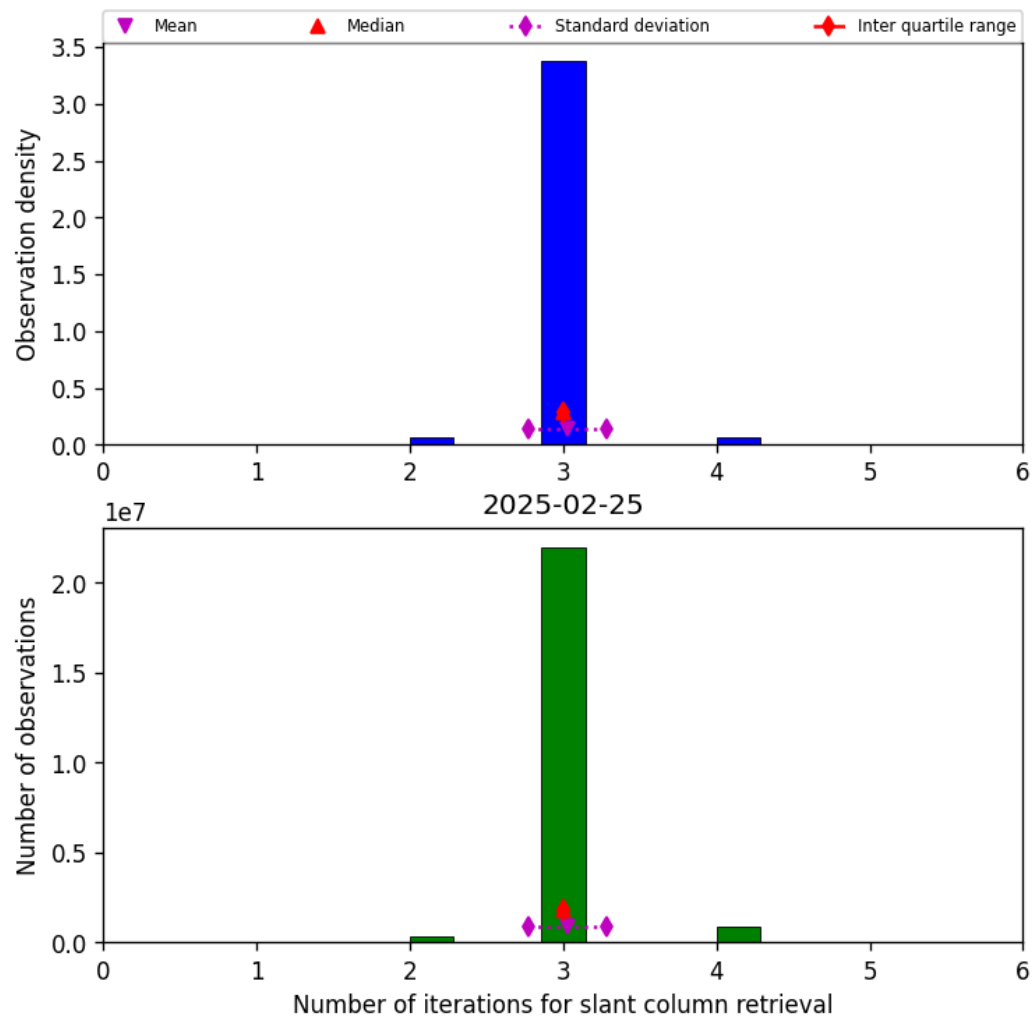
Figure 33: Histogram of “Number of iterations for slant column retrieval” for 2025-02-25 to 2025-02-26
