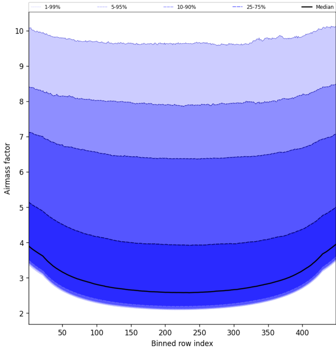
Figure 49: Along track statistics of “Airmass factor” for 2025-02-25 to 2025-02-26
