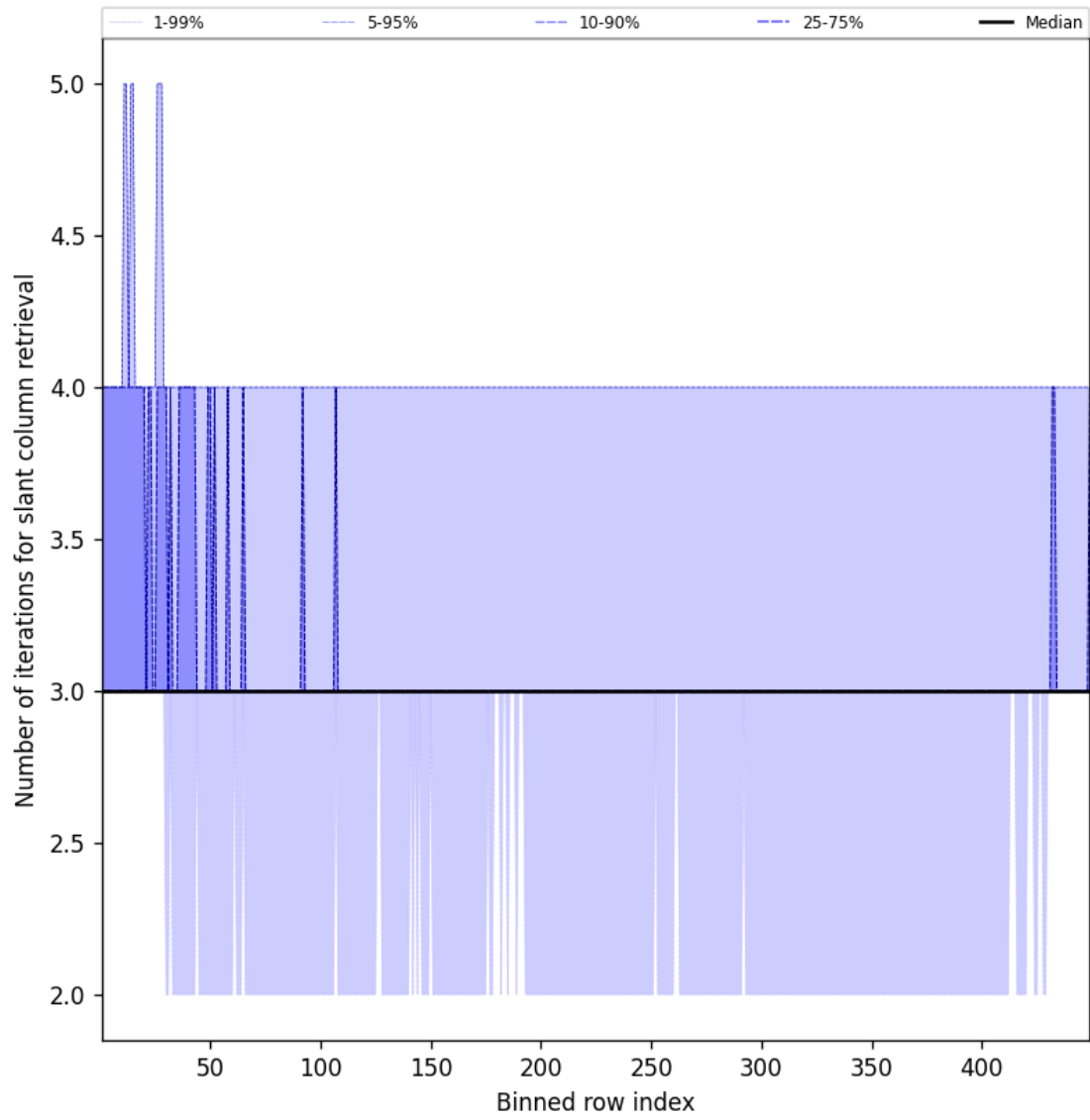
Figure 45: Along track statistics of “Number of iterations for slant column retrieval” for 2025-02-25 to 2025-02-26
