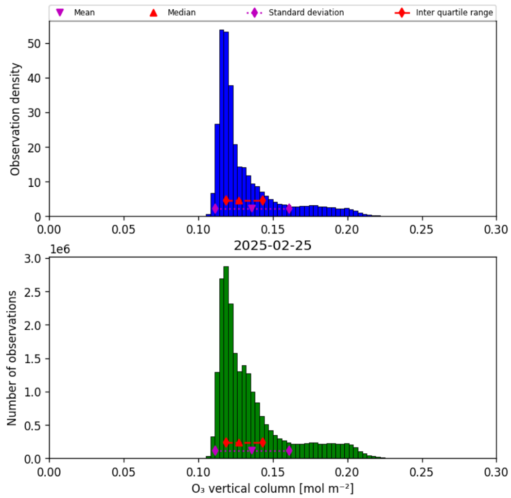
Figure 29: Histogram of “O 3 vertical column” for 2025-02-25 to 2025-02-26
