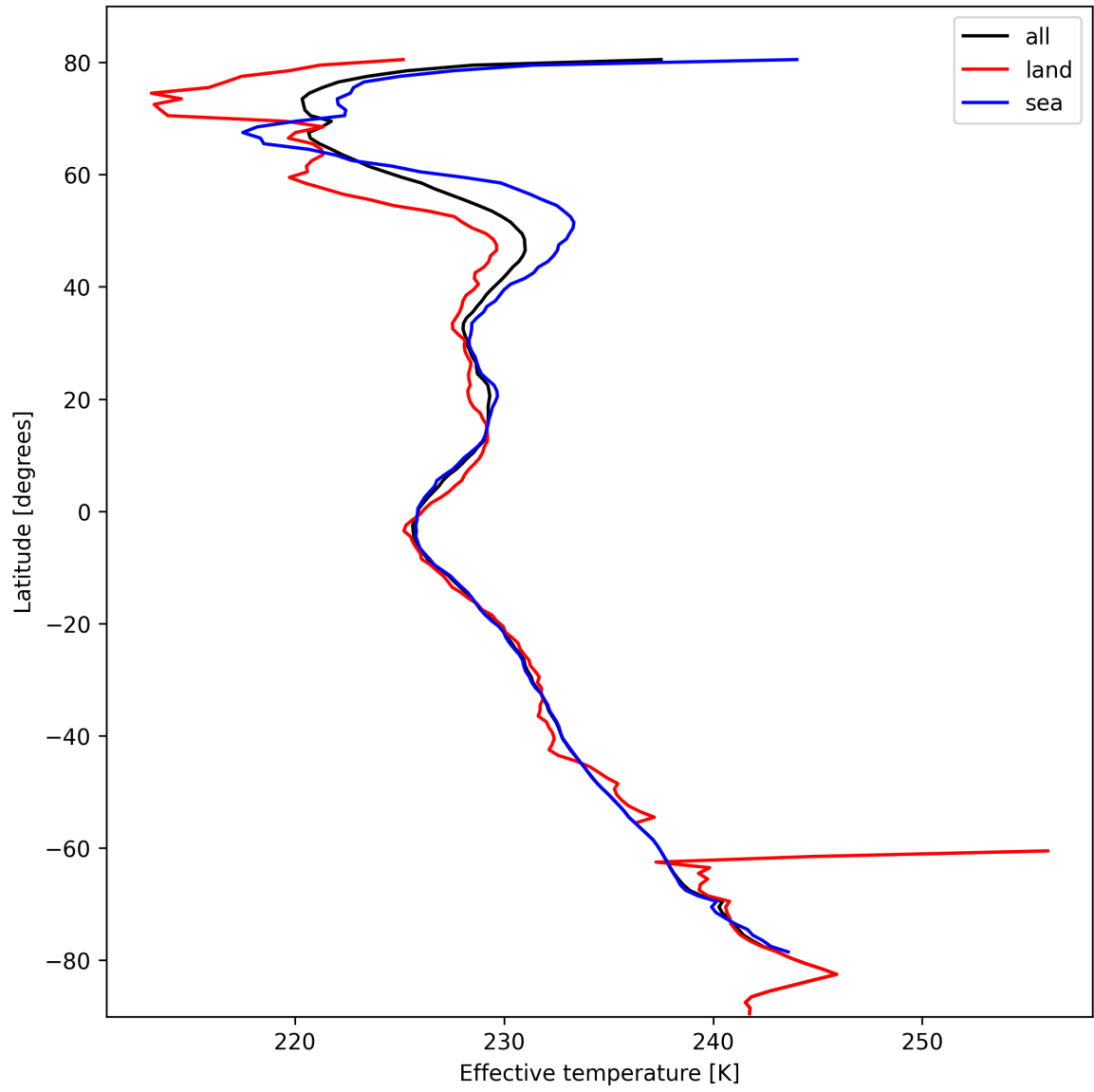
Figure 26: Zonal average of “Effective temperature” for 2025-02-25 to 2025-02-26.
