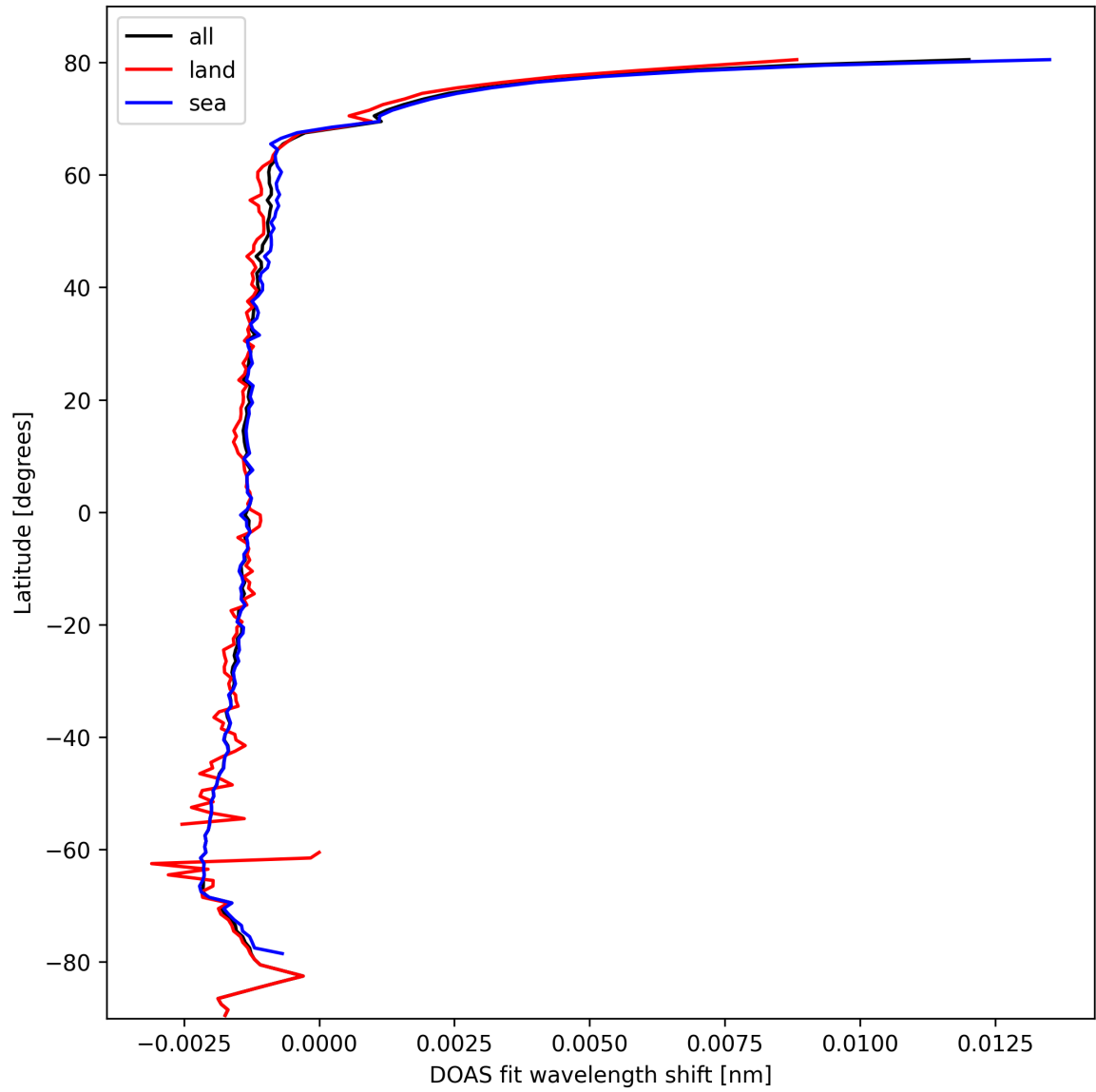
Figure 23: Zonal average of "DOAS fit wavelength shift" for 2025-02-25 to 2025-02-26.
