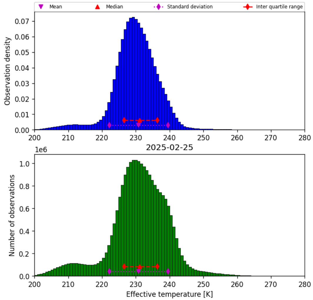
Figure 38: Histogram of “Effective temperature” for 2025-02-25 to 2025-02-26
