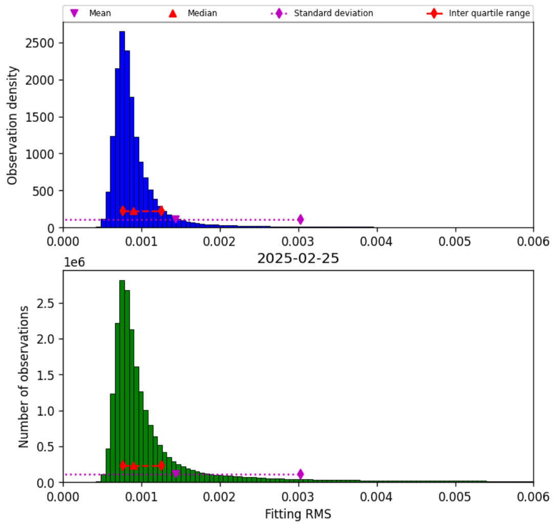
Figure 34: Histogram of “Fitting RMS” for 2025-02-25 to 2025-02-26
