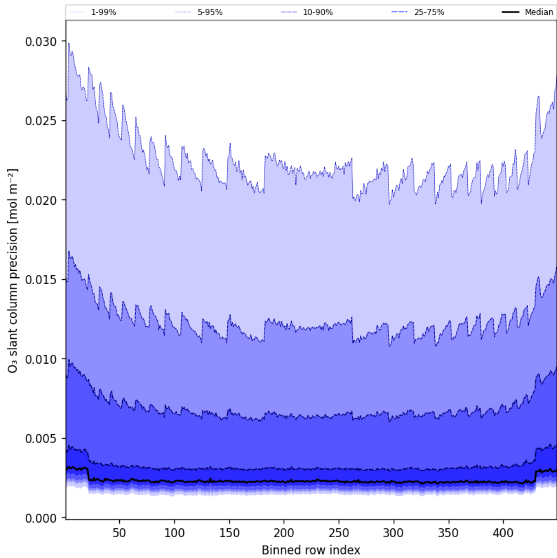
Figure 44: Along track statistics of “O 3 slant column precision” for 2025-02-25 to 2025-02-26
