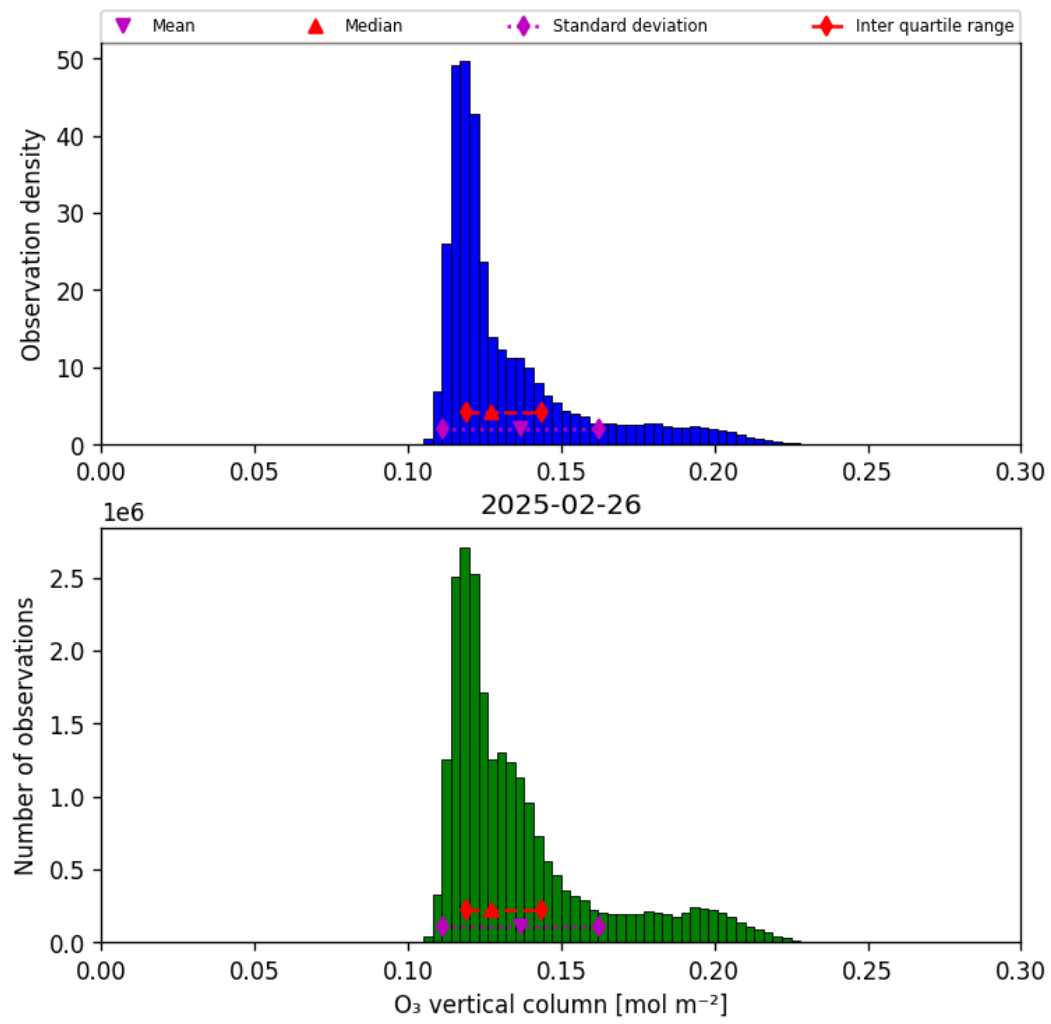
Figure 29: Histogram of “O 3 vertical column” for 2025-02-26 to 2025-02-27
