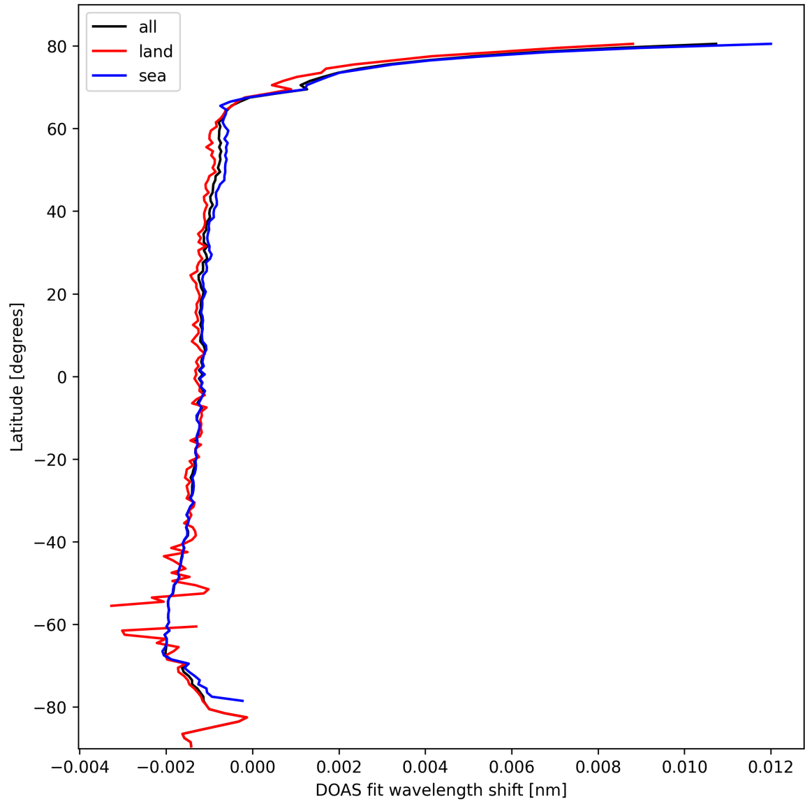
Figure 23: Zonal average of “DOAS fit wavelength shift” for 2025-02-26 to 2025-02-27.
