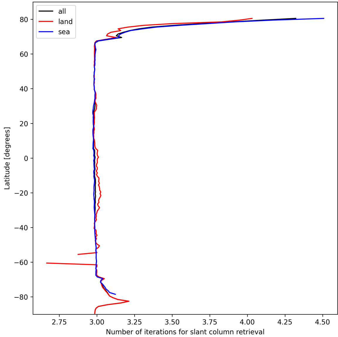
Figure 21: Zonal average of “Number of iterations for slant column retrieval” for 2025-02-26 to 2025-02-27.
