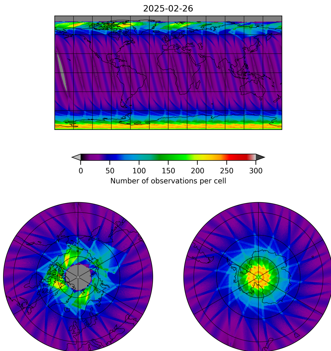
Figure 15: Map of the number of observations for 2025-02-26 to 2025-02-27
