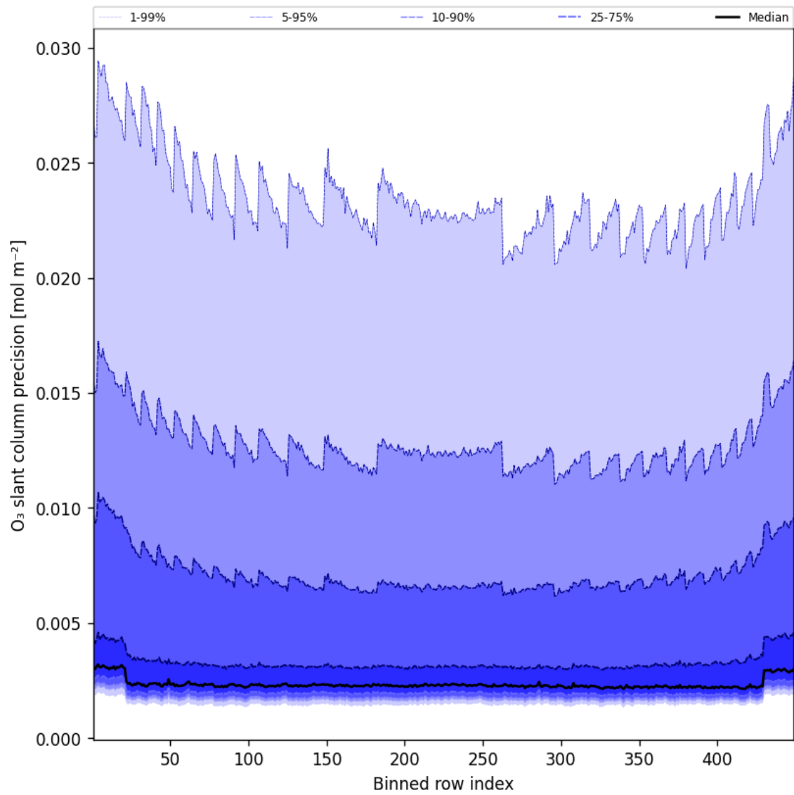
Figure 44: Along track statistics of “O 3 slant column precision” for 2025-02-26 to 2025-02-27
