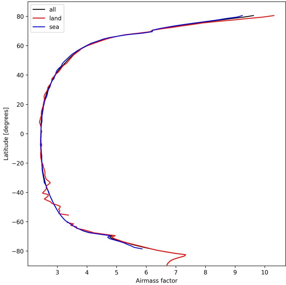
Figure 25: Zonal average of “Airmass factor” for 2025-02-26 to 2025-02-27.
