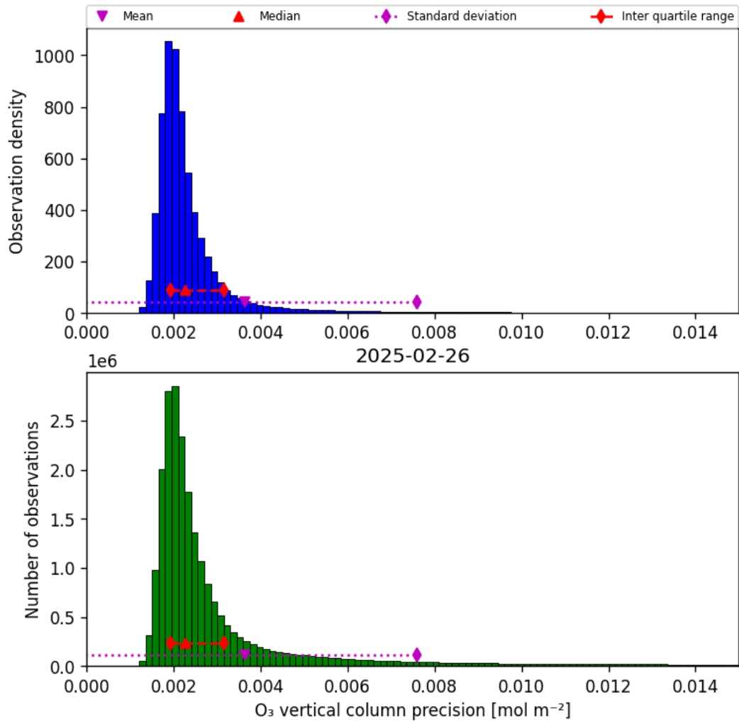
Figure 30: Histogram of “O 3 vertical column precision” for 2025-02-26 to 2025-02-27
