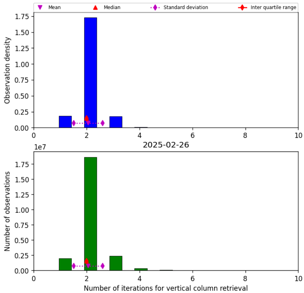
Figure 39: Histogram of “Number of iterations for vertical column retrieval” for 2025-02-26 to 2025-02-27
