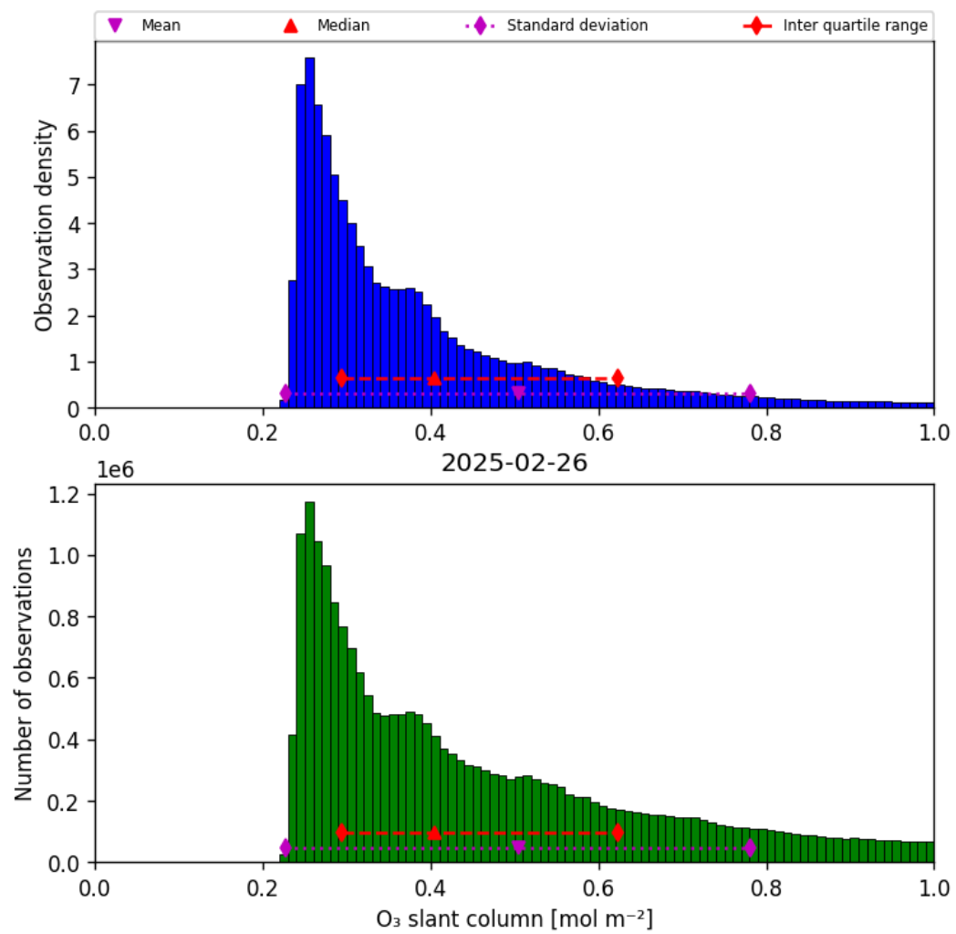
Figure 31: Histogram of “O 3 slant column” for 2025-02-26 to 2025-02-27
