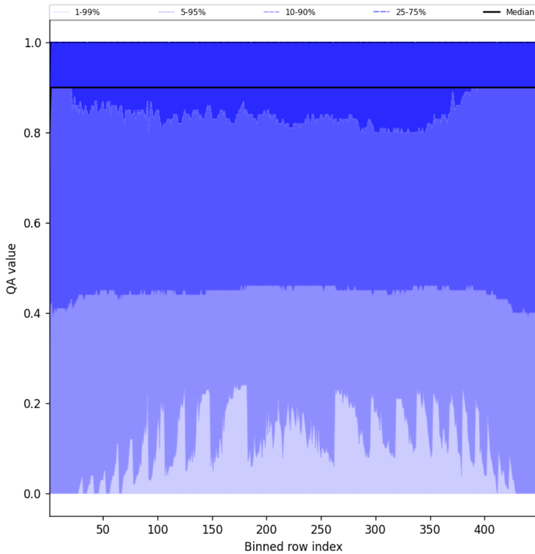
Figure 40: Along track statistics of “QA value” for 2025-02-26 to 2025-02-27
