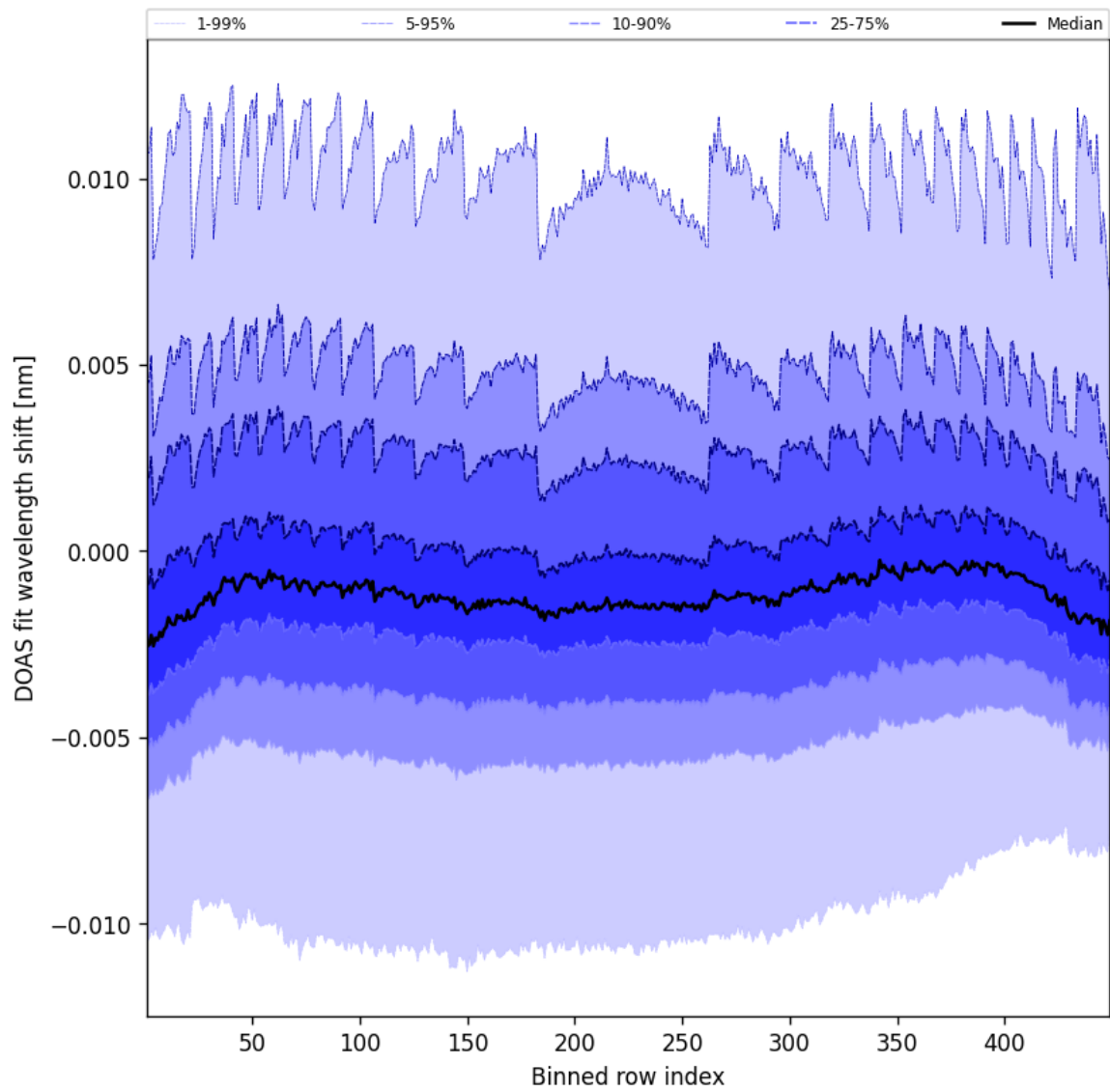
Figure 47: Along track statistics of “DOAS fit wavelength shift” for 2025-02-26 to 2025-02-27
