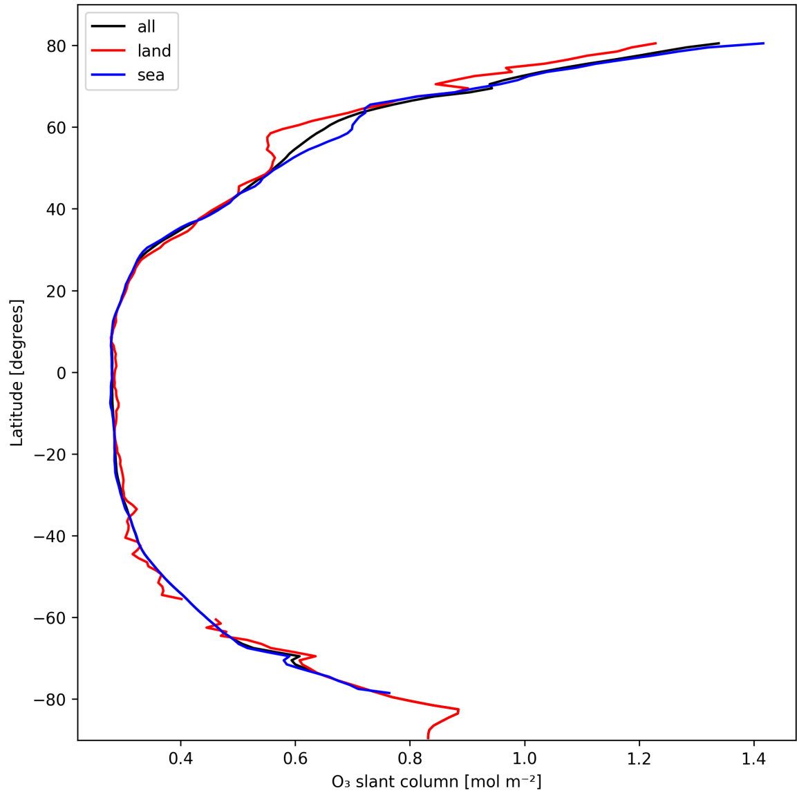
Figure 19: Zonal average of “O 3 slant column” for 2025-02-26 to 2025-02-27.
