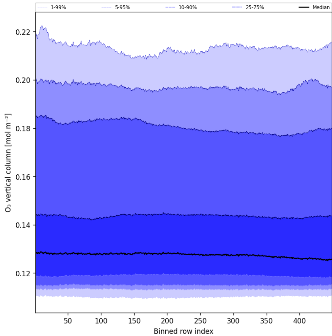
Figure 41: Along track statistics of “O 3 vertical column” for 2025-02-26 to 2025-02-27
