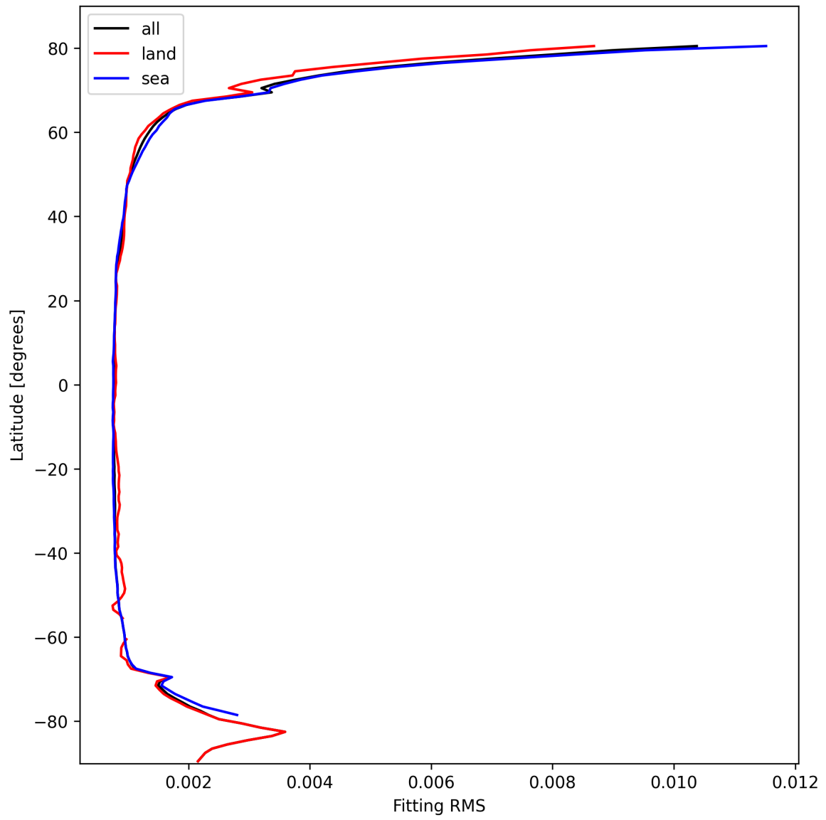
Figure 22: Zonal average of “Fitting RMS” for 2025-02-26 to 2025-02-27.
