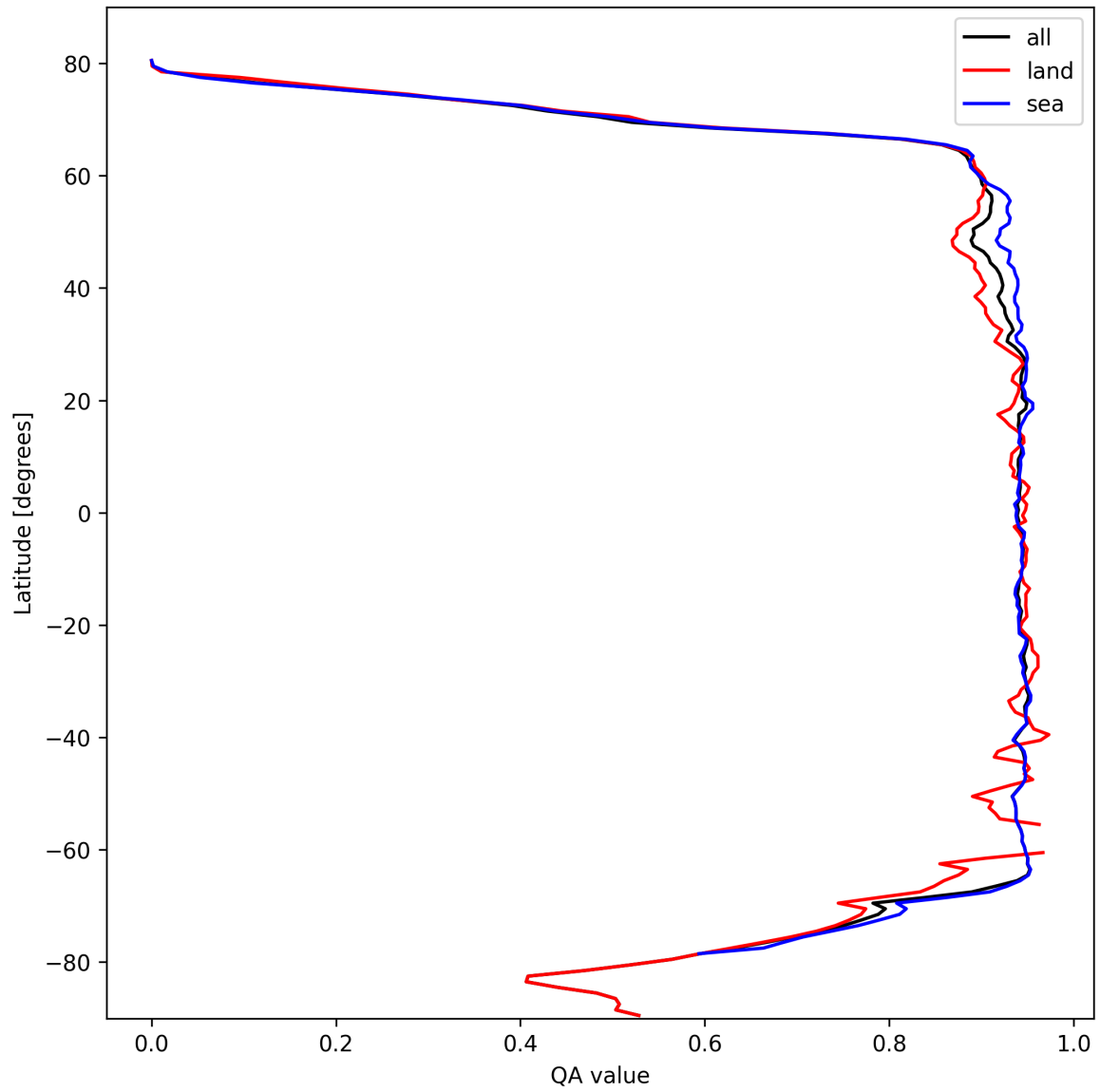
Figure 16: Zonal average of “QA value” for 2025-02-26 to 2025-02-27.
