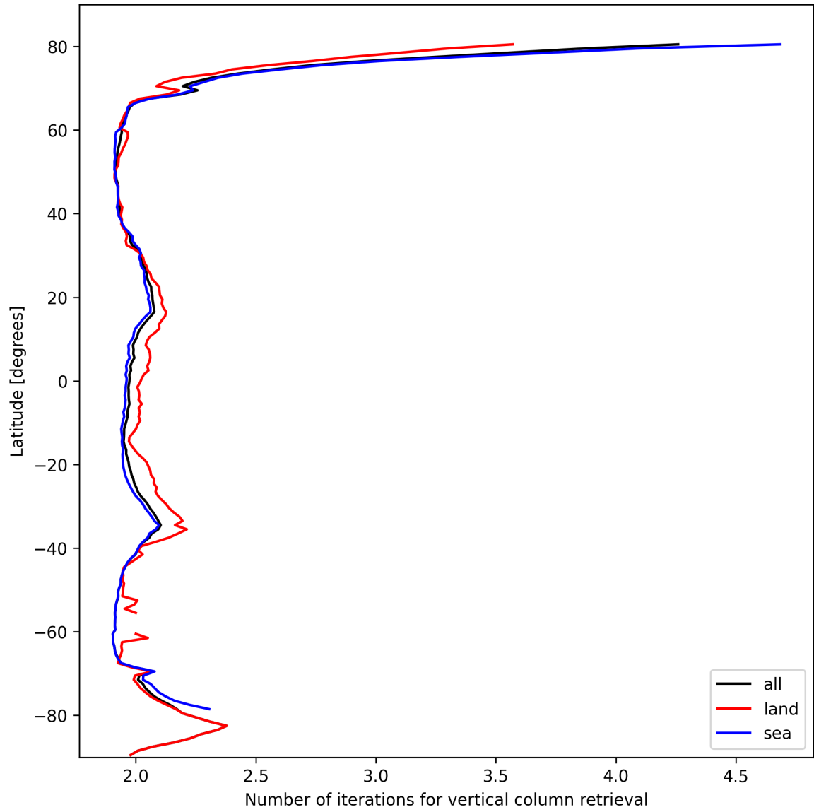
Figure 27: Zonal average of “Number of iterations for vertical column retrieval” for 2025-02-26 to 2025-02-27.
