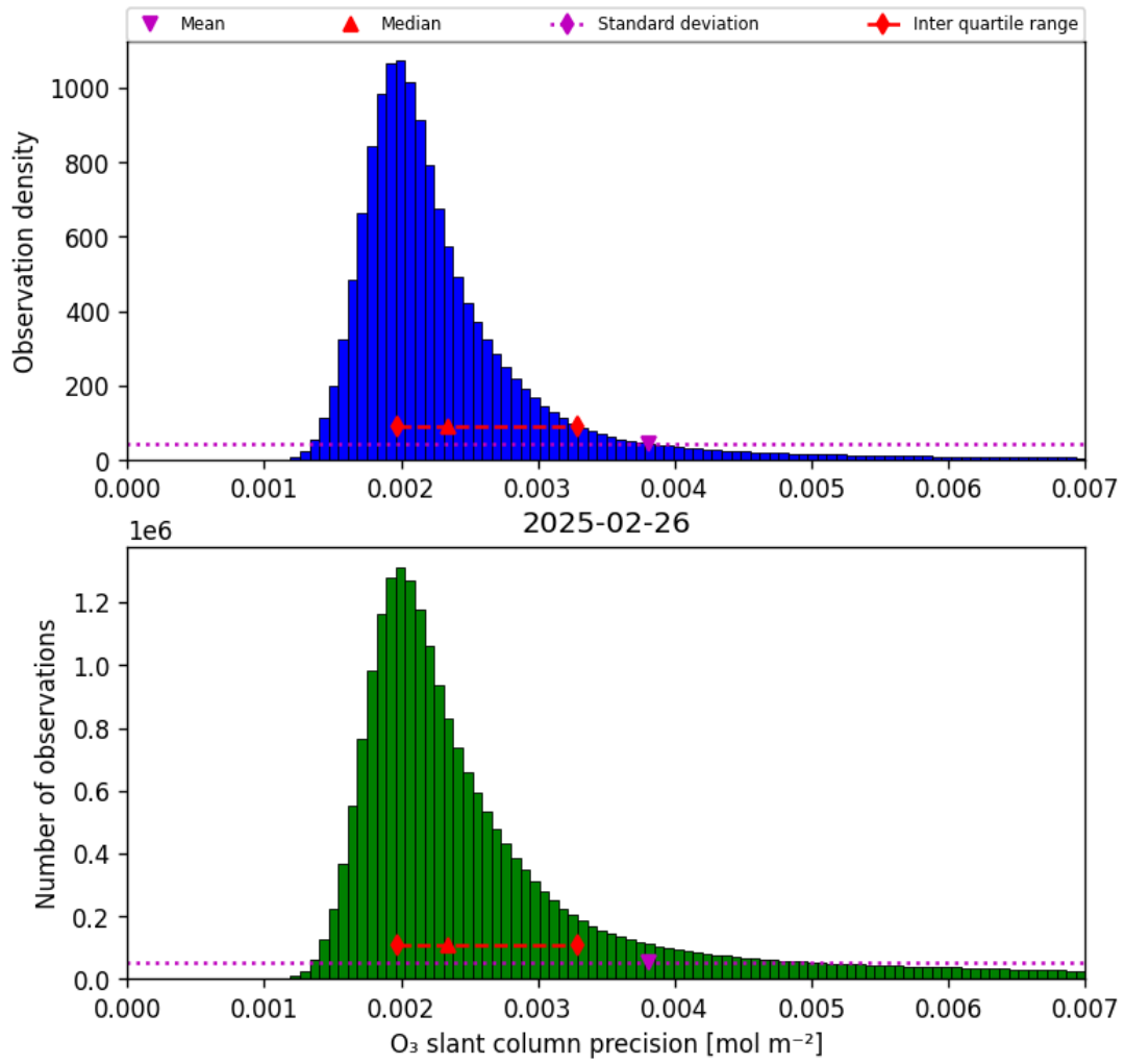
Figure 32: Histogram of “O 3 slant column precision” for 2025-02-26 to 2025-02-27
