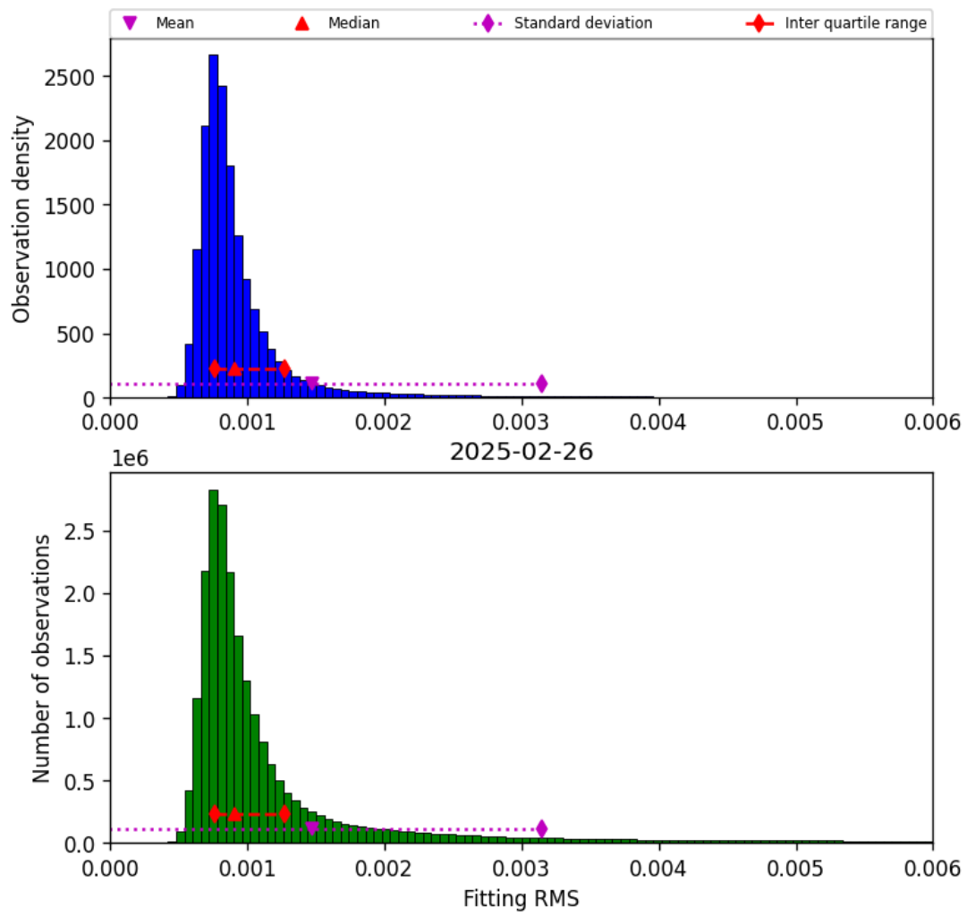
Figure 34: Histogram of “Fitting RMS” for 2025-02-26 to 2025-02-27
