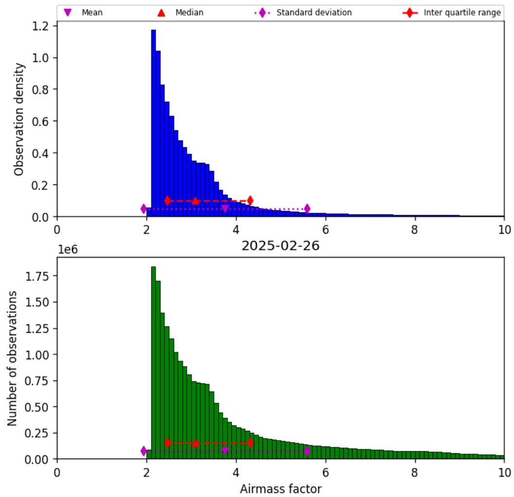
Figure 37: Histogram of “Airmass factor” for 2025-02-26 to 2025-02-27
