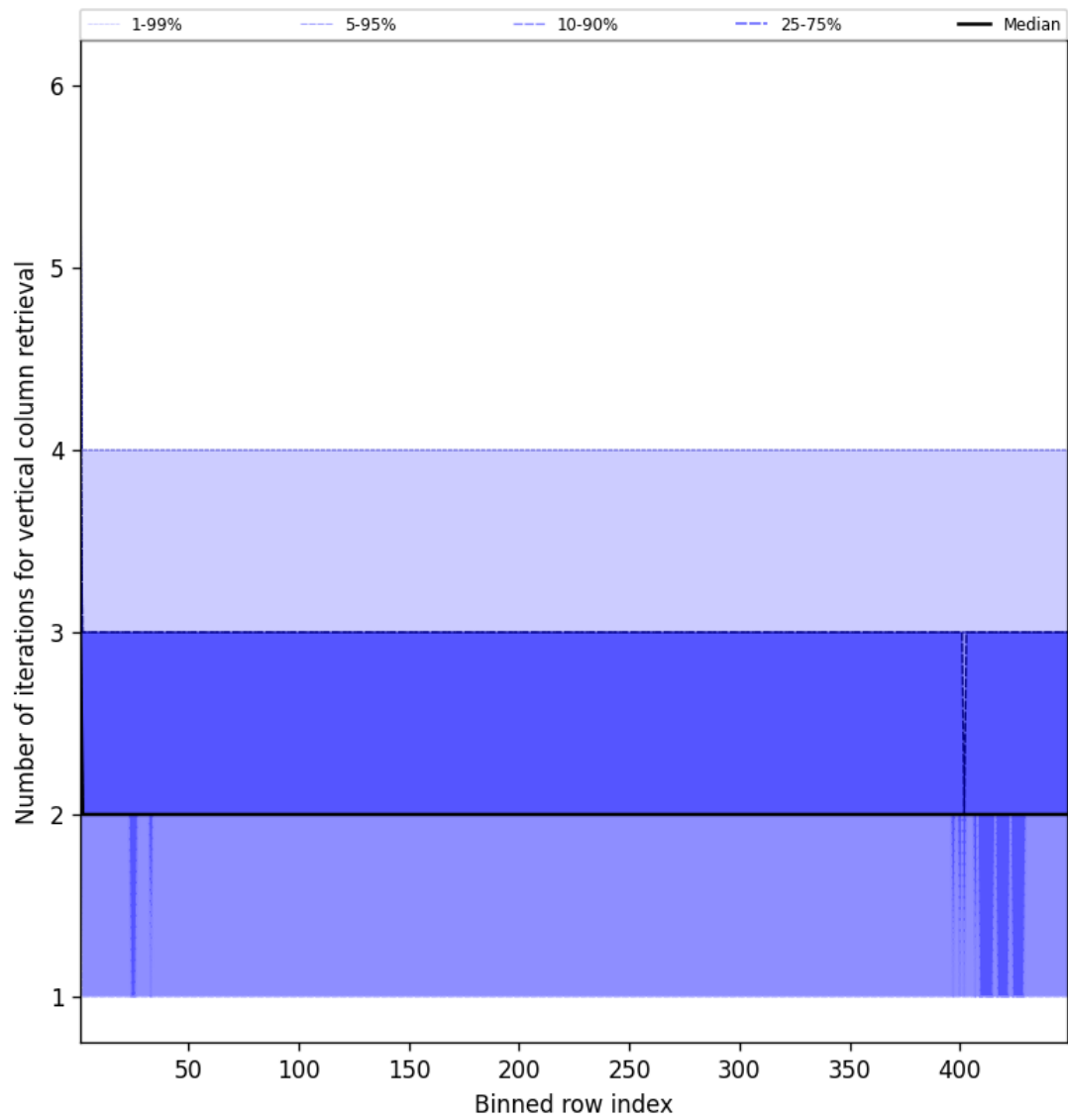
Figure 51: Along track statistics of “Number of iterations for vertical column retrieval” for 2025-02-26 to 2025-02-27
