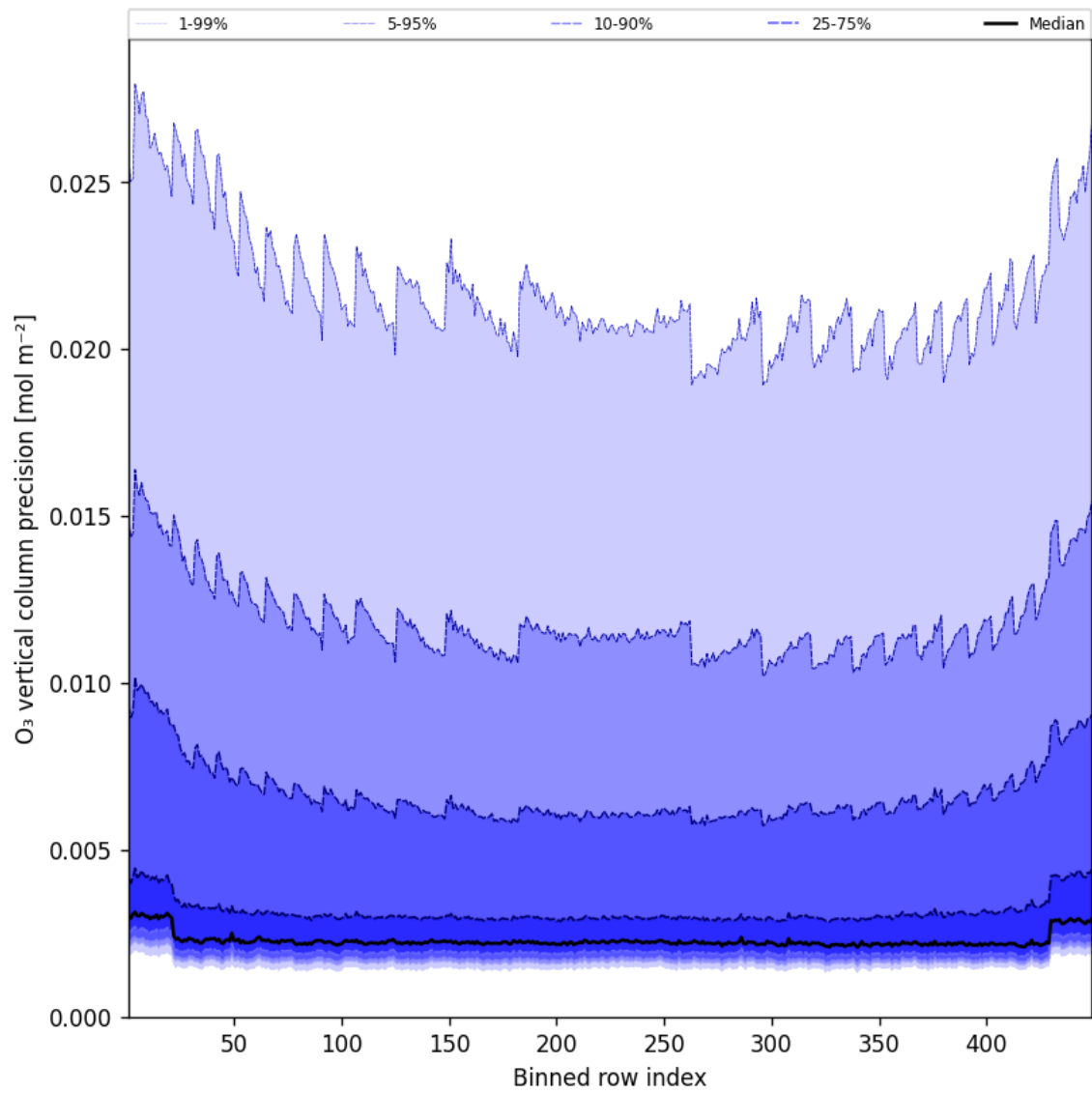
Figure 42: Along track statistics of “O 3 vertical column precision” for 2025-02-26 to 2025-02-27
