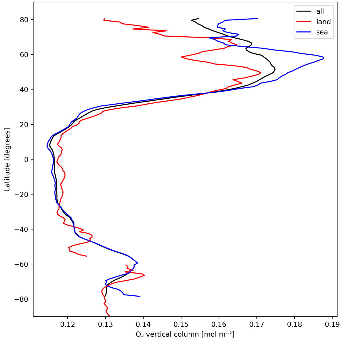
Figure 17: Zonal average of “O 3 vertical column” for 2025-02-26 to 2025-02-27.
