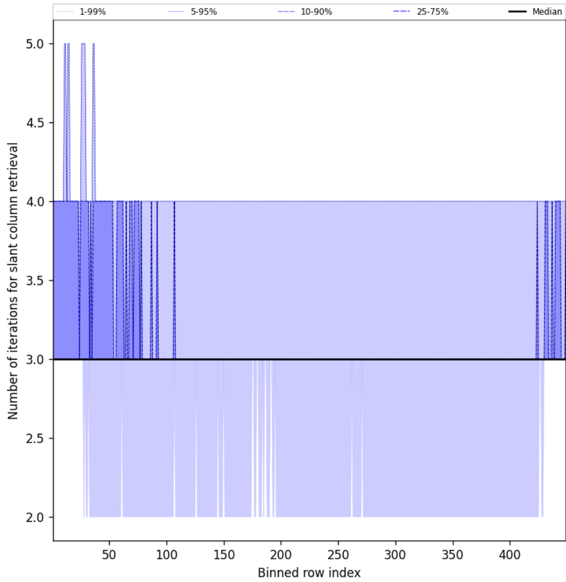
Figure 45: Along track statistics of “Number of iterations for slant column retrieval” for 2025-02-26 to 2025-02-27
