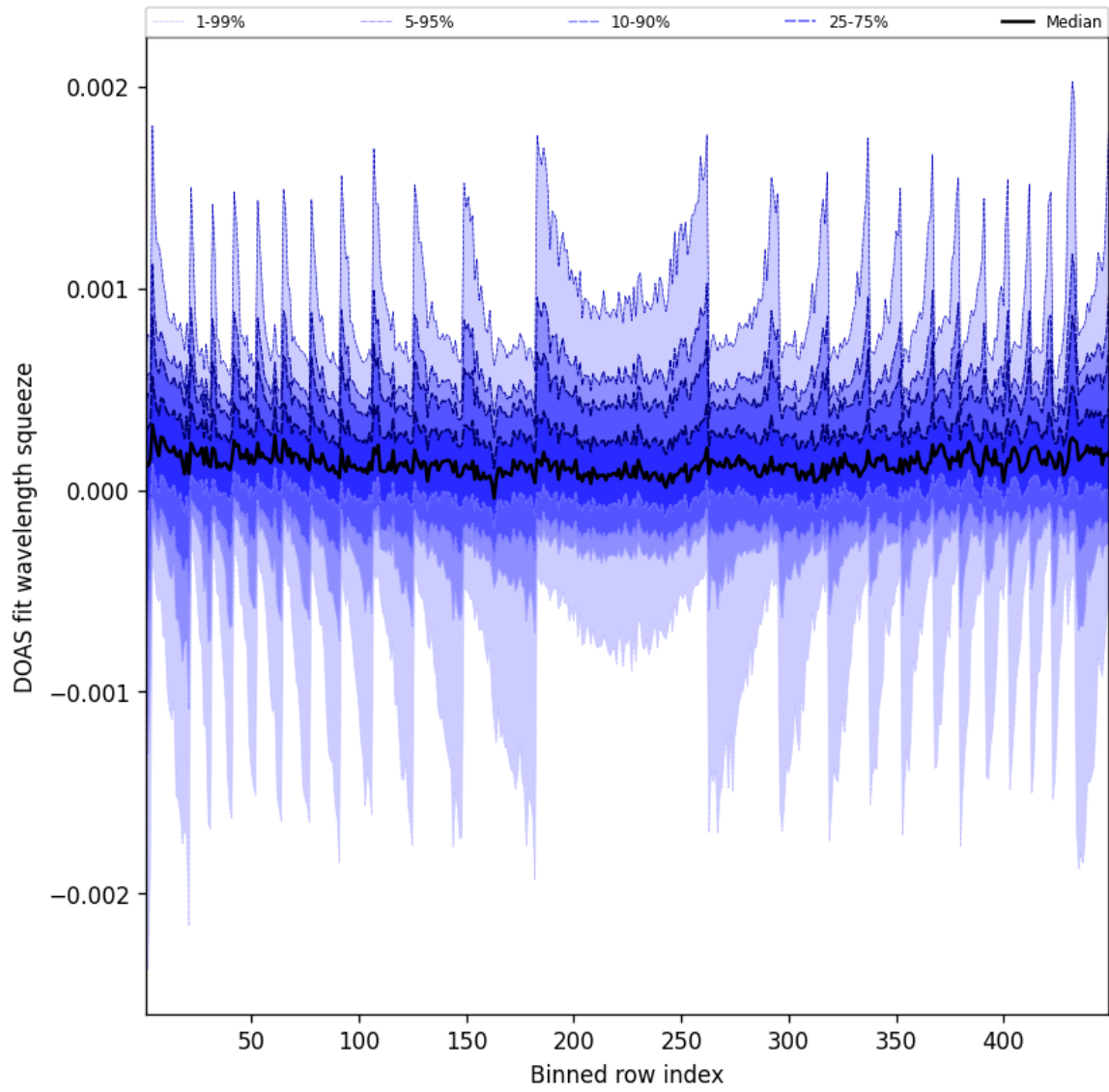
Figure 48: Along track statistics of “DOAS fit wavelength squeeze” for 2025-02-26 to 2025-02-27
