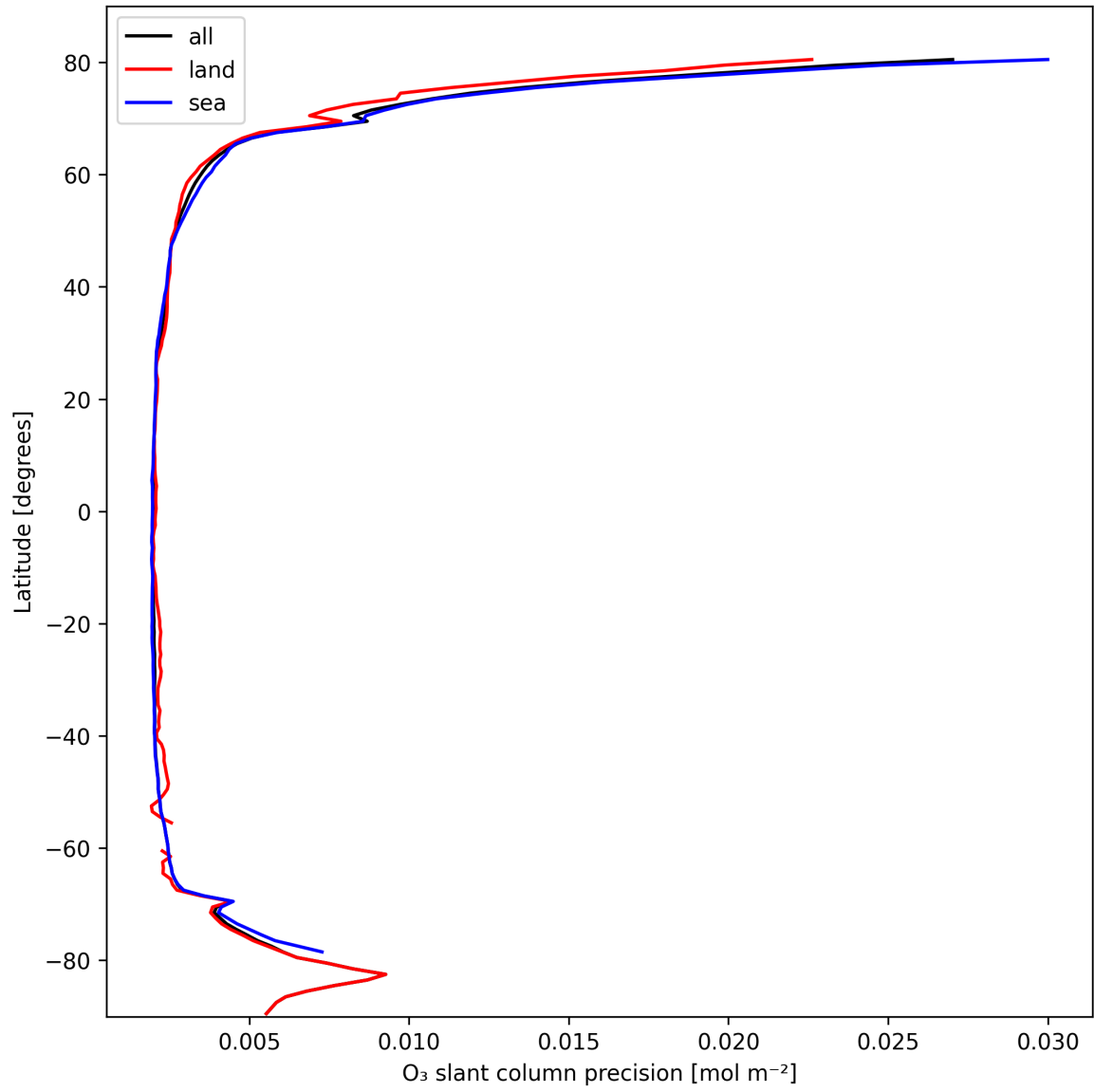
Figure 20: Zonal average of “O 3 slant column precision” for 2025-02-26 to 2025-02-27.
