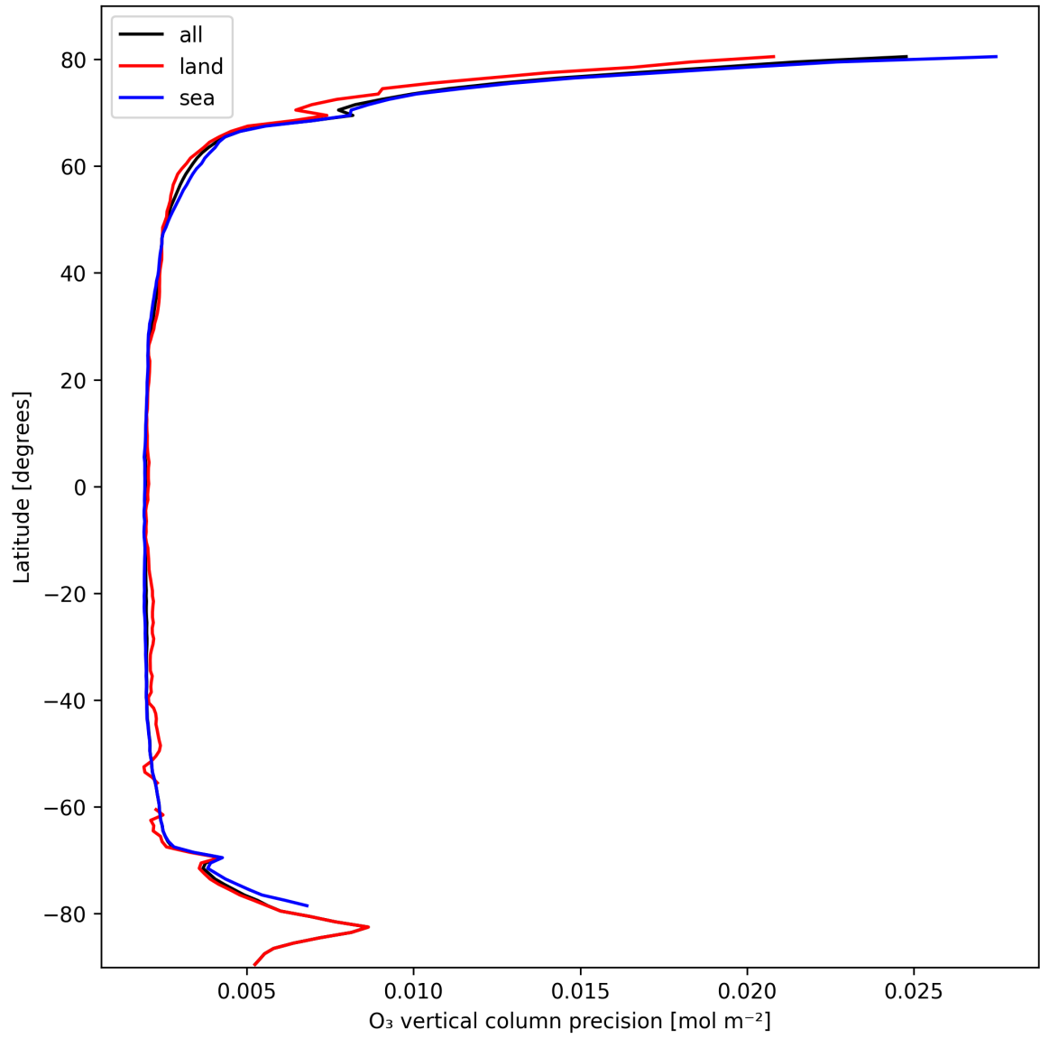
Figure 18: Zonal average of “O 3 vertical column precision” for 2025-02-26 to 2025-02-27.
