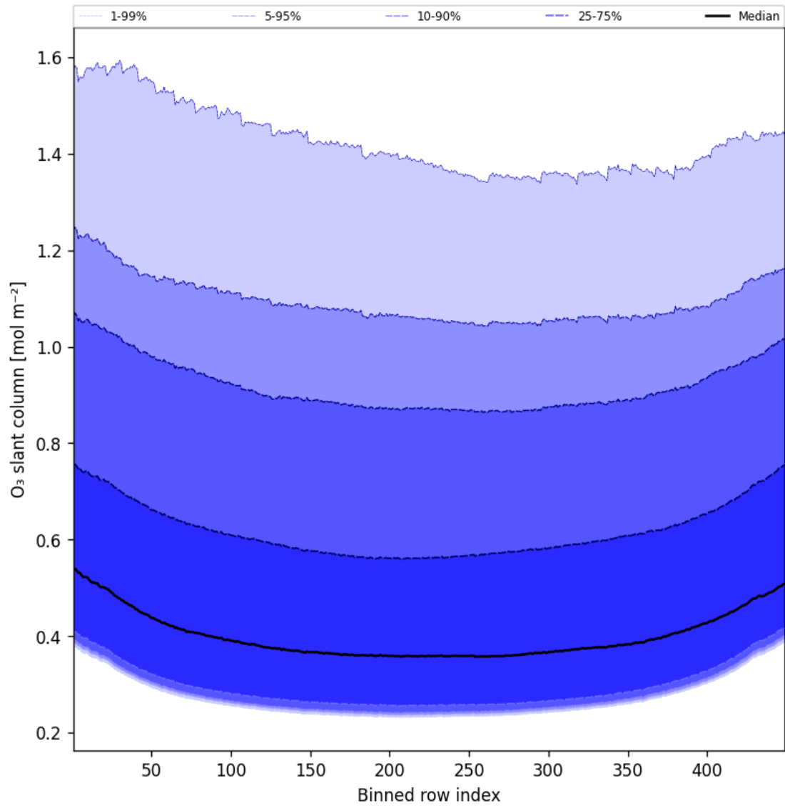
Figure 43: Along track statistics of “O 3 slant column” for 2025-02-26 to 2025-02-27
