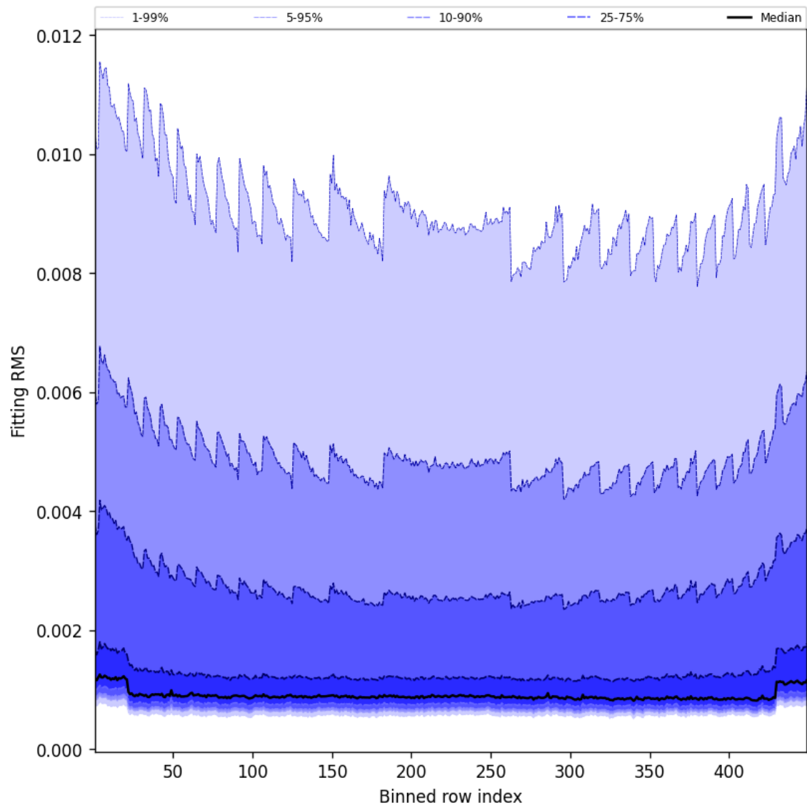
Figure 46: Along track statistics of “Fitting RMS” for 2025-02-26 to 2025-02-27
