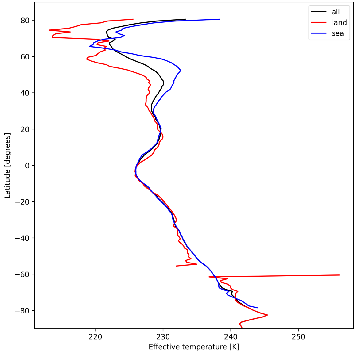
Figure 26: Zonal average of “Effective temperature” for 2025-02-26 to 2025-02-27.
