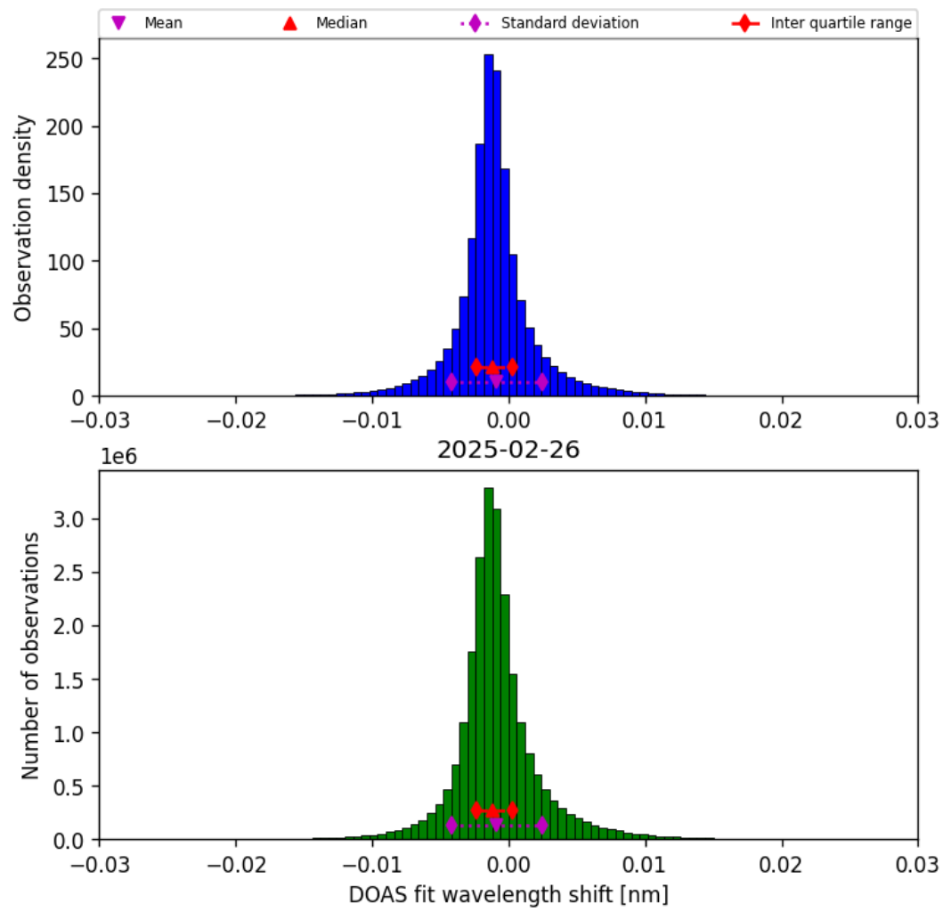
Figure 35: Histogram of “DOAS fit wavelength shift” for 2025-02-26 to 2025-02-27
