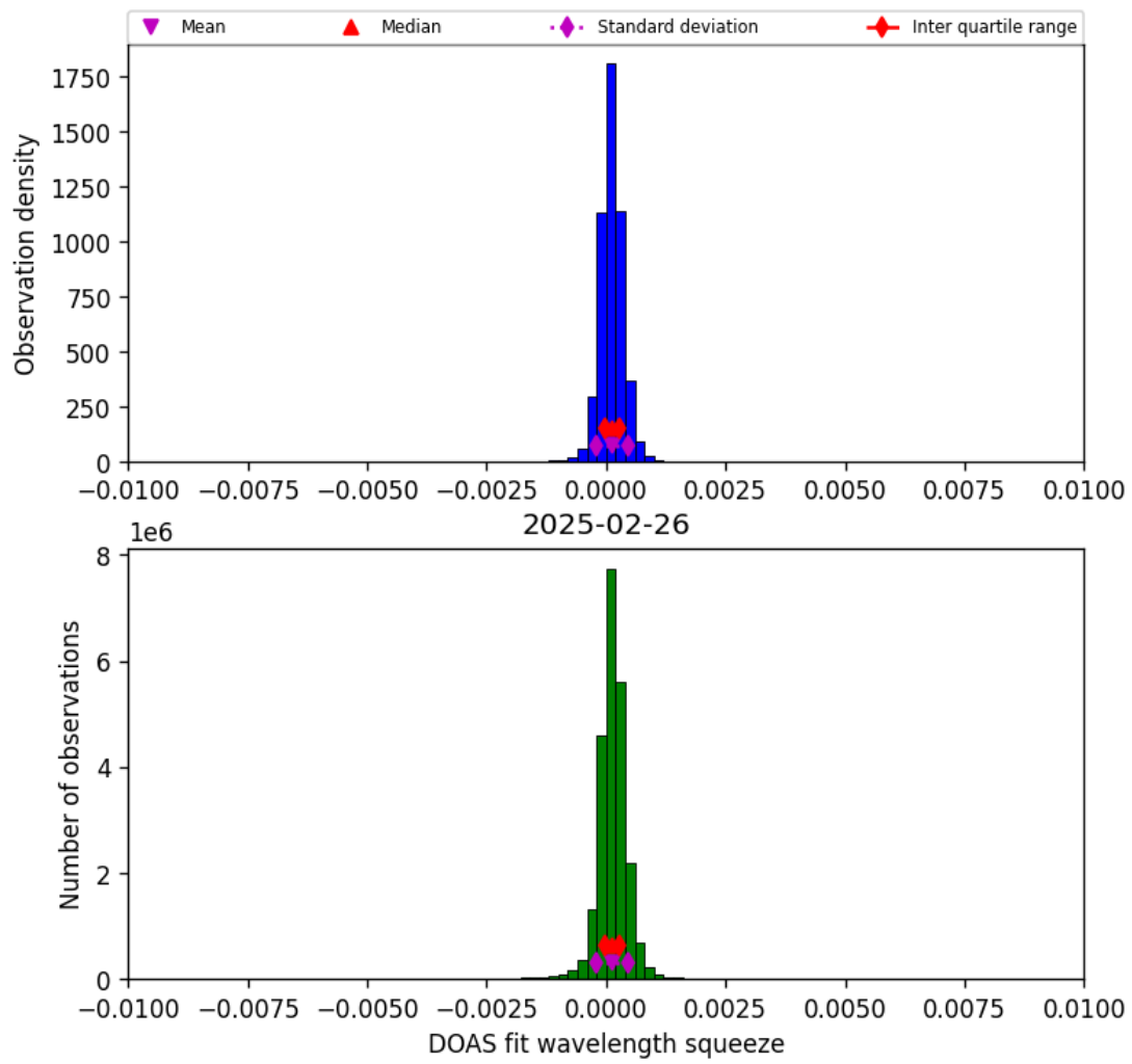
Figure 36: Histogram of “DOAS fit wavelength squeeze” for 2025-02-26 to 2025-02-27
