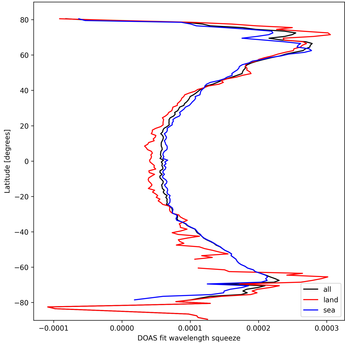
Figure 24: Zonal average of “DOAS fit wavelength squeeze” for 2025-02-26 to 2025-02-27.
