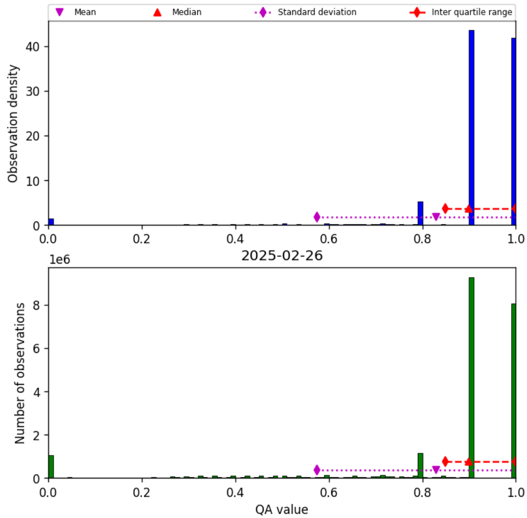
Figure 28: Histogram of “QA value” for 2025-02-26 to 2025-02-27
