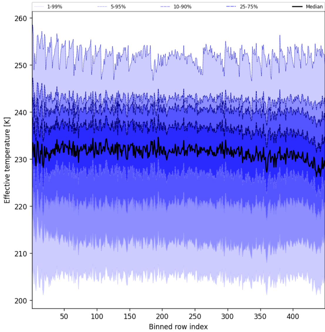
Figure 50: Along track statistics of “Effective temperature” for 2025-02-26 to 2025-02-27
