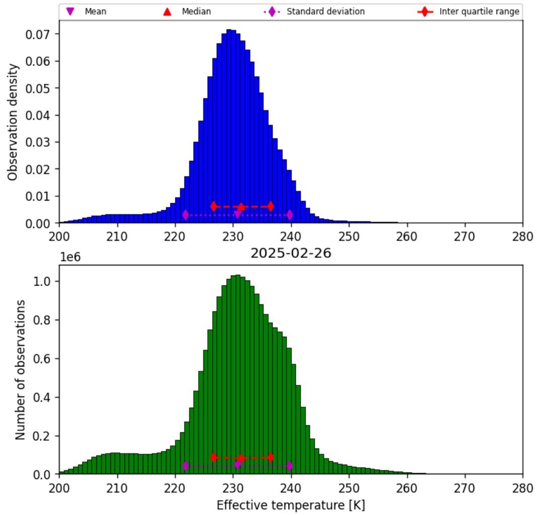
Figure 38: Histogram of “Effective temperature” for 2025-02-26 to 2025-02-27
