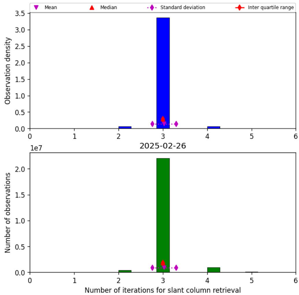
Figure 33: Histogram of "Number of iterations for slant column retrieval" for 2025-02-26 to 2025-02-27
