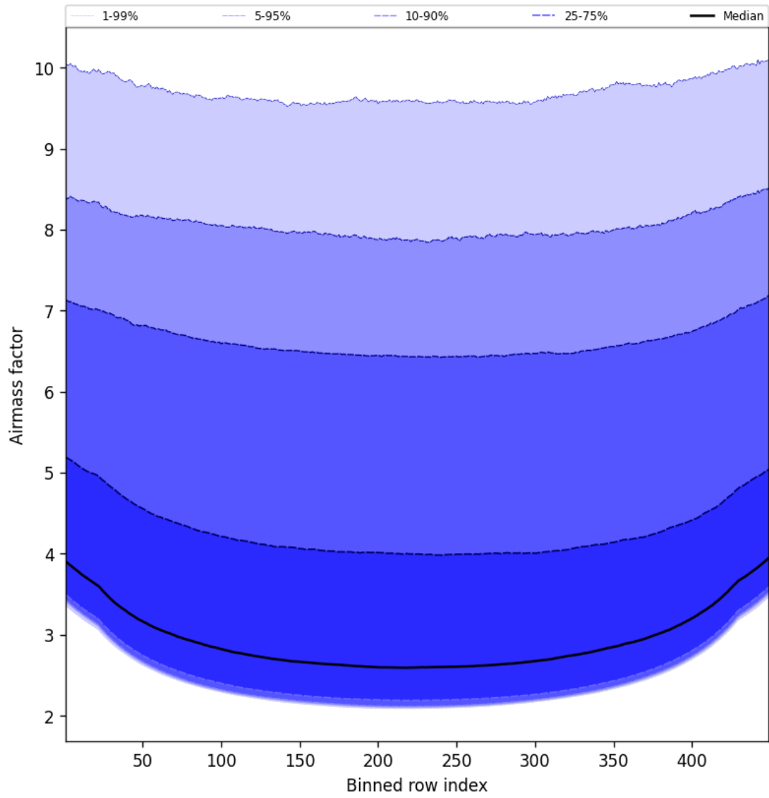
Figure 49: Along track statistics of “Airmass factor” for 2025-02-26 to 2025-02-27
