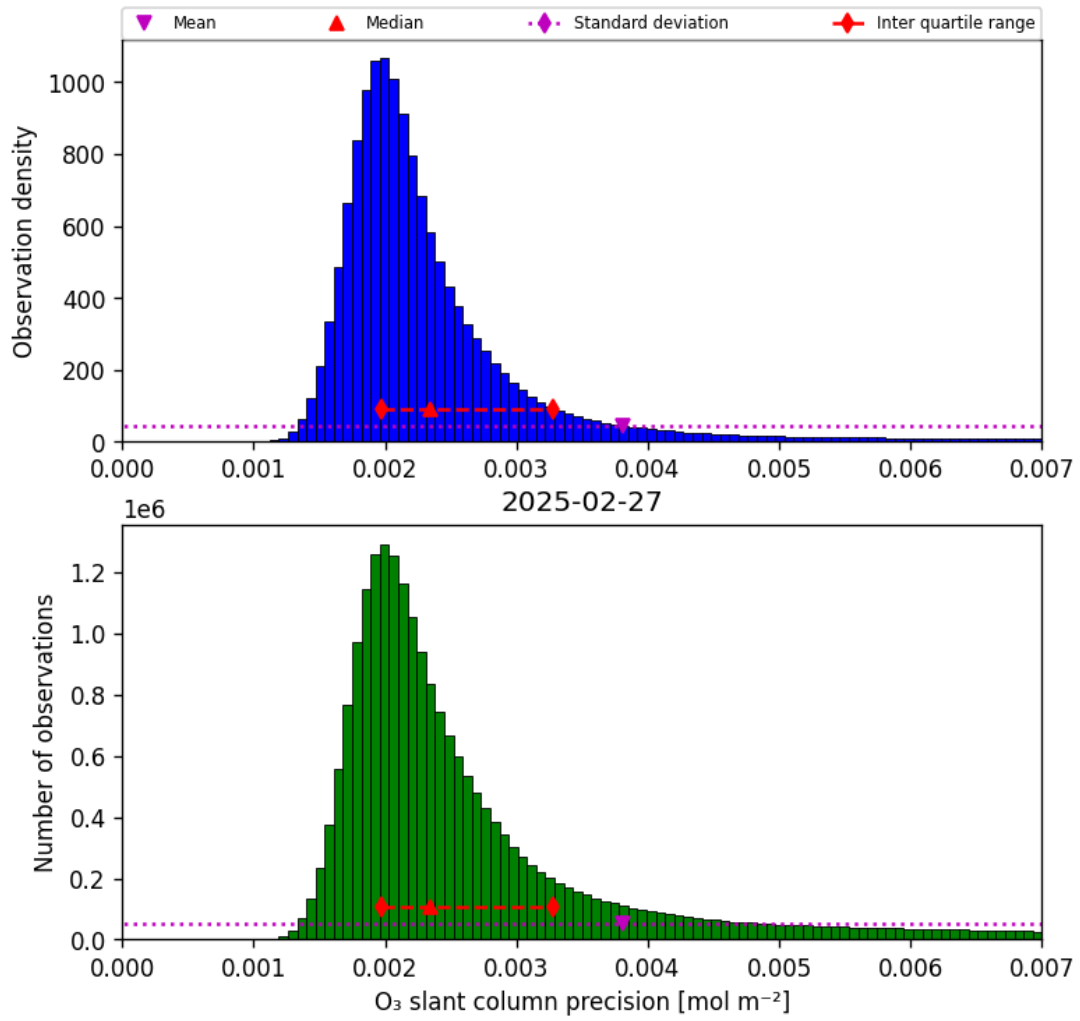
Figure 32: Histogram of “O 3 slant column precision” for 2025-02-27 to 2025-02-27
