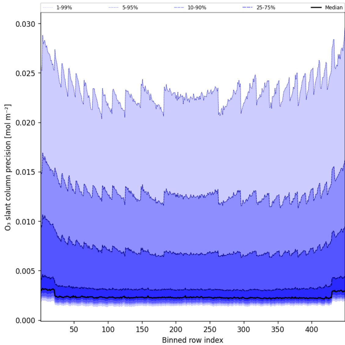
Figure 44: Along track statistics of “O 3 slant column precision” for 2025-02-27 to 2025-02-27
