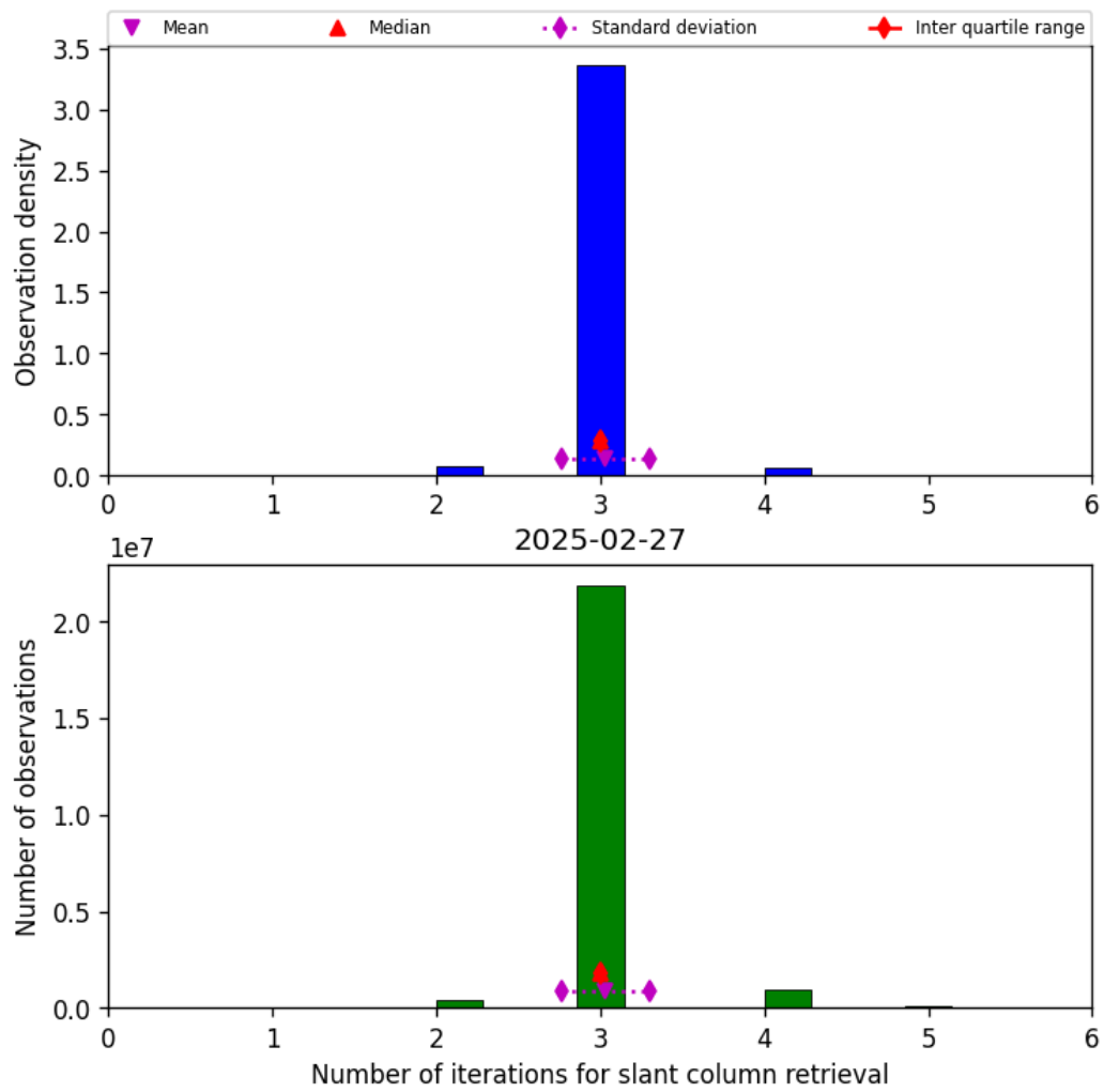
Figure 33: Histogram of “Number of iterations for slant column retrieval” for 2025-02-27 to 2025-02-27
