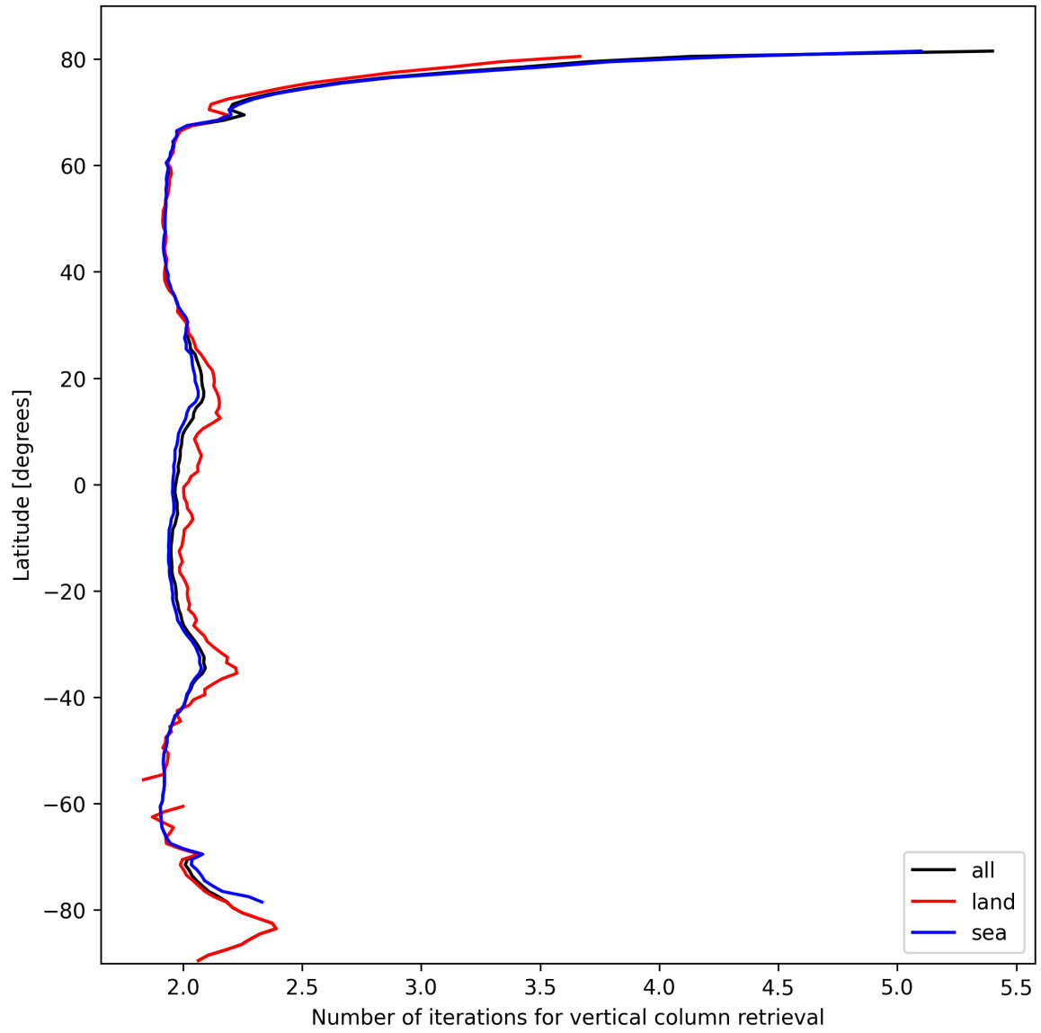
Figure 27: Zonal average of “Number of iterations for vertical column retrieval” for 2025-02-27 to 2025-02-27.
