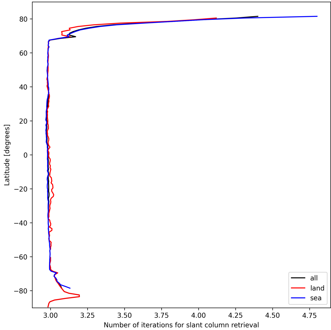
Figure 21: Zonal average of “Number of iterations for slant column retrieval” for 2025-02-27 to 2025-02-27.
