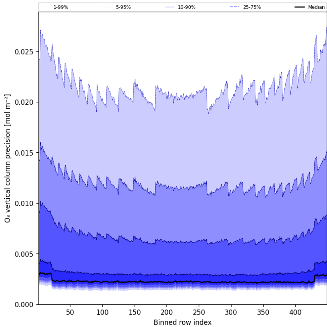
Figure 42: Along track statistics of “O 3 vertical column precision” for 2025-02-27 to 2025-02-27
