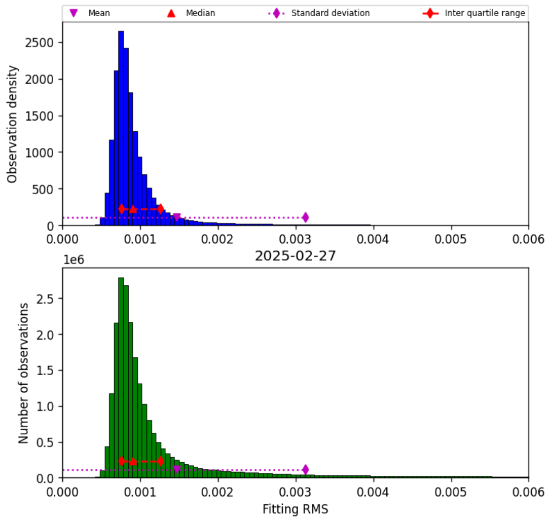
Figure 34: Histogram of “Fitting RMS” for 2025-02-27 to 2025-02-27
