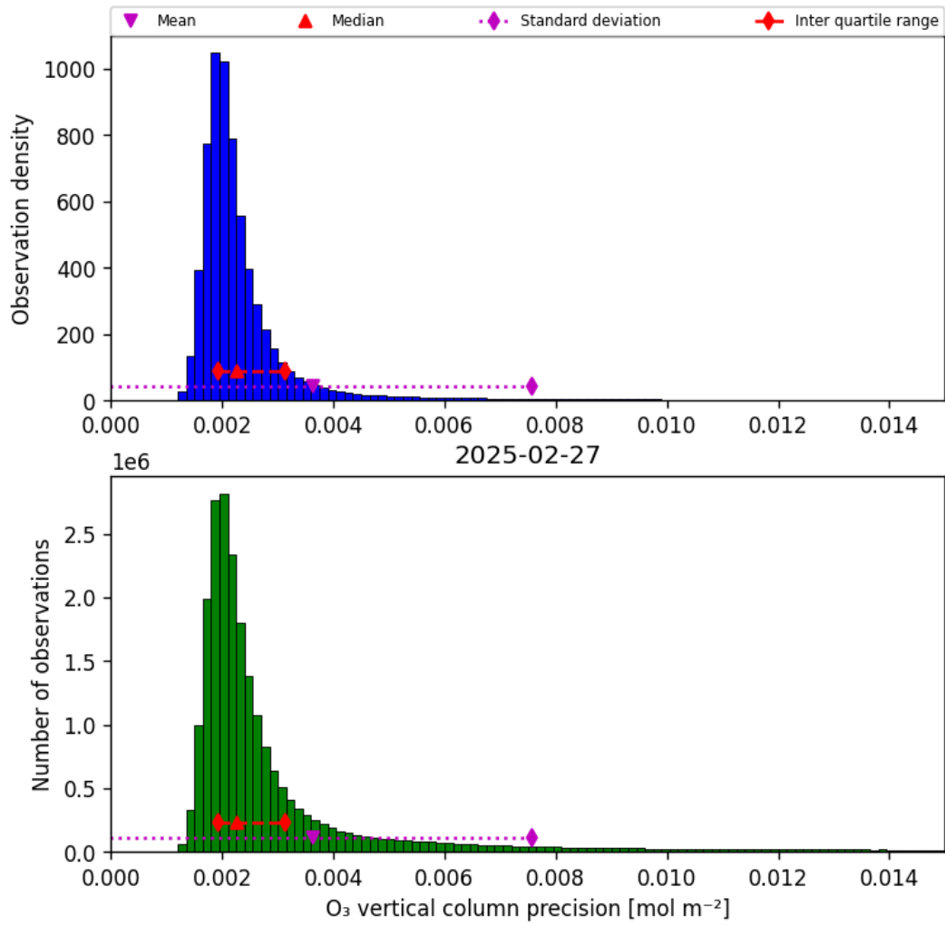
Figure 30: Histogram of “O 3 vertical column precision” for 2025-02-27 to 2025-02-27
