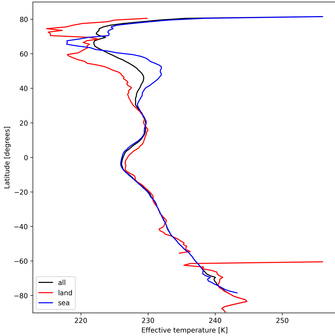
Figure 26: Zonal average of “Effective temperature” for 2025-02-27 to 2025-02-27.
