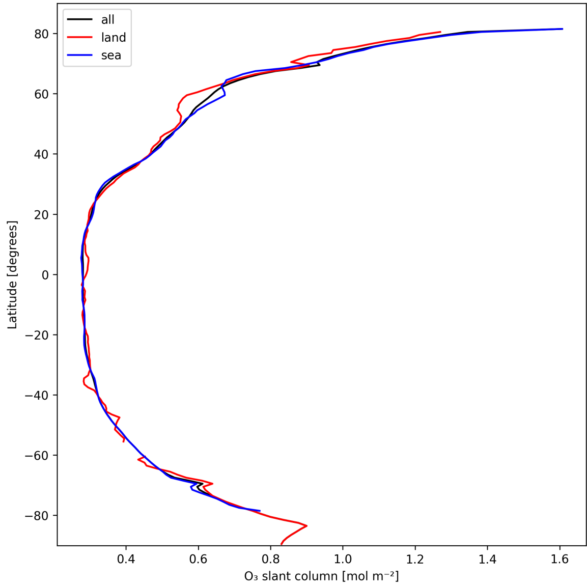
Figure 19: Zonal average of “O 3 slant column” for 2025-02-27 to 2025-02-27.
