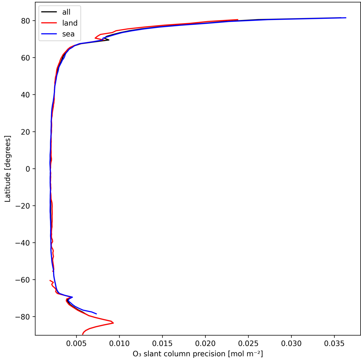
Figure 20: Zonal average of “O 3 slant column precision” for 2025-02-27 to 2025-02-27.
