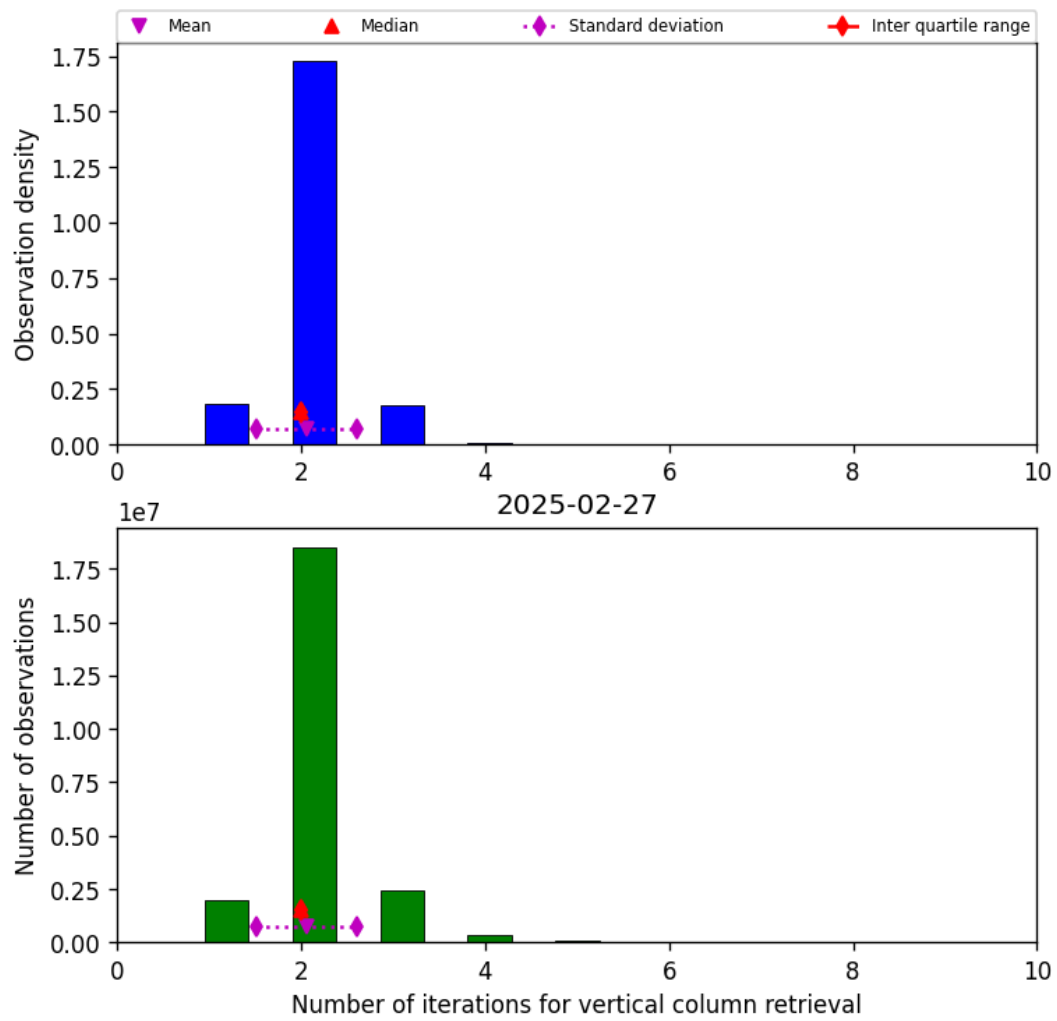
Figure 39: Histogram of “Number of iterations for vertical column retrieval” for 2025-02-27 to 2025-02-27
