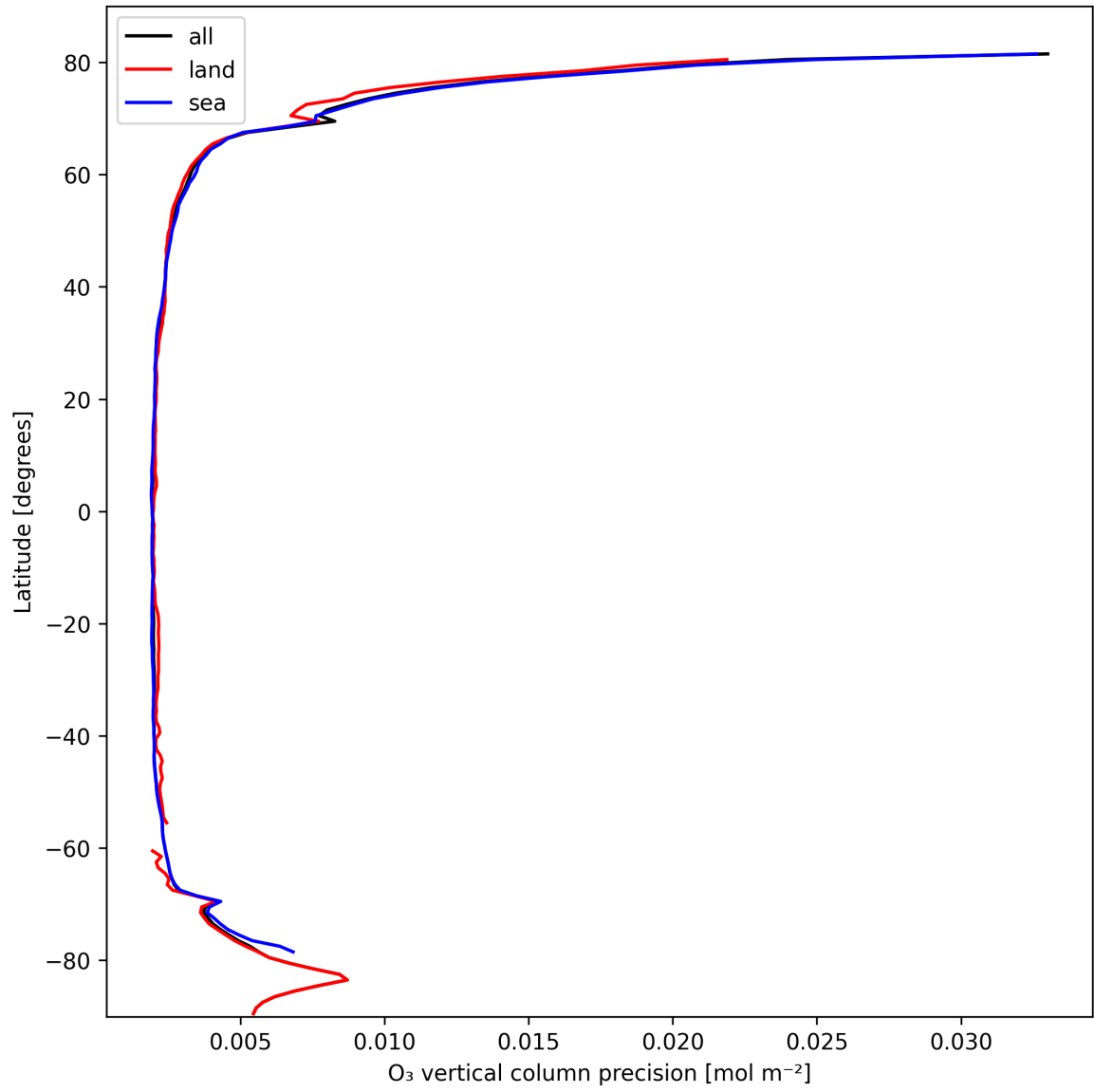
Figure 18: Zonal average of “O 3 vertical column precision” for 2025-02-27 to 2025-02-27.
