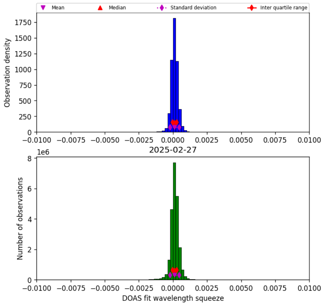
Figure 36: Histogram of “DOAS fit wavelength squeeze” for 2025-02-27 to 2025-02-27
