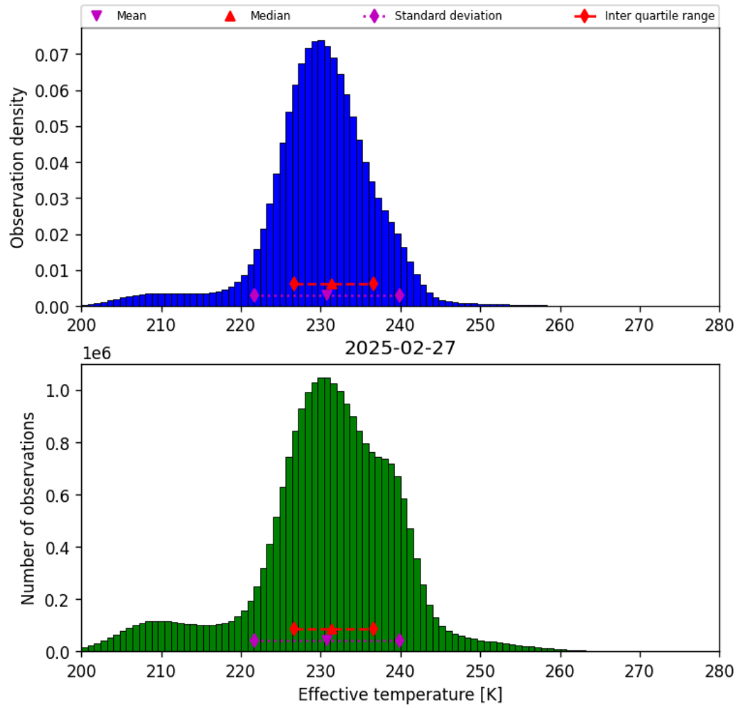
Figure 38: Histogram of “Effective temperature” for 2025-02-27 to 2025-02-27
