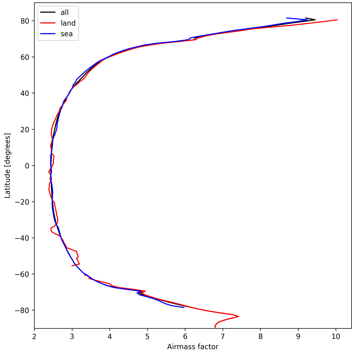
Figure 25: Zonal average of “Airmass factor” for 2025-02-27 to 2025-02-27.
