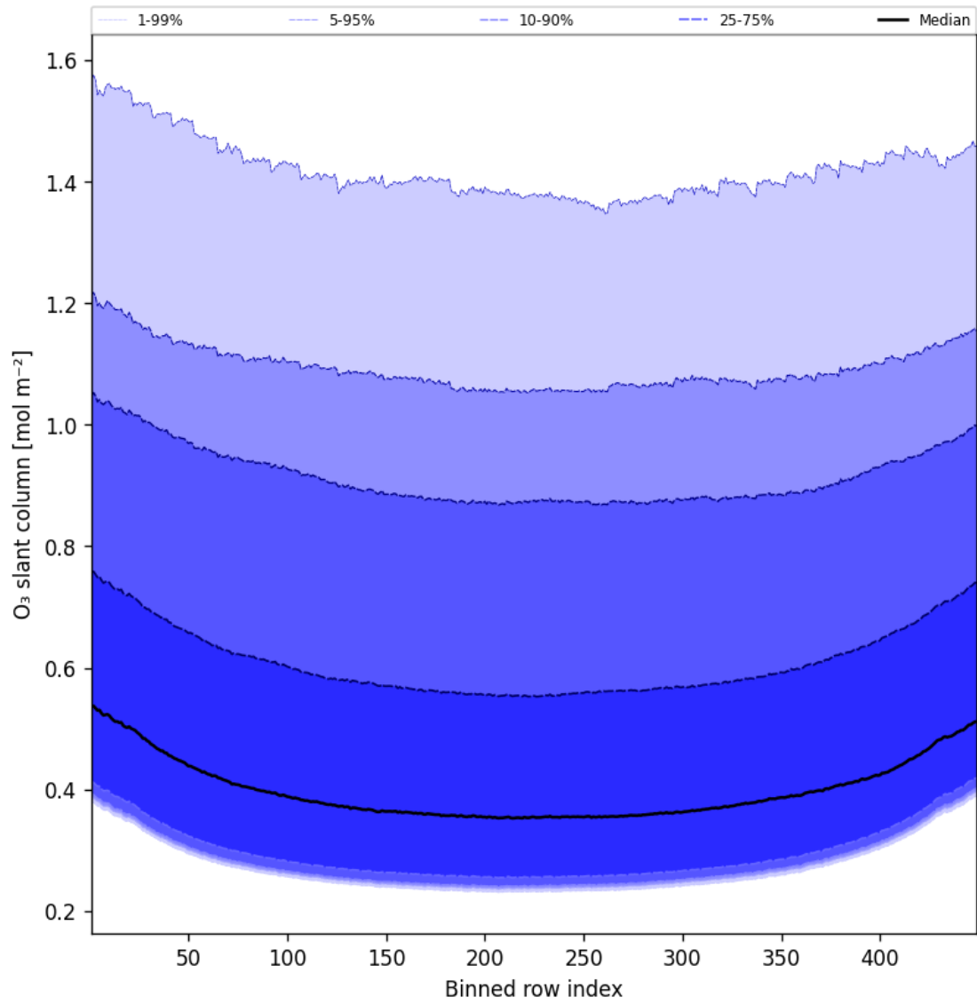
Figure 43: Along track statistics of “O 3 slant column” for 2025-02-27 to 2025-02-27
