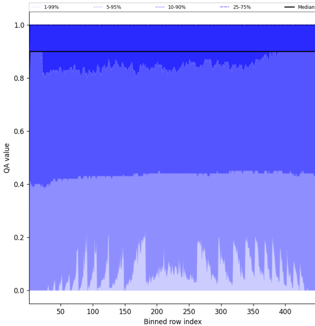
Figure 40: Along track statistics of “QA value” for 2025-02-27 to 2025-02-27
