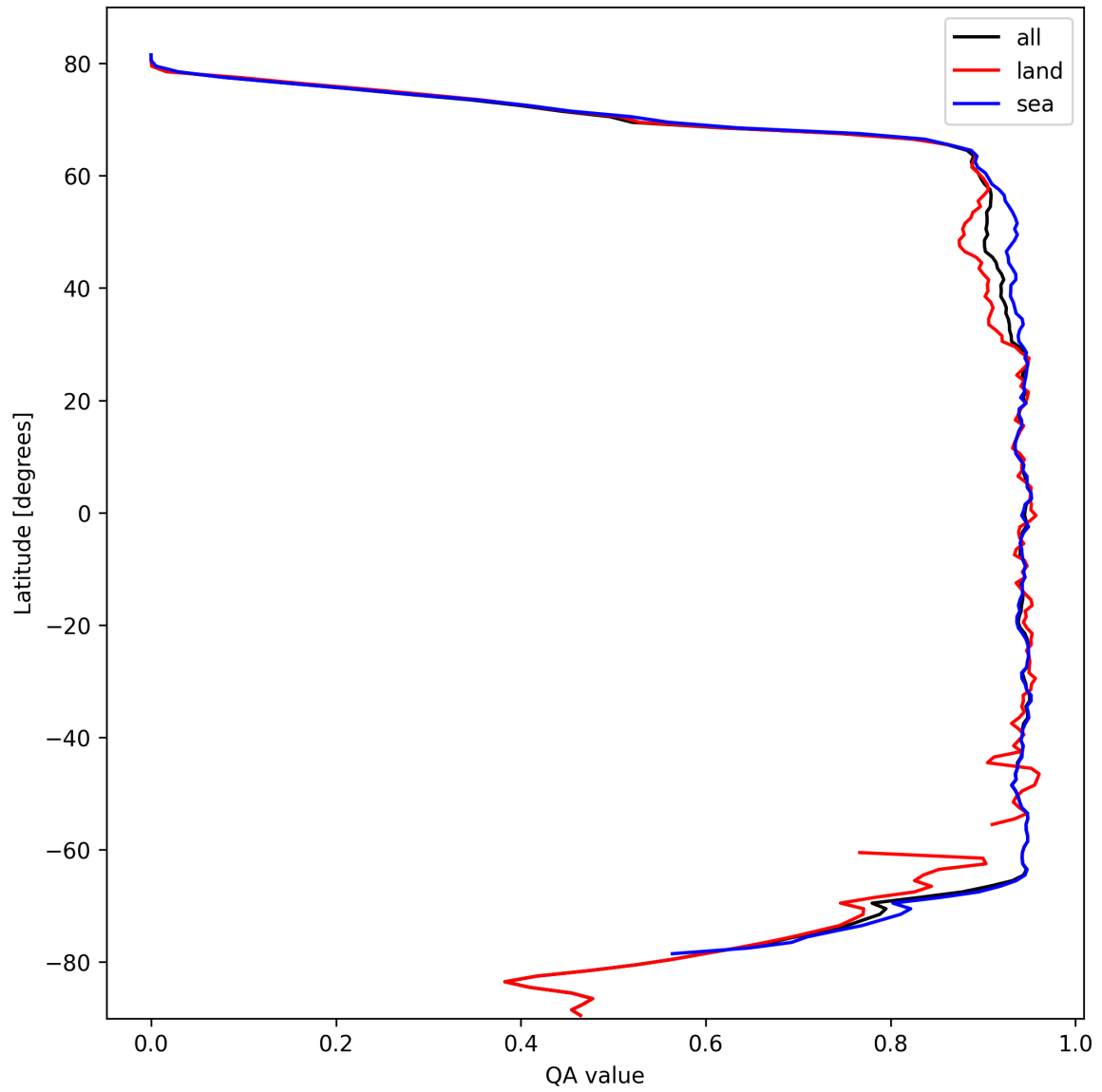
Figure 16: Zonal average of “QA value” for 2025-02-27 to 2025-02-27.
