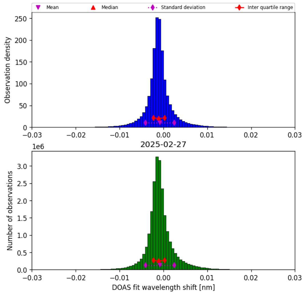
Figure 35: Histogram of “DOAS fit wavelength shift” for 2025-02-27 to 2025-02-27
