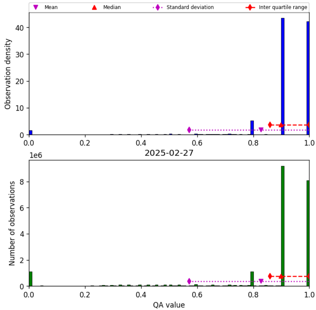
Figure 28: Histogram of “QA value” for 2025-02-27 to 2025-02-27
