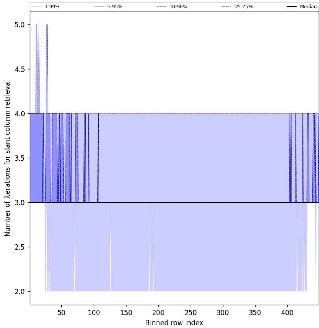
Figure 45: Along track statistics of “Number of iterations for slant column retrieval” for 2025-02-27 to 2025-02-27
