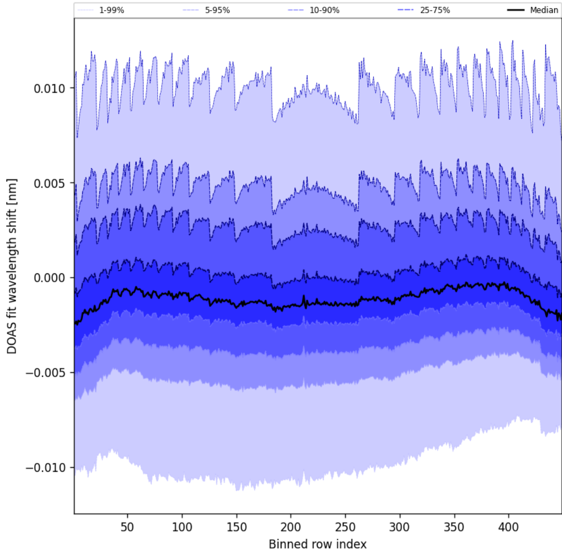
Figure 47: Along track statistics of "DOAS fit wavelength shift" for 2025-02-27 to 2025-02-27
