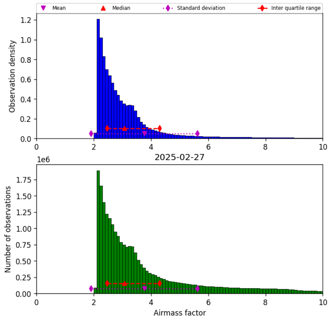
Figure 37: Histogram of “Airmass factor” for 2025-02-27 to 2025-02-27
