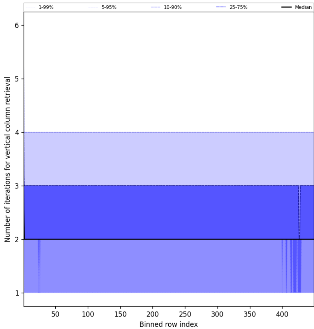
Figure 51: Along track statistics of “Number of iterations for vertical column retrieval” for 2025-02-27 to 2025-02-27
