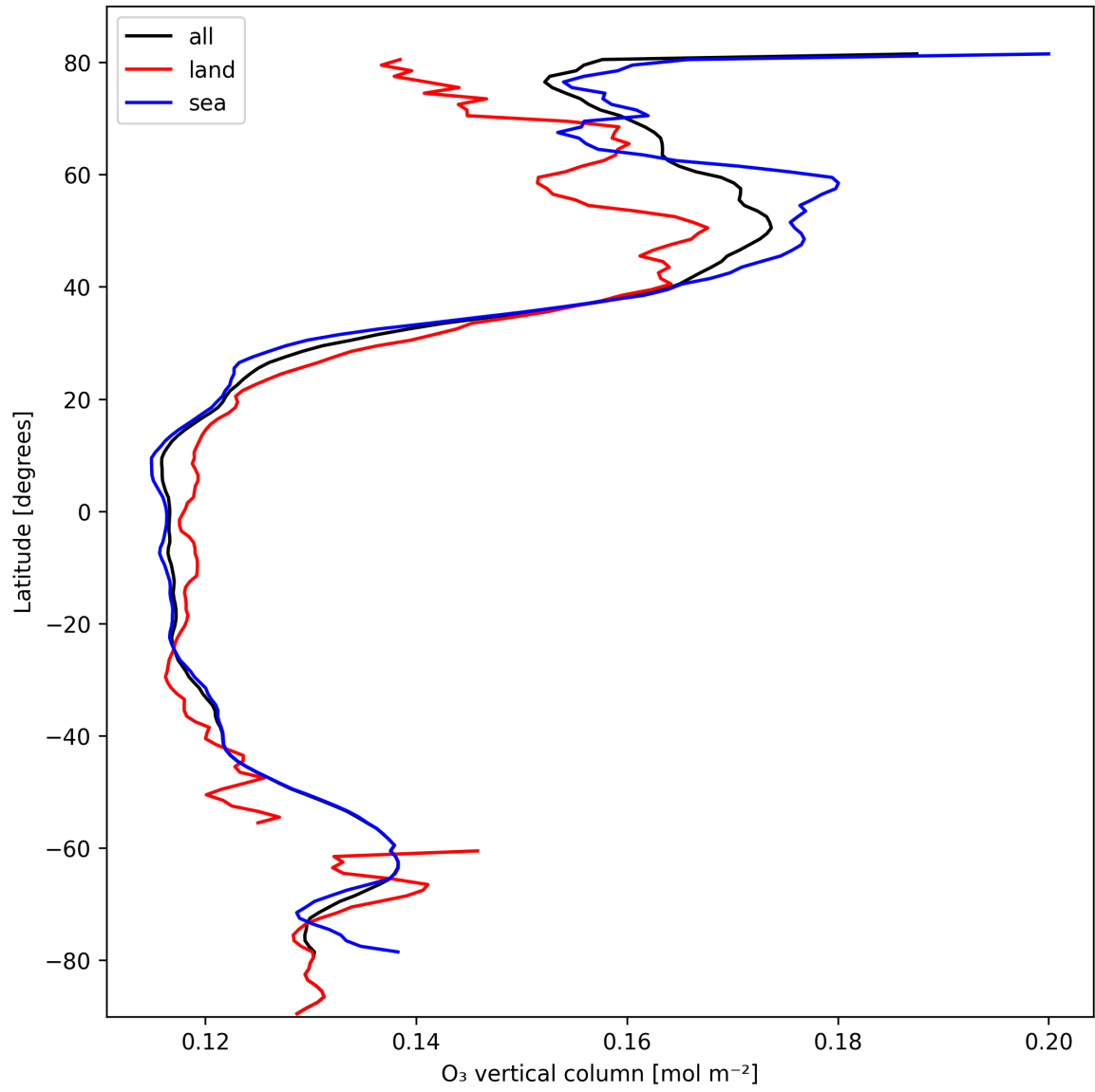
Figure 17: Zonal average of “O 3 vertical column” for 2025-02-27 to 2025-02-27.
