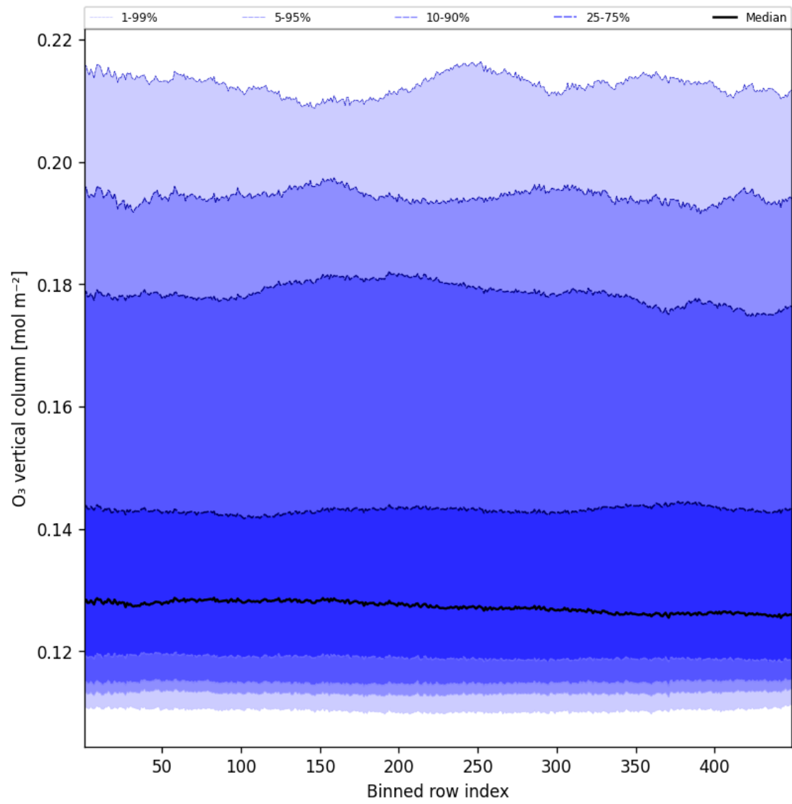
Figure 41: Along track statistics of “O 3 vertical column” for 2025-02-27 to 2025-02-27
