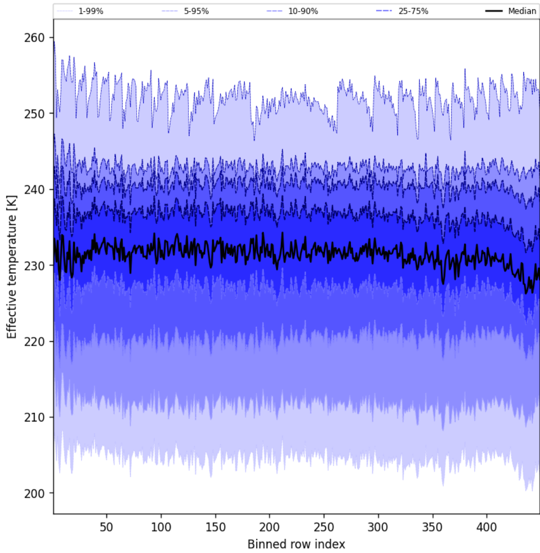
Figure 50: Along track statistics of “Effective temperature” for 2025-02-27 to 2025-02-27
