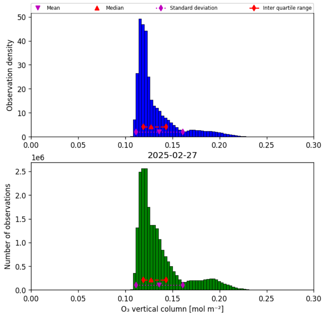
Figure 29: Histogram of “O 3 vertical column” for 2025-02-27 to 2025-02-27
