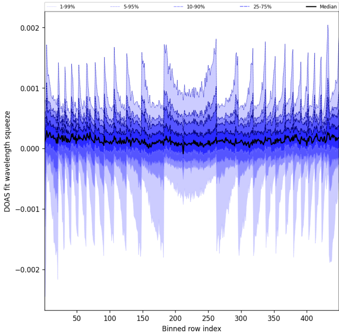
Figure 48: Along track statistics of “DOAS fit wavelength squeeze” for 2025-02-27 to 2025-02-27
