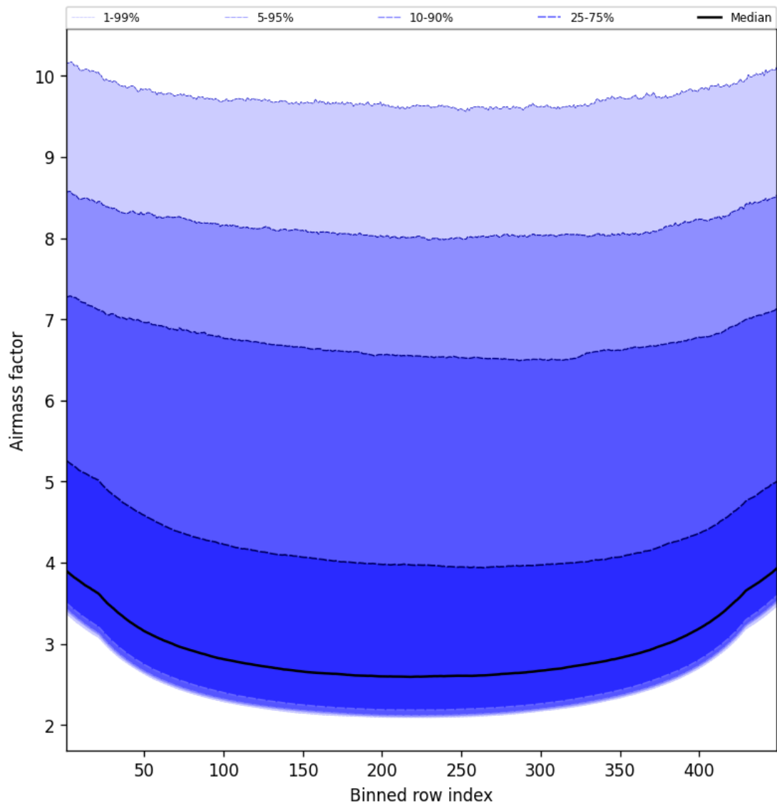
Figure 49: Along track statistics of “Airmass factor” for 2025-02-27 to 2025-02-27
