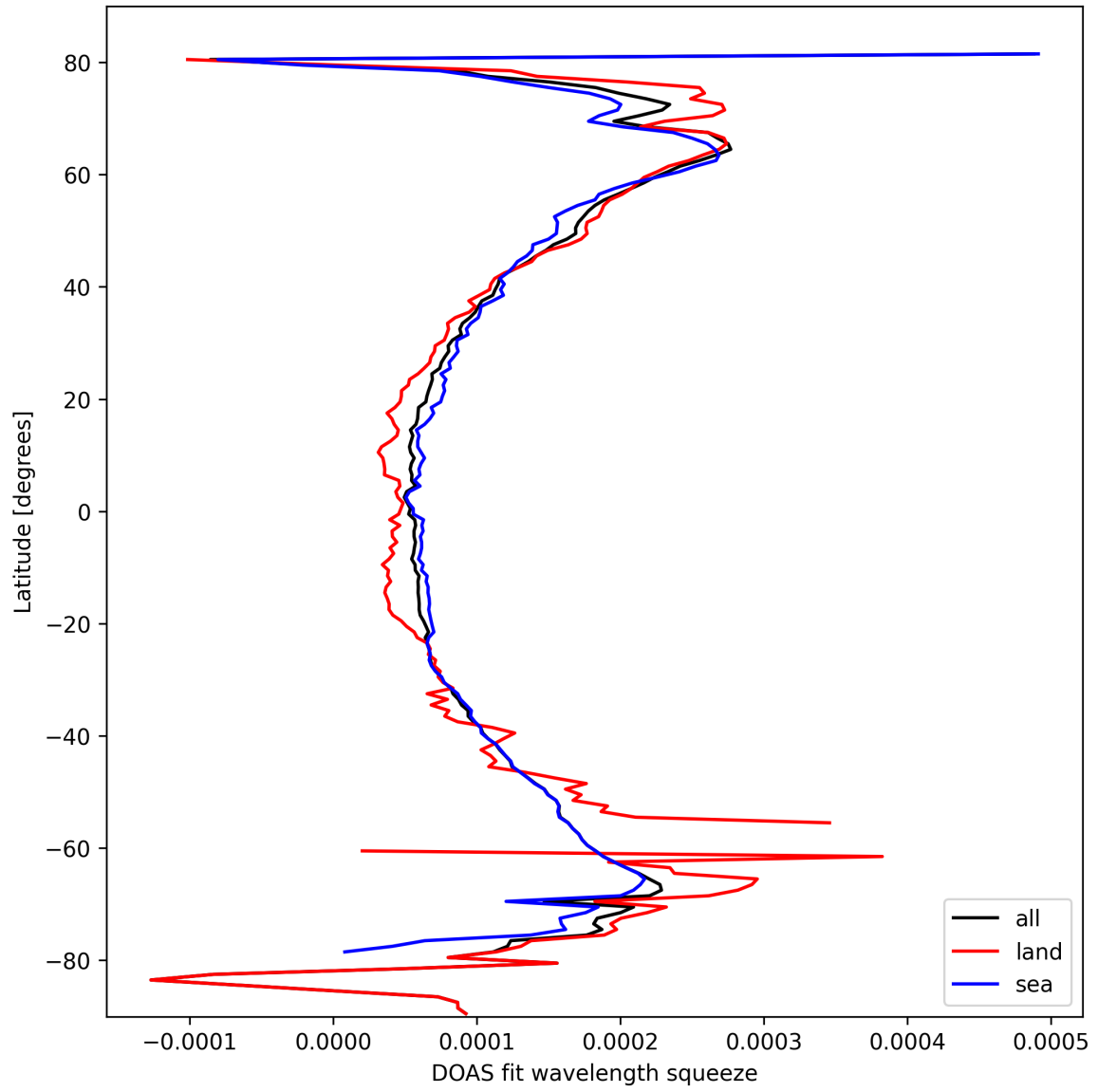
Figure 24: Zonal average of “DOAS fit wavelength squeeze” for 2025-02-27 to 2025-02-27.
