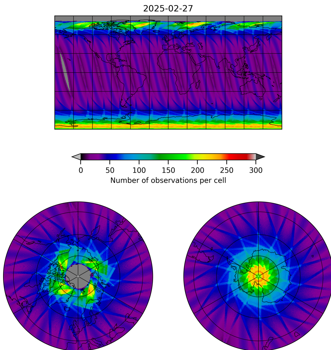
Figure 15: Map of the number of observations for 2025-02-27 to 2025-02-27
