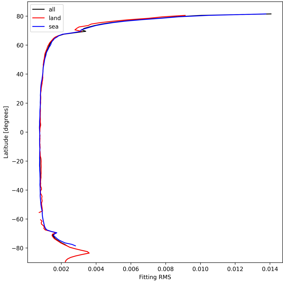
Figure 22: Zonal average of “Fitting RMS” for 2025-02-27 to 2025-02-27.
