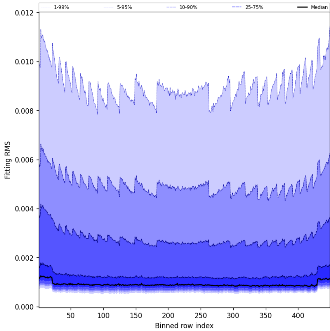
Figure 46: Along track statistics of “Fitting RMS” for 2025-02-27 to 2025-02-27
