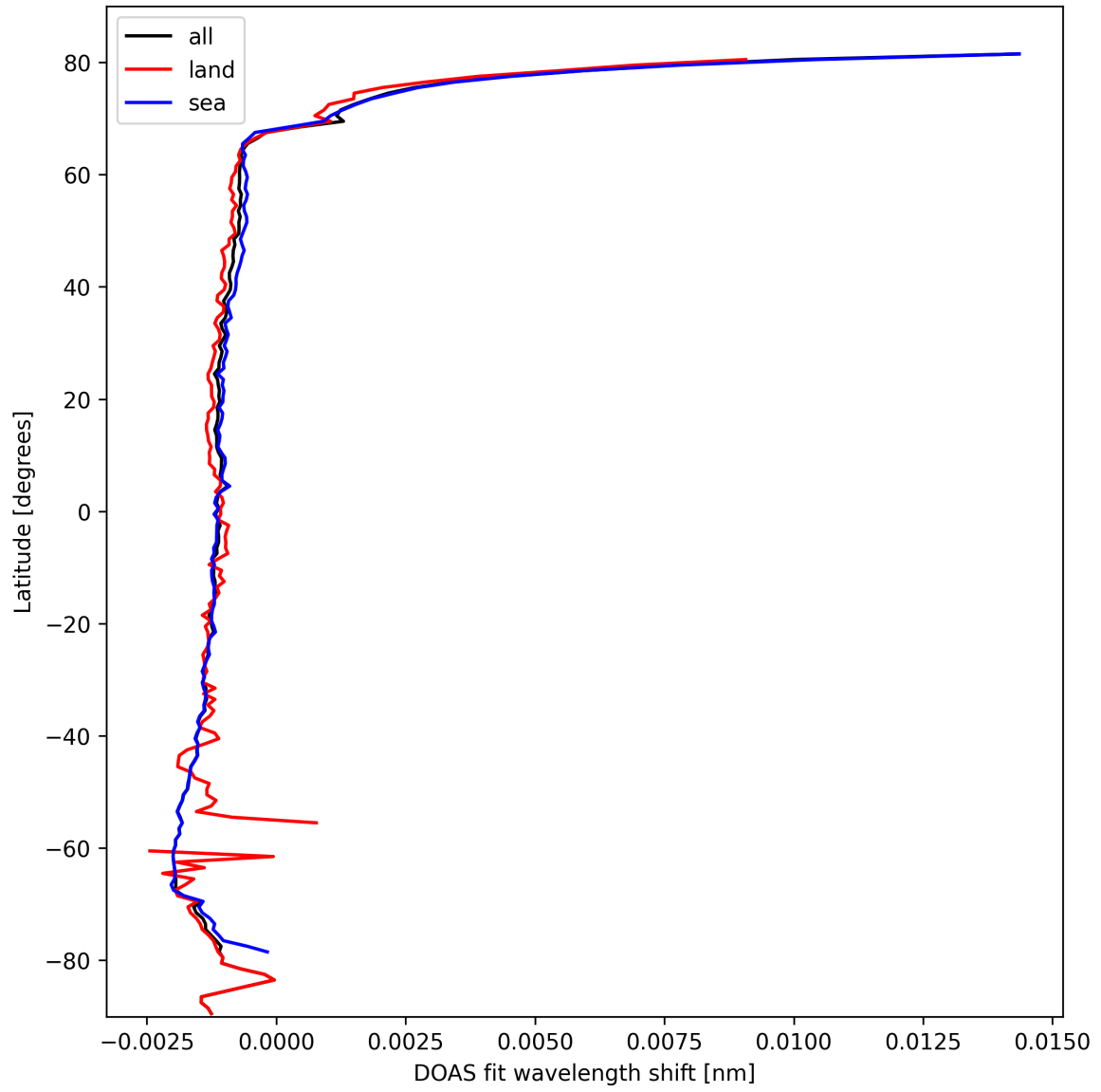
Figure 23: Zonal average of “DOAS fit wavelength shift” for 2025-02-27 to 2025-02-27.
