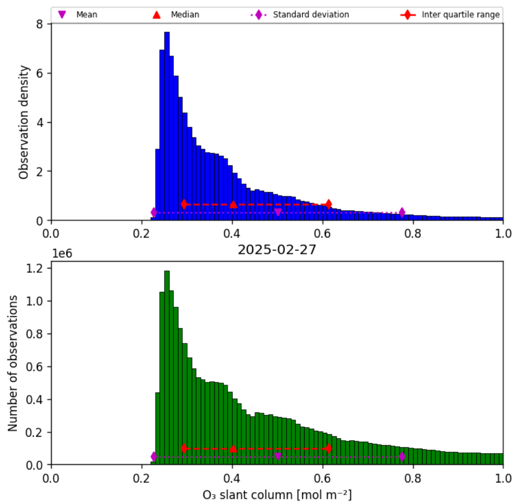
Figure 31: Histogram of “O 3 slant column” for 2025-02-27 to 2025-02-27
