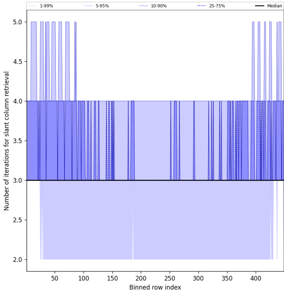
Figure 45: Along track statistics of “Number of iterations for slant column retrieval” for 2025-03-02 to 2025-03-03
