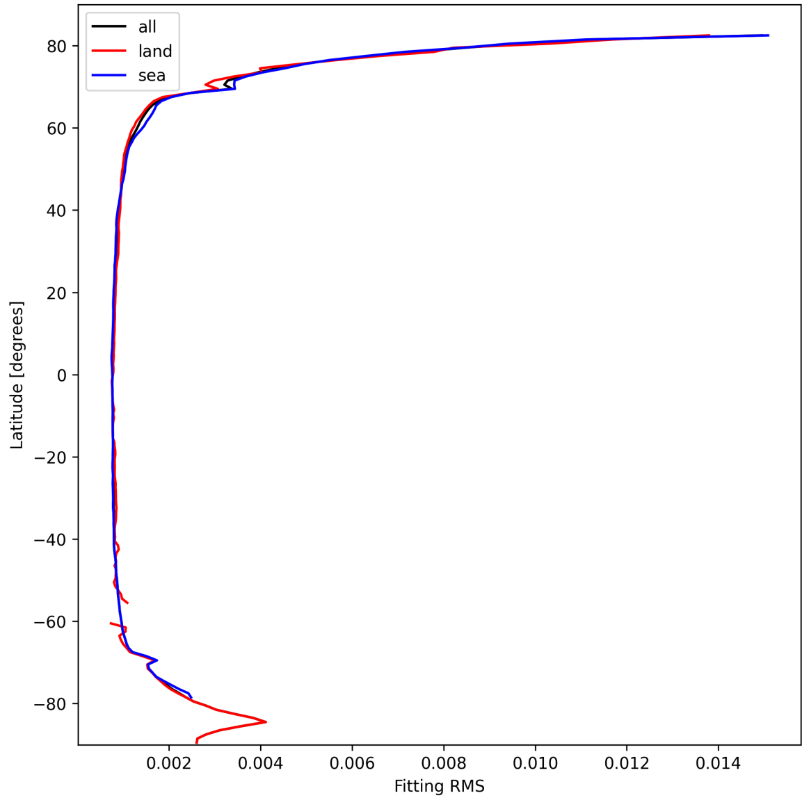
Figure 22: Zonal average of “Fitting RMS” for 2025-03-02 to 2025-03-03.
