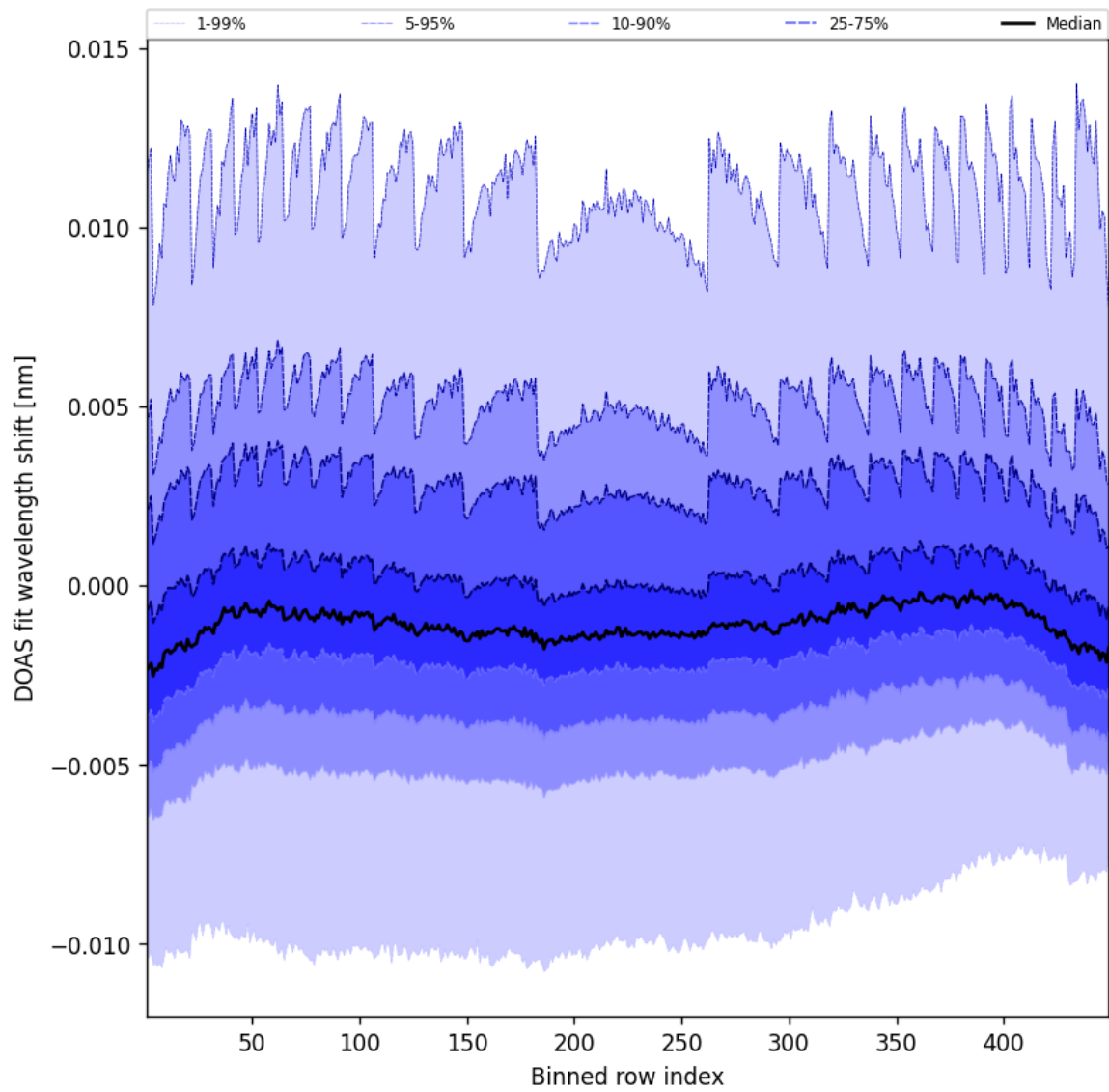
Figure 47: Along track statistics of “DOAS fit wavelength shift” for 2025-03-02 to 2025-03-03
