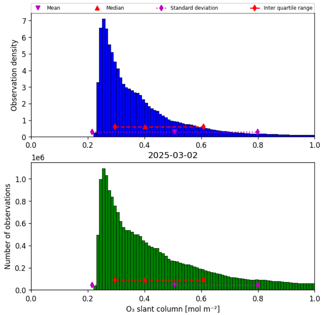
Figure 31: Histogram of “O 3 slant column” for 2025-03-02 to 2025-03-03
