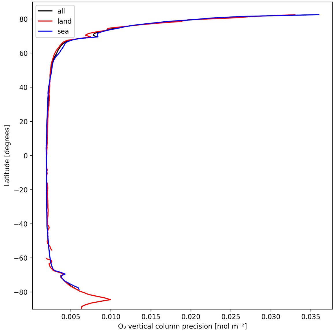
Figure 18: Zonal average of “O 3 vertical column precision” for 2025-03-02 to 2025-03-03.
