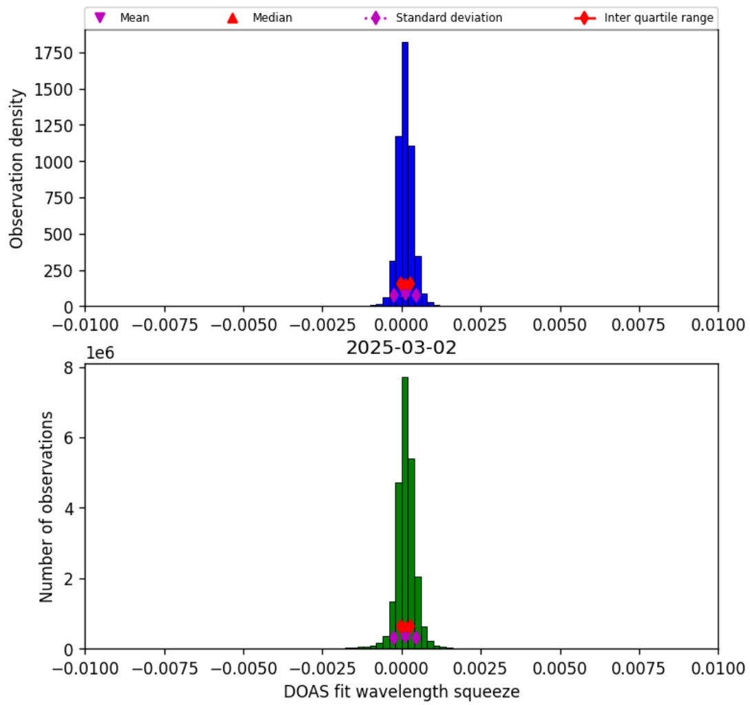
Figure 36: Histogram of “DOAS fit wavelength squeeze” for 2025-03-02 to 2025-03-03
