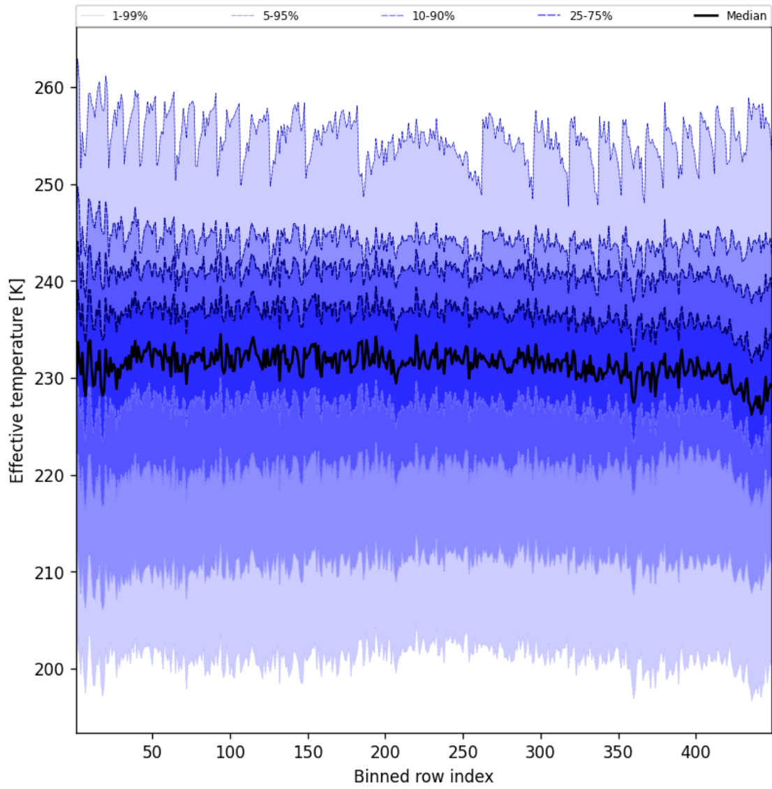
Figure 50: Along track statistics of “Effective temperature” for 2025-03-02 to 2025-03-03
