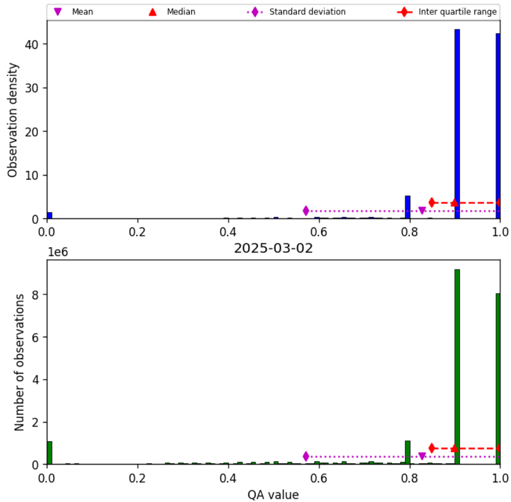
Figure 28: Histogram of “QA value” for 2025-03-02 to 2025-03-03
