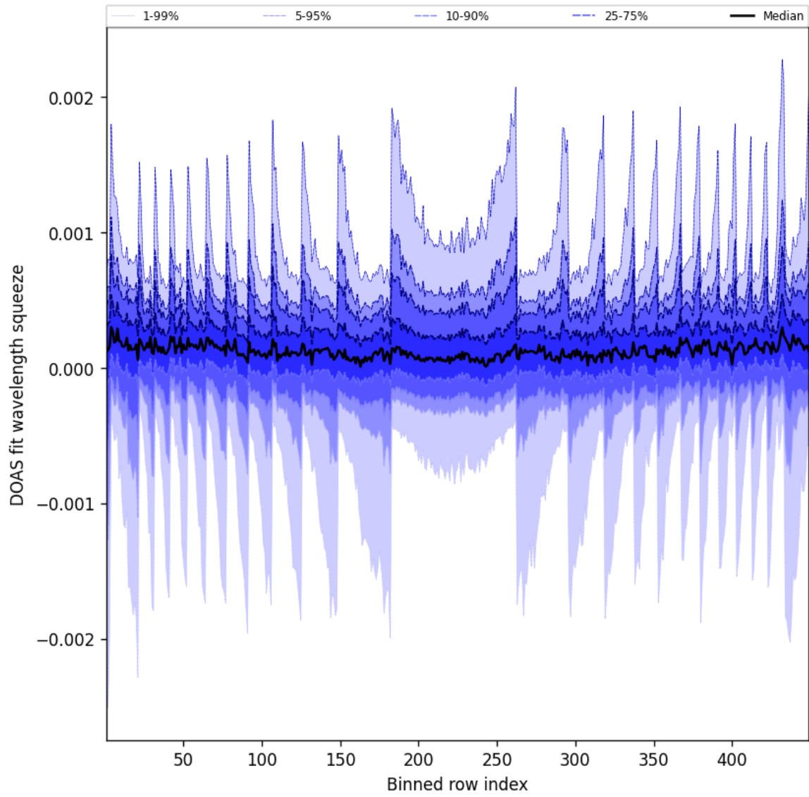
Figure 48: Along track statistics of “DOAS fit wavelength squeeze” for 2025-03-02 to 2025-03-03
