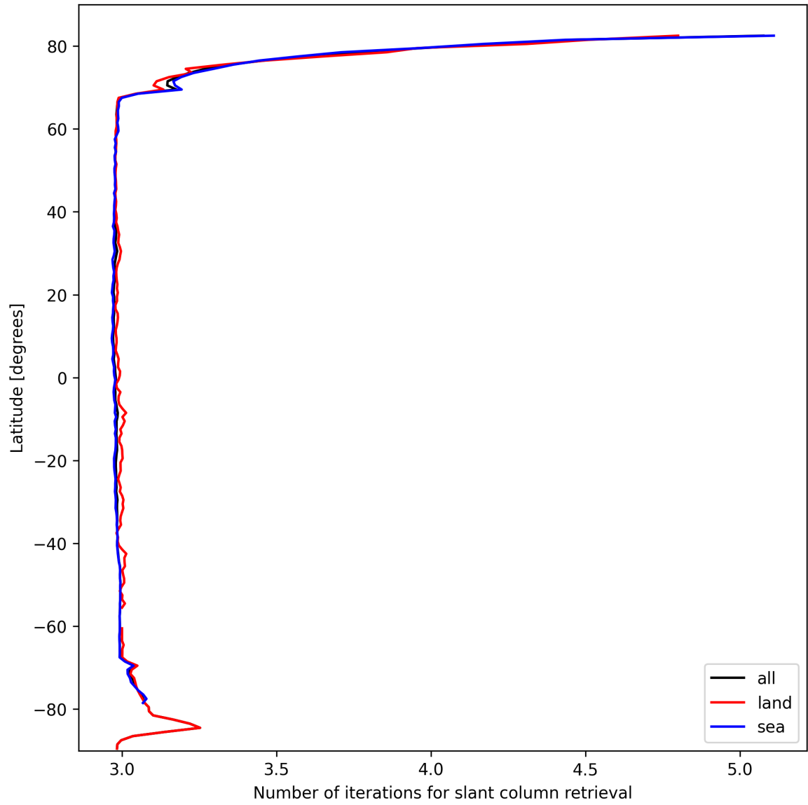
Figure 21: Zonal average of “Number of iterations for slant column retrieval” for 2025-03-02 to 2025-03-03.
