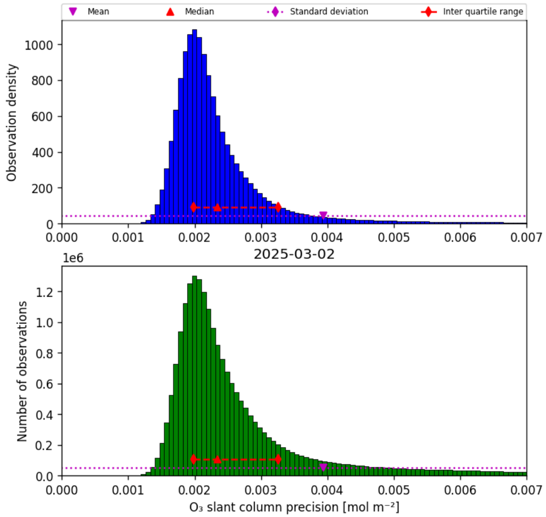
Figure 32: Histogram of “O 3 slant column precision” for 2025-03-02 to 2025-03-03
