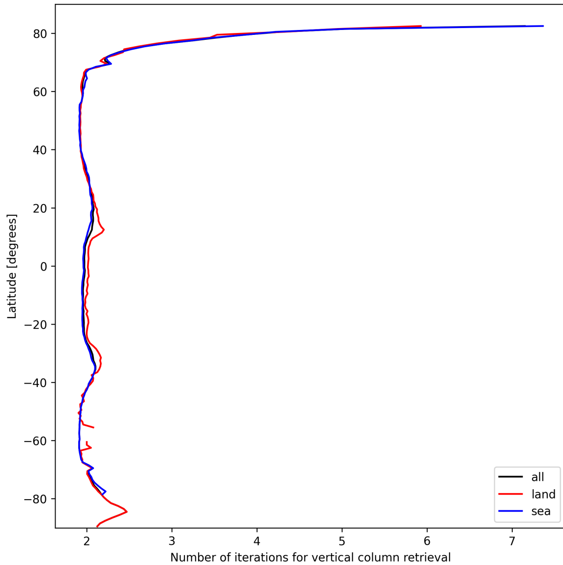
Figure 27: Zonal average of “Number of iterations for vertical column retrieval” for 2025-03-02 to 2025-03-03.
