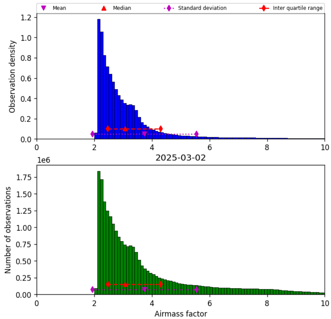
Figure 37: Histogram of “Airmass factor” for 2025-03-02 to 2025-03-03
