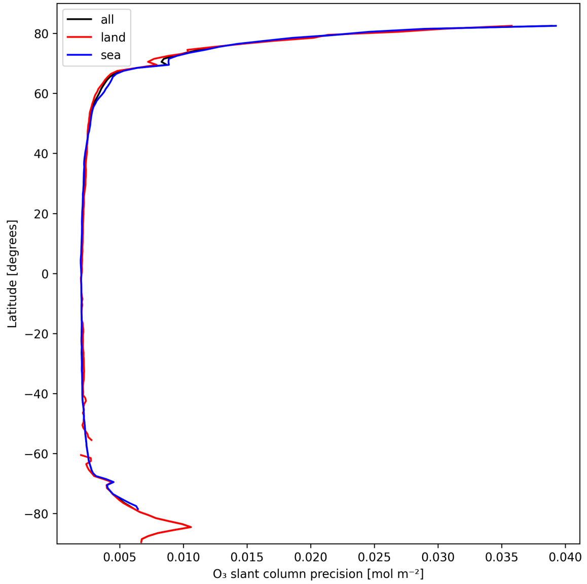
Figure 20: Zonal average of “O 3 slant column precision” for 2025-03-02 to 2025-03-03.
