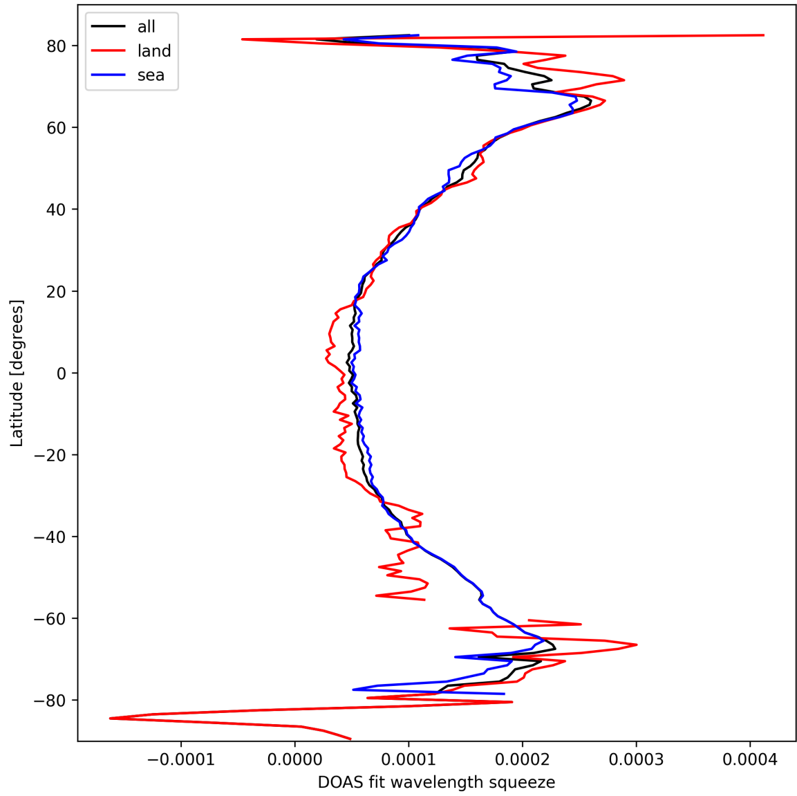
Figure 24: Zonal average of “DOAS fit wavelength squeeze” for 2025-03-02 to 2025-03-03.
