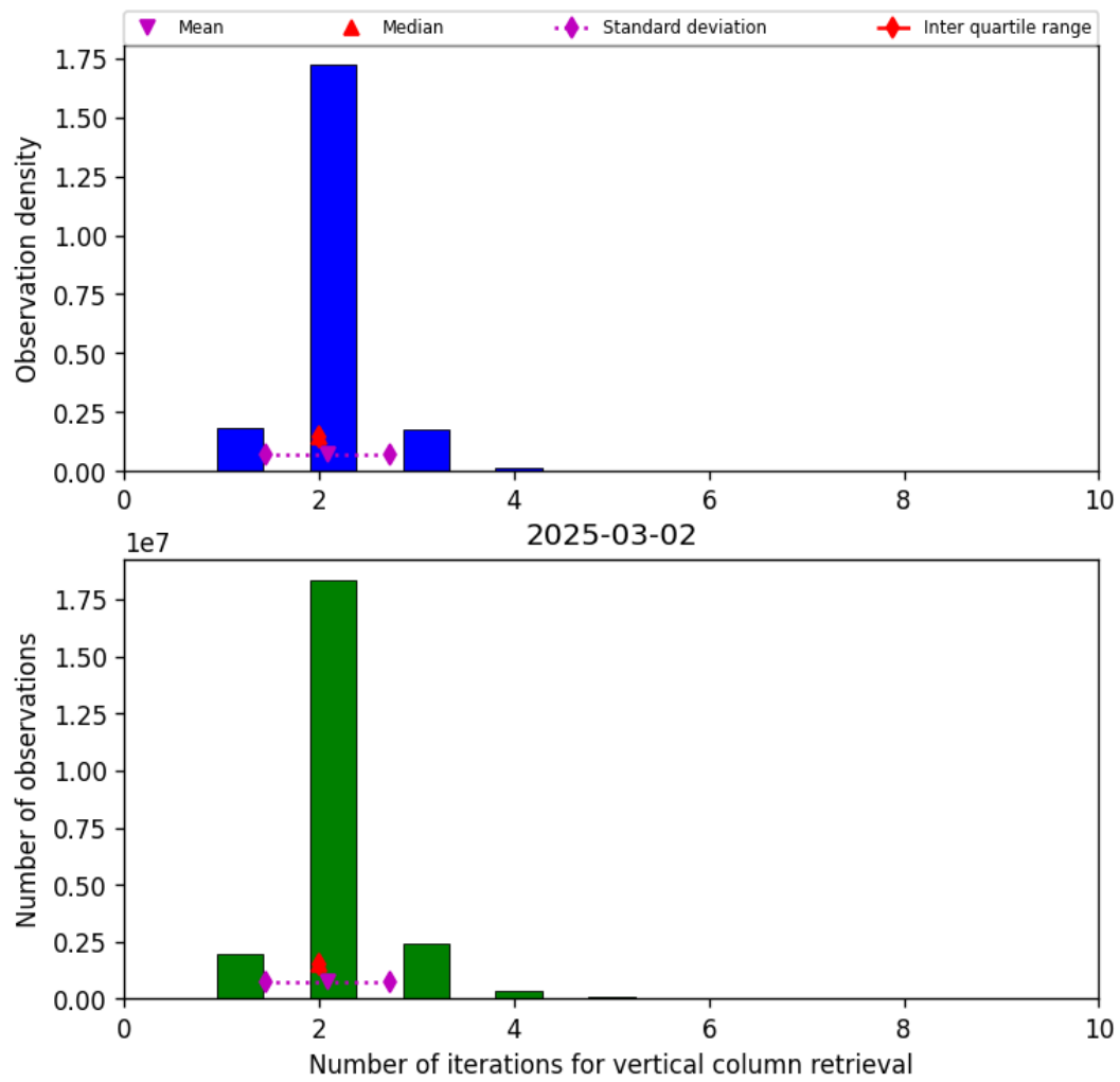
Figure 39: Histogram of “Number of iterations for vertical column retrieval” for 2025-03-02 to 2025-03-03
