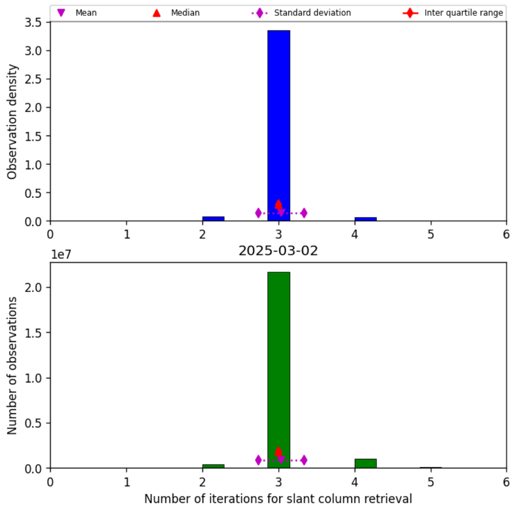
Figure 33: Histogram of “Number of iterations for slant column retrieval” for 2025-03-02 to 2025-03-03
