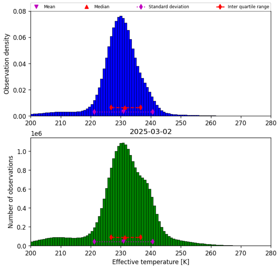
Figure 38: Histogram of “Effective temperature” for 2025-03-02 to 2025-03-03
