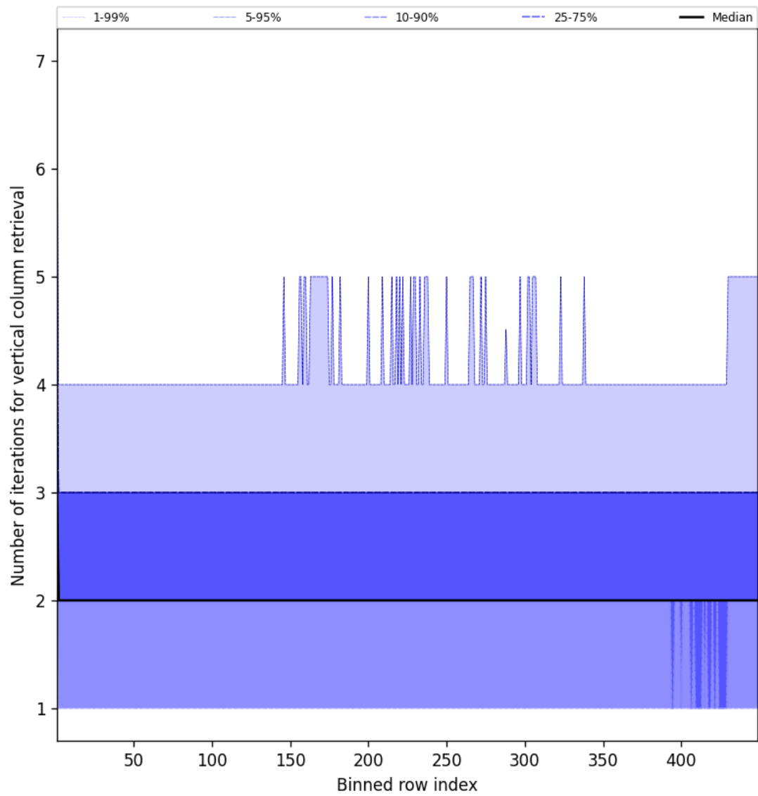
Figure 51: Along track statistics of “Number of iterations for vertical column retrieval” for 2025-03-02 to 2025-03-03
