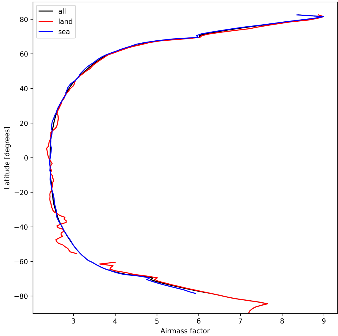
Figure 25: Zonal average of “Airmass factor” for 2025-03-02 to 2025-03-03.
