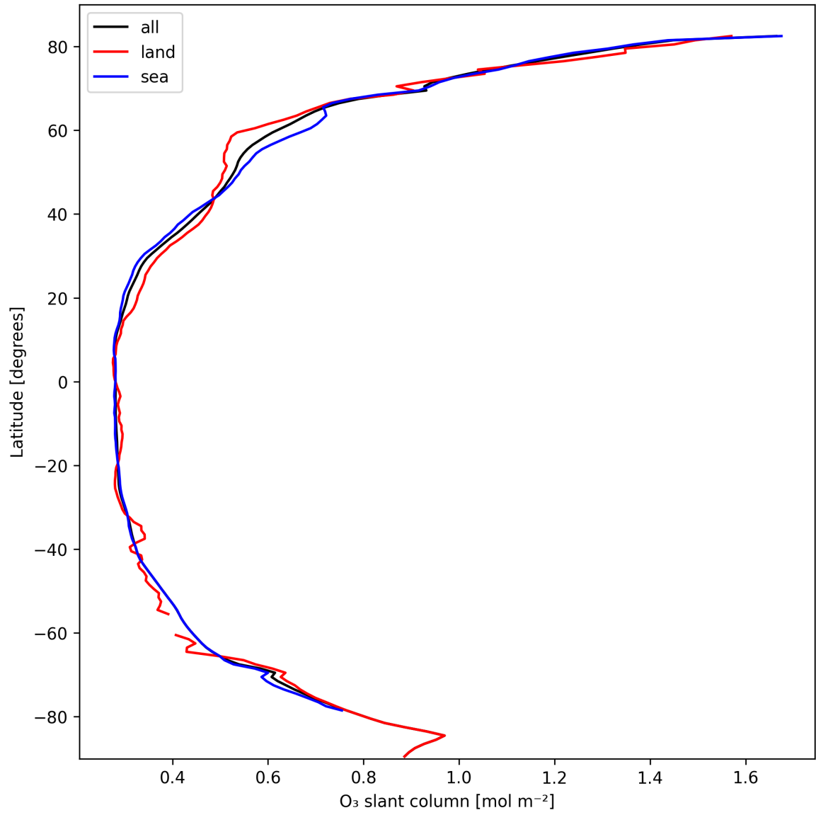
Figure 19: Zonal average of “O 3 slant column” for 2025-03-02 to 2025-03-03.
