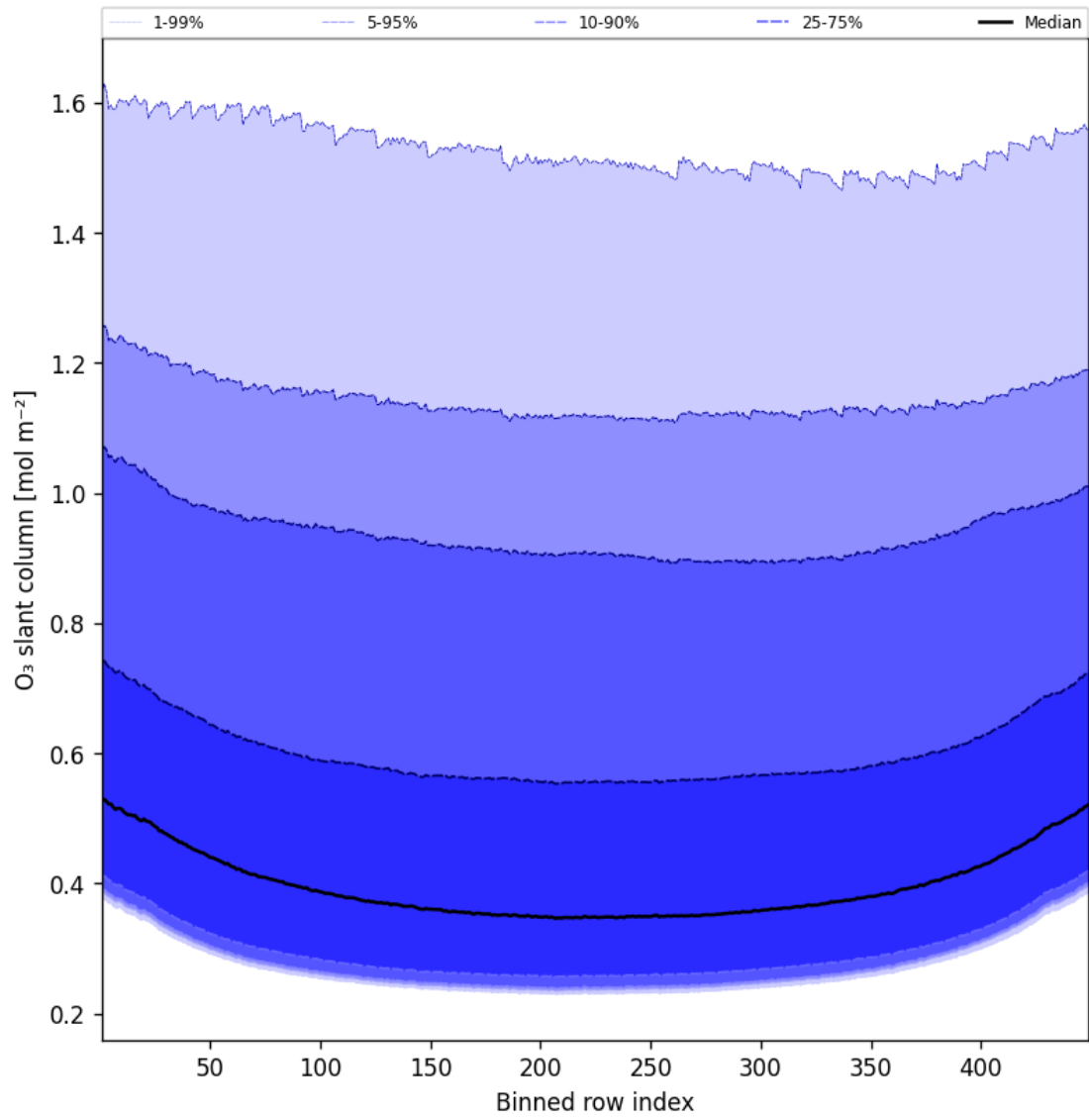
Figure 43: Along track statistics of “O 3 slant column” for 2025-03-02 to 2025-03-03
