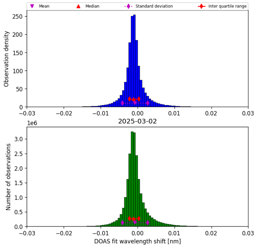
Figure 35: Histogram of “DOAS fit wavelength shift” for 2025-03-02 to 2025-03-03
