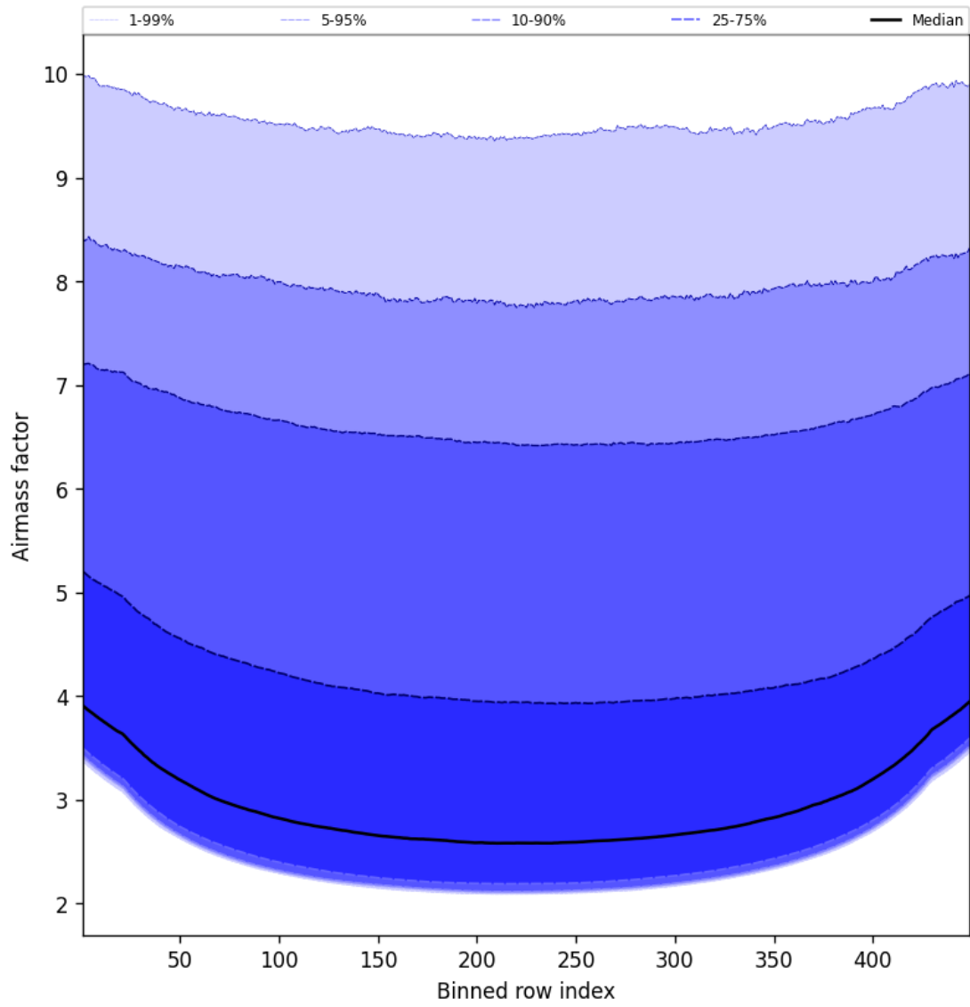
Figure 49: Along track statistics of “Airmass factor” for 2025-03-02 to 2025-03-03
