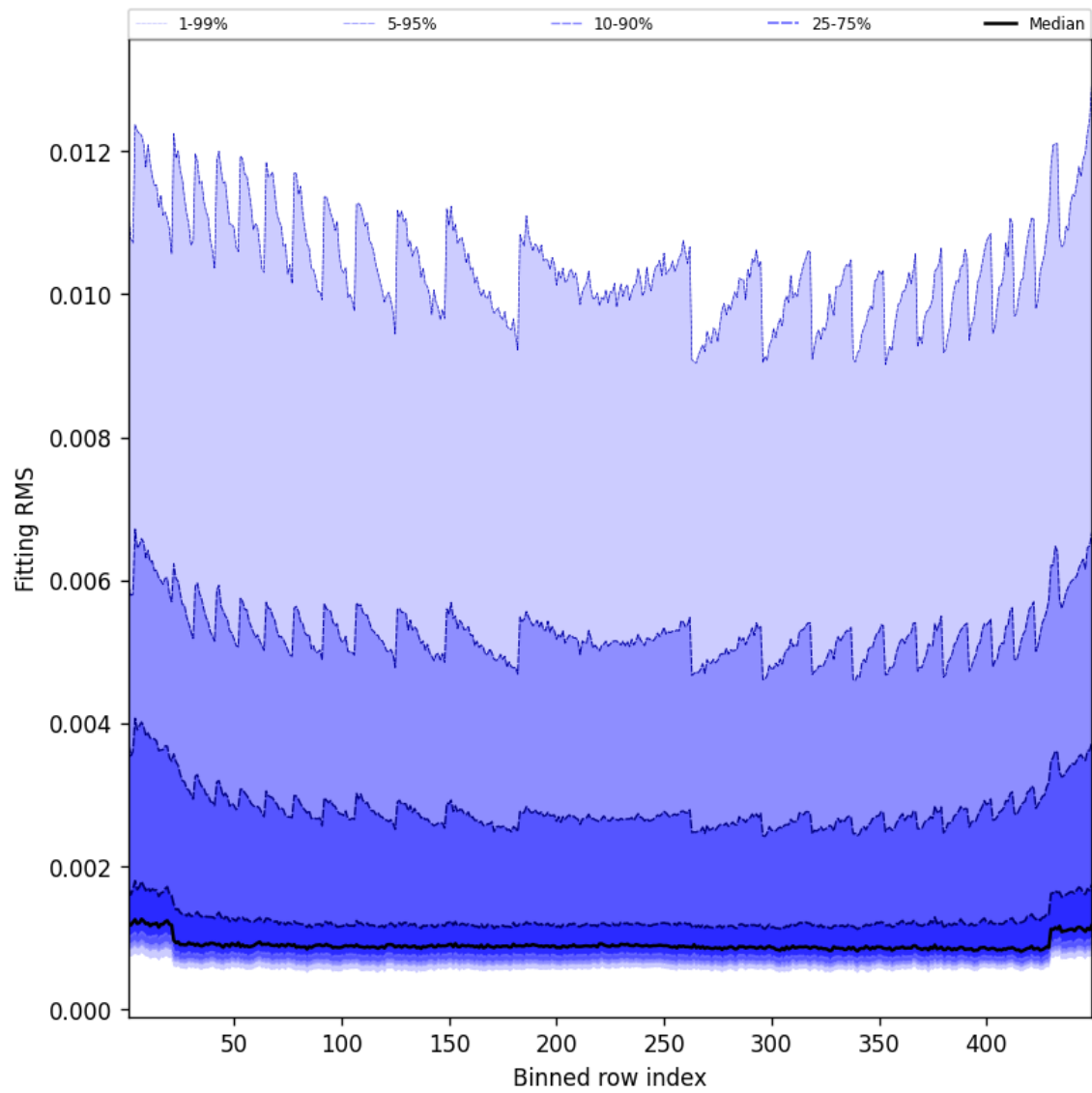
Figure 46: Along track statistics of “Fitting RMS” for 2025-03-02 to 2025-03-03
