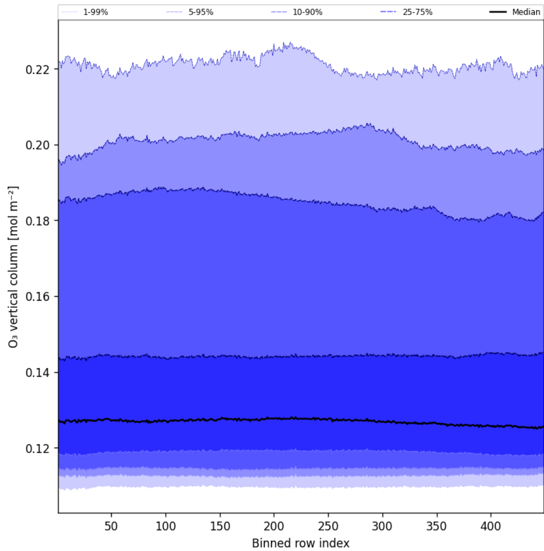
Figure 41: Along track statistics of “O 3 vertical column” for 2025-03-02 to 2025-03-03
