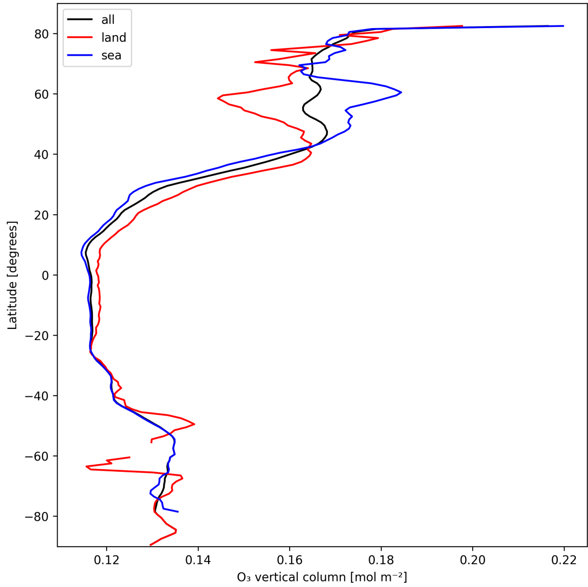
Figure 17: Zonal average of “O 3 vertical column” for 2025-03-02 to 2025-03-03.
