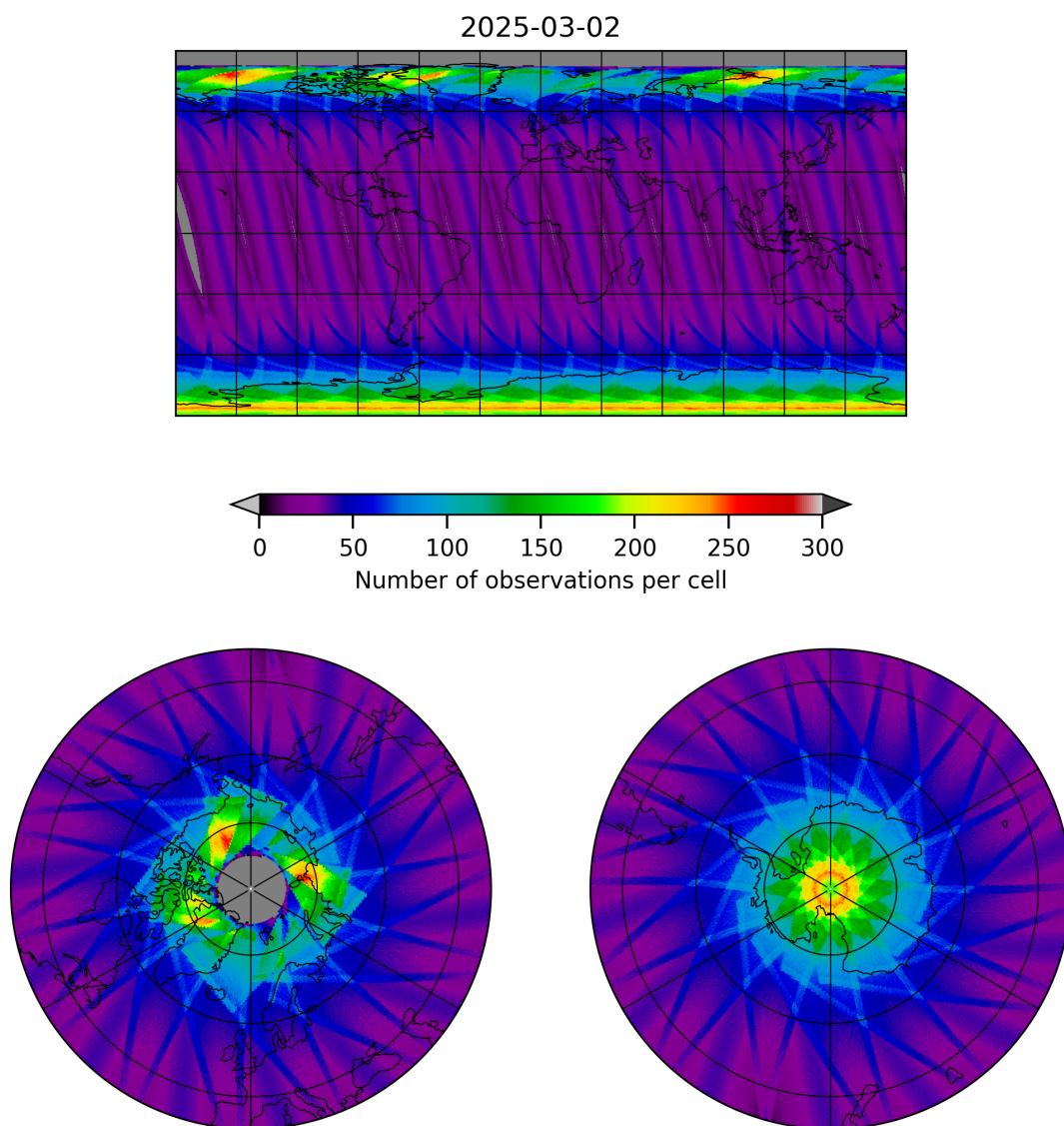
Figure 15: Map of the number of observations for 2025-03-02 to 2025-03-03
