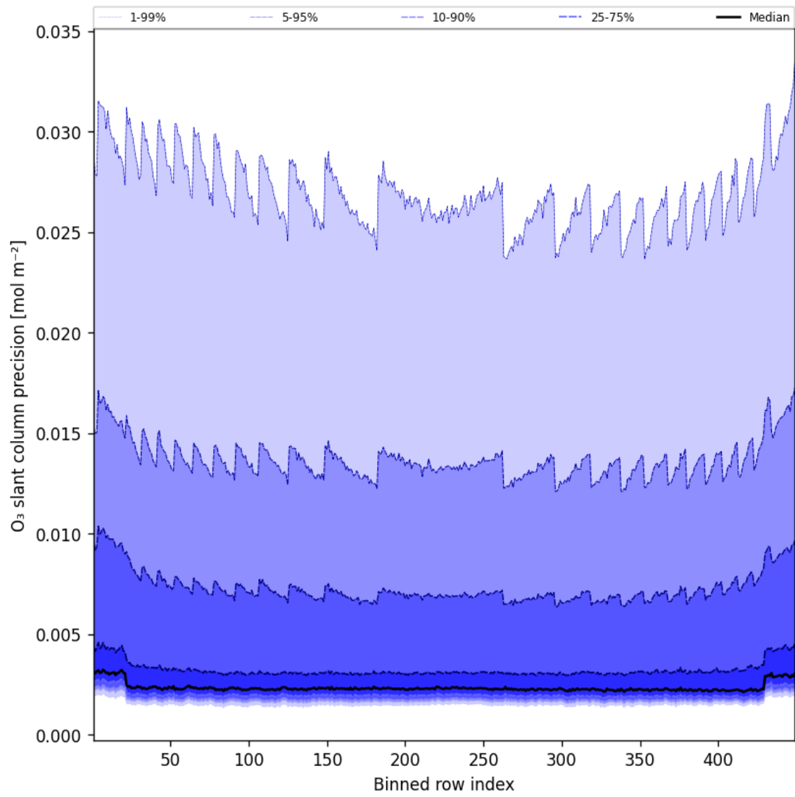
Figure 44: Along track statistics of “O 3 slant column precision” for 2025-03-02 to 2025-03-03
