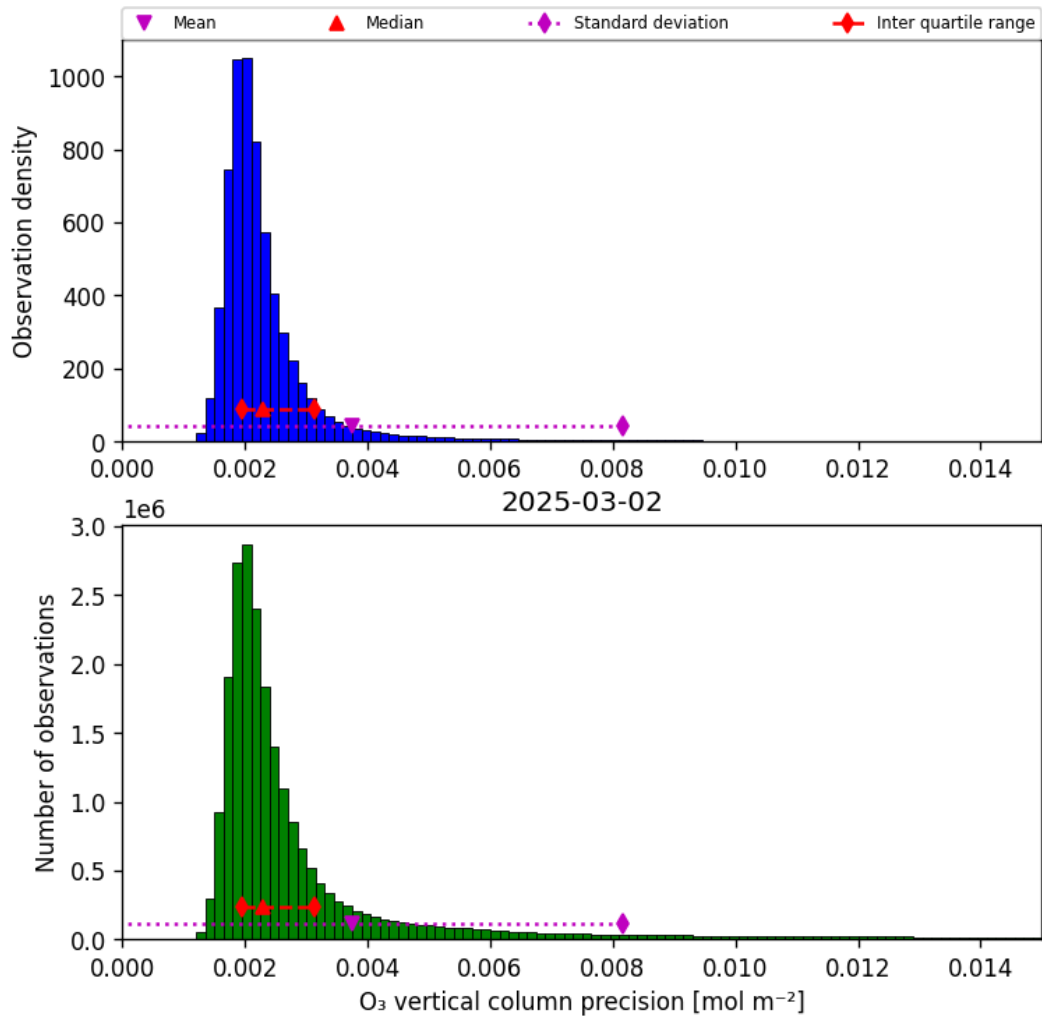
Figure 30: Histogram of “O 3 vertical column precision” for 2025-03-02 to 2025-03-03
