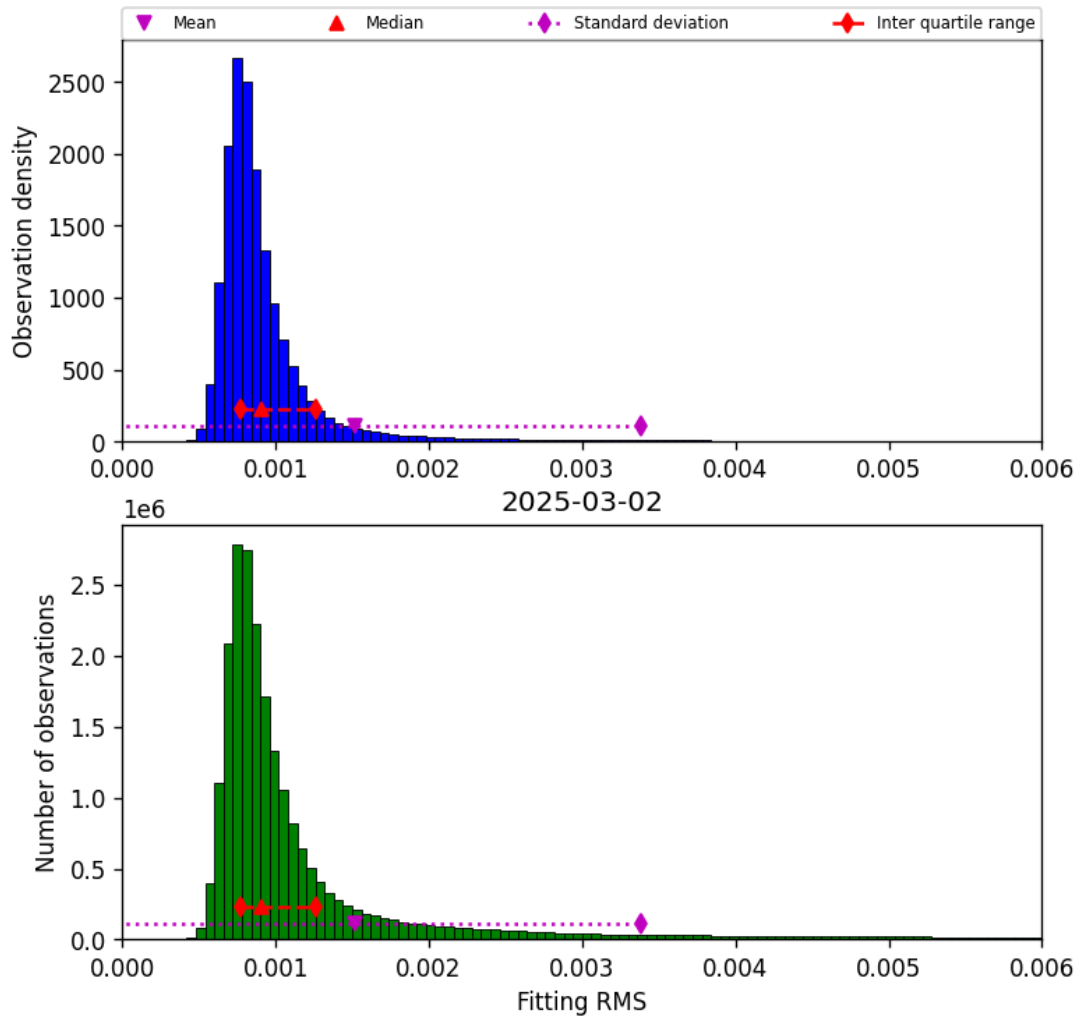
Figure 34: Histogram of “Fitting RMS” for 2025-03-02 to 2025-03-03
