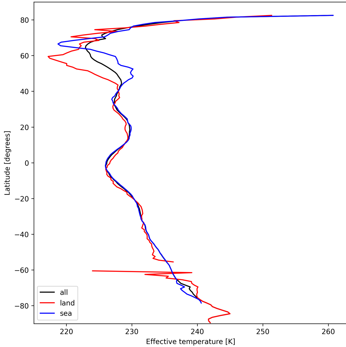
Figure 26: Zonal average of “Effective temperature” for 2025-03-02 to 2025-03-03.
