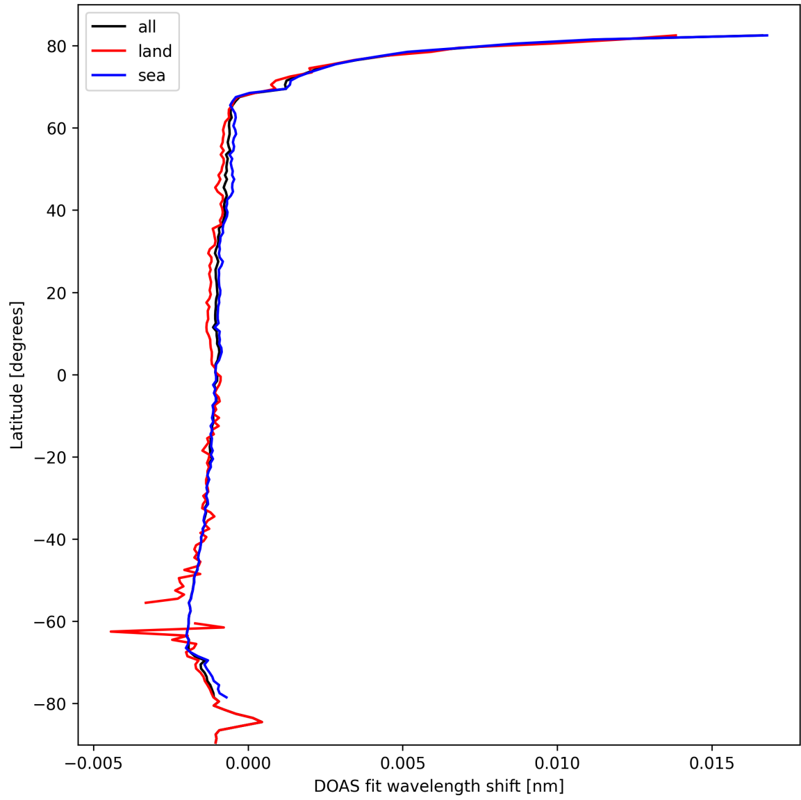
Figure 23: Zonal average of "DOAS fit wavelength shift" for 2025-03-02 to 2025-03-03.
