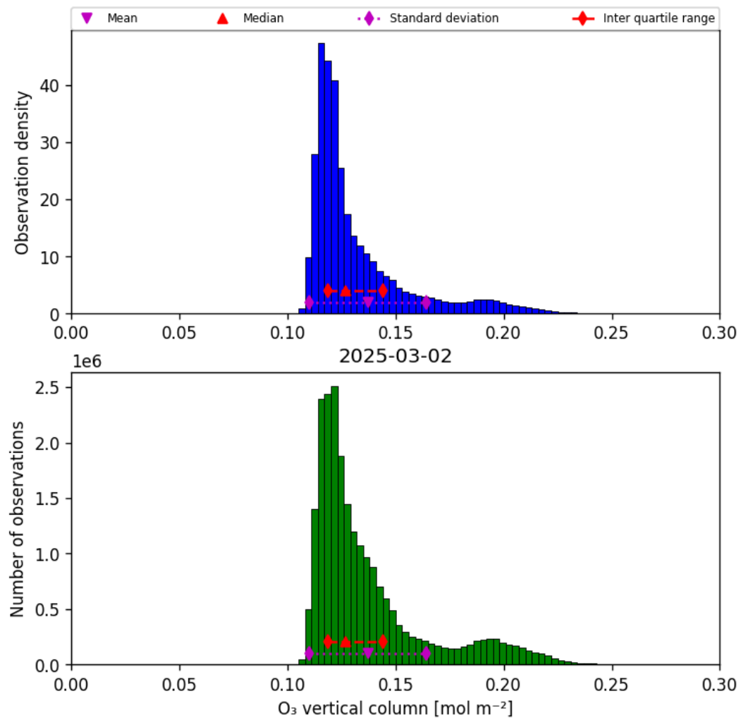
Figure 29: Histogram of “O 3 vertical column” for 2025-03-02 to 2025-03-03
