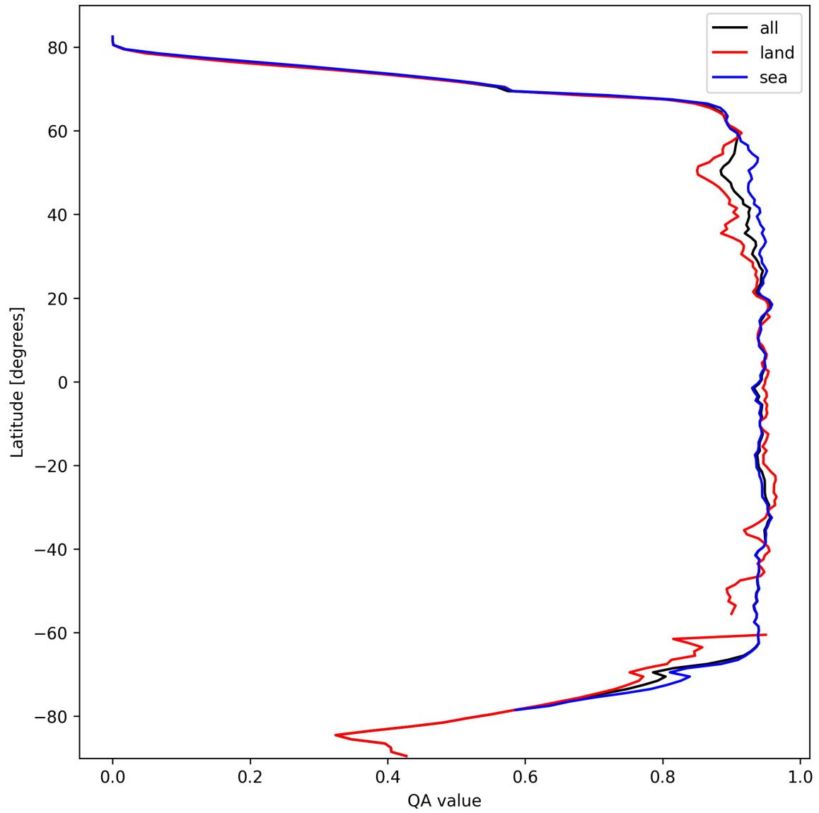
Figure 16: Zonal average of “QA value” for 2025-03-02 to 2025-03-03.
