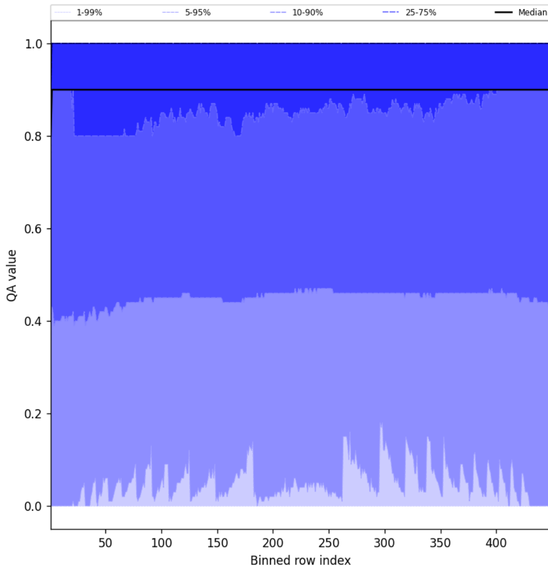
Figure 40: Along track statistics of “QA value” for 2025-03-02 to 2025-03-03
