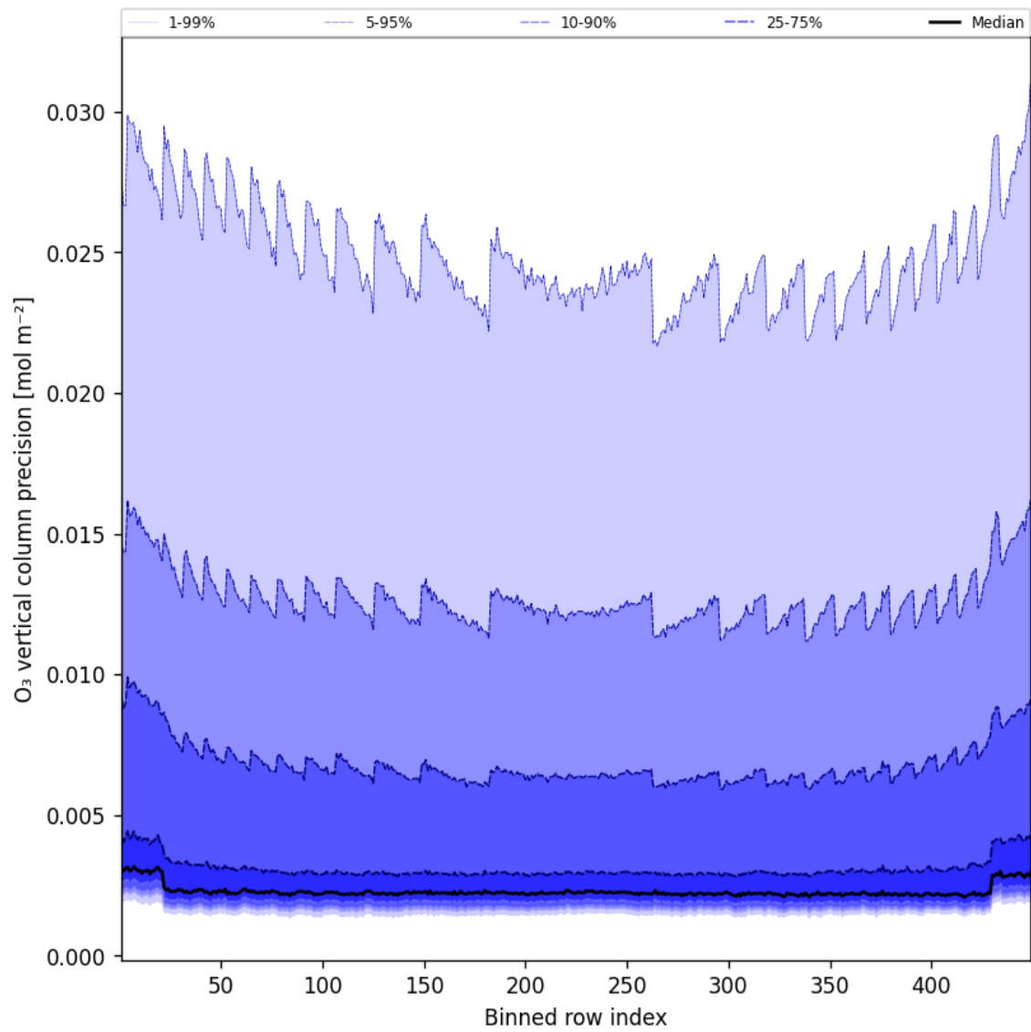
Figure 42: Along track statistics of “O 3 vertical column precision” for 2025-03-02 to 2025-03-03
