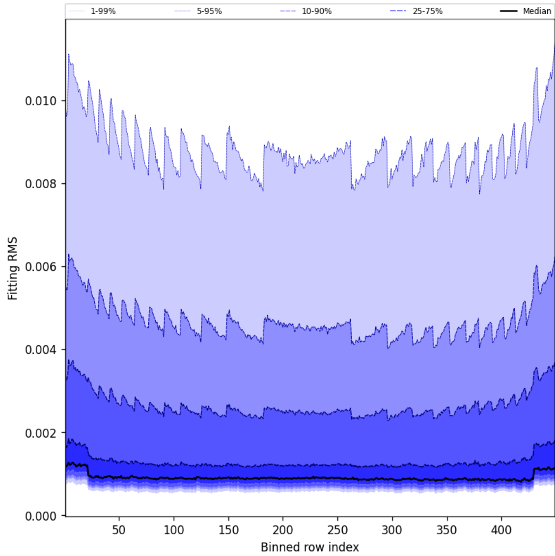
Figure 46: Along track statistics of “Fitting RMS” for 2025-03-04 to 2025-03-04
