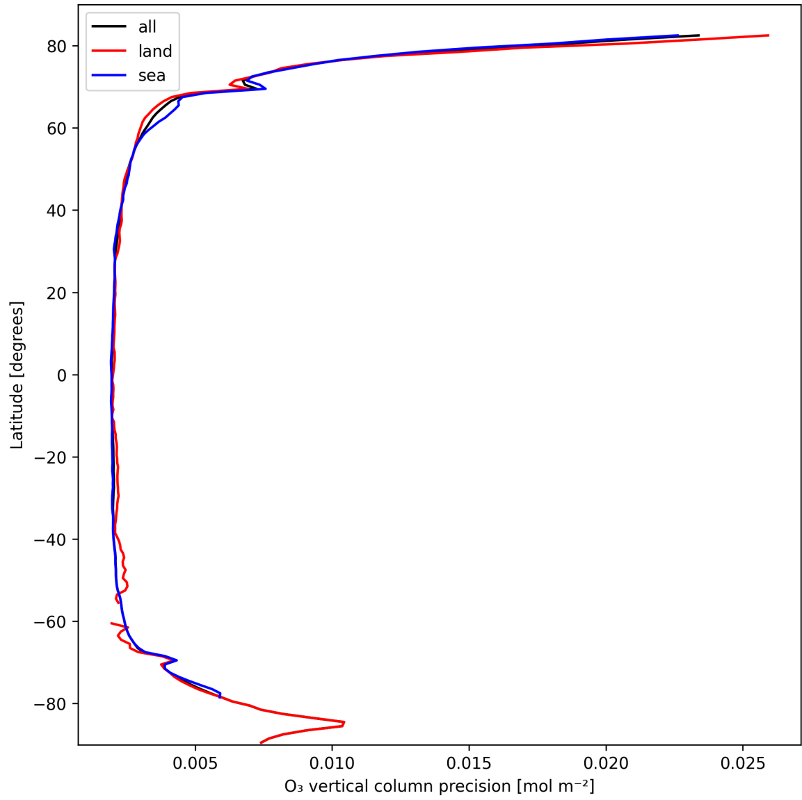
Figure 18: Zonal average of “O 3 vertical column precision” for 2025-03-04 to 2025-03-04.
