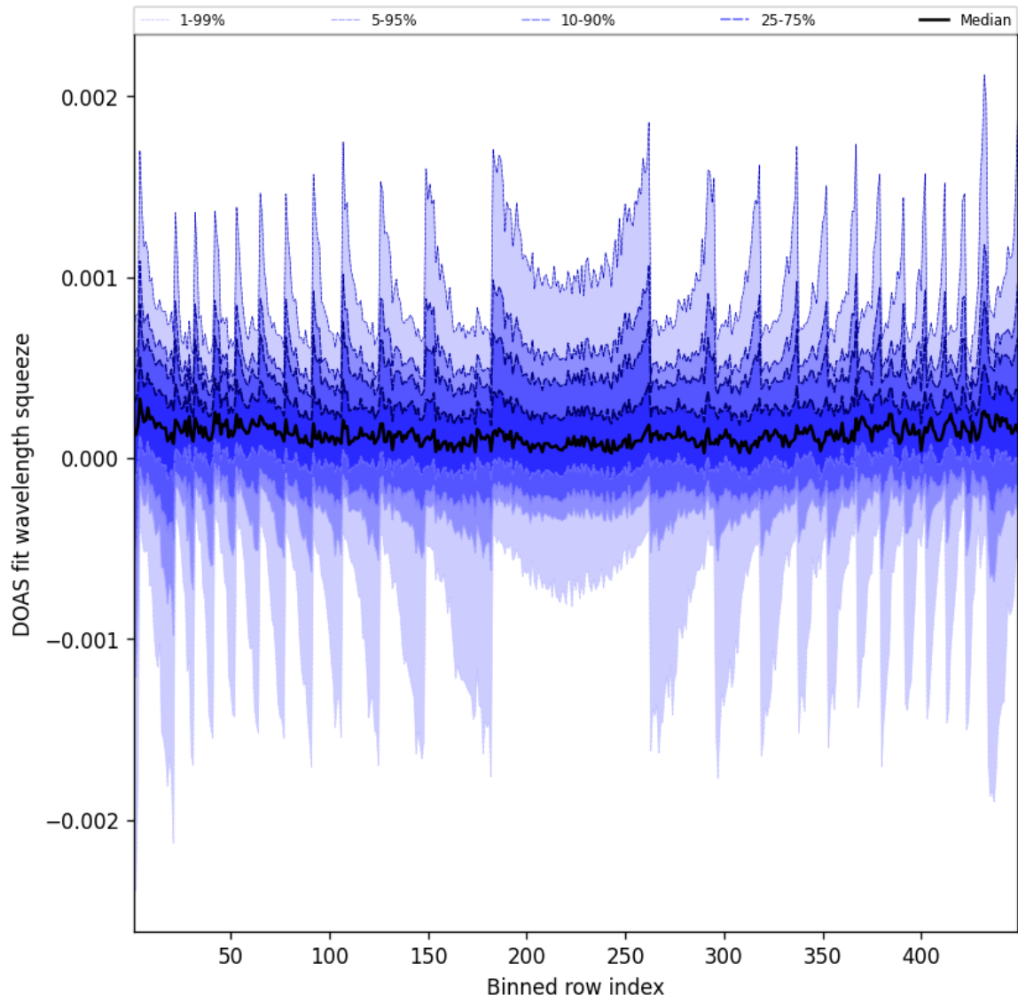
Figure 48: Along track statistics of “DOAS fit wavelength squeeze” for 2025-03-04 to 2025-03-04
