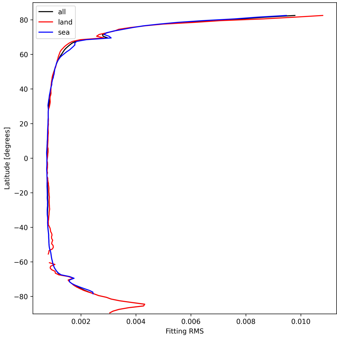
Figure 22: Zonal average of “Fitting RMS” for 2025-03-04 to 2025-03-04.
