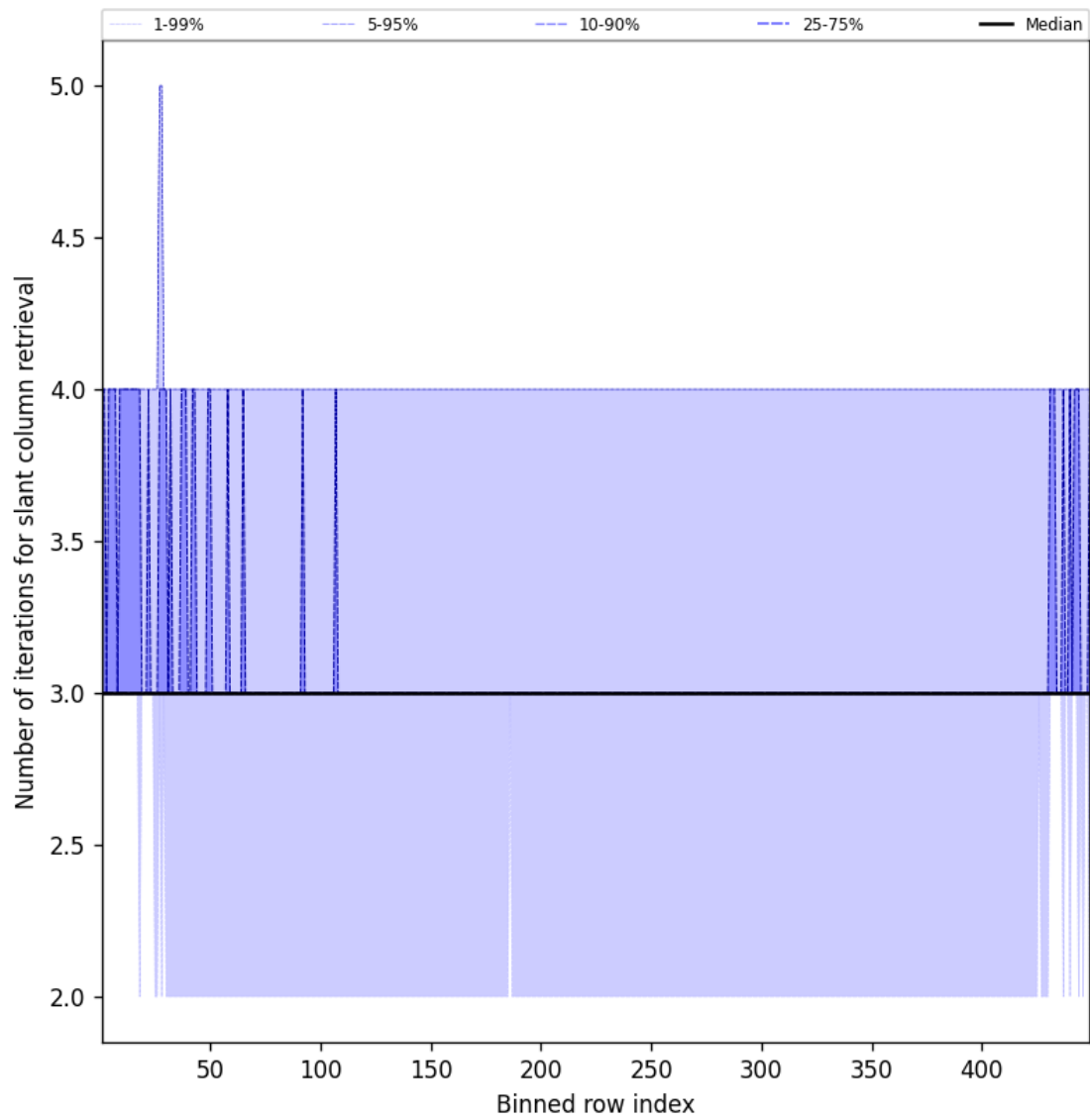
Figure 45: Along track statistics of “Number of iterations for slant column retrieval” for 2025-03-04 to 2025-03-04
