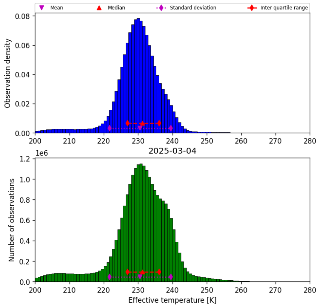
Figure 38: Histogram of “Effective temperature” for 2025-03-04 to 2025-03-04
