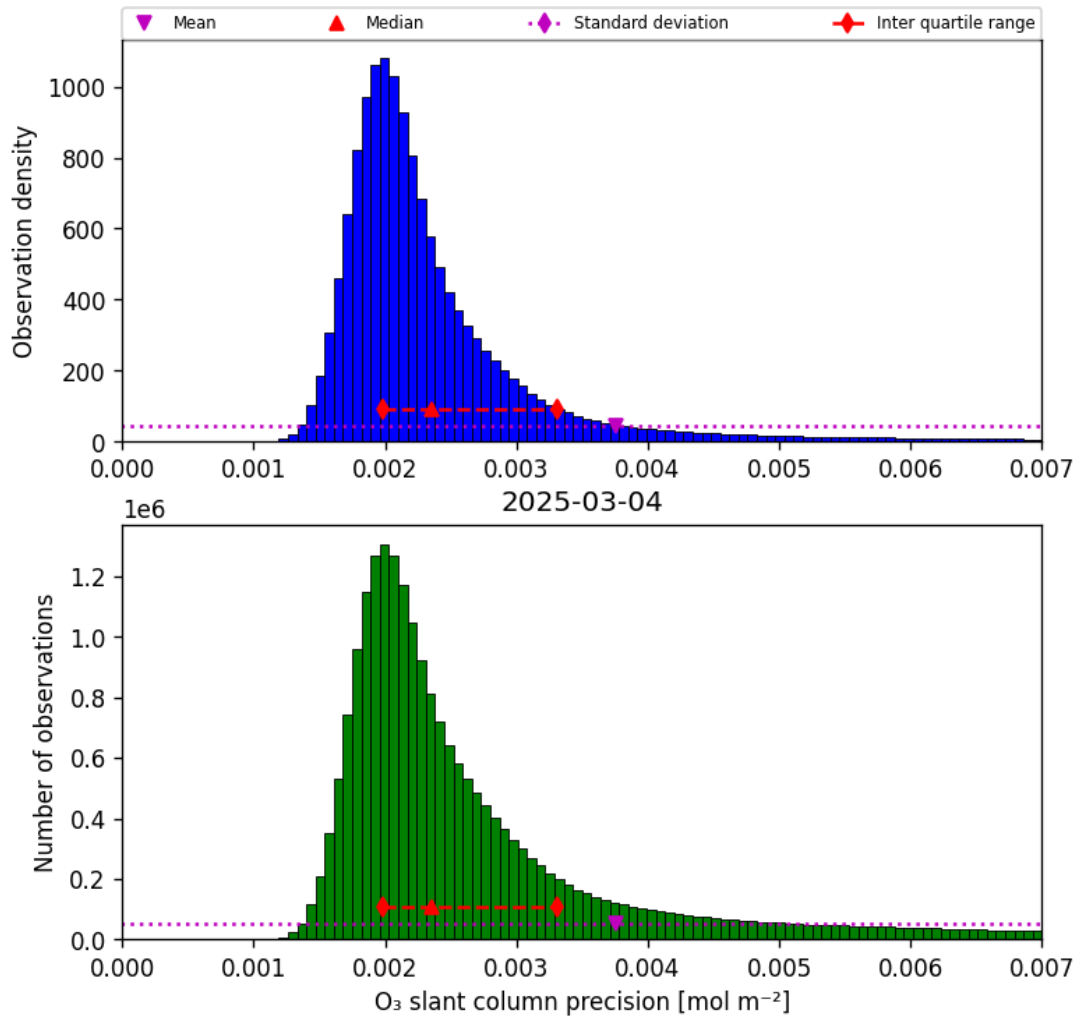
Figure 32: Histogram of “O 3 slant column precision” for 2025-03-04 to 2025-03-04
