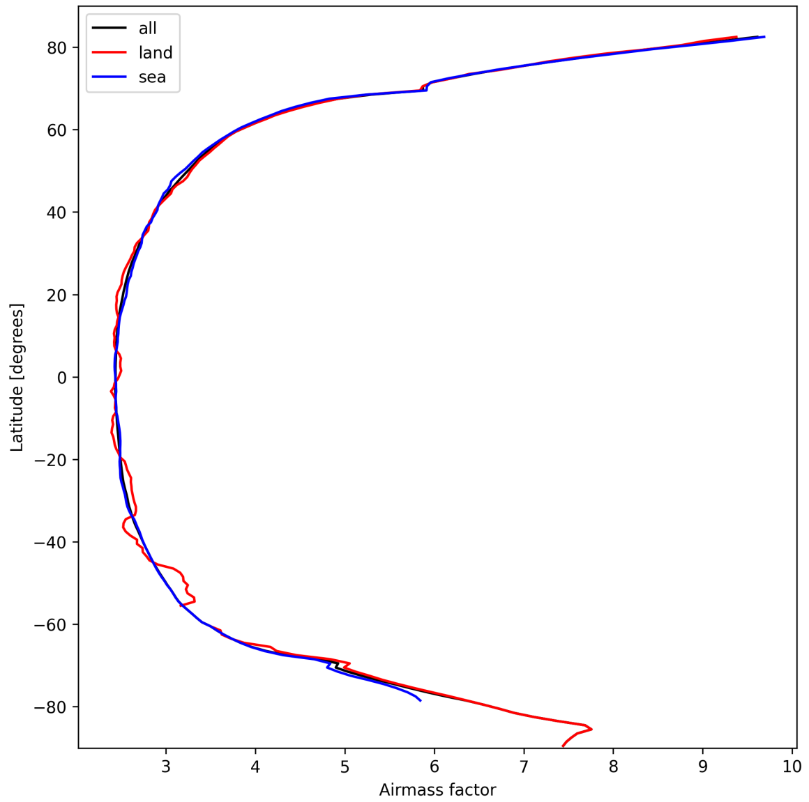
Figure 25: Zonal average of “Airmass factor” for 2025-03-04 to 2025-03-04.
