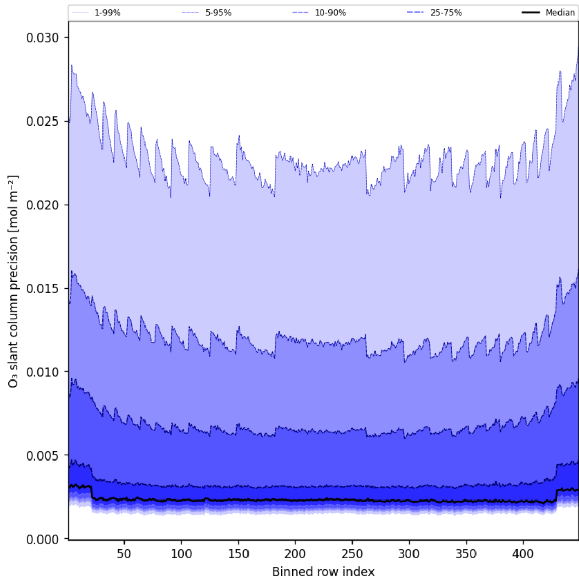
Figure 44: Along track statistics of “O 3 slant column precision” for 2025-03-04 to 2025-03-04
