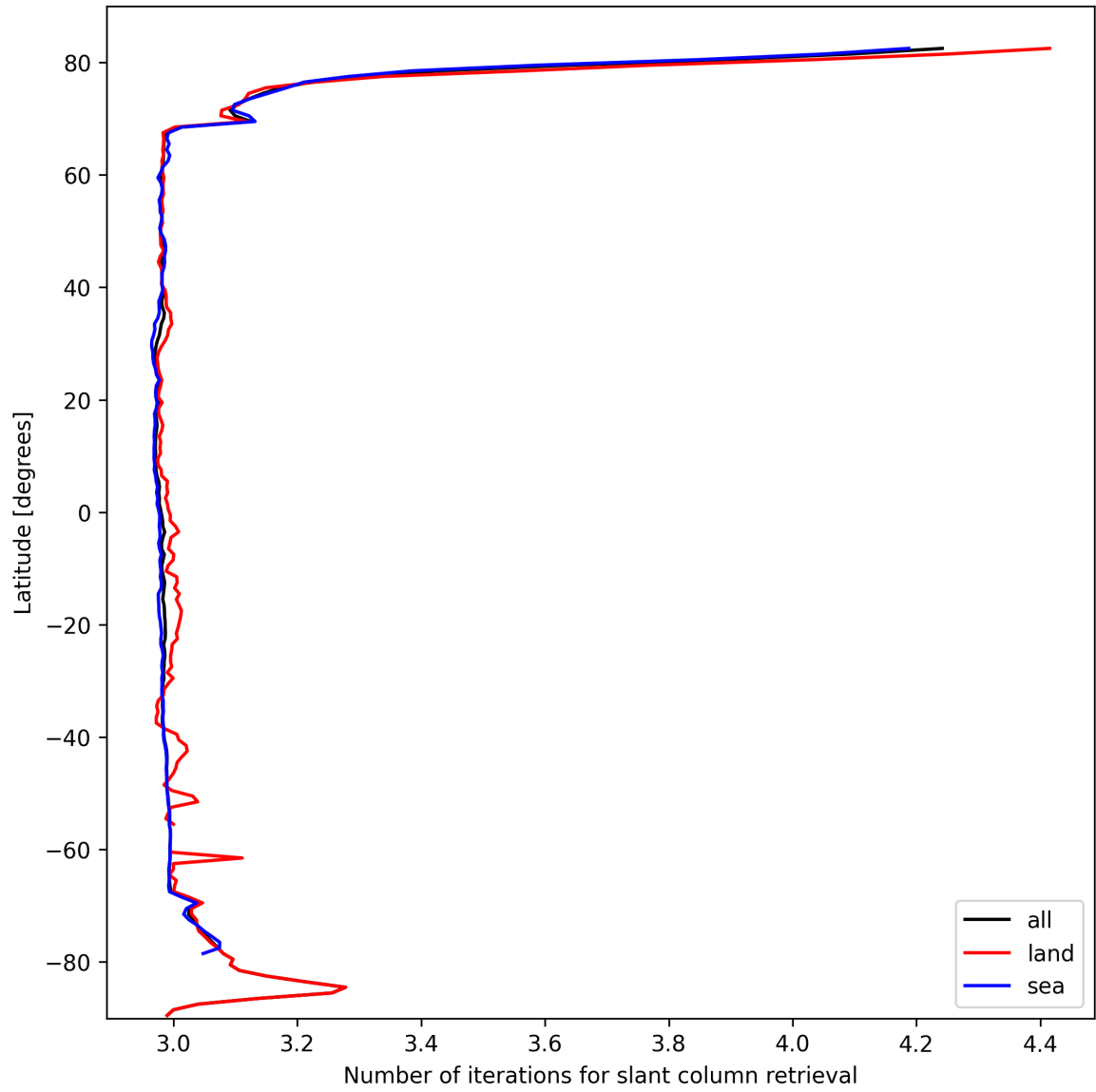
Figure 21: Zonal average of “Number of iterations for slant column retrieval” for 2025-03-04 to 2025-03-04.
