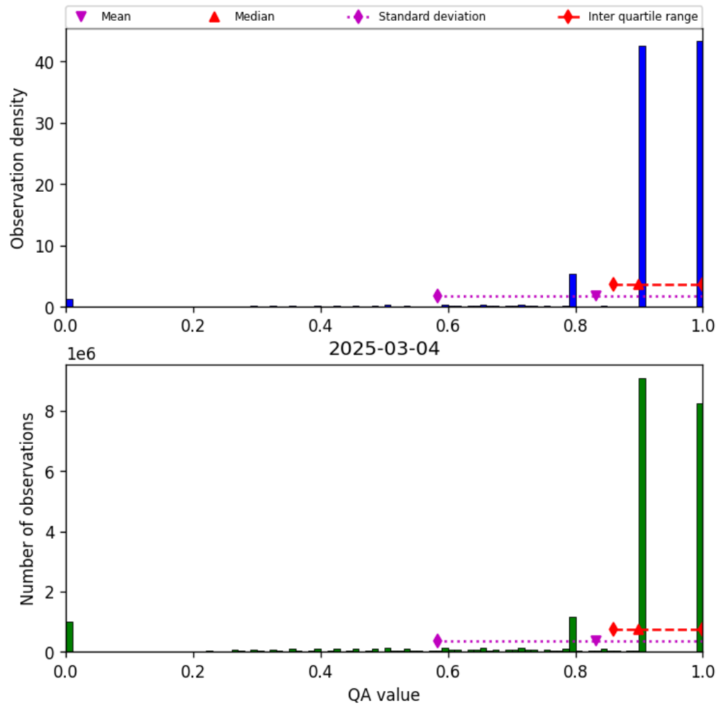
Figure 28: Histogram of “QA value” for 2025-03-04 to 2025-03-04
