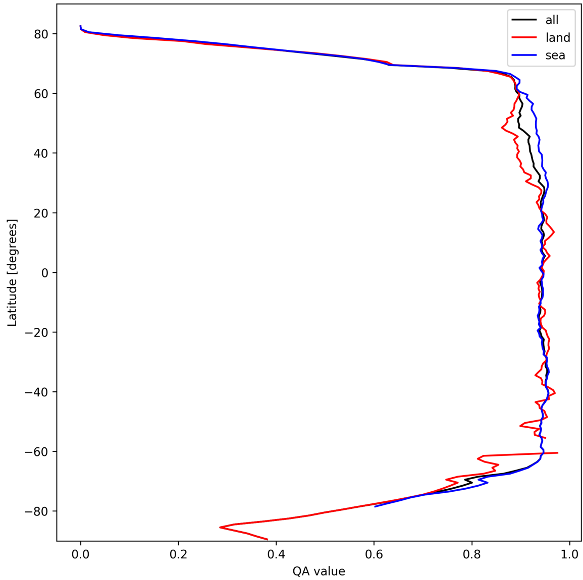
Figure 16: Zonal average of “QA value” for 2025-03-04 to 2025-03-04.
