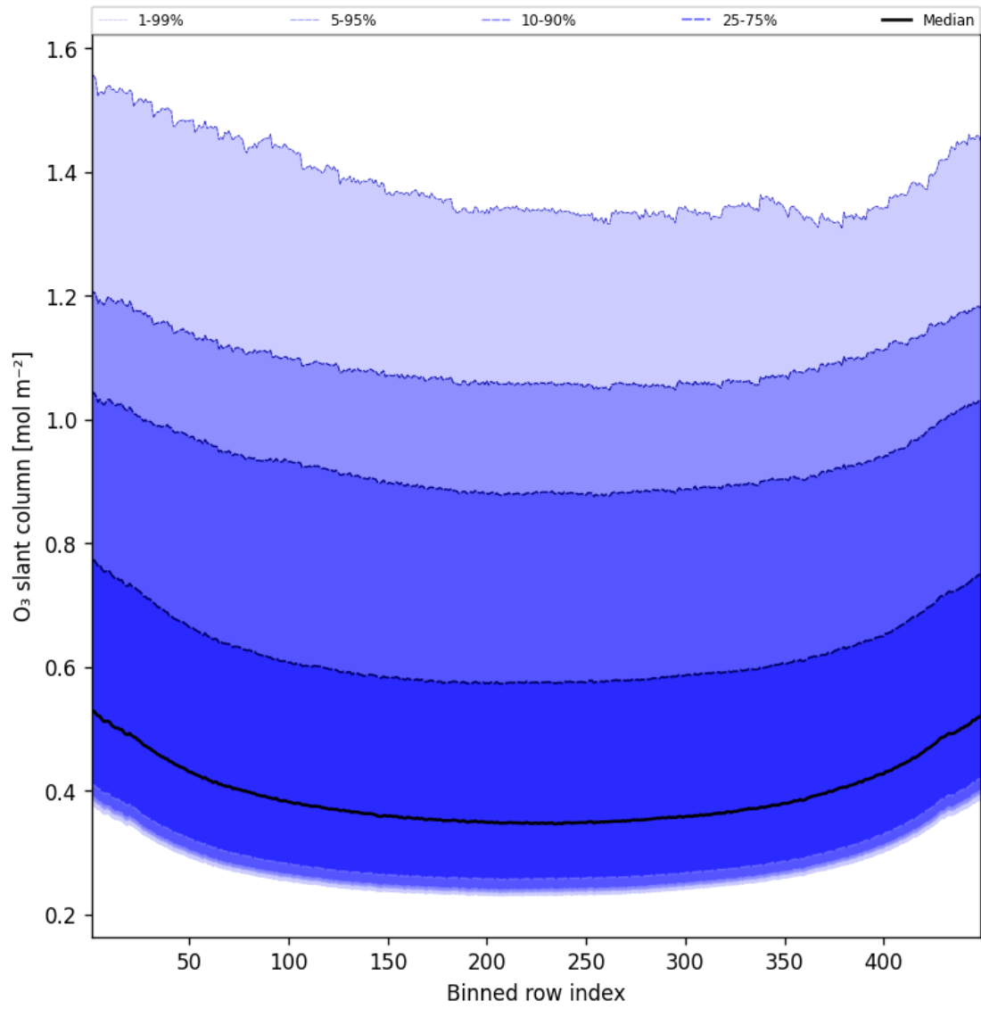
Figure 43: Along track statistics of “O 3 slant column” for 2025-03-04 to 2025-03-04
