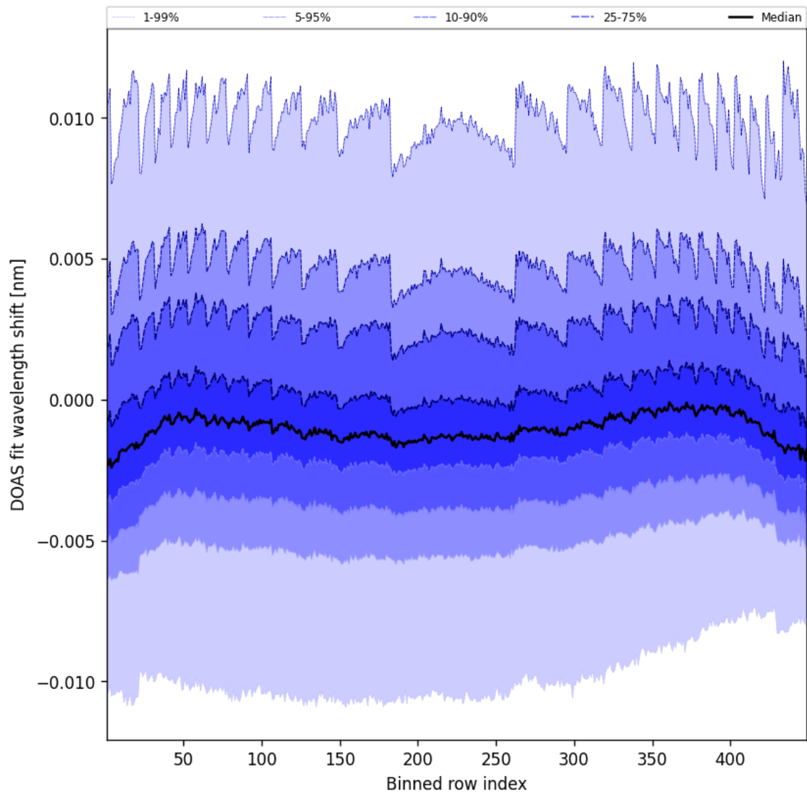
Figure 47: Along track statistics of "DOAS fit wavelength shift" for 2025-03-04 to 2025-03-04
