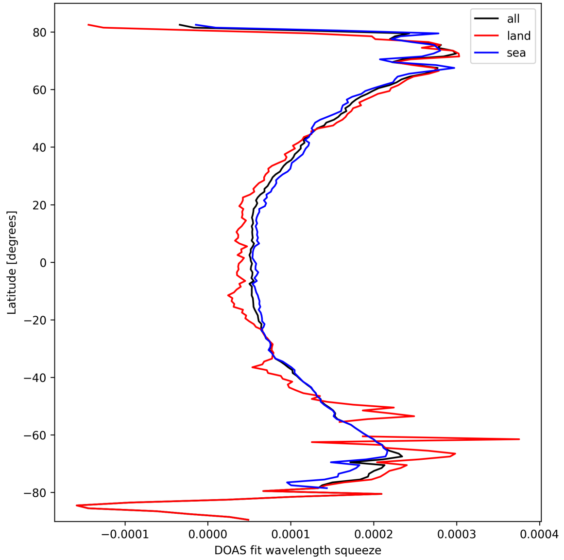
Figure 24: Zonal average of “DOAS fit wavelength squeeze” for 2025-03-04 to 2025-03-04.
