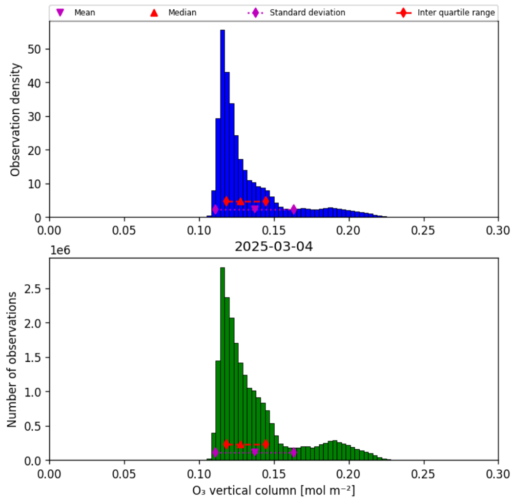
Figure 29: Histogram of “O 3 vertical column” for 2025-03-04 to 2025-03-04
