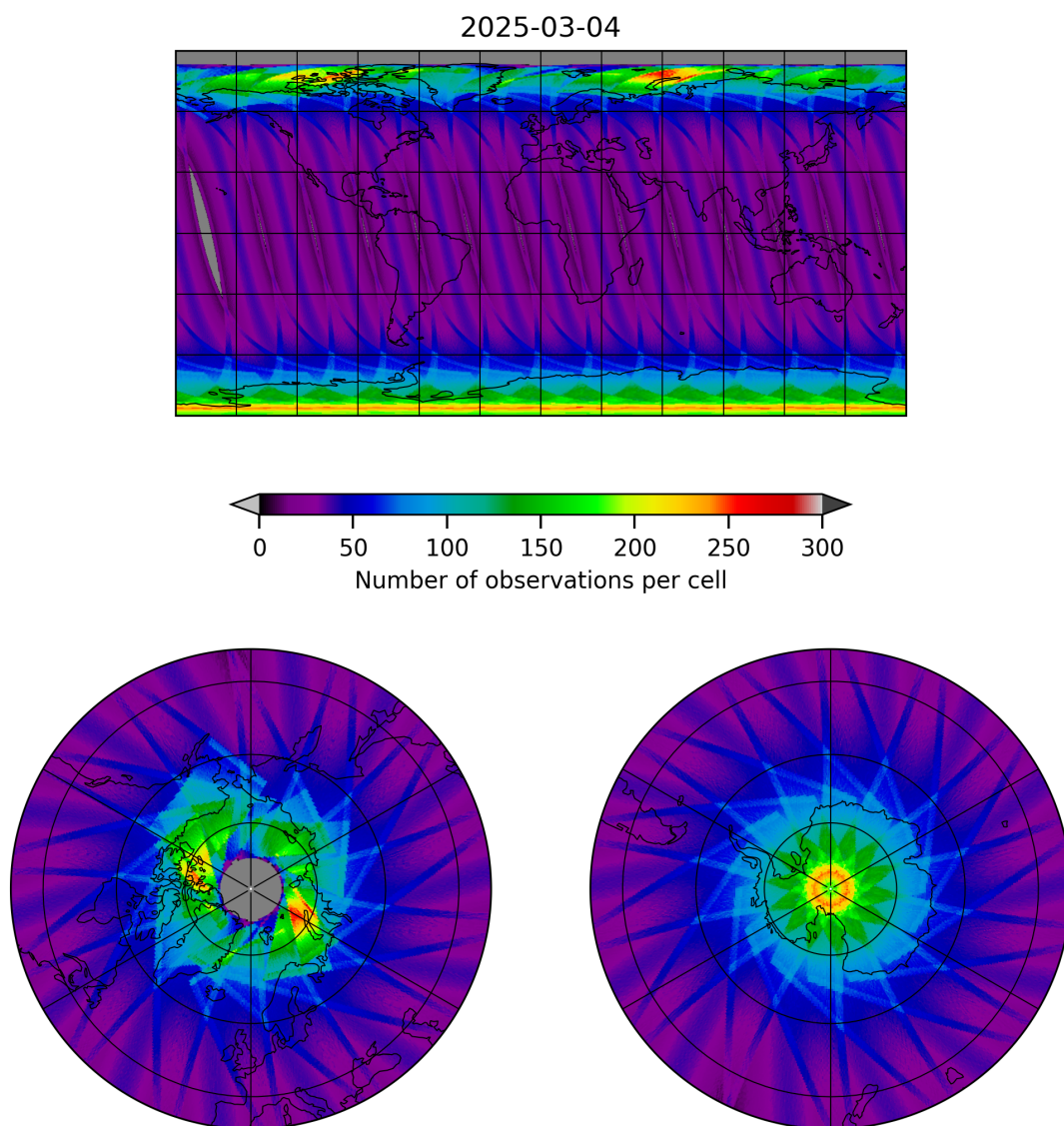
Figure 15: Map of the number of observations for 2025-03-04 to 2025-03-04
