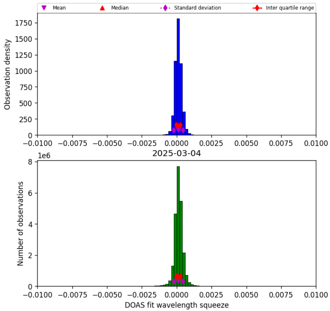
Figure 36: Histogram of “DOAS fit wavelength squeeze” for 2025-03-04 to 2025-03-04
