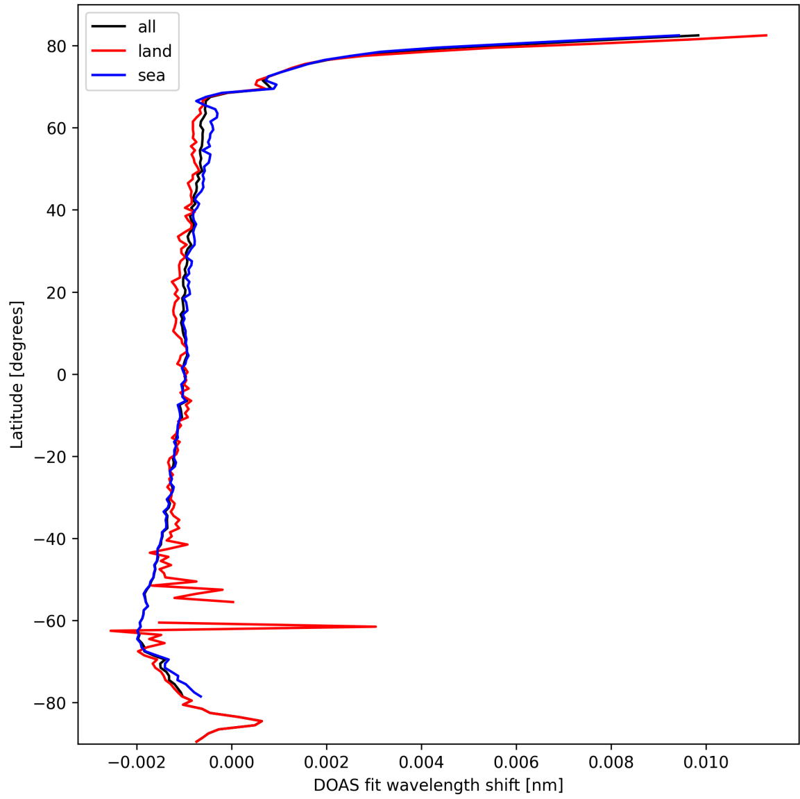
Figure 23: Zonal average of “DOAS fit wavelength shift” for 2025-03-04 to 2025-03-04.
