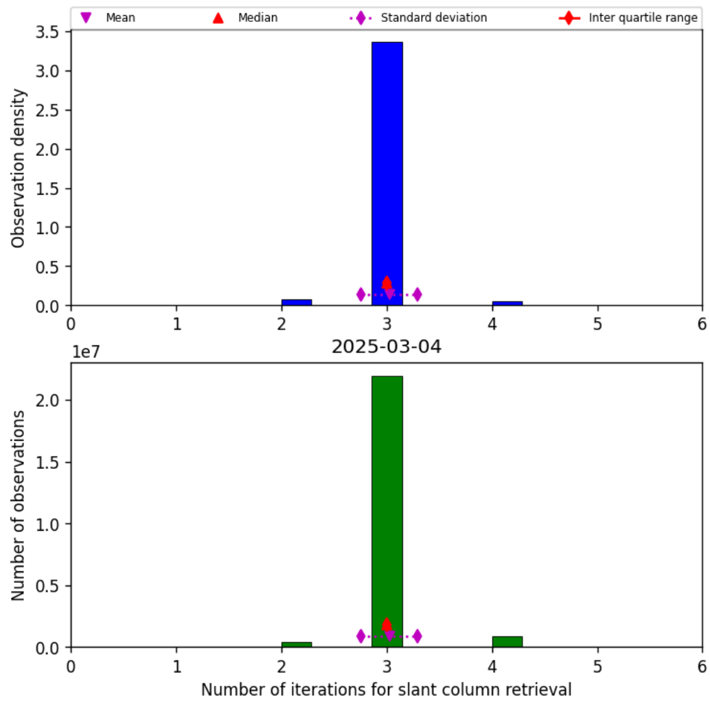
Figure 33: Histogram of “Number of iterations for slant column retrieval” for 2025-03-04 to 2025-03-04
