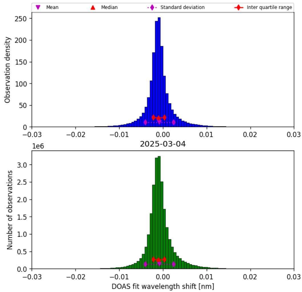
Figure 35: Histogram of “DOAS fit wavelength shift” for 2025-03-04 to 2025-03-04
