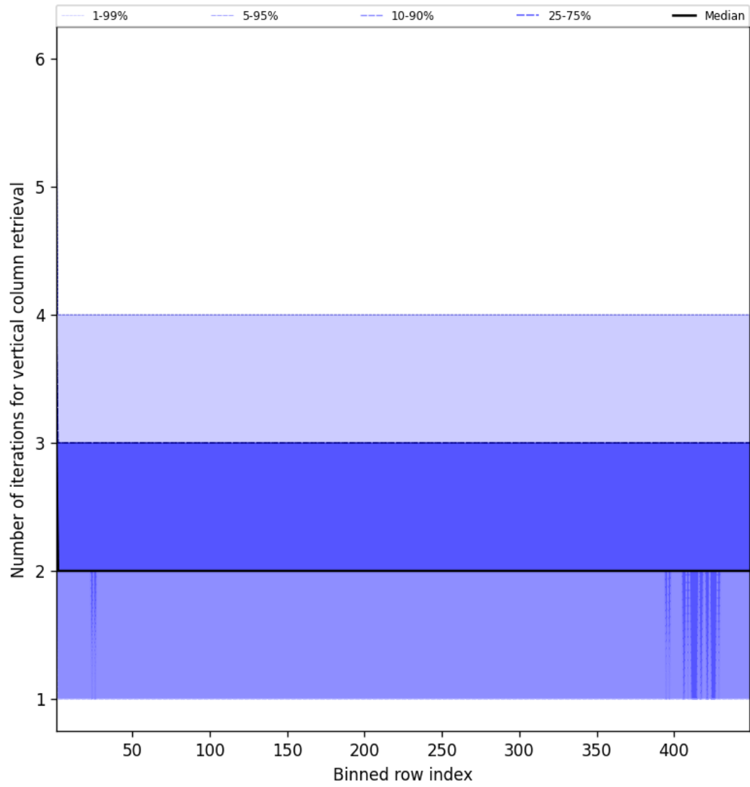
Figure 51: Along track statistics of “Number of iterations for vertical column retrieval” for 2025-03-04 to 2025-03-04
