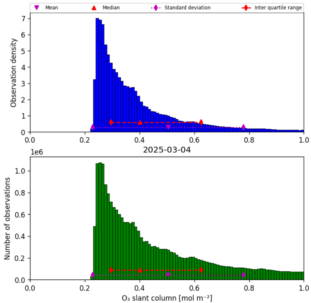
Figure 31: Histogram of “O 3 slant column” for 2025-03-04 to 2025-03-04
