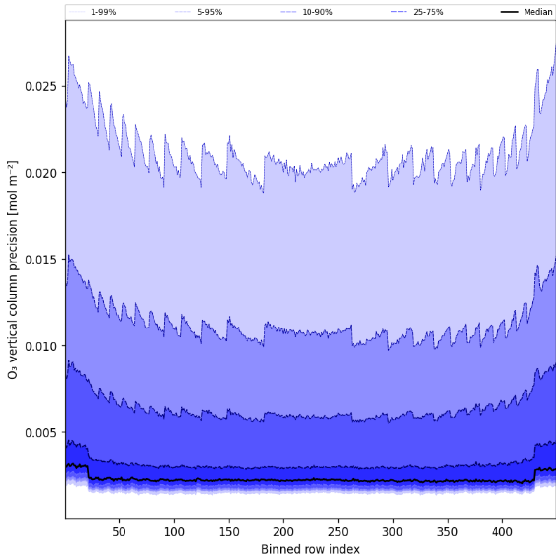
Figure 42: Along track statistics of “O 3 vertical column precision” for 2025-03-04 to 2025-03-04
