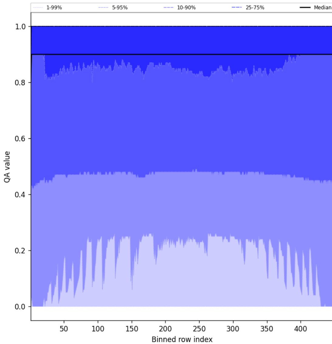
Figure 40: Along track statistics of “QA value” for 2025-03-04 to 2025-03-04
