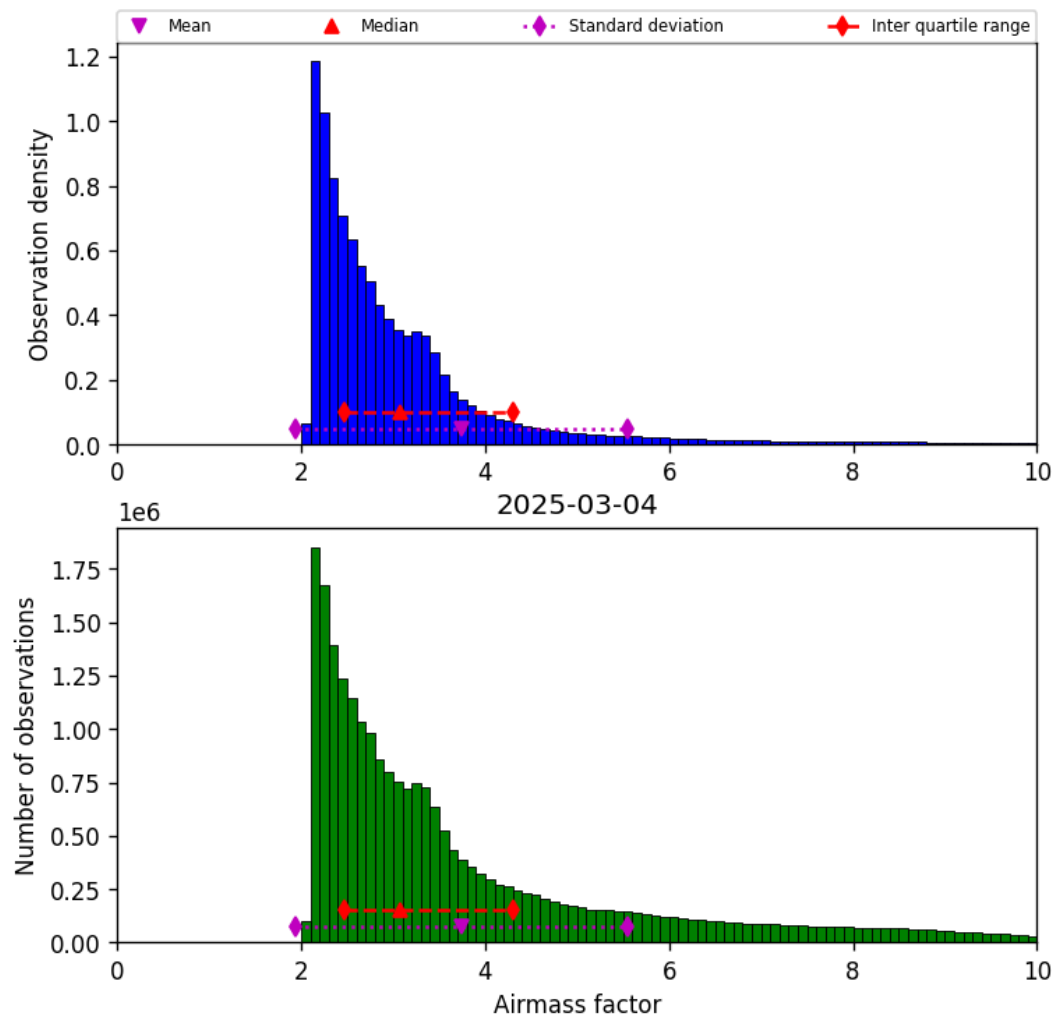
Figure 37: Histogram of “Airmass factor” for 2025-03-04 to 2025-03-04
