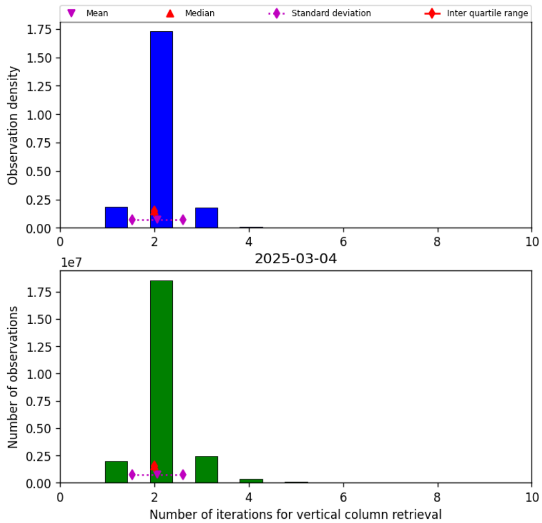
Figure 39: Histogram of “Number of iterations for vertical column retrieval” for 2025-03-04 to 2025-03-04
