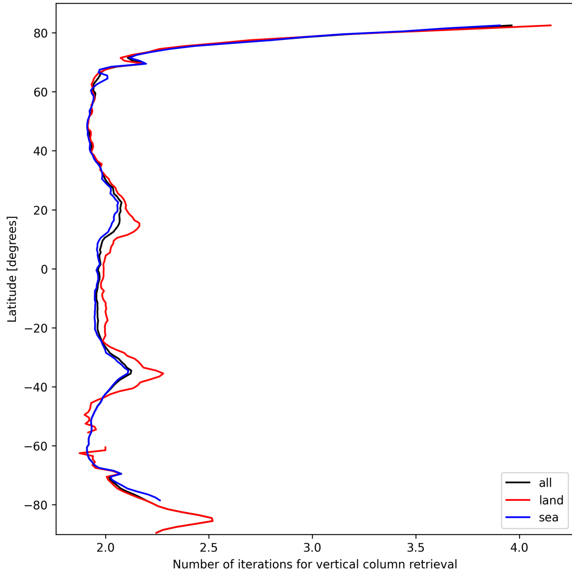
Figure 27: Zonal average of “Number of iterations for vertical column retrieval” for 2025-03-04 to 2025-03-04.
