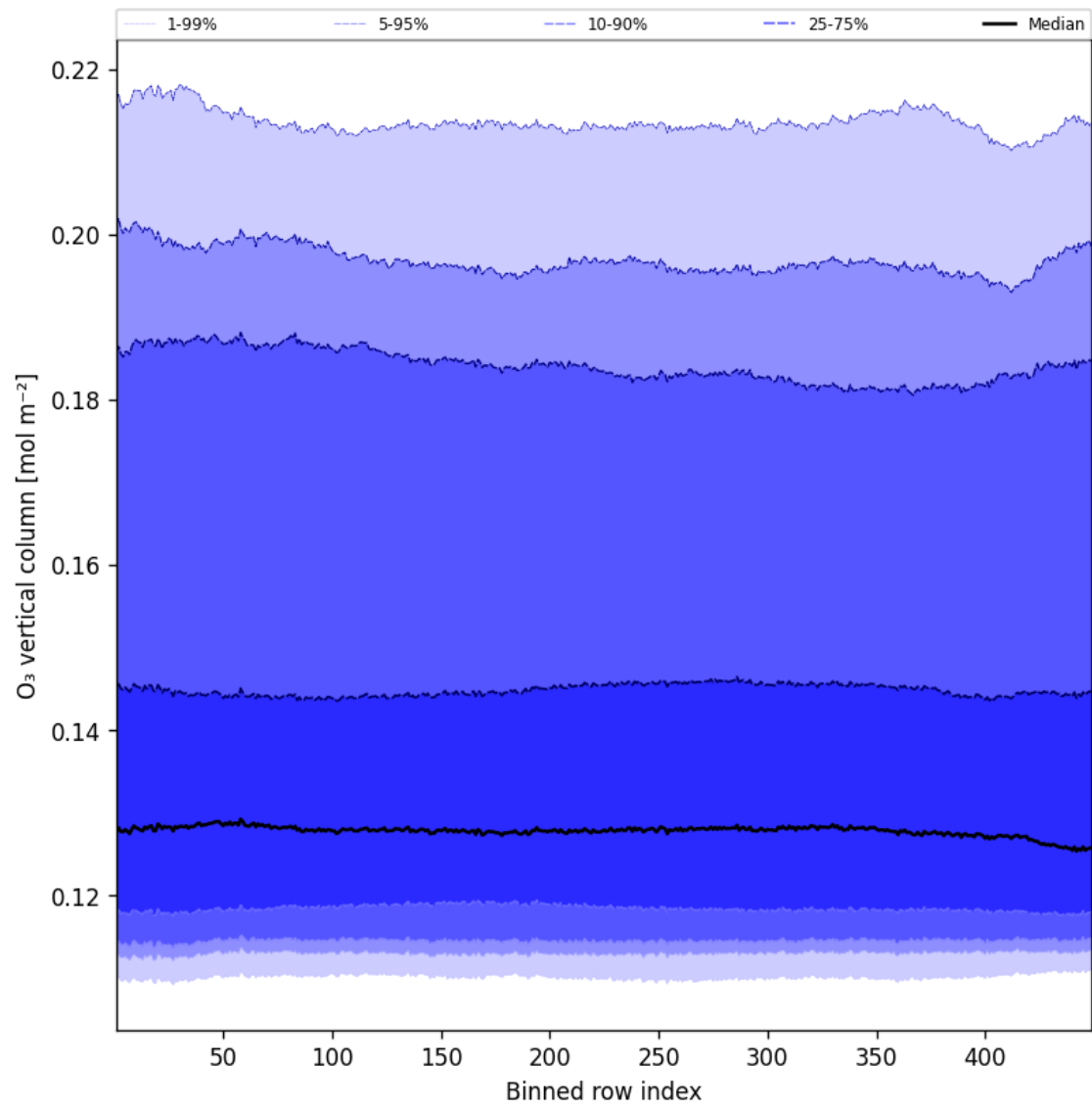
Figure 41: Along track statistics of “ \text{O}_3 vertical column” for 2025-03-04 to 2025-03-04
