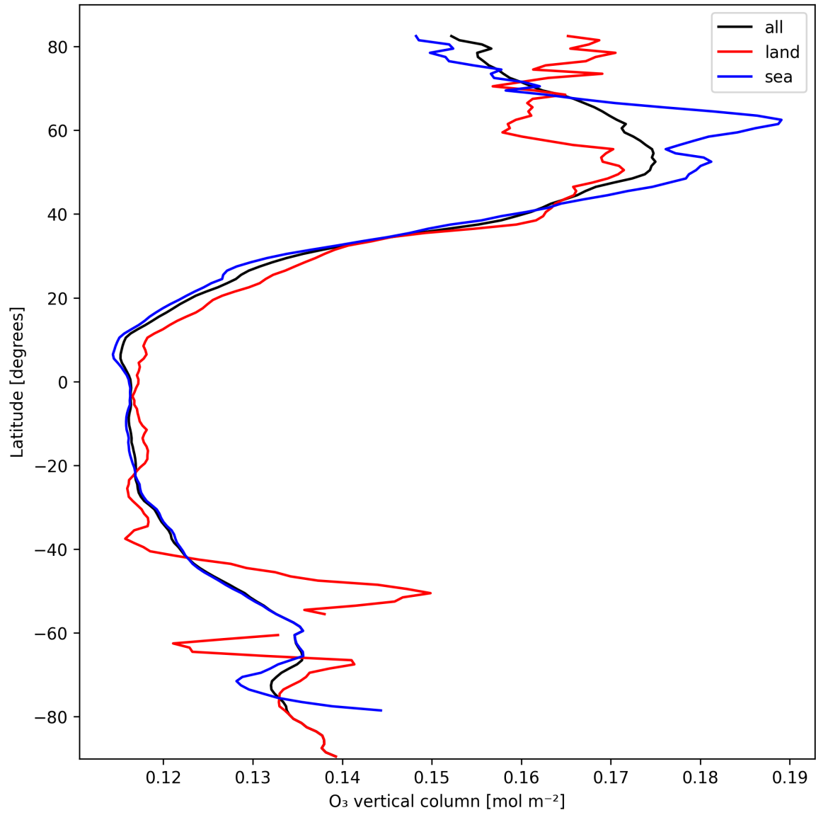
Figure 17: Zonal average of “O 3 vertical column” for 2025-03-04 to 2025-03-04.
