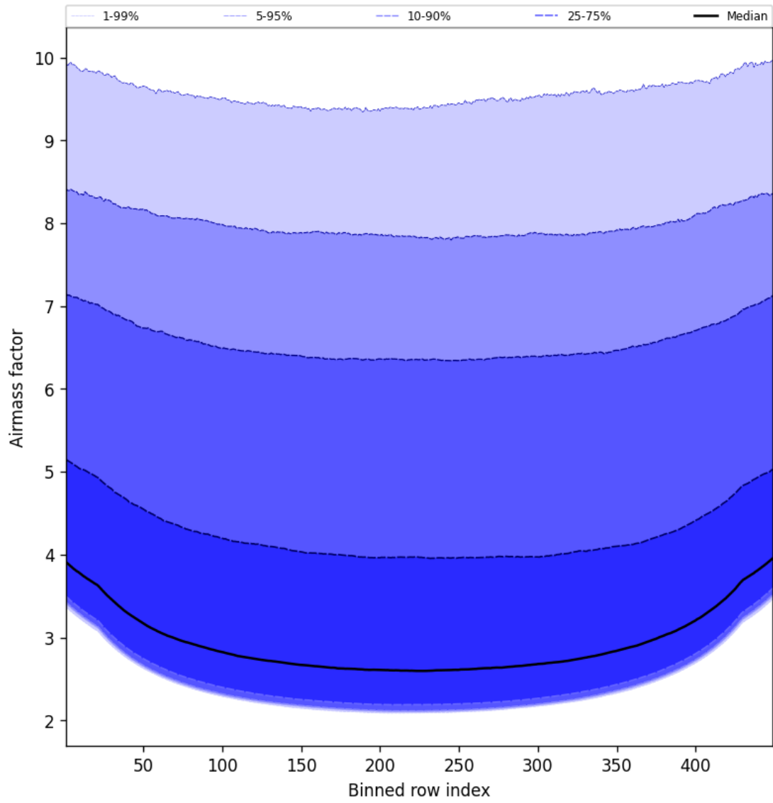
Figure 49: Along track statistics of “Airmass factor” for 2025-03-04 to 2025-03-04
