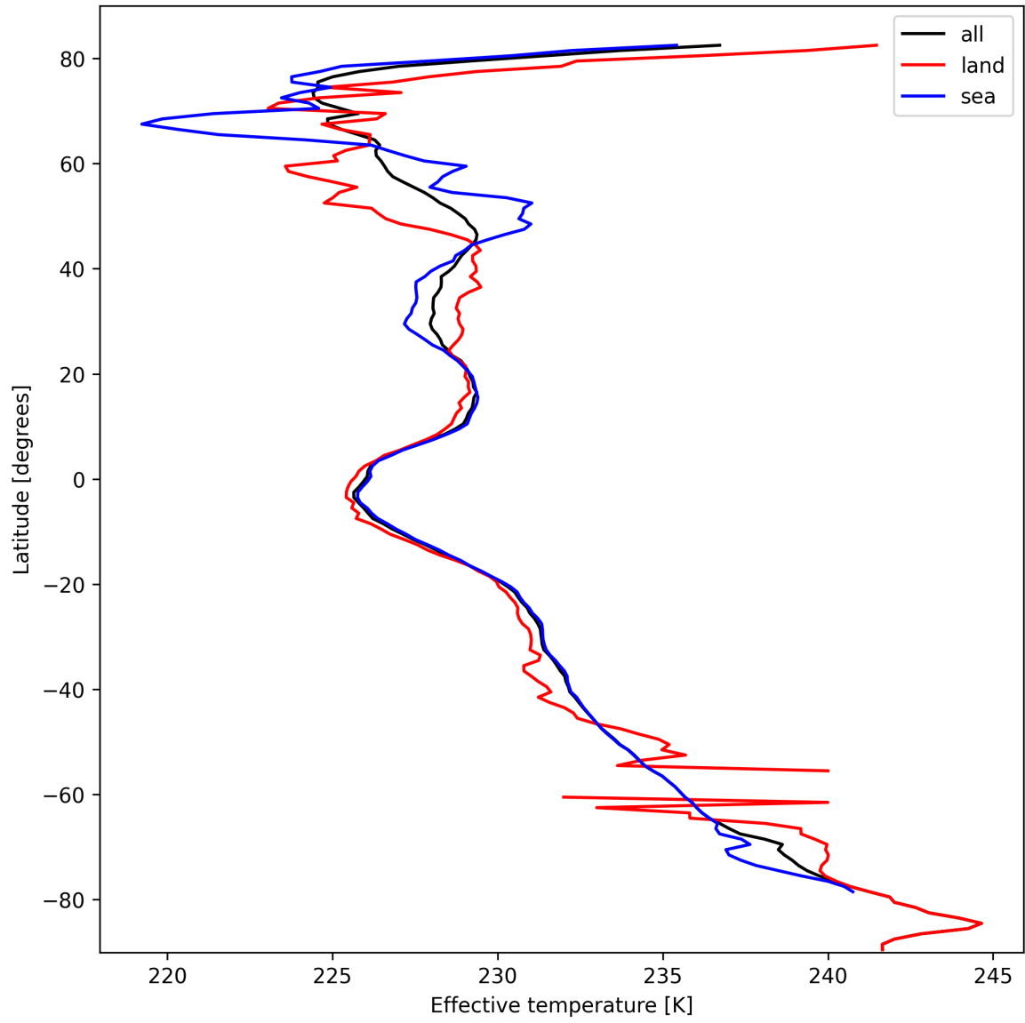
Figure 26: Zonal average of “Effective temperature” for 2025-03-04 to 2025-03-04.
