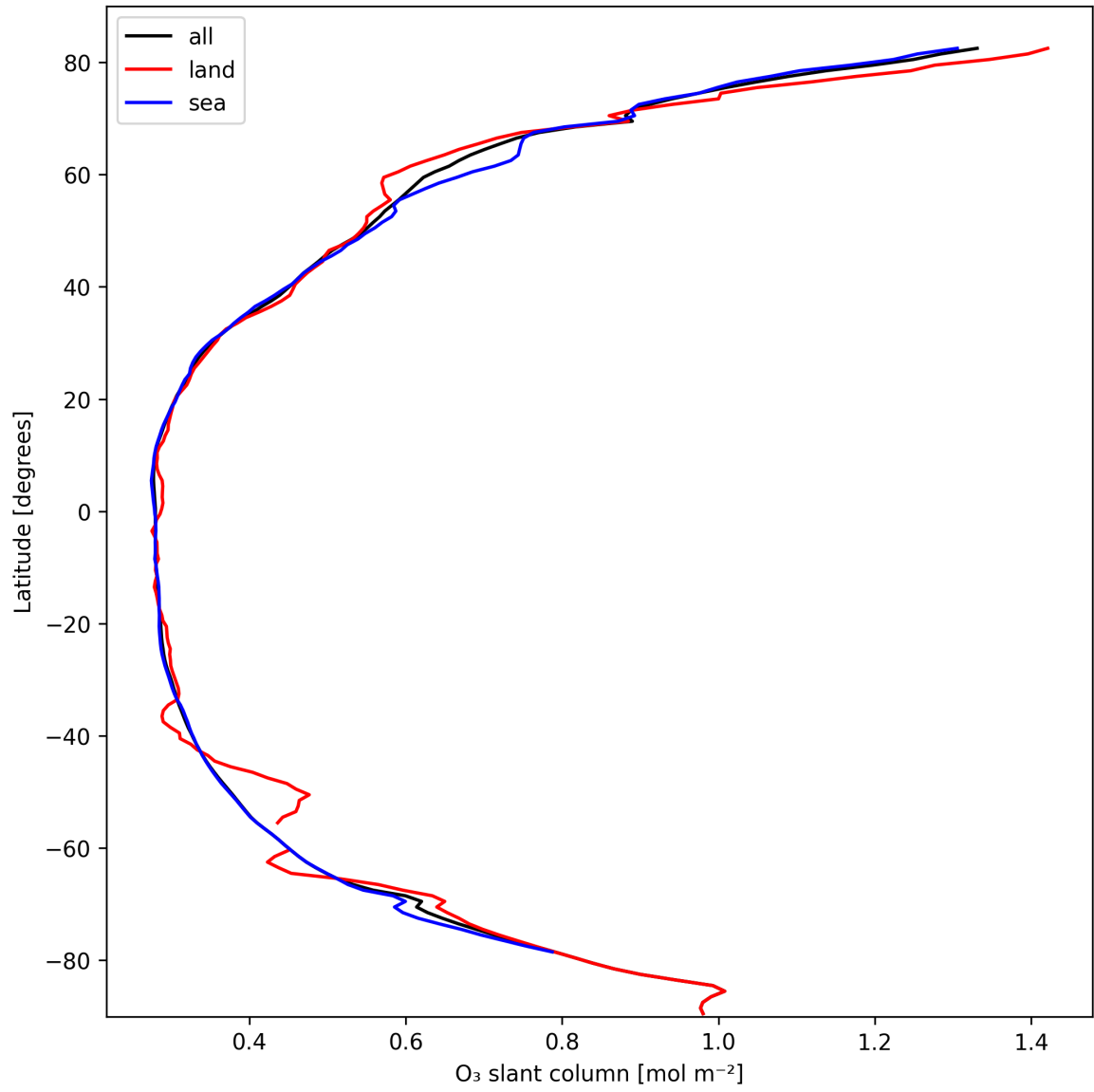
Figure 19: Zonal average of “O 3 slant column” for 2025-03-04 to 2025-03-04.
