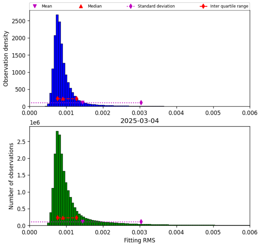
Figure 34: Histogram of “Fitting RMS” for 2025-03-04 to 2025-03-04
