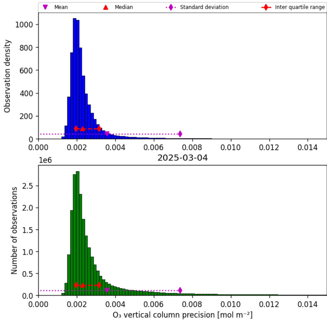
Figure 30: Histogram of "O 3 vertical column precision" for 2025-03-04 to 2025-03-04
