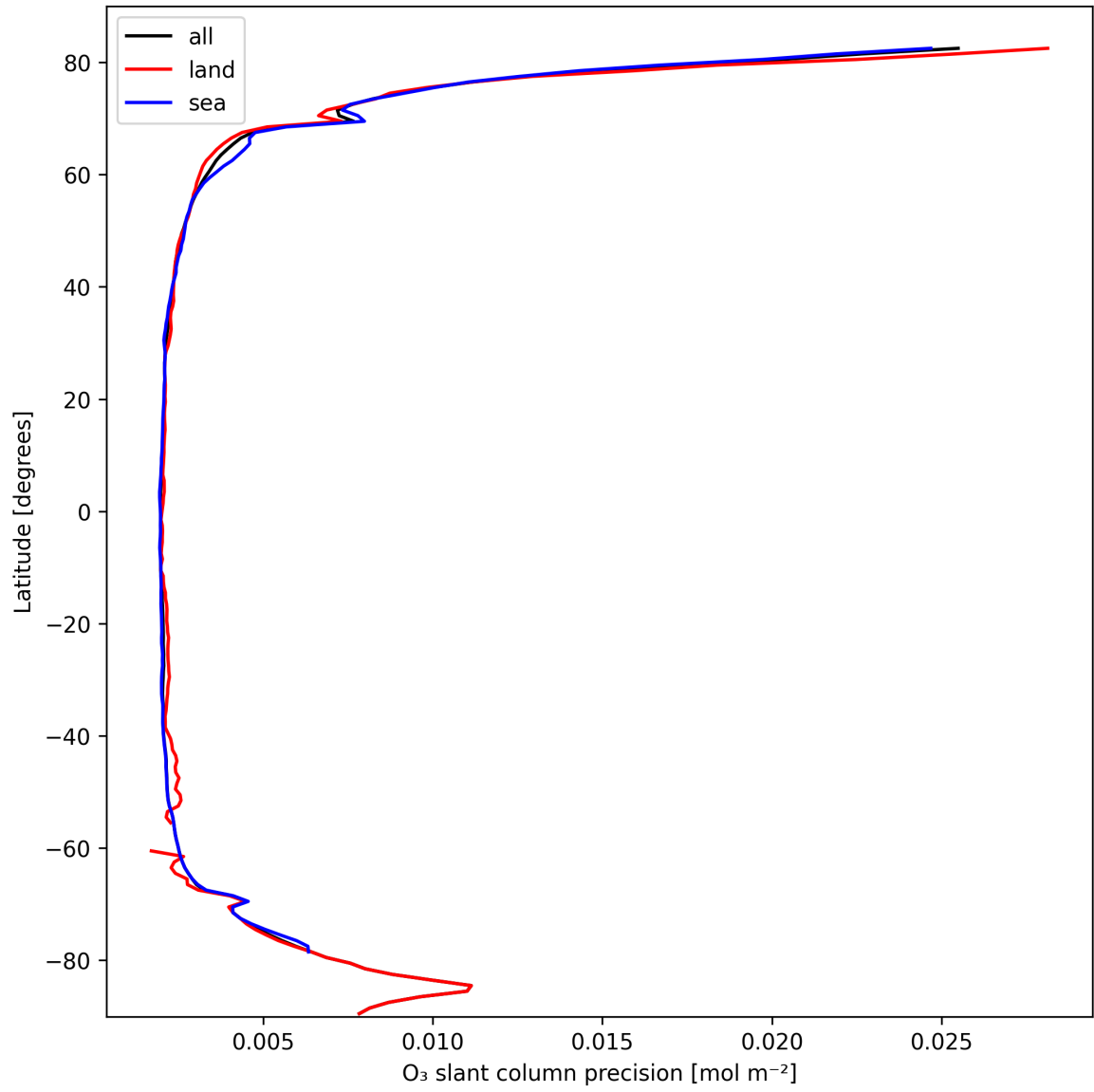
Figure 20: Zonal average of “O 3 slant column precision” for 2025-03-04 to 2025-03-04.
