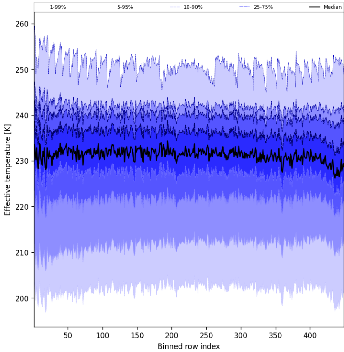
Figure 50: Along track statistics of “Effective temperature” for 2025-03-04 to 2025-03-04
