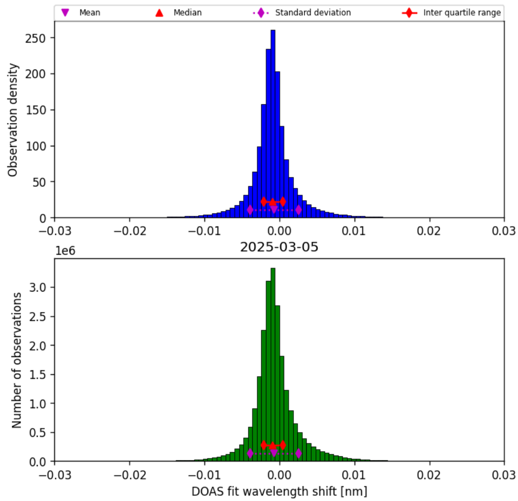
Figure 35: Histogram of “DOAS fit wavelength shift” for 2025-03-05 to 2025-03-05
