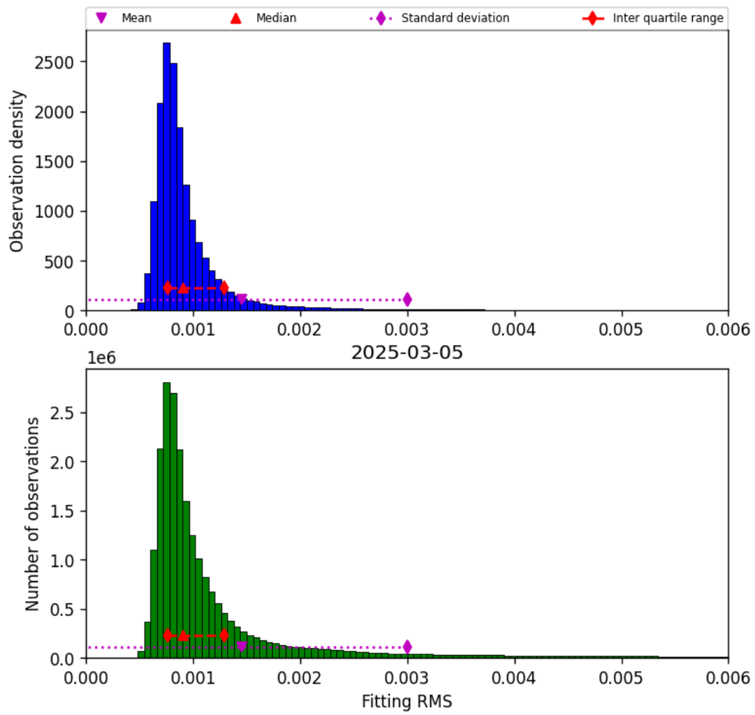
Figure 34: Histogram of “Fitting RMS” for 2025-03-05 to 2025-03-05
