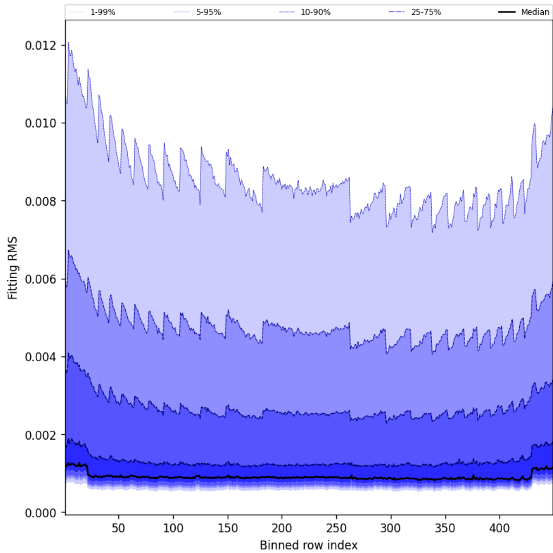
Figure 46: Along track statistics of “Fitting RMS” for 2025-03-05 to 2025-03-05
