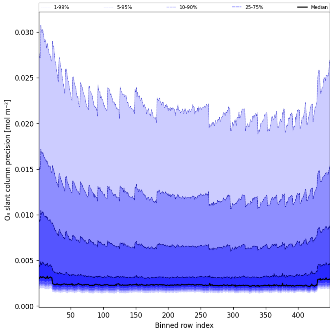
Figure 44: Along track statistics of “O 3 slant column precision” for 2025-03-05 to 2025-03-05
