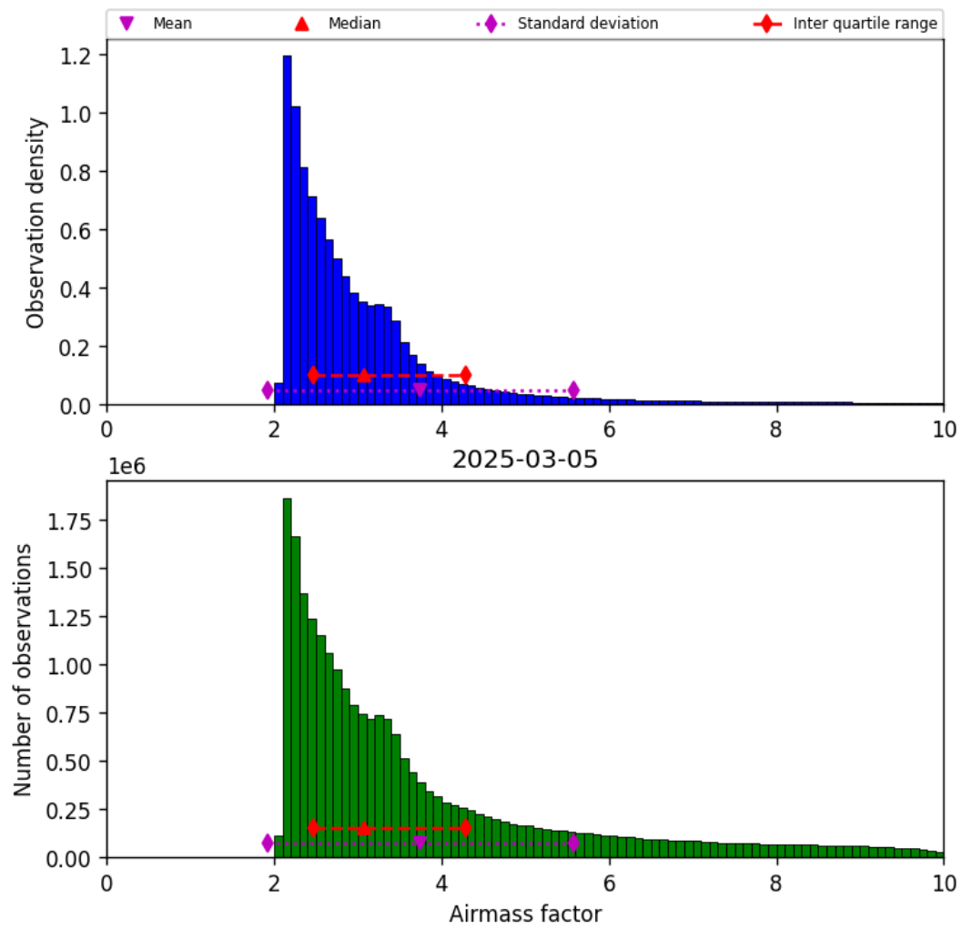
Figure 37: Histogram of “Airmass factor” for 2025-03-05 to 2025-03-05
