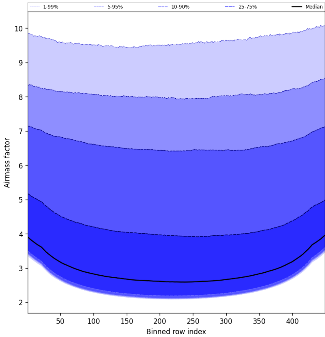
Figure 49: Along track statistics of “Airmass factor” for 2025-03-05 to 2025-03-05
