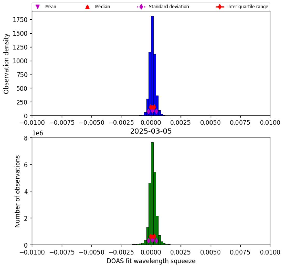
Figure 36: Histogram of “DOAS fit wavelength squeeze” for 2025-03-05 to 2025-03-05
