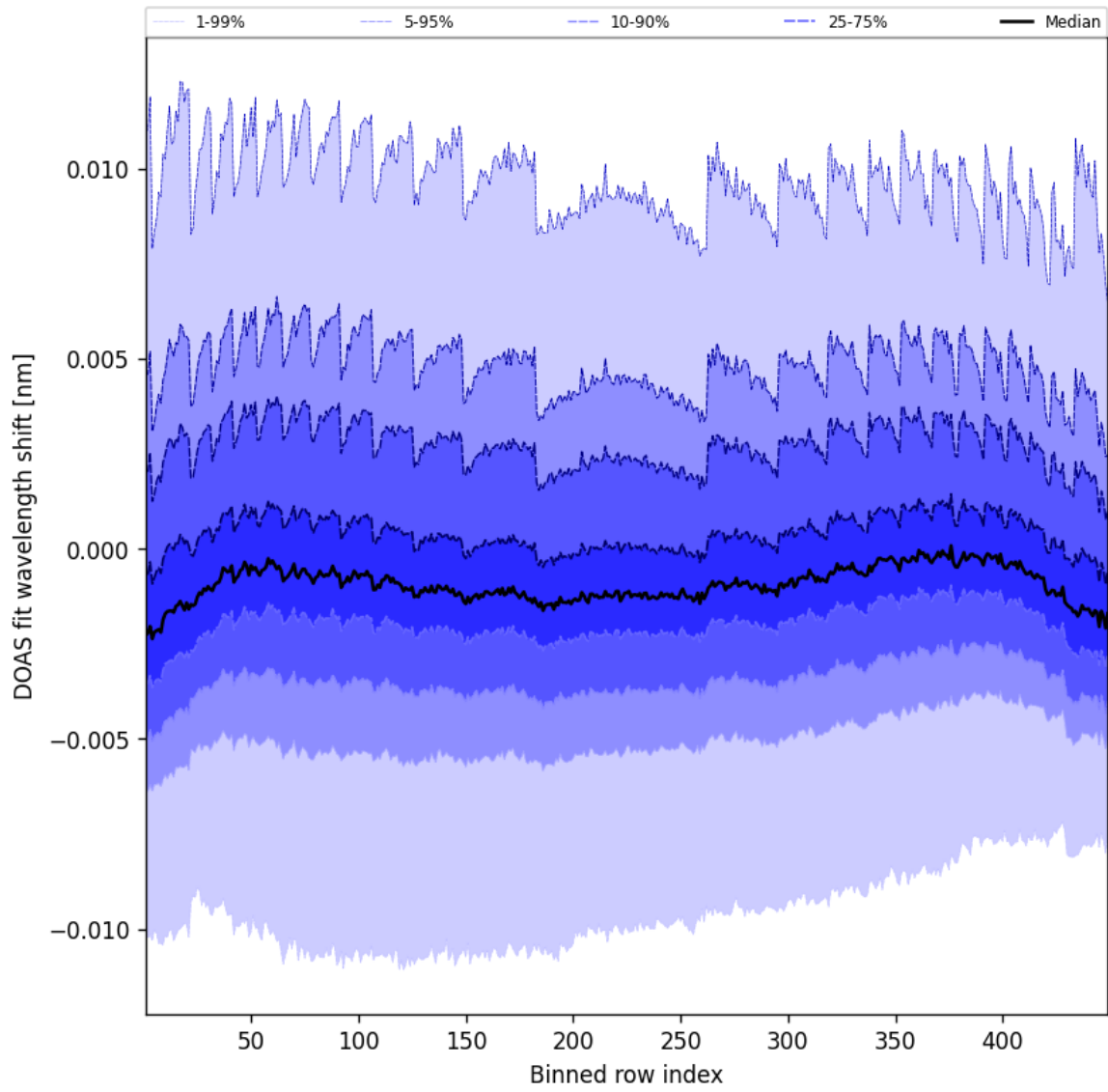
Figure 47: Along track statistics of “DOAS fit wavelength shift” for 2025-03-05 to 2025-03-05
