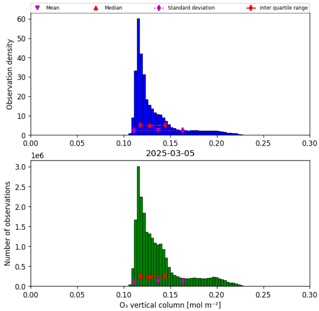
Figure 29: Histogram of “O 3 vertical column” for 2025-03-05 to 2025-03-05
