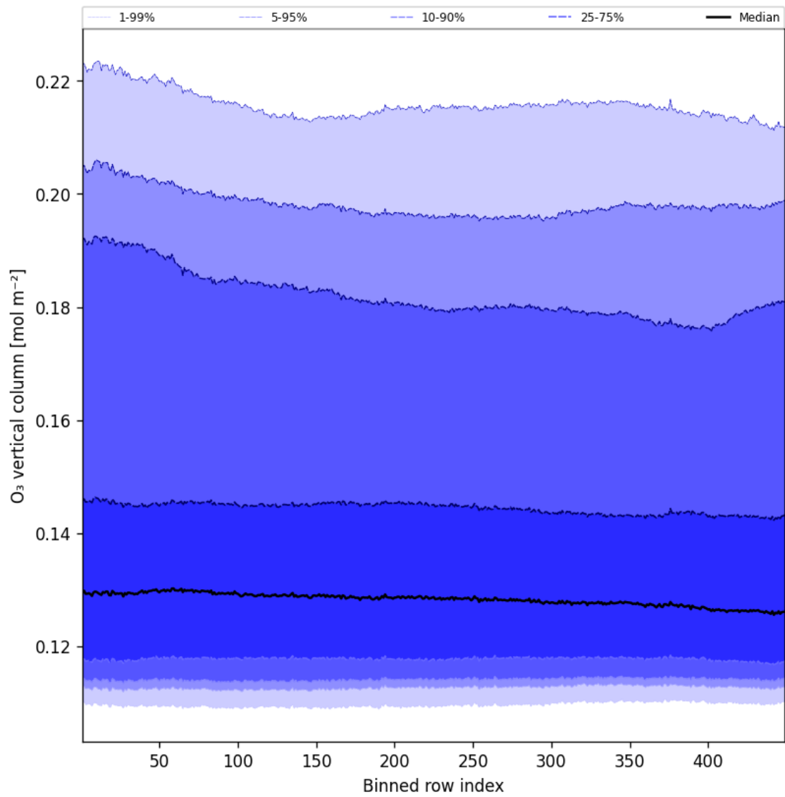
Figure 41: Along track statistics of “O 3 vertical column” for 2025-03-05 to 2025-03-05
