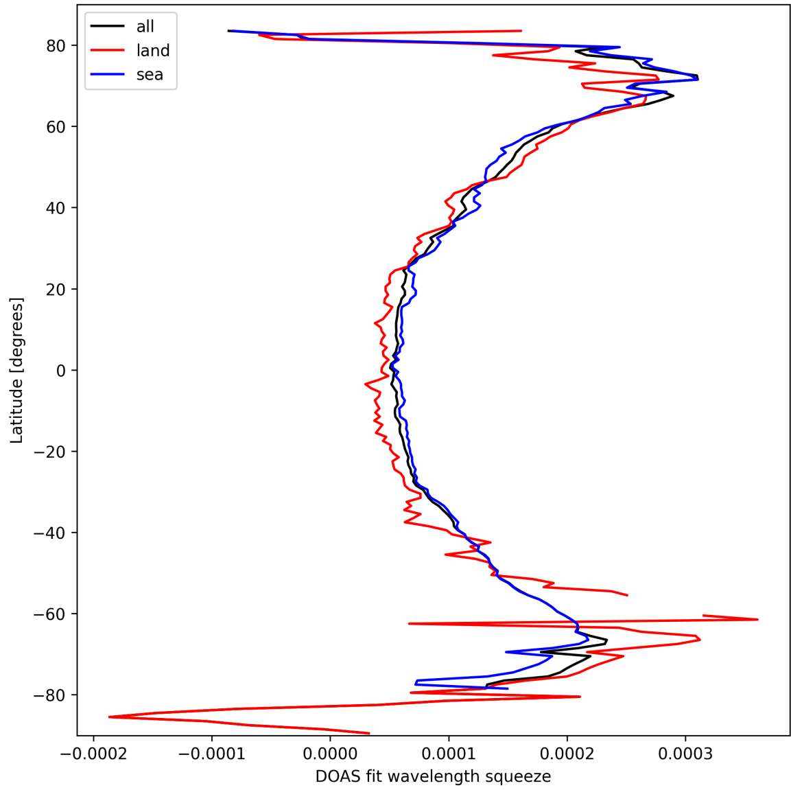
Figure 24: Zonal average of “DOAS fit wavelength squeeze” for 2025-03-05 to 2025-03-05.
