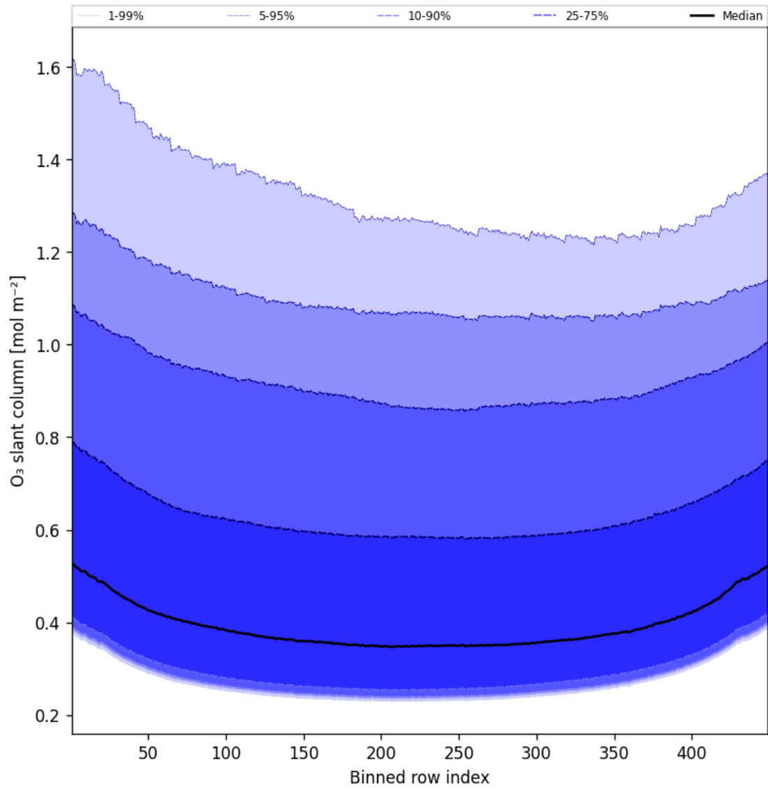
Figure 43: Along track statistics of “O 3 slant column” for 2025-03-05 to 2025-03-05
