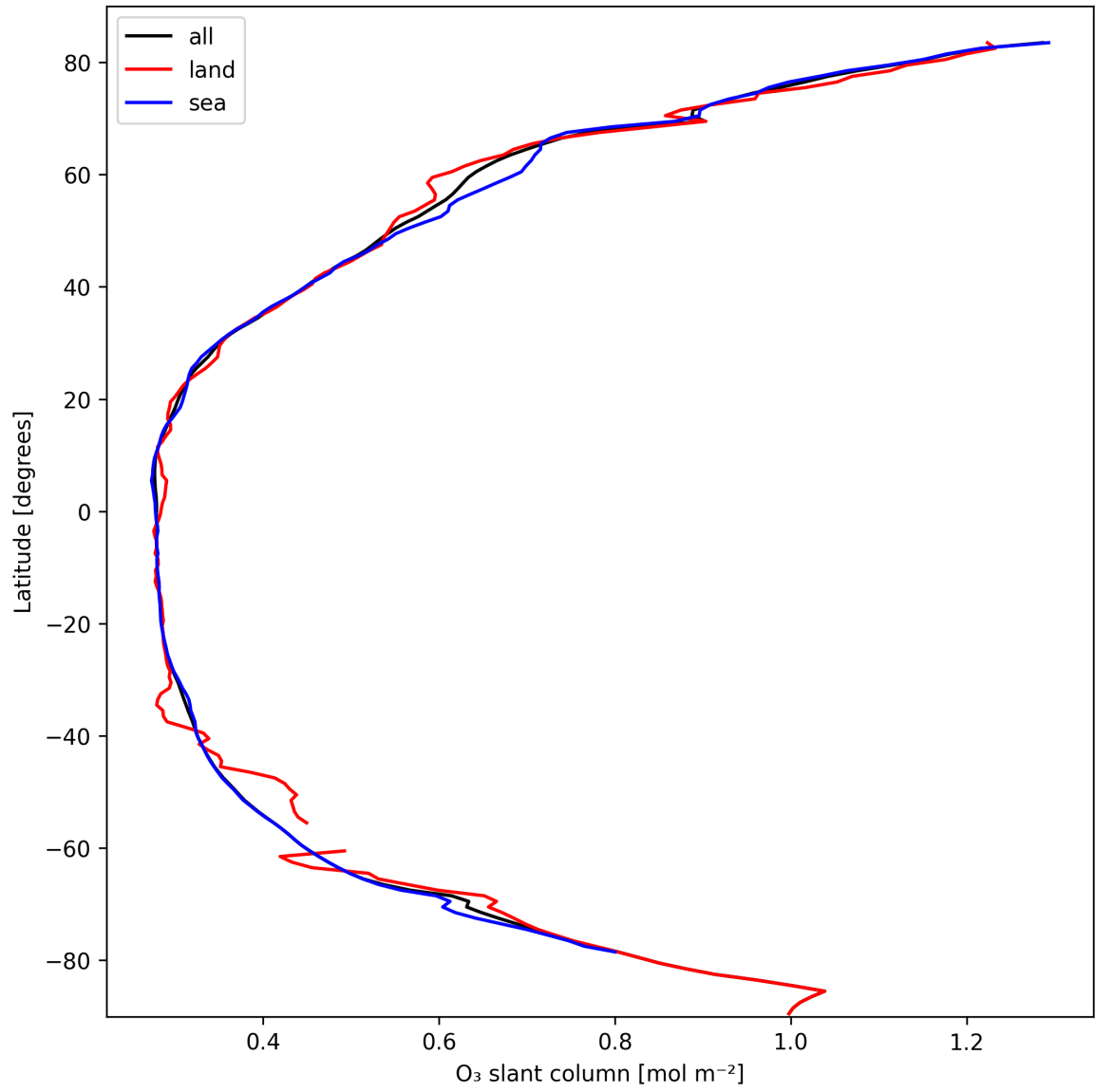
Figure 19: Zonal average of “O 3 slant column” for 2025-03-05 to 2025-03-05.
