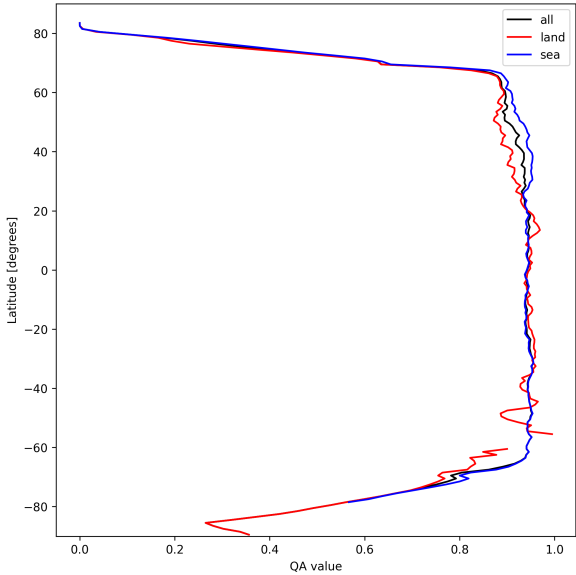
Figure 16: Zonal average of “QA value” for 2025-03-05 to 2025-03-05.
