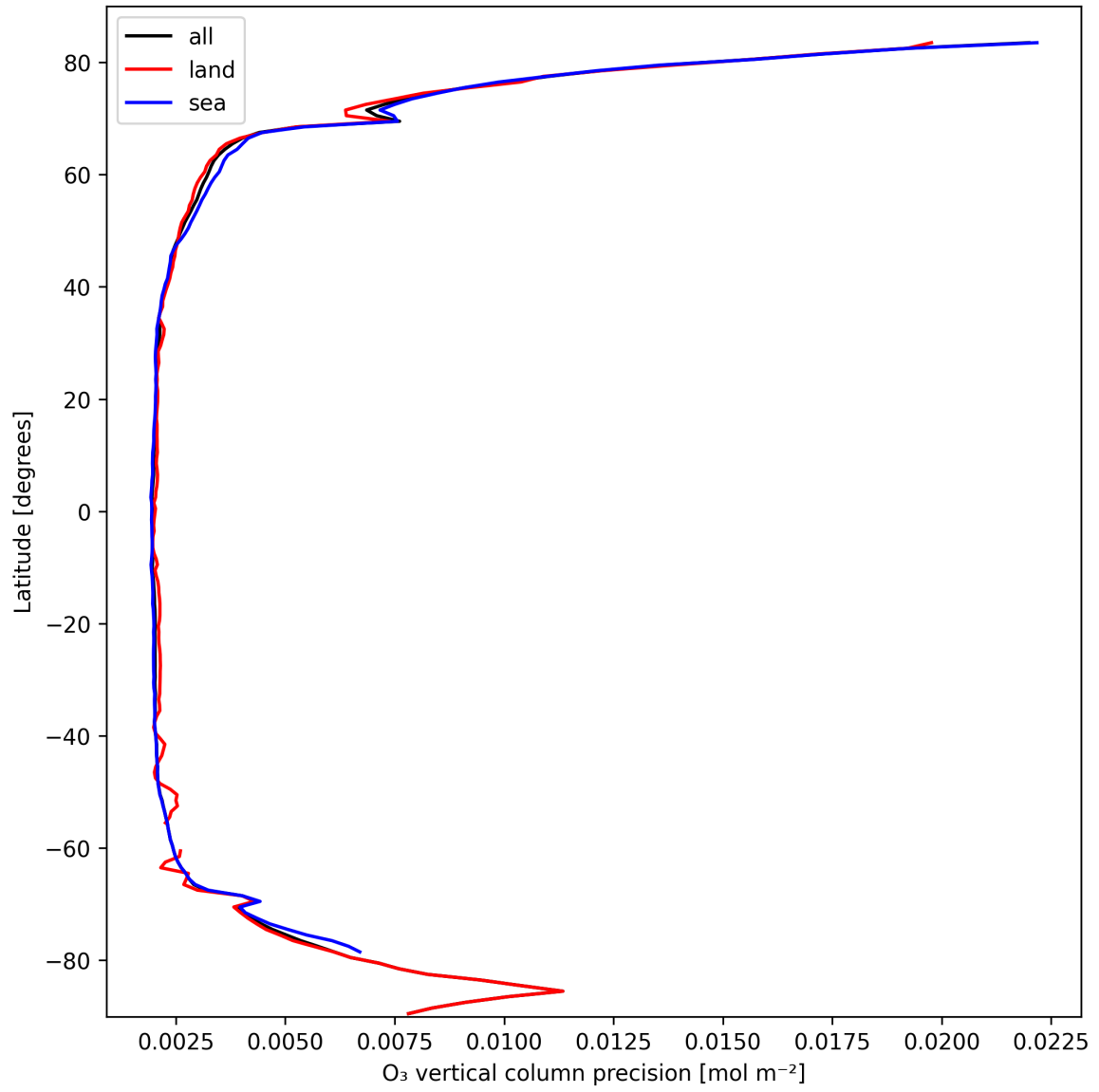
Figure 18: Zonal average of “O 3 vertical column precision” for 2025-03-05 to 2025-03-05.
