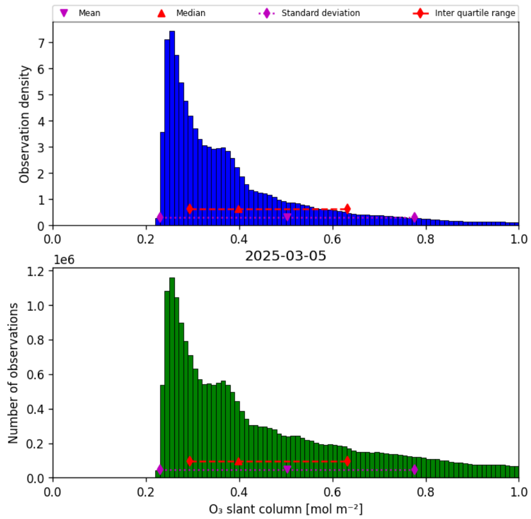
Figure 31: Histogram of “O 3 slant column” for 2025-03-05 to 2025-03-05
