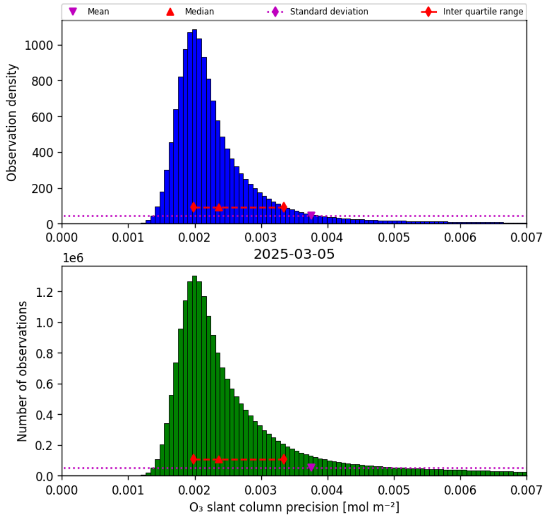
Figure 32: Histogram of “O 3 slant column precision” for 2025-03-05 to 2025-03-05
