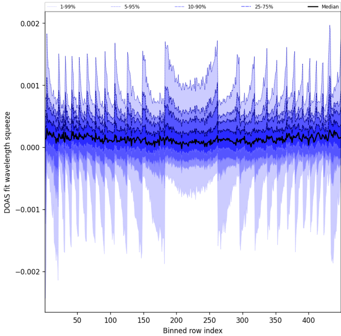
Figure 48: Along track statistics of “DOAS fit wavelength squeeze” for 2025-03-05 to 2025-03-05
