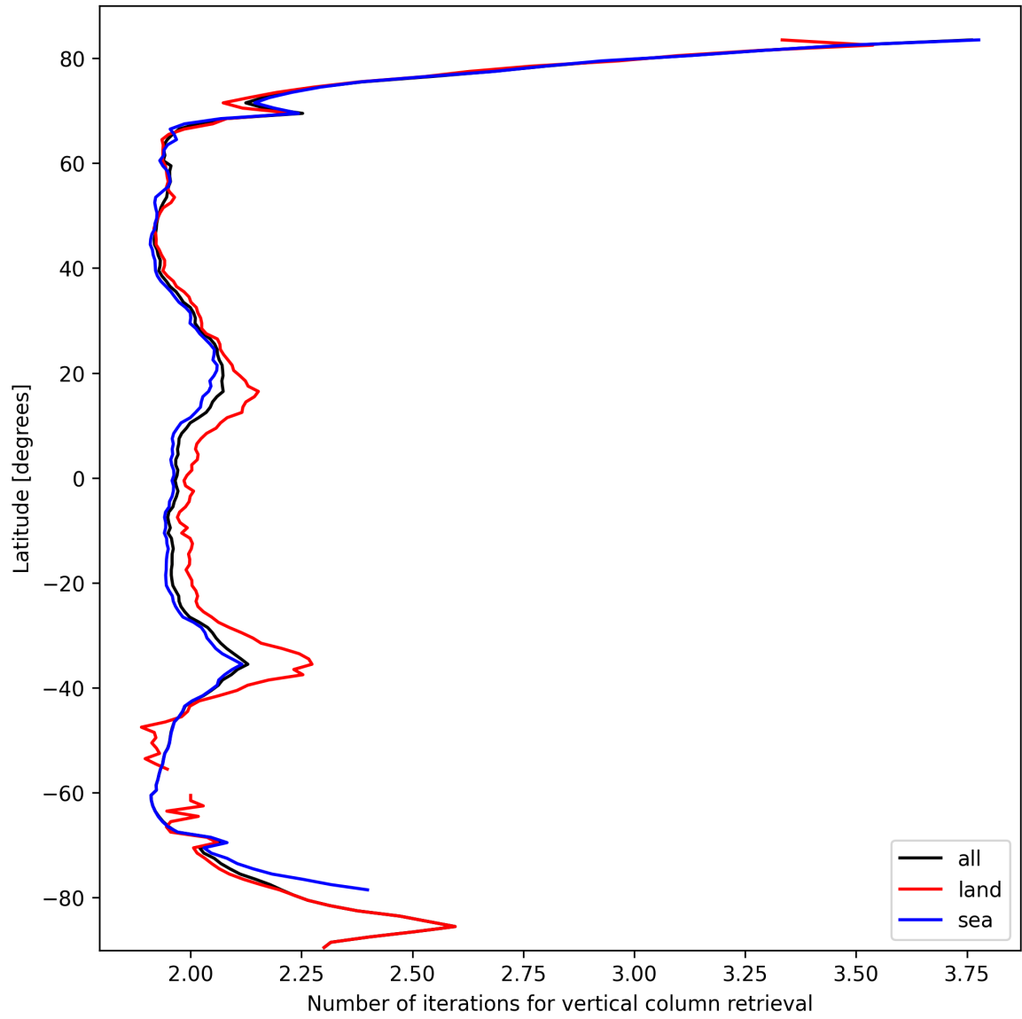
Figure 27: Zonal average of “Number of iterations for vertical column retrieval” for 2025-03-05 to 2025-03-05.
