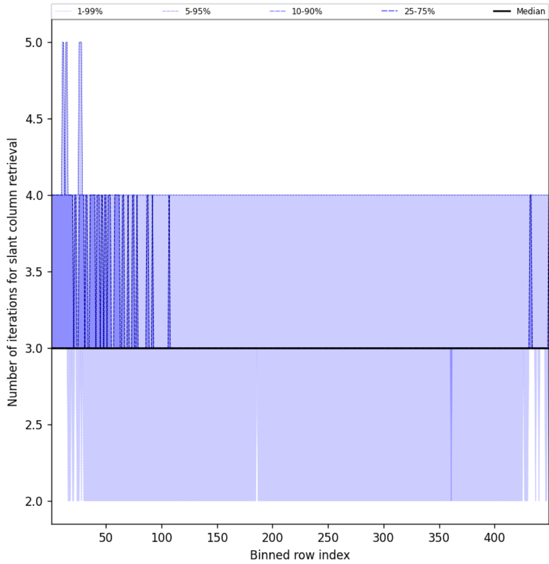
Figure 45: Along track statistics of “Number of iterations for slant column retrieval” for 2025-03-05 to 2025-03-05
