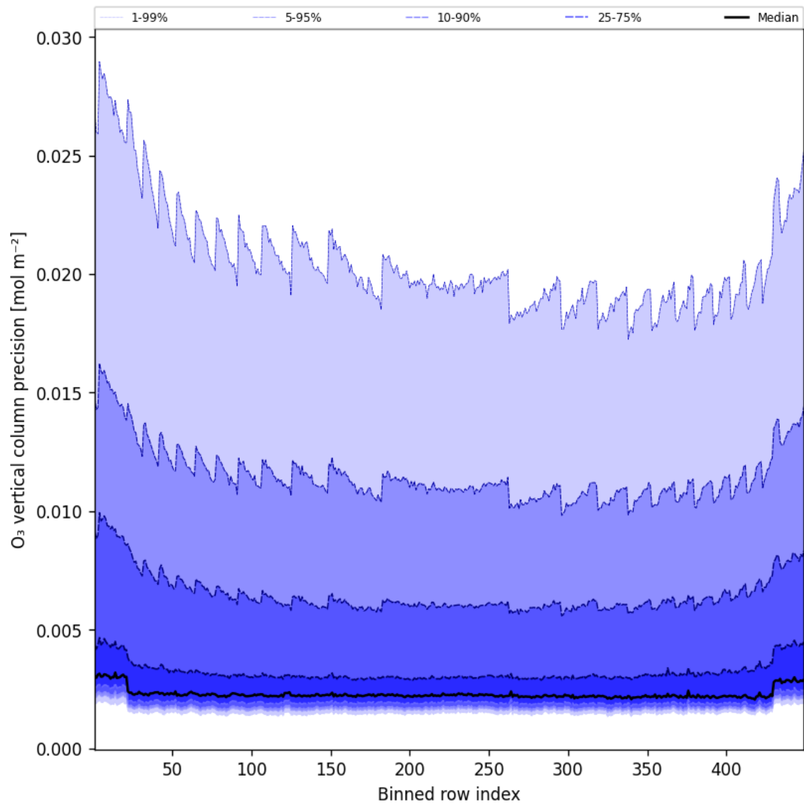
Figure 42: Along track statistics of “O 3 vertical column precision” for 2025-03-05 to 2025-03-05
