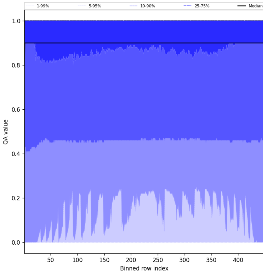
Figure 40: Along track statistics of “QA value” for 2025-03-05 to 2025-03-05
