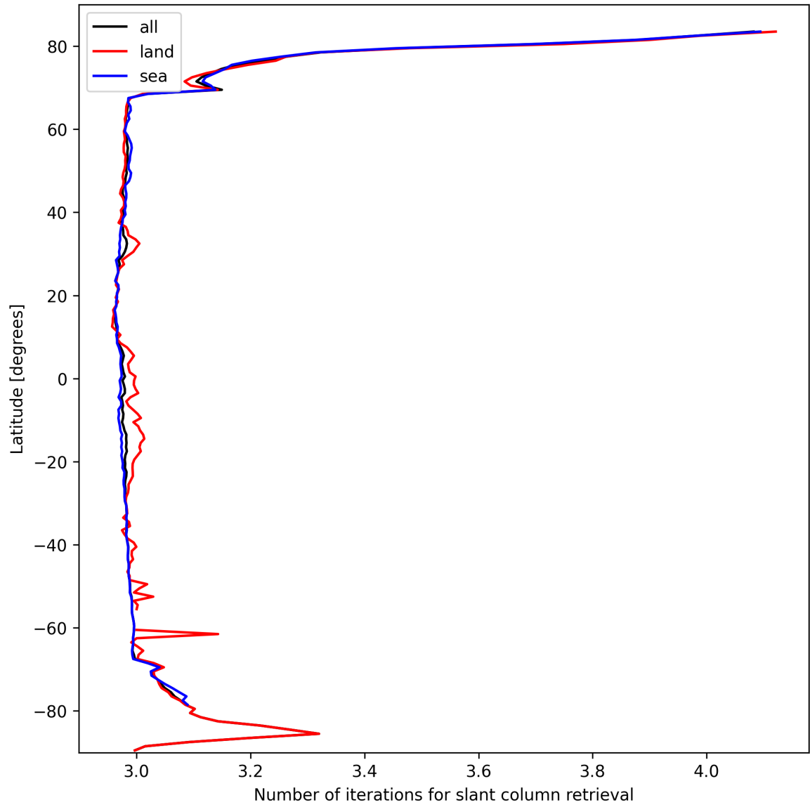
Figure 21: Zonal average of “Number of iterations for slant column retrieval” for 2025-03-05 to 2025-03-05.
