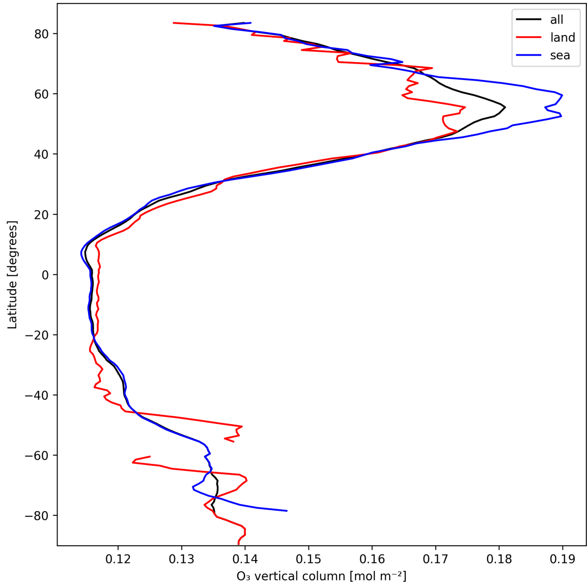
Figure 17: Zonal average of “O 3 vertical column” for 2025-03-05 to 2025-03-05.
