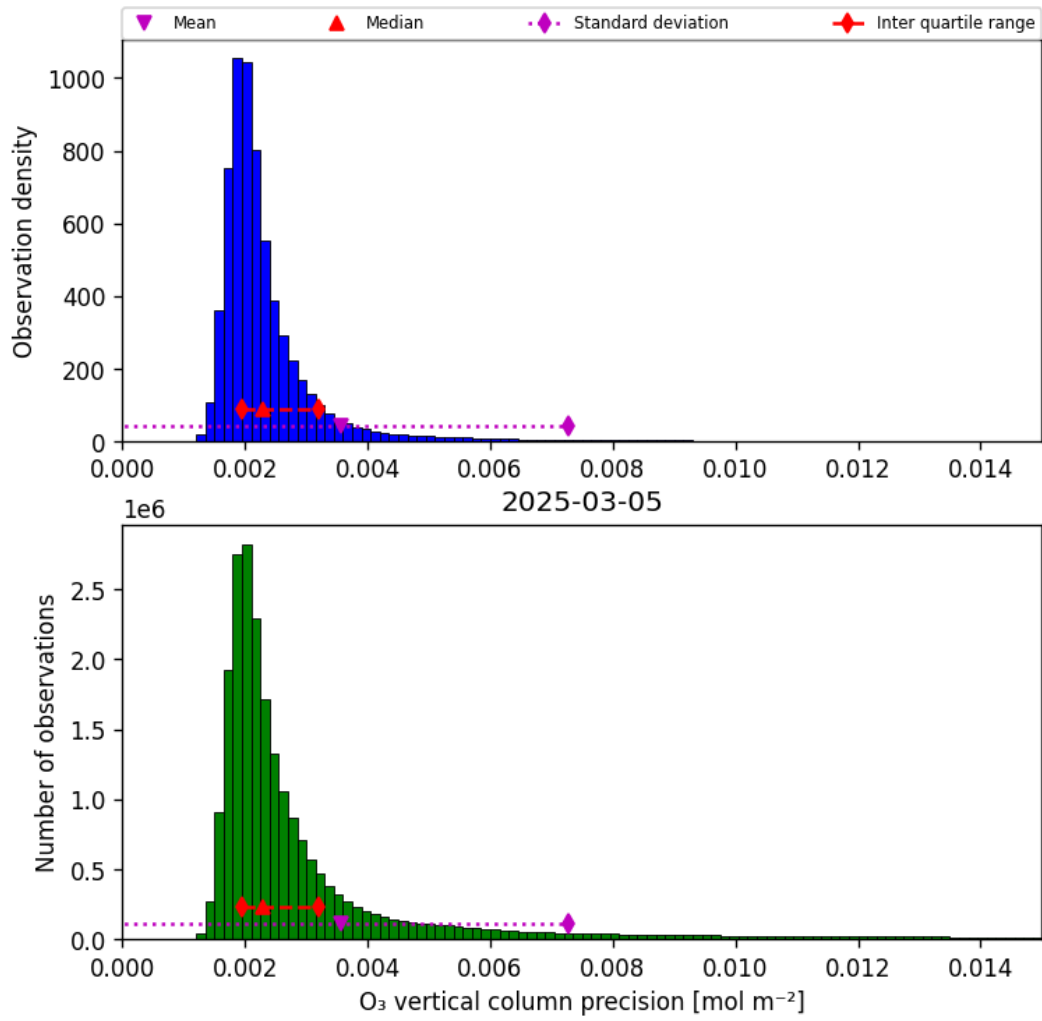
Figure 30: Histogram of "O 3 vertical column precision" for 2025-03-05 to 2025-03-05
