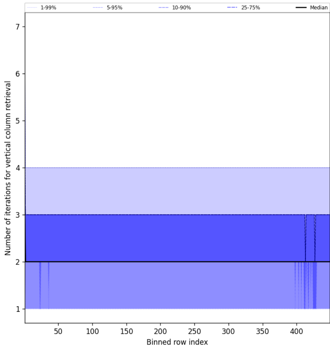
Figure 51: Along track statistics of “Number of iterations for vertical column retrieval” for 2025-03-05 to 2025-03-05
