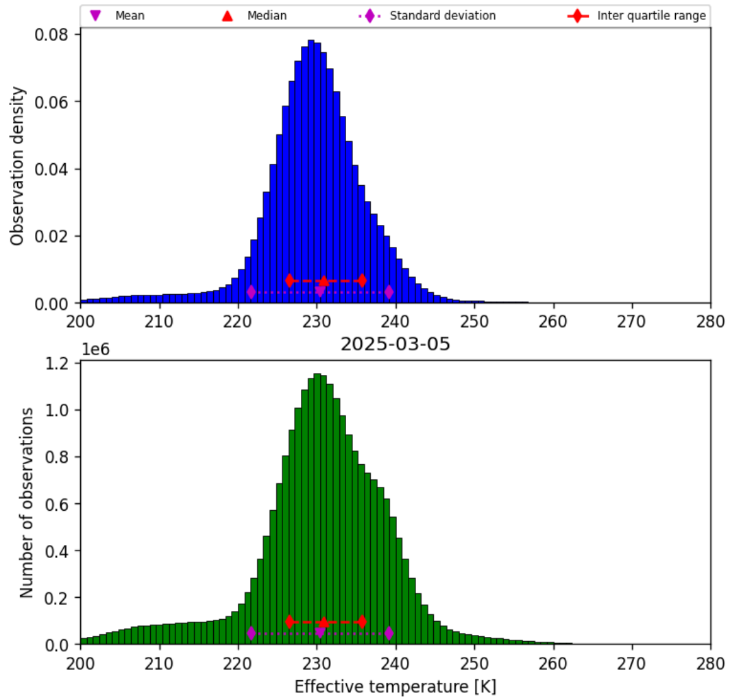
Figure 38: Histogram of “Effective temperature” for 2025-03-05 to 2025-03-05
