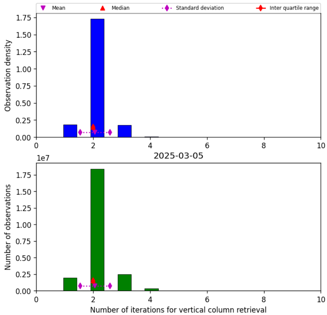
Figure 39: Histogram of “Number of iterations for vertical column retrieval” for 2025-03-05 to 2025-03-05
