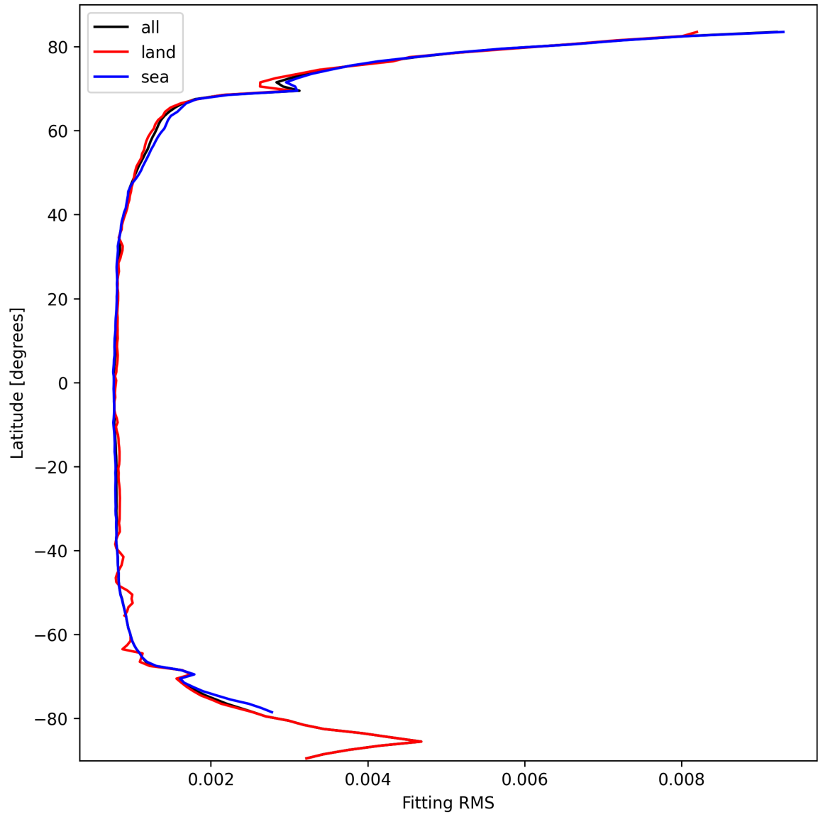
Figure 22: Zonal average of “Fitting RMS” for 2025-03-05 to 2025-03-05.
