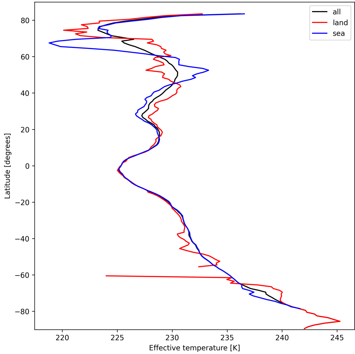
Figure 26: Zonal average of “Effective temperature” for 2025-03-05 to 2025-03-05.
