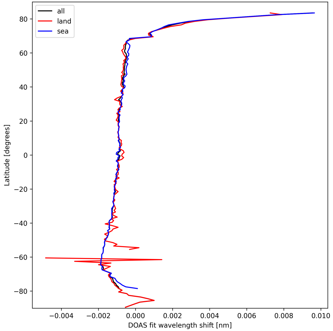
Figure 23: Zonal average of "DOAS fit wavelength shift" for 2025-03-05 to 2025-03-05.
