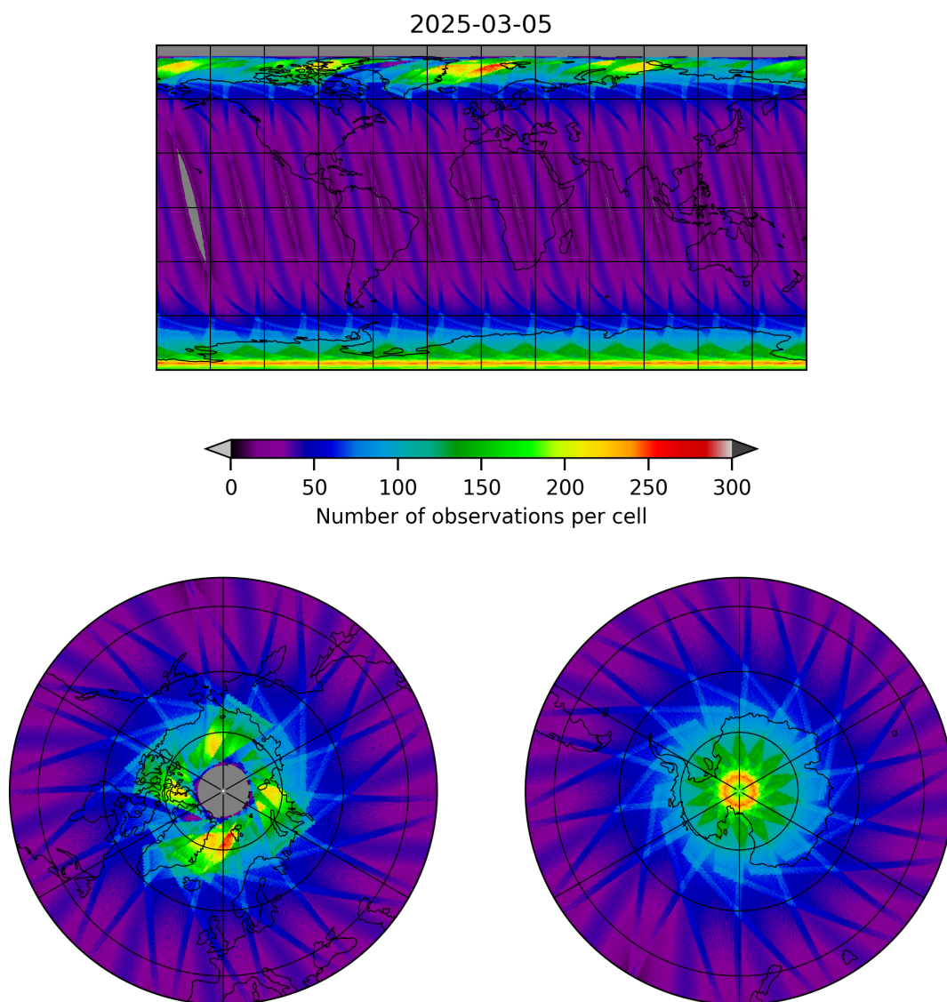
Figure 15: Map of the number of observations for 2025-03-05 to 2025-03-05
