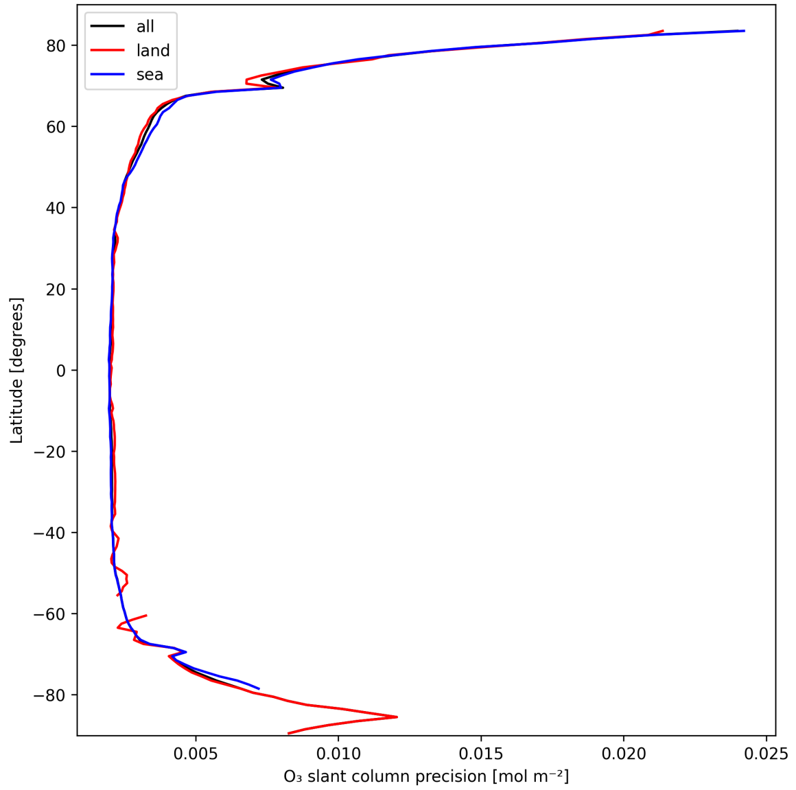
Figure 20: Zonal average of “O 3 slant column precision” for 2025-03-05 to 2025-03-05.
