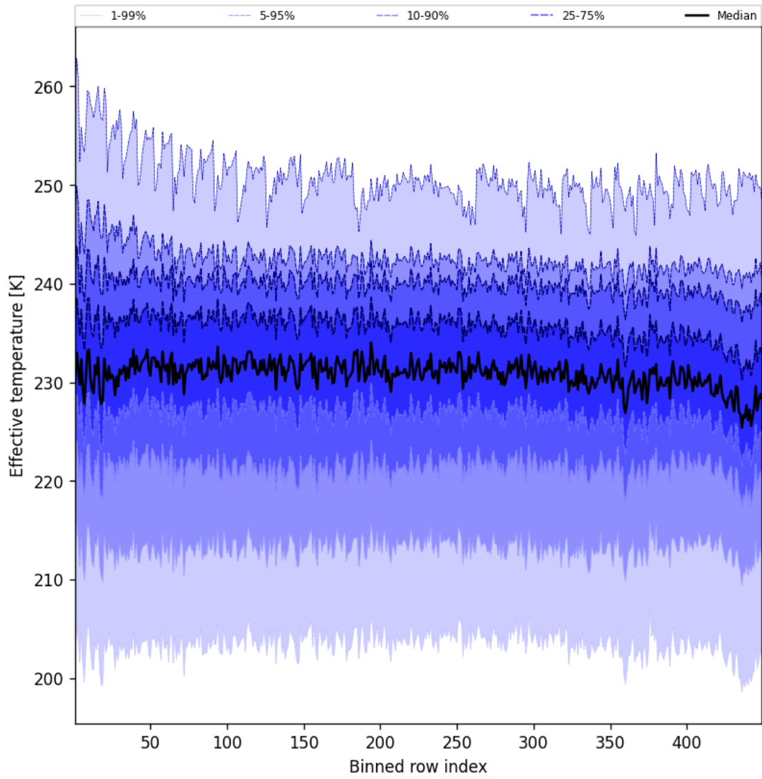
Figure 50: Along track statistics of “Effective temperature” for 2025-03-05 to 2025-03-05
