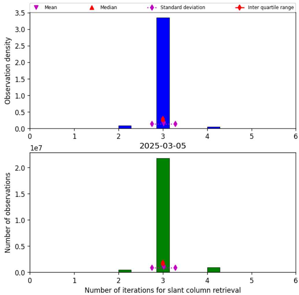
Figure 33: Histogram of "Number of iterations for slant column retrieval" for 2025-03-05 to 2025-03-05
