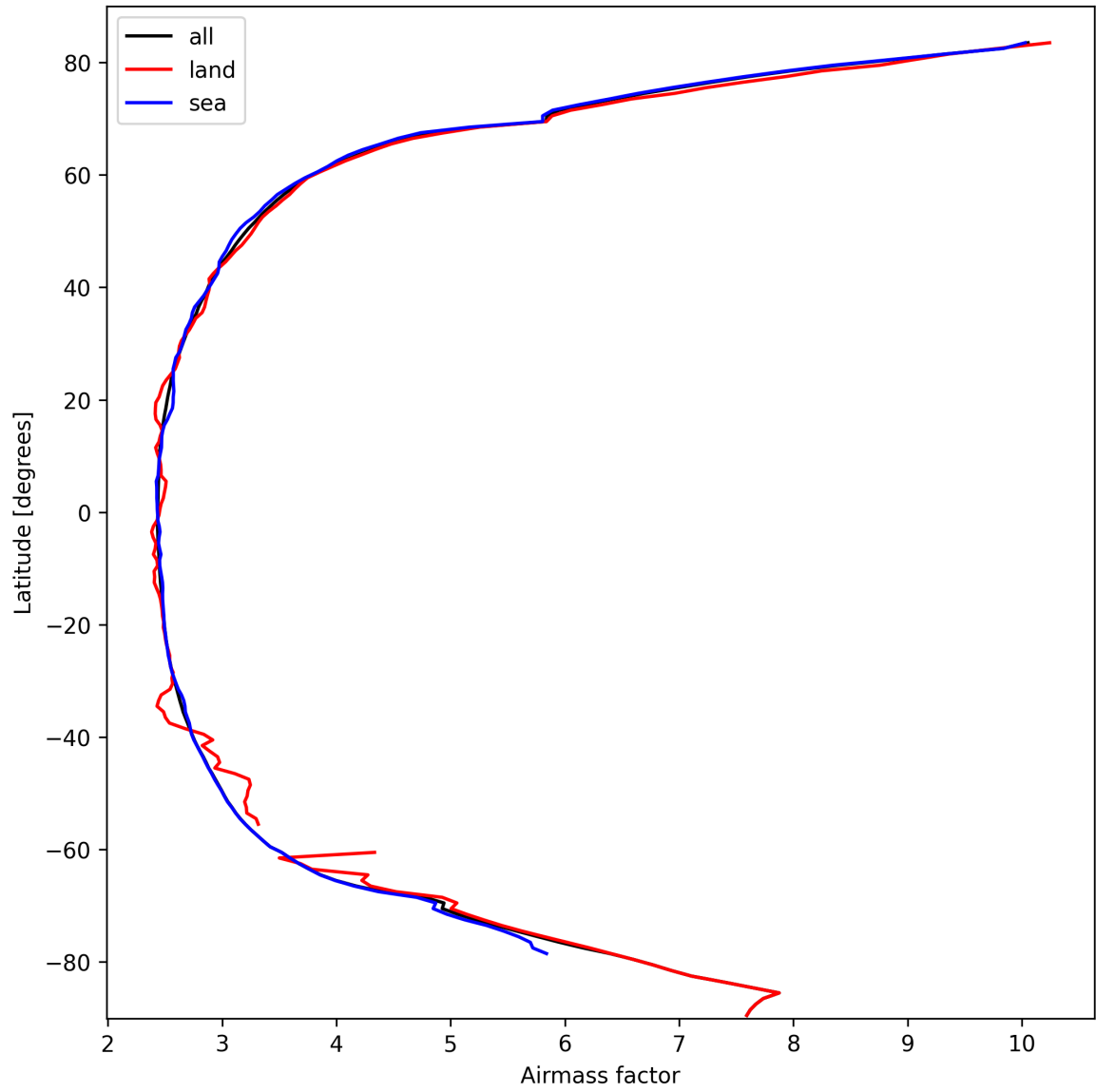
Figure 25: Zonal average of “Airmass factor” for 2025-03-05 to 2025-03-05.
