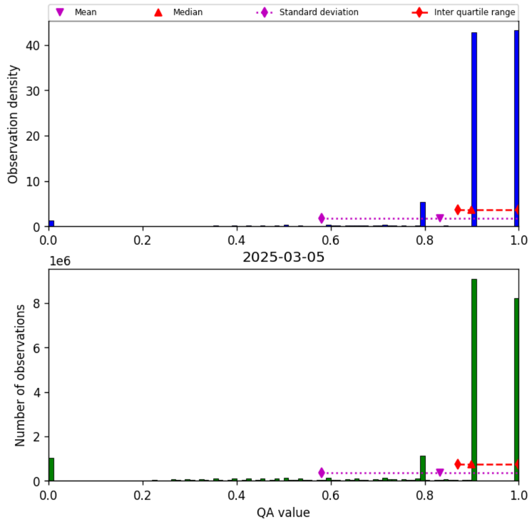
Figure 28: Histogram of “QA value” for 2025-03-05 to 2025-03-05
