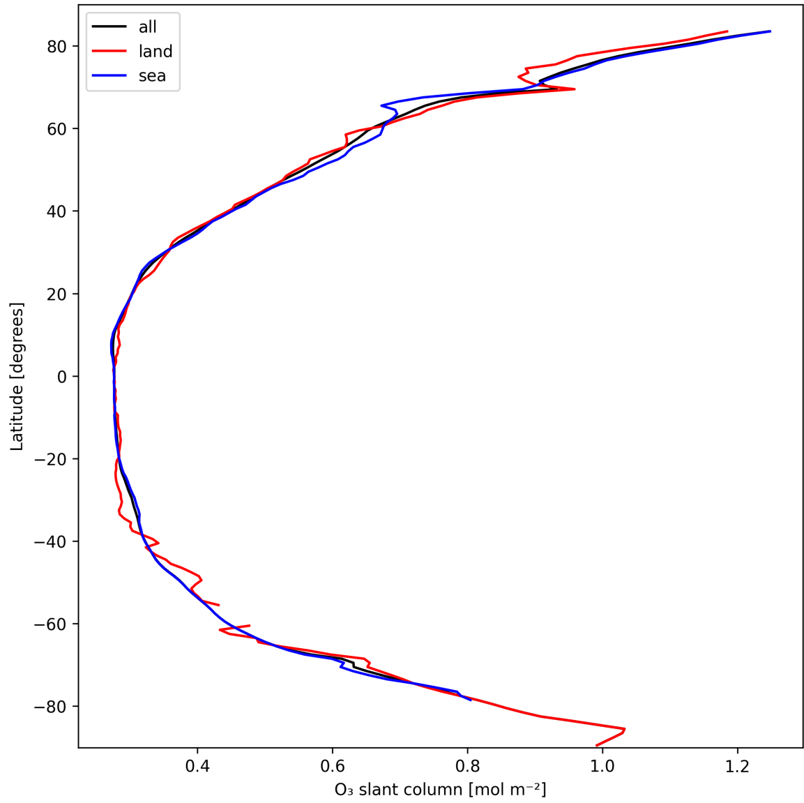
Figure 19: Zonal average of “O 3 slant column” for 2025-03-06 to 2025-03-07.
