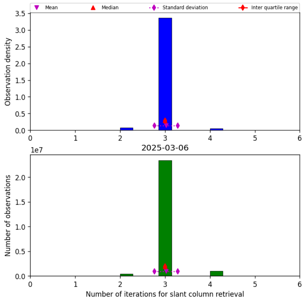
Figure 33: Histogram of “Number of iterations for slant column retrieval” for 2025-03-06 to 2025-03-07
