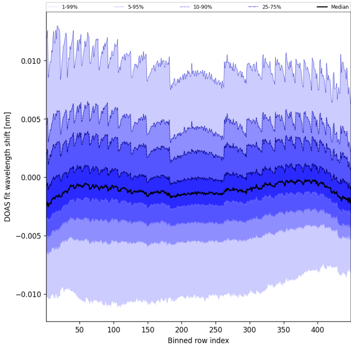
Figure 47: Along track statistics of “DOAS fit wavelength shift” for 2025-03-06 to 2025-03-07
