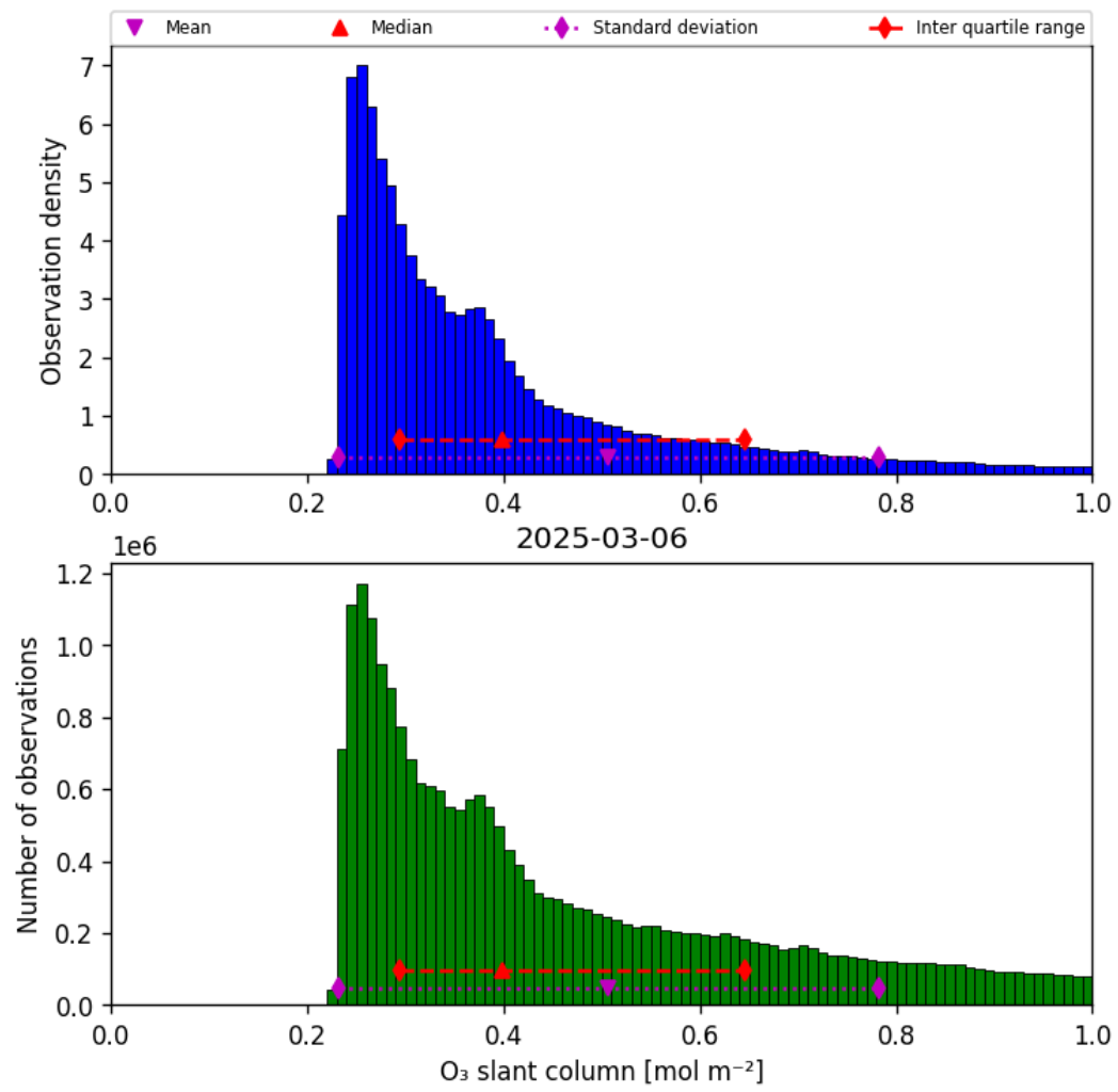
Figure 31: Histogram of “O 3 slant column” for 2025-03-06 to 2025-03-07
