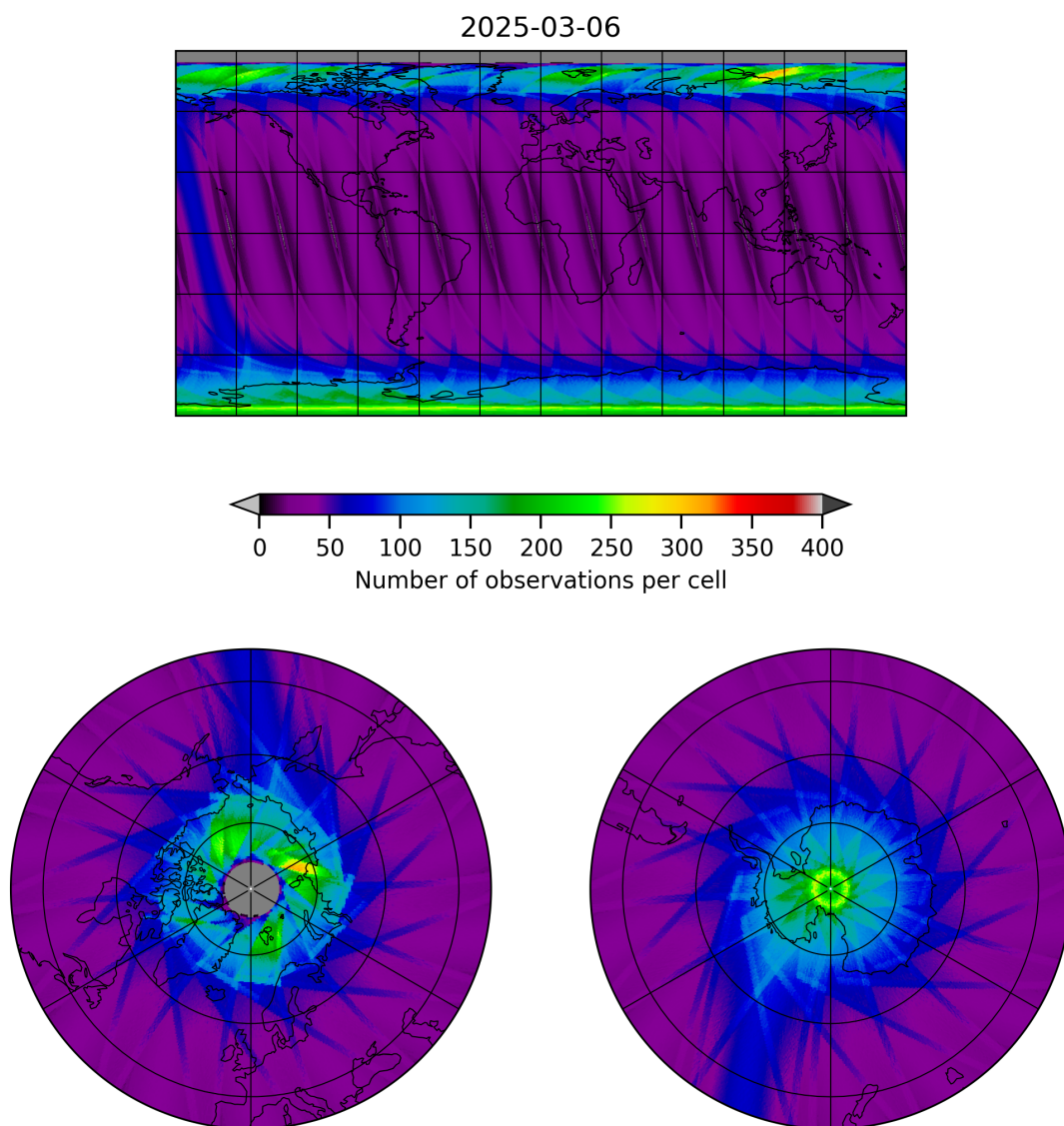
Figure 15: Map of the number of observations for 2025-03-06 to 2025-03-07
