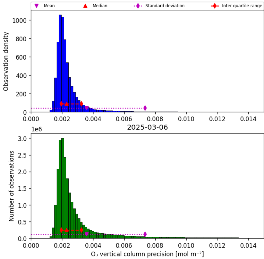
Figure 30: Histogram of "O 3 vertical column precision" for 2025-03-06 to 2025-03-07
