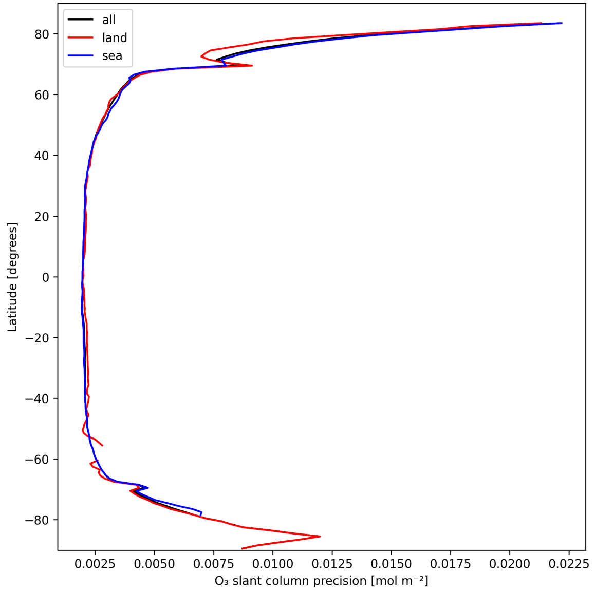
Figure 20: Zonal average of “O 3 slant column precision” for 2025-03-06 to 2025-03-07.
