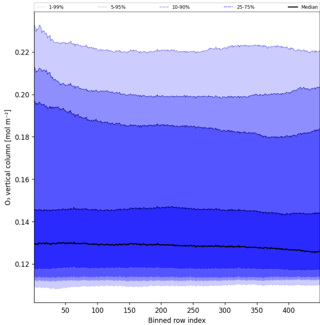
Figure 41: Along track statistics of “O 3 vertical column” for 2025-03-06 to 2025-03-07
