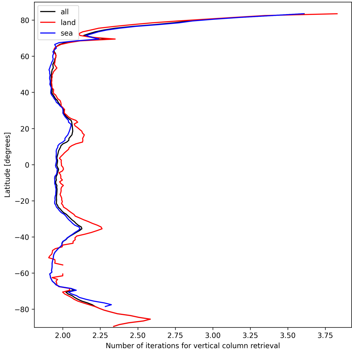
Figure 27: Zonal average of “Number of iterations for vertical column retrieval” for 2025-03-06 to 2025-03-07.
