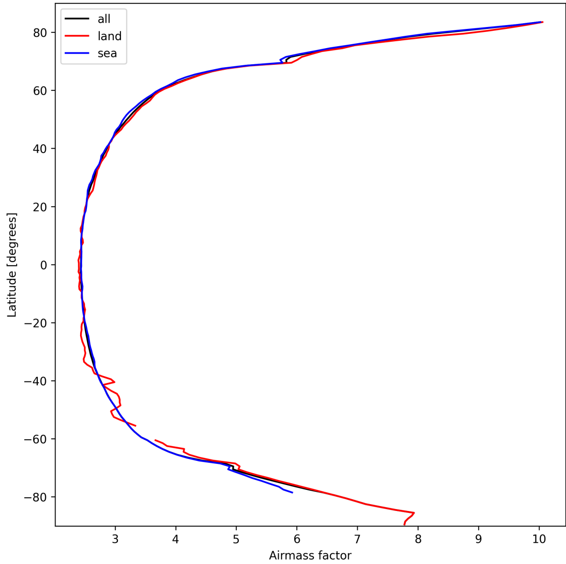
Figure 25: Zonal average of “Airmass factor” for 2025-03-06 to 2025-03-07.
