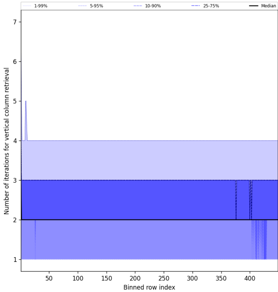
Figure 51: Along track statistics of “Number of iterations for vertical column retrieval” for 2025-03-06 to 2025-03-07
