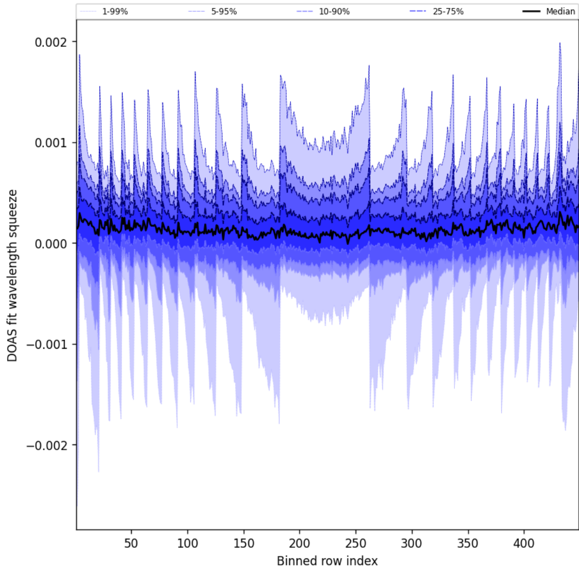
Figure 48: Along track statistics of “DOAS fit wavelength squeeze” for 2025-03-06 to 2025-03-07
