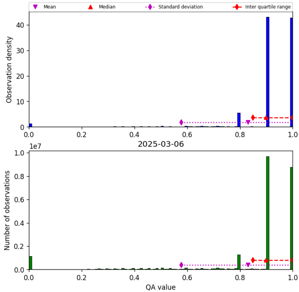
Figure 28: Histogram of “QA value” for 2025-03-06 to 2025-03-07
