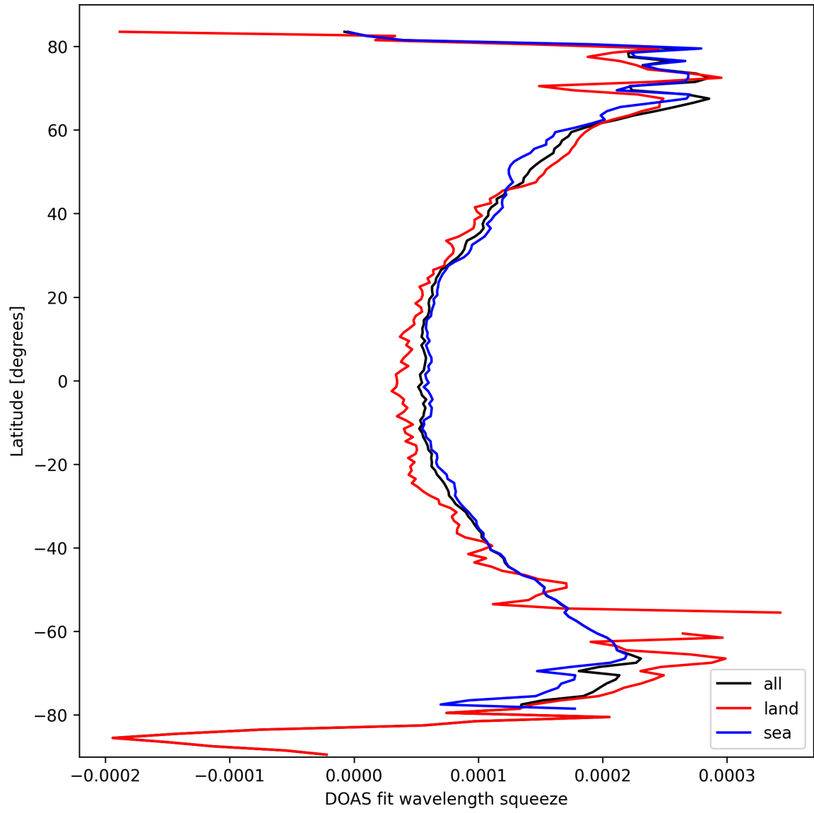
Figure 24: Zonal average of “DOAS fit wavelength squeeze” for 2025-03-06 to 2025-03-07.
