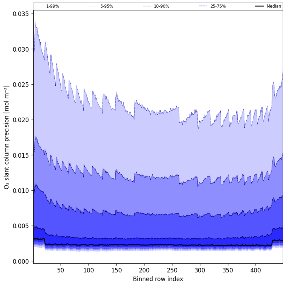
Figure 44: Along track statistics of “O 3 slant column precision” for 2025-03-06 to 2025-03-07
