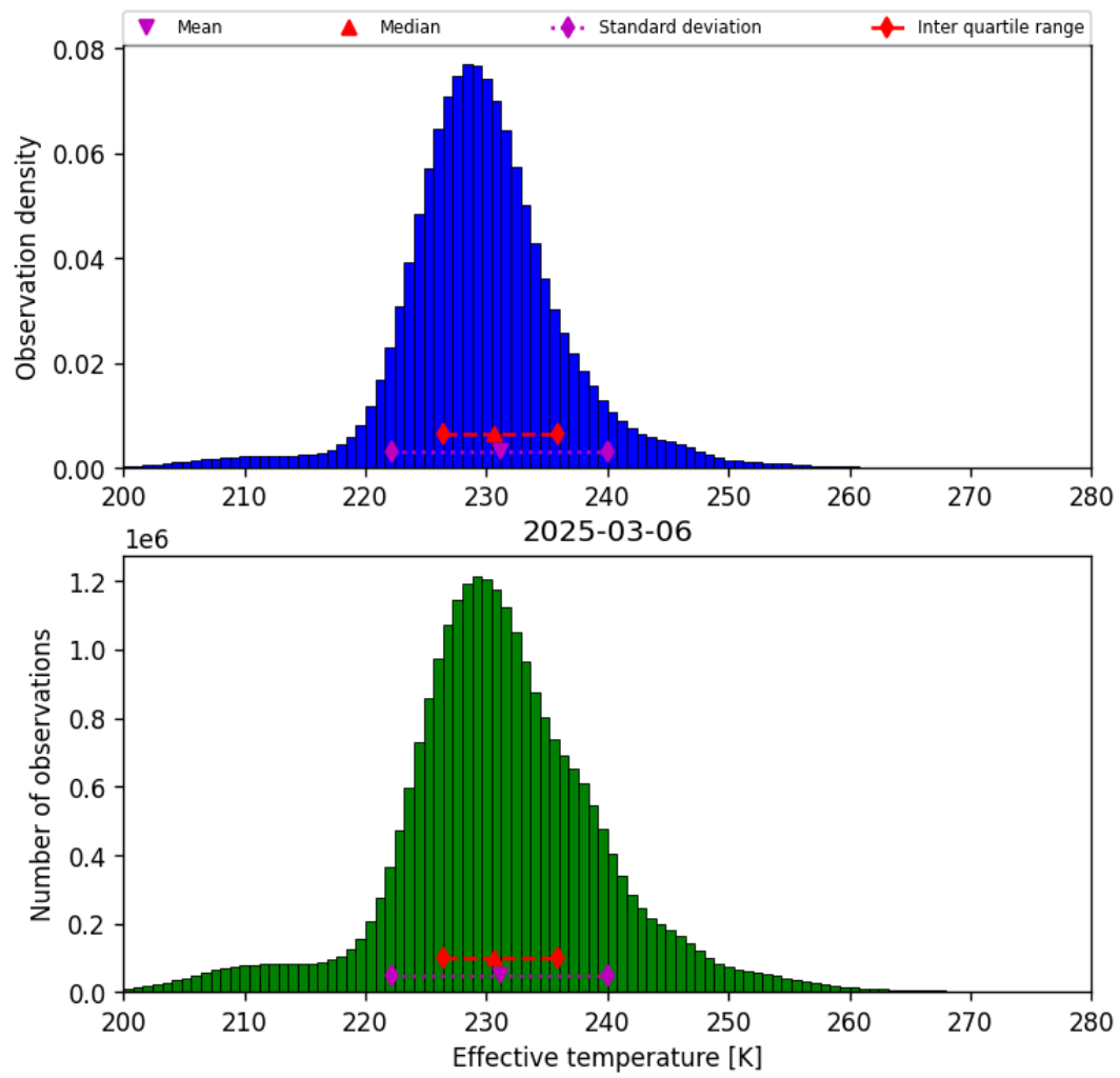
Figure 38: Histogram of “Effective temperature” for 2025-03-06 to 2025-03-07
