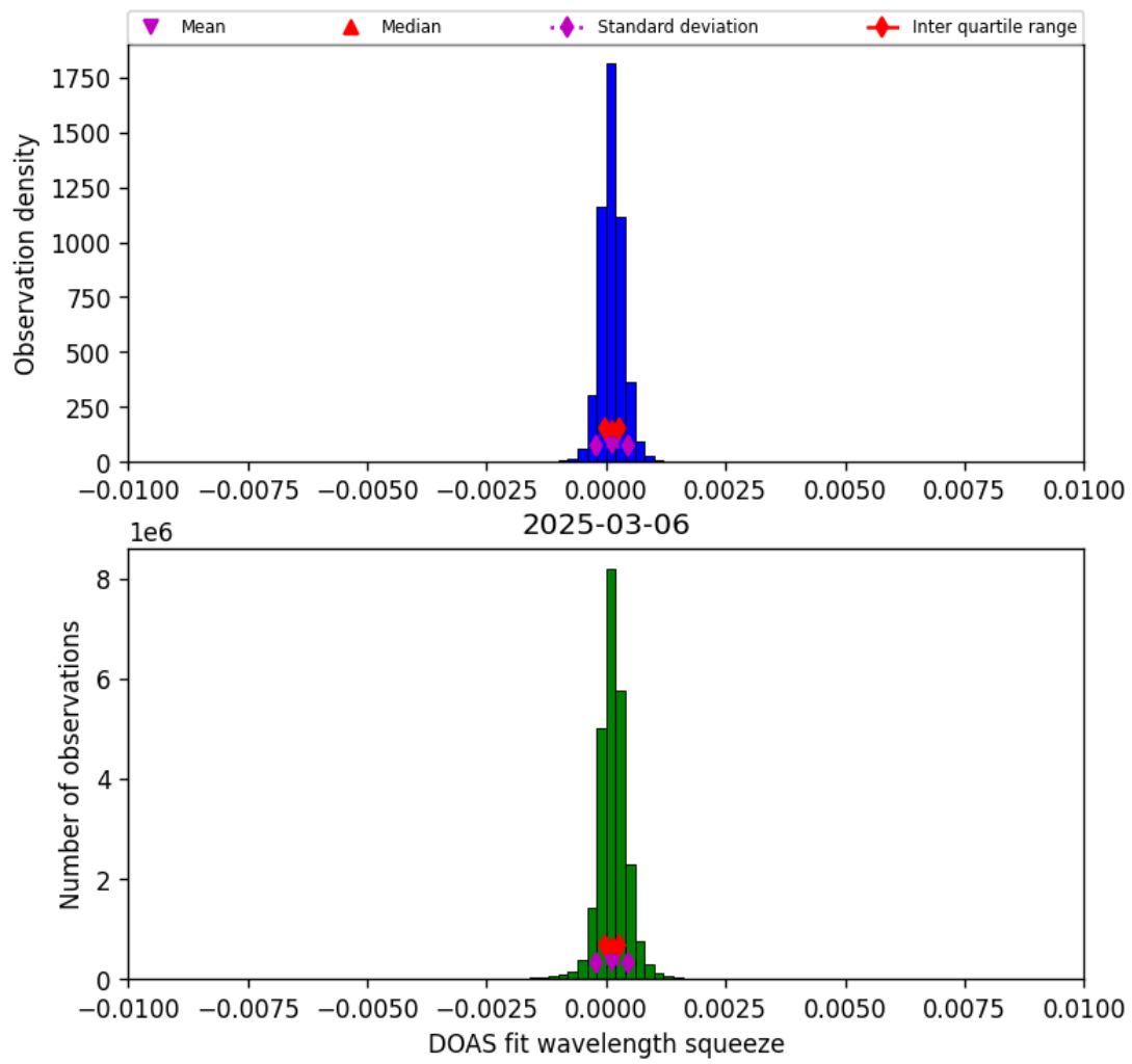
Figure 36: Histogram of “DOAS fit wavelength squeeze” for 2025-03-06 to 2025-03-07
