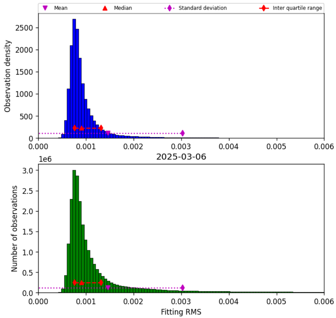
Figure 34: Histogram of “Fitting RMS” for 2025-03-06 to 2025-03-07
