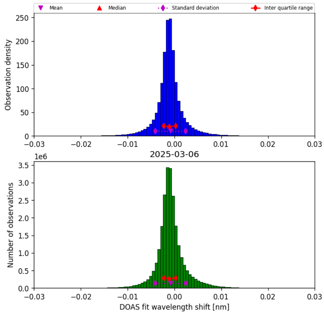
Figure 35: Histogram of “DOAS fit wavelength shift” for 2025-03-06 to 2025-03-07
