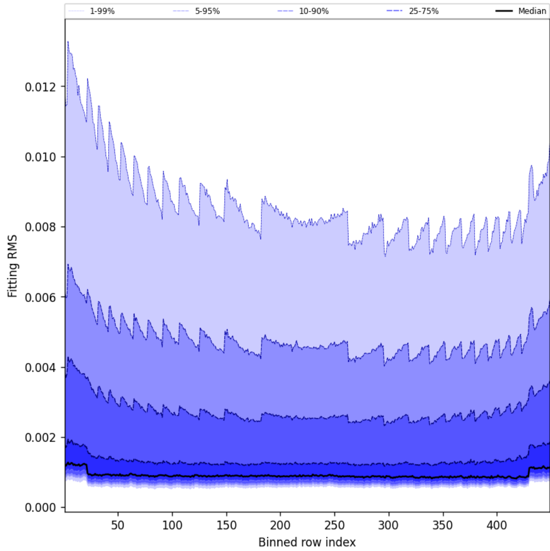
Figure 46: Along track statistics of “Fitting RMS” for 2025-03-06 to 2025-03-07
