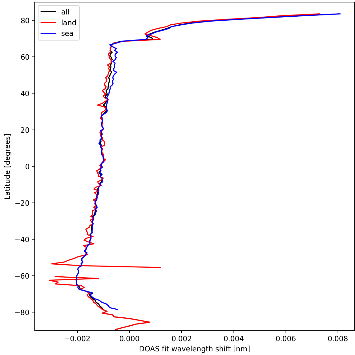
Figure 23: Zonal average of “DOAS fit wavelength shift” for 2025-03-06 to 2025-03-07.
