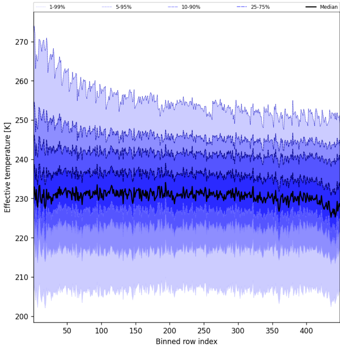
Figure 50: Along track statistics of “Effective temperature” for 2025-03-06 to 2025-03-07
