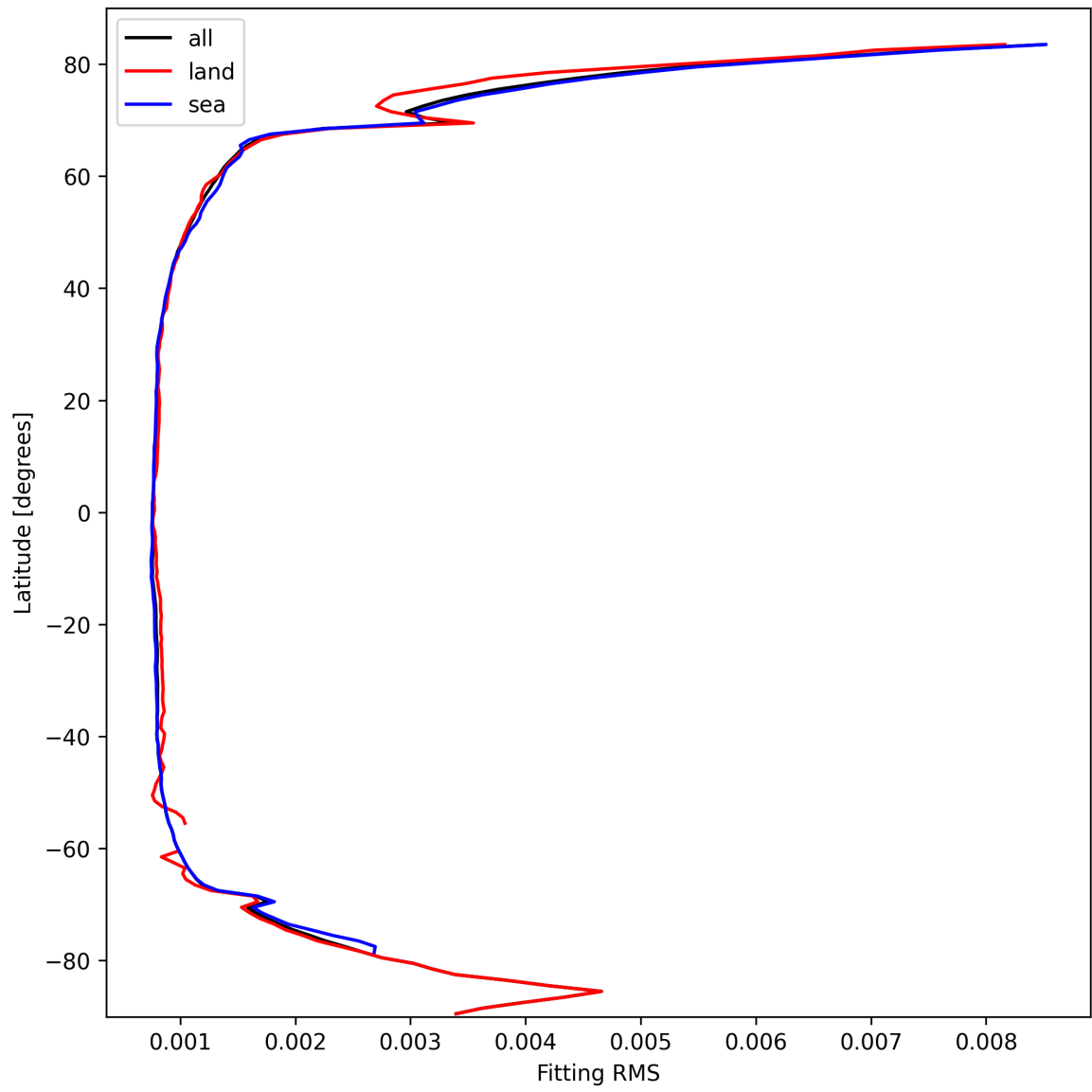
Figure 22: Zonal average of “Fitting RMS” for 2025-03-06 to 2025-03-07.
