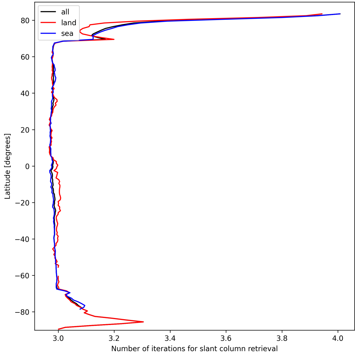
Figure 21: Zonal average of “Number of iterations for slant column retrieval” for 2025-03-06 to 2025-03-07.
