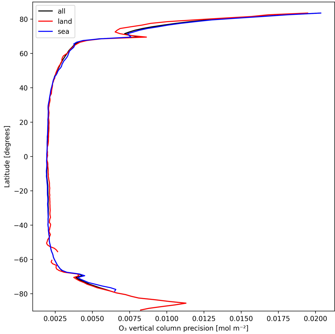
Figure 18: Zonal average of “O 3 vertical column precision” for 2025-03-06 to 2025-03-07.
