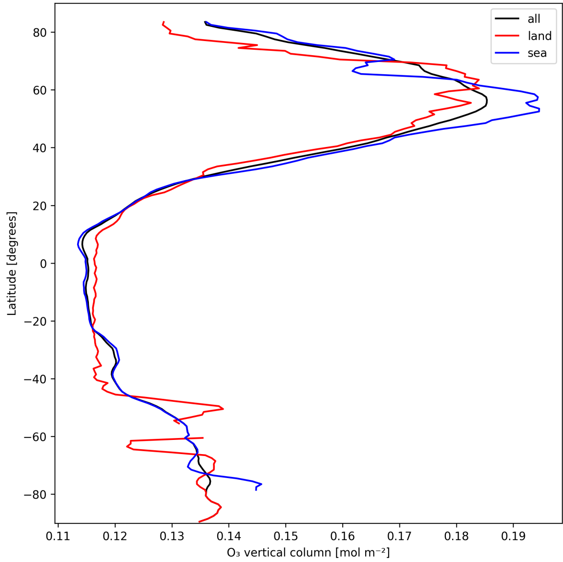
Figure 17: Zonal average of “O 3 vertical column” for 2025-03-06 to 2025-03-07.
