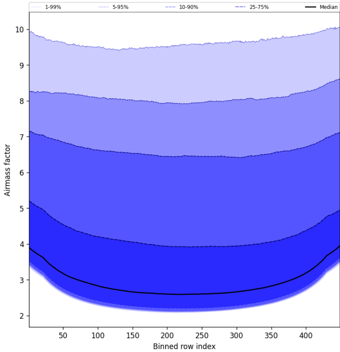
Figure 49: Along track statistics of “Airmass factor” for 2025-03-06 to 2025-03-07
