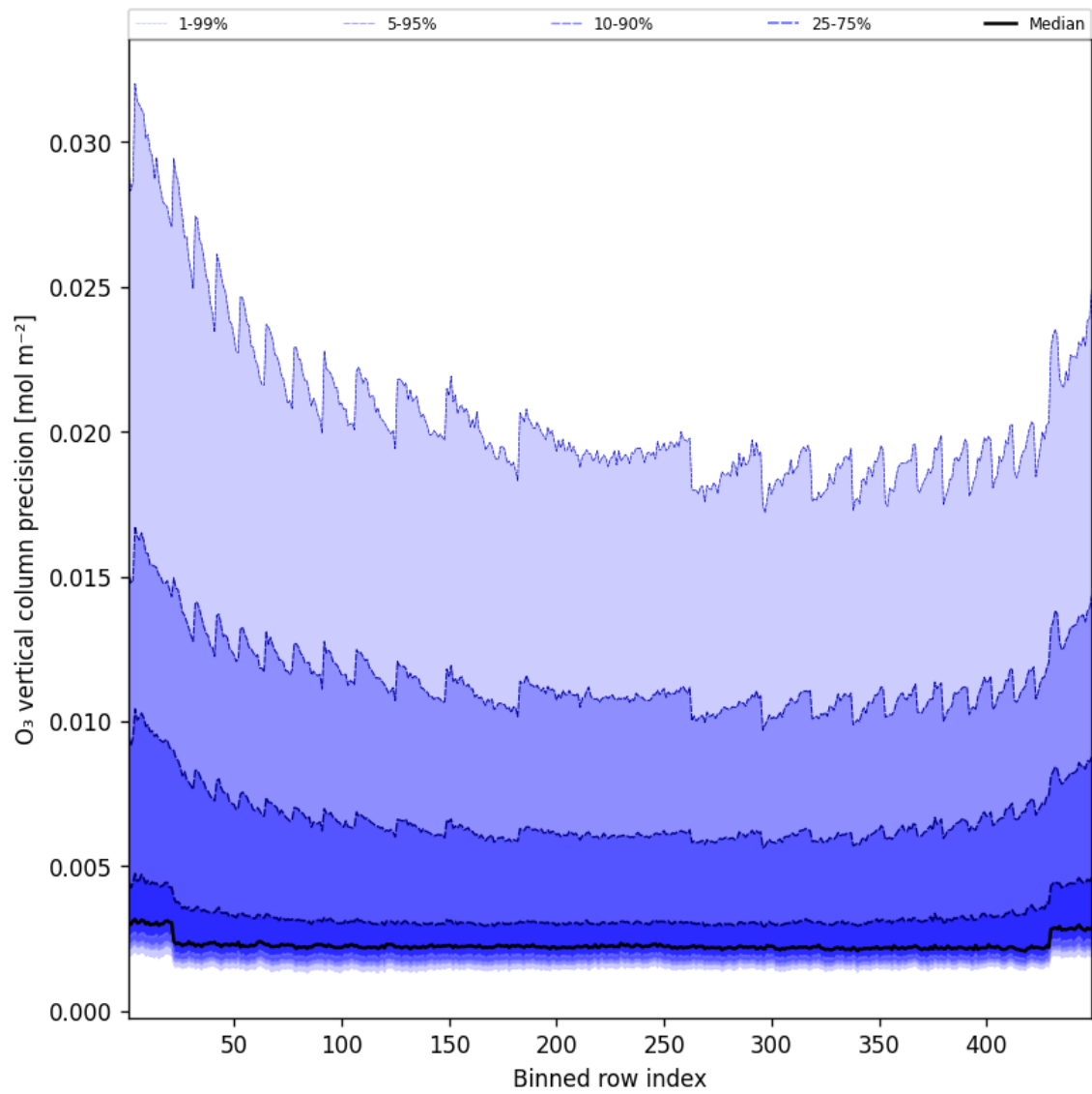
Figure 42: Along track statistics of “O 3 vertical column precision” for 2025-03-06 to 2025-03-07
