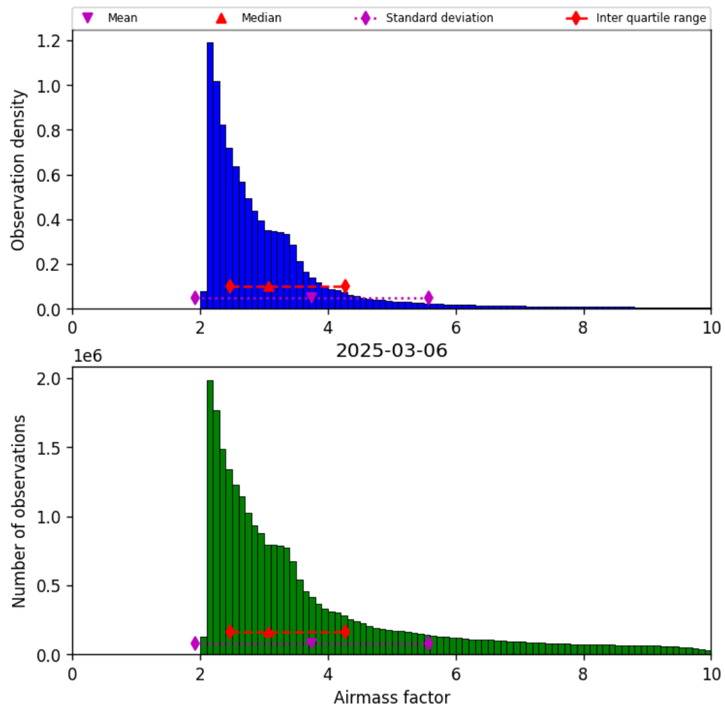
Figure 37: Histogram of “Airmass factor” for 2025-03-06 to 2025-03-07
