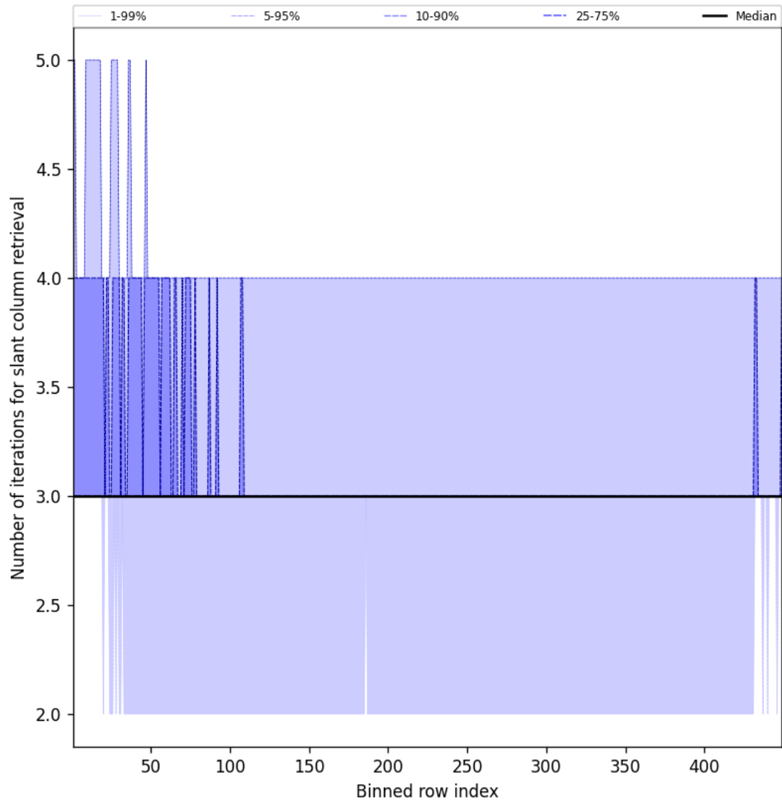
Figure 45: Along track statistics of “Number of iterations for slant column retrieval” for 2025-03-06 to 2025-03-07
