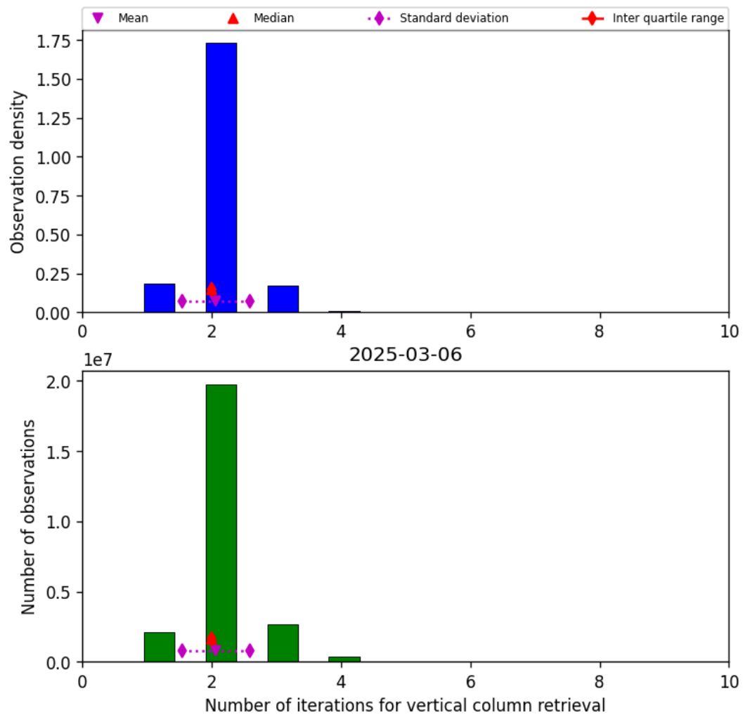
Figure 39: Histogram of “Number of iterations for vertical column retrieval” for 2025-03-06 to 2025-03-07
