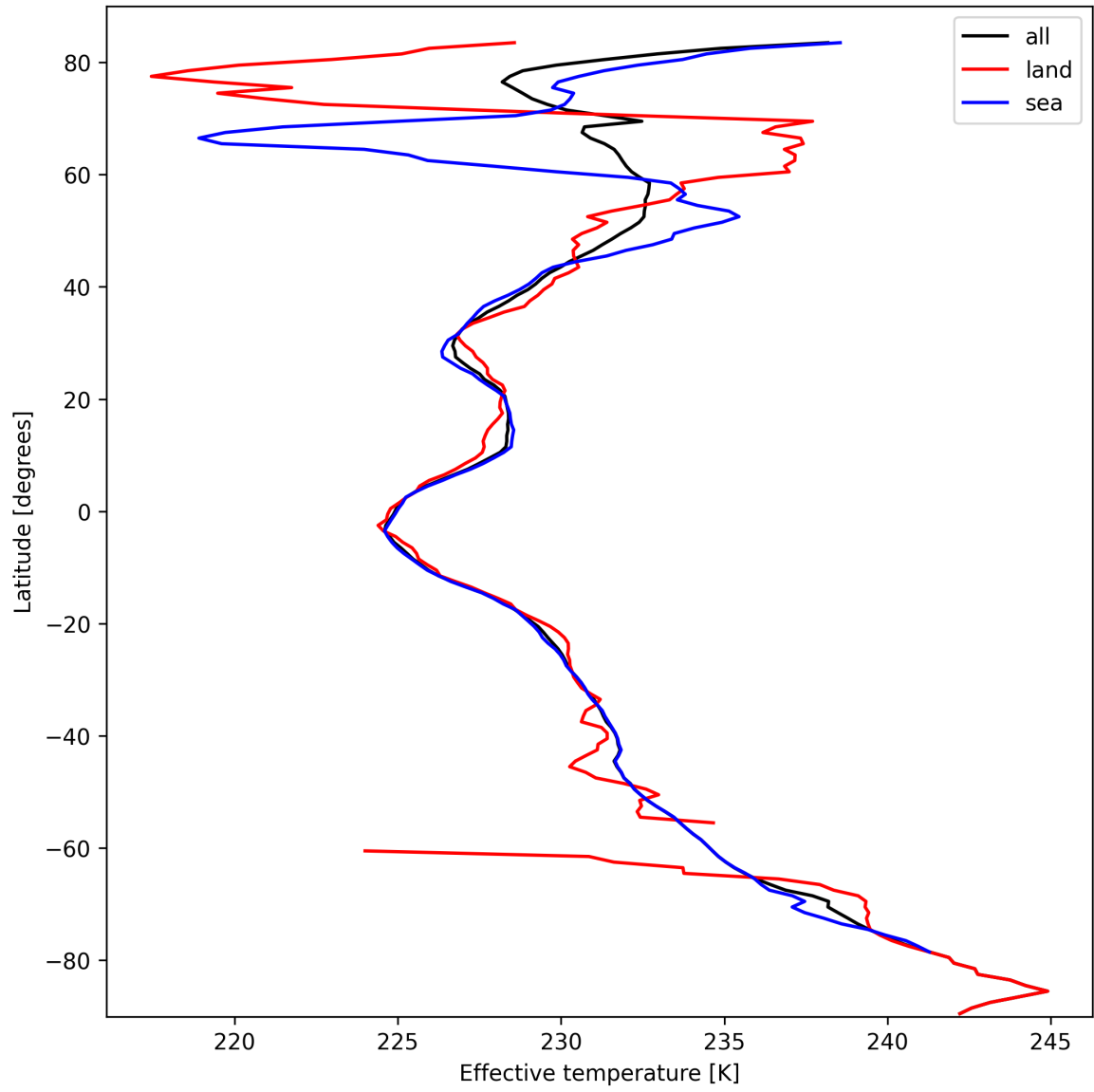
Figure 26: Zonal average of “Effective temperature” for 2025-03-06 to 2025-03-07.
