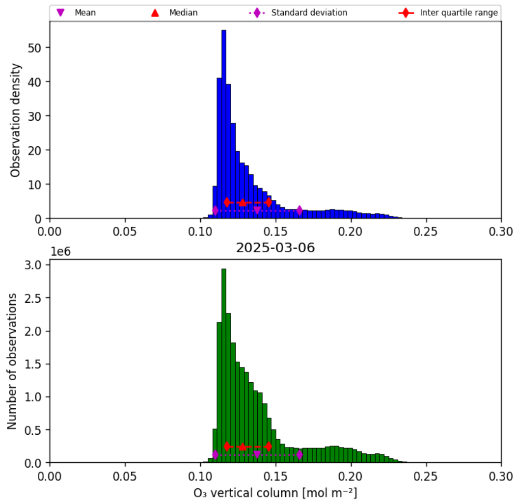
Figure 29: Histogram of “O 3 vertical column” for 2025-03-06 to 2025-03-07
