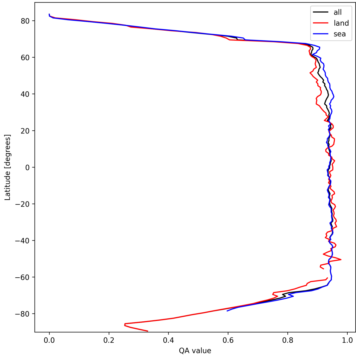
Figure 16: Zonal average of “QA value” for 2025-03-06 to 2025-03-07.
