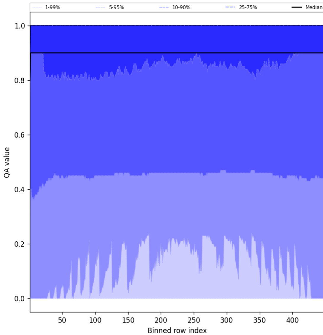
Figure 40: Along track statistics of “QA value” for 2025-03-06 to 2025-03-07
