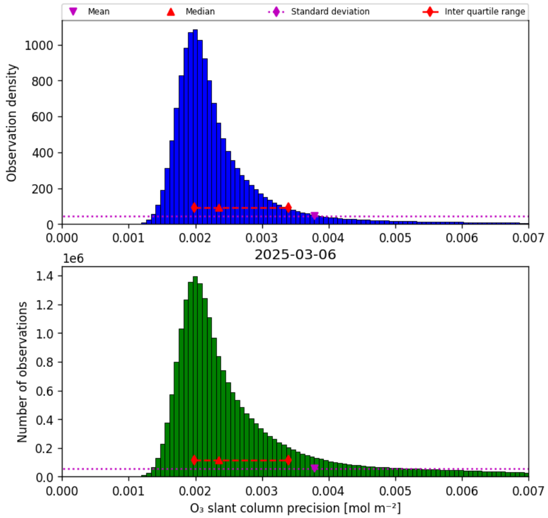
Figure 32: Histogram of “O 3 slant column precision” for 2025-03-06 to 2025-03-07
