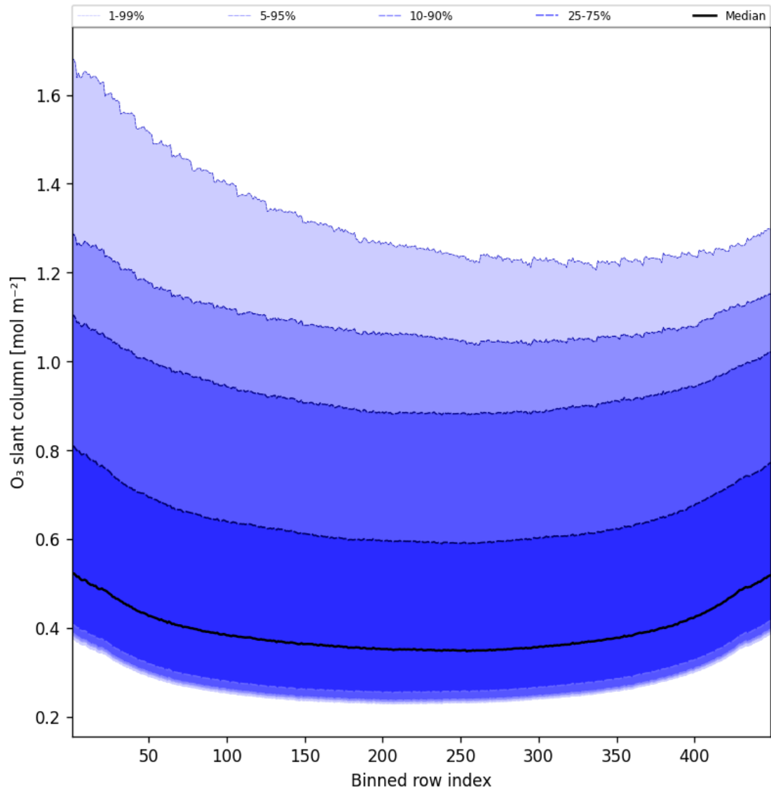
Figure 43: Along track statistics of “O 3 slant column” for 2025-03-06 to 2025-03-07
