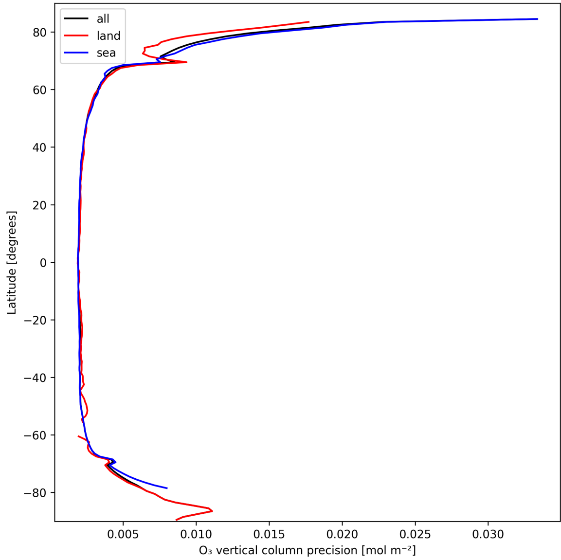
Figure 18: Zonal average of “O 3 vertical column precision” for 2025-03-07 to 2025-03-08.
