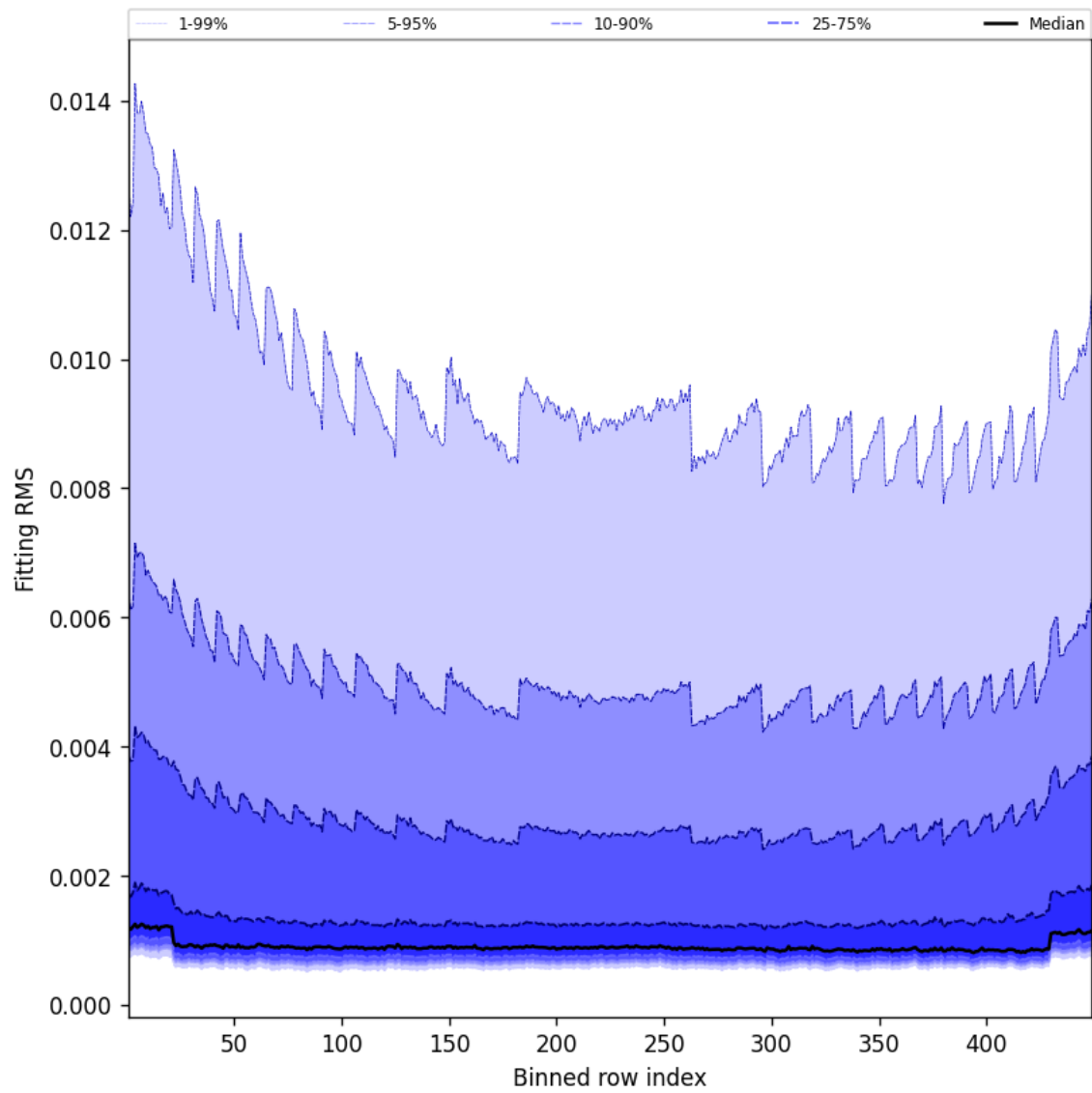
Figure 46: Along track statistics of “Fitting RMS” for 2025-03-07 to 2025-03-08
