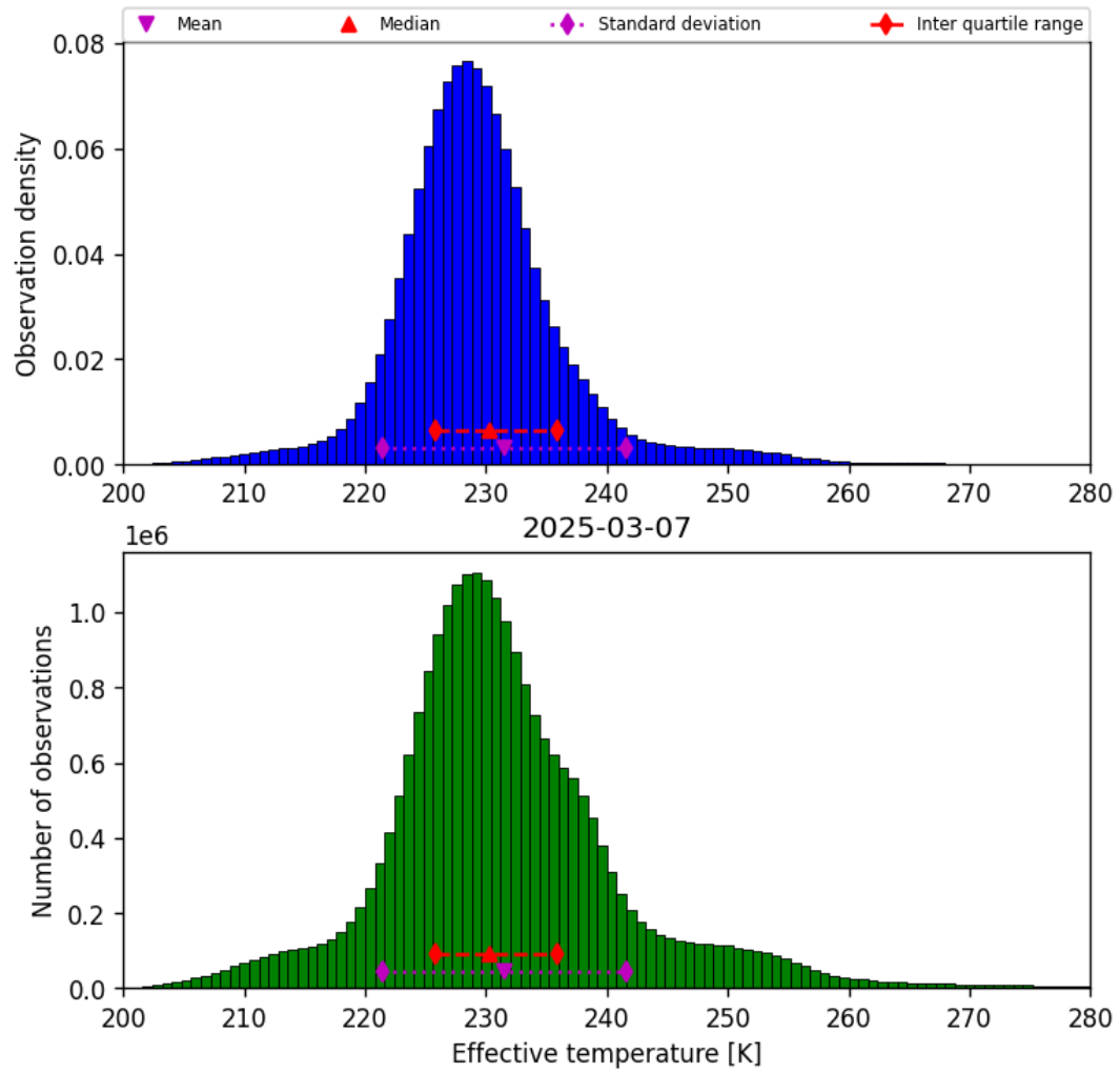
Figure 38: Histogram of “Effective temperature” for 2025-03-07 to 2025-03-08
