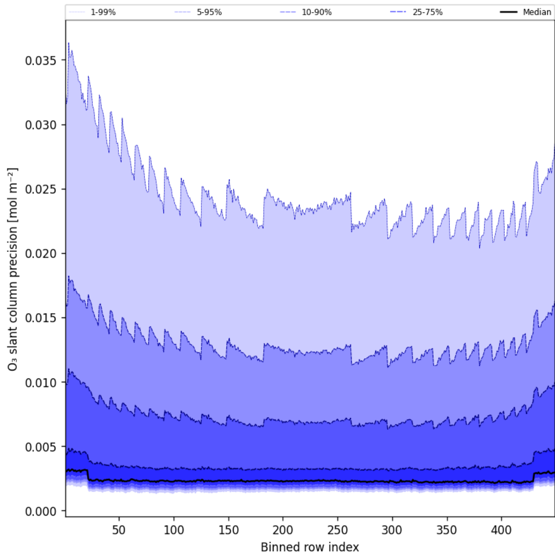
Figure 44: Along track statistics of “O 3 slant column precision” for 2025-03-07 to 2025-03-08
