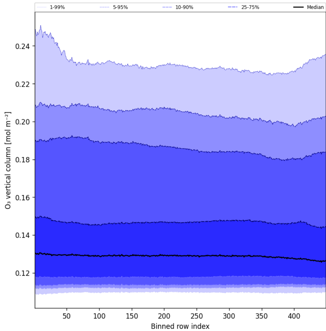
Figure 41: Along track statistics of “O 3 vertical column” for 2025-03-07 to 2025-03-08
