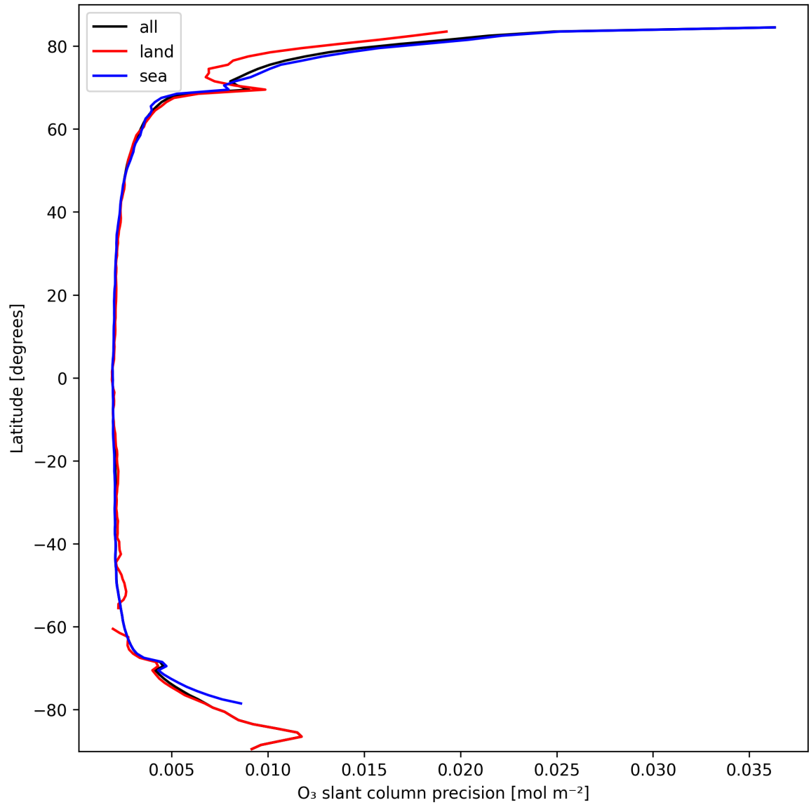
Figure 20: Zonal average of “O 3 slant column precision” for 2025-03-07 to 2025-03-08.
