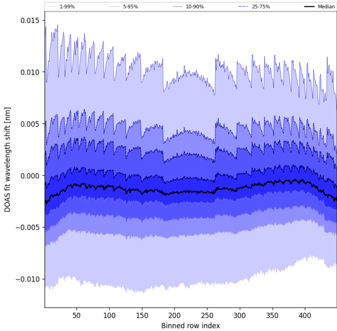
Figure 47: Along track statistics of “DOAS fit wavelength shift” for 2025-03-07 to 2025-03-08
