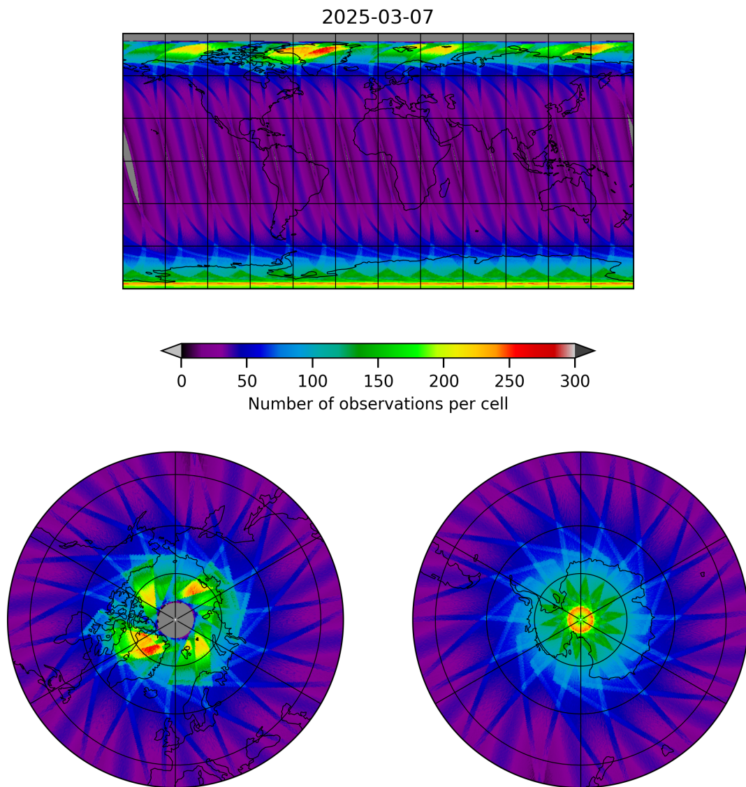
Figure 15: Map of the number of observations for 2025-03-07 to 2025-03-08
