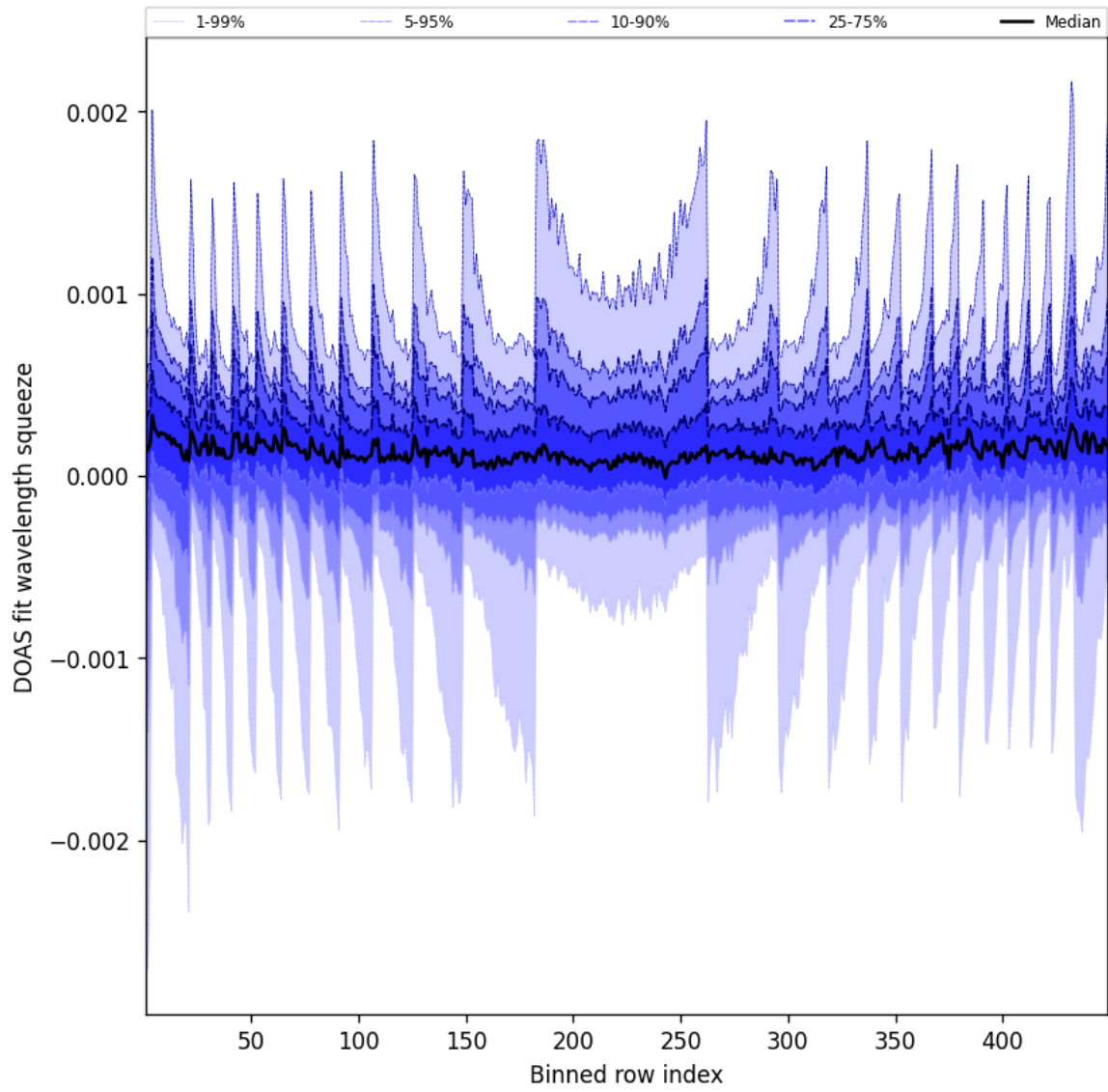
Figure 48: Along track statistics of “DOAS fit wavelength squeeze” for 2025-03-07 to 2025-03-08
