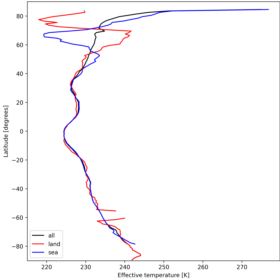
Figure 26: Zonal average of “Effective temperature” for 2025-03-07 to 2025-03-08.
