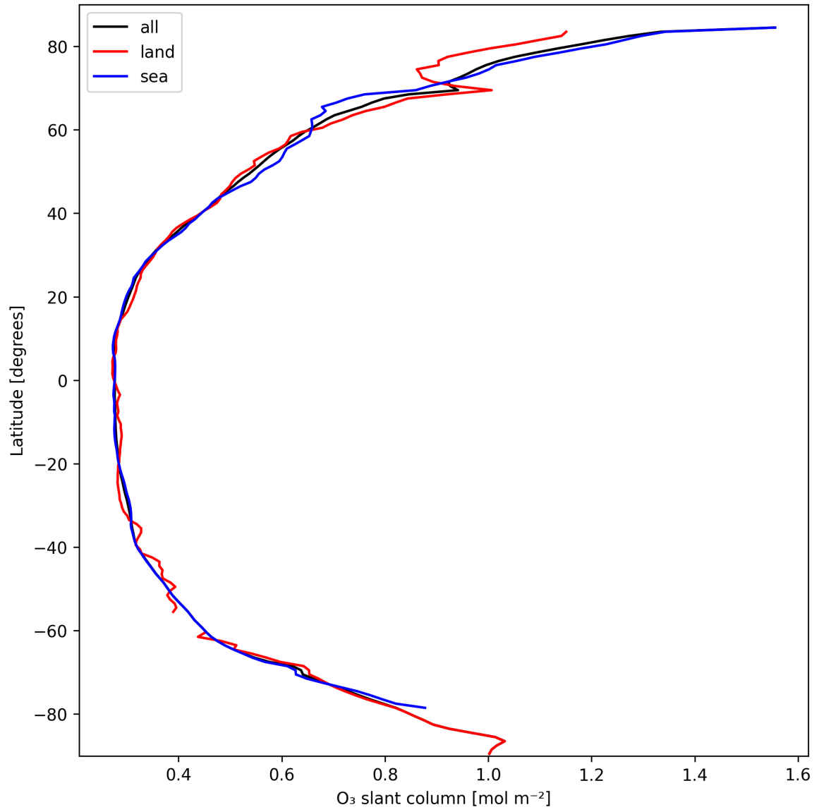
Figure 19: Zonal average of “O 3 slant column” for 2025-03-07 to 2025-03-08.
