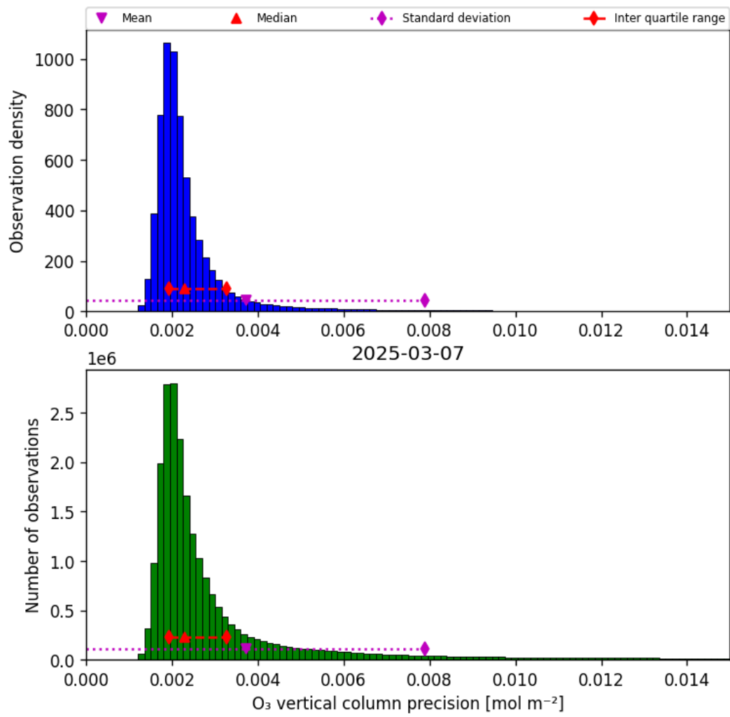
Figure 30: Histogram of “O 3 vertical column precision” for 2025-03-07 to 2025-03-08
