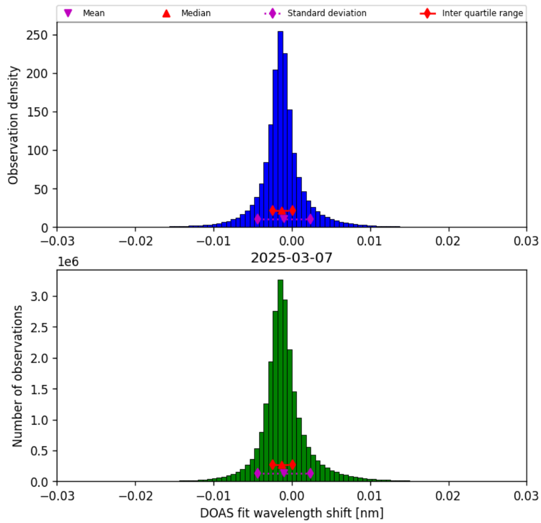
Figure 35: Histogram of “DOAS fit wavelength shift” for 2025-03-07 to 2025-03-08
