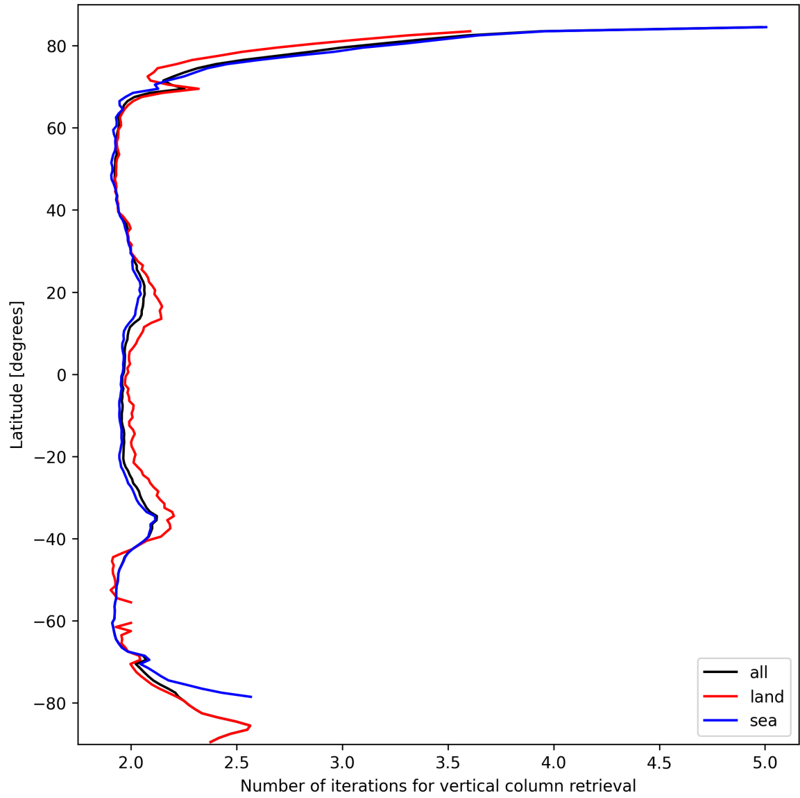
Figure 27: Zonal average of “Number of iterations for vertical column retrieval” for 2025-03-07 to 2025-03-08.
