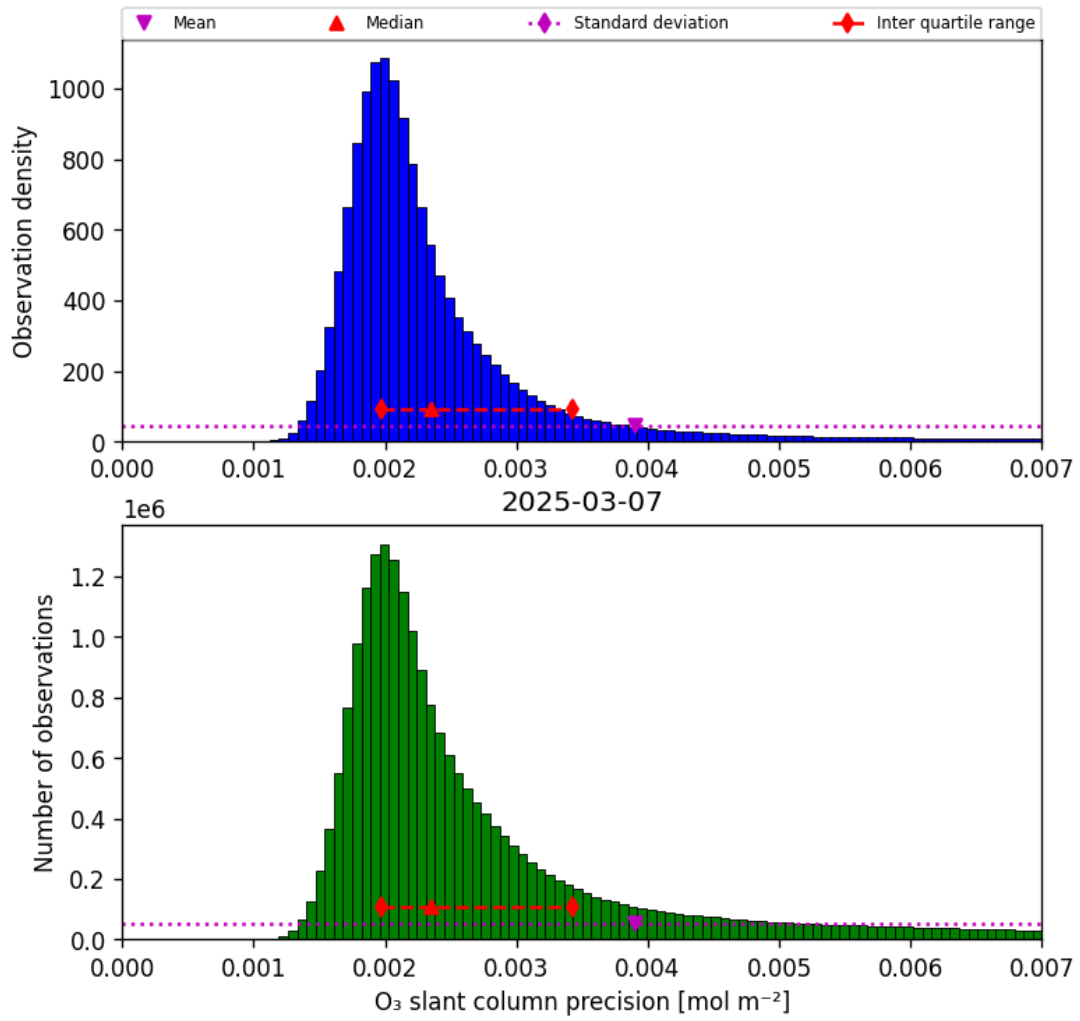
Figure 32: Histogram of “O 3 slant column precision” for 2025-03-07 to 2025-03-08
