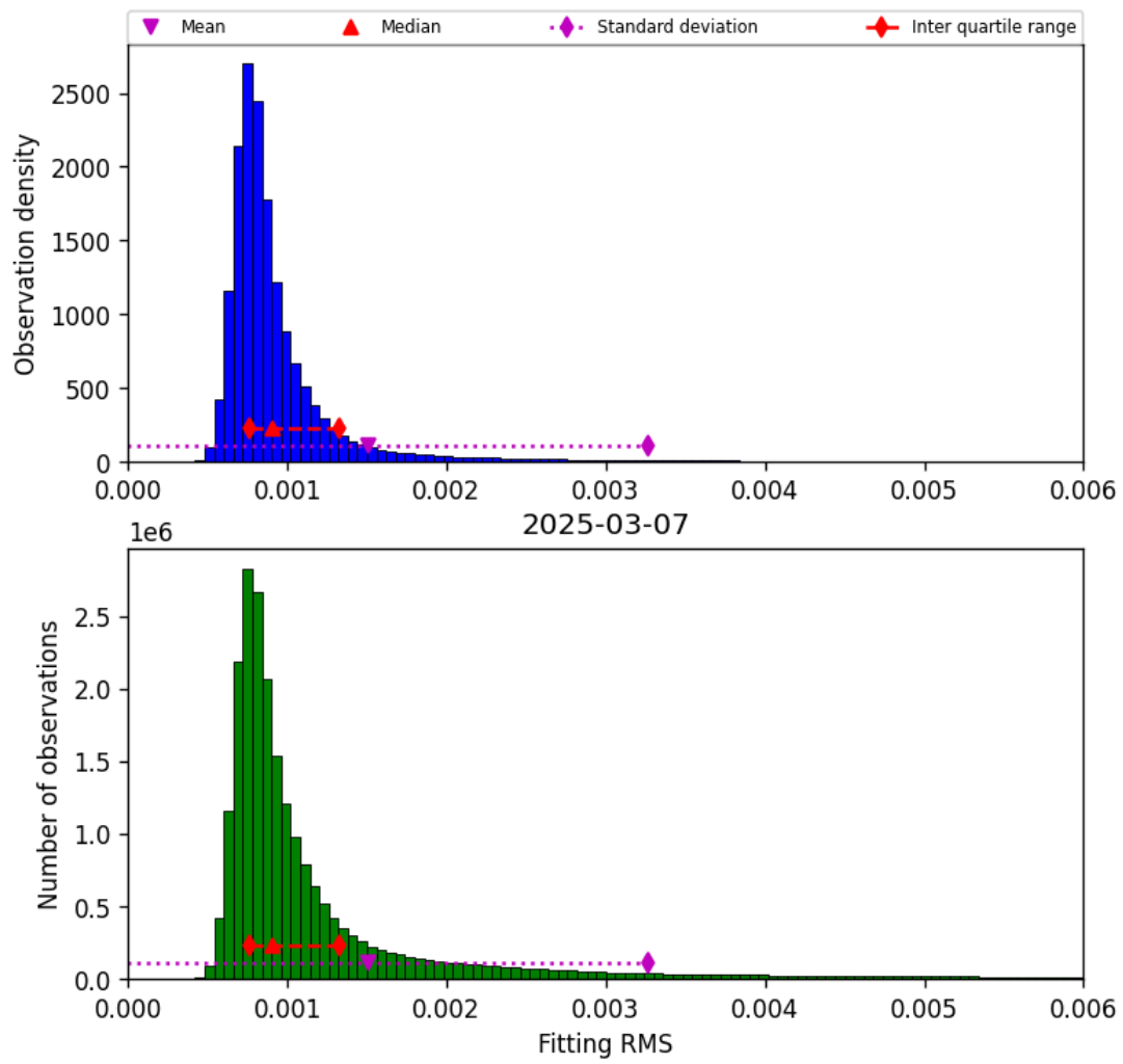
Figure 34: Histogram of “Fitting RMS” for 2025-03-07 to 2025-03-08
