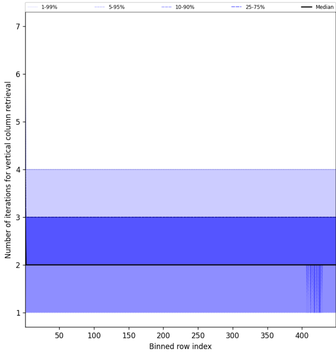
Figure 51: Along track statistics of “Number of iterations for vertical column retrieval” for 2025-03-07 to 2025-03-08
