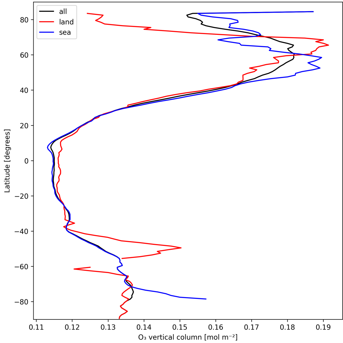
Figure 17: Zonal average of “O 3 vertical column” for 2025-03-07 to 2025-03-08.
