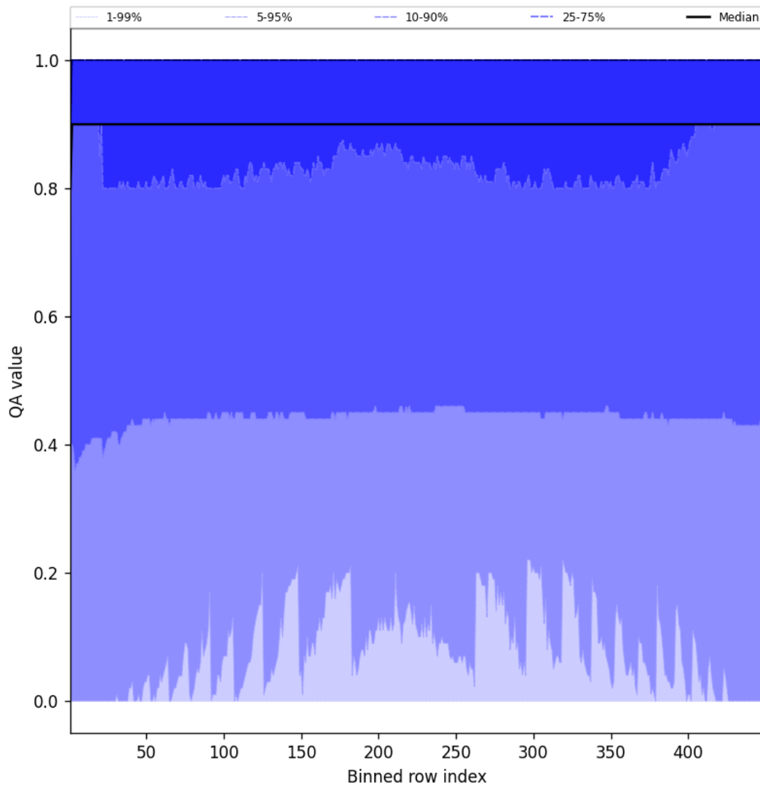
Figure 40: Along track statistics of “QA value” for 2025-03-07 to 2025-03-08
