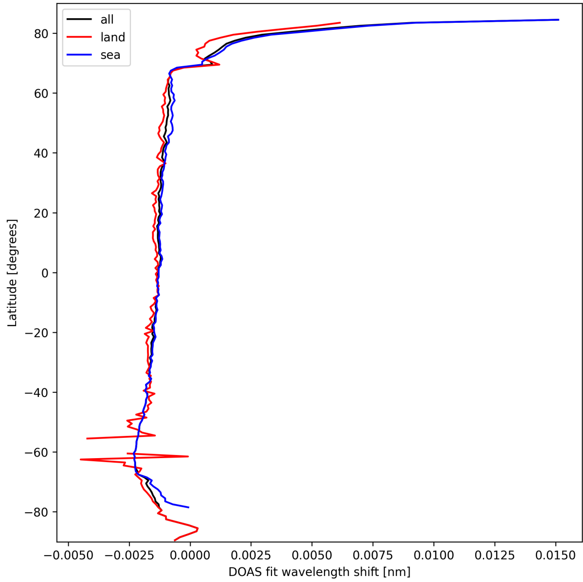
Figure 23: Zonal average of “DOAS fit wavelength shift” for 2025-03-07 to 2025-03-08.
