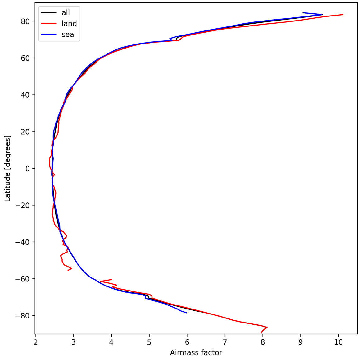
Figure 25: Zonal average of “Airmass factor” for 2025-03-07 to 2025-03-08.
