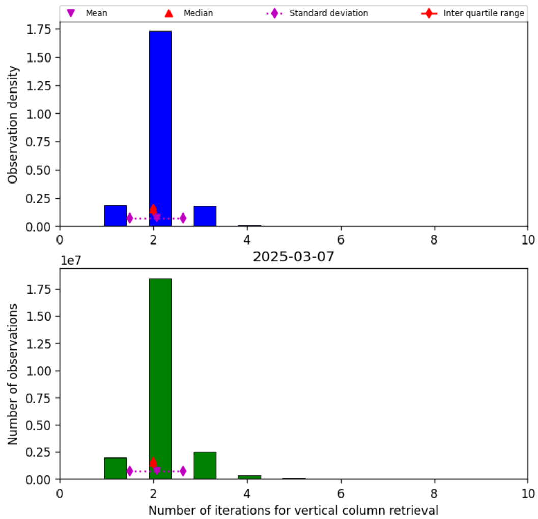
Figure 39: Histogram of “Number of iterations for vertical column retrieval” for 2025-03-07 to 2025-03-08
