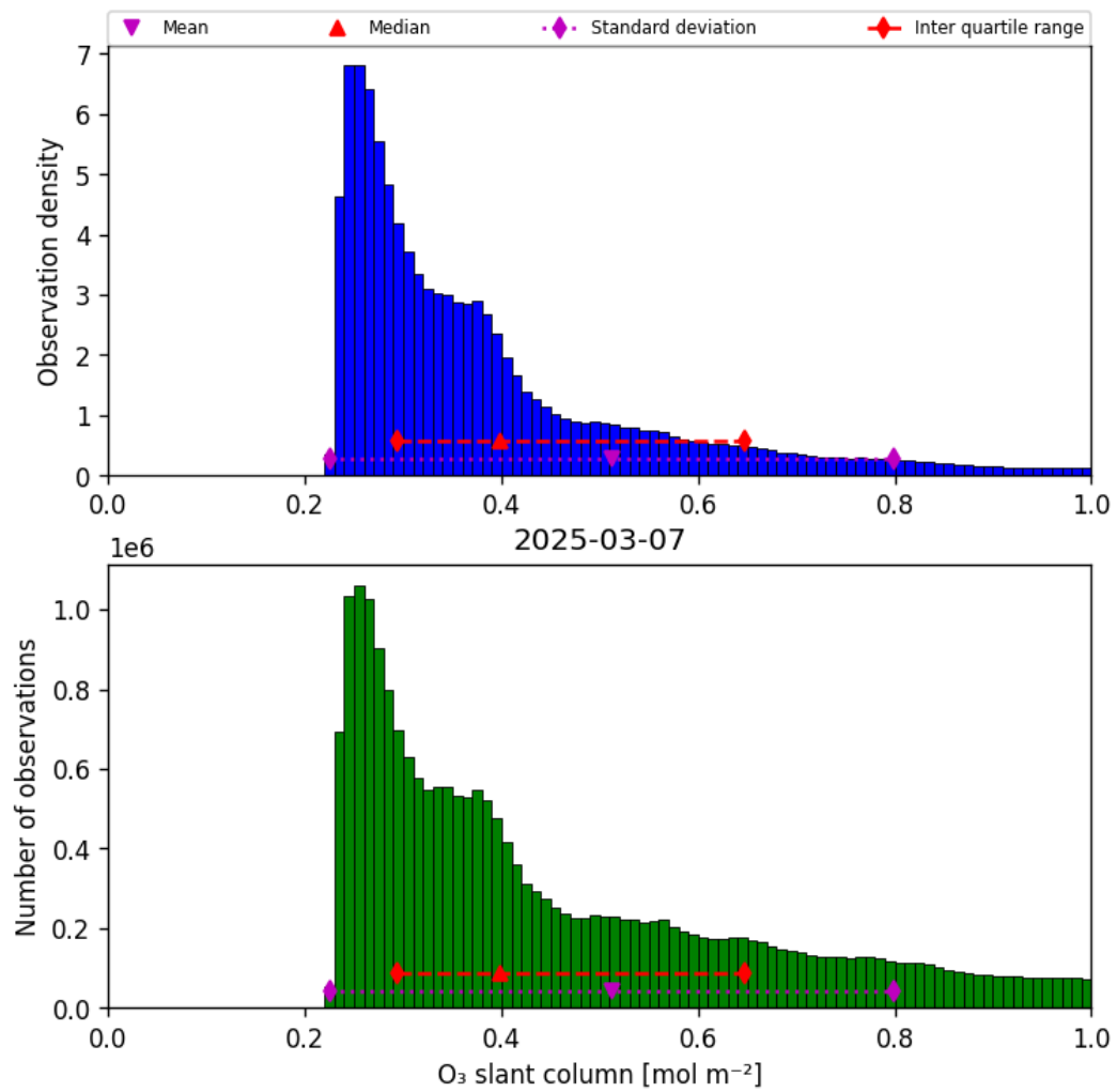
Figure 31: Histogram of “O 3 slant column” for 2025-03-07 to 2025-03-08
