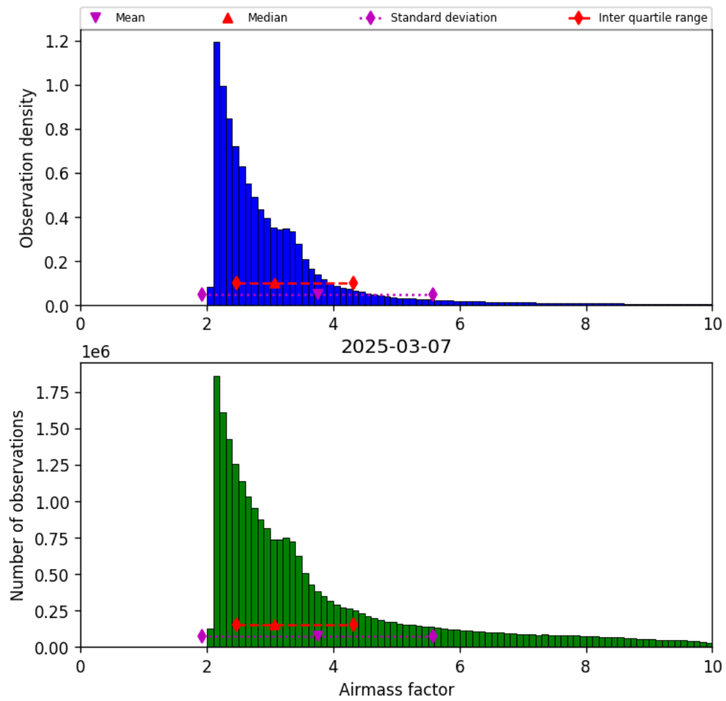
Figure 37: Histogram of “Airmass factor” for 2025-03-07 to 2025-03-08
