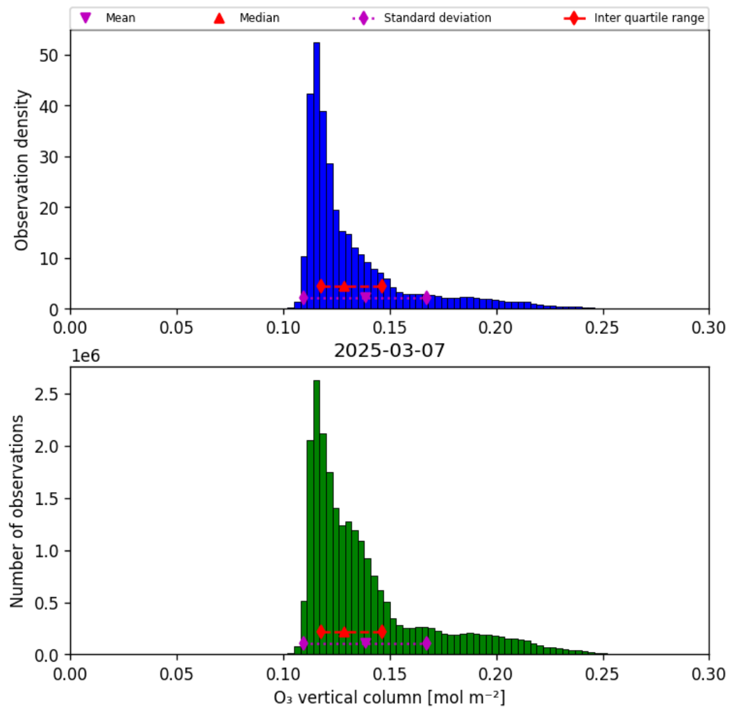
Figure 29: Histogram of “O 3 vertical column” for 2025-03-07 to 2025-03-08
