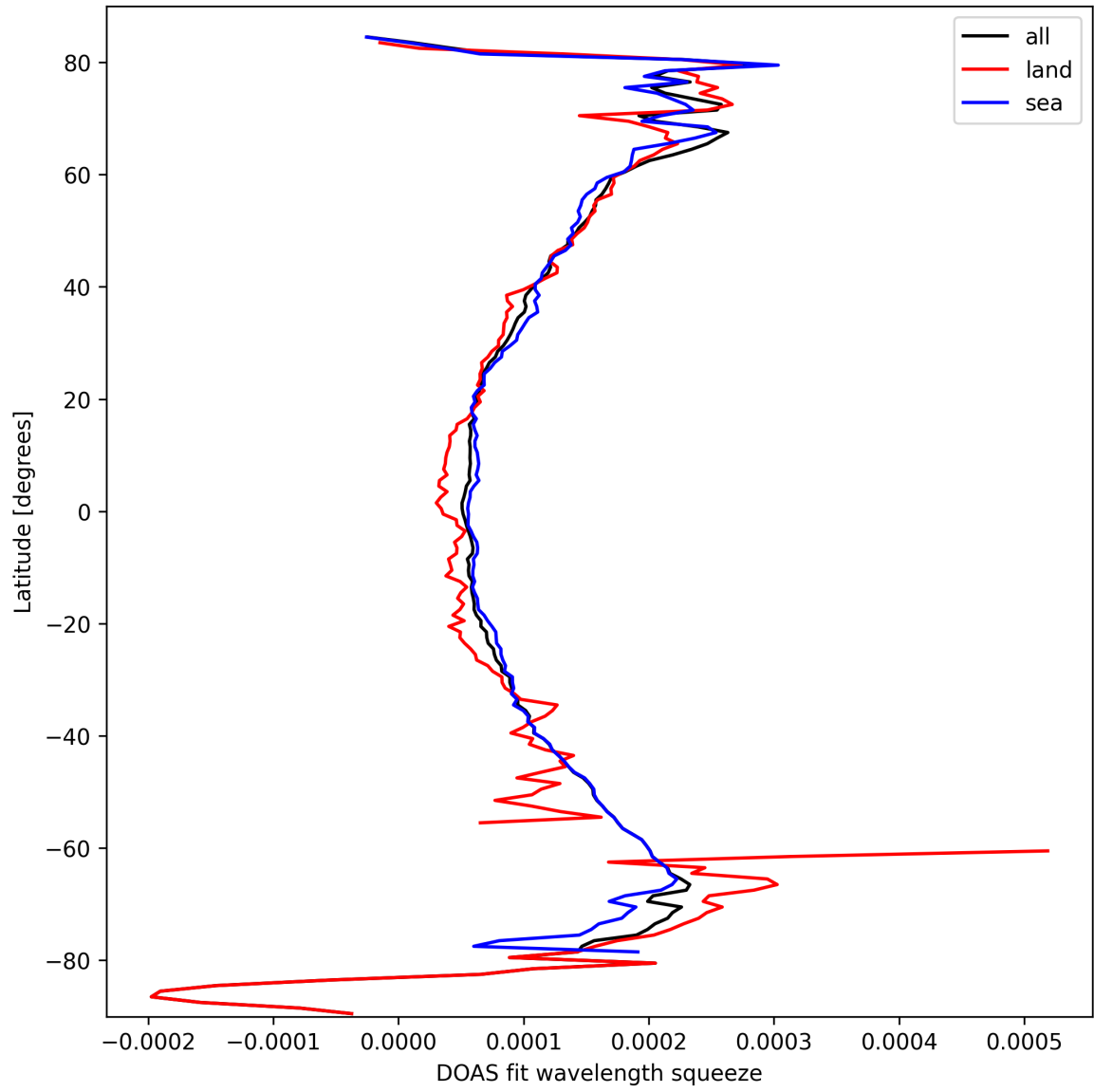
Figure 24: Zonal average of “DOAS fit wavelength squeeze” for 2025-03-07 to 2025-03-08.
