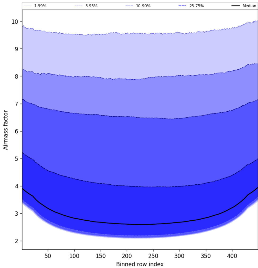
Figure 49: Along track statistics of “Airmass factor” for 2025-03-07 to 2025-03-08
