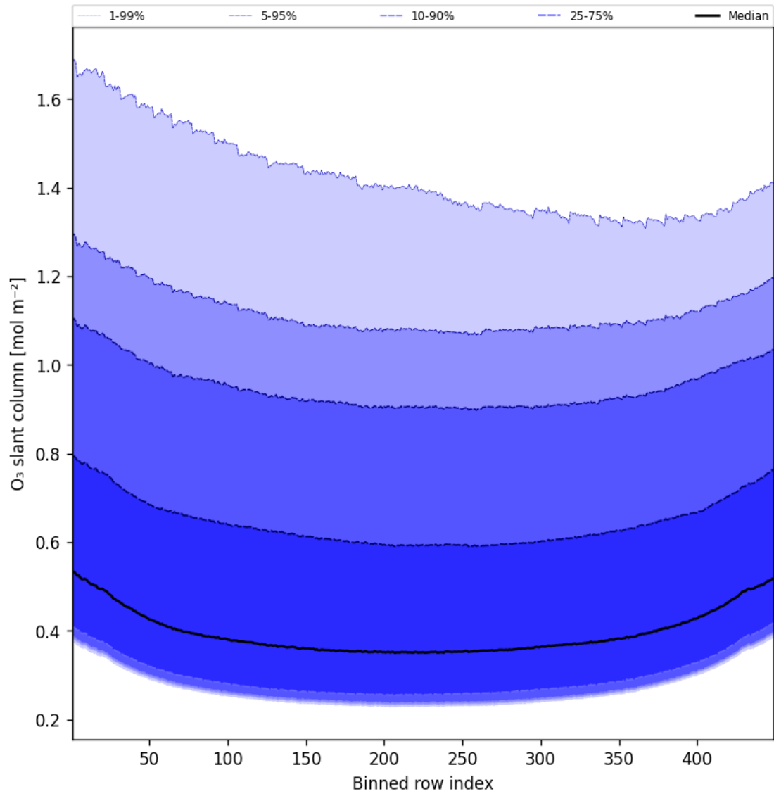
Figure 43: Along track statistics of “O 3 slant column” for 2025-03-07 to 2025-03-08
