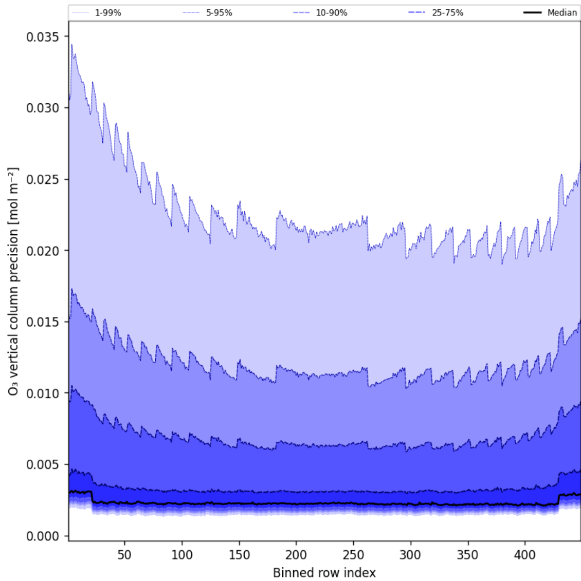
Figure 42: Along track statistics of “O 3 vertical column precision” for 2025-03-07 to 2025-03-08
