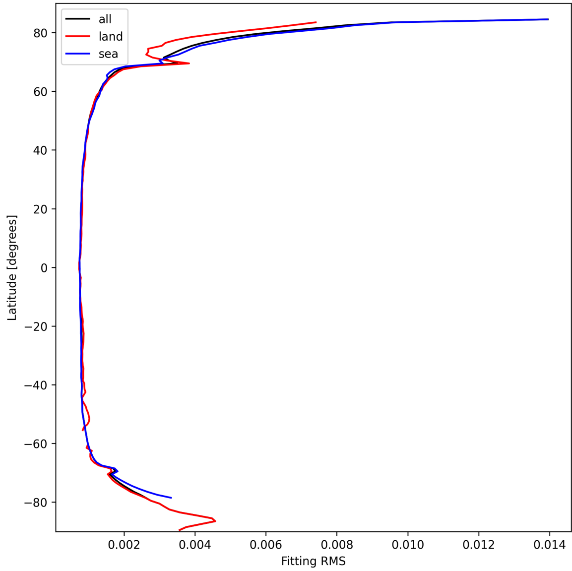
Figure 22: Zonal average of “Fitting RMS” for 2025-03-07 to 2025-03-08.
