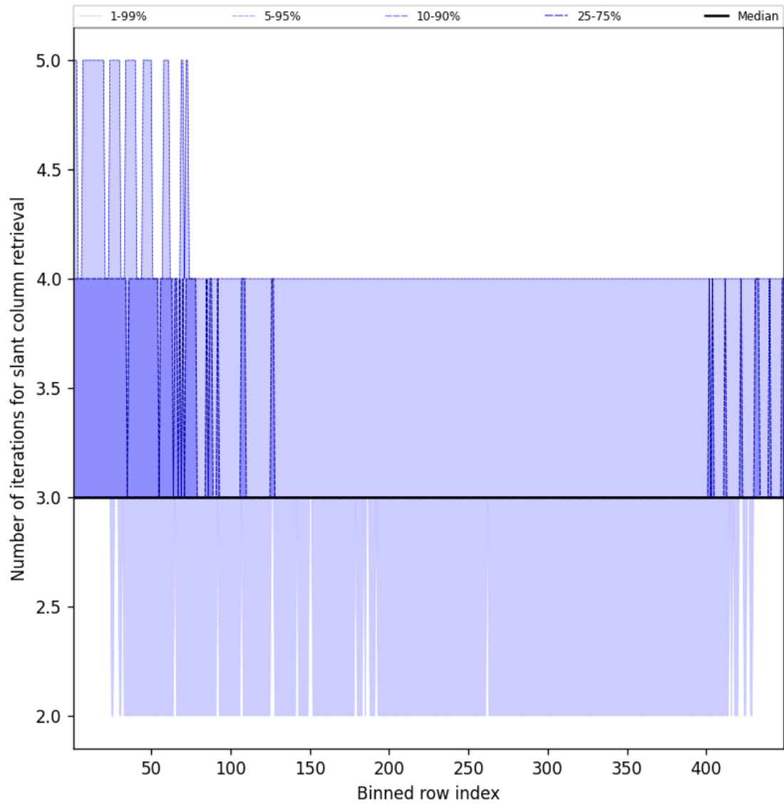
Figure 45: Along track statistics of “Number of iterations for slant column retrieval” for 2025-03-07 to 2025-03-08
