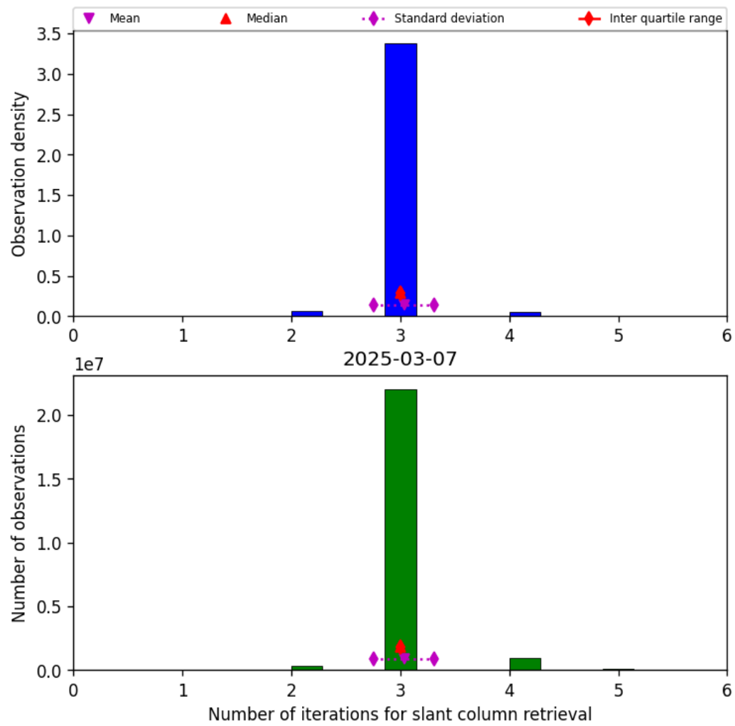
Figure 33: Histogram of “Number of iterations for slant column retrieval” for 2025-03-07 to 2025-03-08
