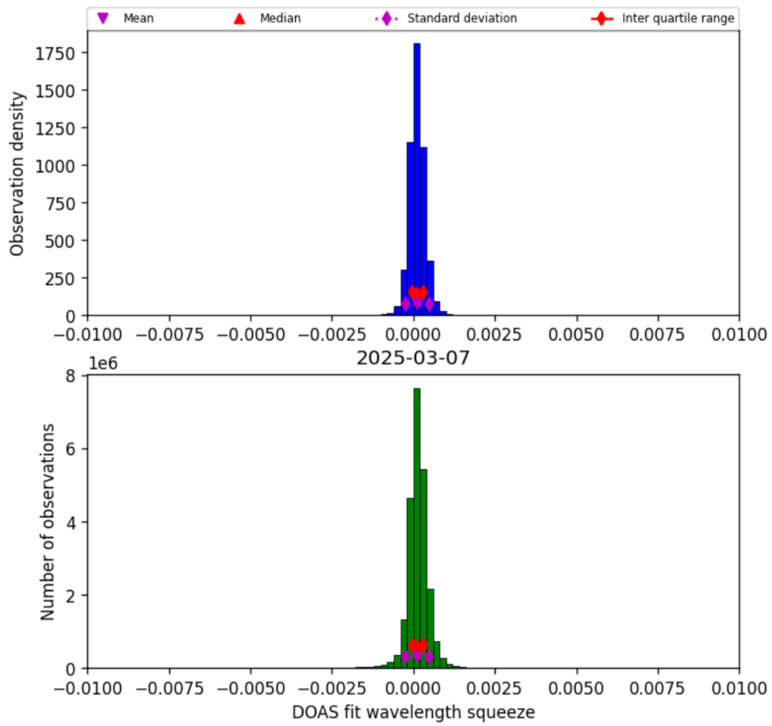
Figure 36: Histogram of “DOAS fit wavelength squeeze” for 2025-03-07 to 2025-03-08
