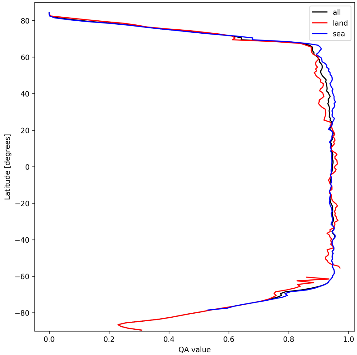
Figure 16: Zonal average of “QA value” for 2025-03-07 to 2025-03-08.
