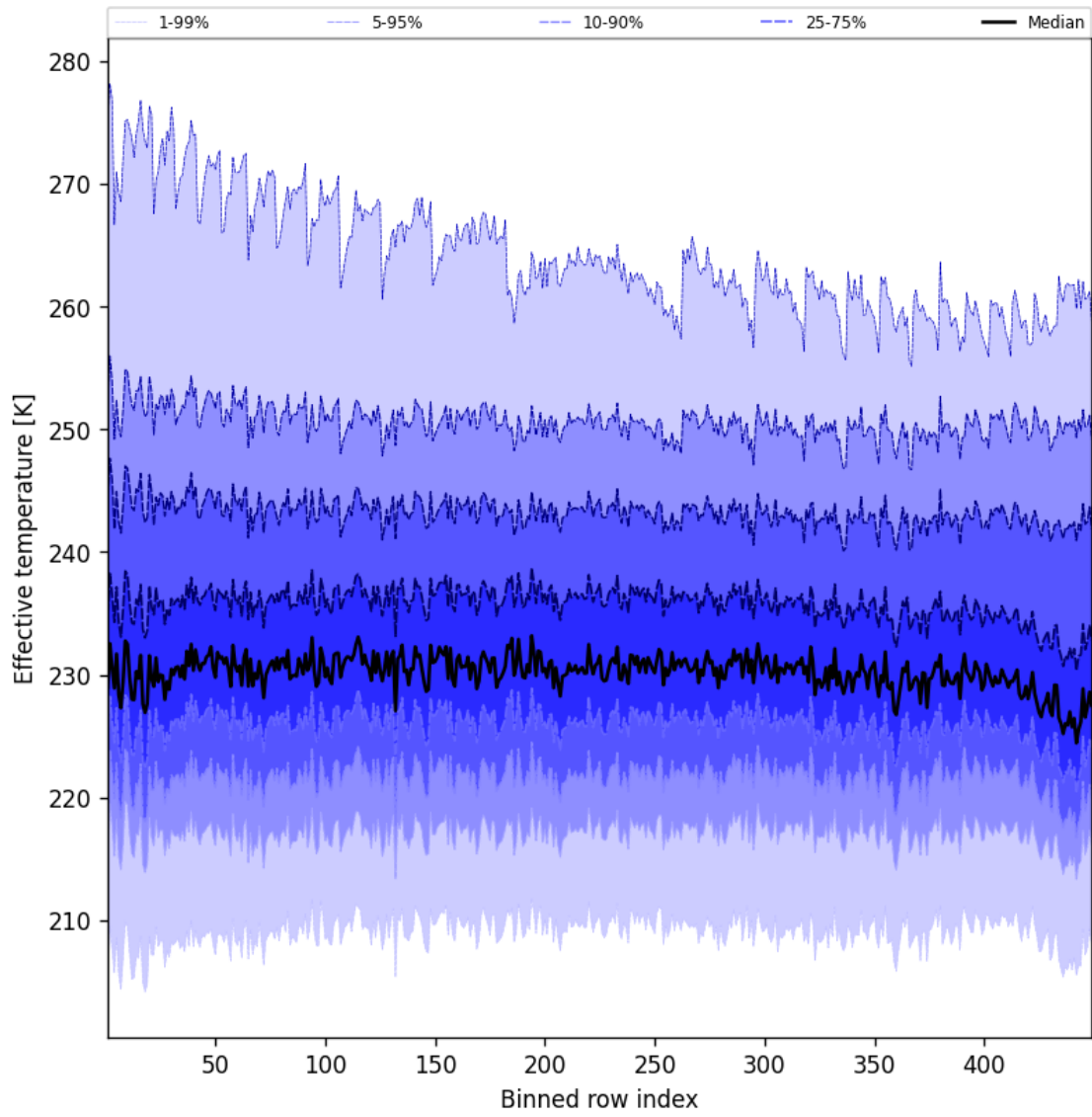
Figure 50: Along track statistics of “Effective temperature” for 2025-03-07 to 2025-03-08
