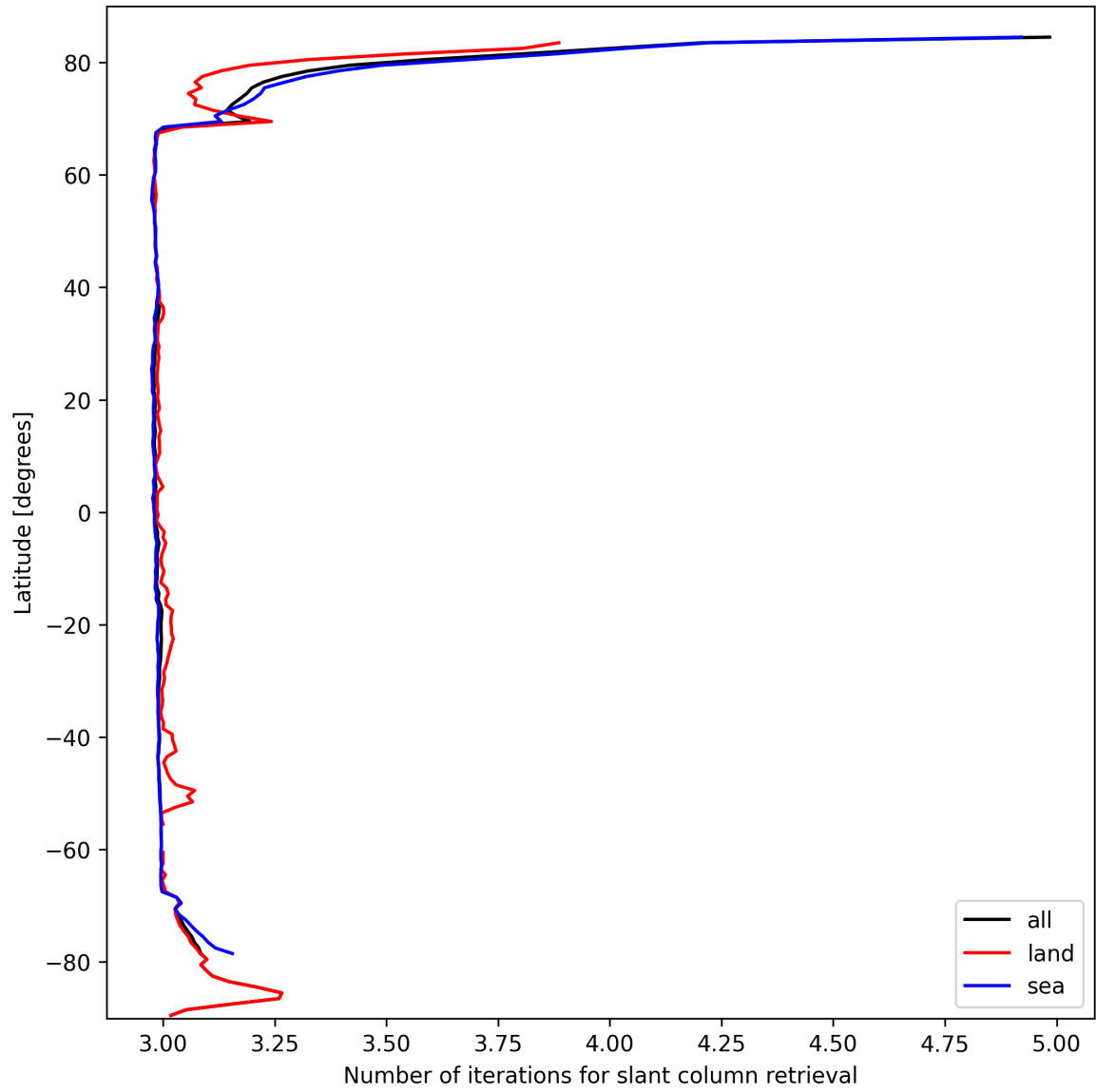
Figure 21: Zonal average of “Number of iterations for slant column retrieval” for 2025-03-07 to 2025-03-08.
