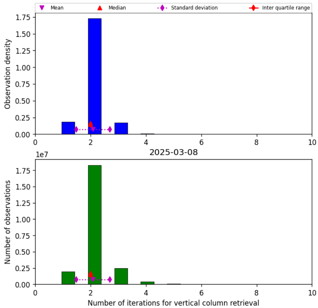
Figure 39: Histogram of “Number of iterations for vertical column retrieval” for 2025-03-08 to 2025-03-09
