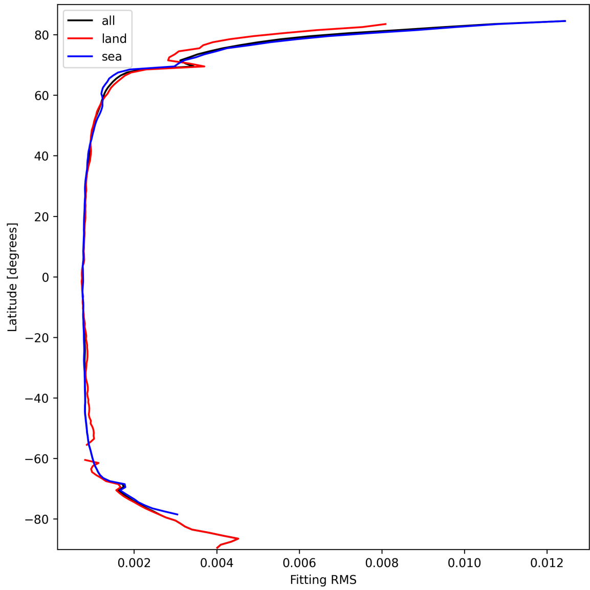
Figure 22: Zonal average of “Fitting RMS” for 2025-03-08 to 2025-03-09.
