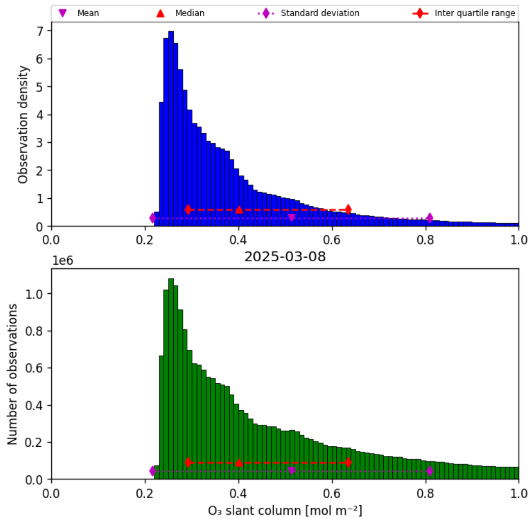
Figure 31: Histogram of “O 3 slant column” for 2025-03-08 to 2025-03-09
