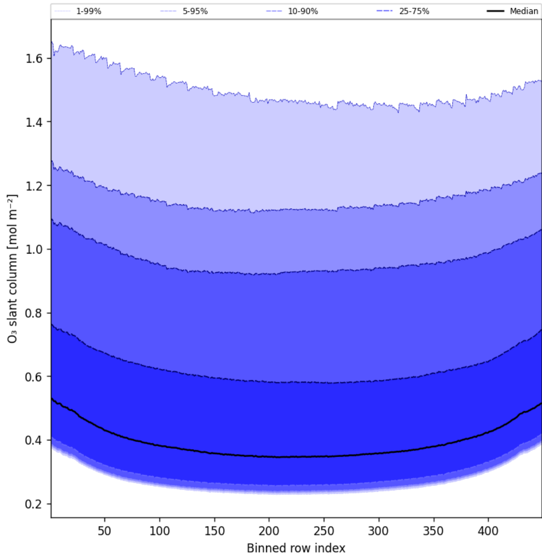
Figure 43: Along track statistics of “O 3 slant column” for 2025-03-08 to 2025-03-09
