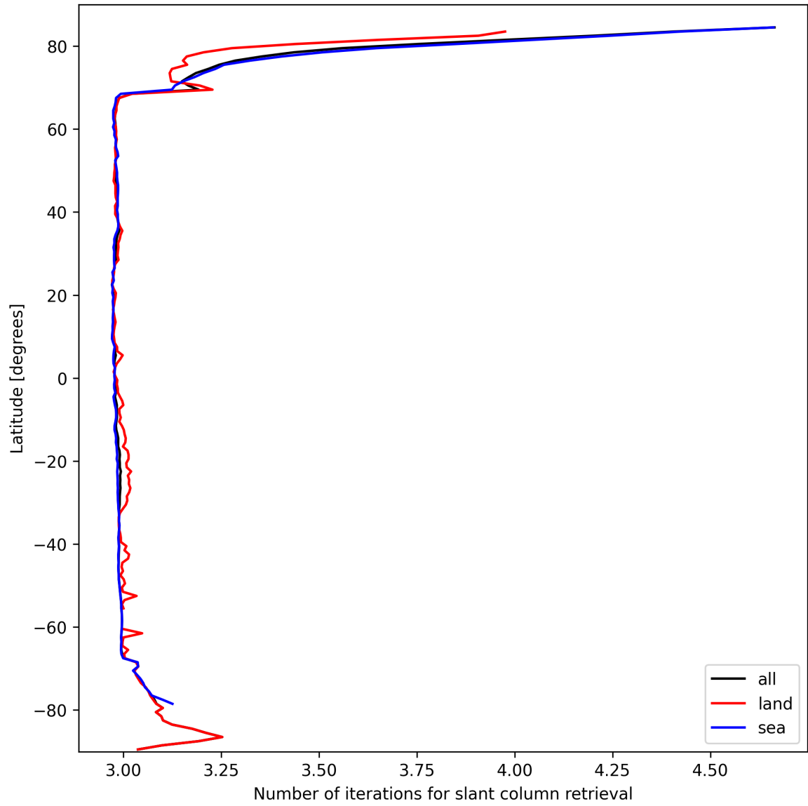
Figure 21: Zonal average of “Number of iterations for slant column retrieval” for 2025-03-08 to 2025-03-09.
