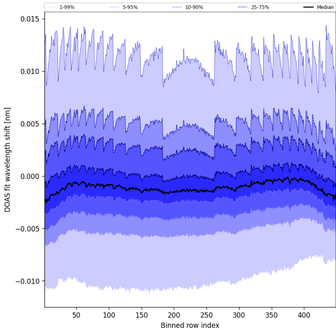
Figure 47: Along track statistics of “DOAS fit wavelength shift” for 2025-03-08 to 2025-03-09
