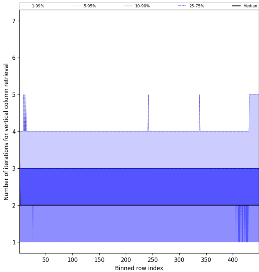
Figure 51: Along track statistics of “Number of iterations for vertical column retrieval” for 2025-03-08 to 2025-03-09
