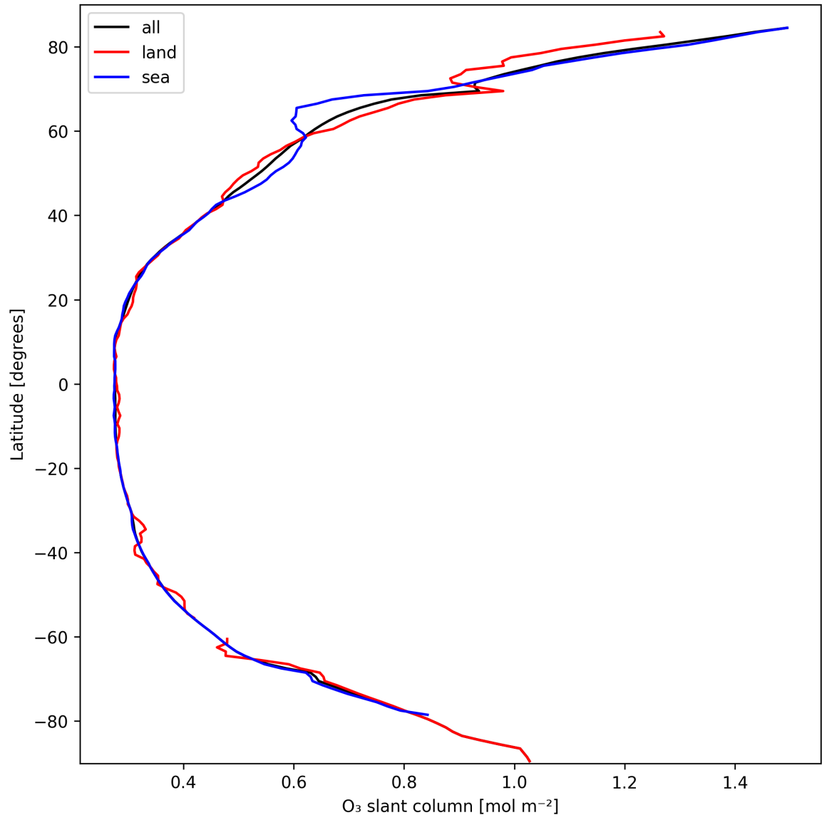
Figure 19: Zonal average of “O 3 slant column” for 2025-03-08 to 2025-03-09.
