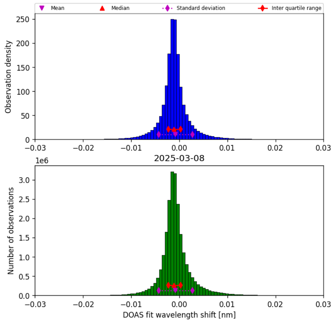
Figure 35: Histogram of “DOAS fit wavelength shift” for 2025-03-08 to 2025-03-09
