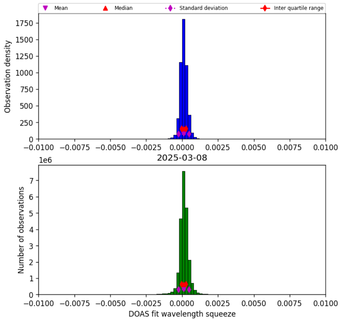
Figure 36: Histogram of “DOAS fit wavelength squeeze” for 2025-03-08 to 2025-03-09
