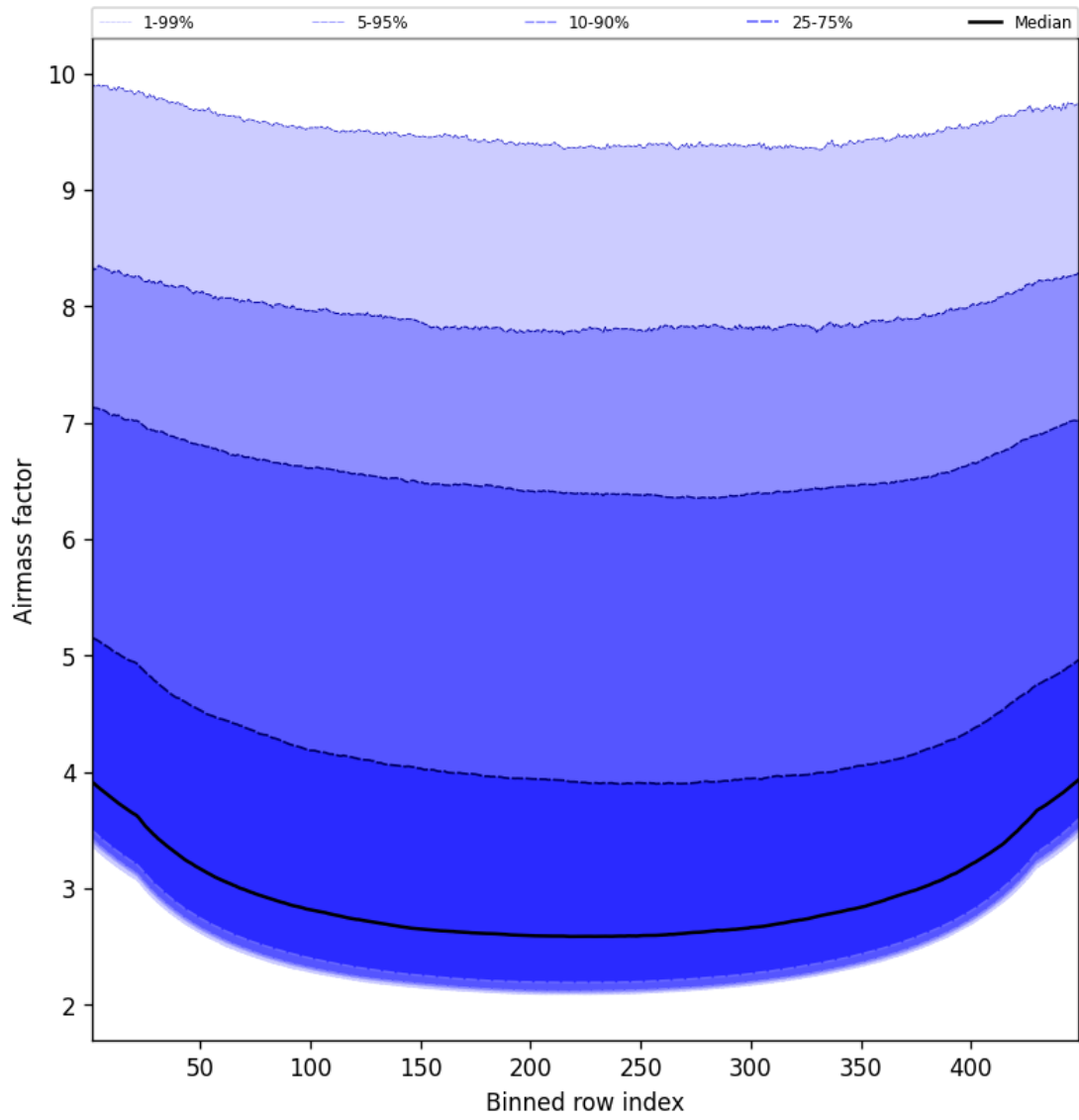
Figure 49: Along track statistics of “Airmass factor” for 2025-03-08 to 2025-03-09
