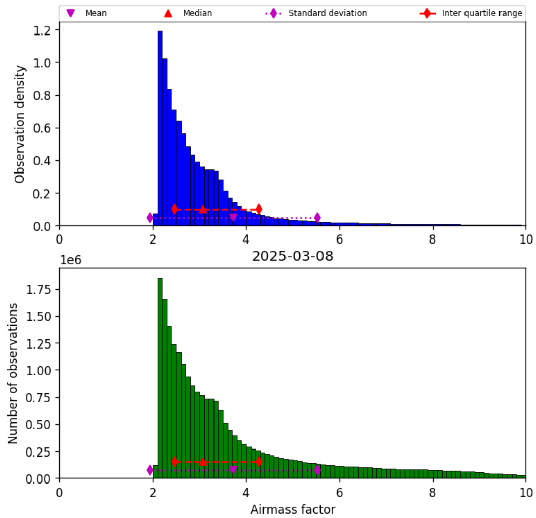
Figure 37: Histogram of “Airmass factor” for 2025-03-08 to 2025-03-09
