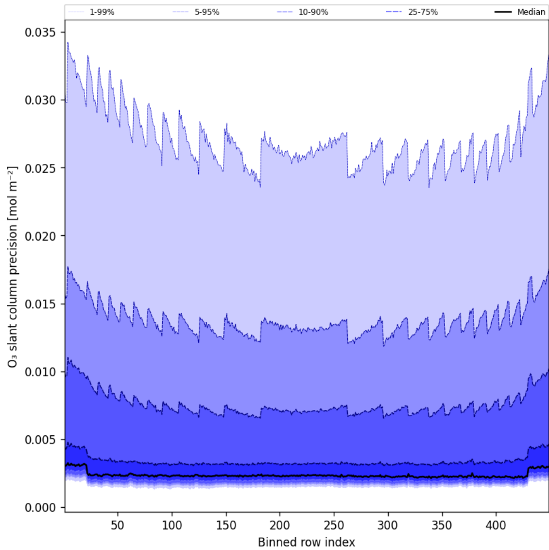
Figure 44: Along track statistics of “O 3 slant column precision” for 2025-03-08 to 2025-03-09
