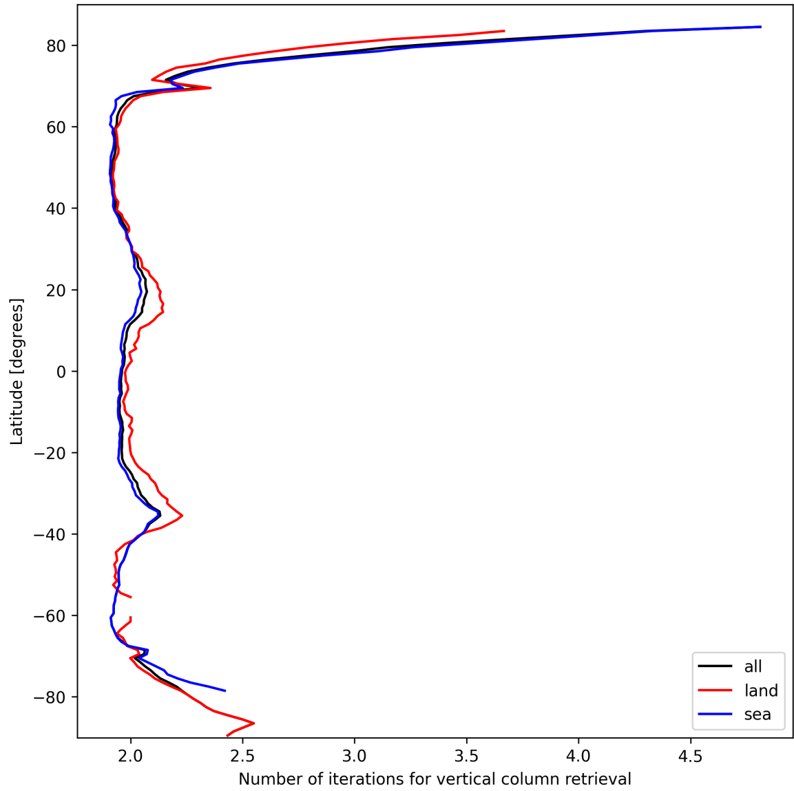
Figure 27: Zonal average of “Number of iterations for vertical column retrieval” for 2025-03-08 to 2025-03-09.
