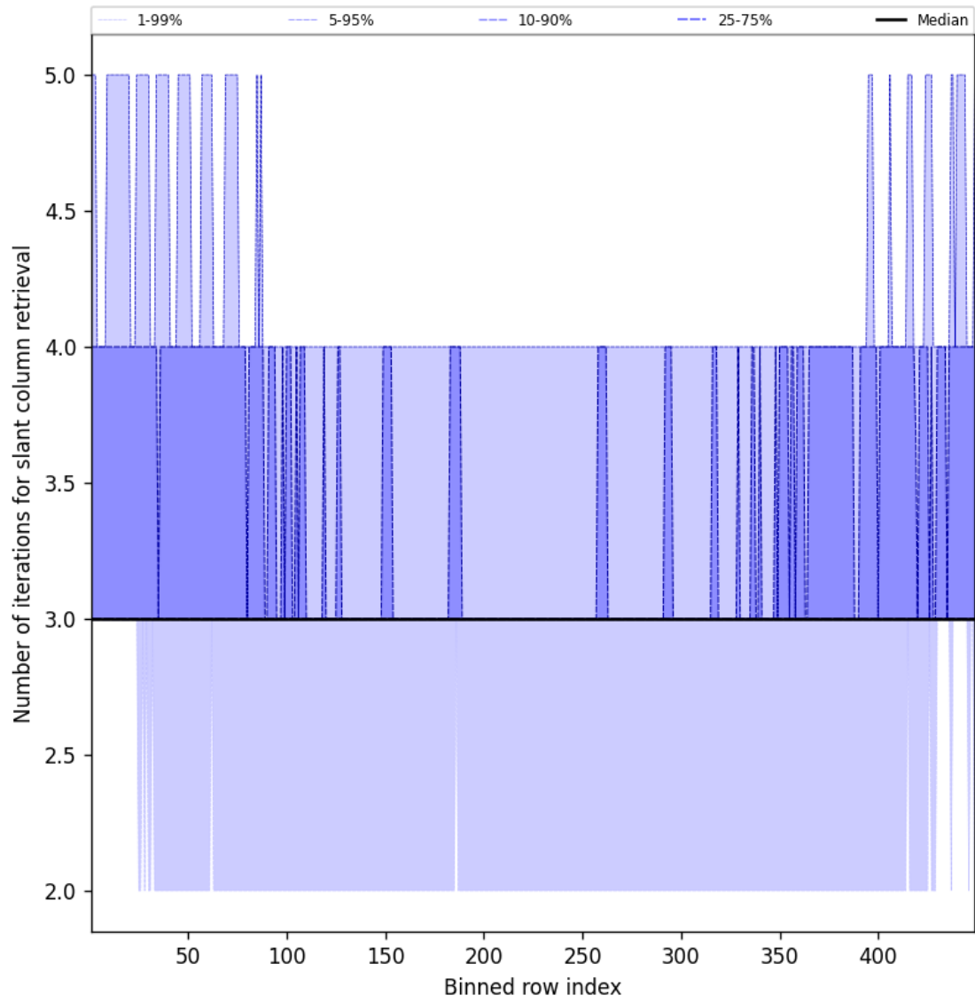
Figure 45: Along track statistics of “Number of iterations for slant column retrieval” for 2025-03-08 to 2025-03-09
