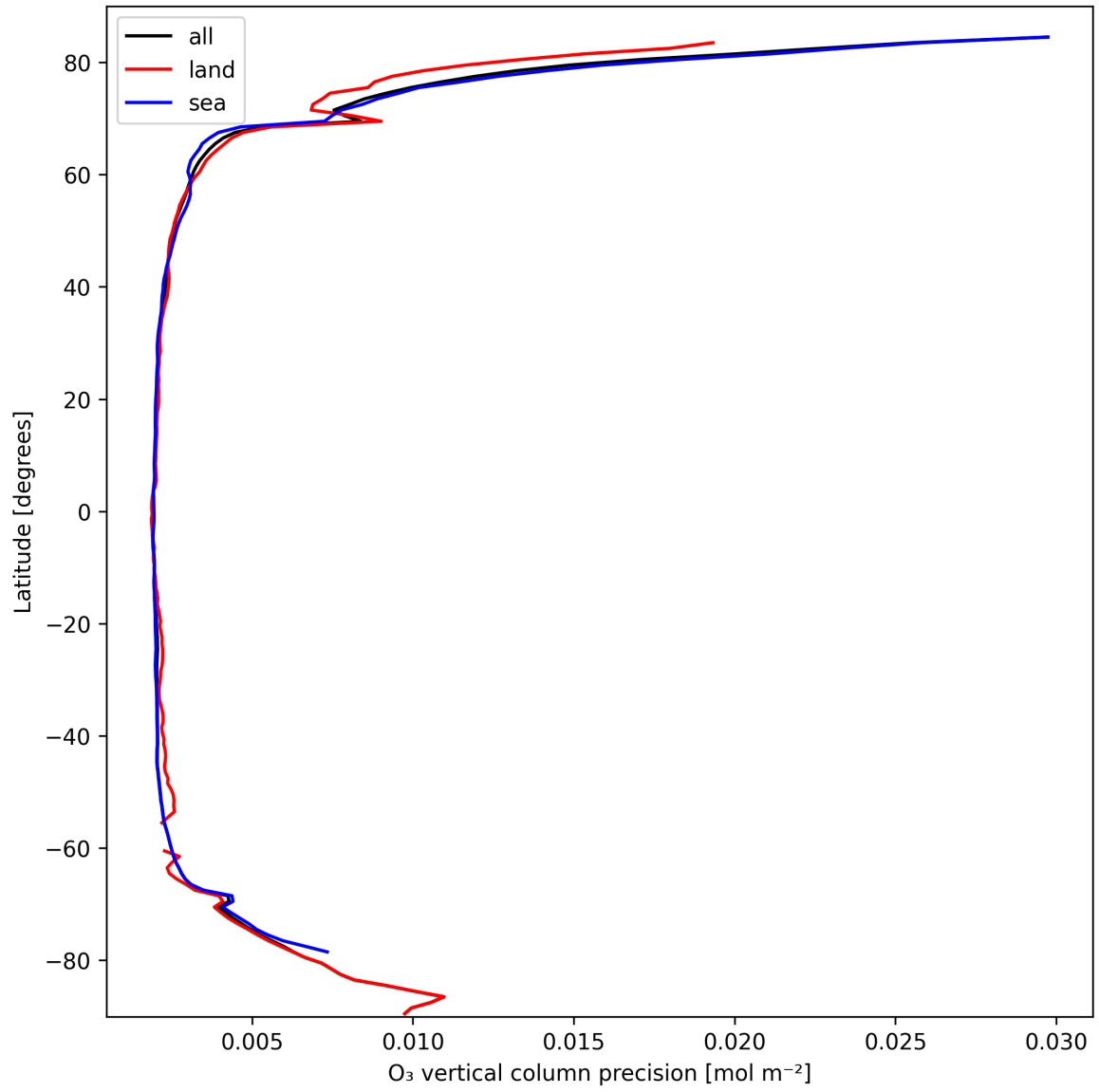
Figure 18: Zonal average of “O 3 vertical column precision” for 2025-03-08 to 2025-03-09.
