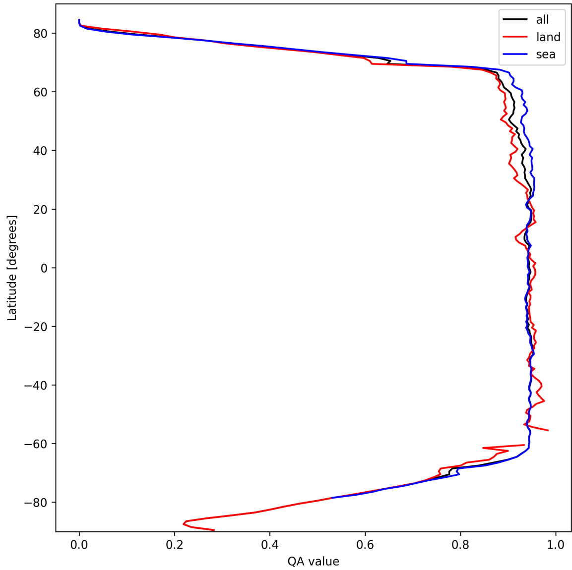
Figure 16: Zonal average of “QA value” for 2025-03-08 to 2025-03-09.
