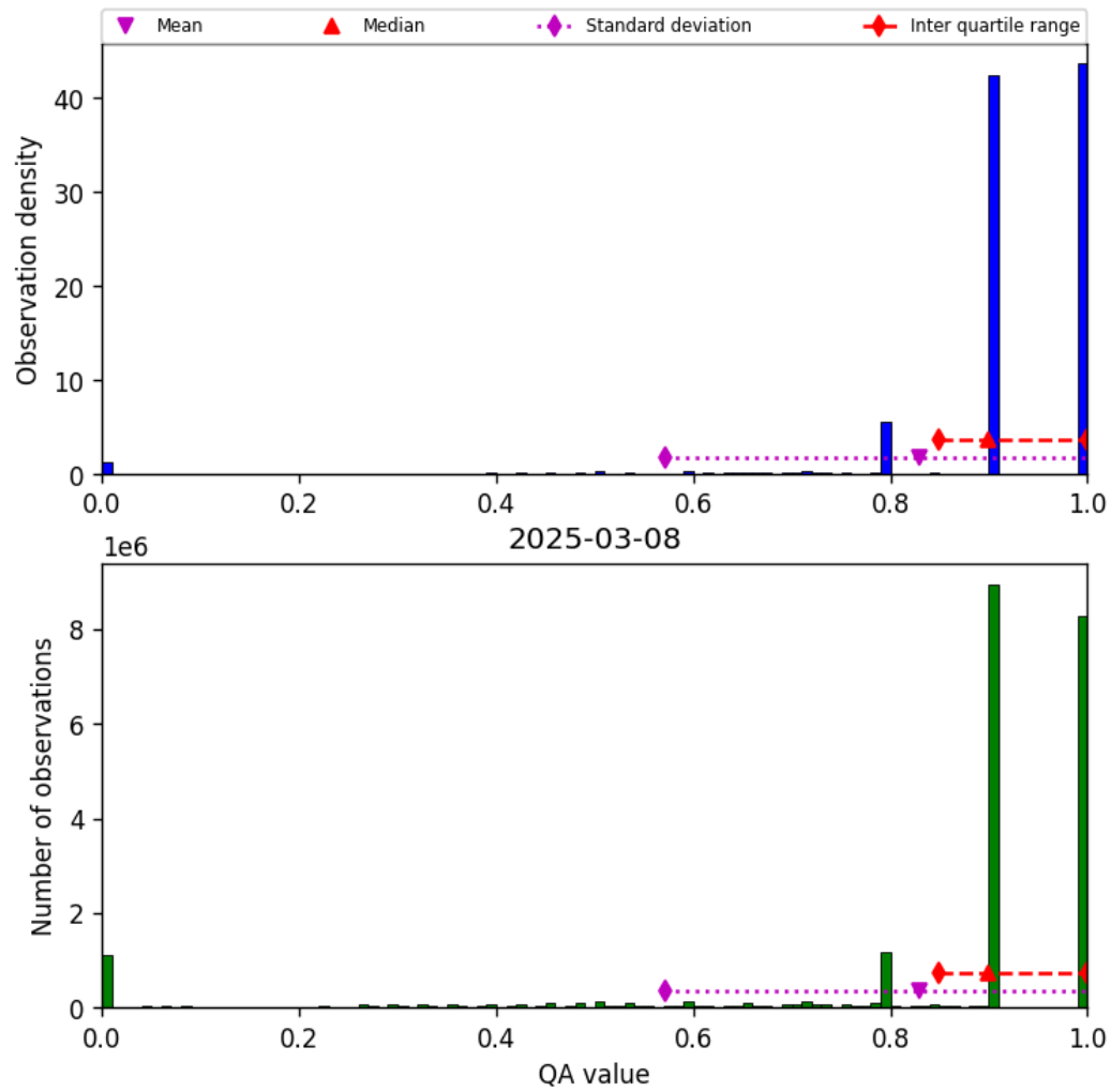
Figure 28: Histogram of “QA value” for 2025-03-08 to 2025-03-09
