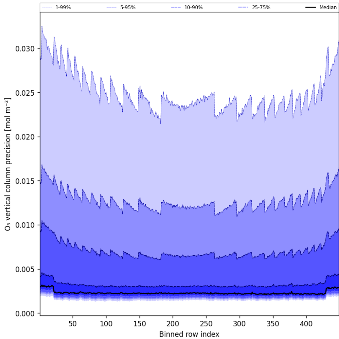
Figure 42: Along track statistics of “O 3 vertical column precision” for 2025-03-08 to 2025-03-09
