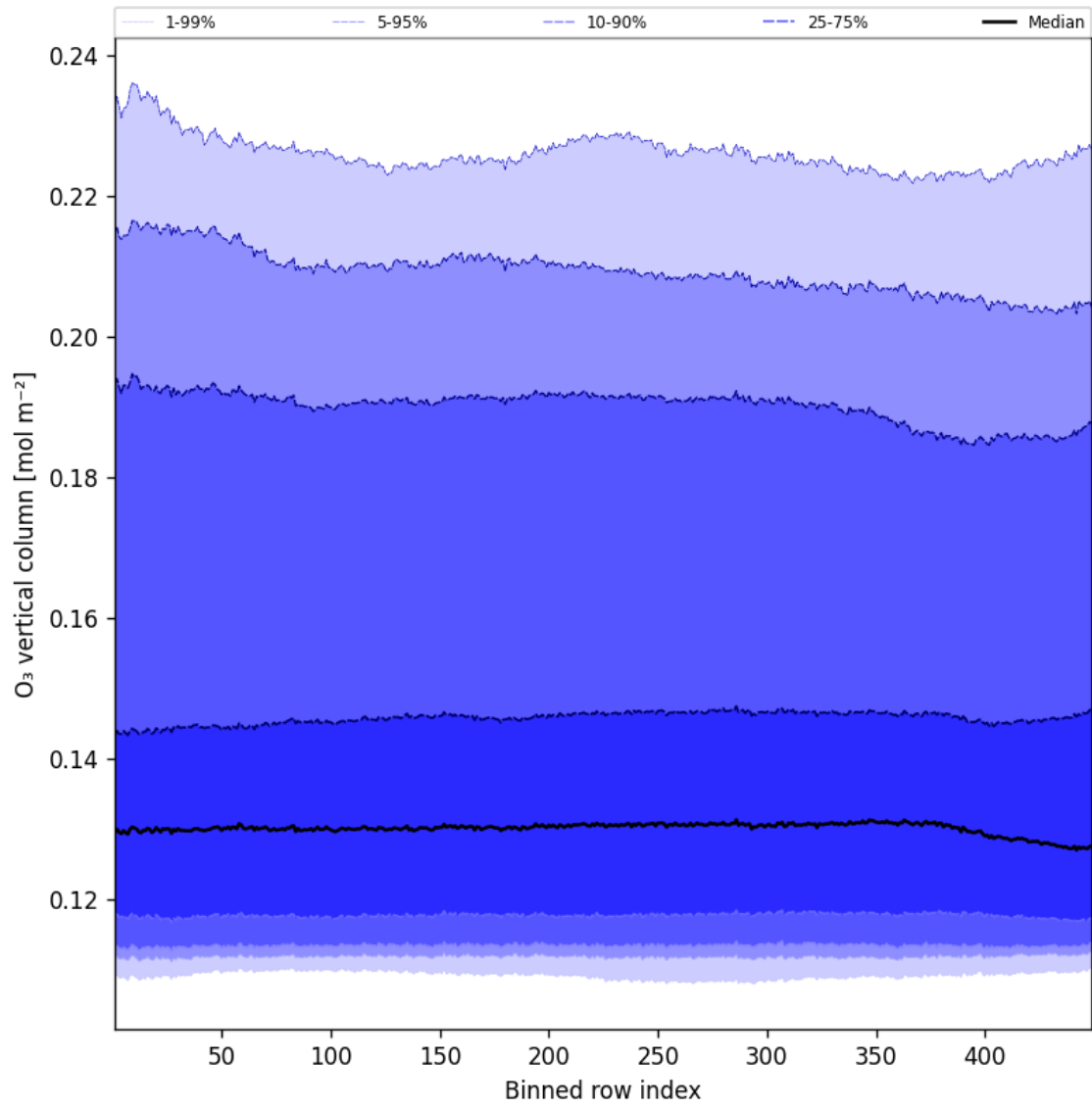
Figure 41: Along track statistics of “O 3 vertical column” for 2025-03-08 to 2025-03-09
