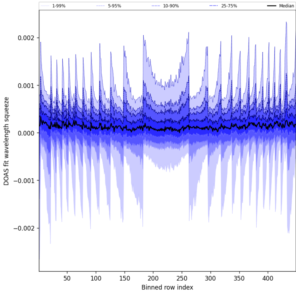
Figure 48: Along track statistics of “DOAS fit wavelength squeeze” for 2025-03-08 to 2025-03-09
