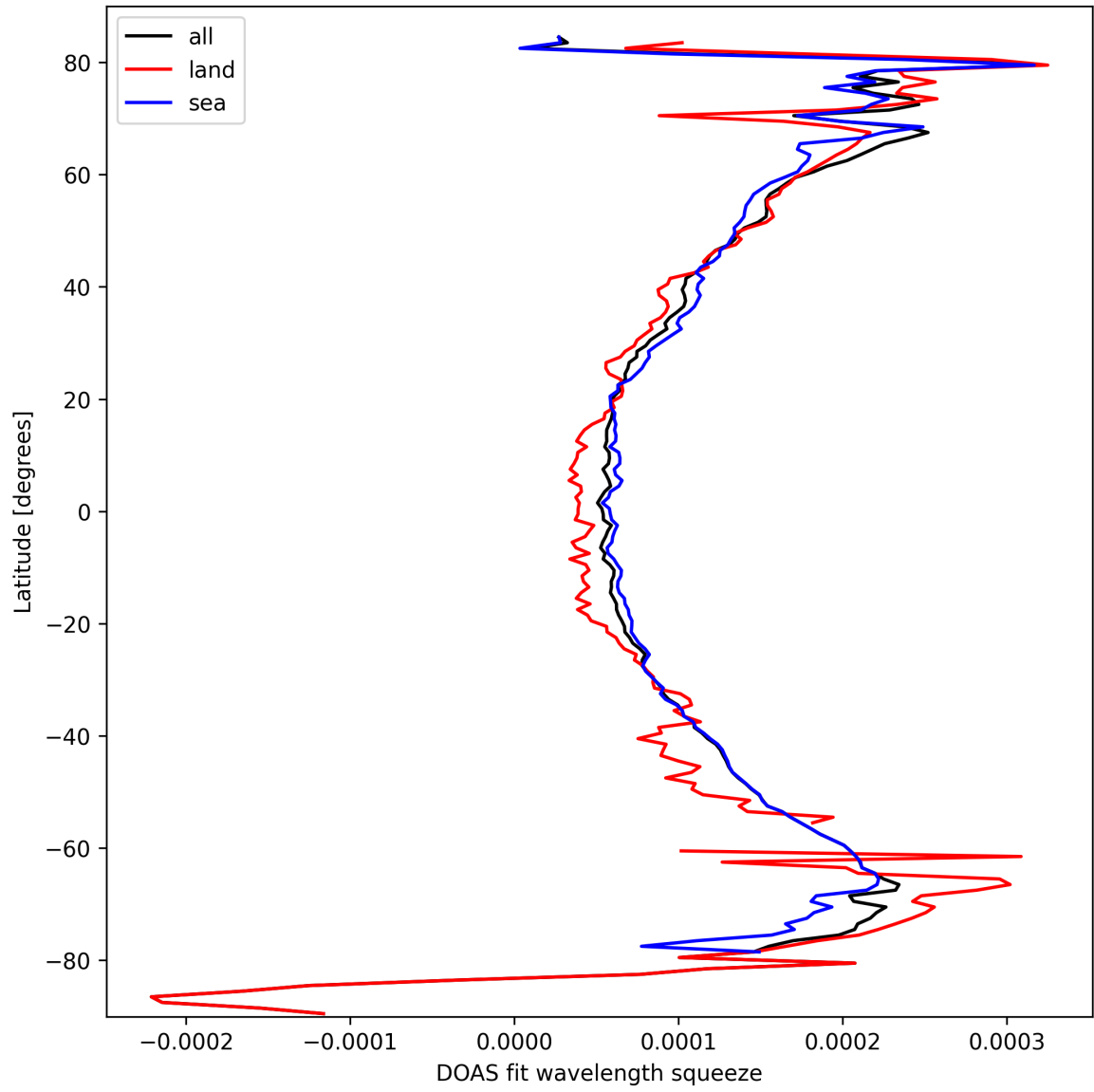
Figure 24: Zonal average of “DOAS fit wavelength squeeze” for 2025-03-08 to 2025-03-09.
