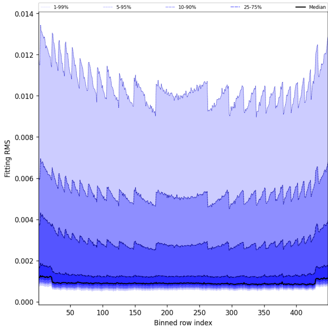
Figure 46: Along track statistics of “Fitting RMS” for 2025-03-08 to 2025-03-09
