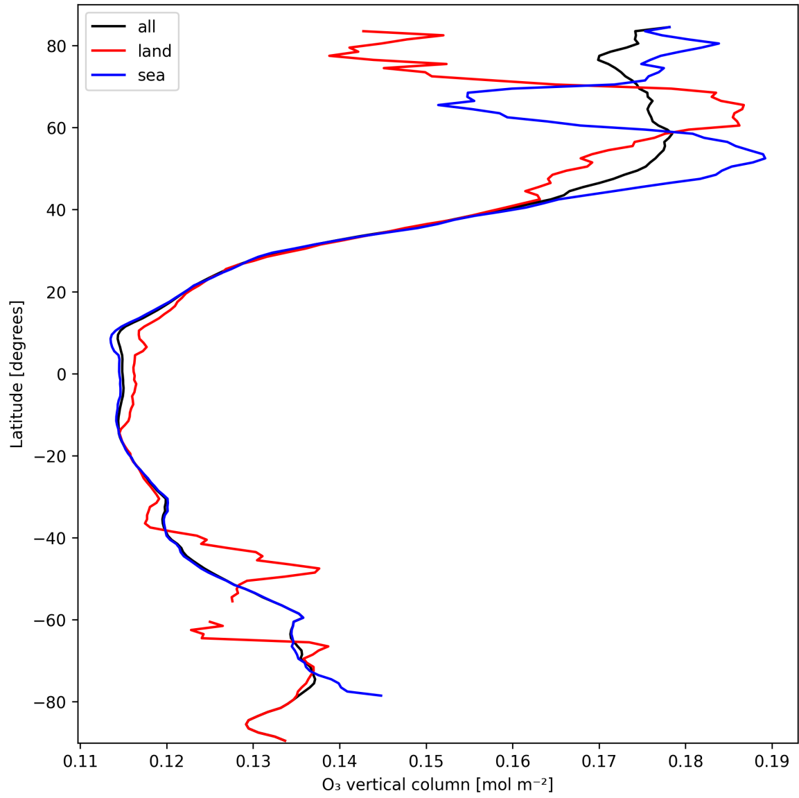
Figure 17: Zonal average of “O 3 vertical column” for 2025-03-08 to 2025-03-09.
