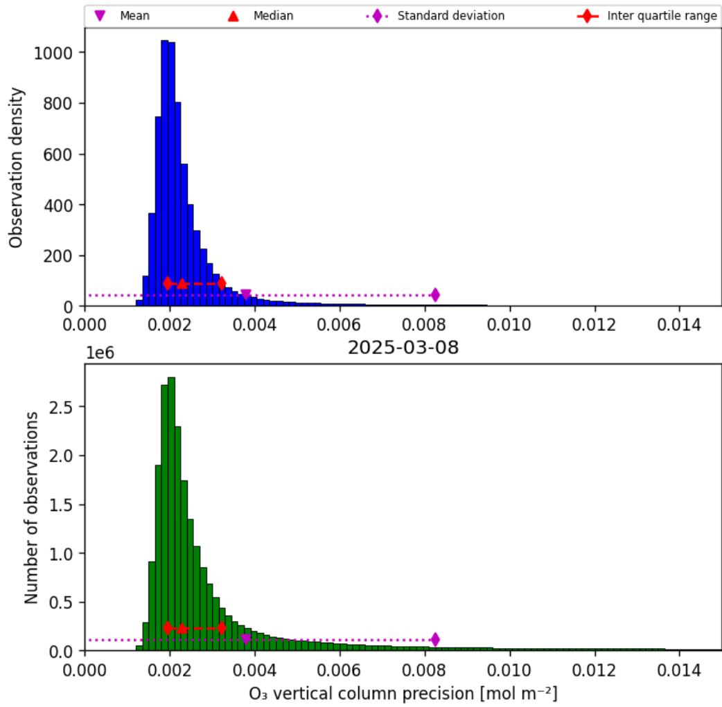
Figure 30: Histogram of “O 3 vertical column precision” for 2025-03-08 to 2025-03-09
