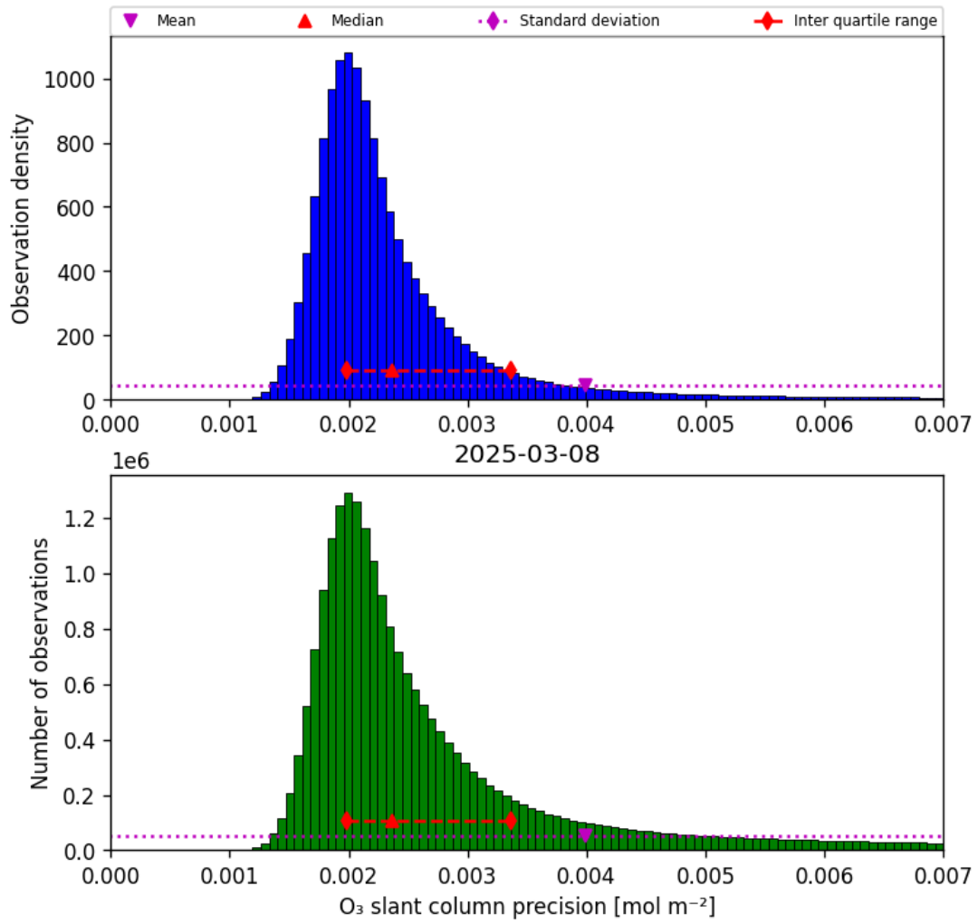
Figure 32: Histogram of “O 3 slant column precision” for 2025-03-08 to 2025-03-09
