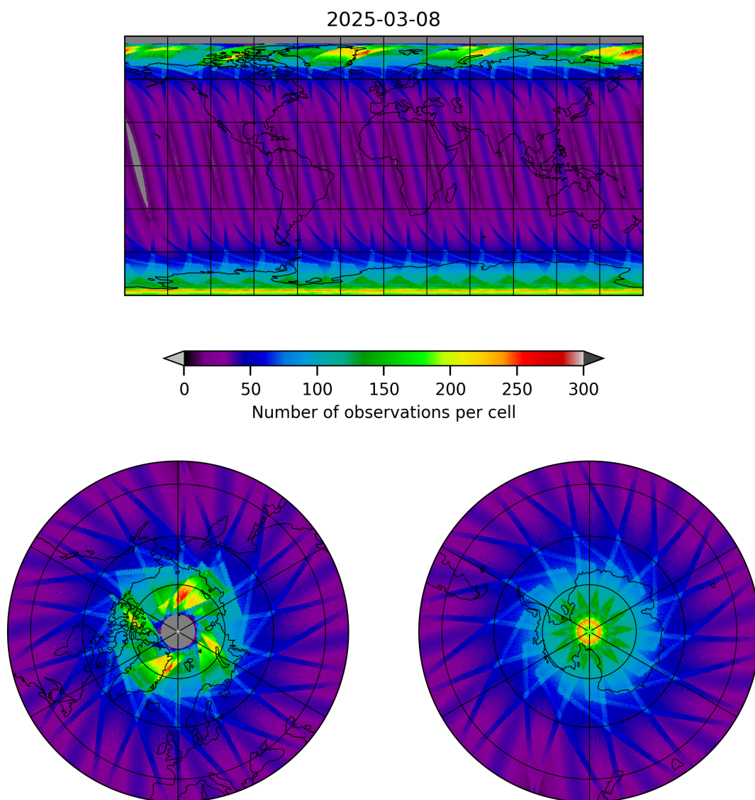
Figure 15: Map of the number of observations for 2025-03-08 to 2025-03-09
