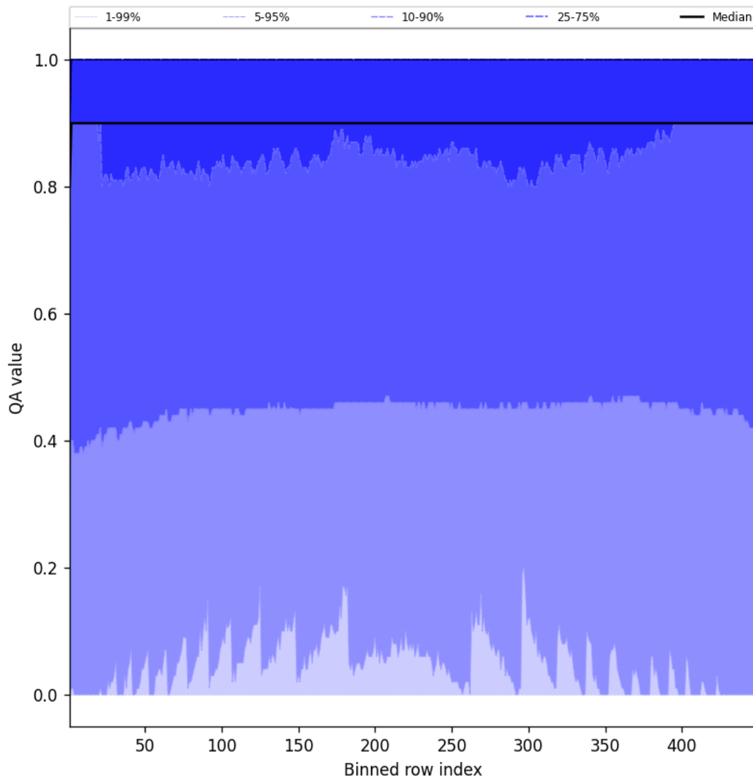
Figure 40: Along track statistics of “QA value” for 2025-03-08 to 2025-03-09
