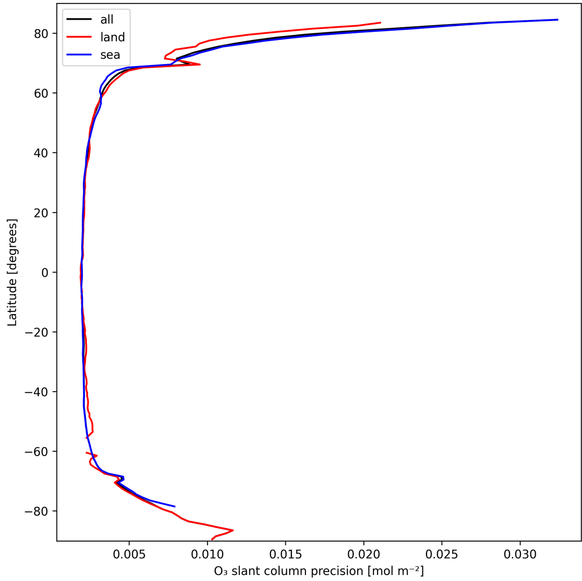
Figure 20: Zonal average of “O 3 slant column precision” for 2025-03-08 to 2025-03-09.
