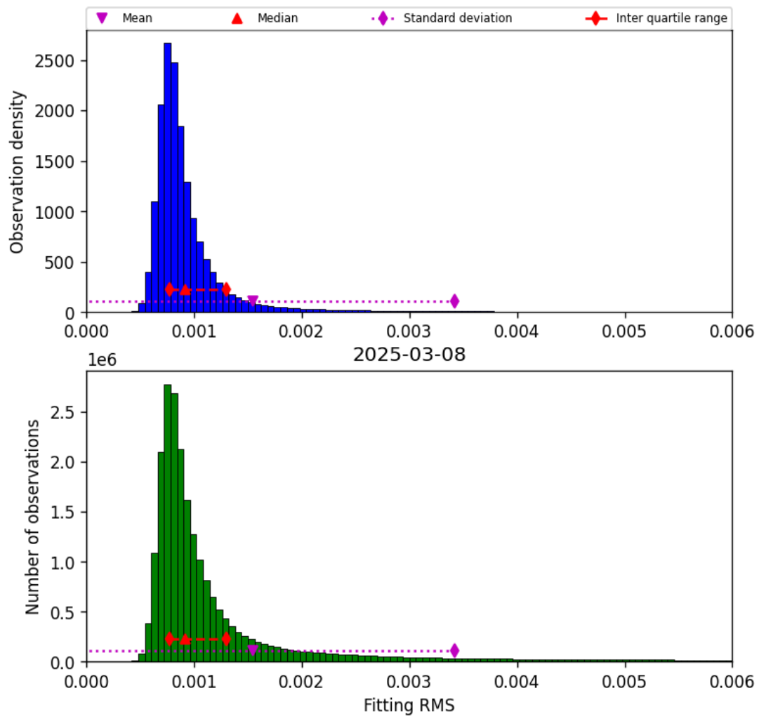
Figure 34: Histogram of “Fitting RMS” for 2025-03-08 to 2025-03-09
