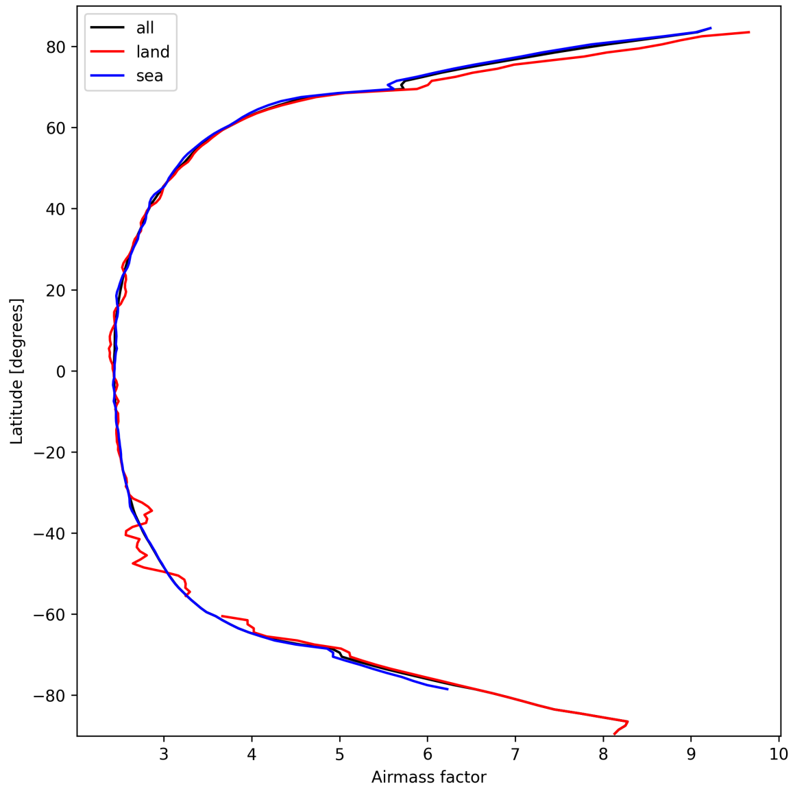
Figure 25: Zonal average of “Airmass factor” for 2025-03-08 to 2025-03-09.
