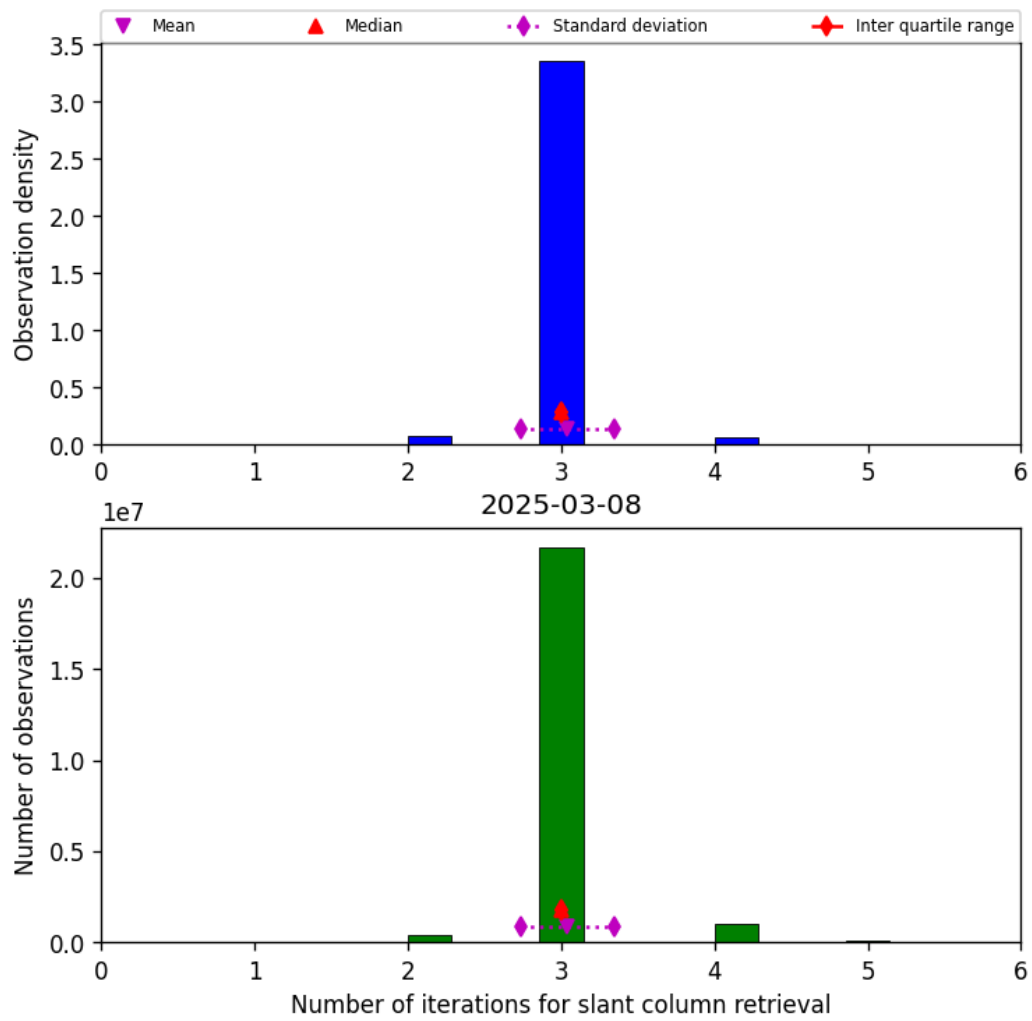
Figure 33: Histogram of “Number of iterations for slant column retrieval” for 2025-03-08 to 2025-03-09
