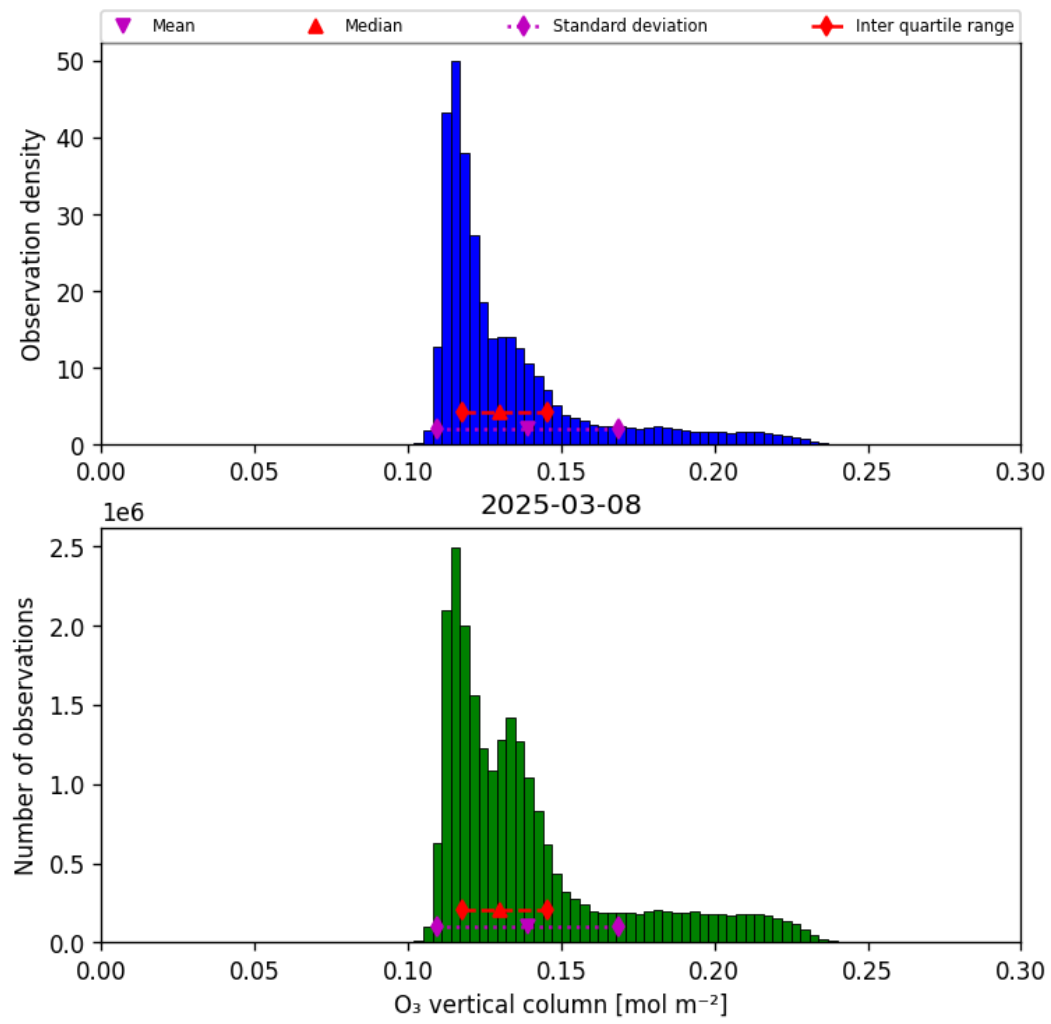
Figure 29: Histogram of “O 3 vertical column” for 2025-03-08 to 2025-03-09
