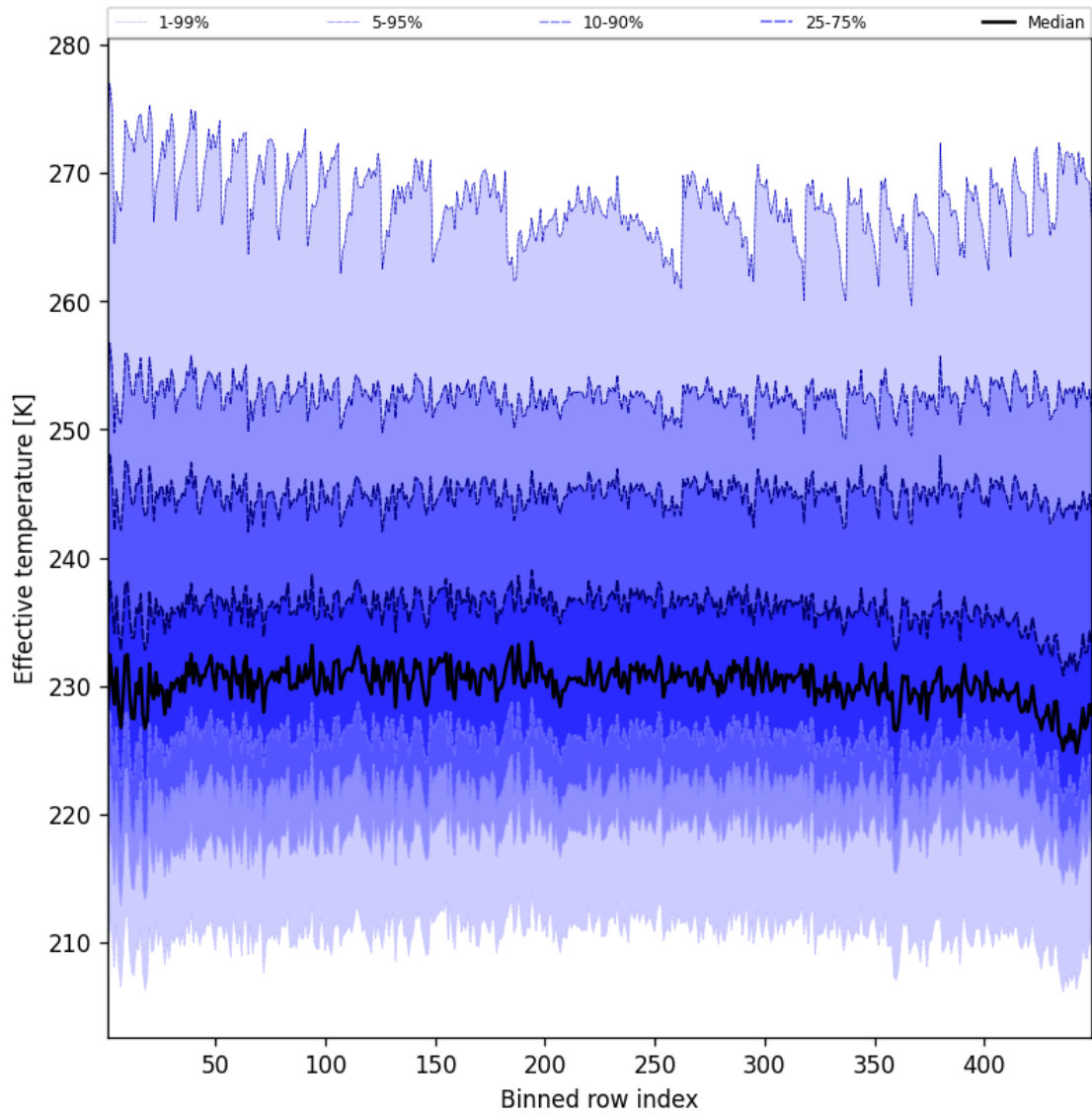
Figure 50: Along track statistics of “Effective temperature” for 2025-03-08 to 2025-03-09
