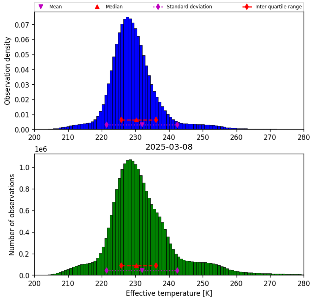
Figure 38: Histogram of “Effective temperature” for 2025-03-08 to 2025-03-09
