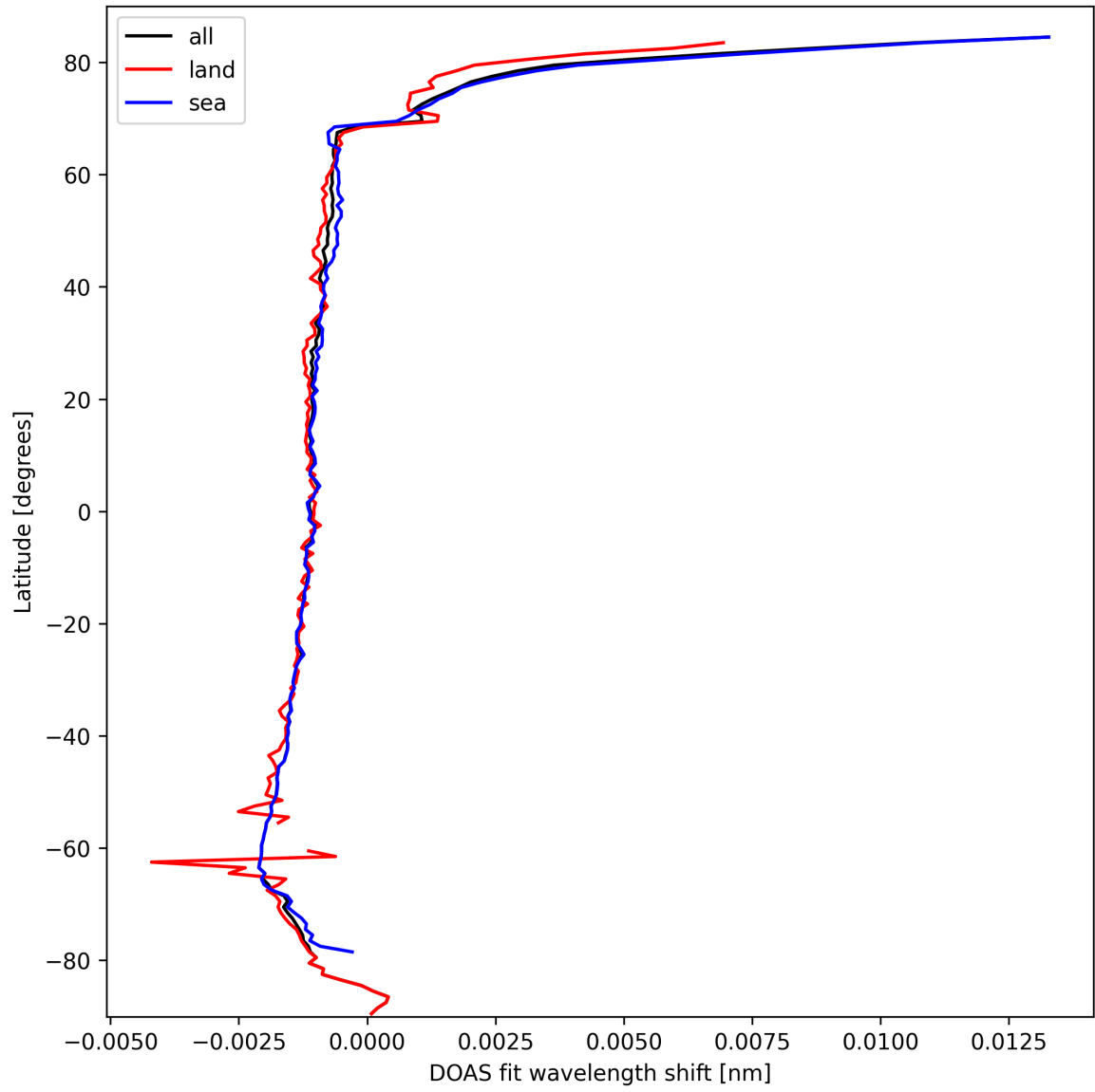
Figure 23: Zonal average of “DOAS fit wavelength shift” for 2025-03-08 to 2025-03-09.
