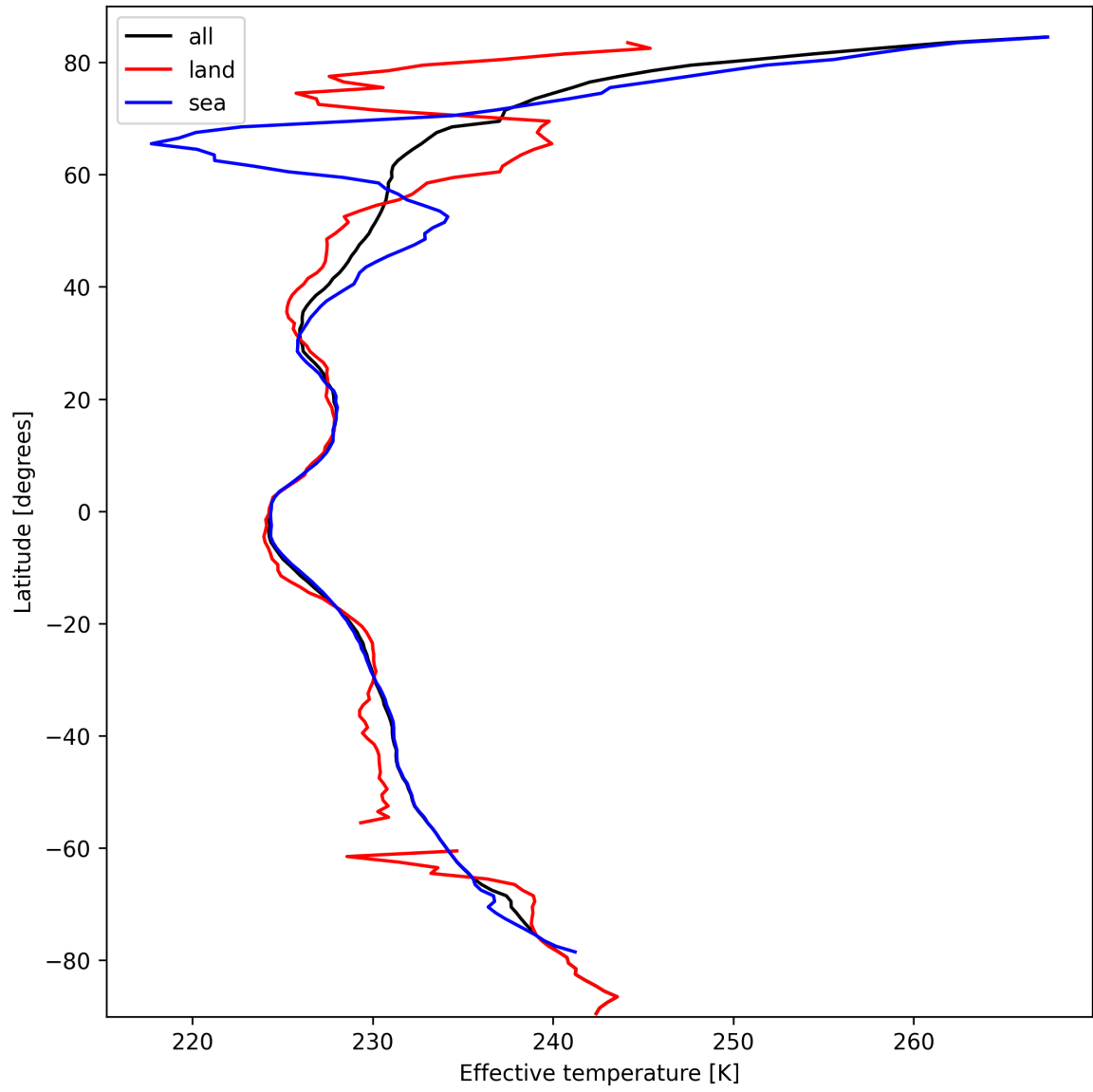
Figure 26: Zonal average of “Effective temperature” for 2025-03-08 to 2025-03-09.
