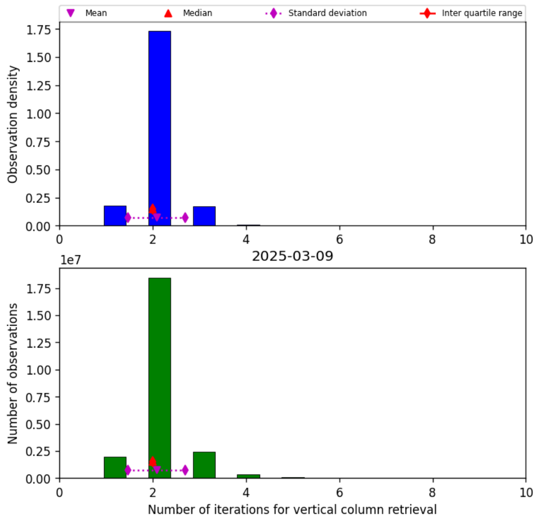
Figure 39: Histogram of “Number of iterations for vertical column retrieval” for 2025-03-09 to 2025-03-10
