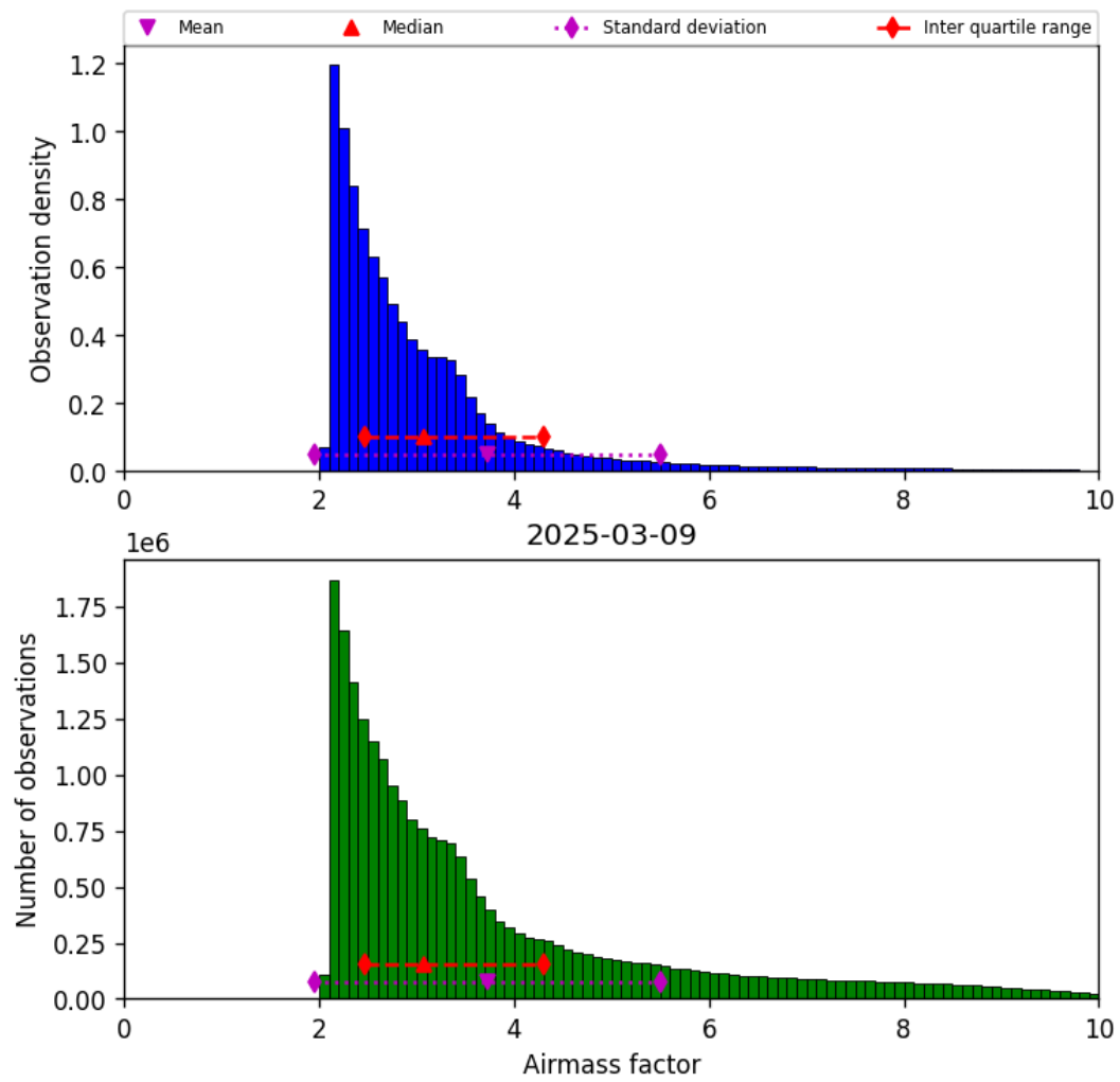
Figure 37: Histogram of “Airmass factor” for 2025-03-09 to 2025-03-10
