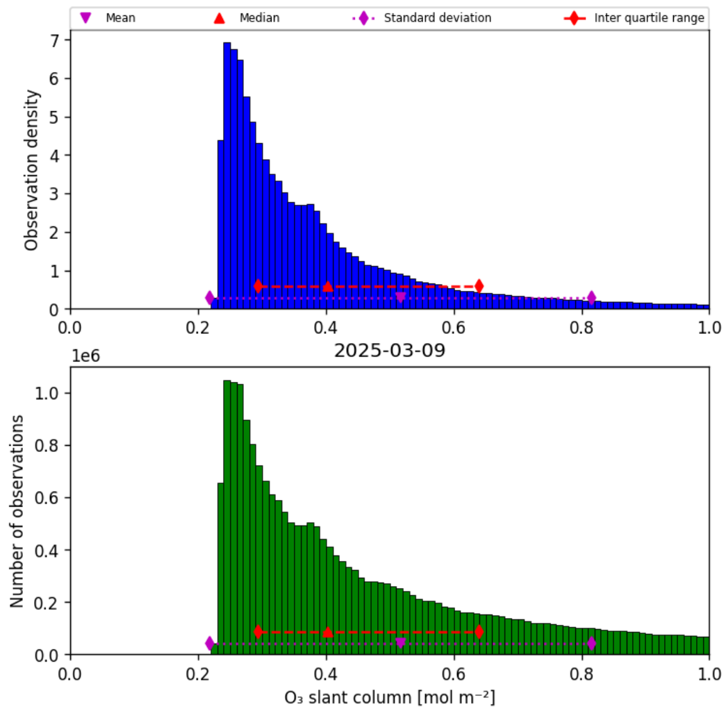
Figure 31: Histogram of “O 3 slant column” for 2025-03-09 to 2025-03-10
