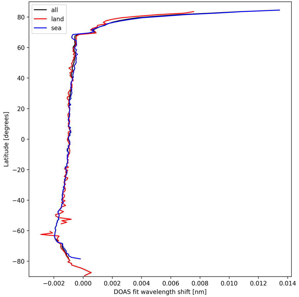
Figure 23: Zonal average of "DOAS fit wavelength shift" for 2025-03-09 to 2025-03-10.
