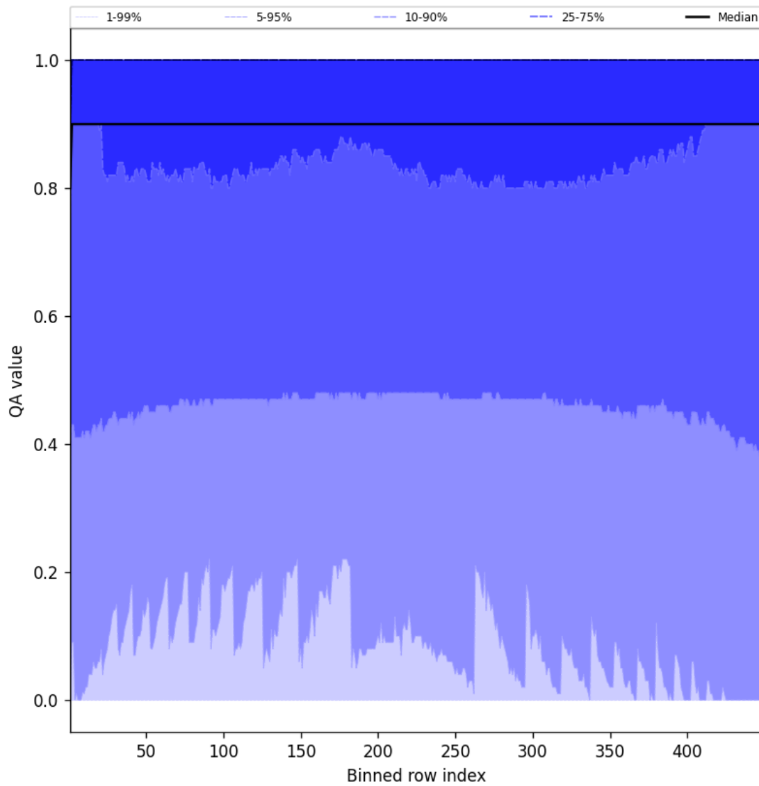
Figure 40: Along track statistics of “QA value” for 2025-03-09 to 2025-03-10
