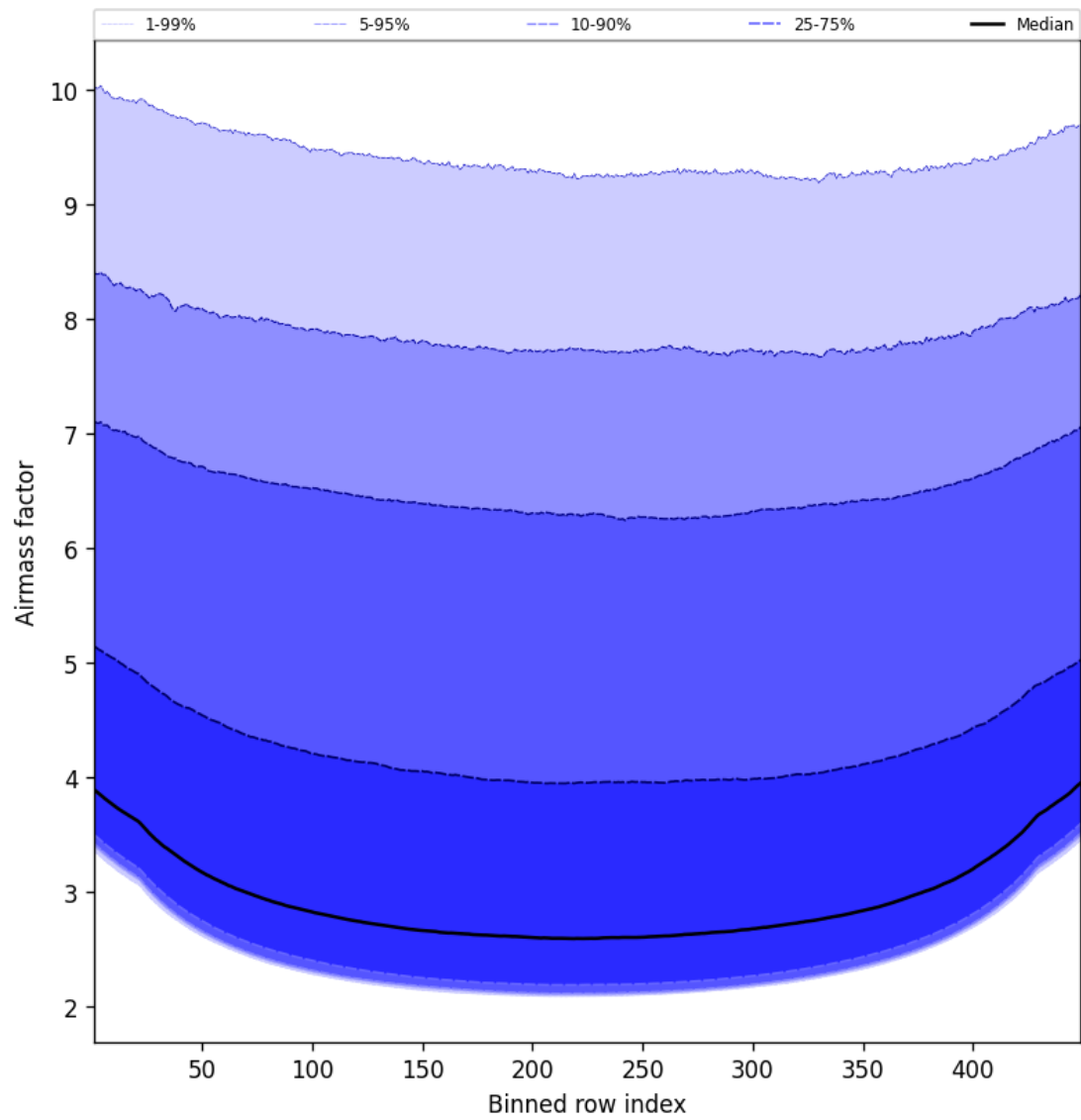
Figure 49: Along track statistics of “Airmass factor” for 2025-03-09 to 2025-03-10
