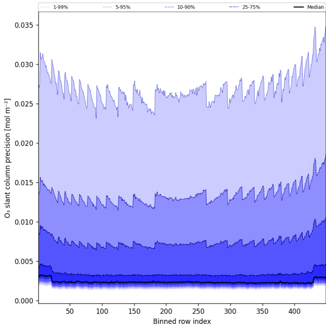
Figure 44: Along track statistics of “O 3 slant column precision” for 2025-03-09 to 2025-03-10
