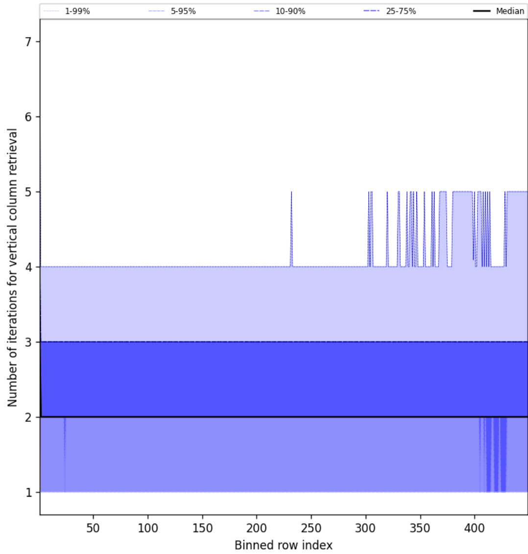
Figure 51: Along track statistics of “Number of iterations for vertical column retrieval” for 2025-03-09 to 2025-03-10
