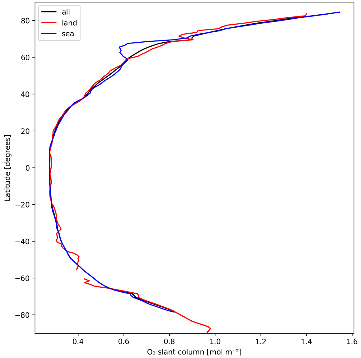
Figure 19: Zonal average of “O 3 slant column” for 2025-03-09 to 2025-03-10.
