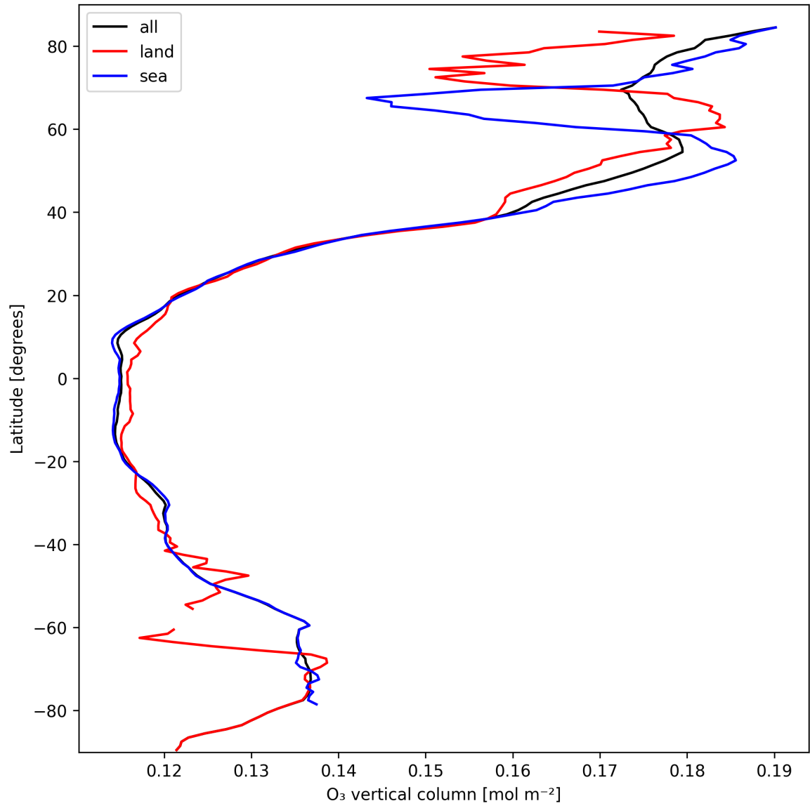
Figure 17: Zonal average of “O 3 vertical column” for 2025-03-09 to 2025-03-10.
