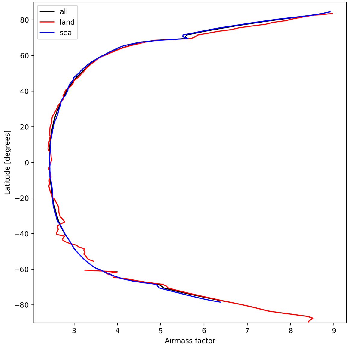
Figure 25: Zonal average of “Airmass factor” for 2025-03-09 to 2025-03-10.
