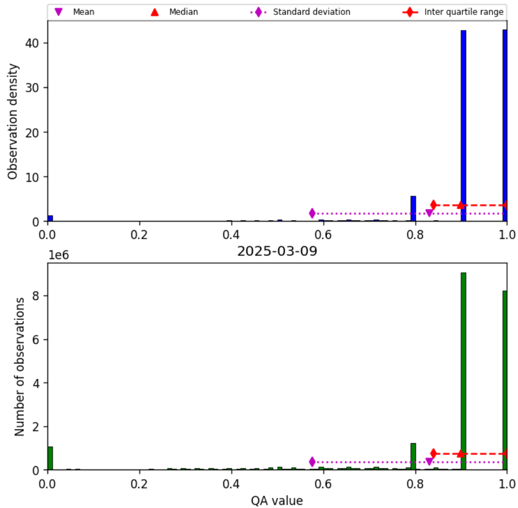
Figure 28: Histogram of “QA value” for 2025-03-09 to 2025-03-10
