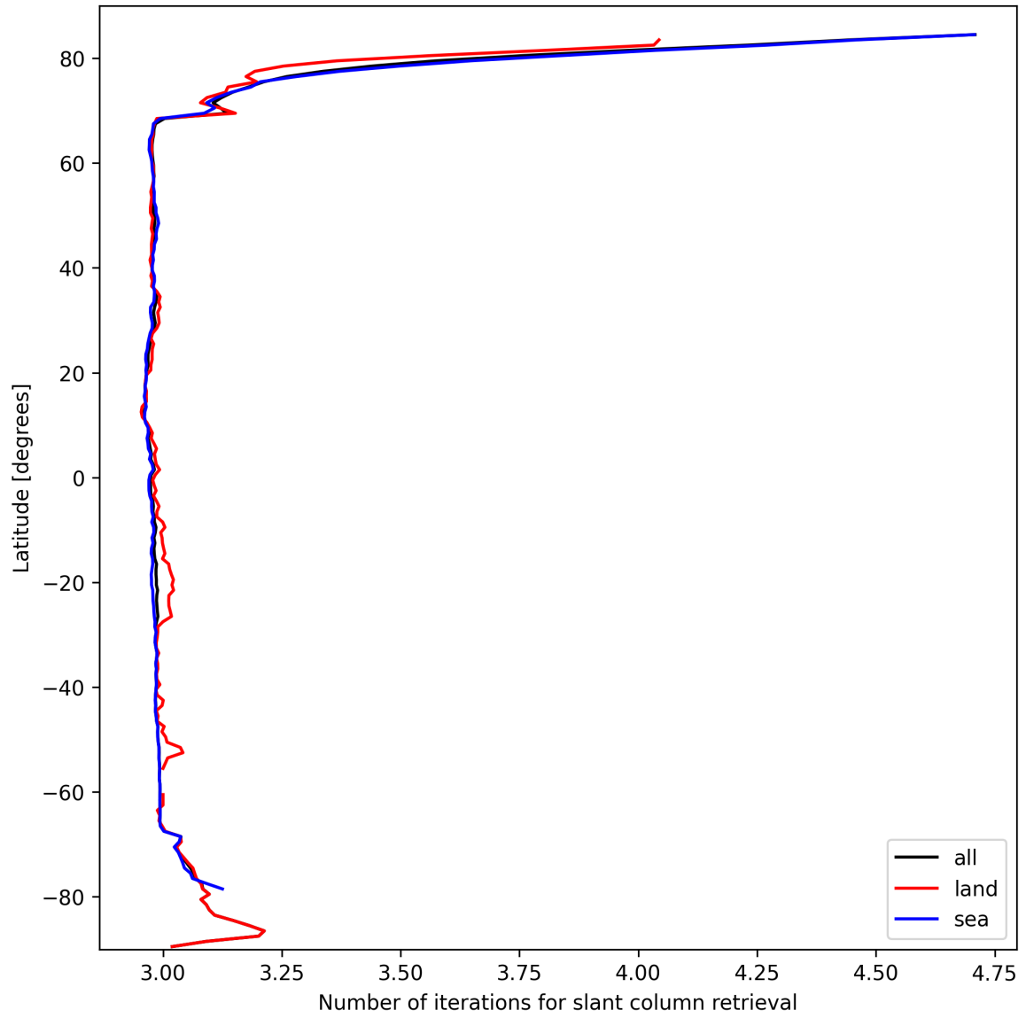
Figure 21: Zonal average of “Number of iterations for slant column retrieval” for 2025-03-09 to 2025-03-10.
