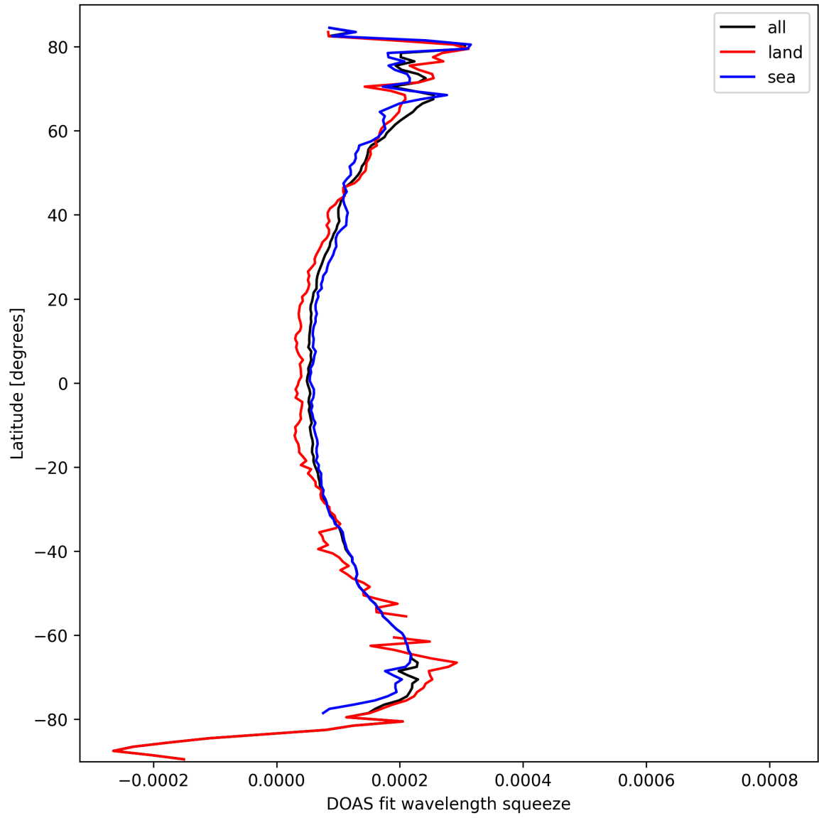
Figure 24: Zonal average of “DOAS fit wavelength squeeze” for 2025-03-09 to 2025-03-10.
