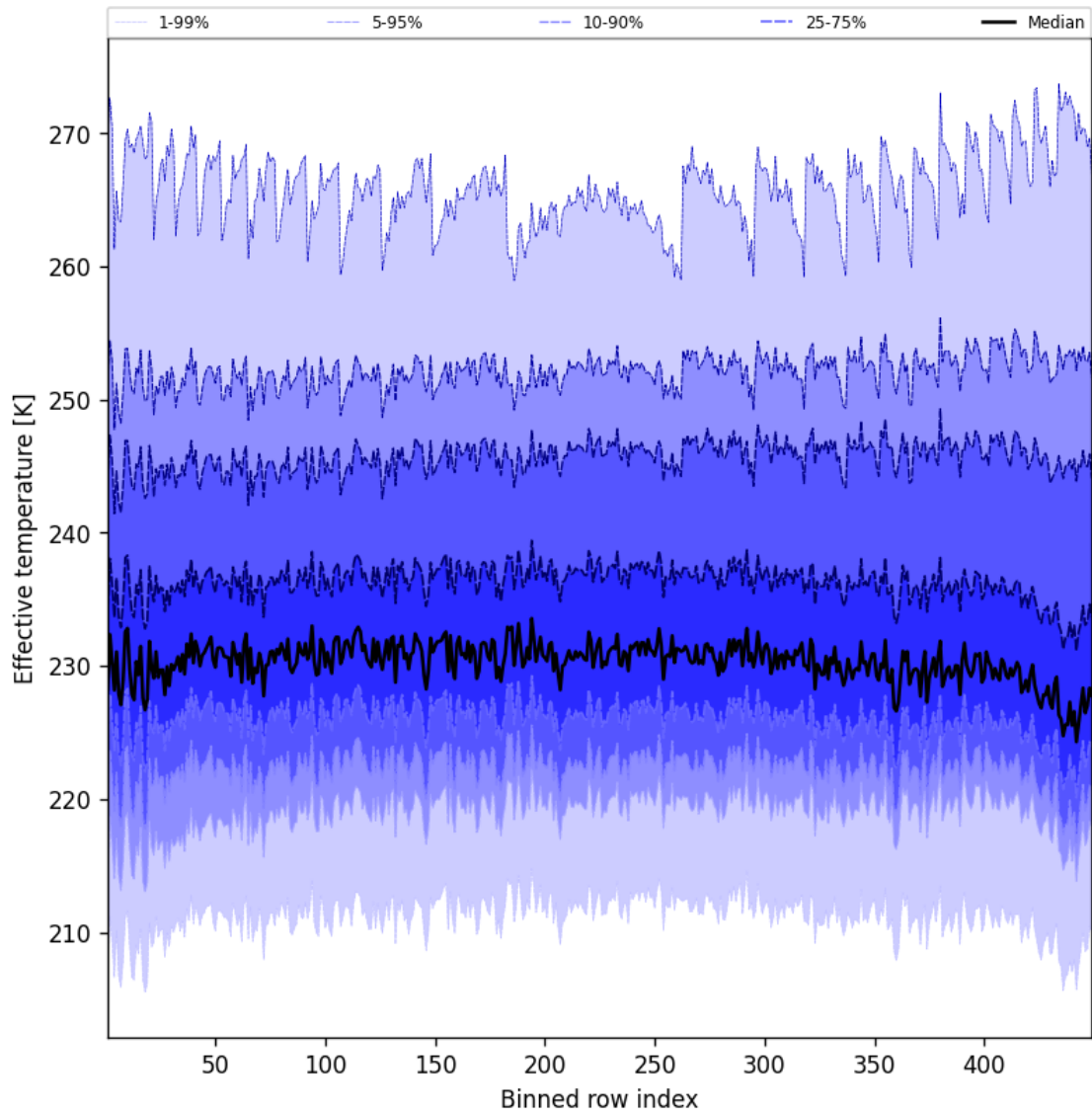
Figure 50: Along track statistics of “Effective temperature” for 2025-03-09 to 2025-03-10
