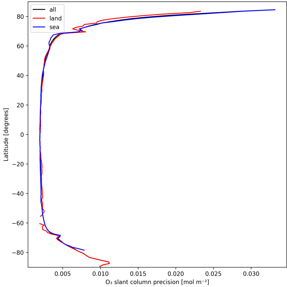
Figure 20: Zonal average of “O 3 slant column precision” for 2025-03-09 to 2025-03-10.
