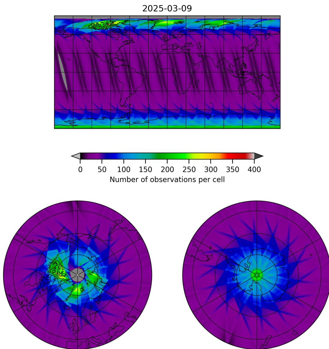
Figure 15: Map of the number of observations for 2025-03-09 to 2025-03-10
