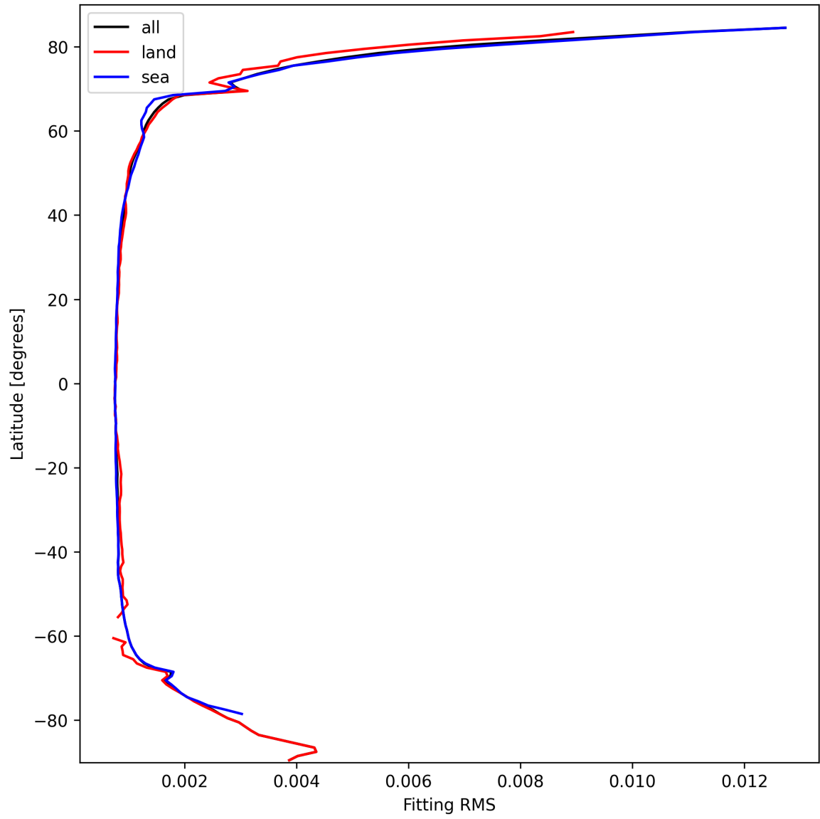
Figure 22: Zonal average of “Fitting RMS” for 2025-03-09 to 2025-03-10.
