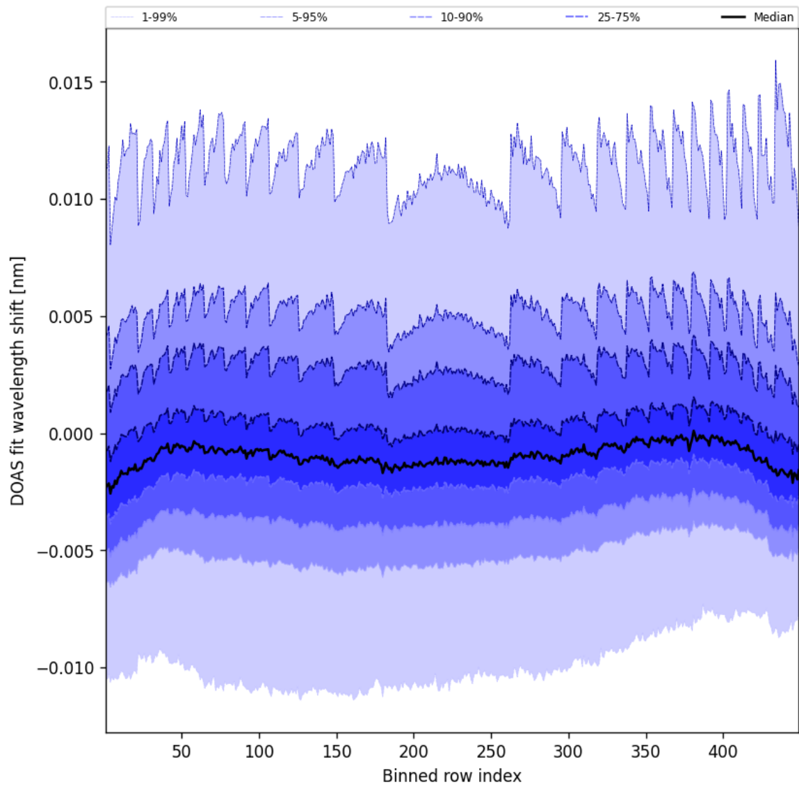
Figure 47: Along track statistics of “DOAS fit wavelength shift” for 2025-03-09 to 2025-03-10
