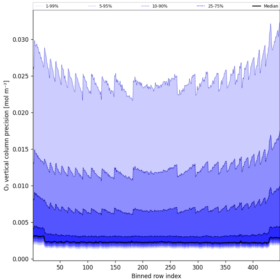
Figure 42: Along track statistics of “O 3 vertical column precision” for 2025-03-09 to 2025-03-10
