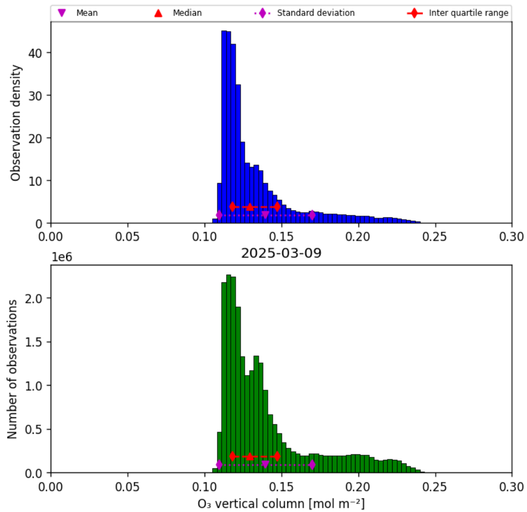
Figure 29: Histogram of “O 3 vertical column” for 2025-03-09 to 2025-03-10
