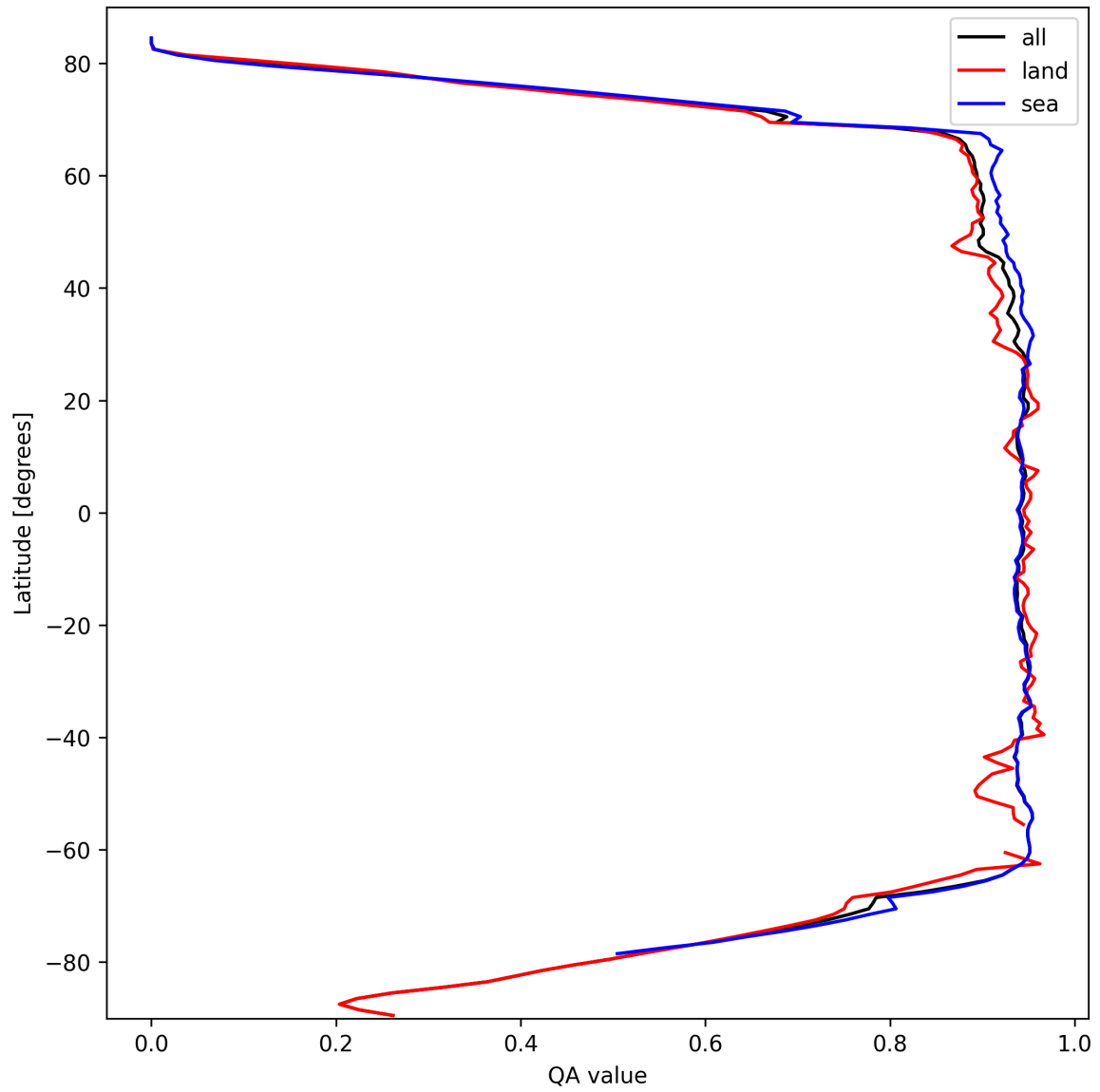
Figure 16: Zonal average of “QA value” for 2025-03-09 to 2025-03-10.
