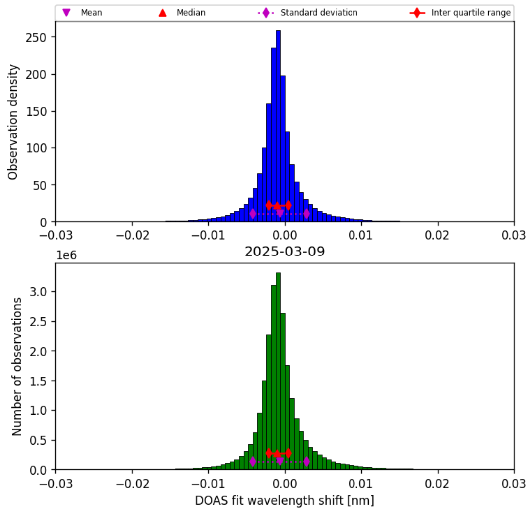
Figure 35: Histogram of “DOAS fit wavelength shift” for 2025-03-09 to 2025-03-10
