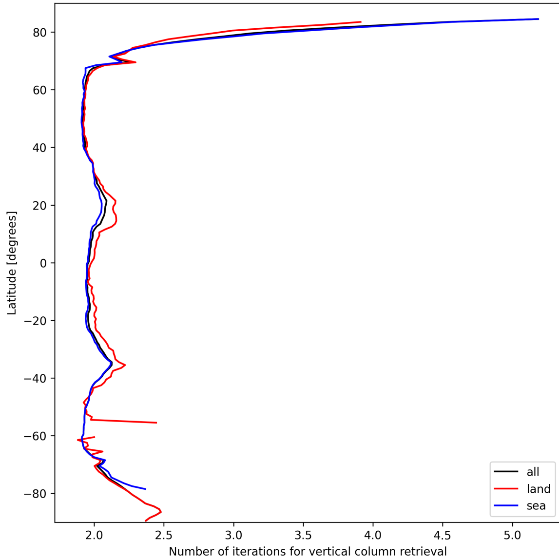
Figure 27: Zonal average of “Number of iterations for vertical column retrieval” for 2025-03-09 to 2025-03-10.
