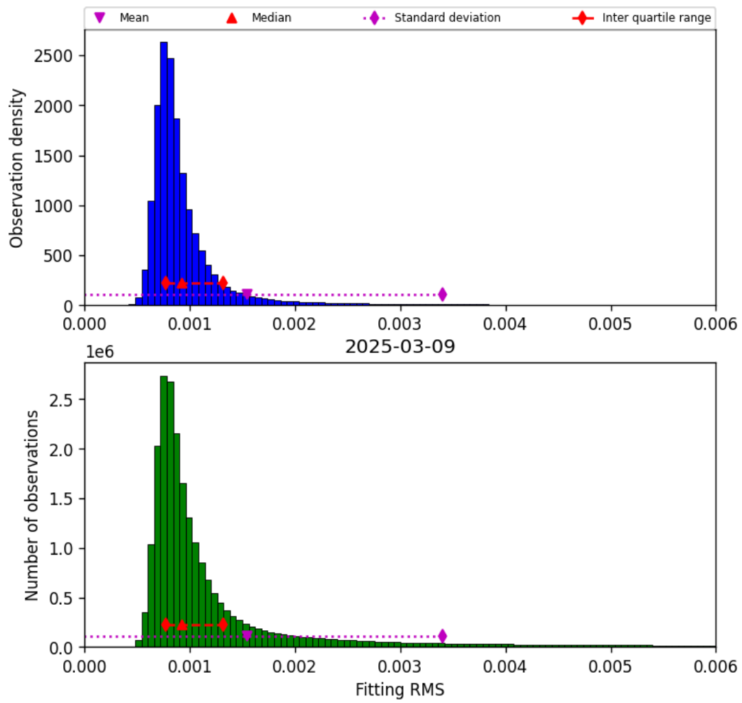
Figure 34: Histogram of “Fitting RMS” for 2025-03-09 to 2025-03-10
