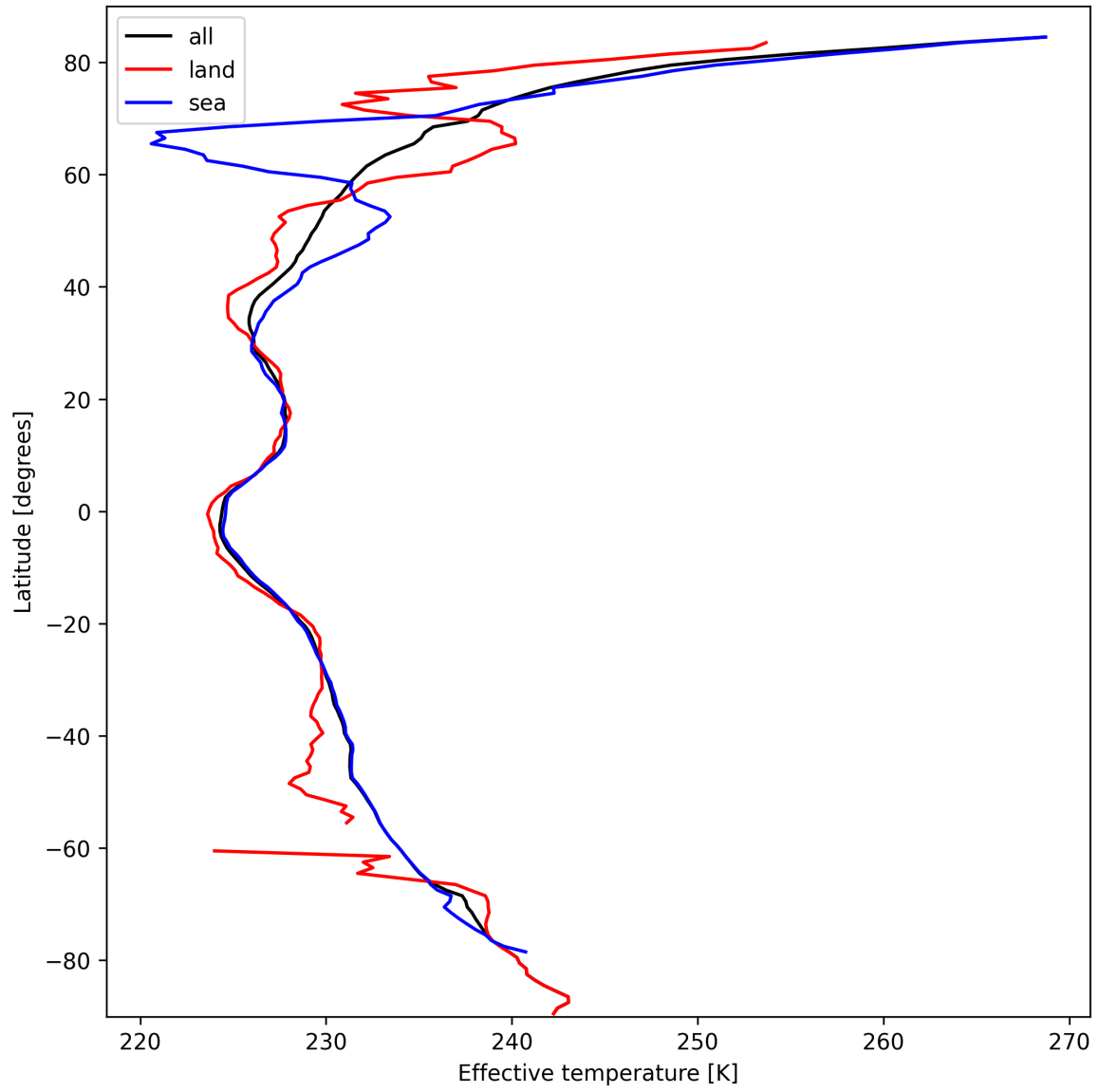
Figure 26: Zonal average of “Effective temperature” for 2025-03-09 to 2025-03-10.
