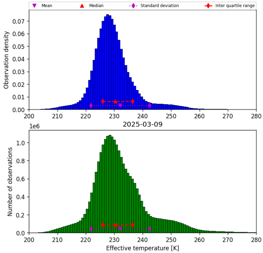
Figure 38: Histogram of “Effective temperature” for 2025-03-09 to 2025-03-10
