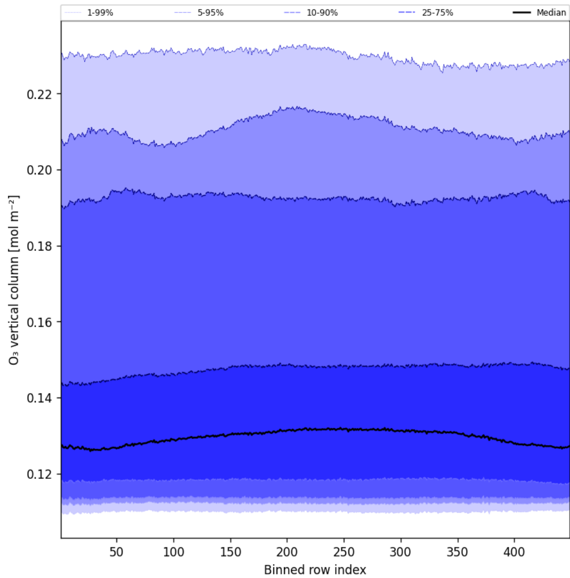
Figure 41: Along track statistics of “O 3 vertical column” for 2025-03-09 to 2025-03-10
