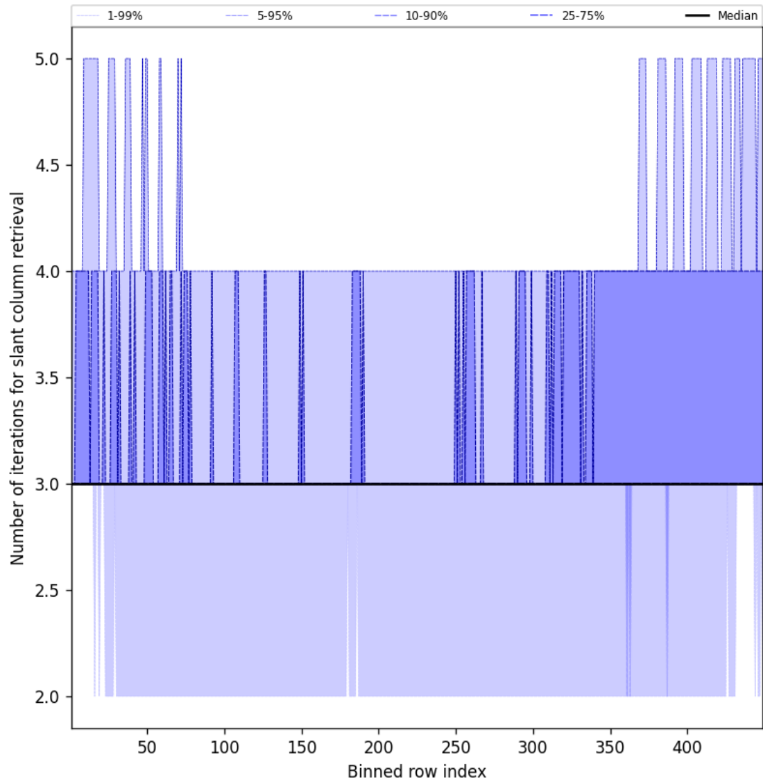
Figure 45: Along track statistics of “Number of iterations for slant column retrieval” for 2025-03-09 to 2025-03-10
