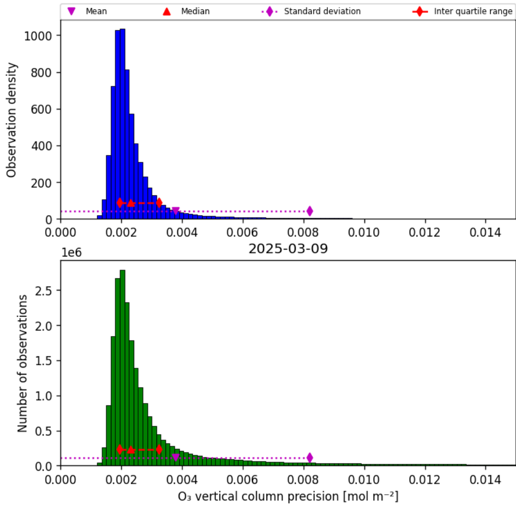
Figure 30: Histogram of “O 3 vertical column precision” for 2025-03-09 to 2025-03-10
