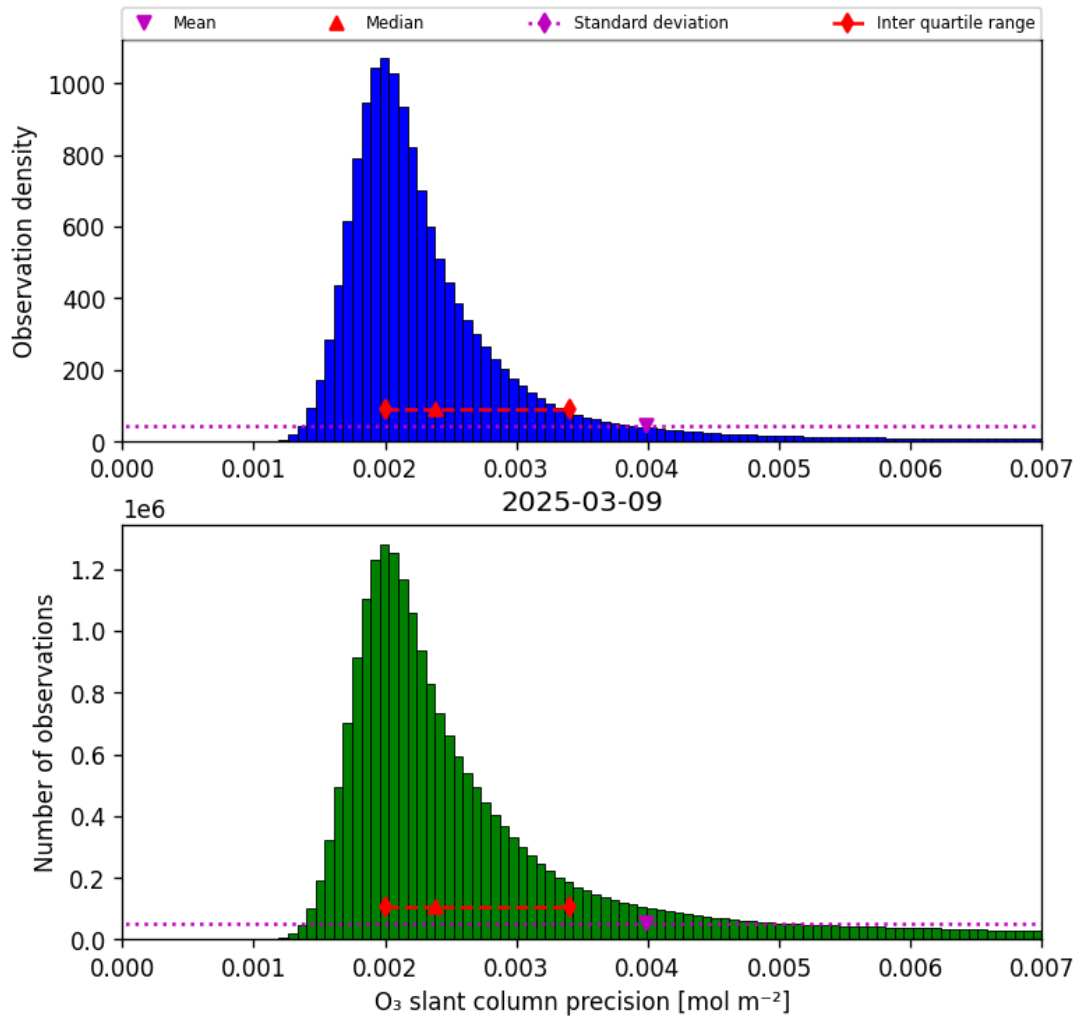
Figure 32: Histogram of “O 3 slant column precision” for 2025-03-09 to 2025-03-10
