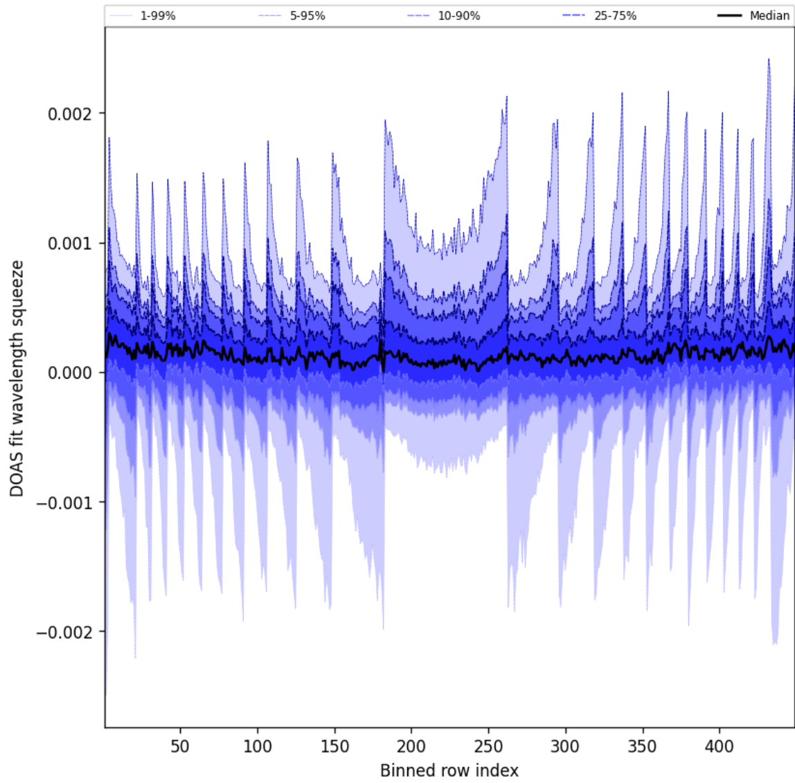
Figure 48: Along track statistics of “DOAS fit wavelength squeeze” for 2025-03-09 to 2025-03-10
