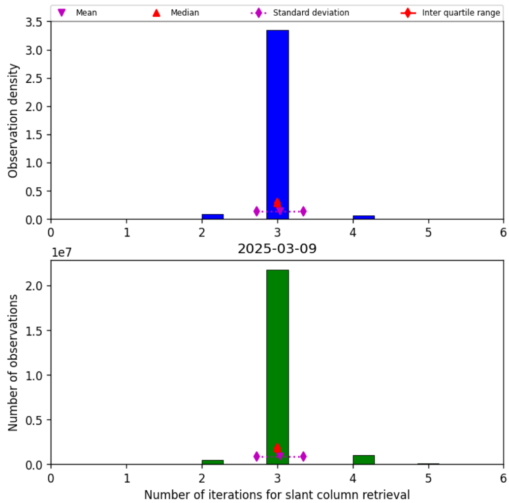
Figure 33: Histogram of “Number of iterations for slant column retrieval” for 2025-03-09 to 2025-03-10
