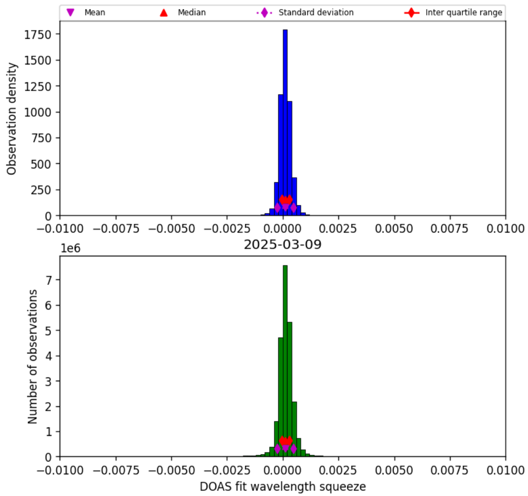
Figure 36: Histogram of “DOAS fit wavelength squeeze” for 2025-03-09 to 2025-03-10
