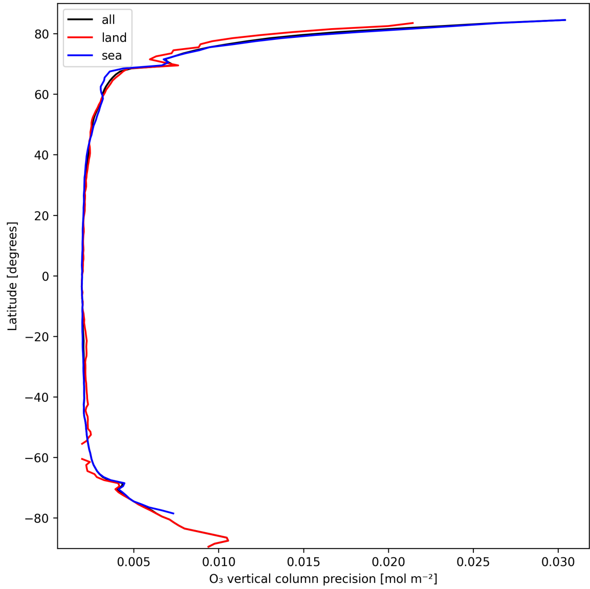
Figure 18: Zonal average of “O 3 vertical column precision” for 2025-03-09 to 2025-03-10.
