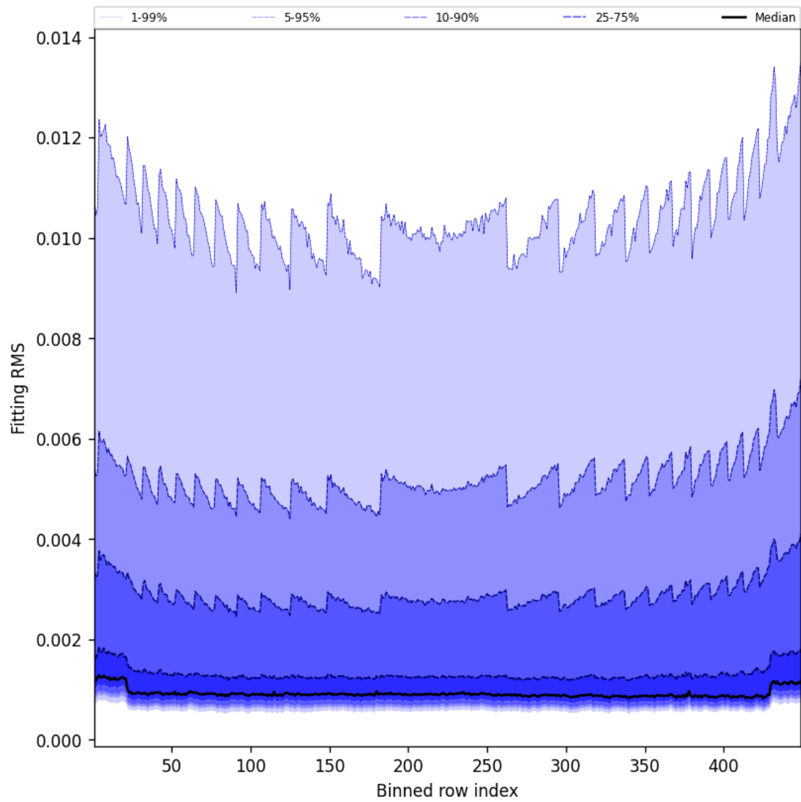
Figure 46: Along track statistics of “Fitting RMS” for 2025-03-09 to 2025-03-10
