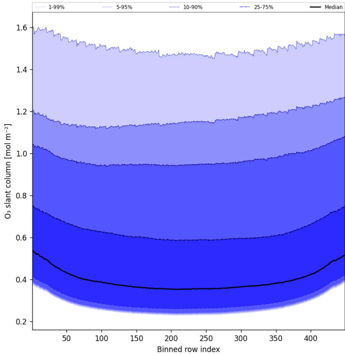
Figure 43: Along track statistics of “O 3 slant column” for 2025-03-09 to 2025-03-10
