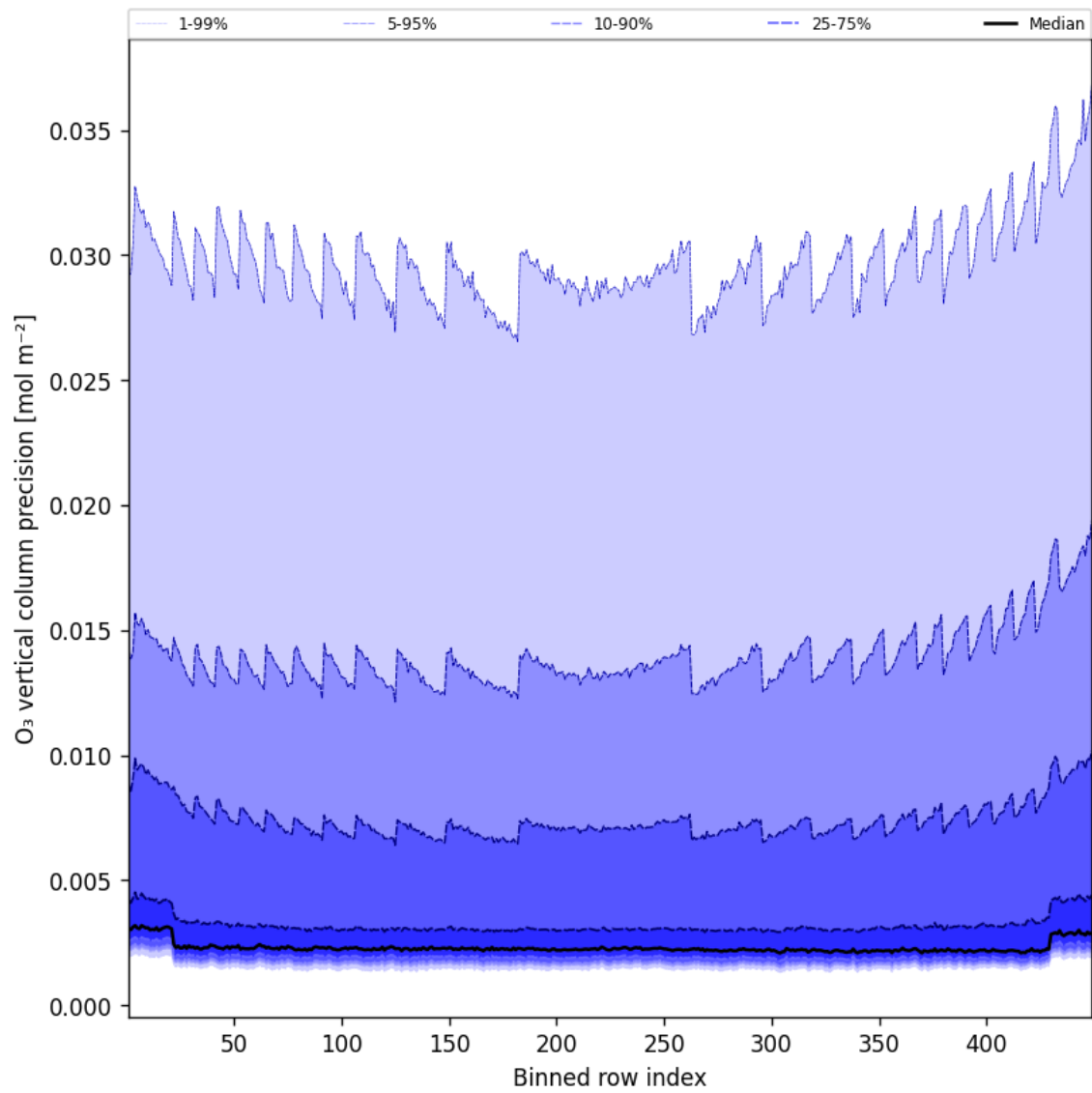
Figure 42: Along track statistics of “O 3 vertical column precision” for 2025-03-10 to 2025-03-10
