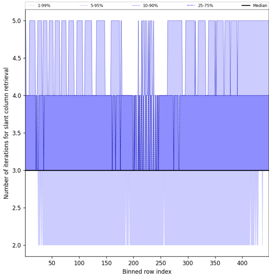
Figure 45: Along track statistics of “Number of iterations for slant column retrieval” for 2025-03-10 to 2025-03-10
