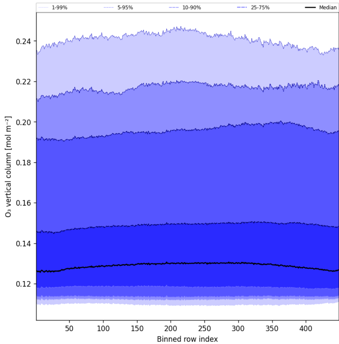
Figure 41: Along track statistics of “ O_3 vertical column” for 2025-03-10 to 2025-03-10
