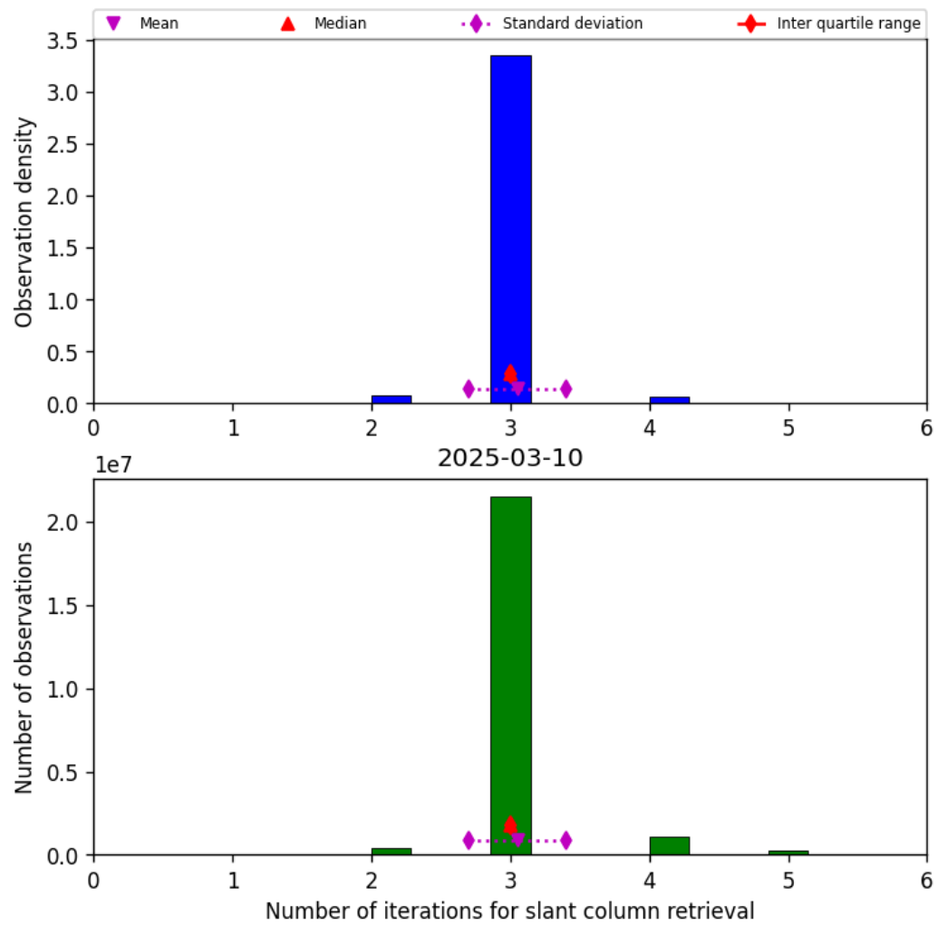
Figure 33: Histogram of “Number of iterations for slant column retrieval” for 2025-03-10 to 2025-03-10
