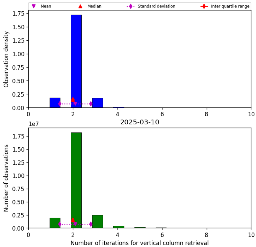
Figure 39: Histogram of “Number of iterations for vertical column retrieval” for 2025-03-10 to 2025-03-10
