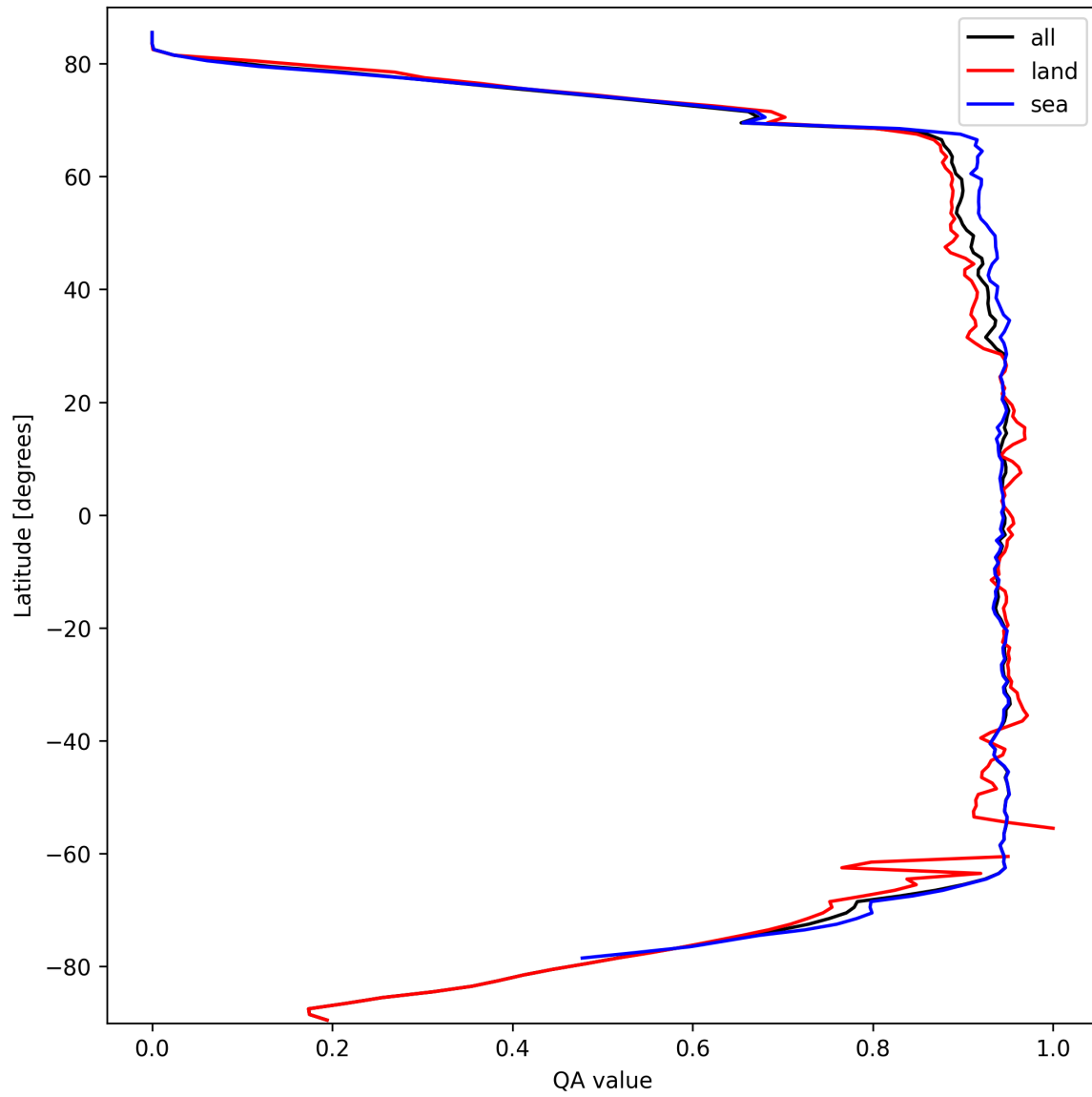
Figure 16: Zonal average of “QA value” for 2025-03-10 to 2025-03-10.
