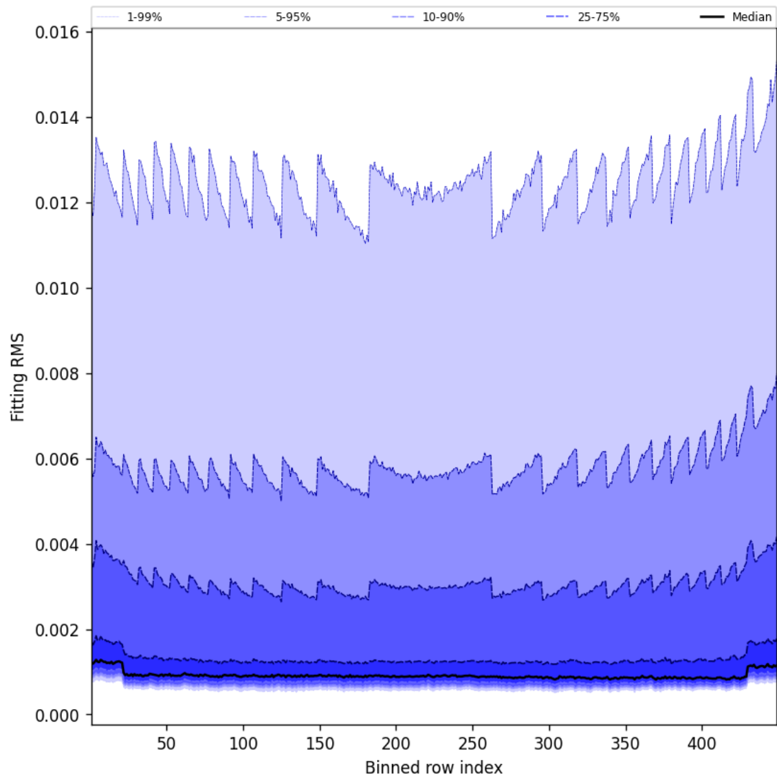
Figure 46: Along track statistics of “Fitting RMS” for 2025-03-10 to 2025-03-10
