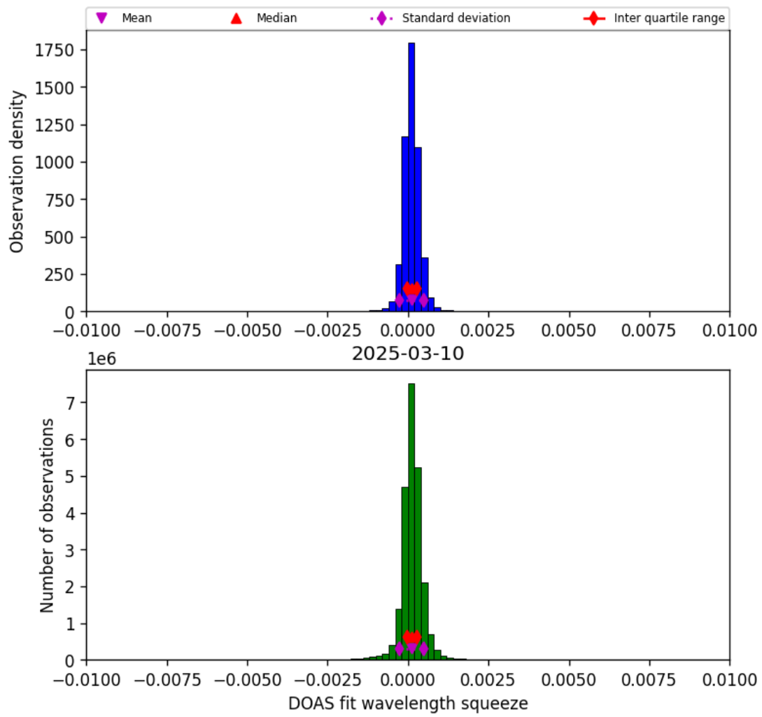
Figure 36: Histogram of “DOAS fit wavelength squeeze” for 2025-03-10 to 2025-03-10
