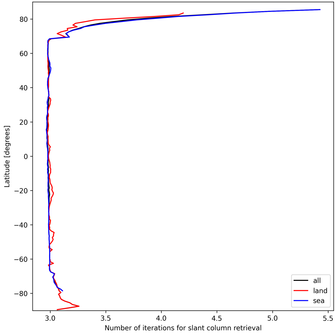
Figure 21: Zonal average of “Number of iterations for slant column retrieval” for 2025-03-10 to 2025-03-10.
