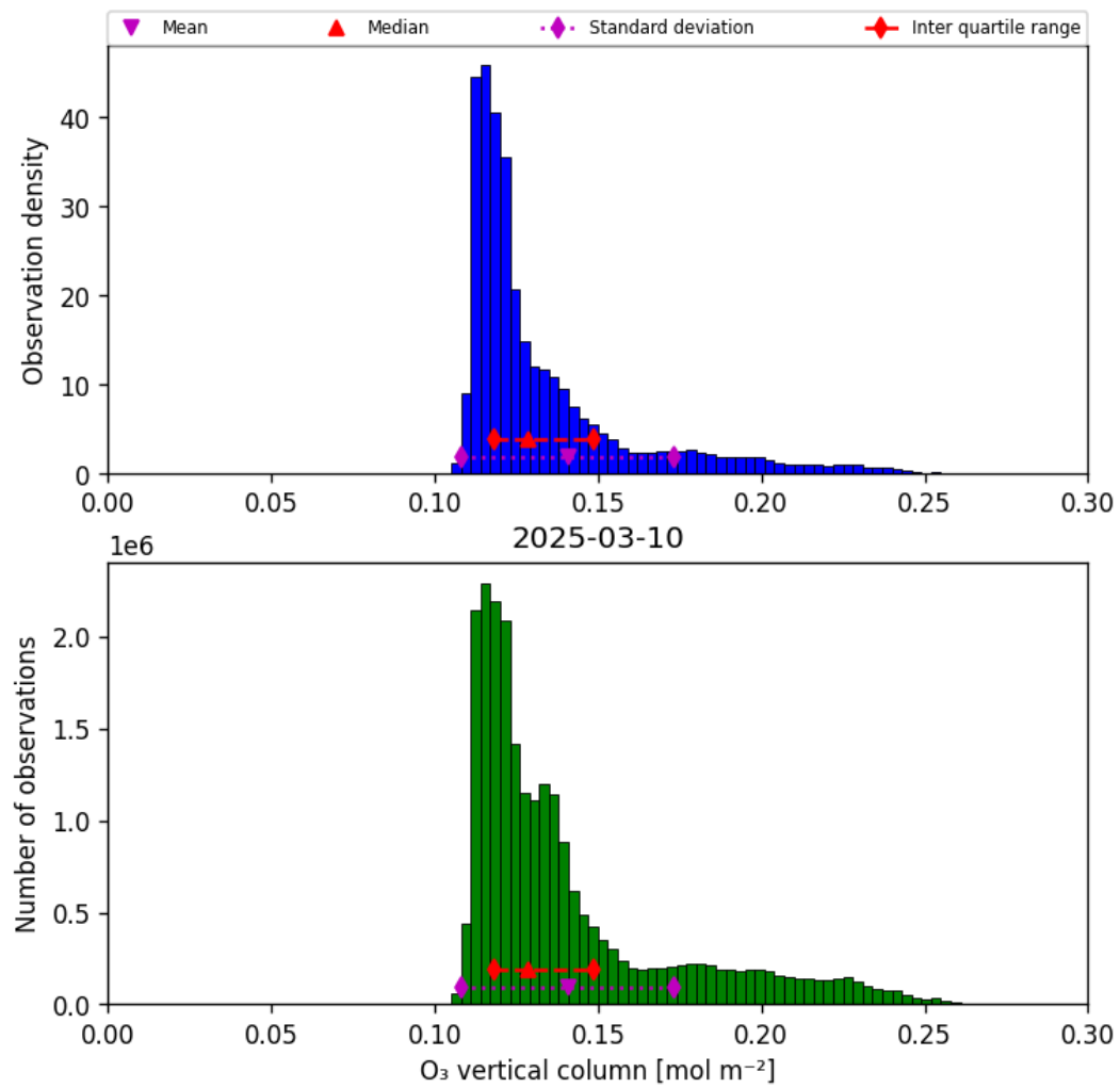
Figure 29: Histogram of “O 3 vertical column” for 2025-03-10 to 2025-03-10
