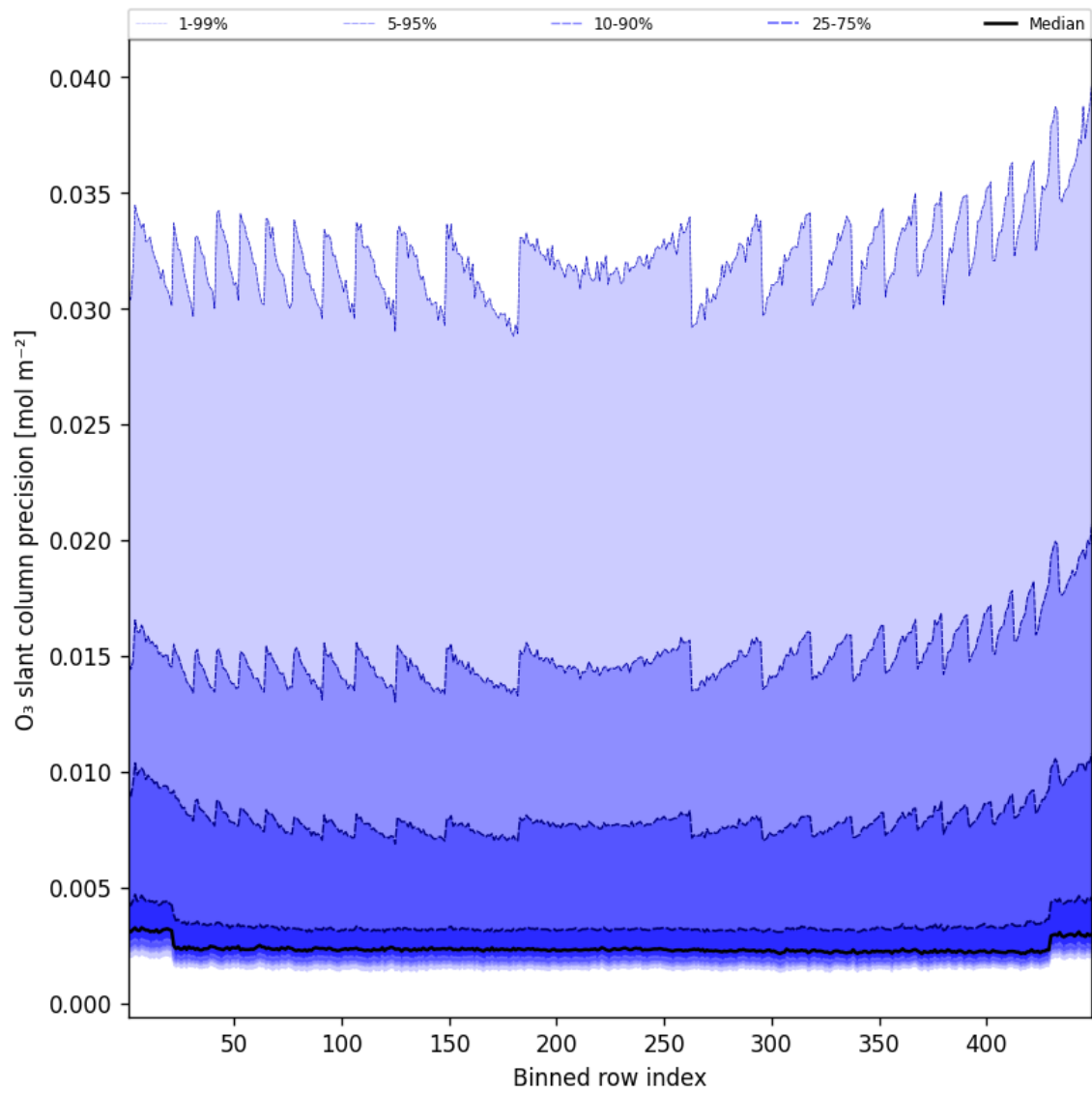
Figure 44: Along track statistics of “O 3 slant column precision” for 2025-03-10 to 2025-03-10
