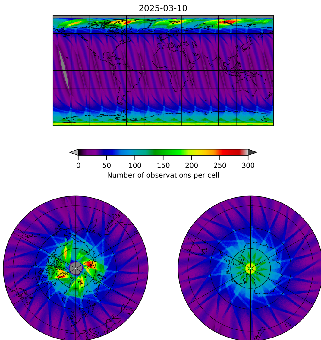
Figure 15: Map of the number of observations for 2025-03-10 to 2025-03-10
