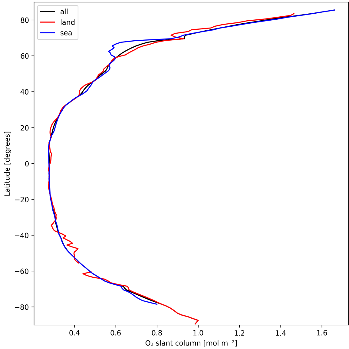
Figure 19: Zonal average of “O 3 slant column” for 2025-03-10 to 2025-03-10.
