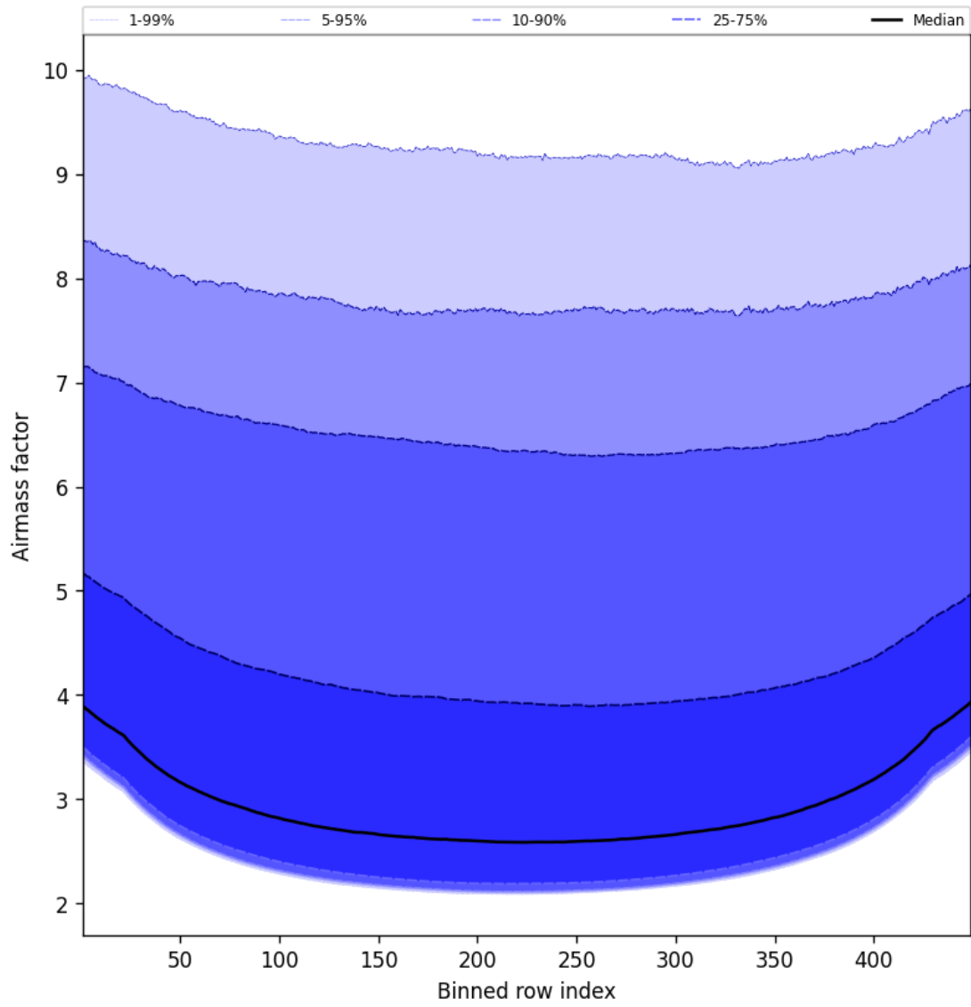
Figure 49: Along track statistics of “Airmass factor” for 2025-03-10 to 2025-03-10
