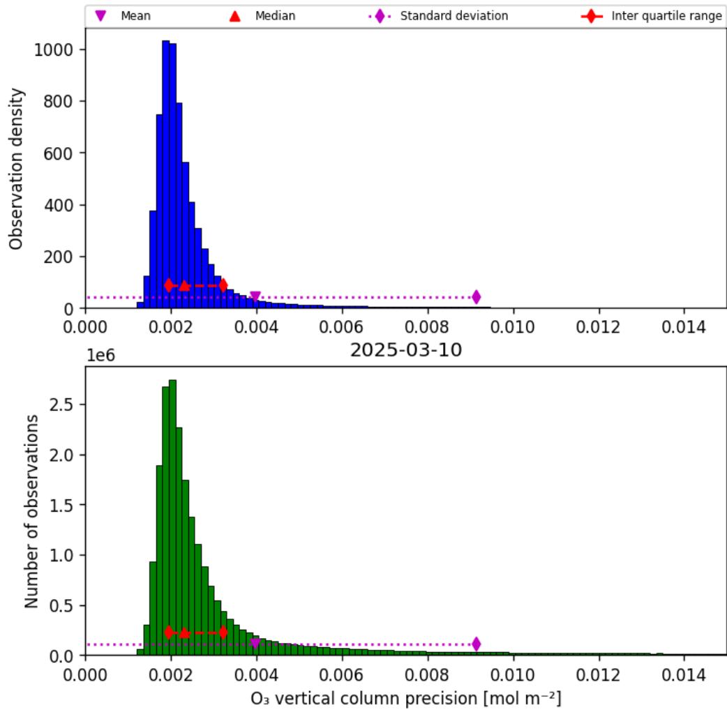
Figure 30: Histogram of “O 3 vertical column precision” for 2025-03-10 to 2025-03-10
