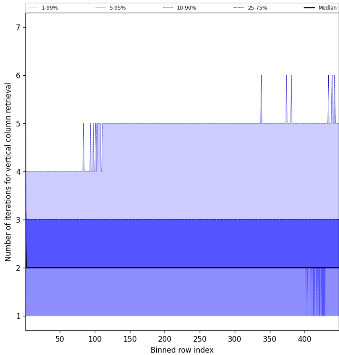
Figure 51: Along track statistics of “Number of iterations for vertical column retrieval” for 2025-03-10 to 2025-03-10
