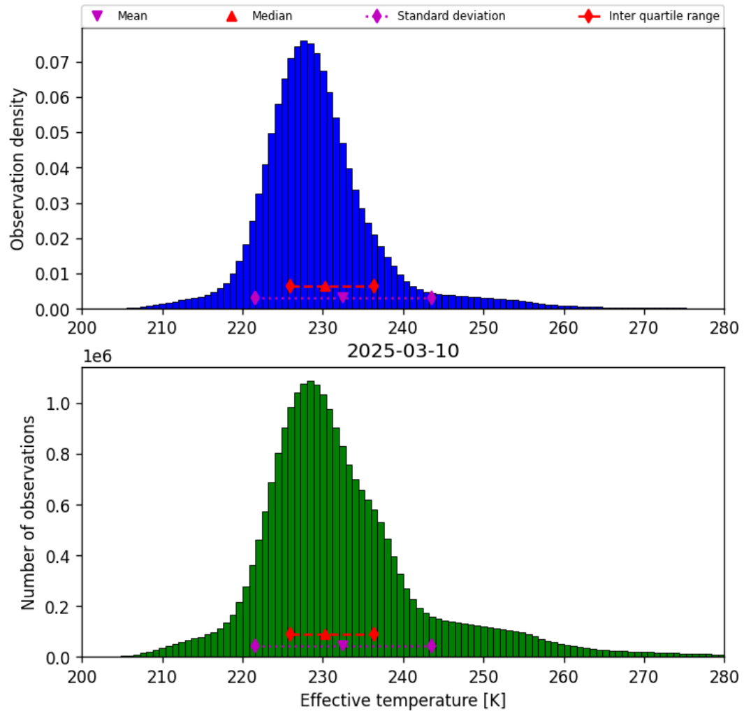
Figure 38: Histogram of “Effective temperature” for 2025-03-10 to 2025-03-10
