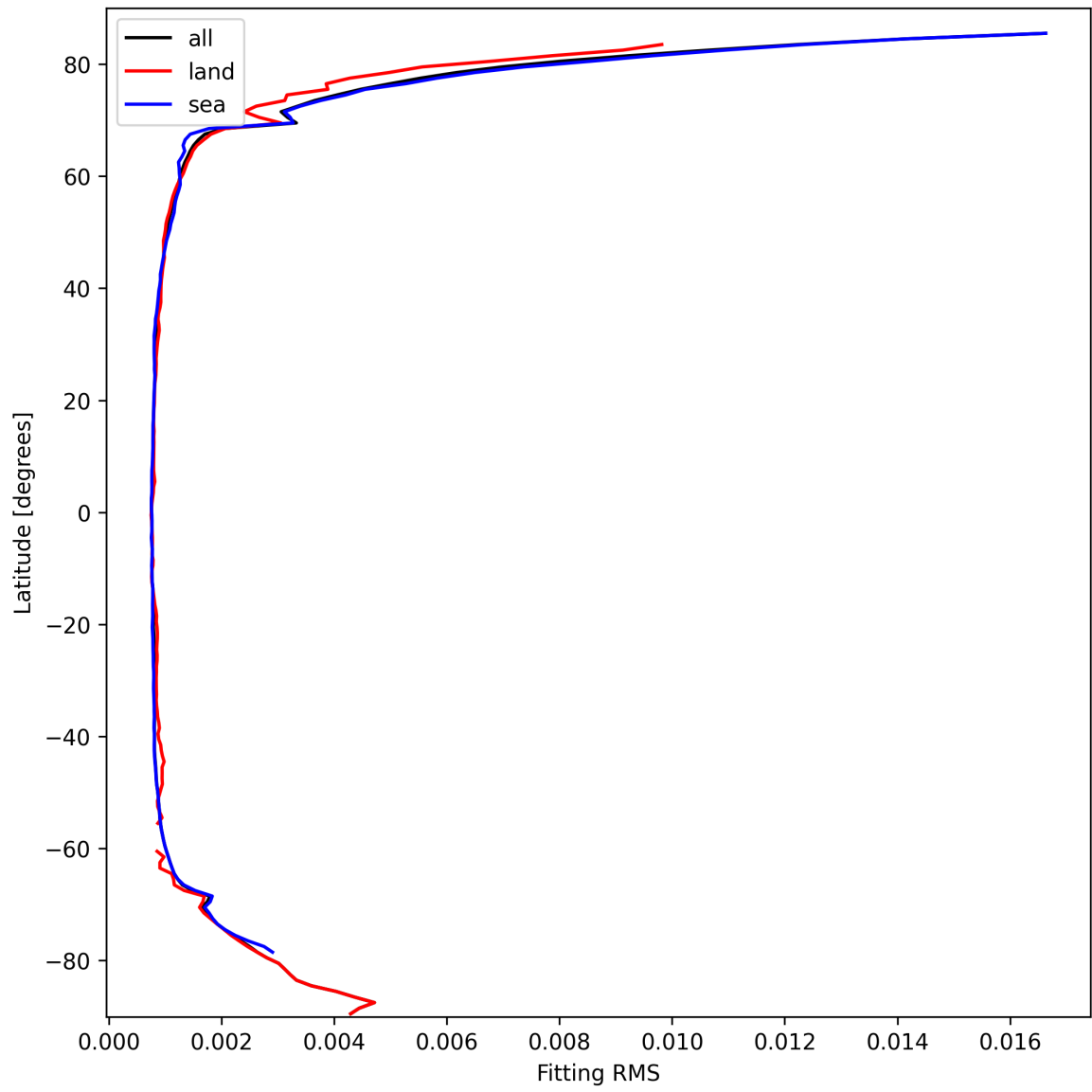
Figure 22: Zonal average of “Fitting RMS” for 2025-03-10 to 2025-03-10.
