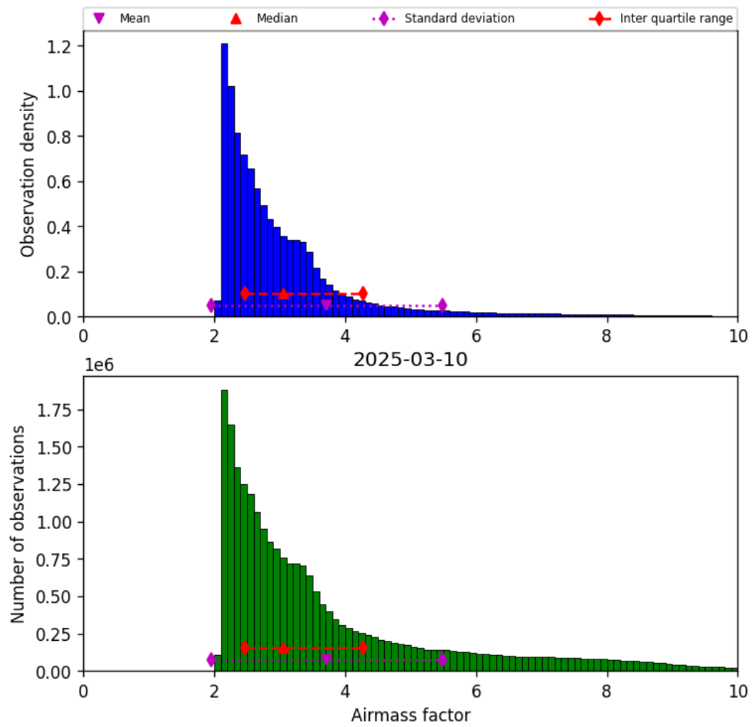
Figure 37: Histogram of “Airmass factor” for 2025-03-10 to 2025-03-10
