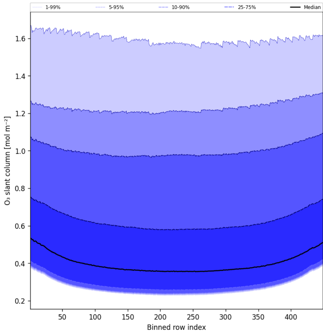
Figure 43: Along track statistics of “O 3 slant column” for 2025-03-10 to 2025-03-10
