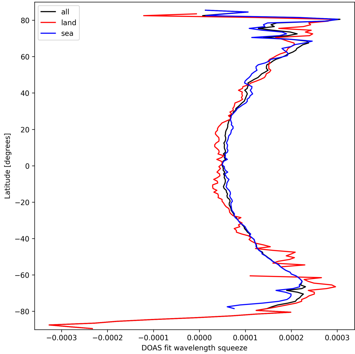
Figure 24: Zonal average of “DOAS fit wavelength squeeze” for 2025-03-10 to 2025-03-10.
