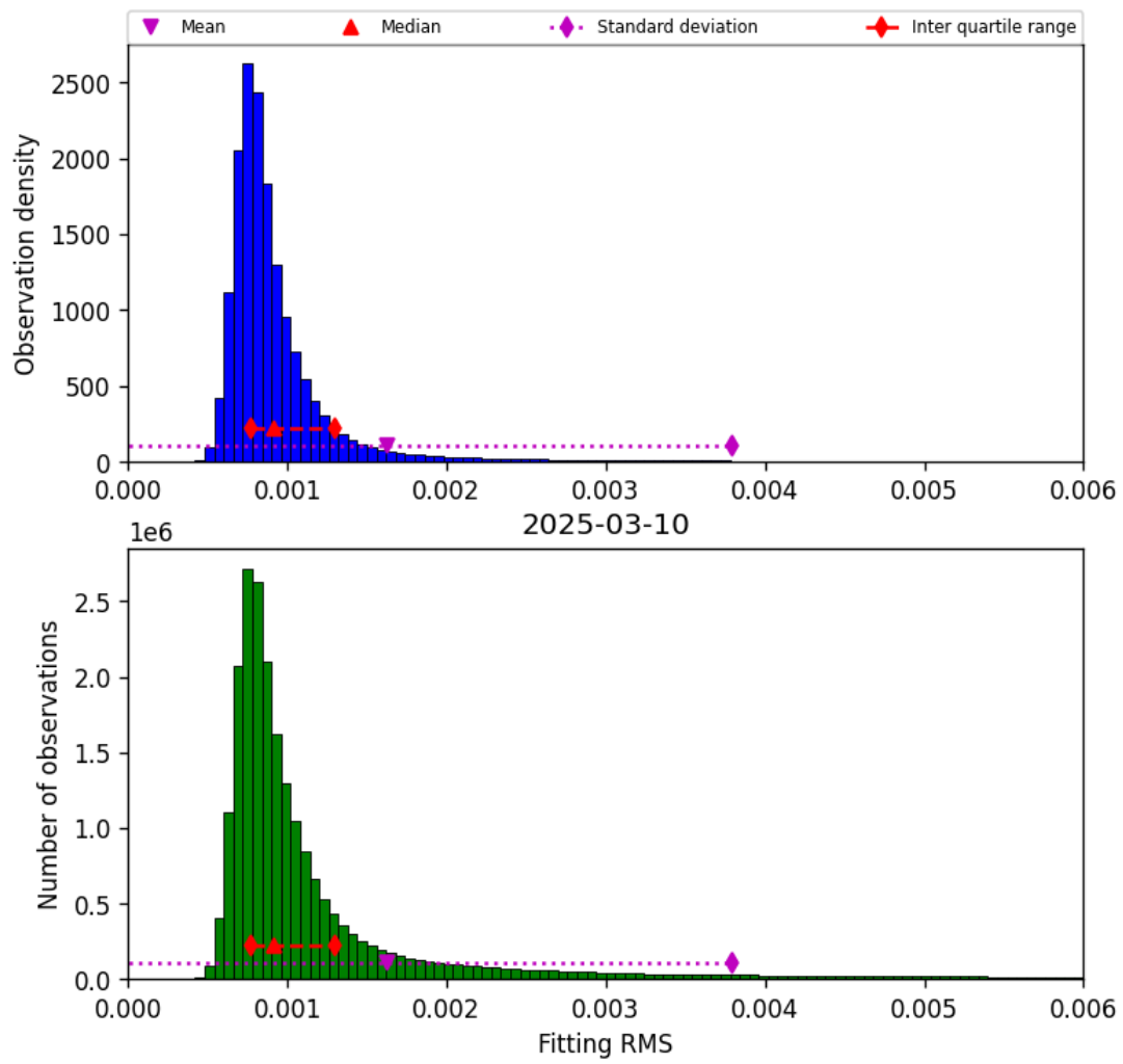
Figure 34: Histogram of “Fitting RMS” for 2025-03-10 to 2025-03-10
