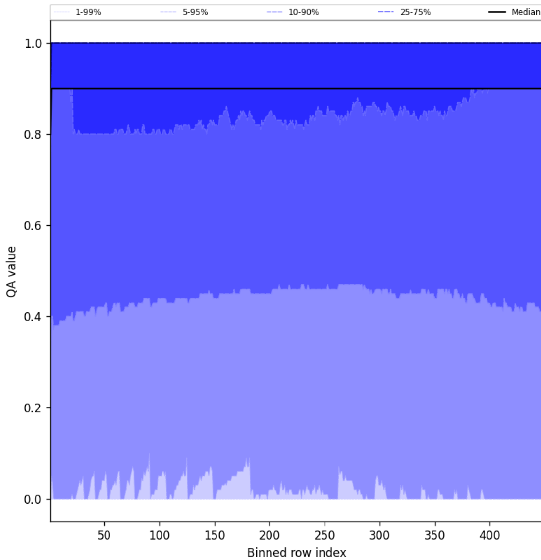
Figure 40: Along track statistics of “QA value” for 2025-03-10 to 2025-03-10
