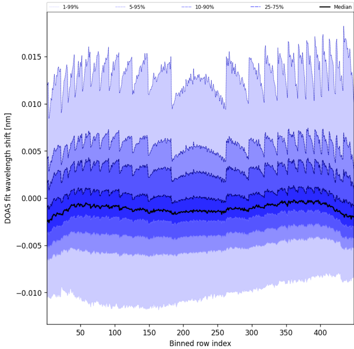
Figure 47: Along track statistics of “DOAS fit wavelength shift” for 2025-03-10 to 2025-03-10
