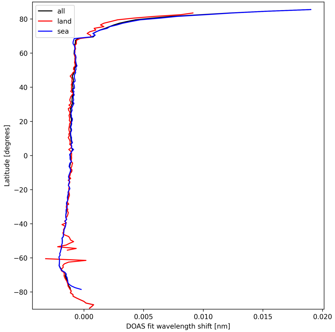
Figure 23: Zonal average of “DOAS fit wavelength shift” for 2025-03-10 to 2025-03-10.
