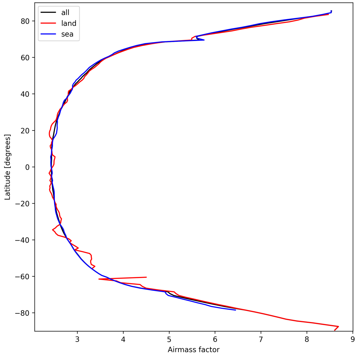
Figure 25: Zonal average of “Airmass factor” for 2025-03-10 to 2025-03-10.
