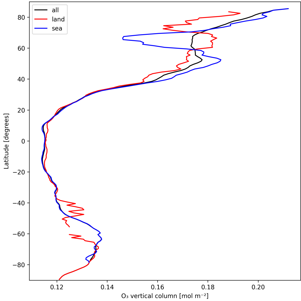
Figure 17: Zonal average of “O 3 vertical column” for 2025-03-10 to 2025-03-10.
