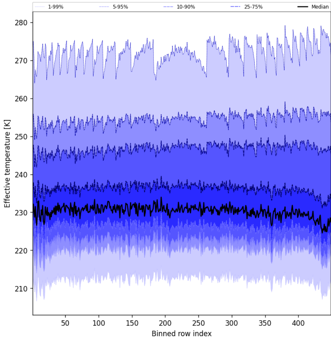
Figure 50: Along track statistics of “Effective temperature” for 2025-03-10 to 2025-03-10
