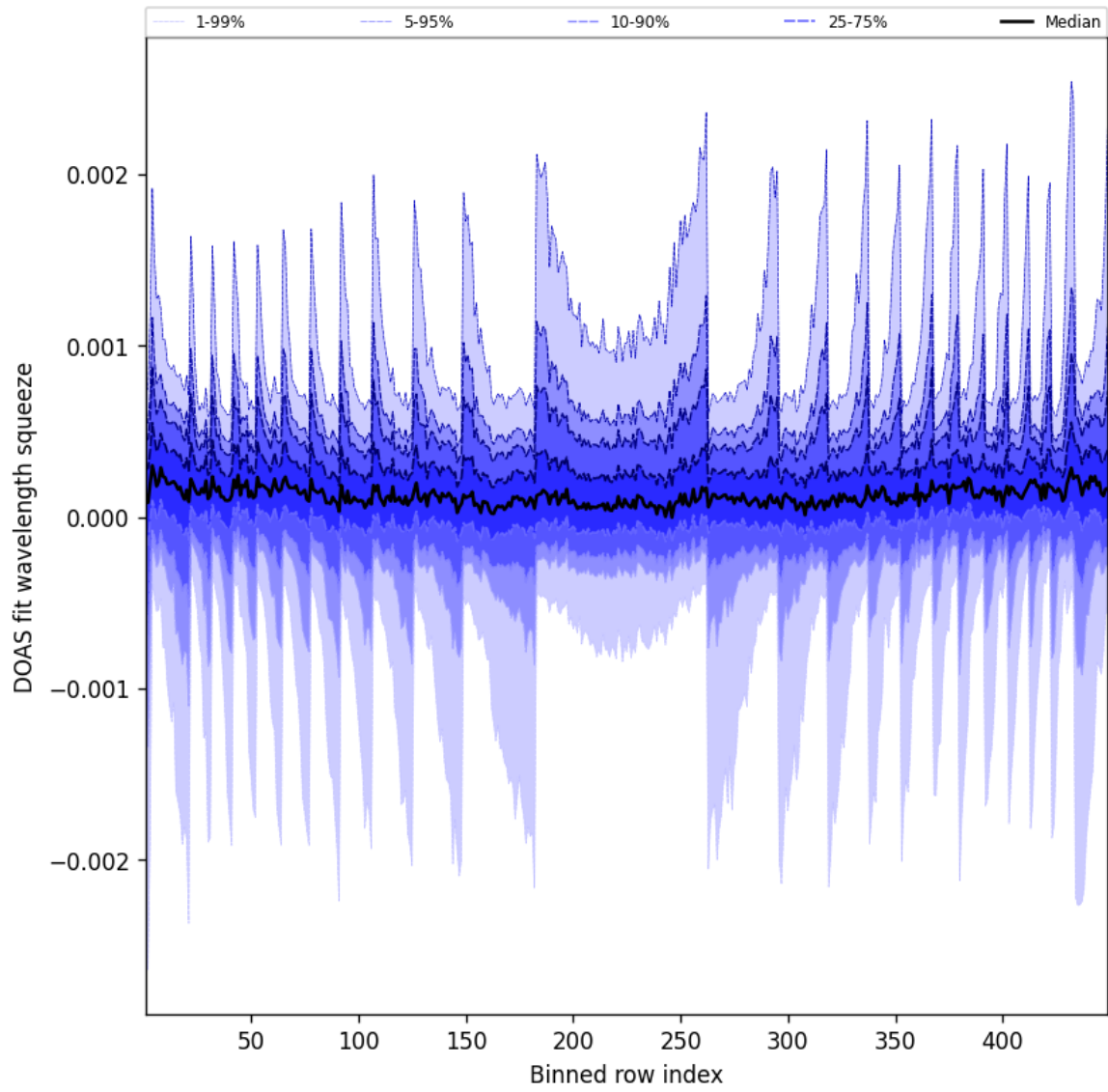
Figure 48: Along track statistics of “DOAS fit wavelength squeeze” for 2025-03-10 to 2025-03-10
