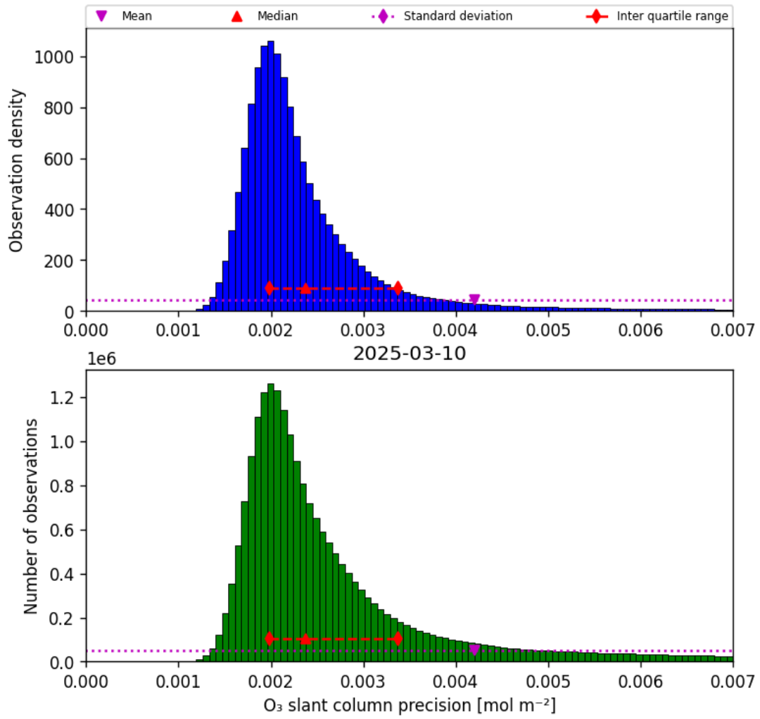
Figure 32: Histogram of “O 3 slant column precision” for 2025-03-10 to 2025-03-10
