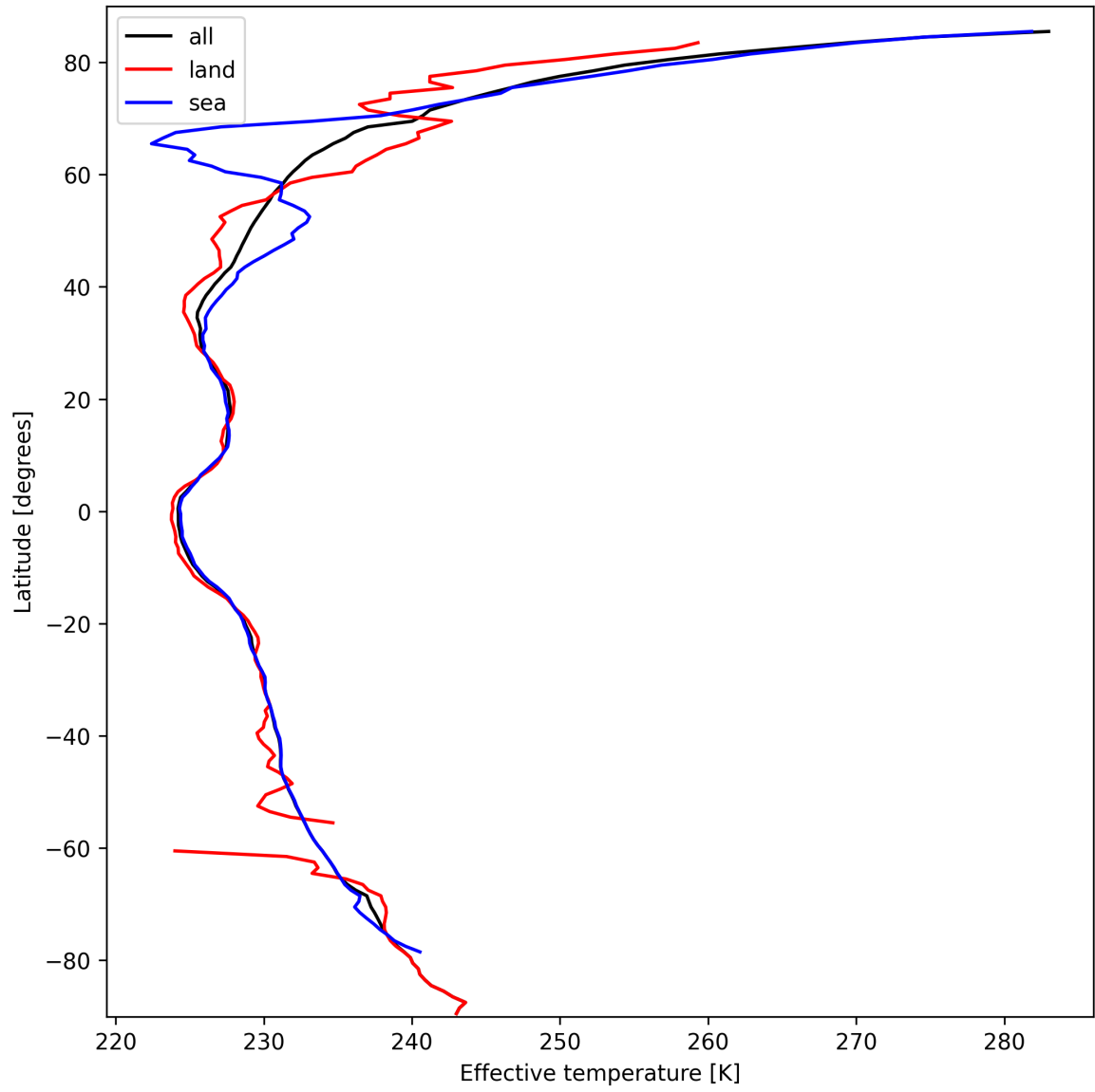
Figure 26: Zonal average of "Effective temperature" for 2025-03-10 to 2025-03-10.
