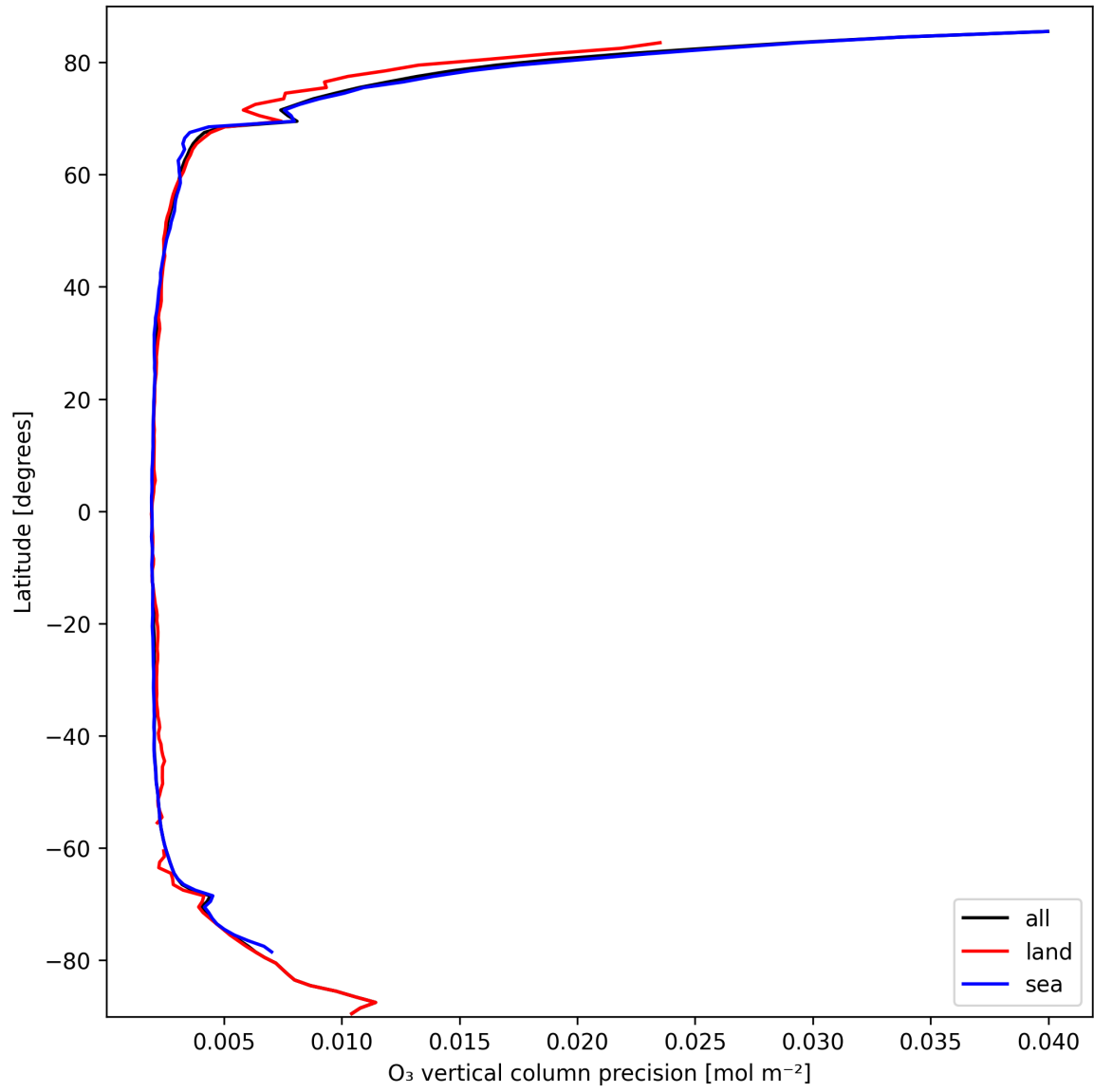
Figure 18: Zonal average of “O 3 vertical column precision” for 2025-03-10 to 2025-03-10.
