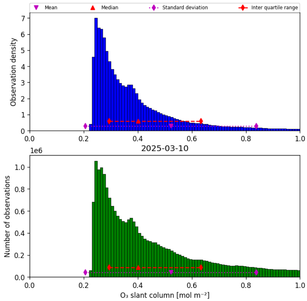
Figure 31: Histogram of "O 3 slant column" for 2025-03-10 to 2025-03-10
