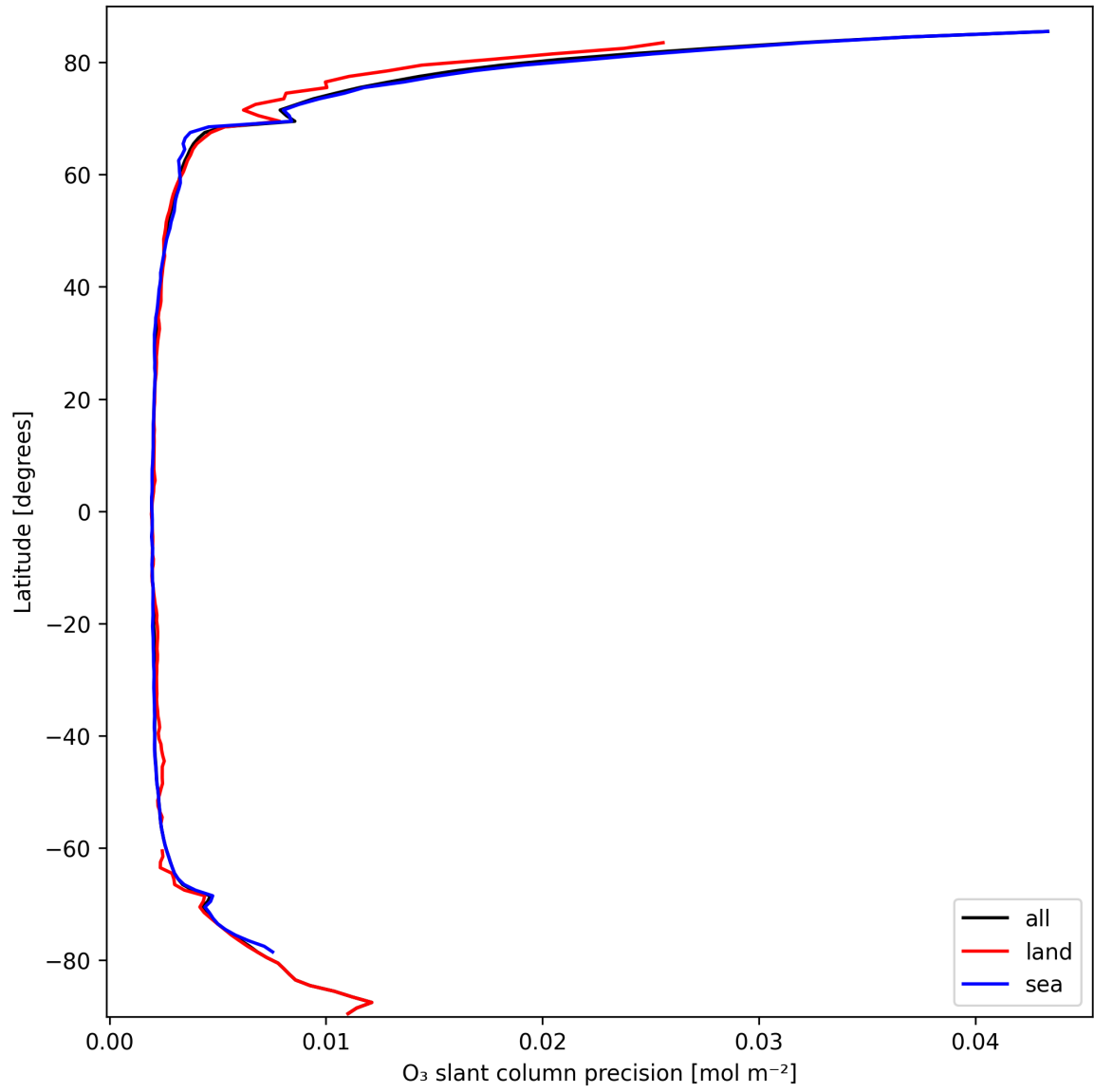
Figure 20: Zonal average of “O 3 slant column precision” for 2025-03-10 to 2025-03-10.
