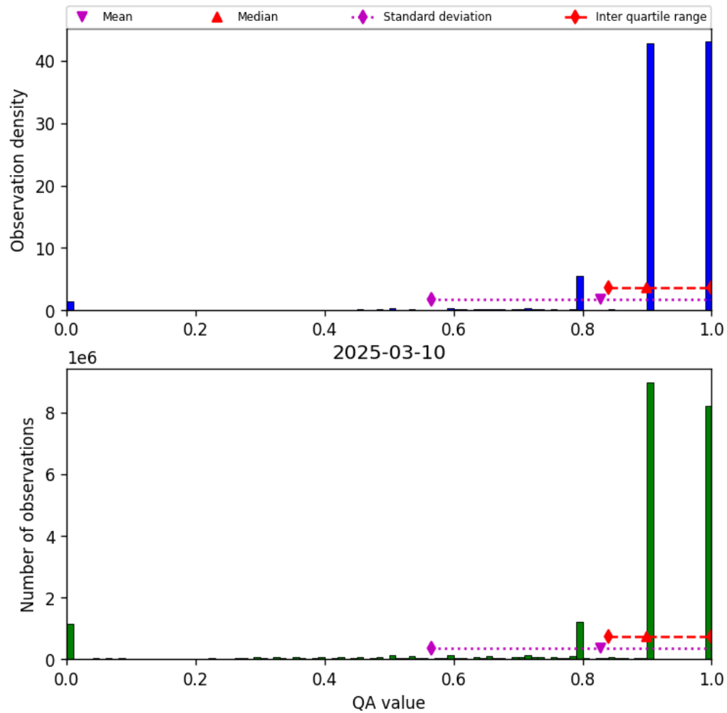
Figure 28: Histogram of “QA value” for 2025-03-10 to 2025-03-10
