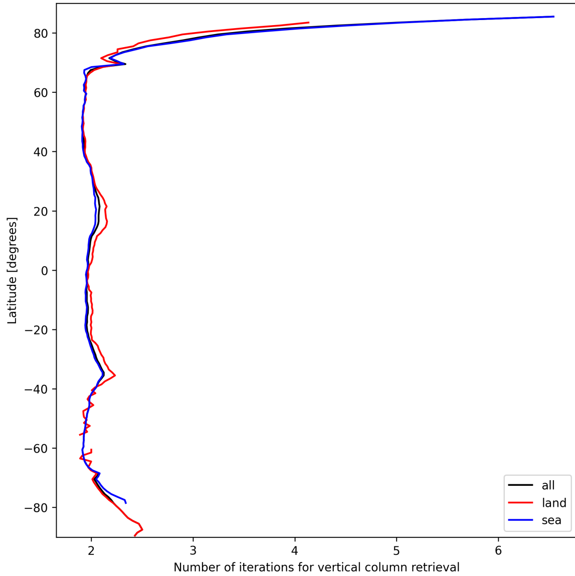
Figure 27: Zonal average of “Number of iterations for vertical column retrieval” for 2025-03-10 to 2025-03-10.
