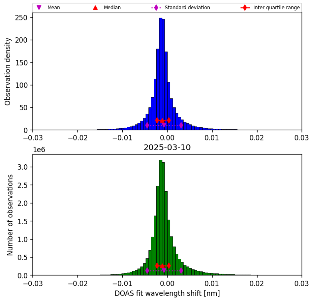
Figure 35: Histogram of “DOAS fit wavelength shift” for 2025-03-10 to 2025-03-10
