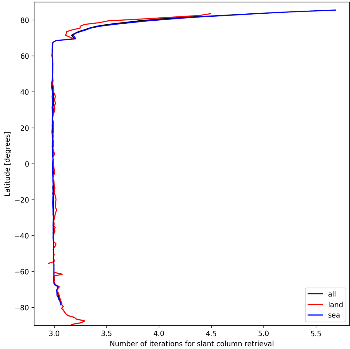
Figure 21: Zonal average of “Number of iterations for slant column retrieval” for 2025-03-11 to 2025-03-12.
