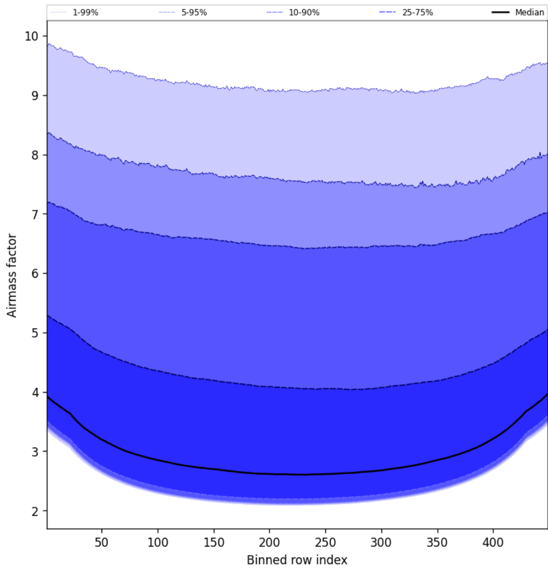
Figure 49: Along track statistics of “Airmass factor” for 2025-03-11 to 2025-03-12
