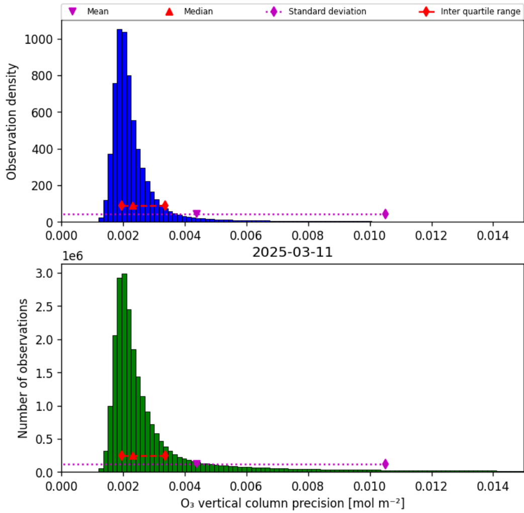
Figure 30: Histogram of “O 3 vertical column precision” for 2025-03-11 to 2025-03-12
