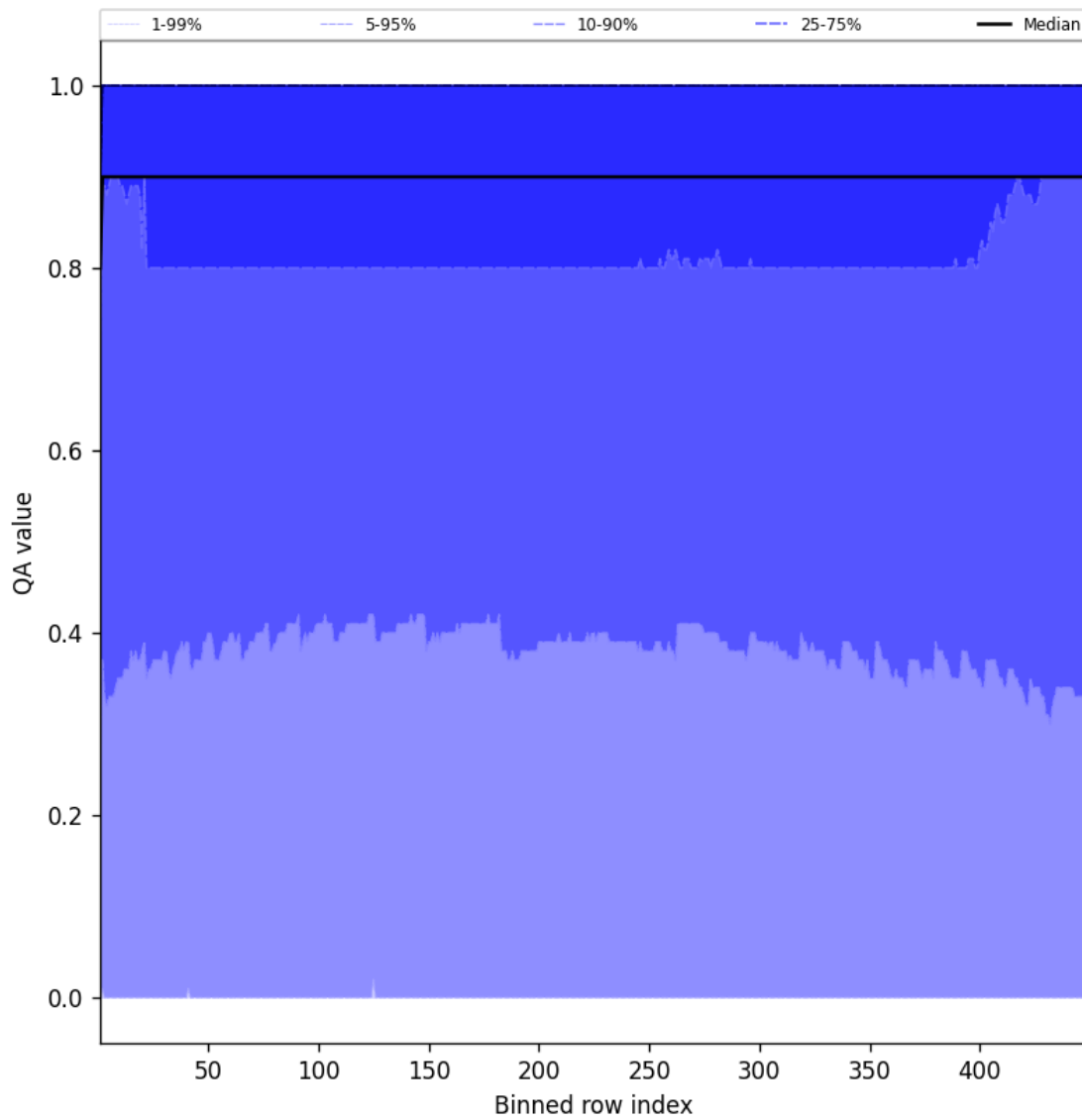
Figure 40: Along track statistics of “QA value” for 2025-03-11 to 2025-03-12
