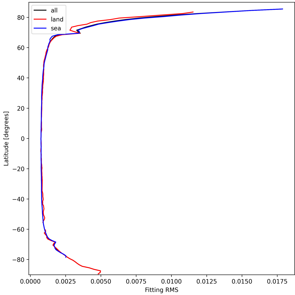
Figure 22: Zonal average of “Fitting RMS” for 2025-03-11 to 2025-03-12.
