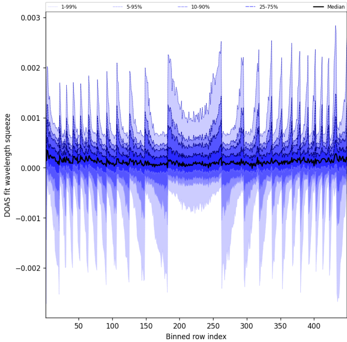
Figure 48: Along track statistics of “DOAS fit wavelength squeeze” for 2025-03-11 to 2025-03-12
