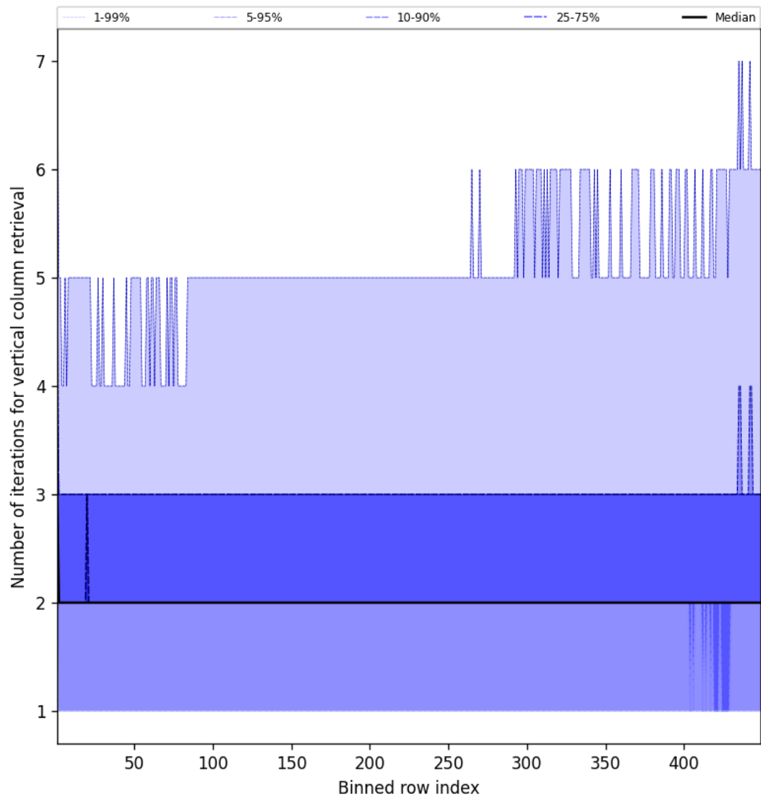
Figure 51: Along track statistics of “Number of iterations for vertical column retrieval” for 2025-03-11 to 2025-03-12
