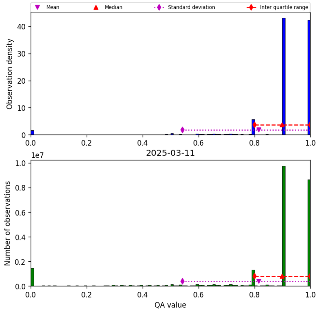
Figure 28: Histogram of “QA value” for 2025-03-11 to 2025-03-12
