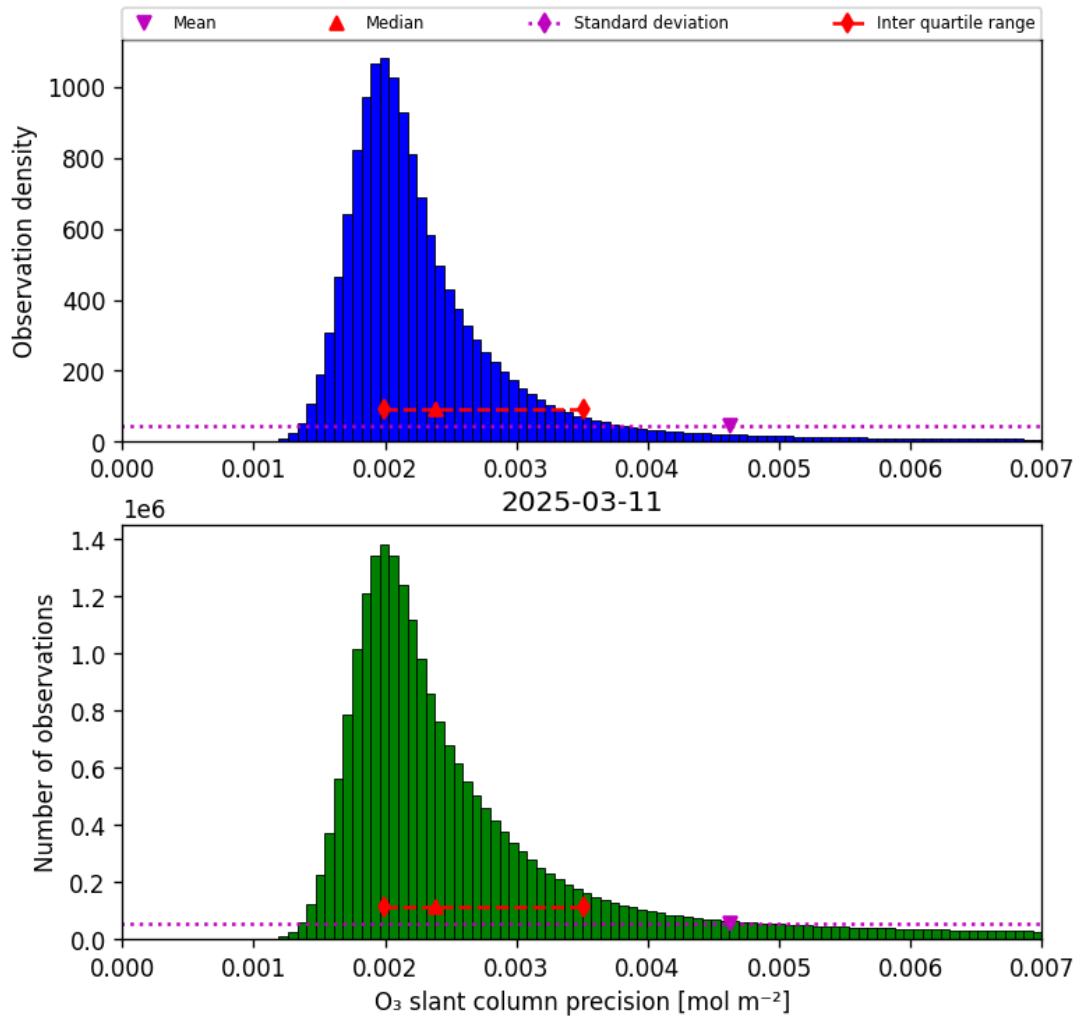
Figure 32: Histogram of “O 3 slant column precision” for 2025-03-11 to 2025-03-12
