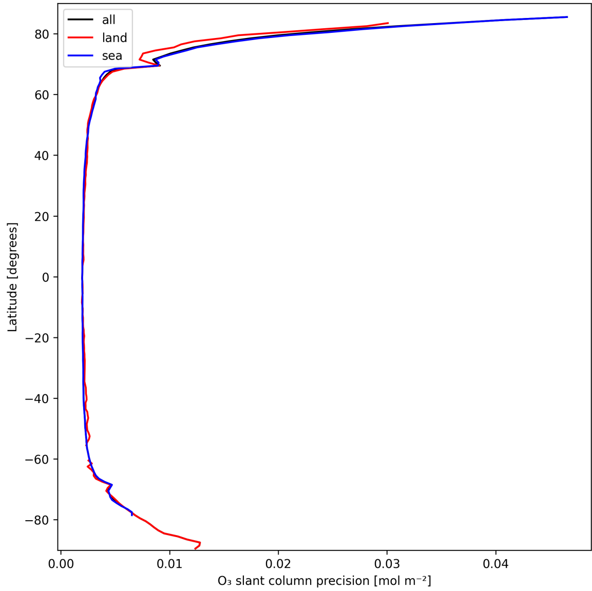
Figure 20: Zonal average of "O 3 slant column precision" for 2025-03-11 to 2025-03-12.
