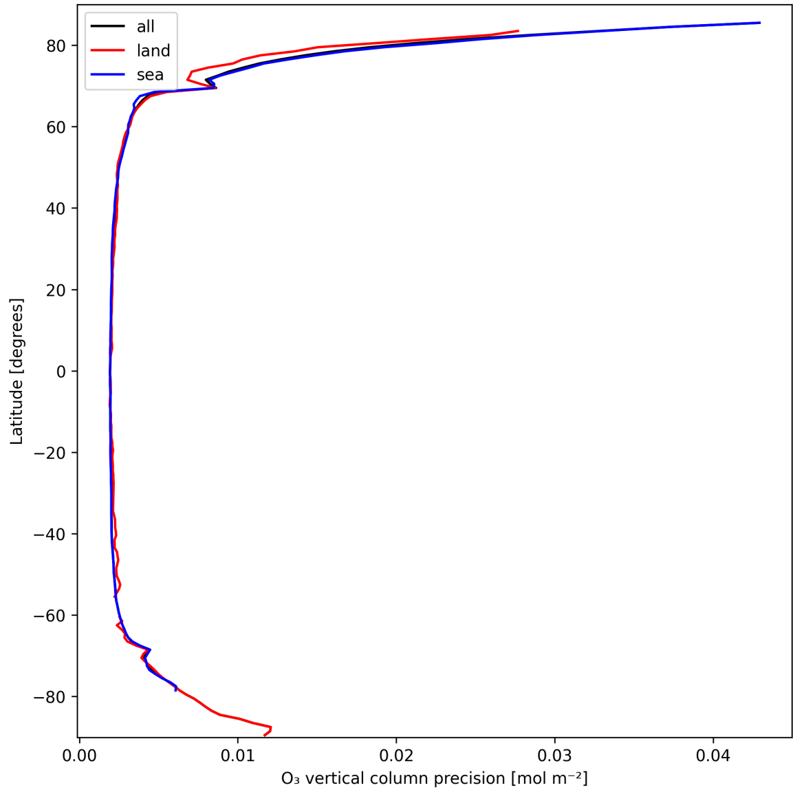
Figure 18: Zonal average of “O 3 vertical column precision” for 2025-03-11 to 2025-03-12.
