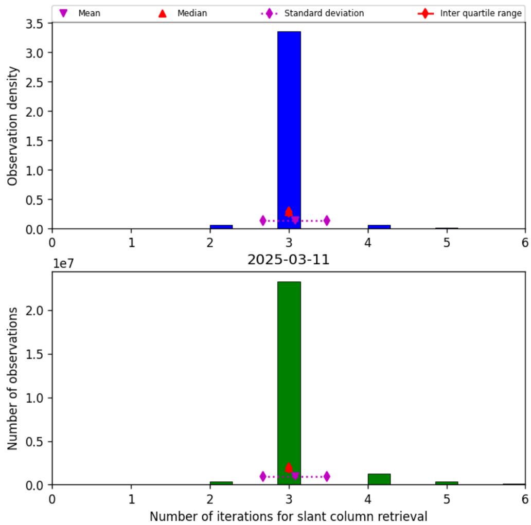
Figure 33: Histogram of “Number of iterations for slant column retrieval” for 2025-03-11 to 2025-03-12
