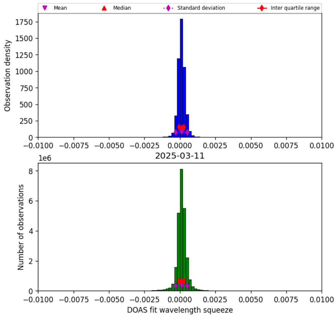
Figure 36: Histogram of “DOAS fit wavelength squeeze” for 2025-03-11 to 2025-03-12
