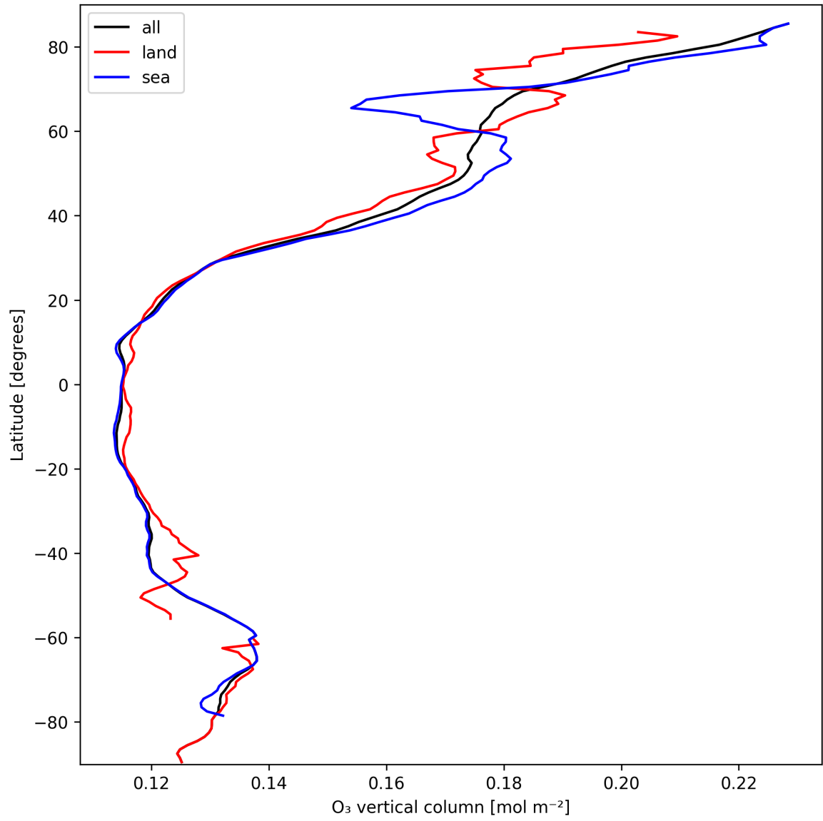
Figure 17: Zonal average of “O 3 vertical column” for 2025-03-11 to 2025-03-12.
