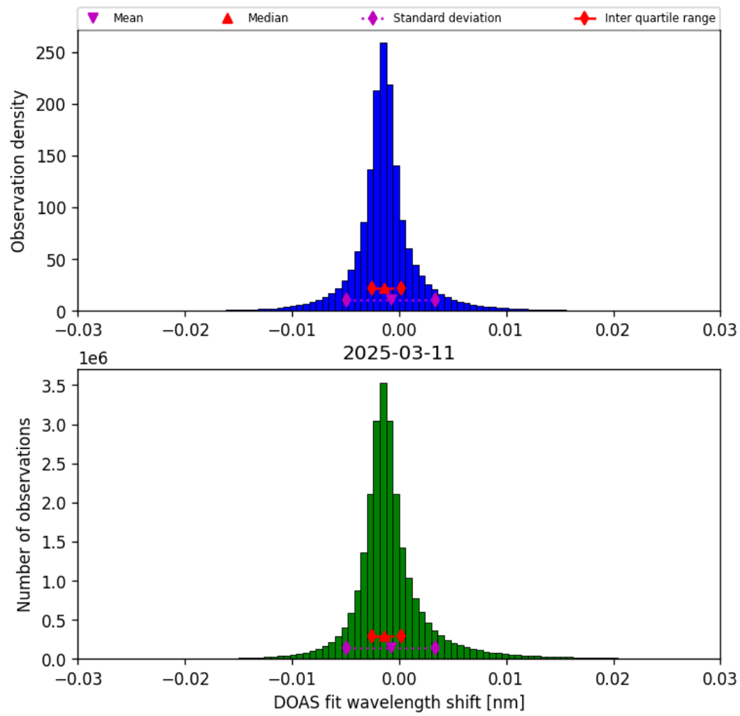
Figure 35: Histogram of “DOAS fit wavelength shift” for 2025-03-11 to 2025-03-12
