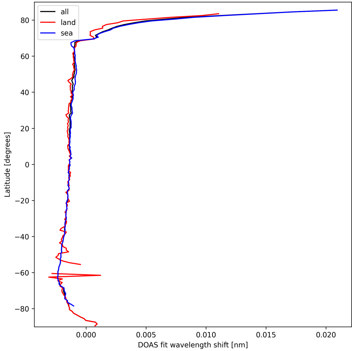
Figure 23: Zonal average of “DOAS fit wavelength shift” for 2025-03-11 to 2025-03-12.
