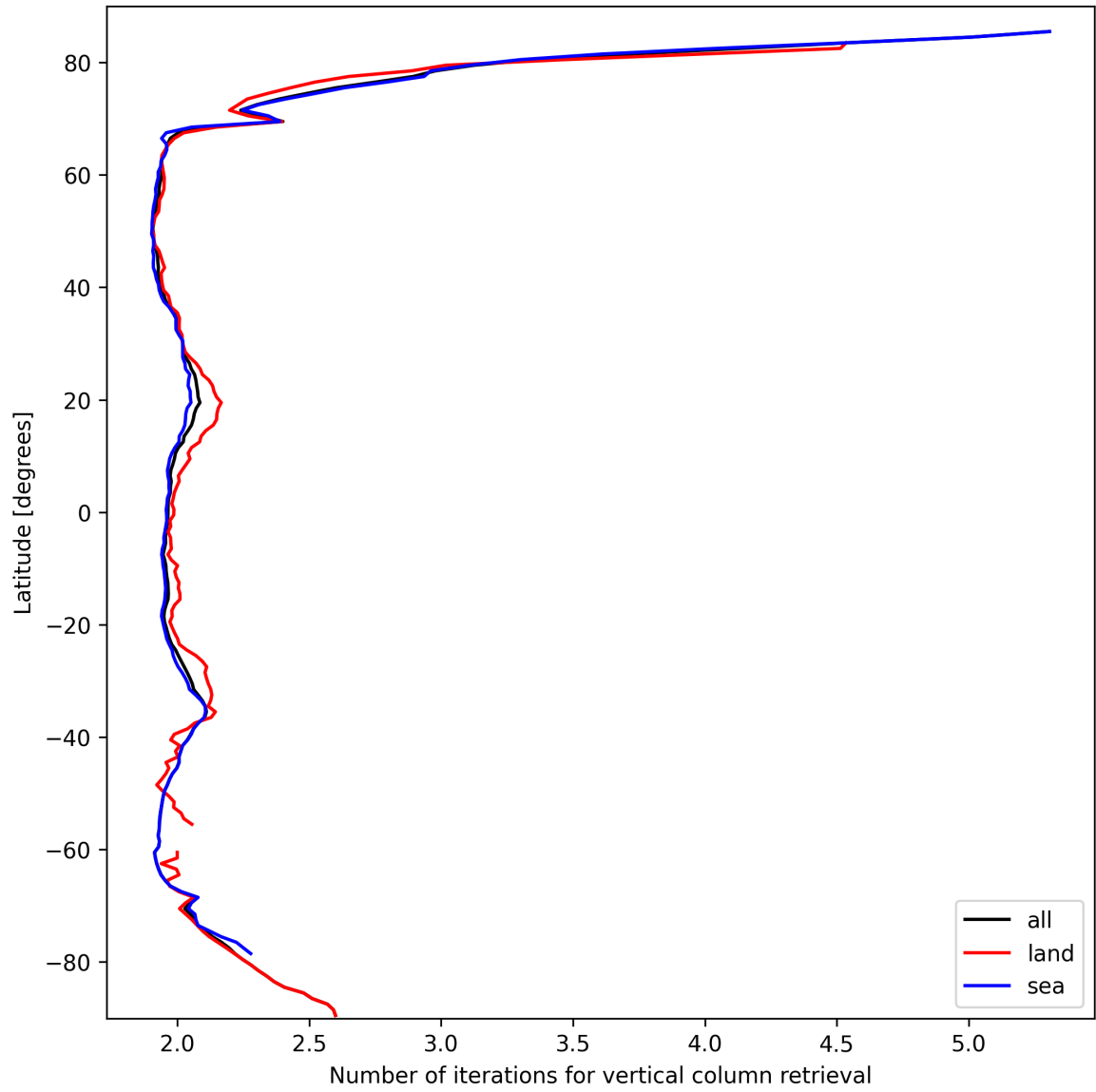
Figure 27: Zonal average of “Number of iterations for vertical column retrieval” for 2025-03-11 to 2025-03-12.
