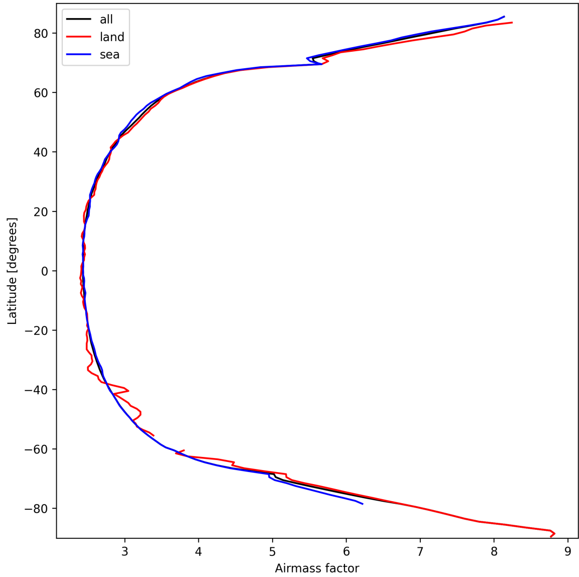
Figure 25: Zonal average of “Airmass factor” for 2025-03-11 to 2025-03-12.
