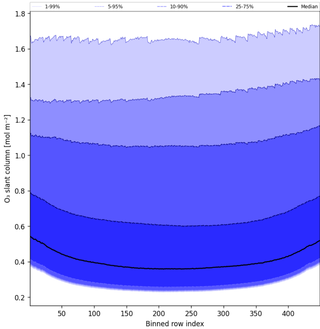
Figure 43: Along track statistics of “O 3 slant column” for 2025-03-11 to 2025-03-12
