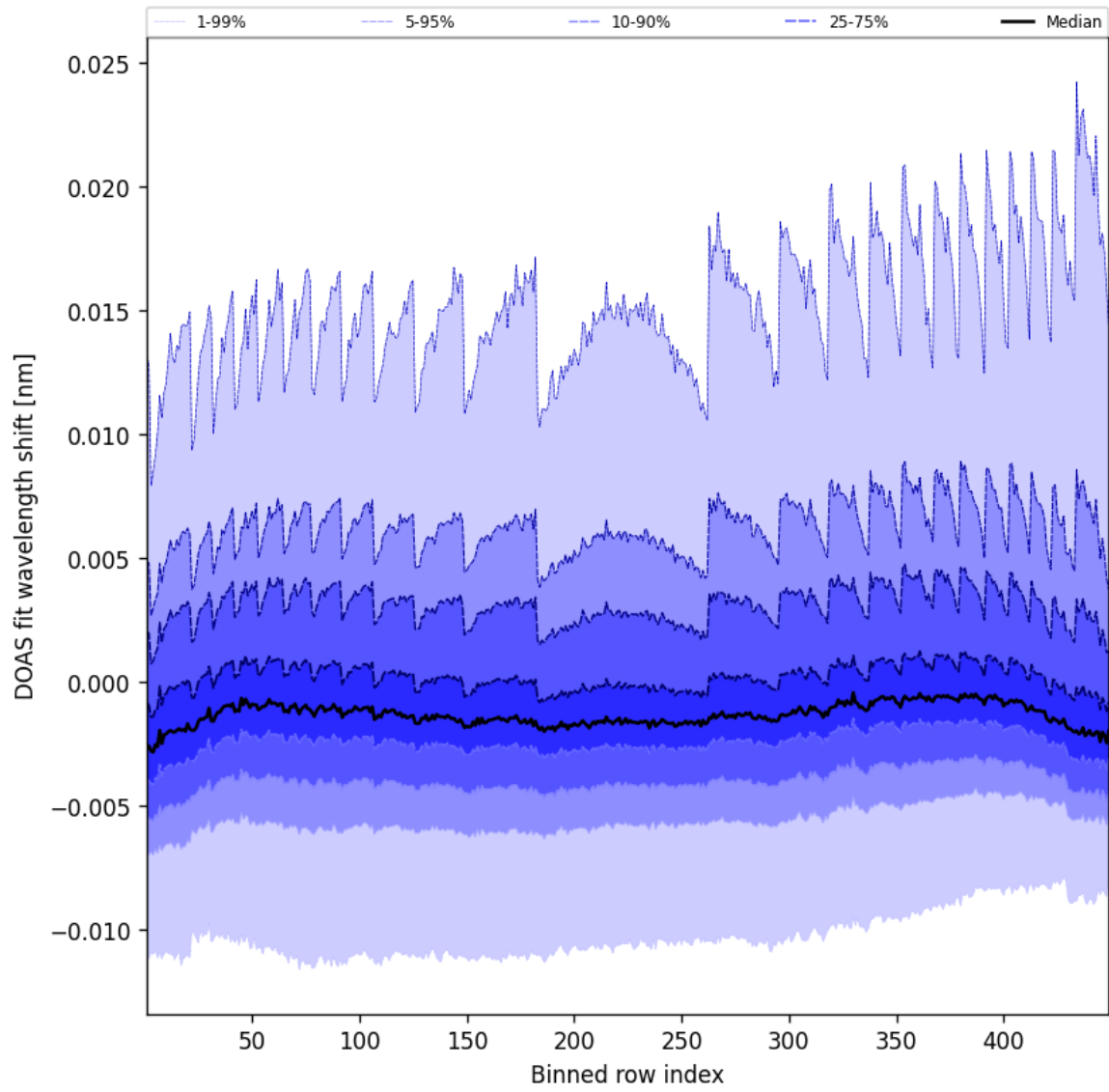
Figure 47: Along track statistics of “DOAS fit wavelength shift” for 2025-03-11 to 2025-03-12
