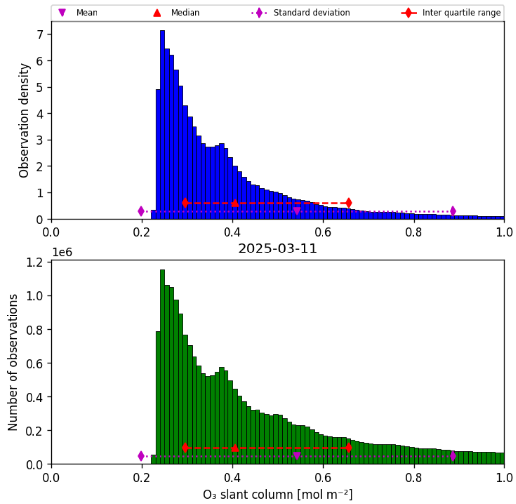
Figure 31: Histogram of “O 3 slant column” for 2025-03-11 to 2025-03-12
