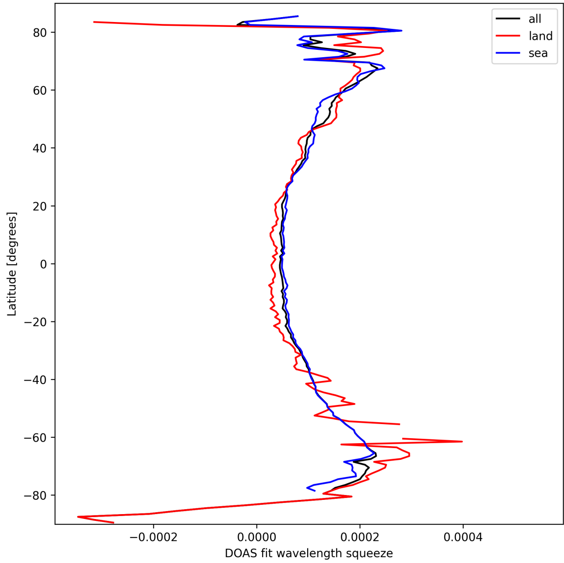
Figure 24: Zonal average of “DOAS fit wavelength squeeze” for 2025-03-11 to 2025-03-12.
