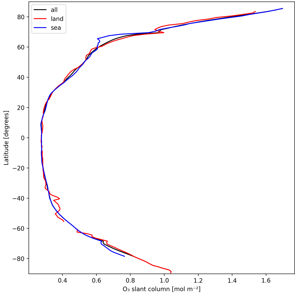
Figure 19: Zonal average of “O 3 slant column” for 2025-03-11 to 2025-03-12.
