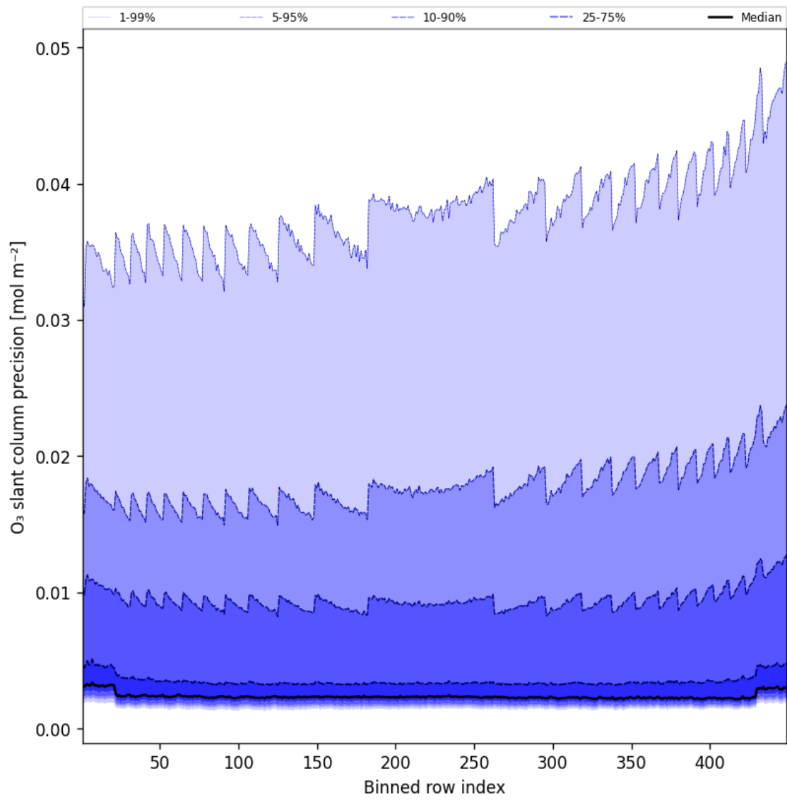
Figure 44: Along track statistics of “O 3 slant column precision” for 2025-03-11 to 2025-03-12
