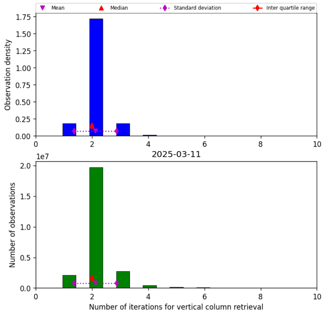
Figure 39: Histogram of “Number of iterations for vertical column retrieval” for 2025-03-11 to 2025-03-12
