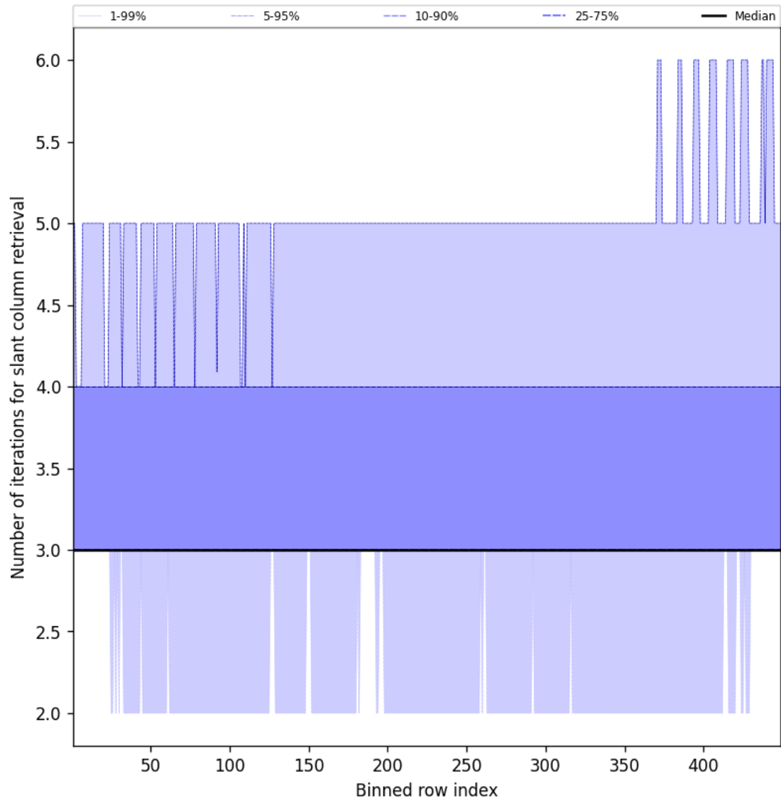
Figure 45: Along track statistics of “Number of iterations for slant column retrieval” for 2025-03-11 to 2025-03-12
