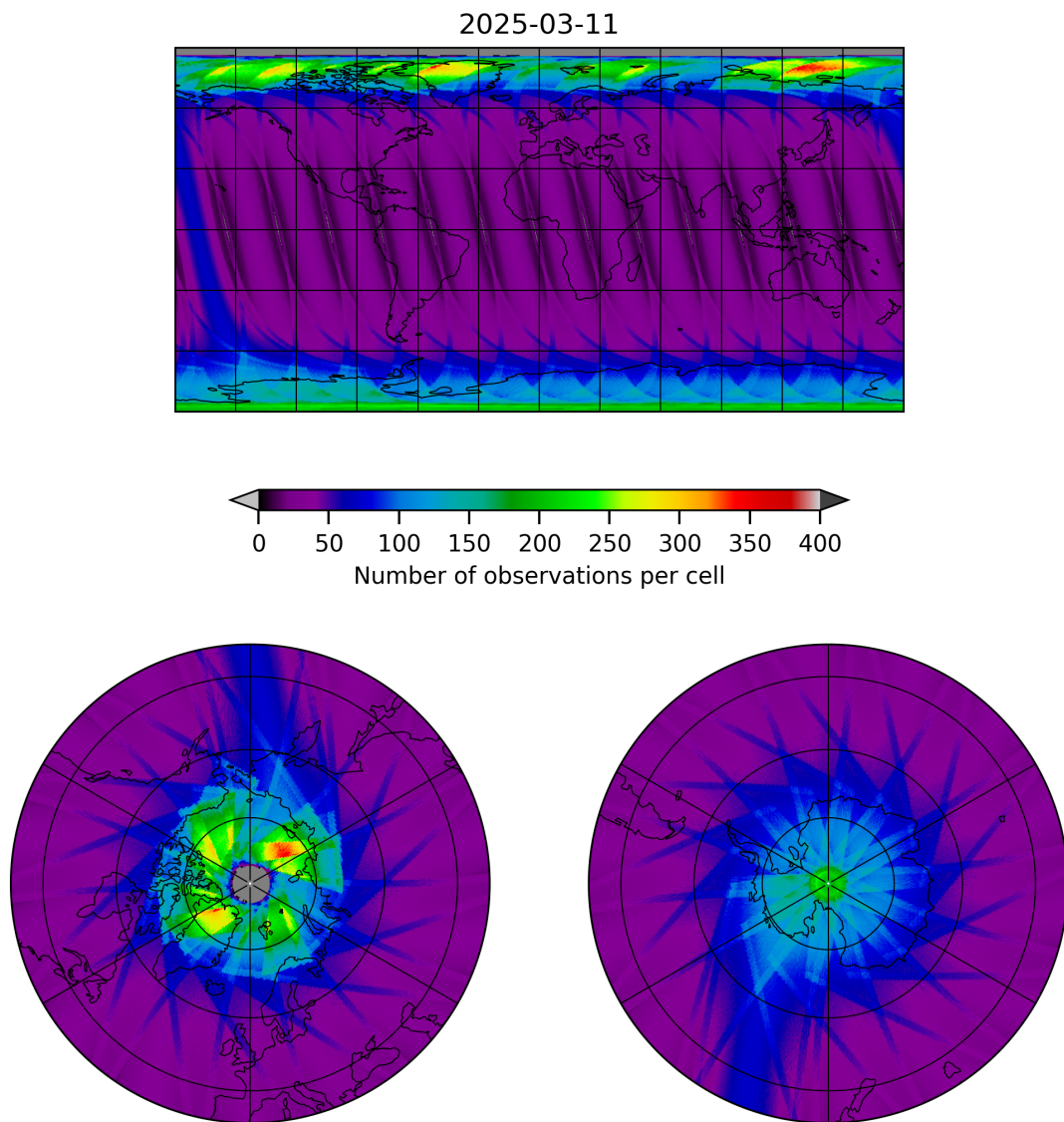
Figure 15: Map of the number of observations for 2025-03-11 to 2025-03-12
