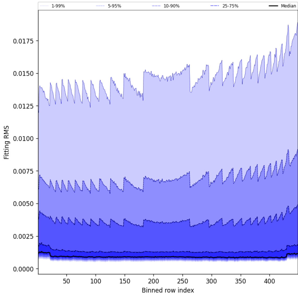
Figure 46: Along track statistics of “Fitting RMS” for 2025-03-11 to 2025-03-12
