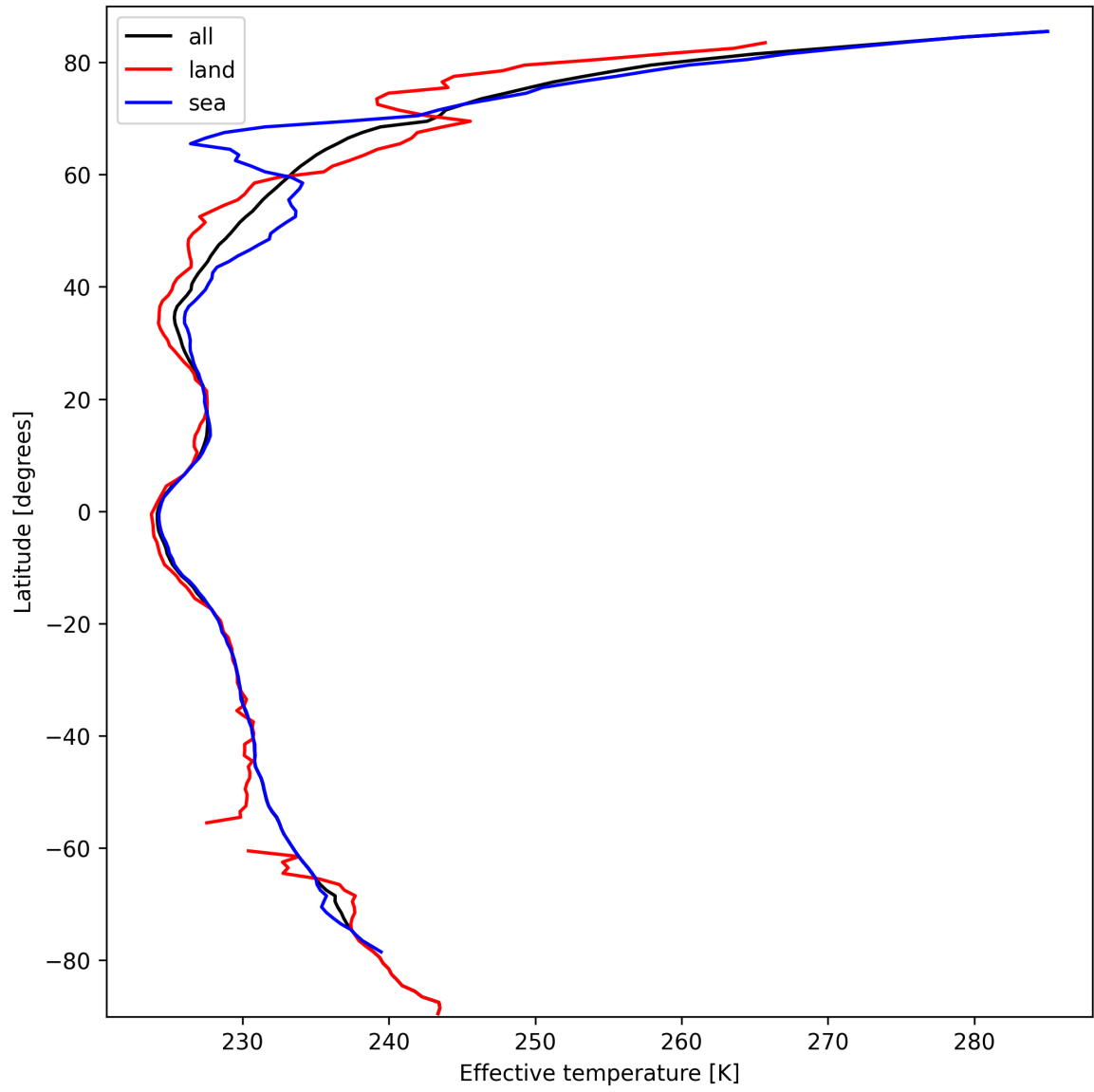
Figure 26: Zonal average of "Effective temperature" for 2025-03-11 to 2025-03-12.
