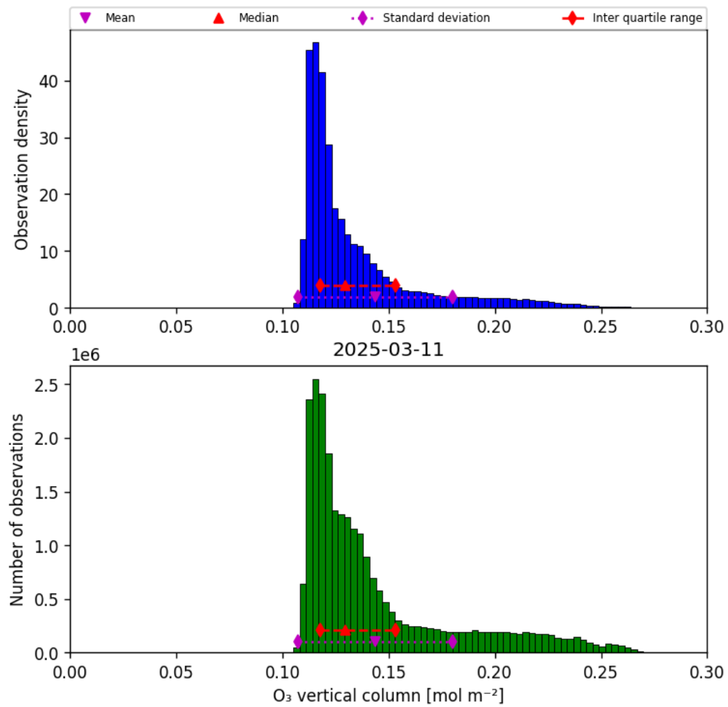
Figure 29: Histogram of “O 3 vertical column” for 2025-03-11 to 2025-03-12
