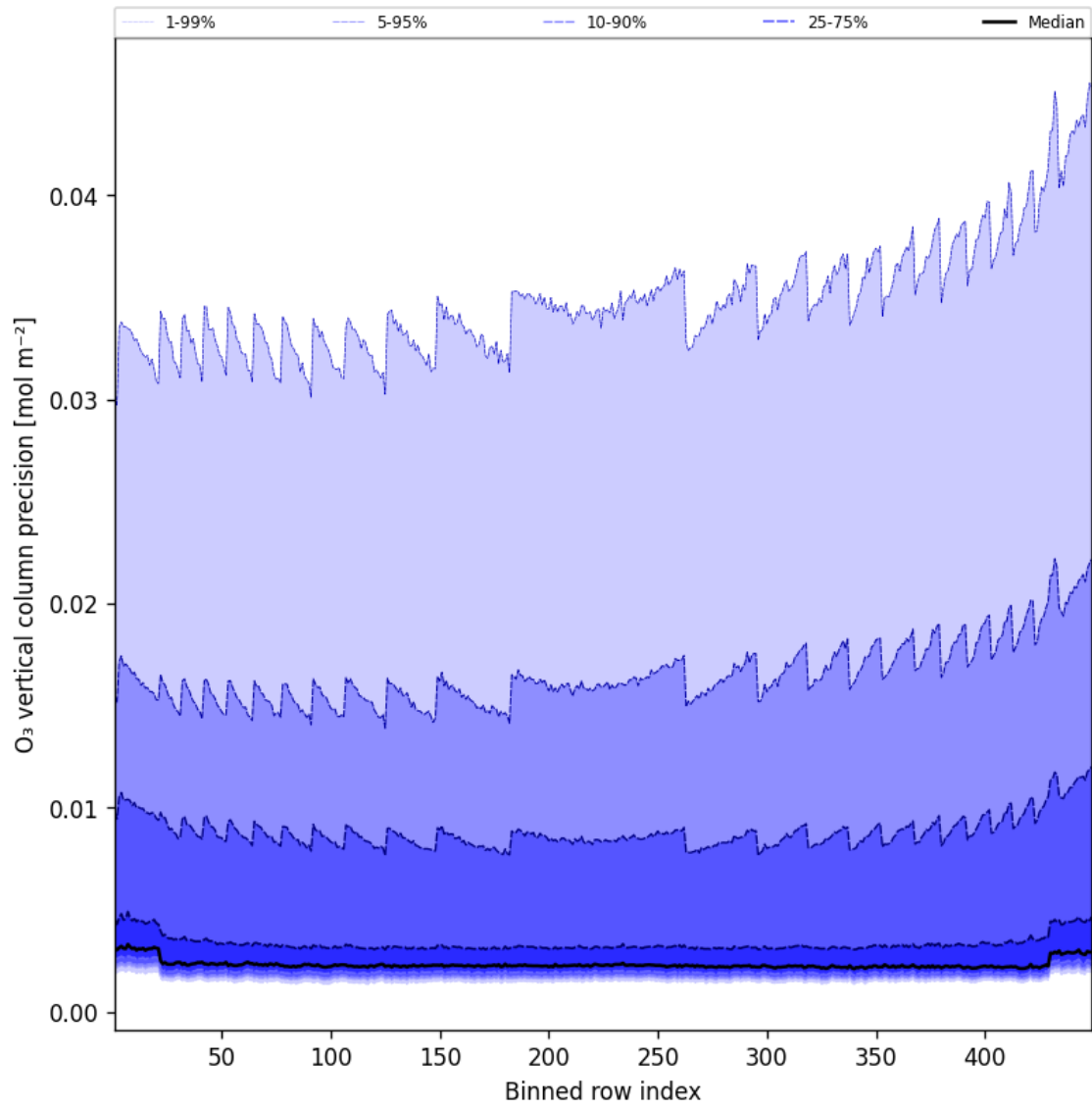
Figure 42: Along track statistics of “O 3 vertical column precision” for 2025-03-11 to 2025-03-12
