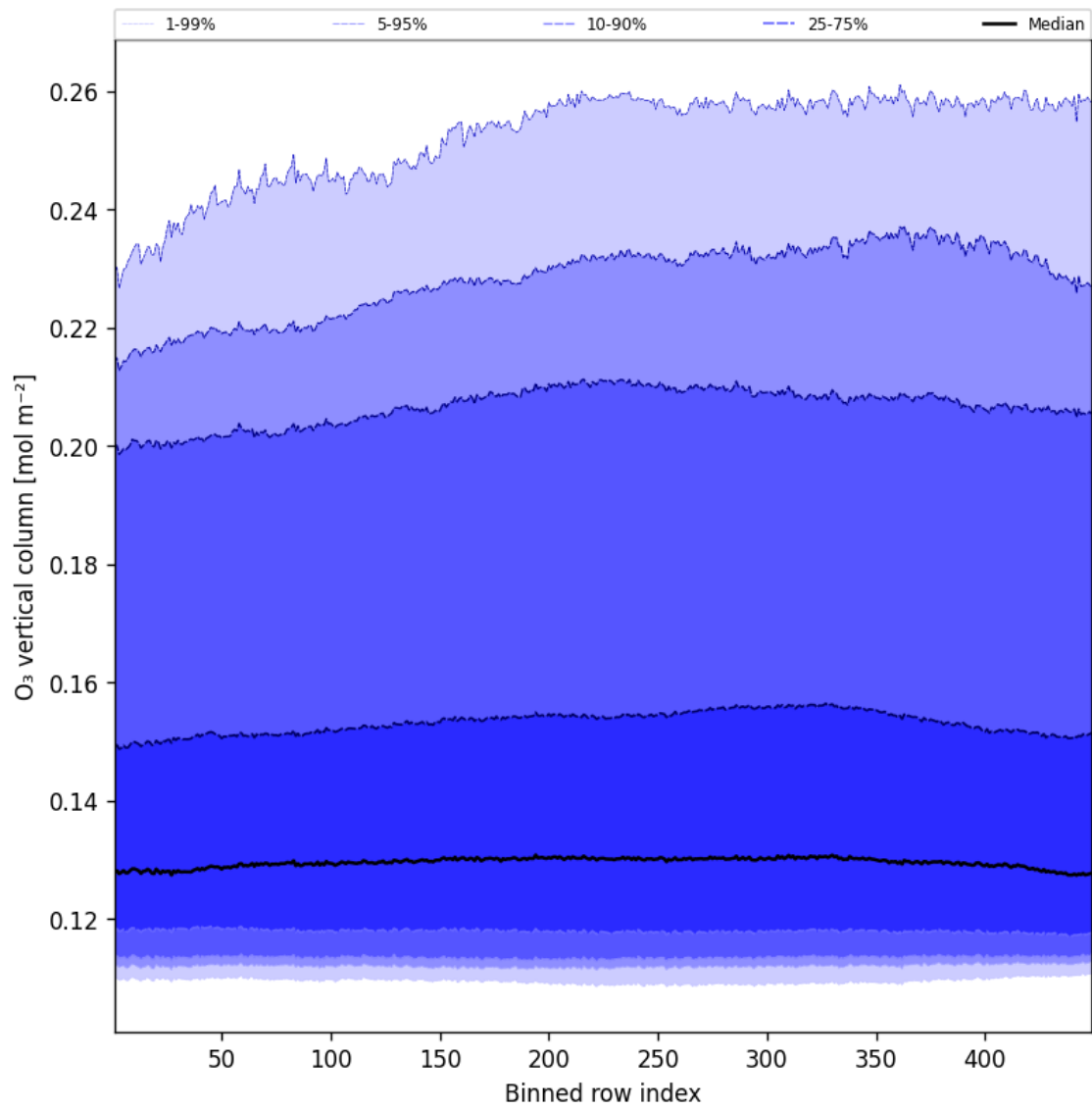
Figure 41: Along track statistics of “O 3 vertical column” for 2025-03-11 to 2025-03-12
