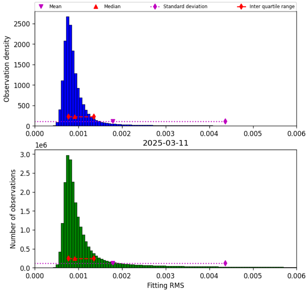
Figure 34: Histogram of “Fitting RMS” for 2025-03-11 to 2025-03-12
