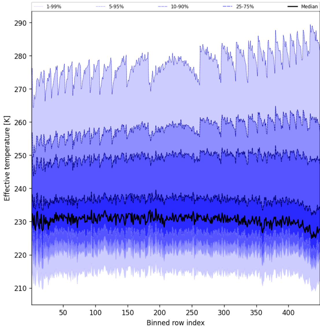
Figure 50: Along track statistics of “Effective temperature” for 2025-03-11 to 2025-03-12
