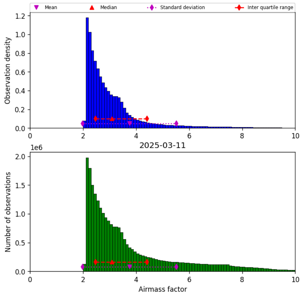
Figure 37: Histogram of “Airmass factor” for 2025-03-11 to 2025-03-12
