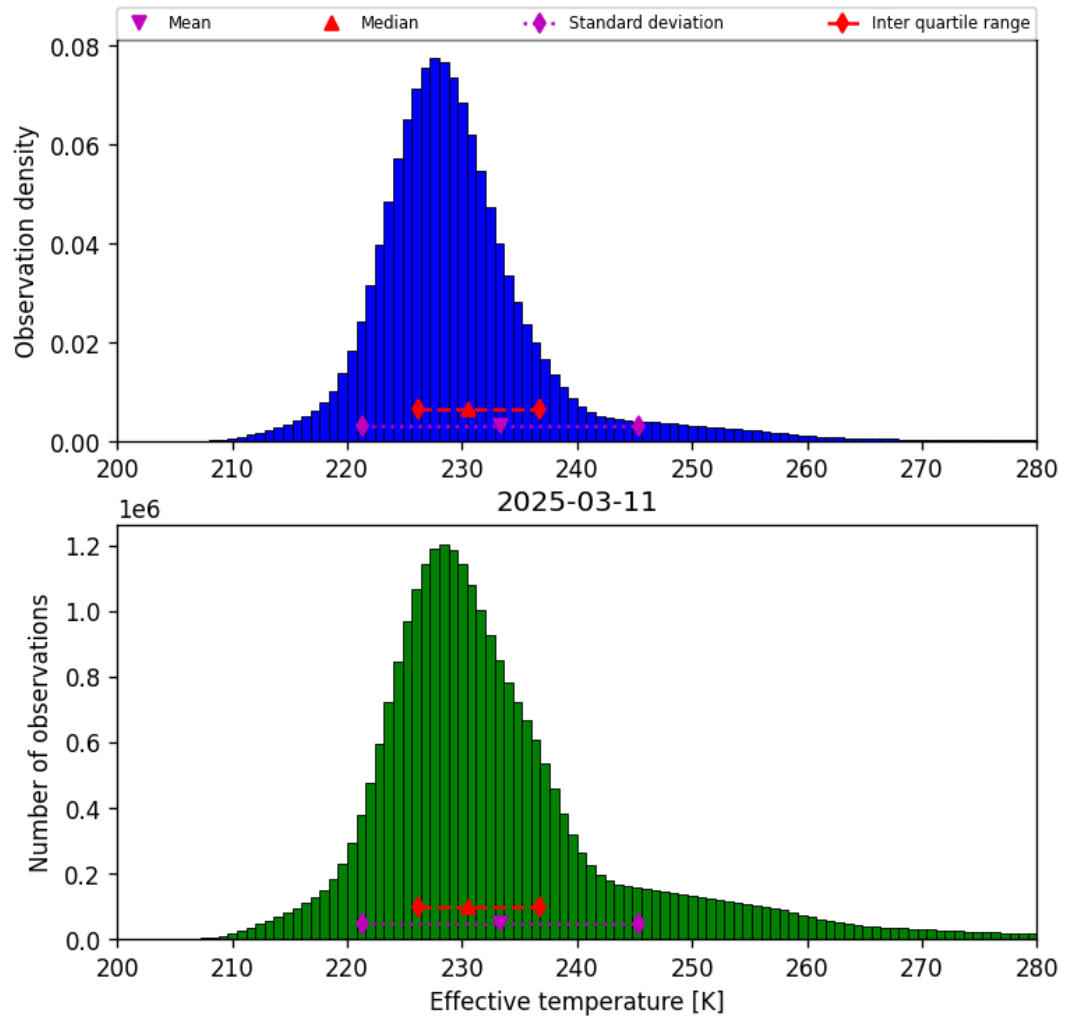
Figure 38: Histogram of “Effective temperature” for 2025-03-11 to 2025-03-12
