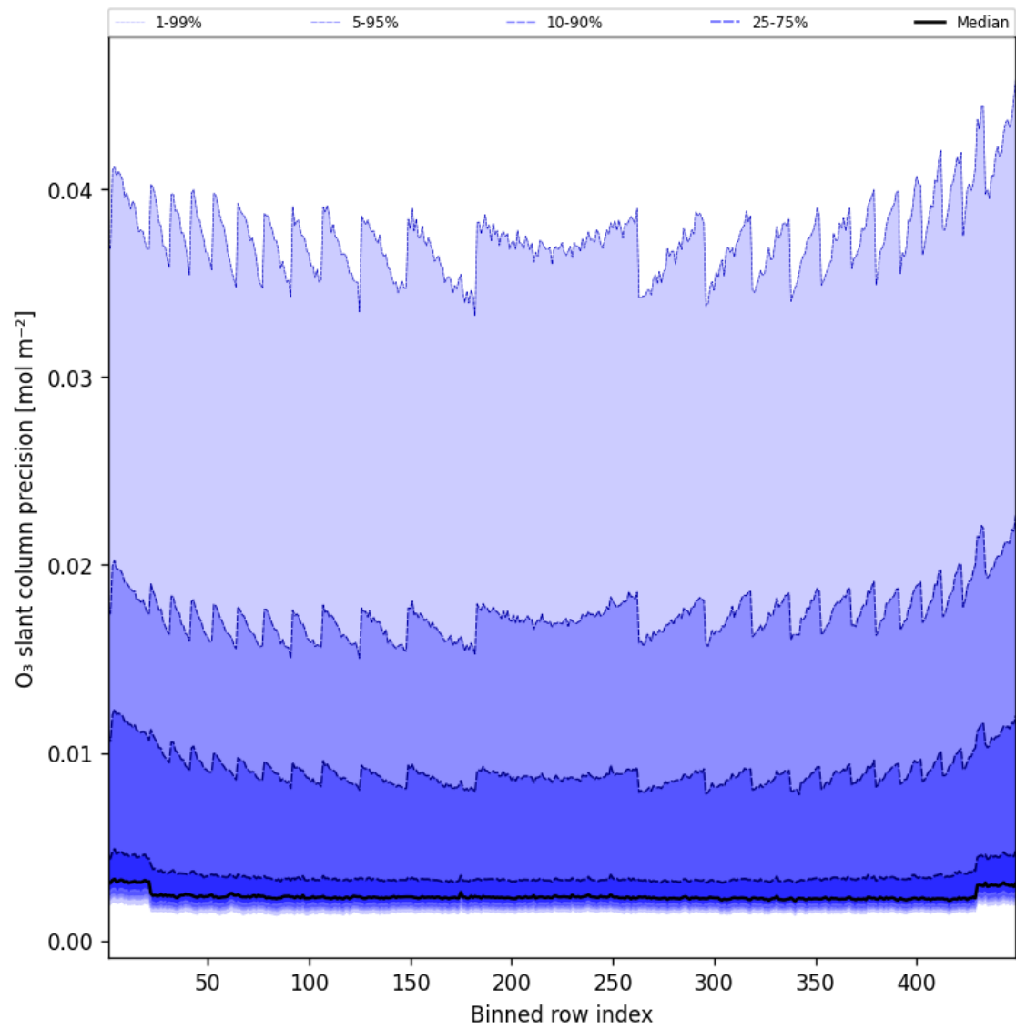
Figure 44: Along track statistics of “O 3 slant column precision” for 2025-03-12 to 2025-03-13
