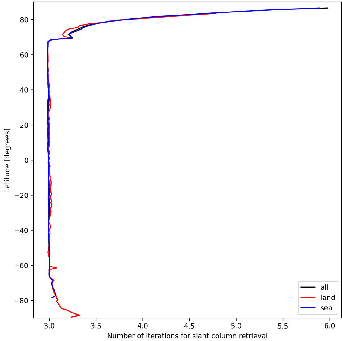
Figure 21: Zonal average of “Number of iterations for slant column retrieval” for 2025-03-12 to 2025-03-13.
