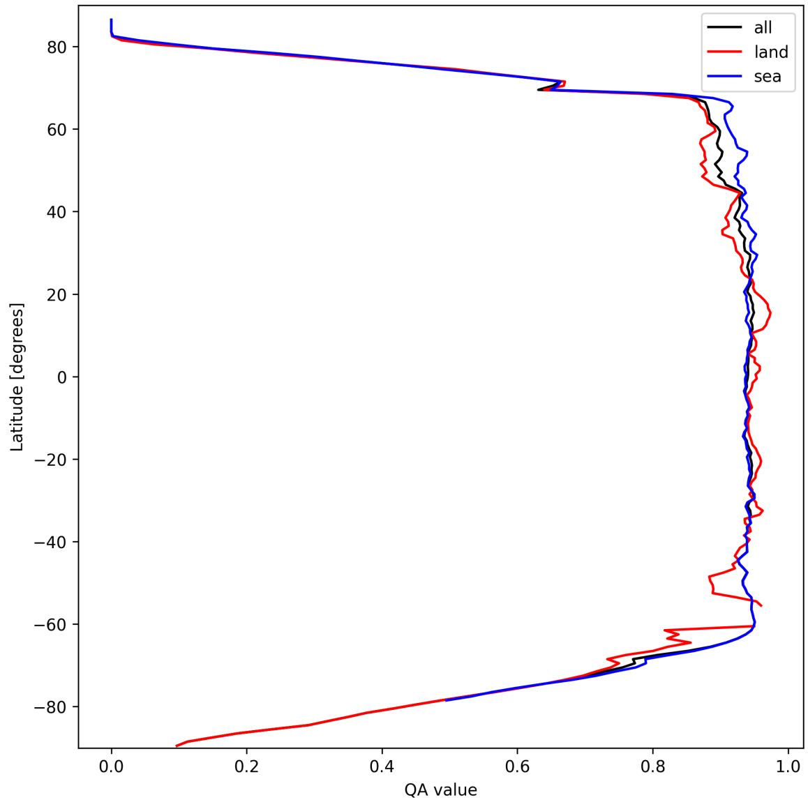
Figure 16: Zonal average of “QA value” for 2025-03-12 to 2025-03-13.
