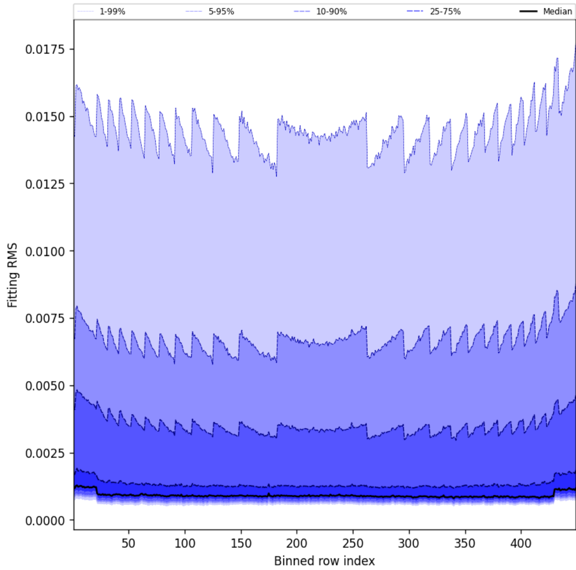
Figure 46: Along track statistics of “Fitting RMS” for 2025-03-12 to 2025-03-13
