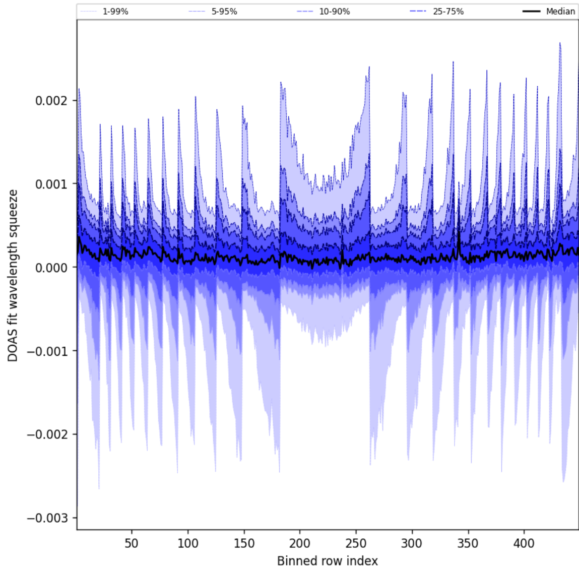
Figure 48: Along track statistics of “DOAS fit wavelength squeeze” for 2025-03-12 to 2025-03-13
