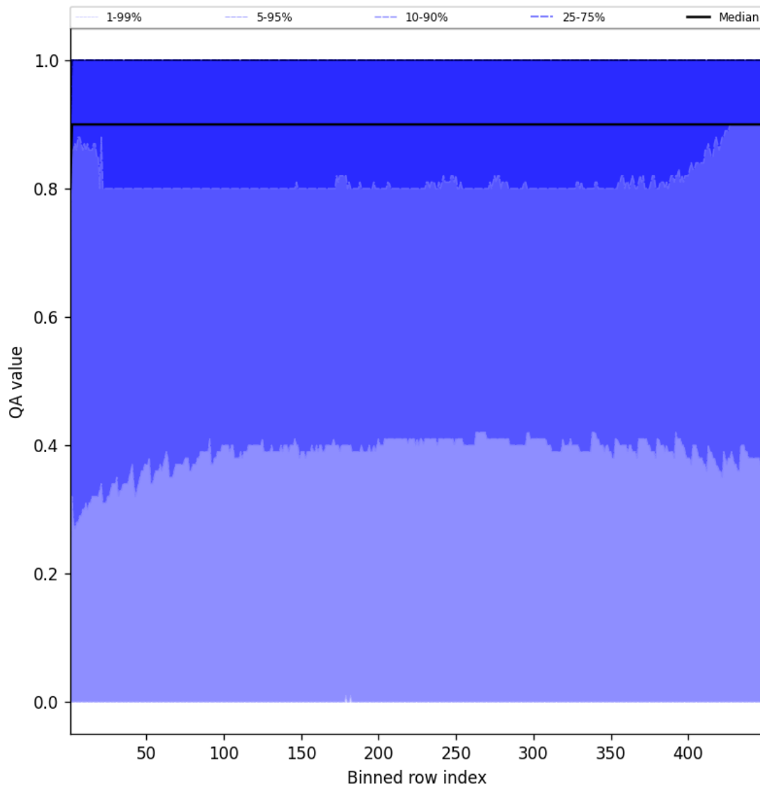
Figure 40: Along track statistics of “QA value” for 2025-03-12 to 2025-03-13
