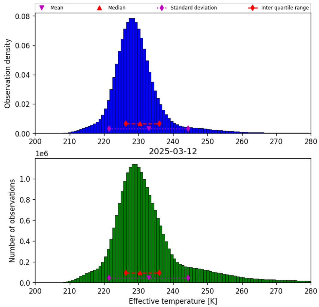
Figure 38: Histogram of “Effective temperature” for 2025-03-12 to 2025-03-13
