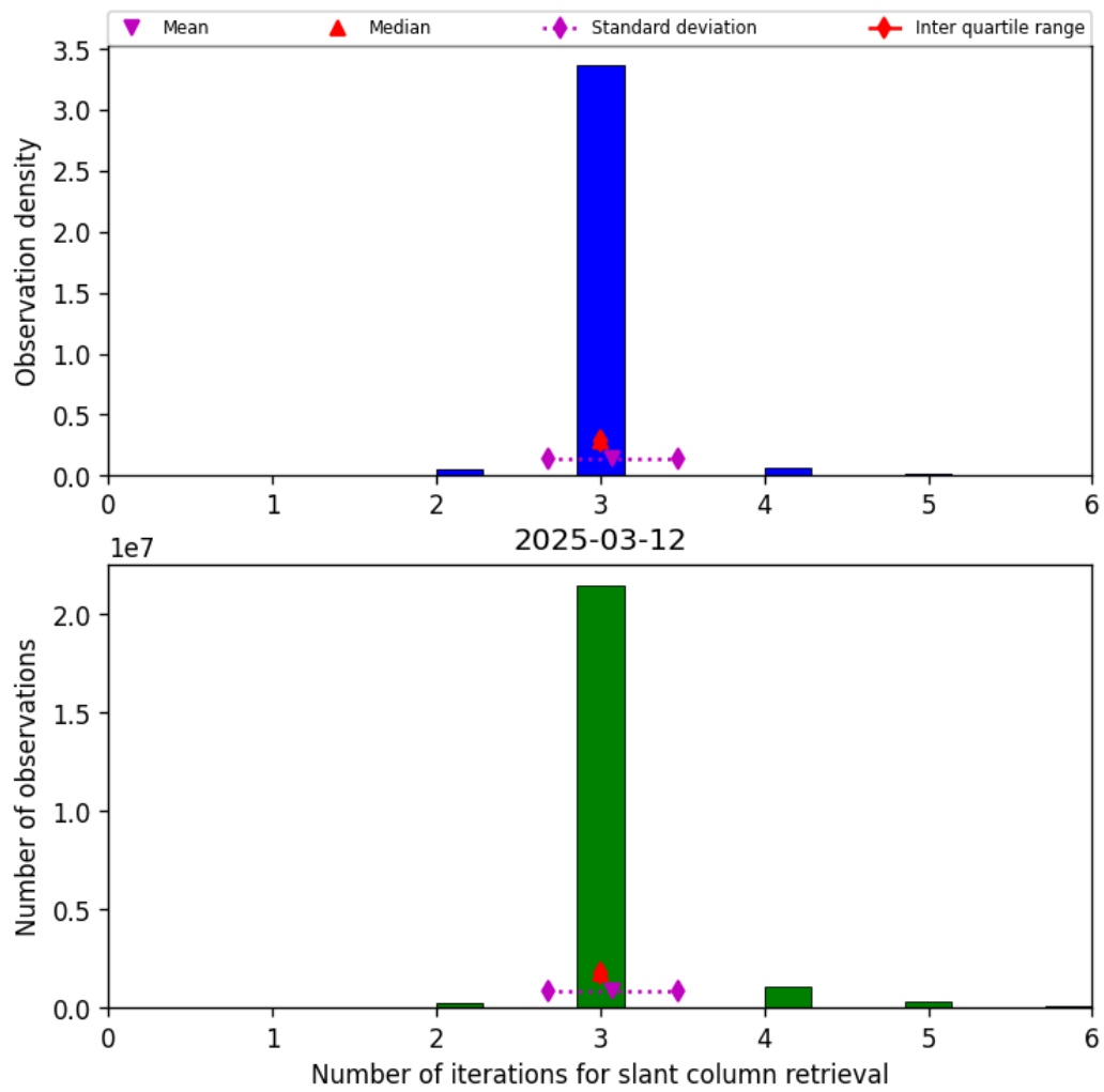
Figure 33: Histogram of “Number of iterations for slant column retrieval” for 2025-03-12 to 2025-03-13
