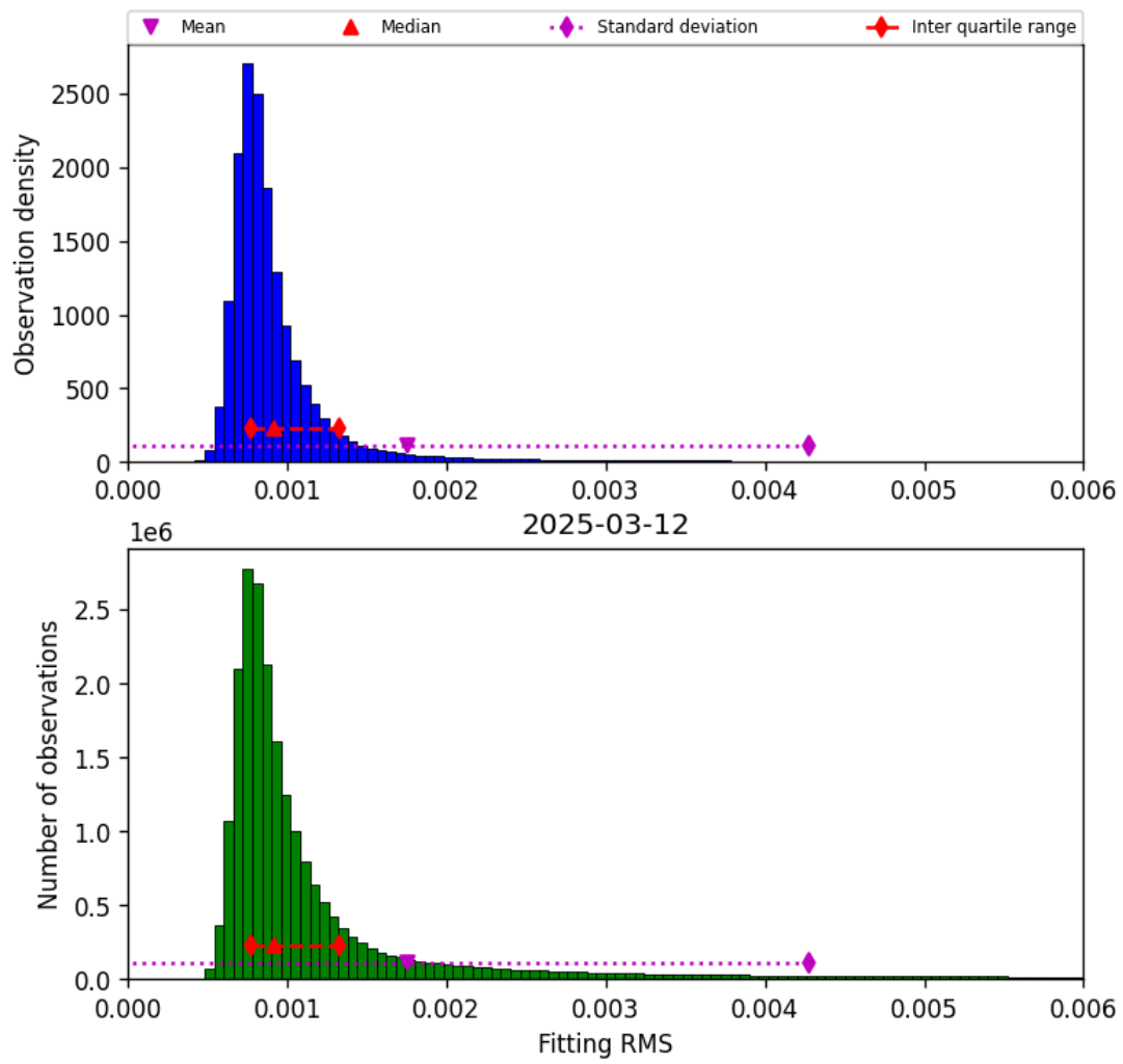
Figure 34: Histogram of “Fitting RMS” for 2025-03-12 to 2025-03-13
