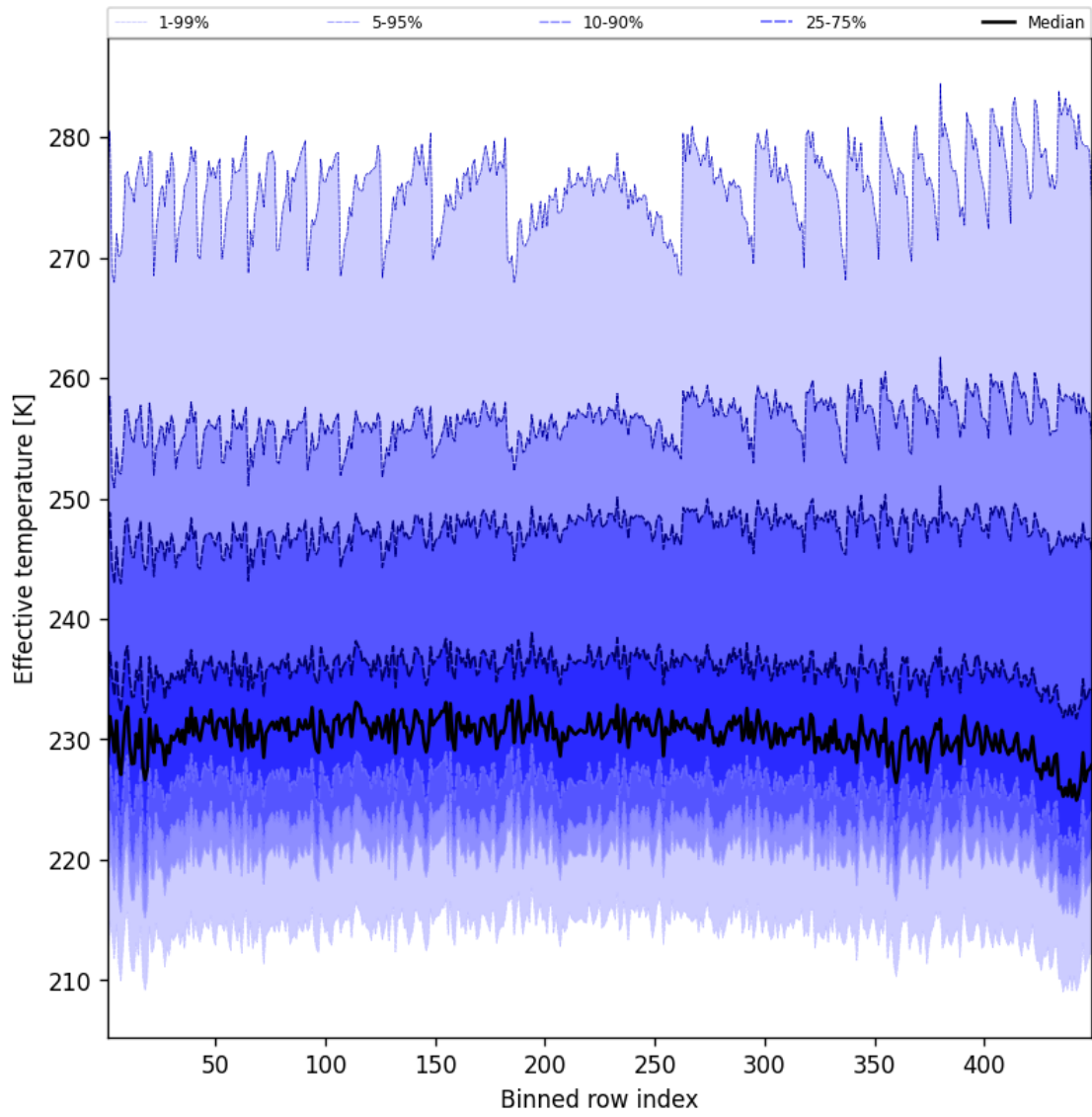
Figure 50: Along track statistics of “Effective temperature” for 2025-03-12 to 2025-03-13
