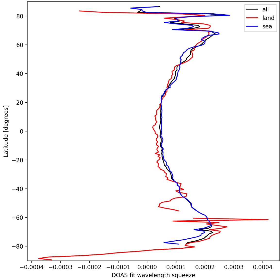
Figure 24: Zonal average of “DOAS fit wavelength squeeze” for 2025-03-12 to 2025-03-13.
