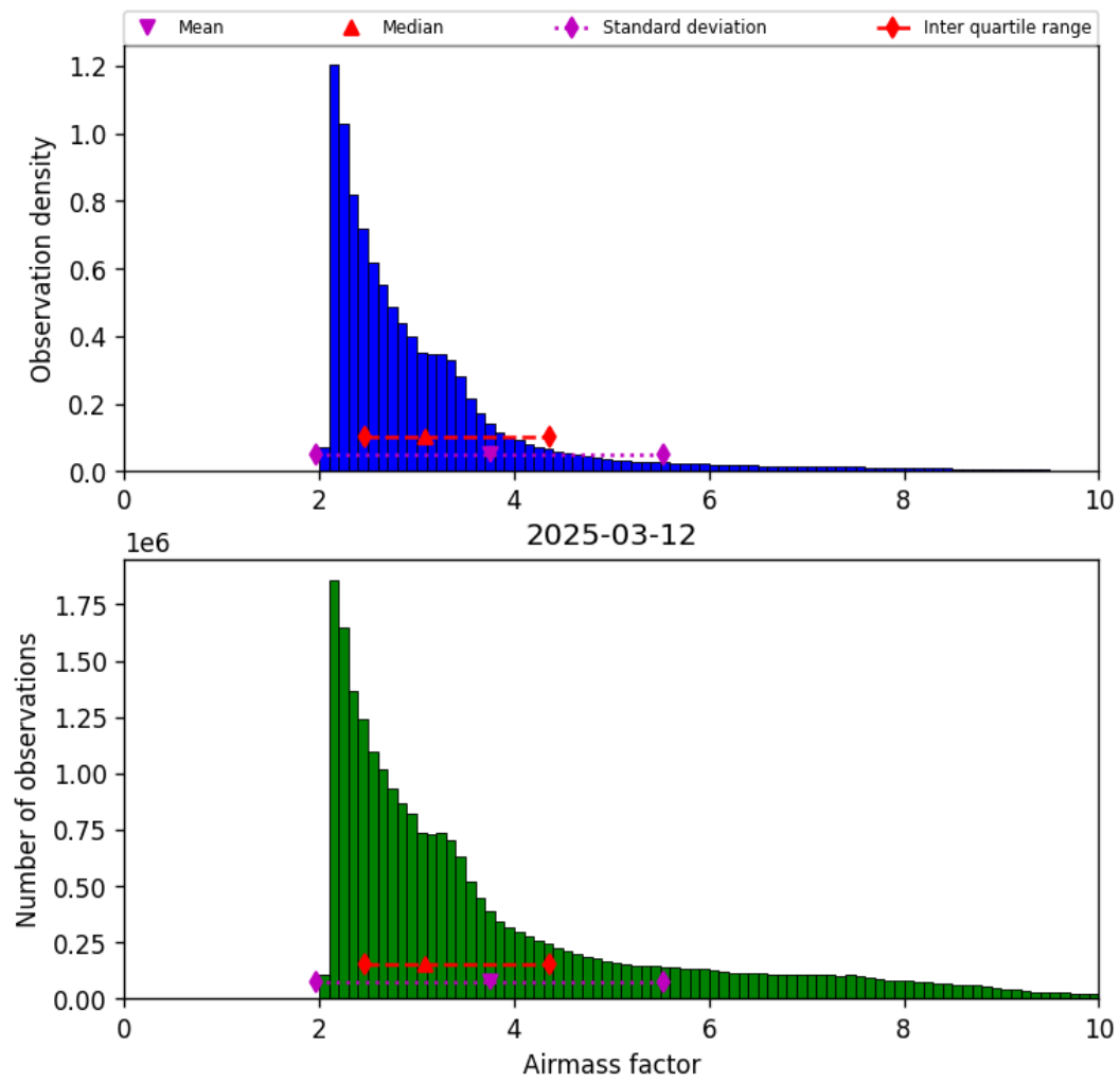
Figure 37: Histogram of “Airmass factor” for 2025-03-12 to 2025-03-13
