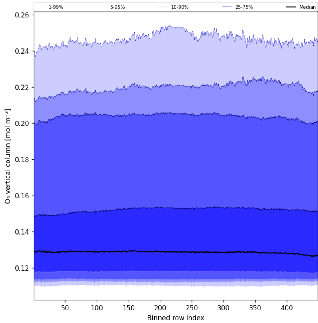
Figure 41: Along track statistics of “O 3 vertical column” for 2025-03-12 to 2025-03-13
