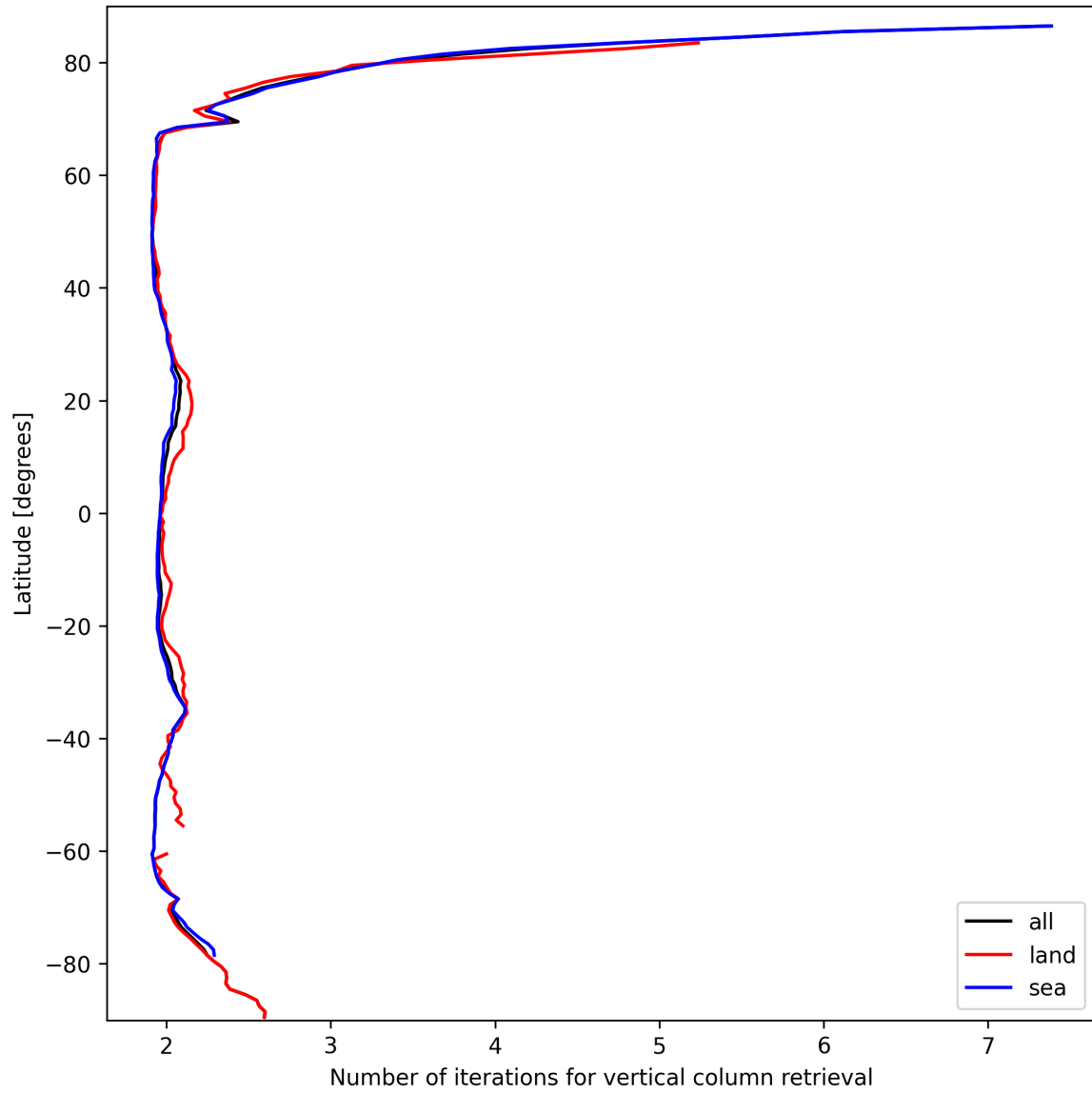
Figure 27: Zonal average of “Number of iterations for vertical column retrieval” for 2025-03-12 to 2025-03-13.
