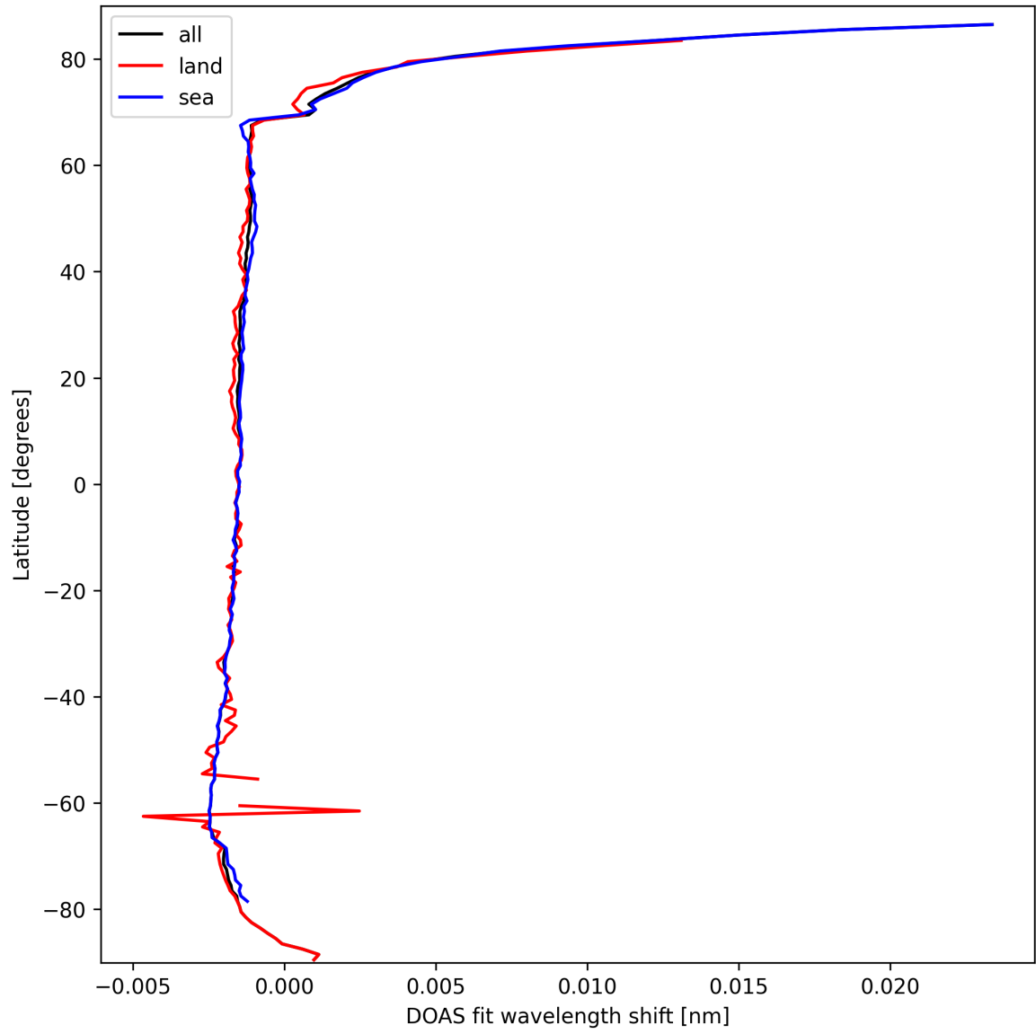
Figure 23: Zonal average of “DOAS fit wavelength shift” for 2025-03-12 to 2025-03-13.
