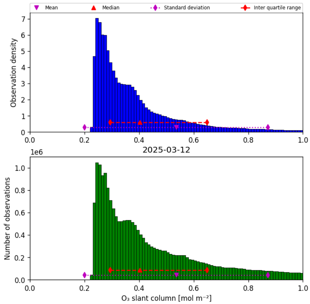
Figure 31: Histogram of “O 3 slant column” for 2025-03-12 to 2025-03-13
