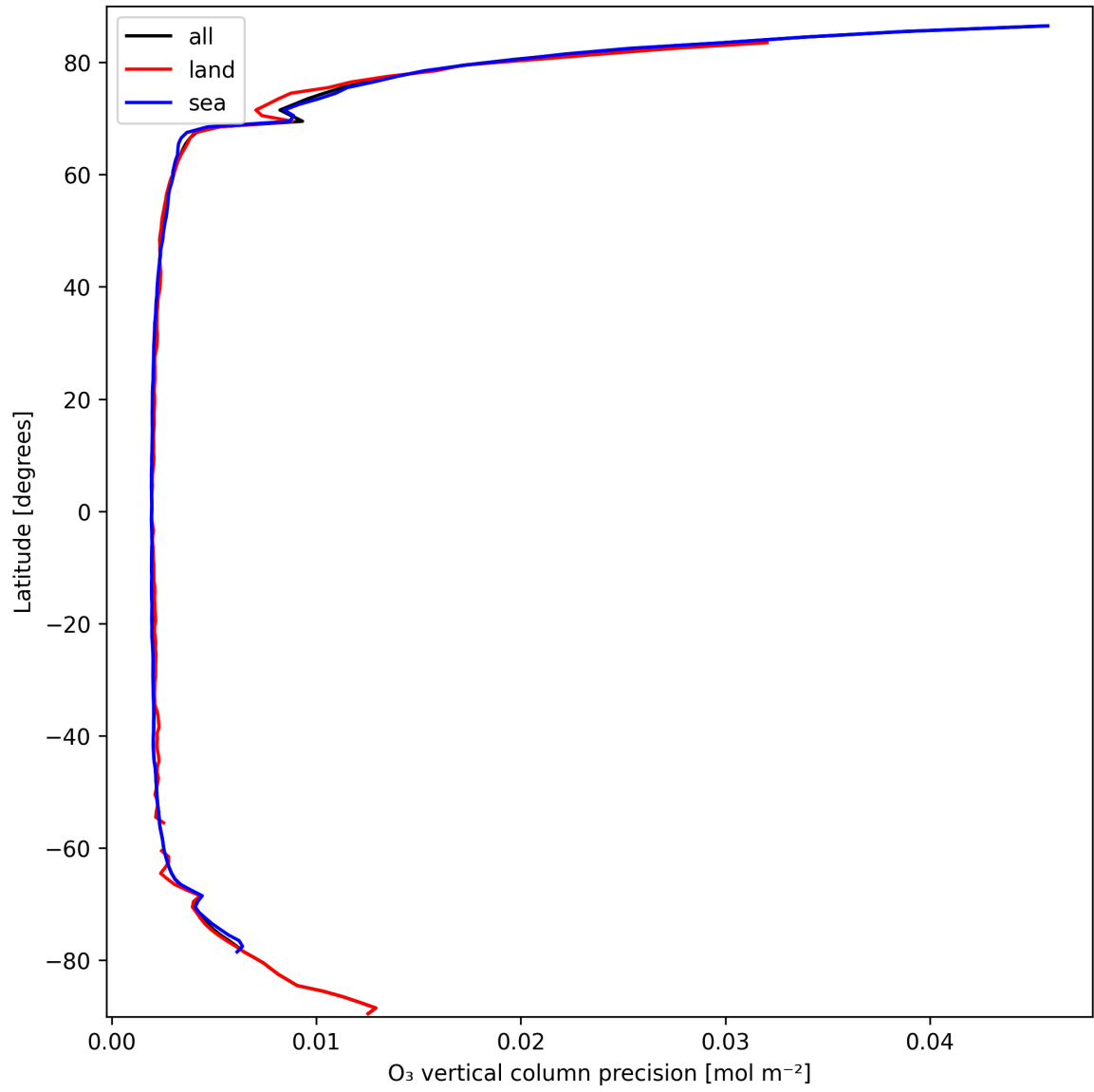
Figure 18: Zonal average of “O 3 vertical column precision” for 2025-03-12 to 2025-03-13.
