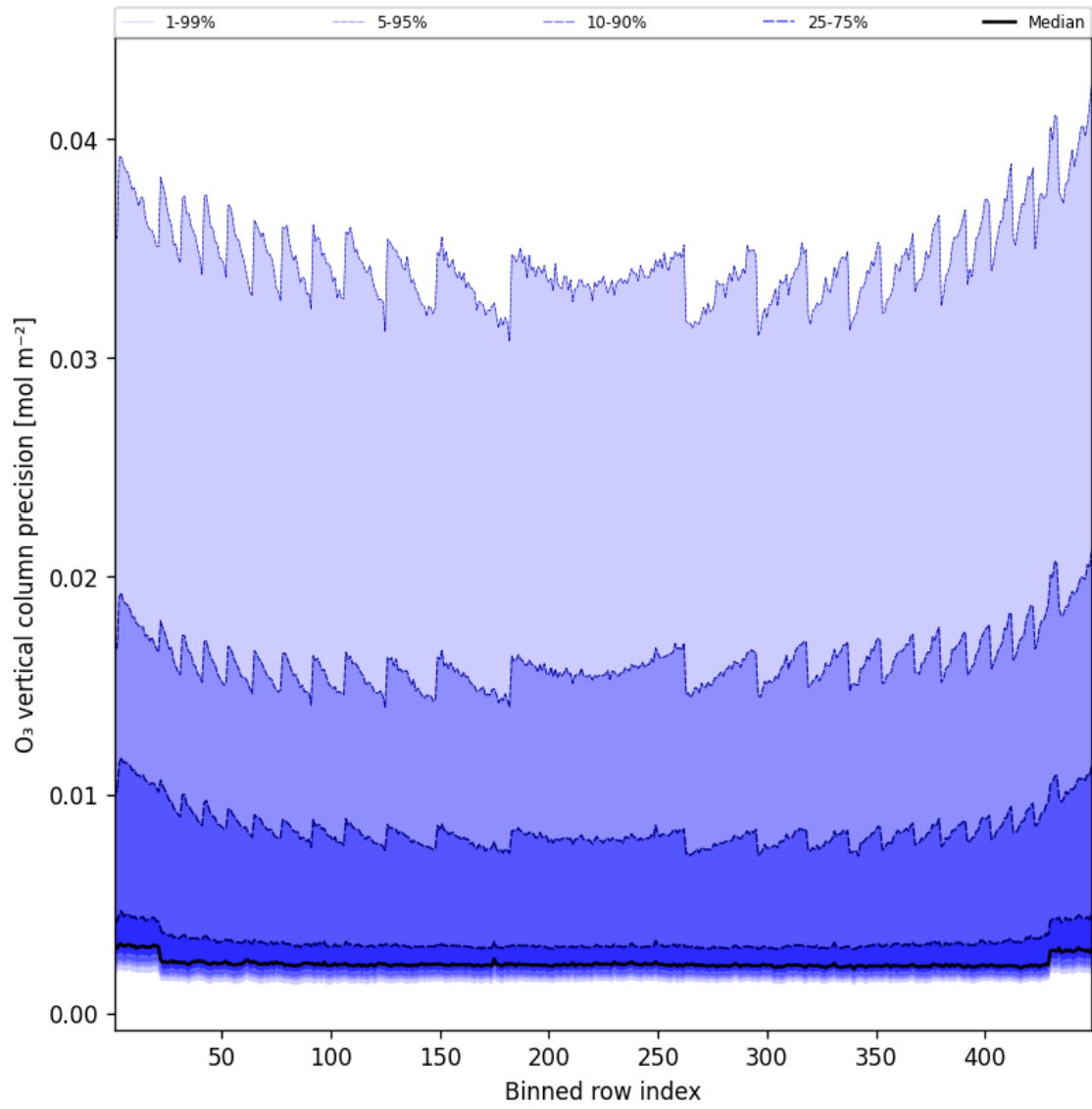
Figure 42: Along track statistics of “O 3 vertical column precision” for 2025-03-12 to 2025-03-13
