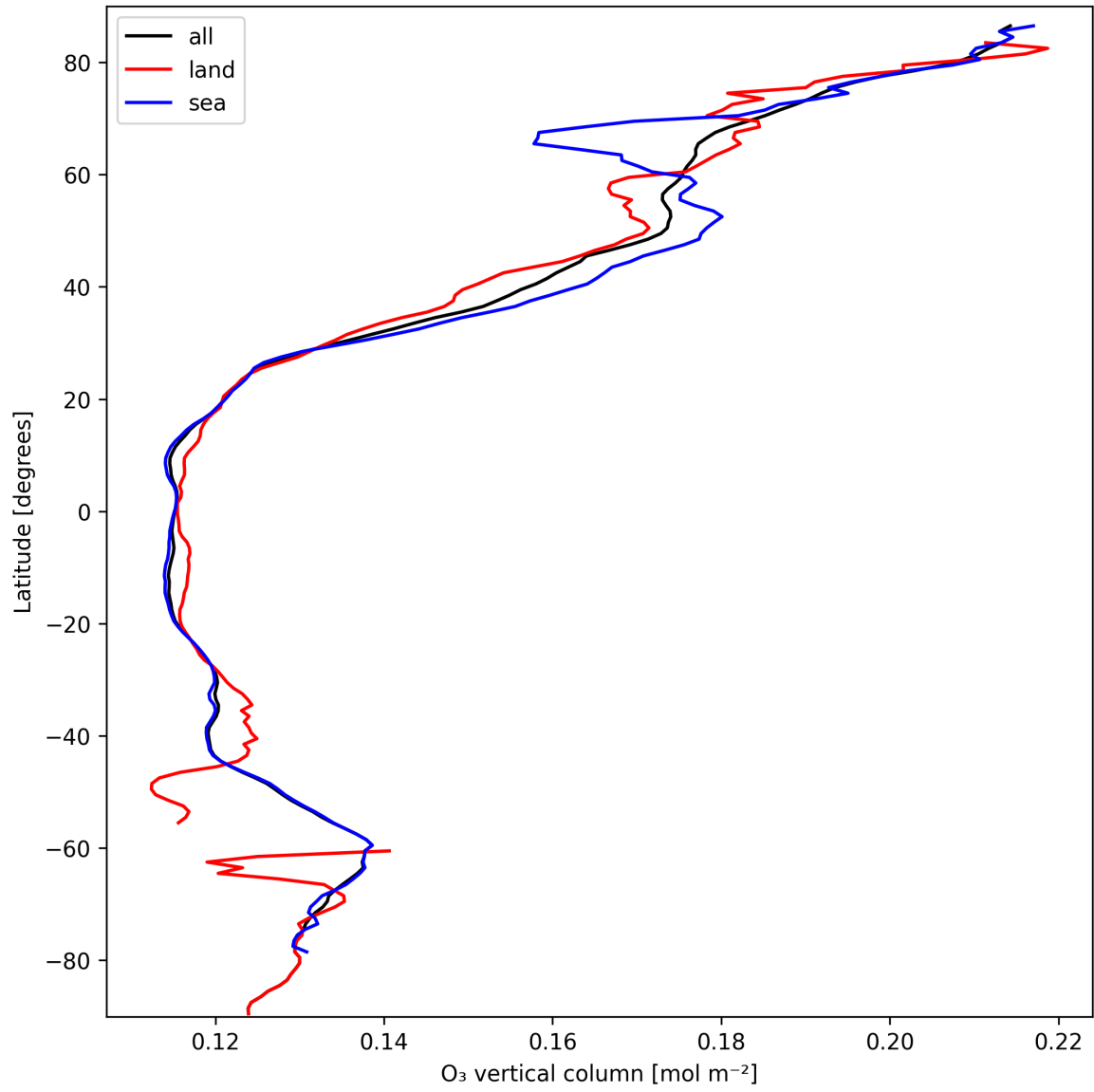
Figure 17: Zonal average of “O 3 vertical column” for 2025-03-12 to 2025-03-13.
