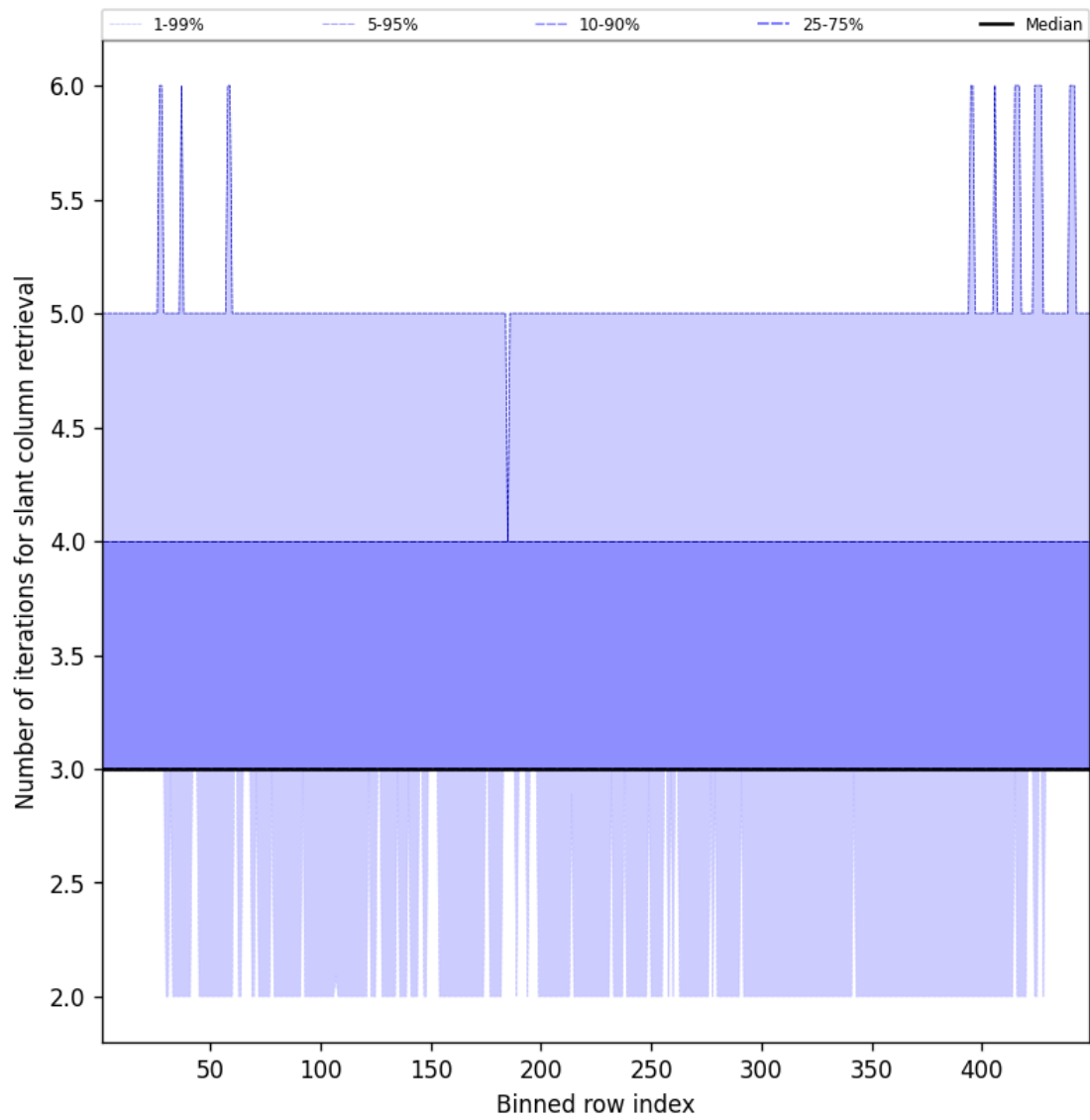
Figure 45: Along track statistics of “Number of iterations for slant column retrieval” for 2025-03-12 to 2025-03-13
