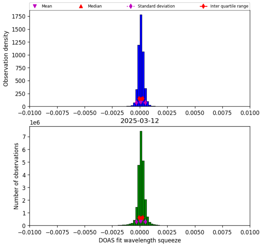
Figure 36: Histogram of “DOAS fit wavelength squeeze” for 2025-03-12 to 2025-03-13
