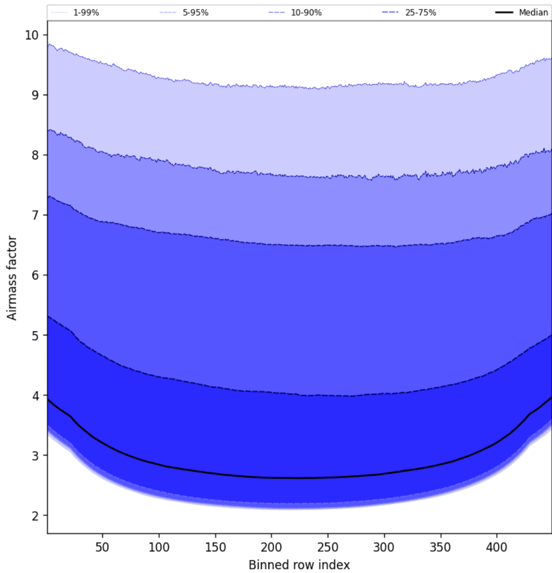
Figure 49: Along track statistics of “Airmass factor” for 2025-03-12 to 2025-03-13
