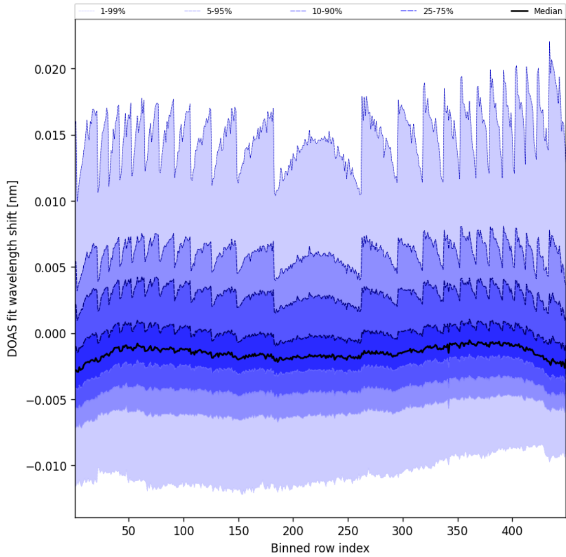
Figure 47: Along track statistics of “DOAS fit wavelength shift” for 2025-03-12 to 2025-03-13
