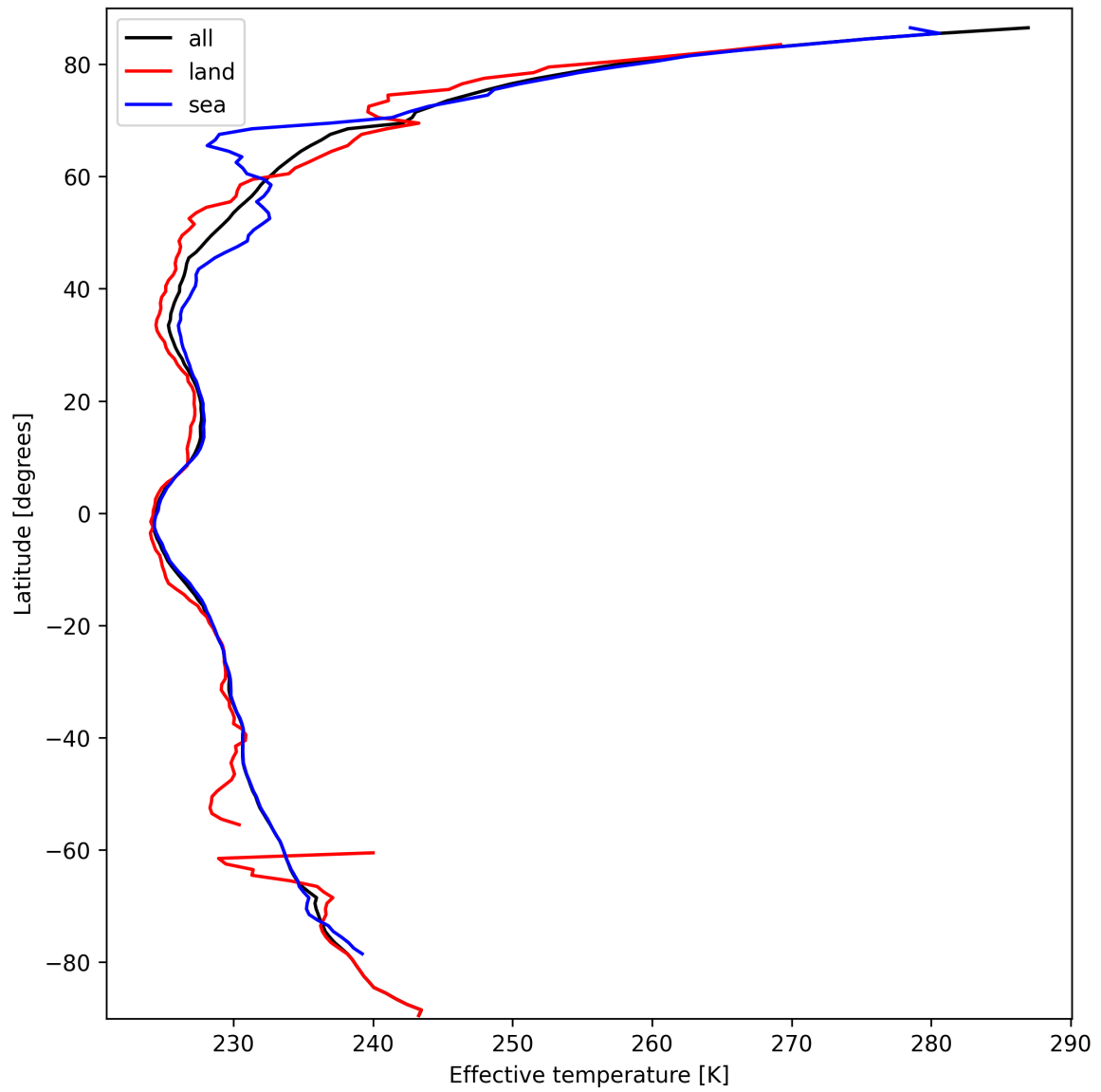
Figure 26: Zonal average of “Effective temperature” for 2025-03-12 to 2025-03-13.
