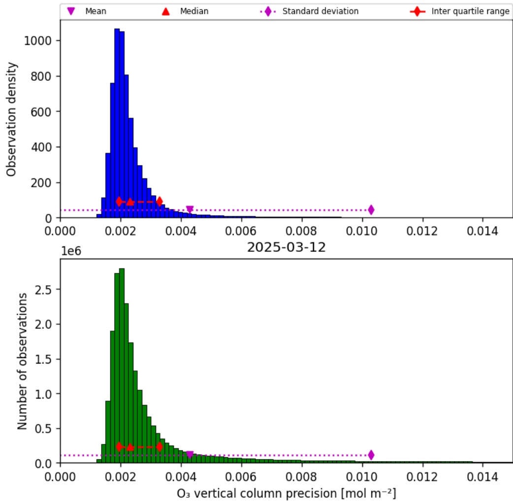
Figure 30: Histogram of “O 3 vertical column precision” for 2025-03-12 to 2025-03-13
