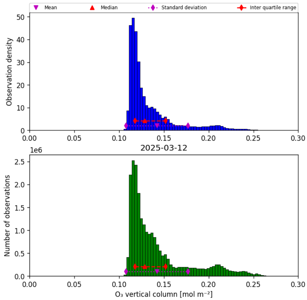
Figure 29: Histogram of “O 3 vertical column” for 2025-03-12 to 2025-03-13
