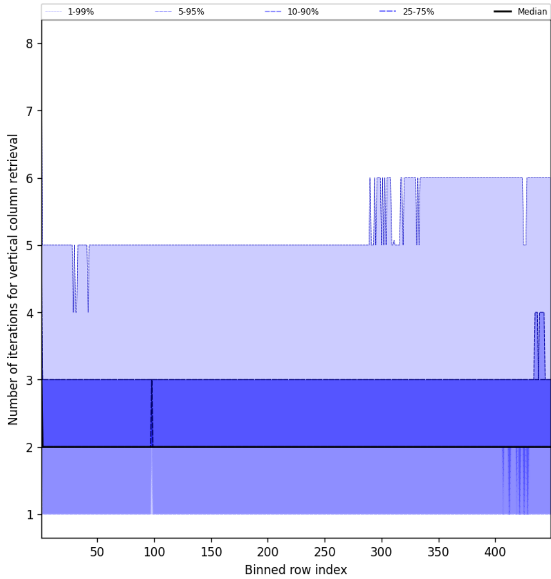
Figure 51: Along track statistics of “Number of iterations for vertical column retrieval” for 2025-03-12 to 2025-03-13
