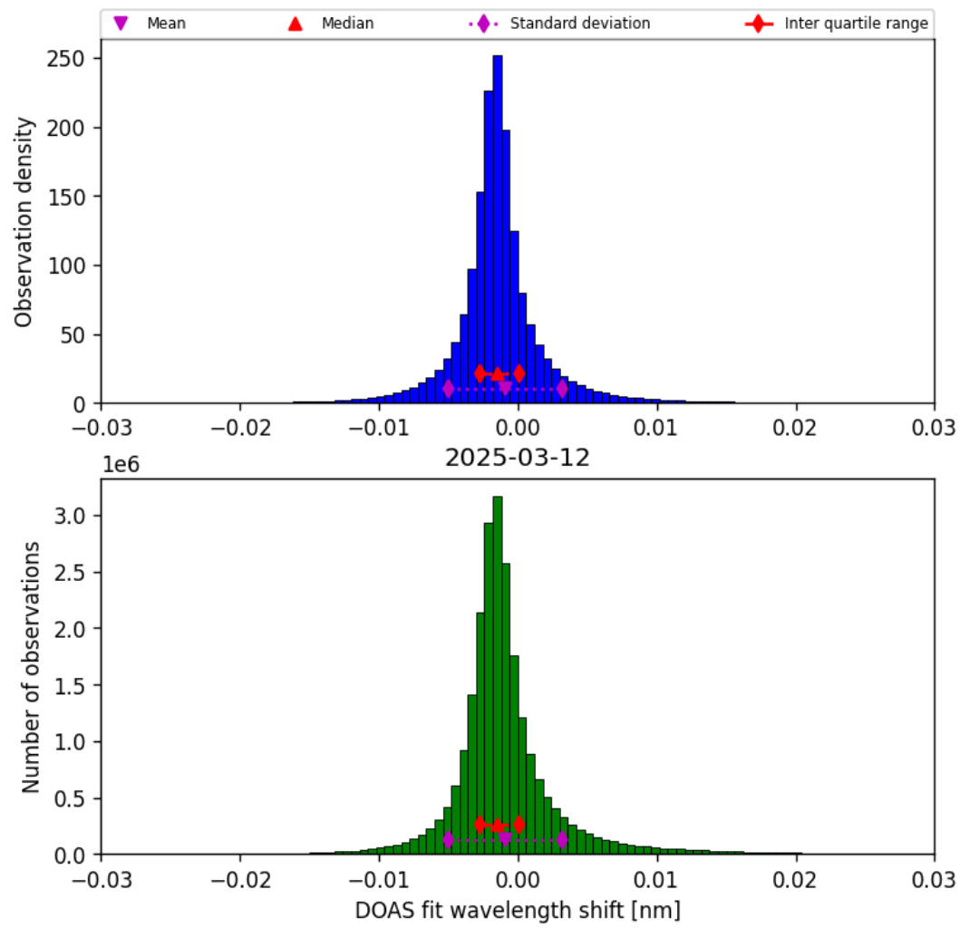
Figure 35: Histogram of “DOAS fit wavelength shift” for 2025-03-12 to 2025-03-13
