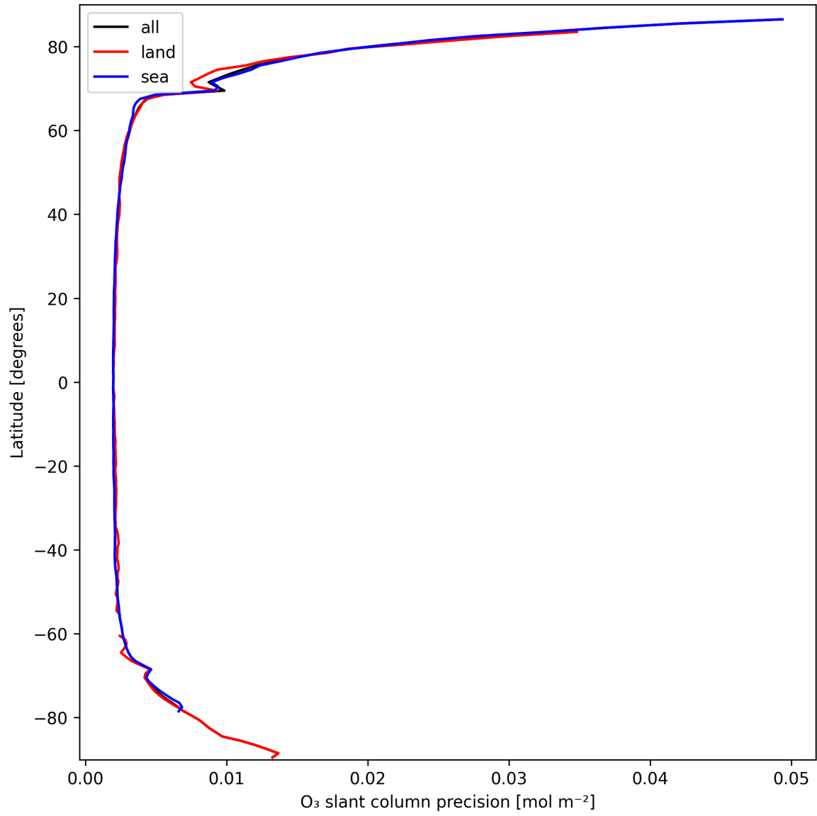
Figure 20: Zonal average of “O 3 slant column precision” for 2025-03-12 to 2025-03-13.
