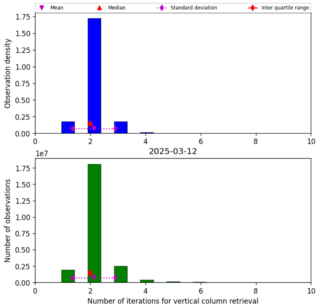
Figure 39: Histogram of “Number of iterations for vertical column retrieval” for 2025-03-12 to 2025-03-13
