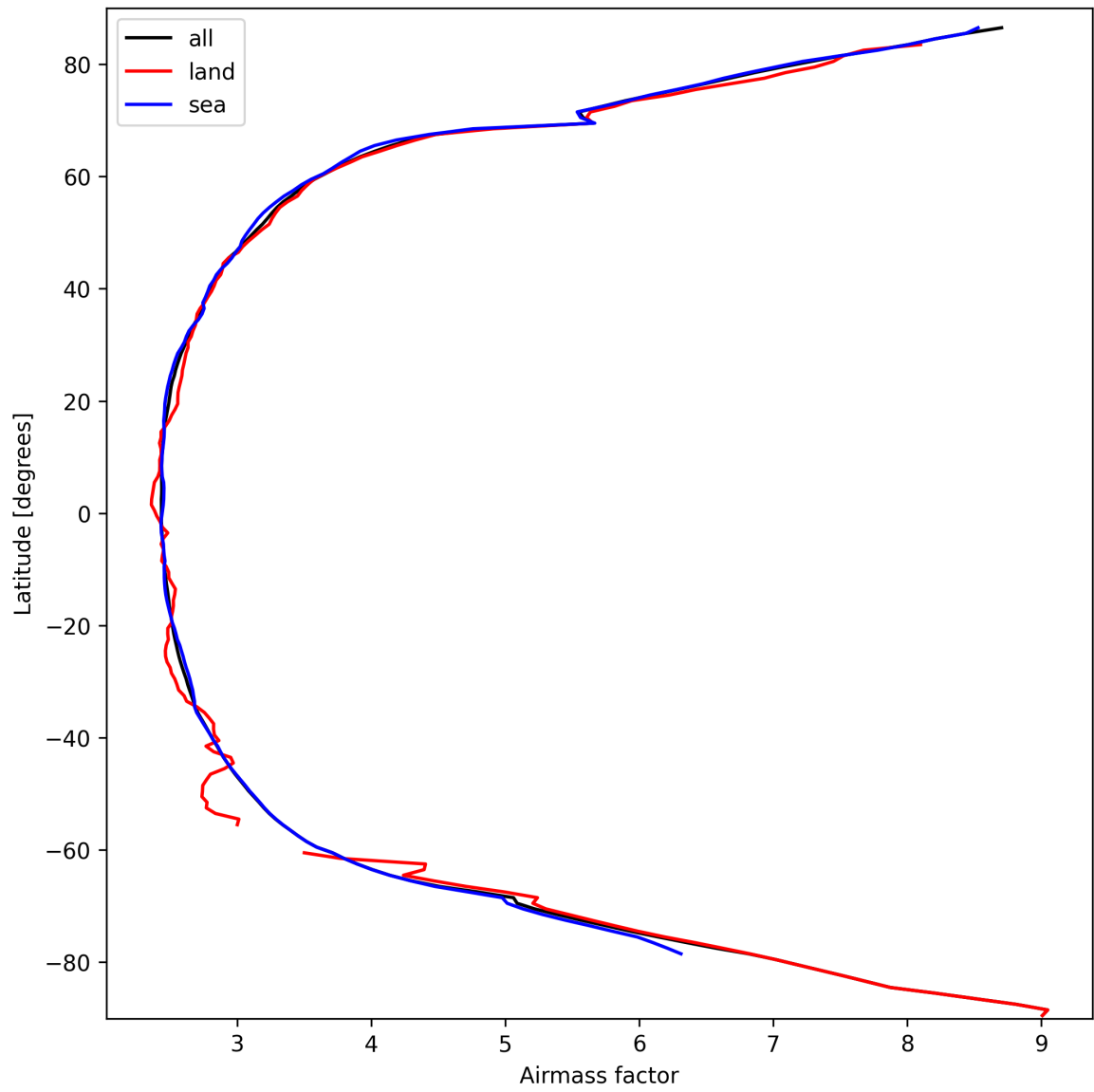
Figure 25: Zonal average of “Airmass factor” for 2025-03-12 to 2025-03-13.
