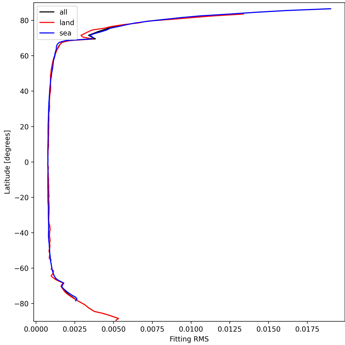
Figure 22: Zonal average of “Fitting RMS” for 2025-03-12 to 2025-03-13.
