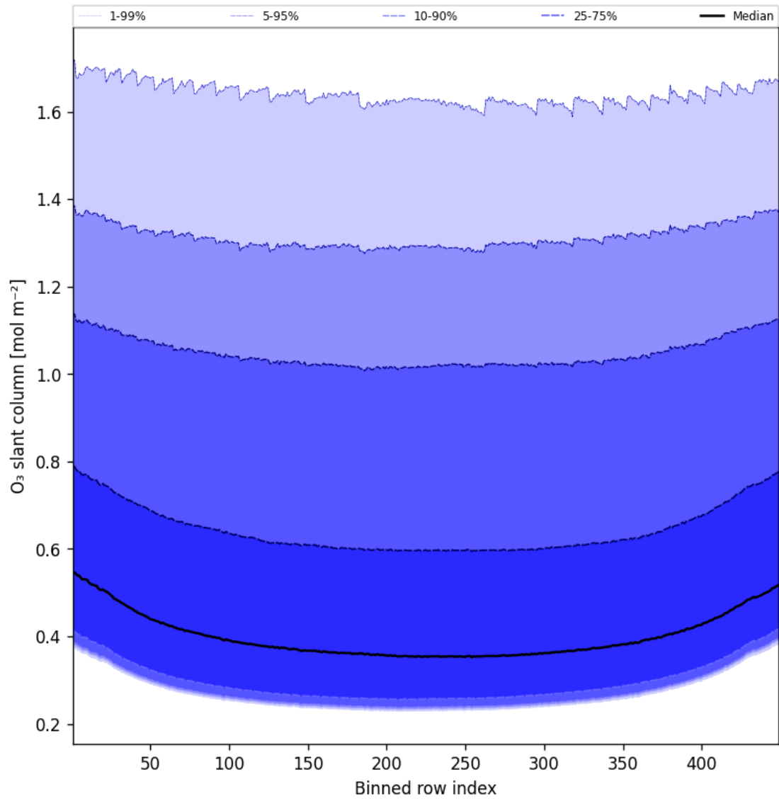
Figure 43: Along track statistics of “O 3 slant column” for 2025-03-12 to 2025-03-13
