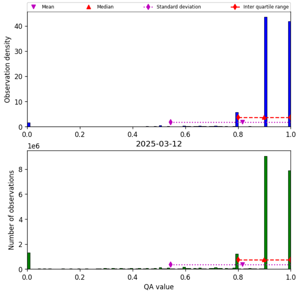
Figure 28: Histogram of “QA value” for 2025-03-12 to 2025-03-13
