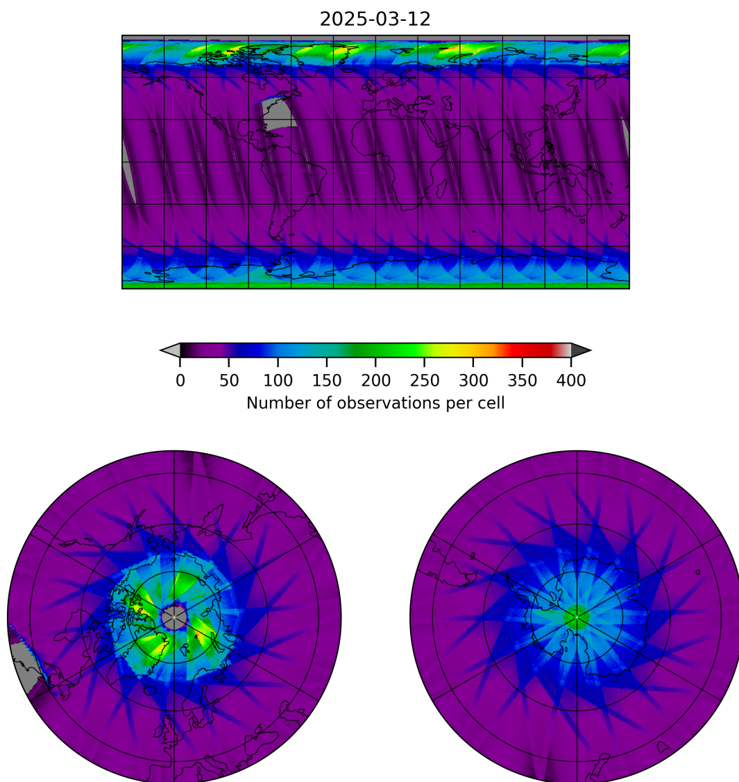
Figure 15: Map of the number of observations for 2025-03-12 to 2025-03-13
