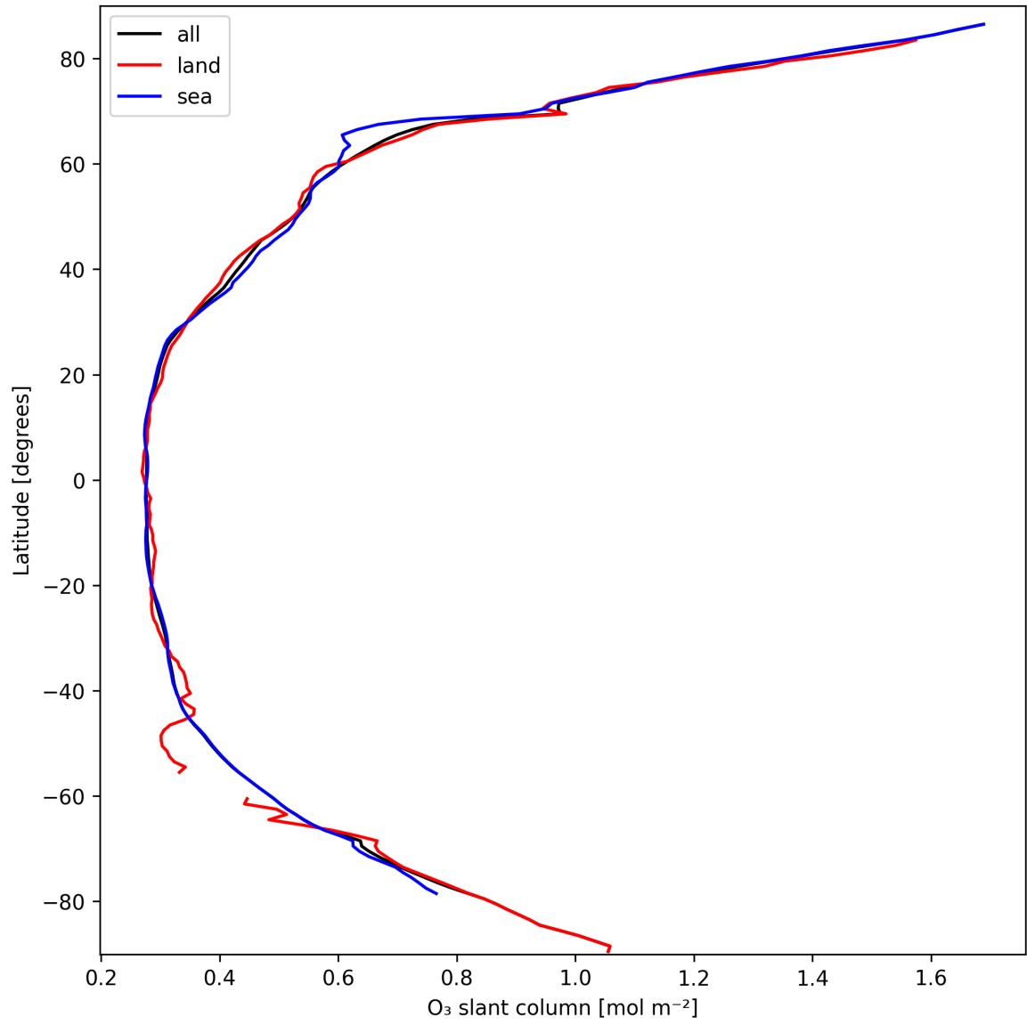
Figure 19: Zonal average of “O 3 slant column” for 2025-03-12 to 2025-03-13.
