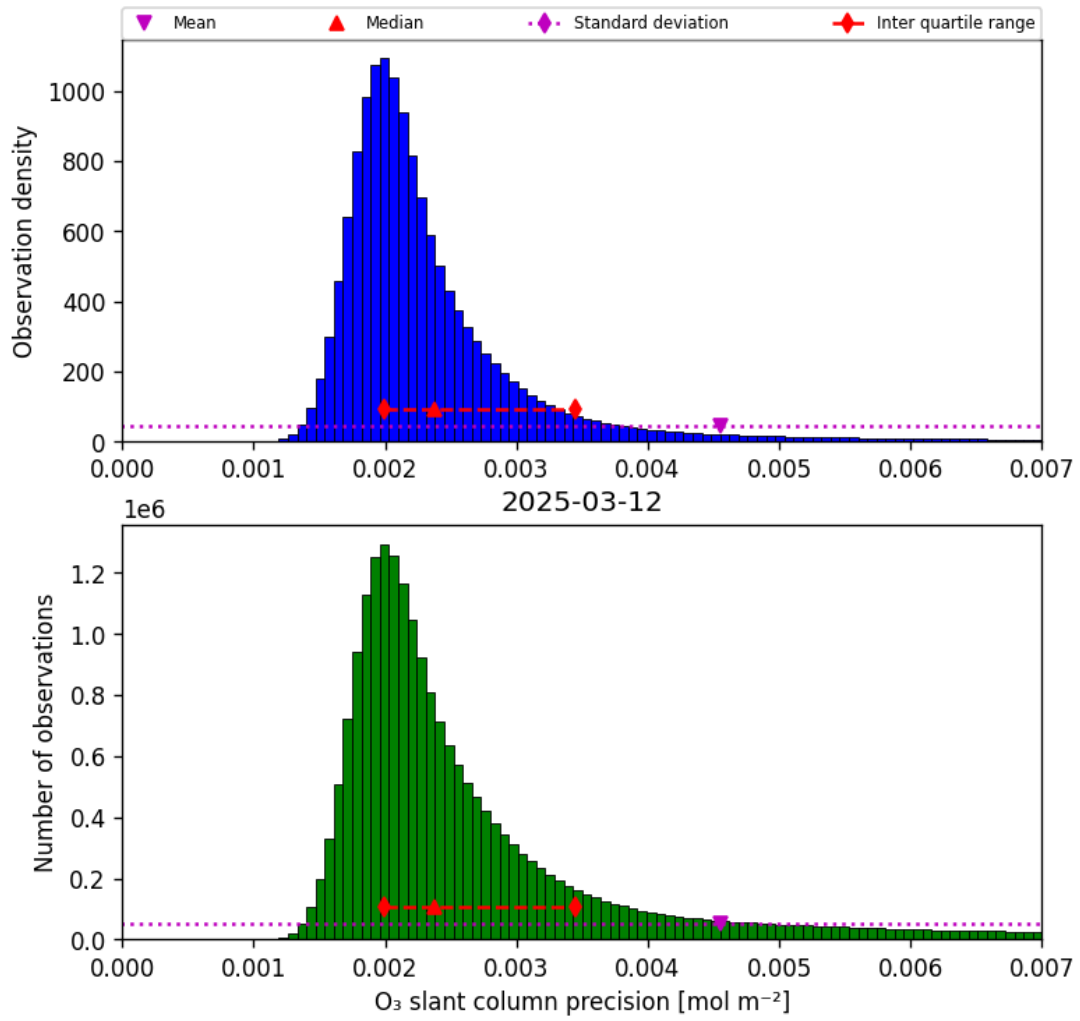
Figure 32: Histogram of “O 3 slant column precision” for 2025-03-12 to 2025-03-13
