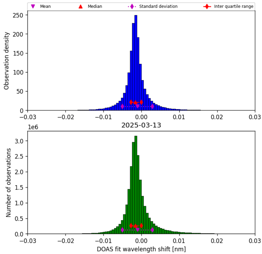
Figure 35: Histogram of “DOAS fit wavelength shift” for 2025-03-13 to 2025-03-14
