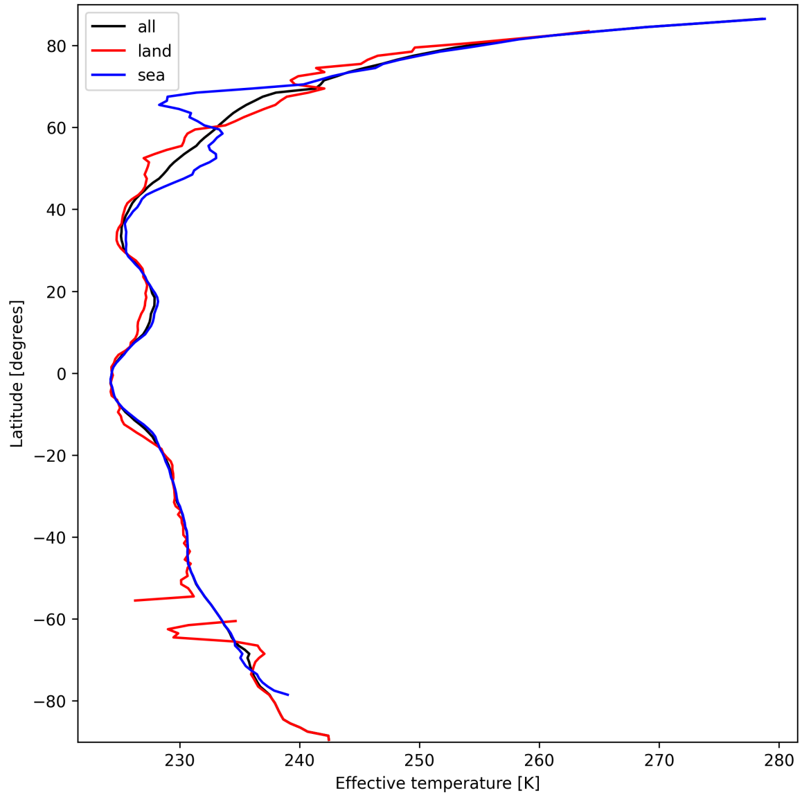
Figure 26: Zonal average of "Effective temperature" for 2025-03-13 to 2025-03-14.
