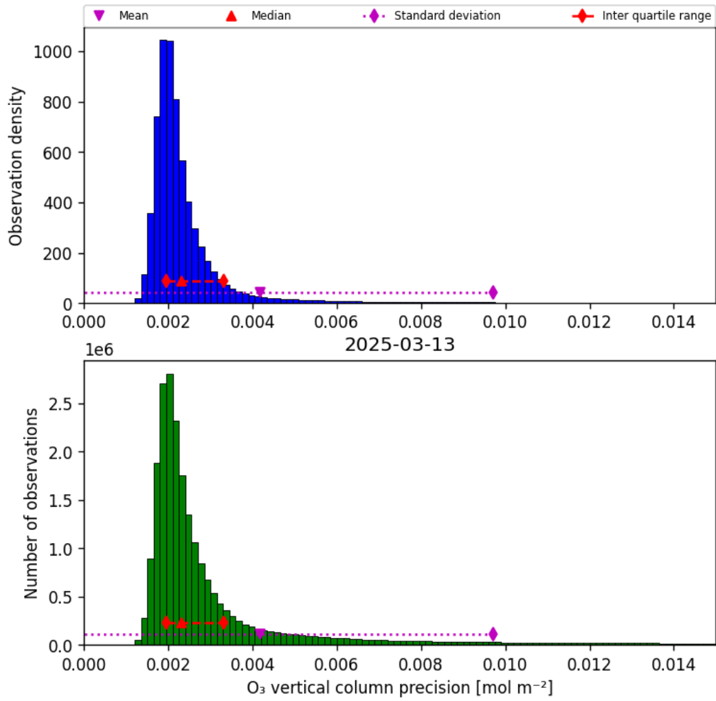
Figure 30: Histogram of “O 3 vertical column precision” for 2025-03-13 to 2025-03-14
