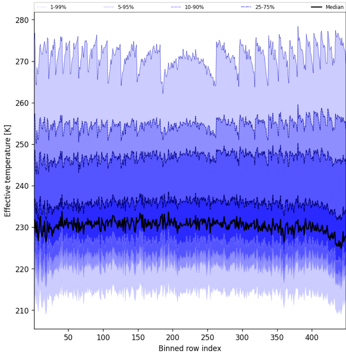
Figure 50: Along track statistics of “Effective temperature” for 2025-03-13 to 2025-03-14
