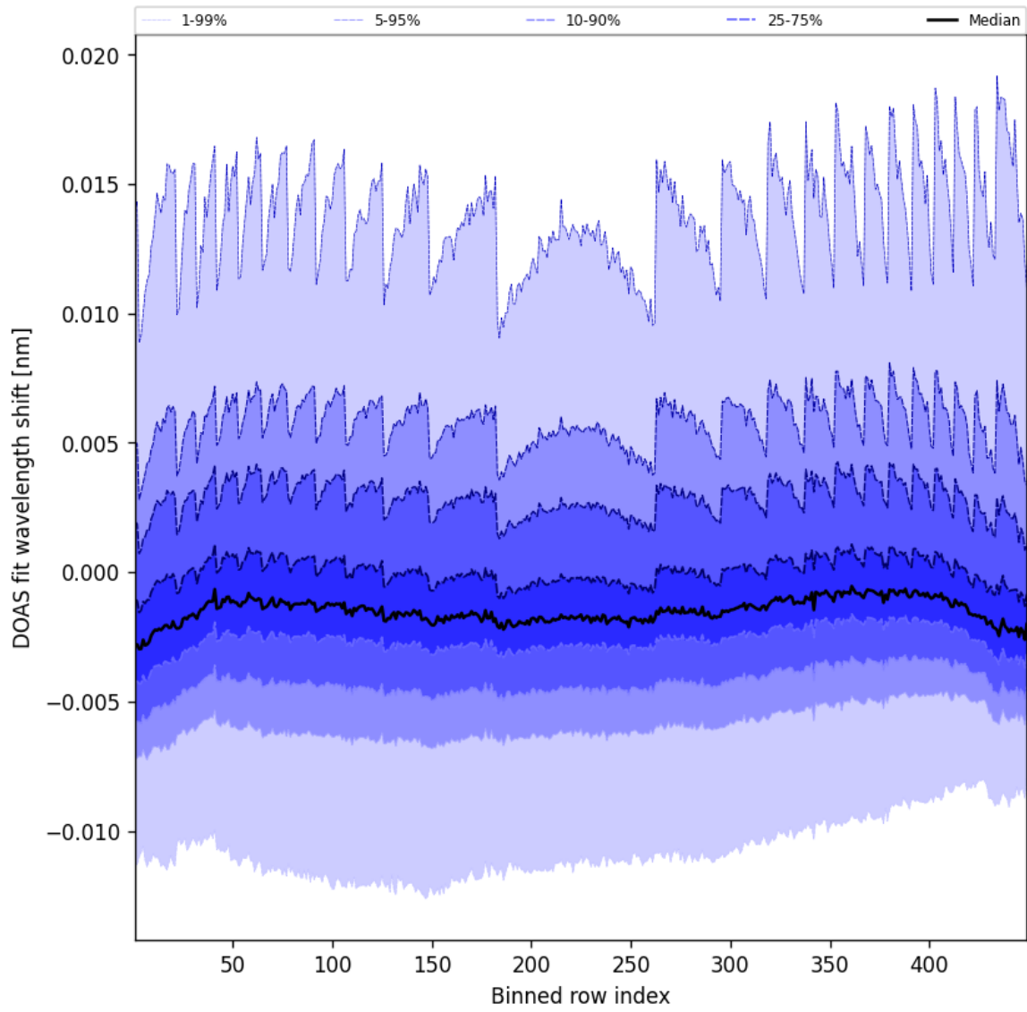
Figure 47: Along track statistics of “DOAS fit wavelength shift” for 2025-03-13 to 2025-03-14
