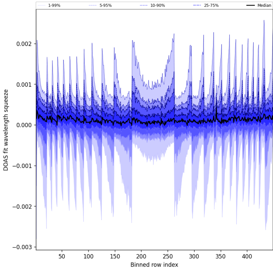
Figure 48: Along track statistics of “DOAS fit wavelength squeeze” for 2025-03-13 to 2025-03-14
