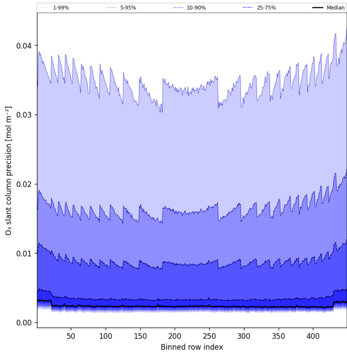
Figure 44: Along track statistics of “O 3 slant column precision” for 2025-03-13 to 2025-03-14
