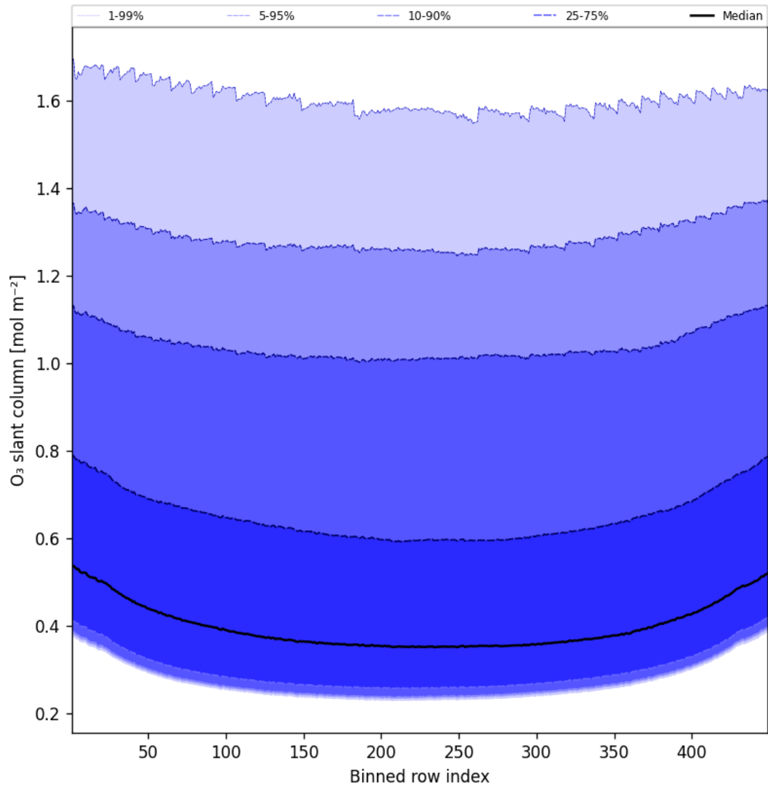
Figure 43: Along track statistics of “O 3 slant column” for 2025-03-13 to 2025-03-14
