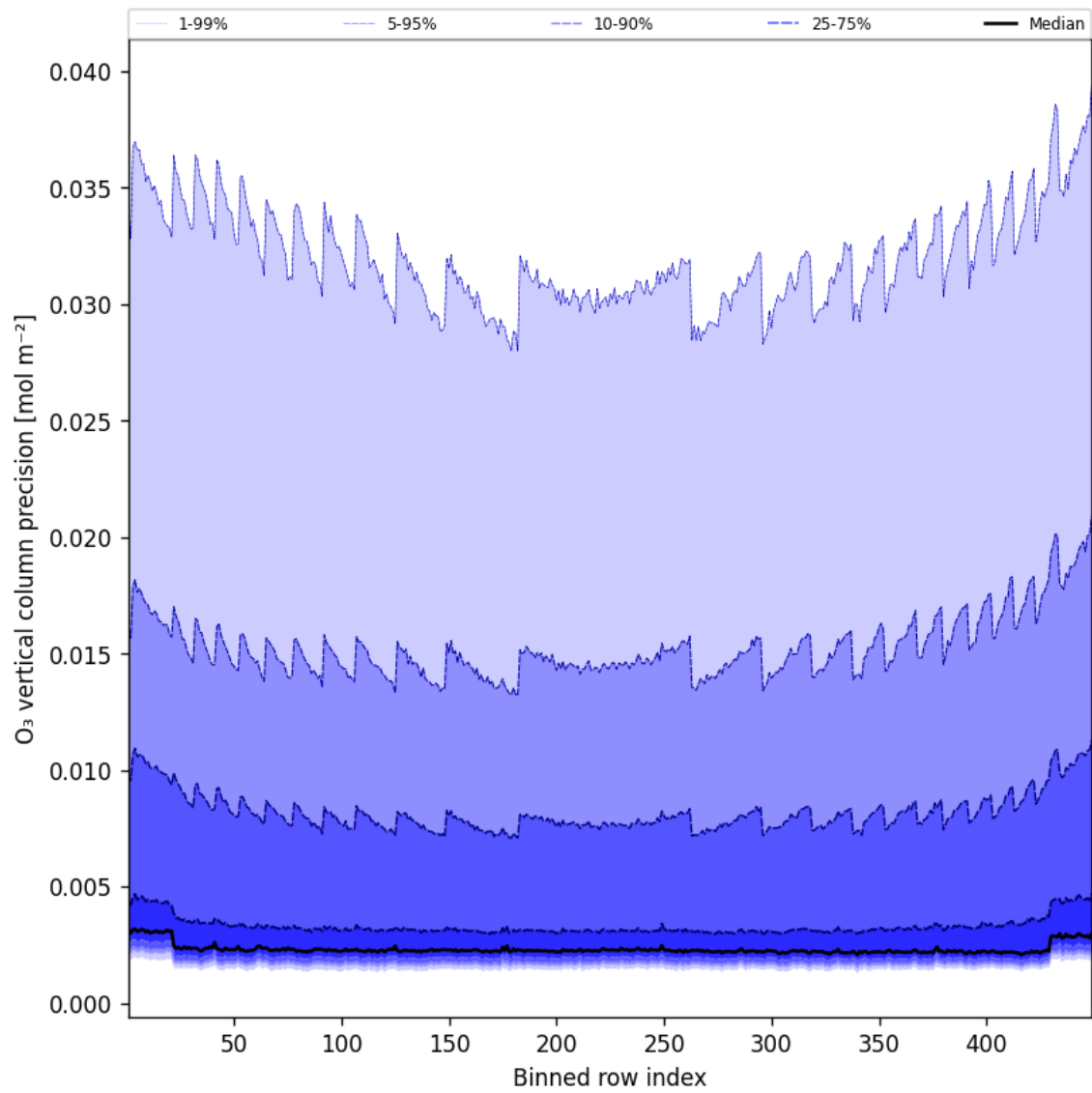
Figure 42: Along track statistics of “O 3 vertical column precision” for 2025-03-13 to 2025-03-14
