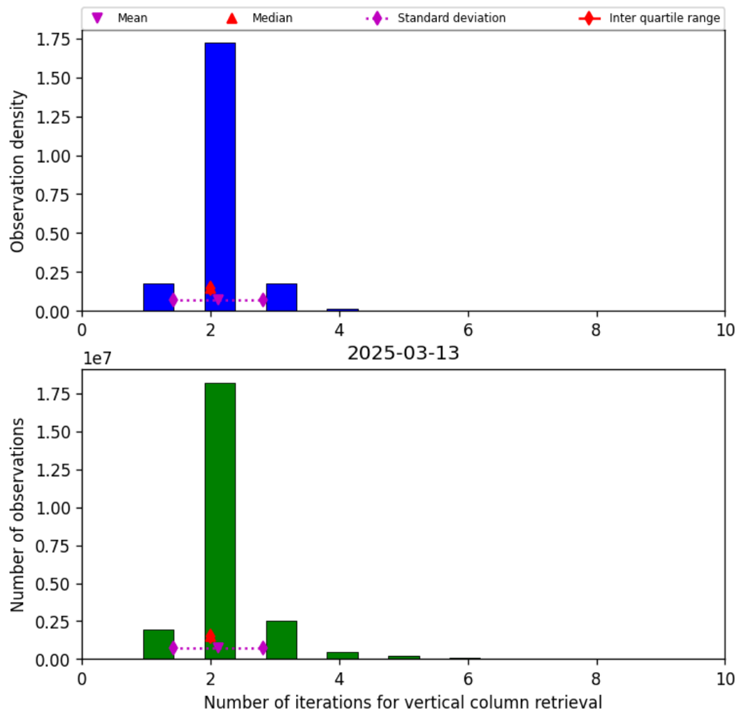
Figure 39: Histogram of “Number of iterations for vertical column retrieval” for 2025-03-13 to 2025-03-14
