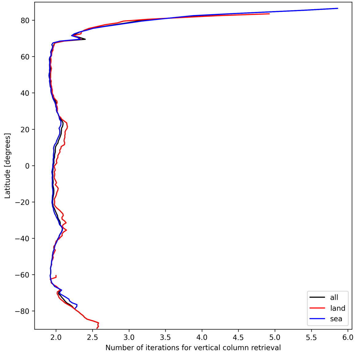
Figure 27: Zonal average of “Number of iterations for vertical column retrieval” for 2025-03-13 to 2025-03-14.
