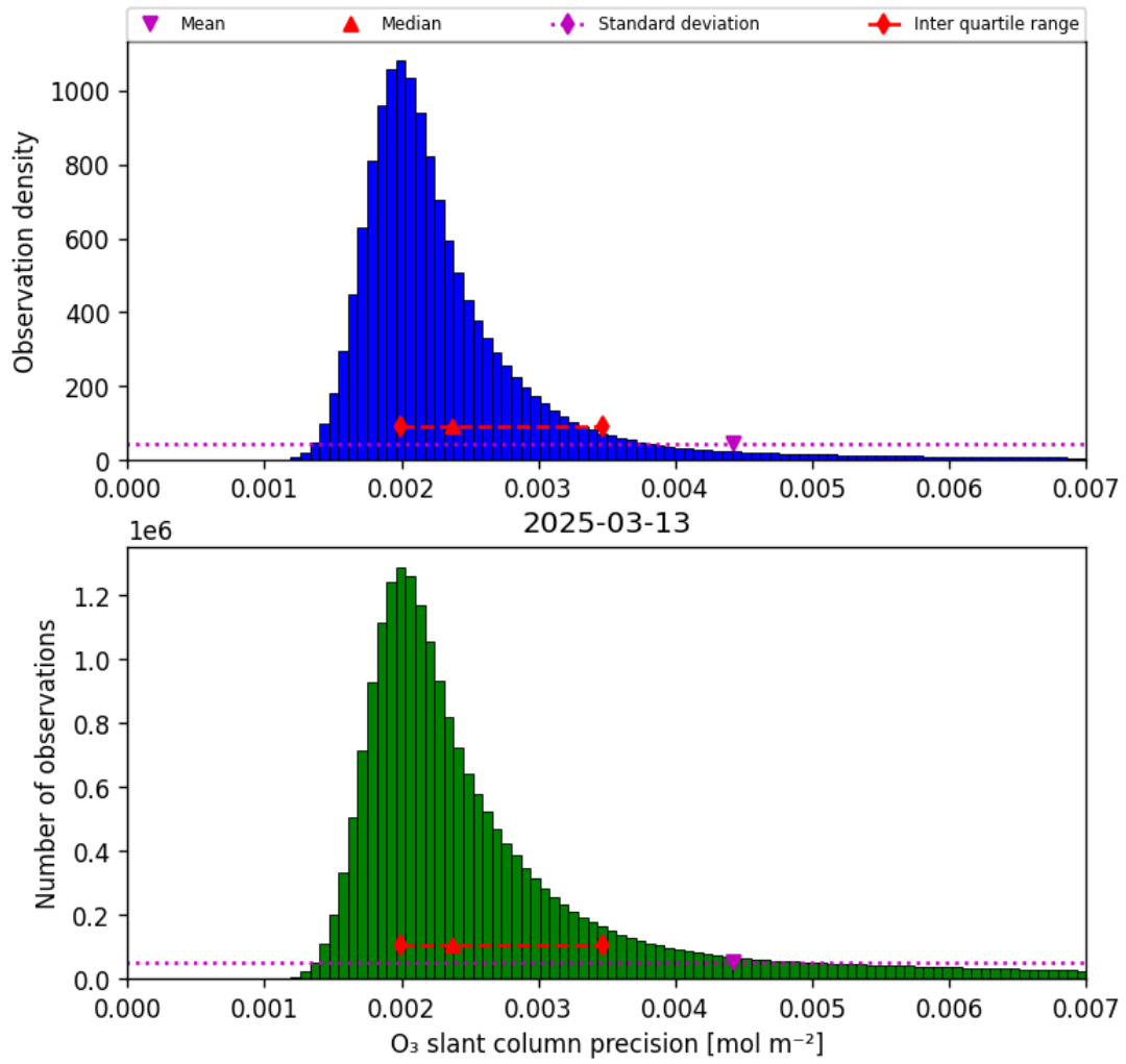
Figure 32: Histogram of “O 3 slant column precision” for 2025-03-13 to 2025-03-14
