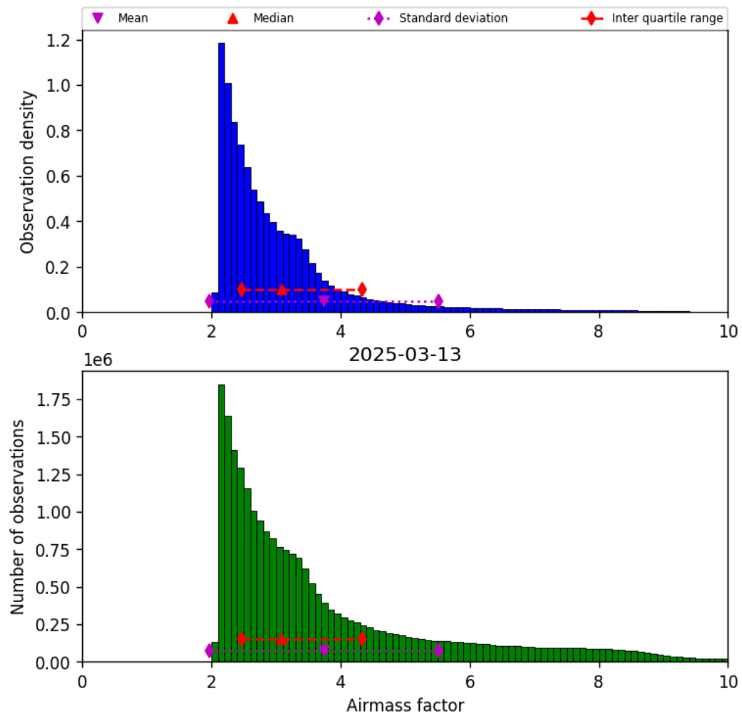
Figure 37: Histogram of “Airmass factor” for 2025-03-13 to 2025-03-14
