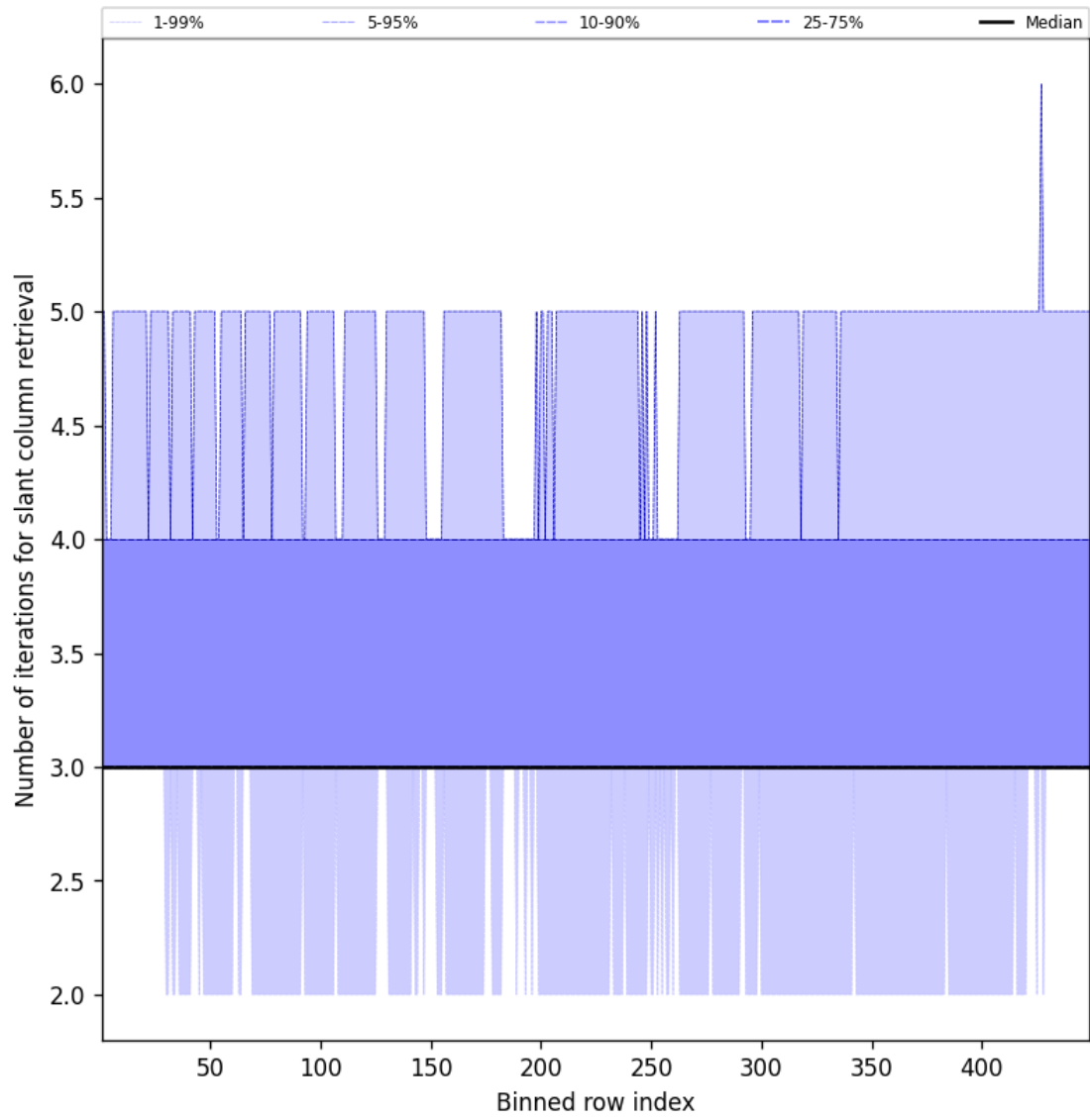
Figure 45: Along track statistics of “Number of iterations for slant column retrieval” for 2025-03-13 to 2025-03-14
