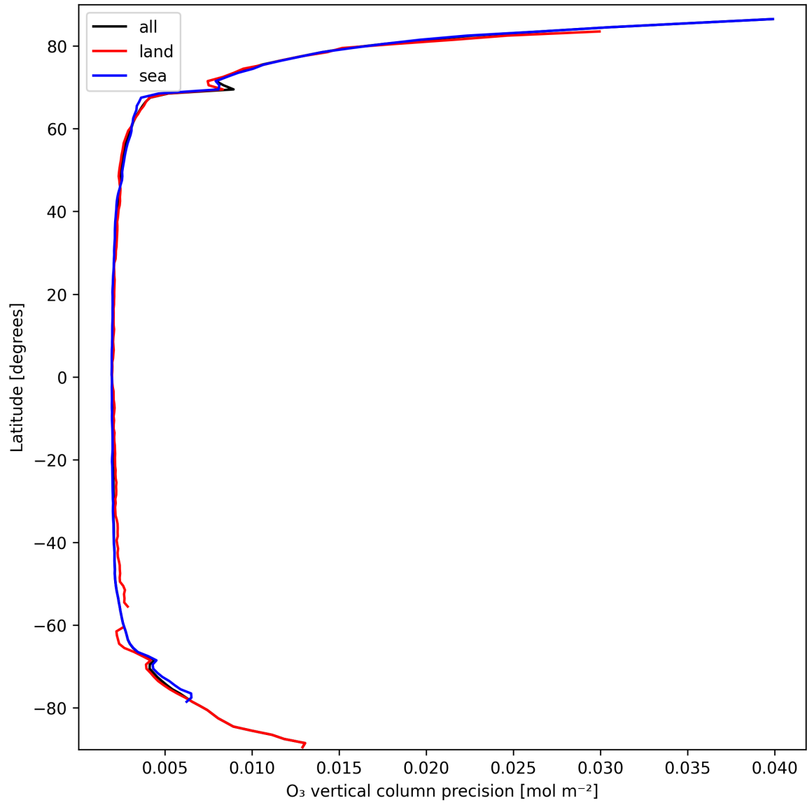
Figure 18: Zonal average of "O 3 vertical column precision" for 2025-03-13 to 2025-03-14.
