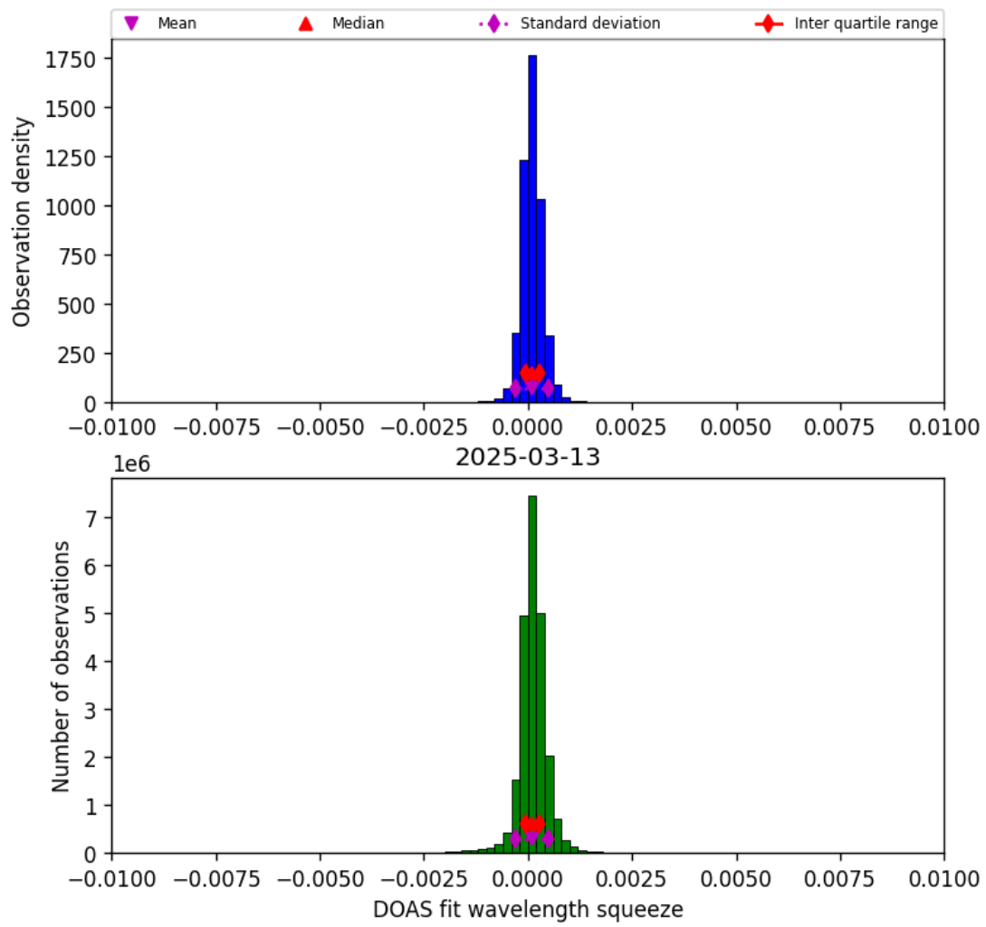
Figure 36: Histogram of “DOAS fit wavelength squeeze” for 2025-03-13 to 2025-03-14
