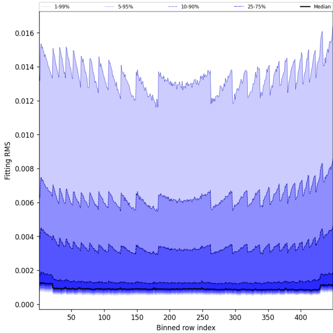
Figure 46: Along track statistics of “Fitting RMS” for 2025-03-13 to 2025-03-14
