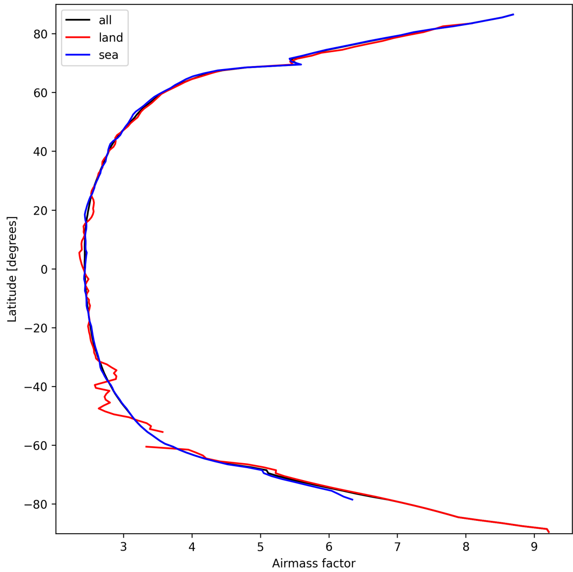
Figure 25: Zonal average of “Airmass factor” for 2025-03-13 to 2025-03-14.
