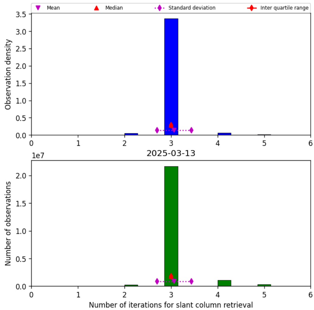
Figure 33: Histogram of “Number of iterations for slant column retrieval” for 2025-03-13 to 2025-03-14
