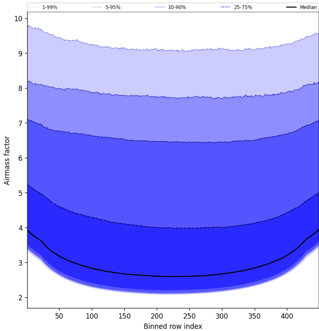
Figure 49: Along track statistics of “Airmass factor” for 2025-03-13 to 2025-03-14
