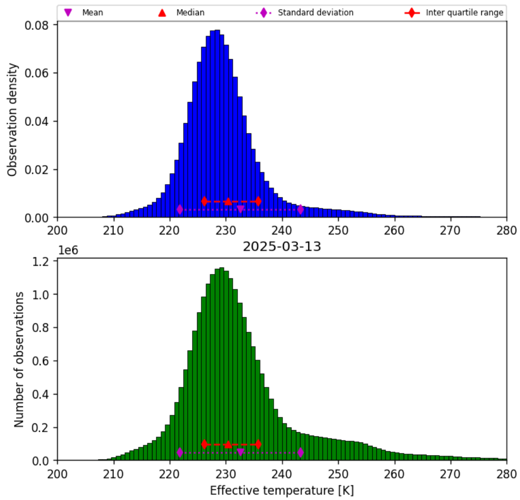
Figure 38: Histogram of “Effective temperature” for 2025-03-13 to 2025-03-14
