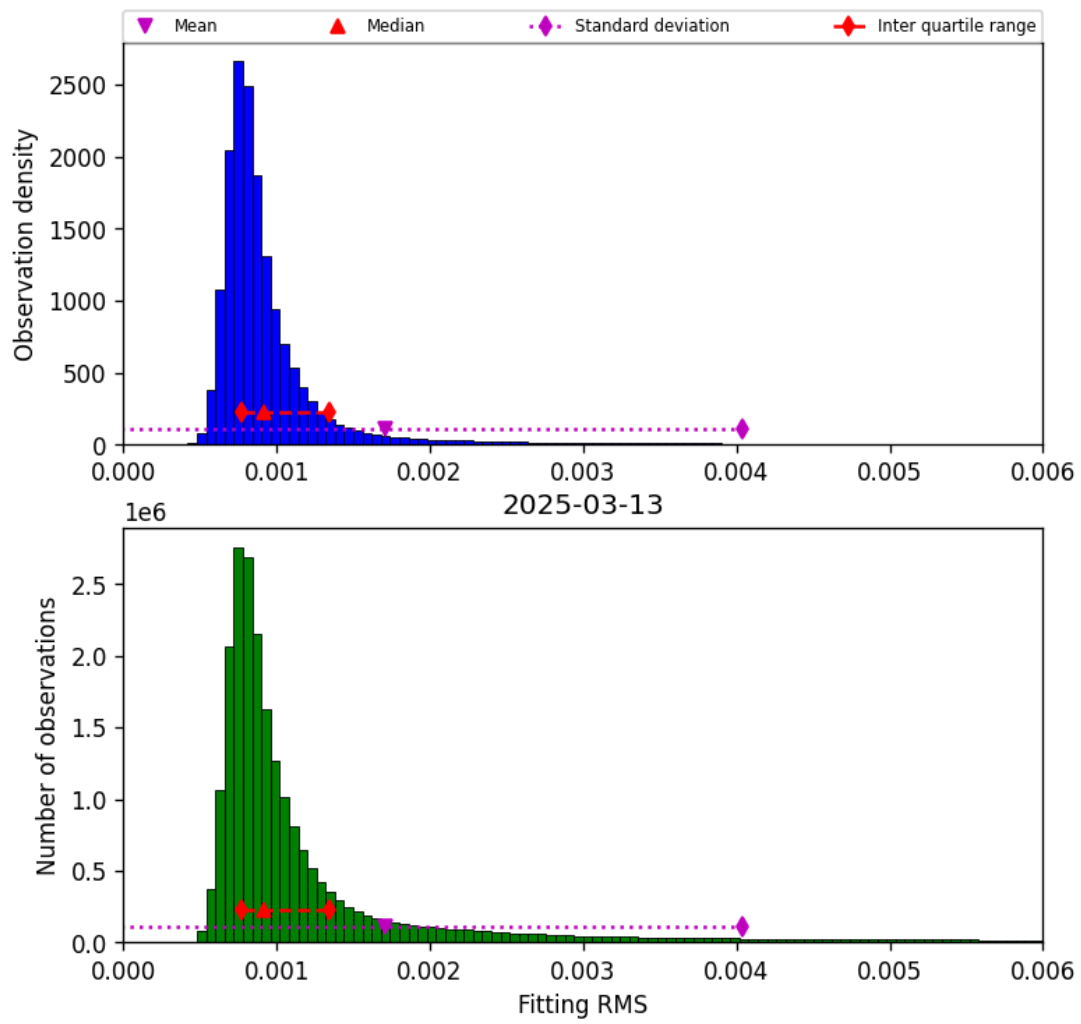
Figure 34: Histogram of “Fitting RMS” for 2025-03-13 to 2025-03-14
