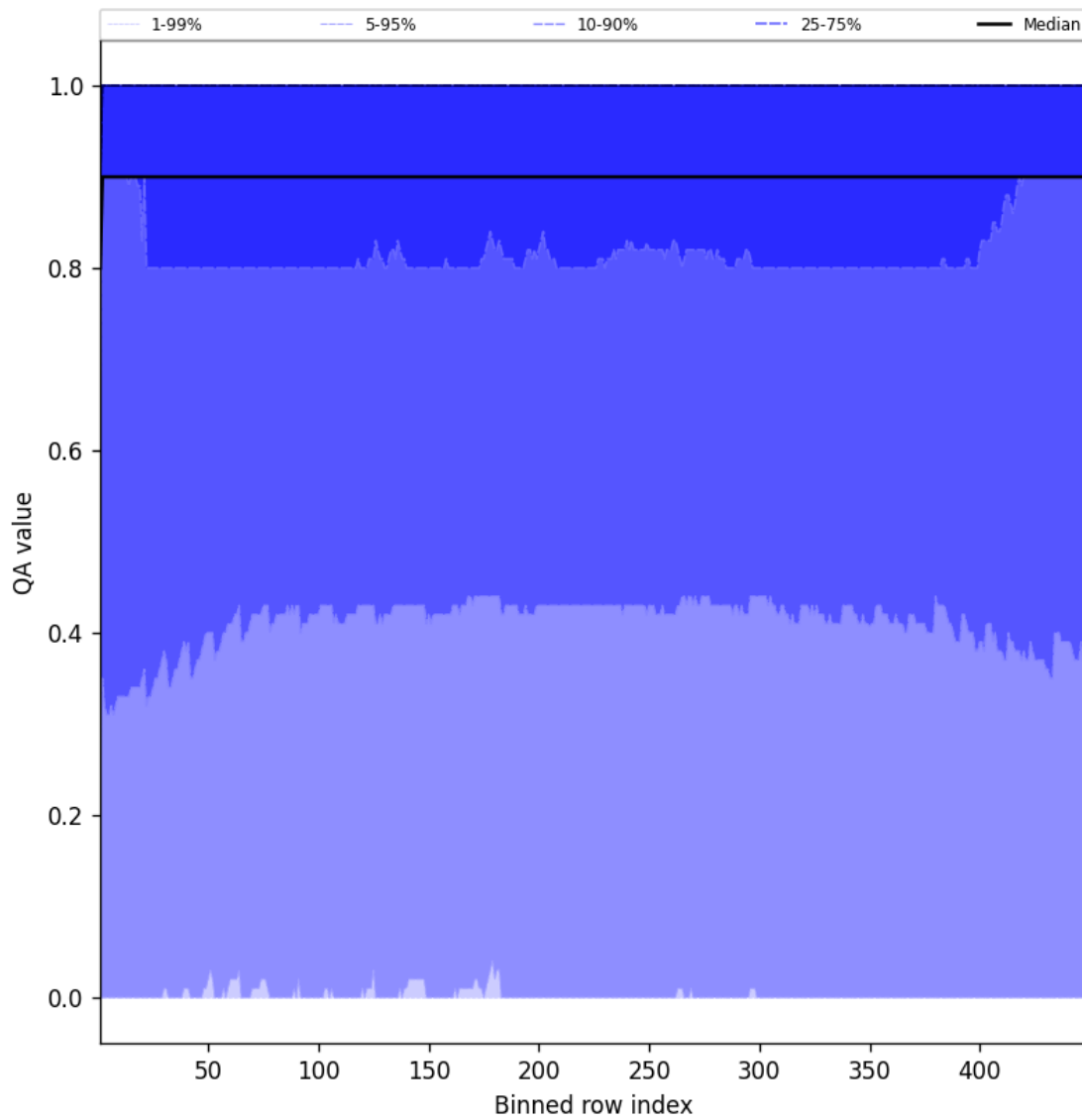
Figure 40: Along track statistics of “QA value” for 2025-03-13 to 2025-03-14
