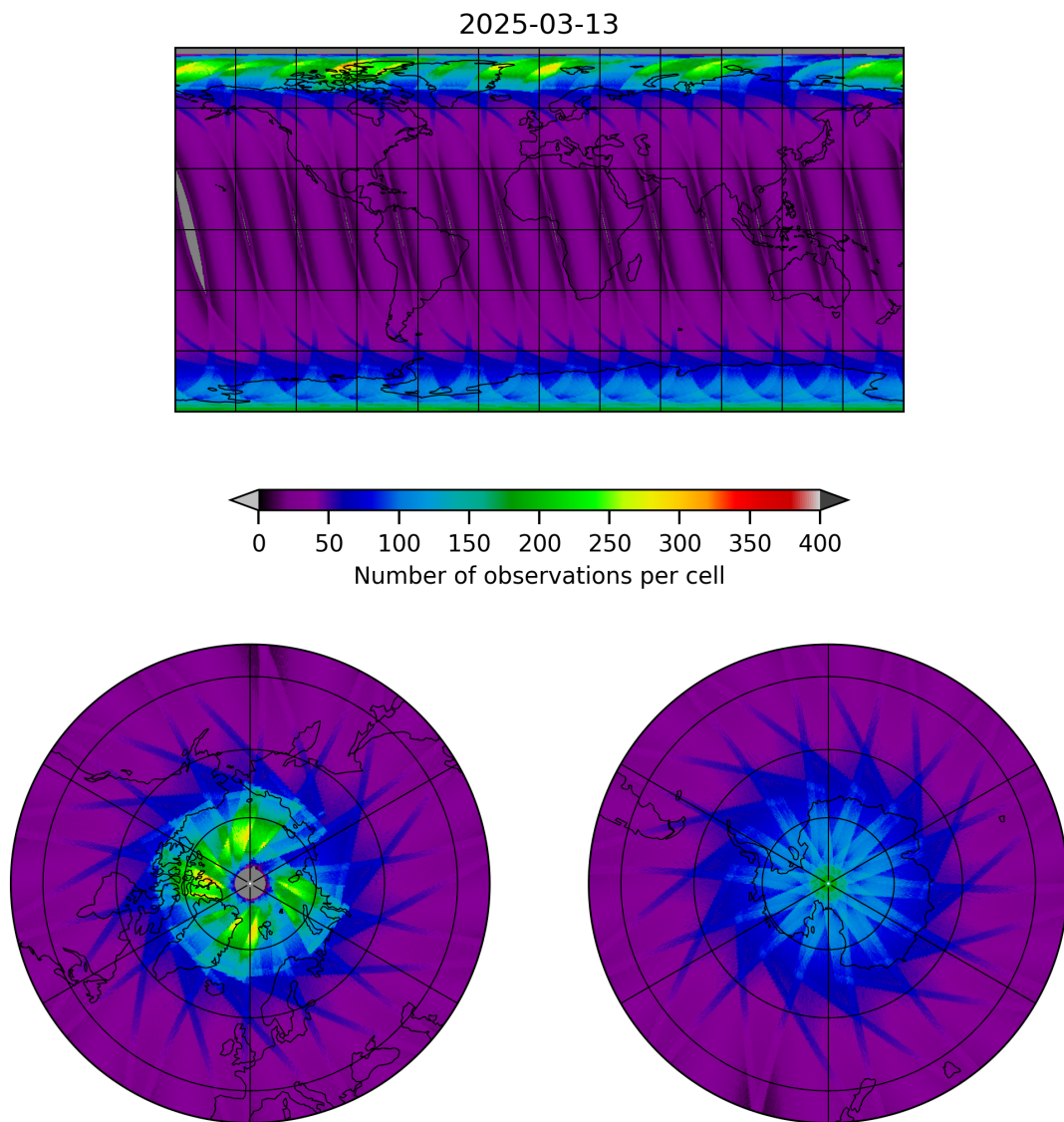
Figure 15: Map of the number of observations for 2025-03-13 to 2025-03-14
