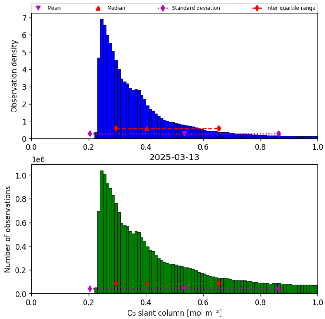
Figure 31: Histogram of “O 3 slant column” for 2025-03-13 to 2025-03-14
