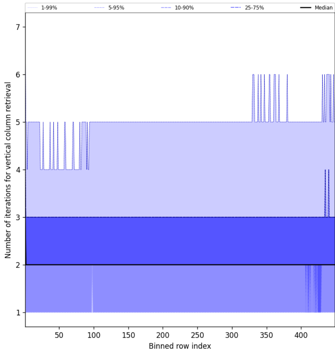
Figure 51: Along track statistics of “Number of iterations for vertical column retrieval” for 2025-03-13 to 2025-03-14
