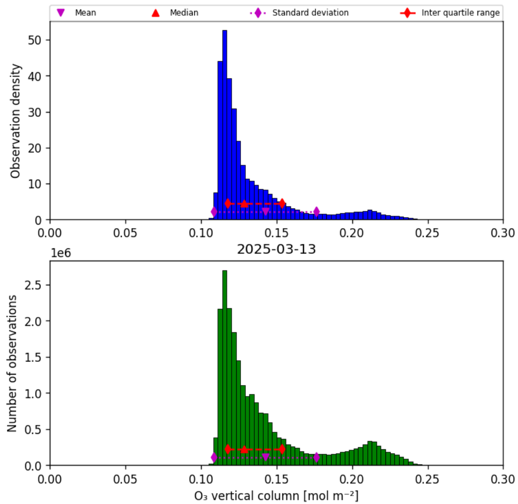
Figure 29: Histogram of “O 3 vertical column” for 2025-03-13 to 2025-03-14
