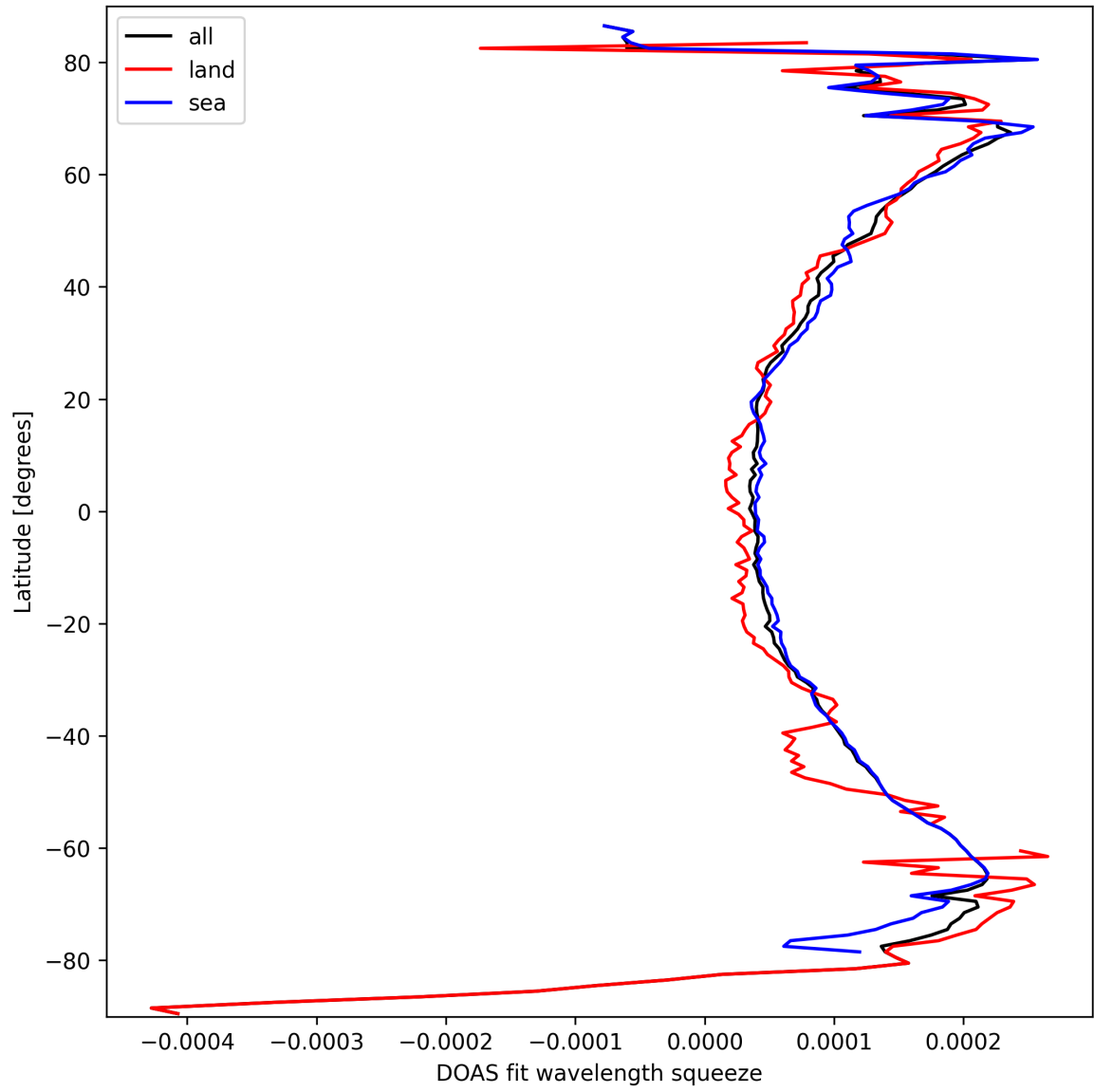
Figure 24: Zonal average of “DOAS fit wavelength squeeze” for 2025-03-13 to 2025-03-14.
