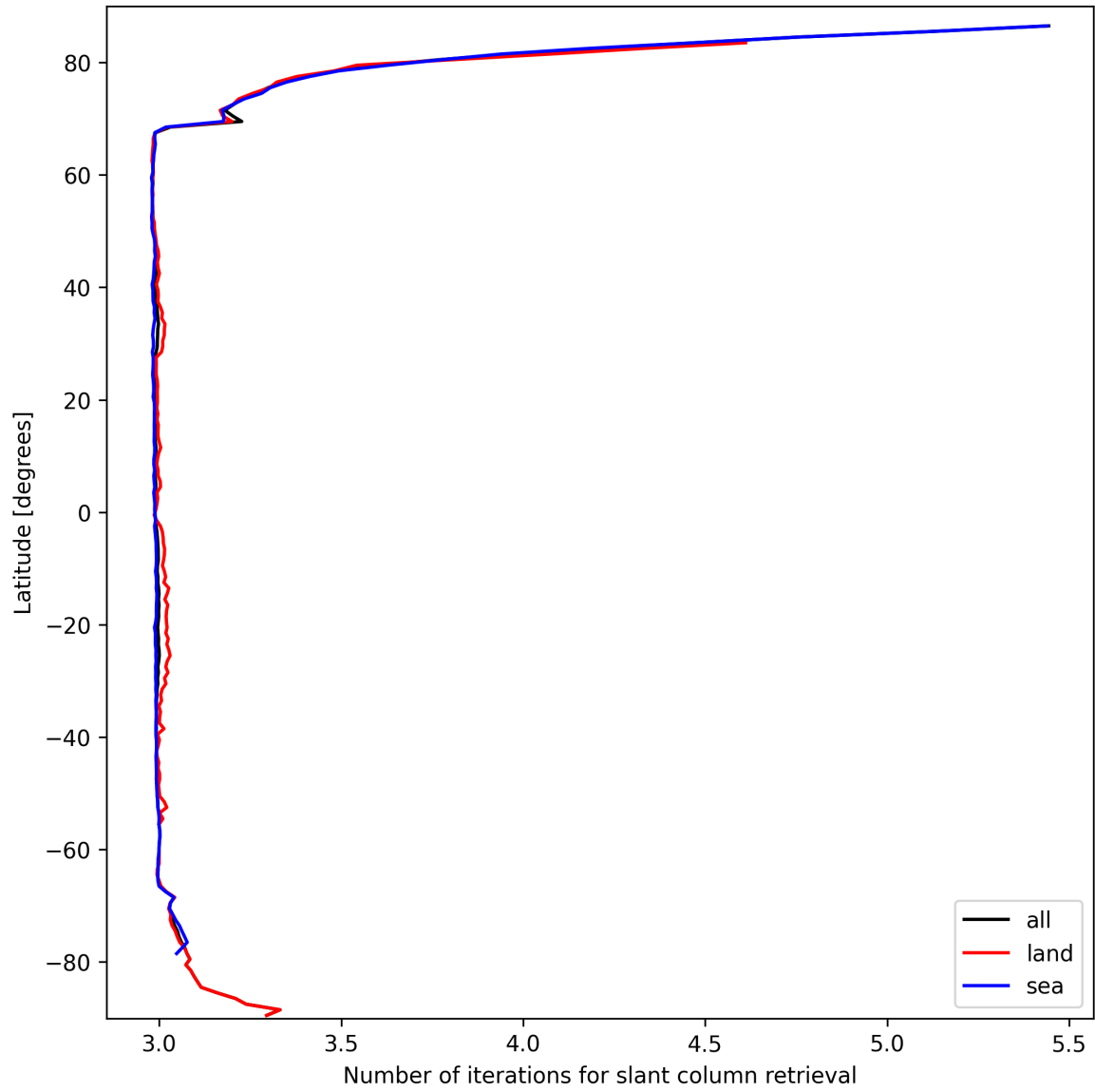
Figure 21: Zonal average of “Number of iterations for slant column retrieval” for 2025-03-13 to 2025-03-14.
