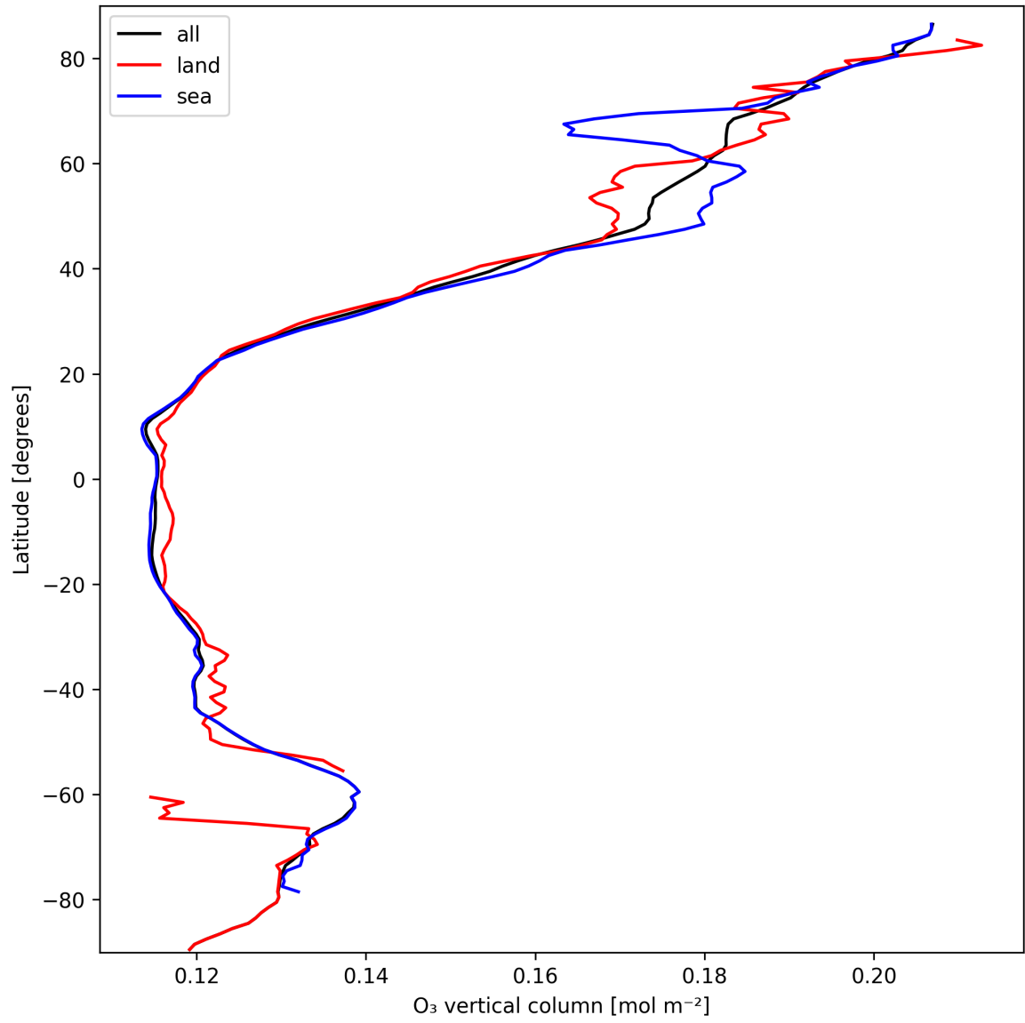
Figure 17: Zonal average of “O 3 vertical column” for 2025-03-13 to 2025-03-14.
