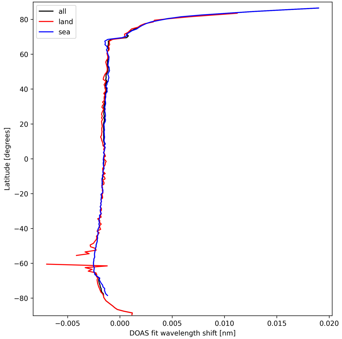
Figure 23: Zonal average of “DOAS fit wavelength shift” for 2025-03-13 to 2025-03-14.
