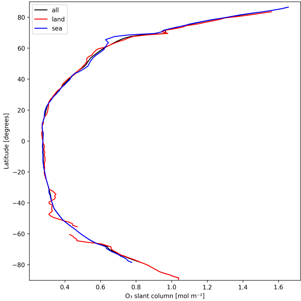
Figure 19: Zonal average of “O 3 slant column” for 2025-03-13 to 2025-03-14.
