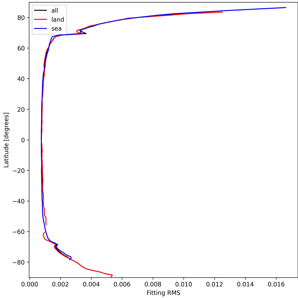
Figure 22: Zonal average of “Fitting RMS” for 2025-03-13 to 2025-03-14.
