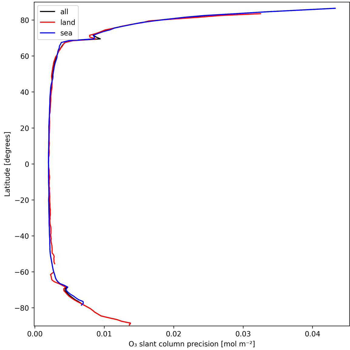
Figure 20: Zonal average of "O 3 slant column precision" for 2025-03-13 to 2025-03-14.
