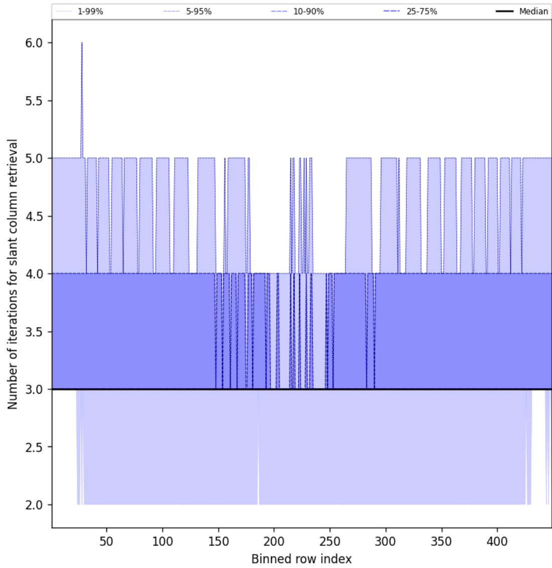
Figure 45: Along track statistics of “Number of iterations for slant column retrieval” for 2025-03-17 to 2025-03-18
