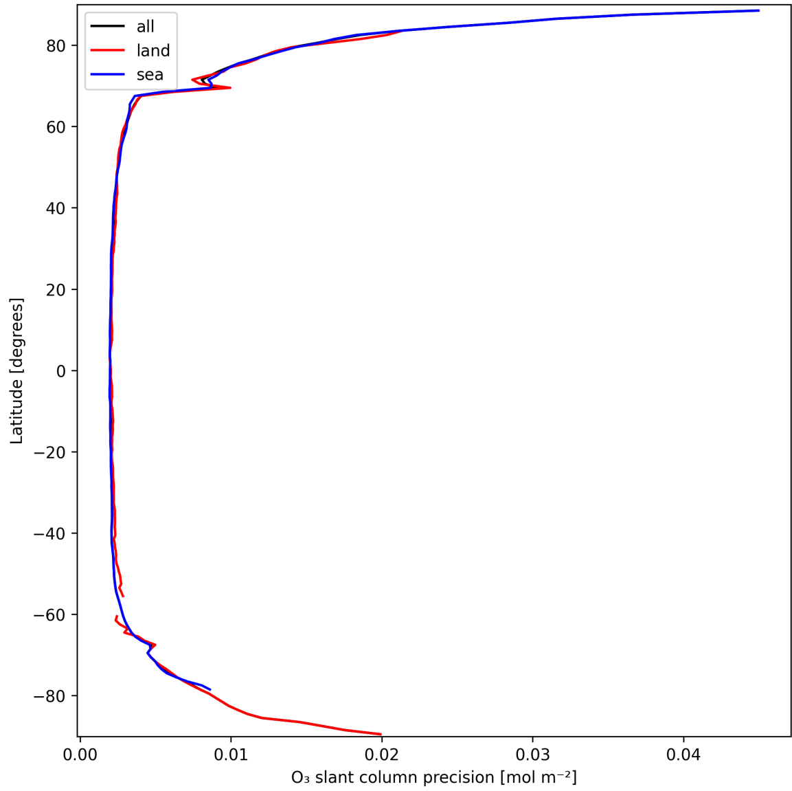
Figure 20: Zonal average of "O 3 slant column precision" for 2025-03-17 to 2025-03-18.
