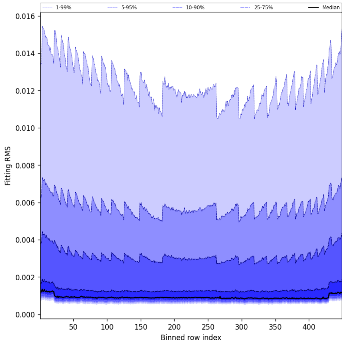
Figure 46: Along track statistics of “Fitting RMS” for 2025-03-17 to 2025-03-18
