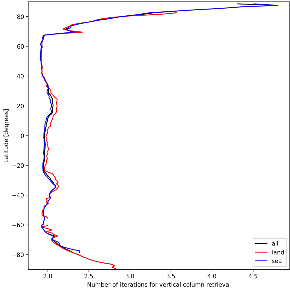
Figure 27: Zonal average of “Number of iterations for vertical column retrieval” for 2025-03-17 to 2025-03-18.
