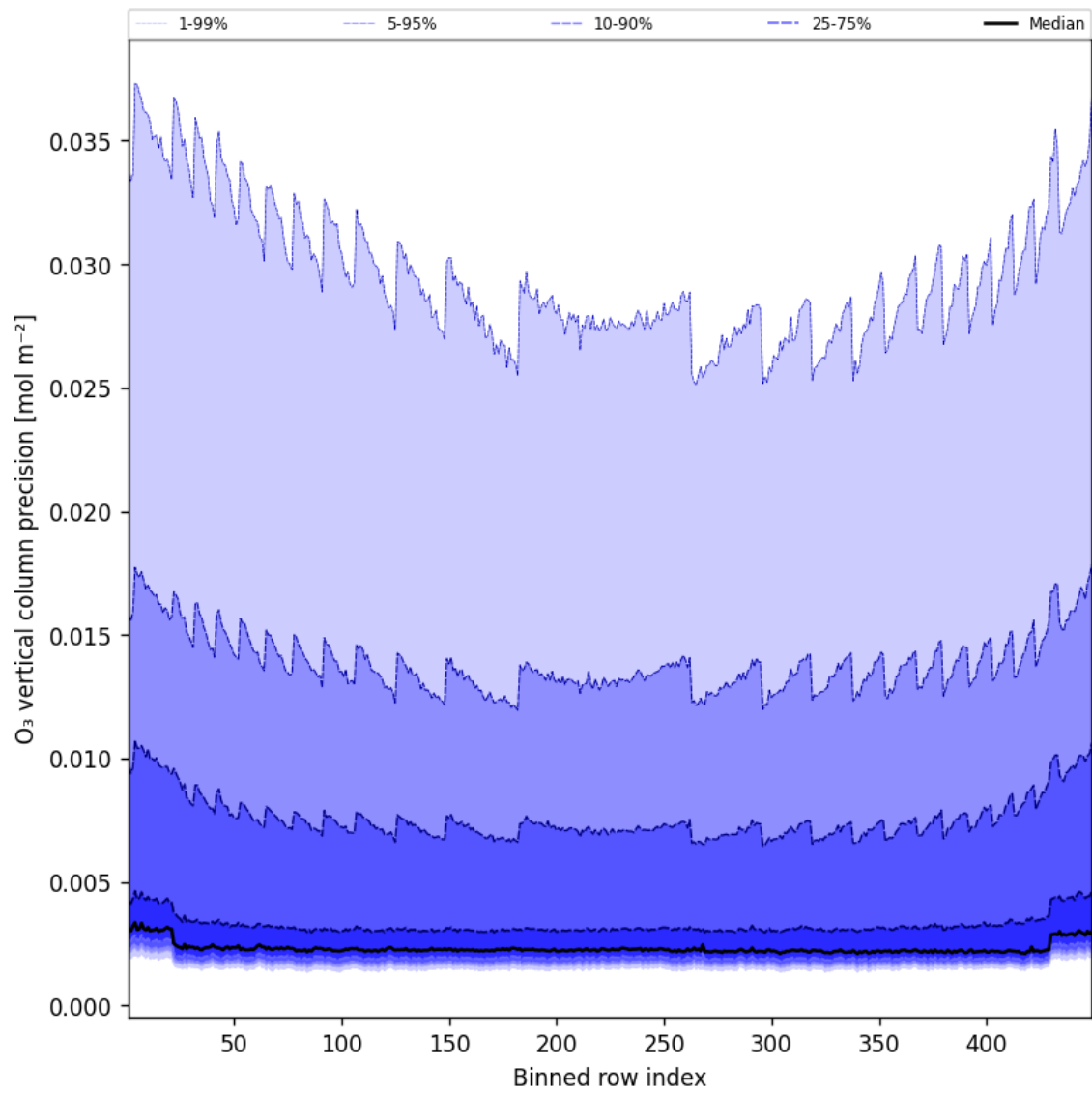
Figure 42: Along track statistics of “O 3 vertical column precision” for 2025-03-17 to 2025-03-18
