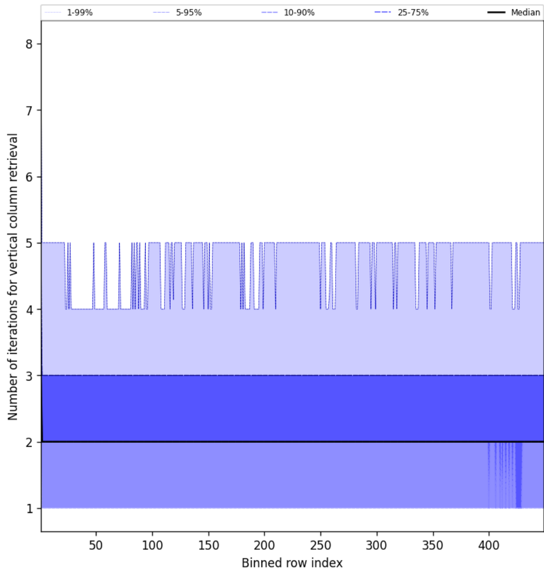
Figure 51: Along track statistics of “Number of iterations for vertical column retrieval” for 2025-03-17 to 2025-03-18
