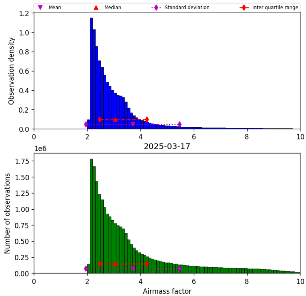
Figure 37: Histogram of “Airmass factor” for 2025-03-17 to 2025-03-18
