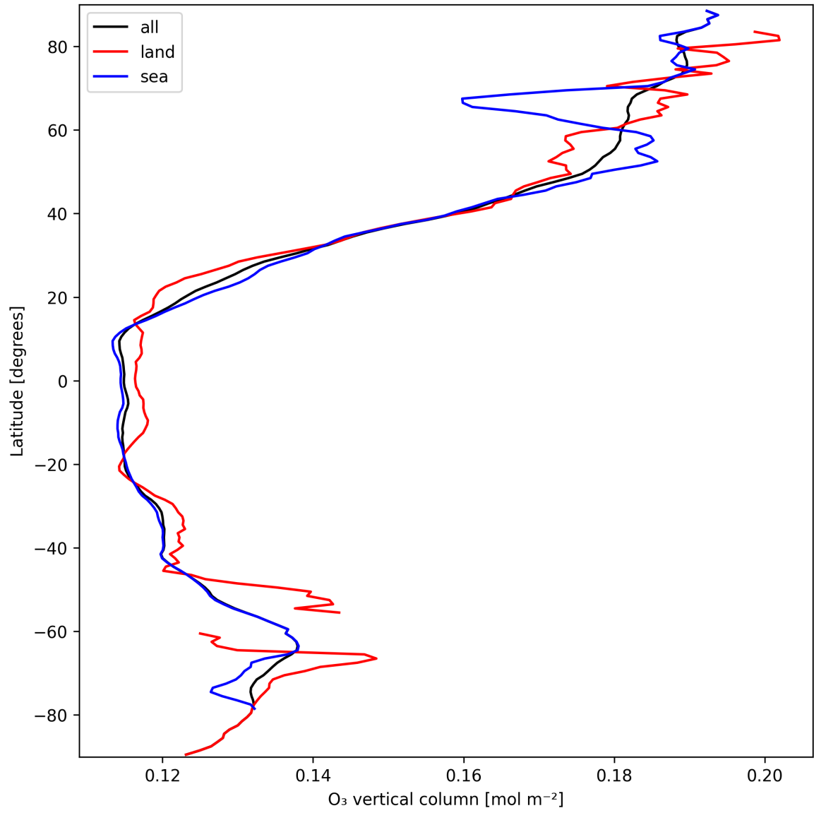
Figure 17: Zonal average of “O 3 vertical column” for 2025-03-17 to 2025-03-18.
