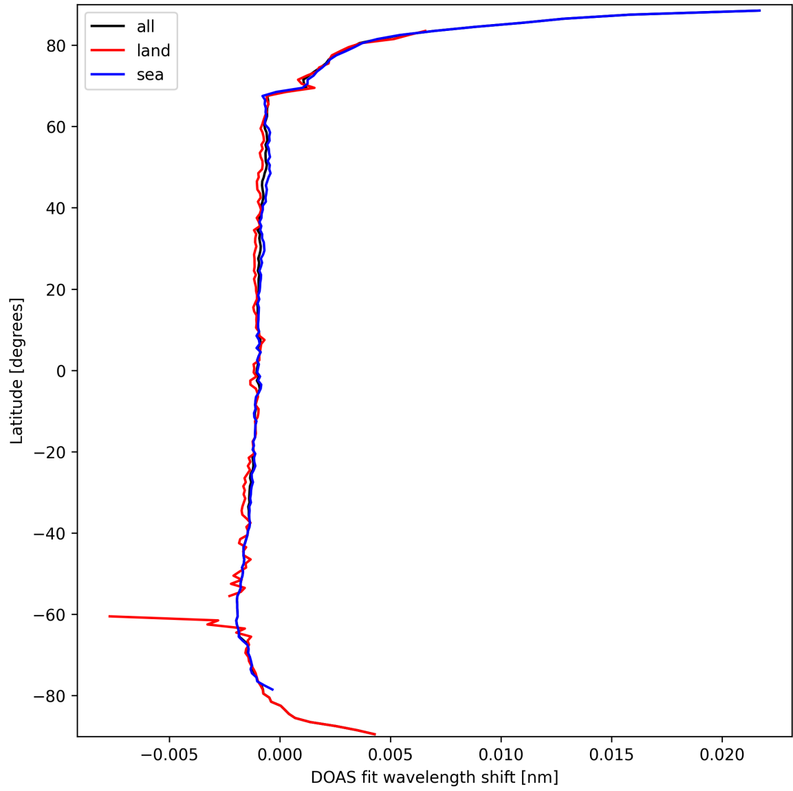
Figure 23: Zonal average of “DOAS fit wavelength shift” for 2025-03-17 to 2025-03-18.
