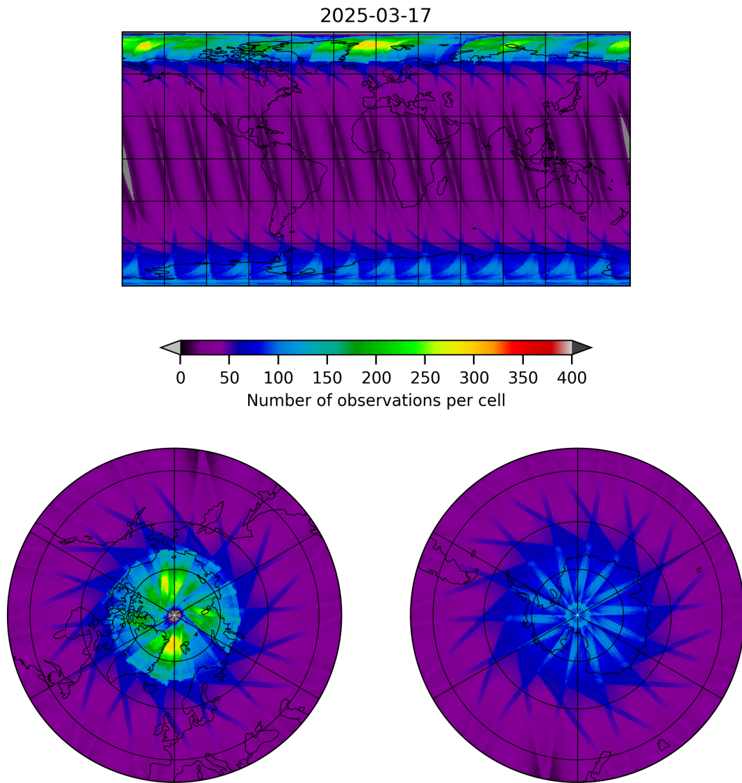
Figure 15: Map of the number of observations for 2025-03-17 to 2025-03-18
