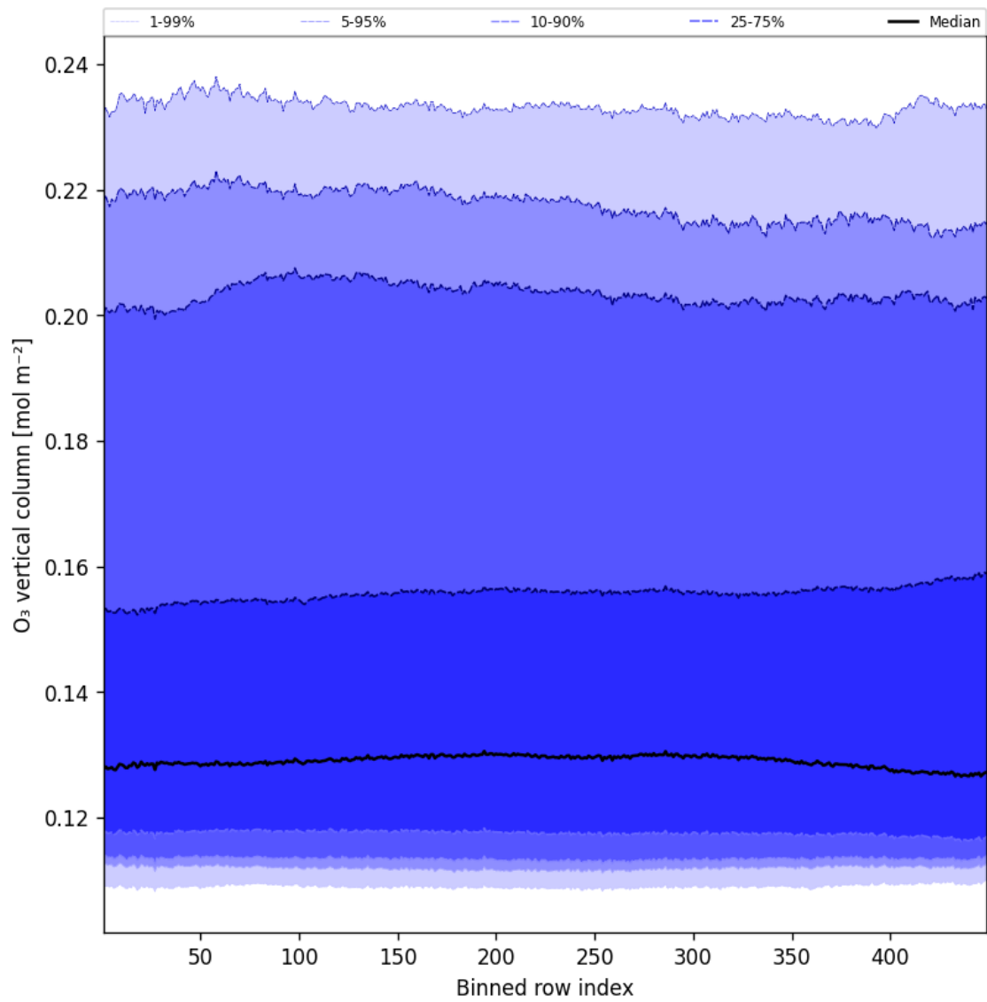
Figure 41: Along track statistics of “ \text{O}_3 vertical column” for 2025-03-17 to 2025-03-18
