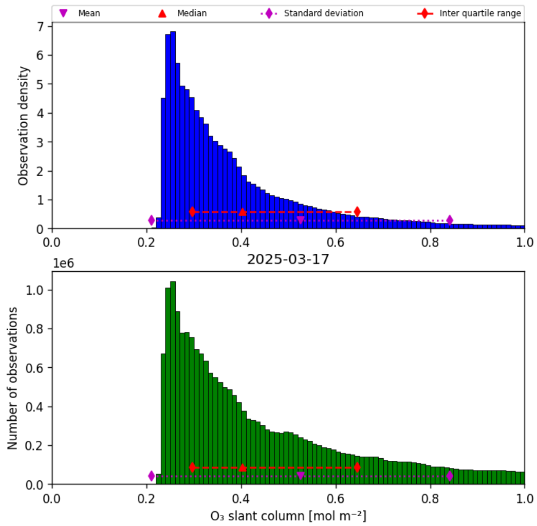
Figure 31: Histogram of “O 3 slant column” for 2025-03-17 to 2025-03-18
