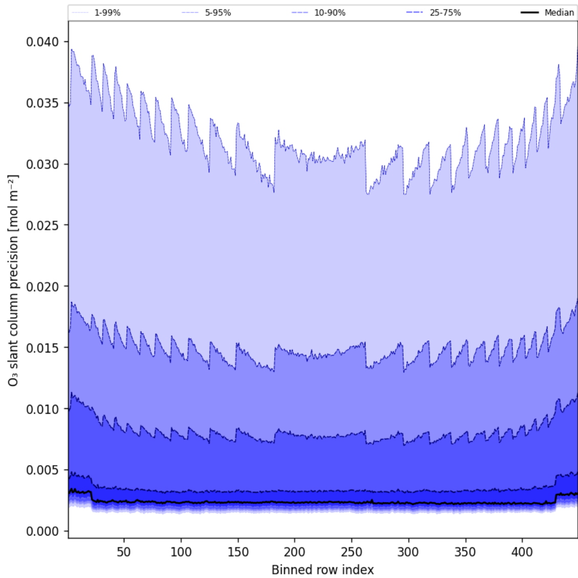
Figure 44: Along track statistics of “O 3 slant column precision” for 2025-03-17 to 2025-03-18
