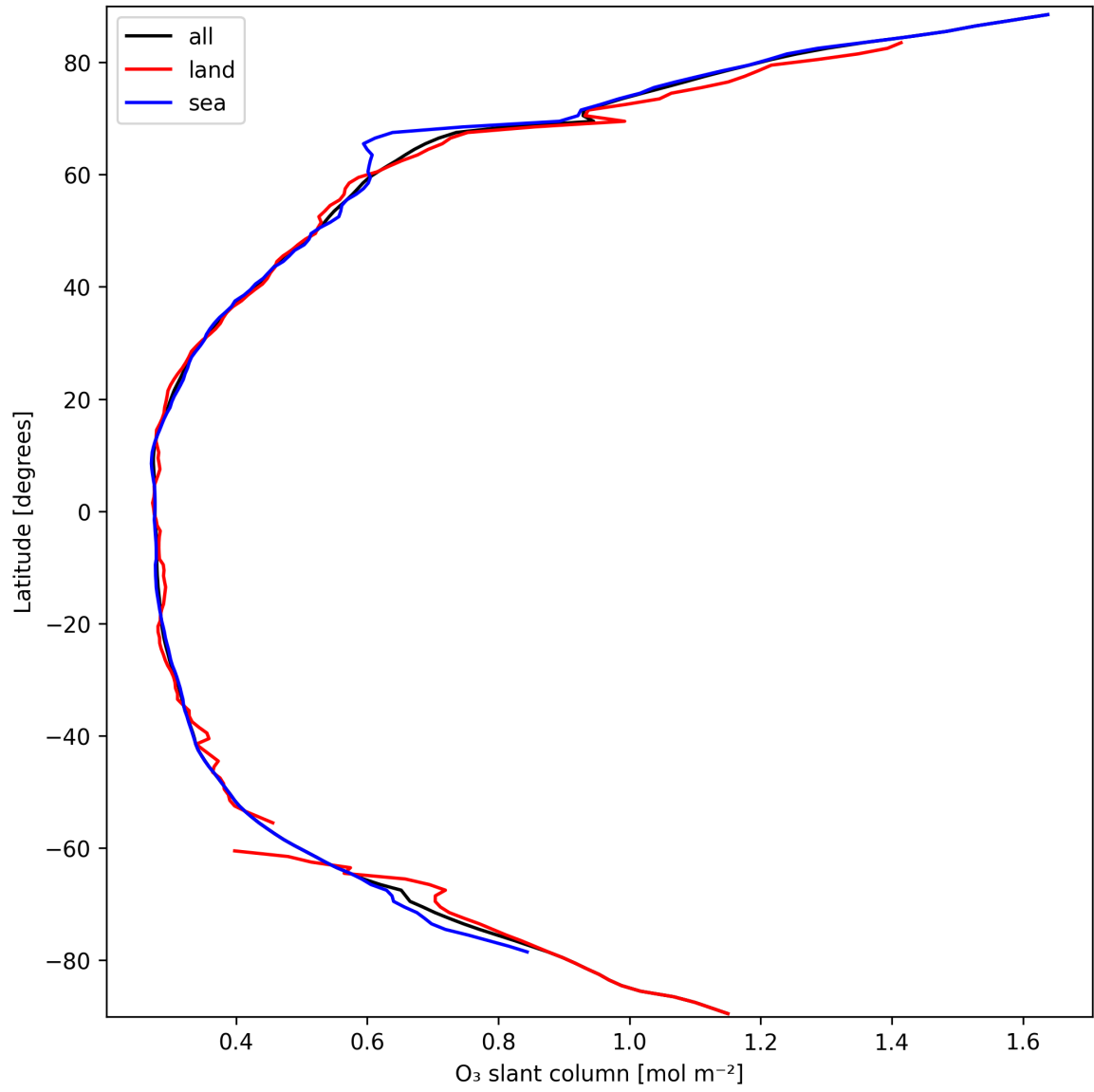
Figure 19: Zonal average of “O 3 slant column” for 2025-03-17 to 2025-03-18.
