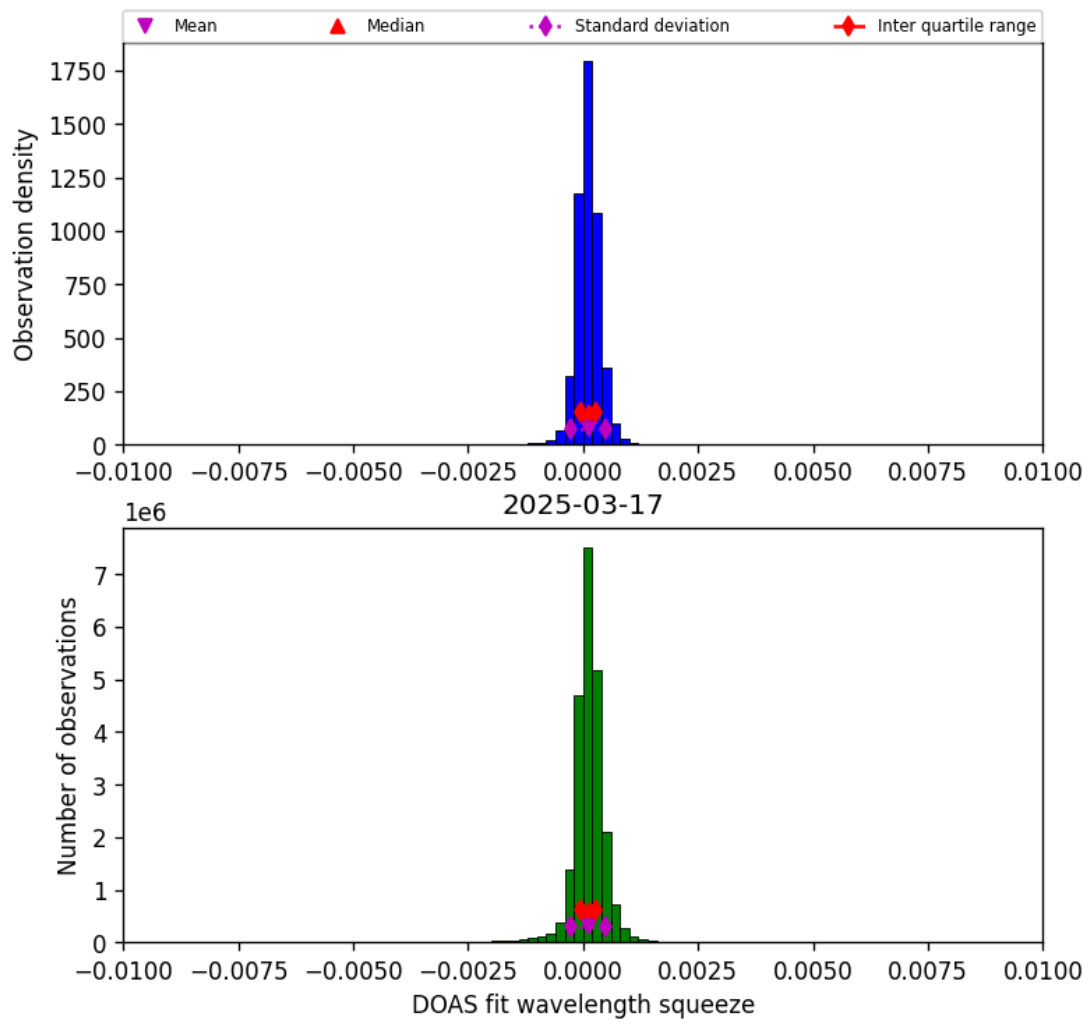
Figure 36: Histogram of “DOAS fit wavelength squeeze” for 2025-03-17 to 2025-03-18
