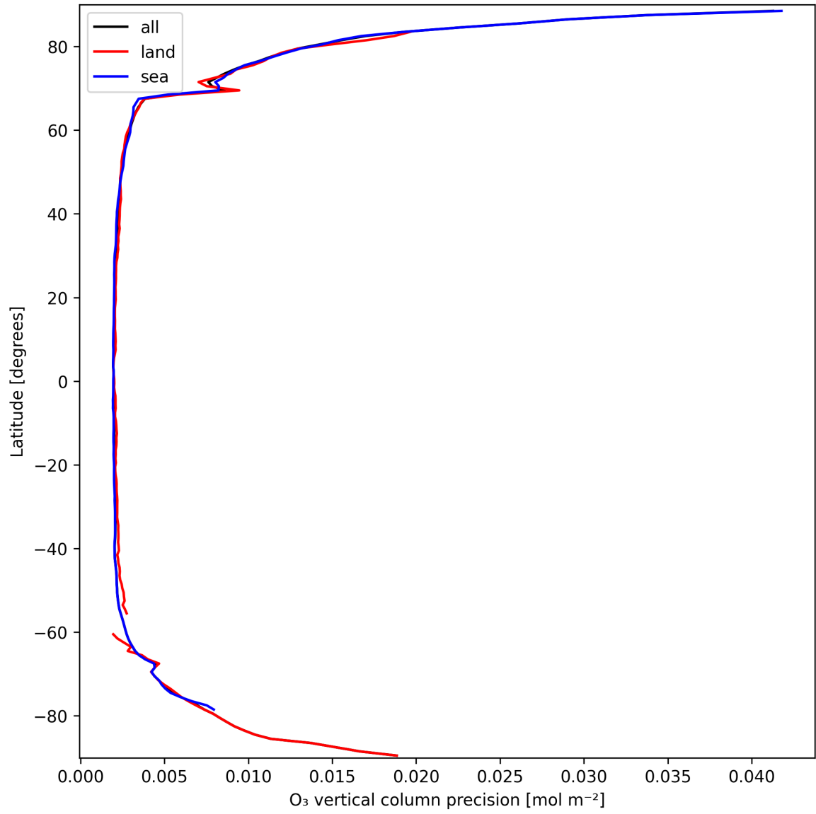
Figure 18: Zonal average of “O 3 vertical column precision” for 2025-03-17 to 2025-03-18.
