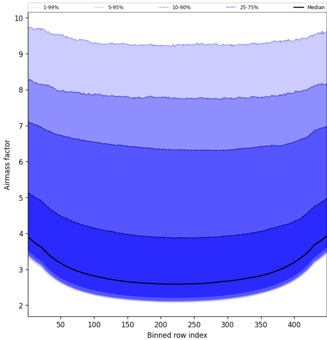
Figure 49: Along track statistics of “Airmass factor” for 2025-03-17 to 2025-03-18
