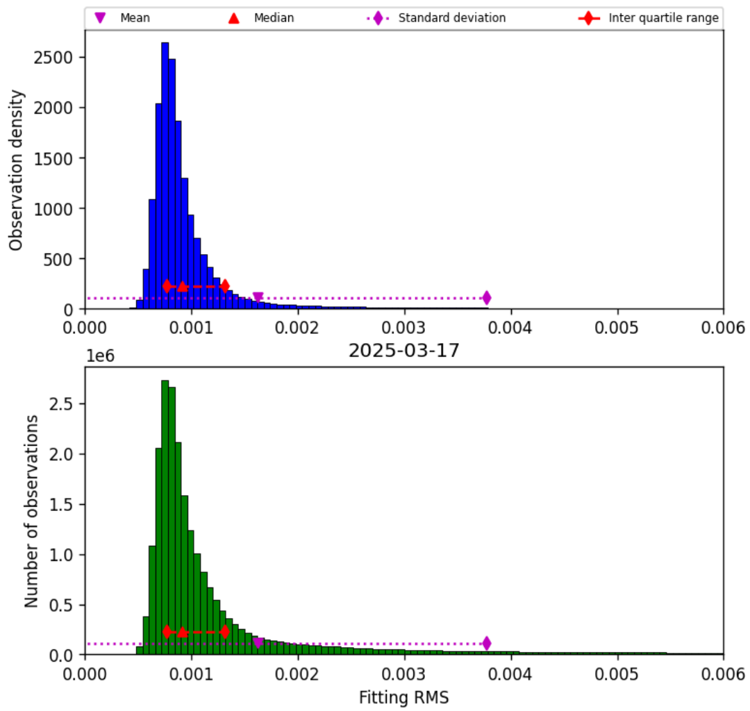
Figure 34: Histogram of “Fitting RMS” for 2025-03-17 to 2025-03-18
