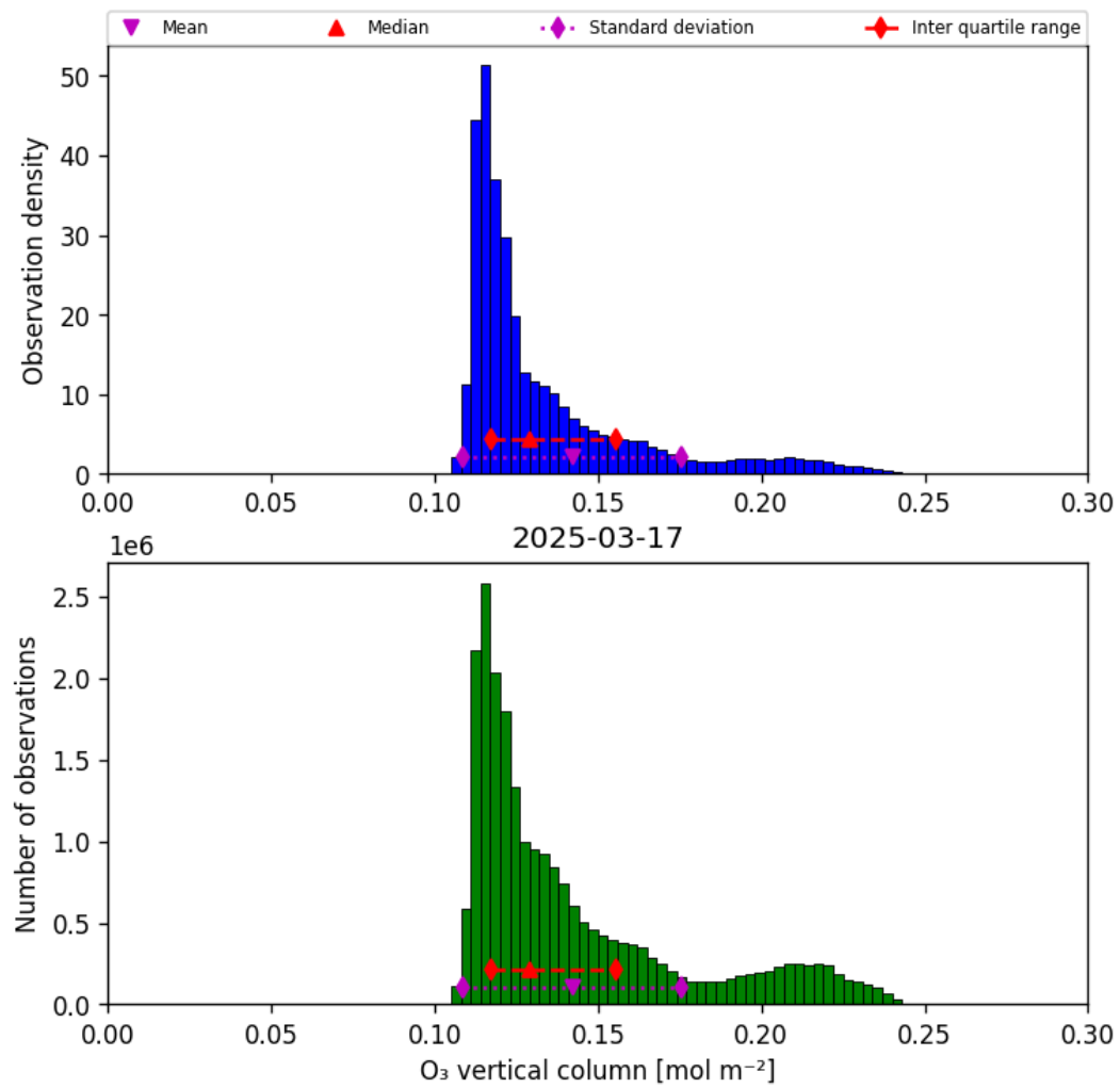
Figure 29: Histogram of “O 3 vertical column” for 2025-03-17 to 2025-03-18
