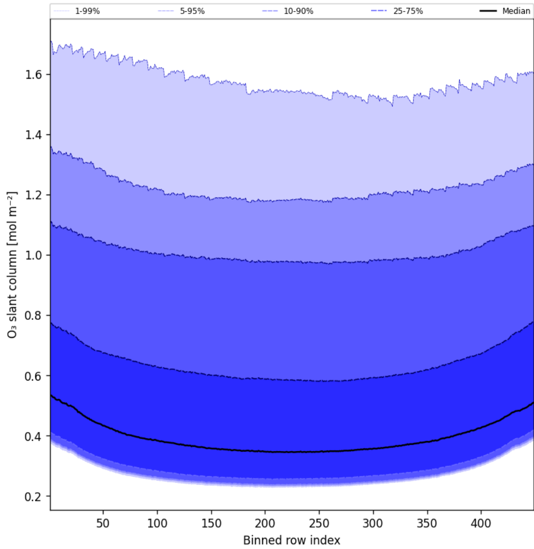
Figure 43: Along track statistics of “O 3 slant column” for 2025-03-17 to 2025-03-18
