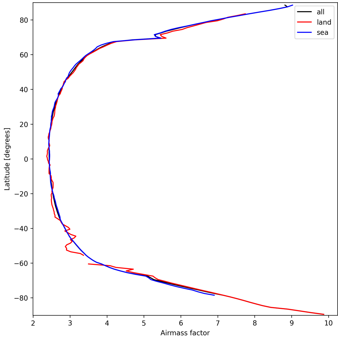
Figure 25: Zonal average of “Airmass factor” for 2025-03-17 to 2025-03-18.
