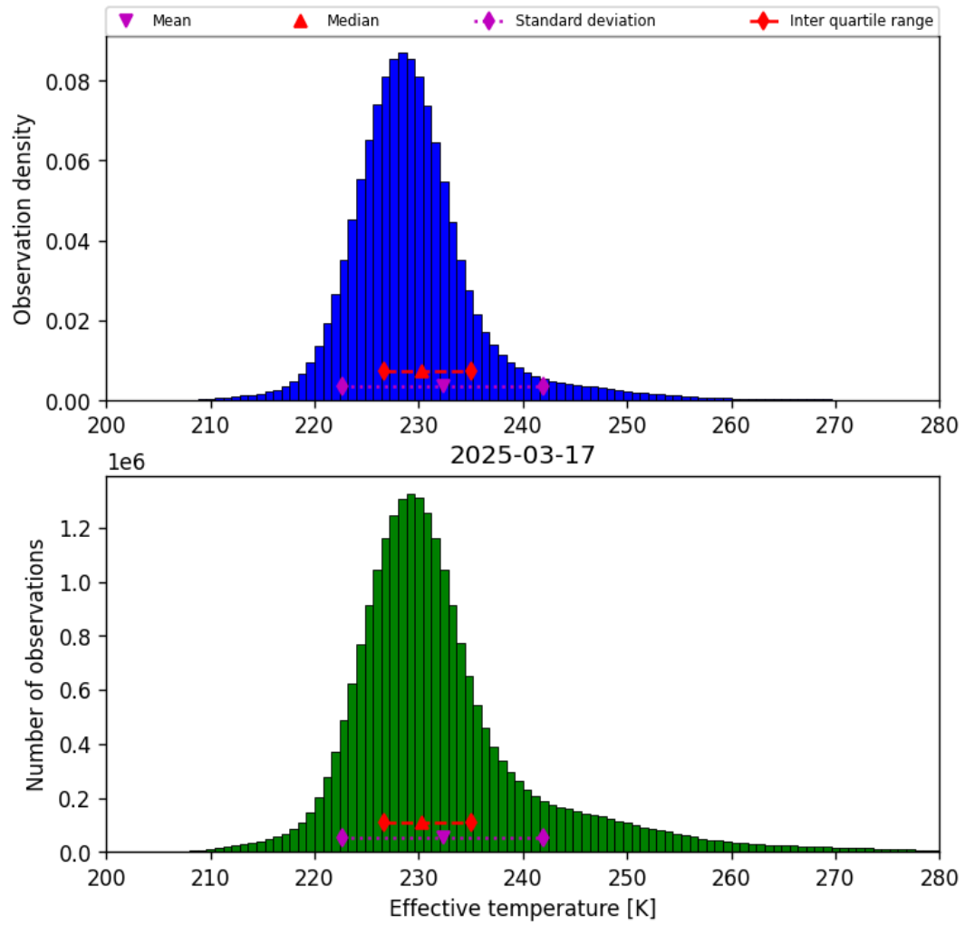
Figure 38: Histogram of “Effective temperature” for 2025-03-17 to 2025-03-18
