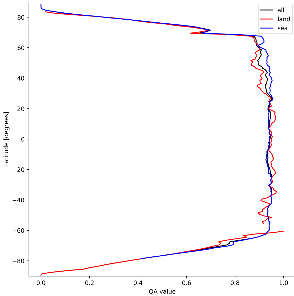
Figure 16: Zonal average of “QA value” for 2025-03-17 to 2025-03-18.
