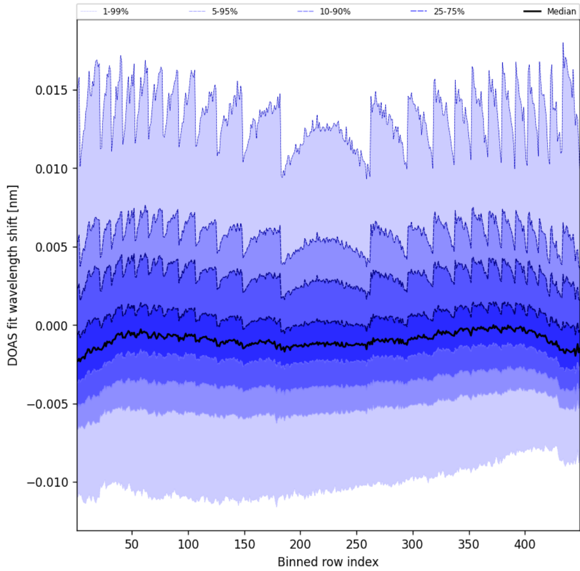
Figure 47: Along track statistics of “DOAS fit wavelength shift” for 2025-03-17 to 2025-03-18
