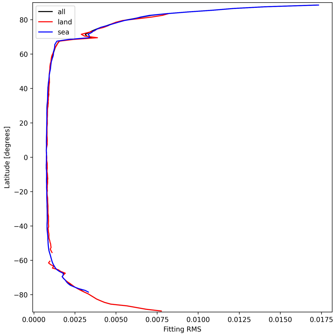
Figure 22: Zonal average of “Fitting RMS” for 2025-03-17 to 2025-03-18.
