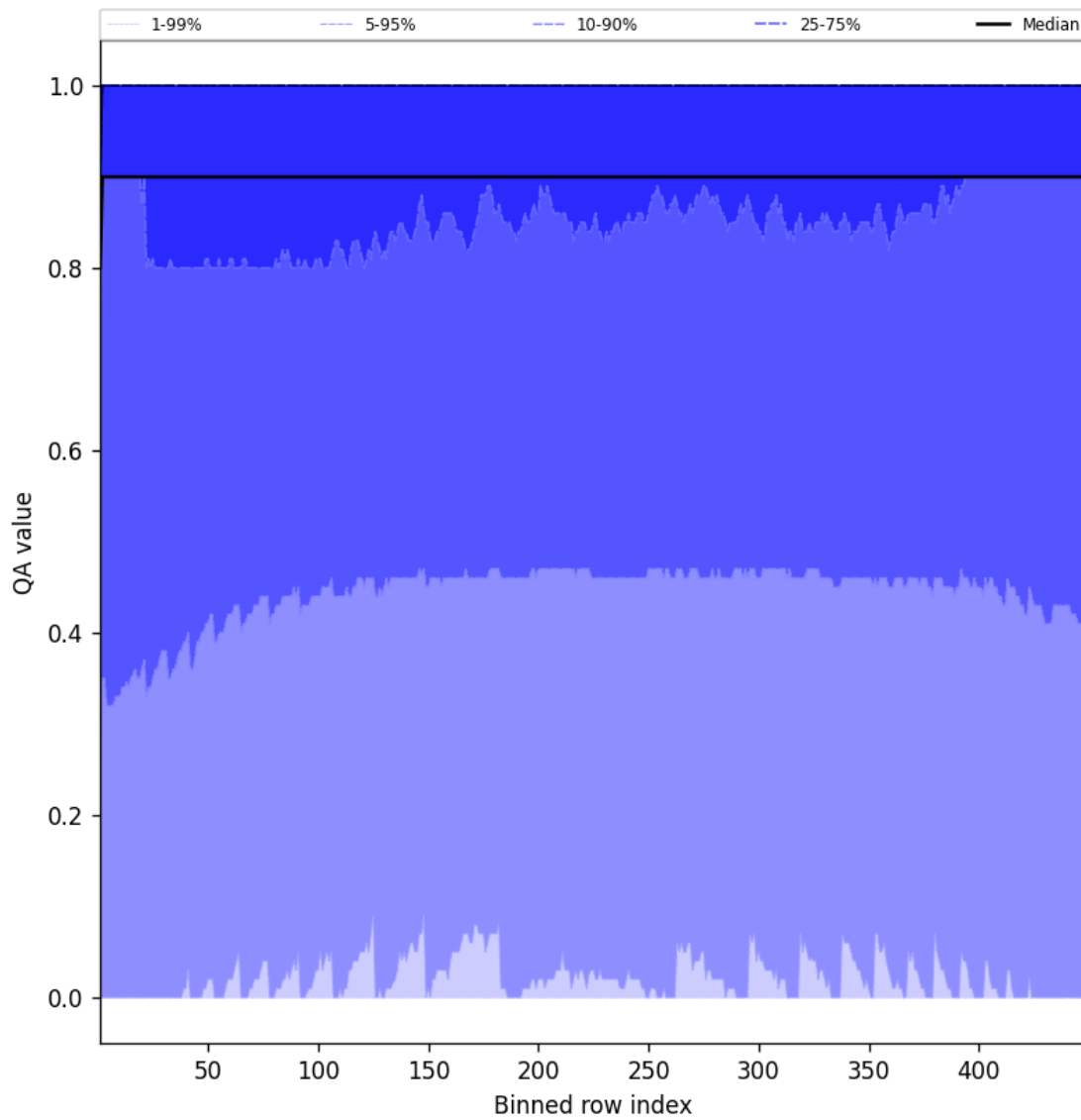
Figure 40: Along track statistics of “QA value” for 2025-03-17 to 2025-03-18
