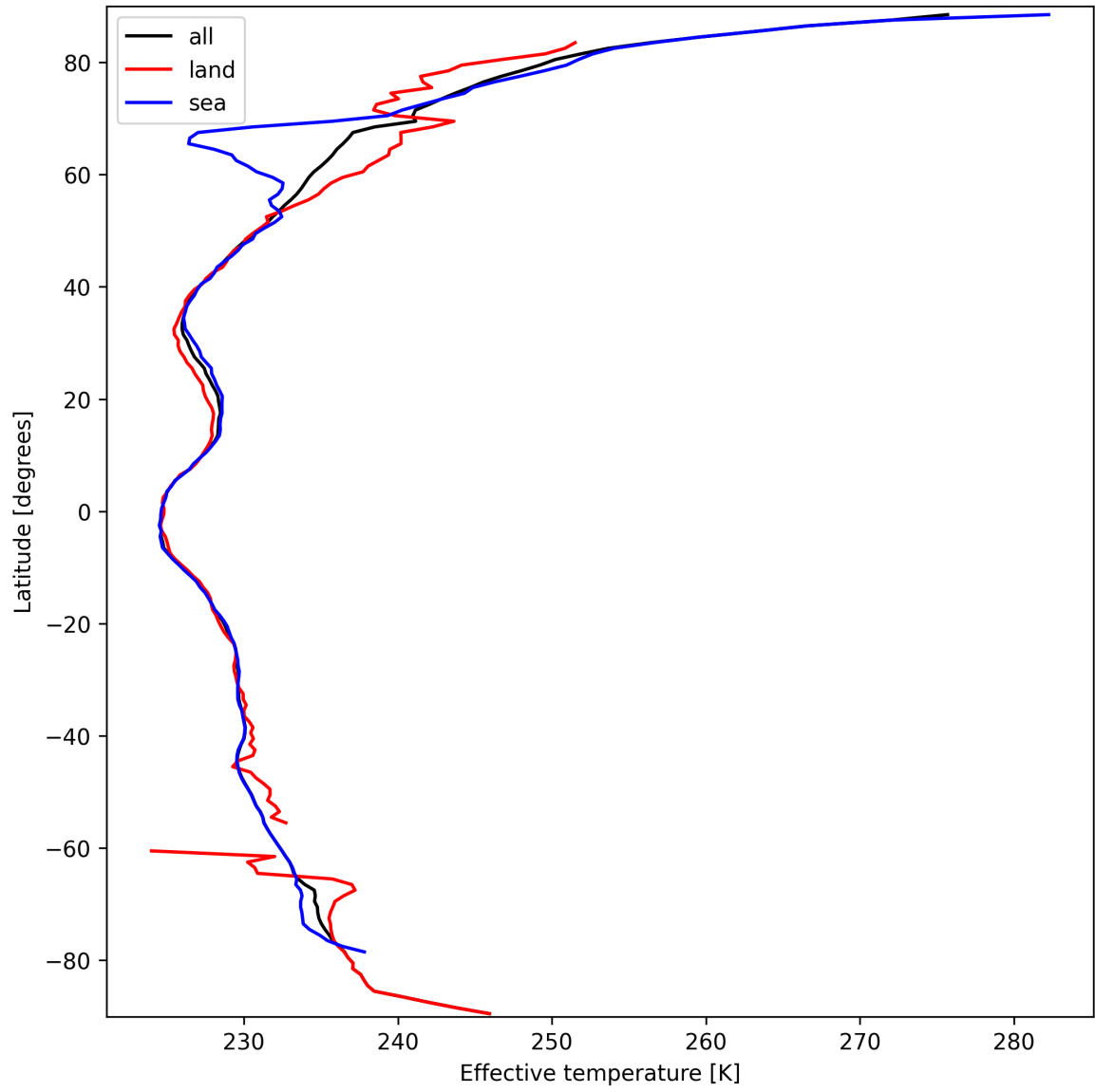
Figure 26: Zonal average of “Effective temperature” for 2025-03-17 to 2025-03-18.
