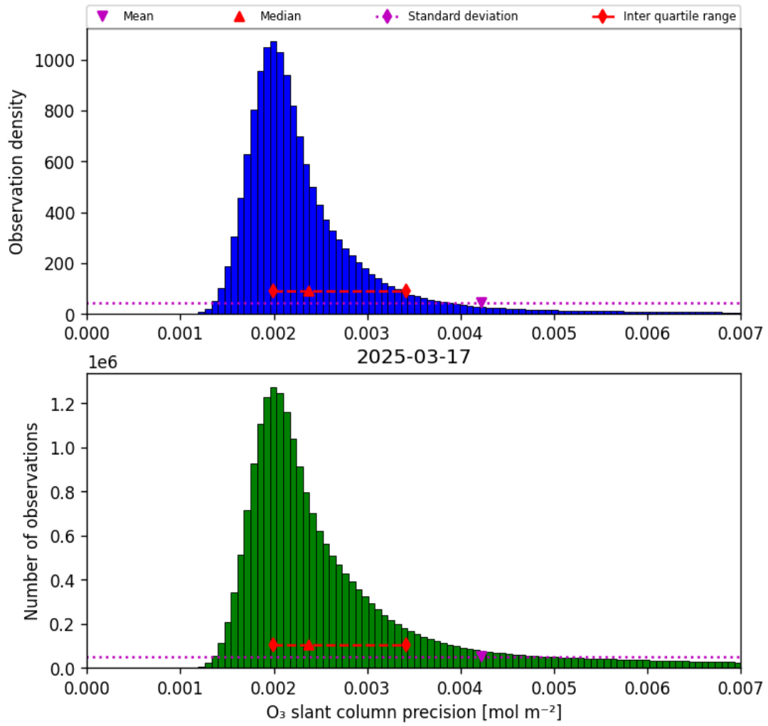
Figure 32: Histogram of “O 3 slant column precision” for 2025-03-17 to 2025-03-18
