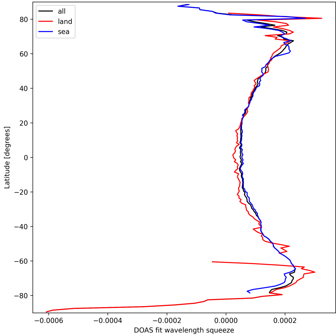
Figure 24: Zonal average of “DOAS fit wavelength squeeze” for 2025-03-17 to 2025-03-18.
