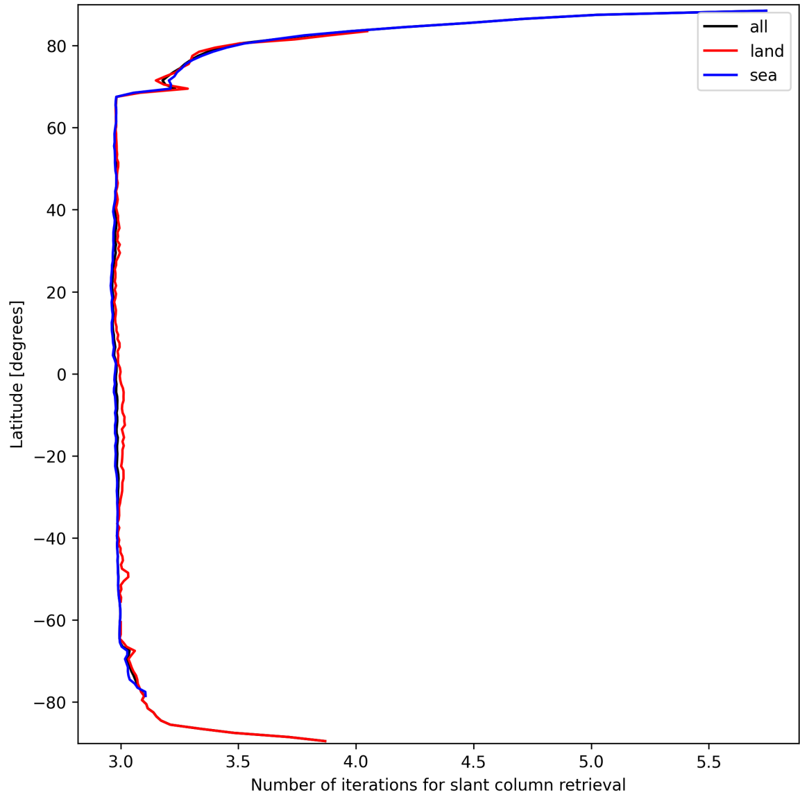
Figure 21: Zonal average of “Number of iterations for slant column retrieval” for 2025-03-17 to 2025-03-18.
