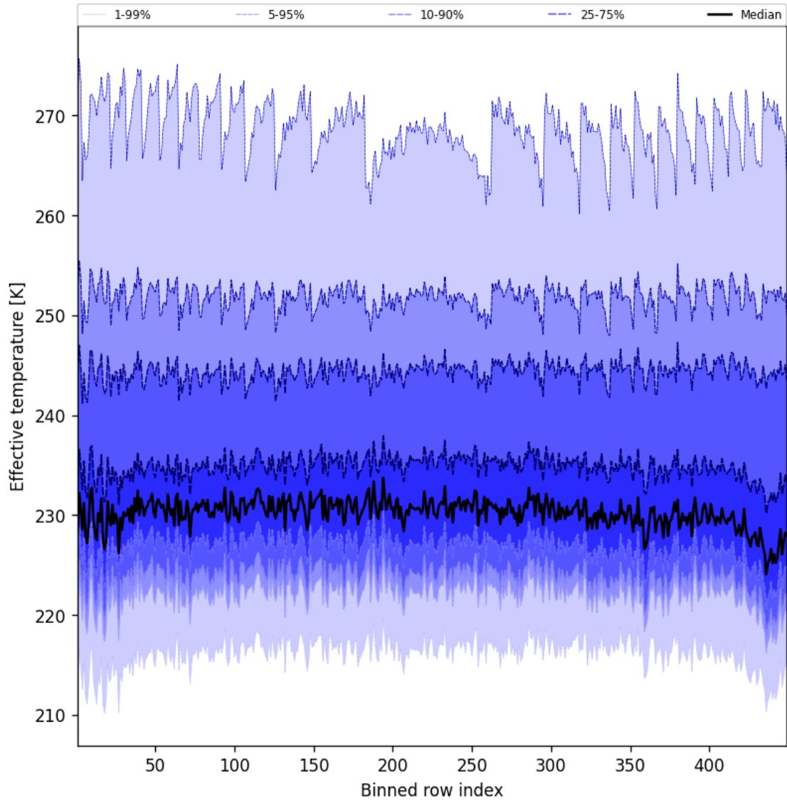
Figure 50: Along track statistics of "Effective temperature" for 2025-03-17 to 2025-03-18
