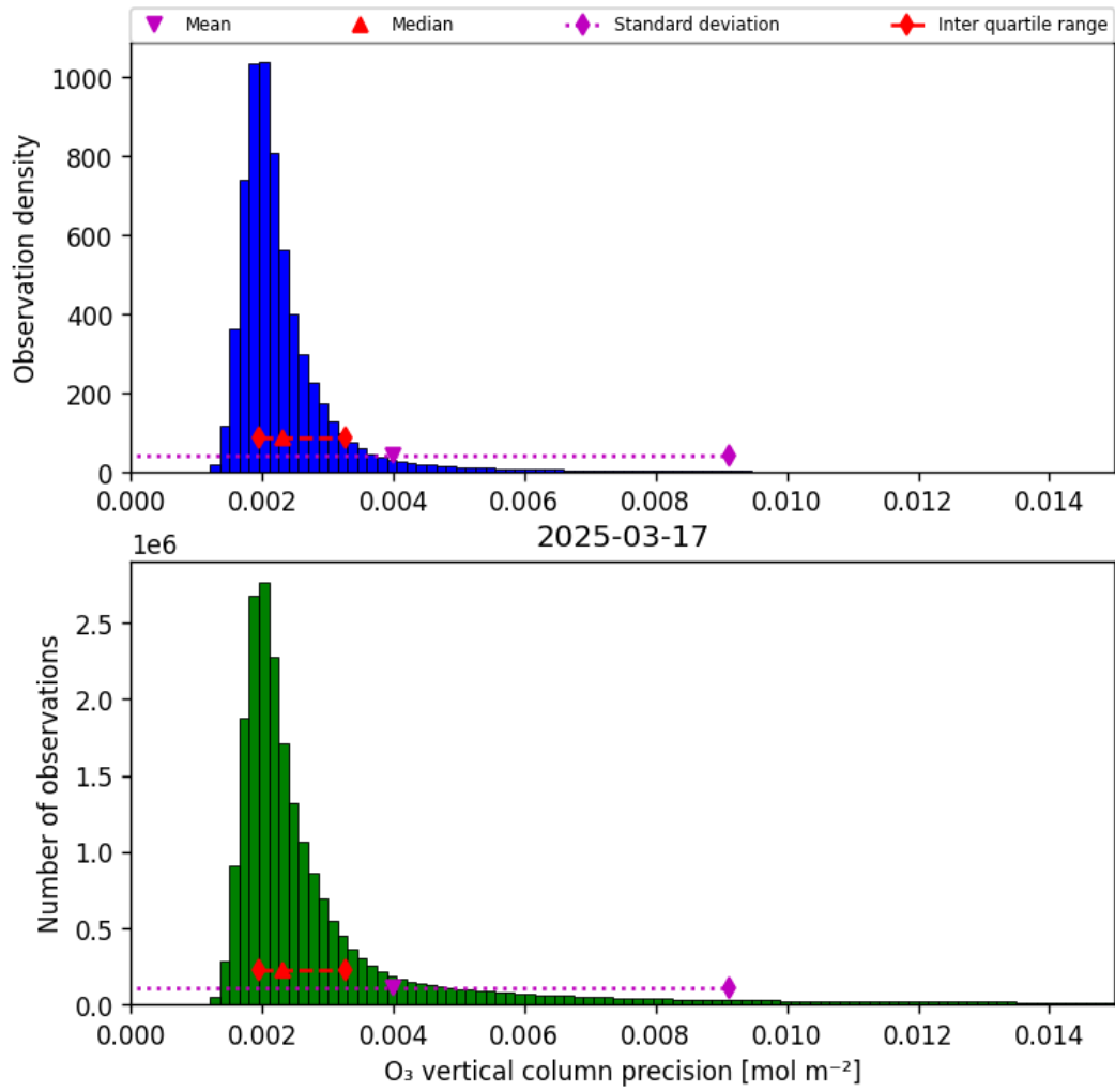
Figure 30: Histogram of “O 3 vertical column precision” for 2025-03-17 to 2025-03-18
