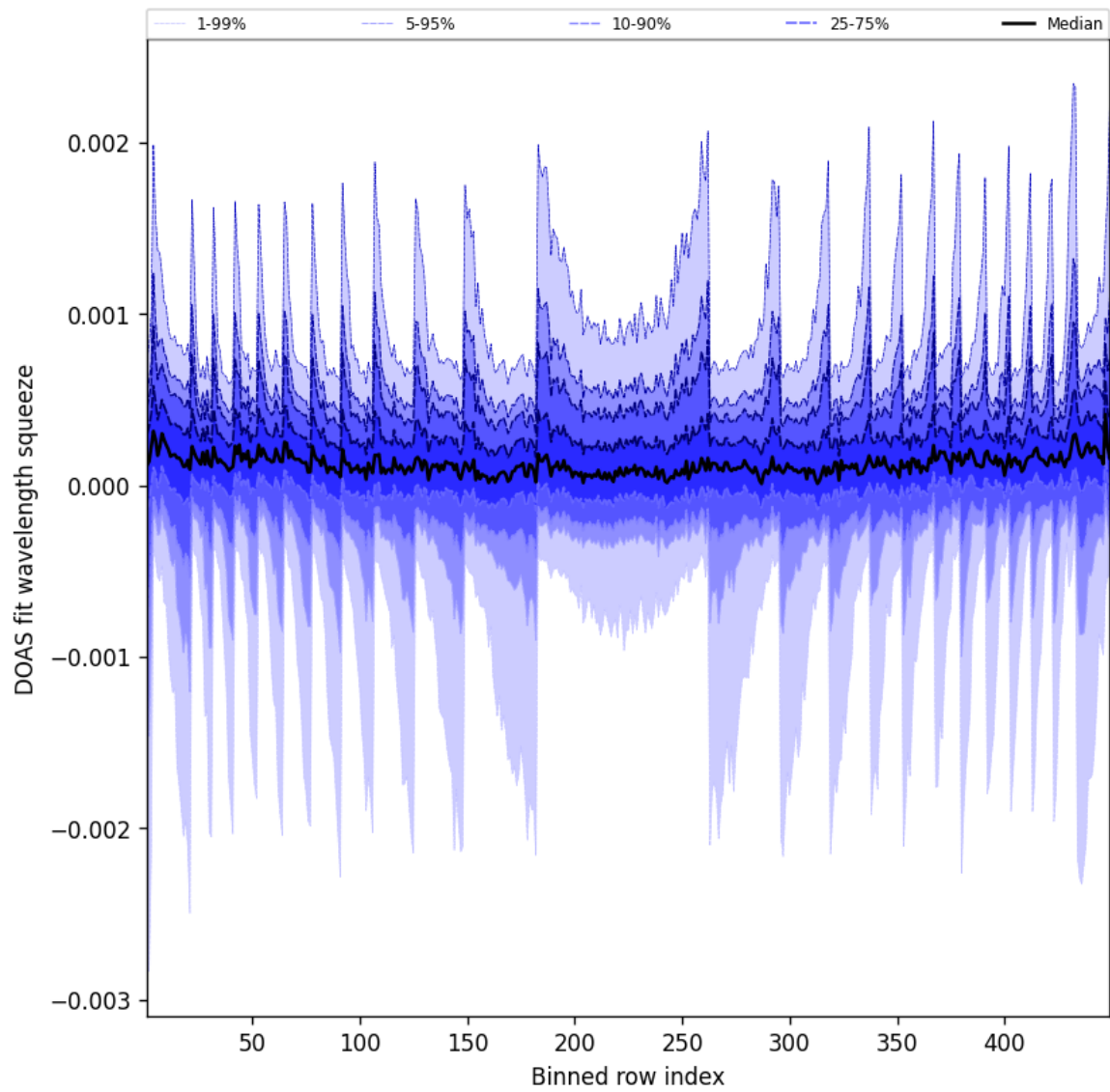
Figure 48: Along track statistics of “DOAS fit wavelength squeeze” for 2025-03-17 to 2025-03-18
