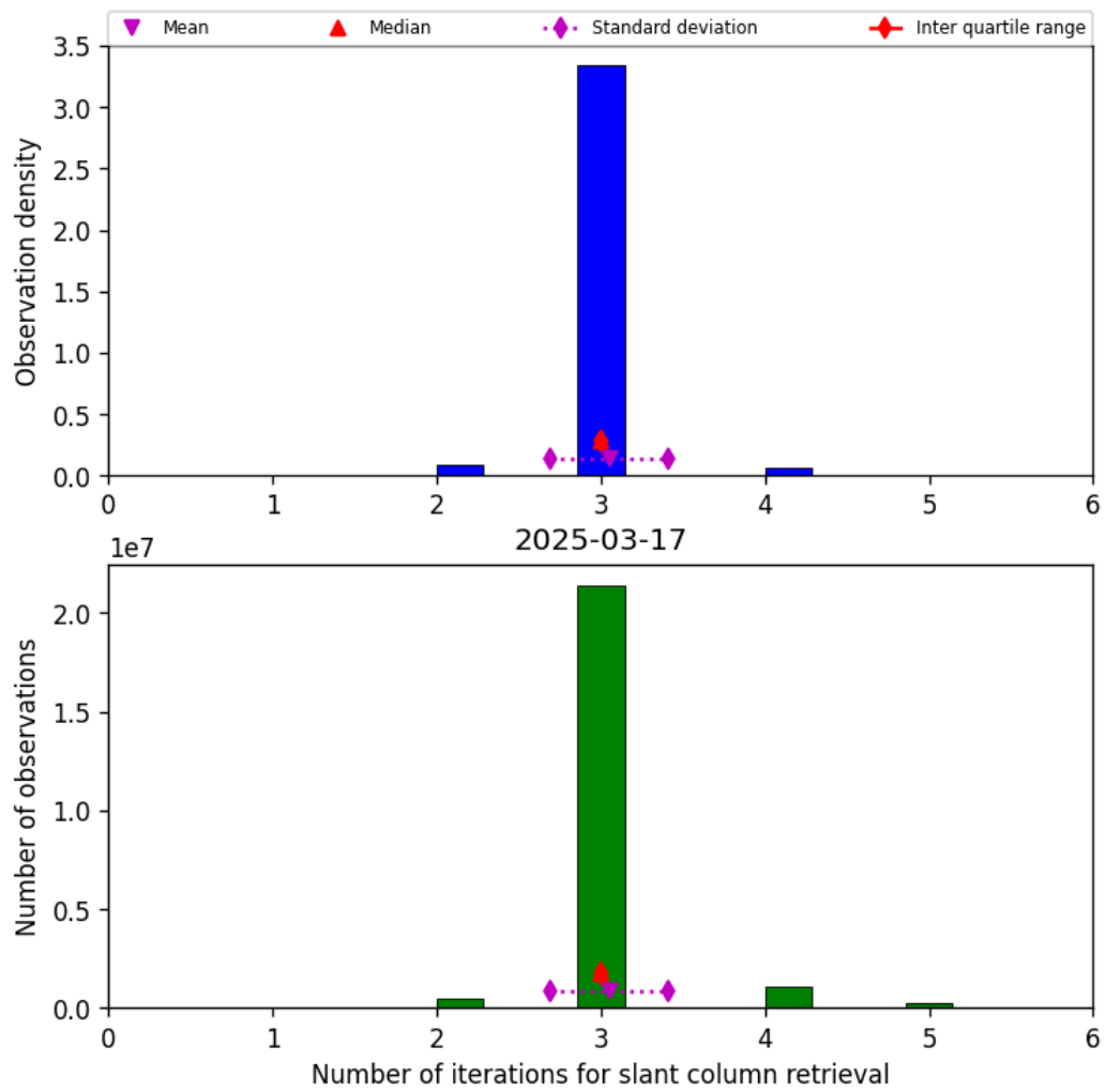
Figure 33: Histogram of “Number of iterations for slant column retrieval” for 2025-03-17 to 2025-03-18
