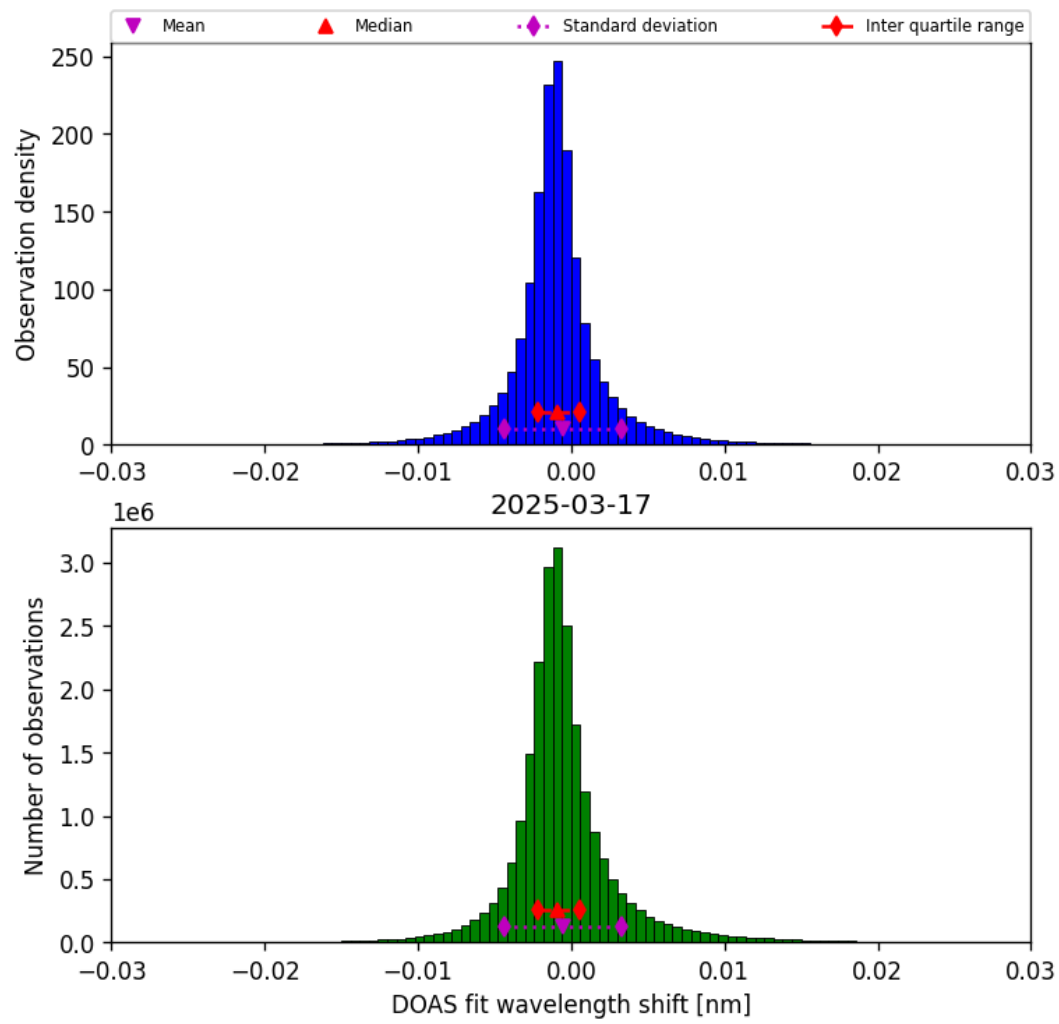
Figure 35: Histogram of “DOAS fit wavelength shift” for 2025-03-17 to 2025-03-18
