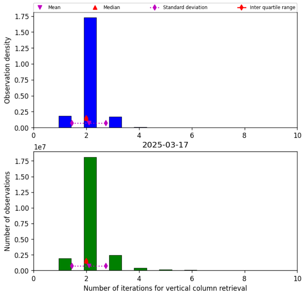
Figure 39: Histogram of “Number of iterations for vertical column retrieval” for 2025-03-17 to 2025-03-18
