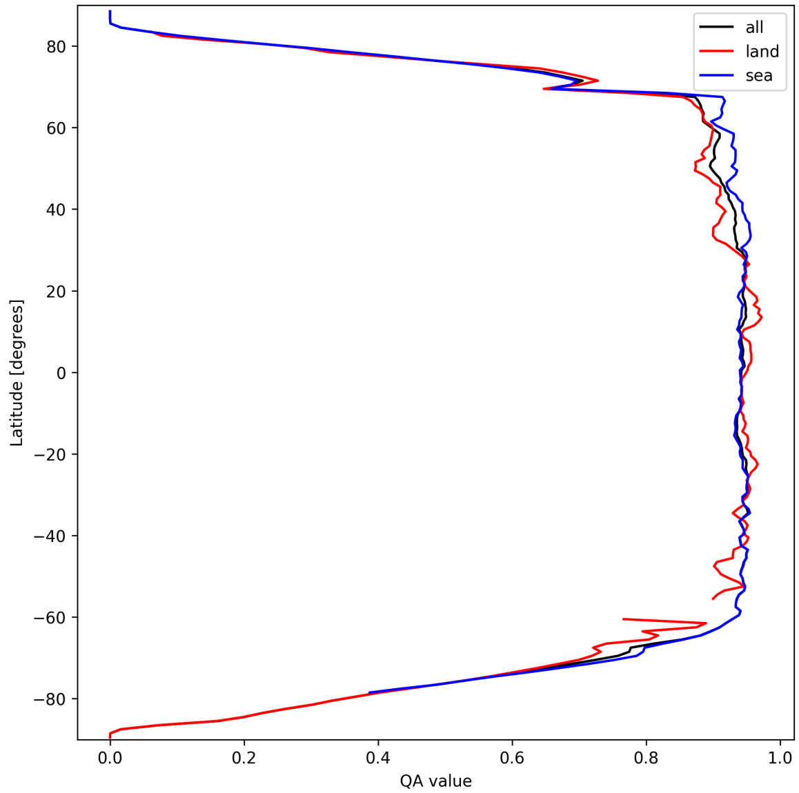
Figure 16: Zonal average of “QA value” for 2025-03-18 to 2025-03-19.
