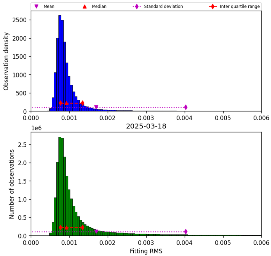
Figure 34: Histogram of “Fitting RMS” for 2025-03-18 to 2025-03-19
