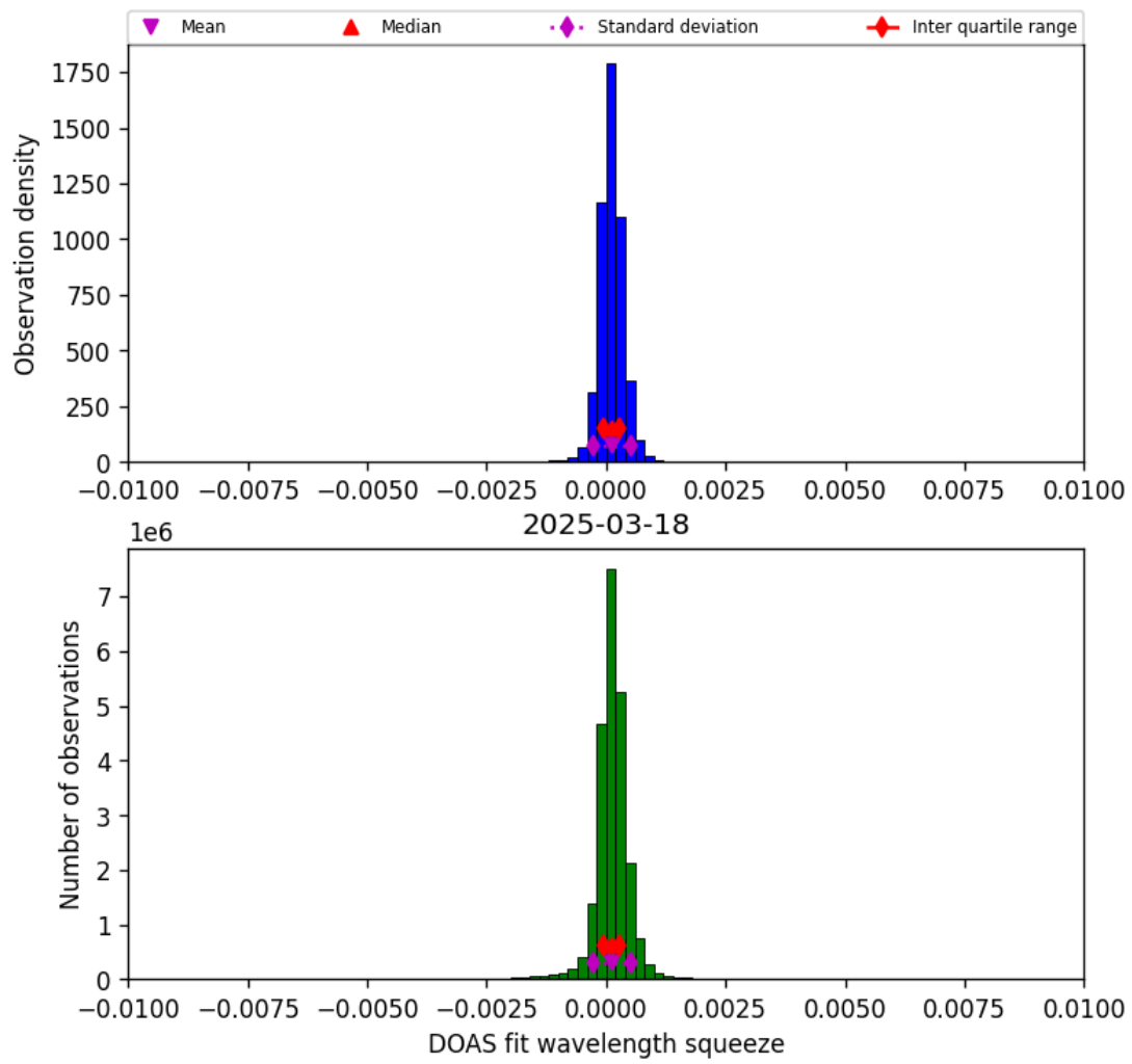
Figure 36: Histogram of “DOAS fit wavelength squeeze” for 2025-03-18 to 2025-03-19
