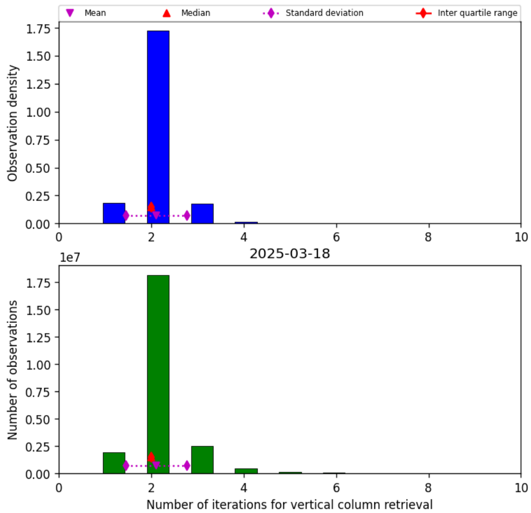
Figure 39: Histogram of “Number of iterations for vertical column retrieval” for 2025-03-18 to 2025-03-19
