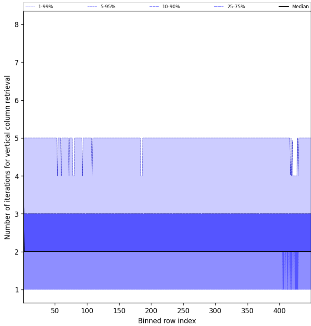
Figure 51: Along track statistics of “Number of iterations for vertical column retrieval” for 2025-03-18 to 2025-03-19
