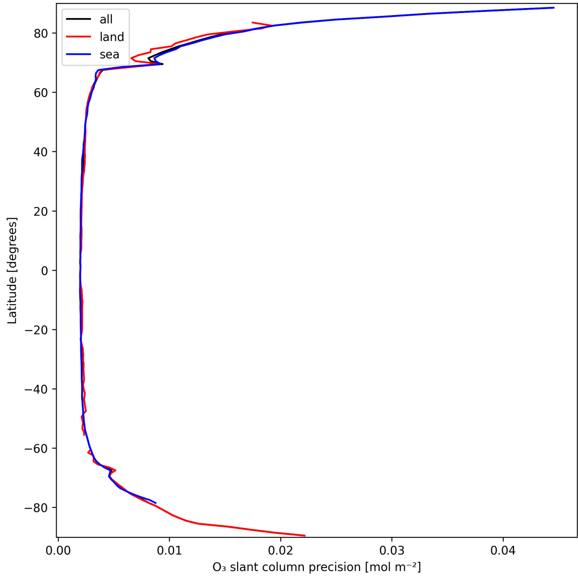
Figure 20: Zonal average of “O 3 slant column precision” for 2025-03-18 to 2025-03-19.
