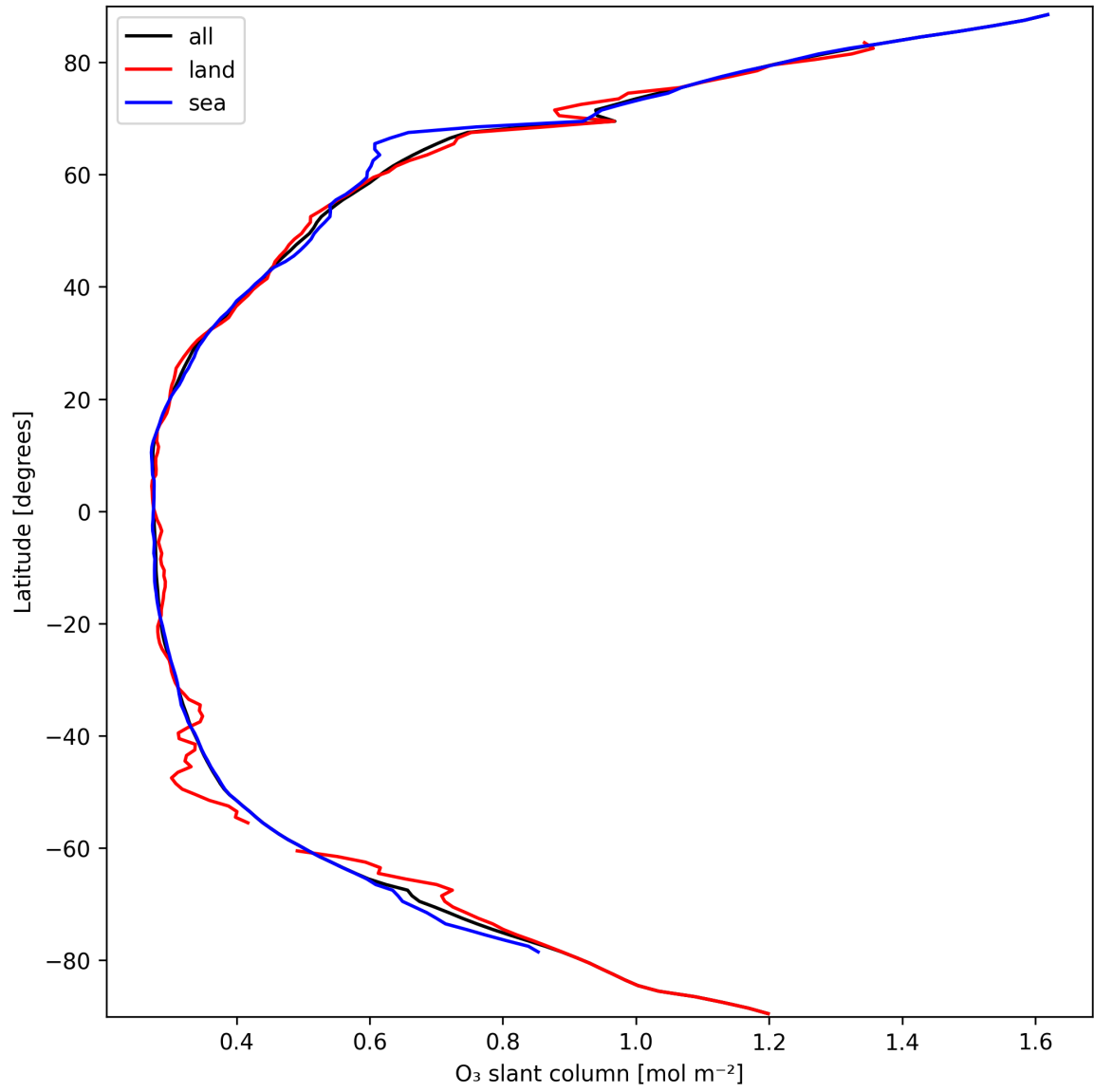
Figure 19: Zonal average of “O 3 slant column” for 2025-03-18 to 2025-03-19.
