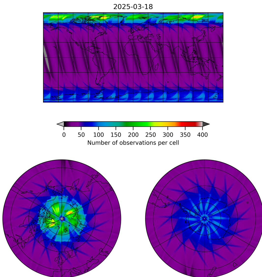
Figure 15: Map of the number of observations for 2025-03-18 to 2025-03-19
