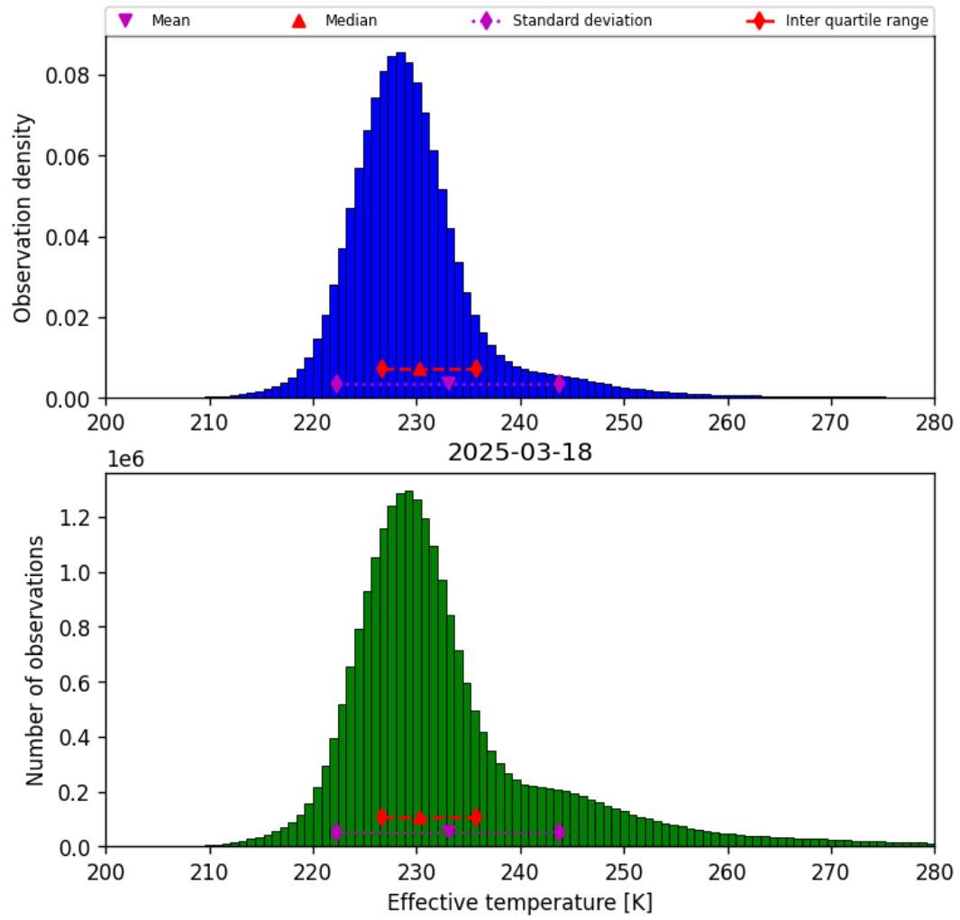
Figure 38: Histogram of “Effective temperature” for 2025-03-18 to 2025-03-19
