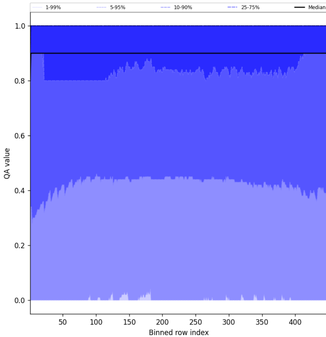
Figure 40: Along track statistics of “QA value” for 2025-03-18 to 2025-03-19
