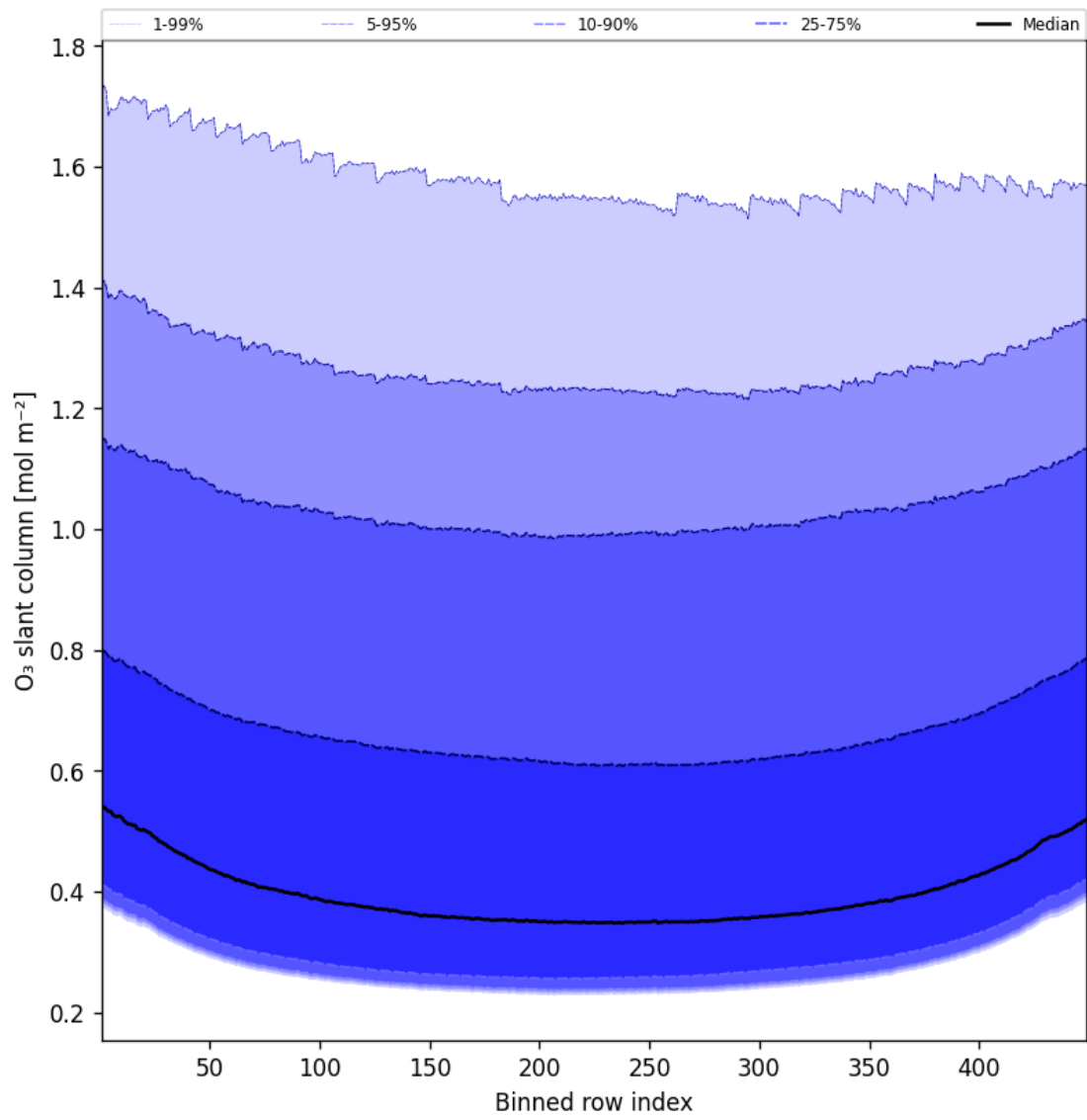
Figure 43: Along track statistics of “O 3 slant column” for 2025-03-18 to 2025-03-19
