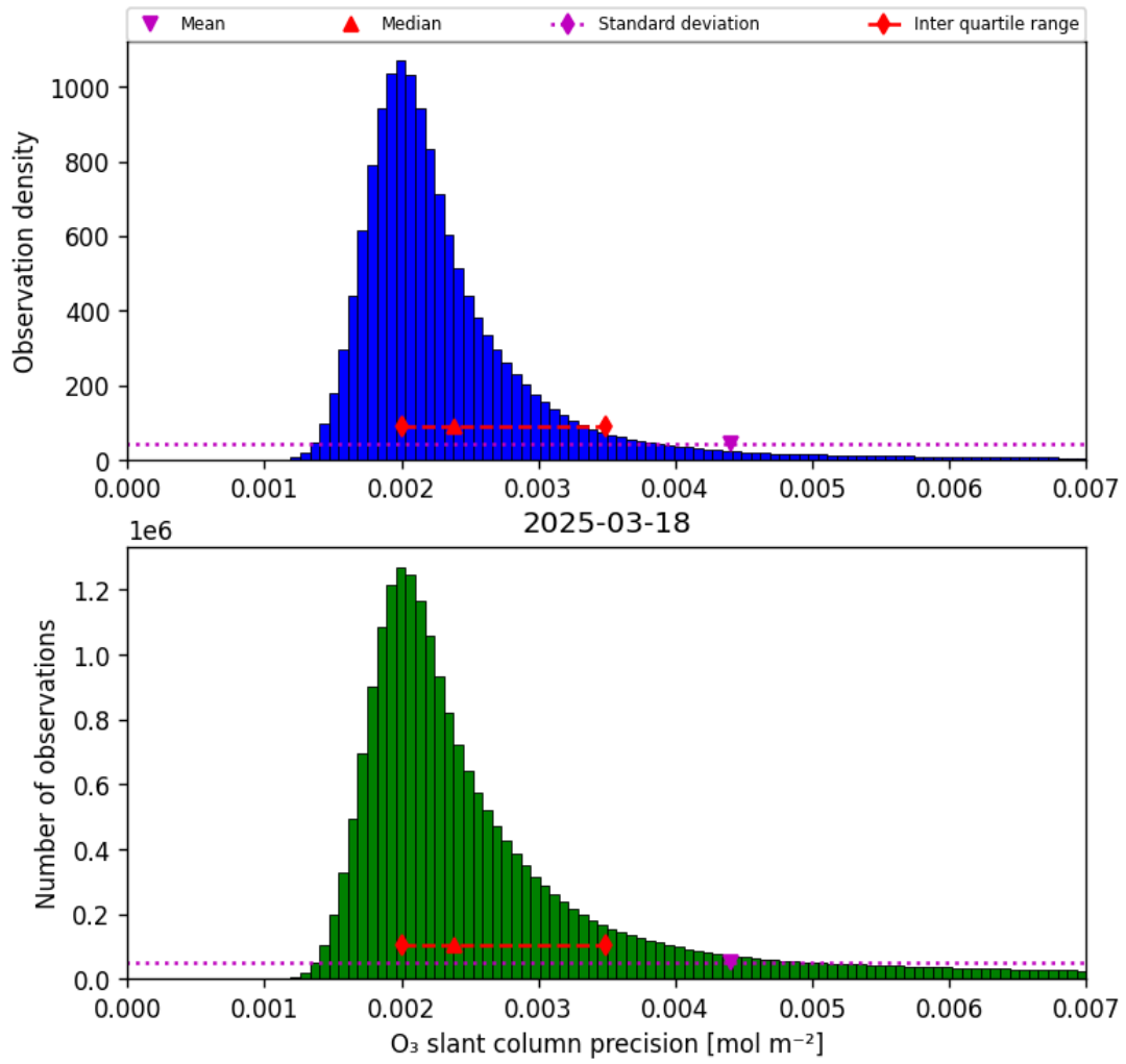
Figure 32: Histogram of “O 3 slant column precision” for 2025-03-18 to 2025-03-19
