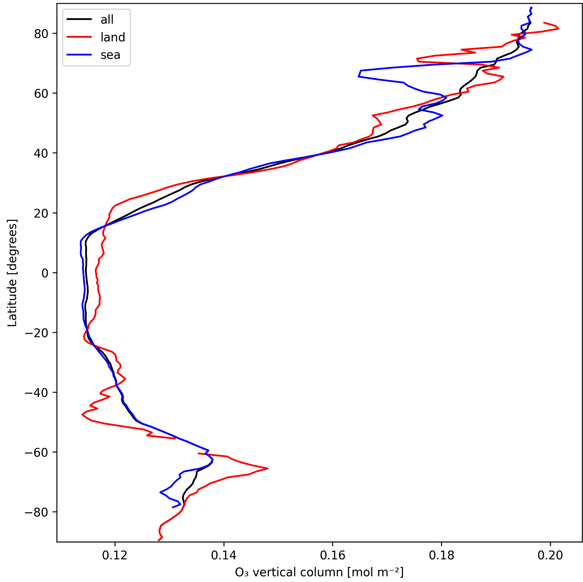
Figure 17: Zonal average of “O 3 vertical column” for 2025-03-18 to 2025-03-19.
