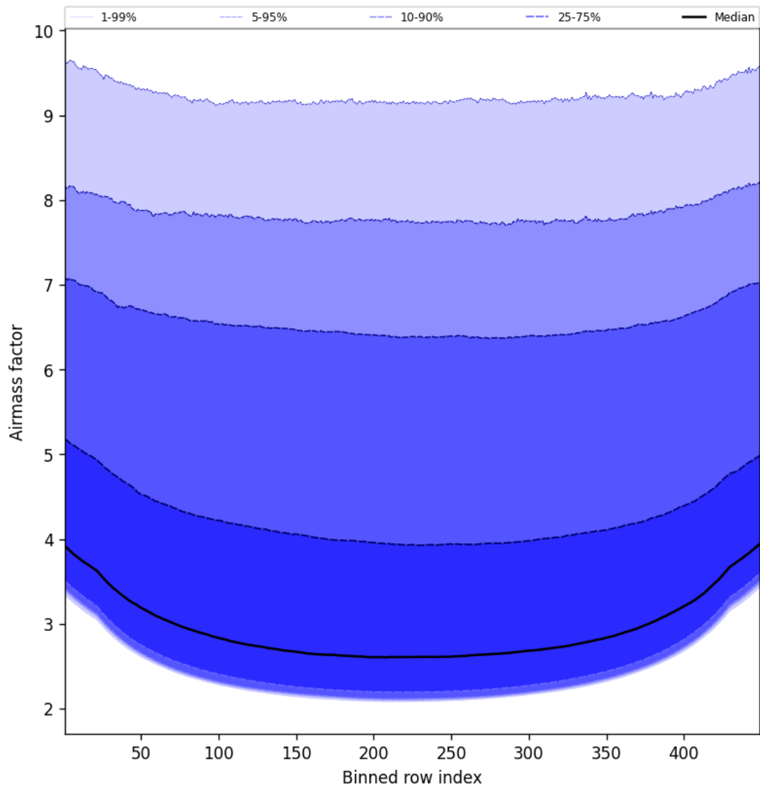
Figure 49: Along track statistics of “Airmass factor” for 2025-03-18 to 2025-03-19
