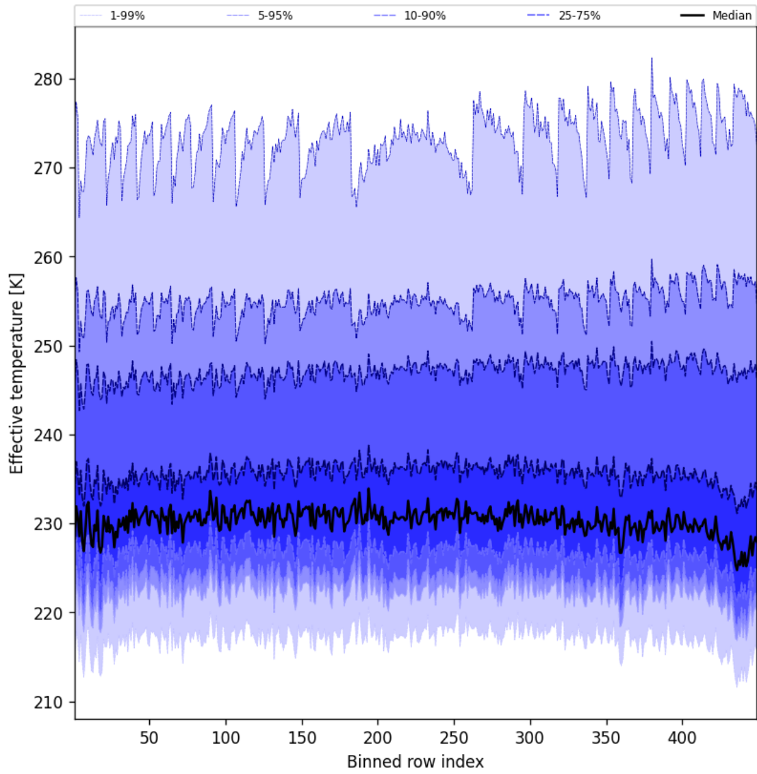
Figure 50: Along track statistics of “Effective temperature” for 2025-03-18 to 2025-03-19
