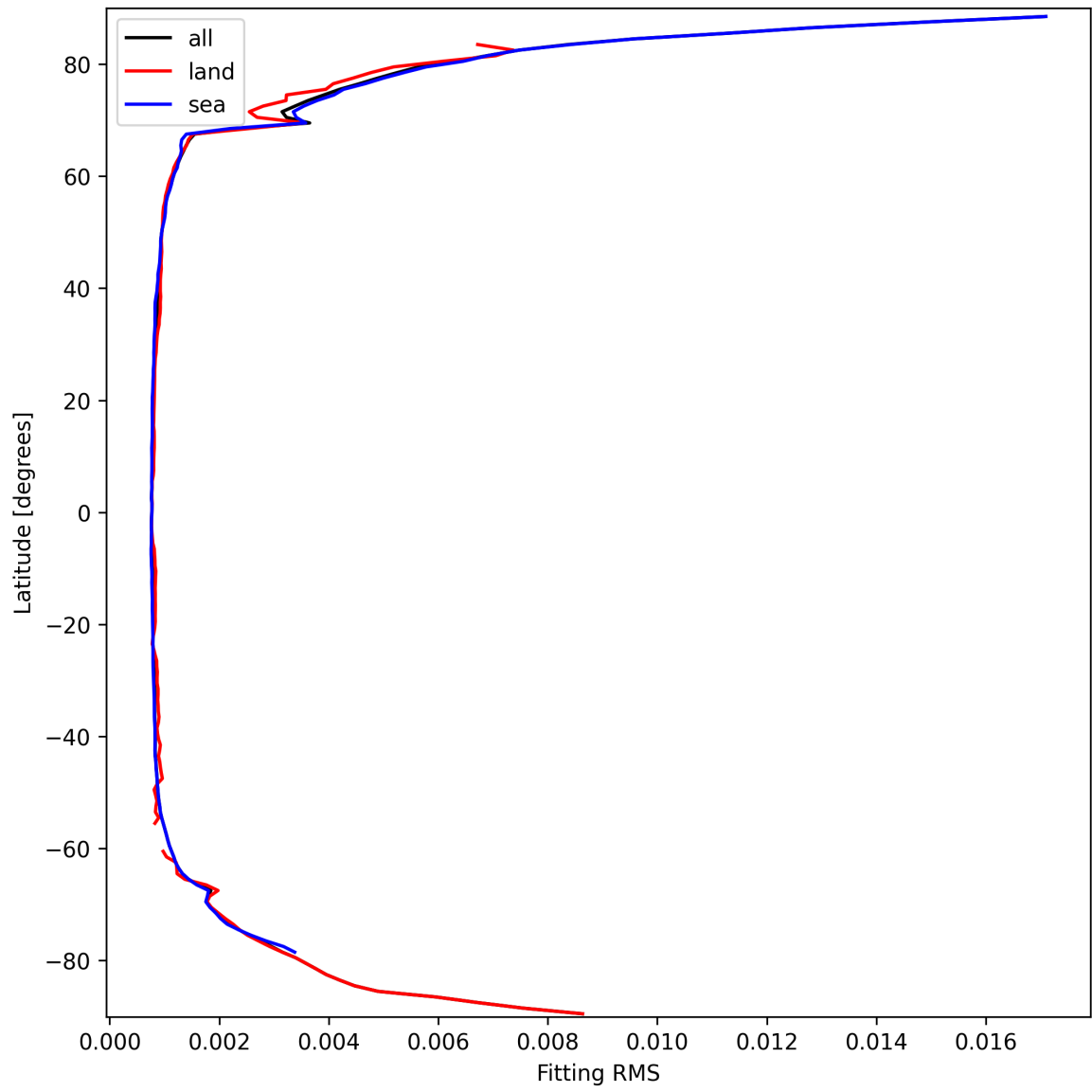
Figure 22: Zonal average of “Fitting RMS” for 2025-03-18 to 2025-03-19.
