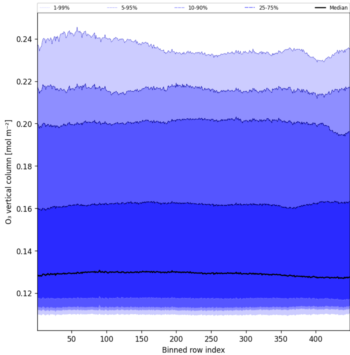
Figure 41: Along track statistics of “O 3 vertical column” for 2025-03-18 to 2025-03-19
