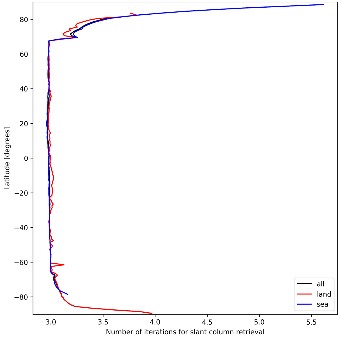
Figure 21: Zonal average of “Number of iterations for slant column retrieval” for 2025-03-18 to 2025-03-19.
