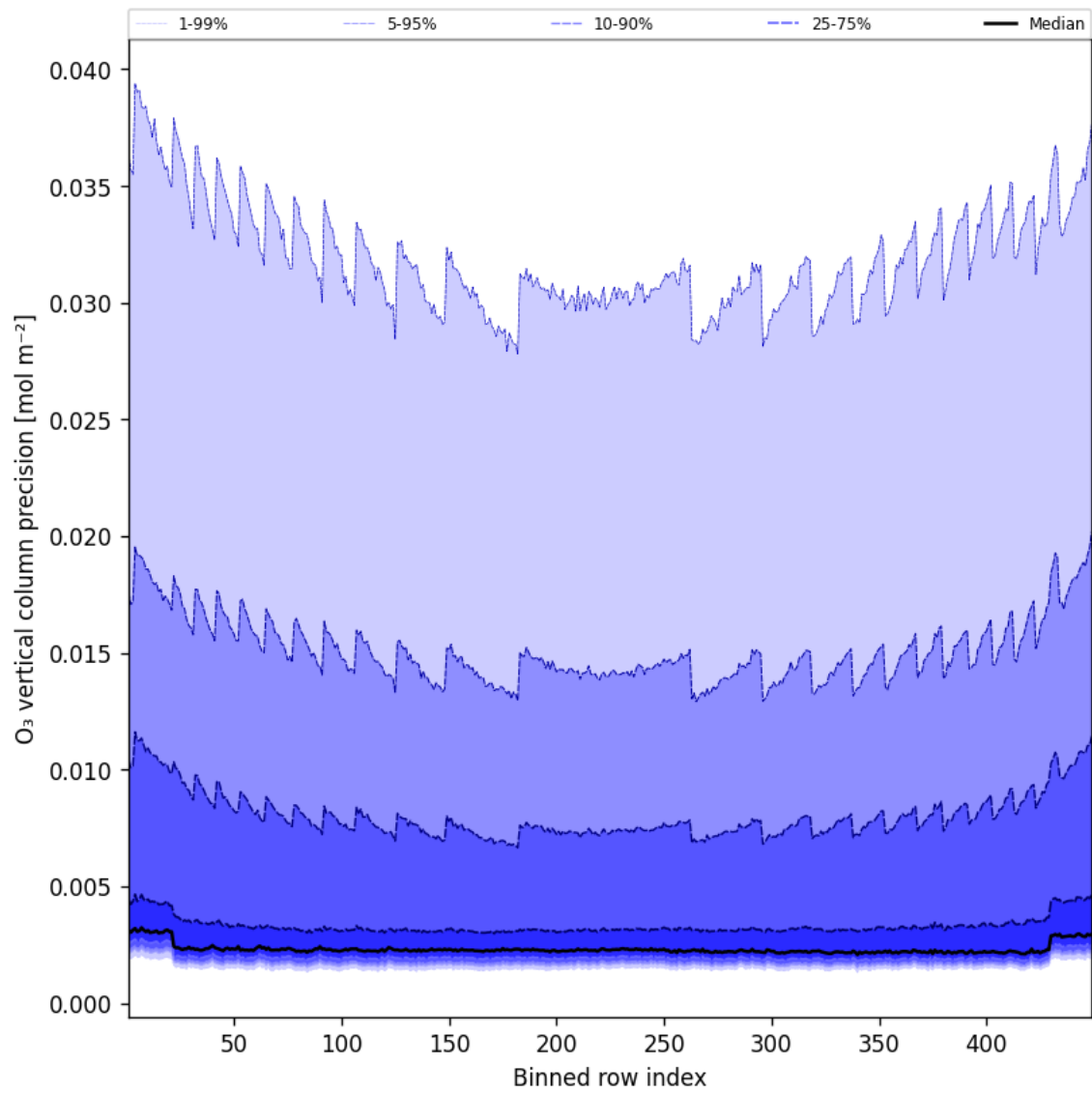
Figure 42: Along track statistics of “O 3 vertical column precision” for 2025-03-18 to 2025-03-19
