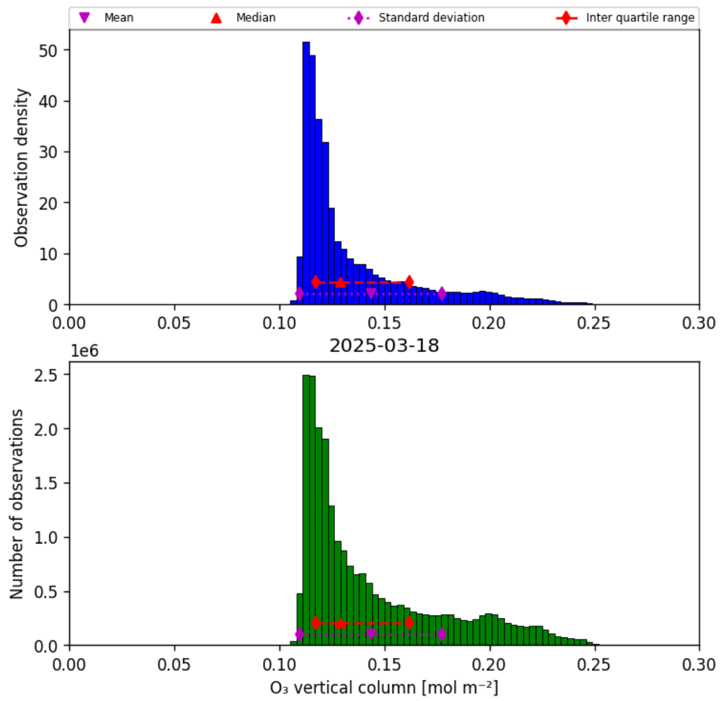
Figure 29: Histogram of “O 3 vertical column” for 2025-03-18 to 2025-03-19
