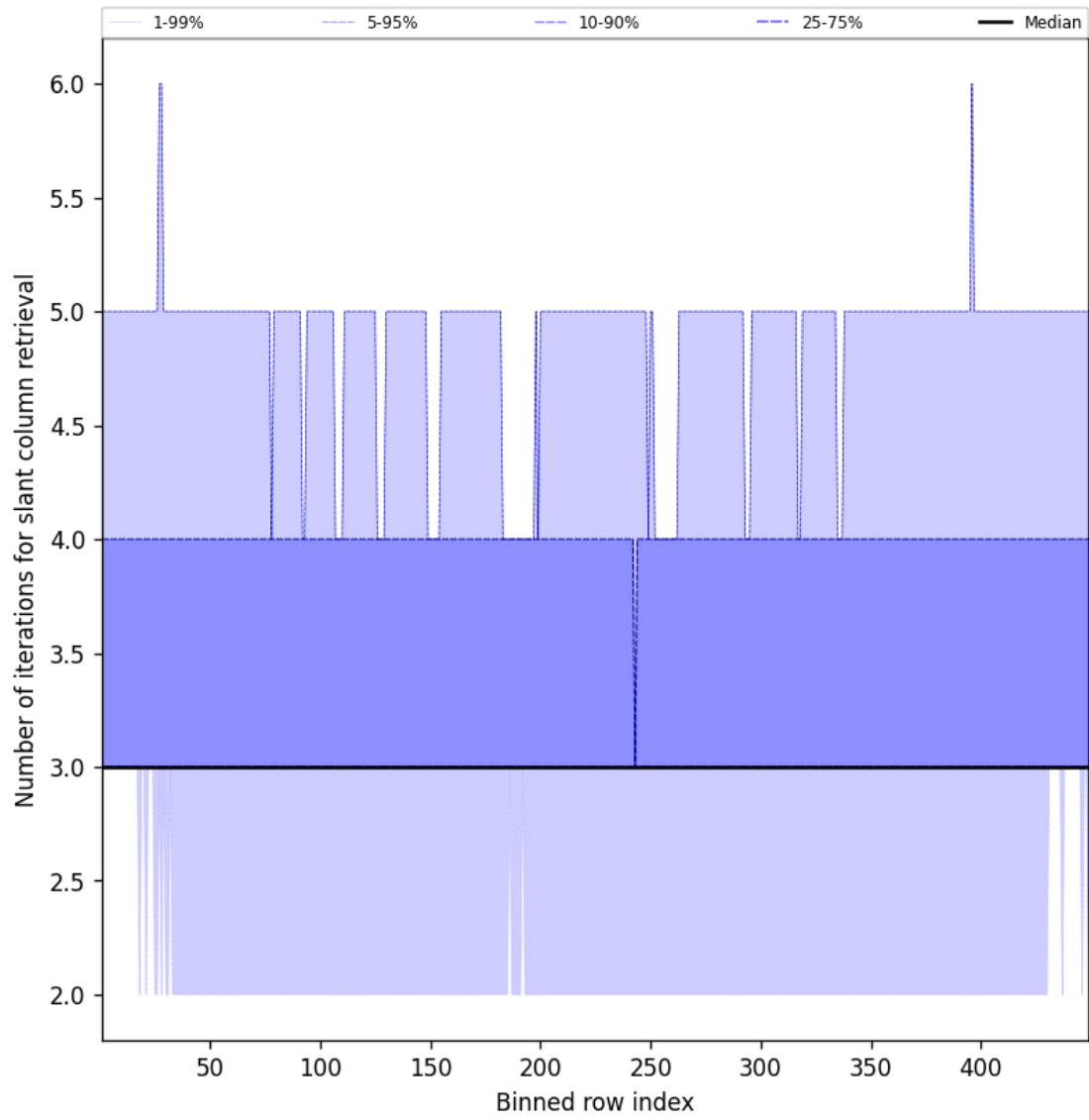
Figure 45: Along track statistics of “Number of iterations for slant column retrieval” for 2025-03-18 to 2025-03-19
