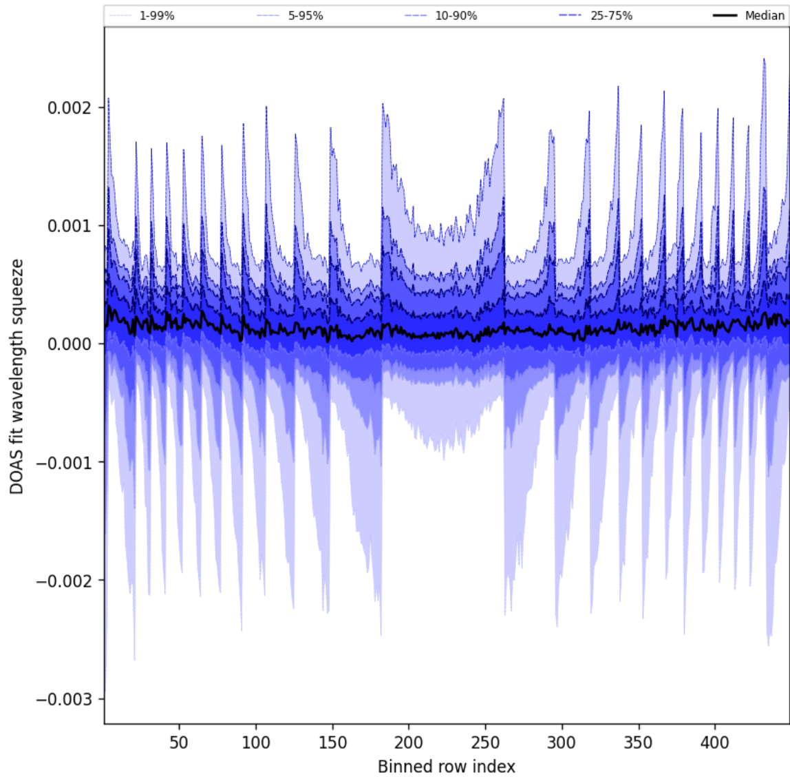
Figure 48: Along track statistics of “DOAS fit wavelength squeeze” for 2025-03-18 to 2025-03-19
