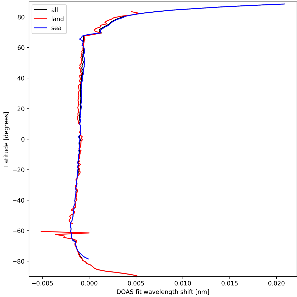
Figure 23: Zonal average of “DOAS fit wavelength shift” for 2025-03-18 to 2025-03-19.
