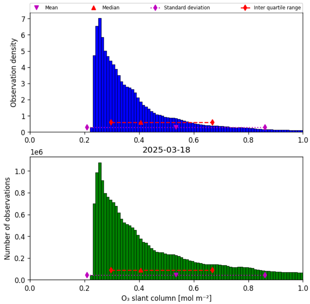
Figure 31: Histogram of “O 3 slant column” for 2025-03-18 to 2025-03-19
