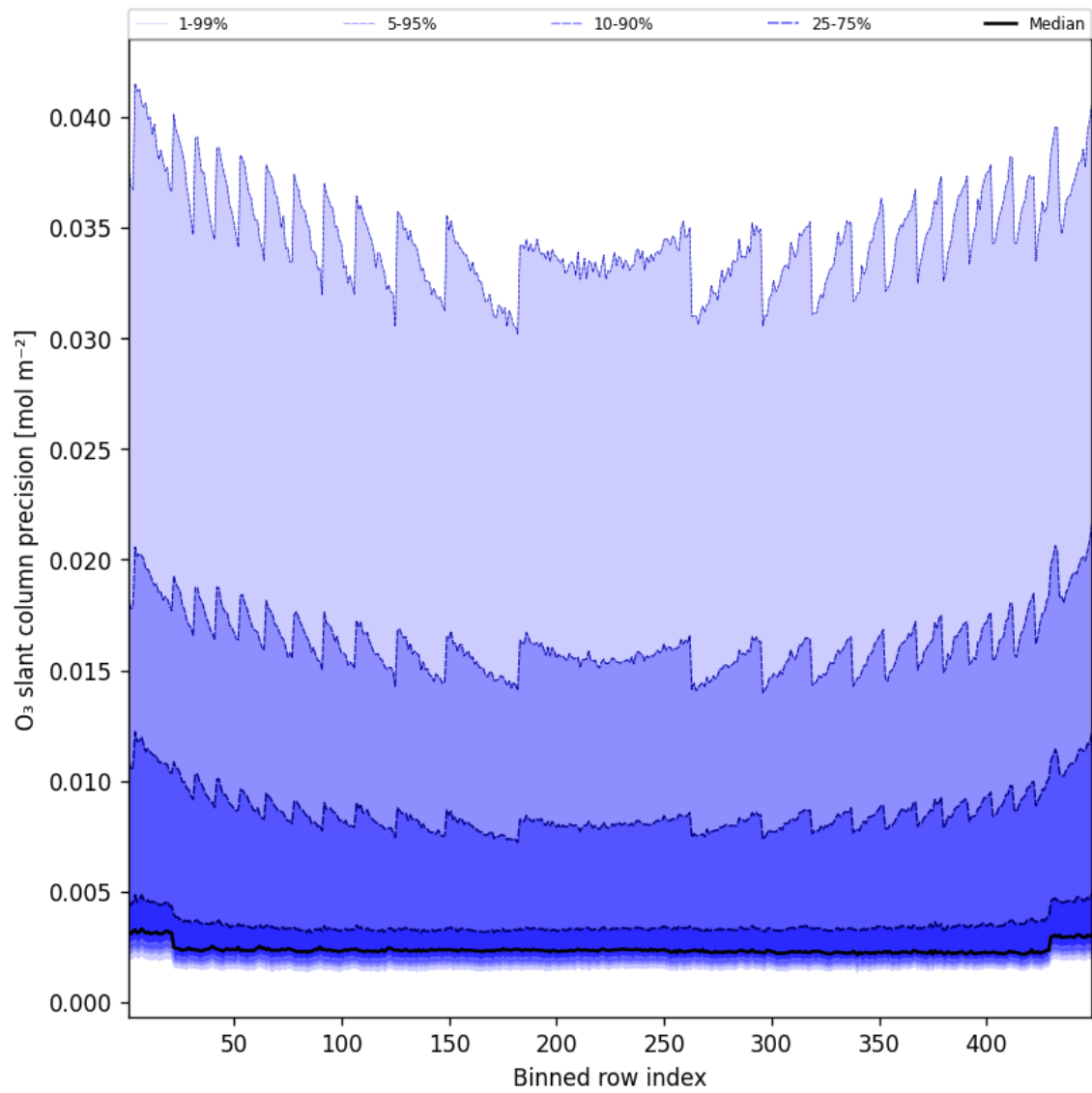
Figure 44: Along track statistics of “O 3 slant column precision” for 2025-03-18 to 2025-03-19
