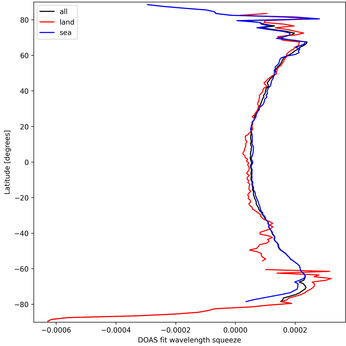
Figure 24: Zonal average of “DOAS fit wavelength squeeze” for 2025-03-18 to 2025-03-19.
