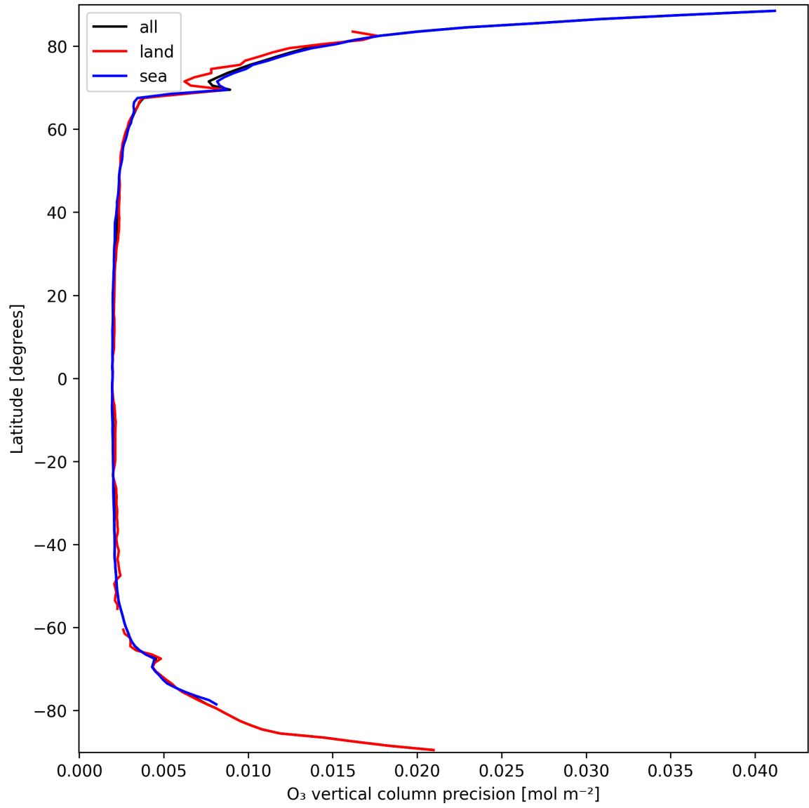
Figure 18: Zonal average of “O 3 vertical column precision” for 2025-03-18 to 2025-03-19.
