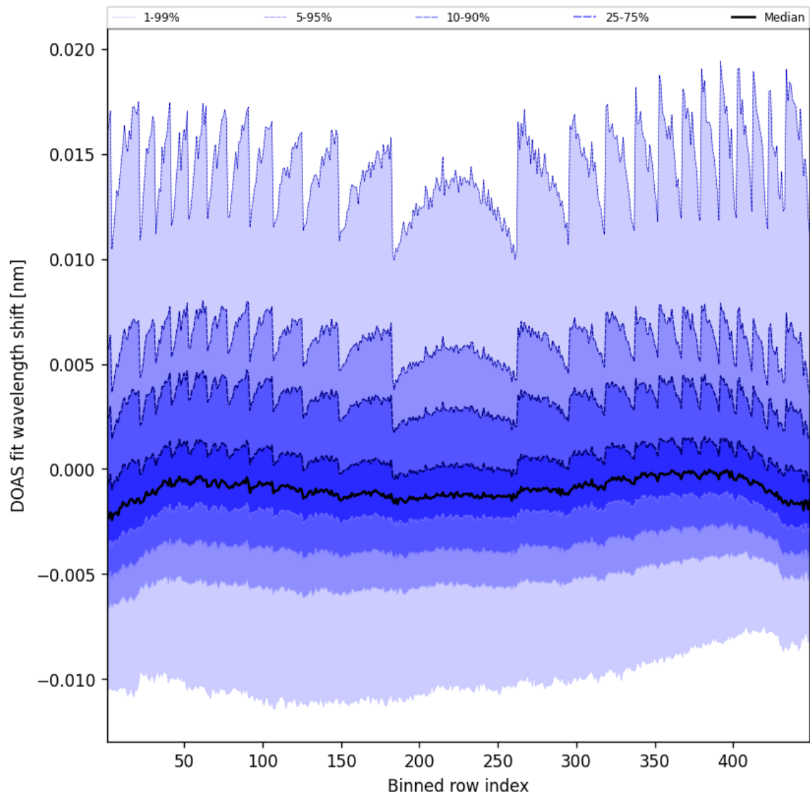
Figure 47: Along track statistics of “DOAS fit wavelength shift” for 2025-03-18 to 2025-03-19
