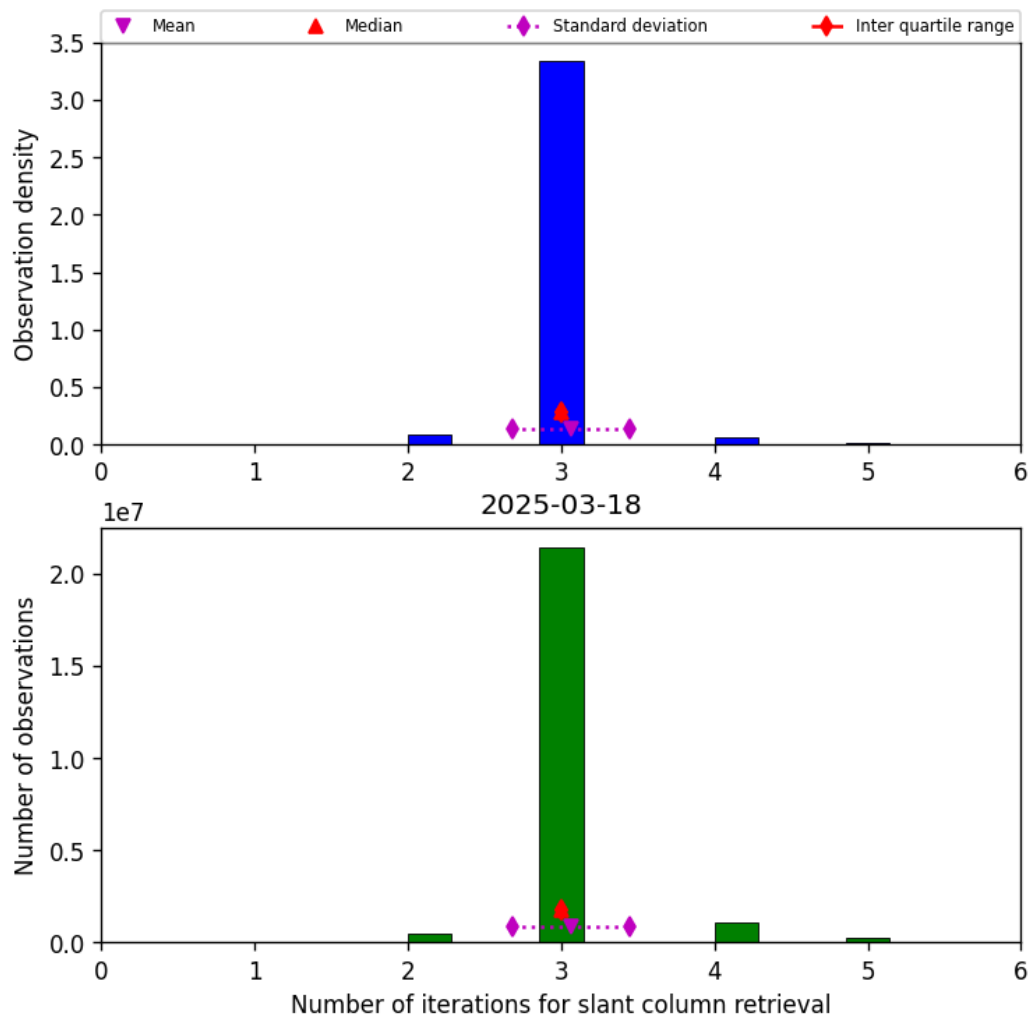
Figure 33: Histogram of “Number of iterations for slant column retrieval” for 2025-03-18 to 2025-03-19
