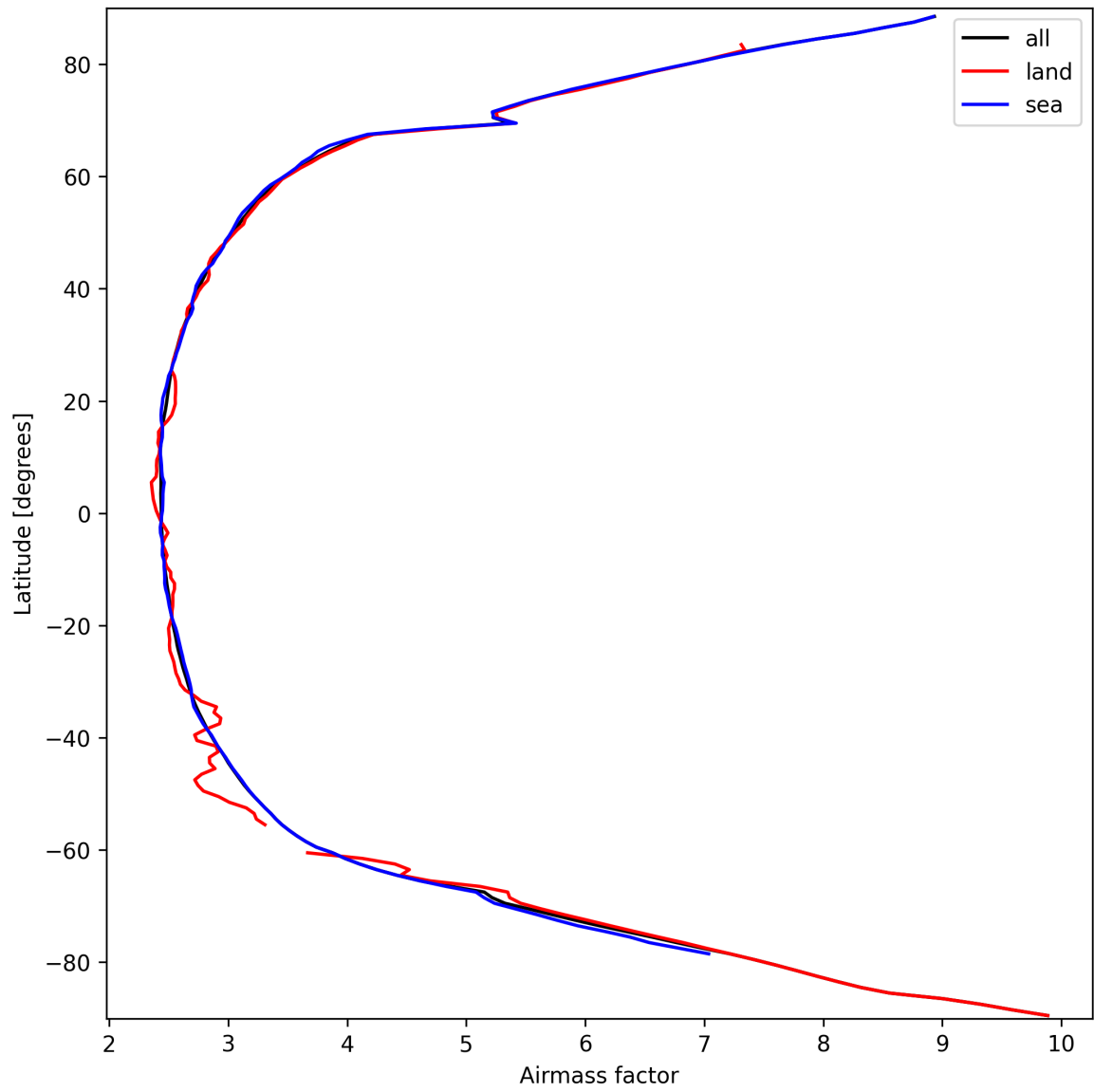
Figure 25: Zonal average of “Airmass factor” for 2025-03-18 to 2025-03-19.
