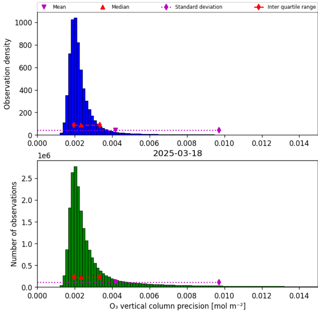
Figure 30: Histogram of “O 3 vertical column precision” for 2025-03-18 to 2025-03-19
