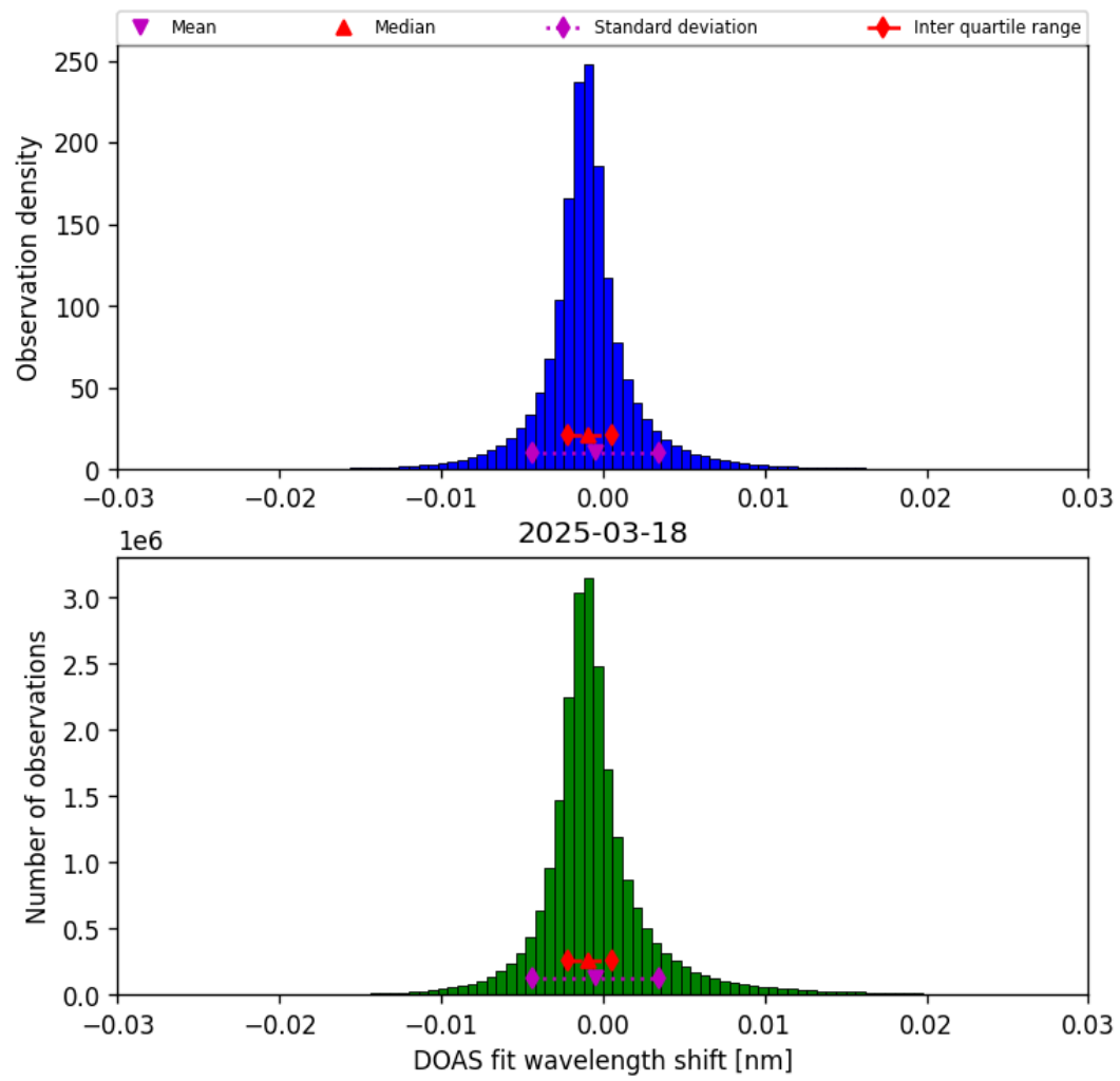
Figure 35: Histogram of “DOAS fit wavelength shift” for 2025-03-18 to 2025-03-19
