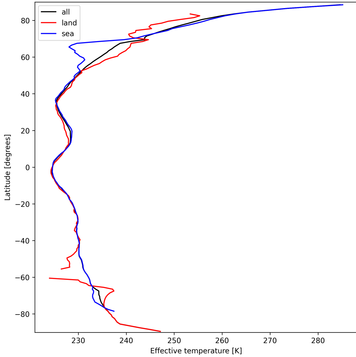
Figure 26: Zonal average of “Effective temperature” for 2025-03-18 to 2025-03-19.
