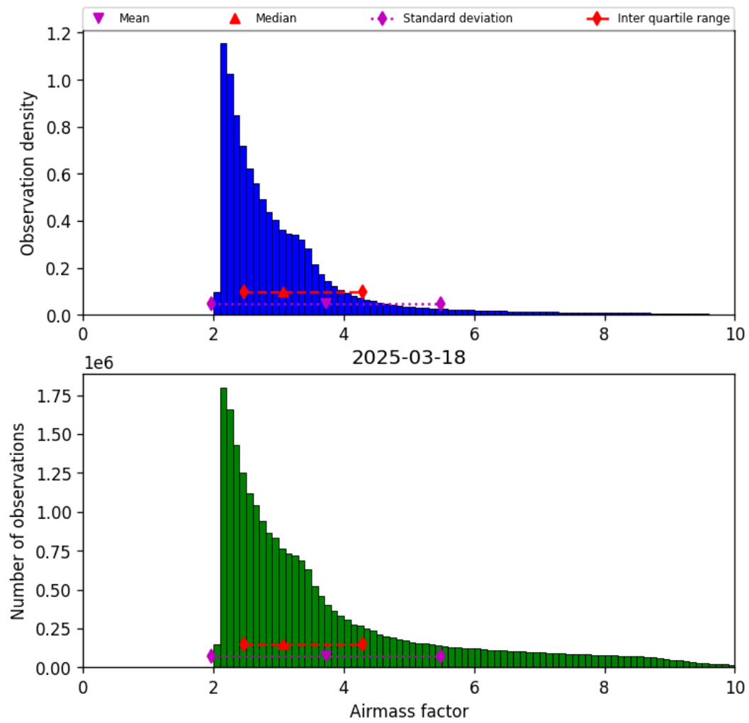
Figure 37: Histogram of “Airmass factor” for 2025-03-18 to 2025-03-19
