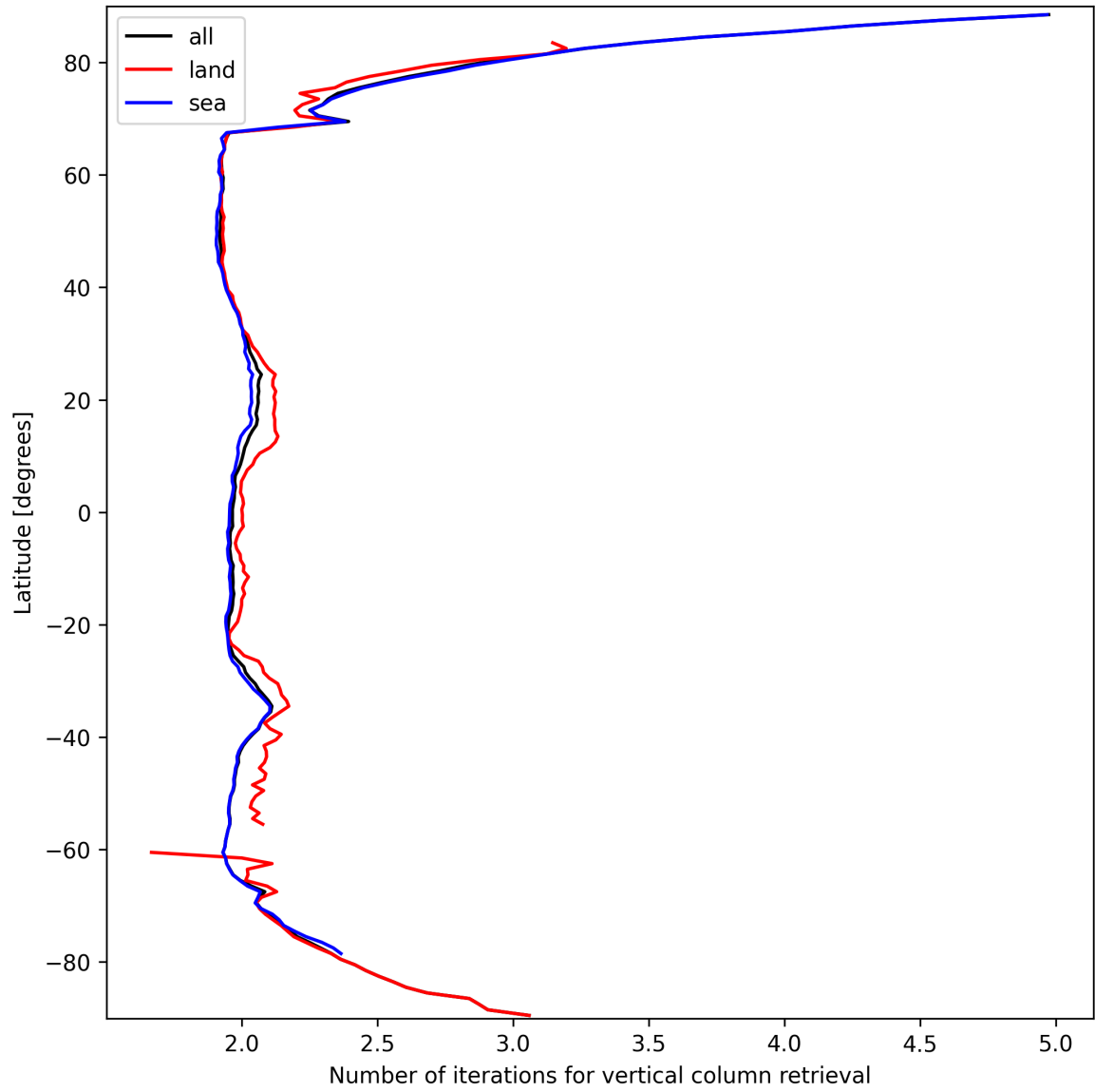
Figure 27: Zonal average of “Number of iterations for vertical column retrieval” for 2025-03-18 to 2025-03-19.
