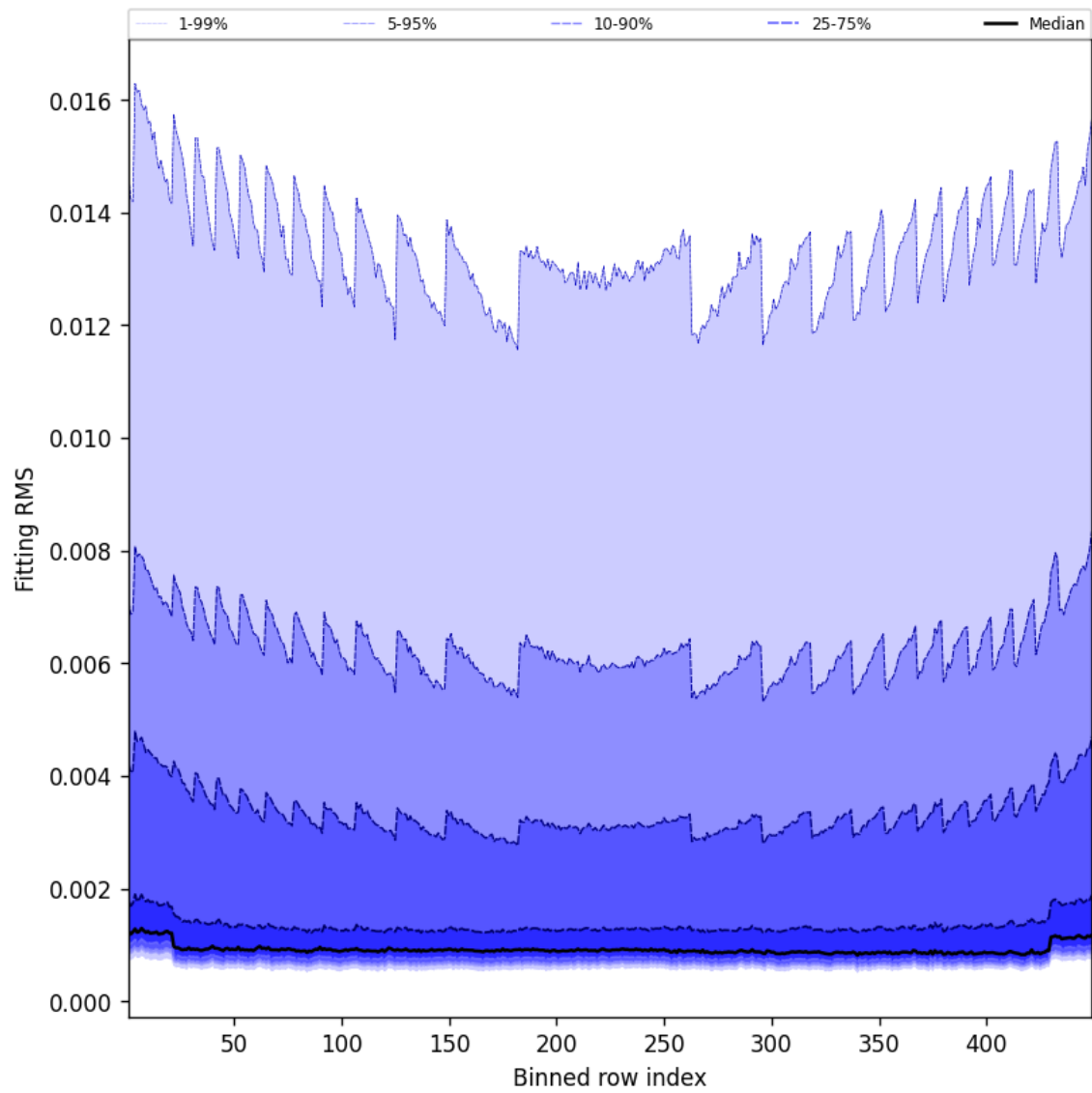
Figure 46: Along track statistics of “Fitting RMS” for 2025-03-18 to 2025-03-19
