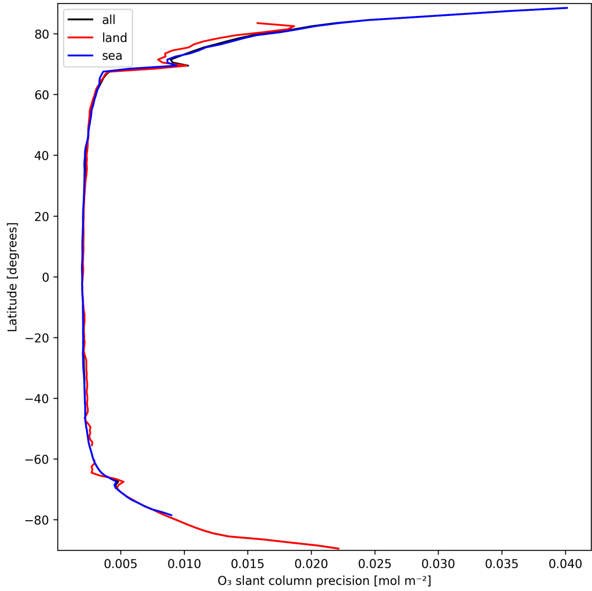
Figure 20: Zonal average of “O 3 slant column precision” for 2025-03-19 to 2025-03-20.
