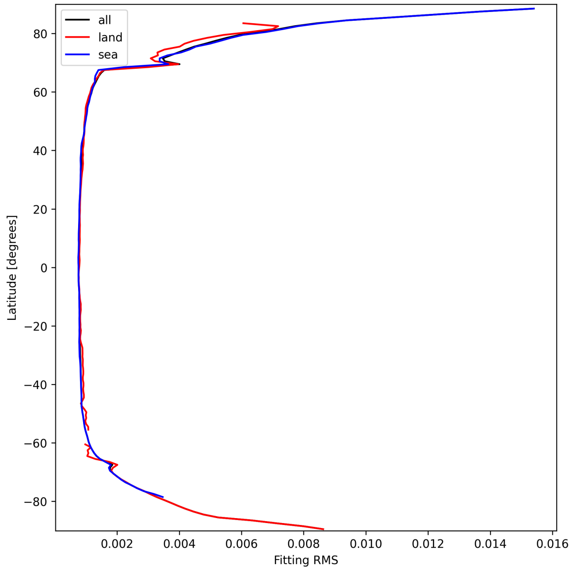
Figure 22: Zonal average of “Fitting RMS” for 2025-03-19 to 2025-03-20.
