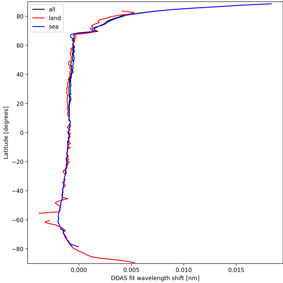
Figure 23: Zonal average of “DOAS fit wavelength shift” for 2025-03-19 to 2025-03-20.
