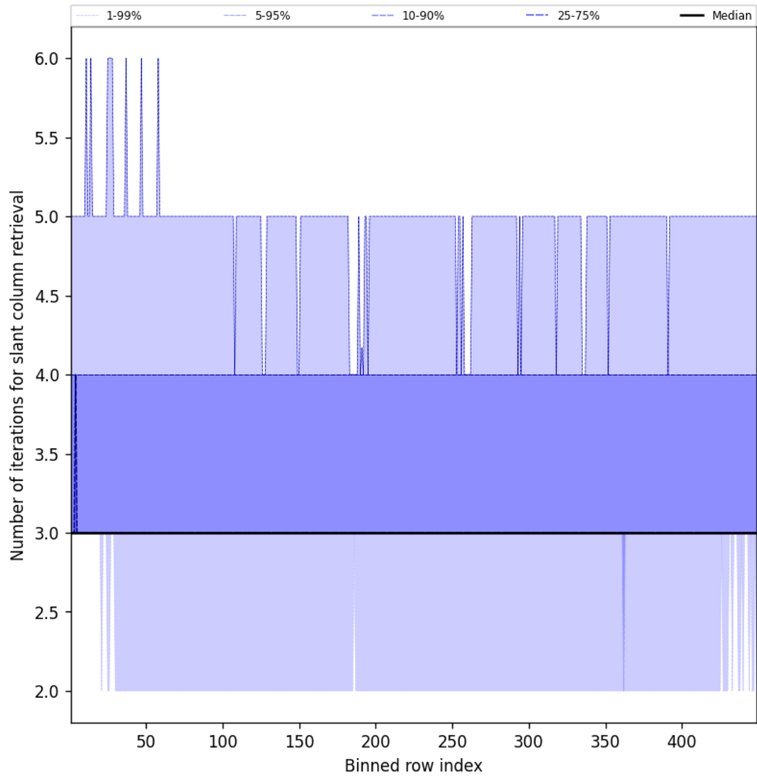
Figure 45: Along track statistics of “Number of iterations for slant column retrieval” for 2025-03-19 to 2025-03-20
