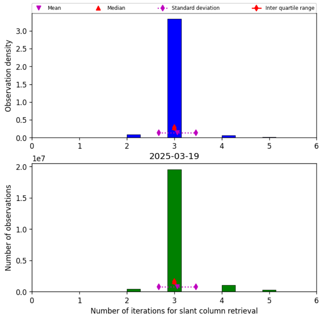
Figure 33: Histogram of “Number of iterations for slant column retrieval” for 2025-03-19 to 2025-03-20
