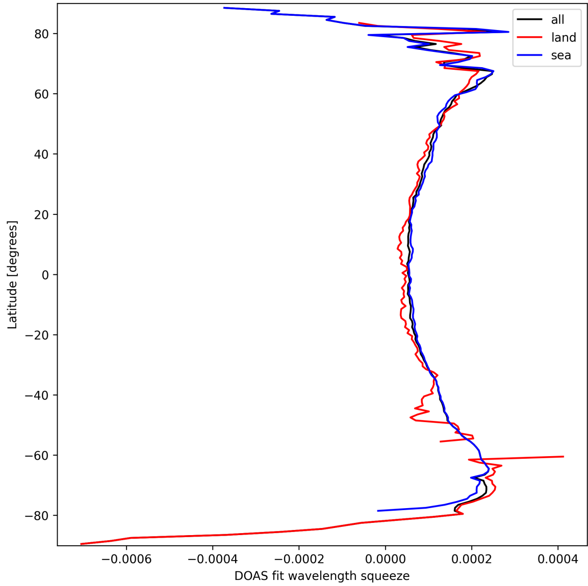
Figure 24: Zonal average of “DOAS fit wavelength squeeze” for 2025-03-19 to 2025-03-20.
