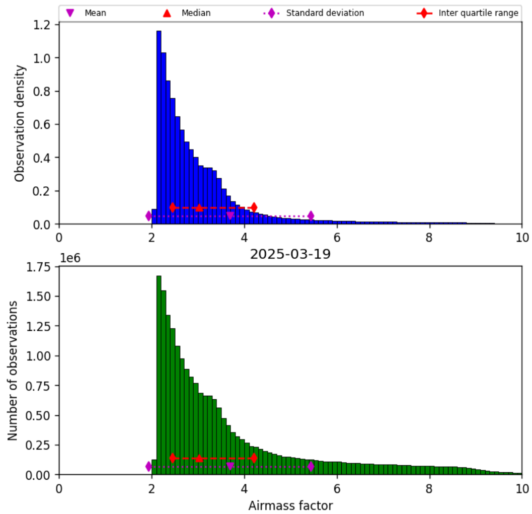
Figure 37: Histogram of “Airmass factor” for 2025-03-19 to 2025-03-20
