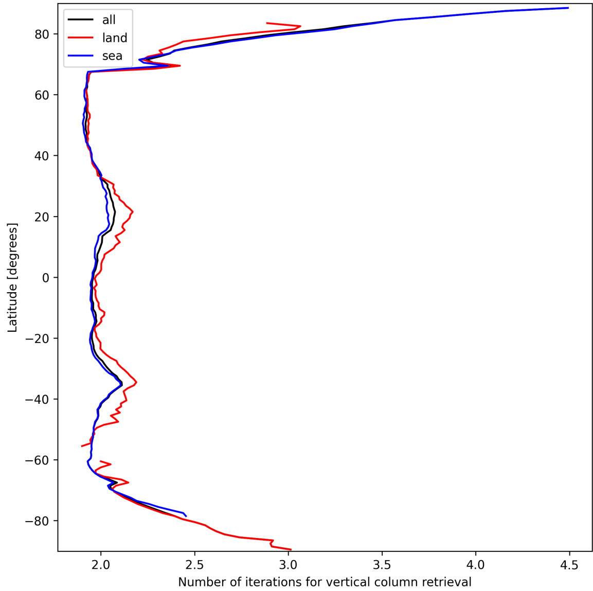
Figure 27: Zonal average of “Number of iterations for vertical column retrieval” for 2025-03-19 to 2025-03-20.
