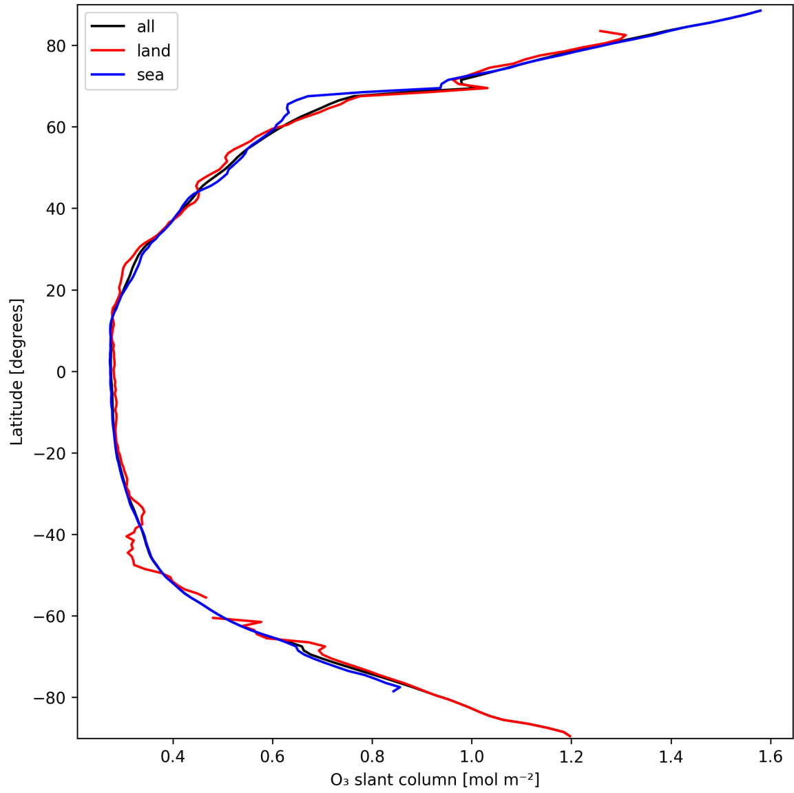
Figure 19: Zonal average of “O 3 slant column” for 2025-03-19 to 2025-03-20.
