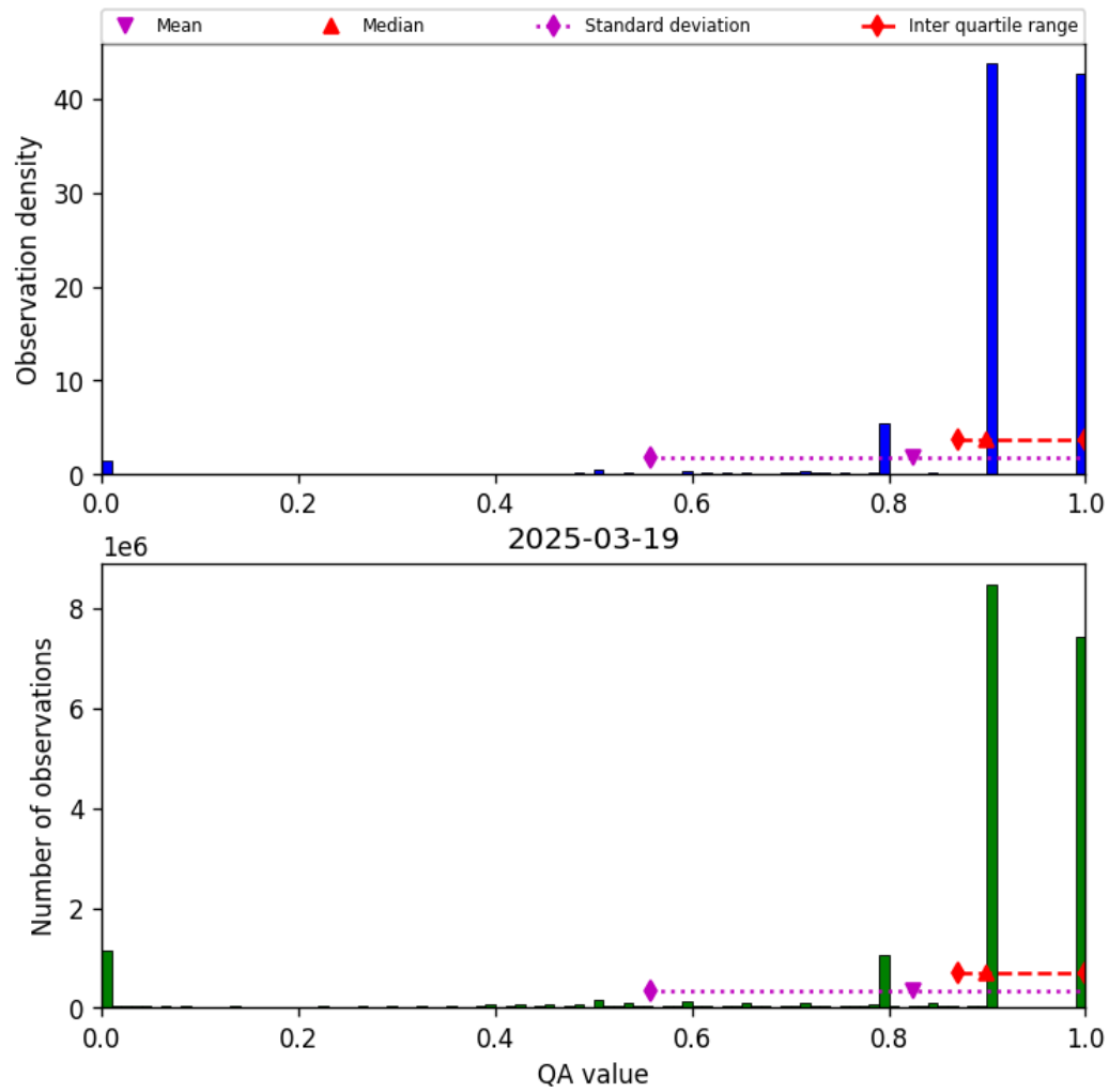
Figure 28: Histogram of “QA value” for 2025-03-19 to 2025-03-20
