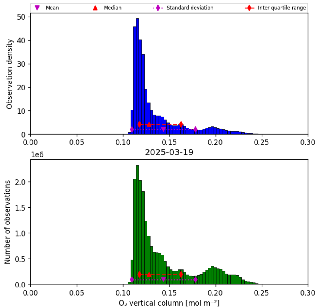
Figure 29: Histogram of “O 3 vertical column” for 2025-03-19 to 2025-03-20
