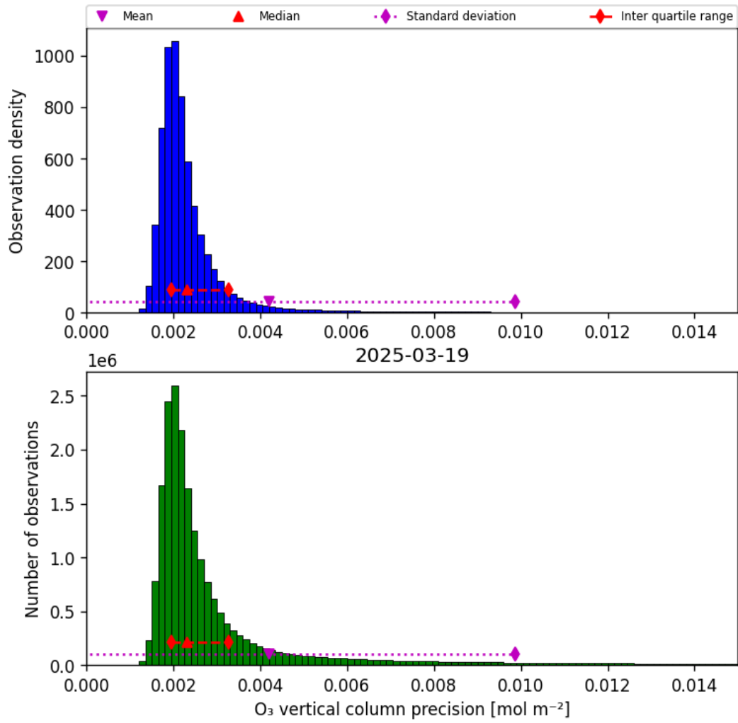
Figure 30: Histogram of “O 3 vertical column precision” for 2025-03-19 to 2025-03-20
