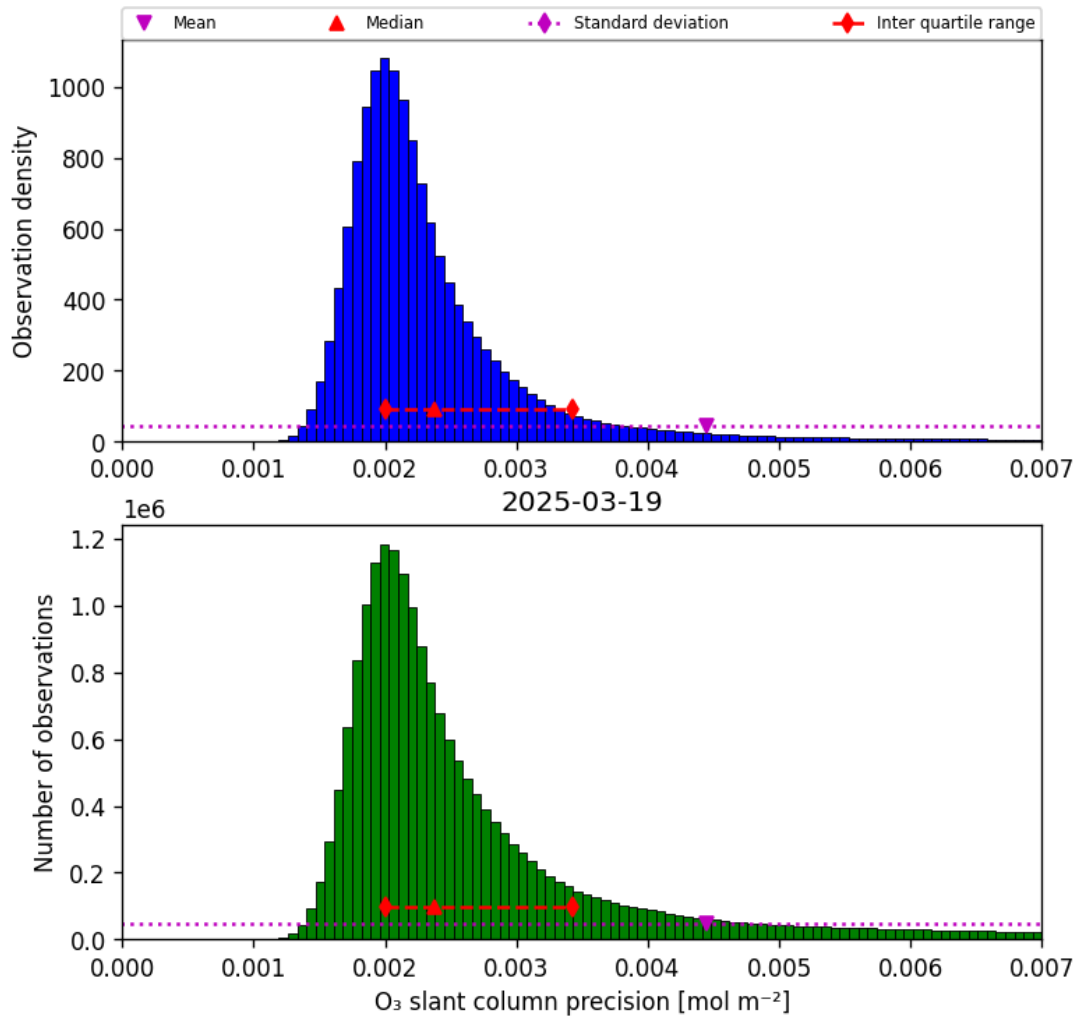
Figure 32: Histogram of “O 3 slant column precision” for 2025-03-19 to 2025-03-20
