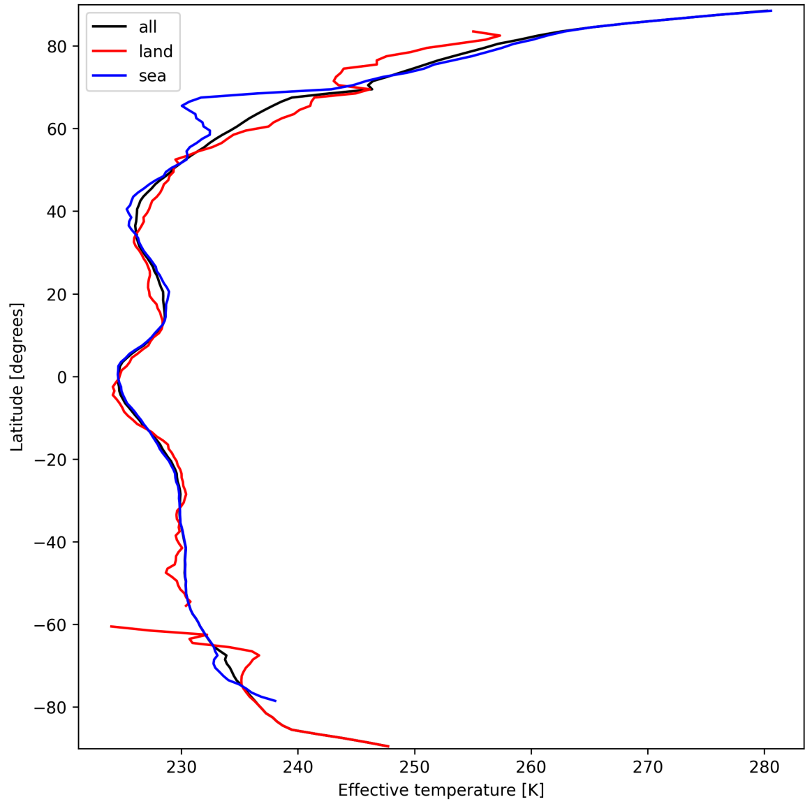
Figure 26: Zonal average of “Effective temperature” for 2025-03-19 to 2025-03-20.
