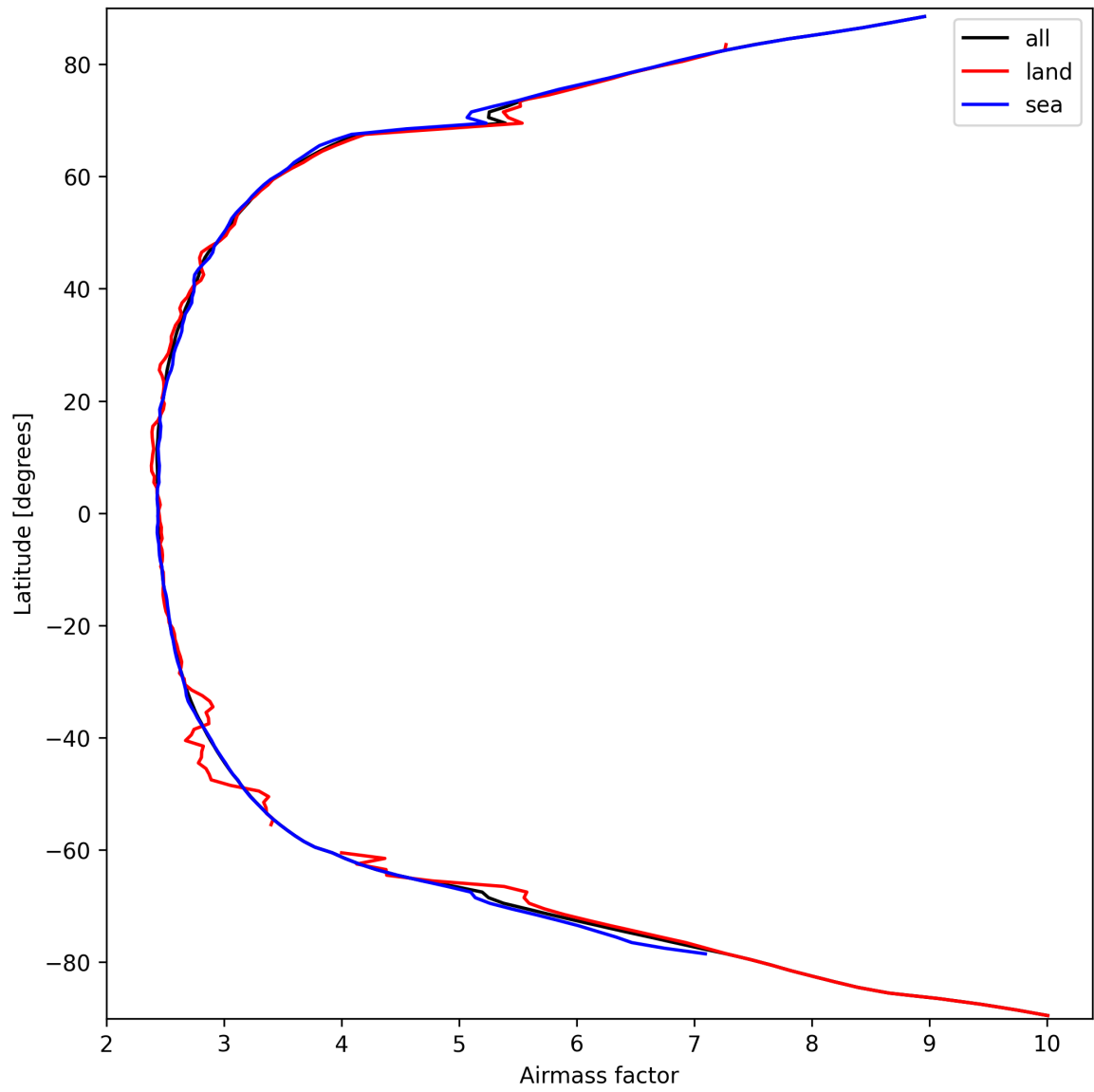
Figure 25: Zonal average of “Airmass factor” for 2025-03-19 to 2025-03-20.
