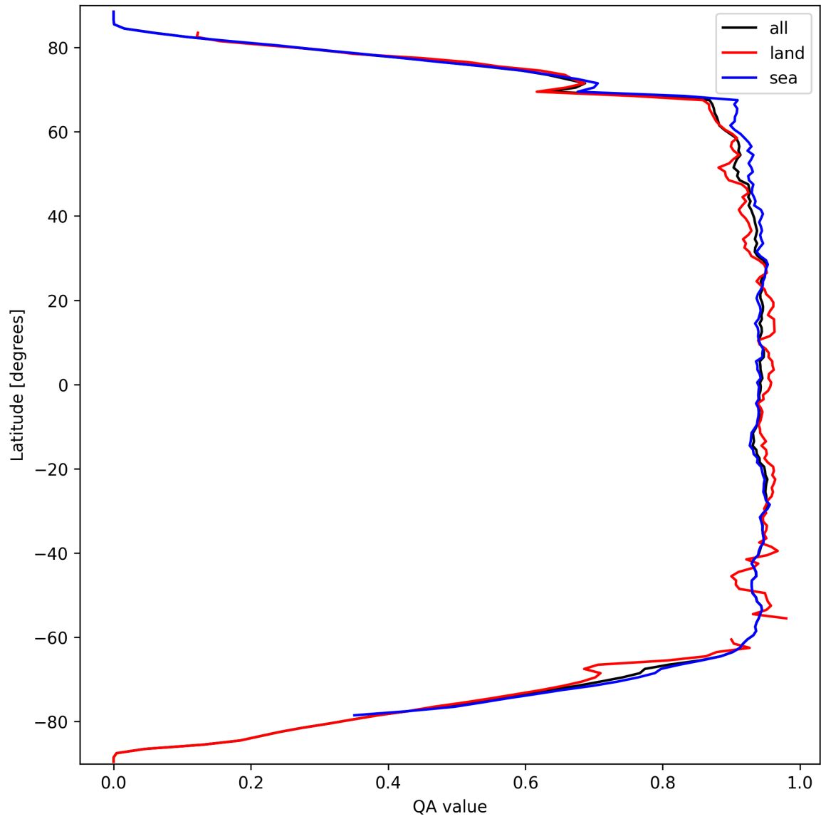
Figure 16: Zonal average of “QA value” for 2025-03-19 to 2025-03-20.
