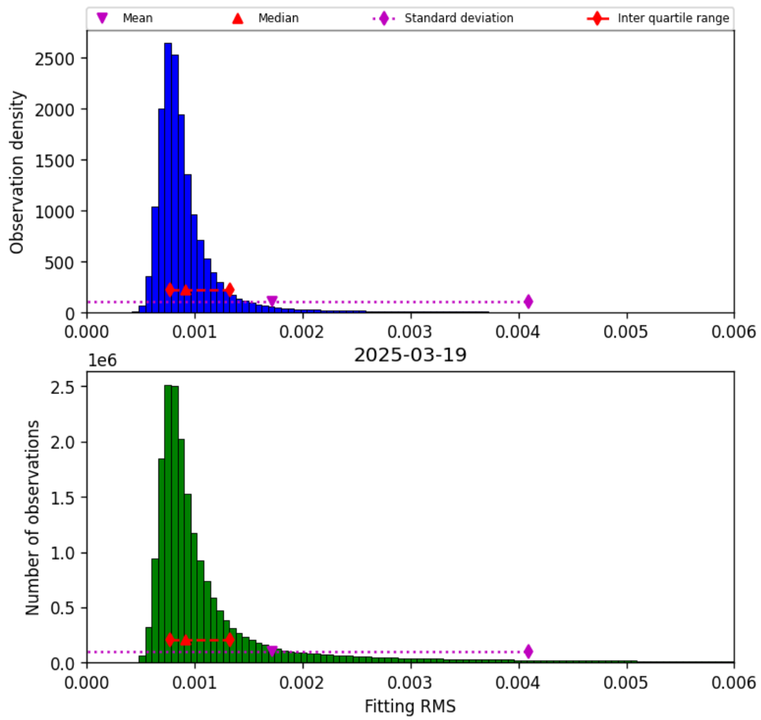
Figure 34: Histogram of “Fitting RMS” for 2025-03-19 to 2025-03-20
