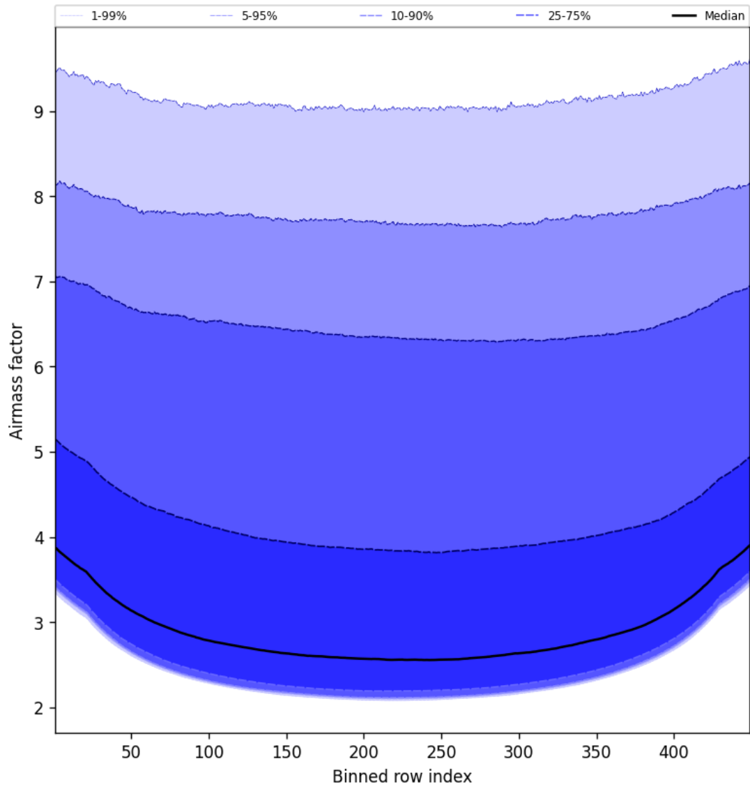
Figure 49: Along track statistics of “Airmass factor” for 2025-03-19 to 2025-03-20
