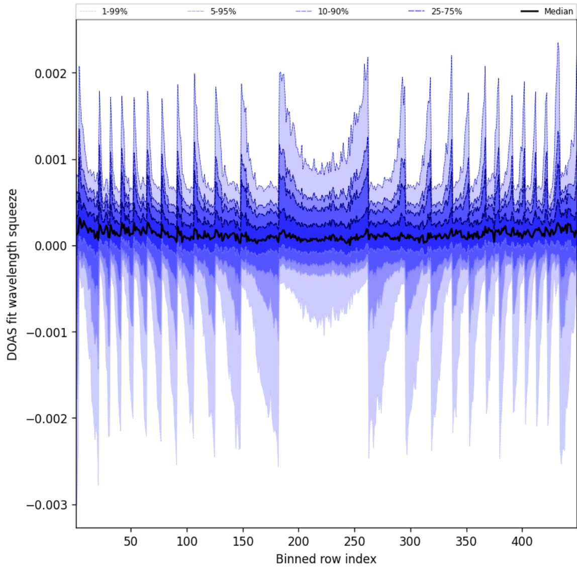
Figure 48: Along track statistics of “DOAS fit wavelength squeeze” for 2025-03-19 to 2025-03-20
