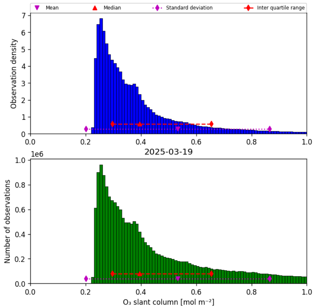
Figure 31: Histogram of “O 3 slant column” for 2025-03-19 to 2025-03-20
