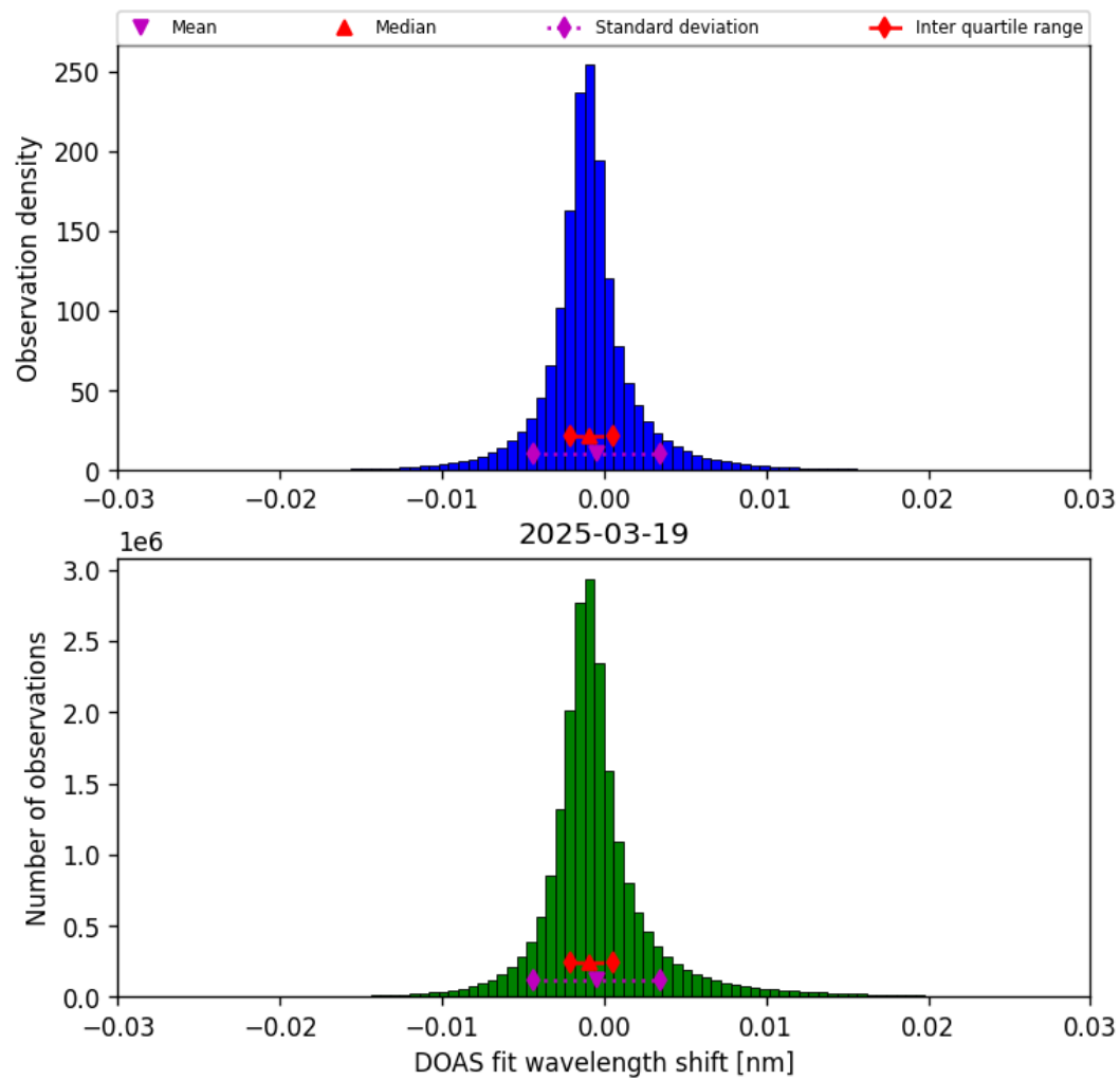
Figure 35: Histogram of “DOAS fit wavelength shift” for 2025-03-19 to 2025-03-20
