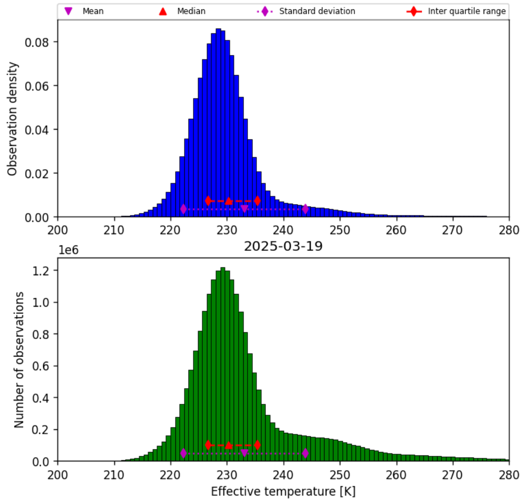
Figure 38: Histogram of “Effective temperature” for 2025-03-19 to 2025-03-20
