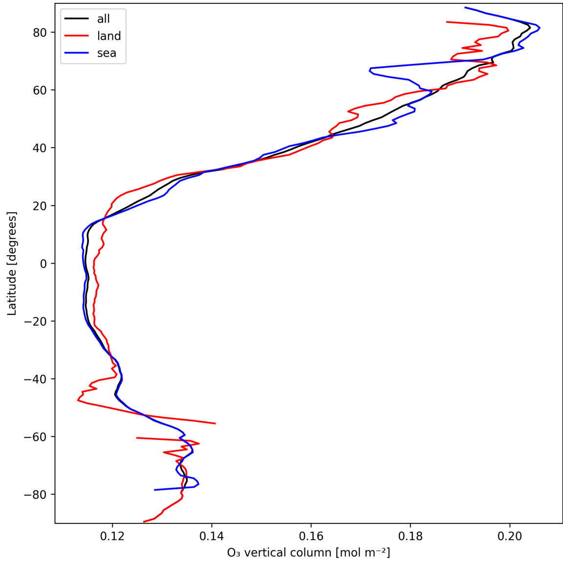
Figure 17: Zonal average of “O 3 vertical column” for 2025-03-19 to 2025-03-20.
