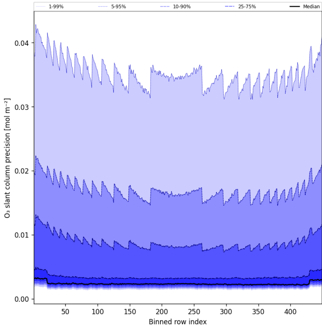
Figure 44: Along track statistics of “O 3 slant column precision” for 2025-03-19 to 2025-03-20
