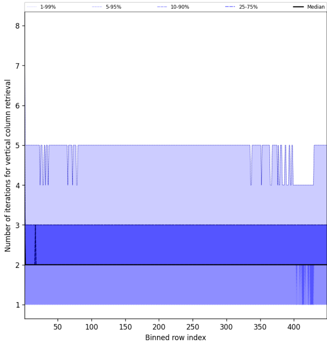
Figure 51: Along track statistics of “Number of iterations for vertical column retrieval” for 2025-03-19 to 2025-03-20
