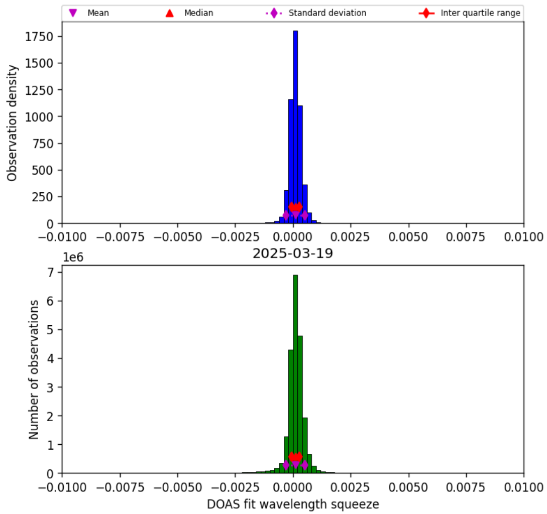
Figure 36: Histogram of “DOAS fit wavelength squeeze” for 2025-03-19 to 2025-03-20
