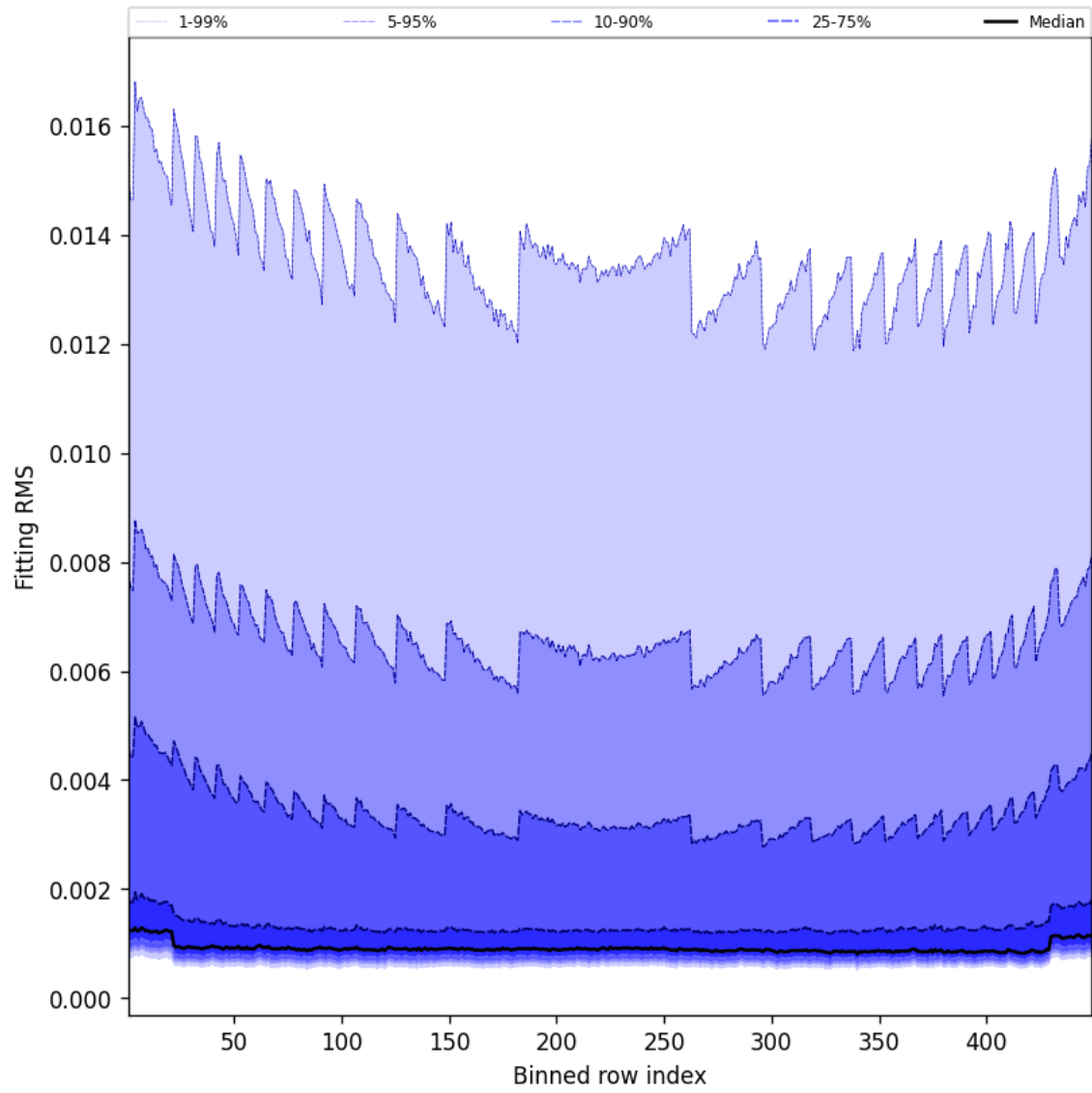
Figure 46: Along track statistics of “Fitting RMS” for 2025-03-19 to 2025-03-20
