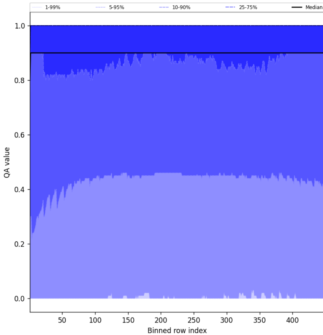
Figure 40: Along track statistics of “QA value” for 2025-03-19 to 2025-03-20
