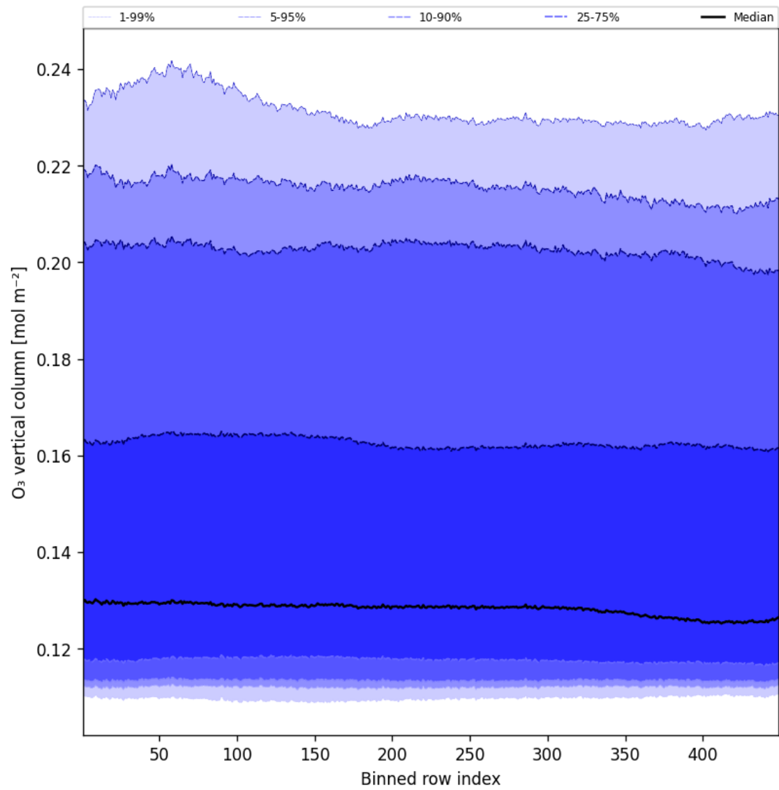
Figure 41: Along track statistics of “ \text{O}_3 vertical column” for 2025-03-19 to 2025-03-20
