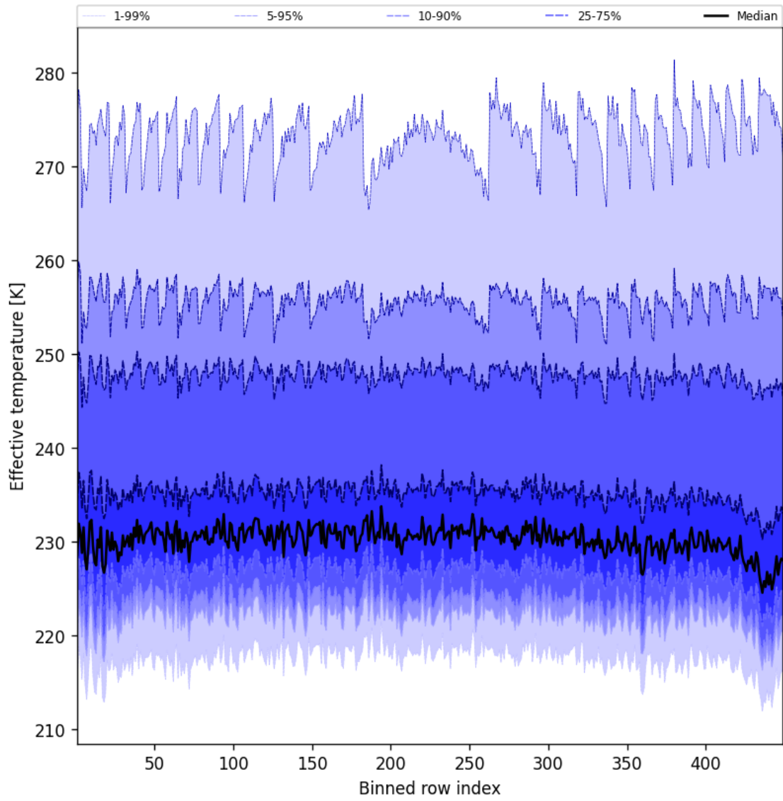
Figure 50: Along track statistics of “Effective temperature” for 2025-03-19 to 2025-03-20
