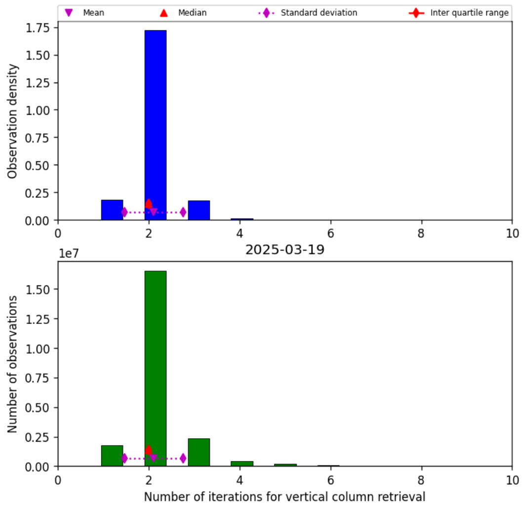
Figure 39: Histogram of “Number of iterations for vertical column retrieval” for 2025-03-19 to 2025-03-20
