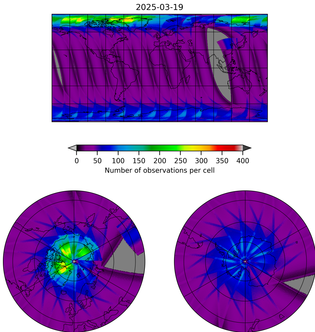
Figure 15: Map of the number of observations for 2025-03-19 to 2025-03-20
