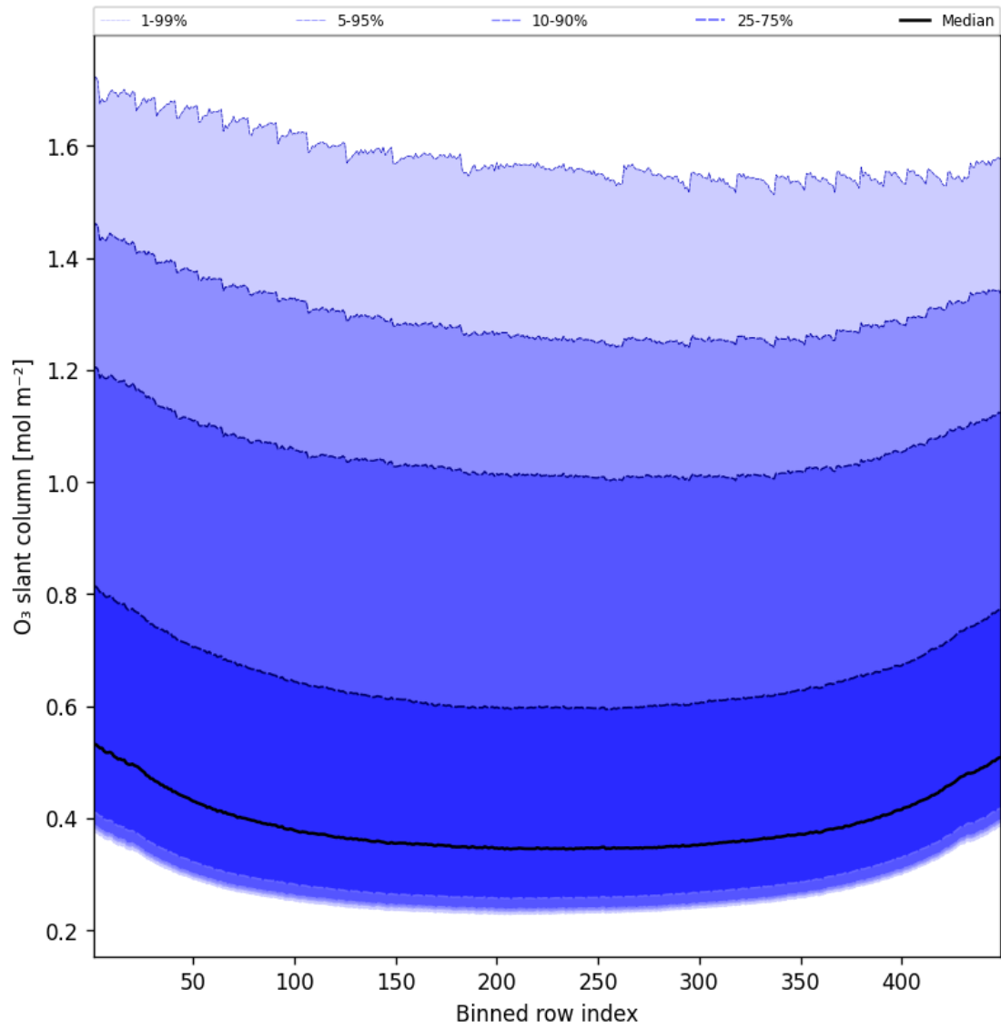
Figure 43: Along track statistics of “O 3 slant column” for 2025-03-19 to 2025-03-20
