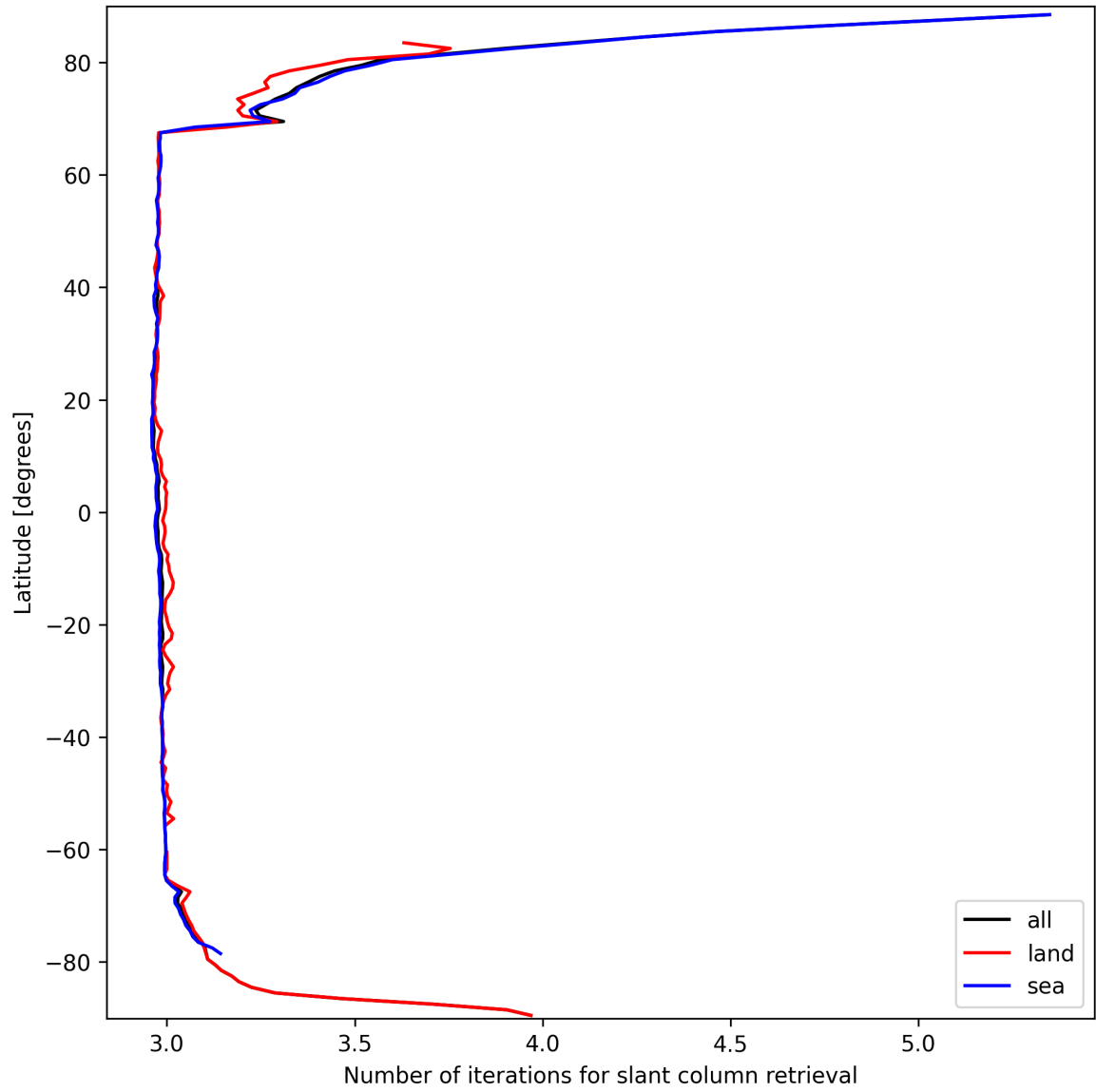
Figure 21: Zonal average of “Number of iterations for slant column retrieval” for 2025-03-19 to 2025-03-20.
