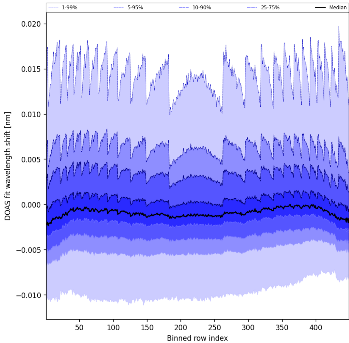
Figure 47: Along track statistics of “DOAS fit wavelength shift” for 2025-03-19 to 2025-03-20
