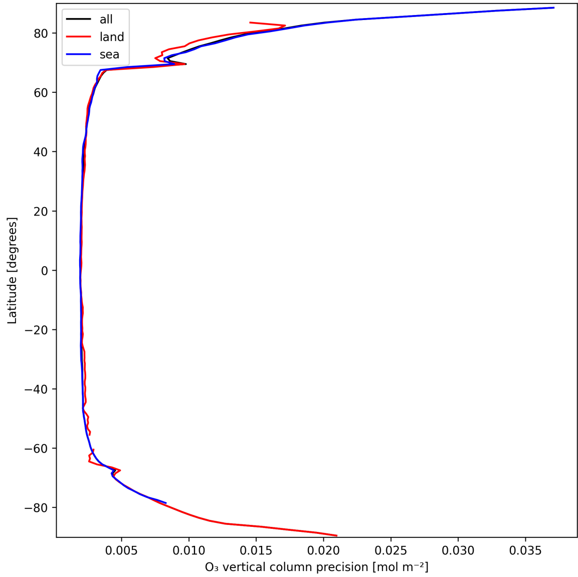
Figure 18: Zonal average of “O 3 vertical column precision” for 2025-03-19 to 2025-03-20.
