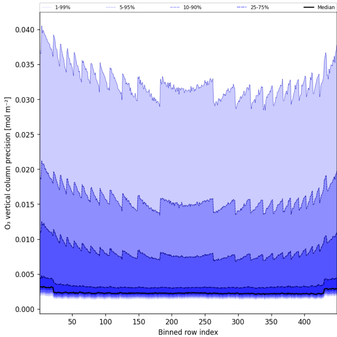
Figure 42: Along track statistics of “O 3 vertical column precision” for 2025-03-19 to 2025-03-20
