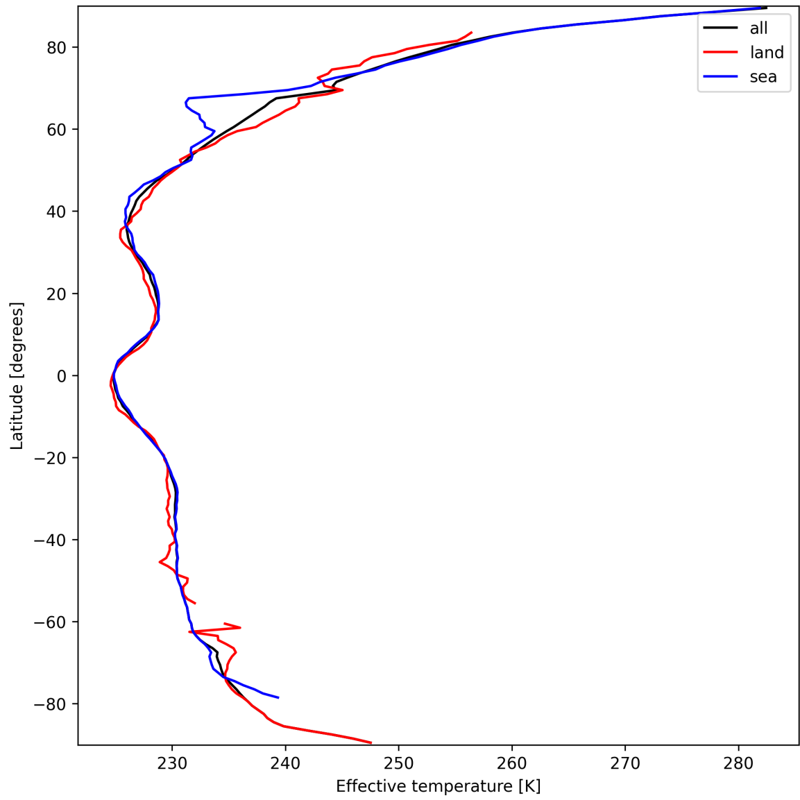
Figure 26: Zonal average of "Effective temperature" for 2025-03-20 to 2025-03-21.
