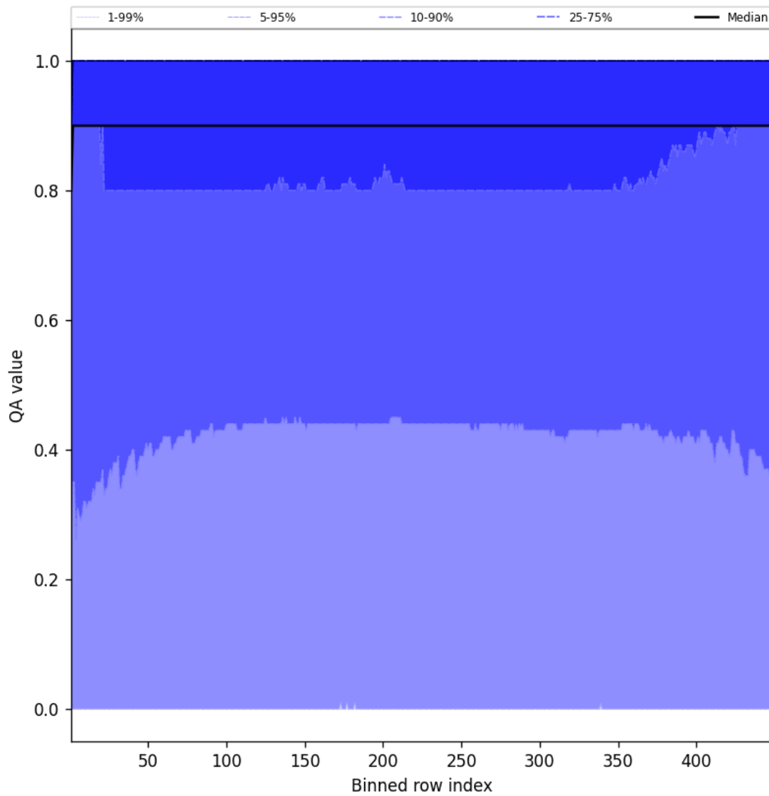
Figure 40: Along track statistics of “QA value” for 2025-03-20 to 2025-03-21
