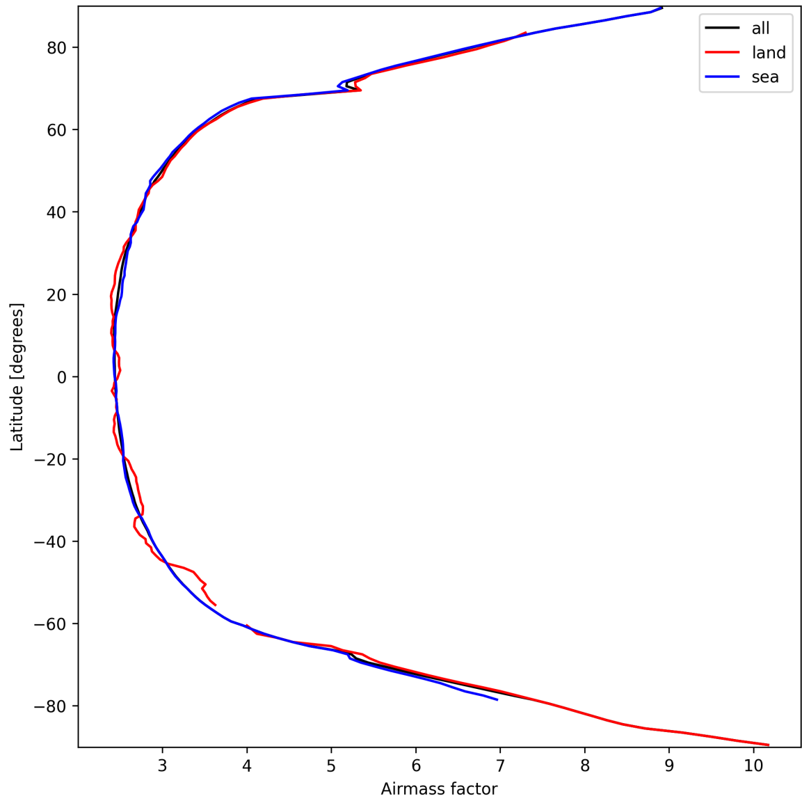
Figure 25: Zonal average of “Airmass factor” for 2025-03-20 to 2025-03-21.
