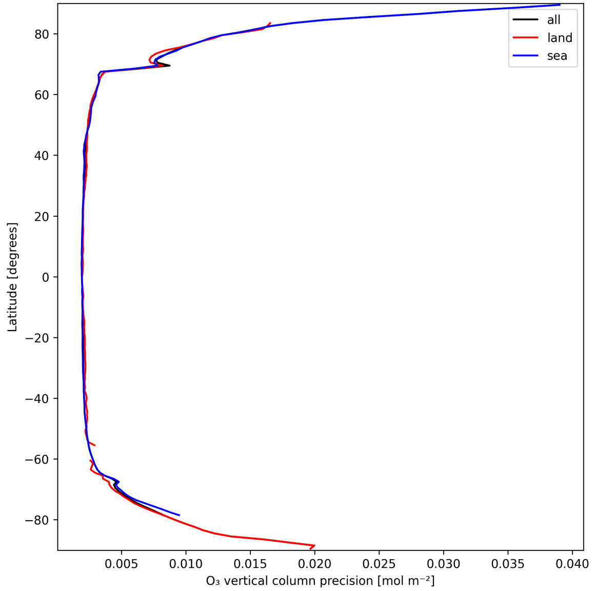
Figure 18: Zonal average of “O 3 vertical column precision” for 2025-03-20 to 2025-03-21.
