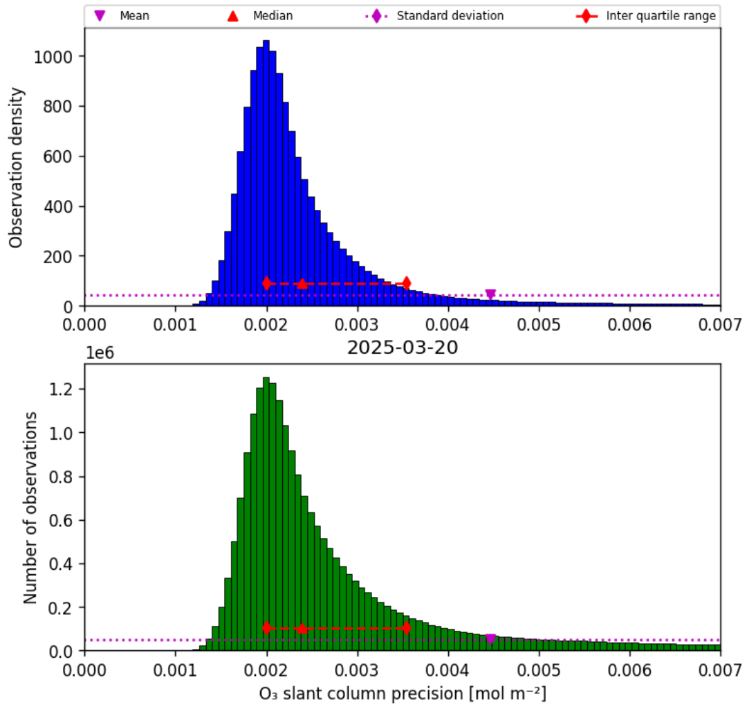
Figure 32: Histogram of “O 3 slant column precision” for 2025-03-20 to 2025-03-21
