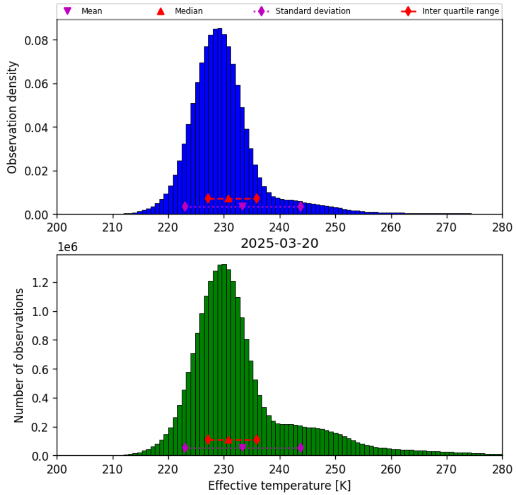
Figure 38: Histogram of “Effective temperature” for 2025-03-20 to 2025-03-21
