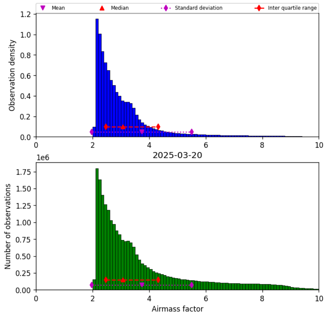
Figure 37: Histogram of “Airmass factor” for 2025-03-20 to 2025-03-21
