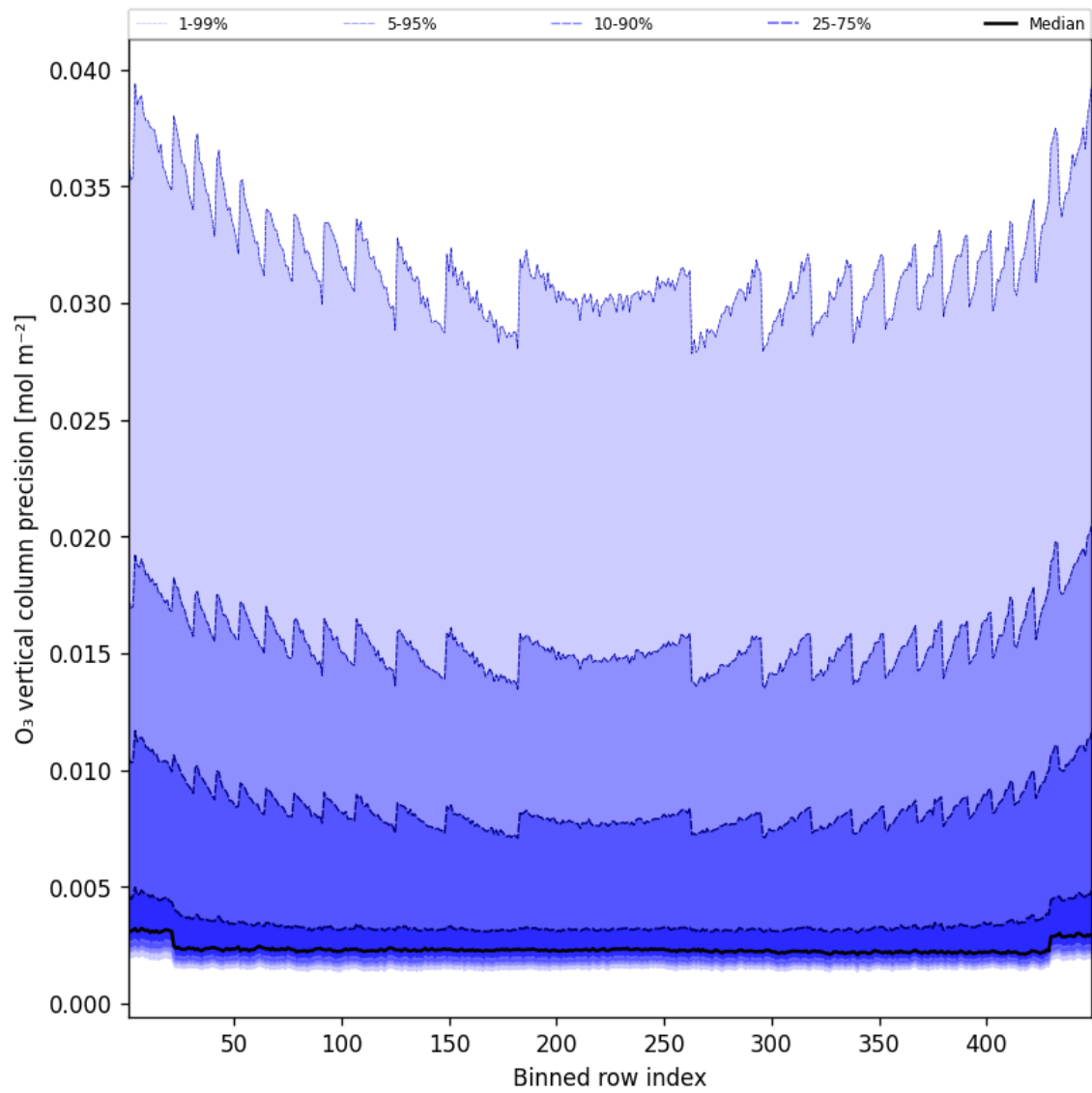
Figure 42: Along track statistics of “O 3 vertical column precision” for 2025-03-20 to 2025-03-21
