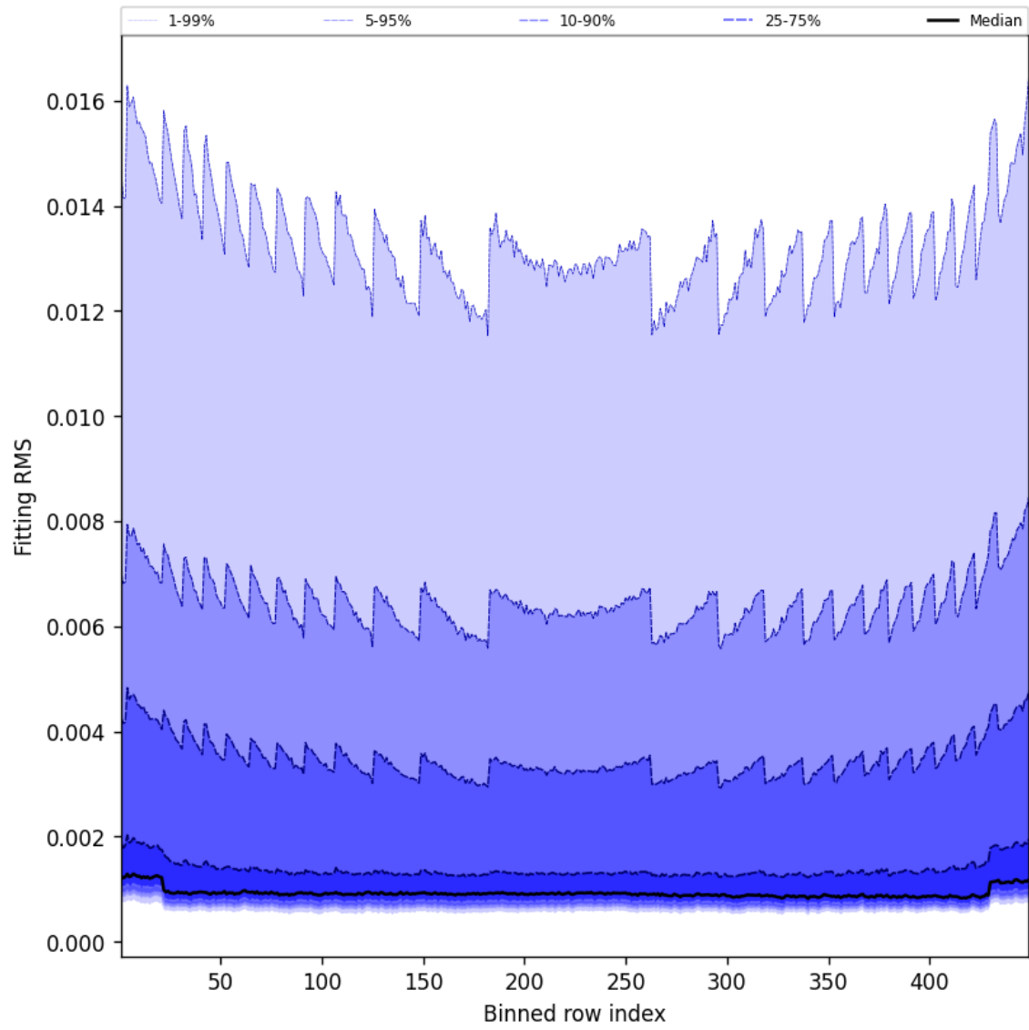
Figure 46: Along track statistics of “Fitting RMS” for 2025-03-20 to 2025-03-21
