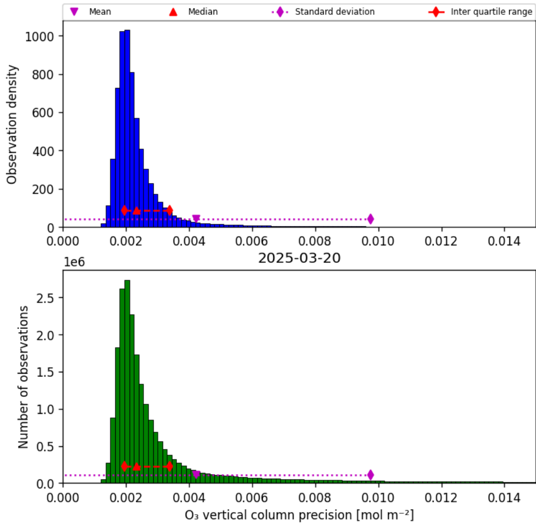
Figure 30: Histogram of “O 3 vertical column precision” for 2025-03-20 to 2025-03-21
