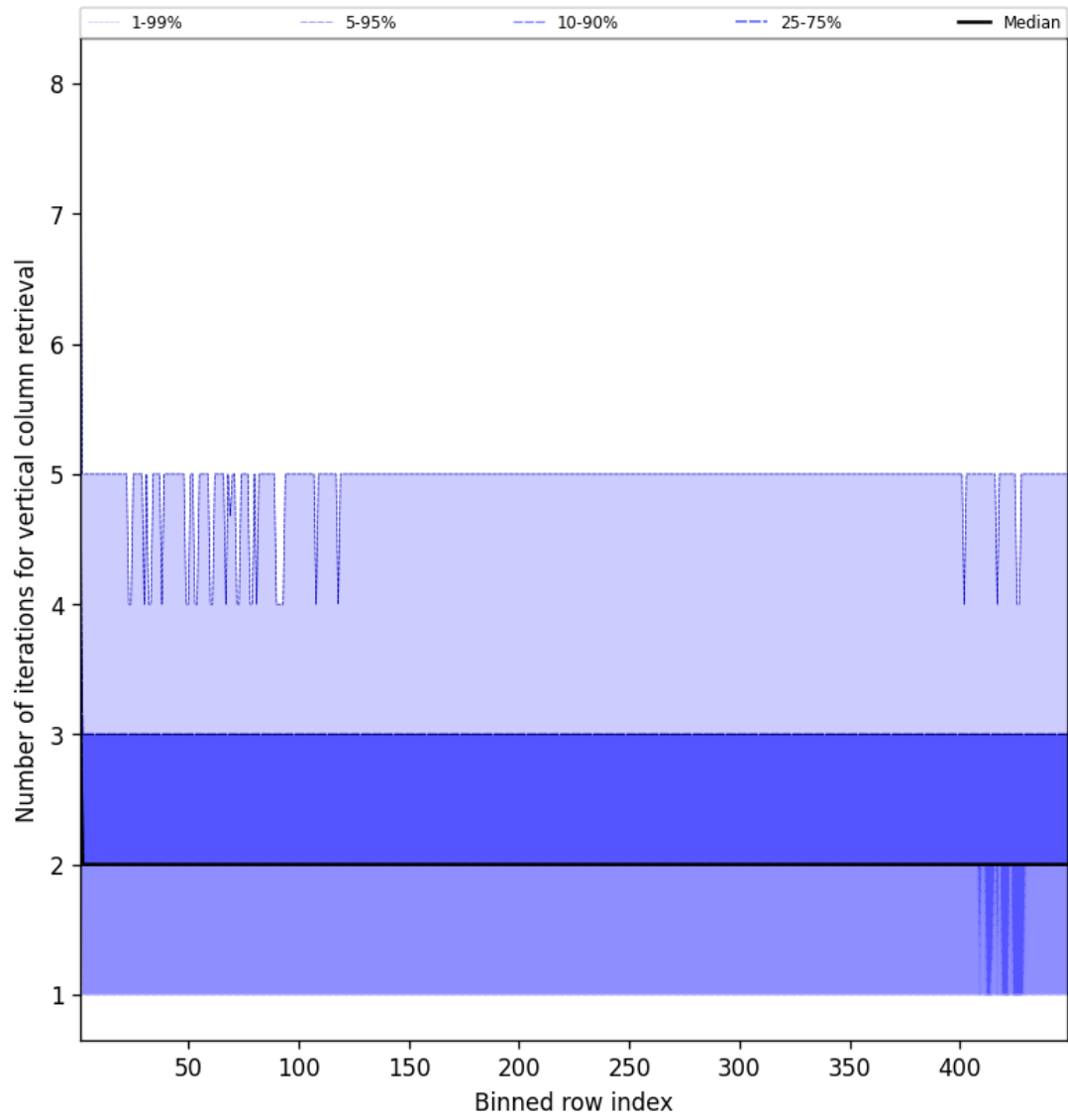
Figure 51: Along track statistics of “Number of iterations for vertical column retrieval” for 2025-03-20 to 2025-03-21
