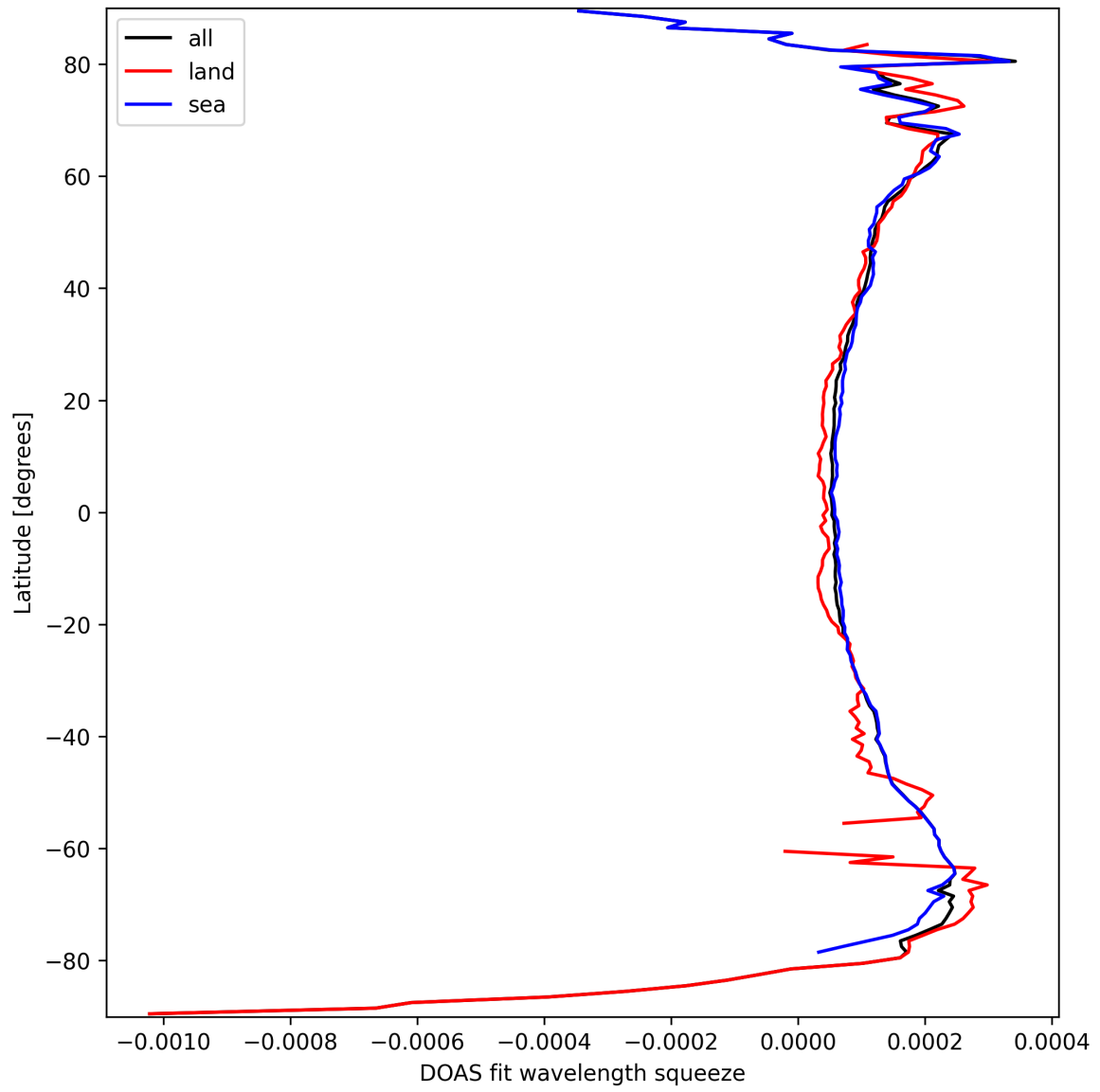
Figure 24: Zonal average of “DOAS fit wavelength squeeze” for 2025-03-20 to 2025-03-21.
