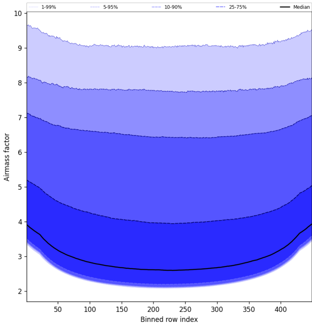
Figure 49: Along track statistics of “Airmass factor” for 2025-03-20 to 2025-03-21
