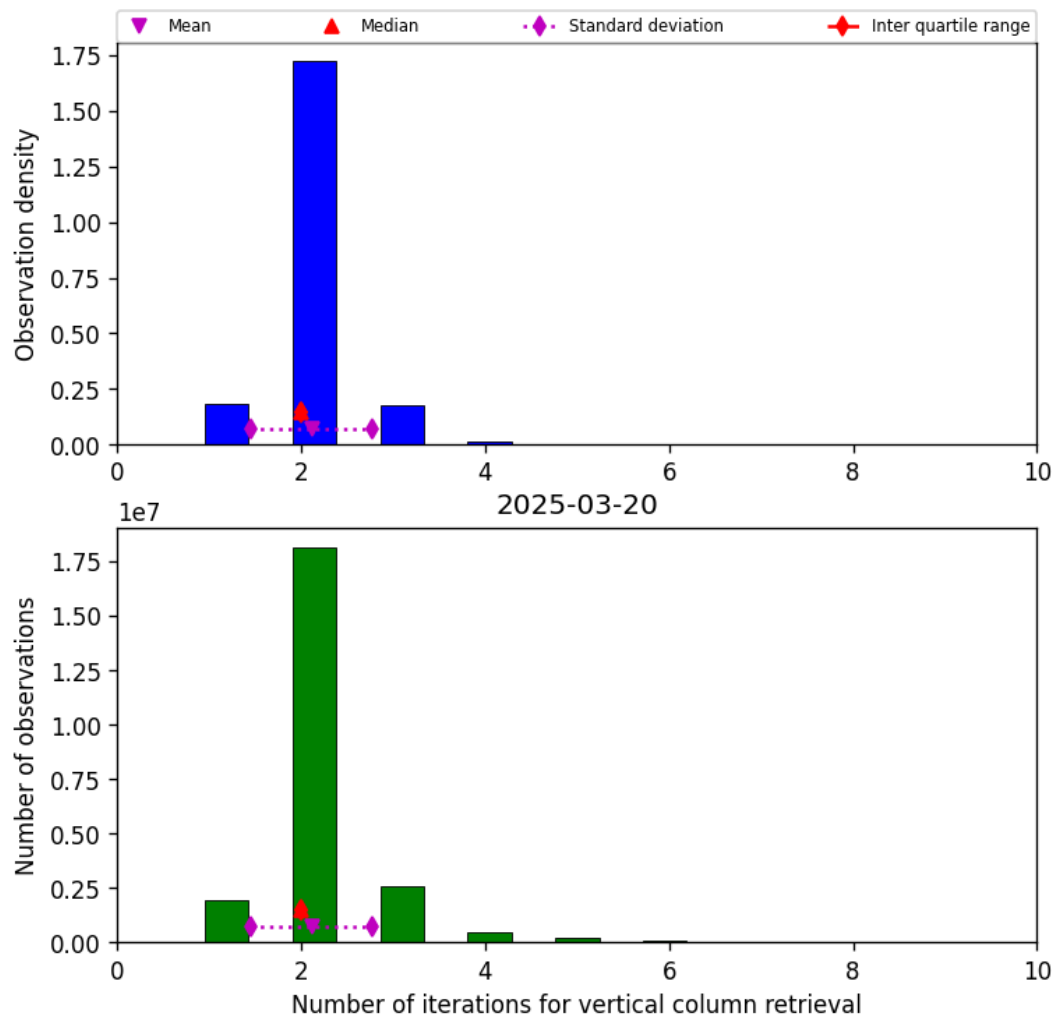
Figure 39: Histogram of “Number of iterations for vertical column retrieval” for 2025-03-20 to 2025-03-21
