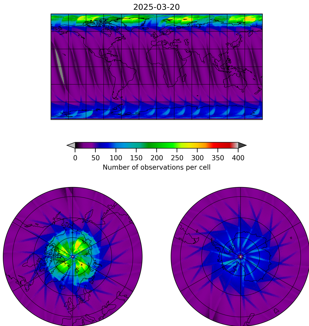
Figure 15: Map of the number of observations for 2025-03-20 to 2025-03-21
