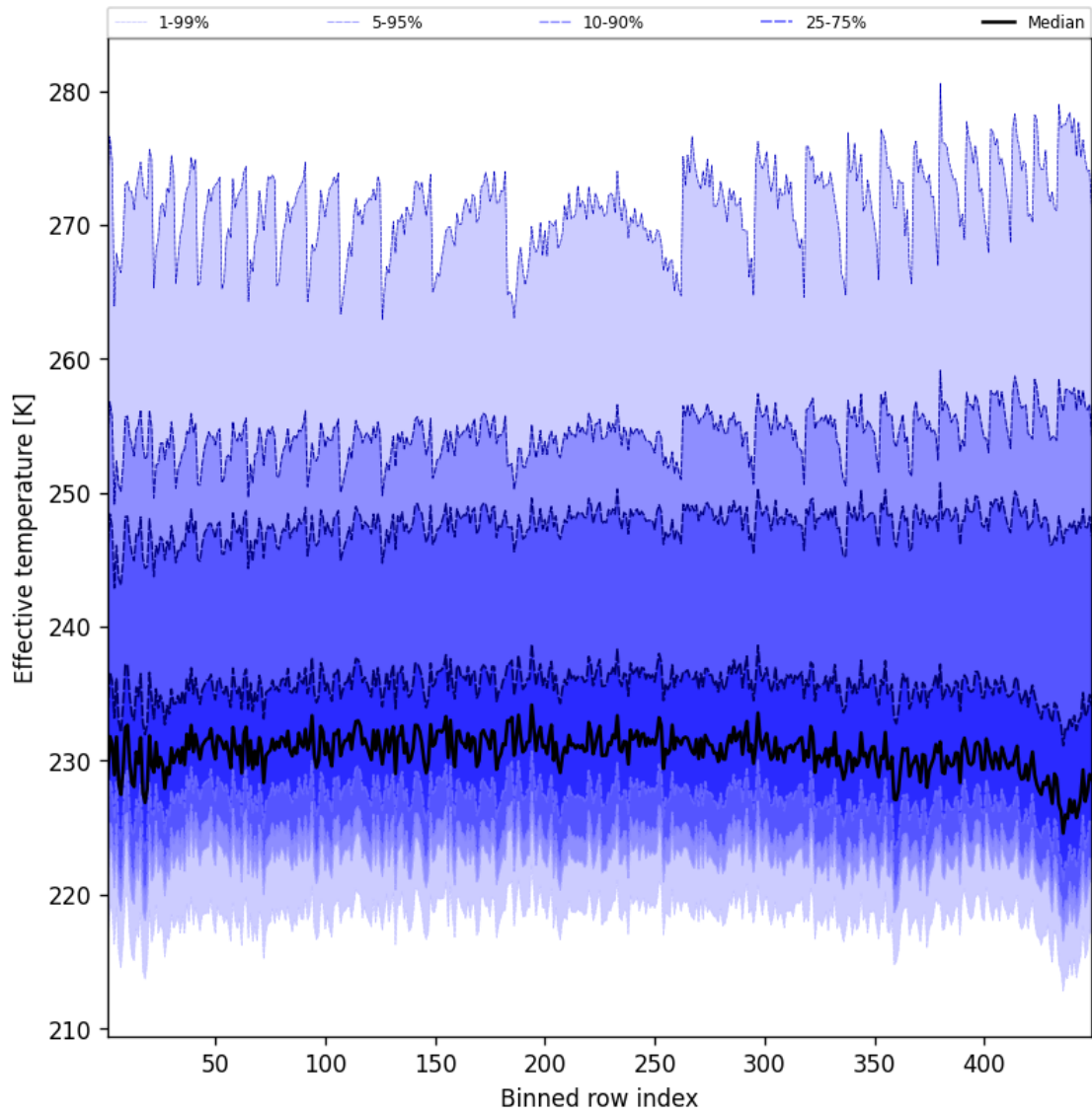
Figure 50: Along track statistics of “Effective temperature” for 2025-03-20 to 2025-03-21
