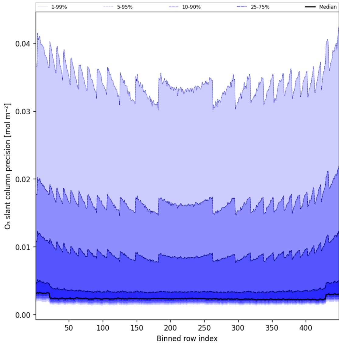
Figure 44: Along track statistics of “O 3 slant column precision” for 2025-03-20 to 2025-03-21
