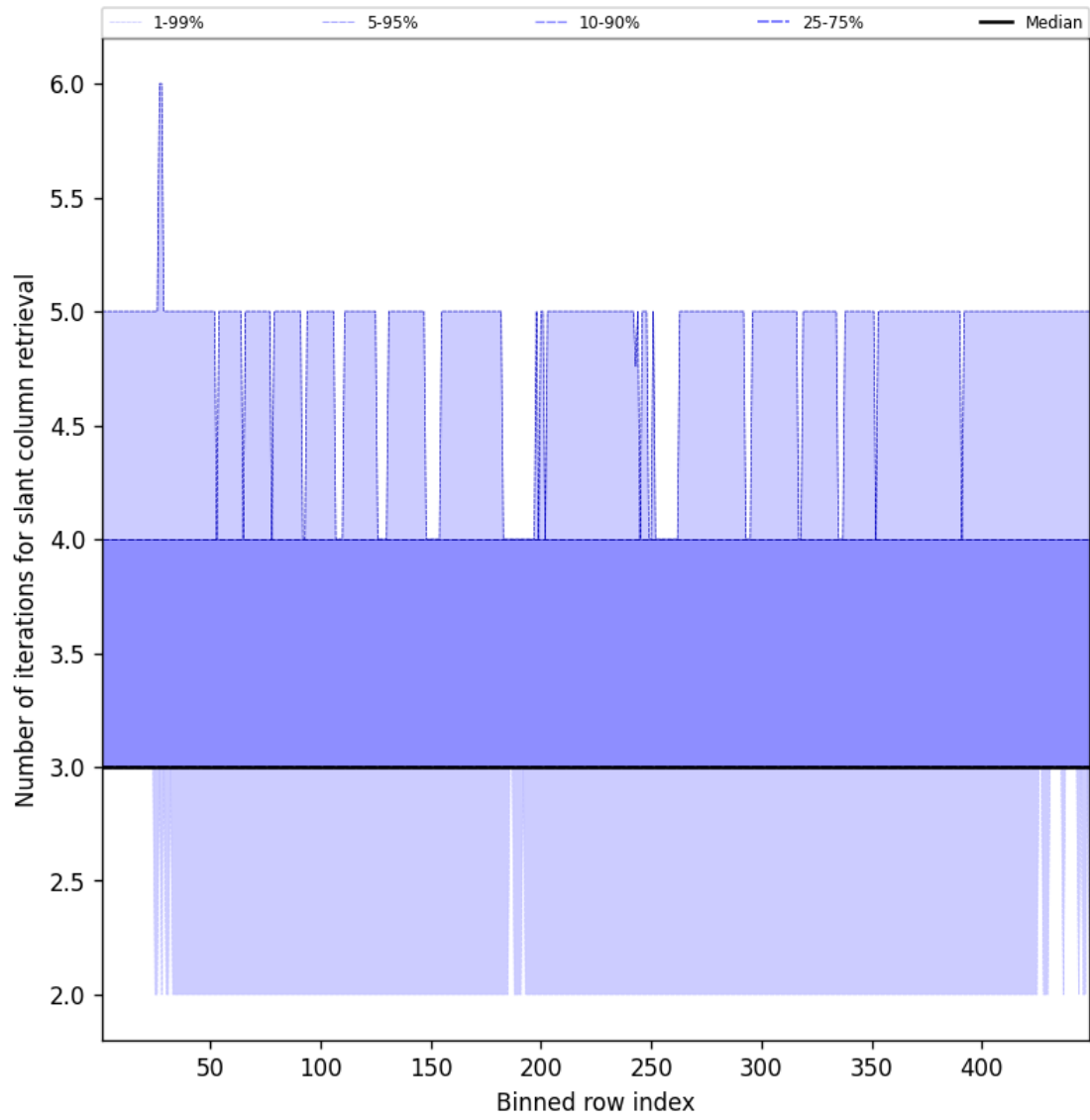
Figure 45: Along track statistics of “Number of iterations for slant column retrieval” for 2025-03-20 to 2025-03-21
