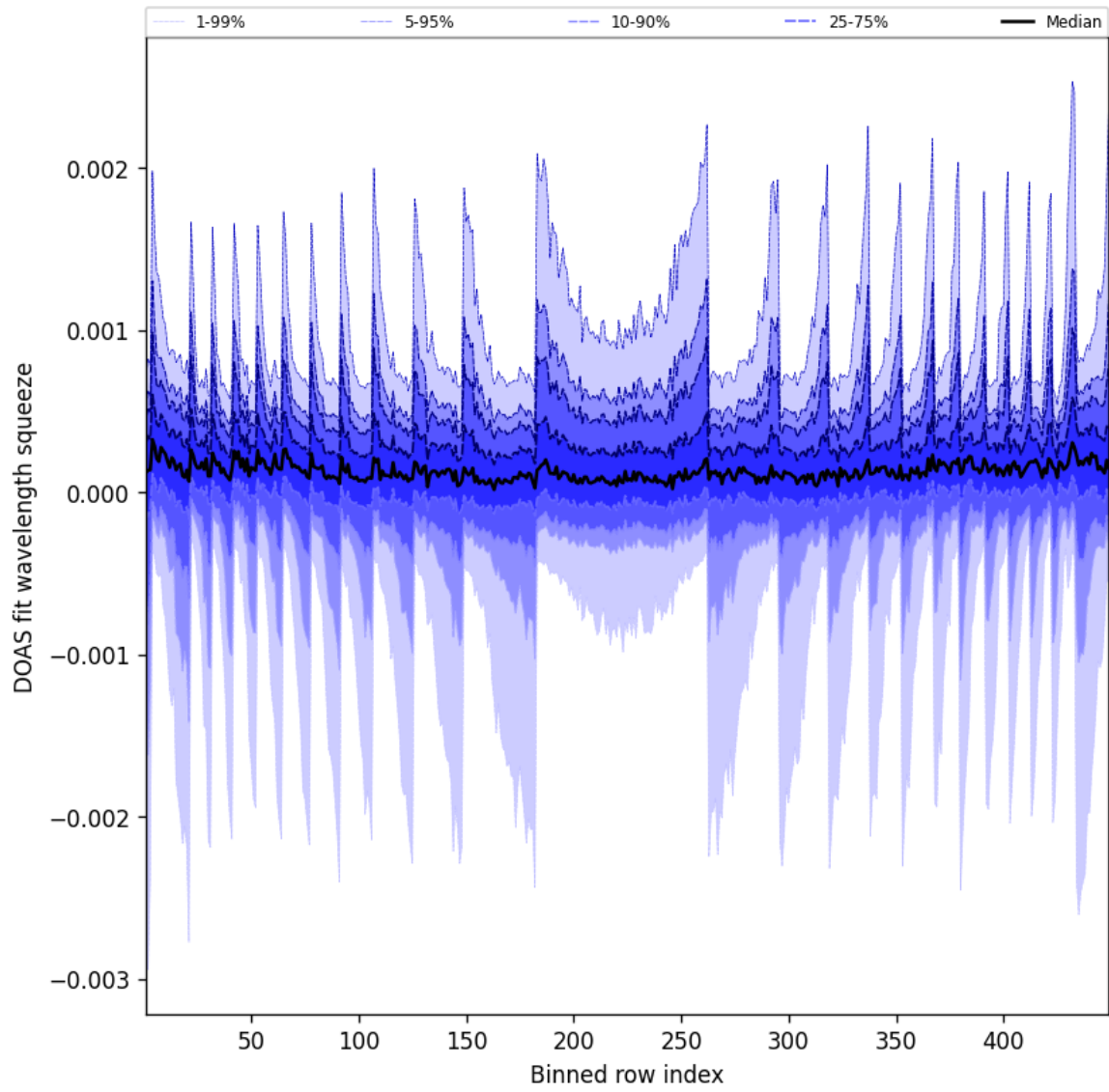
Figure 48: Along track statistics of “DOAS fit wavelength squeeze” for 2025-03-20 to 2025-03-21
