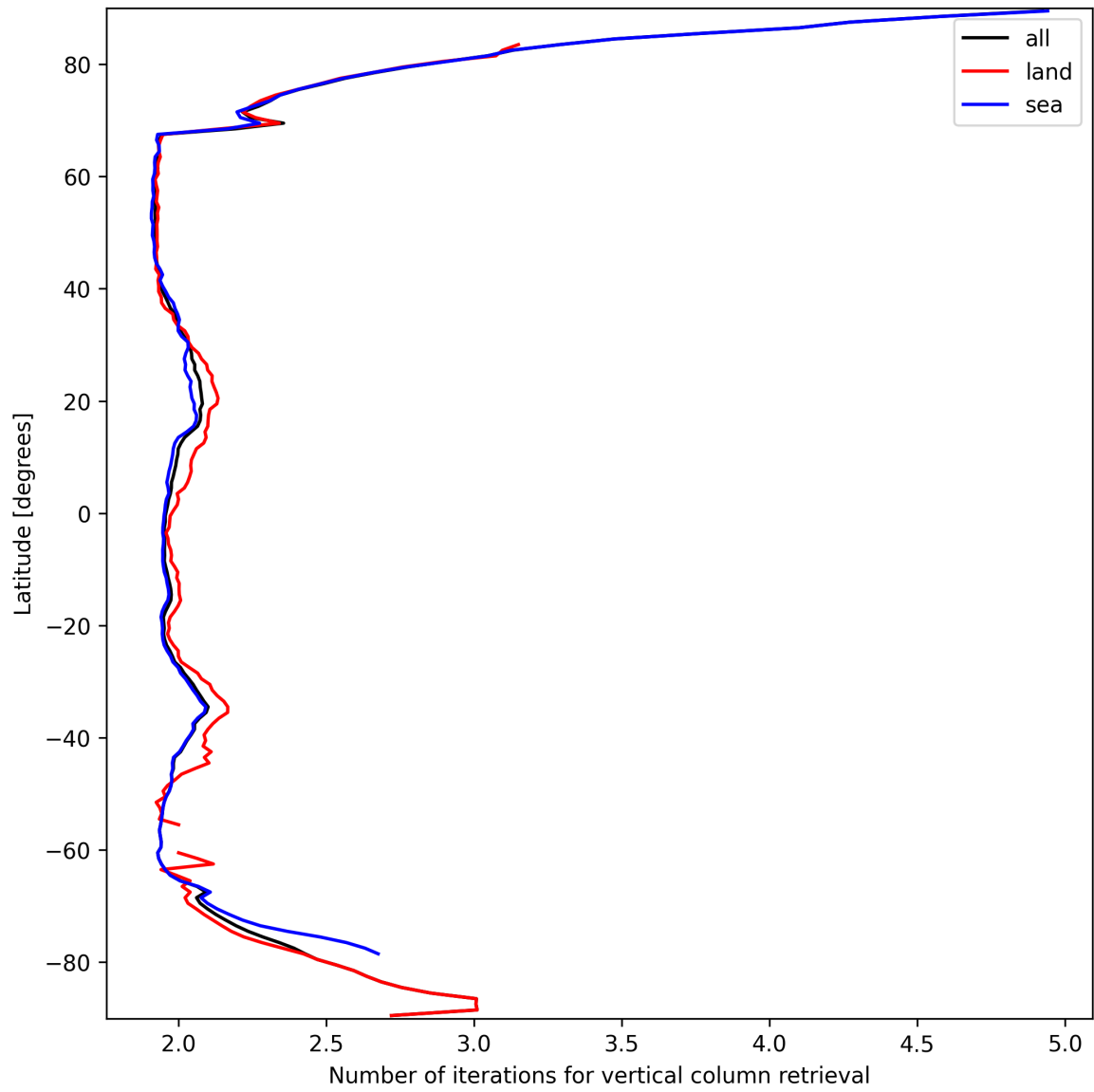
Figure 27: Zonal average of “Number of iterations for vertical column retrieval” for 2025-03-20 to 2025-03-21.
