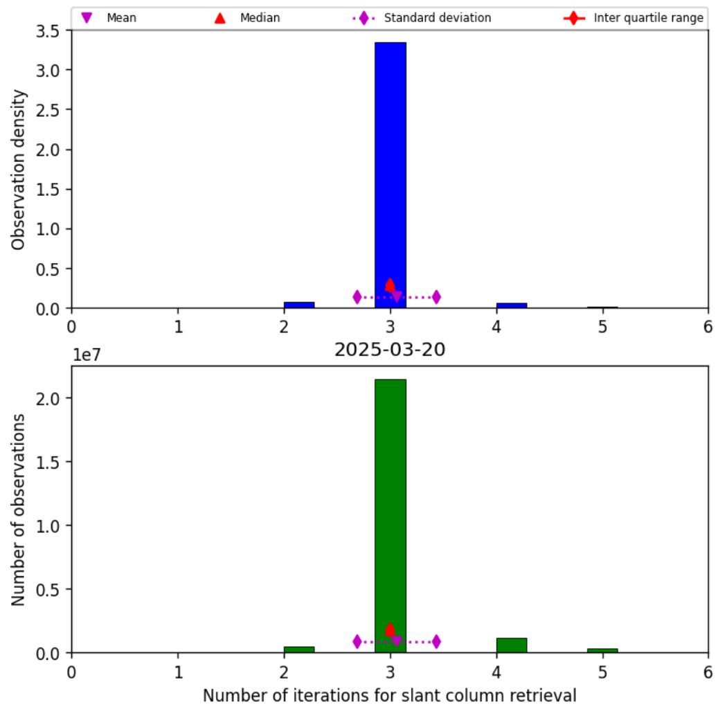
Figure 33: Histogram of “Number of iterations for slant column retrieval” for 2025-03-20 to 2025-03-21
