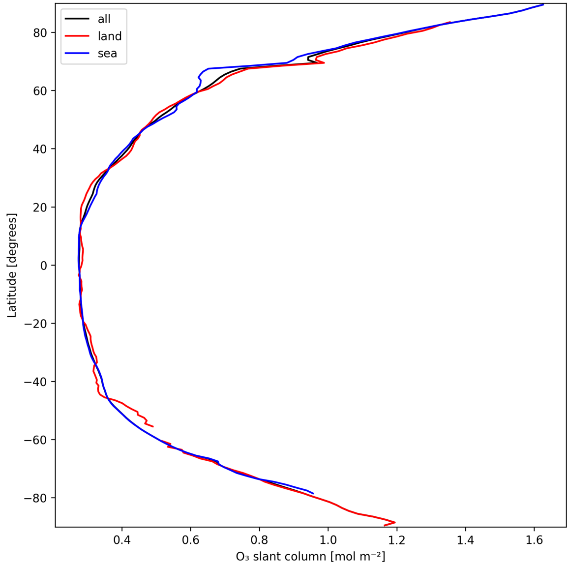
Figure 19: Zonal average of “O 3 slant column” for 2025-03-20 to 2025-03-21.
