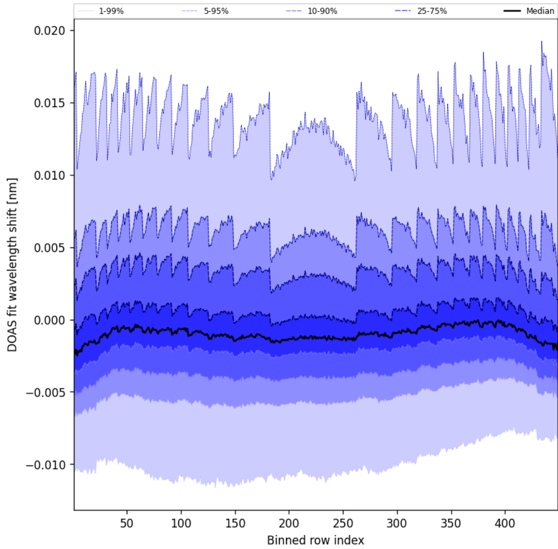
Figure 47: Along track statistics of “DOAS fit wavelength shift” for 2025-03-20 to 2025-03-21
