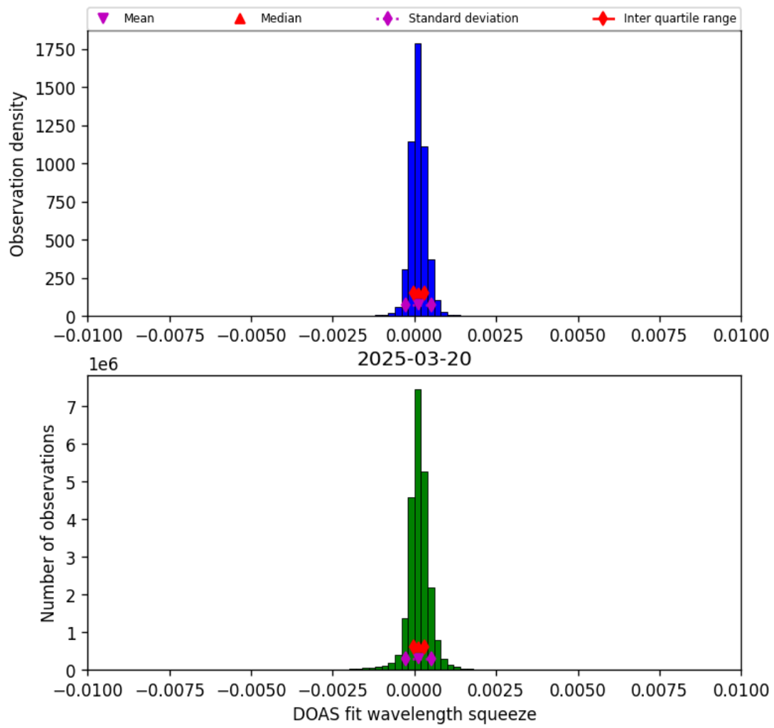
Figure 36: Histogram of “DOAS fit wavelength squeeze” for 2025-03-20 to 2025-03-21
