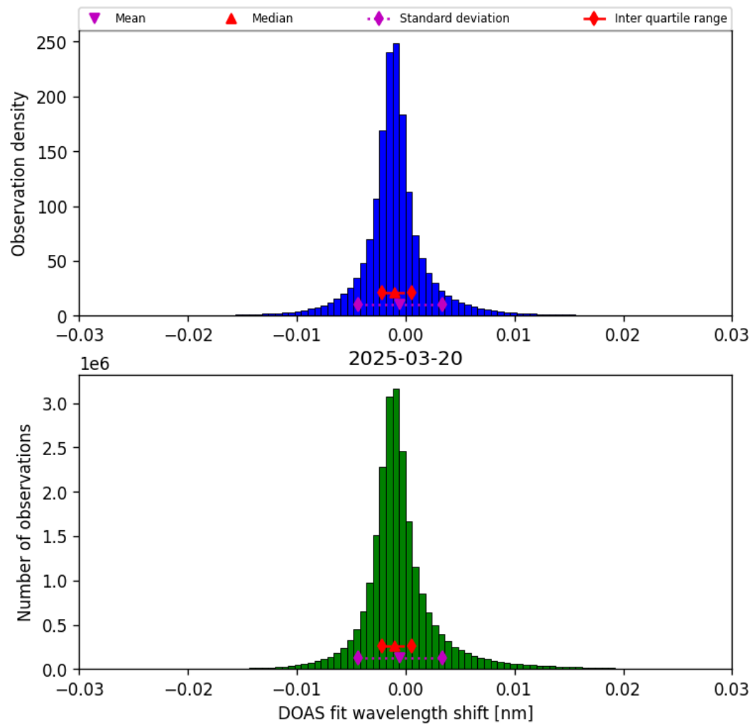
Figure 35: Histogram of “DOAS fit wavelength shift” for 2025-03-20 to 2025-03-21
