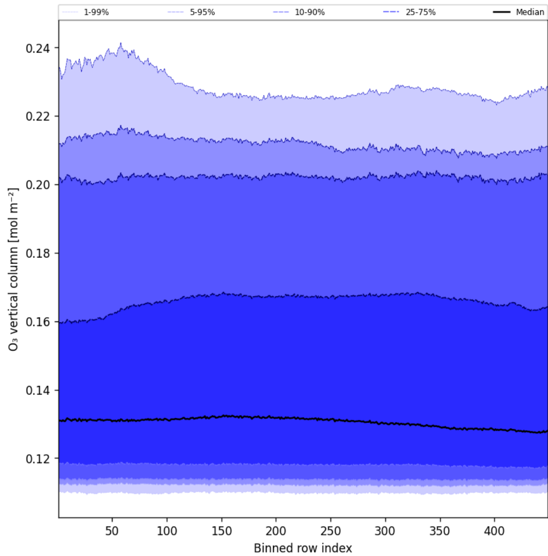
Figure 41: Along track statistics of “O 3 vertical column” for 2025-03-20 to 2025-03-21
