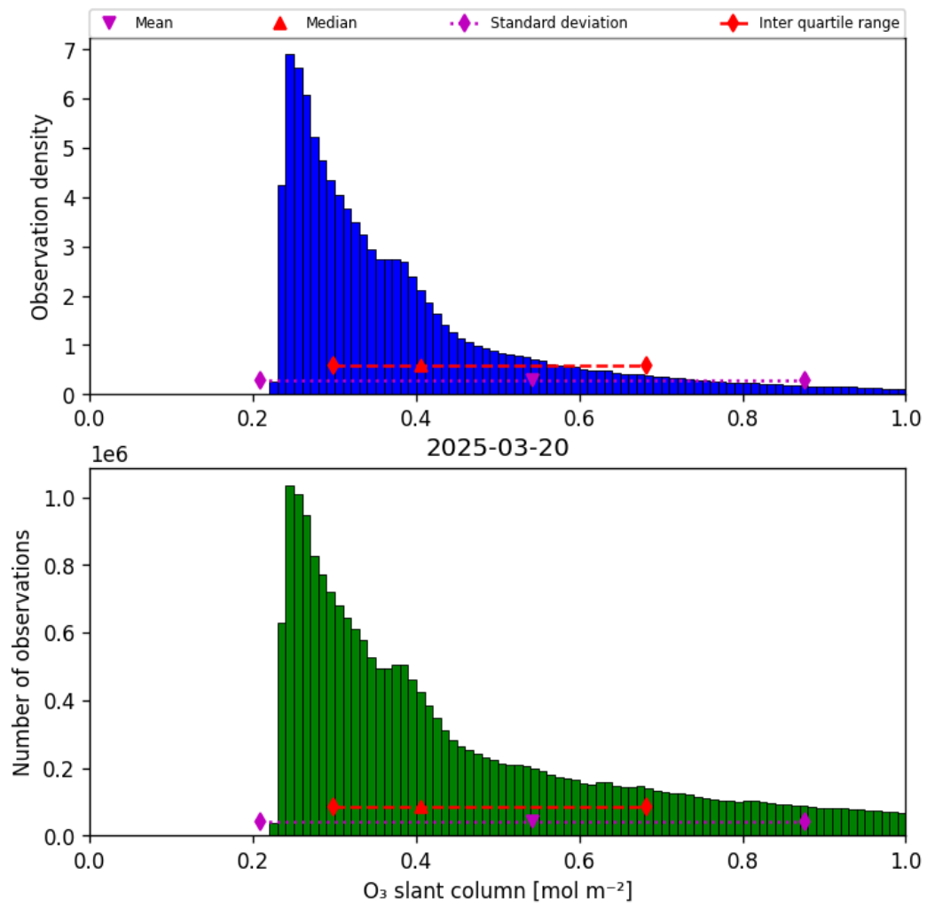
Figure 31: Histogram of “O 3 slant column” for 2025-03-20 to 2025-03-21
