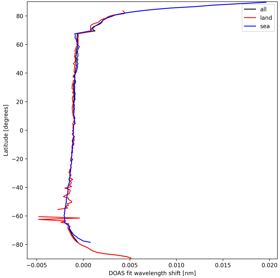
Figure 23: Zonal average of “DOAS fit wavelength shift” for 2025-03-20 to 2025-03-21.
