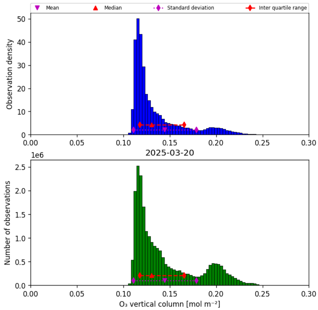
Figure 29: Histogram of “O 3 vertical column” for 2025-03-20 to 2025-03-21
