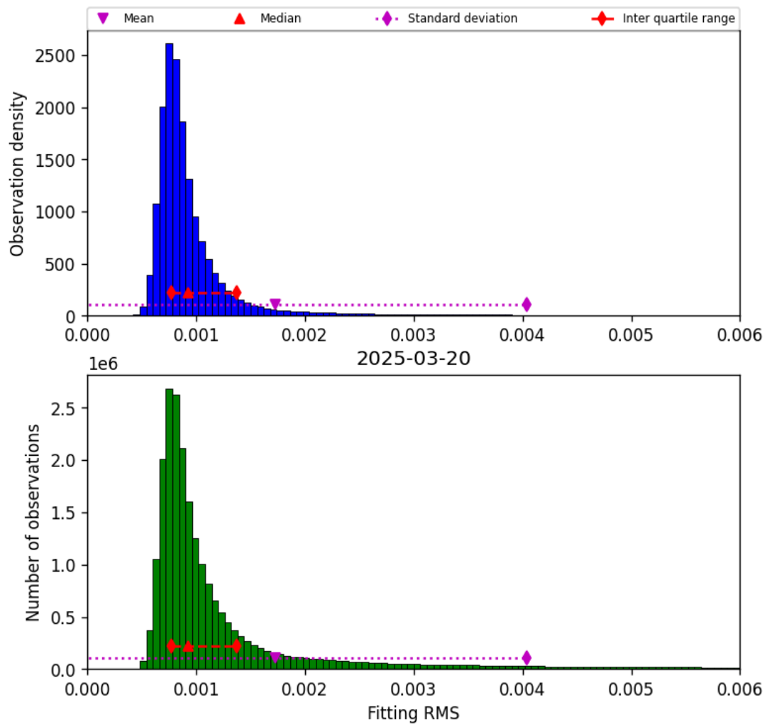
Figure 34: Histogram of “Fitting RMS” for 2025-03-20 to 2025-03-21
