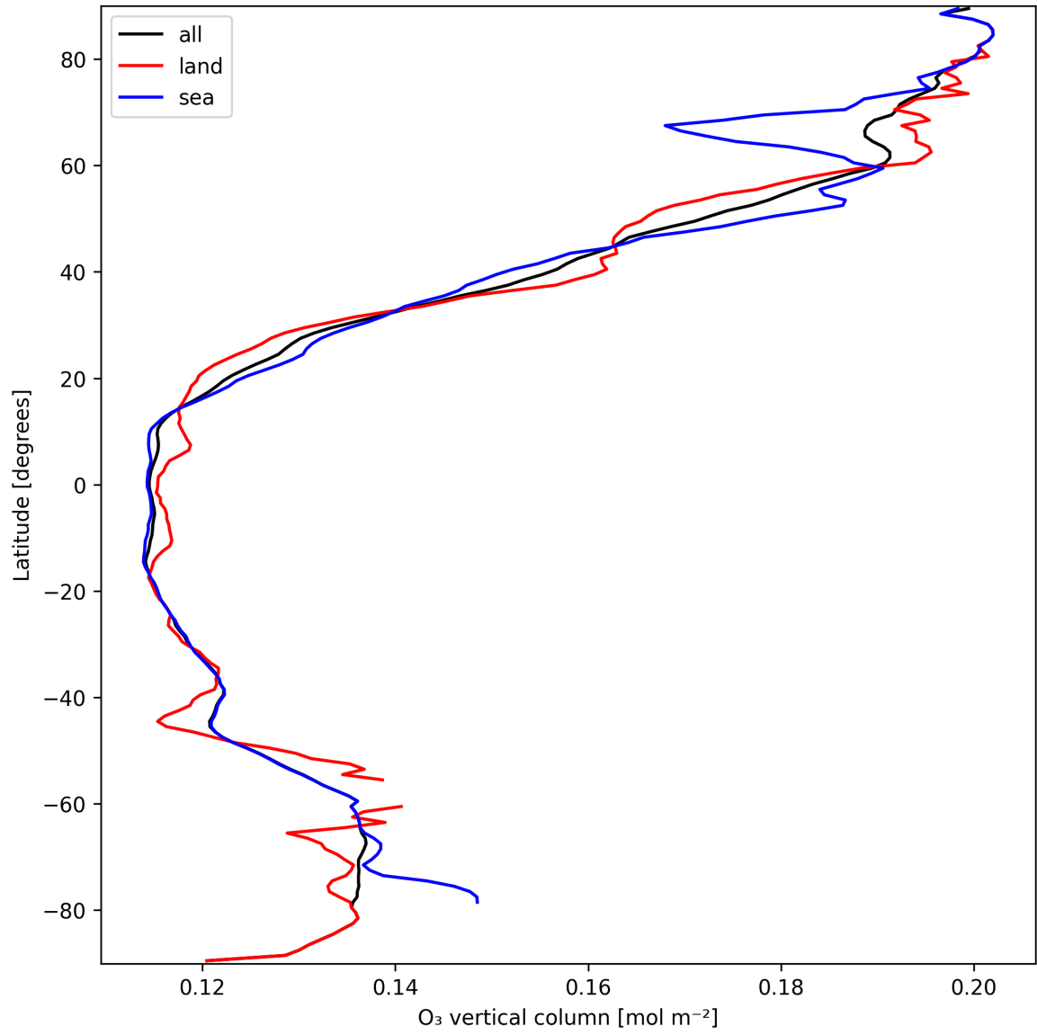
Figure 17: Zonal average of “O 3 vertical column” for 2025-03-20 to 2025-03-21.
