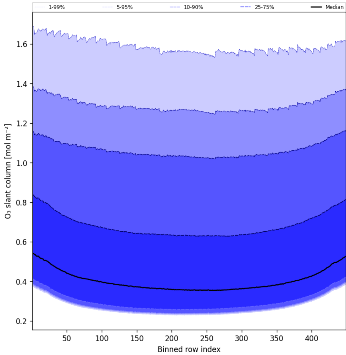
Figure 43: Along track statistics of “O 3 slant column” for 2025-03-20 to 2025-03-21
