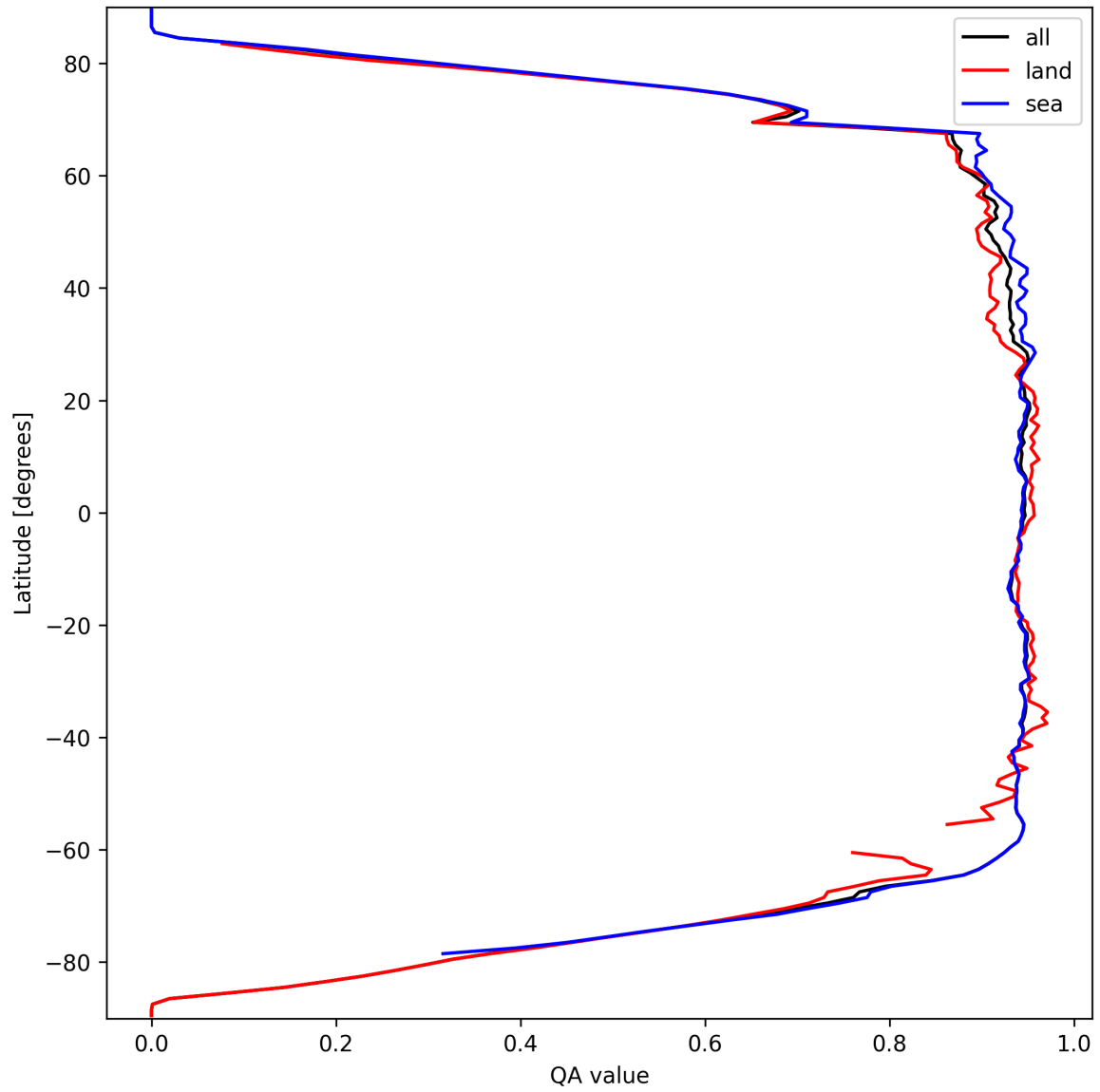
Figure 16: Zonal average of "QA value" for 2025-03-20 to 2025-03-21.
