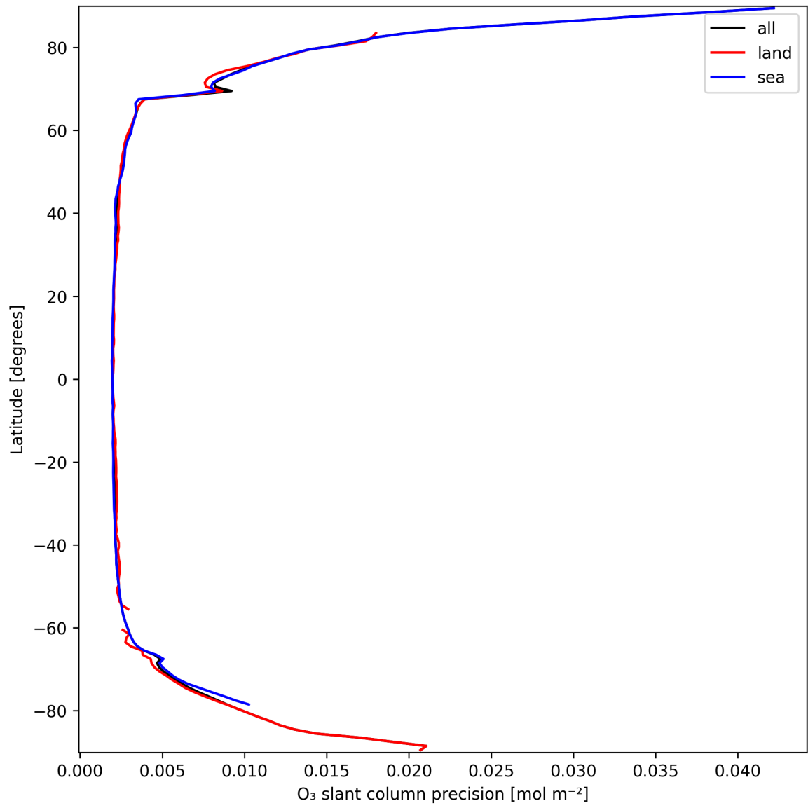
Figure 20: Zonal average of “O 3 slant column precision” for 2025-03-20 to 2025-03-21.
