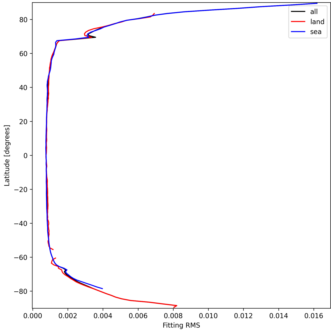
Figure 22: Zonal average of “Fitting RMS” for 2025-03-20 to 2025-03-21.
