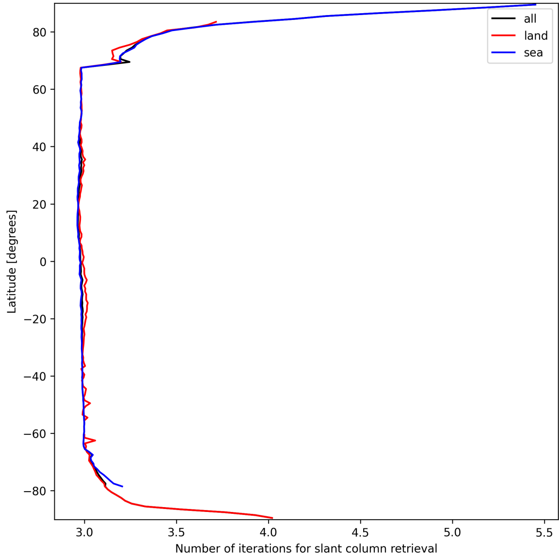
Figure 21: Zonal average of “Number of iterations for slant column retrieval” for 2025-03-20 to 2025-03-21.
