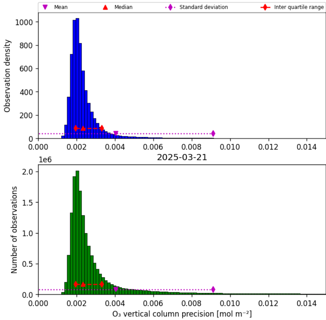
Figure 30: Histogram of “O 3 vertical column precision” for 2025-03-21 to 2025-03-21
