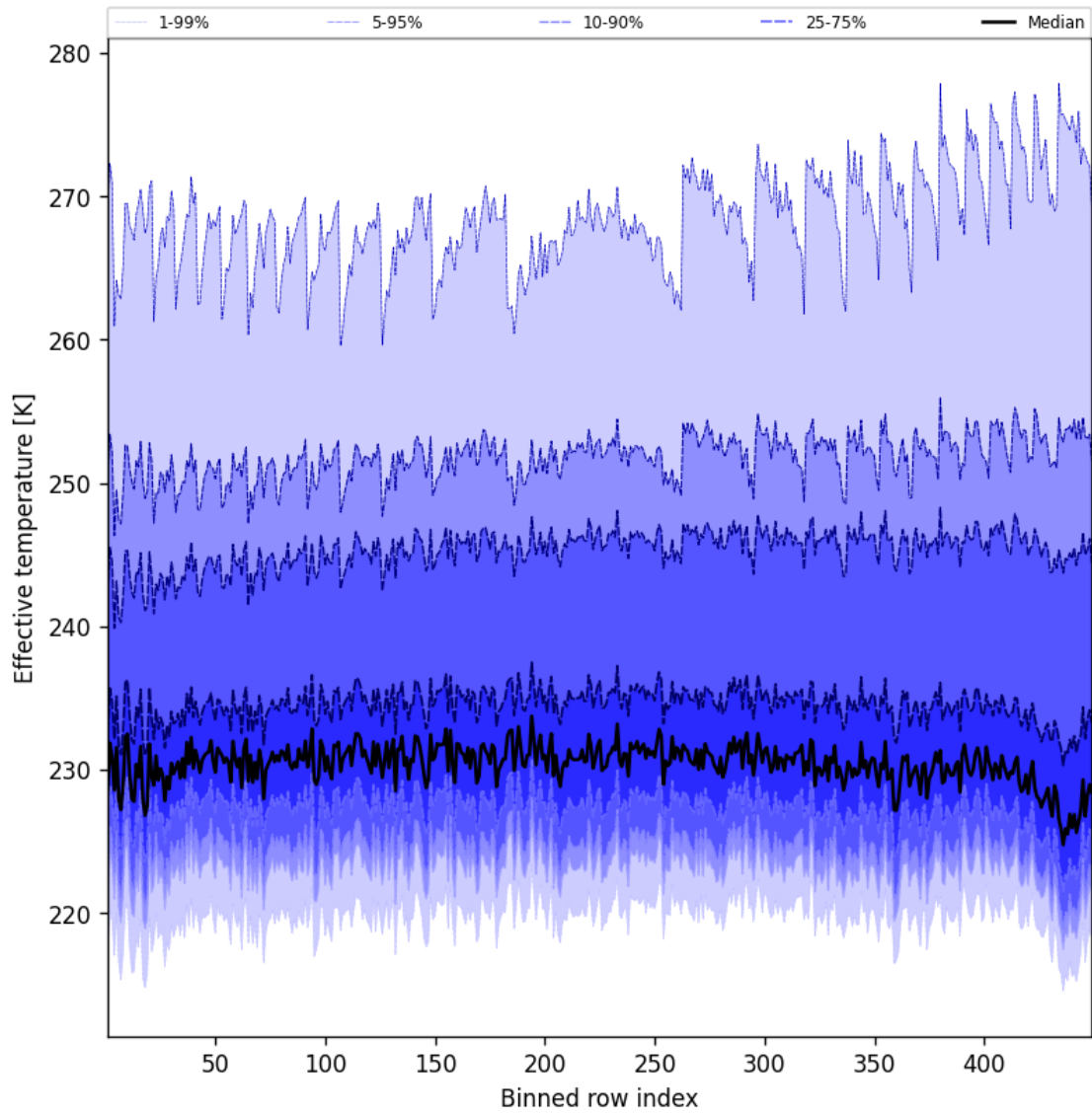
Figure 50: Along track statistics of “Effective temperature” for 2025-03-21 to 2025-03-21
