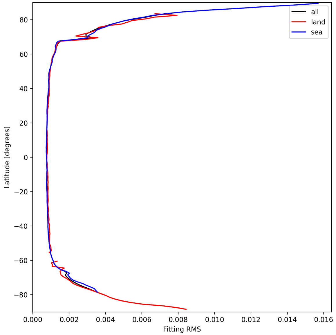
Figure 22: Zonal average of “Fitting RMS” for 2025-03-21 to 2025-03-21.
