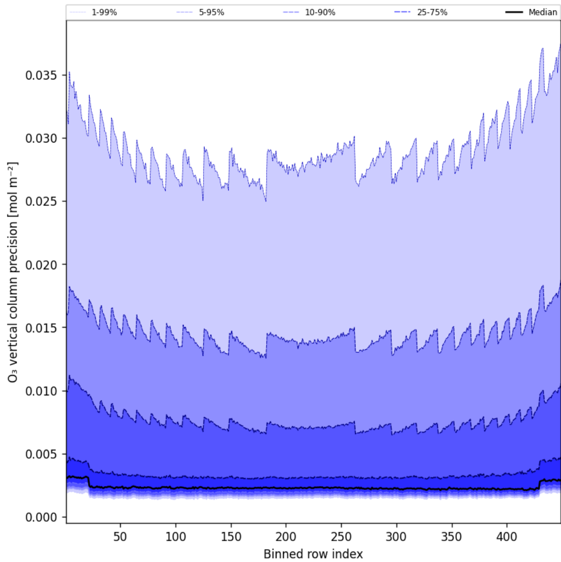
Figure 42: Along track statistics of “O 3 vertical column precision” for 2025-03-21 to 2025-03-21
