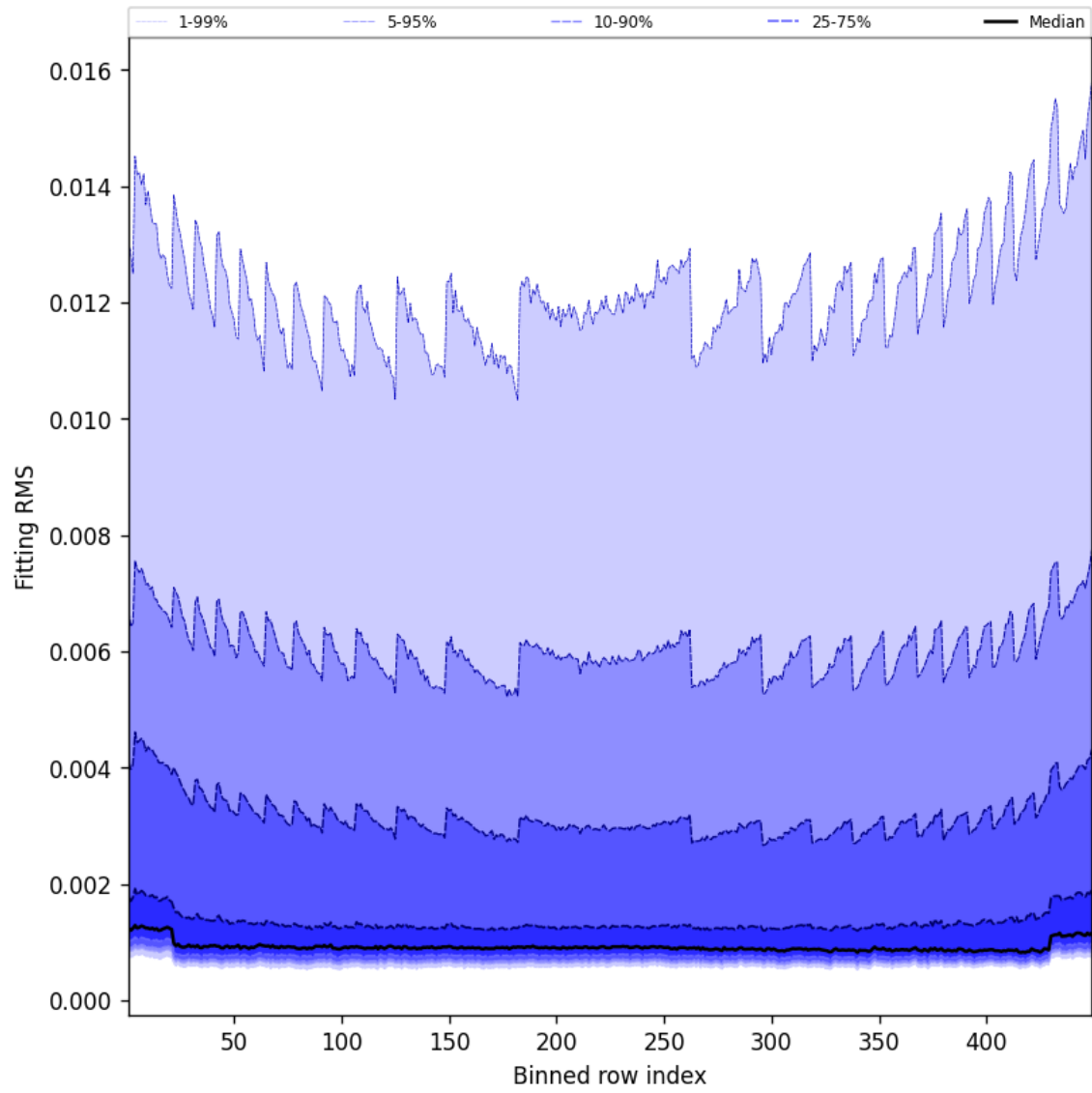
Figure 46: Along track statistics of “Fitting RMS” for 2025-03-21 to 2025-03-21
