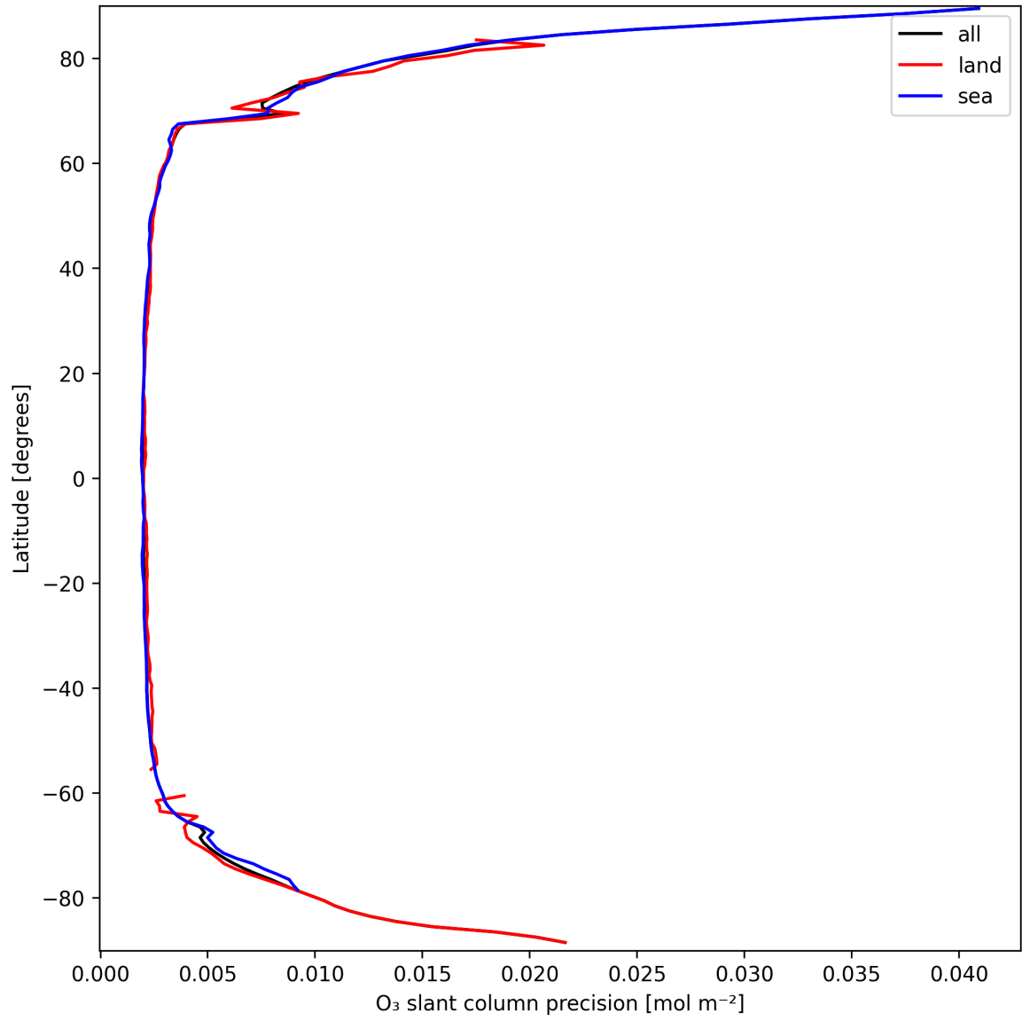
Figure 20: Zonal average of “O 3 slant column precision” for 2025-03-21 to 2025-03-21.
