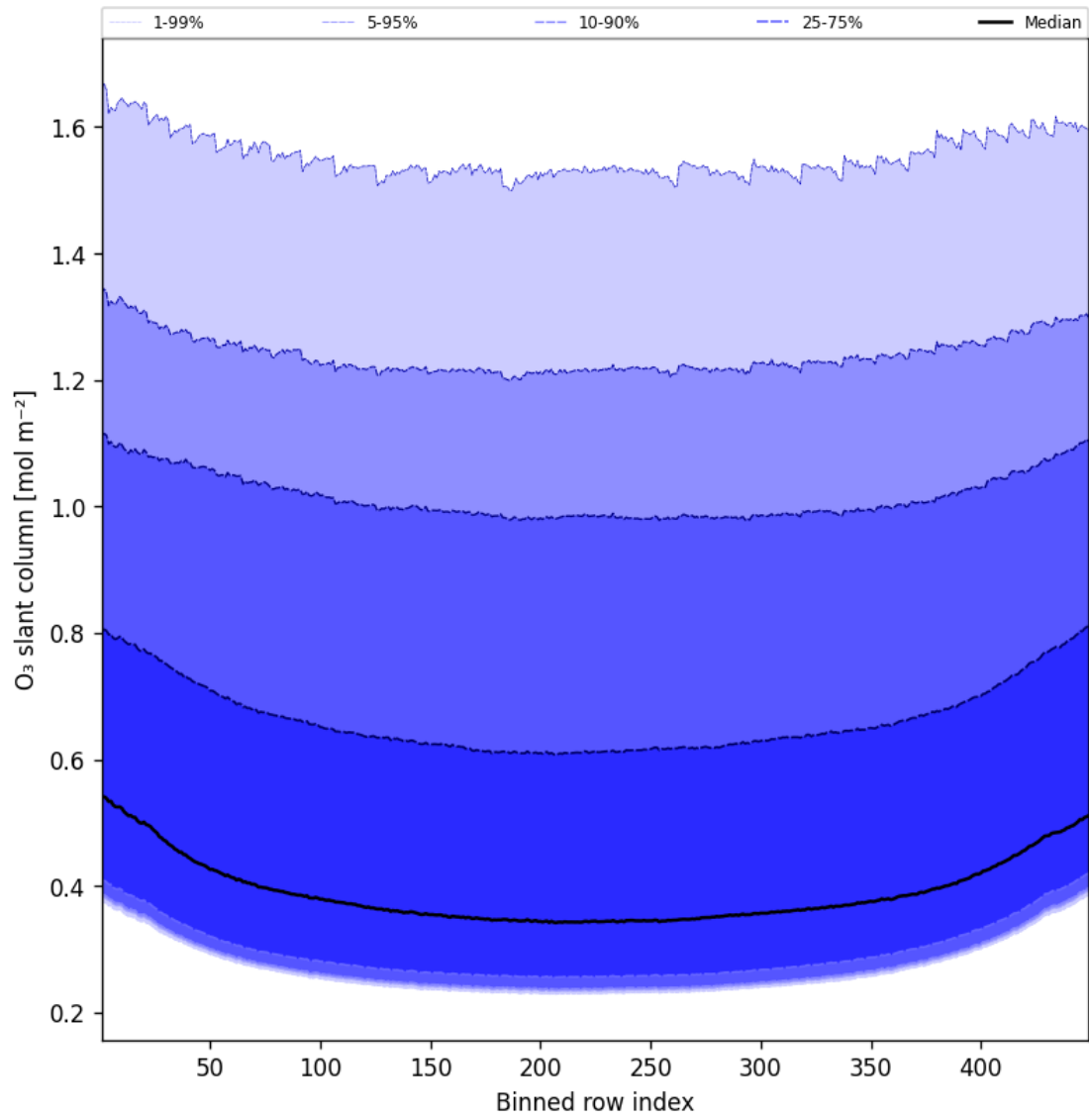
Figure 43: Along track statistics of “O 3 slant column” for 2025-03-21 to 2025-03-21
