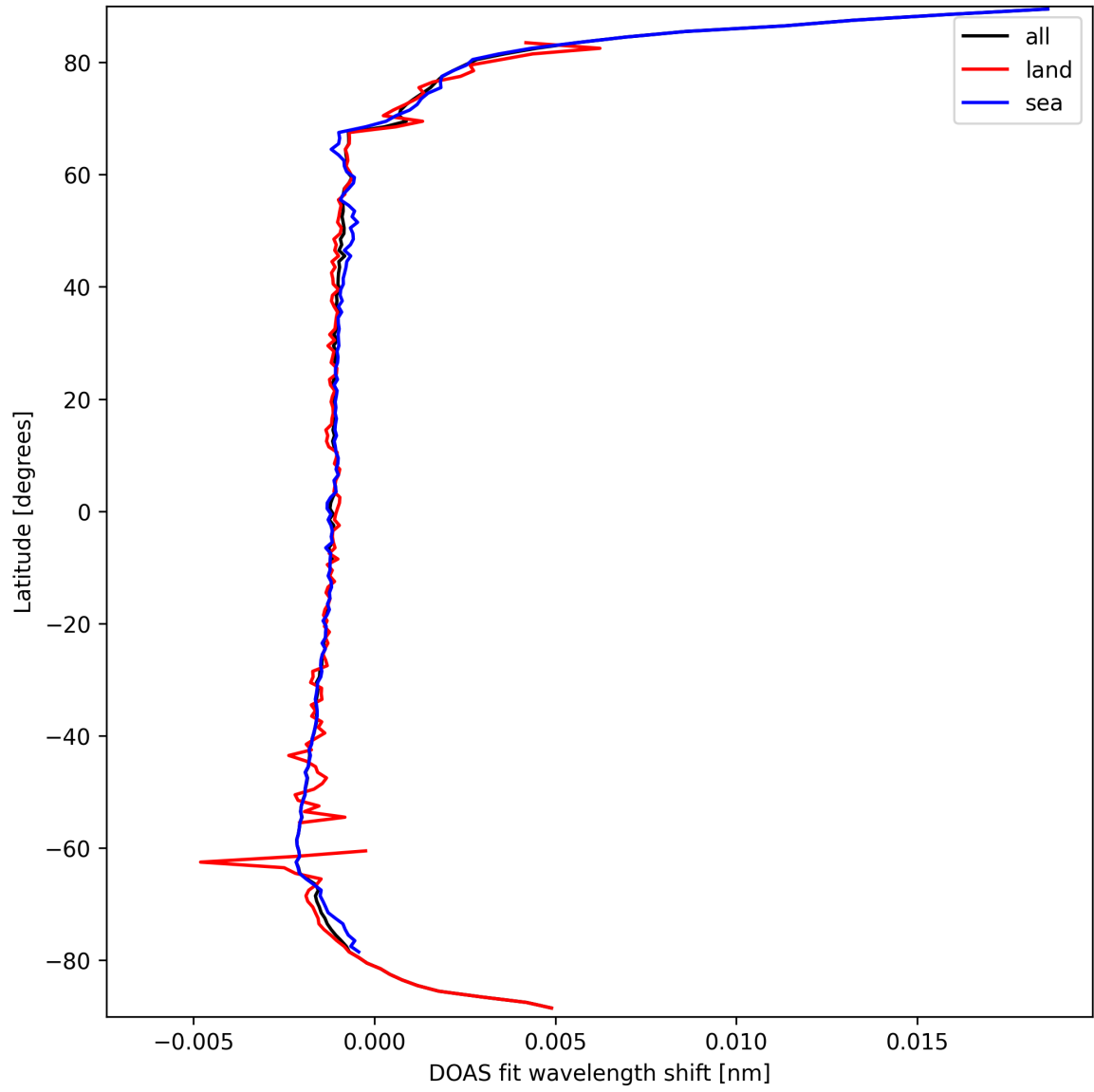
Figure 23: Zonal average of “DOAS fit wavelength shift” for 2025-03-21 to 2025-03-21.
