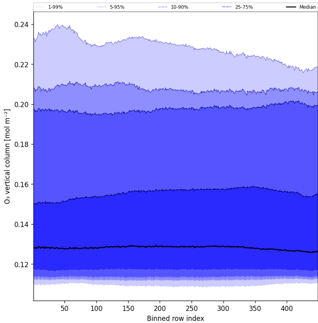
Figure 41: Along track statistics of “O 3 vertical column” for 2025-03-21 to 2025-03-21
