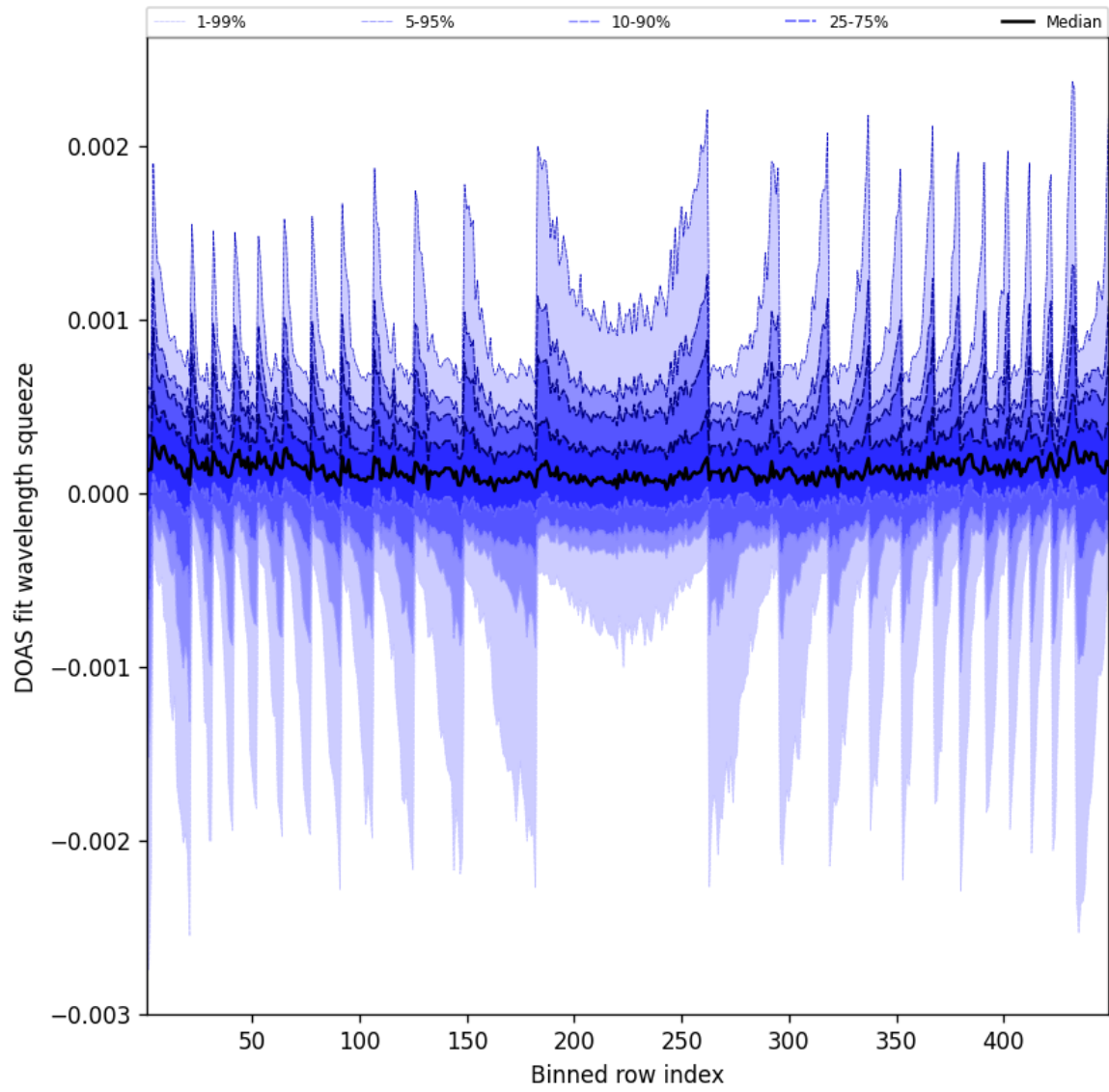
Figure 48: Along track statistics of “DOAS fit wavelength squeeze” for 2025-03-21 to 2025-03-21
