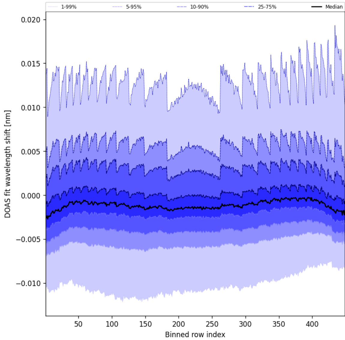
Figure 47: Along track statistics of “DOAS fit wavelength shift” for 2025-03-21 to 2025-03-21
