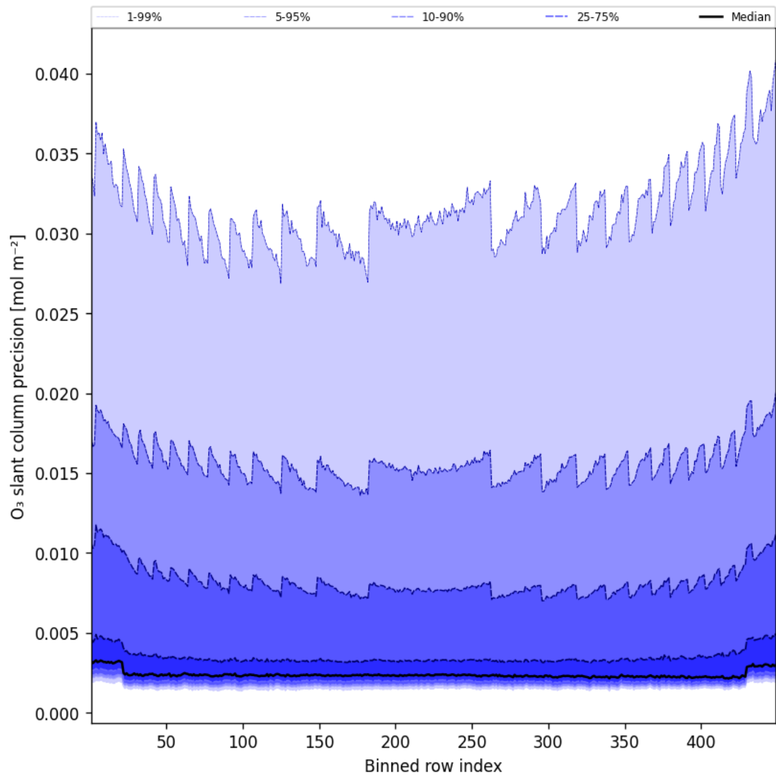
Figure 44: Along track statistics of “O 3 slant column precision” for 2025-03-21 to 2025-03-21
