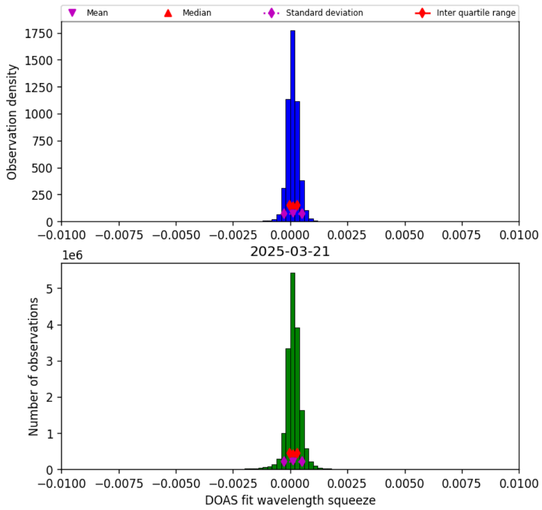
Figure 36: Histogram of “DOAS fit wavelength squeeze” for 2025-03-21 to 2025-03-21
