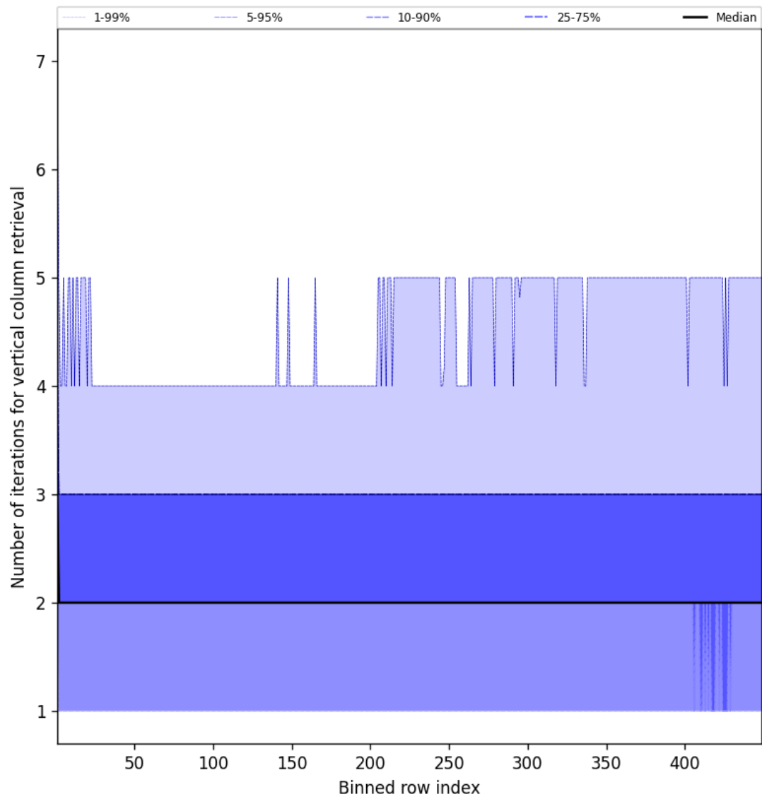
Figure 51: Along track statistics of “Number of iterations for vertical column retrieval” for 2025-03-21 to 2025-03-21
