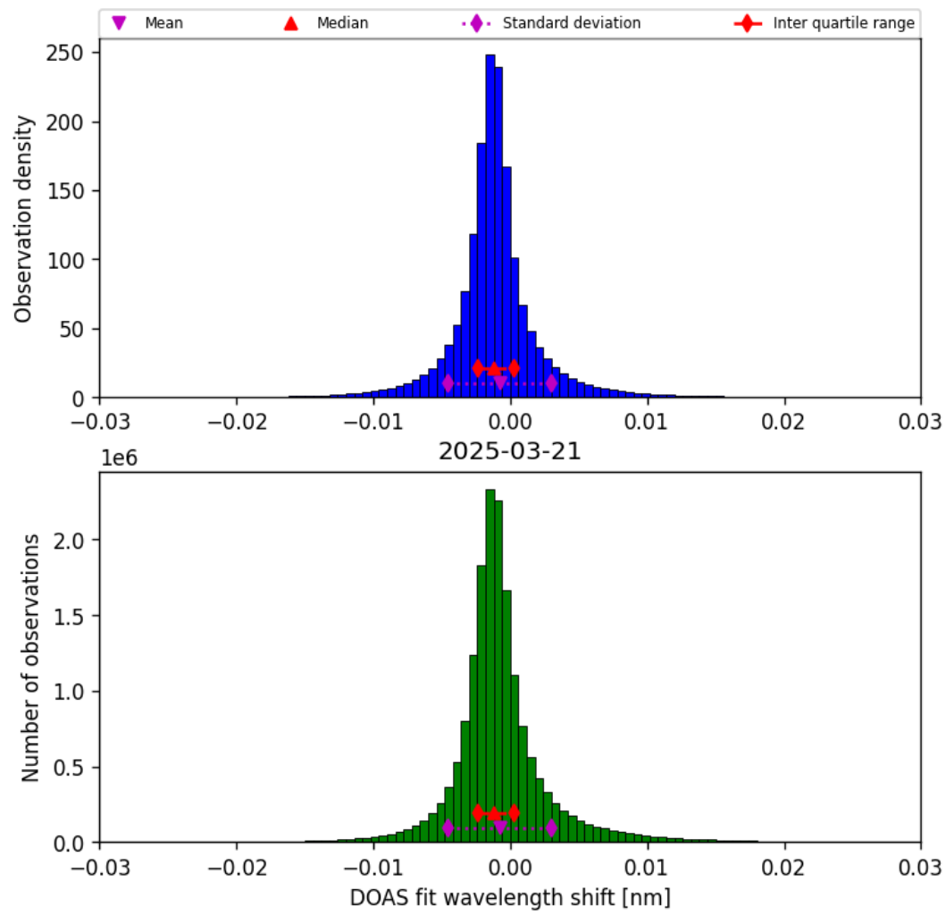
Figure 35: Histogram of “DOAS fit wavelength shift” for 2025-03-21 to 2025-03-21
