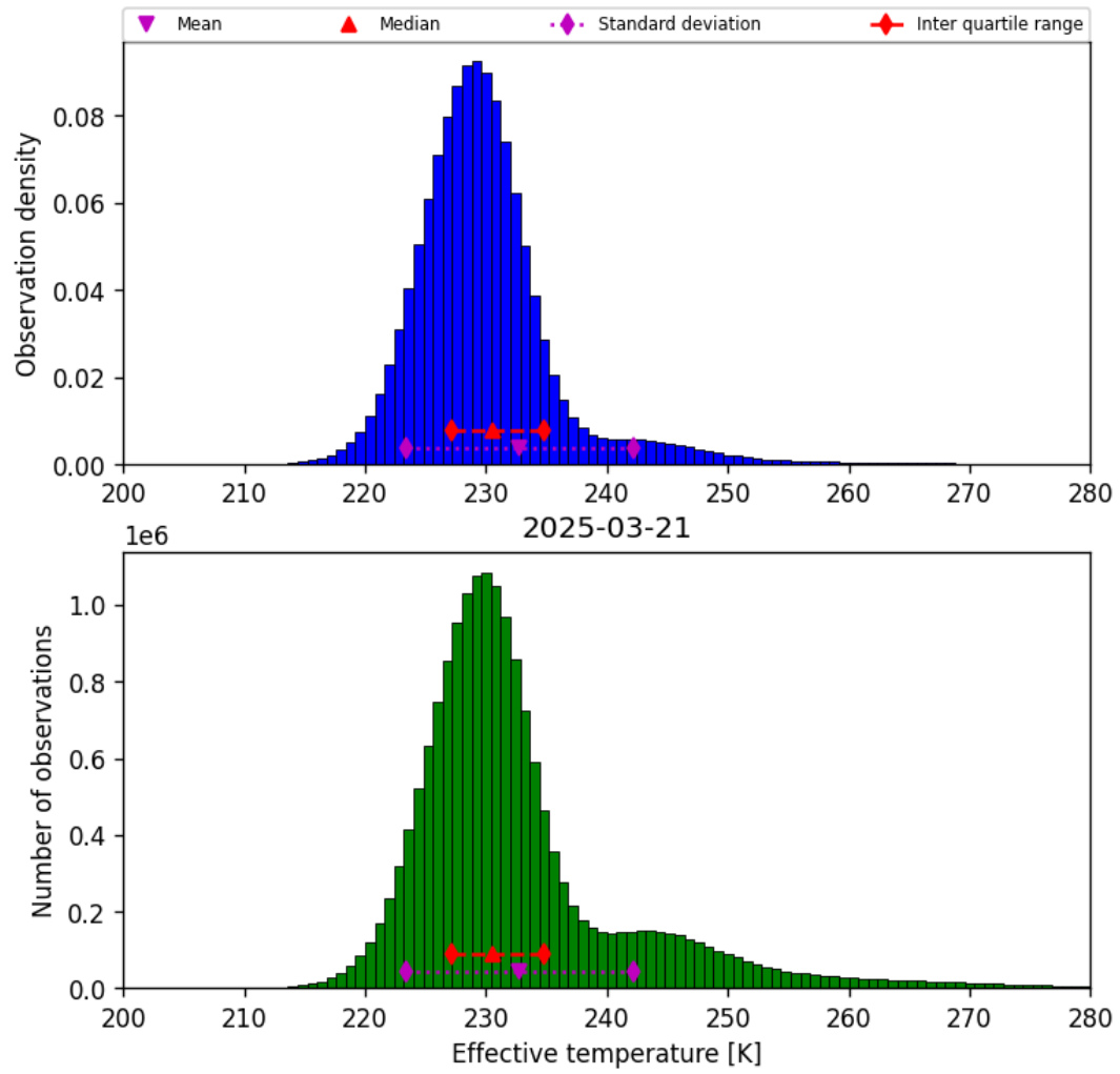
Figure 38: Histogram of “Effective temperature” for 2025-03-21 to 2025-03-21
