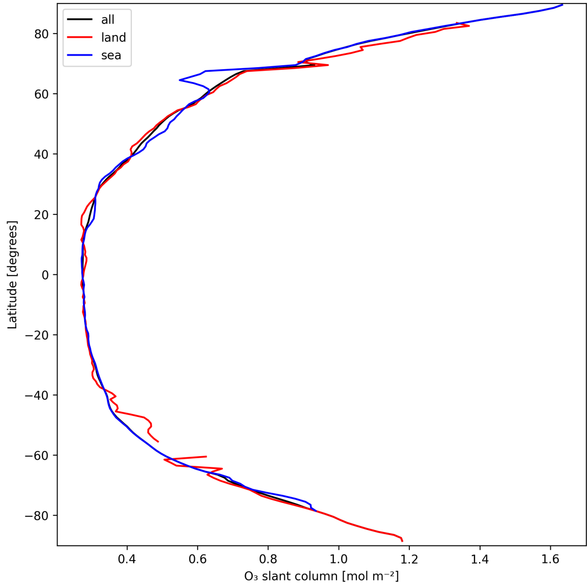
Figure 19: Zonal average of “O 3 slant column” for 2025-03-21 to 2025-03-21.
