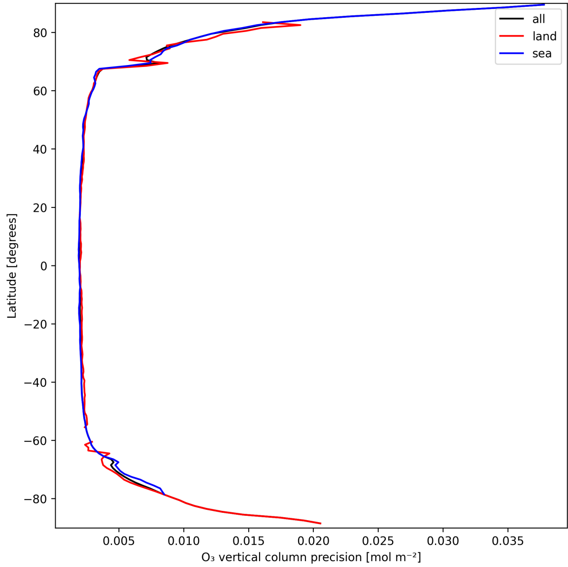
Figure 18: Zonal average of “O 3 vertical column precision” for 2025-03-21 to 2025-03-21.
