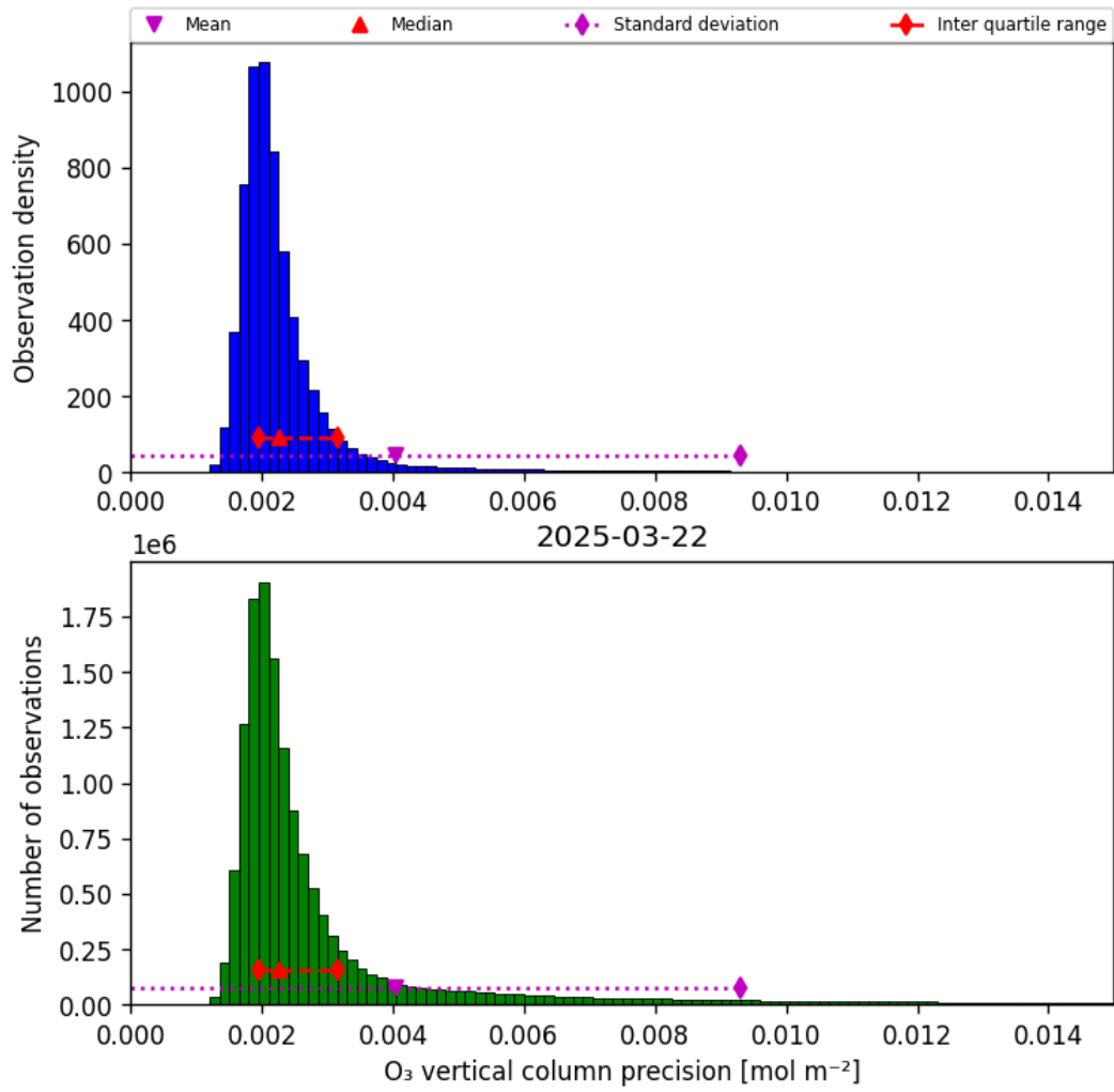
Figure 30: Histogram of “O 3 vertical column precision” for 2025-03-22 to 2025-03-22
