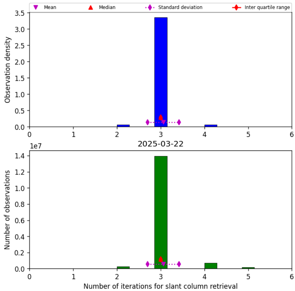
Figure 33: Histogram of “Number of iterations for slant column retrieval” for 2025-03-22 to 2025-03-22
