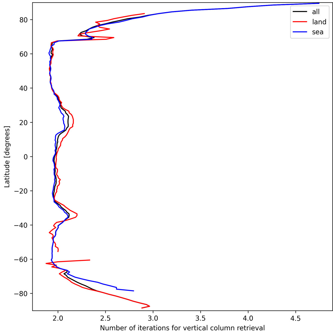
Figure 27: Zonal average of “Number of iterations for vertical column retrieval” for 2025-03-22 to 2025-03-22.
