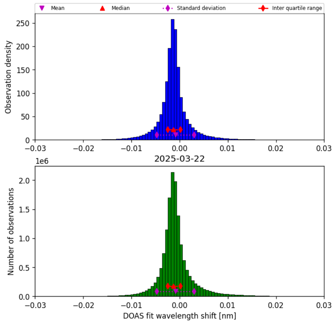
Figure 35: Histogram of “DOAS fit wavelength shift” for 2025-03-22 to 2025-03-22
