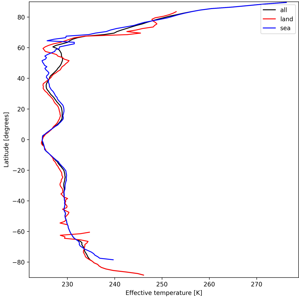
Figure 26: Zonal average of "Effective temperature" for 2025-03-22 to 2025-03-22.
