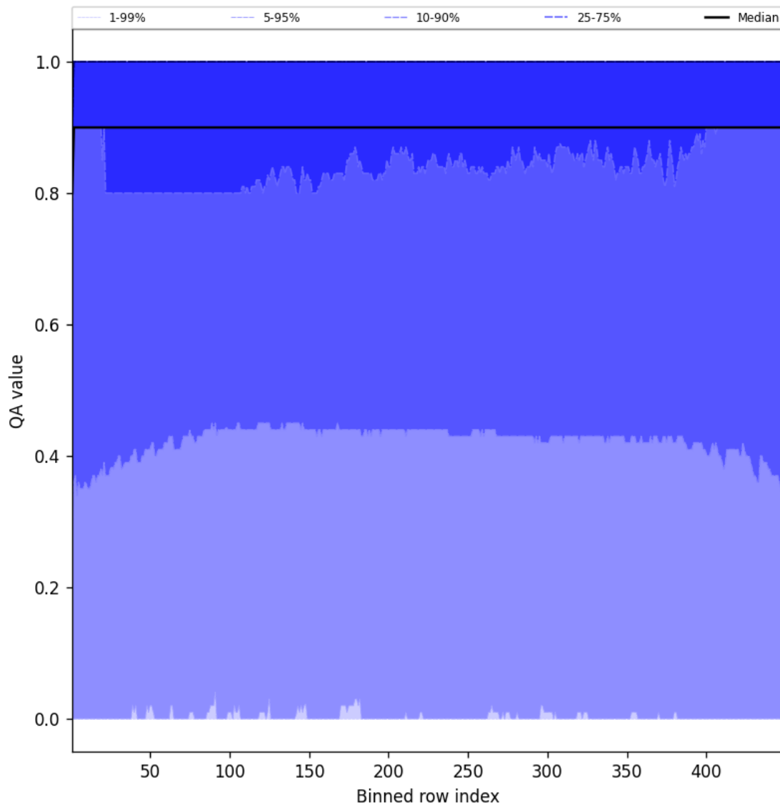
Figure 40: Along track statistics of “QA value” for 2025-03-22 to 2025-03-22
