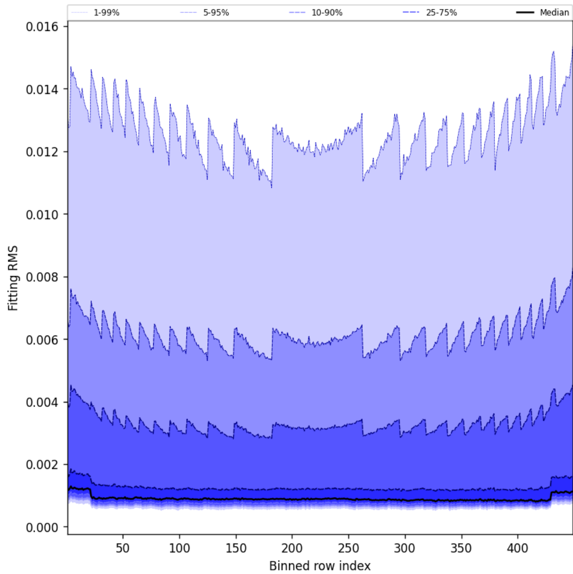
Figure 46: Along track statistics of “Fitting RMS” for 2025-03-22 to 2025-03-22
