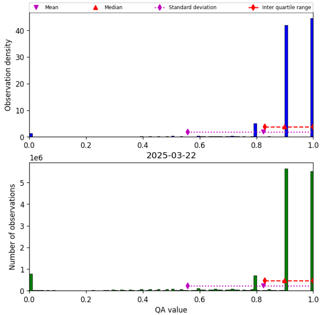
Figure 28: Histogram of “QA value” for 2025-03-22 to 2025-03-22
