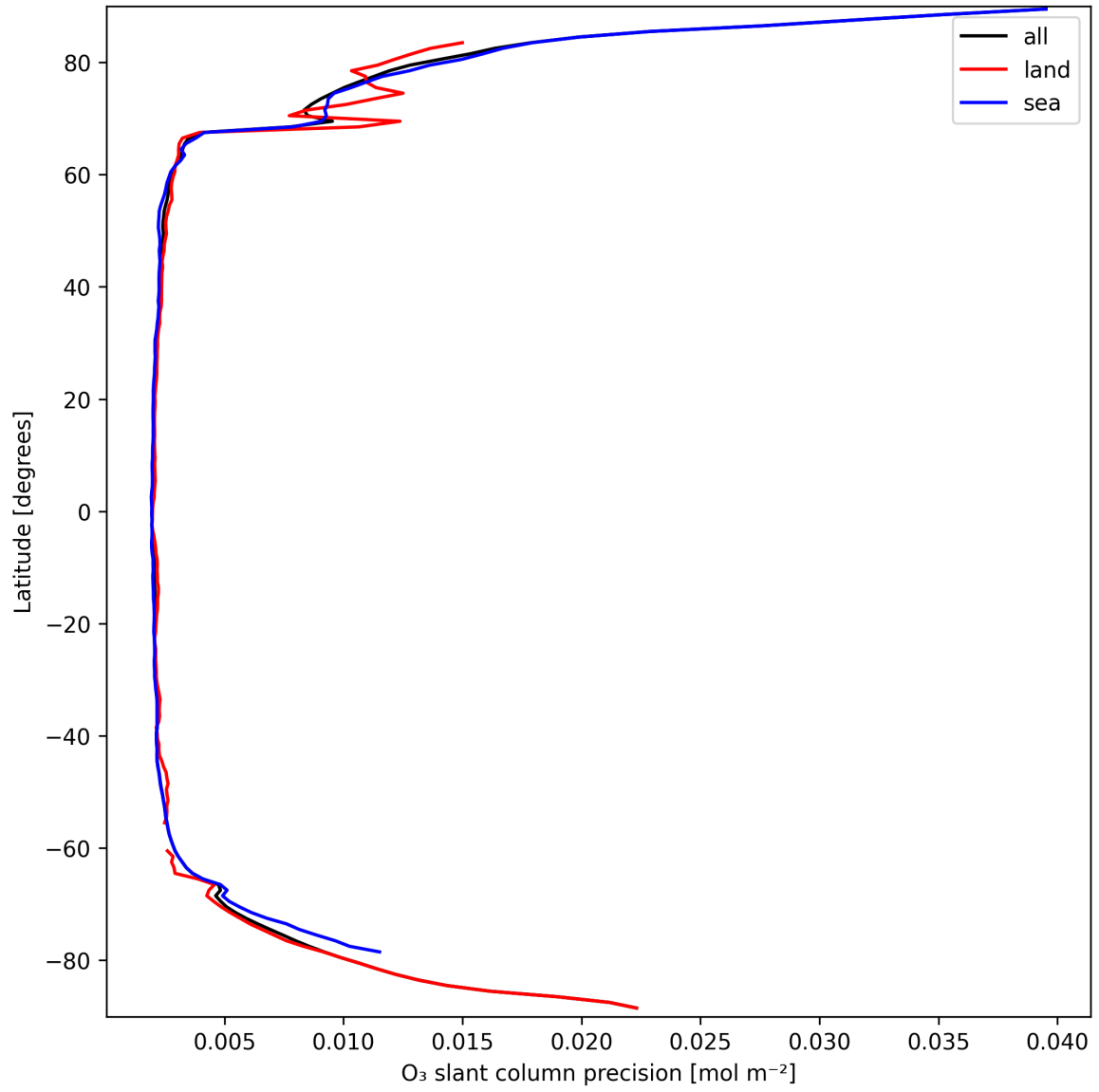
Figure 20: Zonal average of “O 3 slant column precision” for 2025-03-22 to 2025-03-22.
