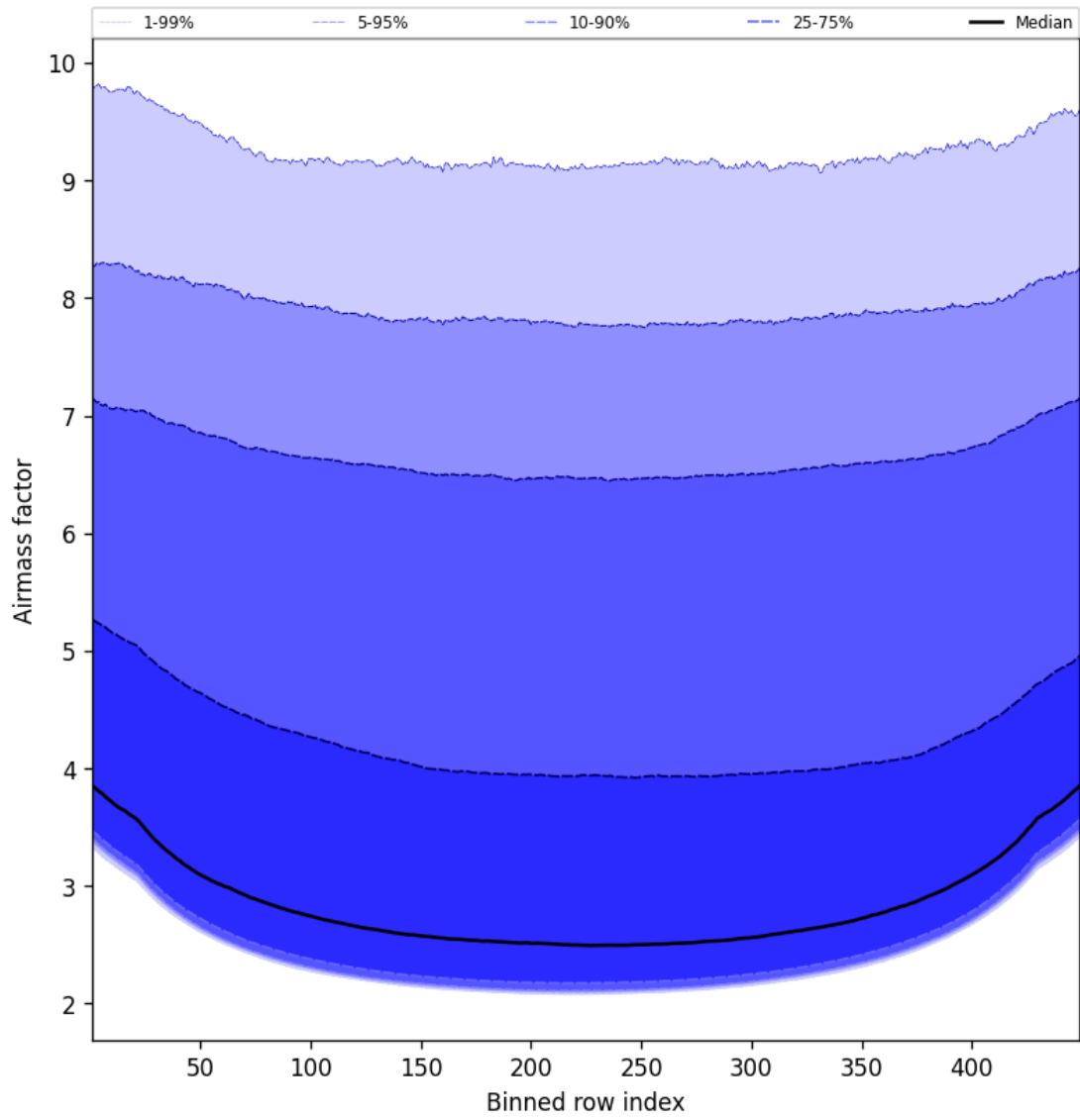
Figure 49: Along track statistics of “Airmass factor” for 2025-03-22 to 2025-03-22
