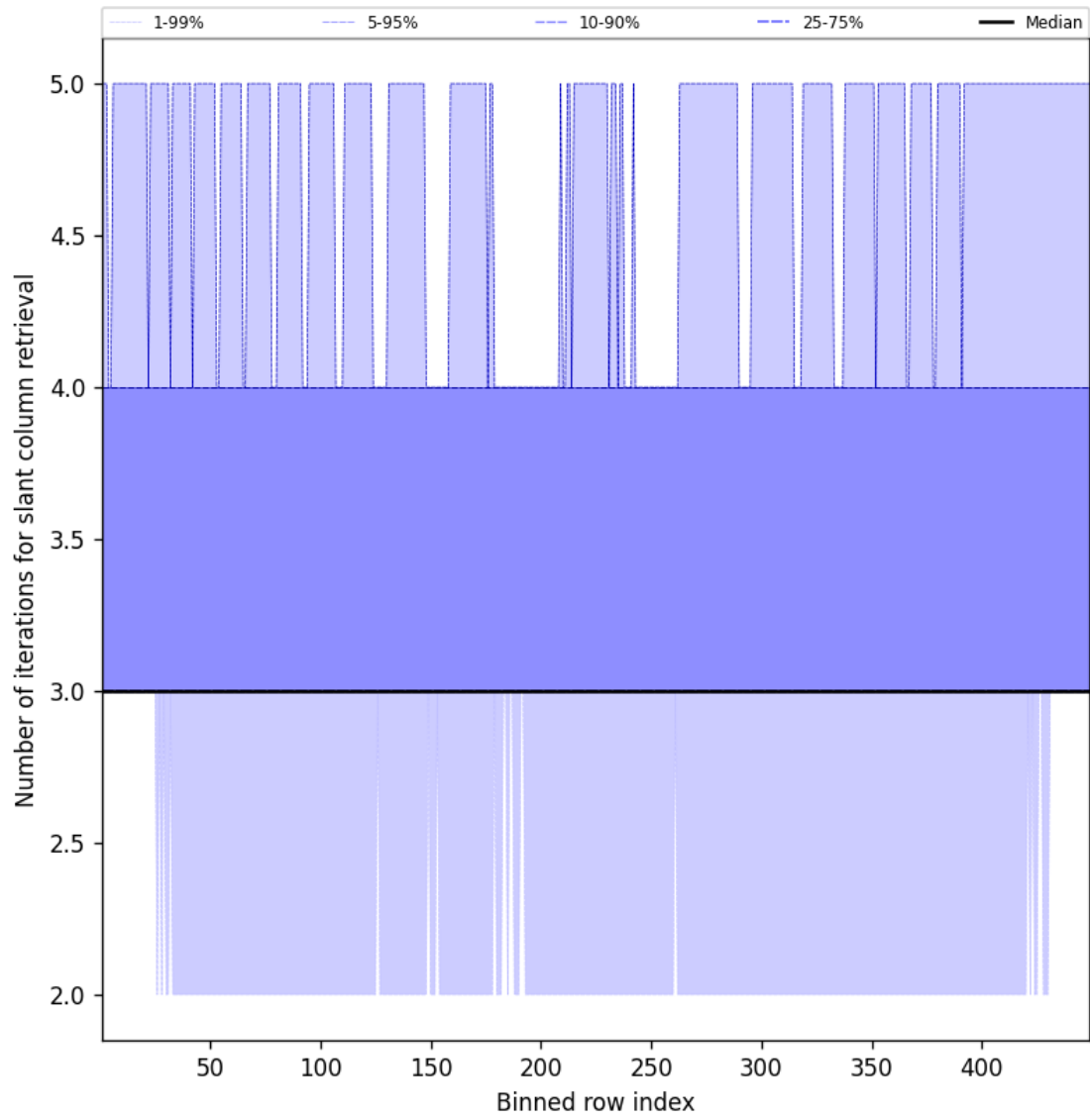
Figure 45: Along track statistics of “Number of iterations for slant column retrieval” for 2025-03-22 to 2025-03-22
