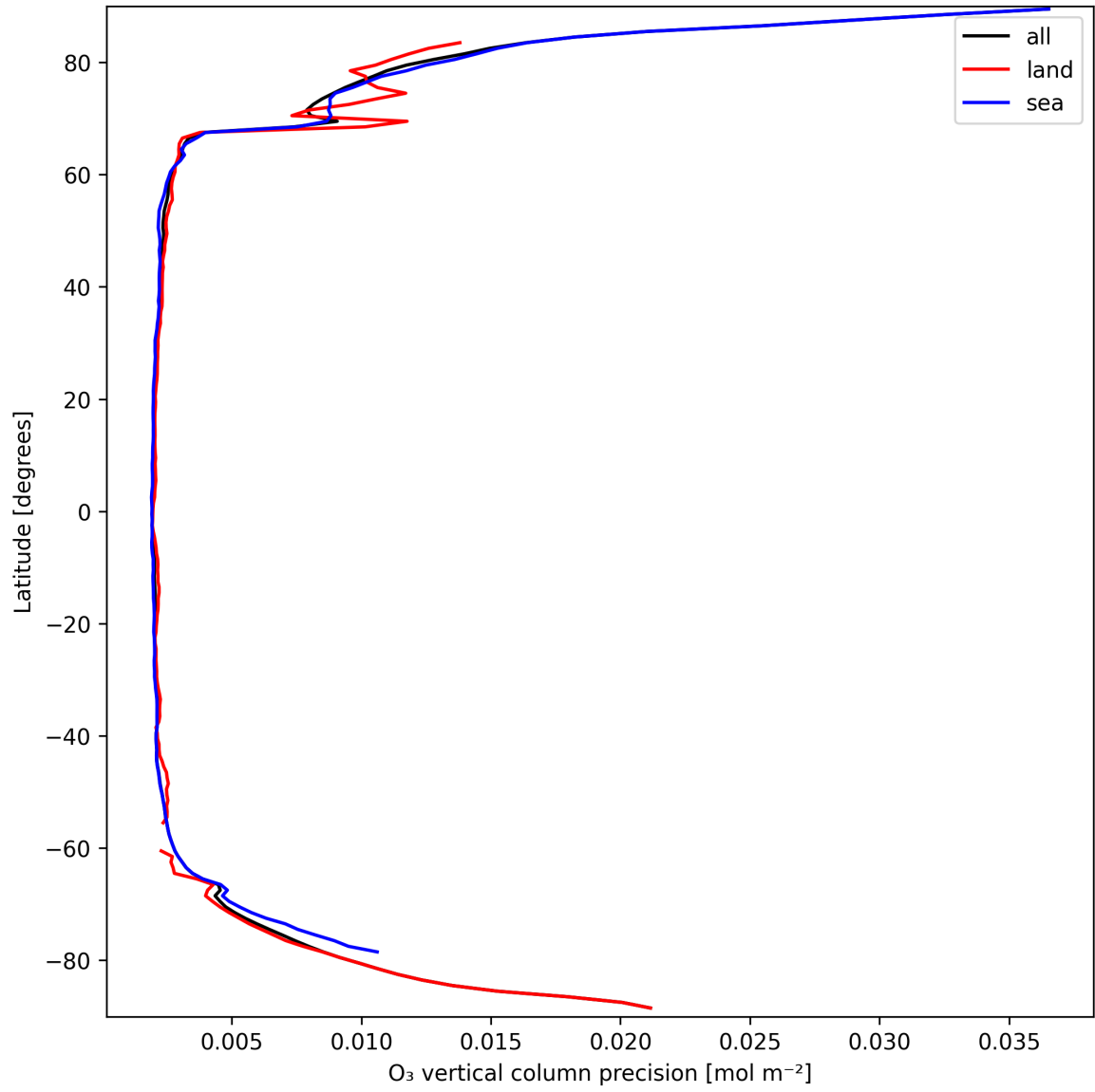
Figure 18: Zonal average of “O 3 vertical column precision” for 2025-03-22 to 2025-03-22.
