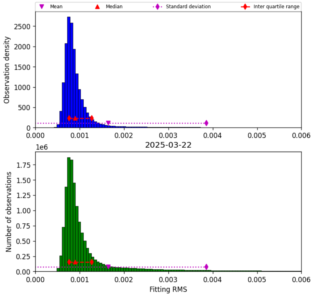
Figure 34: Histogram of “Fitting RMS” for 2025-03-22 to 2025-03-22
