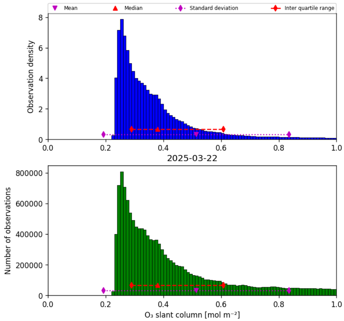
Figure 31: Histogram of “O 3 slant column” for 2025-03-22 to 2025-03-22
