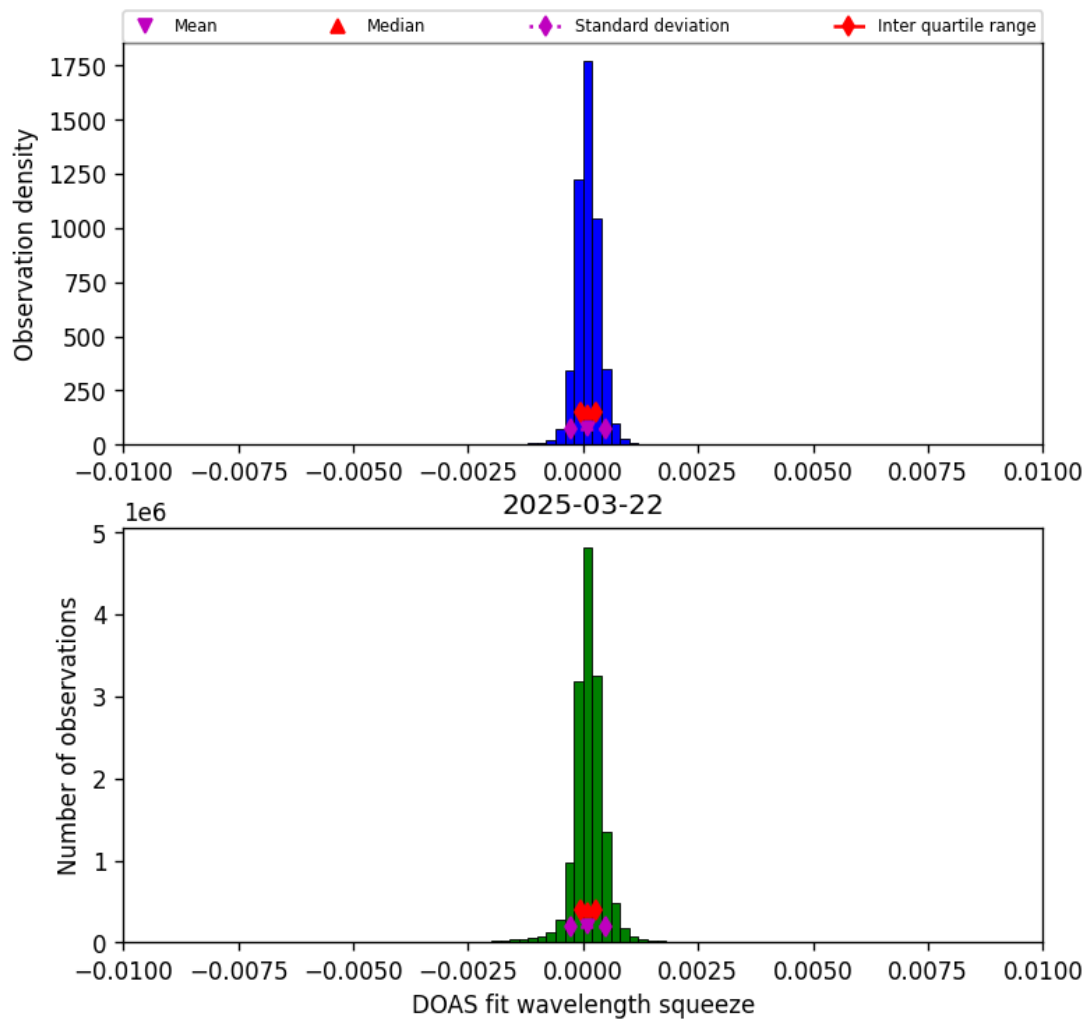
Figure 36: Histogram of “DOAS fit wavelength squeeze” for 2025-03-22 to 2025-03-22
