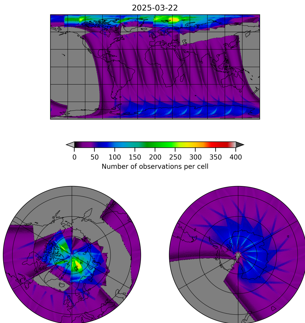
Figure 15: Map of the number of observations for 2025-03-22 to 2025-03-22
