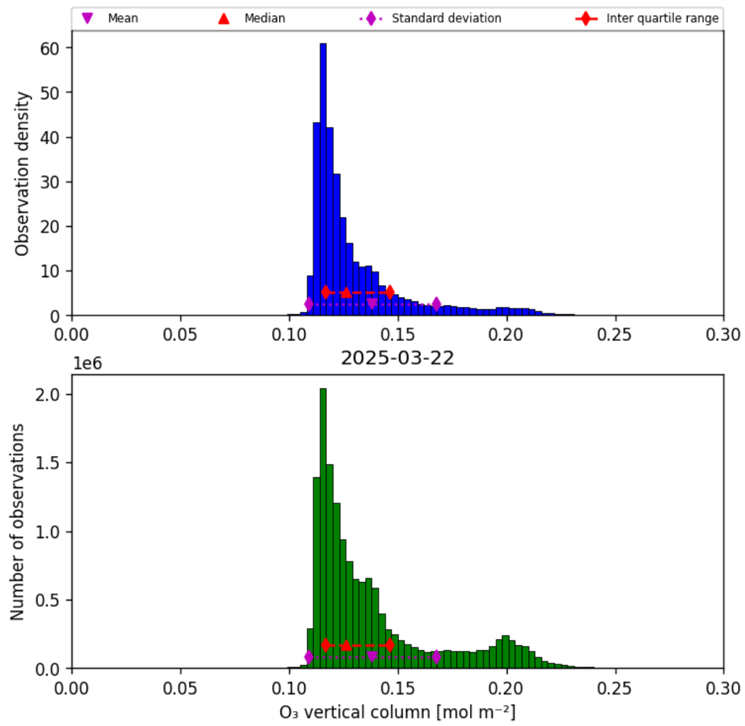
Figure 29: Histogram of “O 3 vertical column” for 2025-03-22 to 2025-03-22
