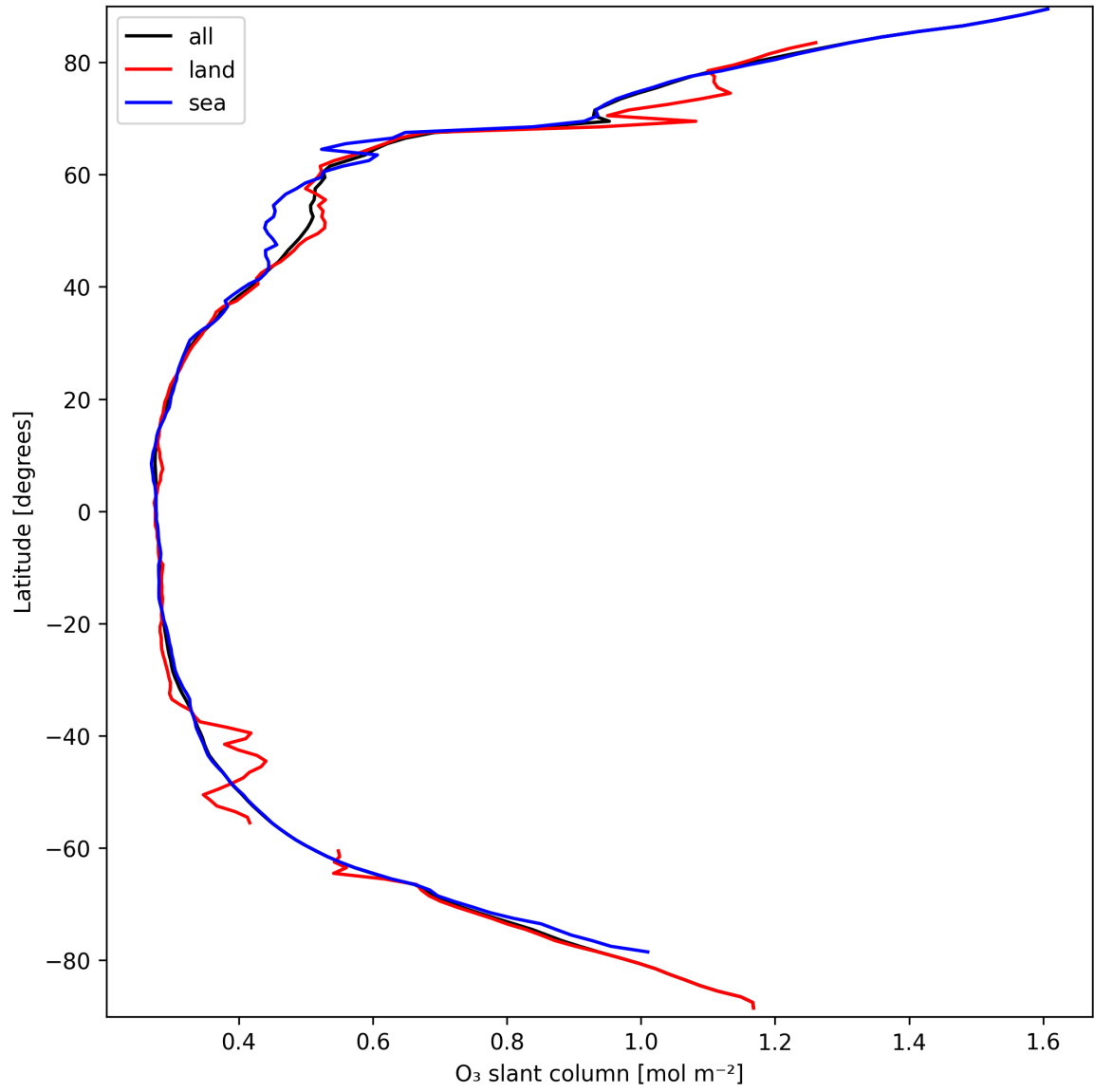
Figure 19: Zonal average of “O 3 slant column” for 2025-03-22 to 2025-03-22.
