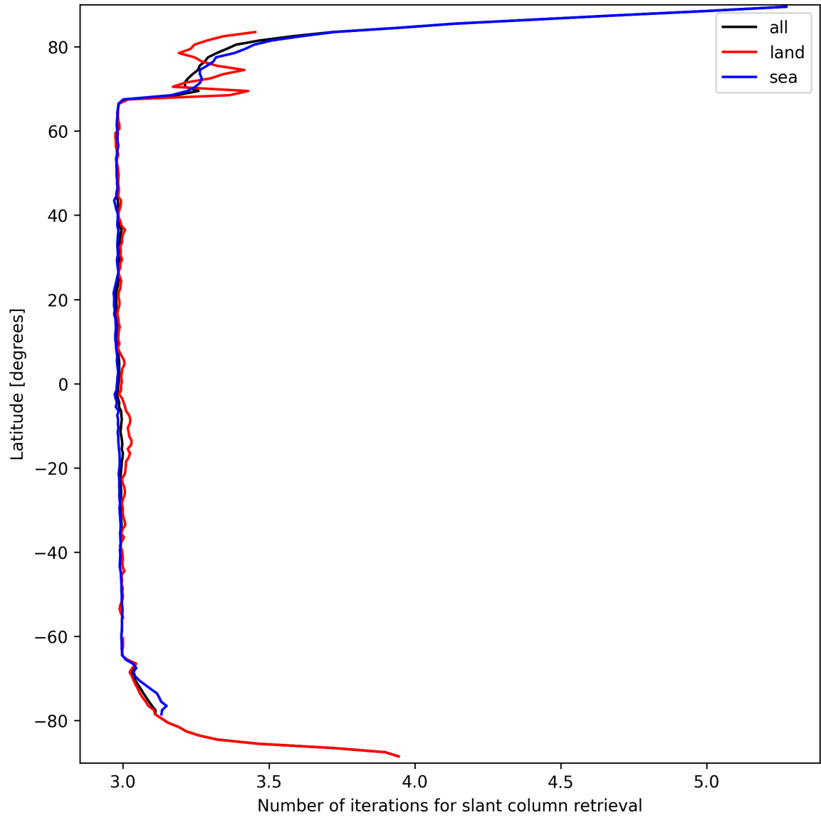
Figure 21: Zonal average of “Number of iterations for slant column retrieval” for 2025-03-22 to 2025-03-22.
