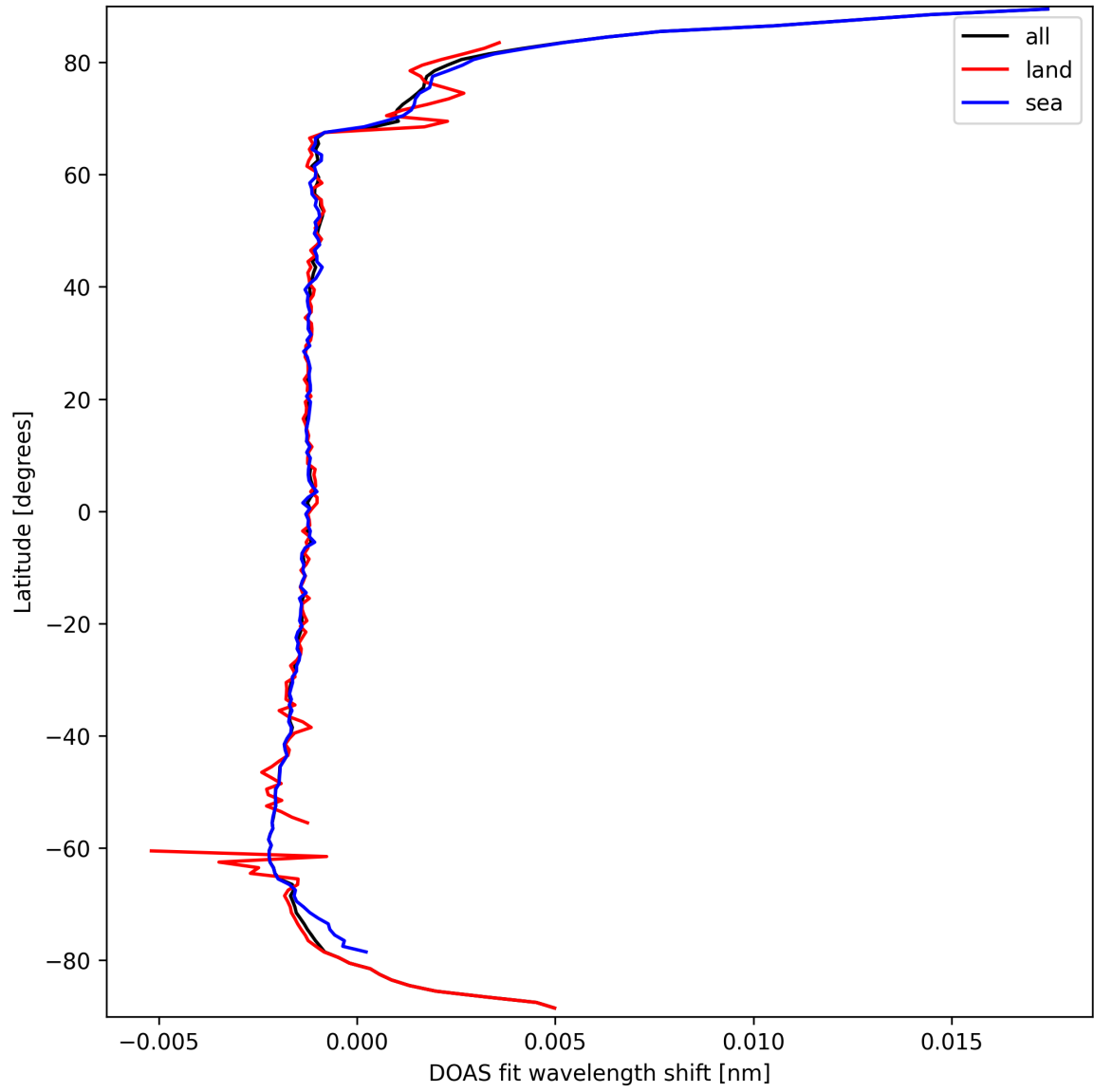
Figure 23: Zonal average of “DOAS fit wavelength shift” for 2025-03-22 to 2025-03-22.
