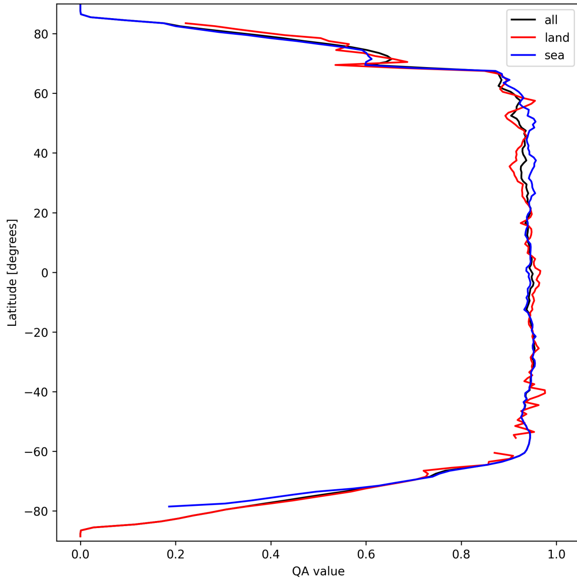
Figure 16: Zonal average of “QA value” for 2025-03-22 to 2025-03-22.
