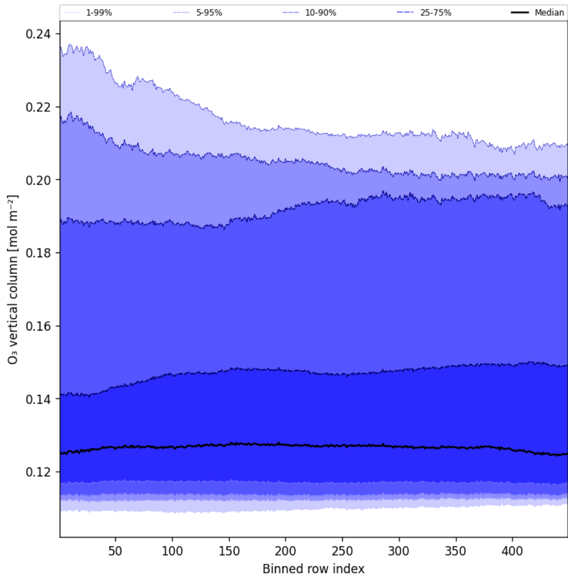
Figure 41: Along track statistics of “O 3 vertical column” for 2025-03-22 to 2025-03-22
