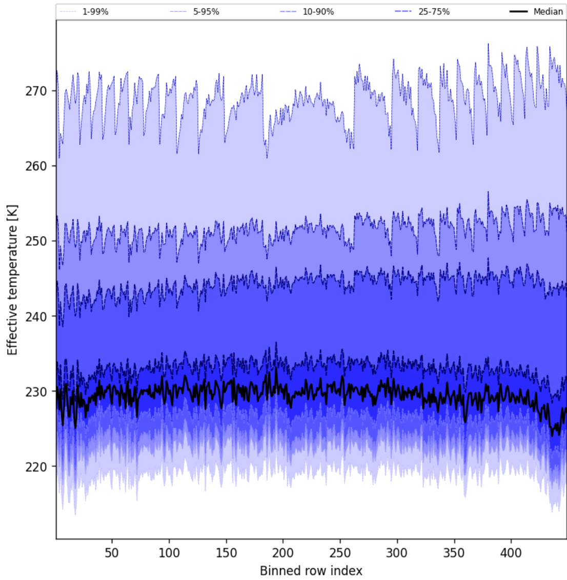
Figure 50: Along track statistics of “Effective temperature” for 2025-03-22 to 2025-03-22
