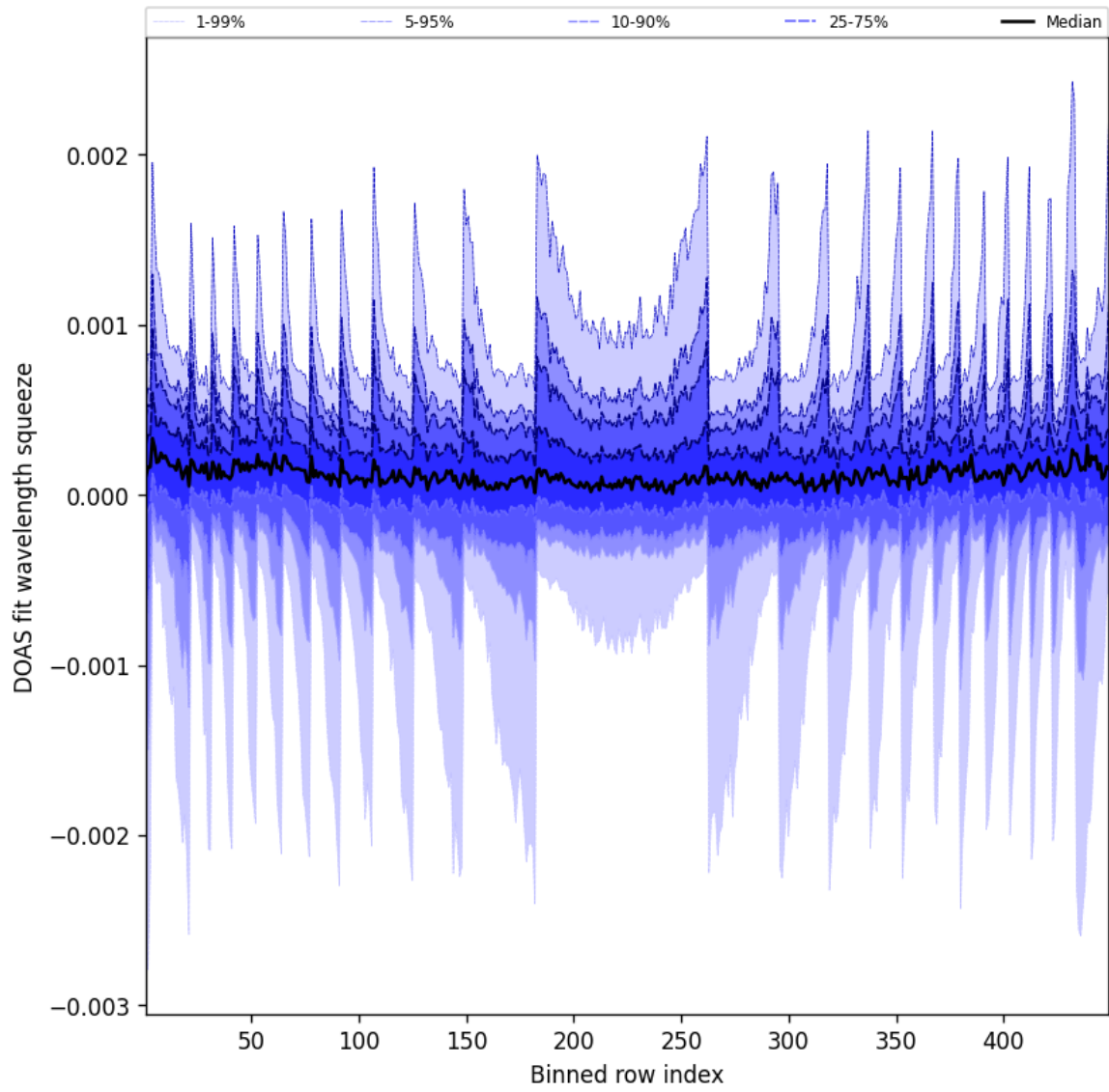
Figure 48: Along track statistics of “DOAS fit wavelength squeeze” for 2025-03-22 to 2025-03-22
