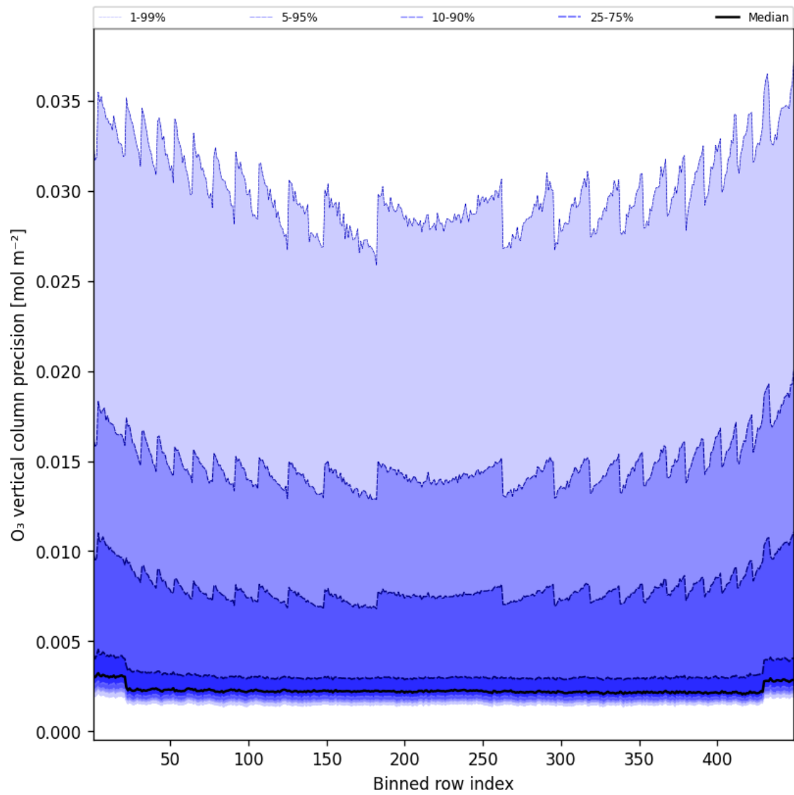
Figure 42: Along track statistics of “O 3 vertical column precision” for 2025-03-22 to 2025-03-22
