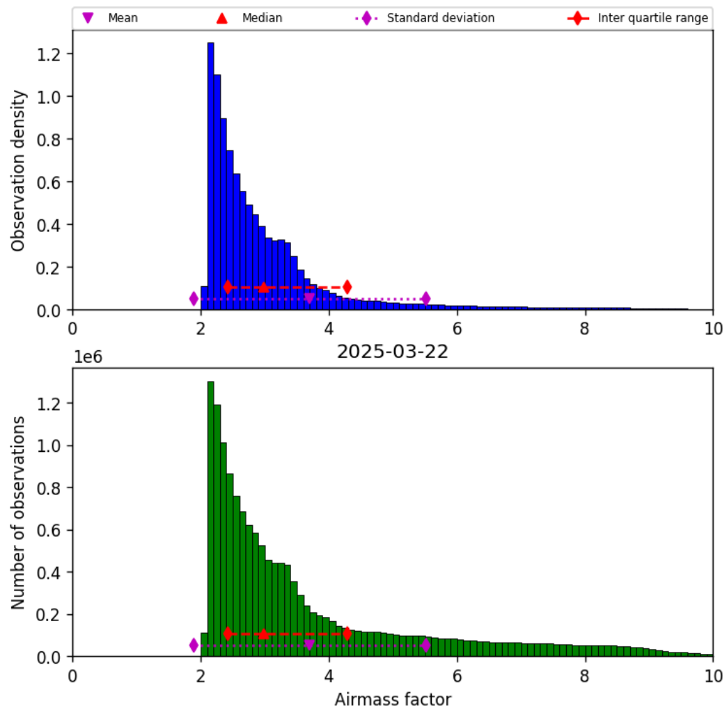
Figure 37: Histogram of “Airmass factor” for 2025-03-22 to 2025-03-22
