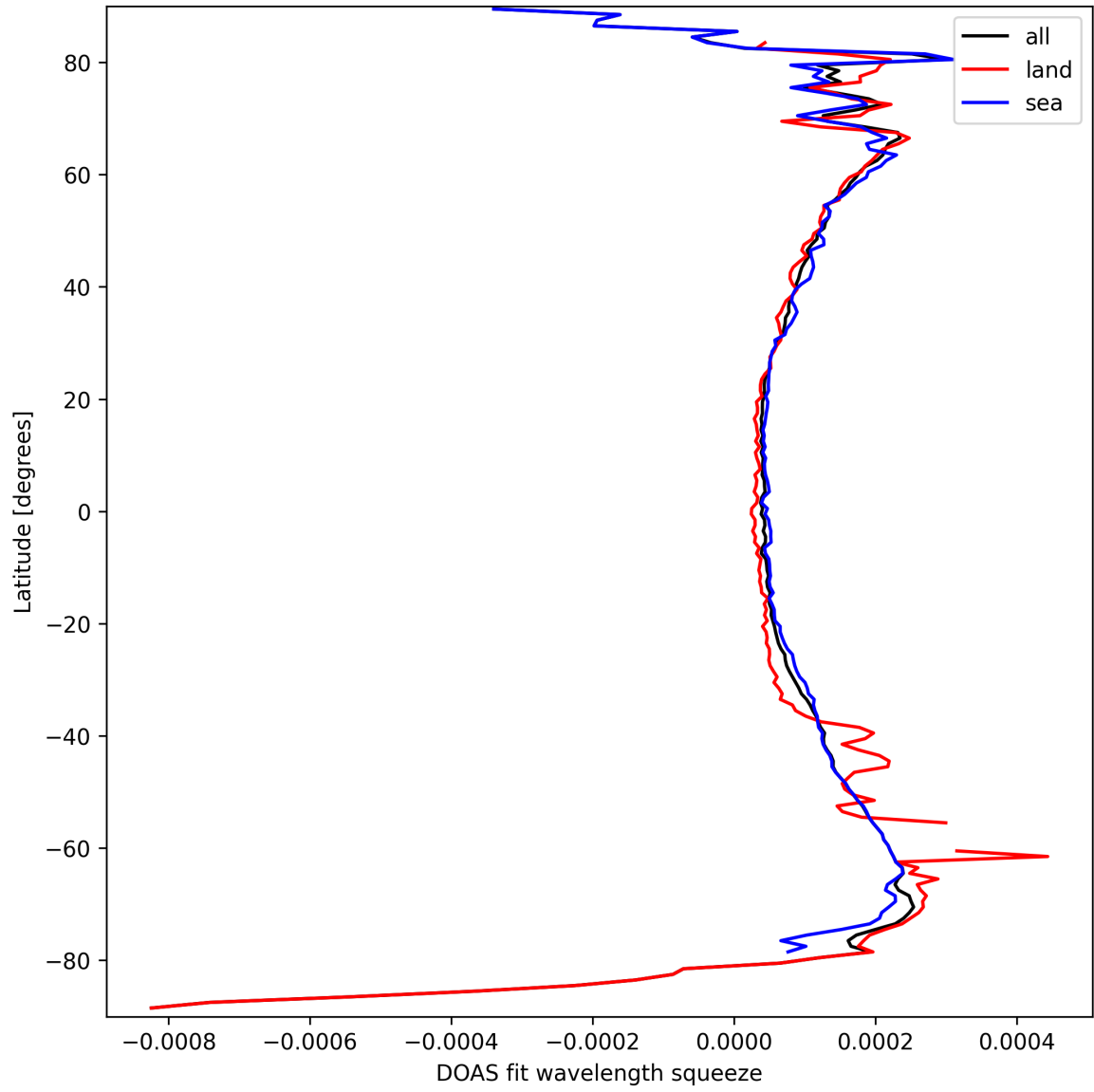
Figure 24: Zonal average of “DOAS fit wavelength squeeze” for 2025-03-22 to 2025-03-22.
