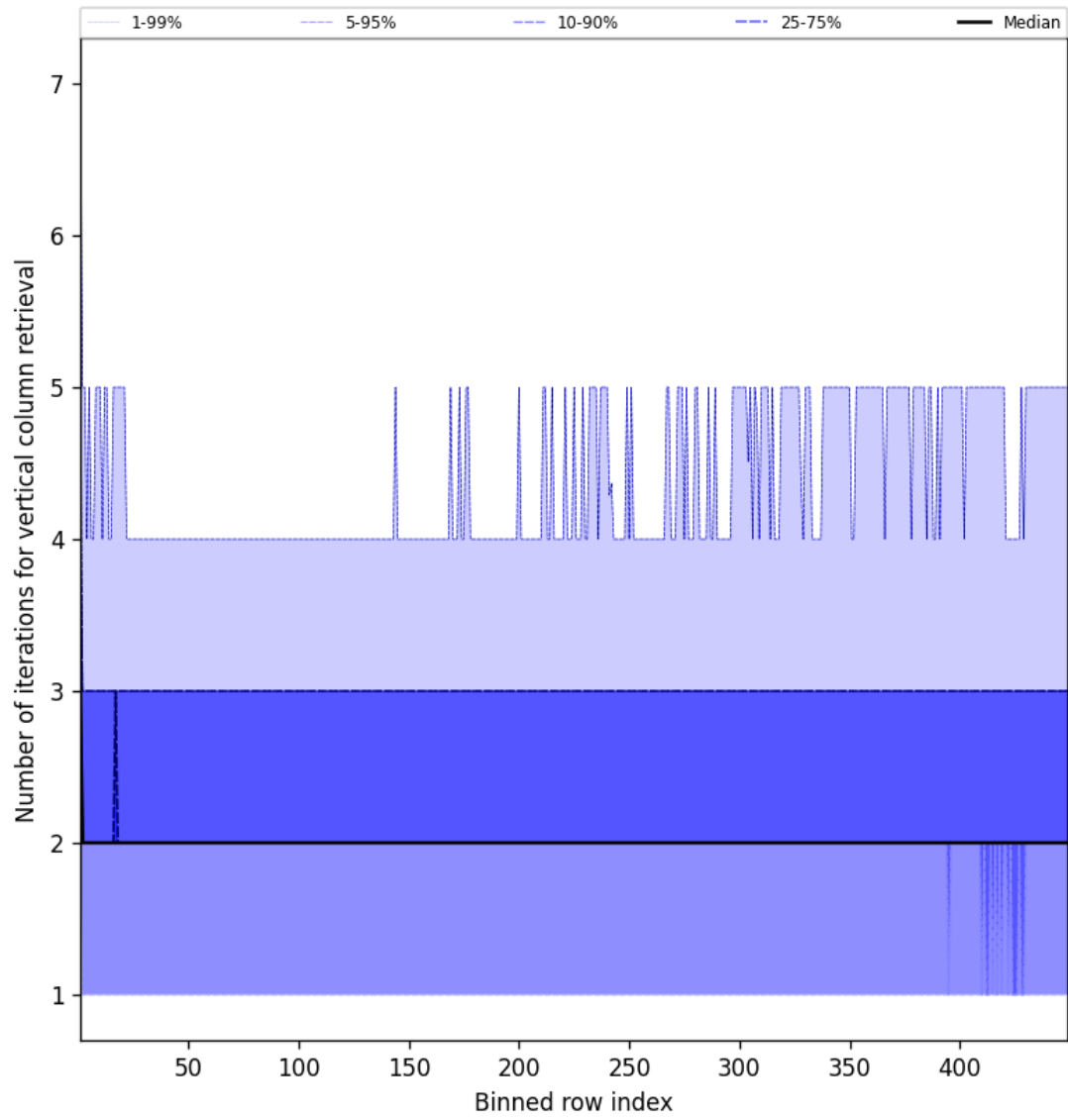
Figure 51: Along track statistics of “Number of iterations for vertical column retrieval” for 2025-03-22 to 2025-03-22
