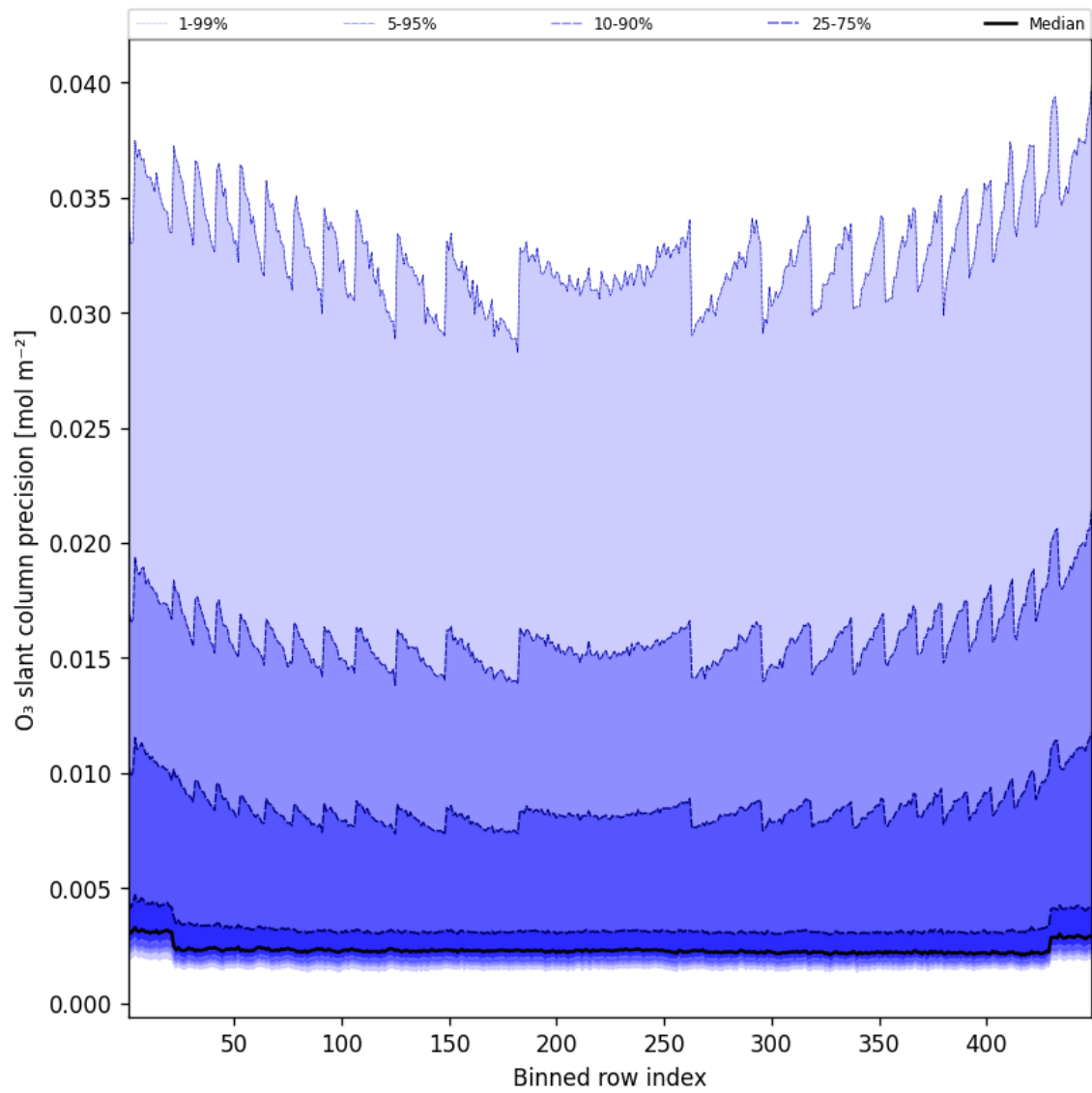
Figure 44: Along track statistics of “O 3 slant column precision” for 2025-03-22 to 2025-03-22
