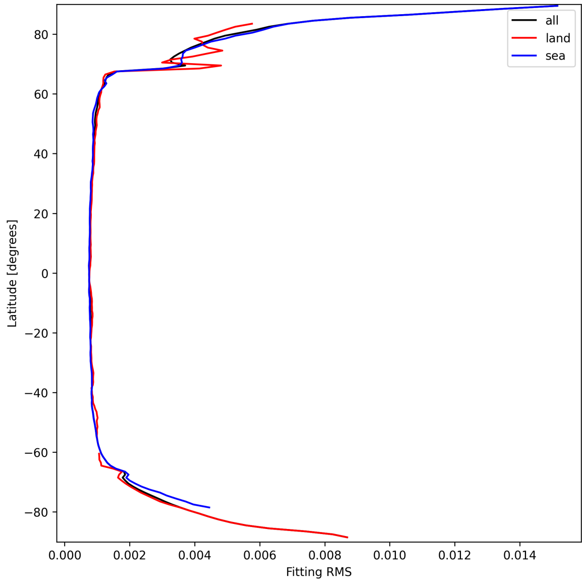
Figure 22: Zonal average of “Fitting RMS” for 2025-03-22 to 2025-03-22.
