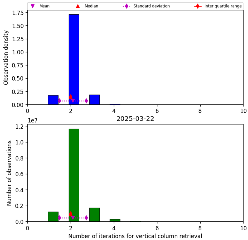
Figure 39: Histogram of “Number of iterations for vertical column retrieval” for 2025-03-22 to 2025-03-22
