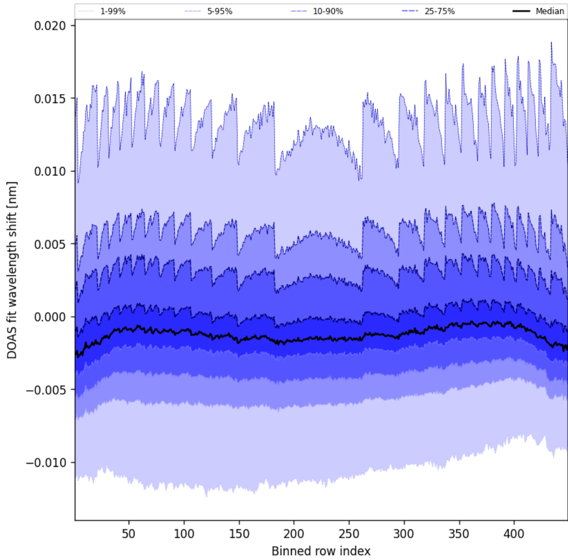
Figure 47: Along track statistics of “DOAS fit wavelength shift” for 2025-03-22 to 2025-03-22
