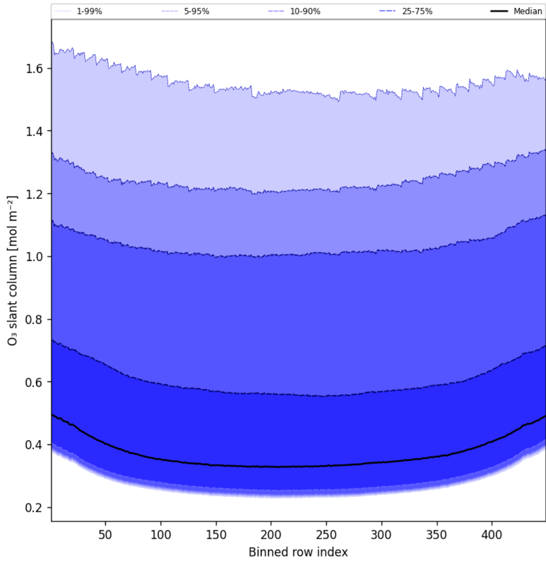
Figure 43: Along track statistics of “O 3 slant column” for 2025-03-22 to 2025-03-22
