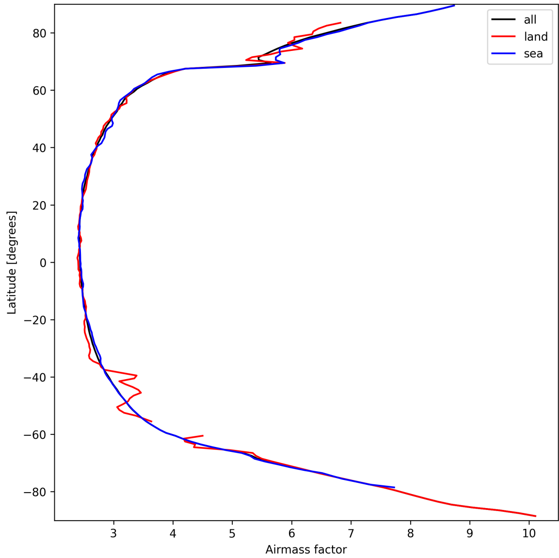
Figure 25: Zonal average of “Airmass factor” for 2025-03-22 to 2025-03-22.
