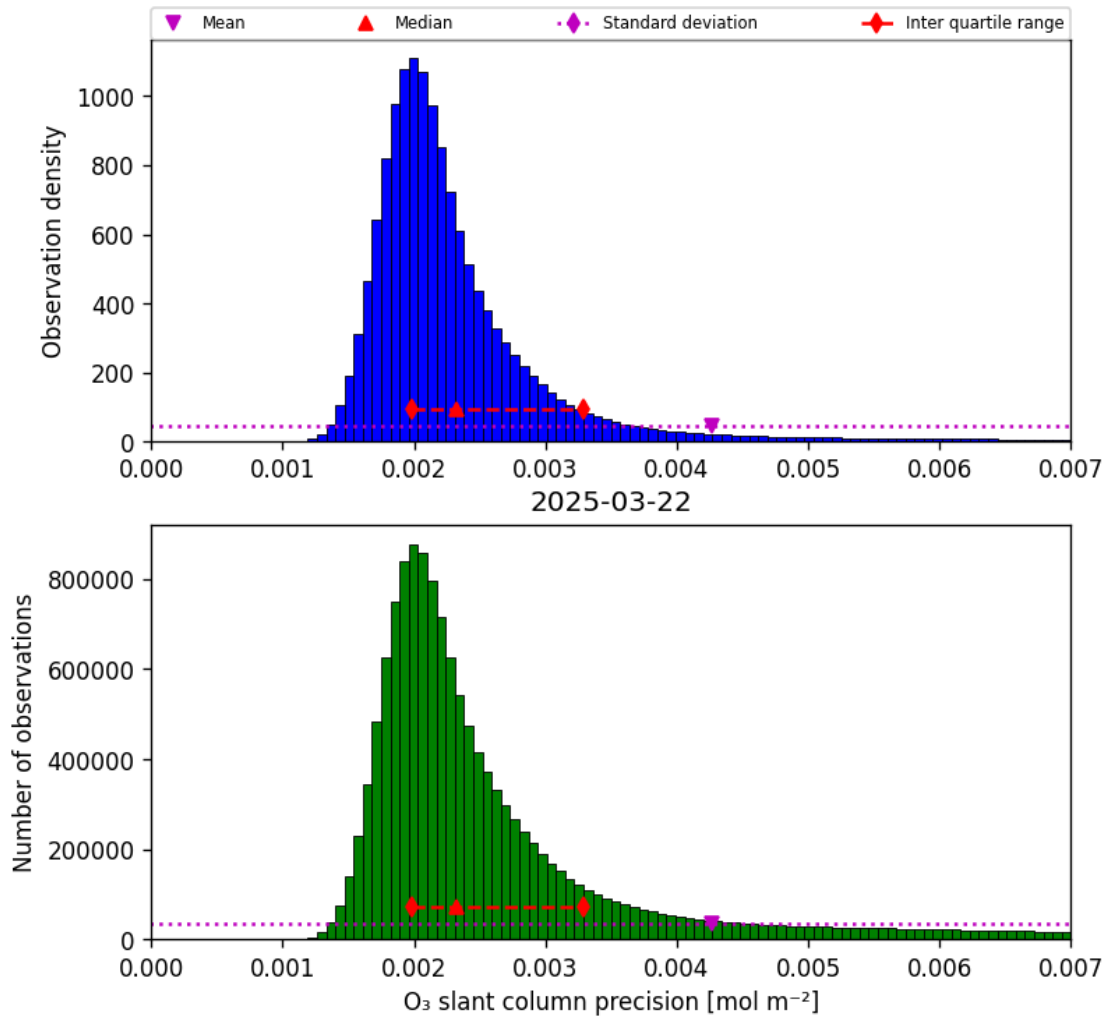
Figure 32: Histogram of "O 3 slant column precision" for 2025-03-22 to 2025-03-22
