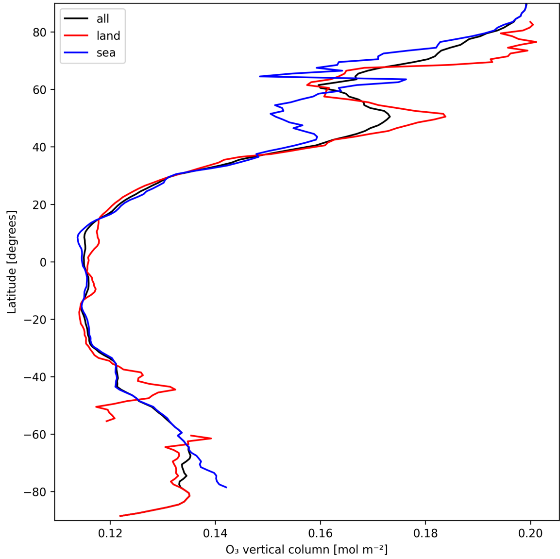
Figure 17: Zonal average of “O 3 vertical column” for 2025-03-22 to 2025-03-22.
