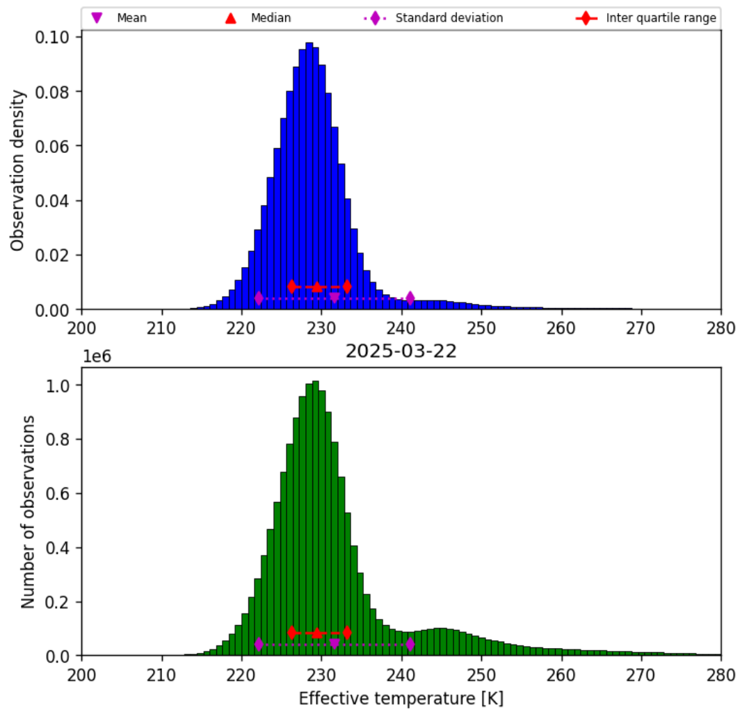
Figure 38: Histogram of “Effective temperature” for 2025-03-22 to 2025-03-22
