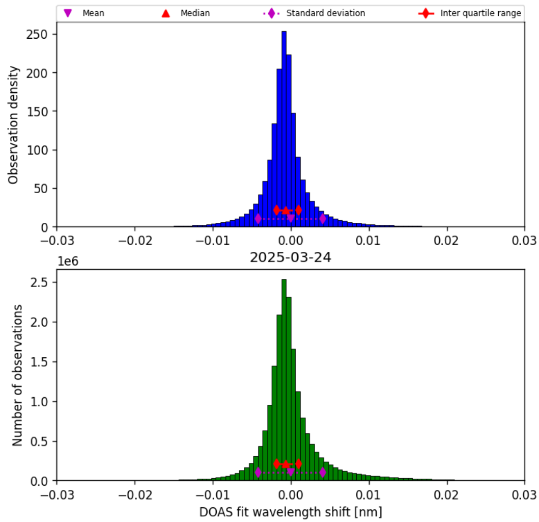
Figure 35: Histogram of “DOAS fit wavelength shift” for 2025-03-24 to 2025-03-25
