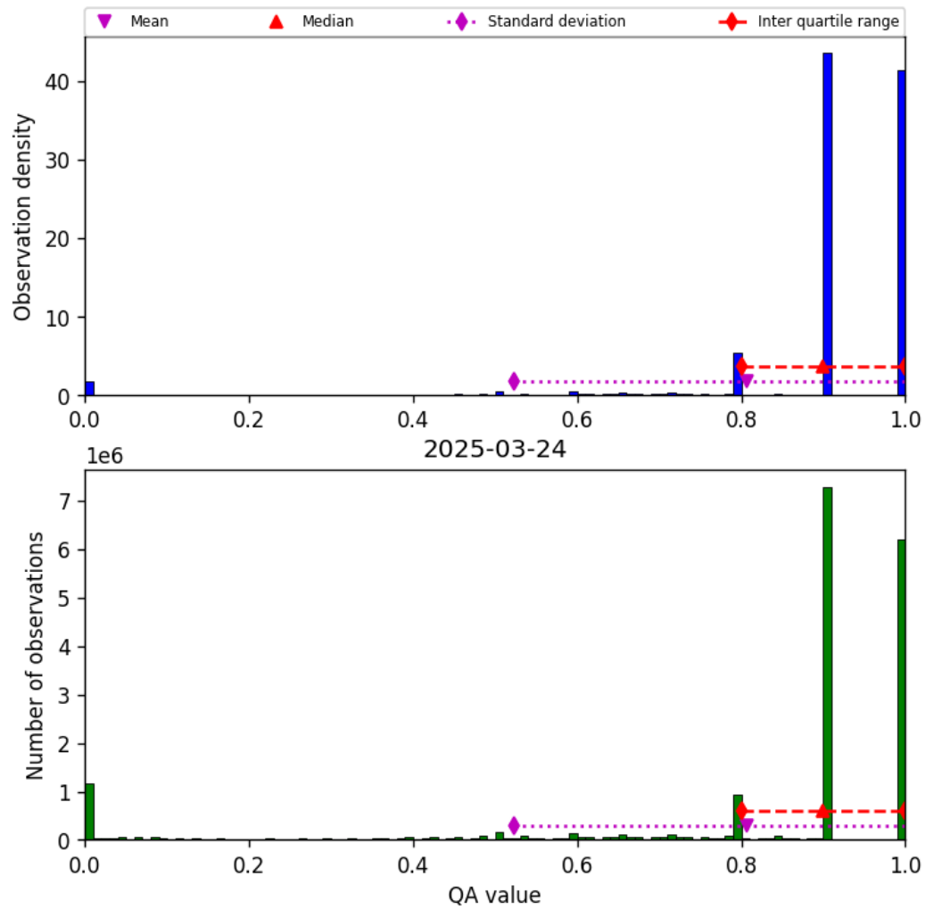
Figure 28: Histogram of “QA value” for 2025-03-24 to 2025-03-25
