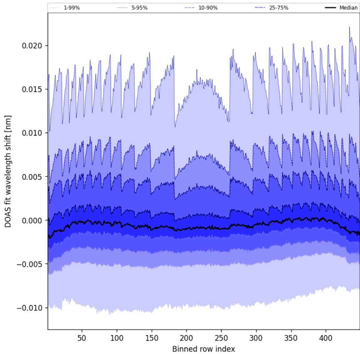
Figure 47: Along track statistics of “DOAS fit wavelength shift” for 2025-03-24 to 2025-03-25
