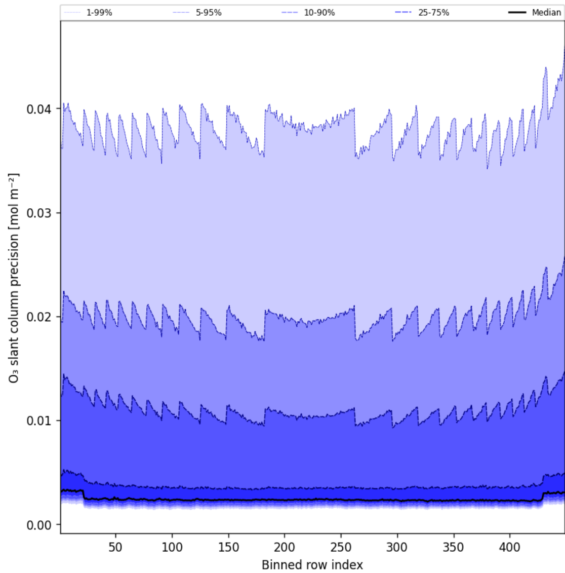
Figure 44: Along track statistics of “O 3 slant column precision” for 2025-03-24 to 2025-03-25
