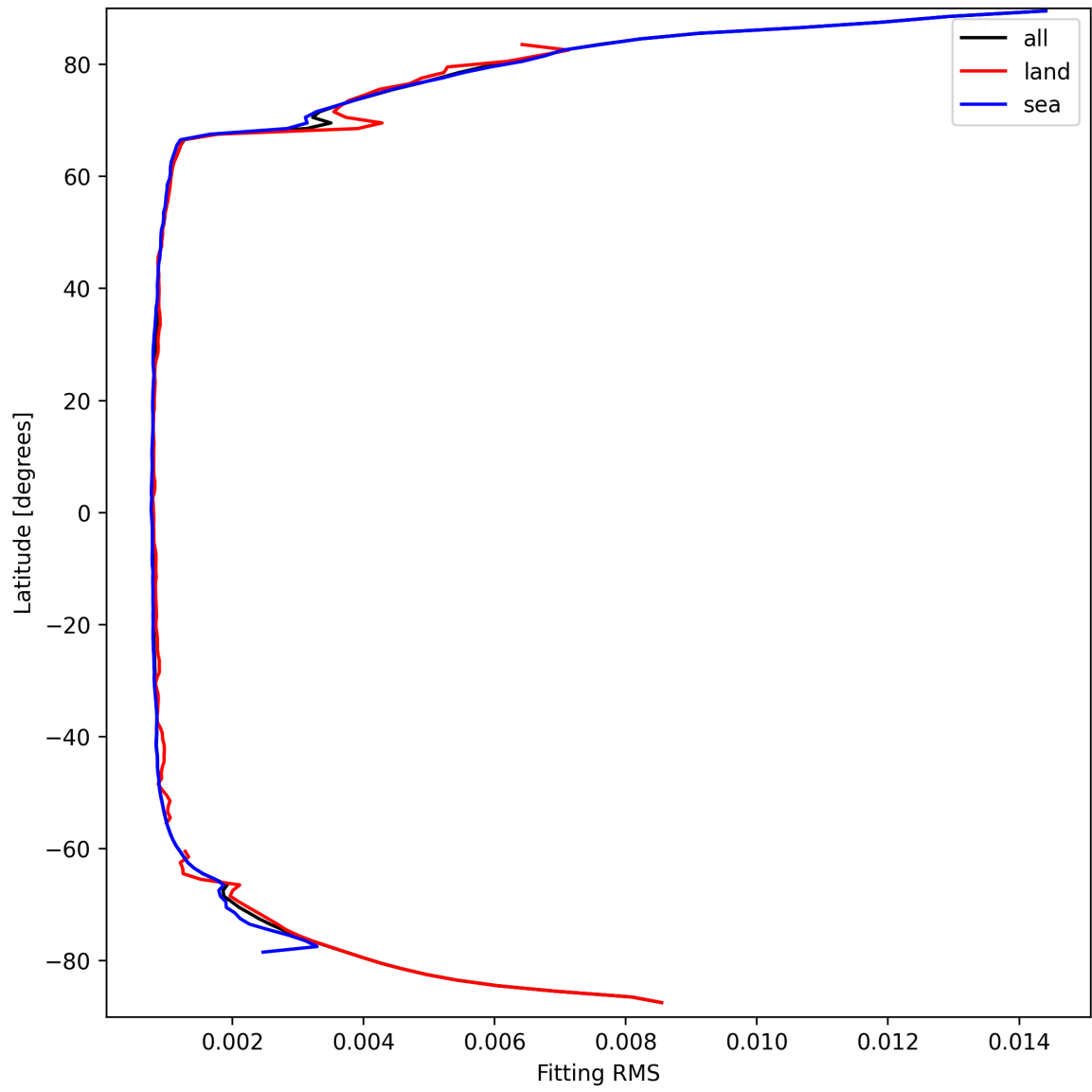
Figure 22: Zonal average of “Fitting RMS” for 2025-03-24 to 2025-03-25.
