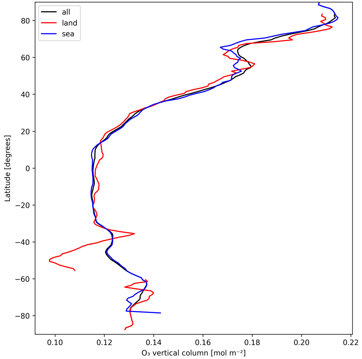
Figure 17: Zonal average of “O 3 vertical column” for 2025-03-24 to 2025-03-25.
