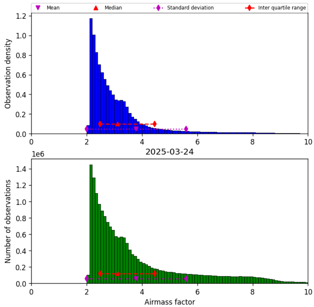
Figure 37: Histogram of “Airmass factor” for 2025-03-24 to 2025-03-25
