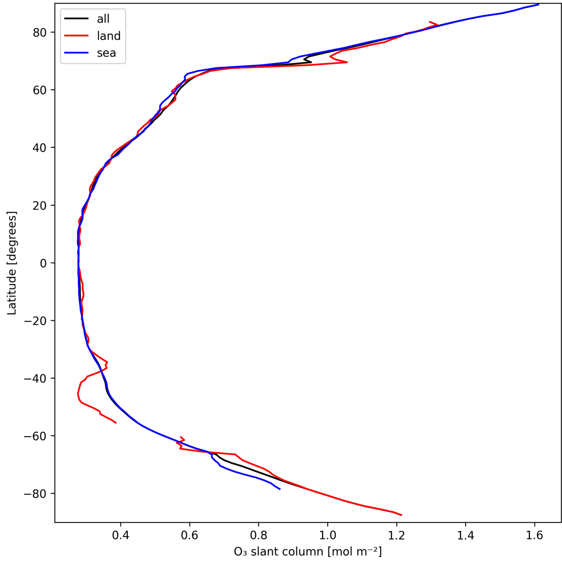
Figure 19: Zonal average of “O 3 slant column” for 2025-03-24 to 2025-03-25.
