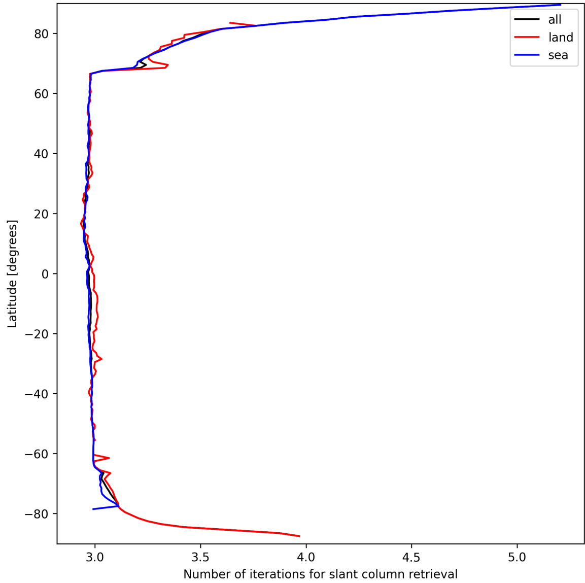
Figure 21: Zonal average of “Number of iterations for slant column retrieval” for 2025-03-24 to 2025-03-25.
