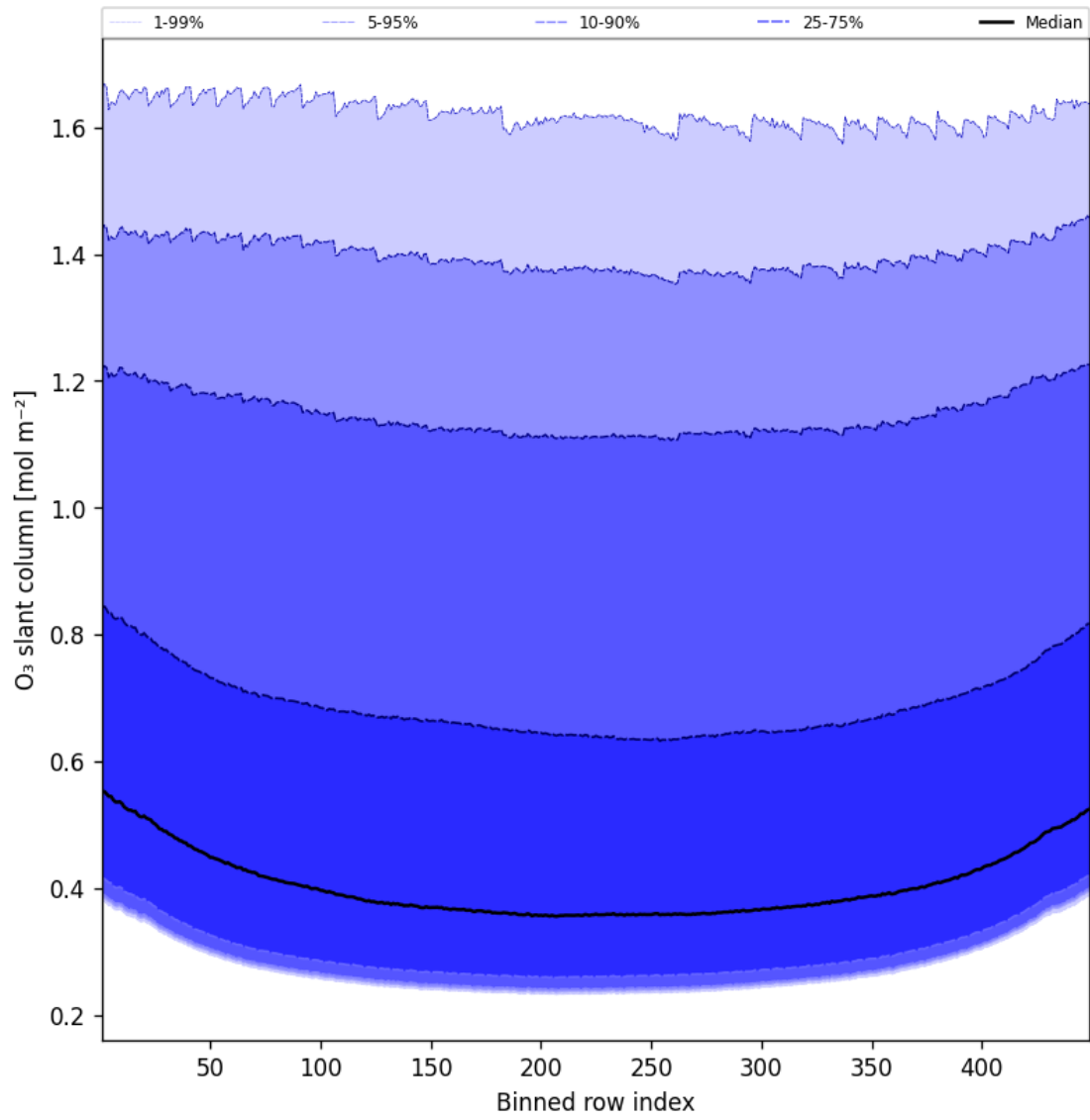
Figure 43: Along track statistics of “O 3 slant column” for 2025-03-24 to 2025-03-25
