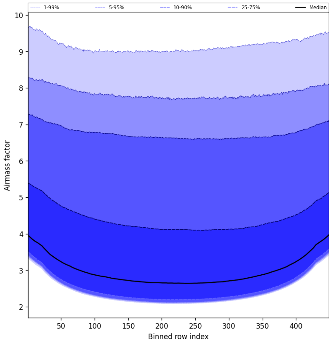
Figure 49: Along track statistics of “Airmass factor” for 2025-03-24 to 2025-03-25
