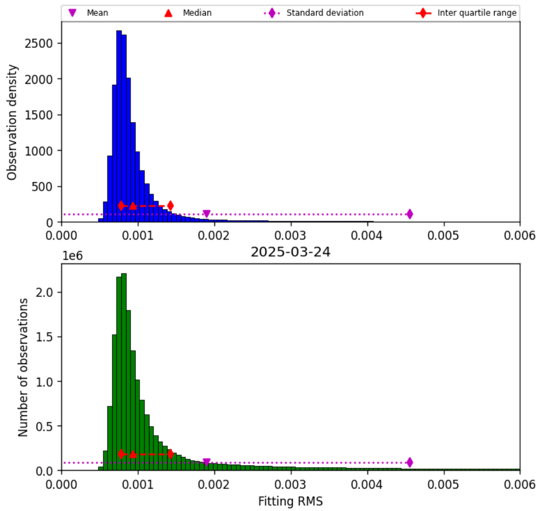
Figure 34: Histogram of “Fitting RMS” for 2025-03-24 to 2025-03-25
