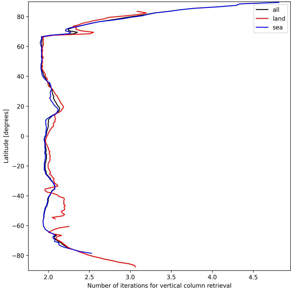
Figure 27: Zonal average of “Number of iterations for vertical column retrieval” for 2025-03-24 to 2025-03-25.
