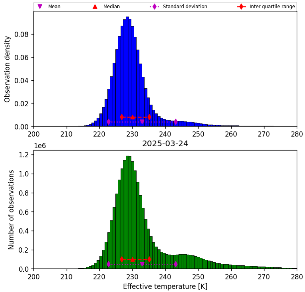
Figure 38: Histogram of “Effective temperature” for 2025-03-24 to 2025-03-25
