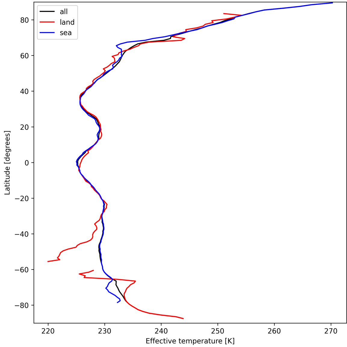
Figure 26: Zonal average of “Effective temperature” for 2025-03-24 to 2025-03-25.
