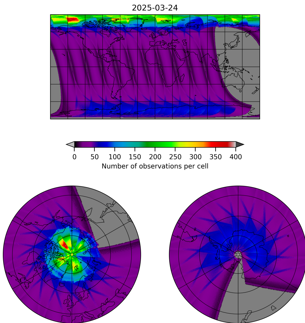
Figure 15: Map of the number of observations for 2025-03-24 to 2025-03-25
