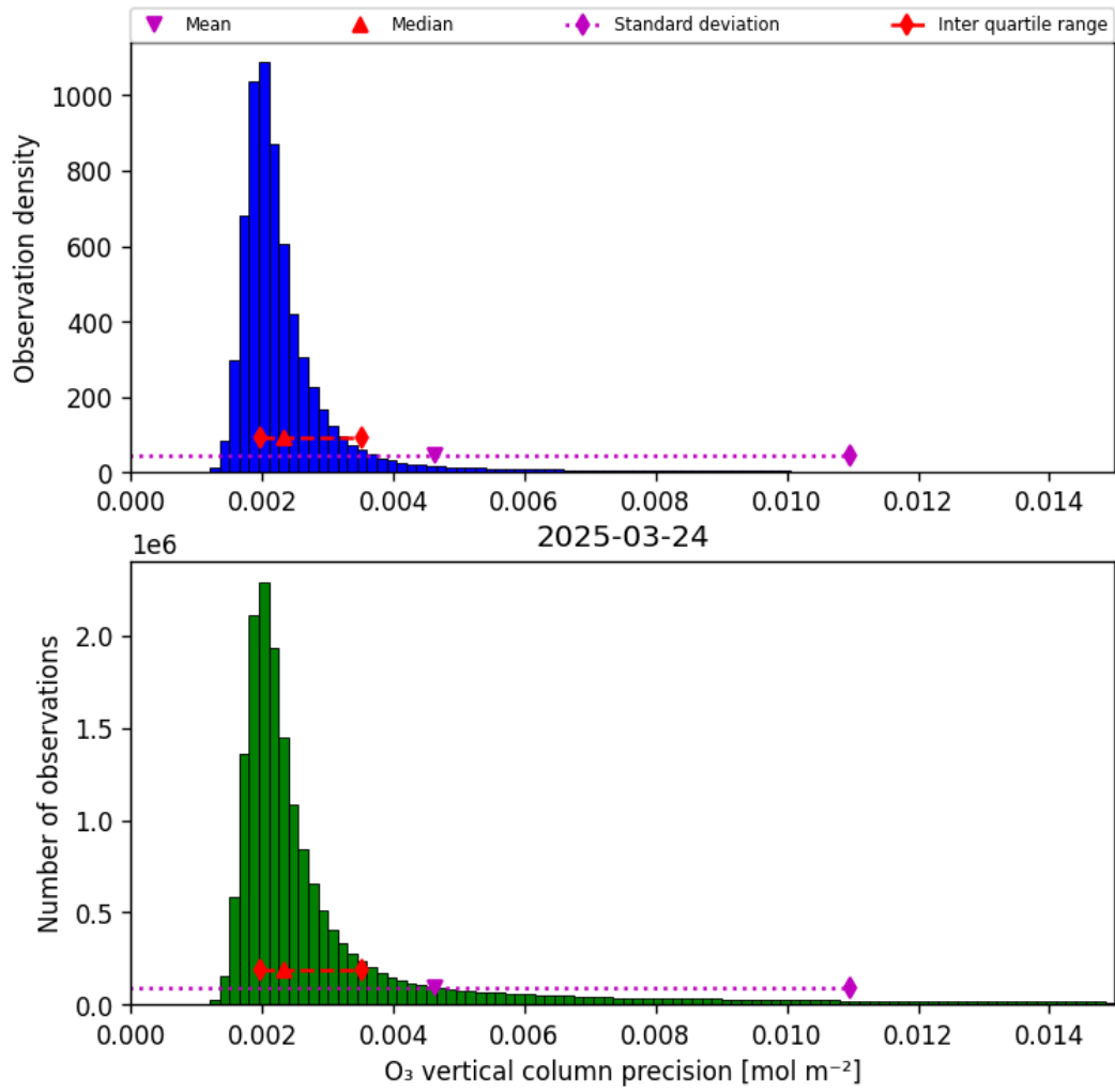
Figure 30: Histogram of “O 3 vertical column precision” for 2025-03-24 to 2025-03-25
