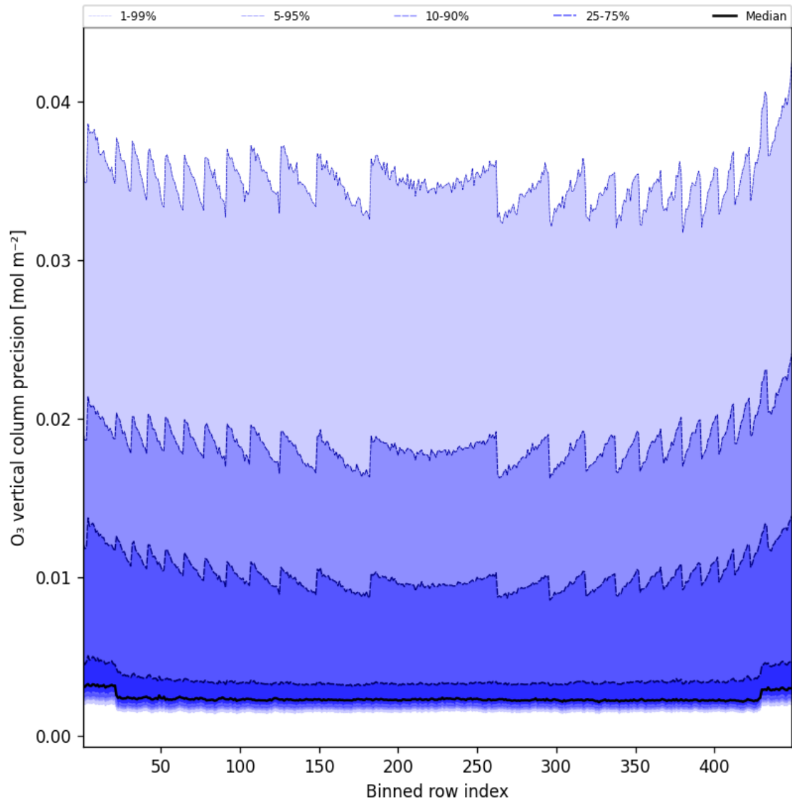
Figure 42: Along track statistics of “O 3 vertical column precision” for 2025-03-24 to 2025-03-25
