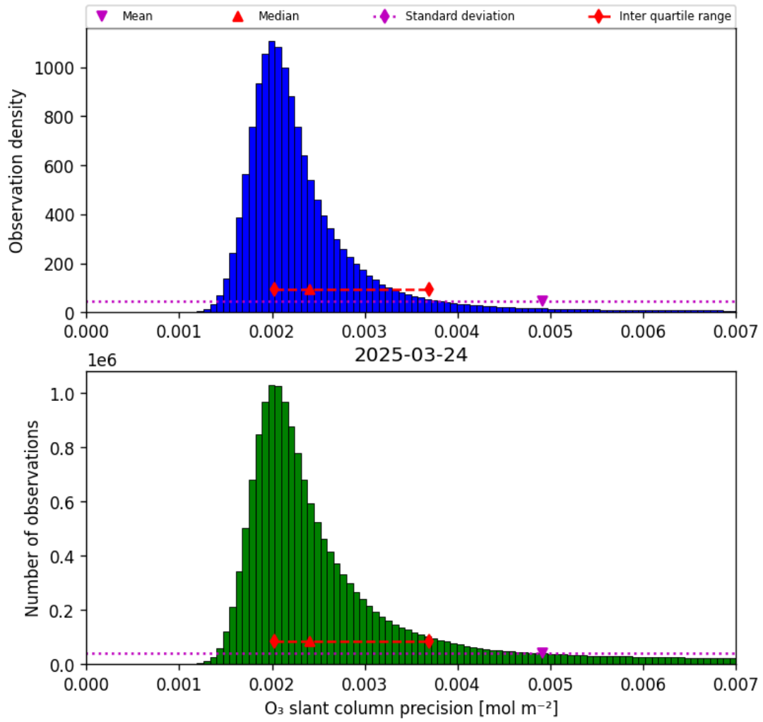
Figure 32: Histogram of “O 3 slant column precision” for 2025-03-24 to 2025-03-25
