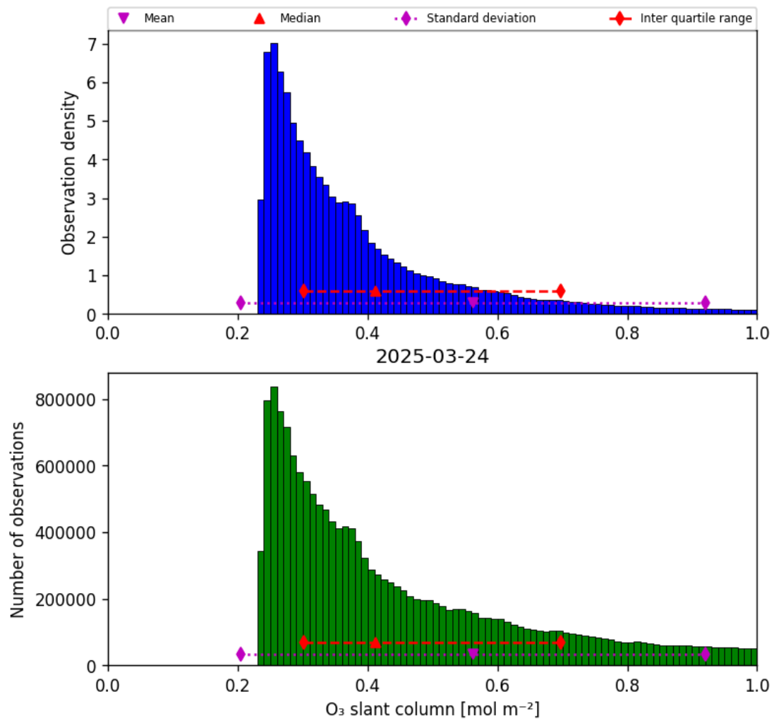
Figure 31: Histogram of “O 3 slant column” for 2025-03-24 to 2025-03-25
