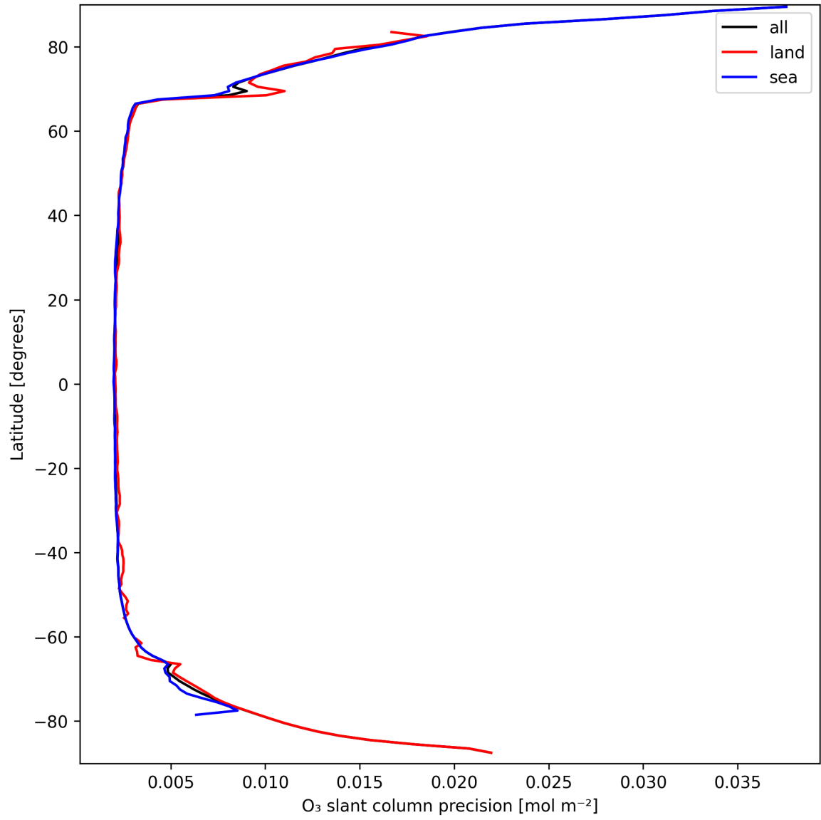
Figure 20: Zonal average of “O 3 slant column precision” for 2025-03-24 to 2025-03-25.
