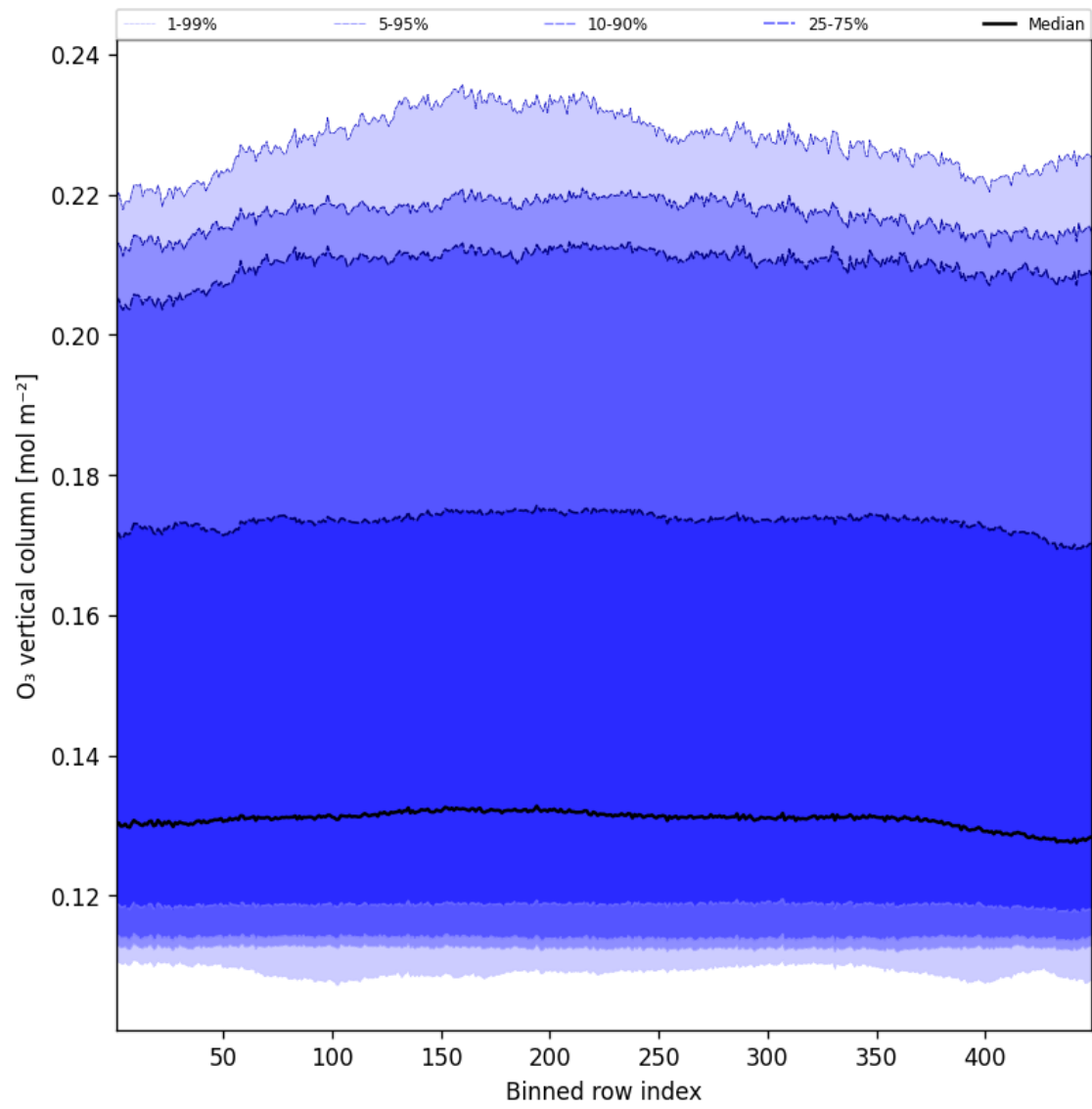
Figure 41: Along track statistics of “O 3 vertical column” for 2025-03-24 to 2025-03-25
