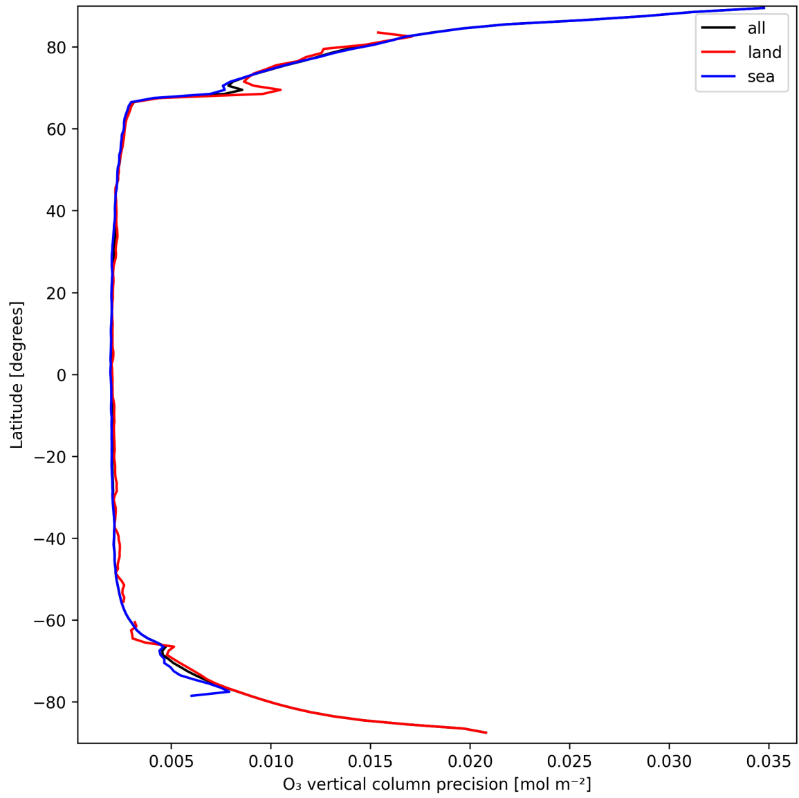
Figure 18: Zonal average of “O 3 vertical column precision” for 2025-03-24 to 2025-03-25.
