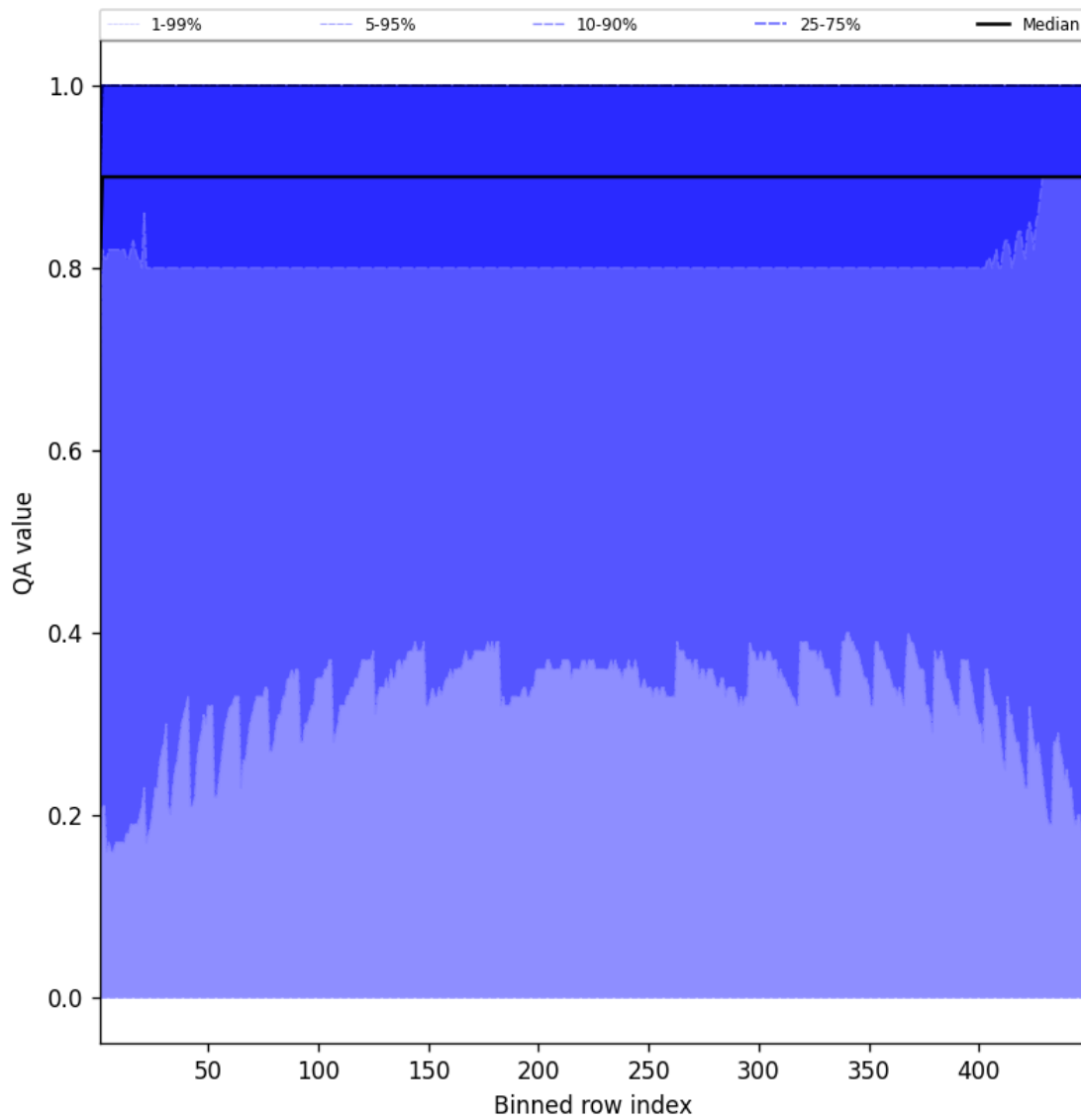
Figure 40: Along track statistics of “QA value” for 2025-03-24 to 2025-03-25
