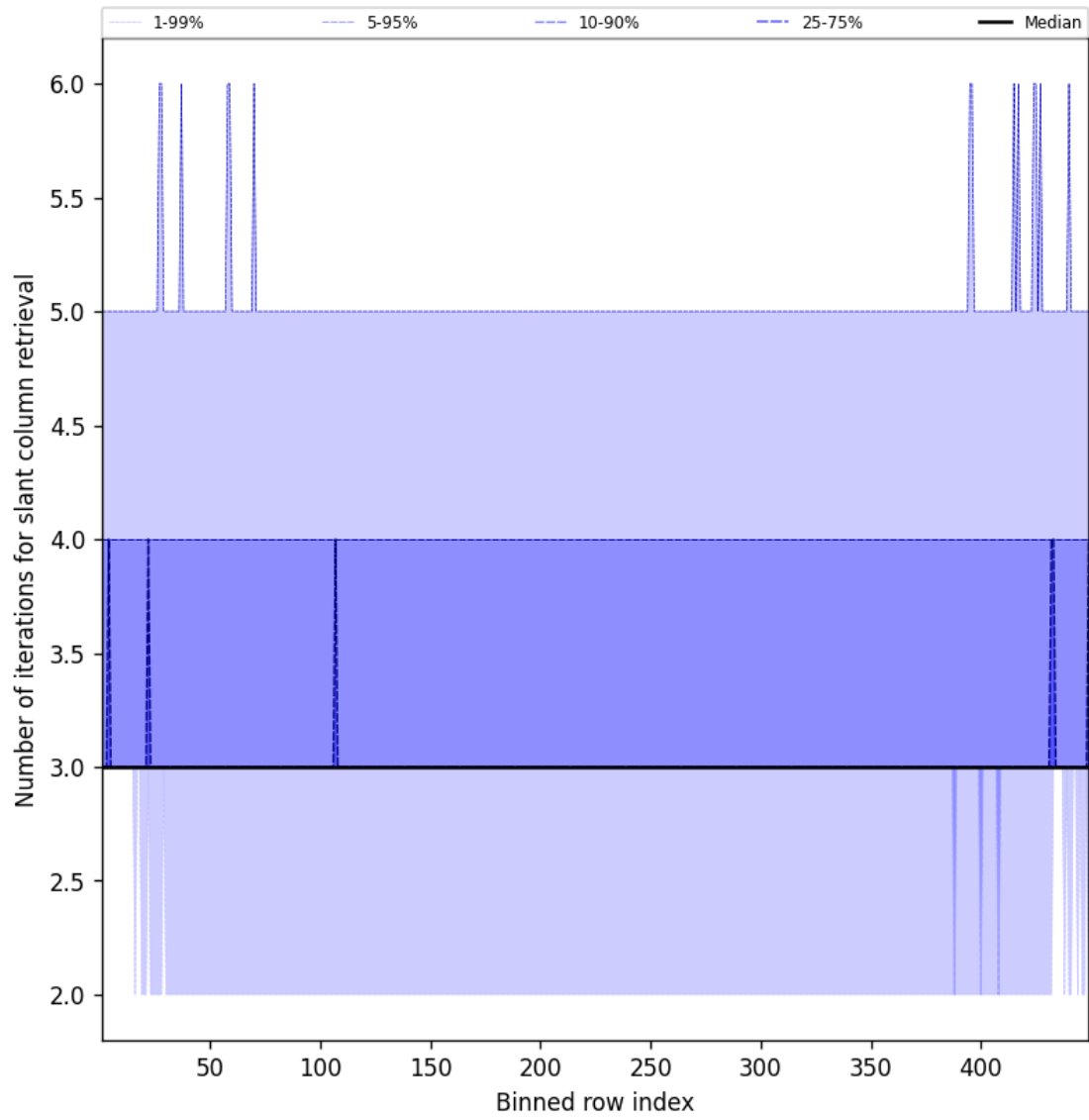
Figure 45: Along track statistics of “Number of iterations for slant column retrieval” for 2025-03-24 to 2025-03-25
