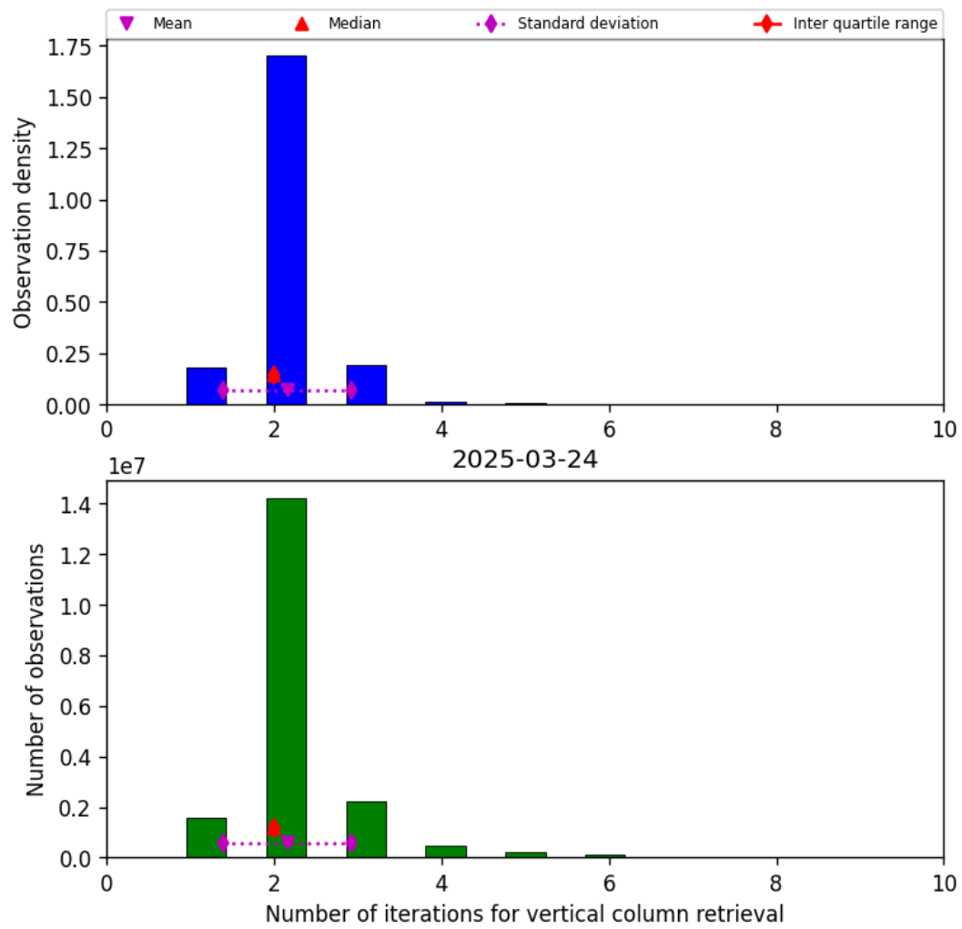
Figure 39: Histogram of “Number of iterations for vertical column retrieval” for 2025-03-24 to 2025-03-25
