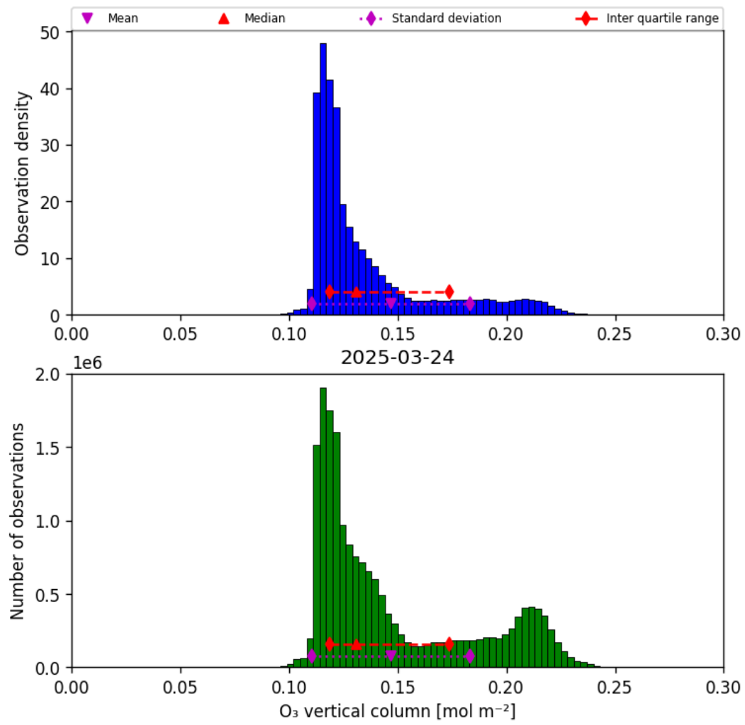
Figure 29: Histogram of “O 3 vertical column” for 2025-03-24 to 2025-03-25
