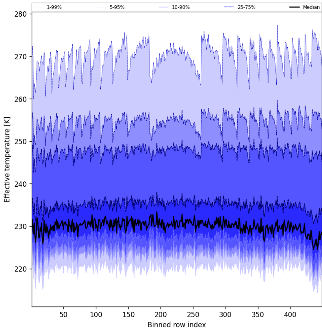
Figure 50: Along track statistics of “Effective temperature” for 2025-03-24 to 2025-03-25
