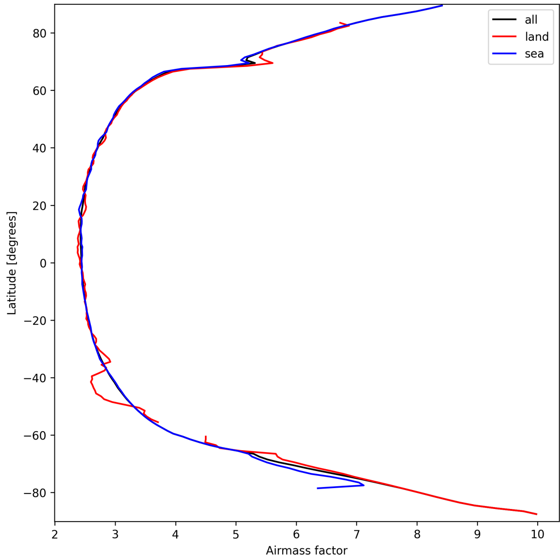
Figure 25: Zonal average of “Airmass factor” for 2025-03-24 to 2025-03-25.
