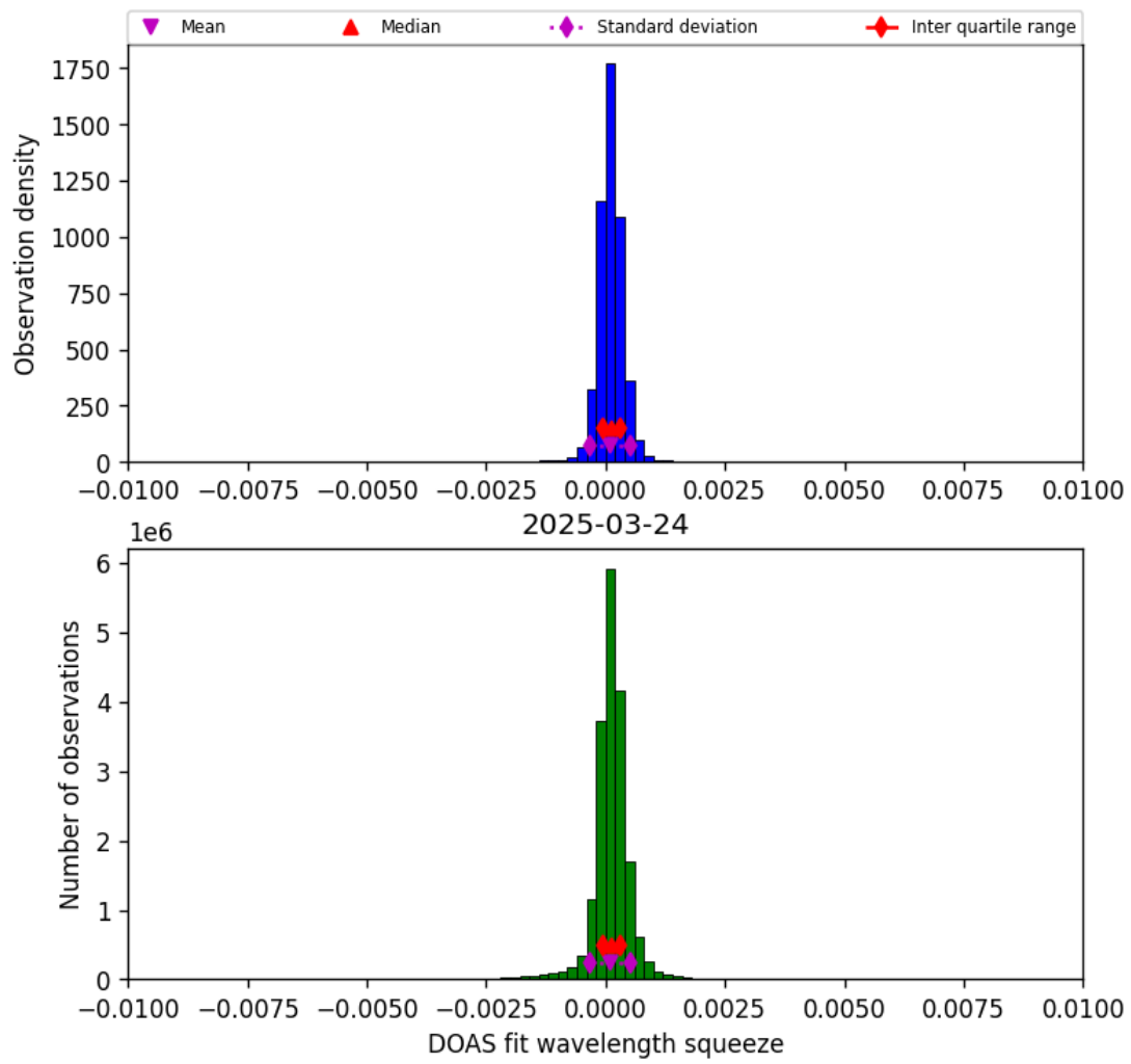
Figure 36: Histogram of “DOAS fit wavelength squeeze” for 2025-03-24 to 2025-03-25
