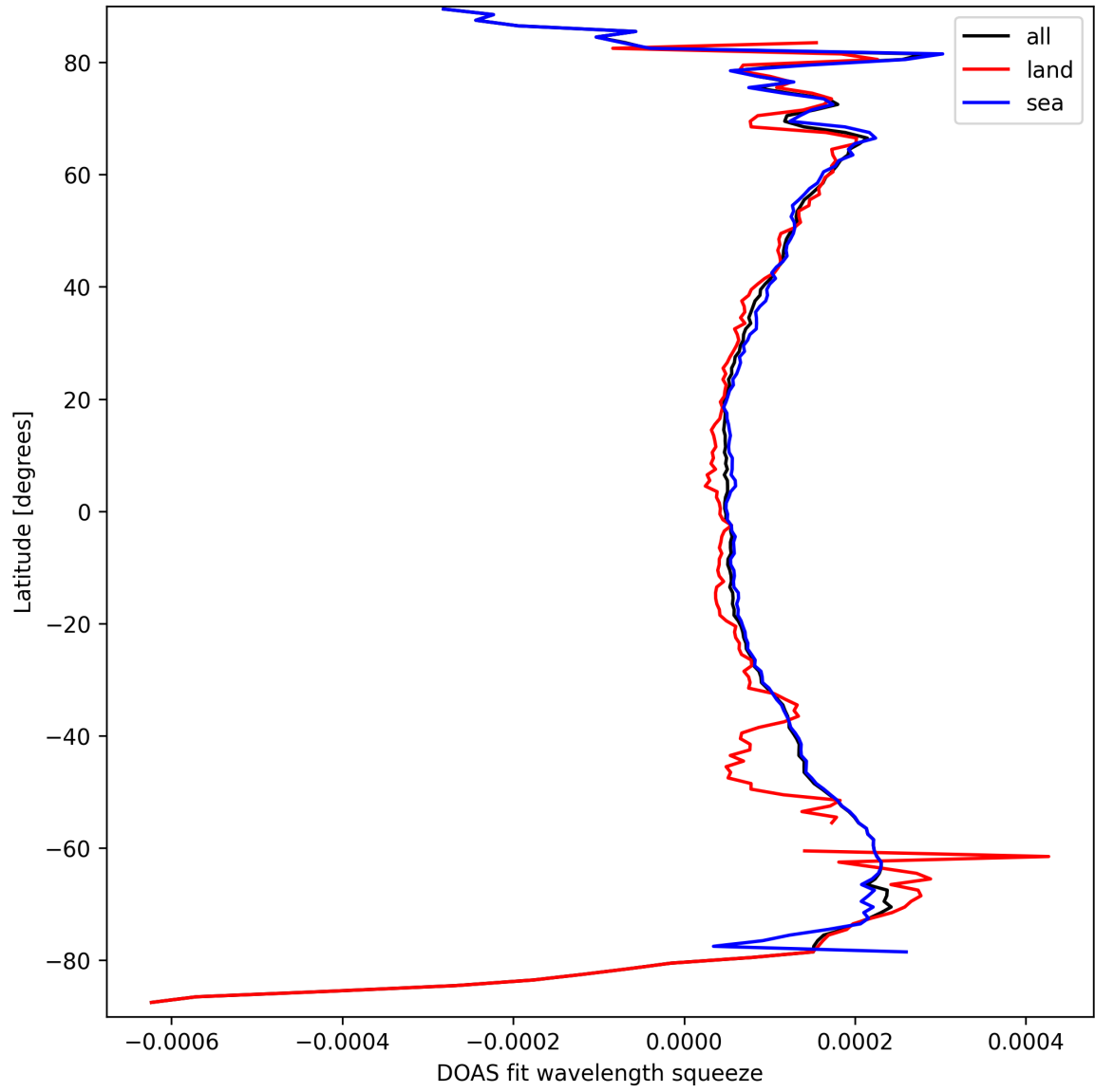
Figure 24: Zonal average of “DOAS fit wavelength squeeze” for 2025-03-24 to 2025-03-25.
