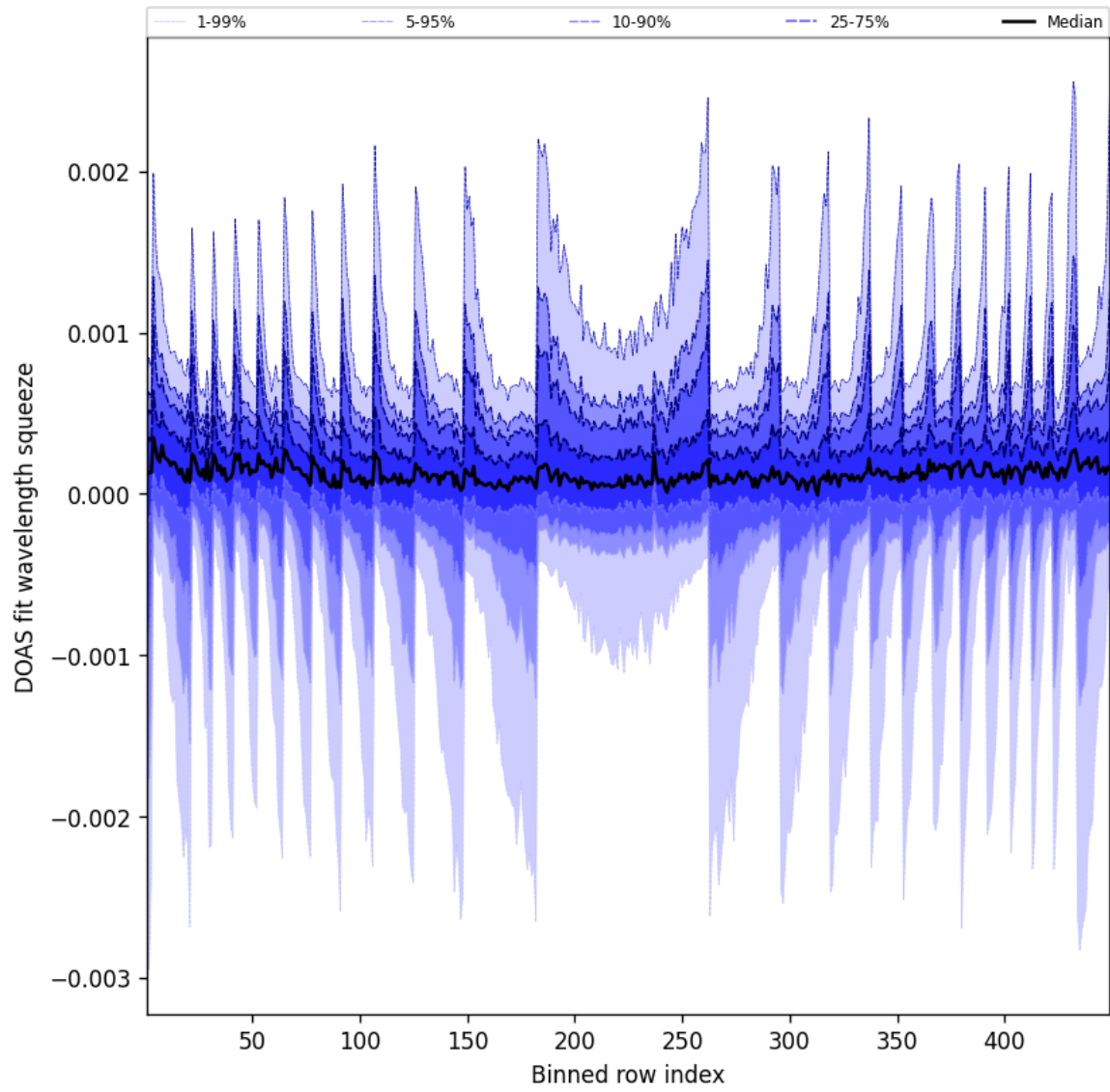
Figure 48: Along track statistics of “DOAS fit wavelength squeeze” for 2025-03-24 to 2025-03-25
