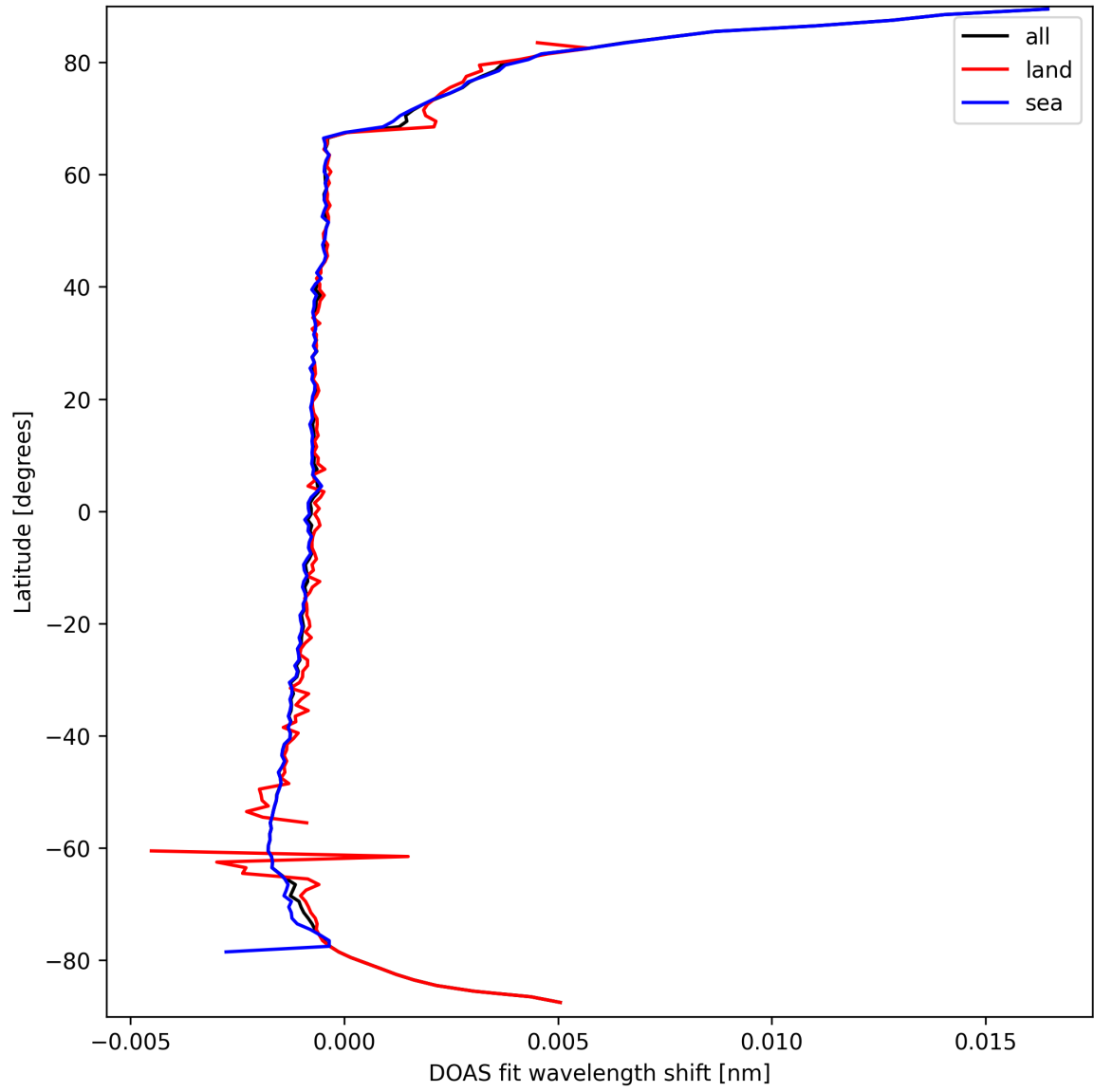
Figure 23: Zonal average of “DOAS fit wavelength shift” for 2025-03-24 to 2025-03-25.
