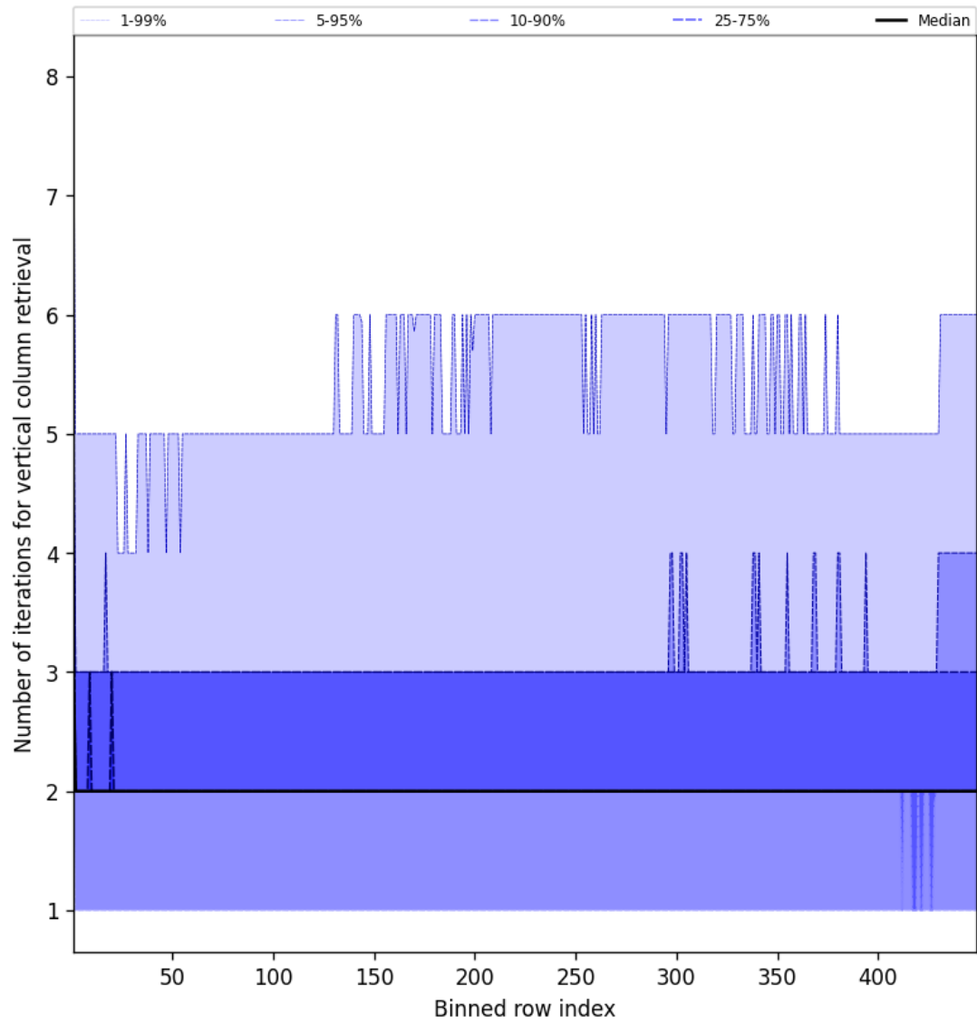
Figure 51: Along track statistics of “Number of iterations for vertical column retrieval” for 2025-03-24 to 2025-03-25
