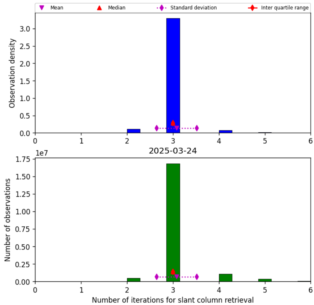
Figure 33: Histogram of “Number of iterations for slant column retrieval” for 2025-03-24 to 2025-03-25
