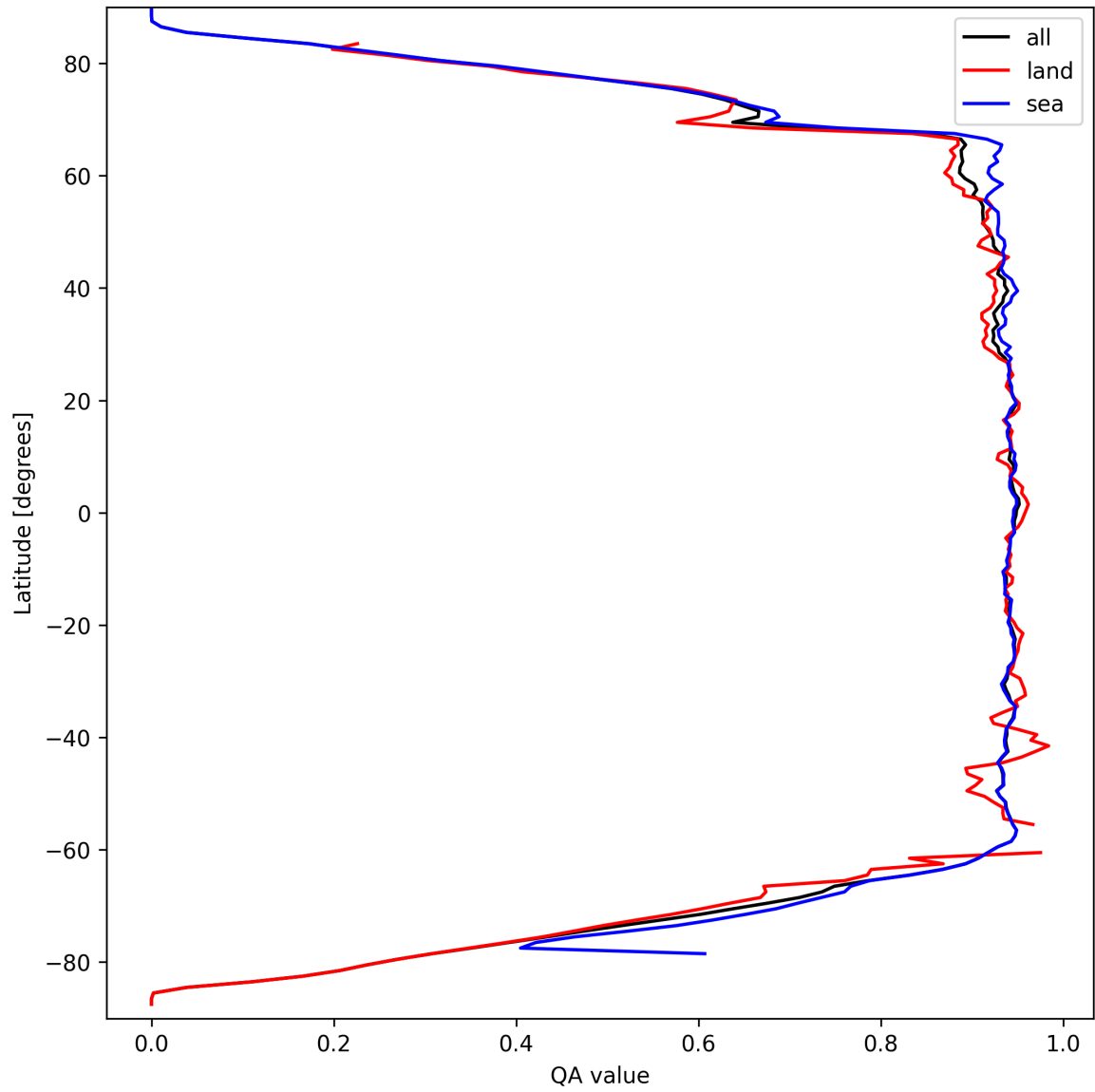
Figure 16: Zonal average of “QA value” for 2025-03-24 to 2025-03-25.
