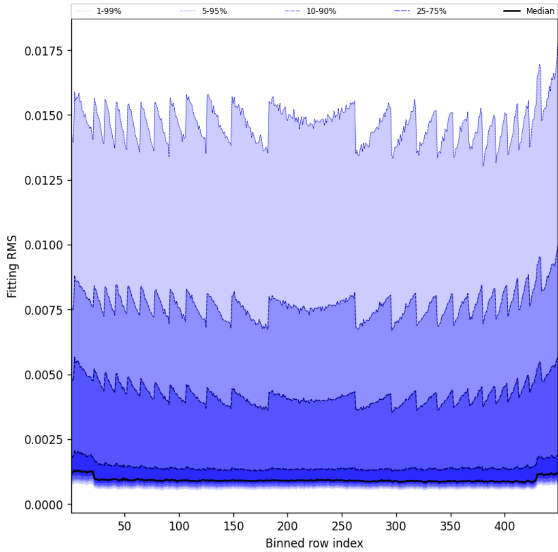
Figure 46: Along track statistics of “Fitting RMS” for 2025-03-24 to 2025-03-25
