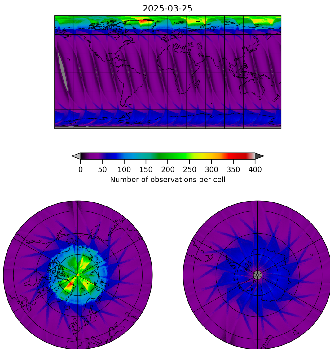
Figure 15: Map of the number of observations for 2025-03-25 to 2025-03-26
