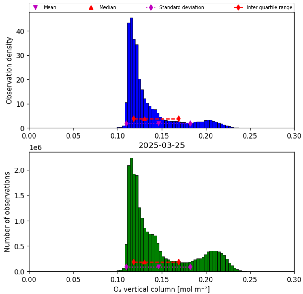
Figure 29: Histogram of “O 3 vertical column” for 2025-03-25 to 2025-03-26
