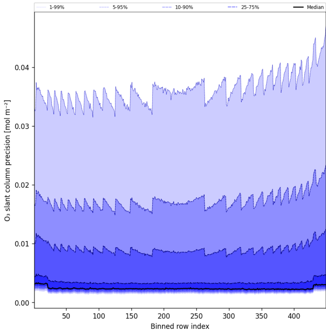
Figure 44: Along track statistics of “O 3 slant column precision” for 2025-03-25 to 2025-03-26
