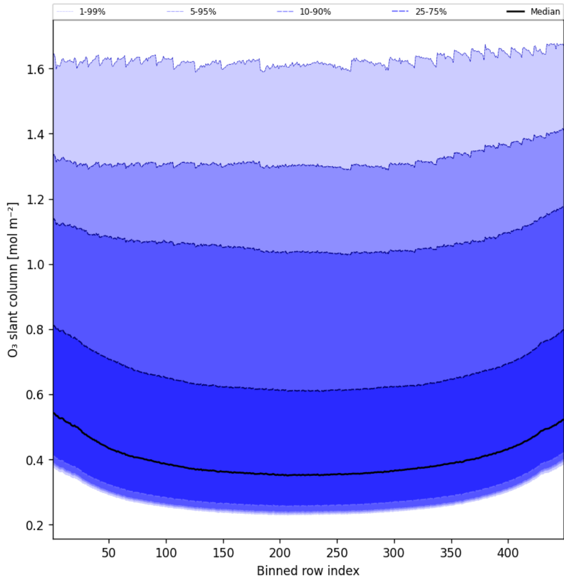
Figure 43: Along track statistics of “O 3 slant column” for 2025-03-25 to 2025-03-26
