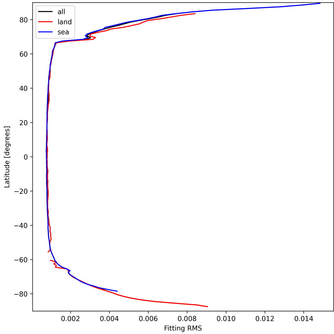
Figure 22: Zonal average of “Fitting RMS” for 2025-03-25 to 2025-03-26.
