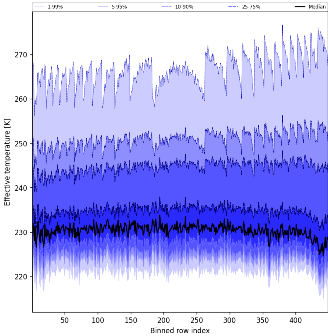
Figure 50: Along track statistics of “Effective temperature” for 2025-03-25 to 2025-03-26
