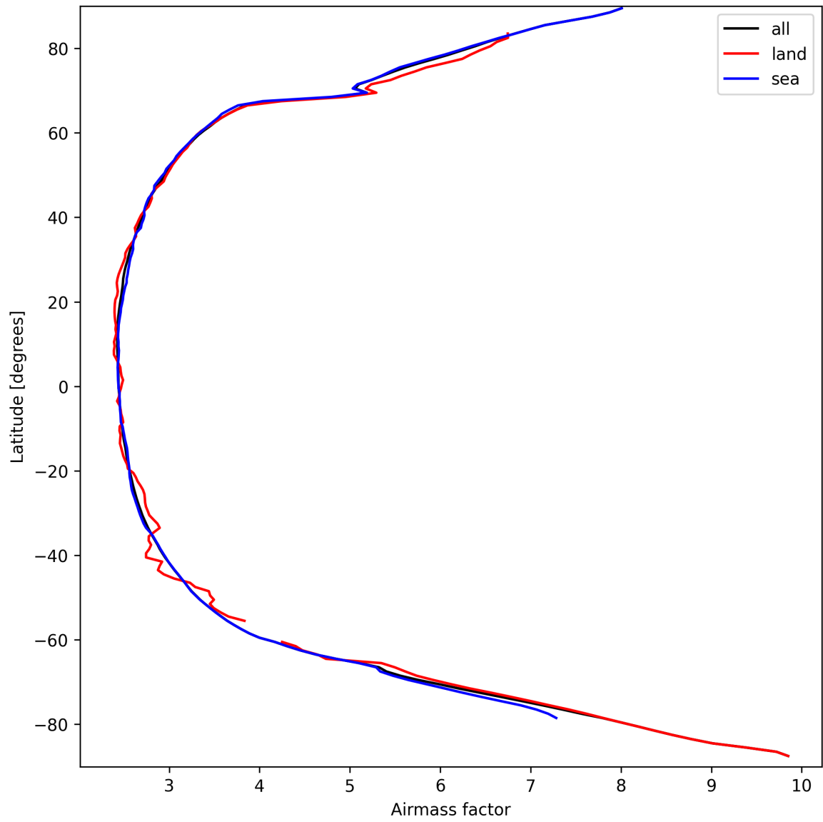
Figure 25: Zonal average of “Airmass factor” for 2025-03-25 to 2025-03-26.
