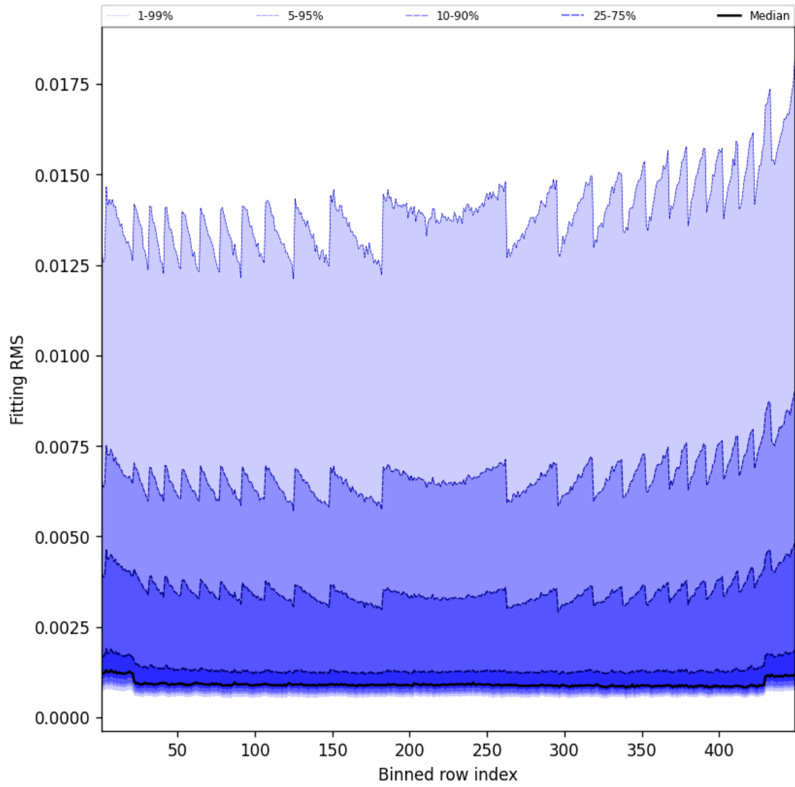
Figure 46: Along track statistics of “Fitting RMS” for 2025-03-25 to 2025-03-26
