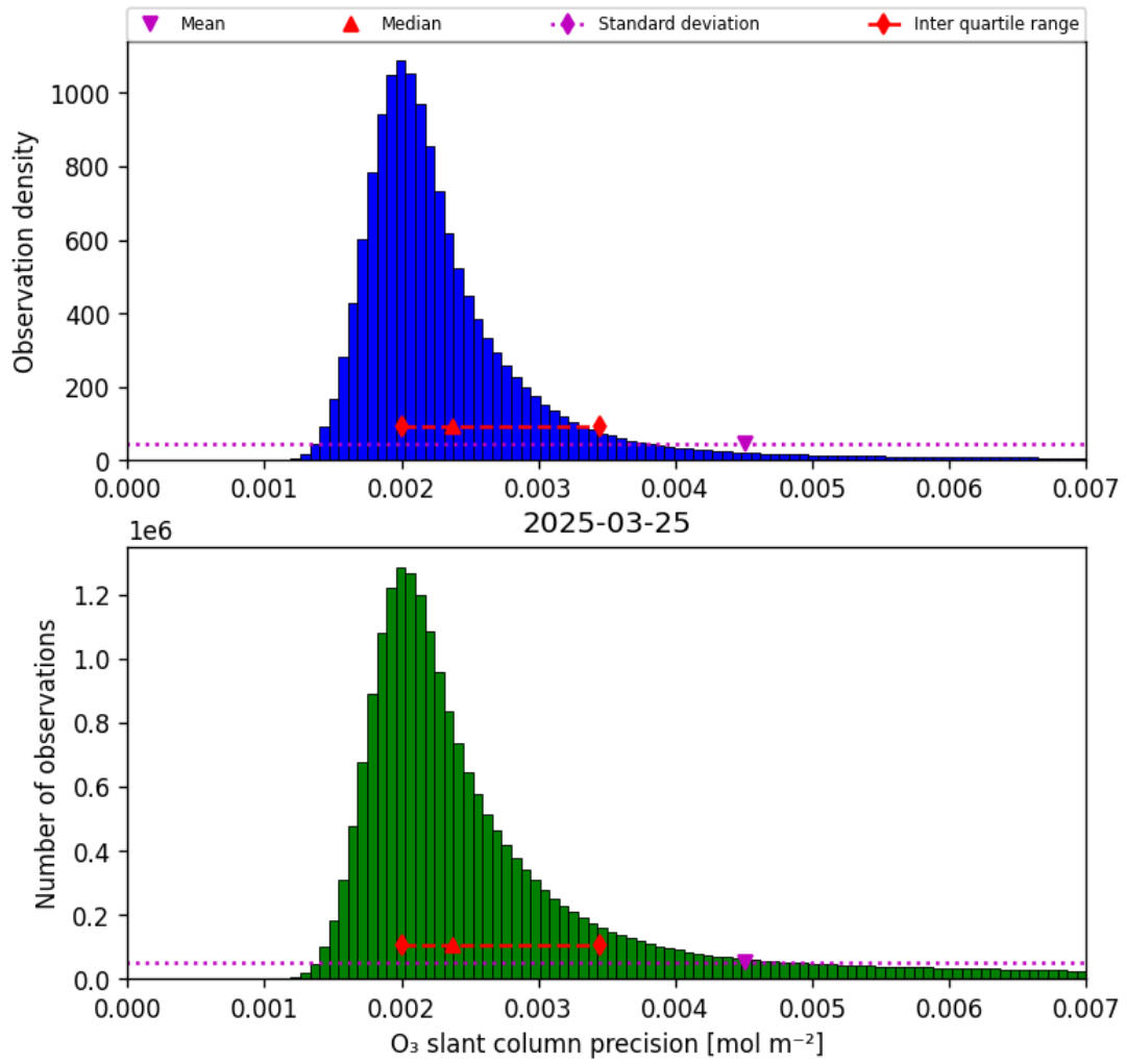
Figure 32: Histogram of “O 3 slant column precision” for 2025-03-25 to 2025-03-26
