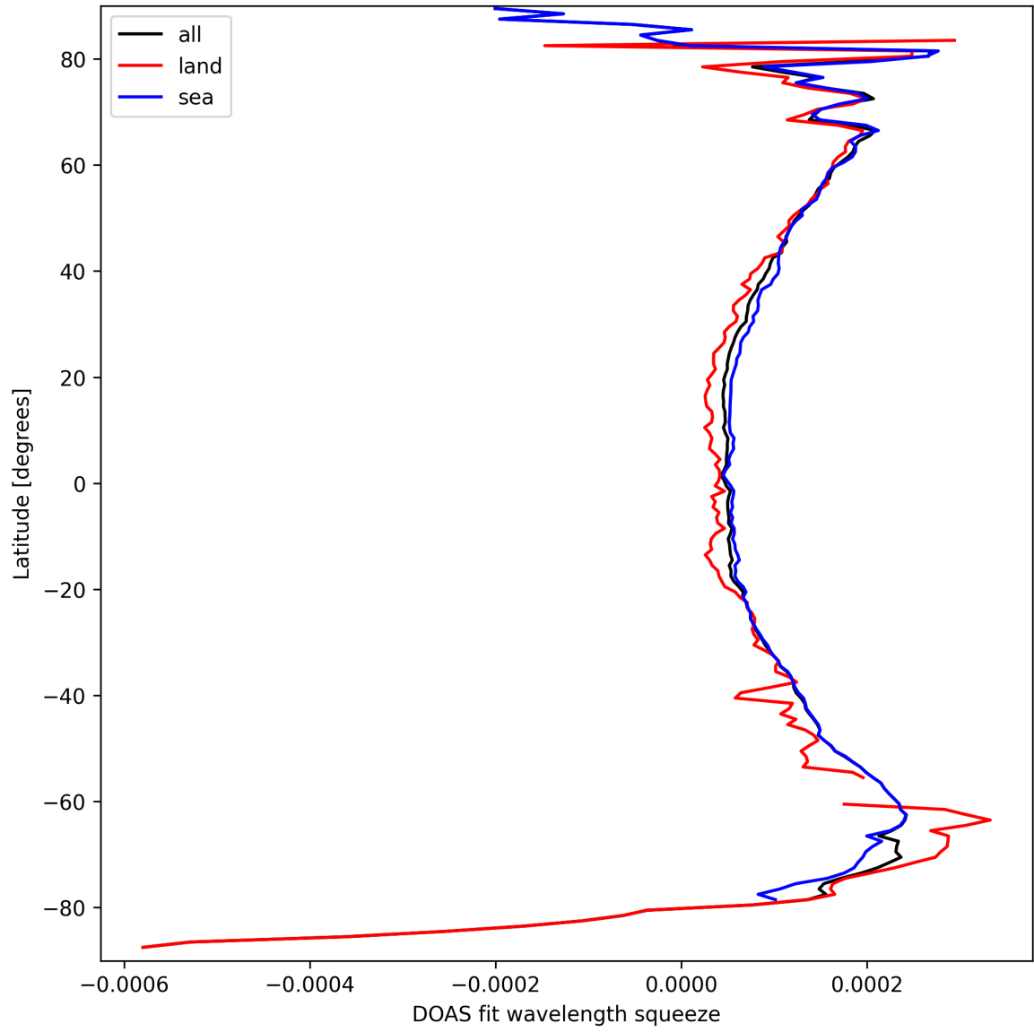
Figure 24: Zonal average of “DOAS fit wavelength squeeze” for 2025-03-25 to 2025-03-26.
