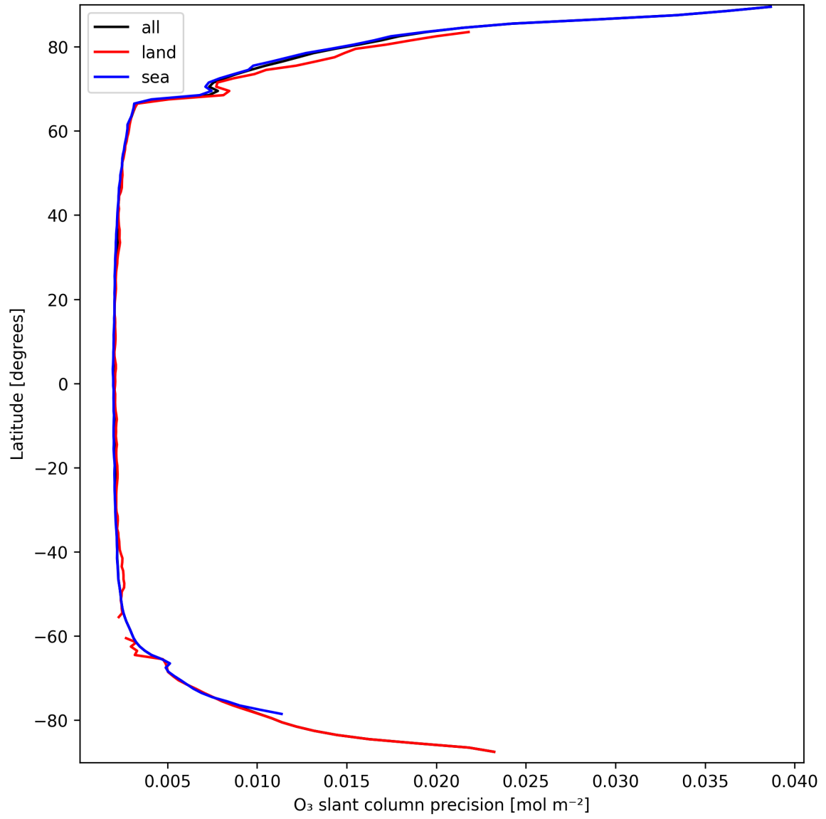
Figure 20: Zonal average of “O 3 slant column precision” for 2025-03-25 to 2025-03-26.
