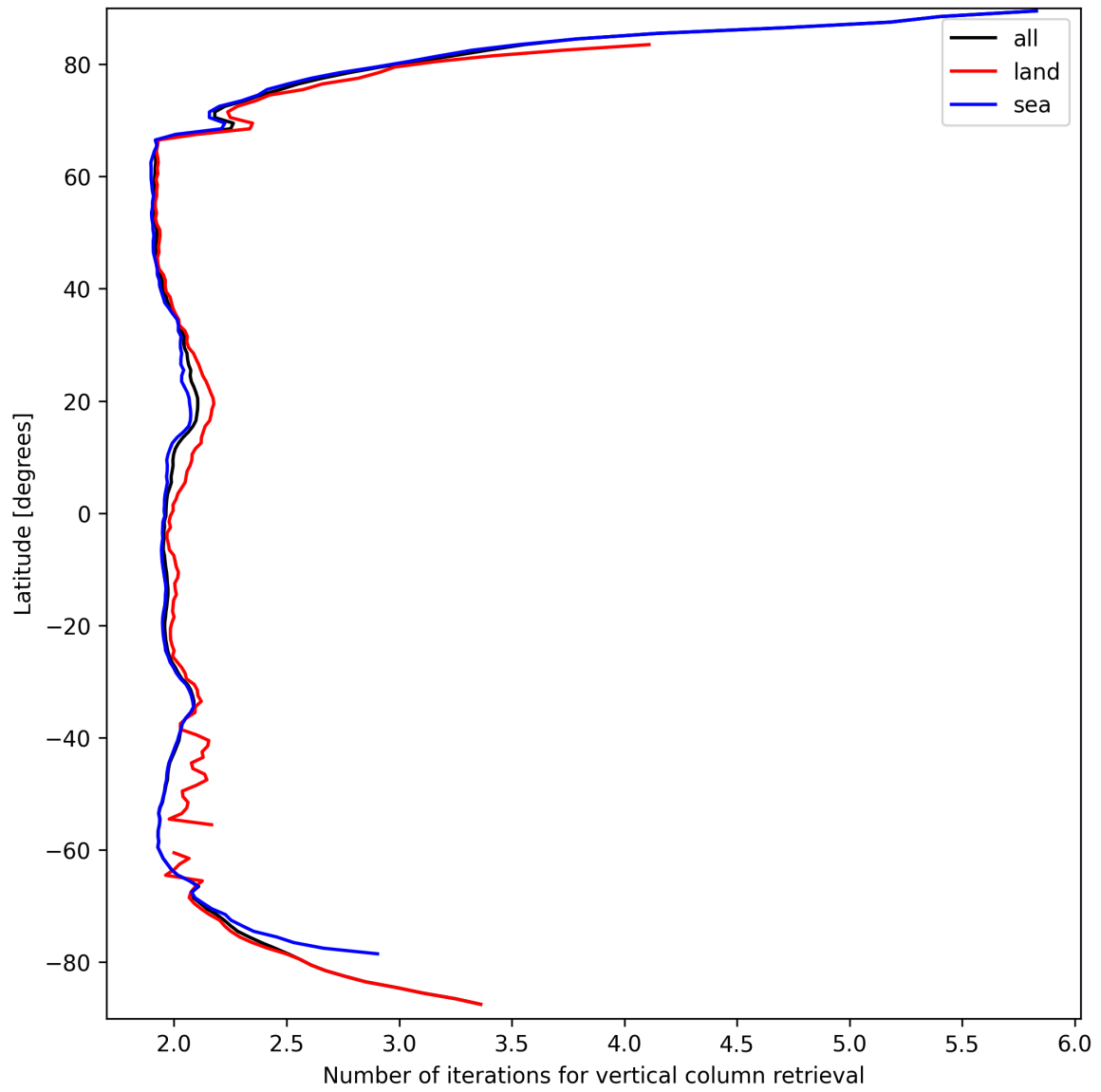
Figure 27: Zonal average of “Number of iterations for vertical column retrieval” for 2025-03-25 to 2025-03-26.
