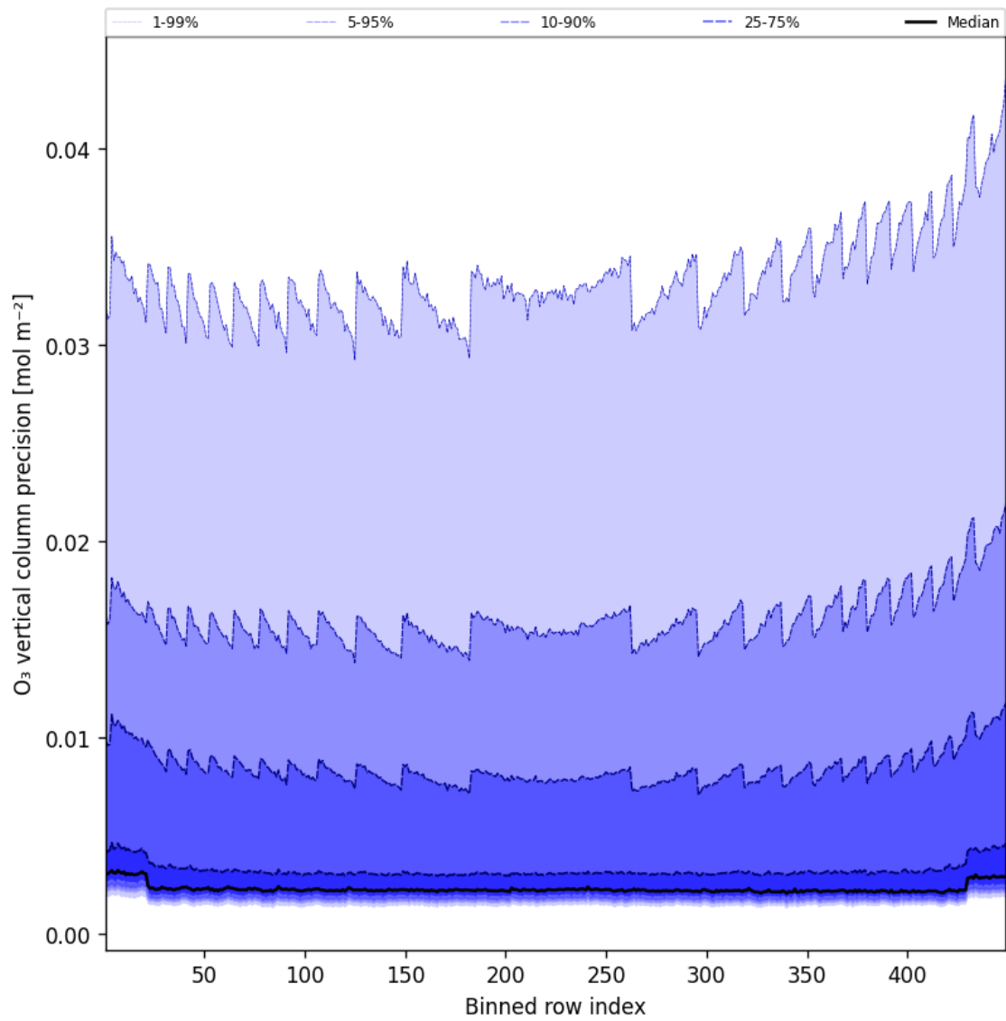
Figure 42: Along track statistics of “O 3 vertical column precision” for 2025-03-25 to 2025-03-26
