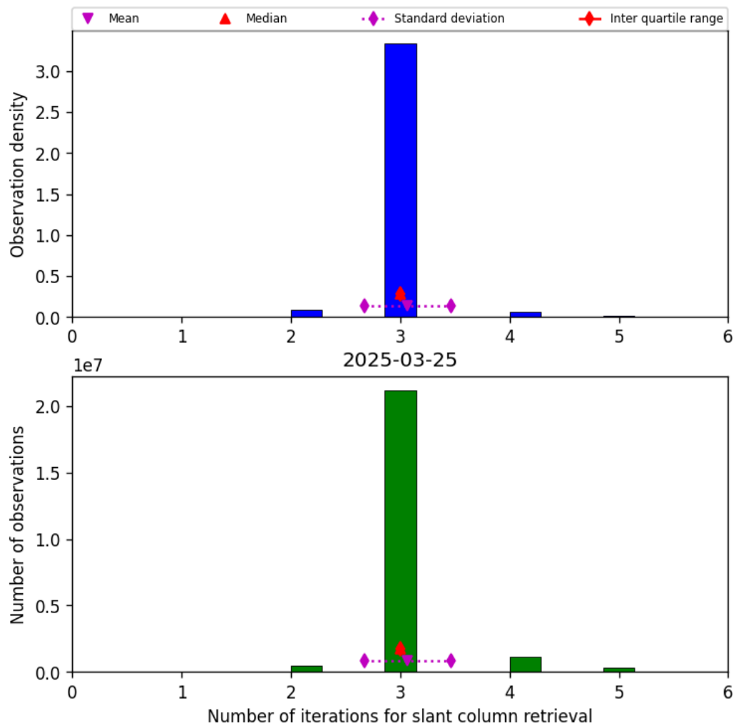
Figure 33: Histogram of “Number of iterations for slant column retrieval” for 2025-03-25 to 2025-03-26
