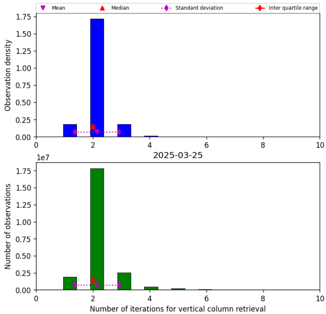
Figure 39: Histogram of “Number of iterations for vertical column retrieval” for 2025-03-25 to 2025-03-26
