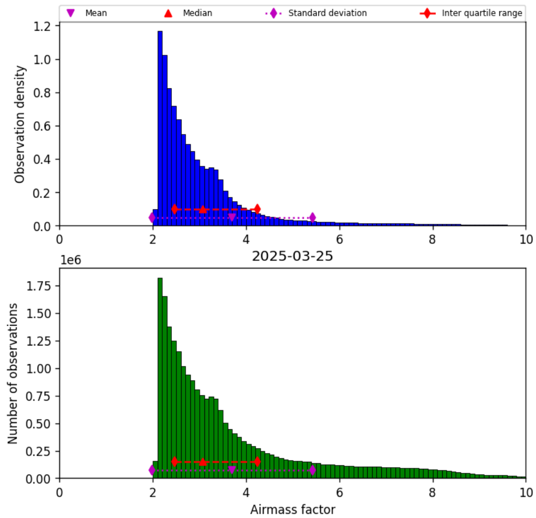
Figure 37: Histogram of “Airmass factor” for 2025-03-25 to 2025-03-26
