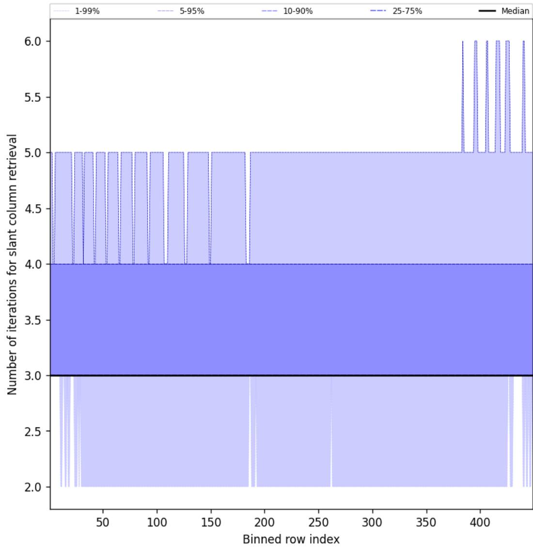
Figure 45: Along track statistics of “Number of iterations for slant column retrieval” for 2025-03-25 to 2025-03-26
