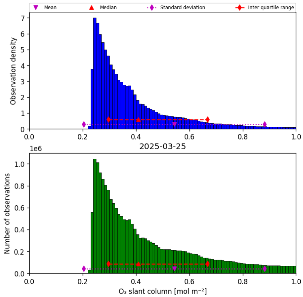
Figure 31: Histogram of “O 3 slant column” for 2025-03-25 to 2025-03-26
