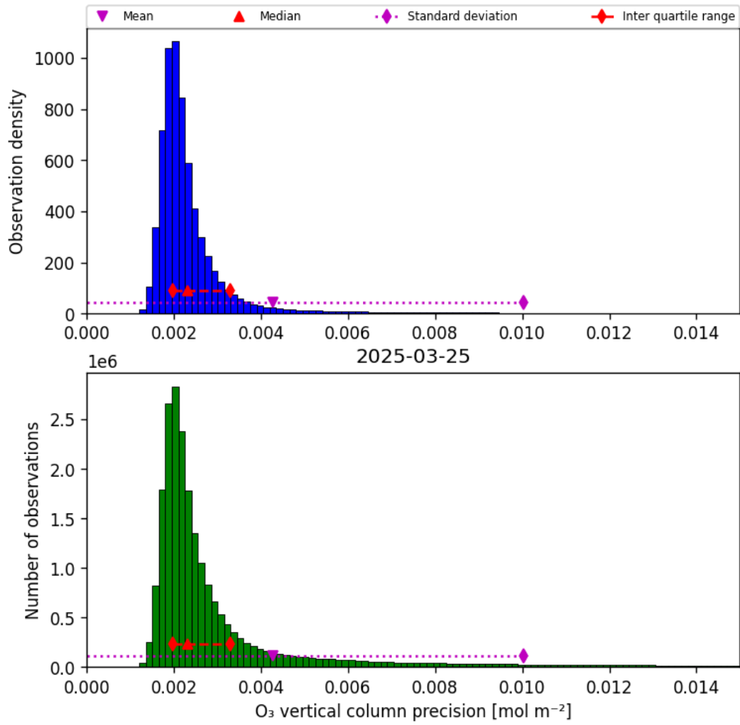
Figure 30: Histogram of “O 3 vertical column precision” for 2025-03-25 to 2025-03-26
