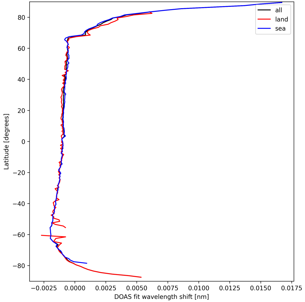
Figure 23: Zonal average of “DOAS fit wavelength shift” for 2025-03-25 to 2025-03-26.
