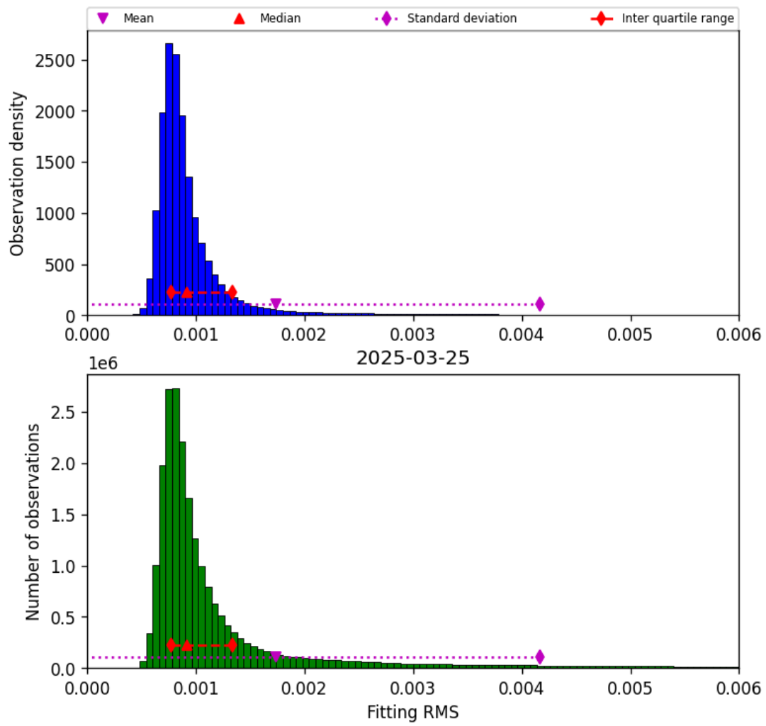
Figure 34: Histogram of “Fitting RMS” for 2025-03-25 to 2025-03-26
