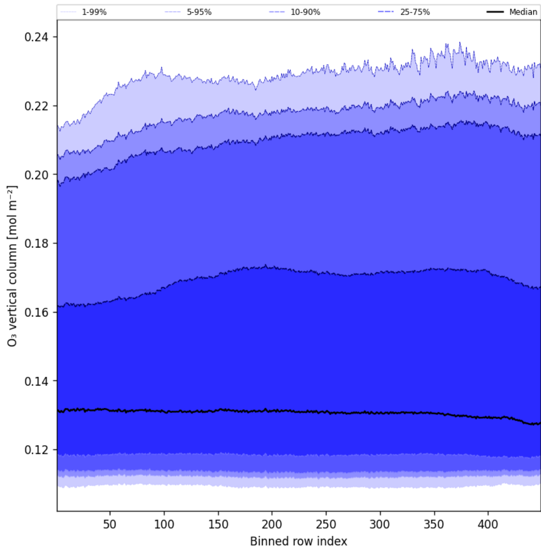
Figure 41: Along track statistics of “O 3 vertical column” for 2025-03-25 to 2025-03-26
