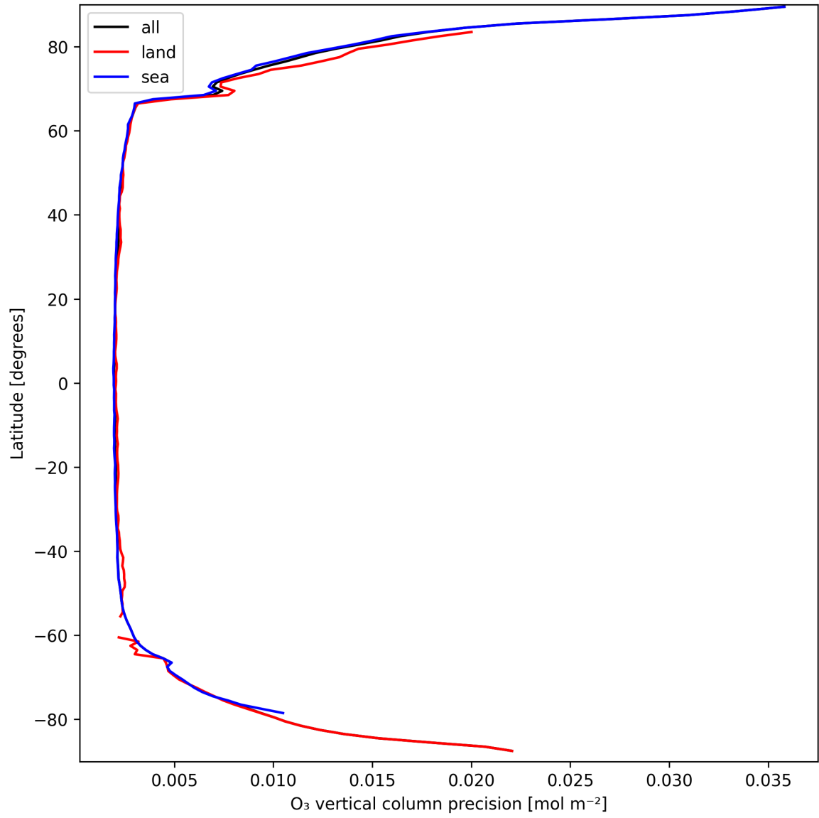
Figure 18: Zonal average of "O 3 vertical column precision" for 2025-03-25 to 2025-03-26.
