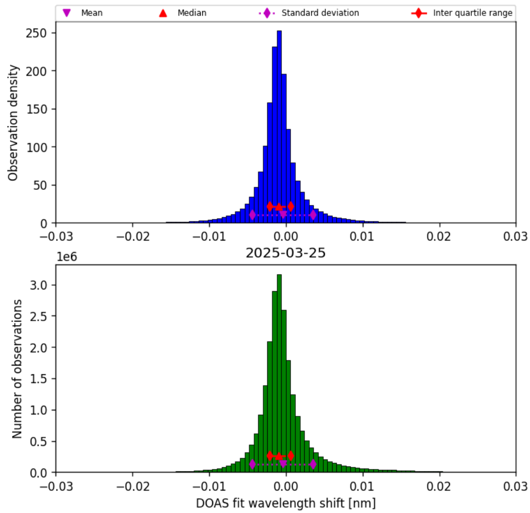
Figure 35: Histogram of “DOAS fit wavelength shift” for 2025-03-25 to 2025-03-26
