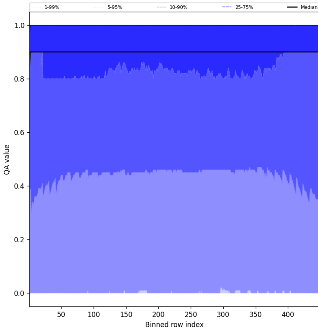
Figure 40: Along track statistics of “QA value” for 2025-03-25 to 2025-03-26
