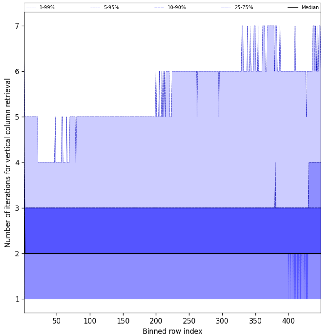
Figure 51: Along track statistics of “Number of iterations for vertical column retrieval” for 2025-03-25 to 2025-03-26
