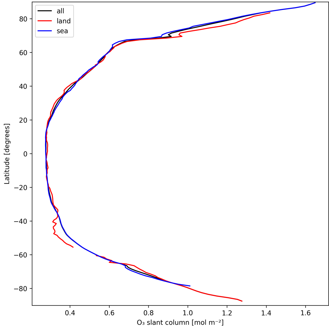
Figure 19: Zonal average of “O 3 slant column” for 2025-03-25 to 2025-03-26.
