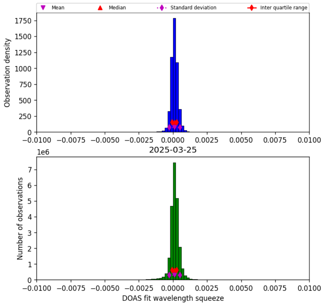
Figure 36: Histogram of “DOAS fit wavelength squeeze” for 2025-03-25 to 2025-03-26
