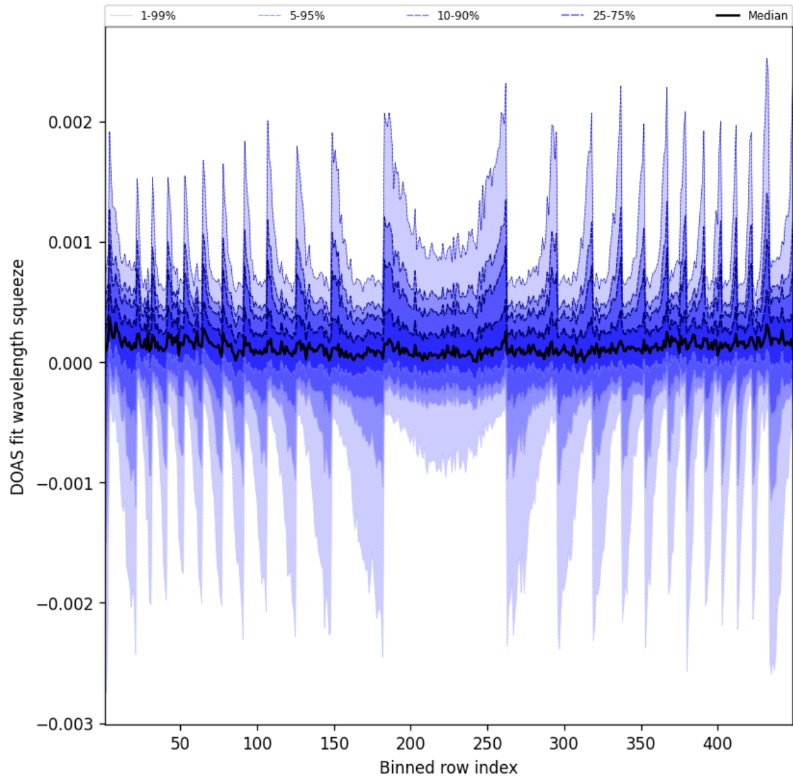
Figure 48: Along track statistics of “DOAS fit wavelength squeeze” for 2025-03-25 to 2025-03-26
