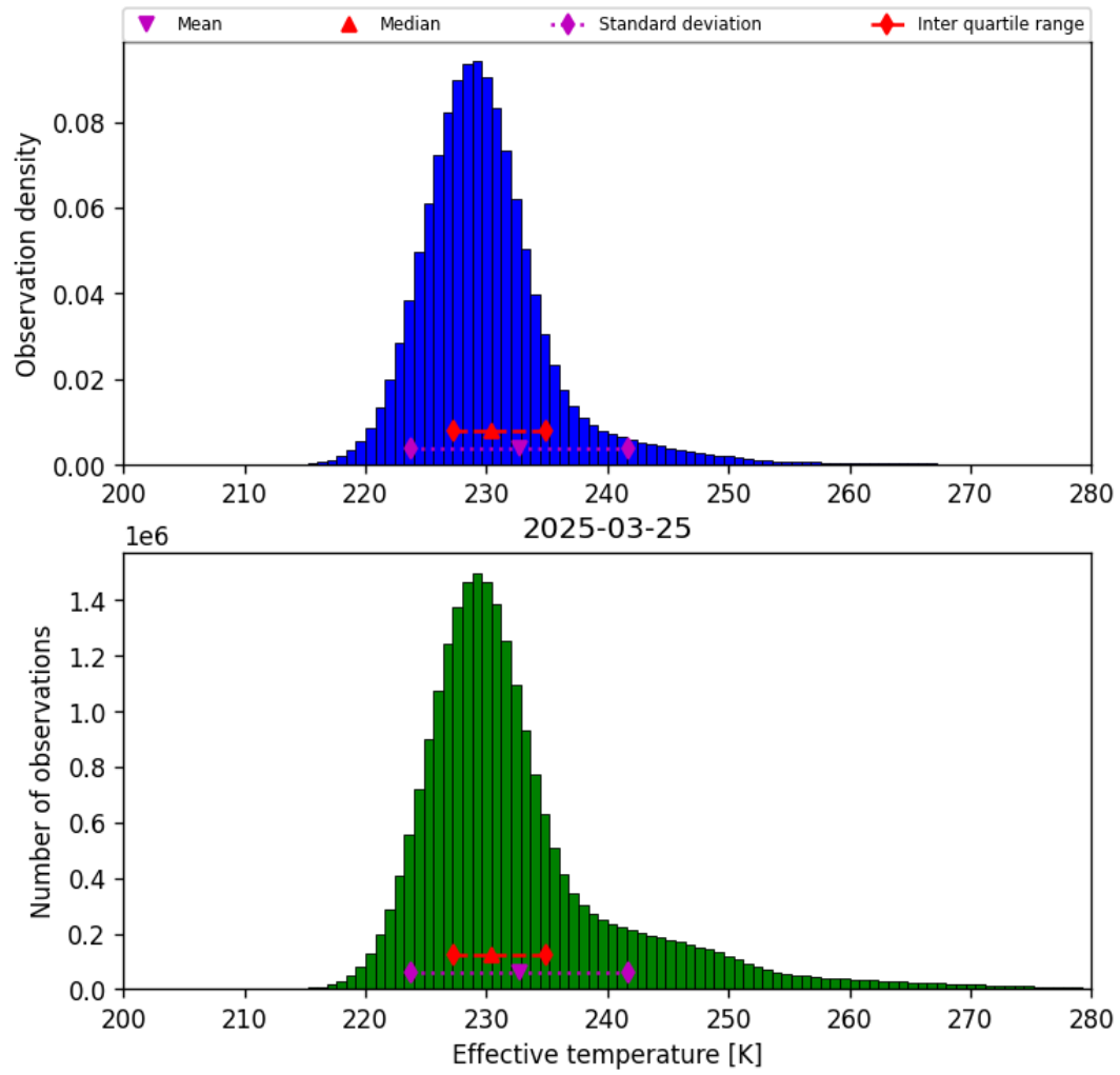
Figure 38: Histogram of “Effective temperature” for 2025-03-25 to 2025-03-26
