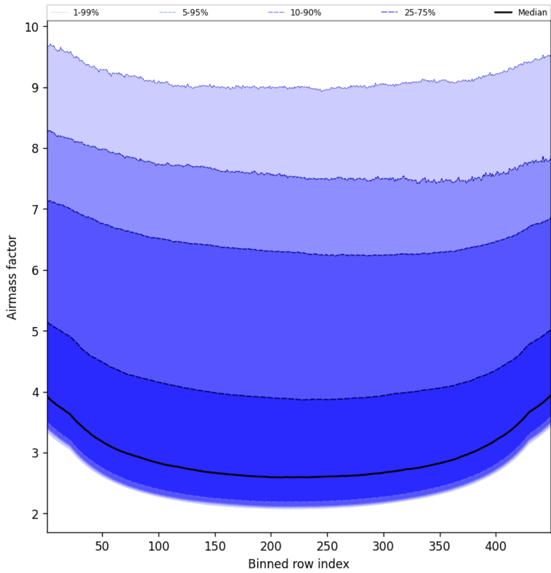
Figure 49: Along track statistics of “Airmass factor” for 2025-03-25 to 2025-03-26
