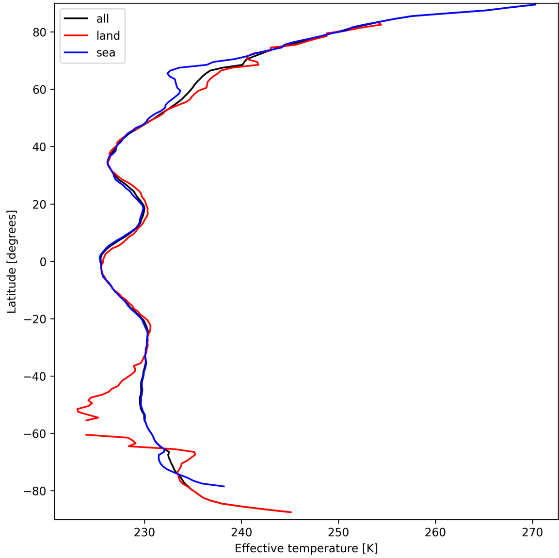
Figure 26: Zonal average of “Effective temperature” for 2025-03-25 to 2025-03-26.
