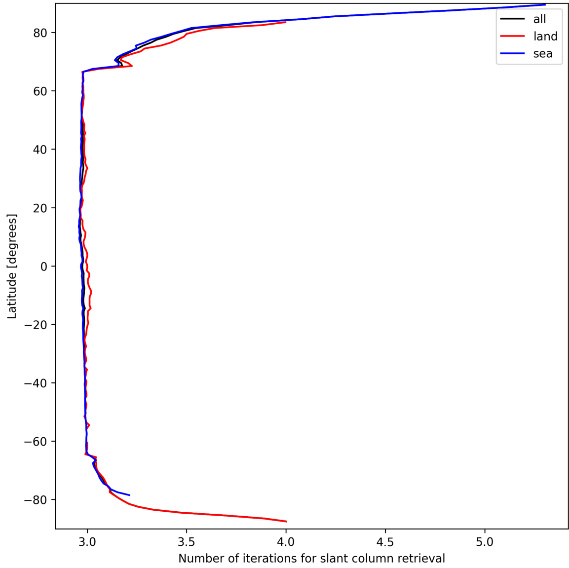
Figure 21: Zonal average of “Number of iterations for slant column retrieval” for 2025-03-25 to 2025-03-26.
