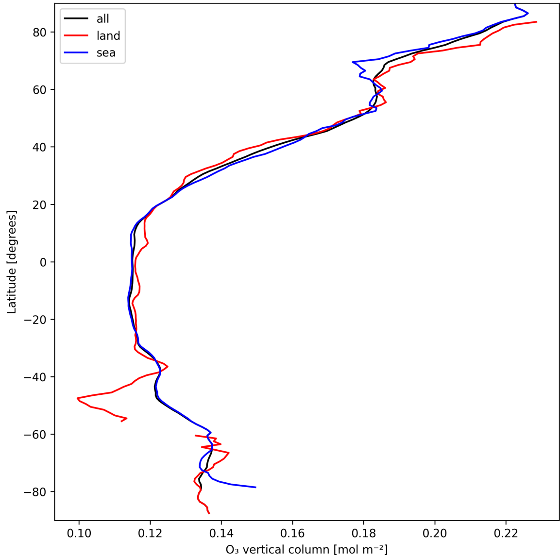
Figure 17: Zonal average of “O 3 vertical column” for 2025-03-25 to 2025-03-26.
