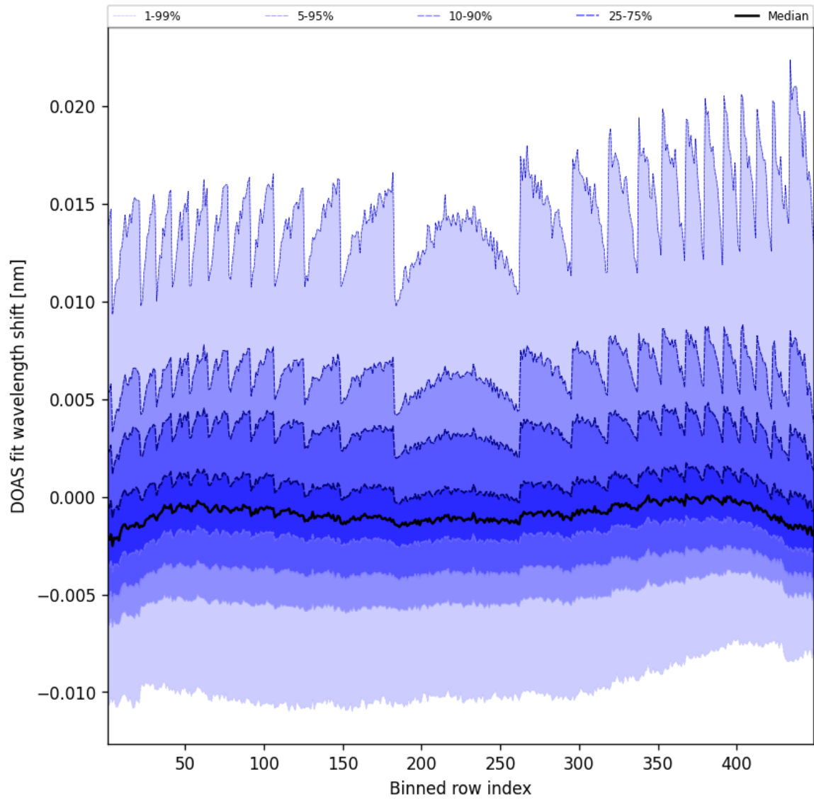
Figure 47: Along track statistics of "DOAS fit wavelength shift" for 2025-03-25 to 2025-03-26
