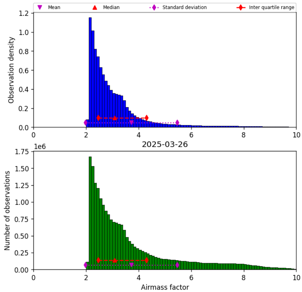
Figure 37: Histogram of “Airmass factor” for 2025-03-26 to 2025-03-26
