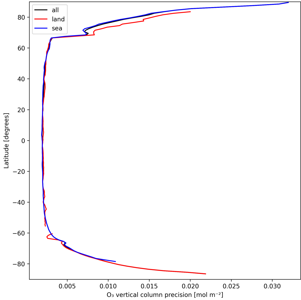
Figure 18: Zonal average of “O 3 vertical column precision” for 2025-03-26 to 2025-03-26.
