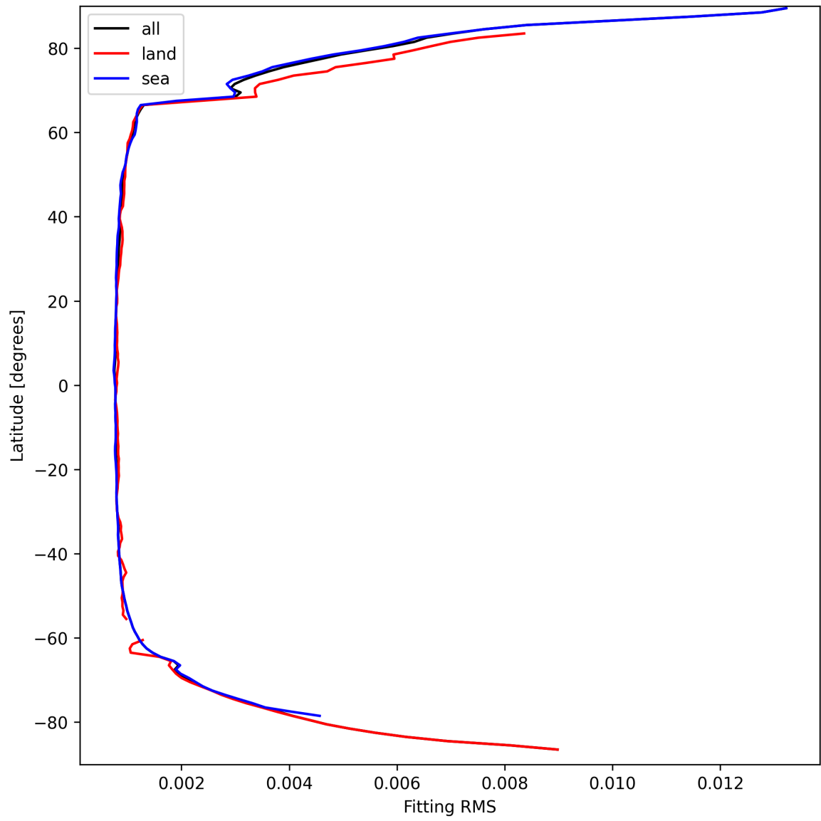
Figure 22: Zonal average of “Fitting RMS” for 2025-03-26 to 2025-03-26.
