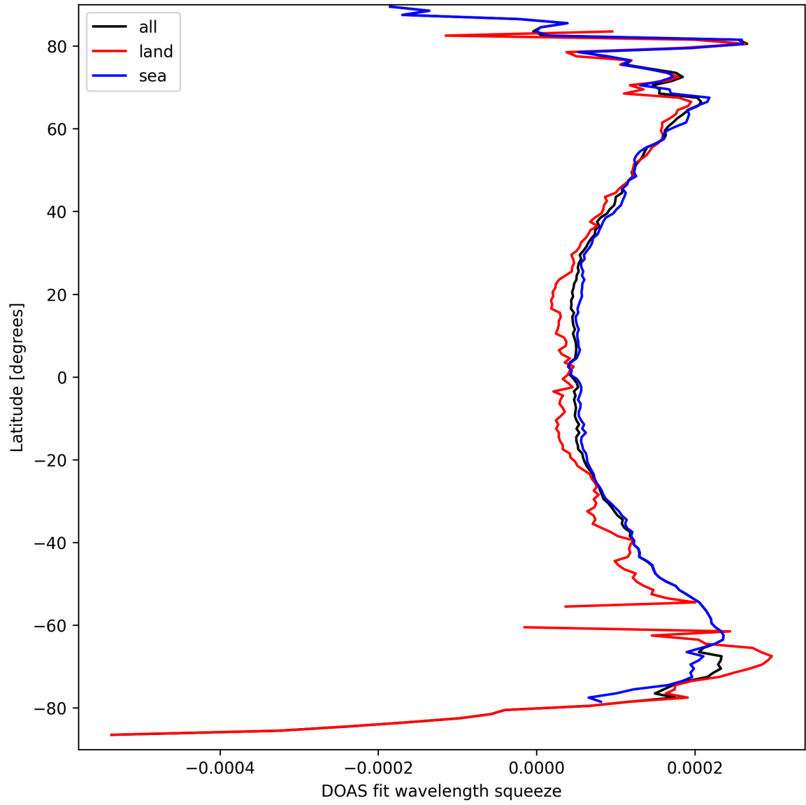
Figure 24: Zonal average of “DOAS fit wavelength squeeze” for 2025-03-26 to 2025-03-26.
