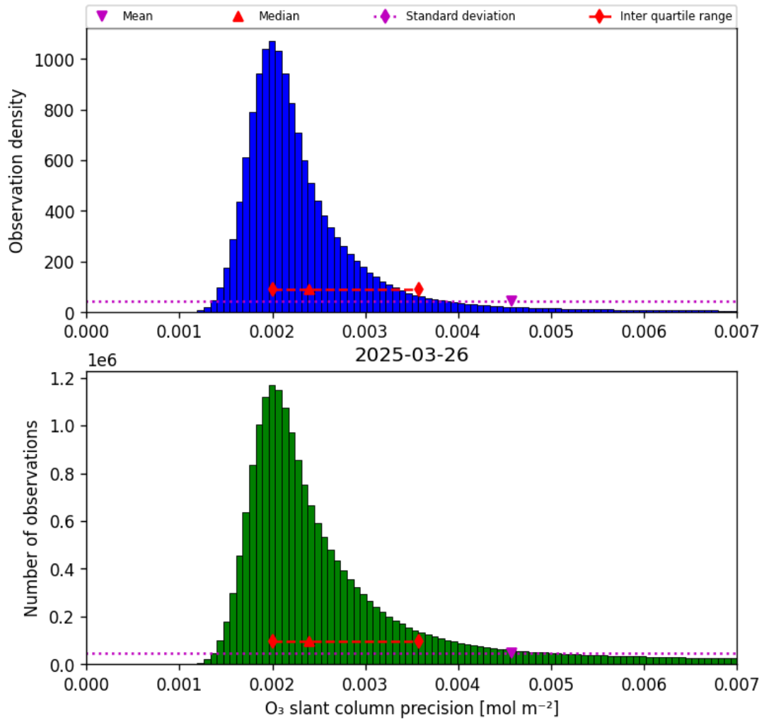
Figure 32: Histogram of “O 3 slant column precision” for 2025-03-26 to 2025-03-26
