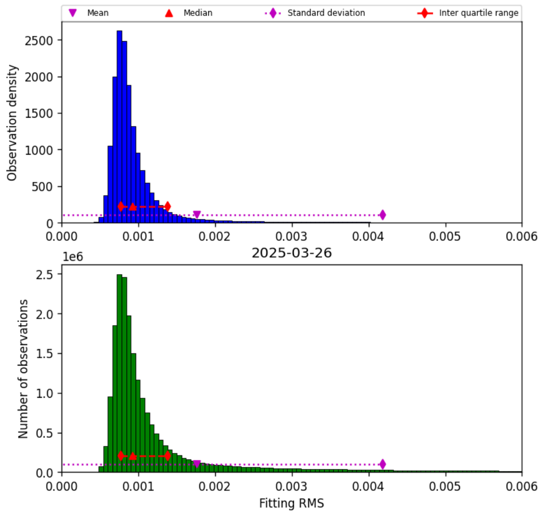
Figure 34: Histogram of “Fitting RMS” for 2025-03-26 to 2025-03-26
