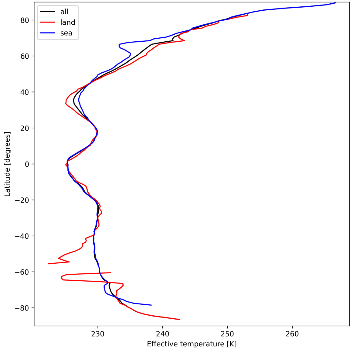
Figure 26: Zonal average of "Effective temperature" for 2025-03-26 to 2025-03-26.
