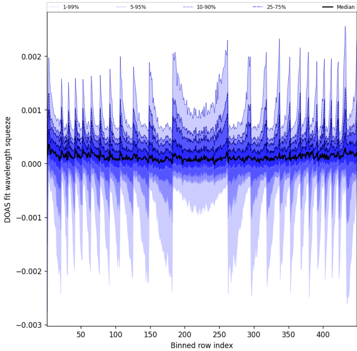
Figure 48: Along track statistics of “DOAS fit wavelength squeeze” for 2025-03-26 to 2025-03-26
