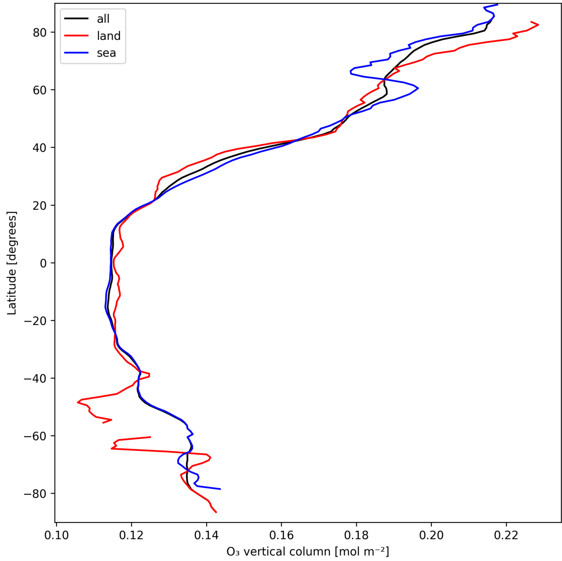
Figure 17: Zonal average of “O 3 vertical column” for 2025-03-26 to 2025-03-26.
