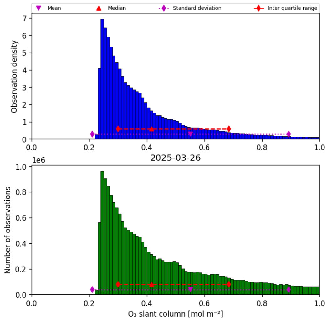
Figure 31: Histogram of “O 3 slant column” for 2025-03-26 to 2025-03-26
