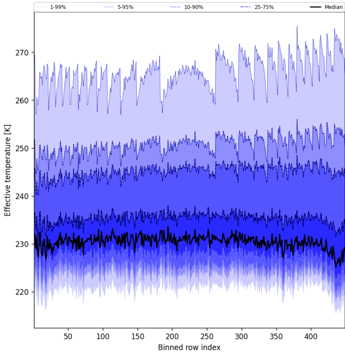
Figure 50: Along track statistics of “Effective temperature” for 2025-03-26 to 2025-03-26
