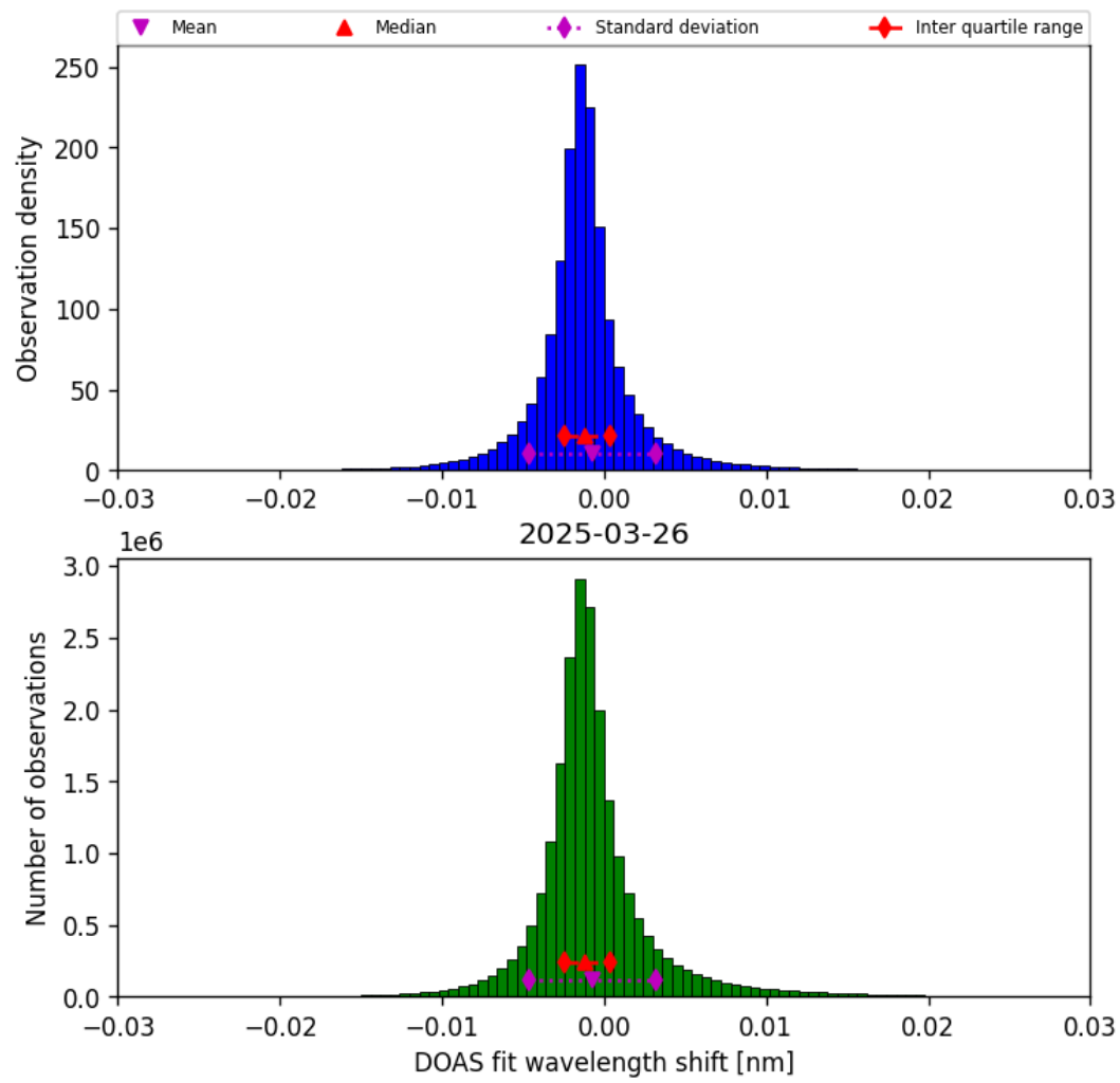
Figure 35: Histogram of “DOAS fit wavelength shift” for 2025-03-26 to 2025-03-26
