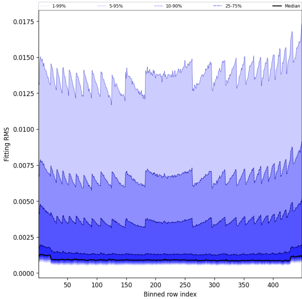
Figure 46: Along track statistics of “Fitting RMS” for 2025-03-26 to 2025-03-26
