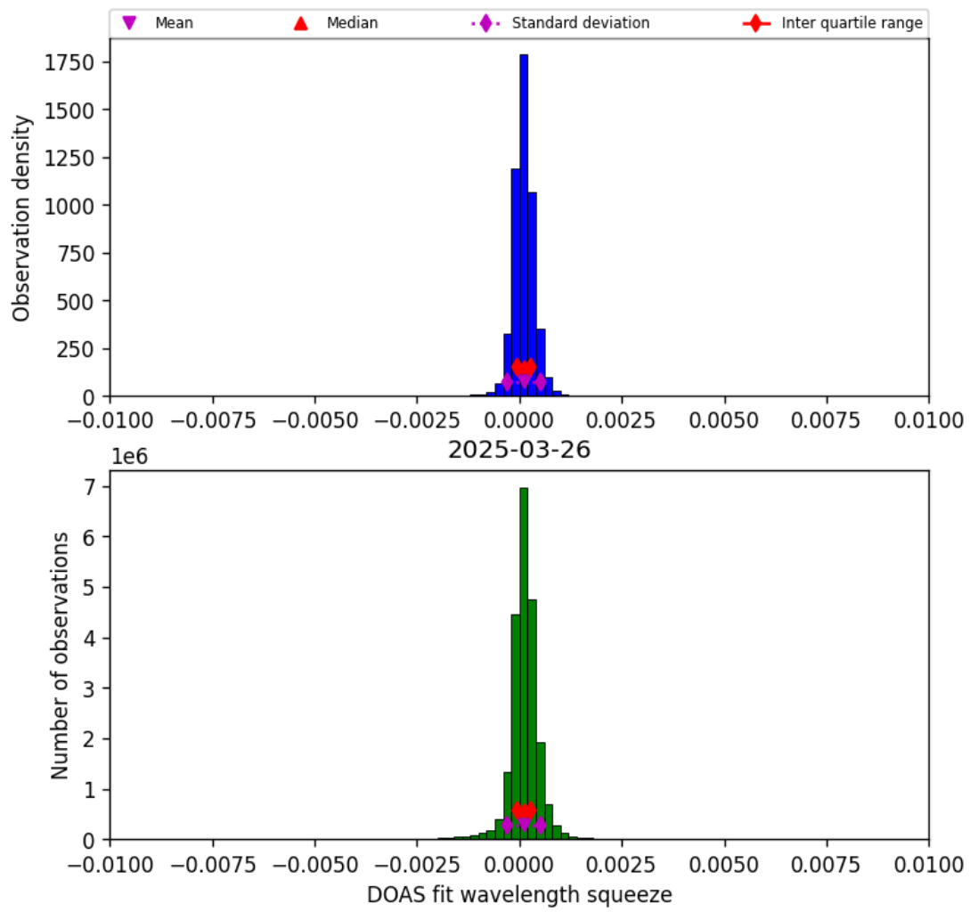
Figure 36: Histogram of “DOAS fit wavelength squeeze” for 2025-03-26 to 2025-03-26
