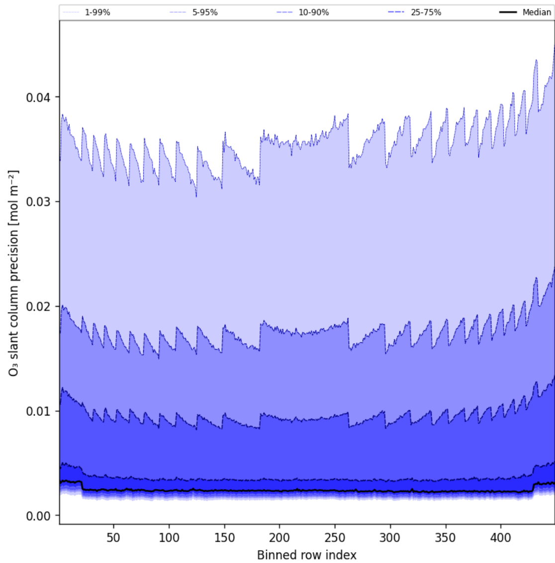
Figure 44: Along track statistics of “O 3 slant column precision” for 2025-03-26 to 2025-03-26
