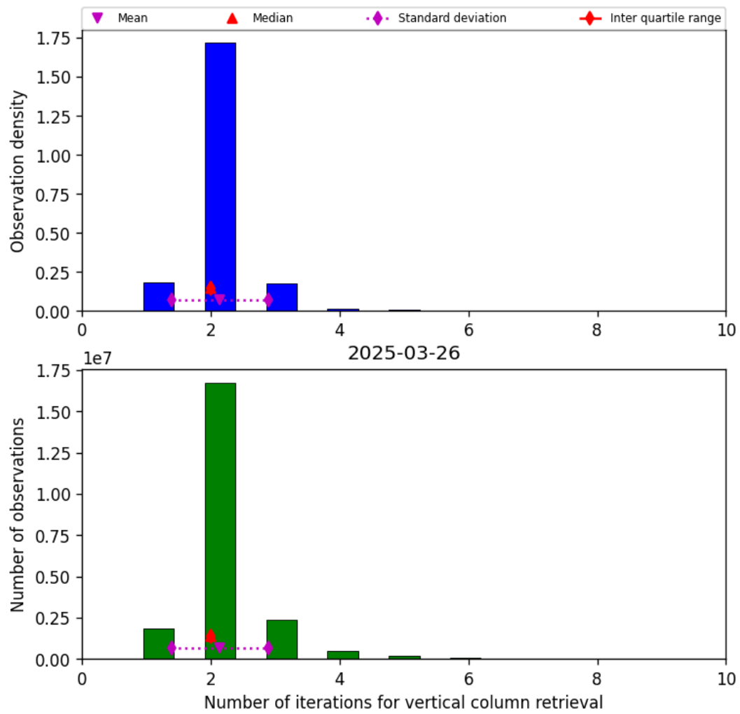
Figure 39: Histogram of “Number of iterations for vertical column retrieval” for 2025-03-26 to 2025-03-26
