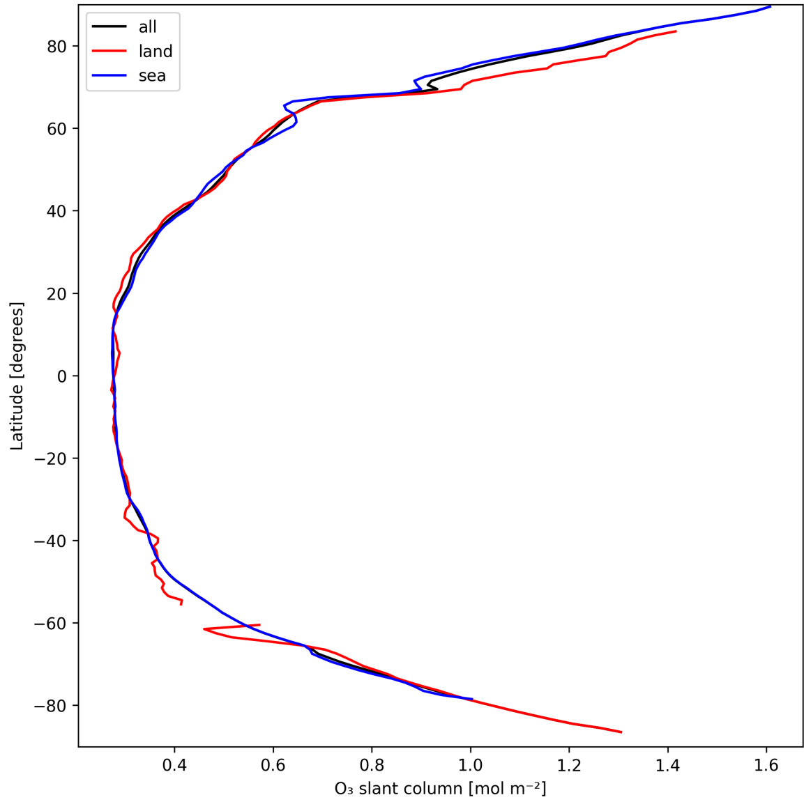
Figure 19: Zonal average of “O 3 slant column” for 2025-03-26 to 2025-03-26.
