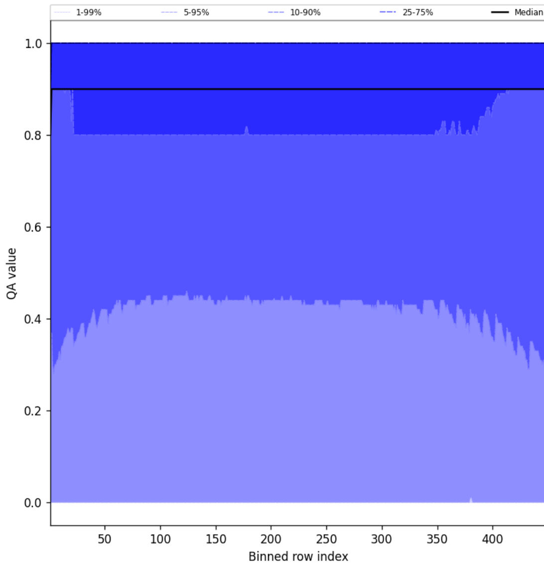
Figure 40: Along track statistics of “QA value” for 2025-03-26 to 2025-03-26
