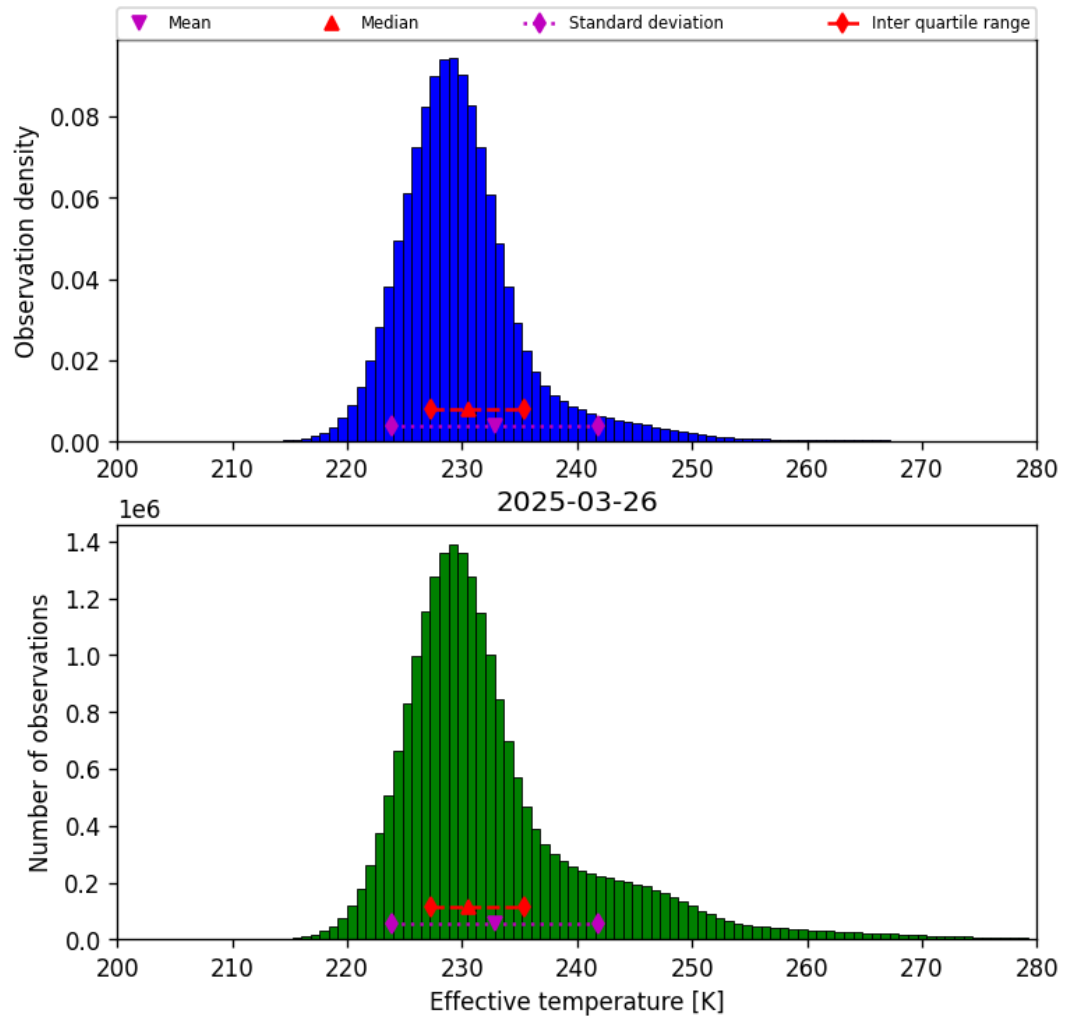
Figure 38: Histogram of “Effective temperature” for 2025-03-26 to 2025-03-26
