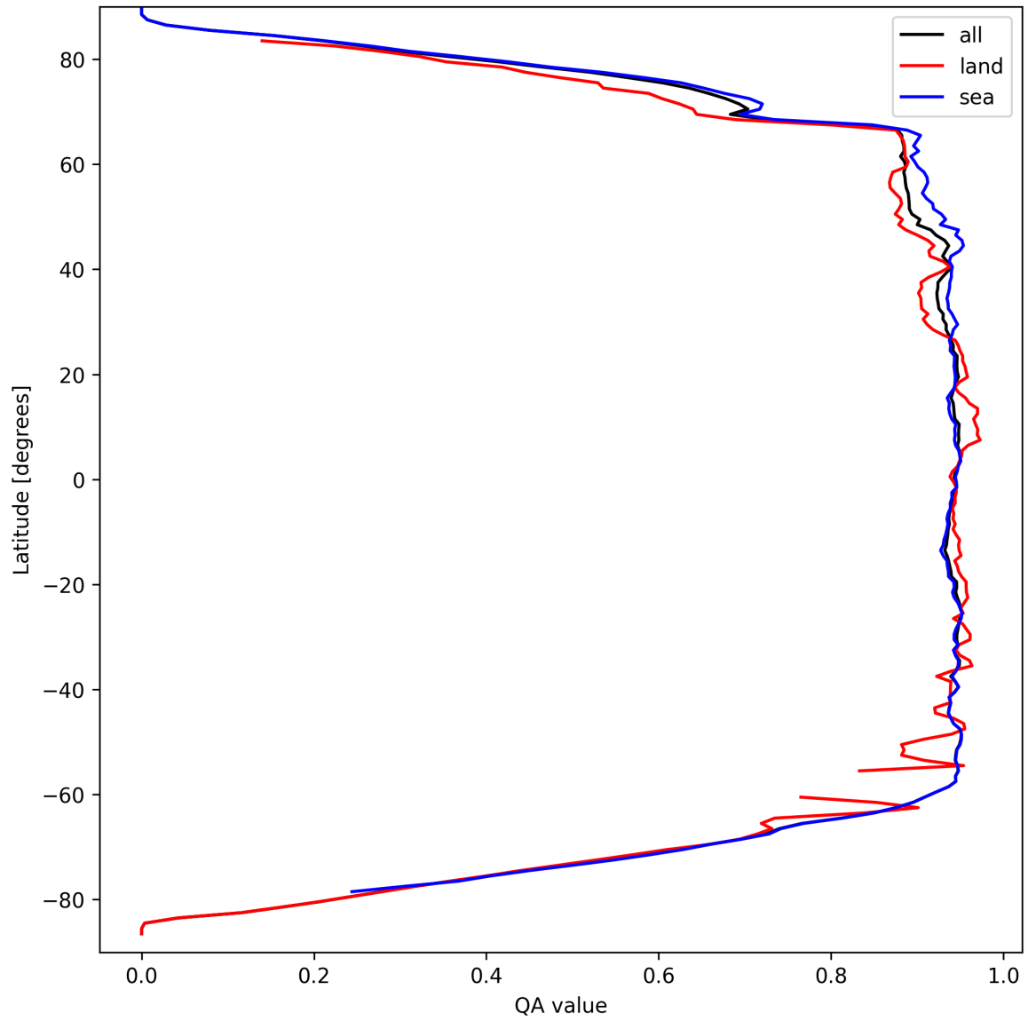
Figure 16: Zonal average of “QA value” for 2025-03-26 to 2025-03-26.
