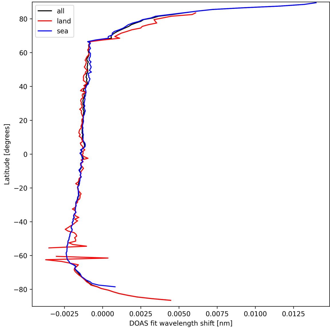
Figure 23: Zonal average of “DOAS fit wavelength shift” for 2025-03-26 to 2025-03-26.
