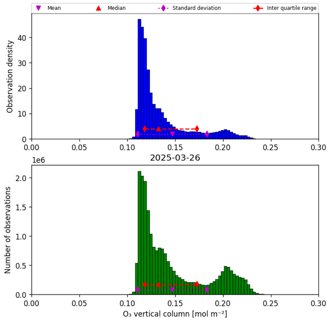
Figure 29: Histogram of “O 3 vertical column” for 2025-03-26 to 2025-03-26
