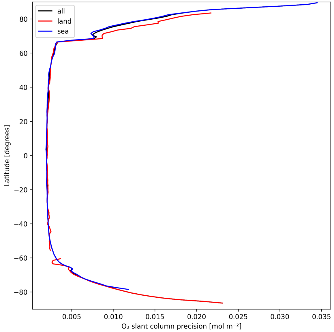
Figure 20: Zonal average of “O 3 slant column precision” for 2025-03-26 to 2025-03-26.
