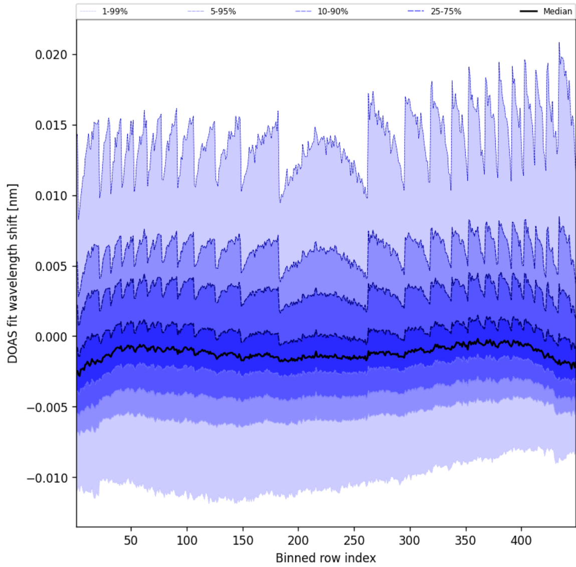
Figure 47: Along track statistics of “DOAS fit wavelength shift” for 2025-03-26 to 2025-03-26
