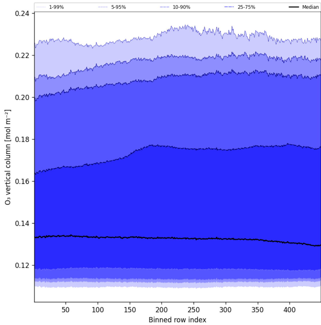
Figure 41: Along track statistics of “O 3 vertical column” for 2025-03-26 to 2025-03-26
