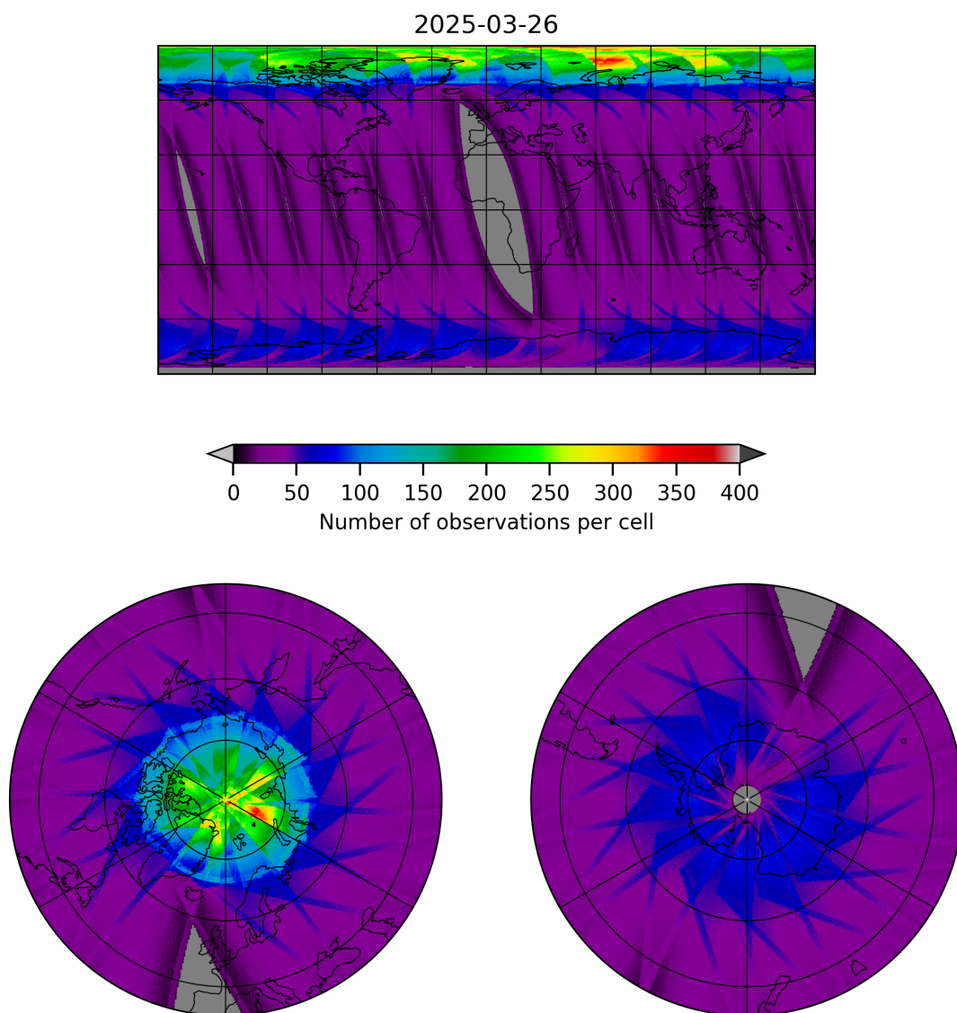
Figure 15: Map of the number of observations for 2025-03-26 to 2025-03-26
