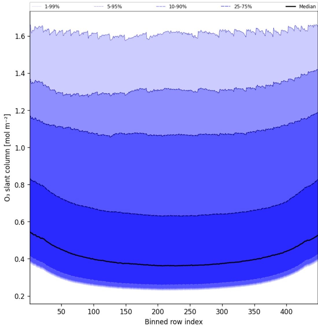
Figure 43: Along track statistics of “O 3 slant column” for 2025-03-26 to 2025-03-26
