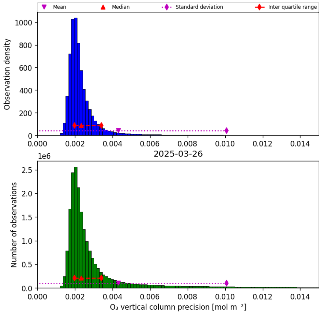
Figure 30: Histogram of “O 3 vertical column precision” for 2025-03-26 to 2025-03-26
