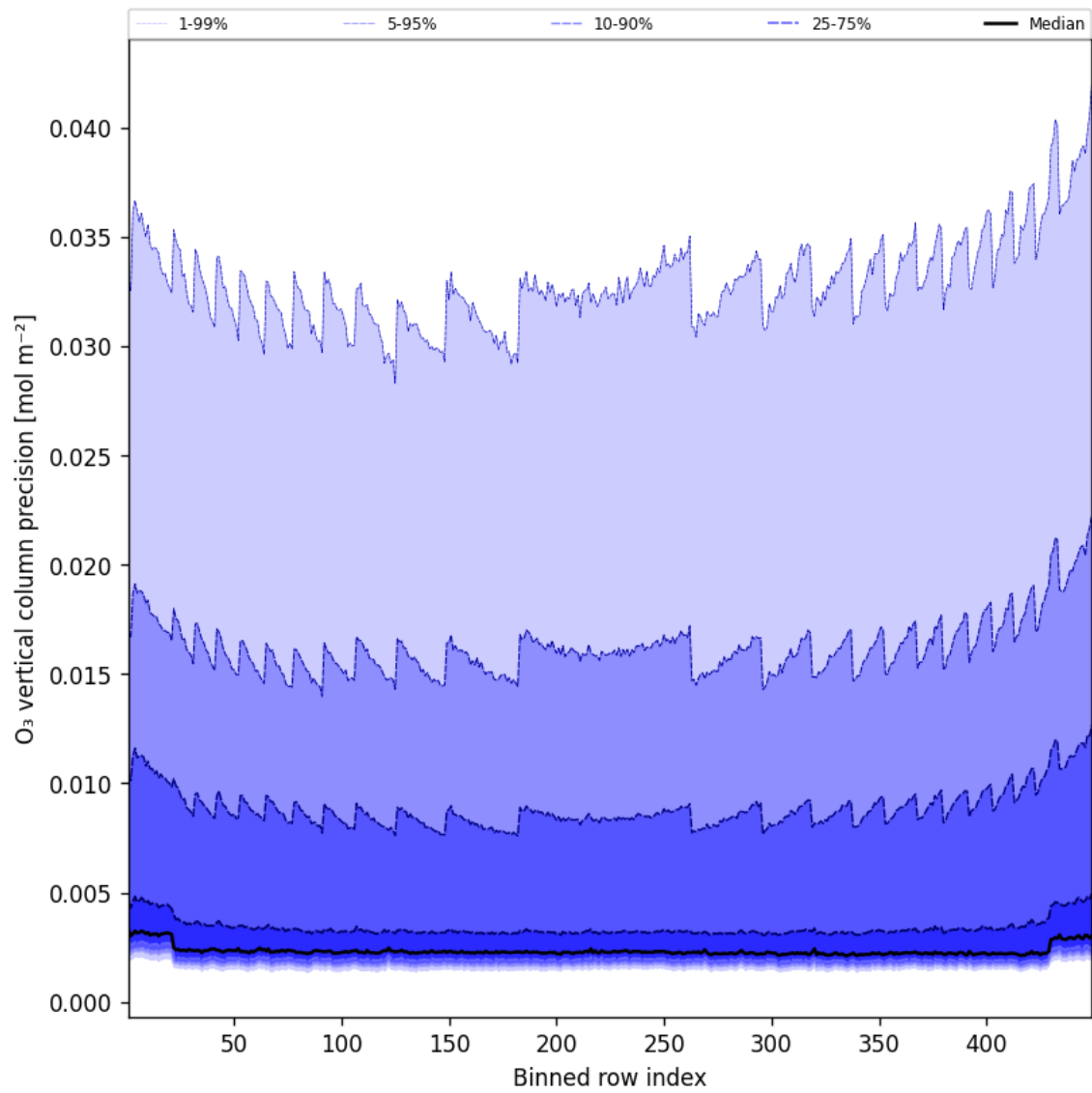
Figure 42: Along track statistics of “O 3 vertical column precision” for 2025-03-26 to 2025-03-26
