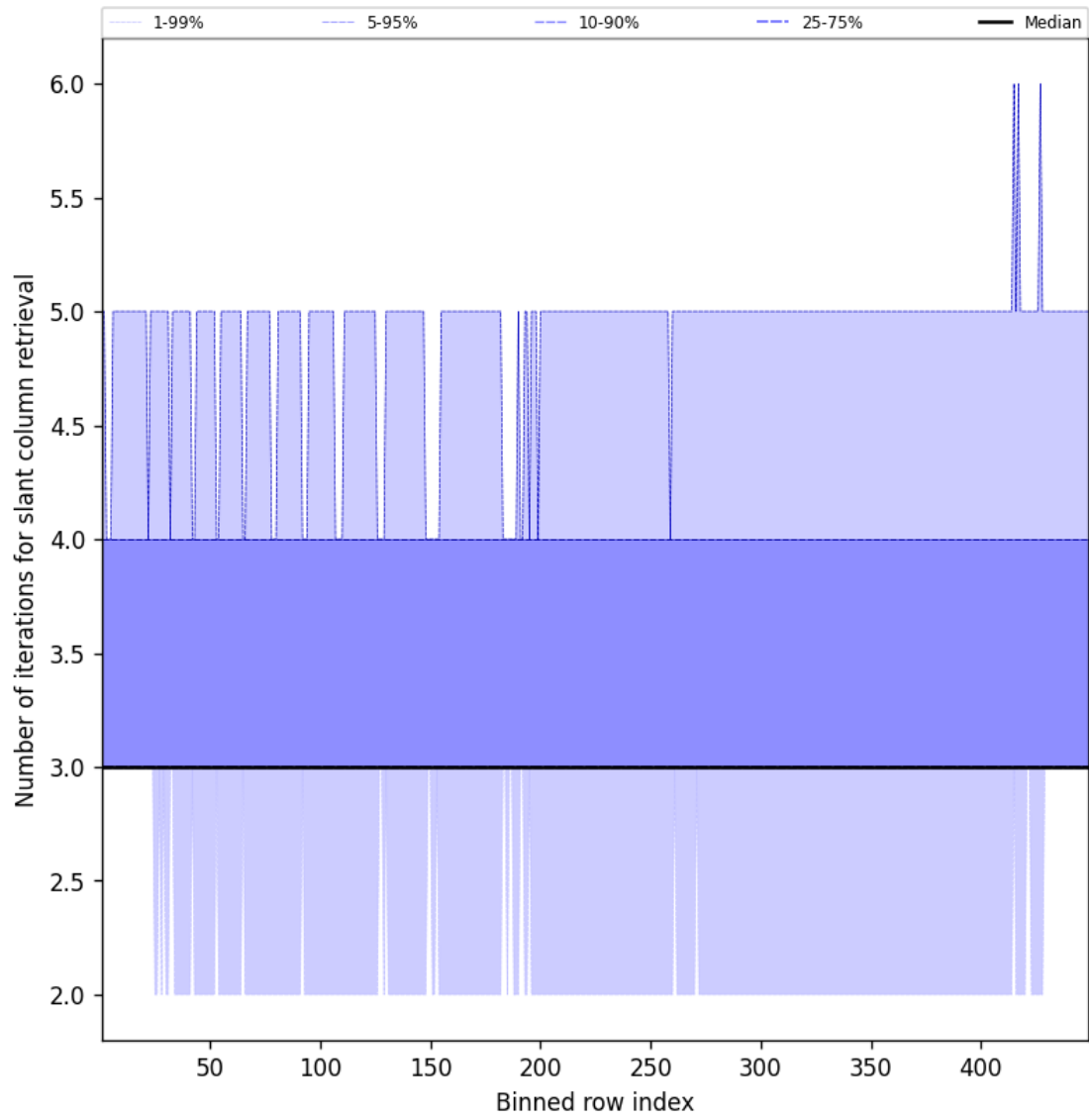
Figure 45: Along track statistics of “Number of iterations for slant column retrieval” for 2025-03-26 to 2025-03-26
