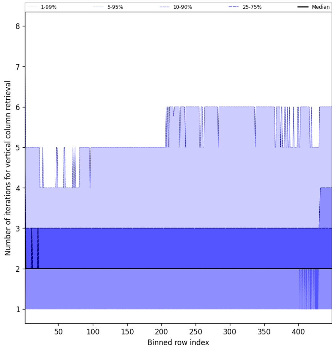
Figure 51: Along track statistics of “Number of iterations for vertical column retrieval” for 2025-03-26 to 2025-03-26
