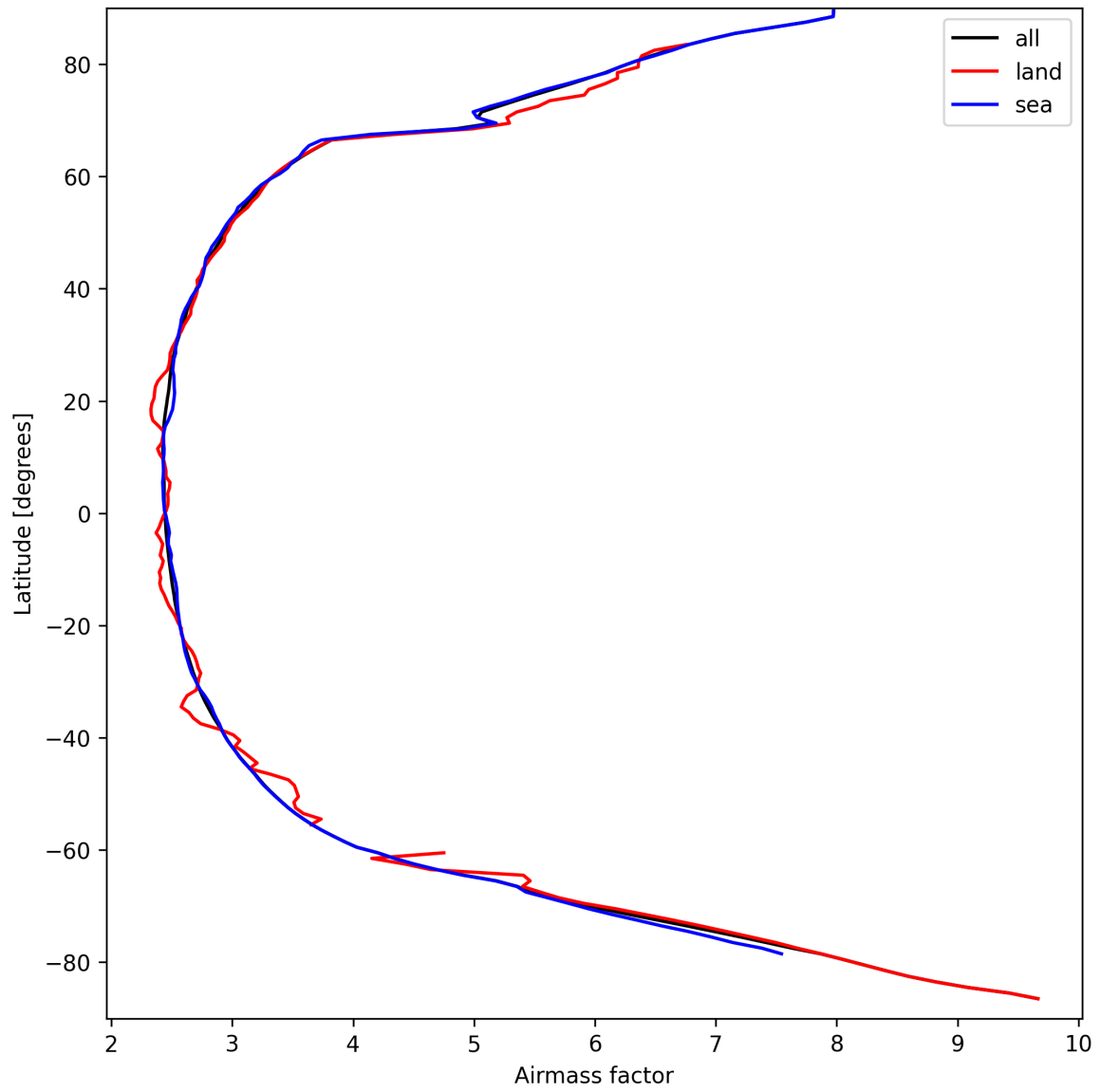
Figure 25: Zonal average of “Airmass factor” for 2025-03-26 to 2025-03-26.
