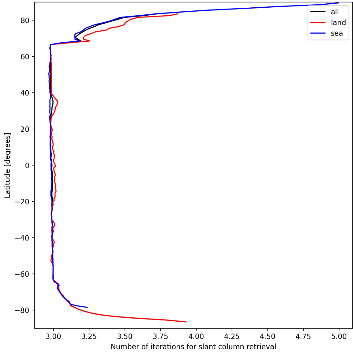
Figure 21: Zonal average of “Number of iterations for slant column retrieval” for 2025-03-26 to 2025-03-26.
