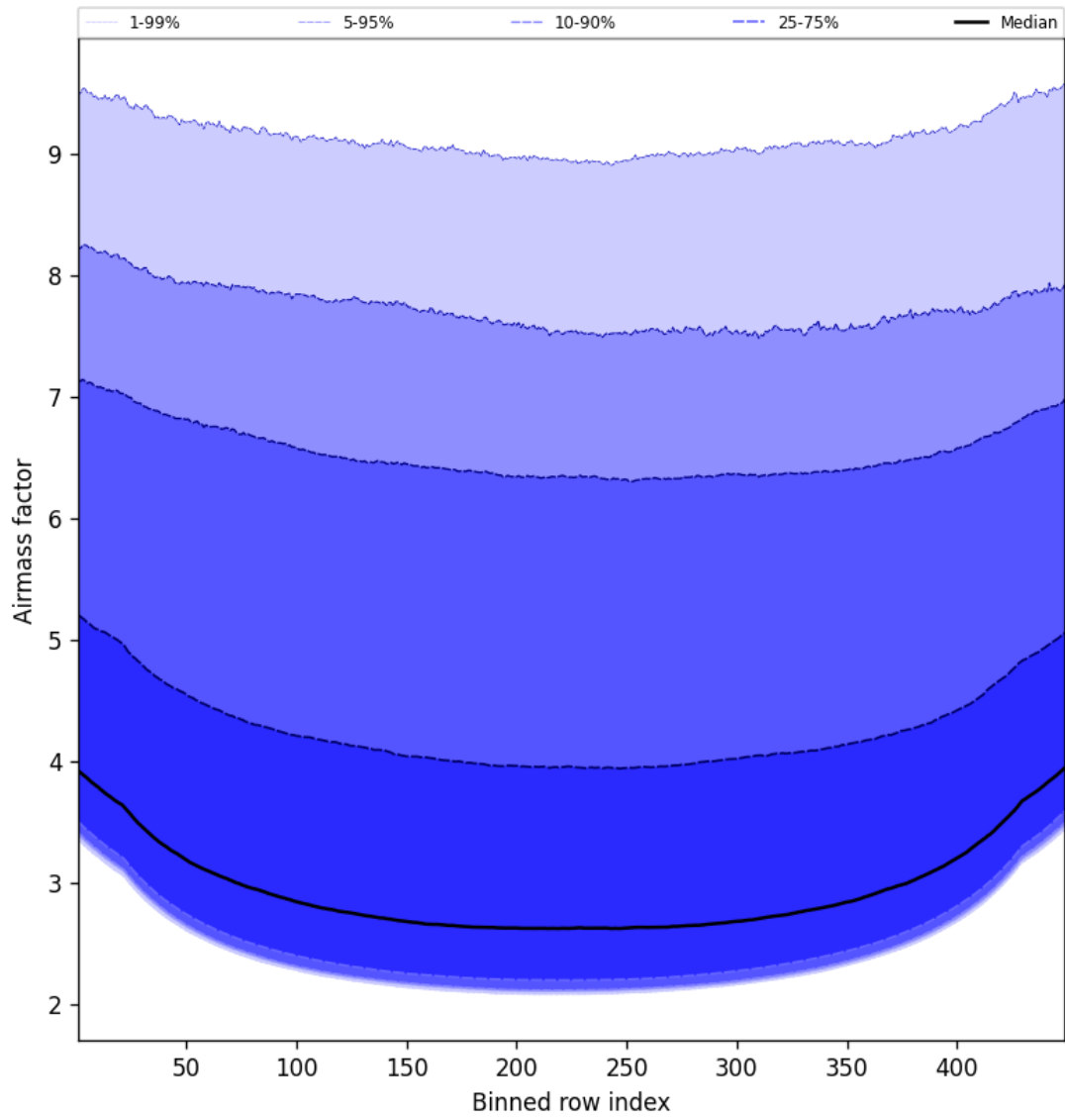
Figure 49: Along track statistics of “Airmass factor” for 2025-03-26 to 2025-03-26
