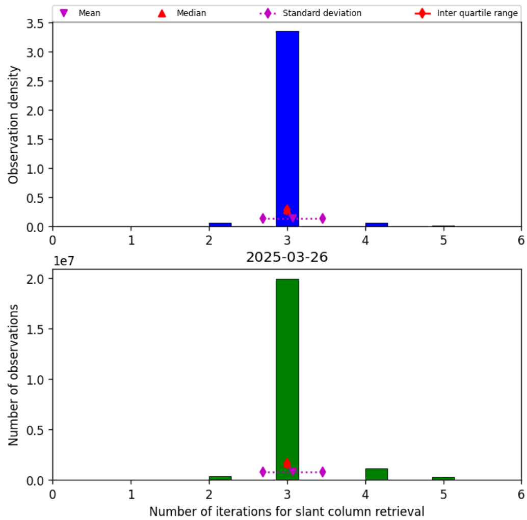
Figure 33: Histogram of "Number of iterations for slant column retrieval" for 2025-03-26 to 2025-03-26
