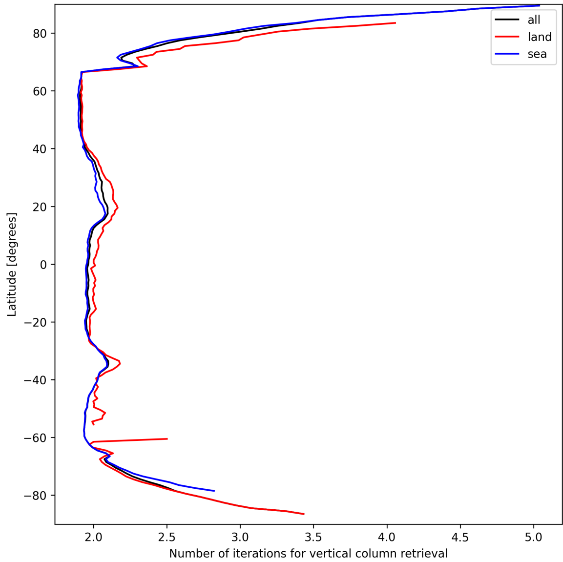
Figure 27: Zonal average of “Number of iterations for vertical column retrieval” for 2025-03-26 to 2025-03-26.
