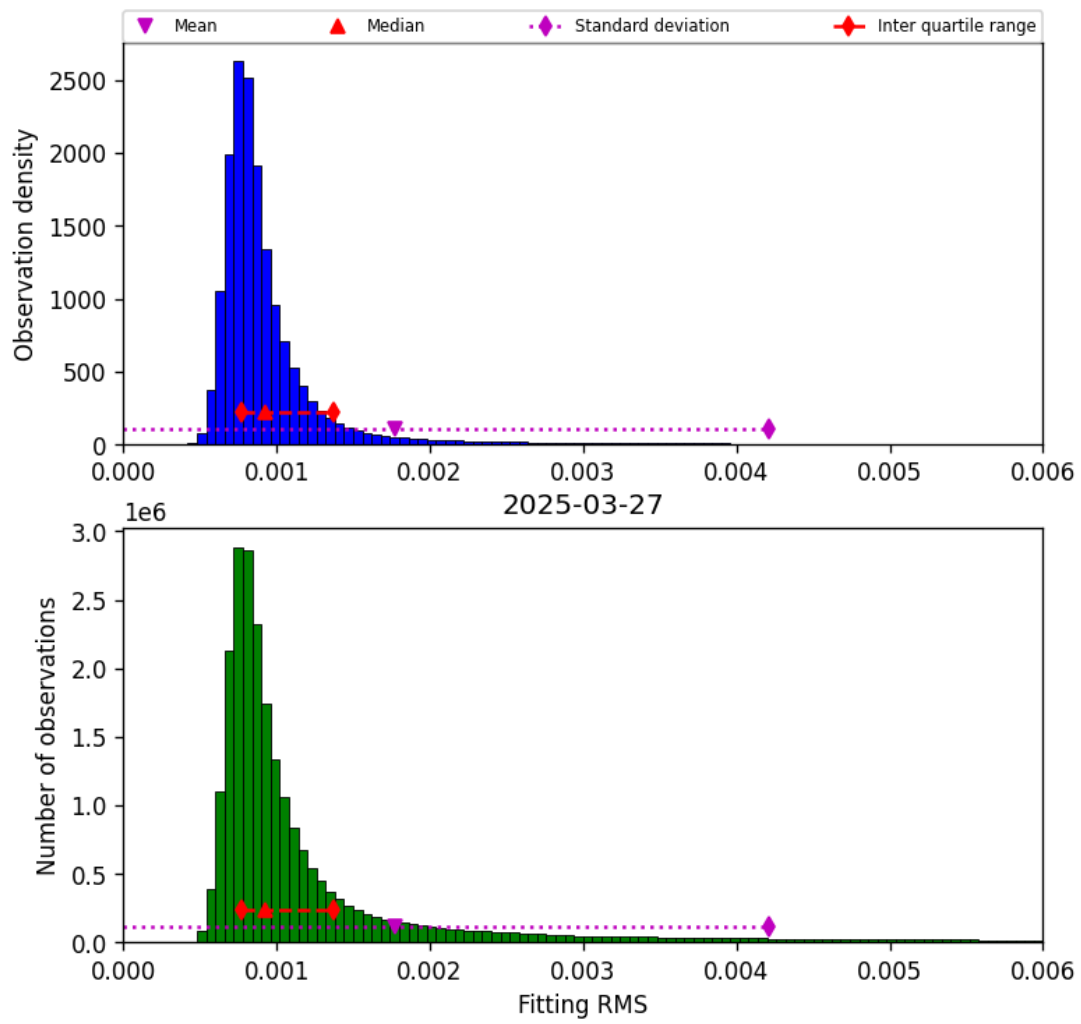
Figure 34: Histogram of “Fitting RMS” for 2025-03-27 to 2025-03-28
