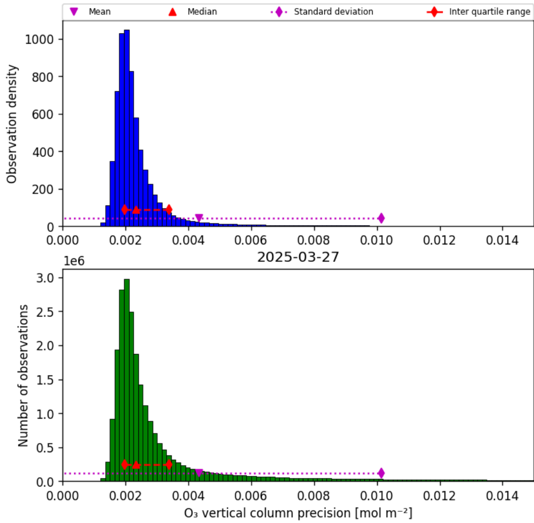
Figure 30: Histogram of “O 3 vertical column precision” for 2025-03-27 to 2025-03-28
