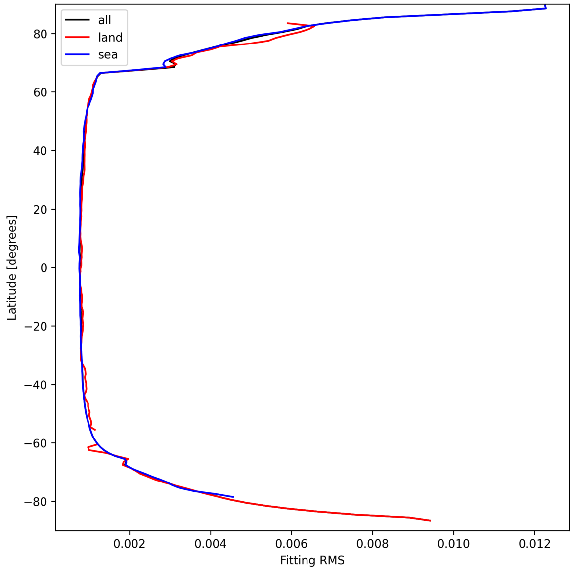
Figure 22: Zonal average of “Fitting RMS” for 2025-03-27 to 2025-03-28.
