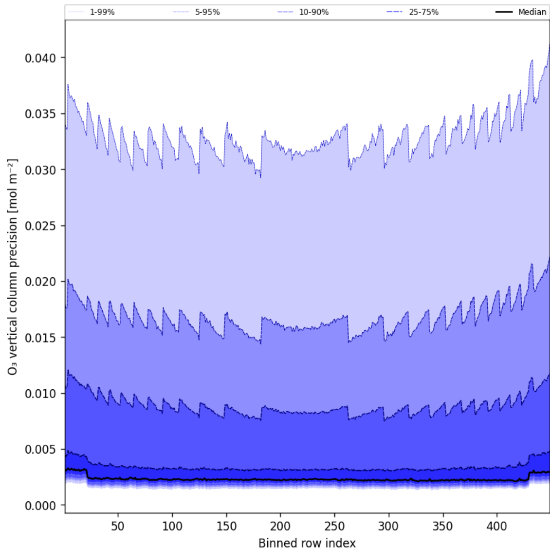
Figure 42: Along track statistics of “O 3 vertical column precision” for 2025-03-27 to 2025-03-28
