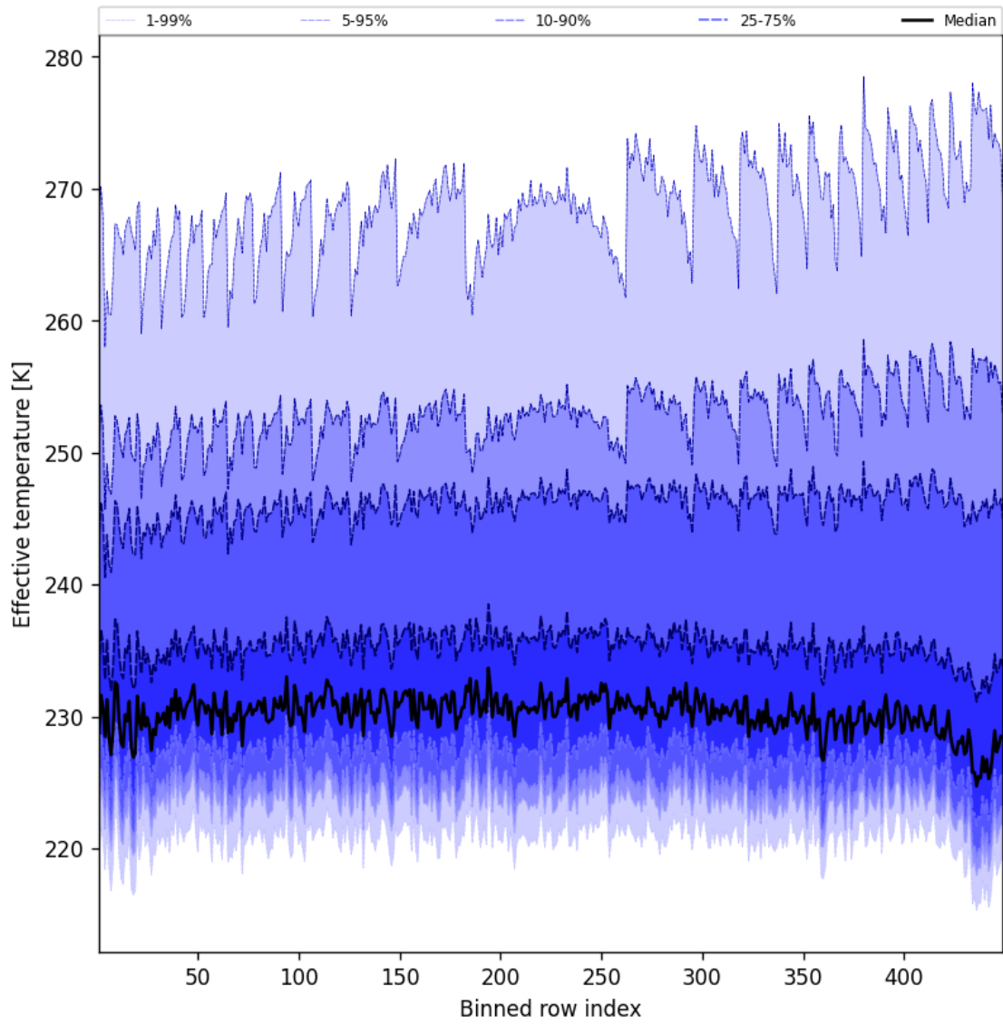
Figure 50: Along track statistics of “Effective temperature” for 2025-03-27 to 2025-03-28
