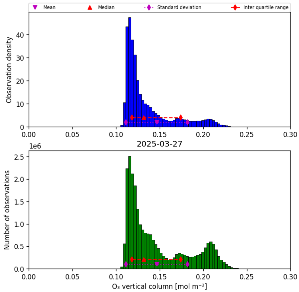
Figure 29: Histogram of “O 3 vertical column” for 2025-03-27 to 2025-03-28
