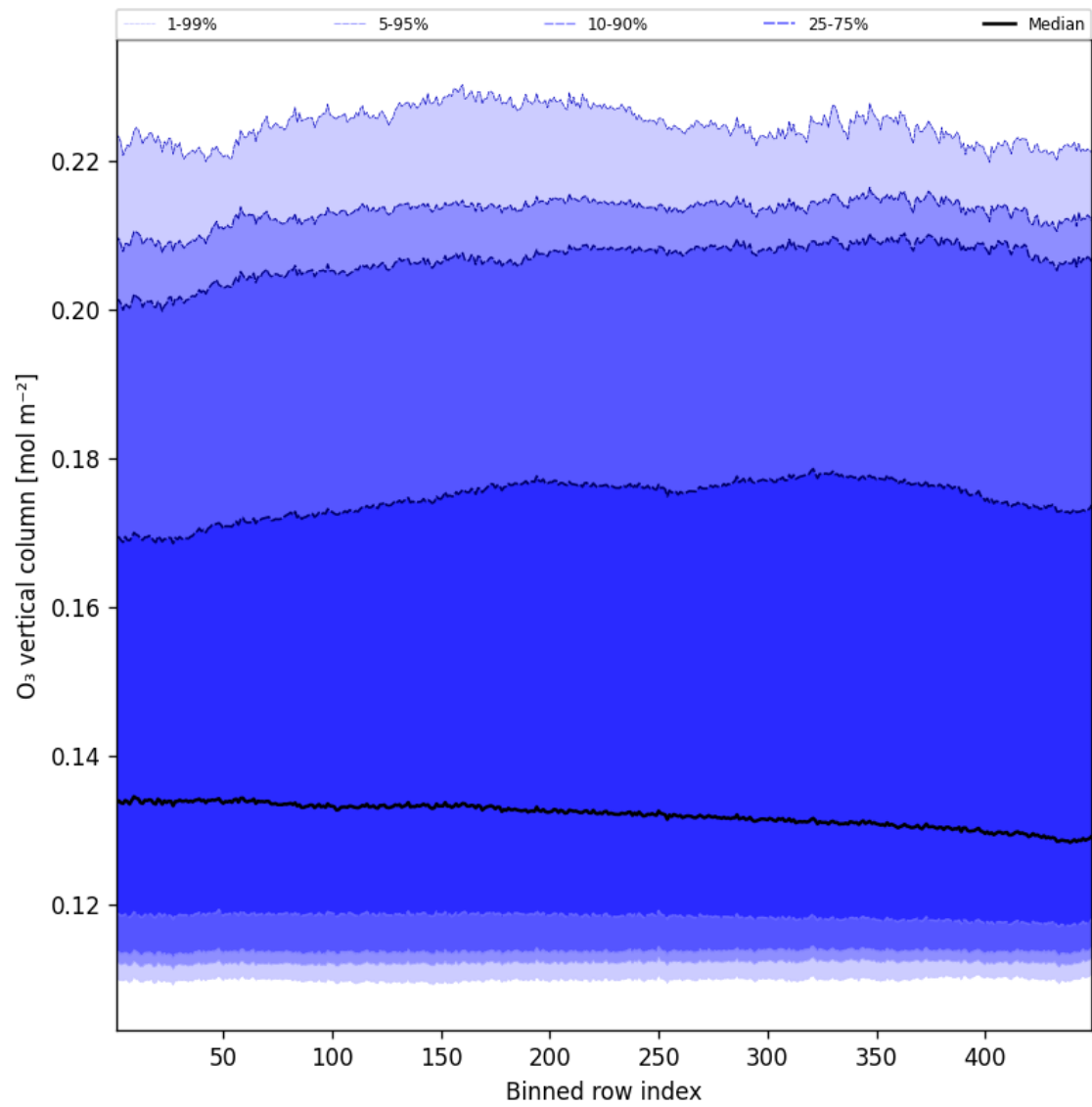
Figure 41: Along track statistics of “O 3 vertical column” for 2025-03-27 to 2025-03-28
