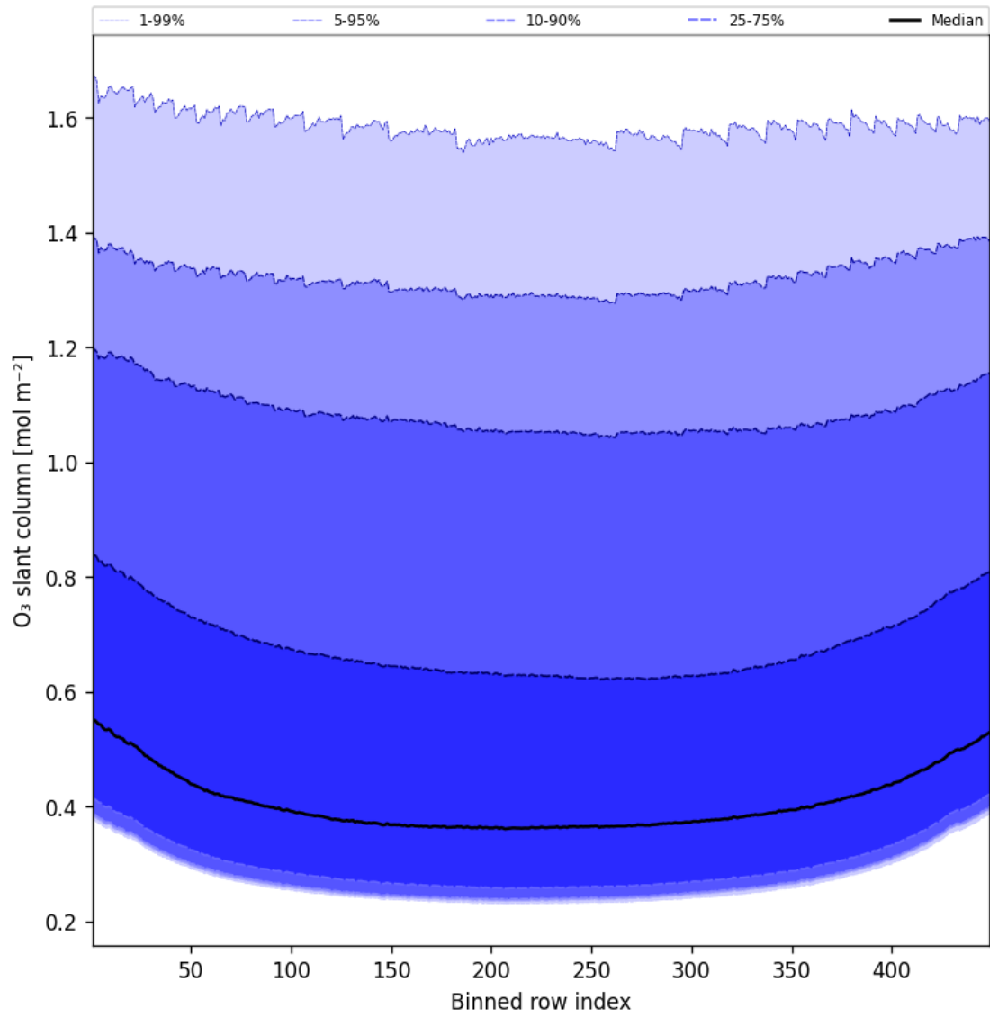
Figure 43: Along track statistics of “O 3 slant column” for 2025-03-27 to 2025-03-28
