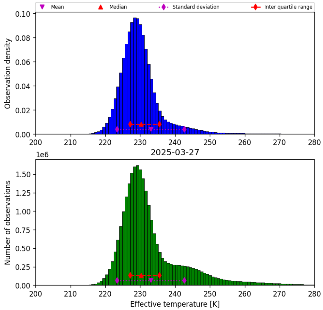
Figure 38: Histogram of “Effective temperature” for 2025-03-27 to 2025-03-28
