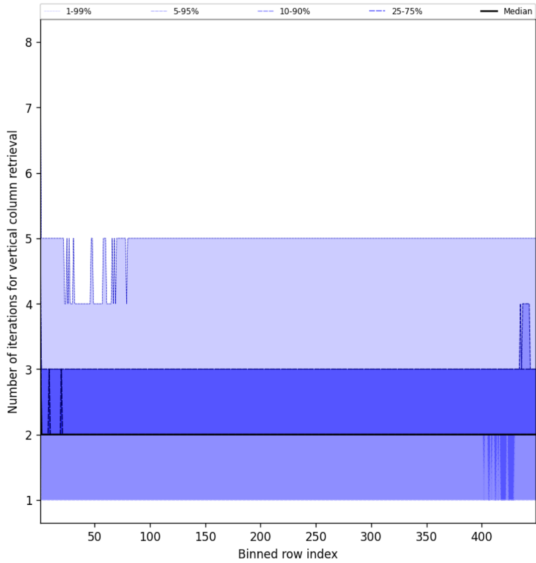
Figure 51: Along track statistics of “Number of iterations for vertical column retrieval” for 2025-03-27 to 2025-03-28
