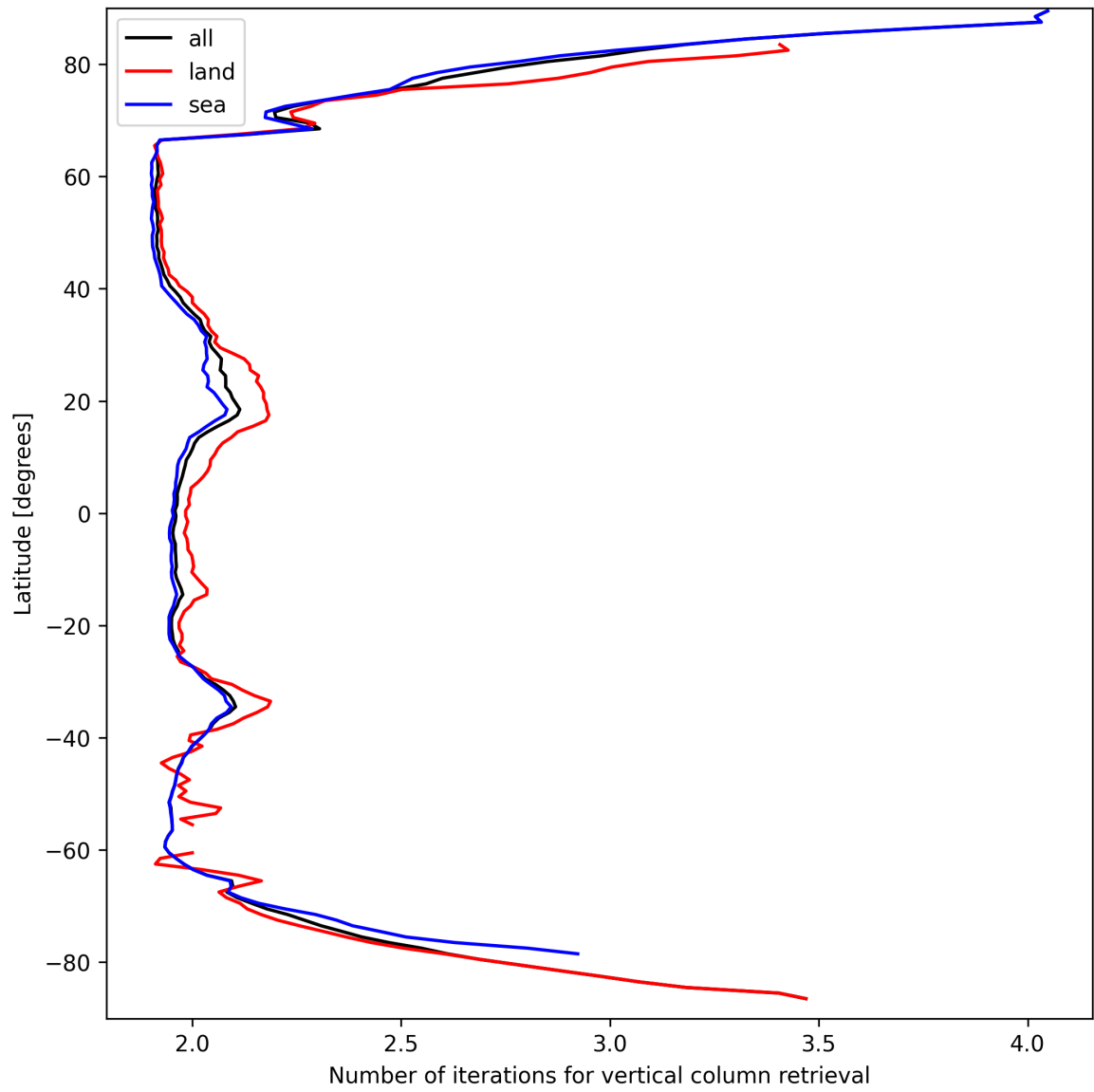
Figure 27: Zonal average of “Number of iterations for vertical column retrieval” for 2025-03-27 to 2025-03-28.
