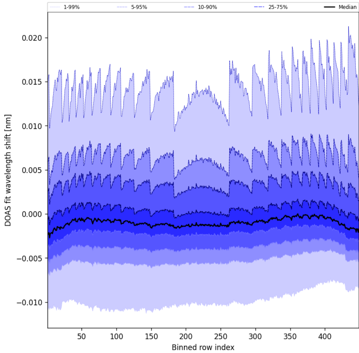
Figure 47: Along track statistics of “DOAS fit wavelength shift” for 2025-03-27 to 2025-03-28
