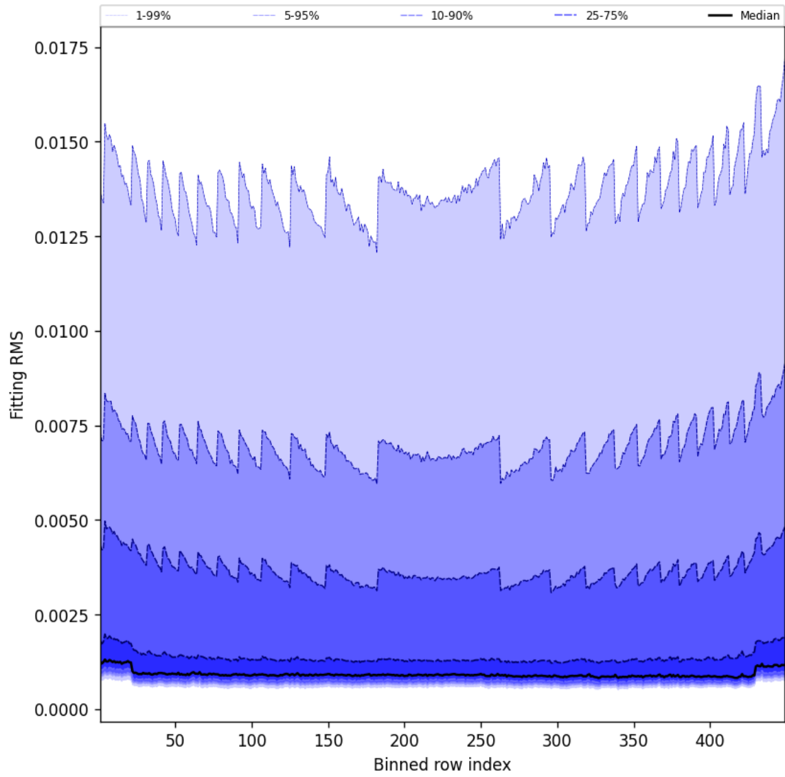
Figure 46: Along track statistics of “Fitting RMS” for 2025-03-27 to 2025-03-28
