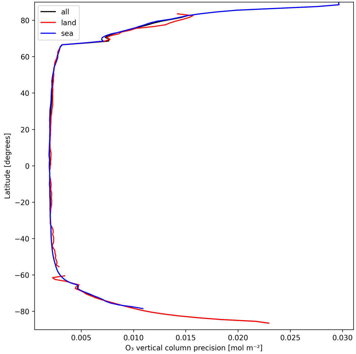
Figure 18: Zonal average of "O 3 vertical column precision" for 2025-03-27 to 2025-03-28.
