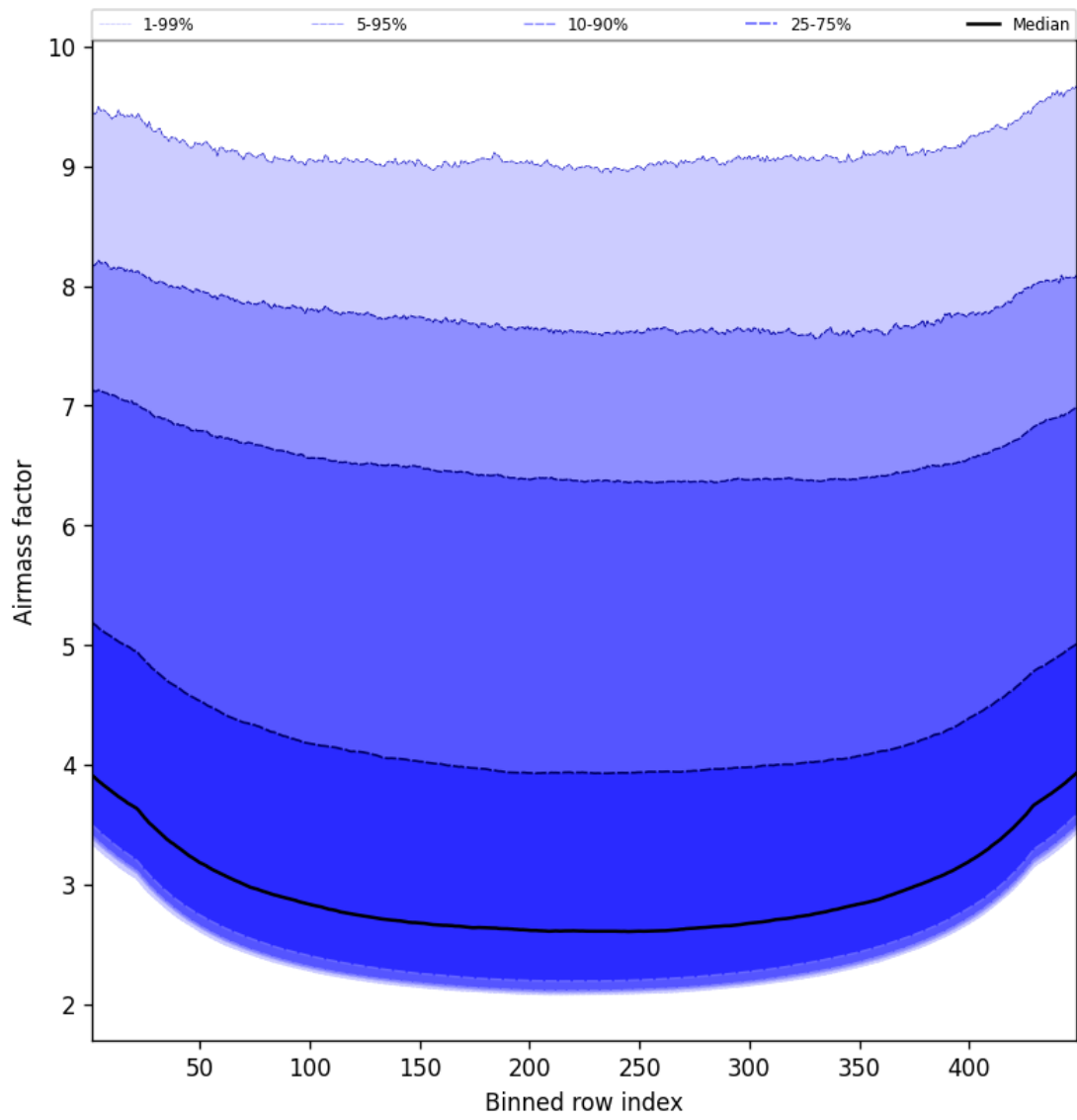
Figure 49: Along track statistics of “Airmass factor” for 2025-03-27 to 2025-03-28
