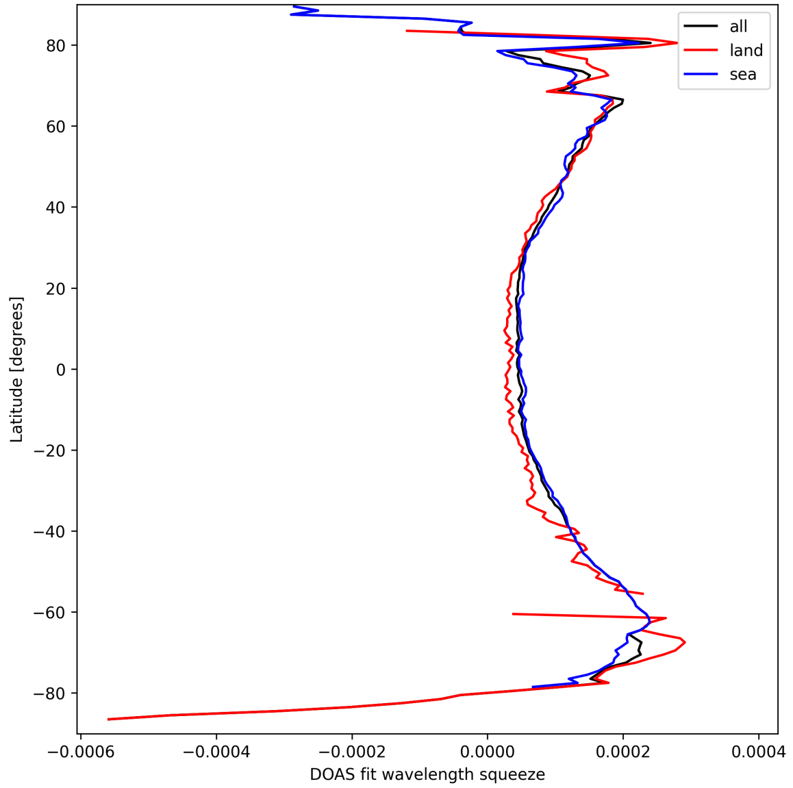
Figure 24: Zonal average of “DOAS fit wavelength squeeze” for 2025-03-27 to 2025-03-28.
