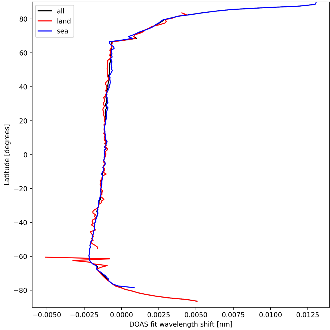
Figure 23: Zonal average of “DOAS fit wavelength shift” for 2025-03-27 to 2025-03-28.
