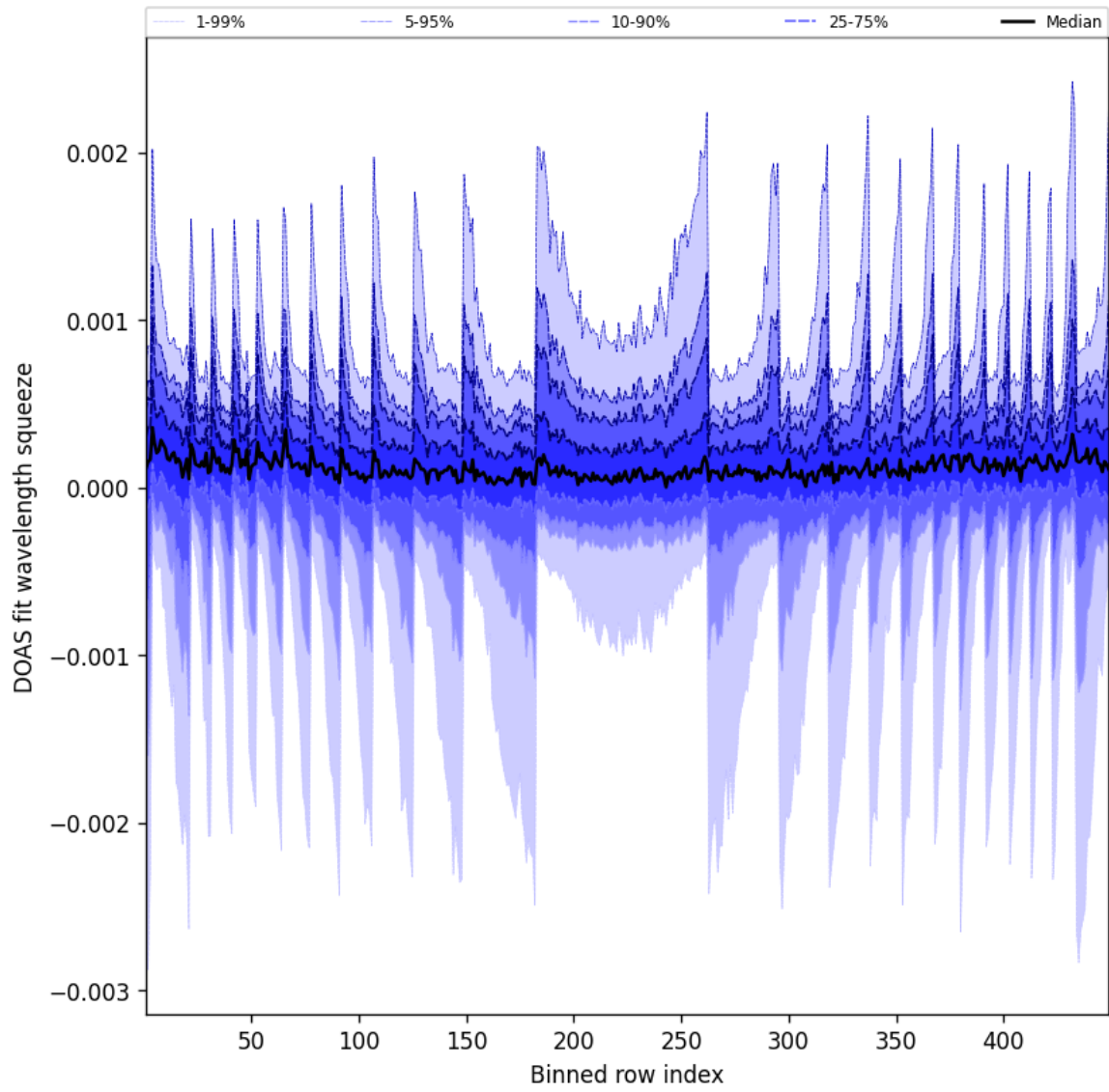
Figure 48: Along track statistics of “DOAS fit wavelength squeeze” for 2025-03-27 to 2025-03-28
