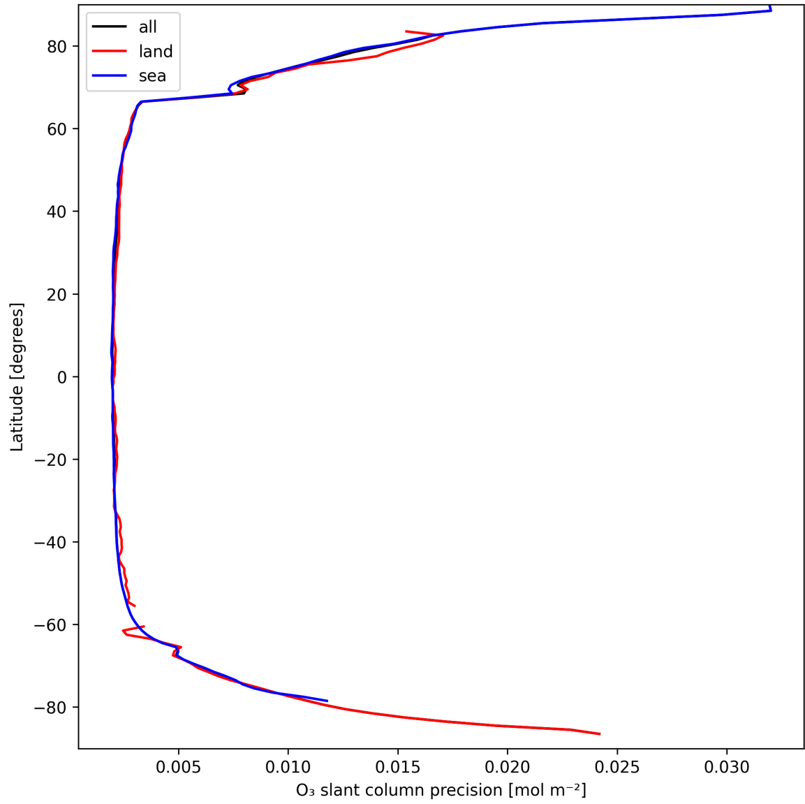
Figure 20: Zonal average of “O 3 slant column precision” for 2025-03-27 to 2025-03-28.
