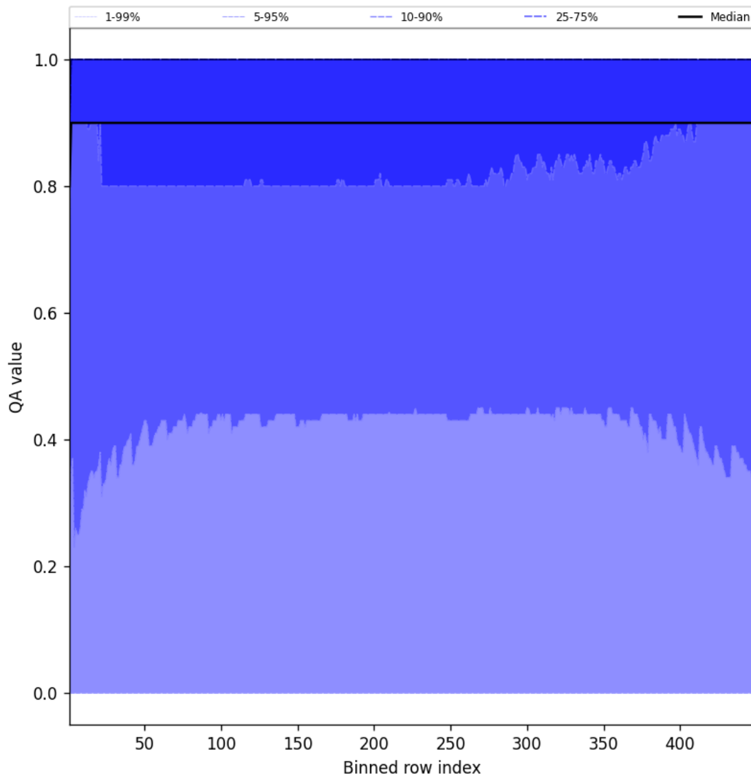
Figure 40: Along track statistics of “QA value” for 2025-03-27 to 2025-03-28
