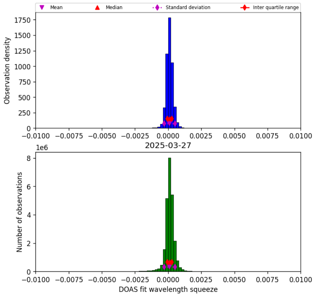
Figure 36: Histogram of “DOAS fit wavelength squeeze” for 2025-03-27 to 2025-03-28
