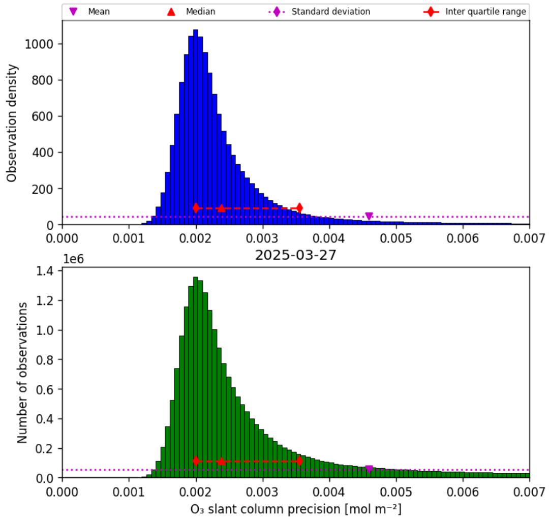
Figure 32: Histogram of “O 3 slant column precision” for 2025-03-27 to 2025-03-28
