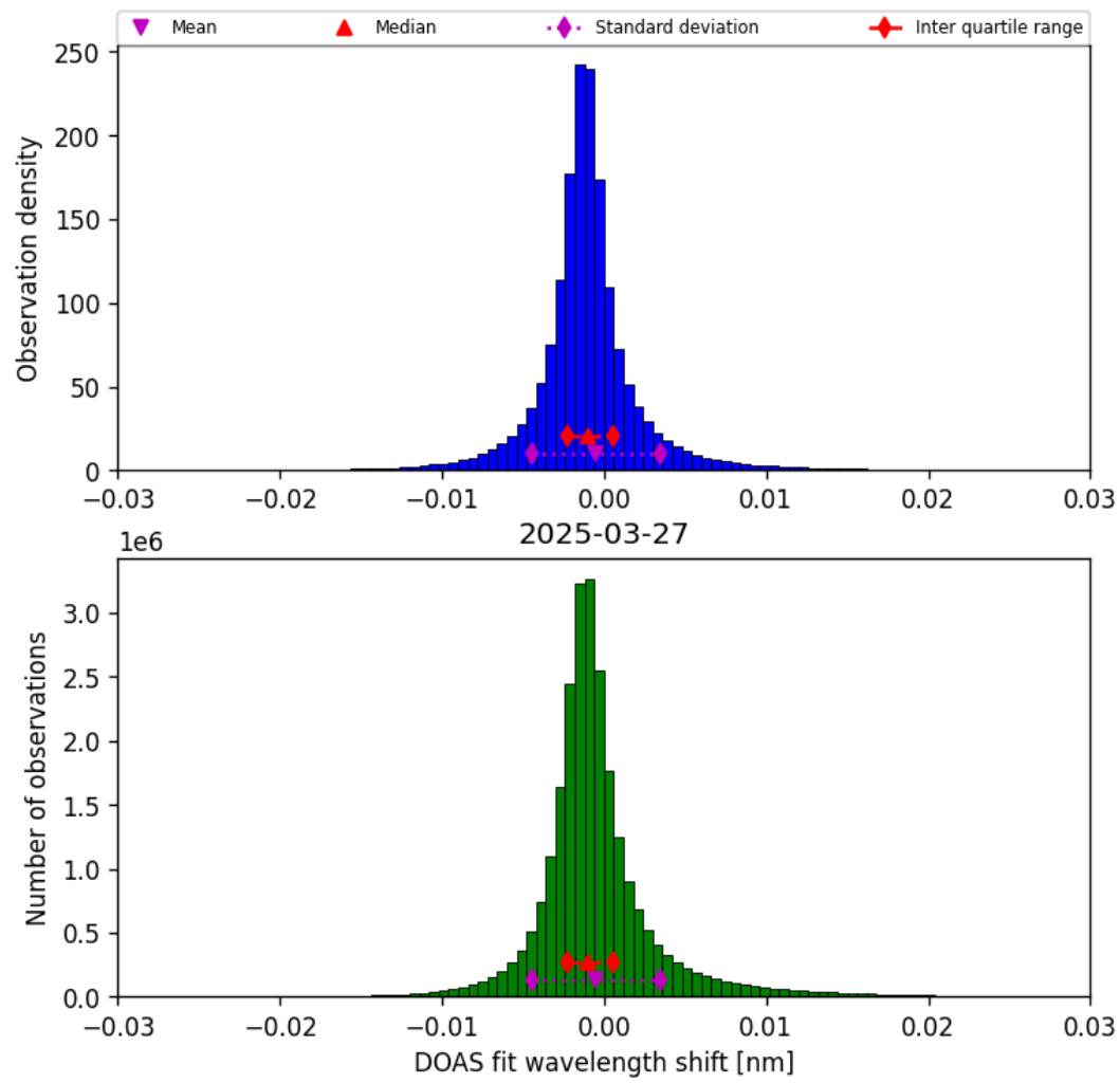
Figure 35: Histogram of “DOAS fit wavelength shift” for 2025-03-27 to 2025-03-28
