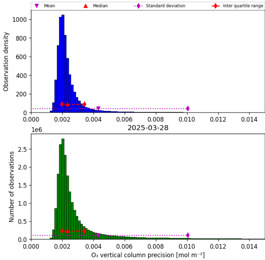
Figure 30: Histogram of “O 3 vertical column precision” for 2025-03-28 to 2025-03-29
