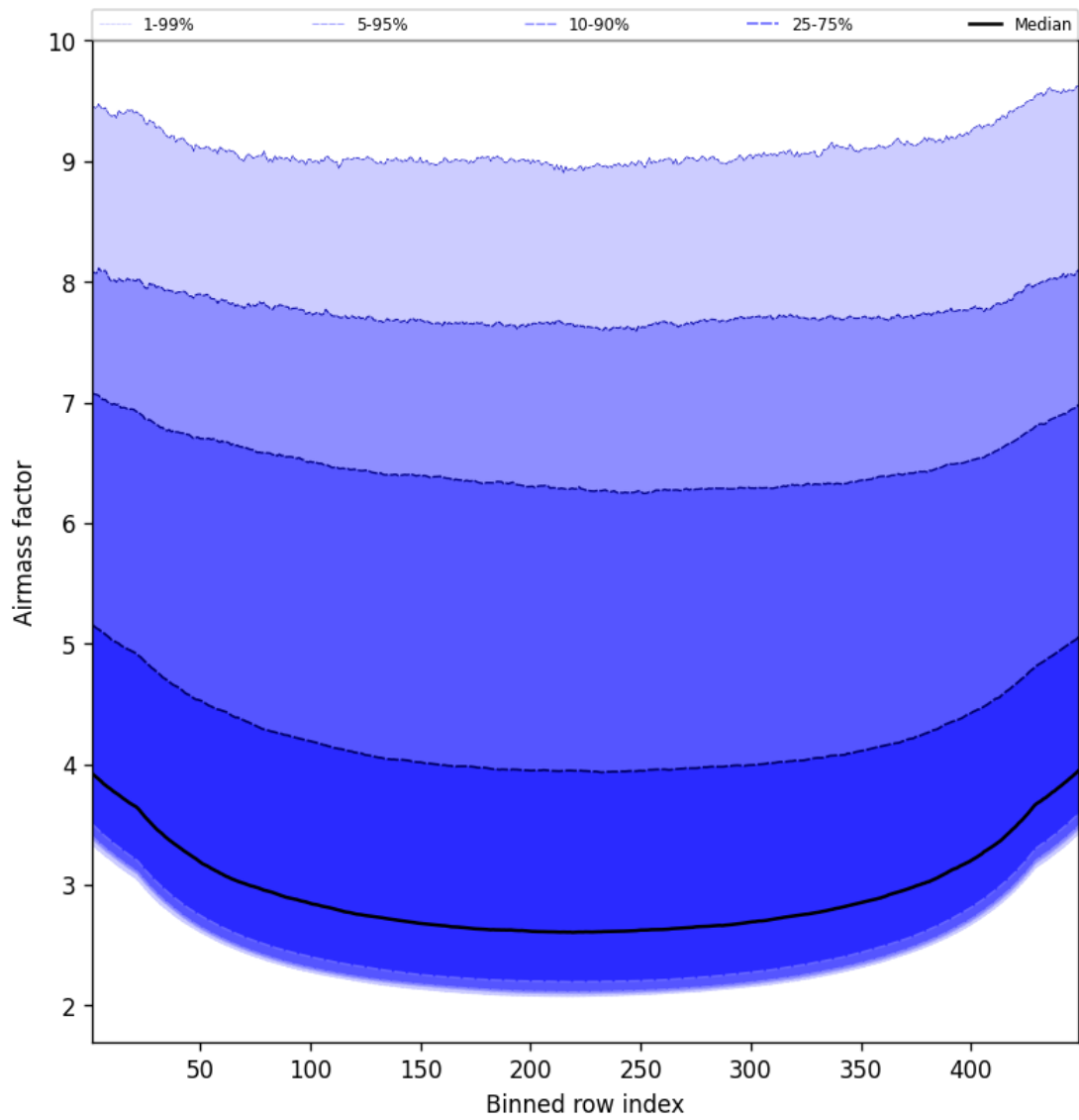
Figure 49: Along track statistics of “Airmass factor” for 2025-03-28 to 2025-03-29
