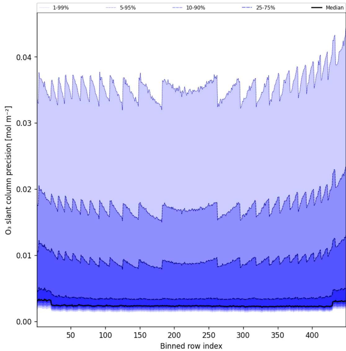
Figure 44: Along track statistics of “O 3 slant column precision” for 2025-03-28 to 2025-03-29
