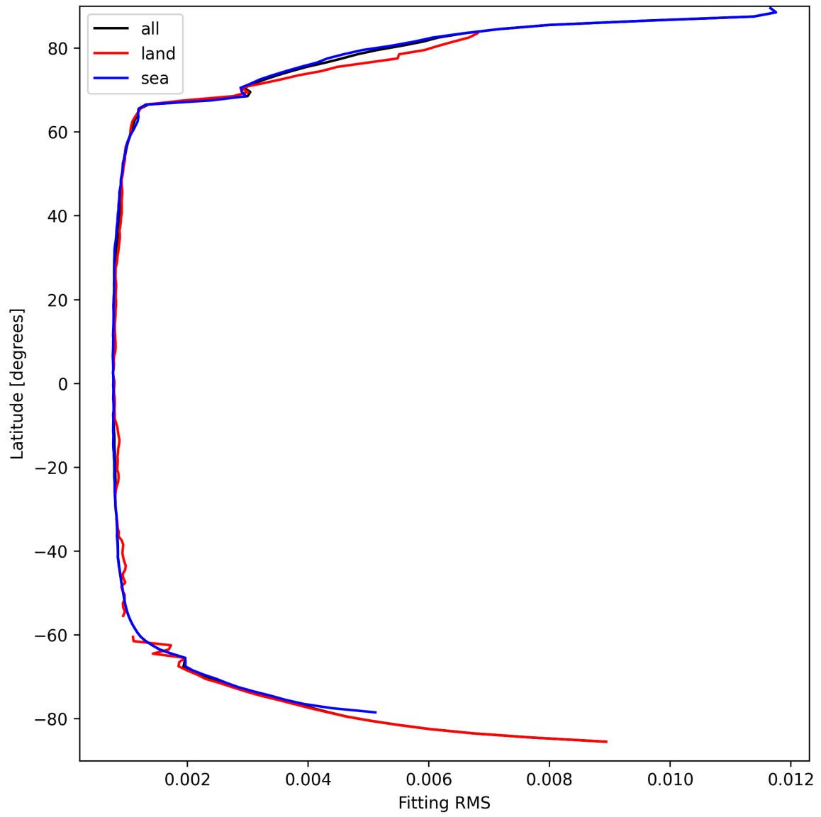
Figure 22: Zonal average of “Fitting RMS” for 2025-03-28 to 2025-03-29.
