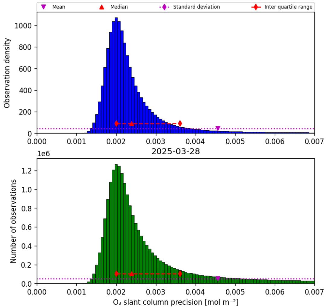
Figure 32: Histogram of “O 3 slant column precision” for 2025-03-28 to 2025-03-29
