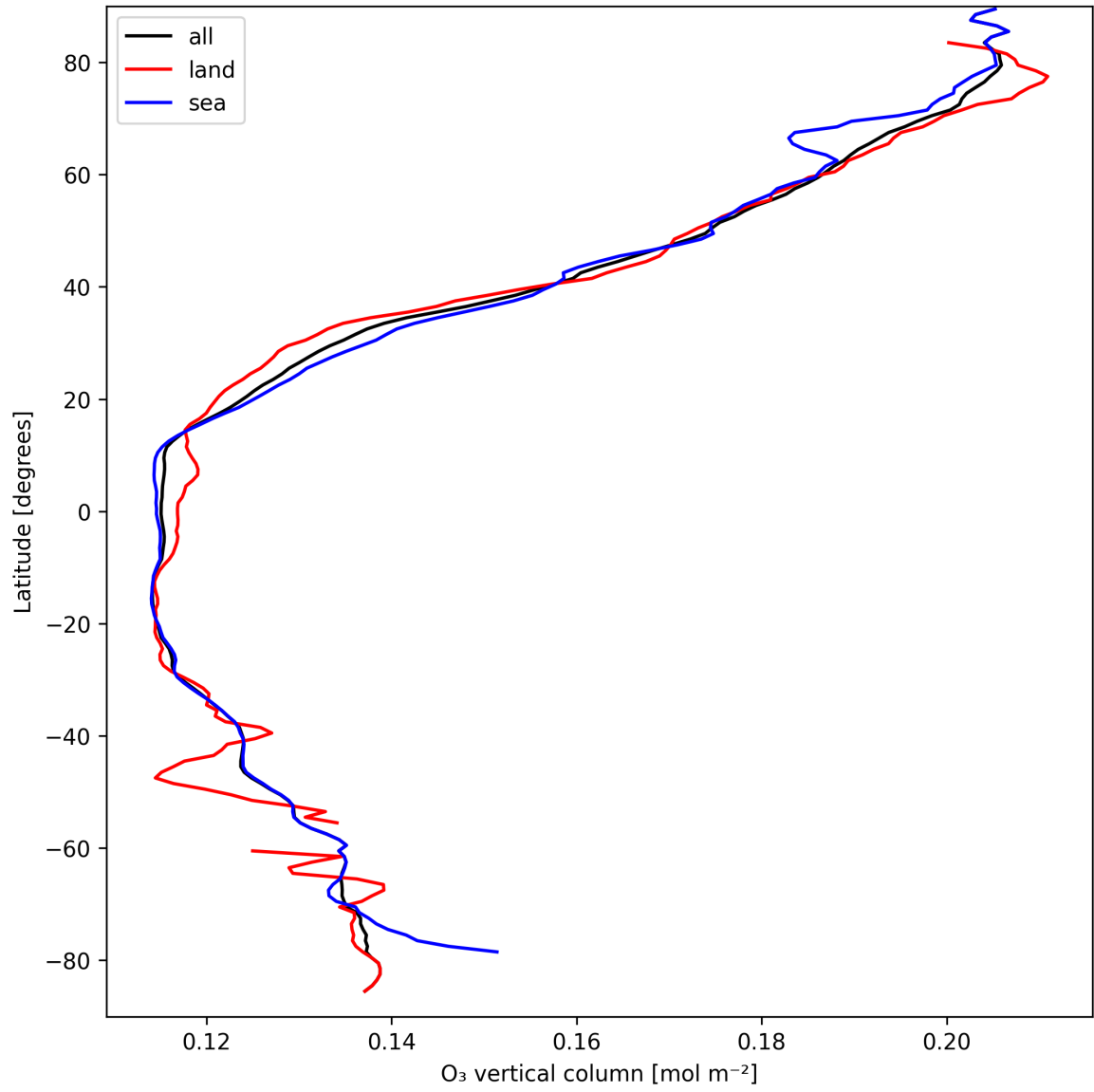
Figure 17: Zonal average of “O 3 vertical column” for 2025-03-28 to 2025-03-29.
