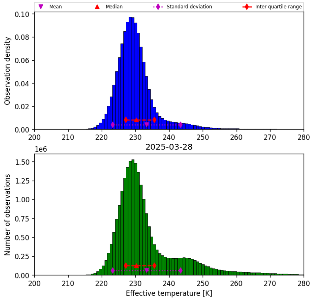
Figure 38: Histogram of “Effective temperature” for 2025-03-28 to 2025-03-29
