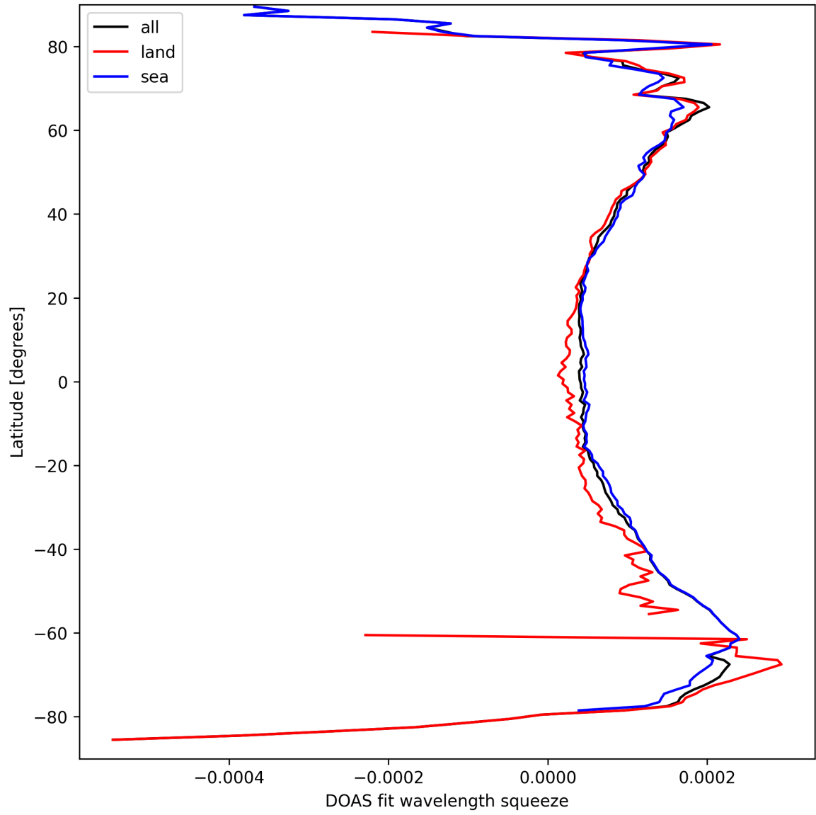
Figure 24: Zonal average of “DOAS fit wavelength squeeze” for 2025-03-28 to 2025-03-29.
