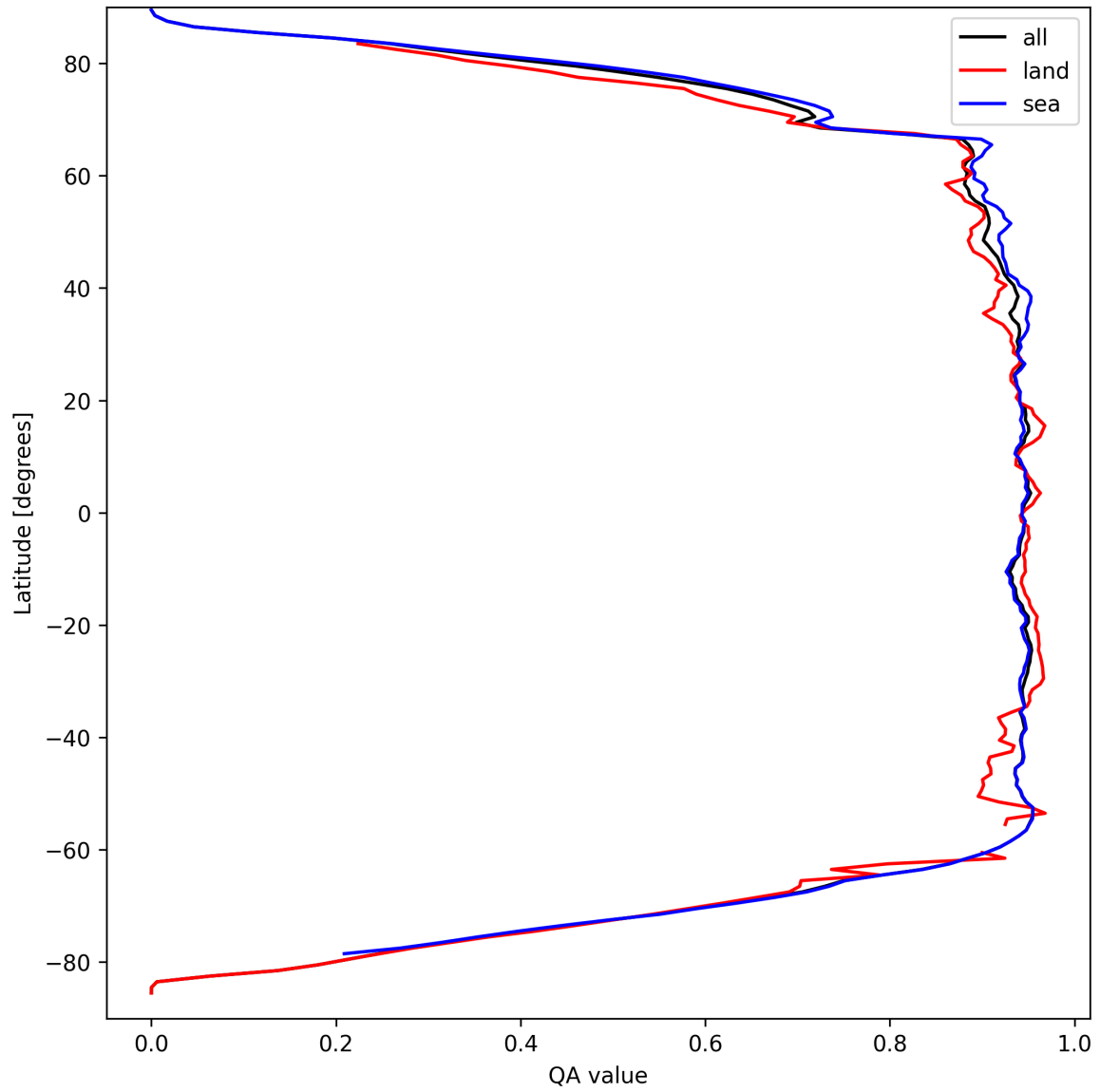
Figure 16: Zonal average of “QA value” for 2025-03-28 to 2025-03-29.
