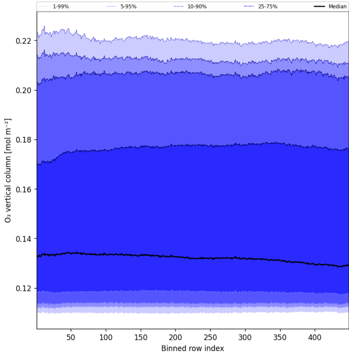
Figure 41: Along track statistics of "O 3 vertical column" for 2025-03-28 to 2025-03-29
