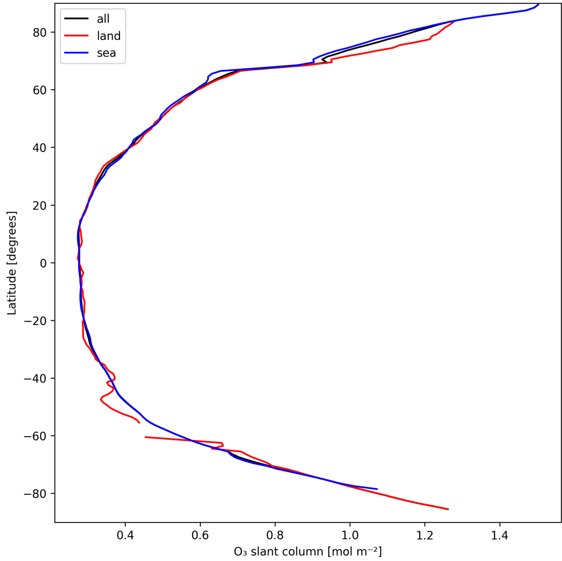
Figure 19: Zonal average of “O 3 slant column” for 2025-03-28 to 2025-03-29.
