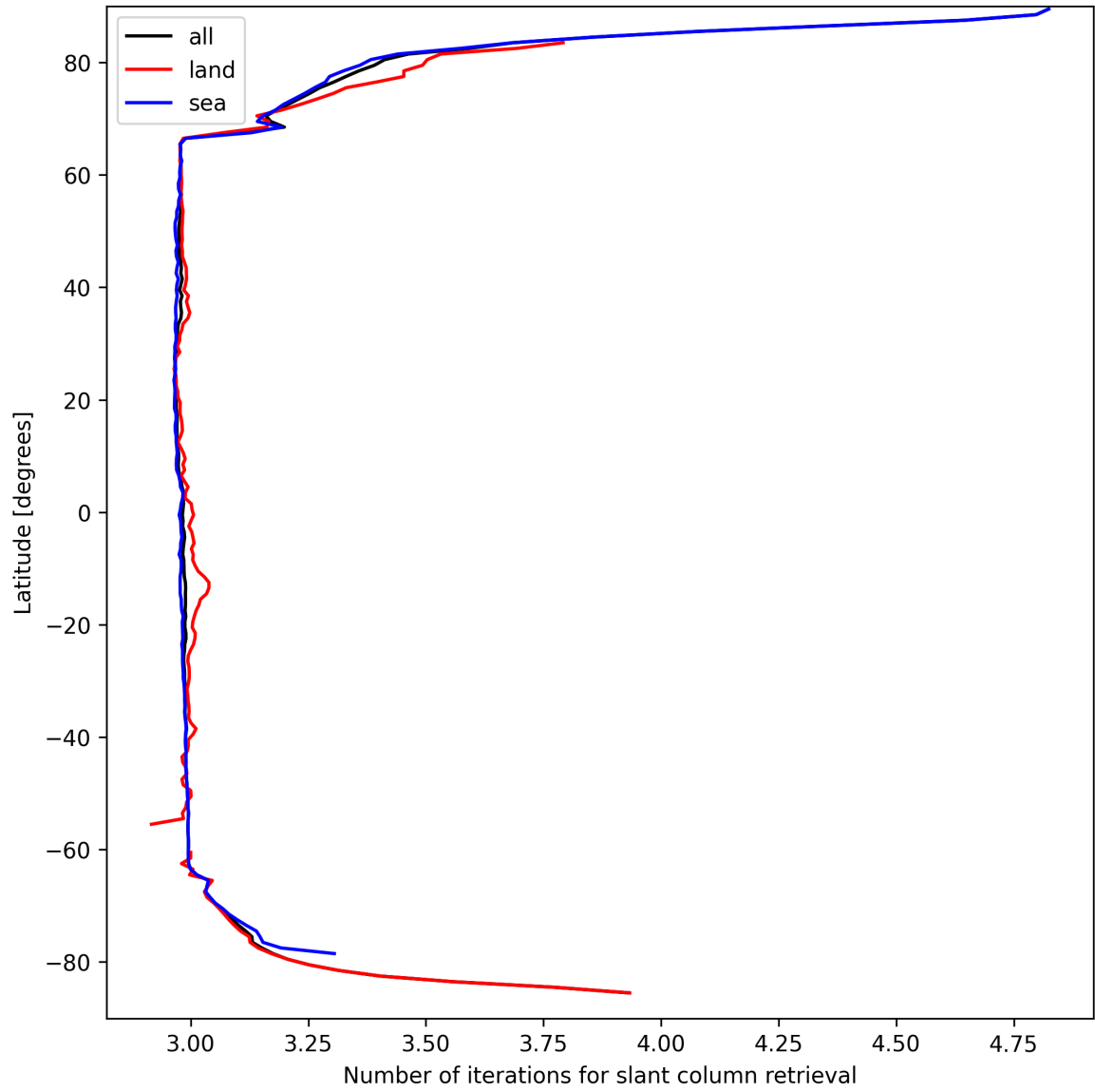
Figure 21: Zonal average of “Number of iterations for slant column retrieval” for 2025-03-28 to 2025-03-29.
