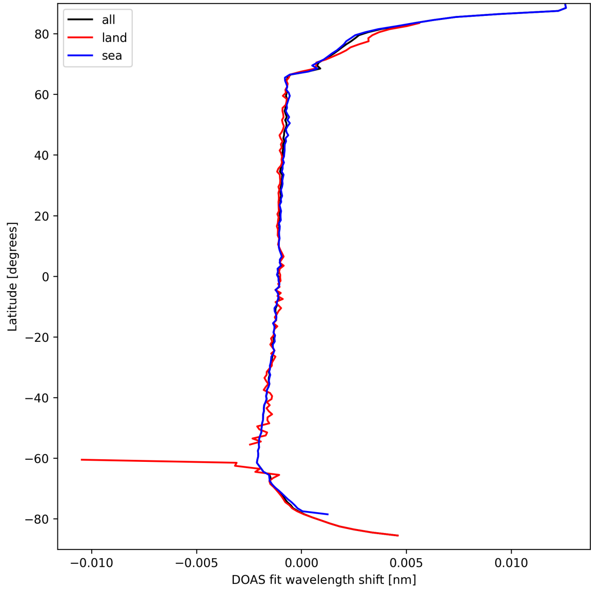
Figure 23: Zonal average of “DOAS fit wavelength shift” for 2025-03-28 to 2025-03-29.
