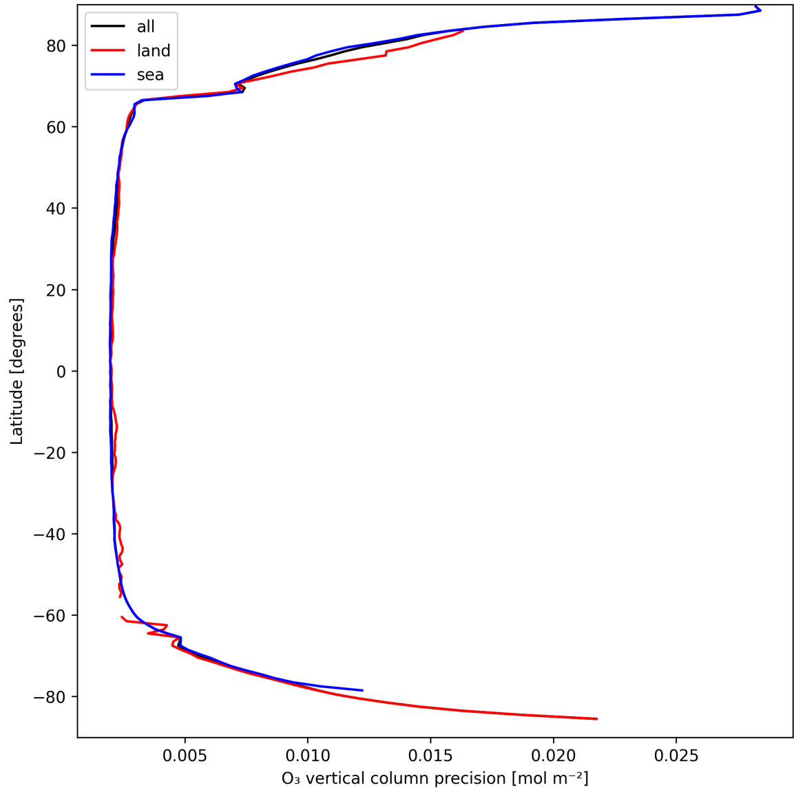
Figure 18: Zonal average of “O 3 vertical column precision” for 2025-03-28 to 2025-03-29.
