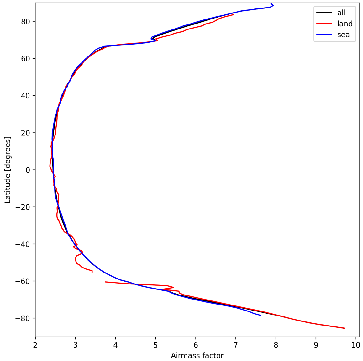
Figure 25: Zonal average of “Airmass factor” for 2025-03-28 to 2025-03-29.
