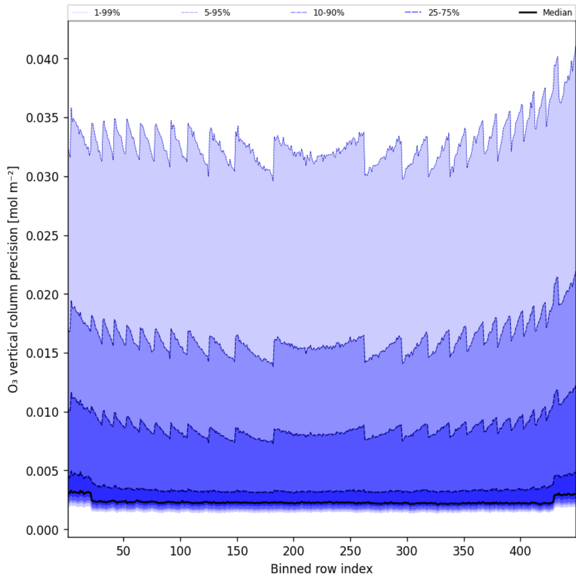
Figure 42: Along track statistics of “O 3 vertical column precision” for 2025-03-28 to 2025-03-29
