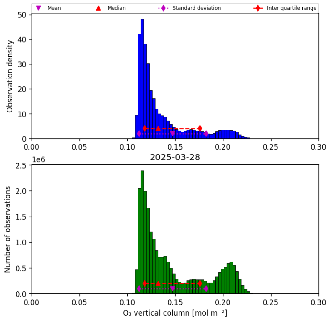
Figure 29: Histogram of “O 3 vertical column” for 2025-03-28 to 2025-03-29
