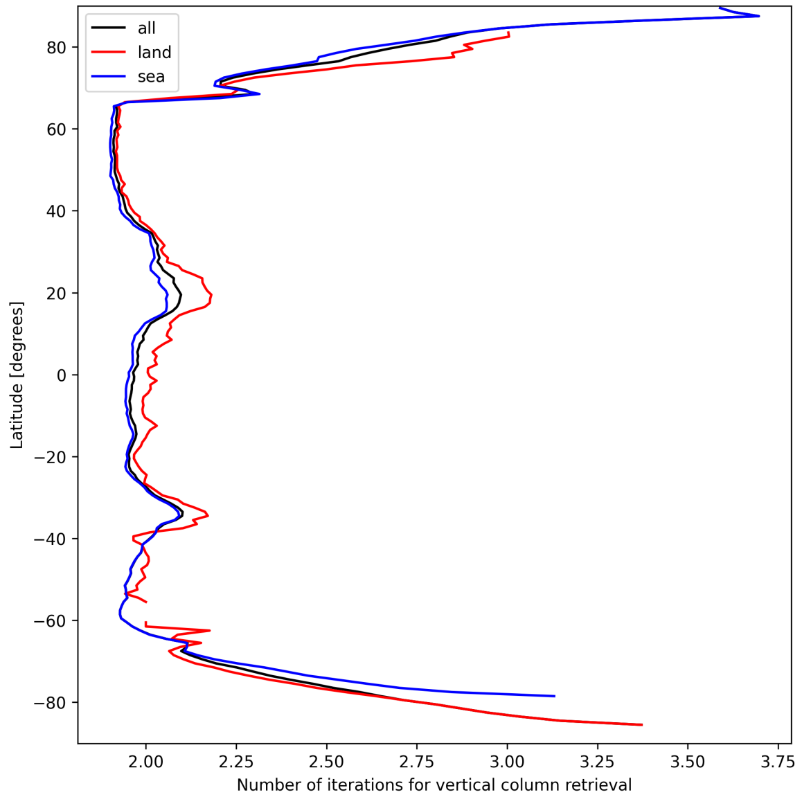
Figure 27: Zonal average of “Number of iterations for vertical column retrieval” for 2025-03-28 to 2025-03-29.
