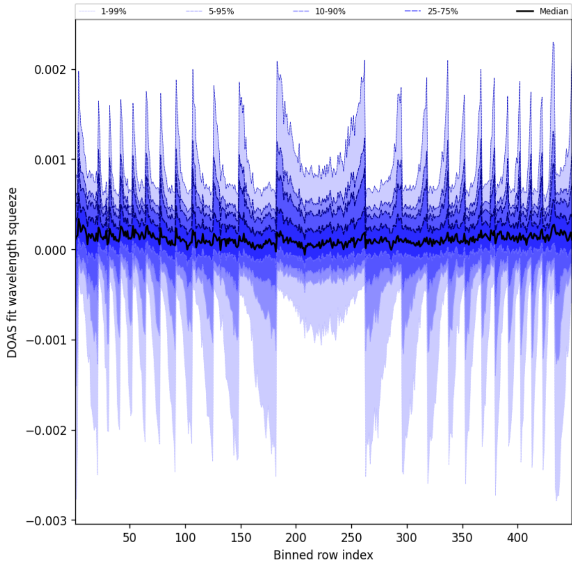
Figure 48: Along track statistics of “DOAS fit wavelength squeeze” for 2025-03-28 to 2025-03-29
