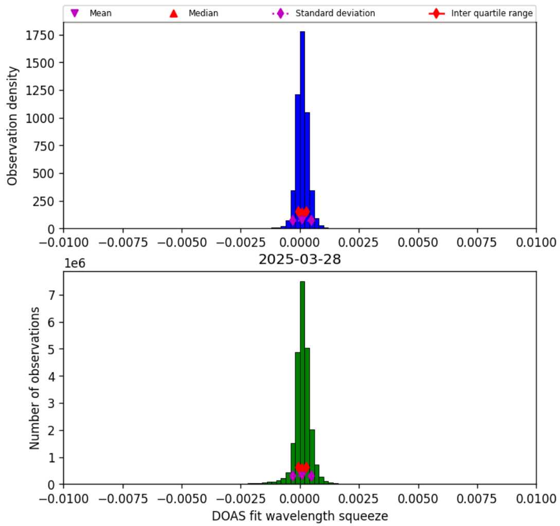
Figure 36: Histogram of “DOAS fit wavelength squeeze” for 2025-03-28 to 2025-03-29
