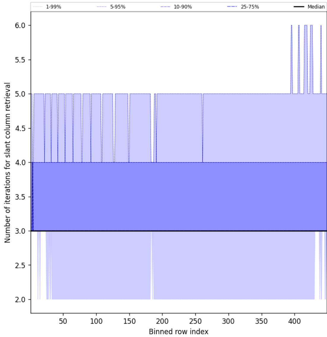
Figure 45: Along track statistics of “Number of iterations for slant column retrieval” for 2025-03-28 to 2025-03-29
