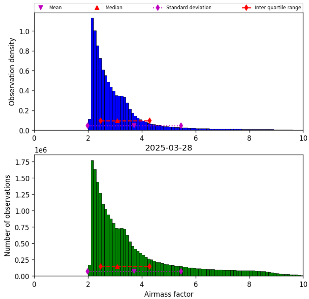
Figure 37: Histogram of “Airmass factor” for 2025-03-28 to 2025-03-29
