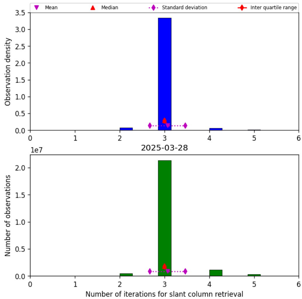
Figure 33: Histogram of “Number of iterations for slant column retrieval” for 2025-03-28 to 2025-03-29
