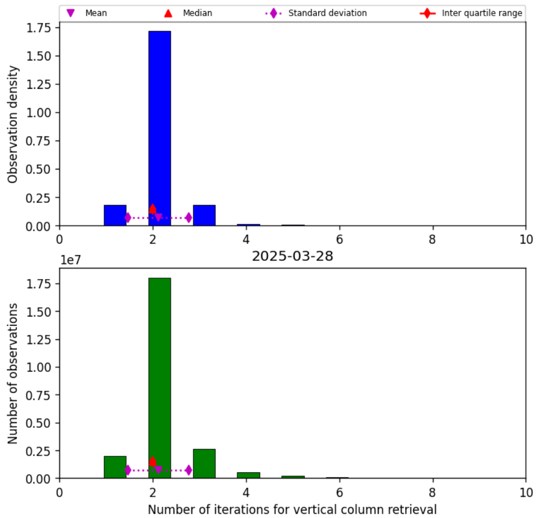
Figure 39: Histogram of “Number of iterations for vertical column retrieval” for 2025-03-28 to 2025-03-29
