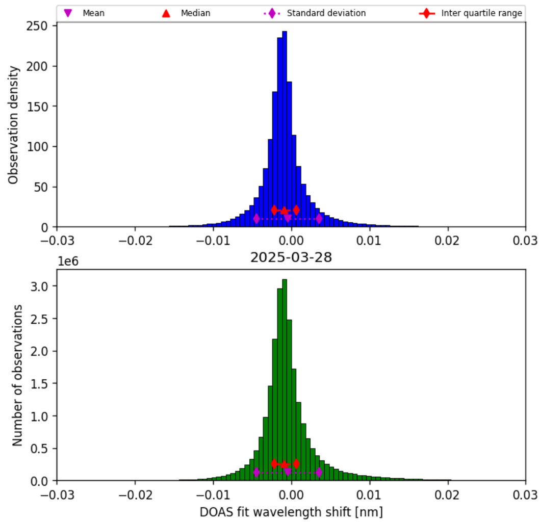
Figure 35: Histogram of “DOAS fit wavelength shift” for 2025-03-28 to 2025-03-29
