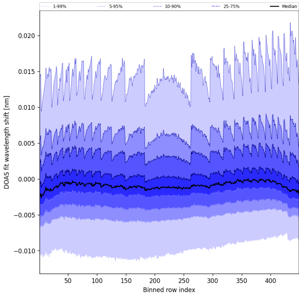
Figure 47: Along track statistics of “DOAS fit wavelength shift” for 2025-03-28 to 2025-03-29
