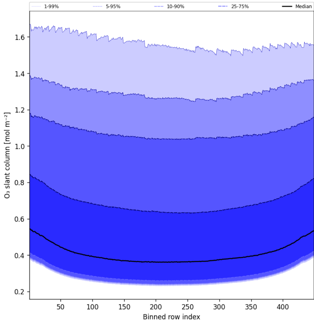
Figure 43: Along track statistics of "O 3 slant column" for 2025-03-28 to 2025-03-29
