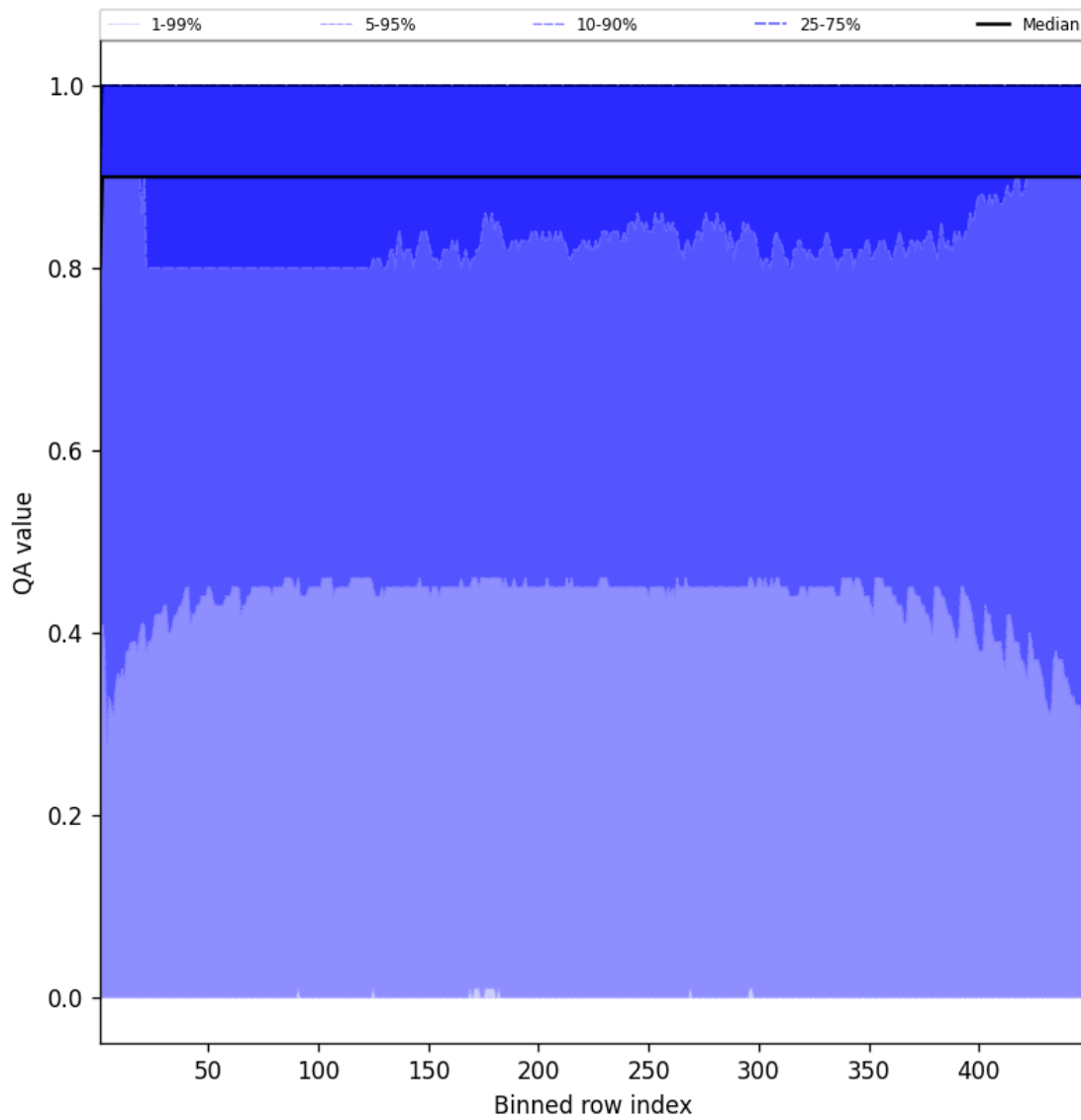
Figure 40: Along track statistics of “QA value” for 2025-03-28 to 2025-03-29
