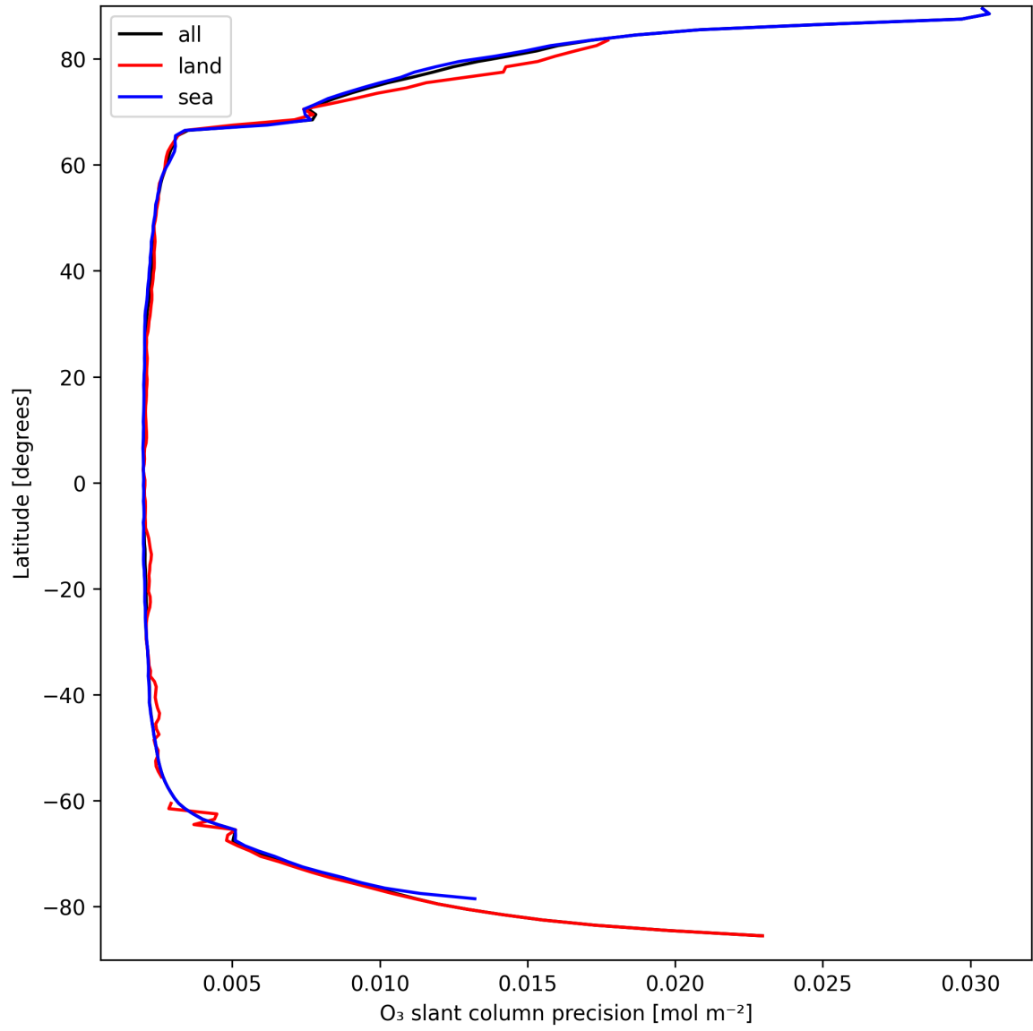
Figure 20: Zonal average of "O 3 slant column precision" for 2025-03-28 to 2025-03-29.
