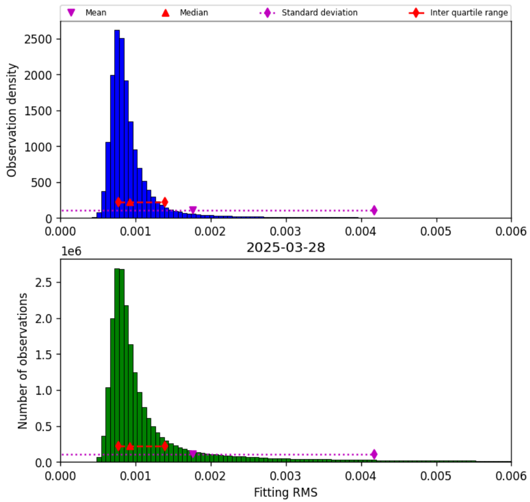
Figure 34: Histogram of “Fitting RMS” for 2025-03-28 to 2025-03-29
