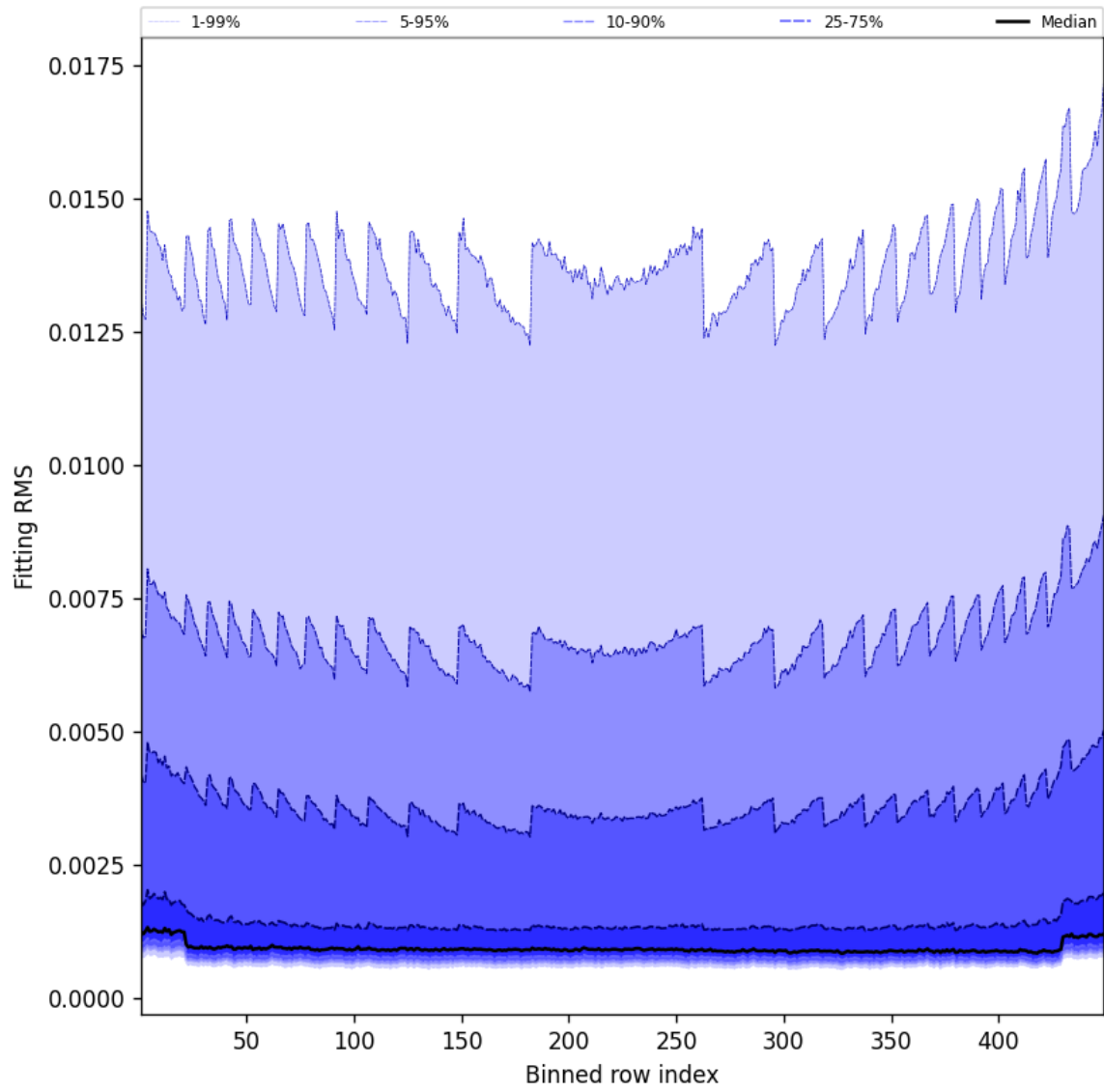
Figure 46: Along track statistics of “Fitting RMS” for 2025-03-28 to 2025-03-29
