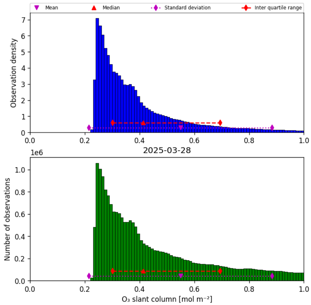
Figure 31: Histogram of “O 3 slant column” for 2025-03-28 to 2025-03-29
