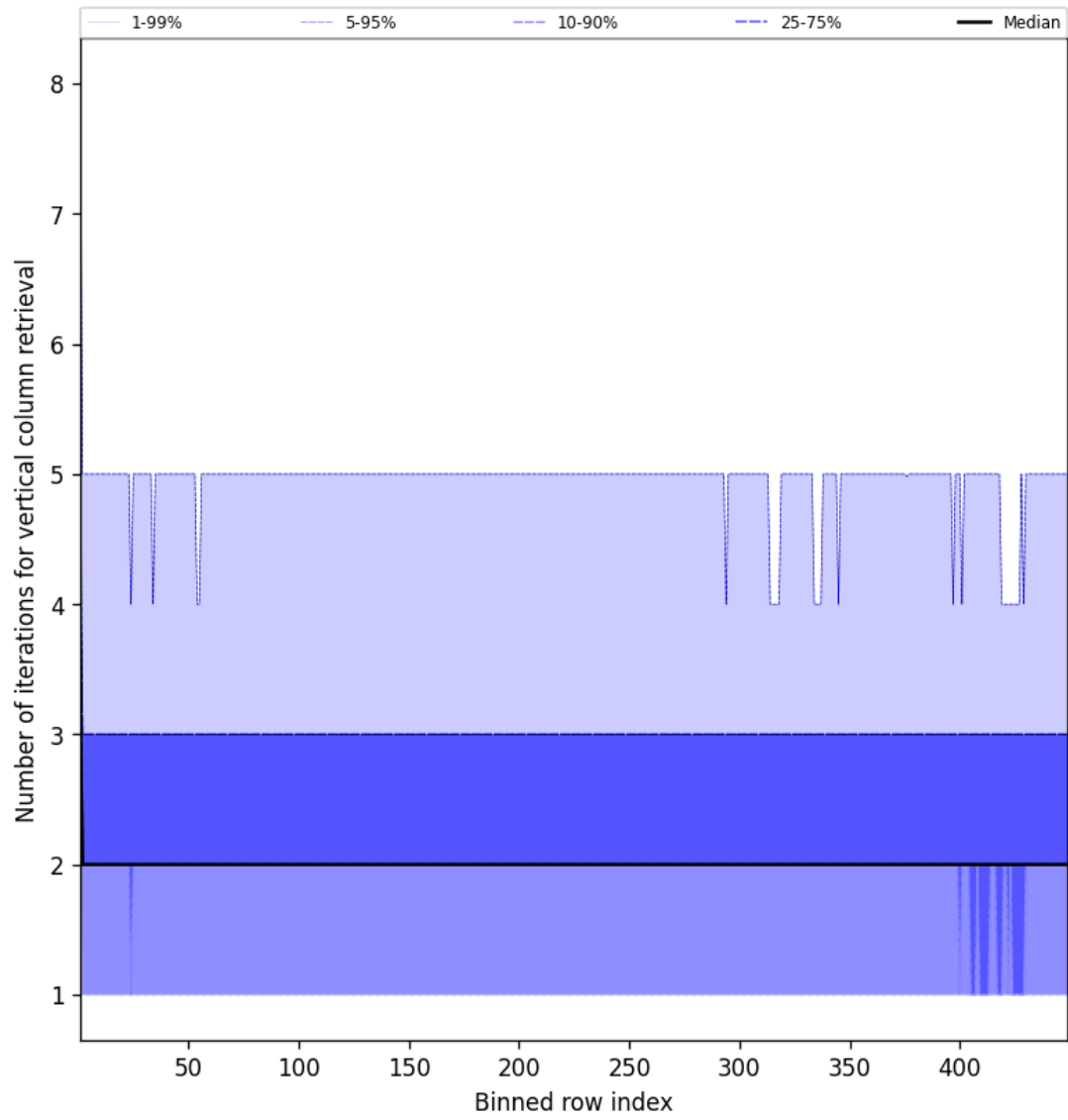
Figure 51: Along track statistics of “Number of iterations for vertical column retrieval” for 2025-03-28 to 2025-03-29
