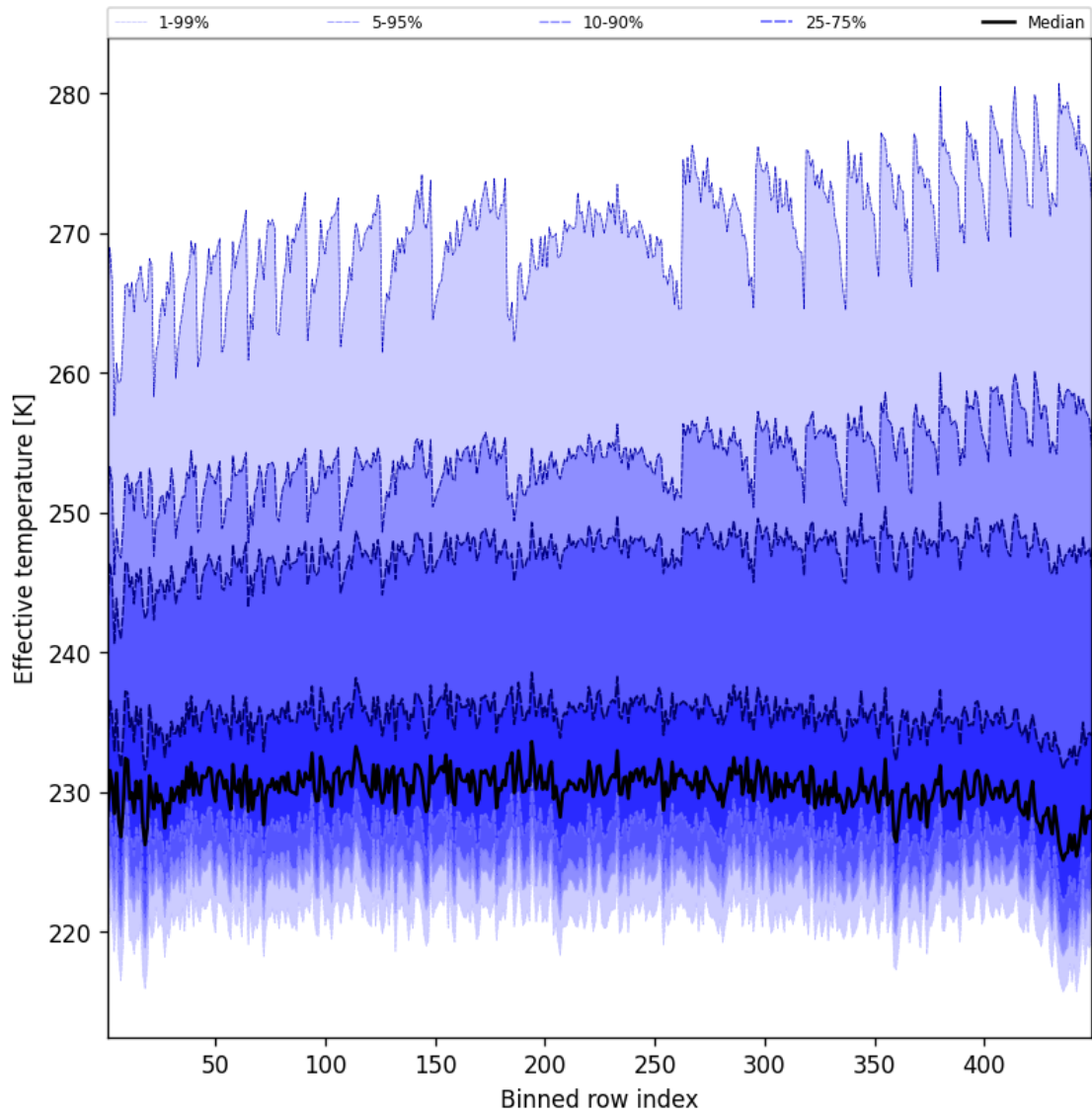
Figure 50: Along track statistics of “Effective temperature” for 2025-03-28 to 2025-03-29
