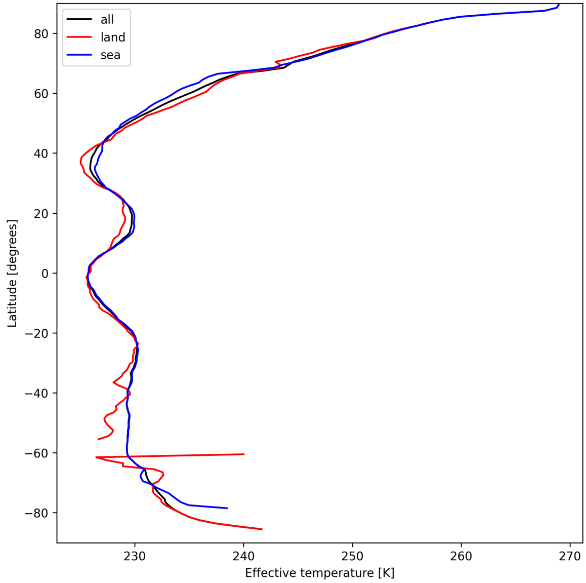
Figure 26: Zonal average of “Effective temperature” for 2025-03-28 to 2025-03-29.
