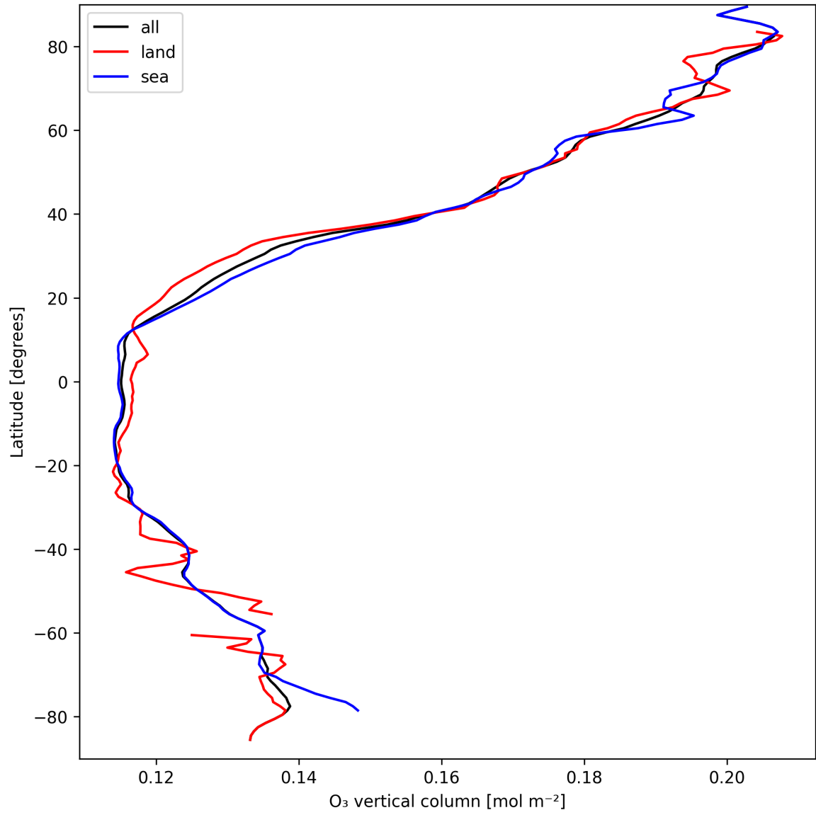
Figure 17: Zonal average of “O 3 vertical column” for 2025-03-29 to 2025-03-30.
