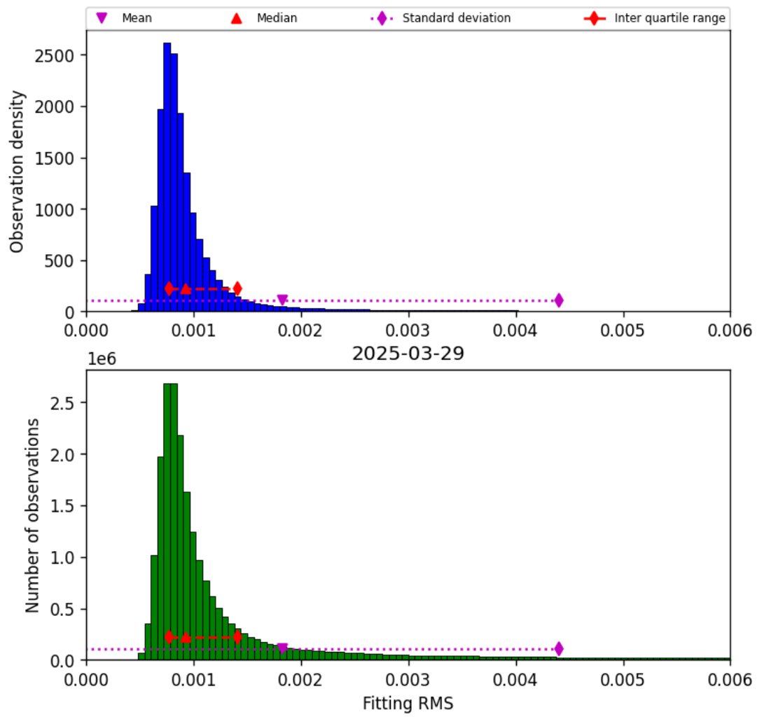
Figure 34: Histogram of “Fitting RMS” for 2025-03-29 to 2025-03-30
