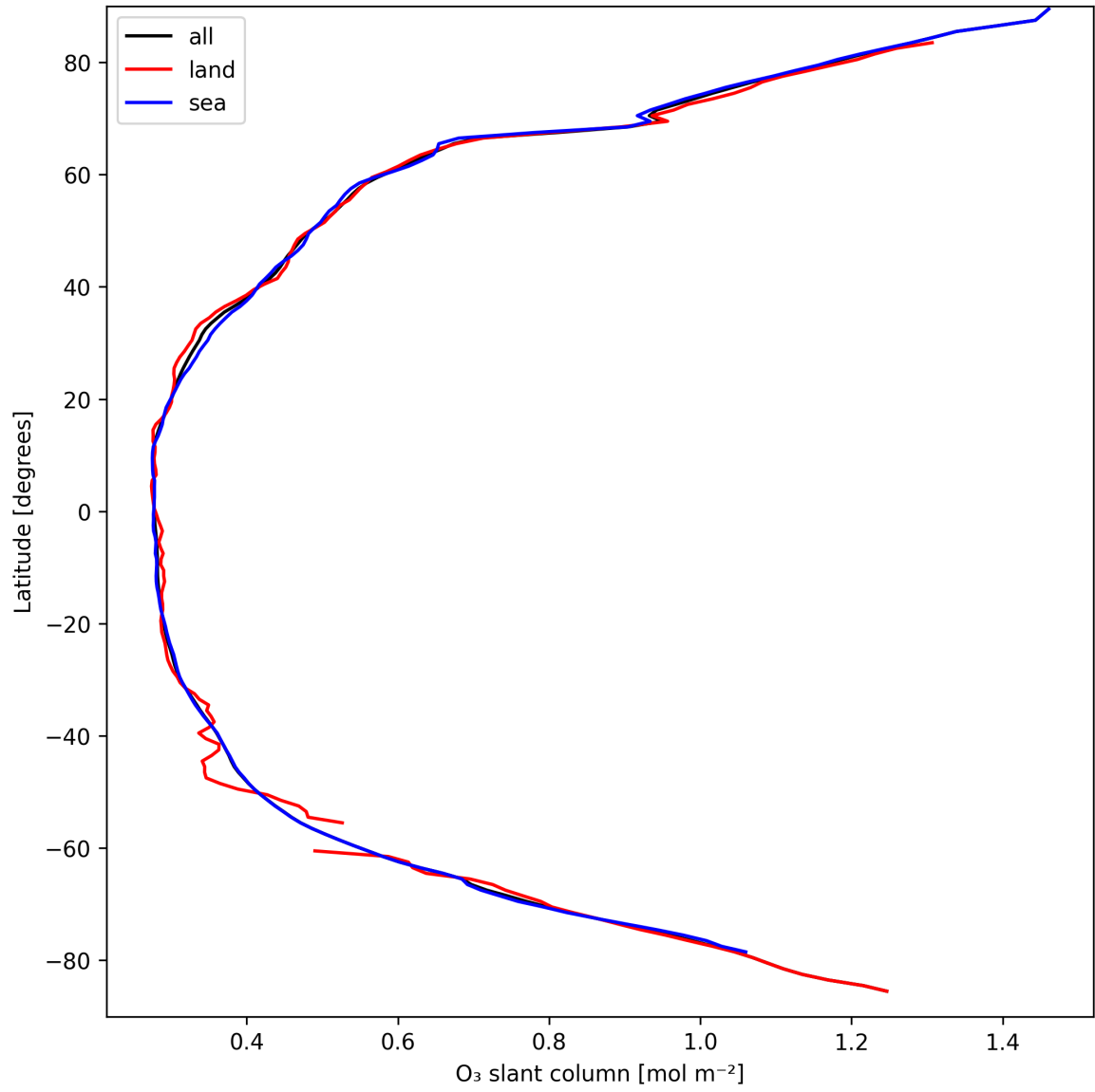
Figure 19: Zonal average of “O 3 slant column” for 2025-03-29 to 2025-03-30.
