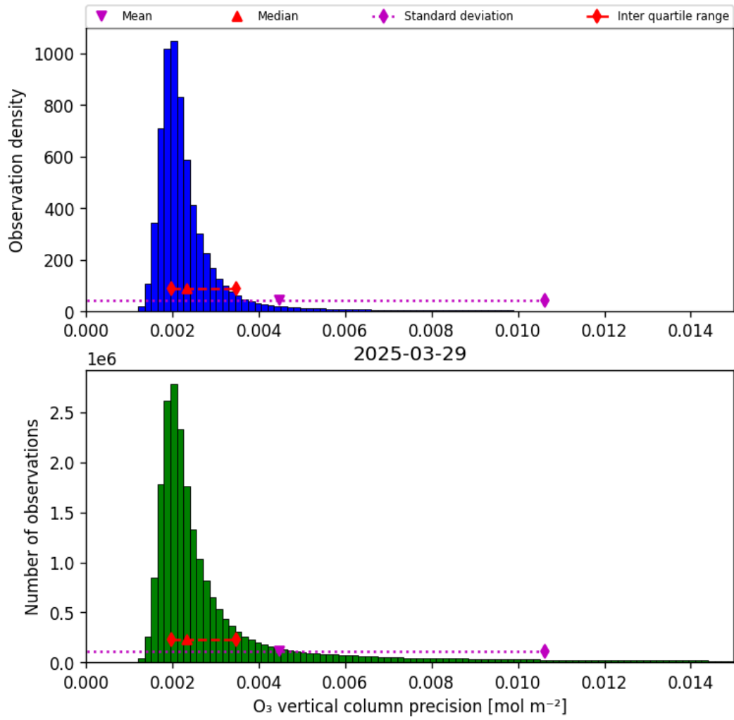
Figure 30: Histogram of “O 3 vertical column precision” for 2025-03-29 to 2025-03-30
