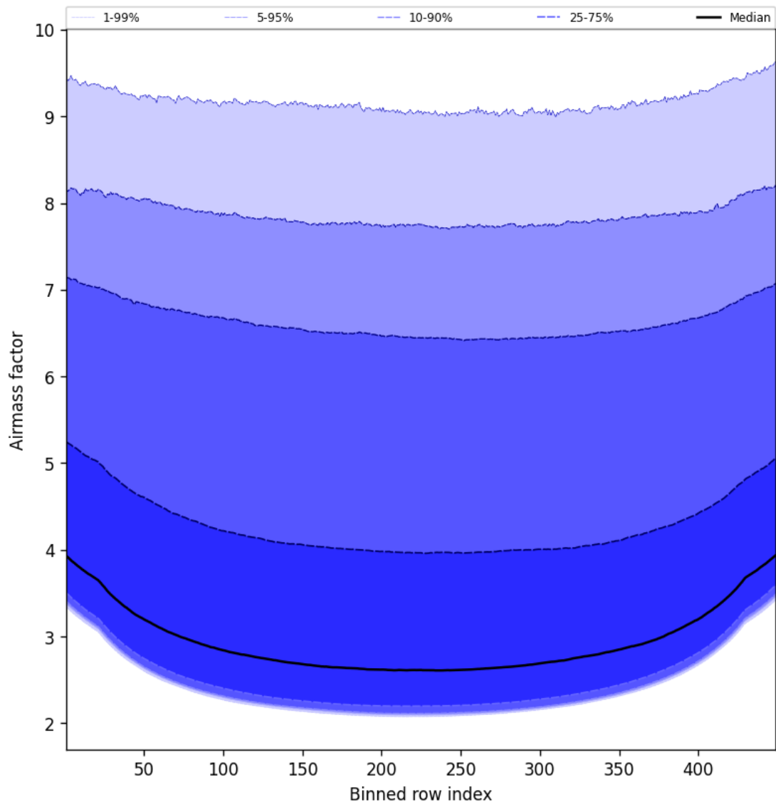
Figure 49: Along track statistics of “Airmass factor” for 2025-03-29 to 2025-03-30
