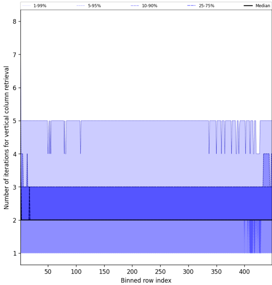
Figure 51: Along track statistics of “Number of iterations for vertical column retrieval” for 2025-03-29 to 2025-03-30
