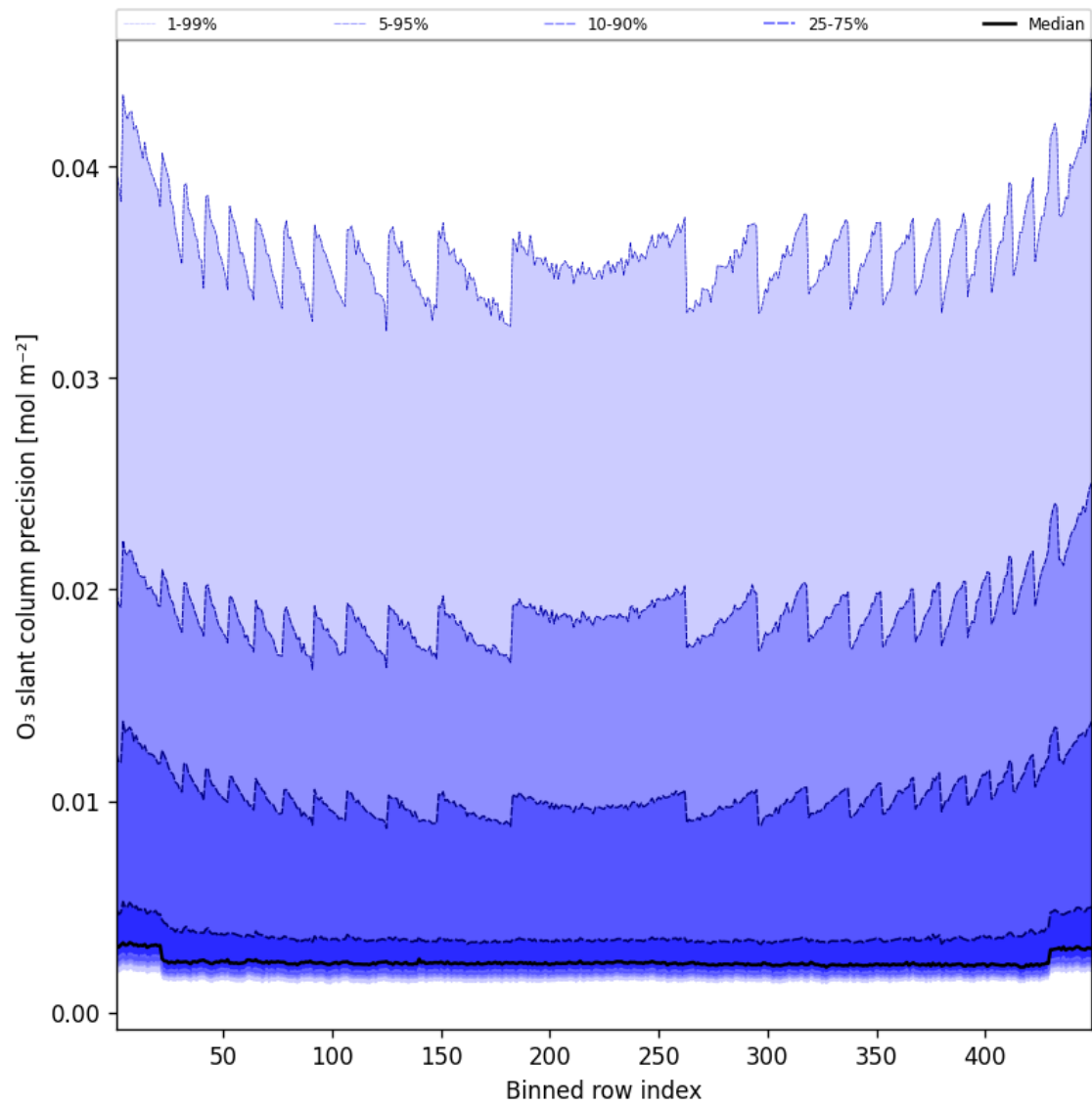
Figure 44: Along track statistics of “O 3 slant column precision” for 2025-03-29 to 2025-03-30
