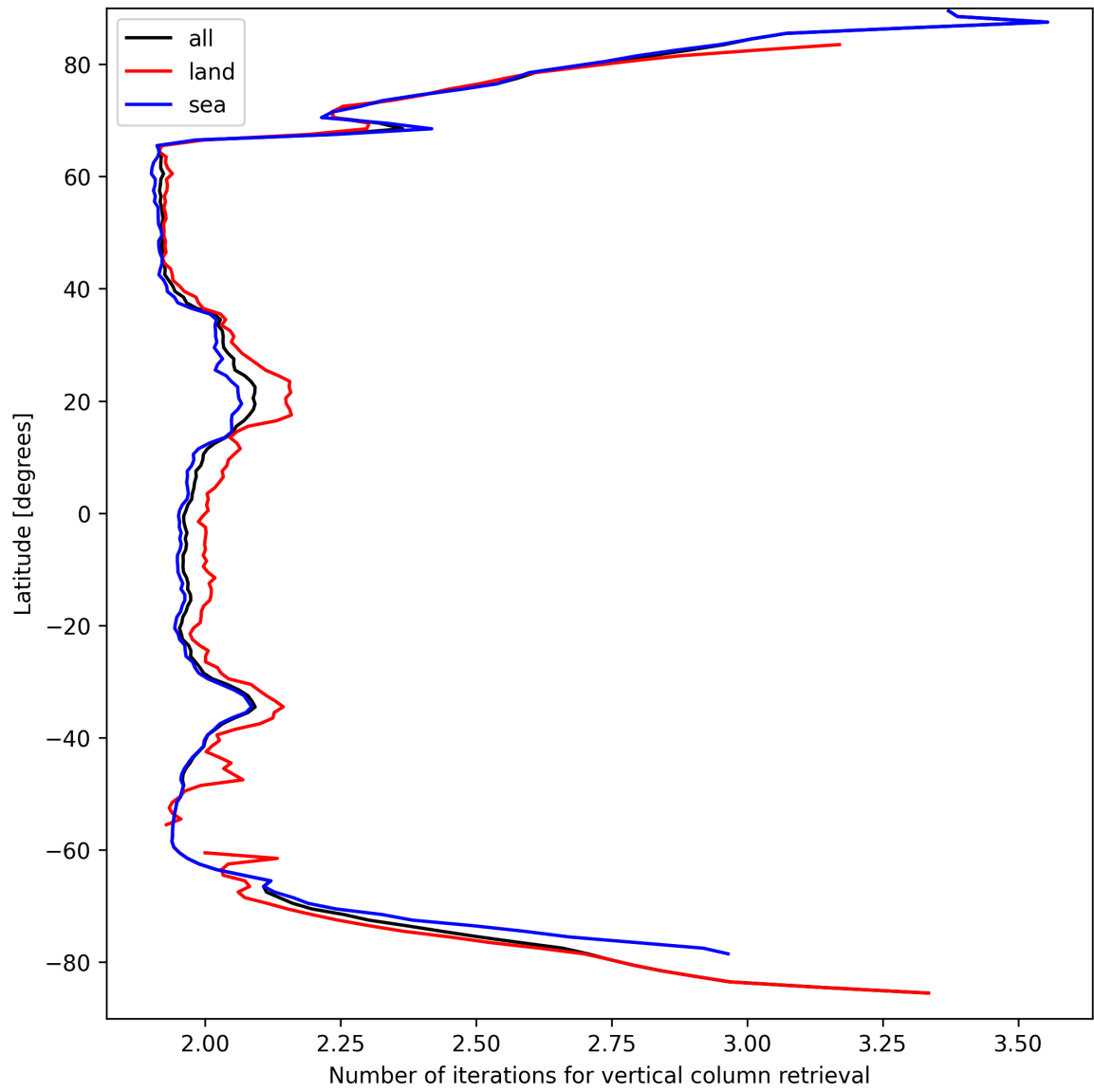
Figure 27: Zonal average of “Number of iterations for vertical column retrieval” for 2025-03-29 to 2025-03-30.
