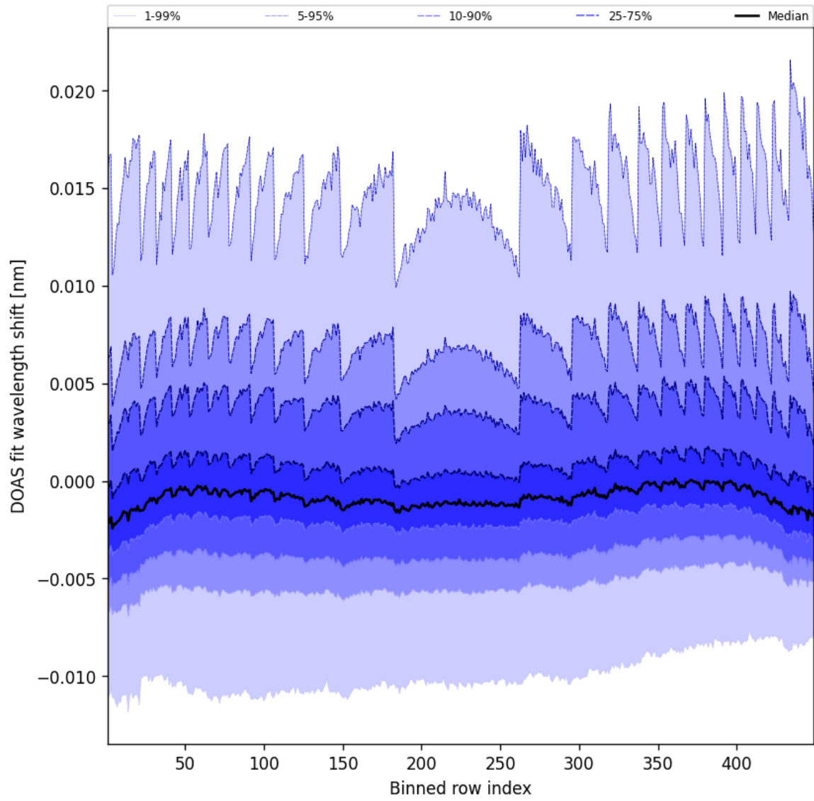
Figure 47: Along track statistics of “DOAS fit wavelength shift” for 2025-03-29 to 2025-03-30
