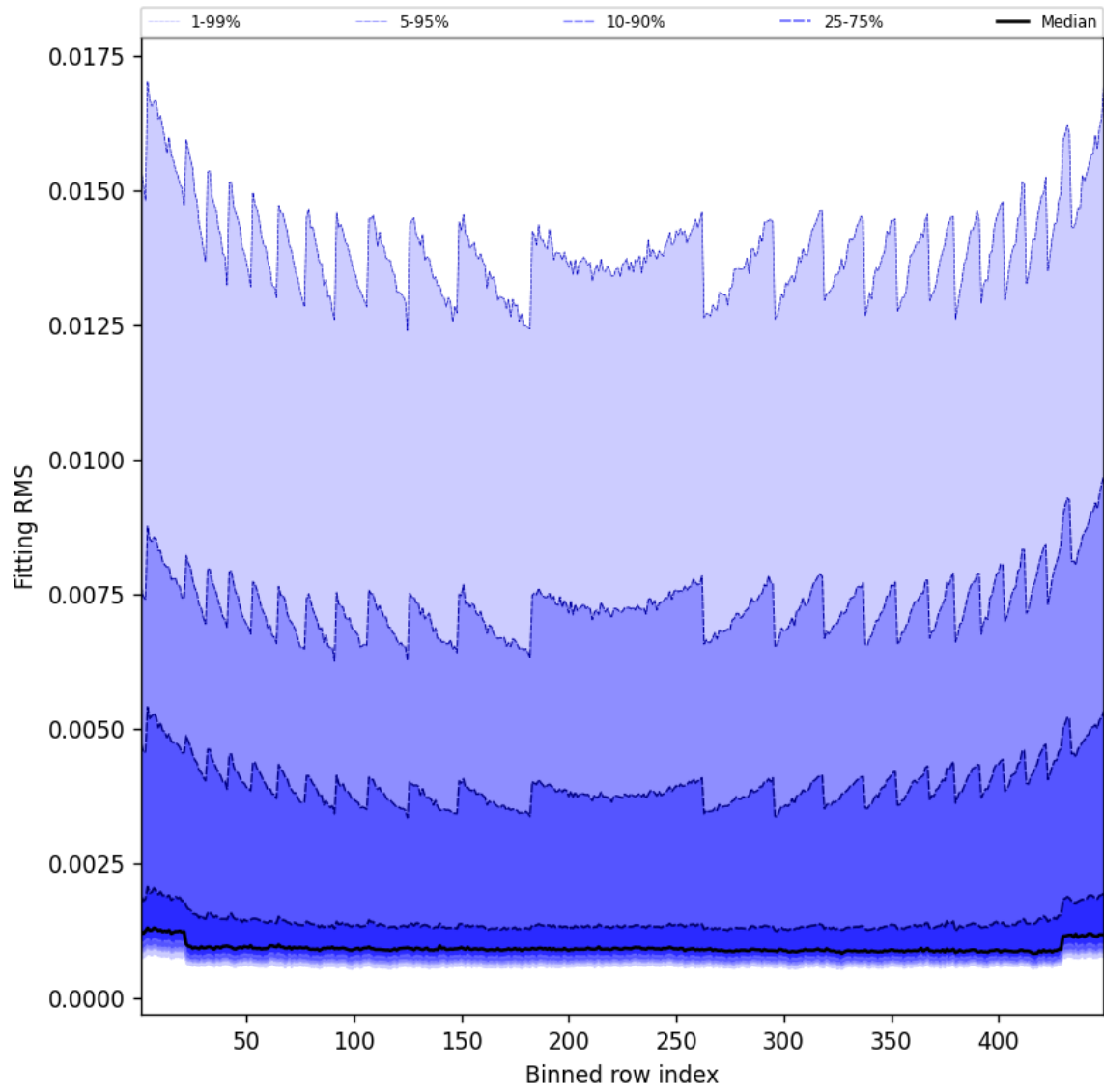
Figure 46: Along track statistics of “Fitting RMS” for 2025-03-29 to 2025-03-30
