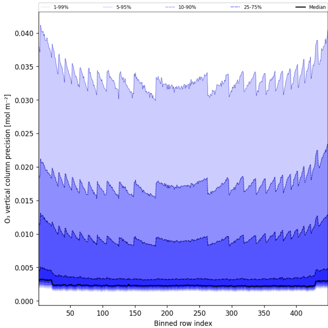
Figure 42: Along track statistics of “O 3 vertical column precision” for 2025-03-29 to 2025-03-30
