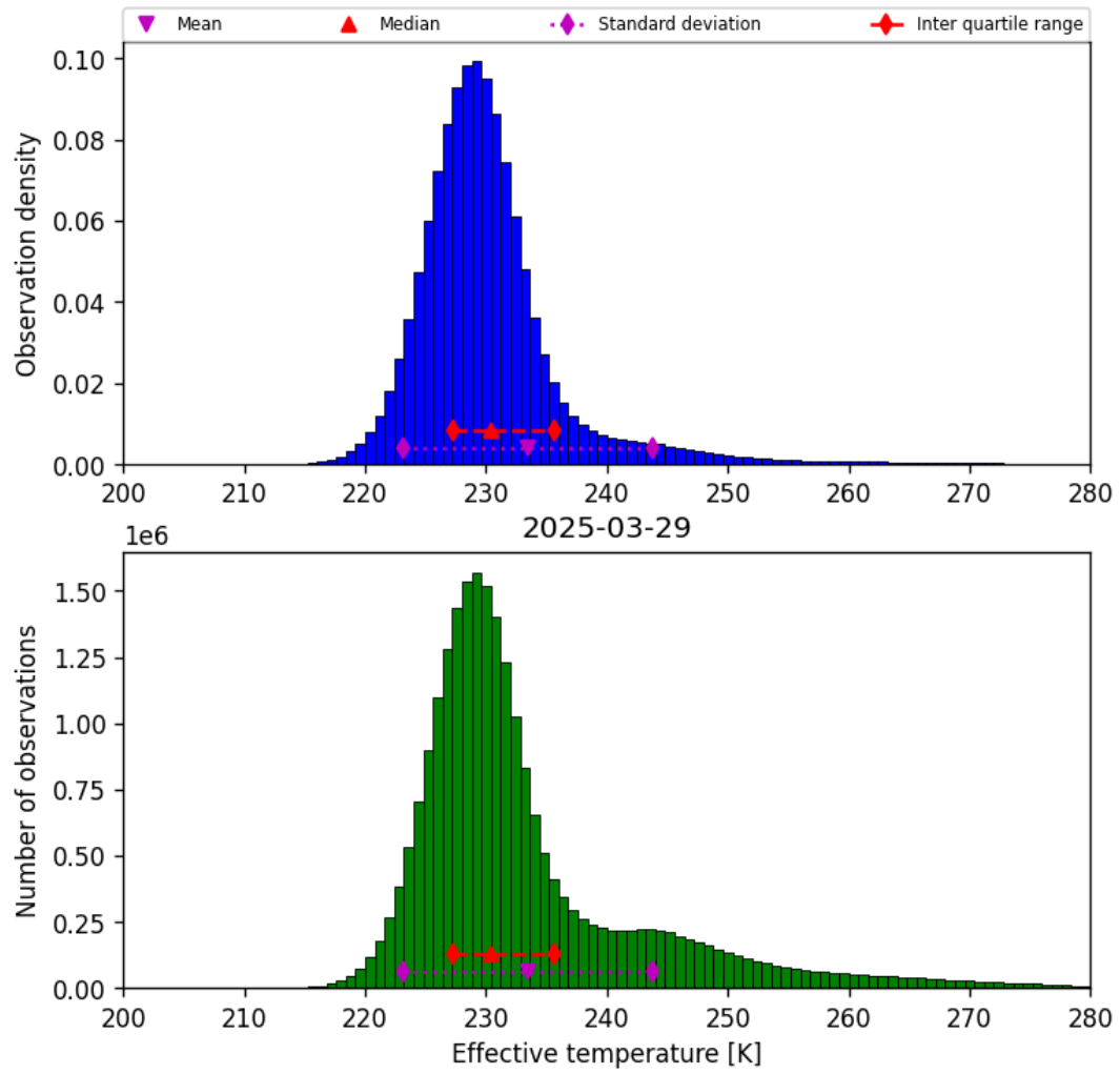
Figure 38: Histogram of “Effective temperature” for 2025-03-29 to 2025-03-30
