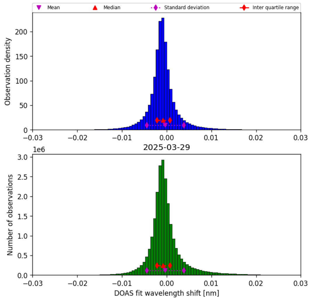
Figure 35: Histogram of “DOAS fit wavelength shift” for 2025-03-29 to 2025-03-30
