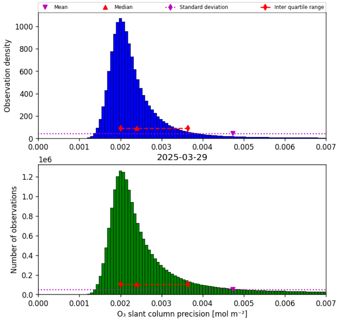
Figure 32: Histogram of “O 3 slant column precision” for 2025-03-29 to 2025-03-30
