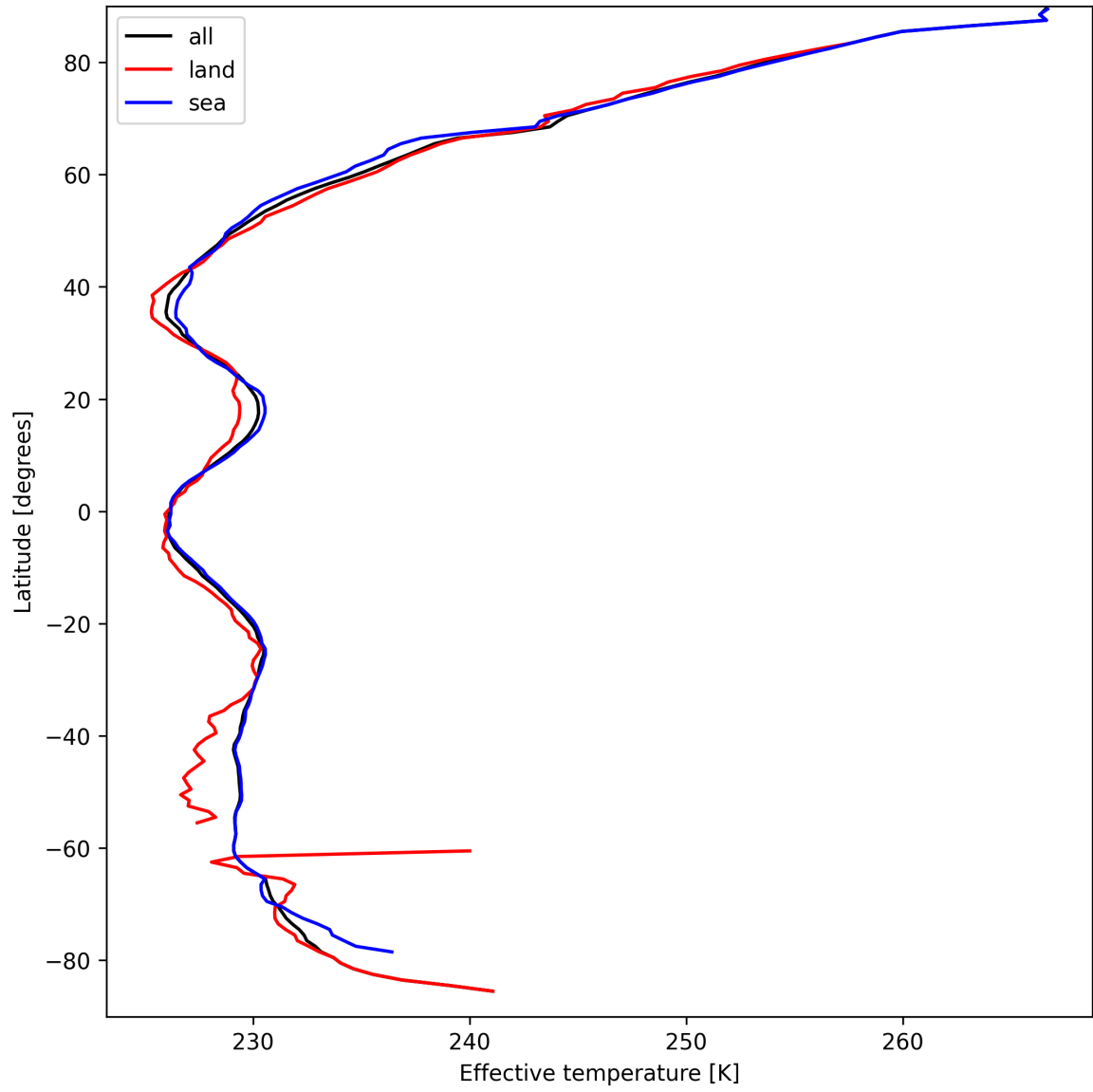
Figure 26: Zonal average of “Effective temperature” for 2025-03-29 to 2025-03-30.
