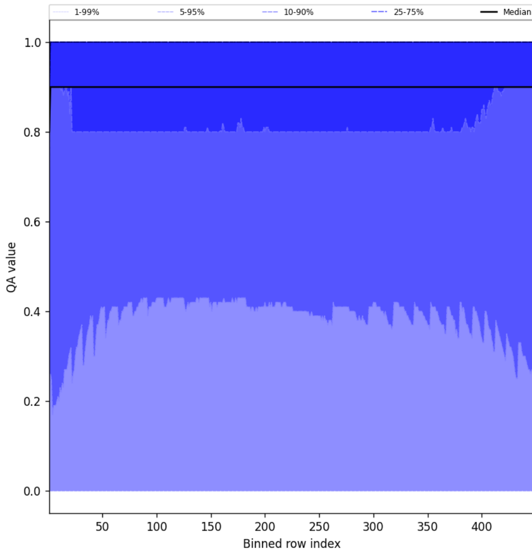
Figure 40: Along track statistics of “QA value” for 2025-03-29 to 2025-03-30
