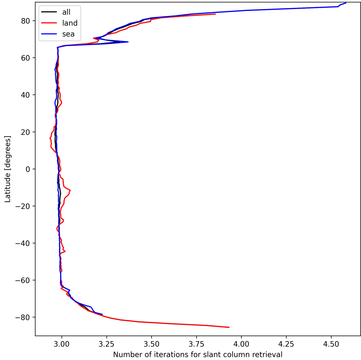
Figure 21: Zonal average of “Number of iterations for slant column retrieval” for 2025-03-29 to 2025-03-30.
