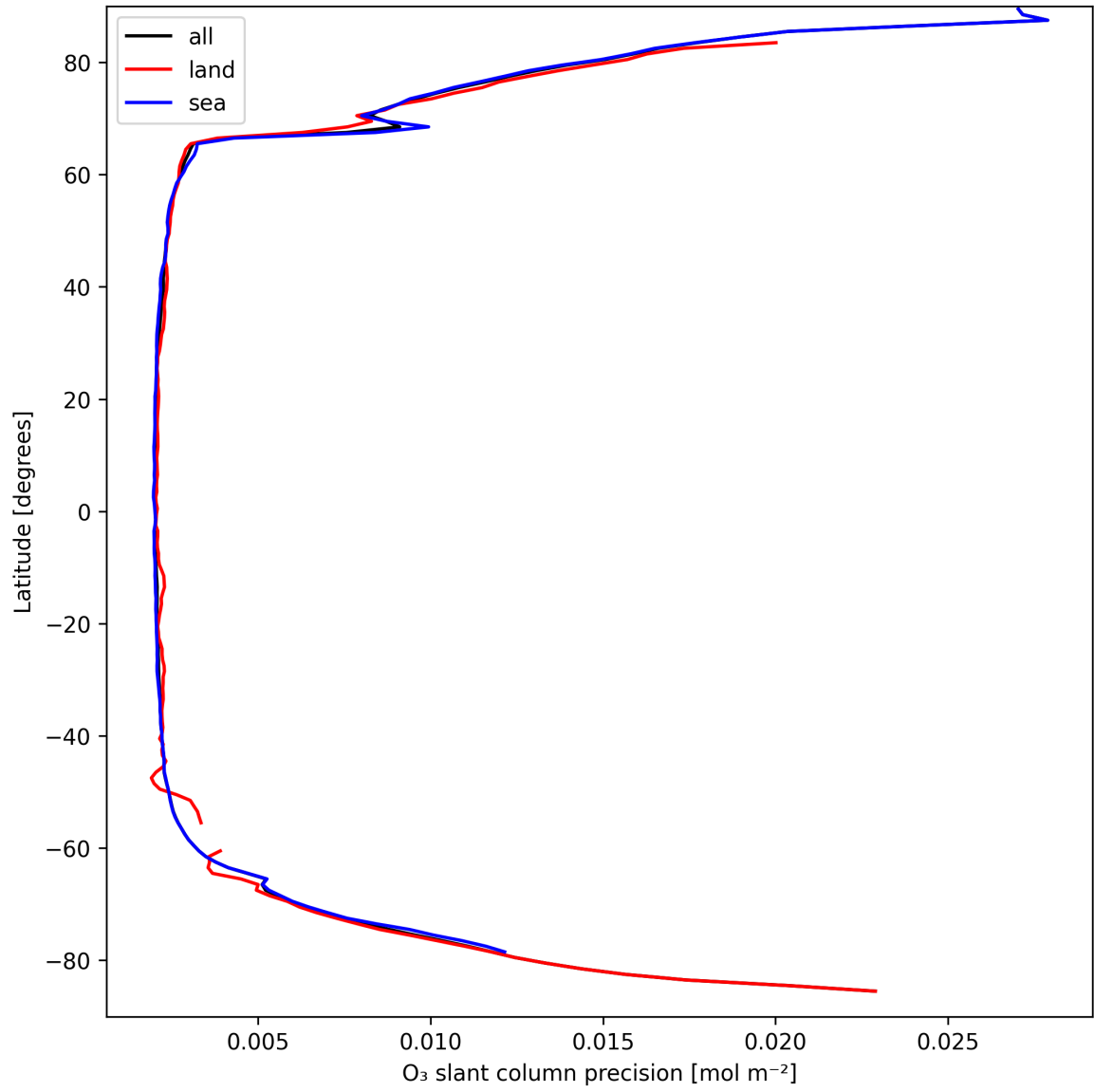
Figure 20: Zonal average of "O 3 slant column precision" for 2025-03-29 to 2025-03-30.
