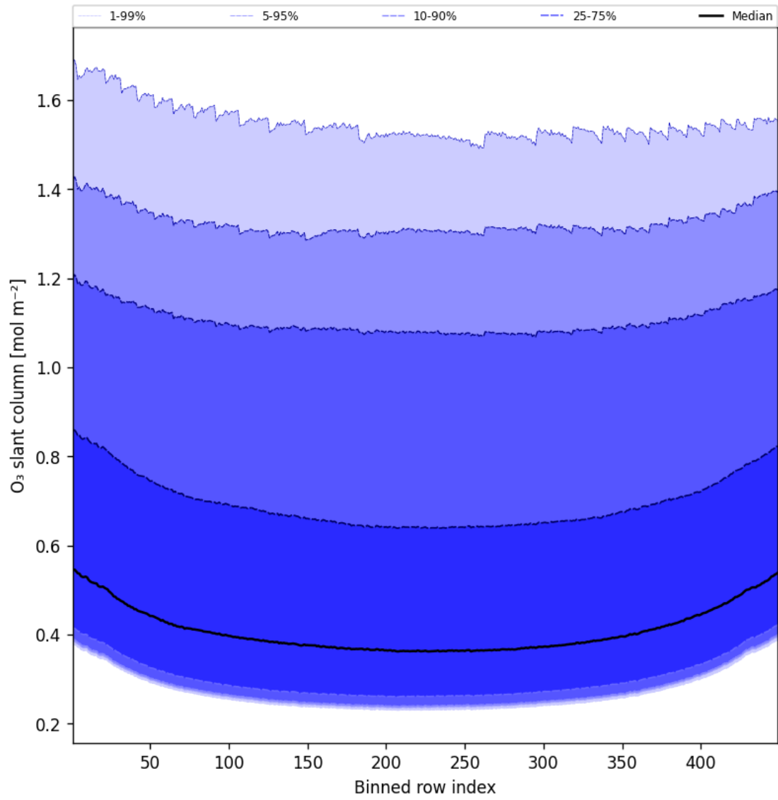
Figure 43: Along track statistics of “O 3 slant column” for 2025-03-29 to 2025-03-30
