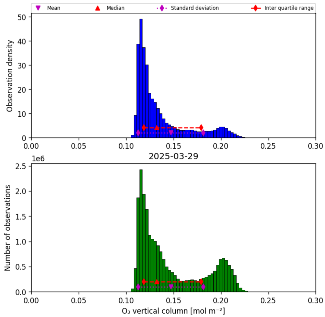
Figure 29: Histogram of “O 3 vertical column” for 2025-03-29 to 2025-03-30
