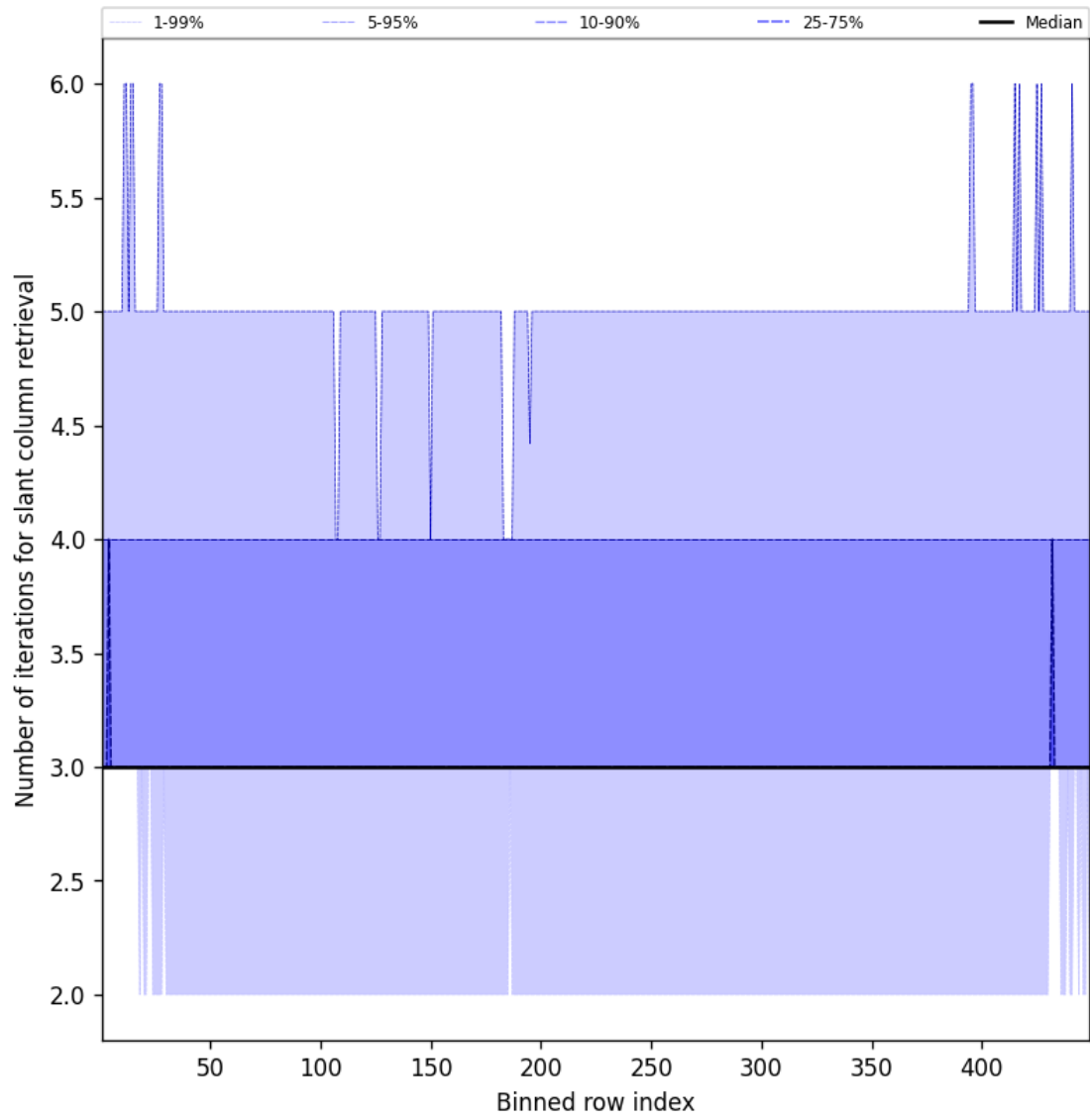
Figure 45: Along track statistics of “Number of iterations for slant column retrieval” for 2025-03-29 to 2025-03-30
