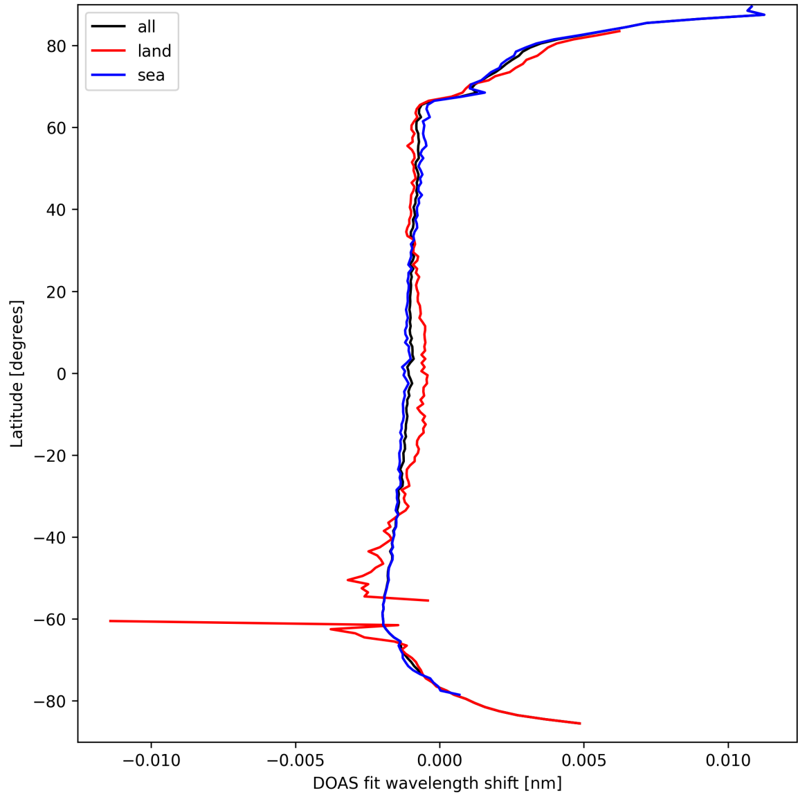
Figure 23: Zonal average of “DOAS fit wavelength shift” for 2025-03-29 to 2025-03-30.
