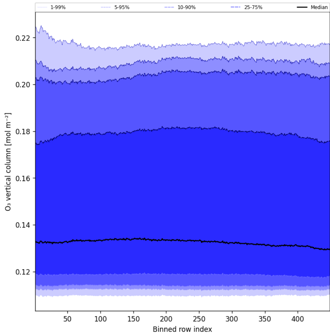
Figure 41: Along track statistics of “O 3 vertical column” for 2025-03-29 to 2025-03-30
