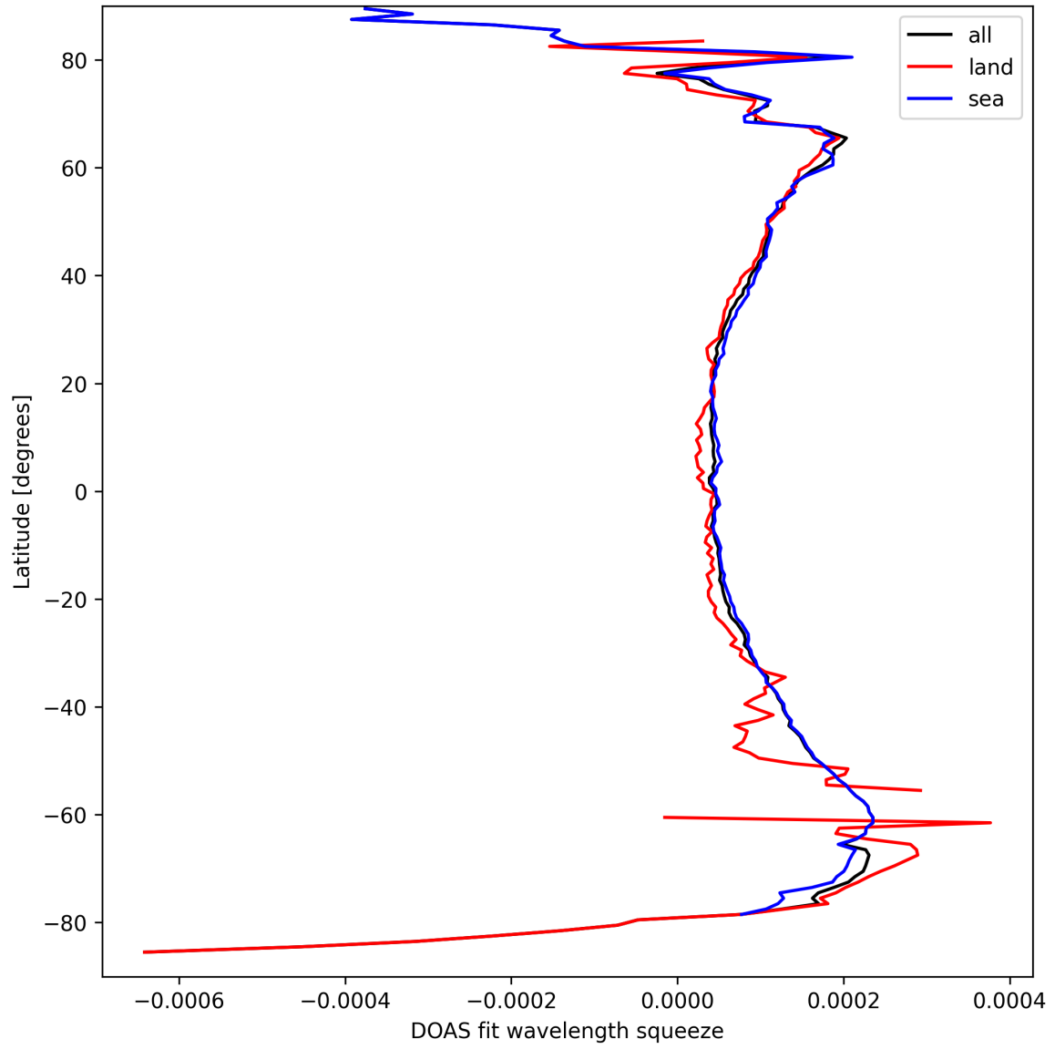
Figure 24: Zonal average of “DOAS fit wavelength squeeze” for 2025-03-29 to 2025-03-30.
