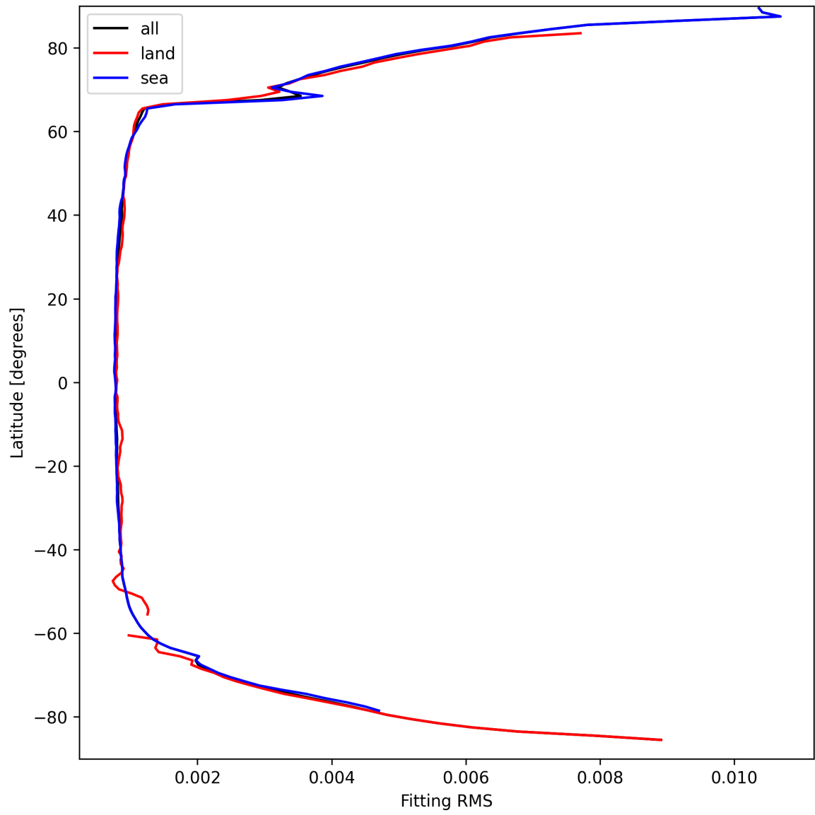
Figure 22: Zonal average of “Fitting RMS” for 2025-03-29 to 2025-03-30.
