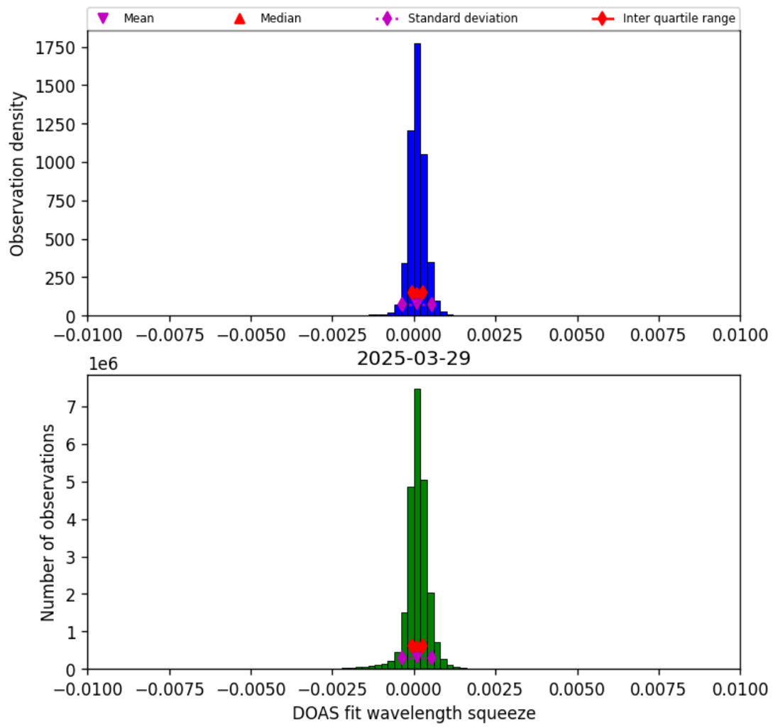
Figure 36: Histogram of “DOAS fit wavelength squeeze” for 2025-03-29 to 2025-03-30
