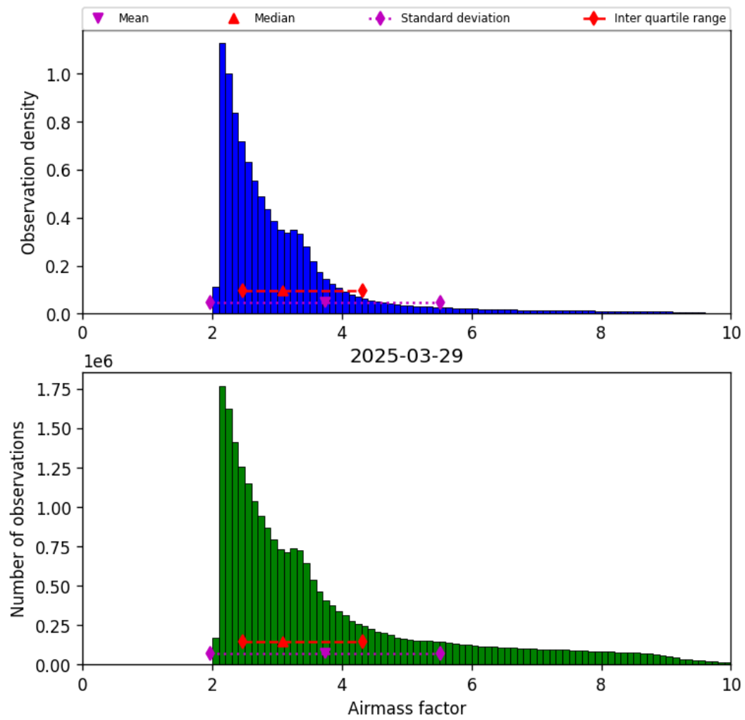
Figure 37: Histogram of “Airmass factor” for 2025-03-29 to 2025-03-30
