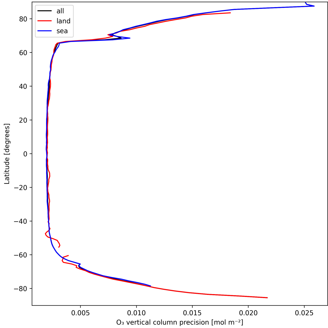
Figure 18: Zonal average of “O 3 vertical column precision” for 2025-03-29 to 2025-03-30.
