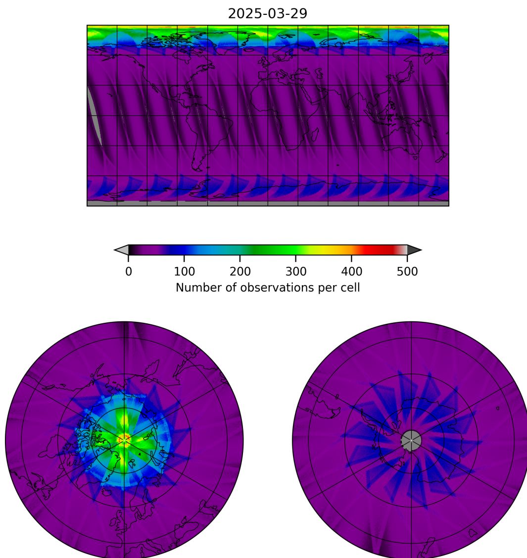
Figure 15: Map of the number of observations for 2025-03-29 to 2025-03-30
