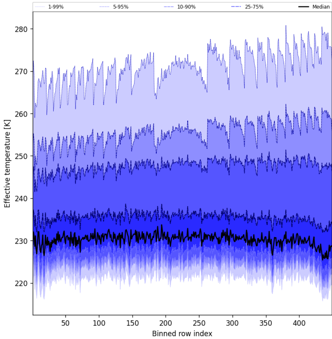
Figure 50: Along track statistics of “Effective temperature” for 2025-03-29 to 2025-03-30
