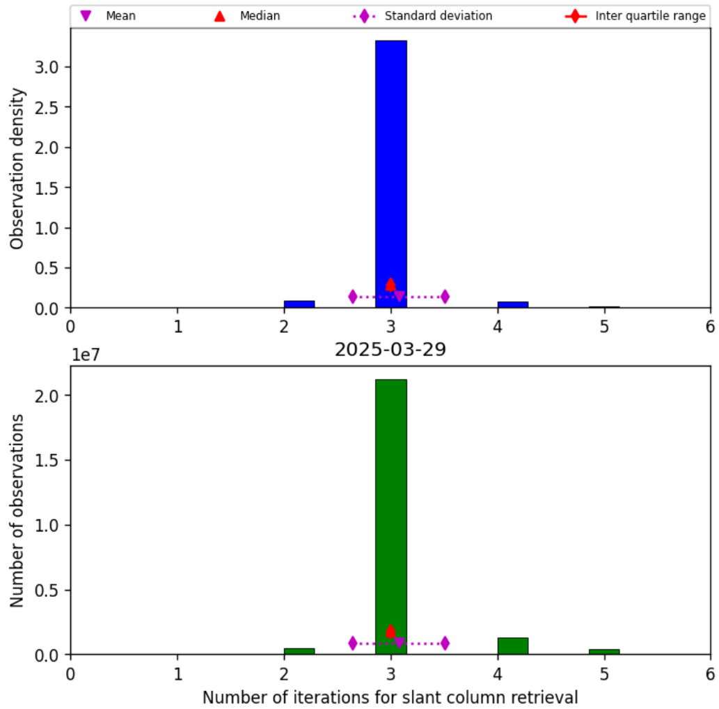
Figure 33: Histogram of “Number of iterations for slant column retrieval” for 2025-03-29 to 2025-03-30
