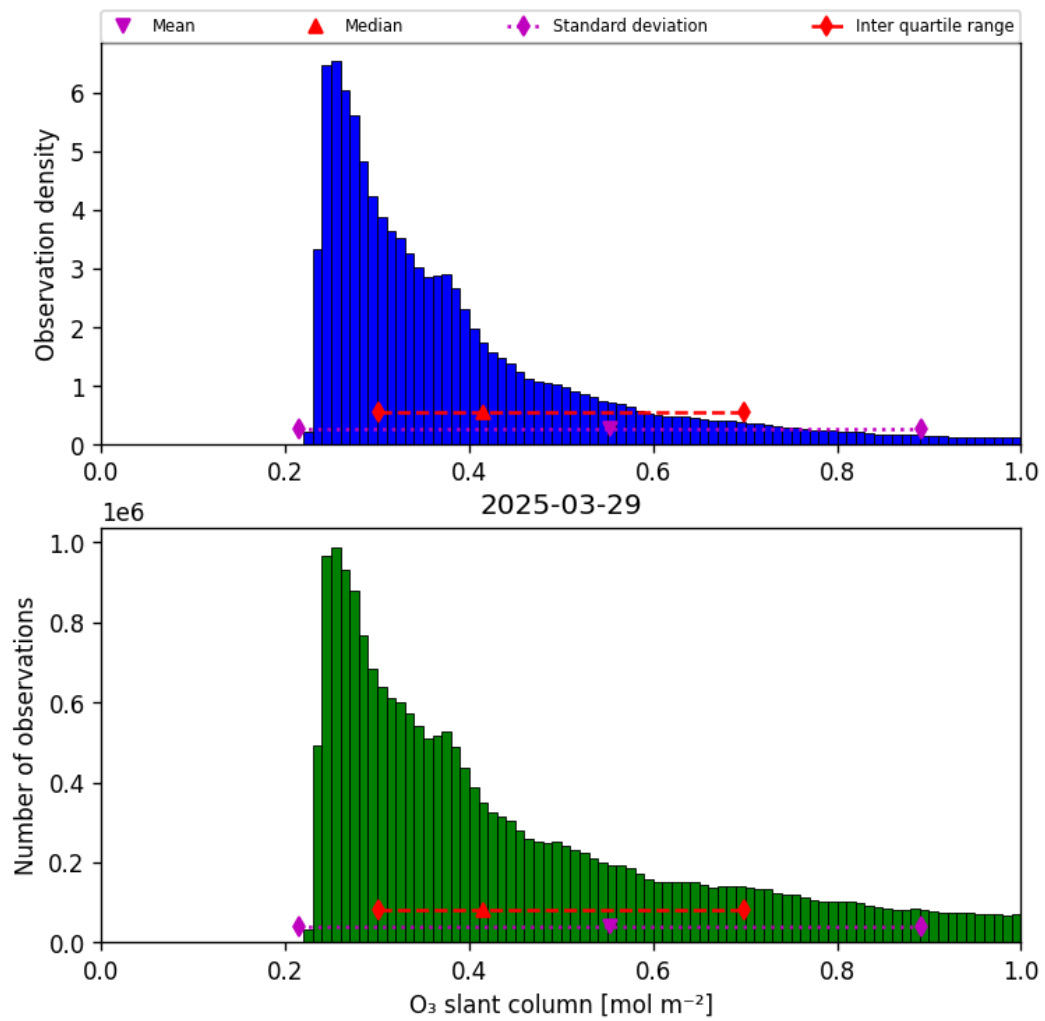
Figure 31: Histogram of “O 3 slant column” for 2025-03-29 to 2025-03-30
