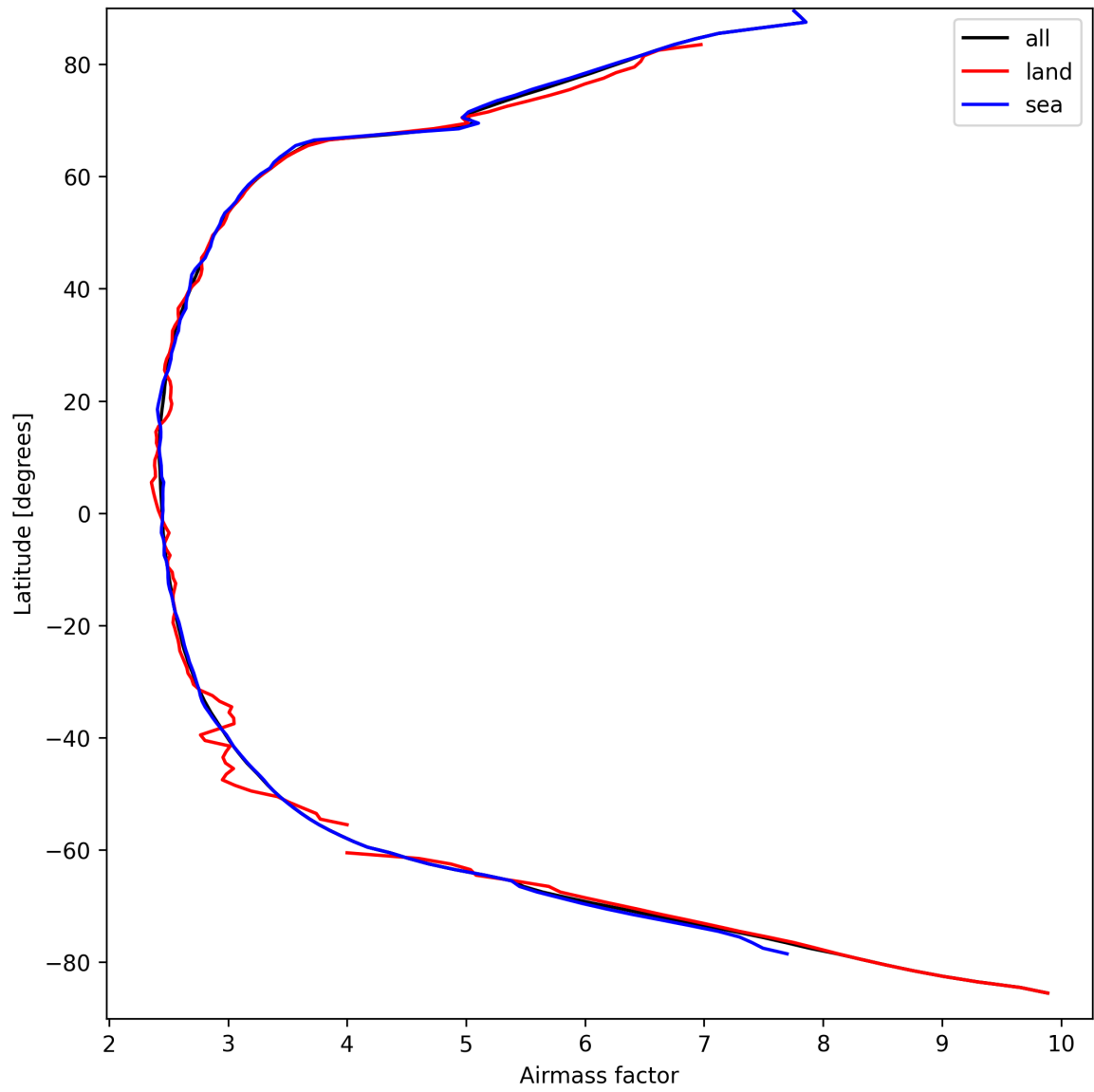
Figure 25: Zonal average of “Airmass factor” for 2025-03-29 to 2025-03-30.
