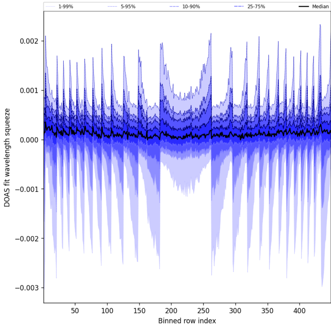
Figure 48: Along track statistics of “DOAS fit wavelength squeeze” for 2025-03-29 to 2025-03-30
