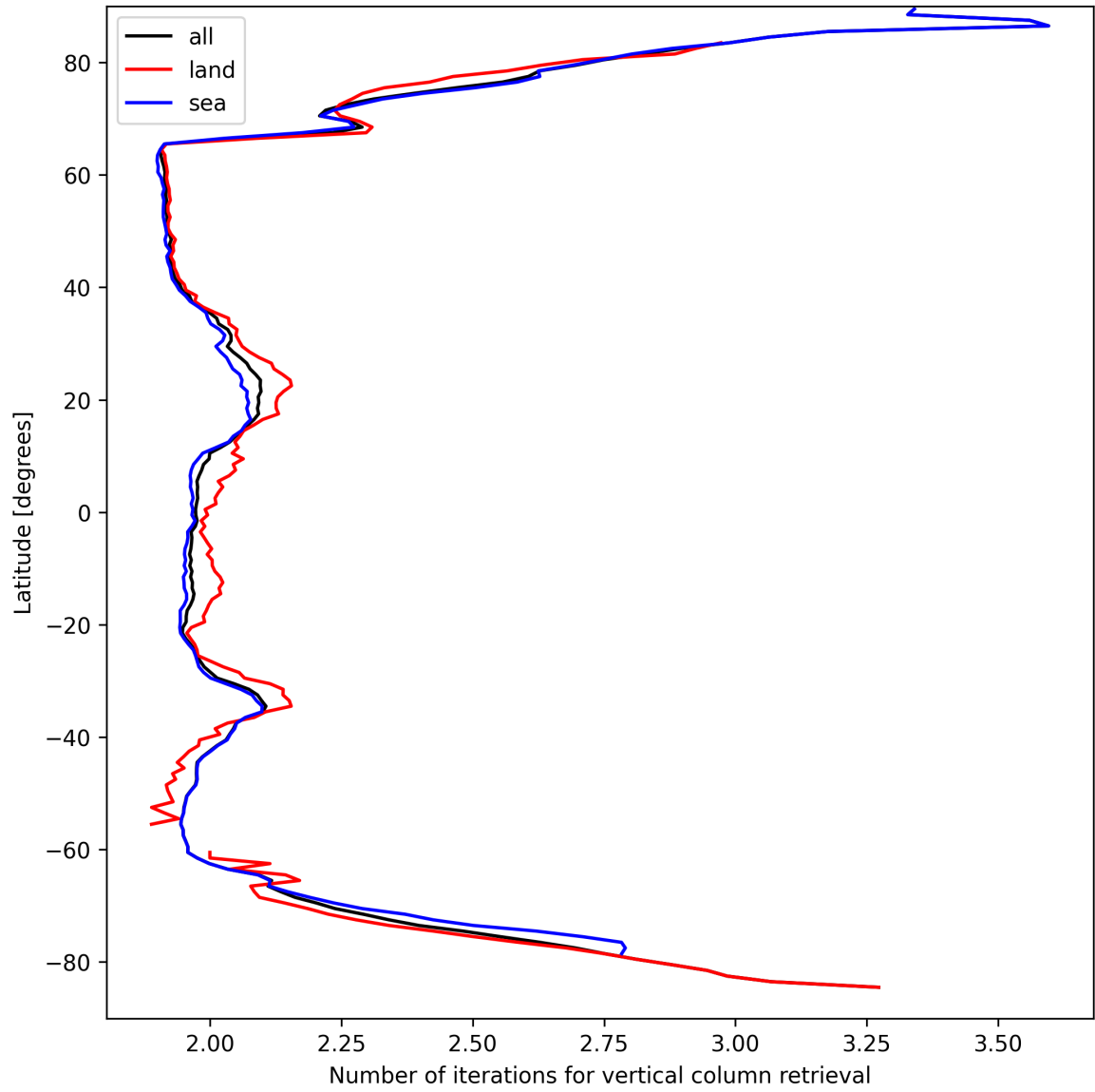
Figure 27: Zonal average of “Number of iterations for vertical column retrieval” for 2025-03-31 to 2025-03-31.
