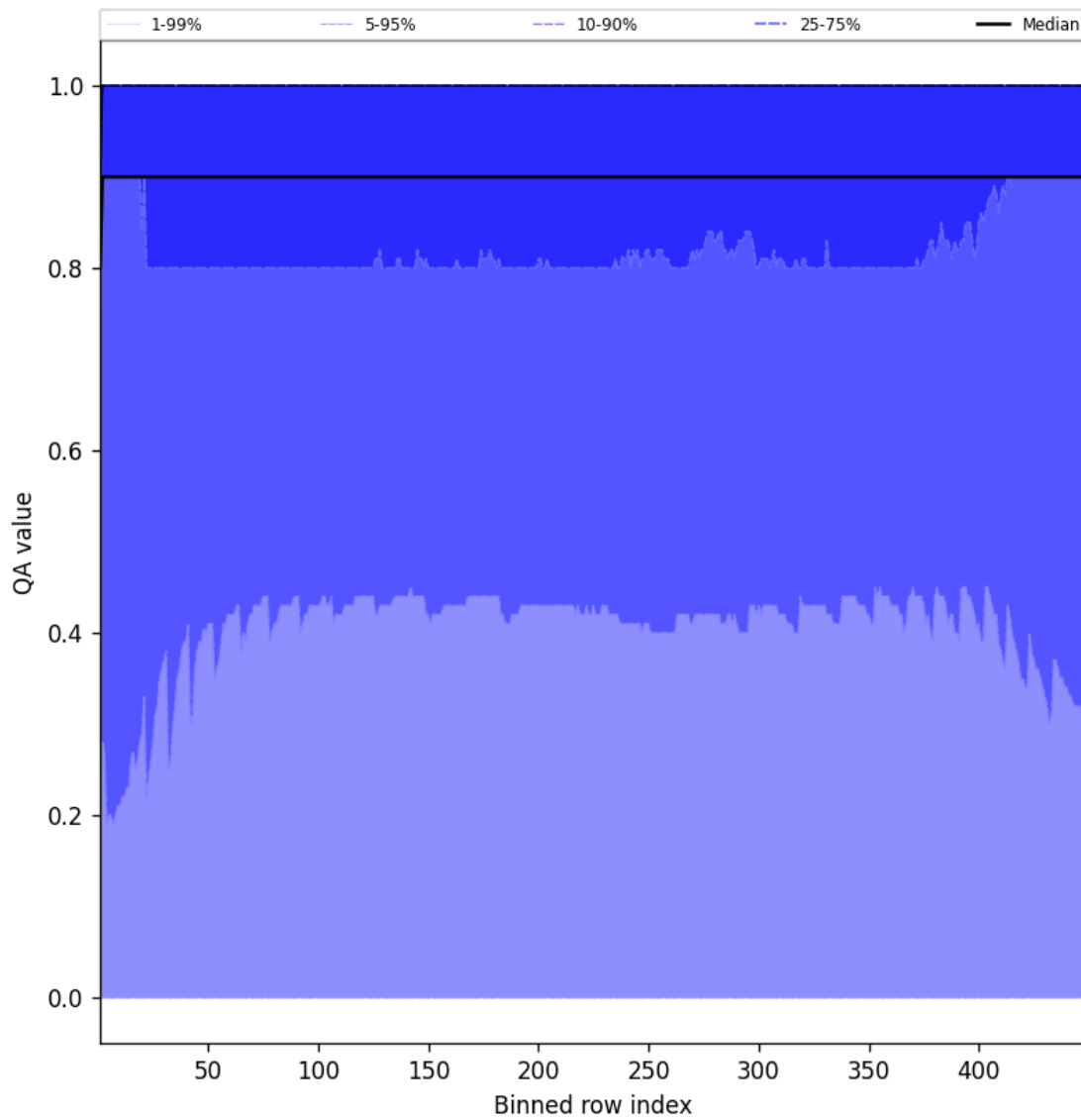
Figure 40: Along track statistics of “QA value” for 2025-03-31 to 2025-03-31
