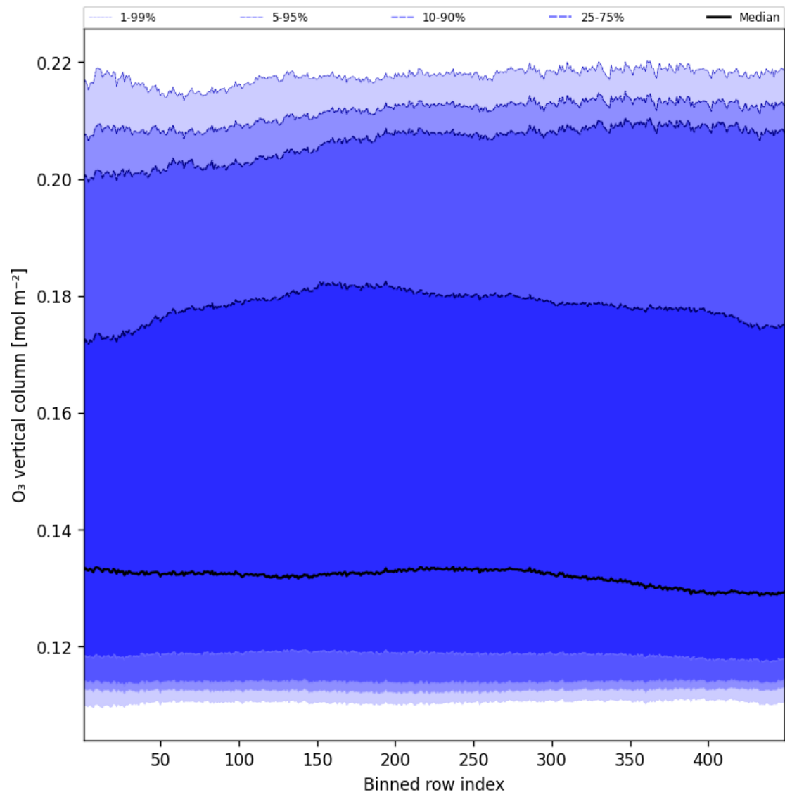
Figure 41: Along track statistics of “O 3 vertical column” for 2025-03-31 to 2025-03-31
