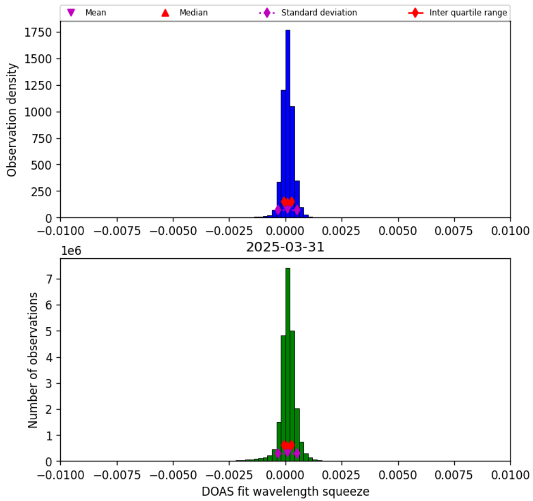
Figure 36: Histogram of “DOAS fit wavelength squeeze” for 2025-03-31 to 2025-03-31
