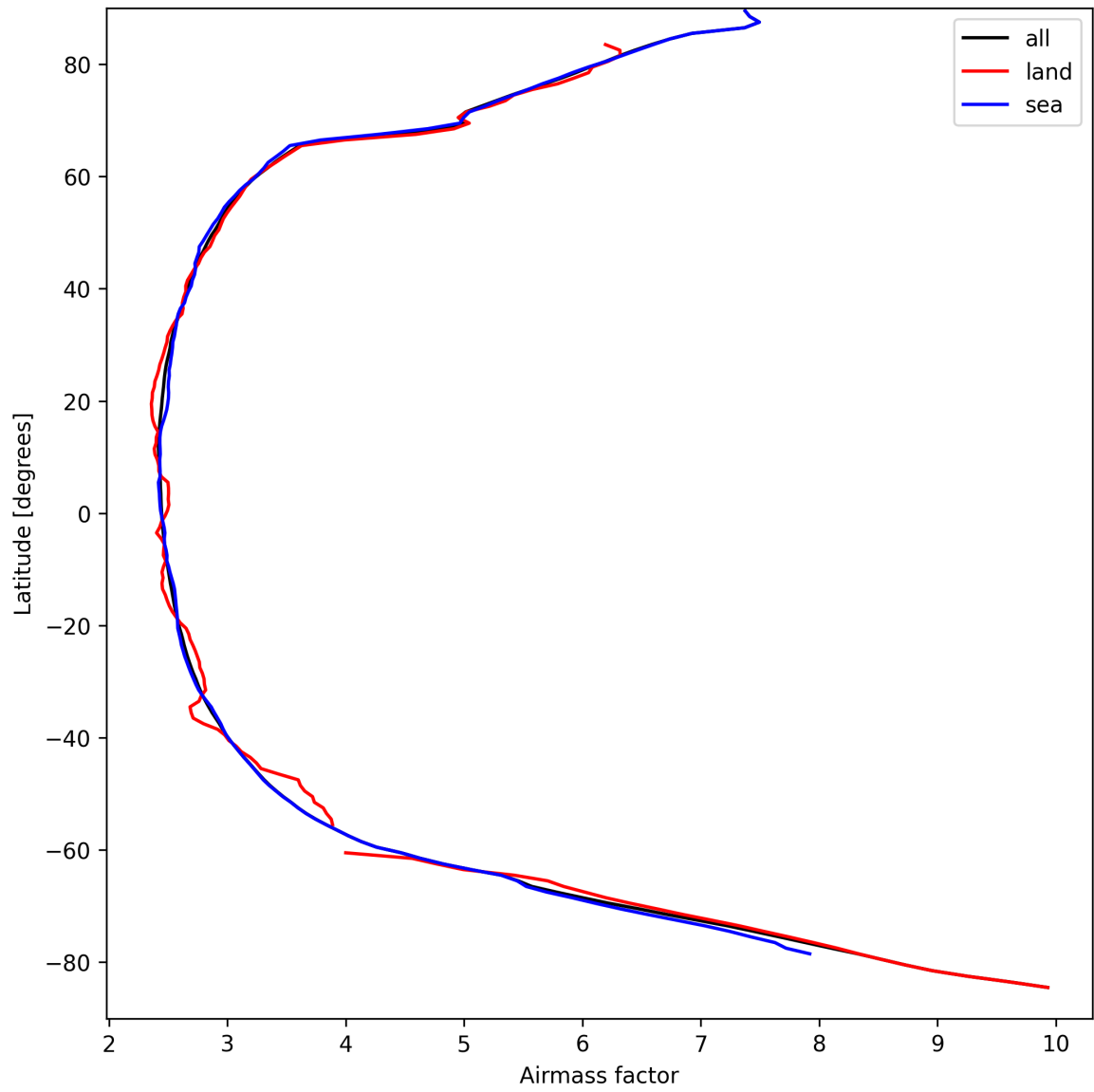
Figure 25: Zonal average of “Airmass factor” for 2025-03-31 to 2025-03-31.
