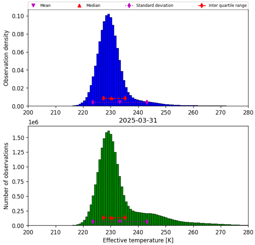
Figure 38: Histogram of “Effective temperature” for 2025-03-31 to 2025-03-31
