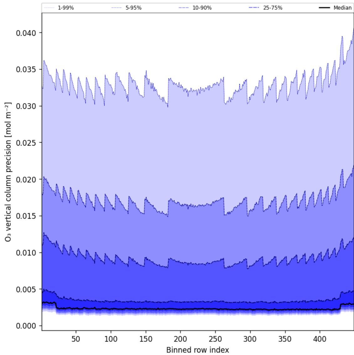
Figure 42: Along track statistics of “O 3 vertical column precision” for 2025-03-31 to 2025-03-31
