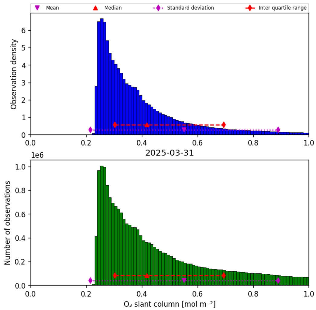
Figure 31: Histogram of “O 3 slant column” for 2025-03-31 to 2025-03-31
