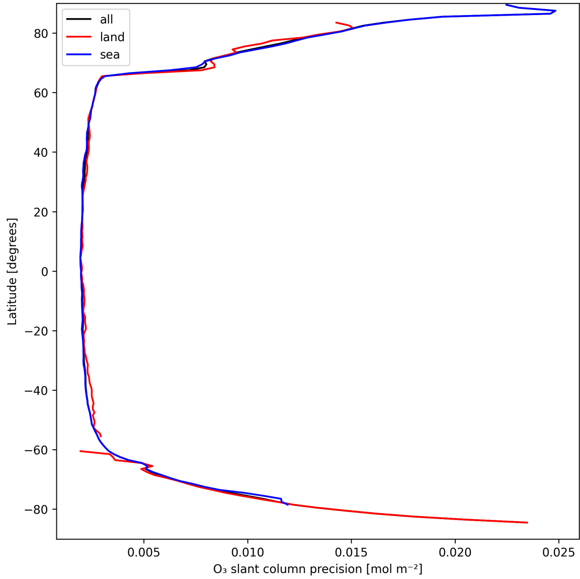
Figure 20: Zonal average of "O 3 slant column precision" for 2025-03-31 to 2025-03-31.
