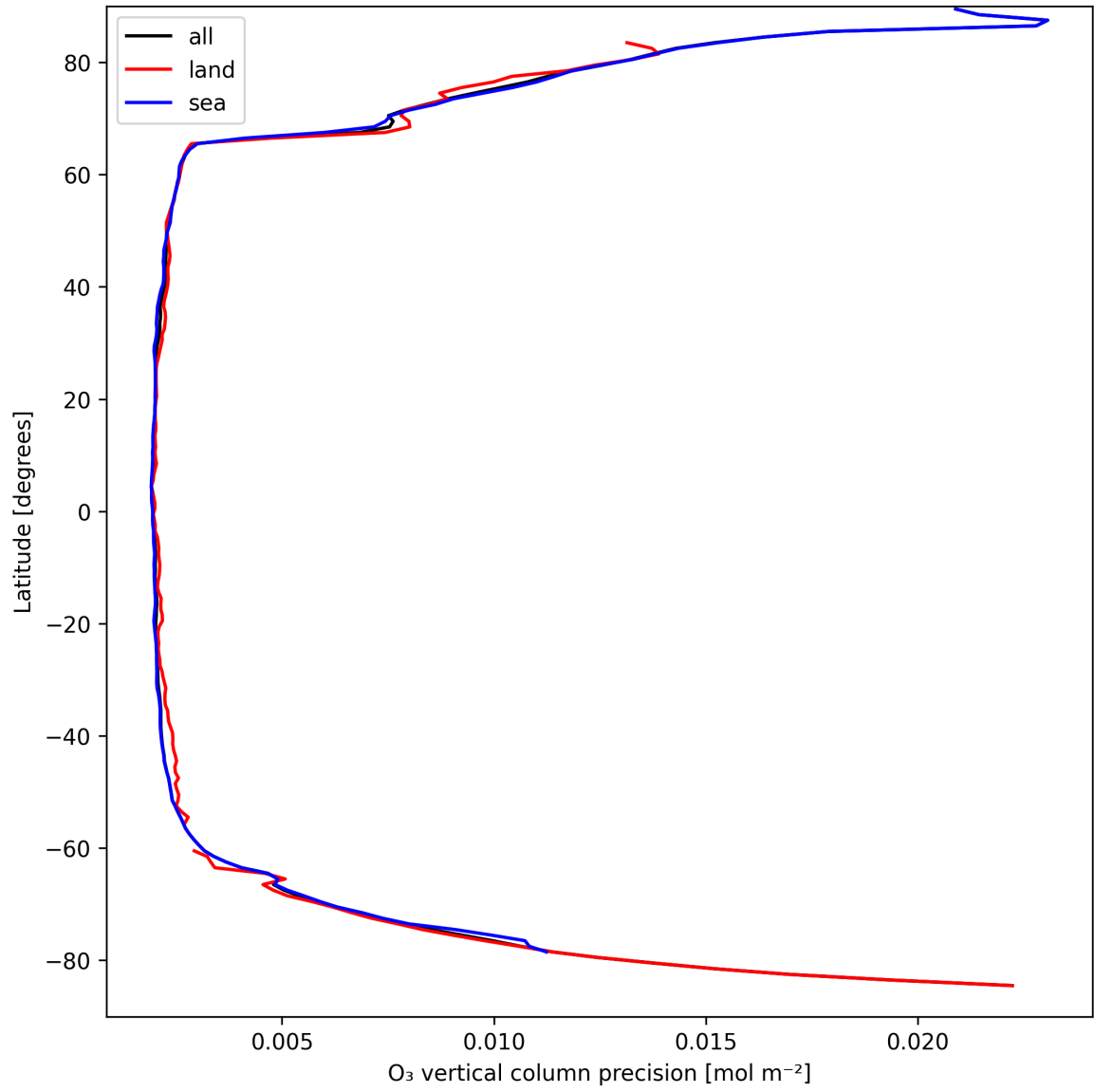
Figure 18: Zonal average of "O 3 vertical column precision" for 2025-03-31 to 2025-03-31.
