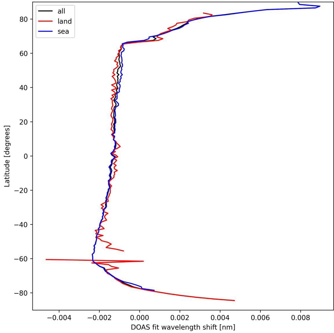
Figure 23: Zonal average of “DOAS fit wavelength shift” for 2025-03-31 to 2025-03-31.
