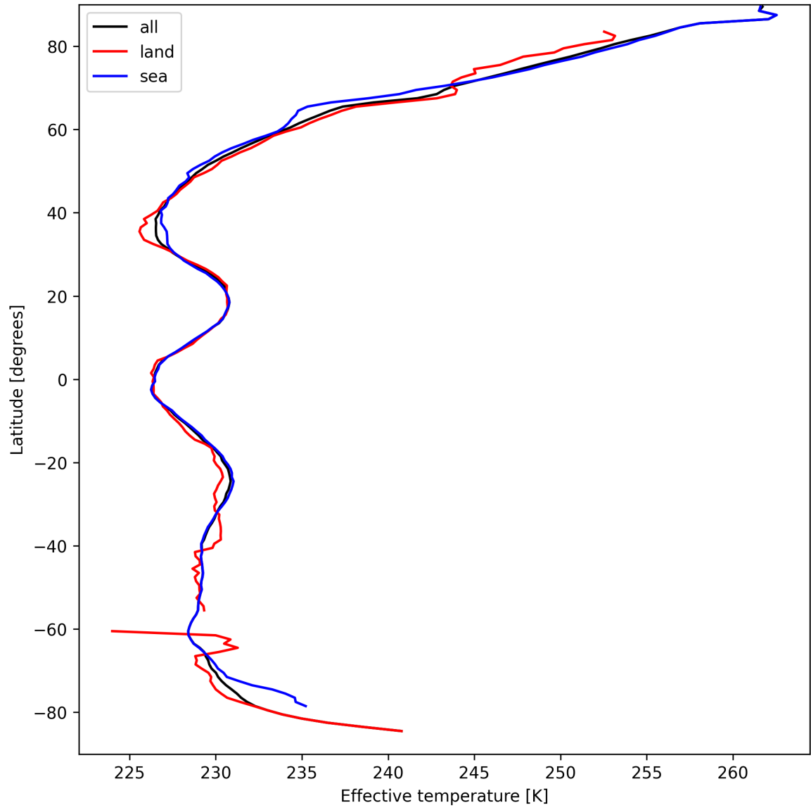
Figure 26: Zonal average of "Effective temperature" for 2025-03-31 to 2025-03-31.
