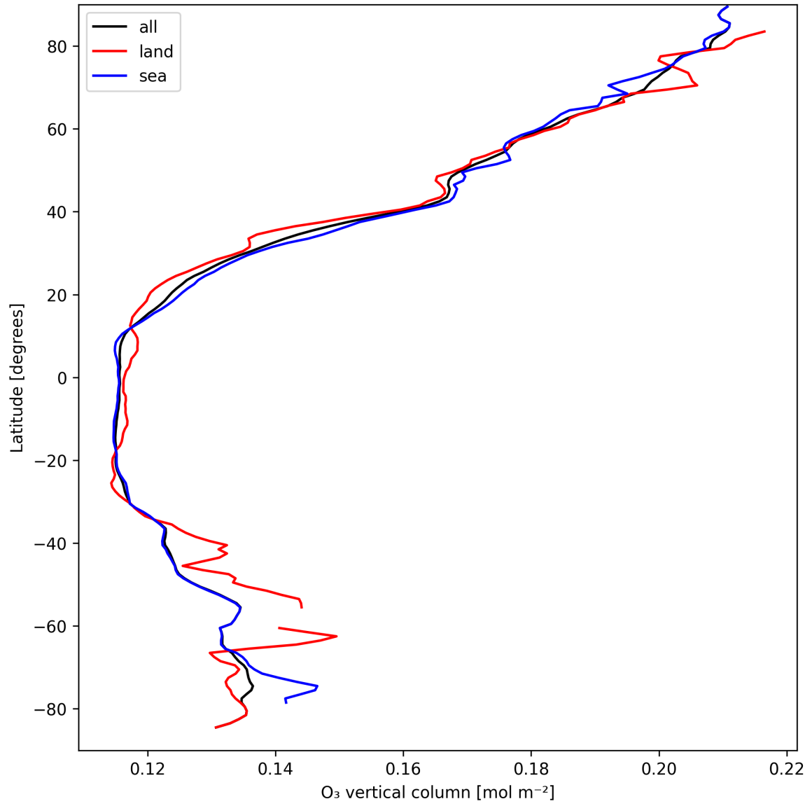
Figure 17: Zonal average of “O 3 vertical column” for 2025-03-31 to 2025-03-31.
