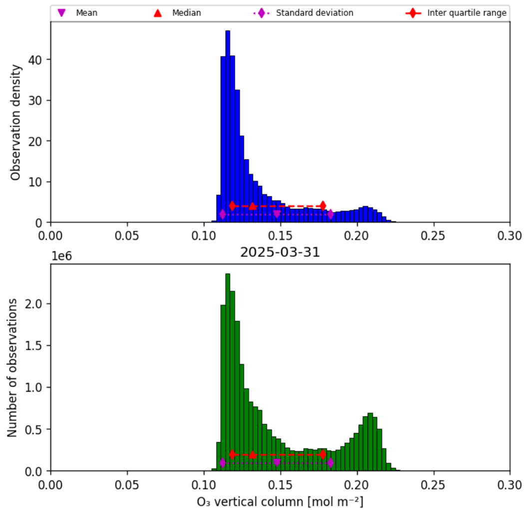
Figure 29: Histogram of “O 3 vertical column” for 2025-03-31 to 2025-03-31
