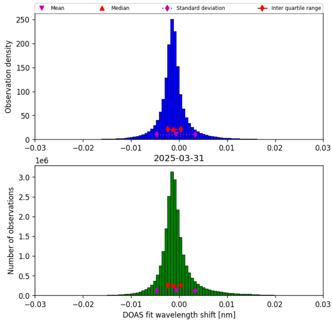
Figure 35: Histogram of “DOAS fit wavelength shift” for 2025-03-31 to 2025-03-31
