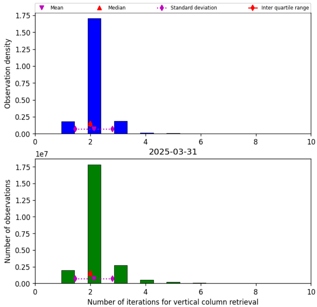
Figure 39: Histogram of “Number of iterations for vertical column retrieval” for 2025-03-31 to 2025-03-31
