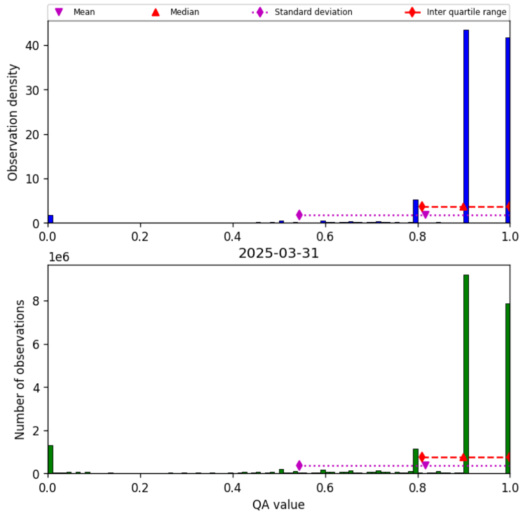
Figure 28: Histogram of “QA value” for 2025-03-31 to 2025-03-31
