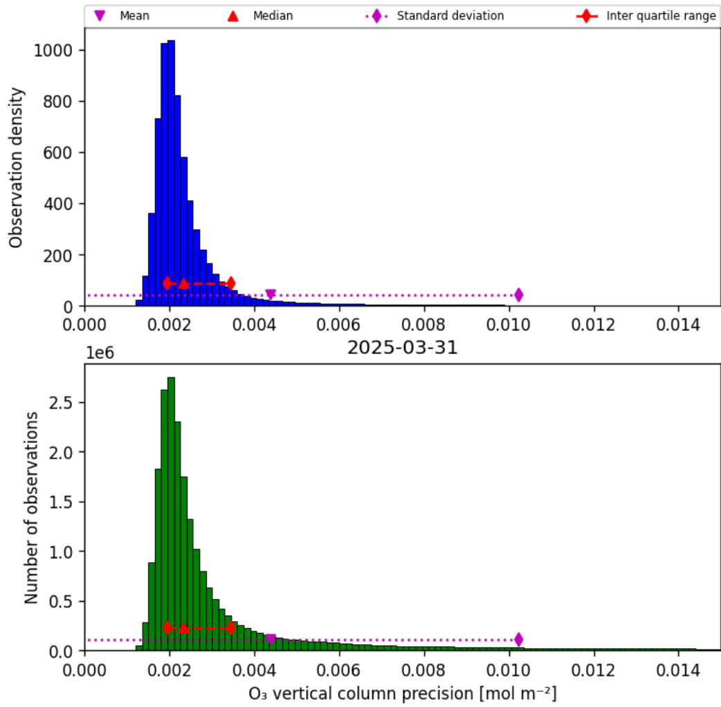
Figure 30: Histogram of "O 3 vertical column precision" for 2025-03-31 to 2025-03-31
