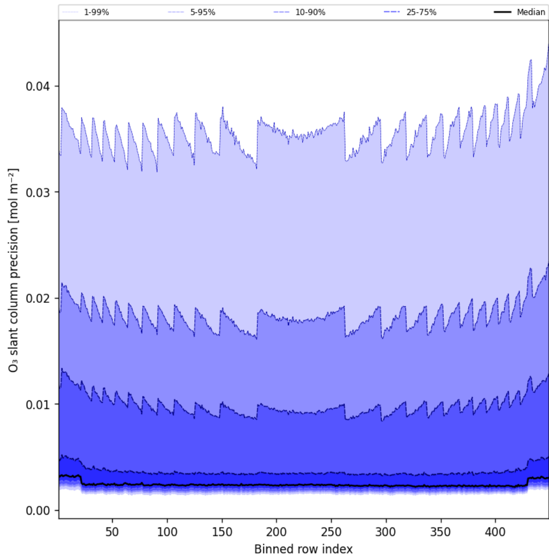
Figure 44: Along track statistics of “O 3 slant column precision” for 2025-03-31 to 2025-03-31
