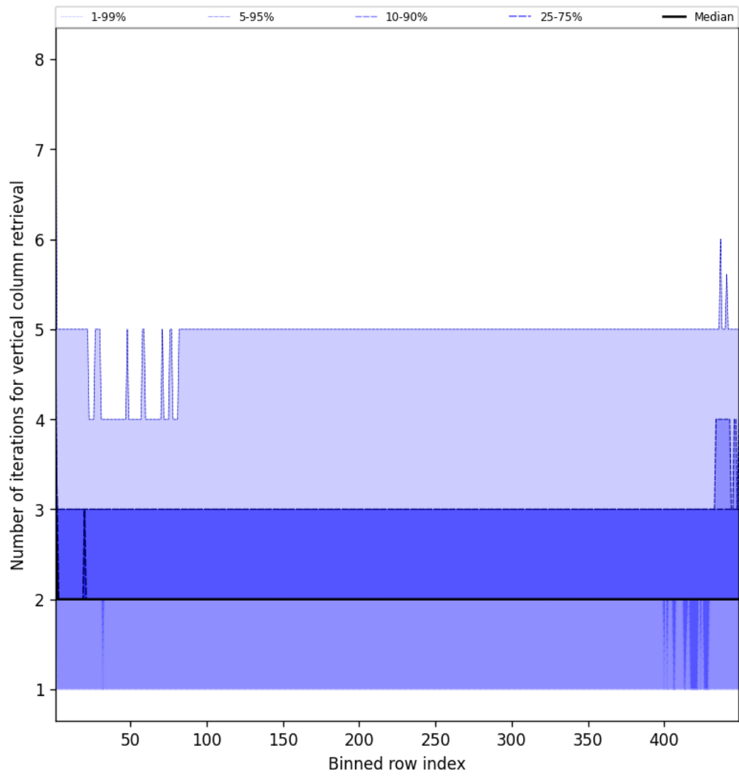
Figure 51: Along track statistics of “Number of iterations for vertical column retrieval” for 2025-03-31 to 2025-03-31
