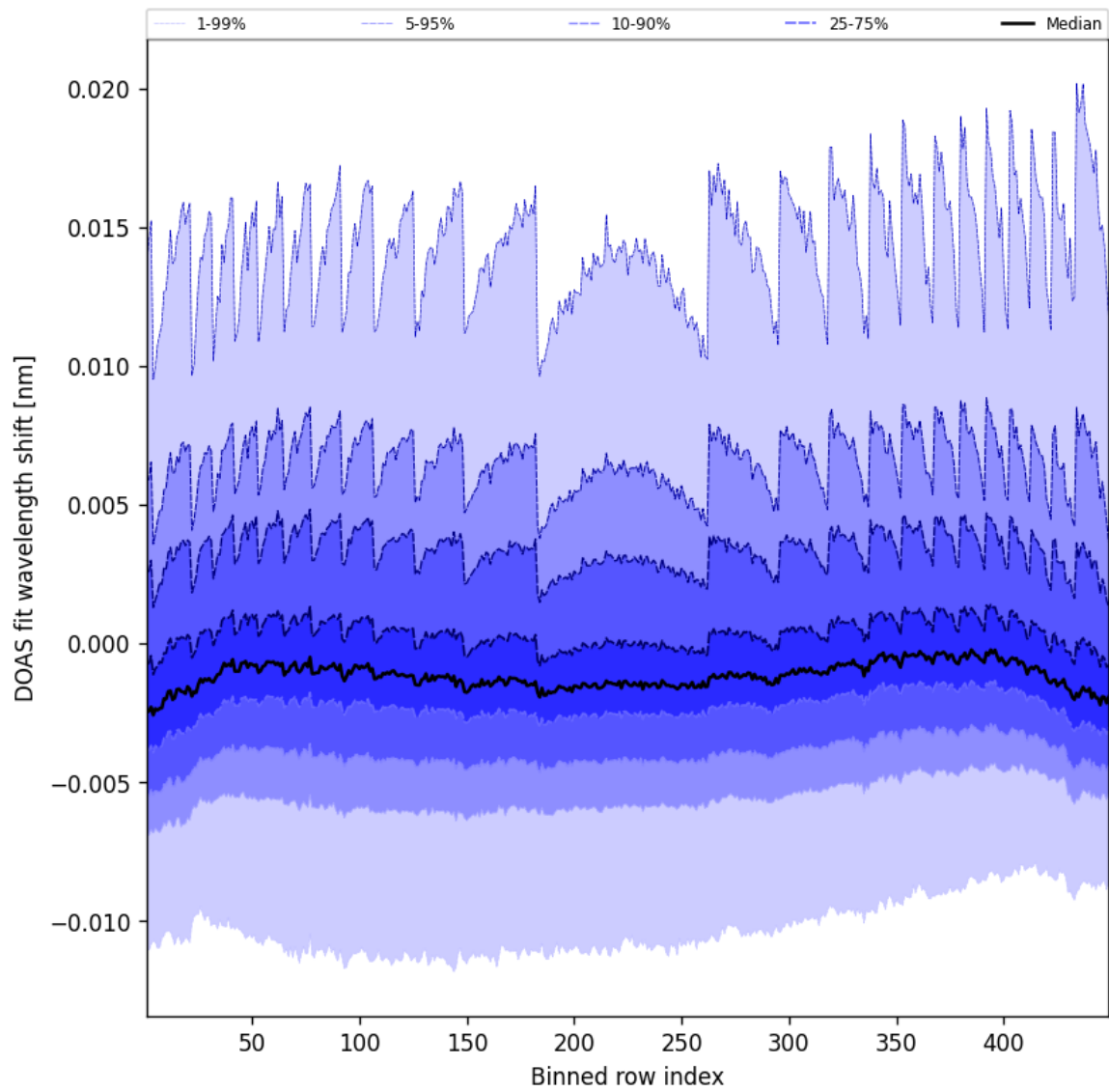
Figure 47: Along track statistics of “DOAS fit wavelength shift” for 2025-03-31 to 2025-03-31
