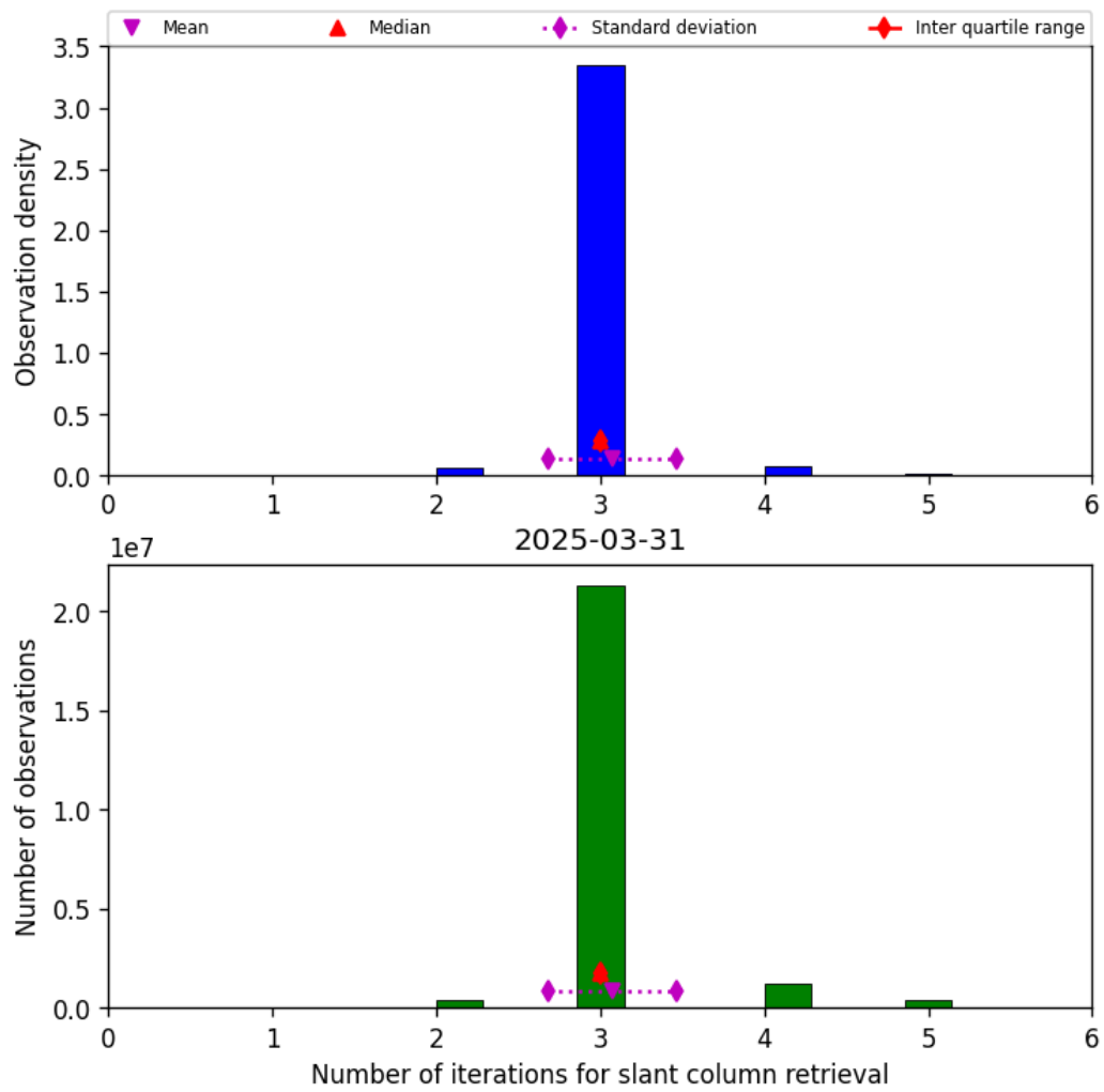
Figure 33: Histogram of “Number of iterations for slant column retrieval” for 2025-03-31 to 2025-03-31
