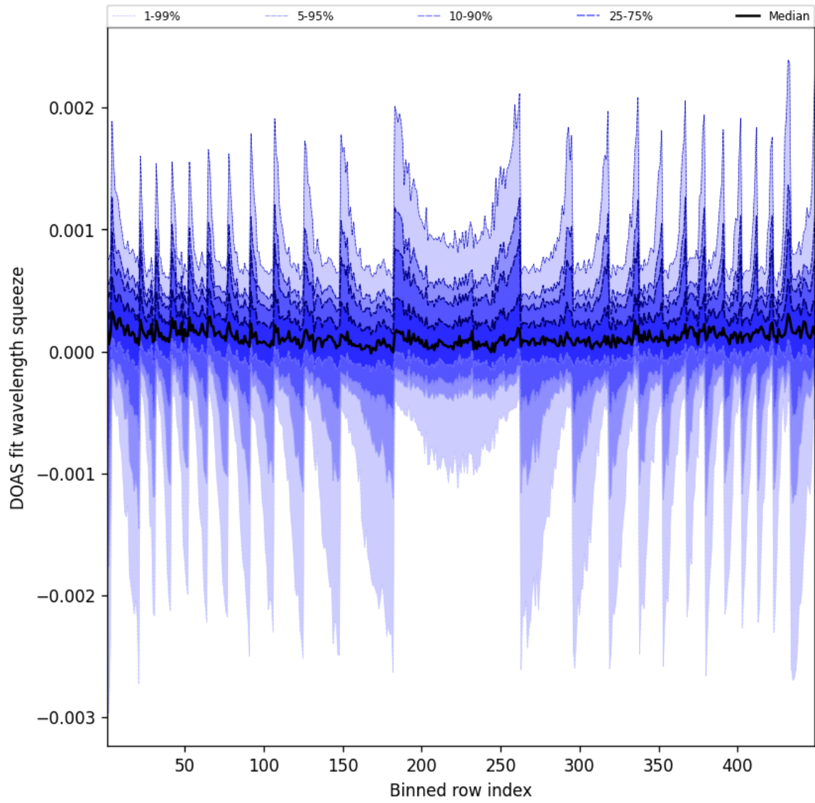
Figure 48: Along track statistics of “DOAS fit wavelength squeeze” for 2025-03-31 to 2025-03-31
