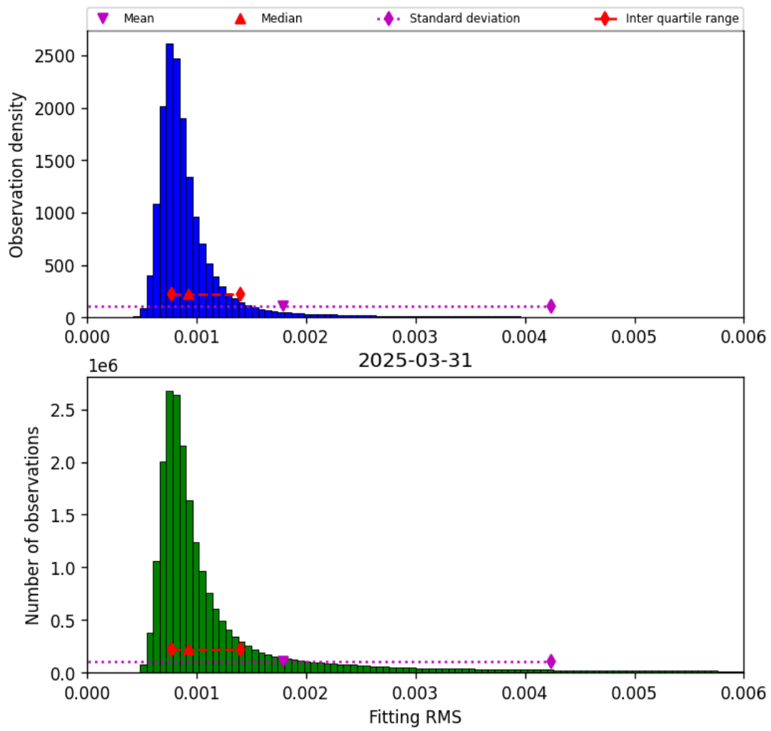
Figure 34: Histogram of “Fitting RMS” for 2025-03-31 to 2025-03-31
