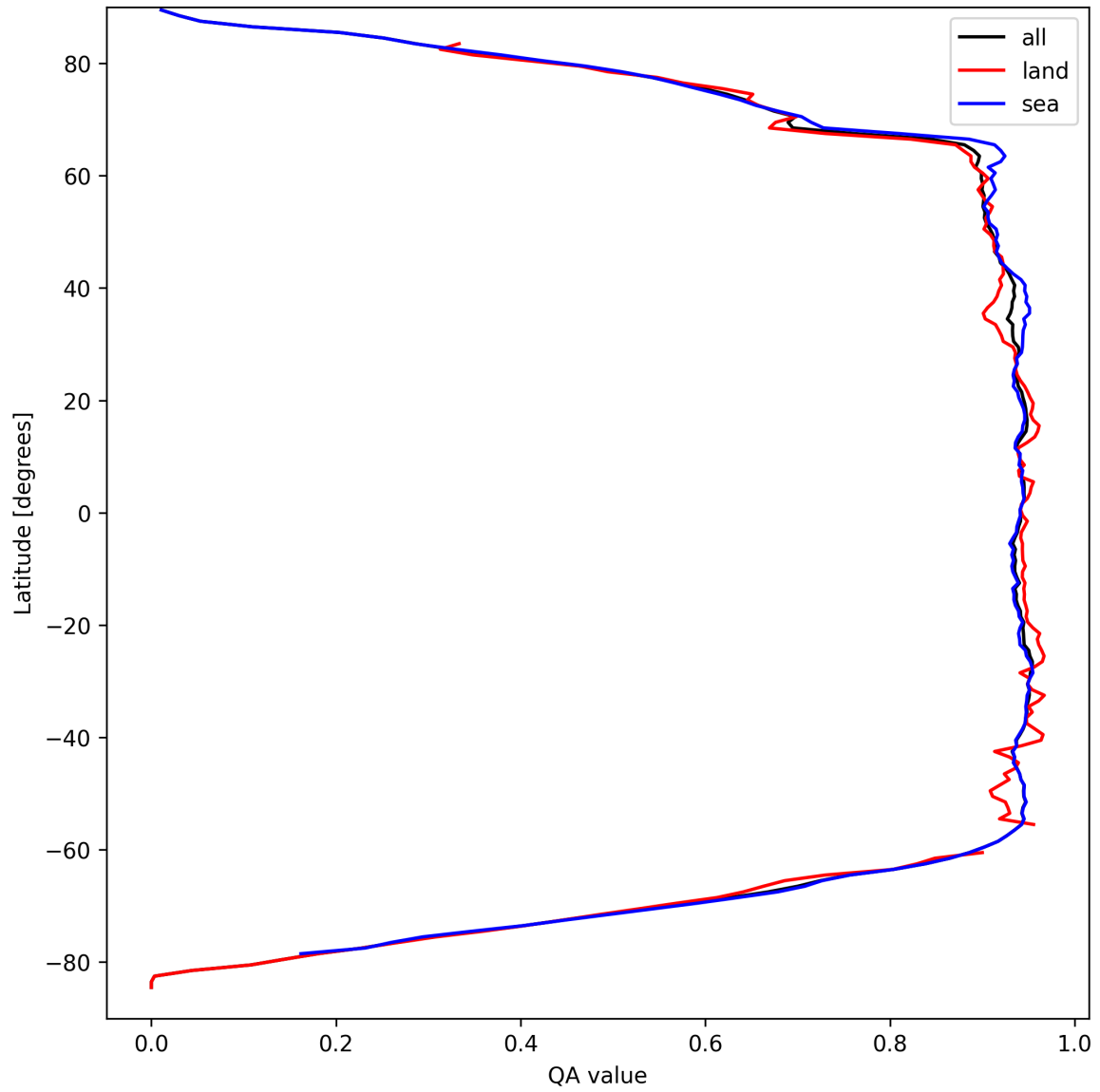
Figure 16: Zonal average of “QA value” for 2025-03-31 to 2025-03-31.
