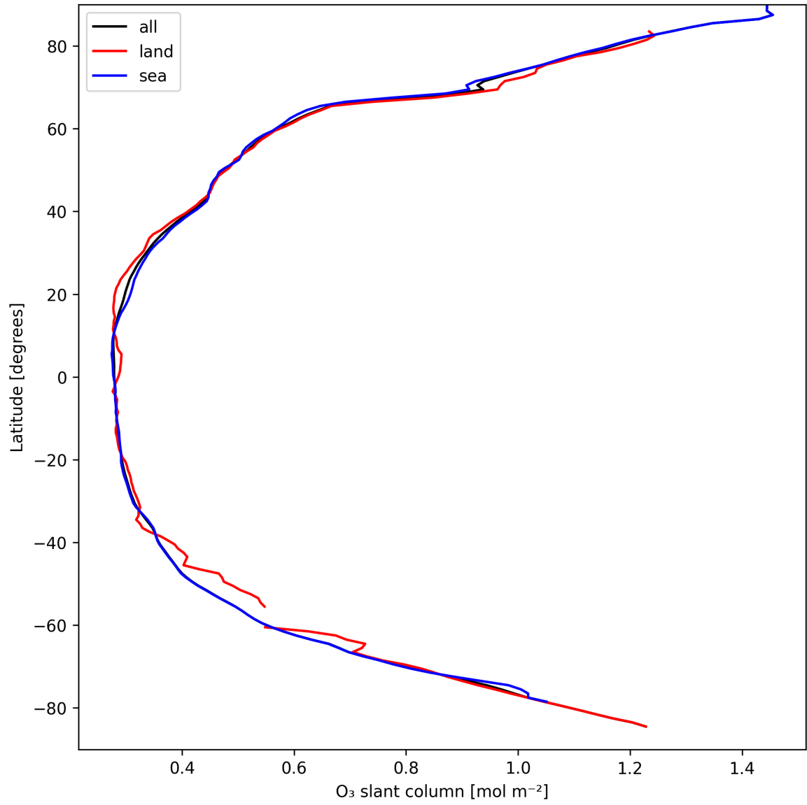
Figure 19: Zonal average of “O 3 slant column” for 2025-03-31 to 2025-03-31.
