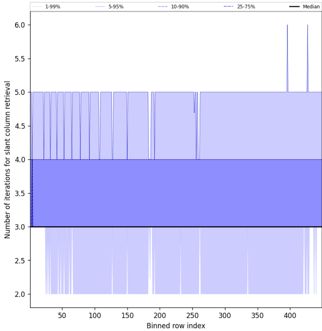
Figure 45: Along track statistics of “Number of iterations for slant column retrieval” for 2025-03-31 to 2025-03-31
