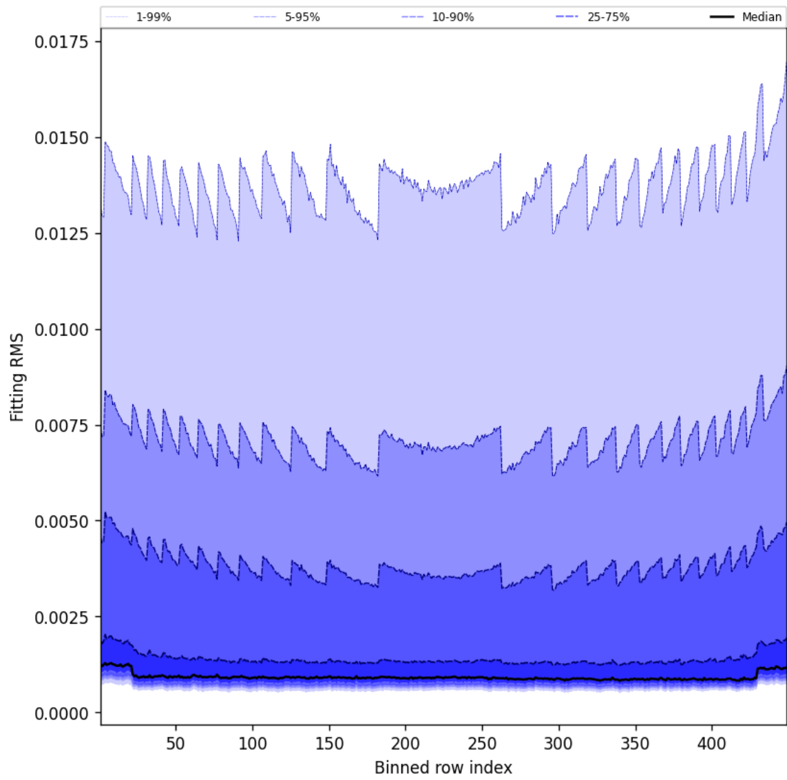
Figure 46: Along track statistics of "Fitting RMS" for 2025-03-31 to 2025-03-31
