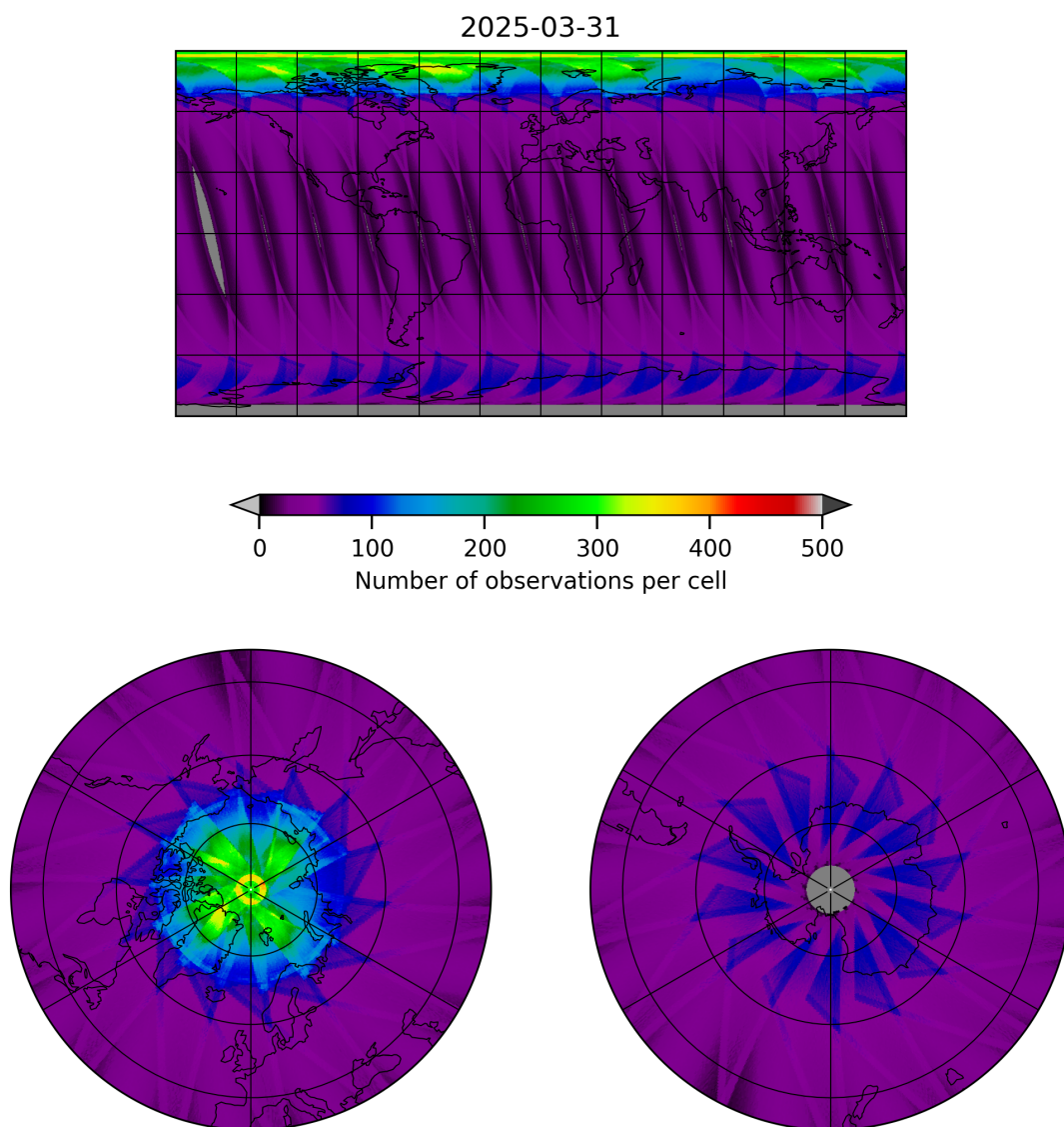
Figure 15: Map of the number of observations for 2025-03-31 to 2025-03-31
