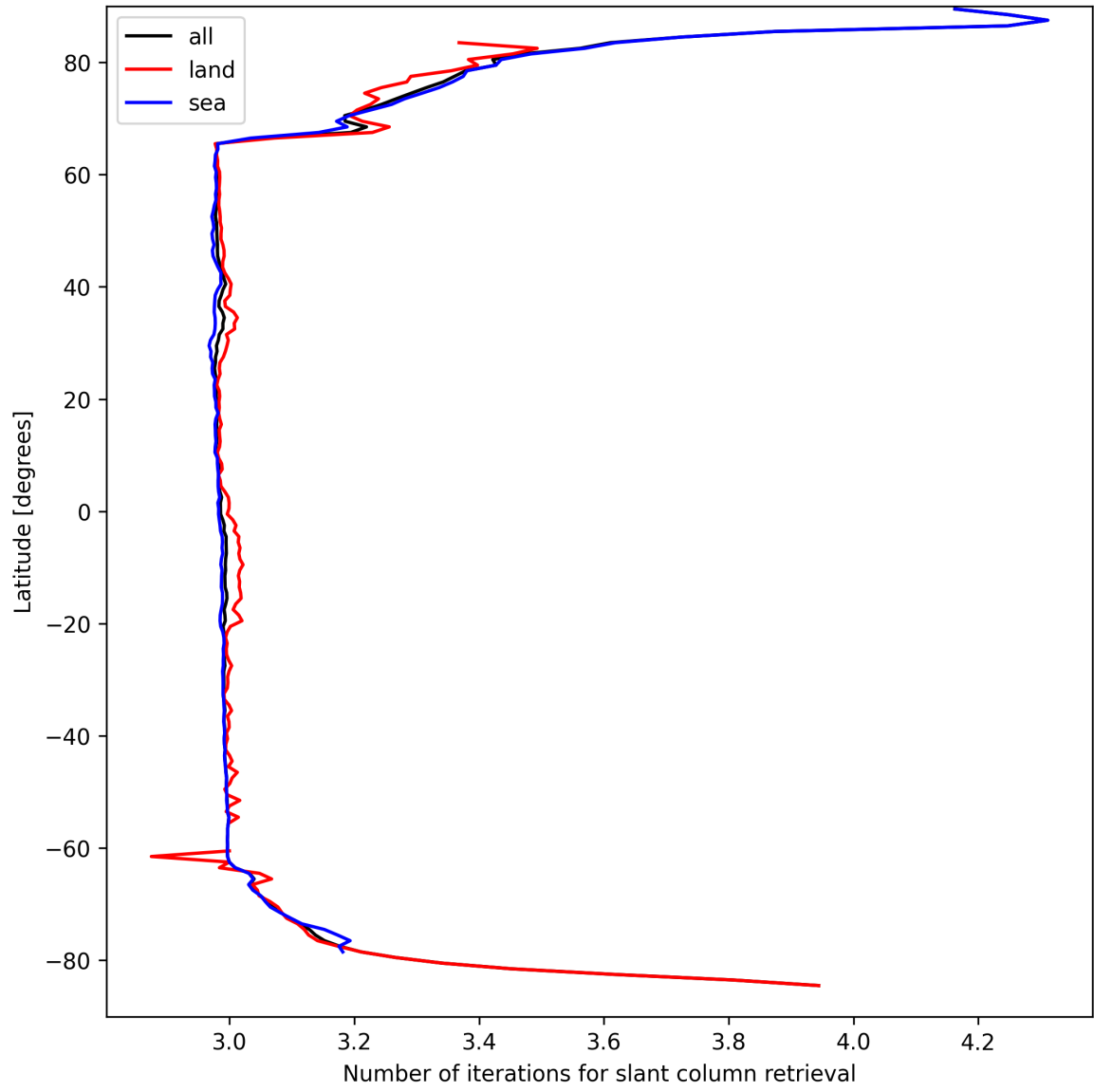
Figure 21: Zonal average of “Number of iterations for slant column retrieval” for 2025-03-31 to 2025-03-31.
