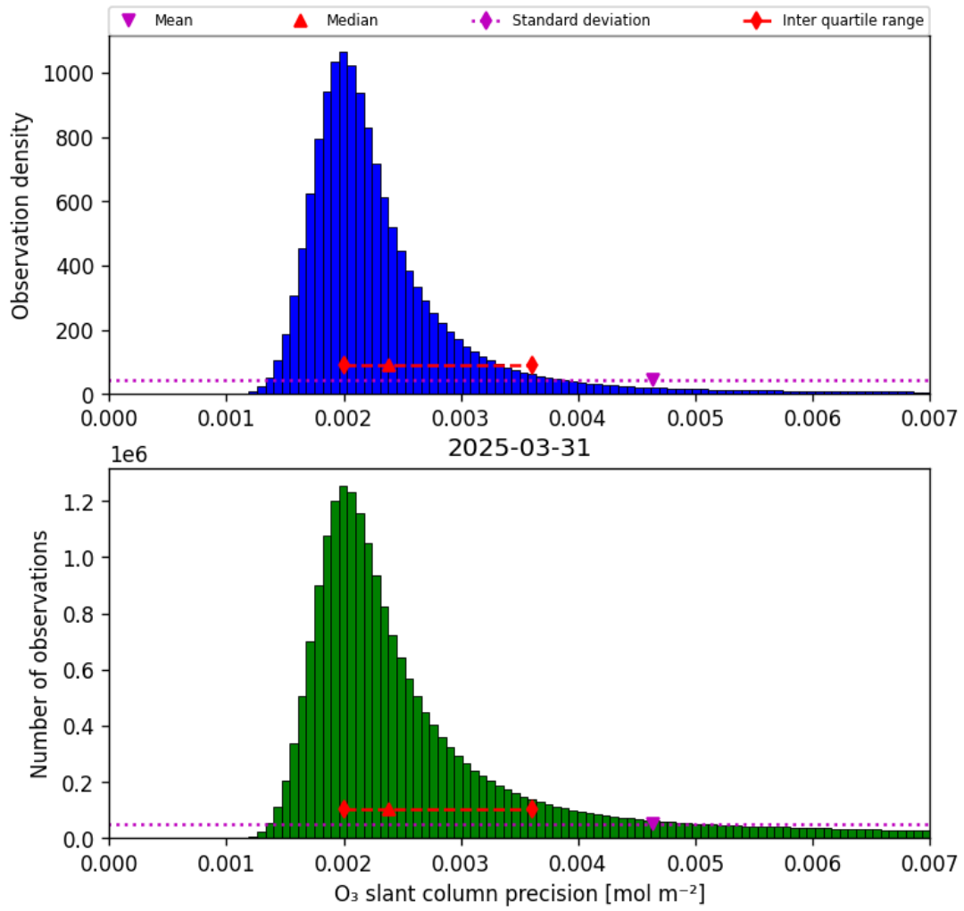
Figure 32: Histogram of “O 3 slant column precision” for 2025-03-31 to 2025-03-31
