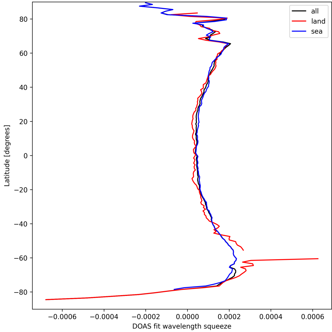
Figure 24: Zonal average of “DOAS fit wavelength squeeze” for 2025-03-31 to 2025-03-31.
