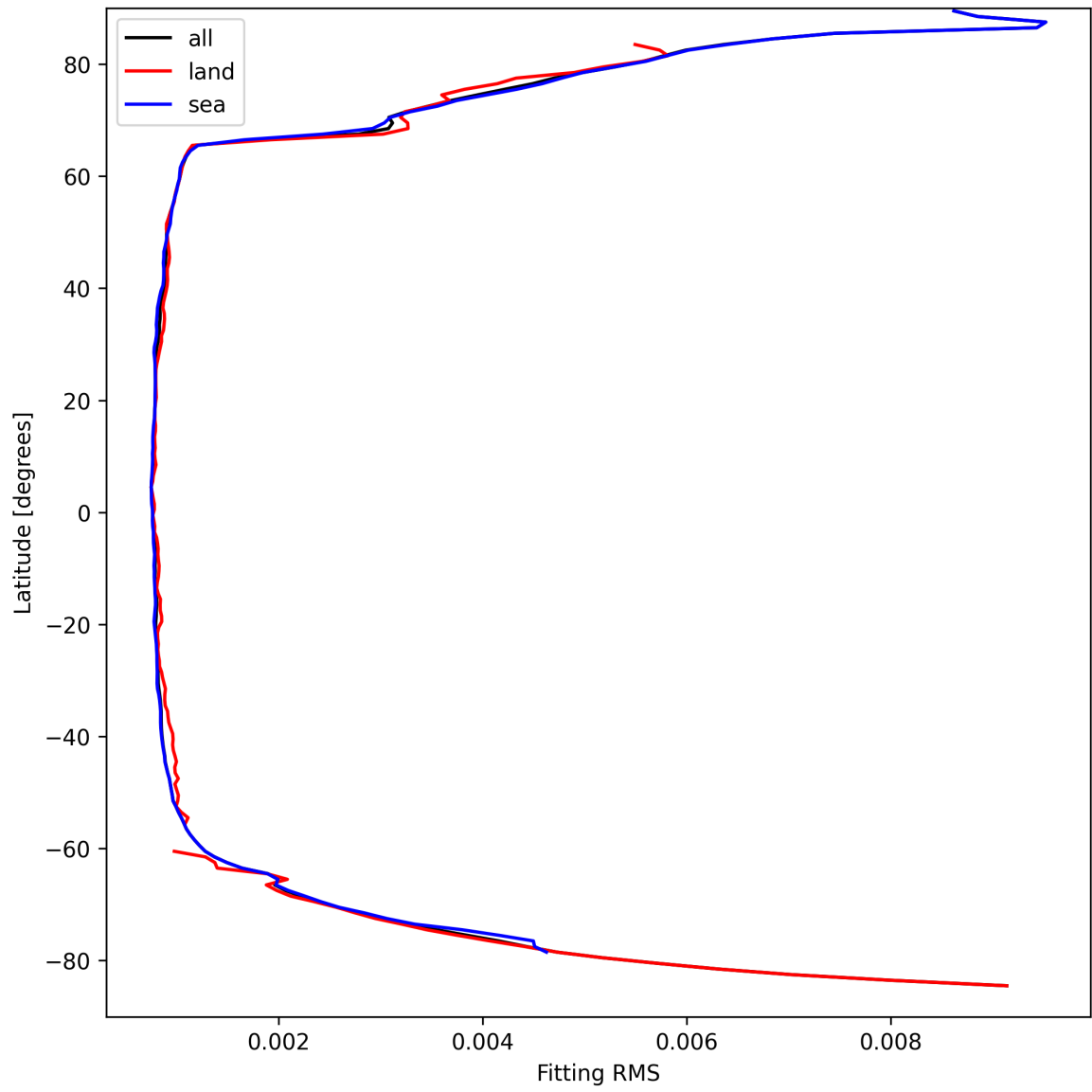
Figure 22: Zonal average of “Fitting RMS” for 2025-03-31 to 2025-03-31.
