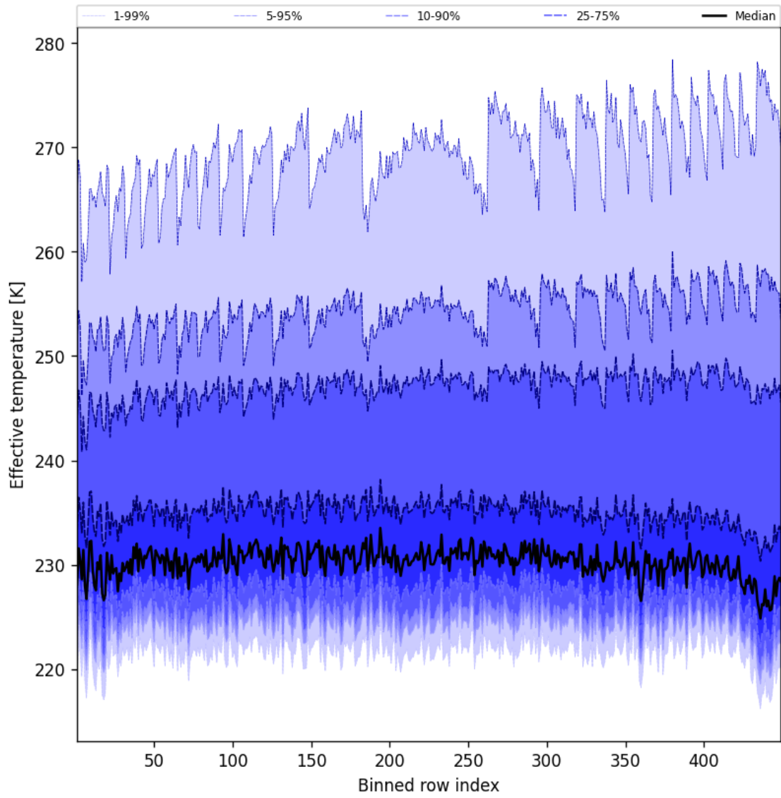
Figure 50: Along track statistics of “Effective temperature” for 2025-03-31 to 2025-03-31
