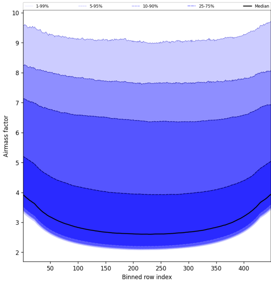
Figure 49: Along track statistics of “Airmass factor” for 2025-03-31 to 2025-03-31
