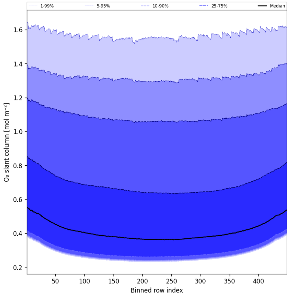
Figure 43: Along track statistics of “O 3 slant column” for 2025-03-31 to 2025-03-31
