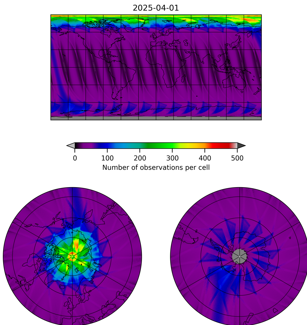
Figure 15: Map of the number of observations for 2025-04-01 to 2025-04-02
