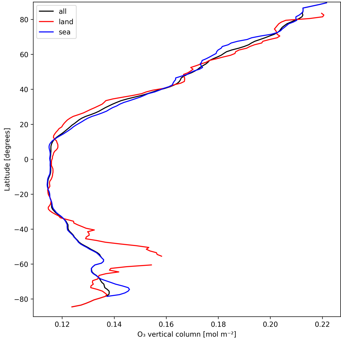
Figure 17: Zonal average of “O 3 vertical column” for 2025-04-01 to 2025-04-02.
