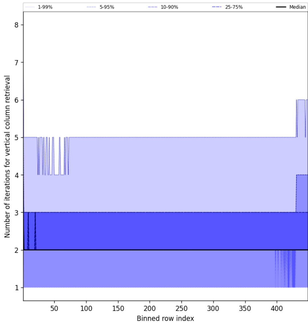
Figure 51: Along track statistics of “Number of iterations for vertical column retrieval” for 2025-04-01 to 2025-04-02
