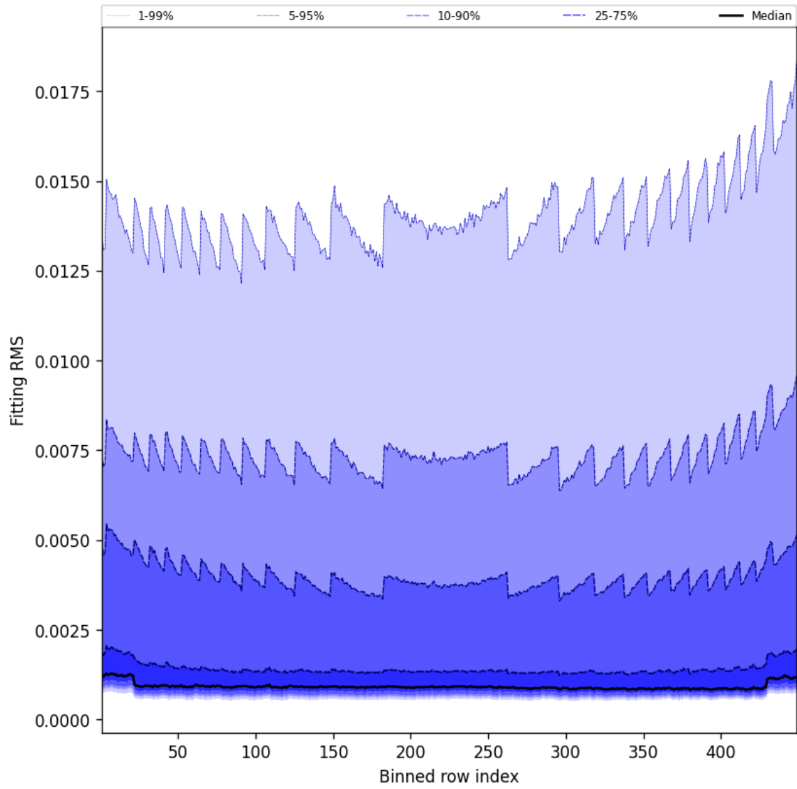
Figure 46: Along track statistics of “Fitting RMS” for 2025-04-01 to 2025-04-02
