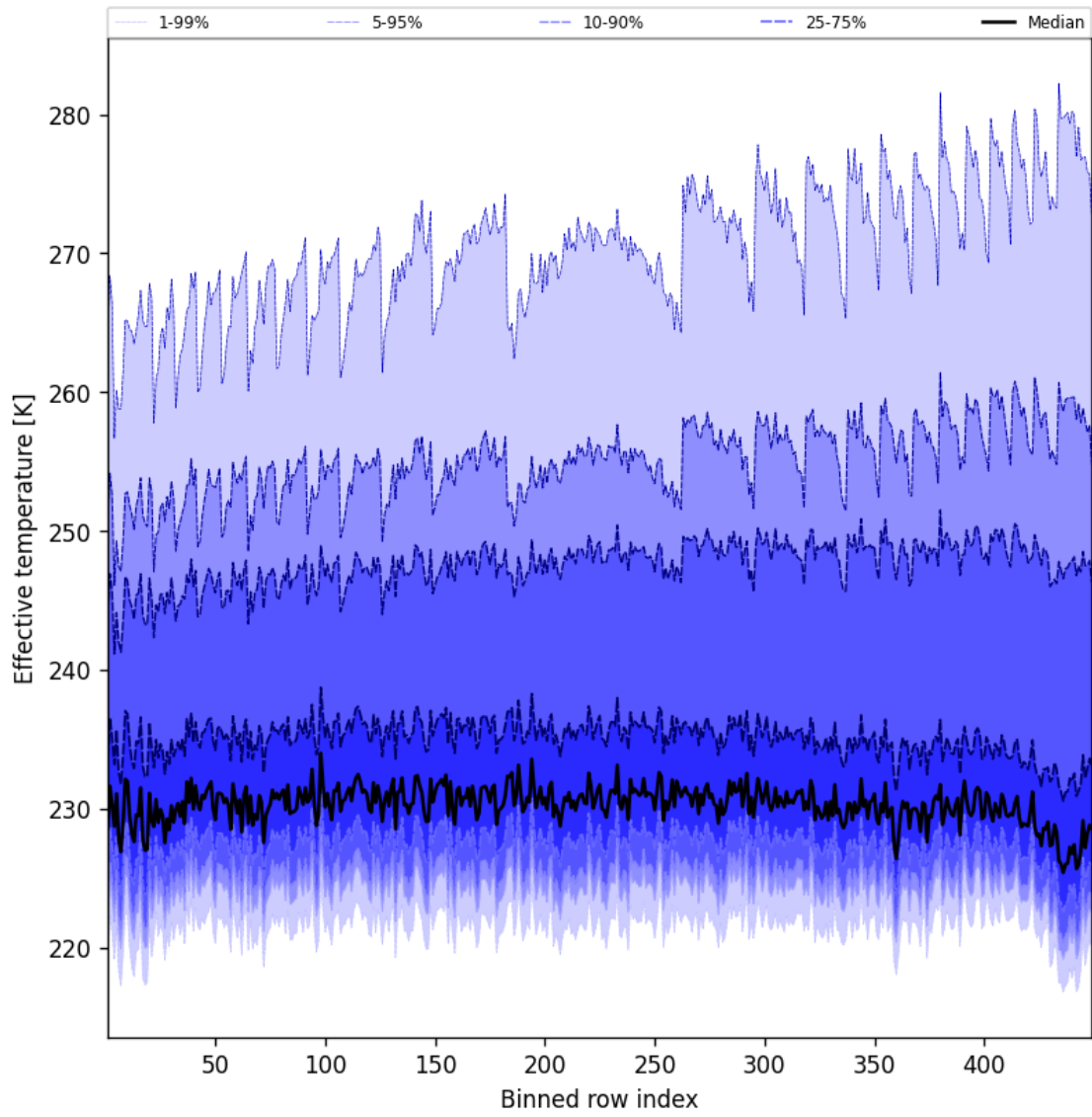
Figure 50: Along track statistics of “Effective temperature” for 2025-04-01 to 2025-04-02
