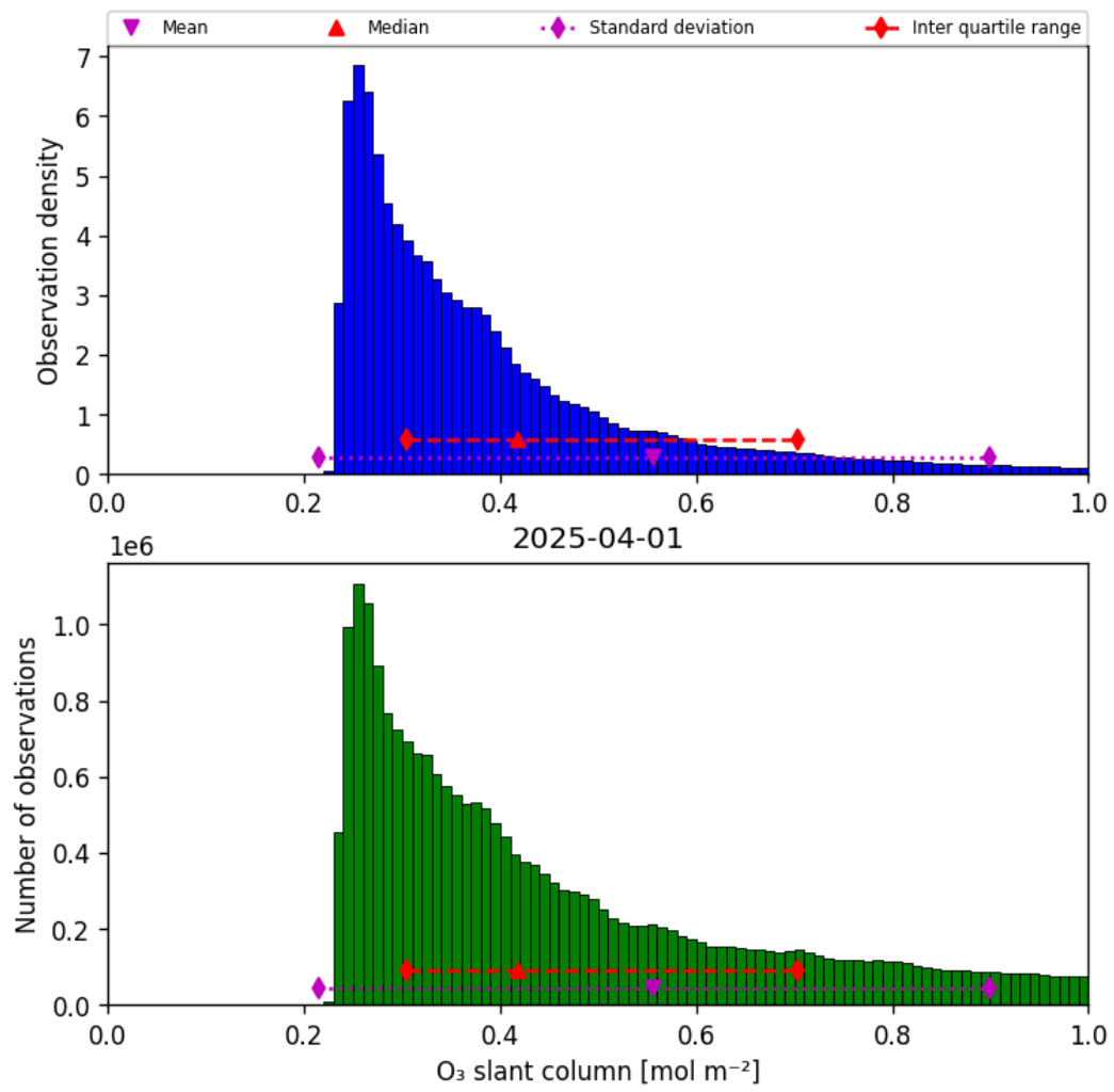
Figure 31: Histogram of “O 3 slant column” for 2025-04-01 to 2025-04-02
