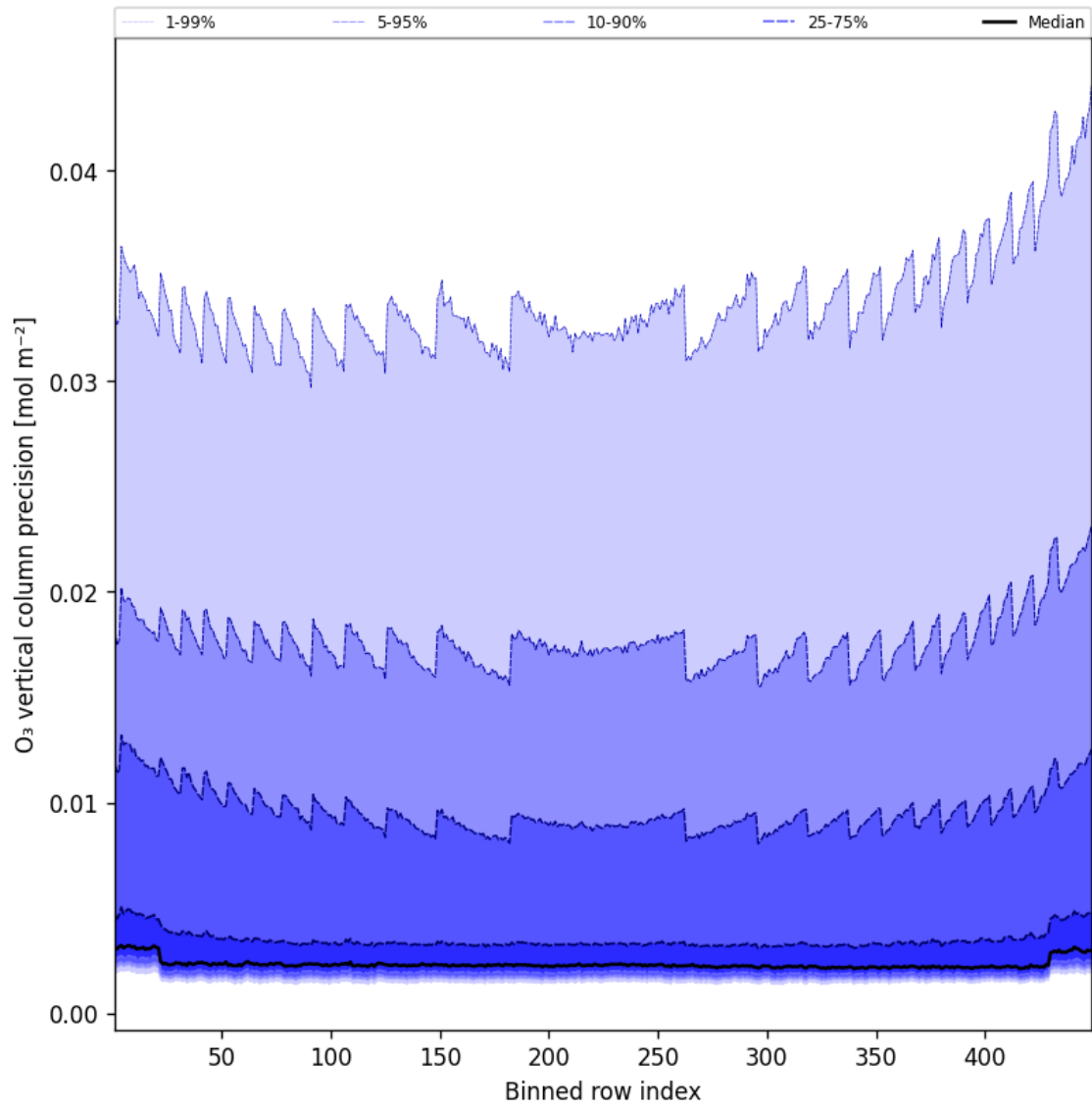
Figure 42: Along track statistics of “O 3 vertical column precision” for 2025-04-01 to 2025-04-02
