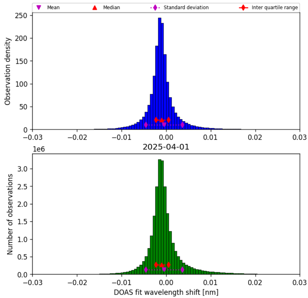
Figure 35: Histogram of “DOAS fit wavelength shift” for 2025-04-01 to 2025-04-02
