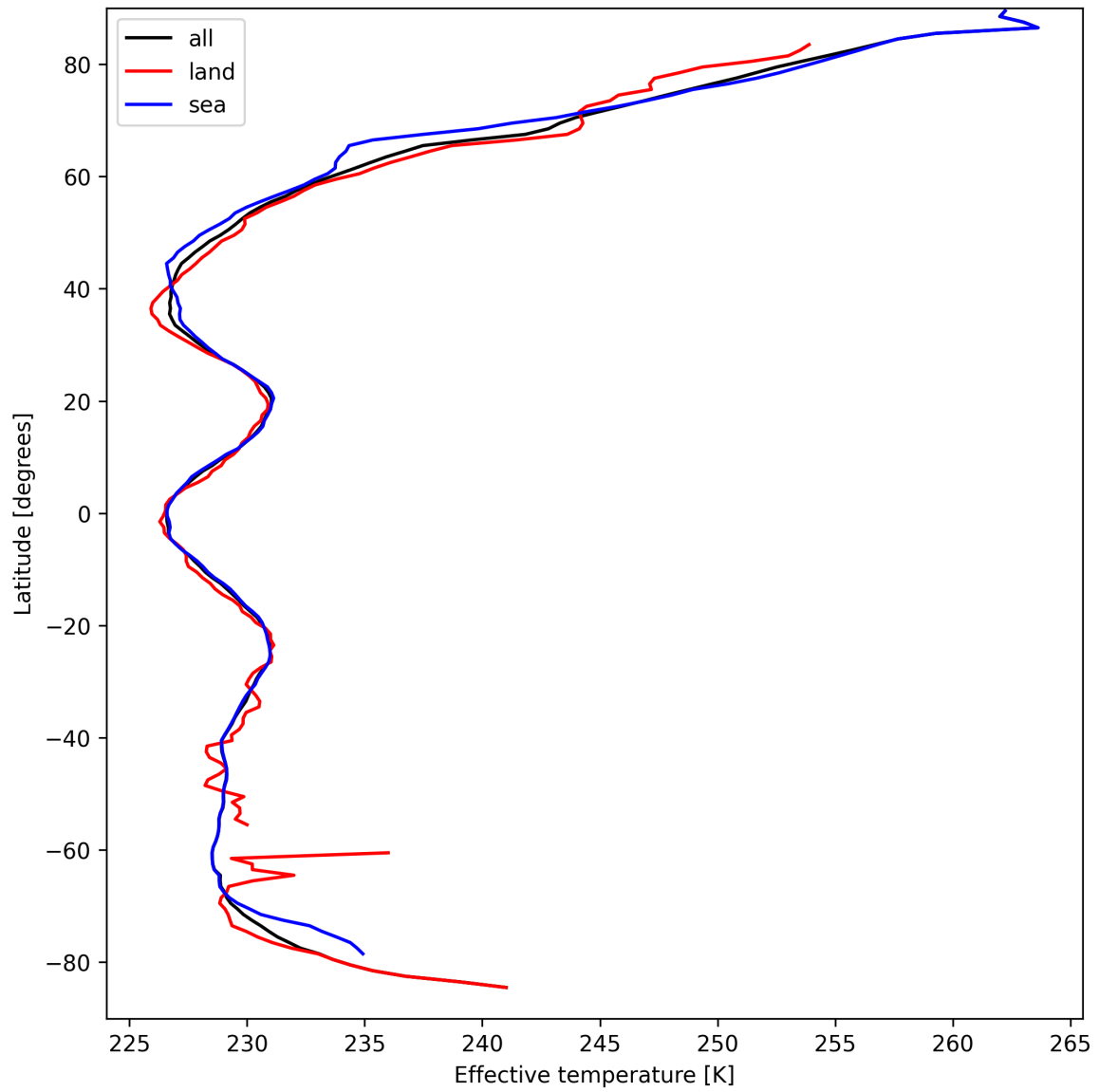
Figure 26: Zonal average of “Effective temperature” for 2025-04-01 to 2025-04-02.
