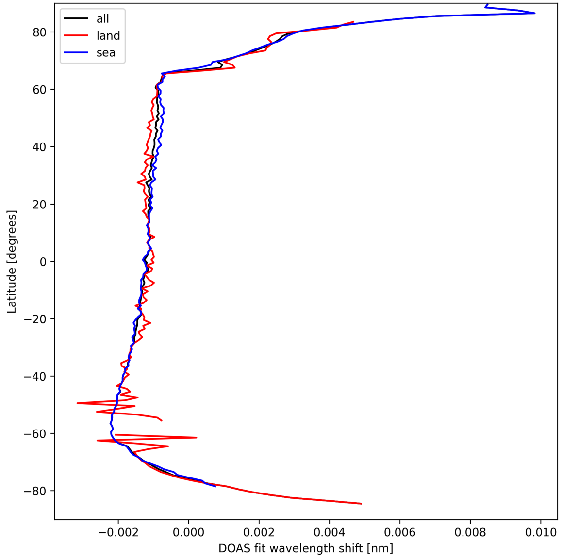
Figure 23: Zonal average of “DOAS fit wavelength shift” for 2025-04-01 to 2025-04-02.
