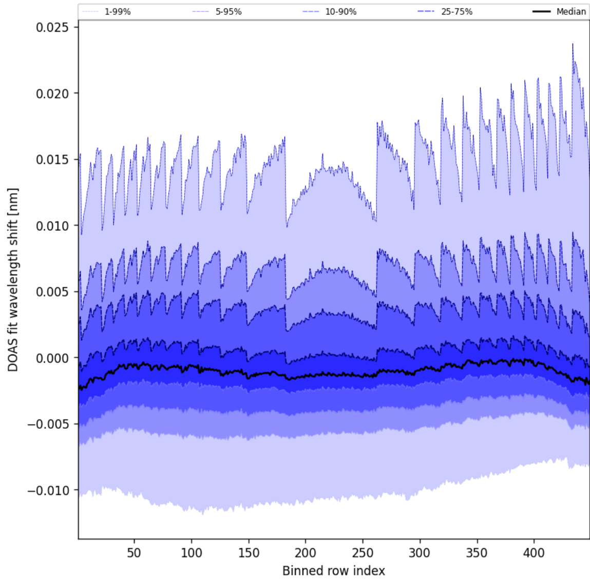
Figure 47: Along track statistics of “DOAS fit wavelength shift” for 2025-04-01 to 2025-04-02
