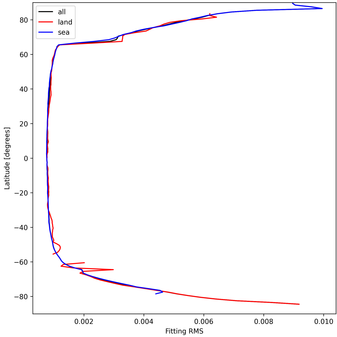
Figure 22: Zonal average of “Fitting RMS” for 2025-04-01 to 2025-04-02.
