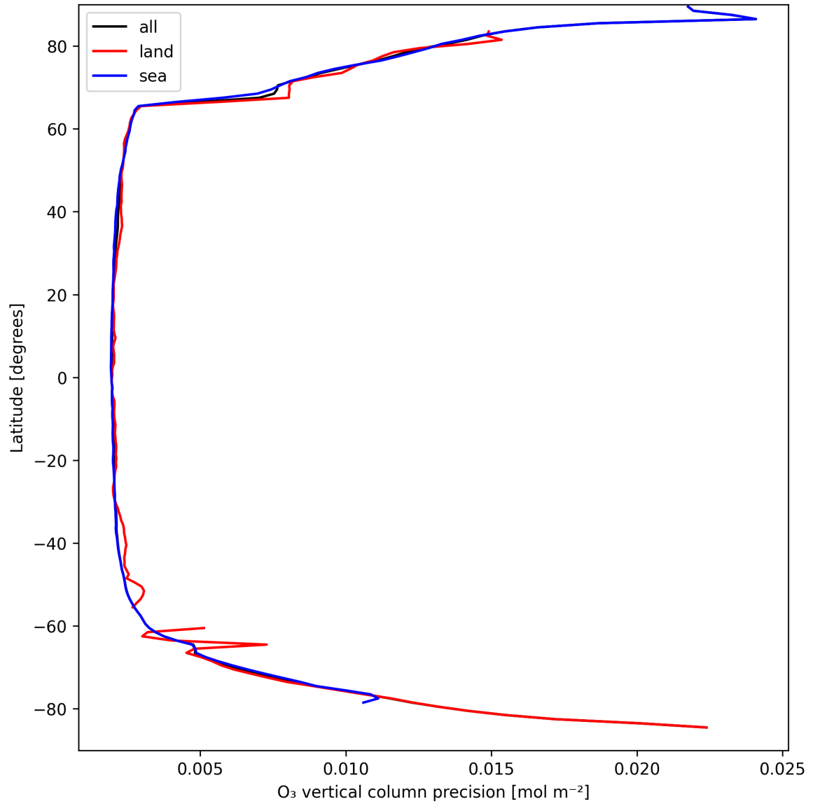
Figure 18: Zonal average of “O 3 vertical column precision” for 2025-04-01 to 2025-04-02.
