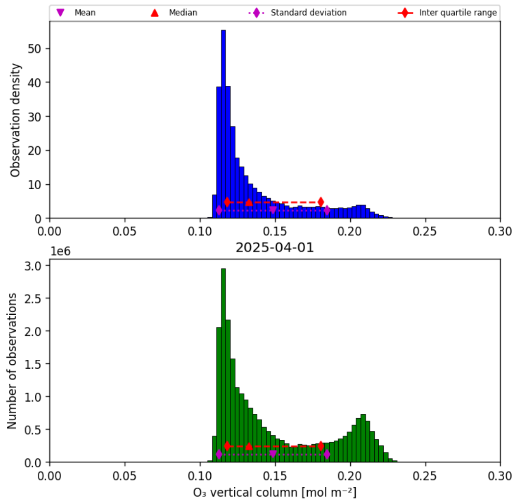
Figure 29: Histogram of “O 3 vertical column” for 2025-04-01 to 2025-04-02
