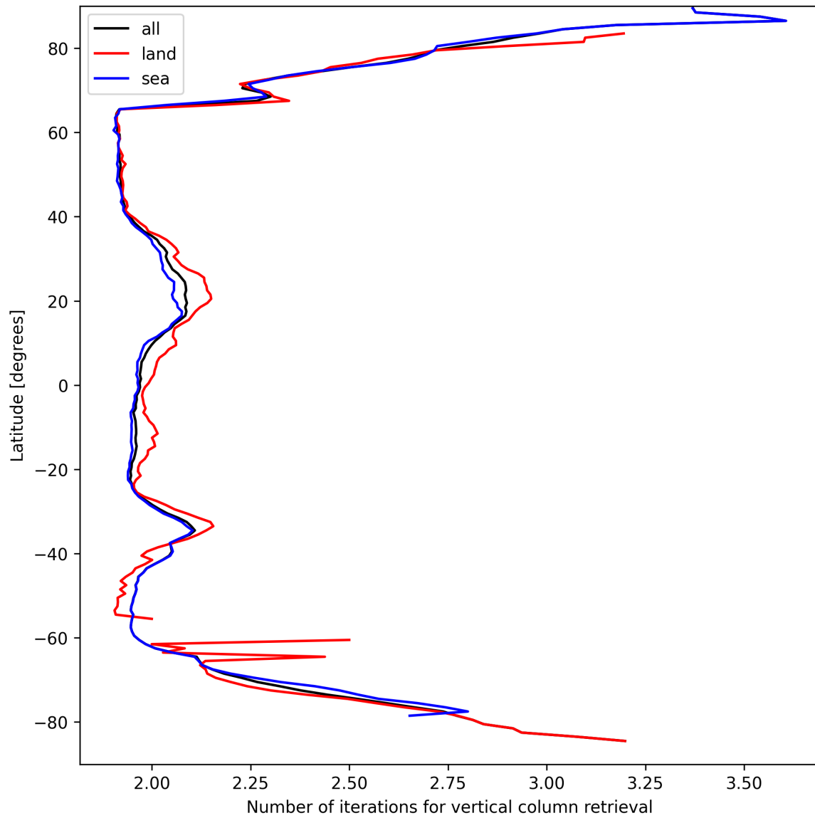
Figure 27: Zonal average of “Number of iterations for vertical column retrieval” for 2025-04-01 to 2025-04-02.
