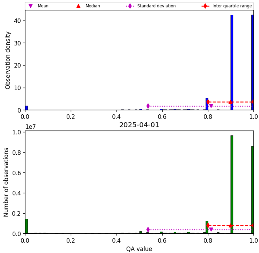
Figure 28: Histogram of “QA value” for 2025-04-01 to 2025-04-02
