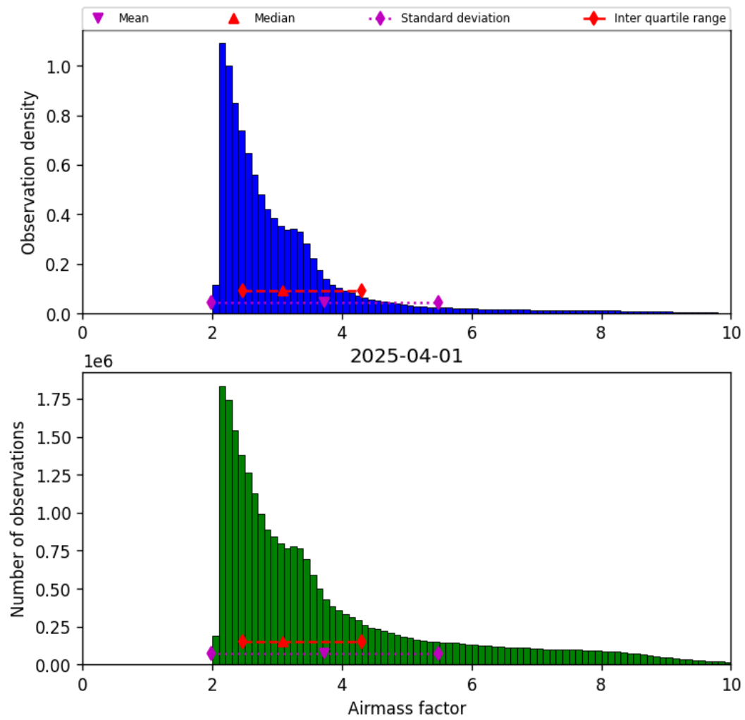
Figure 37: Histogram of “Airmass factor” for 2025-04-01 to 2025-04-02
