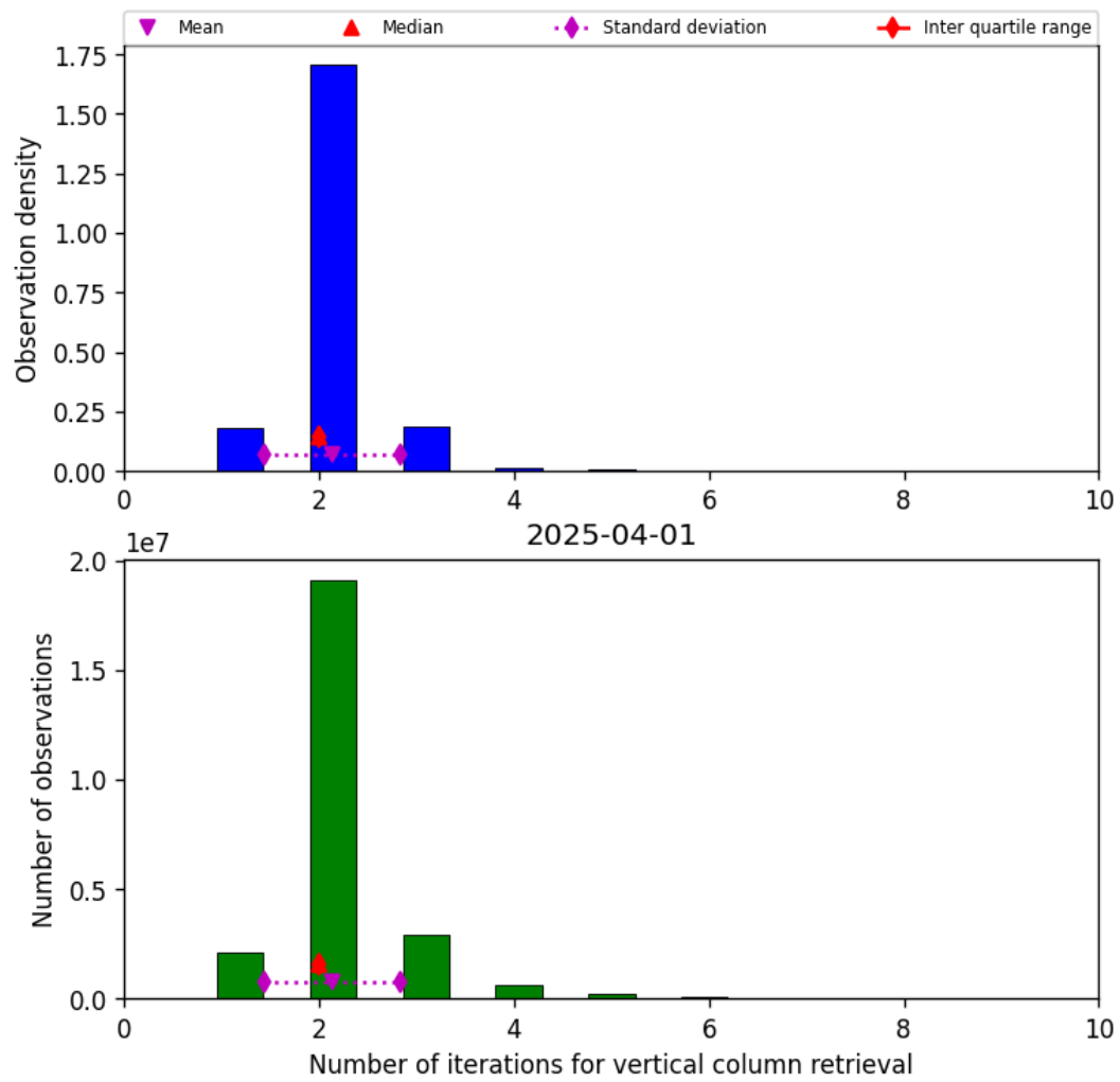
Figure 39: Histogram of “Number of iterations for vertical column retrieval” for 2025-04-01 to 2025-04-02
