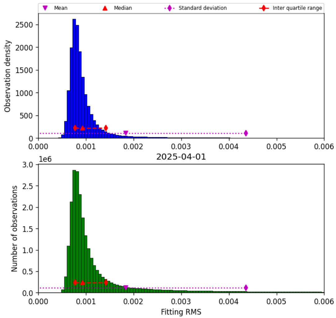
Figure 34: Histogram of “Fitting RMS” for 2025-04-01 to 2025-04-02
