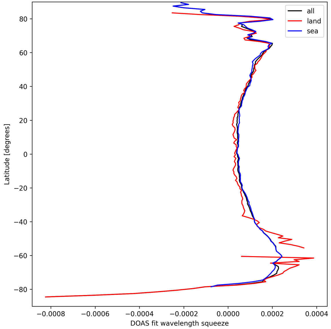
Figure 24: Zonal average of “DOAS fit wavelength squeeze” for 2025-04-01 to 2025-04-02.
