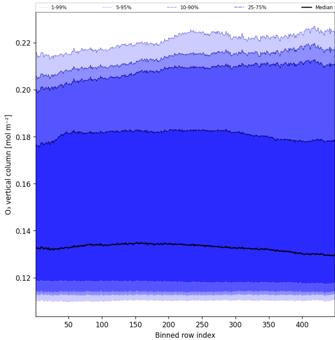
Figure 41: Along track statistics of “O 3 vertical column” for 2025-04-01 to 2025-04-02
