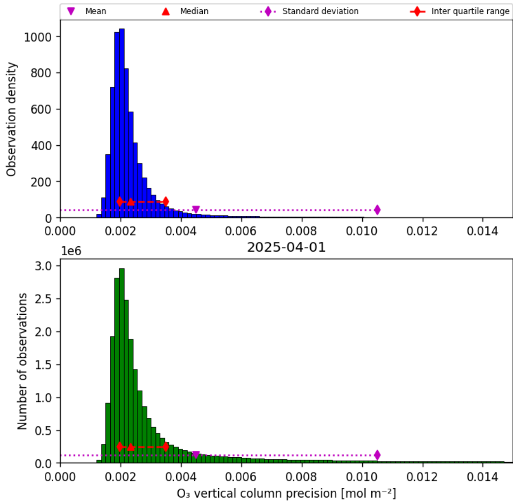
Figure 30: Histogram of “O 3 vertical column precision” for 2025-04-01 to 2025-04-02
