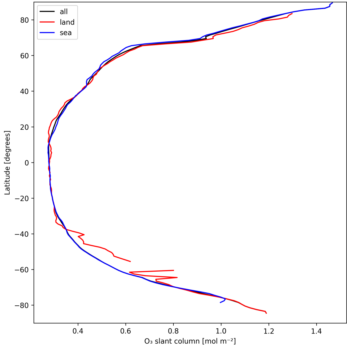
Figure 19: Zonal average of “O 3 slant column” for 2025-04-01 to 2025-04-02.
