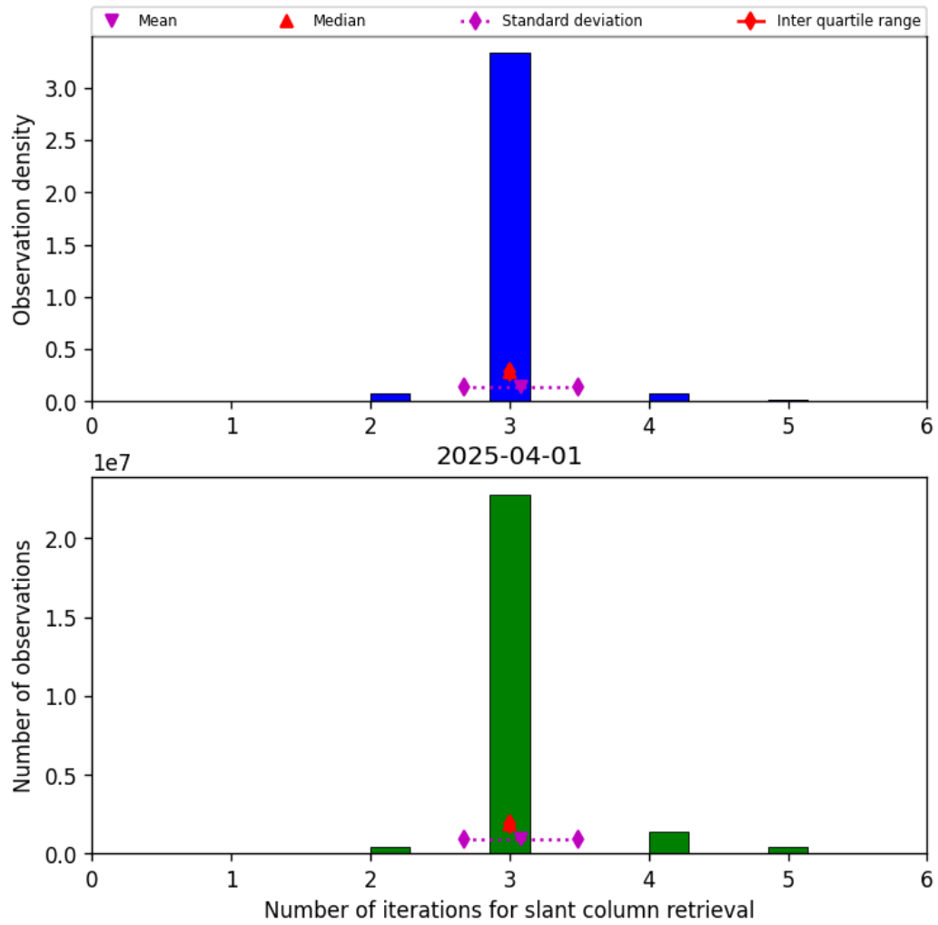
Figure 33: Histogram of “Number of iterations for slant column retrieval” for 2025-04-01 to 2025-04-02
