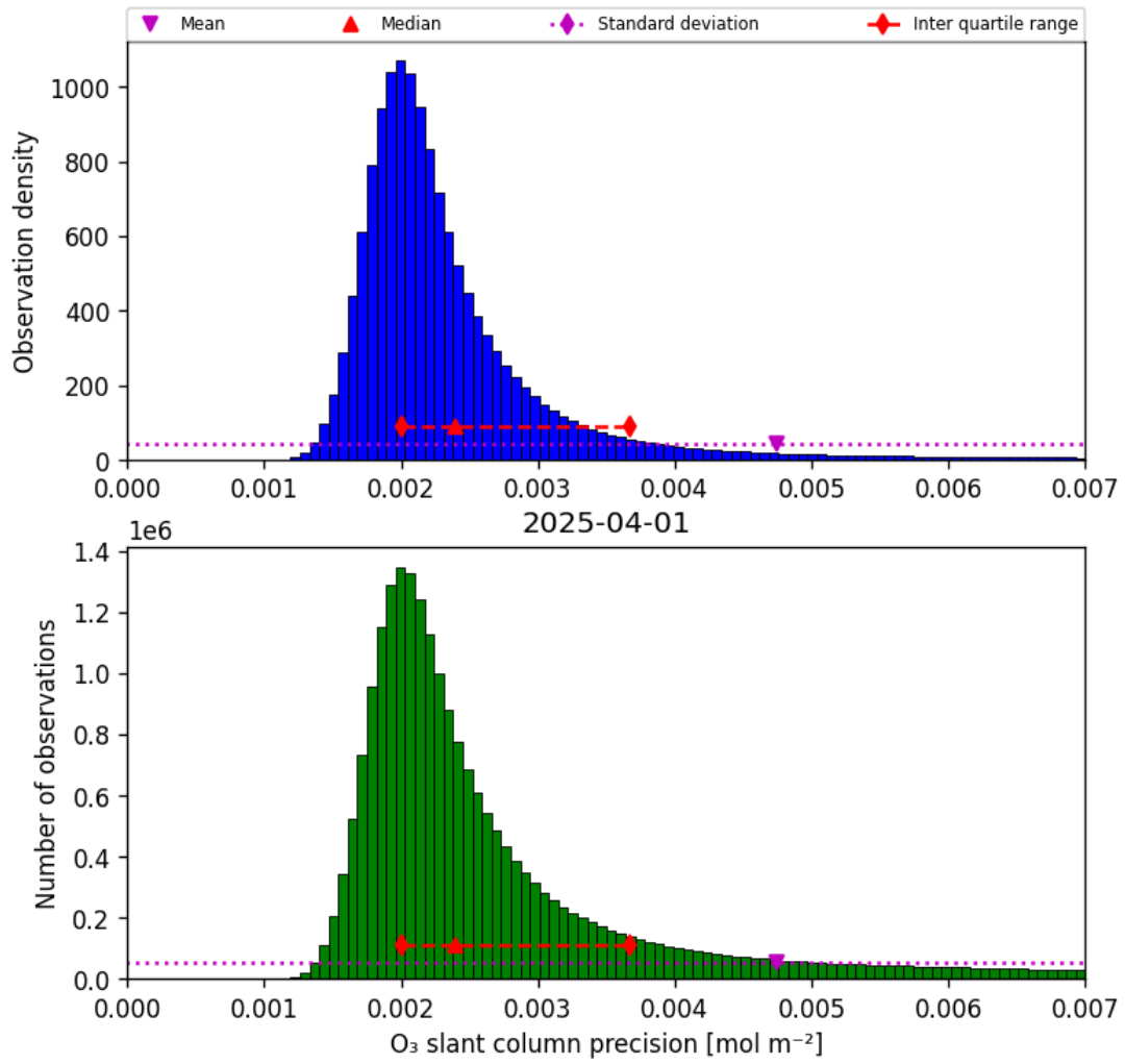
Figure 32: Histogram of “O 3 slant column precision” for 2025-04-01 to 2025-04-02
