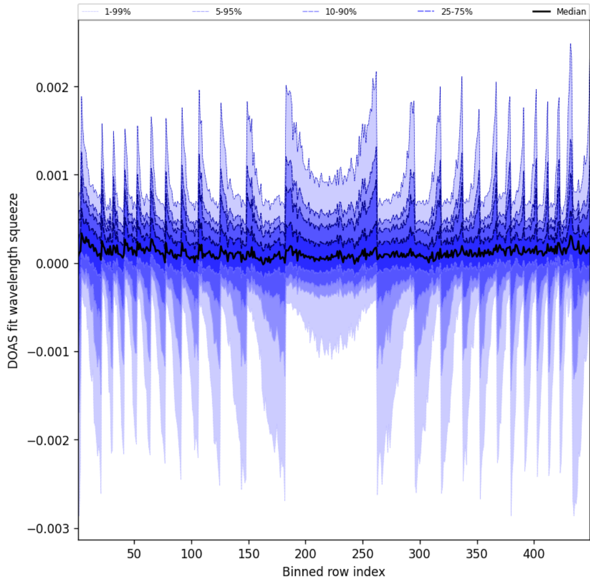
Figure 48: Along track statistics of “DOAS fit wavelength squeeze” for 2025-04-01 to 2025-04-02
