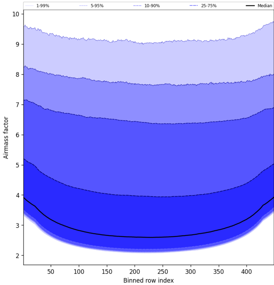
Figure 49: Along track statistics of “Airmass factor” for 2025-04-01 to 2025-04-02
