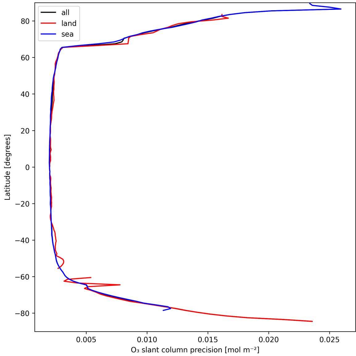
Figure 20: Zonal average of “O 3 slant column precision” for 2025-04-01 to 2025-04-02.
