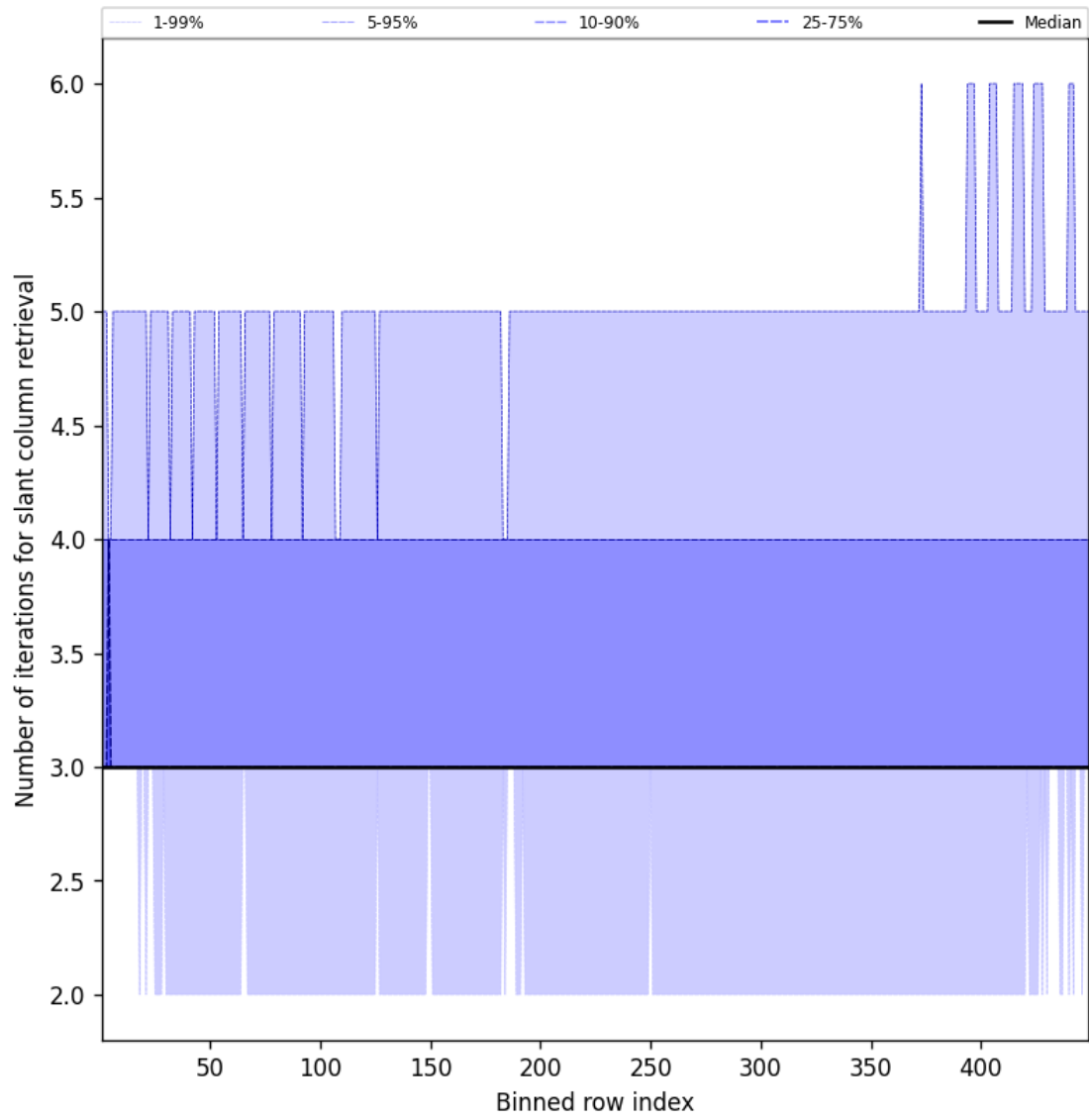
Figure 45: Along track statistics of “Number of iterations for slant column retrieval” for 2025-04-01 to 2025-04-02
