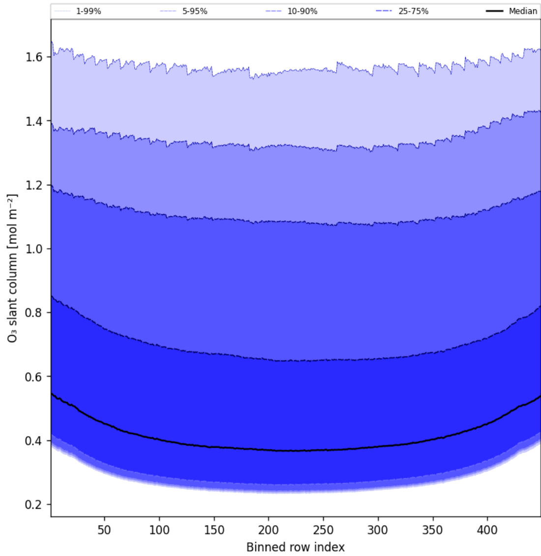
Figure 43: Along track statistics of “O 3 slant column” for 2025-04-01 to 2025-04-02
