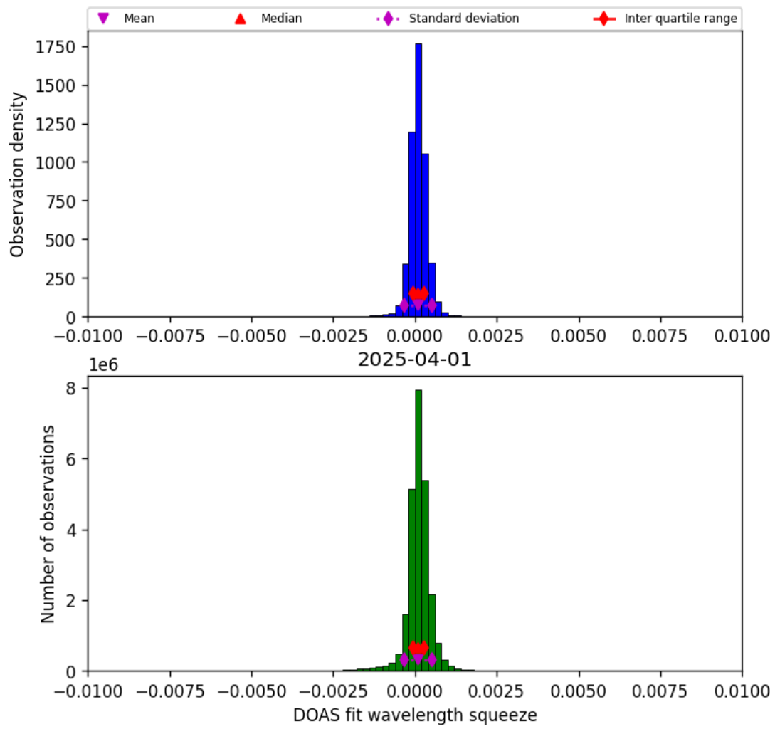
Figure 36: Histogram of “DOAS fit wavelength squeeze” for 2025-04-01 to 2025-04-02
