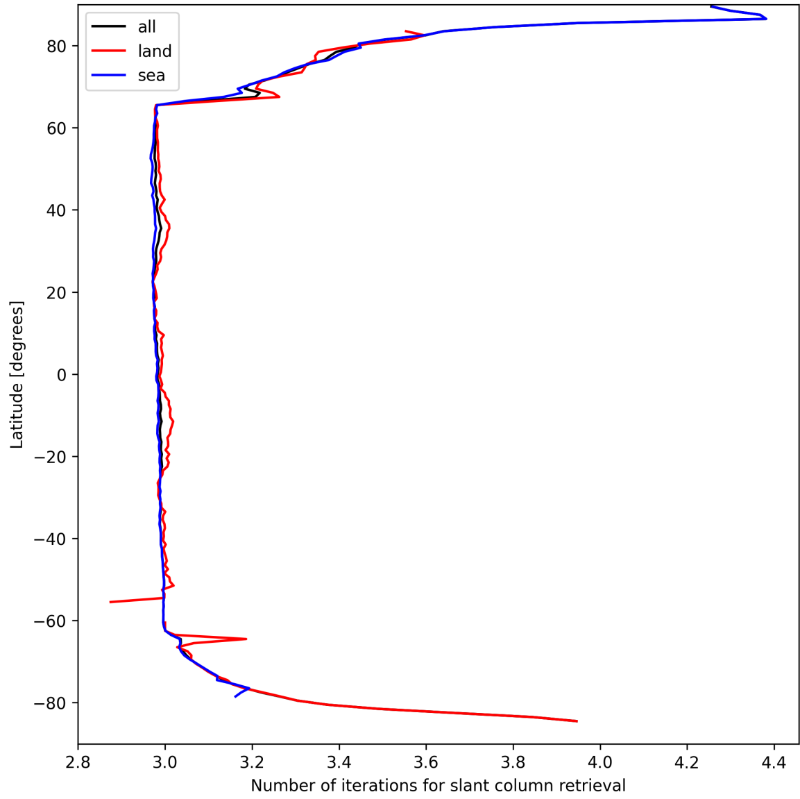
Figure 21: Zonal average of “Number of iterations for slant column retrieval” for 2025-04-01 to 2025-04-02.
