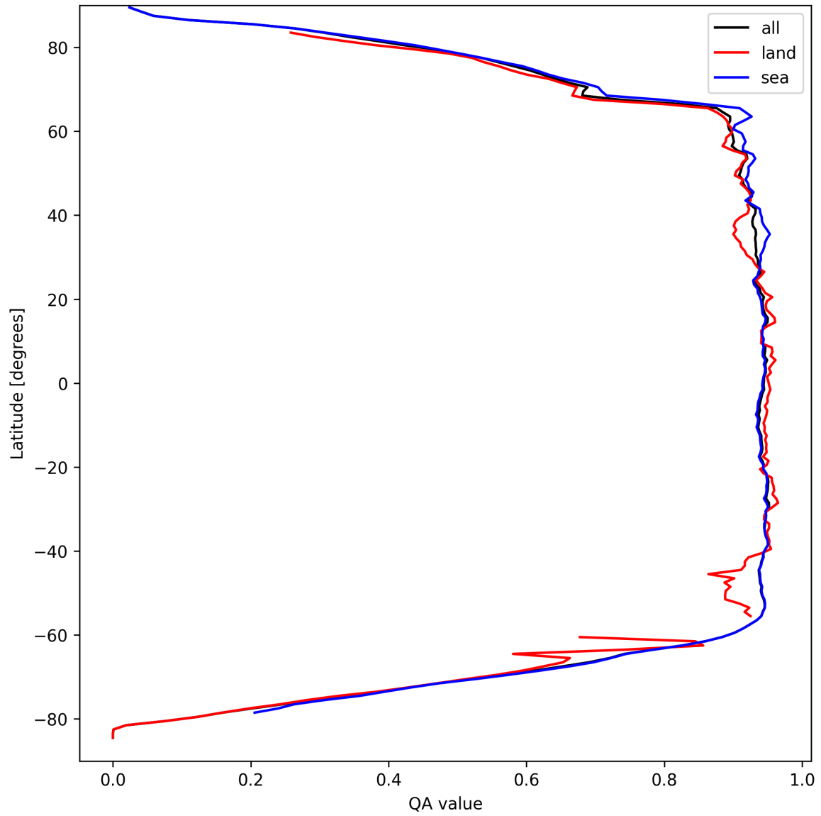
Figure 16: Zonal average of “QA value” for 2025-04-01 to 2025-04-02.
