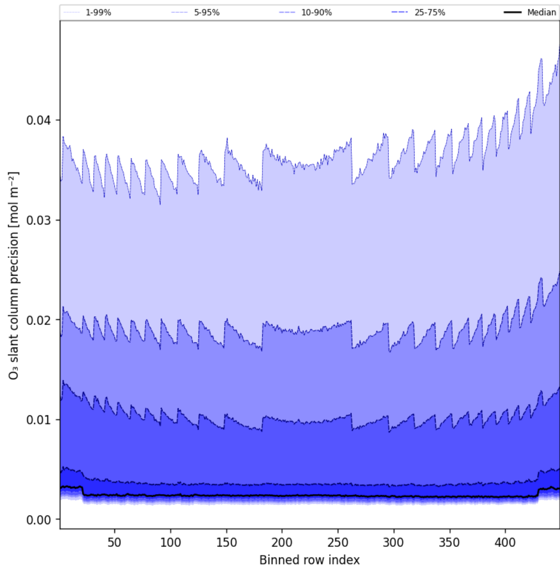
Figure 44: Along track statistics of “O 3 slant column precision” for 2025-04-01 to 2025-04-02
