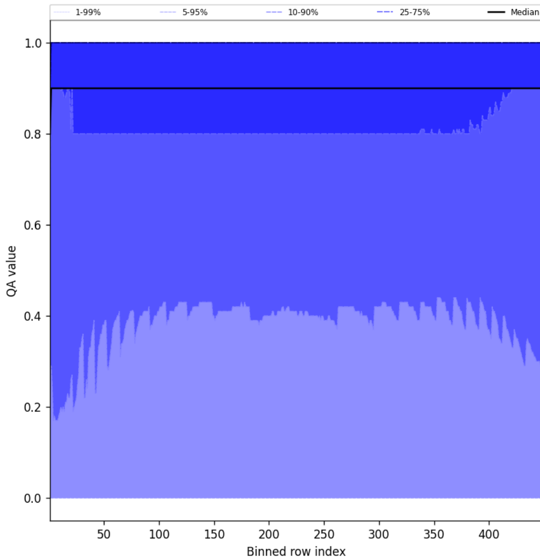
Figure 40: Along track statistics of “QA value” for 2025-04-01 to 2025-04-02
