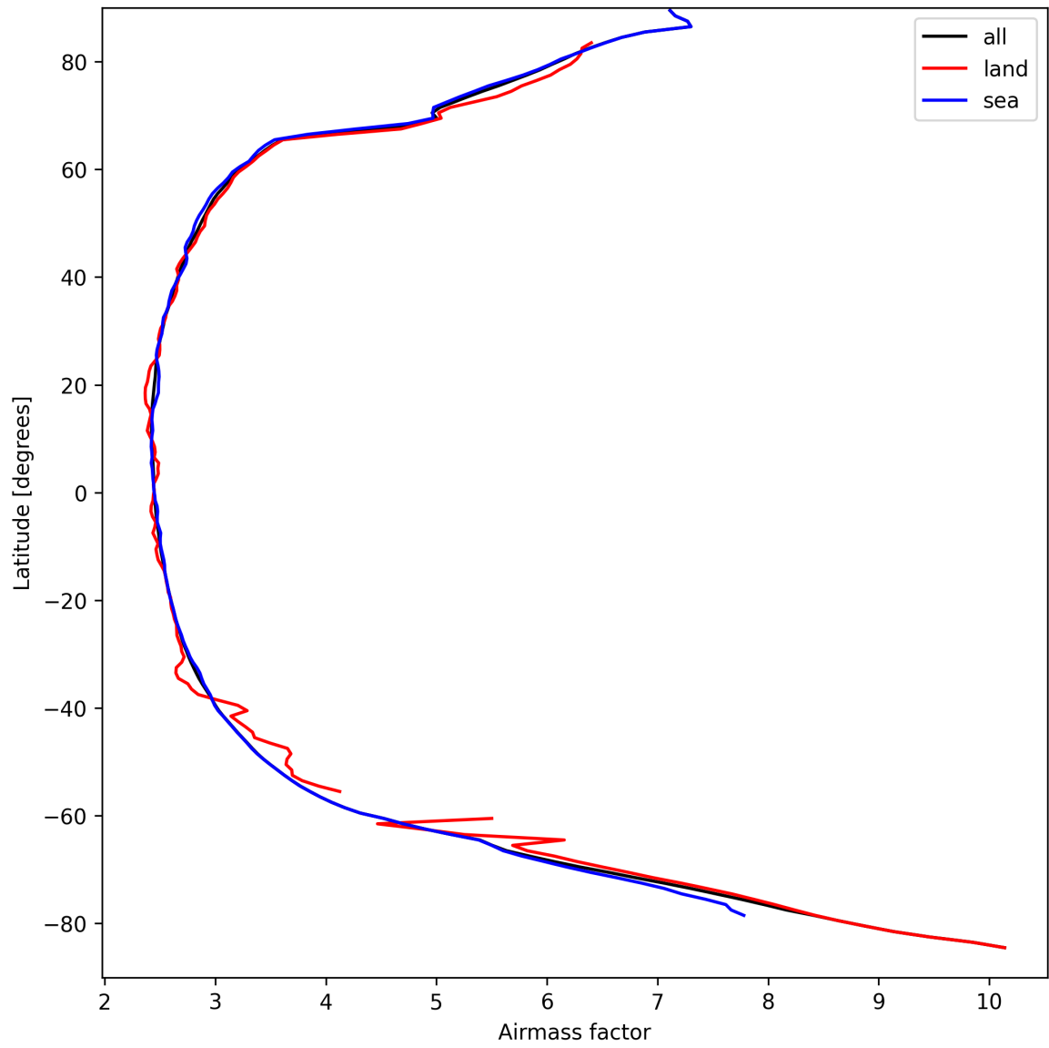
Figure 25: Zonal average of “Airmass factor” for 2025-04-01 to 2025-04-02.
