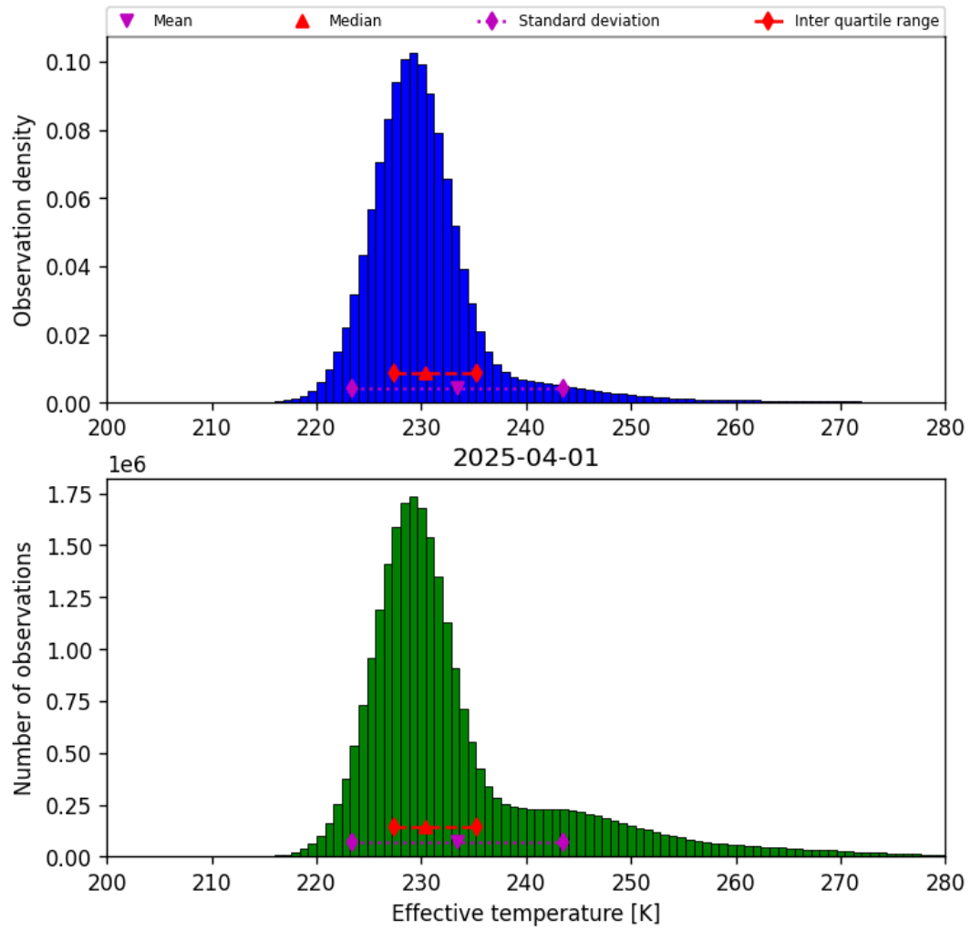
Figure 38: Histogram of “Effective temperature” for 2025-04-01 to 2025-04-02
