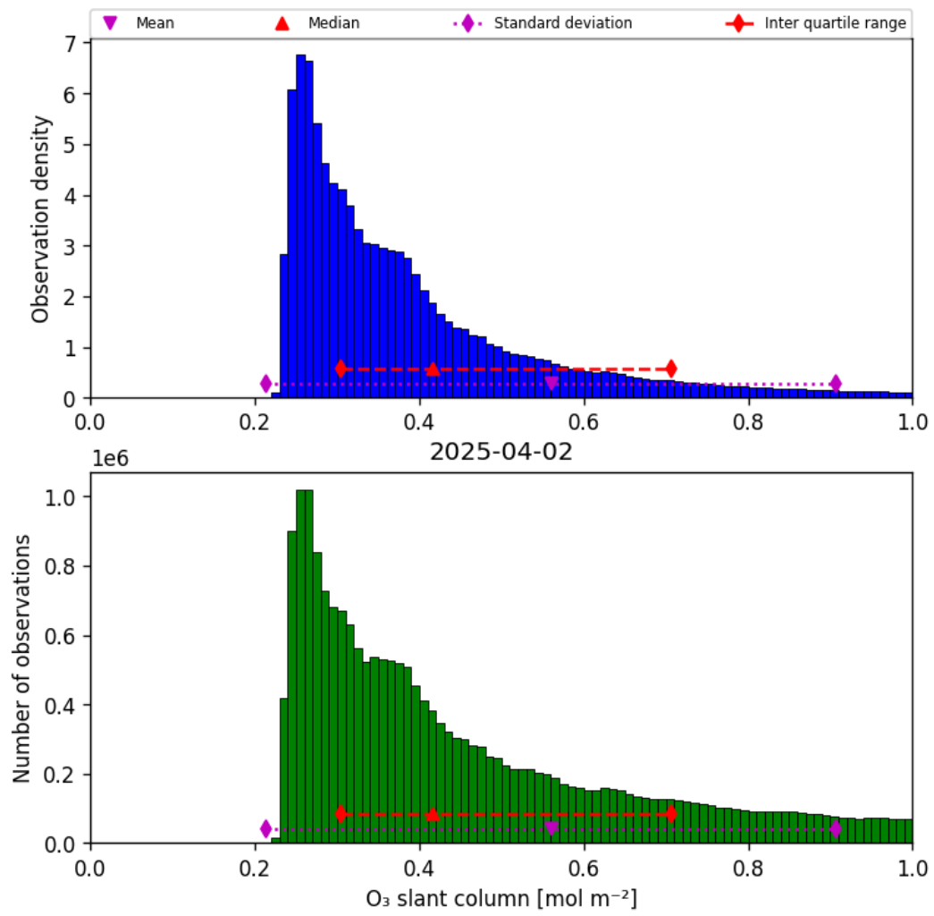
Figure 31: Histogram of “O 3 slant column” for 2025-04-02 to 2025-04-03
