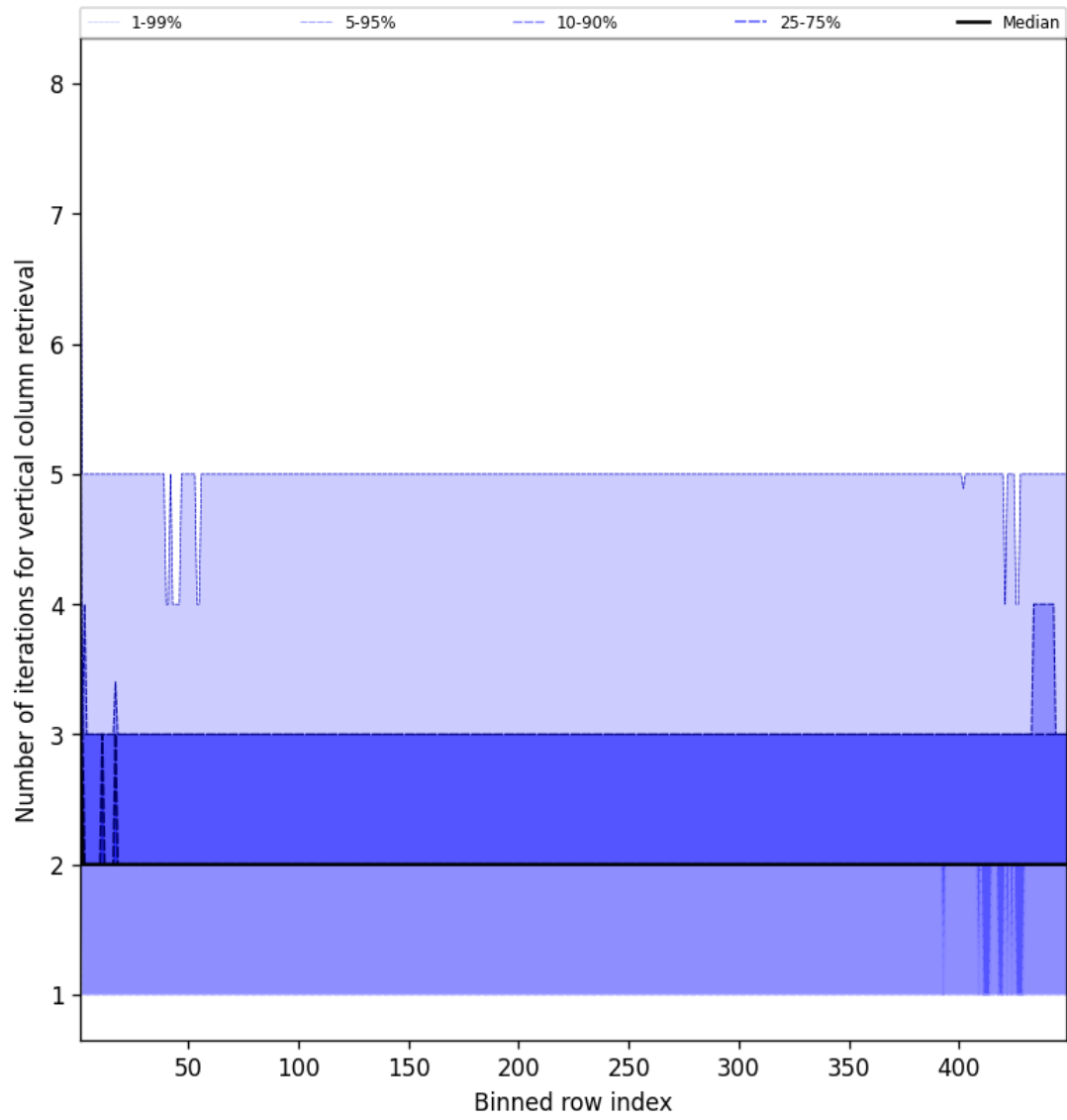
Figure 51: Along track statistics of “Number of iterations for vertical column retrieval” for 2025-04-02 to 2025-04-03
