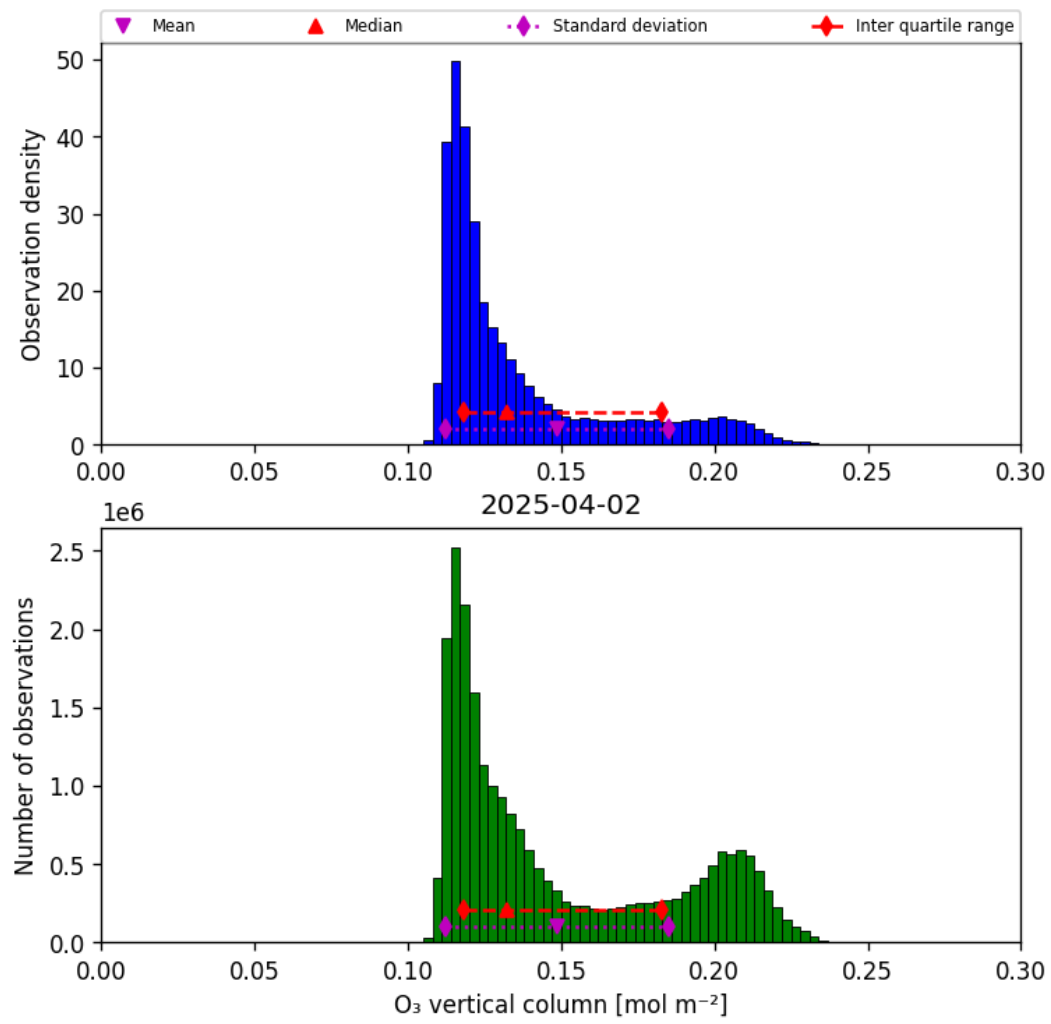
Figure 29: Histogram of “O 3 vertical column” for 2025-04-02 to 2025-04-03
