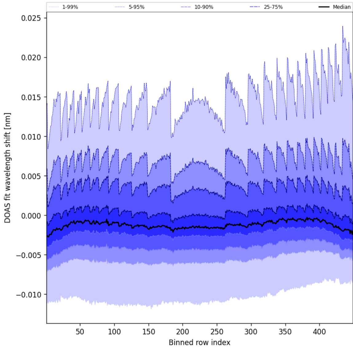
Figure 47: Along track statistics of "DOAS fit wavelength shift" for 2025-04-02 to 2025-04-03
