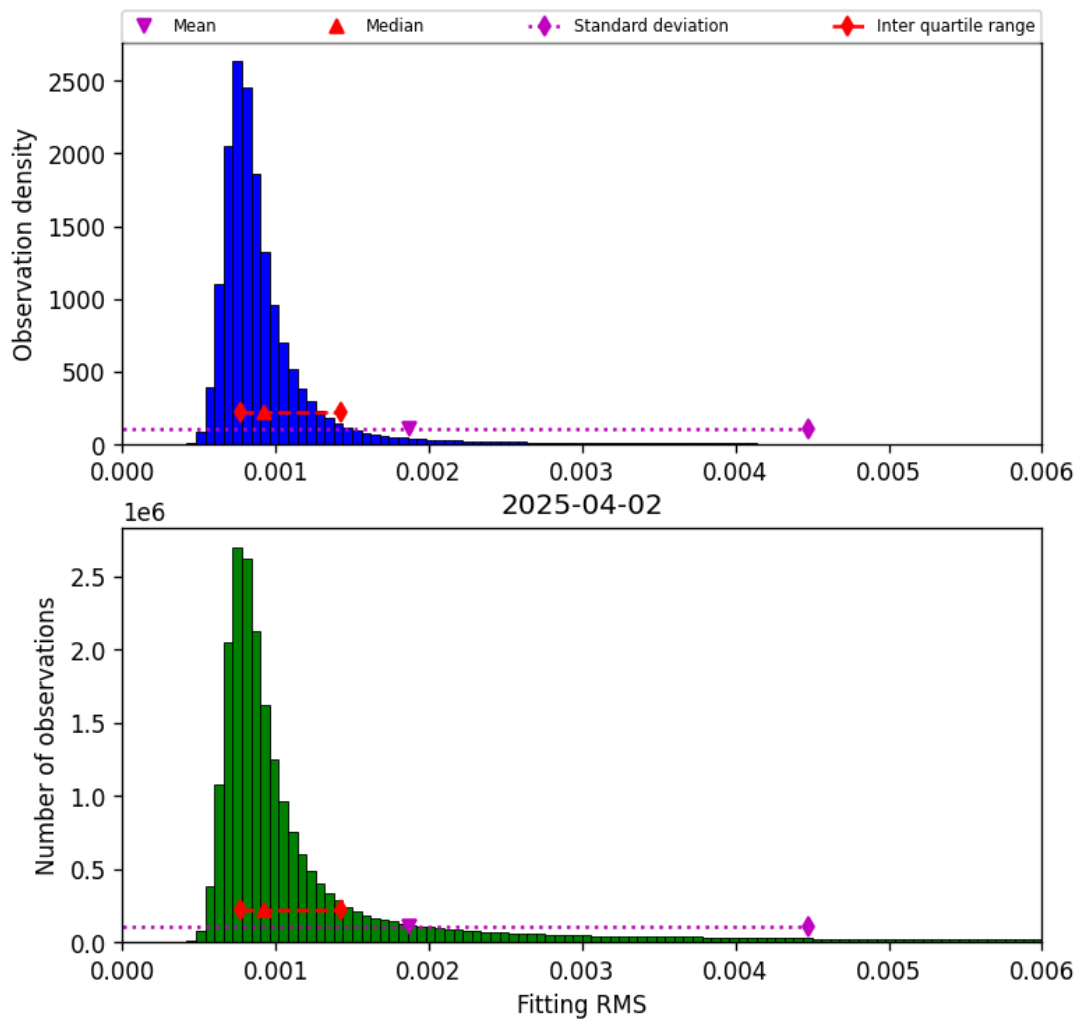
Figure 34: Histogram of “Fitting RMS” for 2025-04-02 to 2025-04-03
