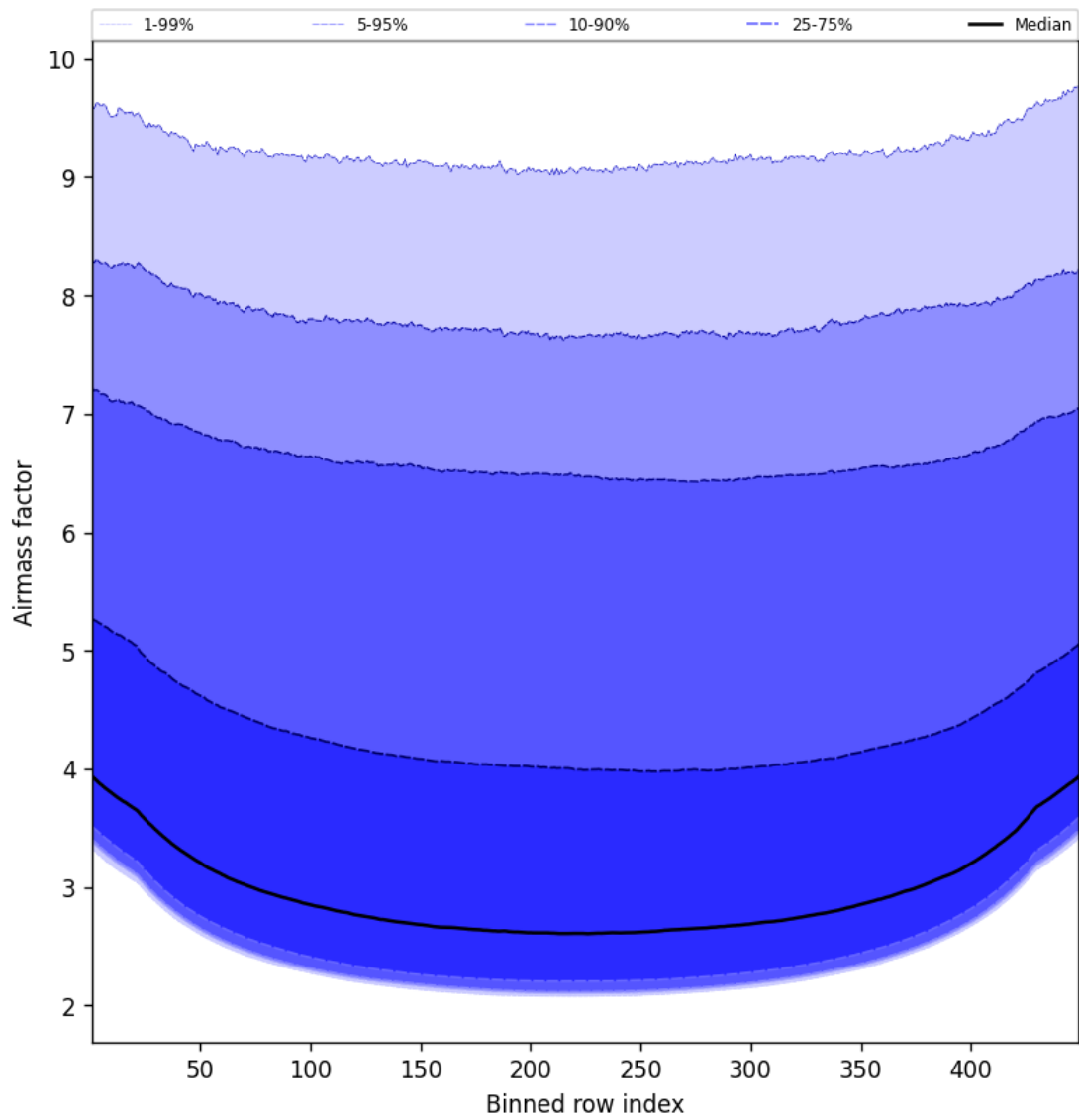
Figure 49: Along track statistics of “Airmass factor” for 2025-04-02 to 2025-04-03
