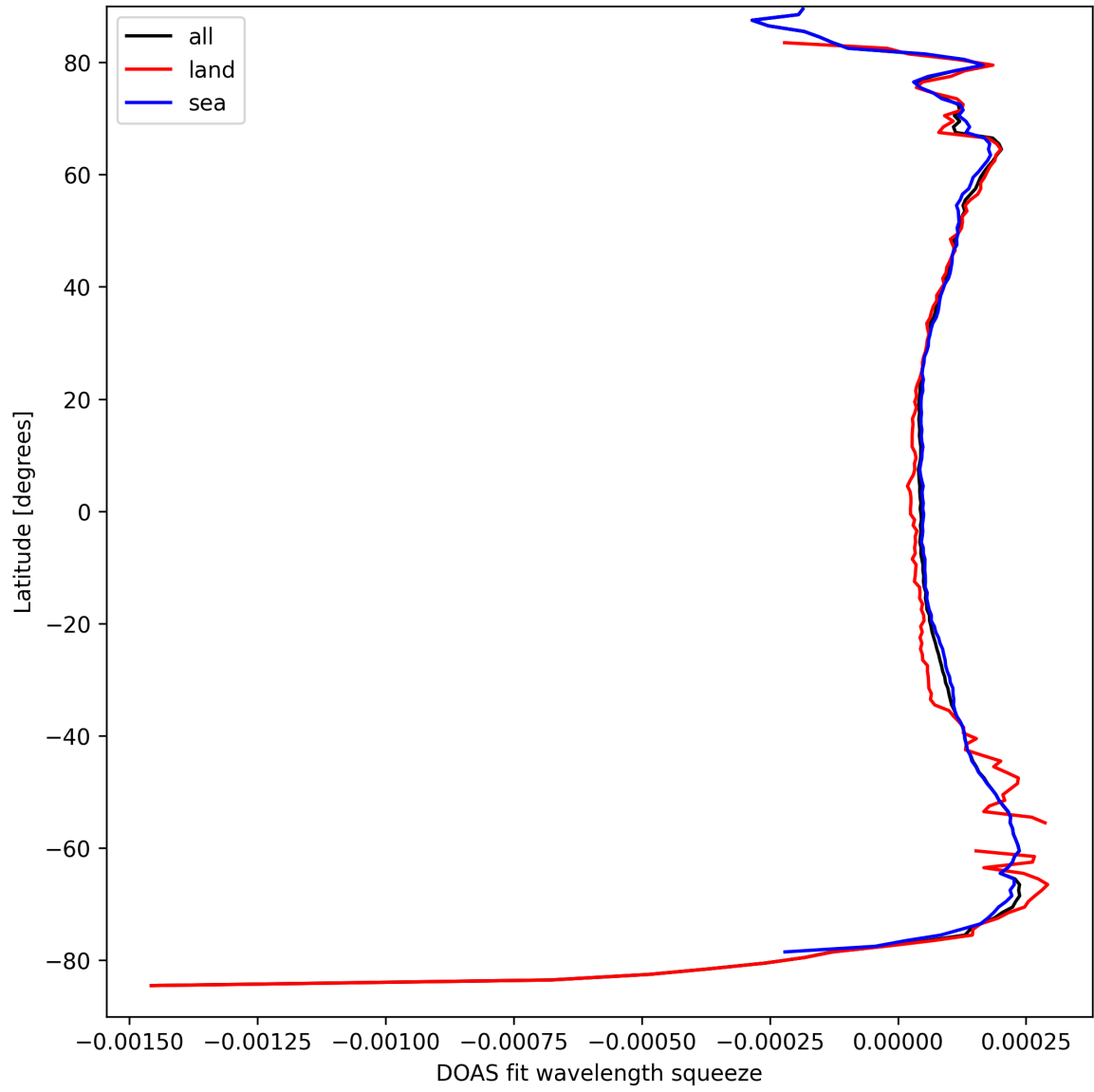
Figure 24: Zonal average of "DOAS fit wavelength squeeze" for 2025-04-02 to 2025-04-03.
