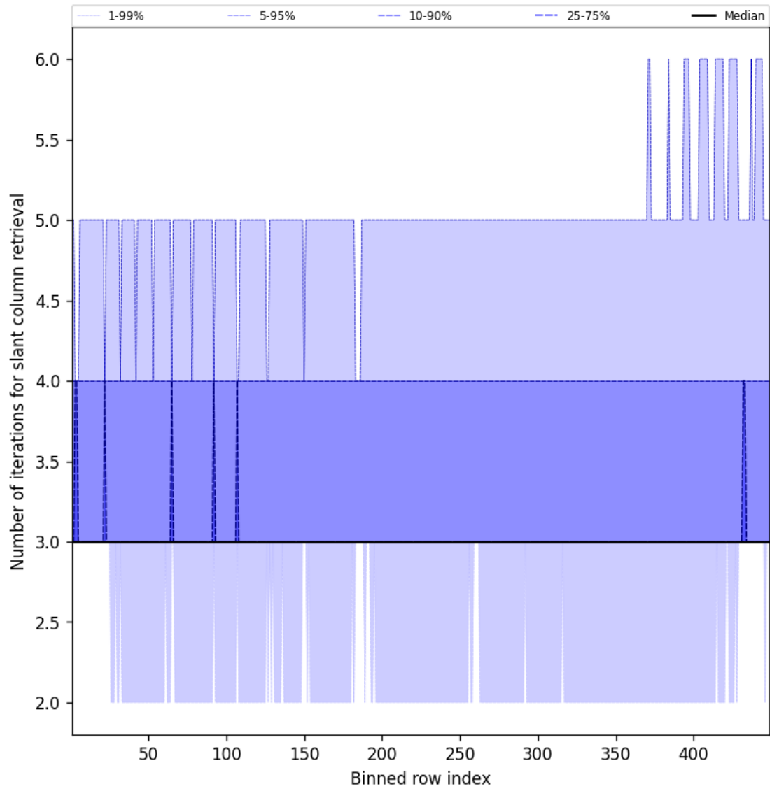
Figure 45: Along track statistics of “Number of iterations for slant column retrieval” for 2025-04-02 to 2025-04-03
