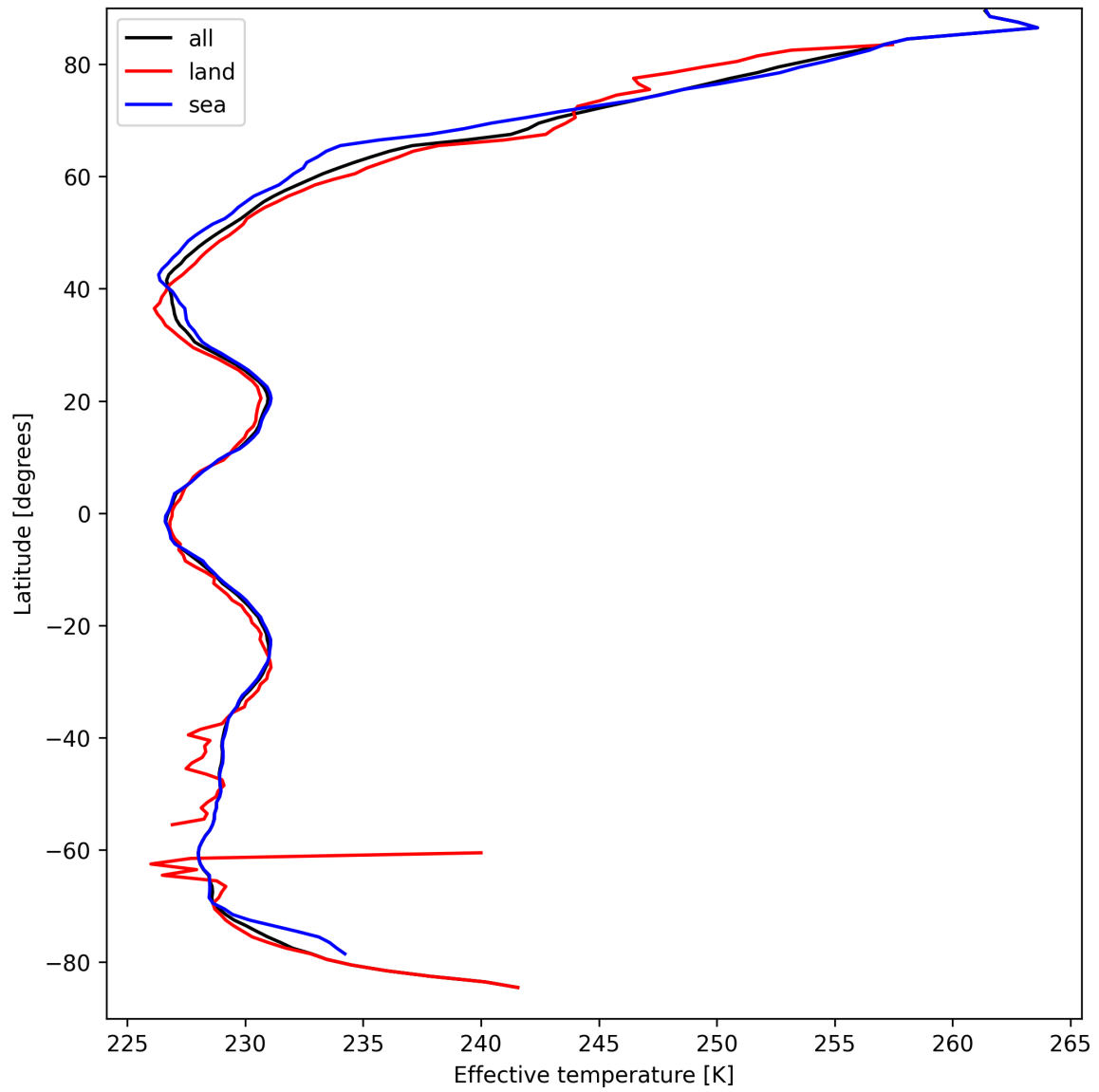
Figure 26: Zonal average of “Effective temperature” for 2025-04-02 to 2025-04-03.
