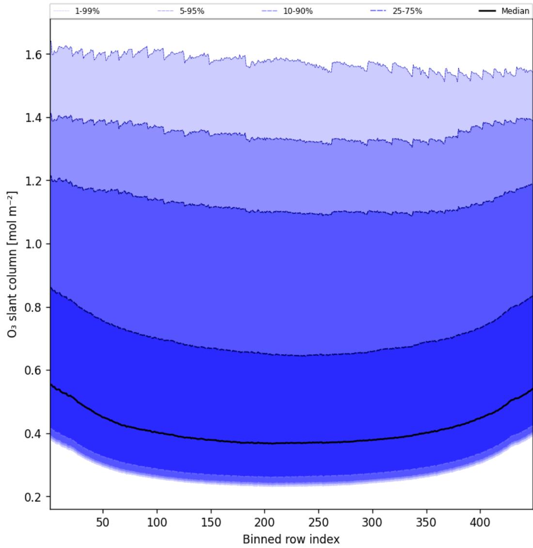
Figure 43: Along track statistics of “O 3 slant column” for 2025-04-02 to 2025-04-03
