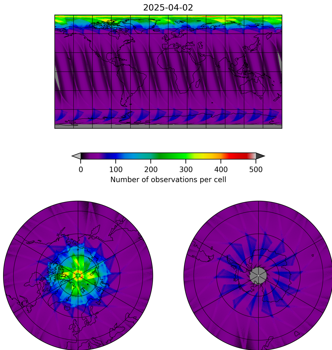
Figure 15: Map of the number of observations for 2025-04-02 to 2025-04-03
