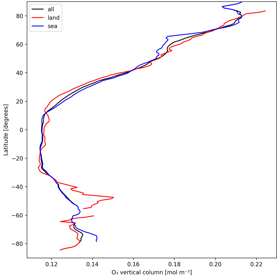
Figure 17: Zonal average of “O 3 vertical column” for 2025-04-02 to 2025-04-03.
