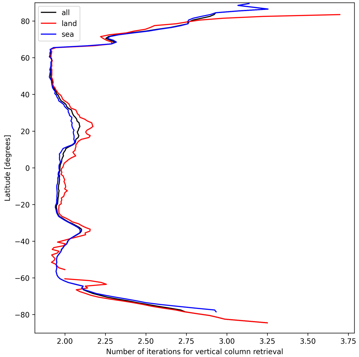
Figure 27: Zonal average of “Number of iterations for vertical column retrieval” for 2025-04-02 to 2025-04-03.
