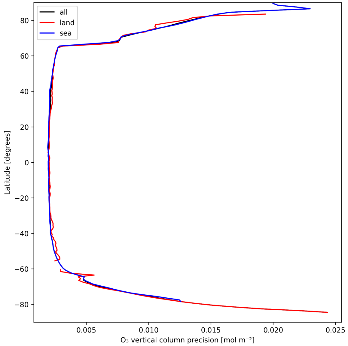
Figure 18: Zonal average of “O 3 vertical column precision” for 2025-04-02 to 2025-04-03.
