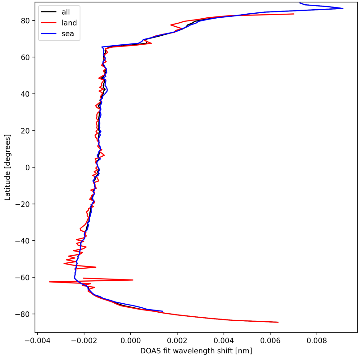
Figure 23: Zonal average of “DOAS fit wavelength shift” for 2025-04-02 to 2025-04-03.
