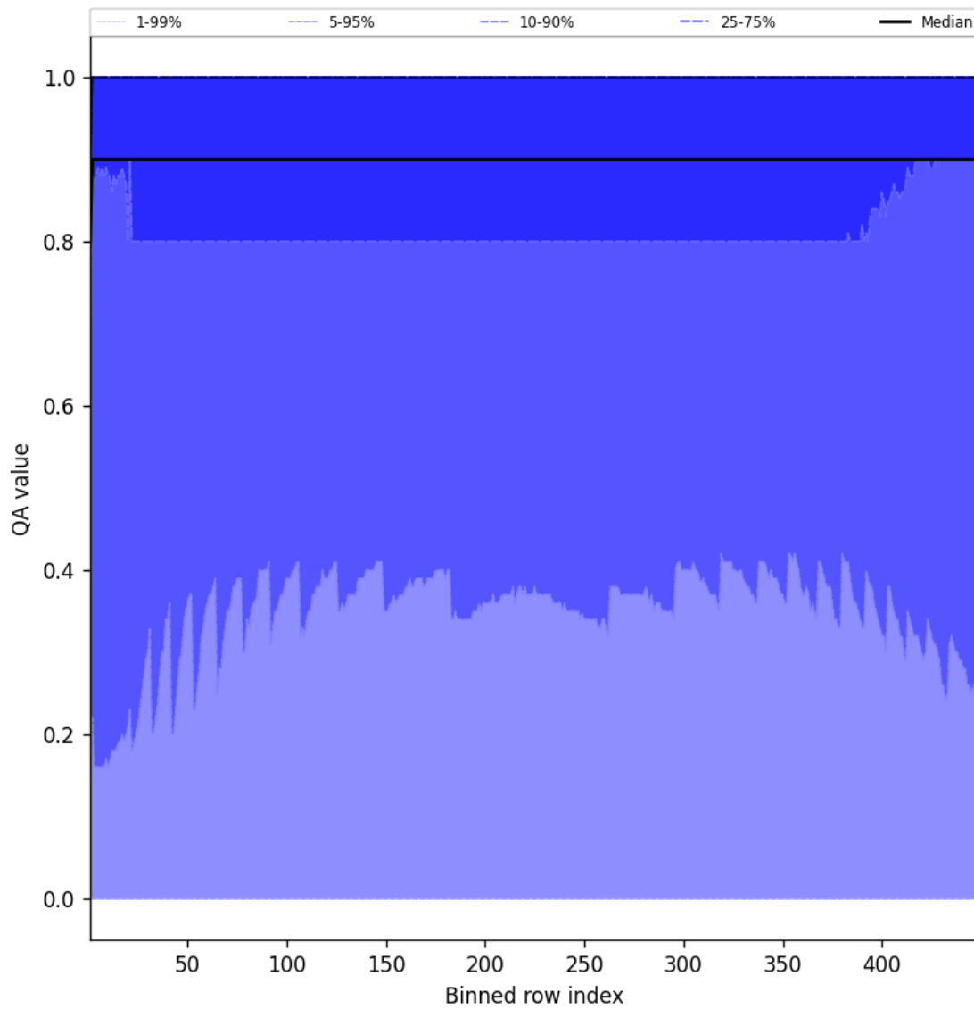
Figure 40: Along track statistics of “QA value” for 2025-04-02 to 2025-04-03
