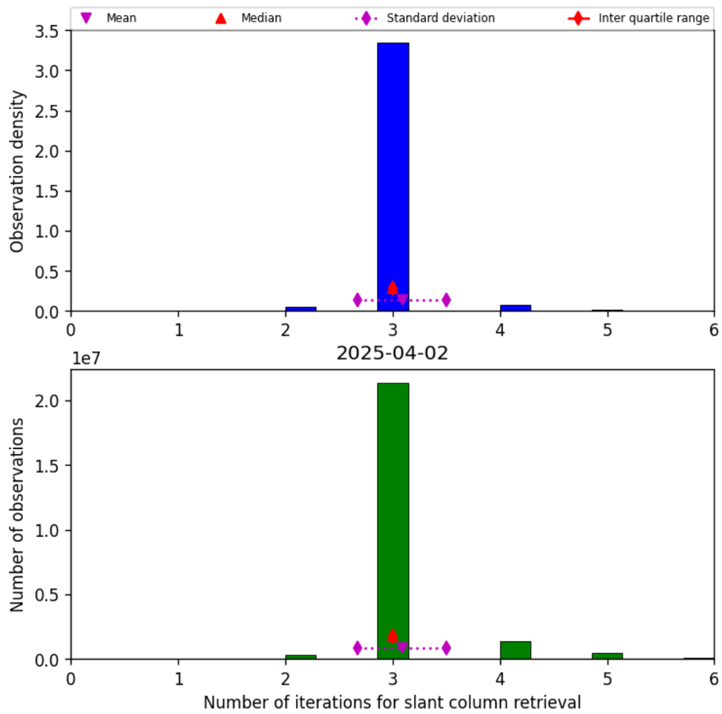
Figure 33: Histogram of “Number of iterations for slant column retrieval” for 2025-04-02 to 2025-04-03
