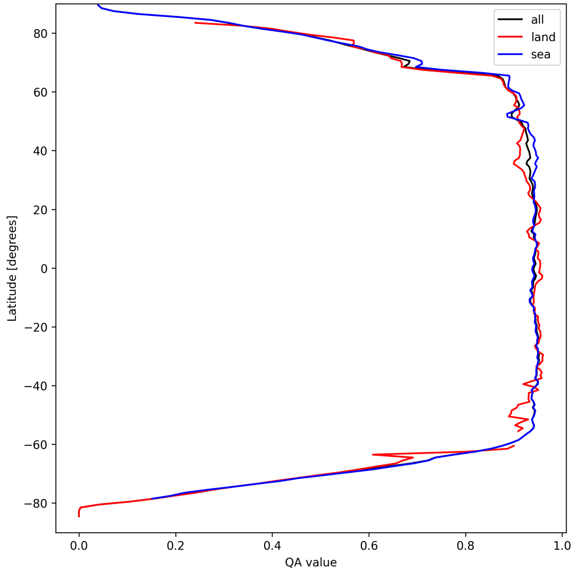
Figure 16: Zonal average of “QA value” for 2025-04-02 to 2025-04-03.
