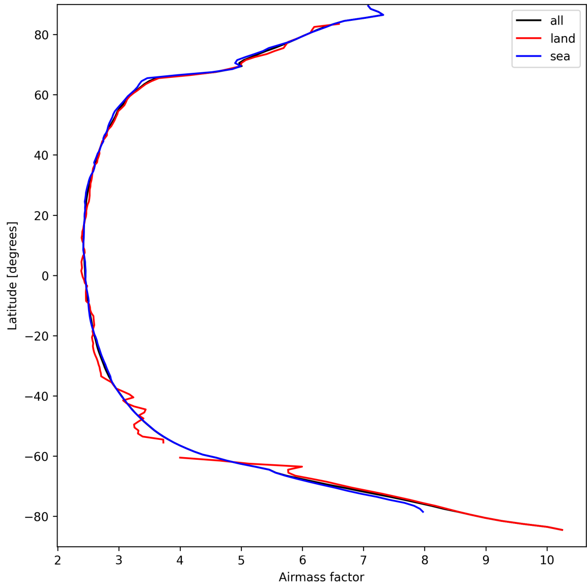
Figure 25: Zonal average of “Airmass factor” for 2025-04-02 to 2025-04-03.
