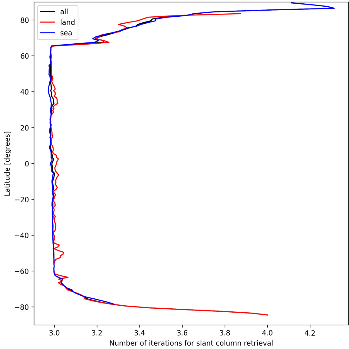
Figure 21: Zonal average of “Number of iterations for slant column retrieval” for 2025-04-02 to 2025-04-03.
