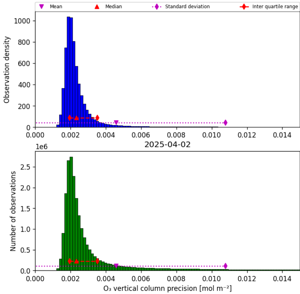
Figure 30: Histogram of “O 3 vertical column precision” for 2025-04-02 to 2025-04-03
