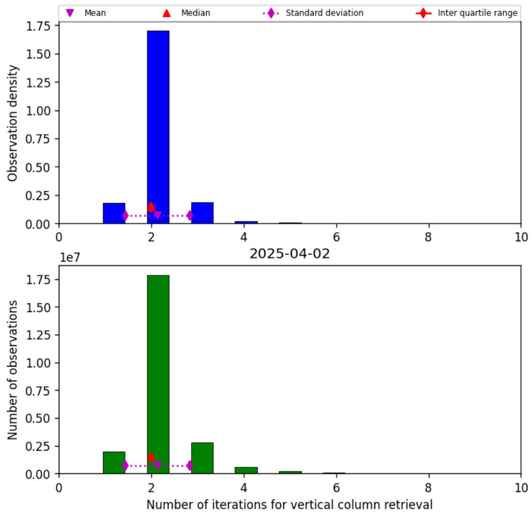
Figure 39: Histogram of “Number of iterations for vertical column retrieval” for 2025-04-02 to 2025-04-03
