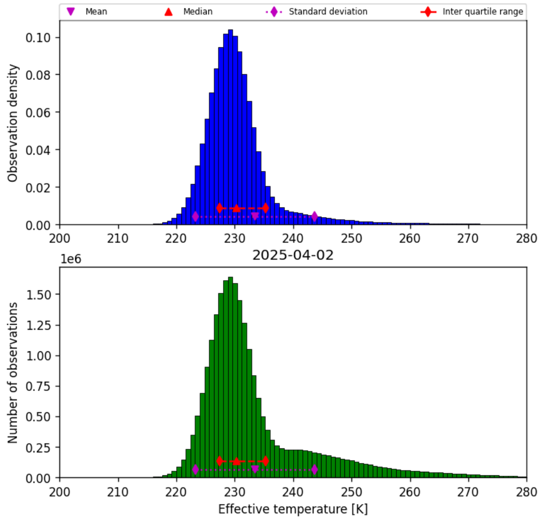
Figure 38: Histogram of “Effective temperature” for 2025-04-02 to 2025-04-03
