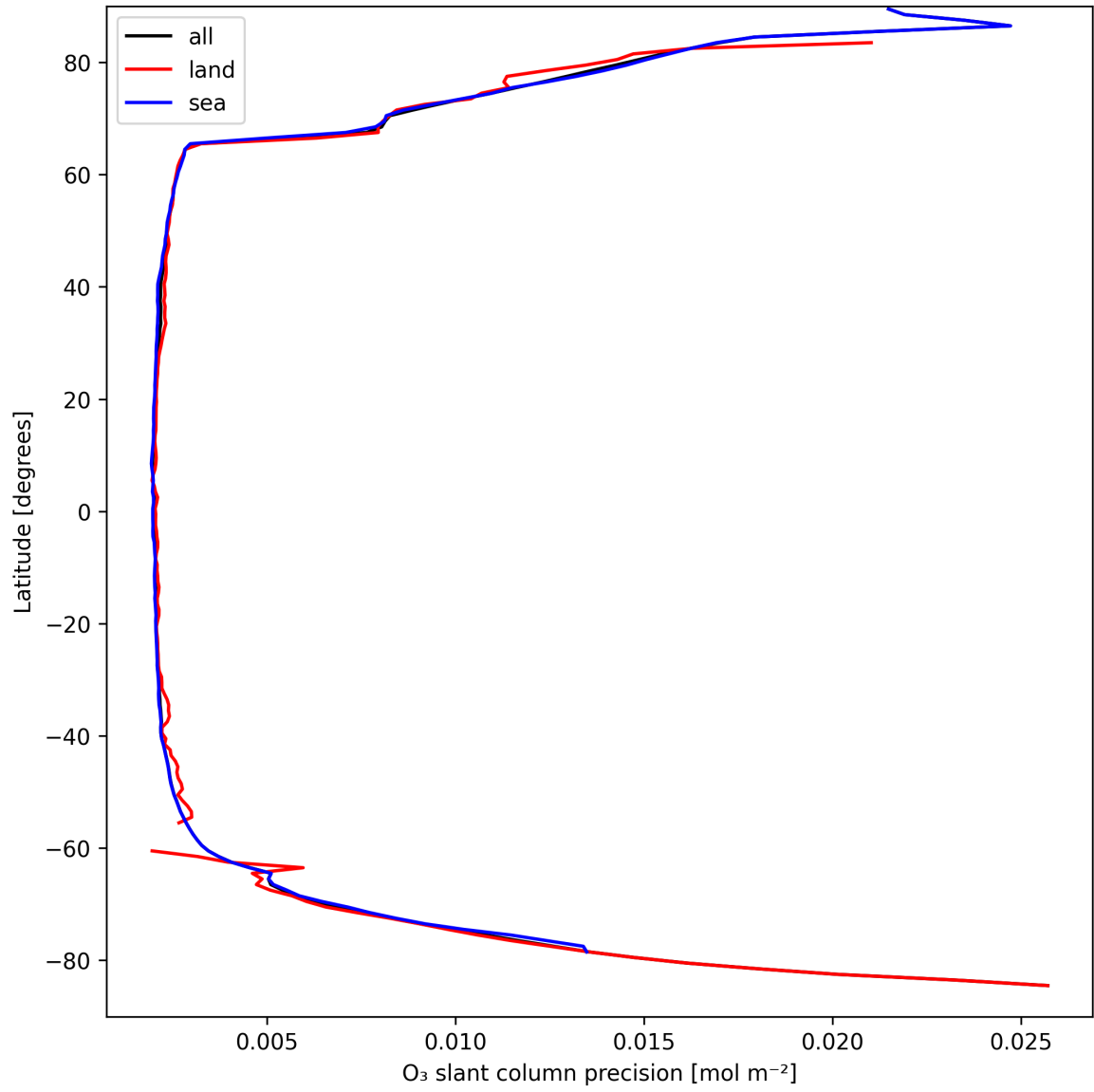
Figure 20: Zonal average of “O 3 slant column precision” for 2025-04-02 to 2025-04-03.
