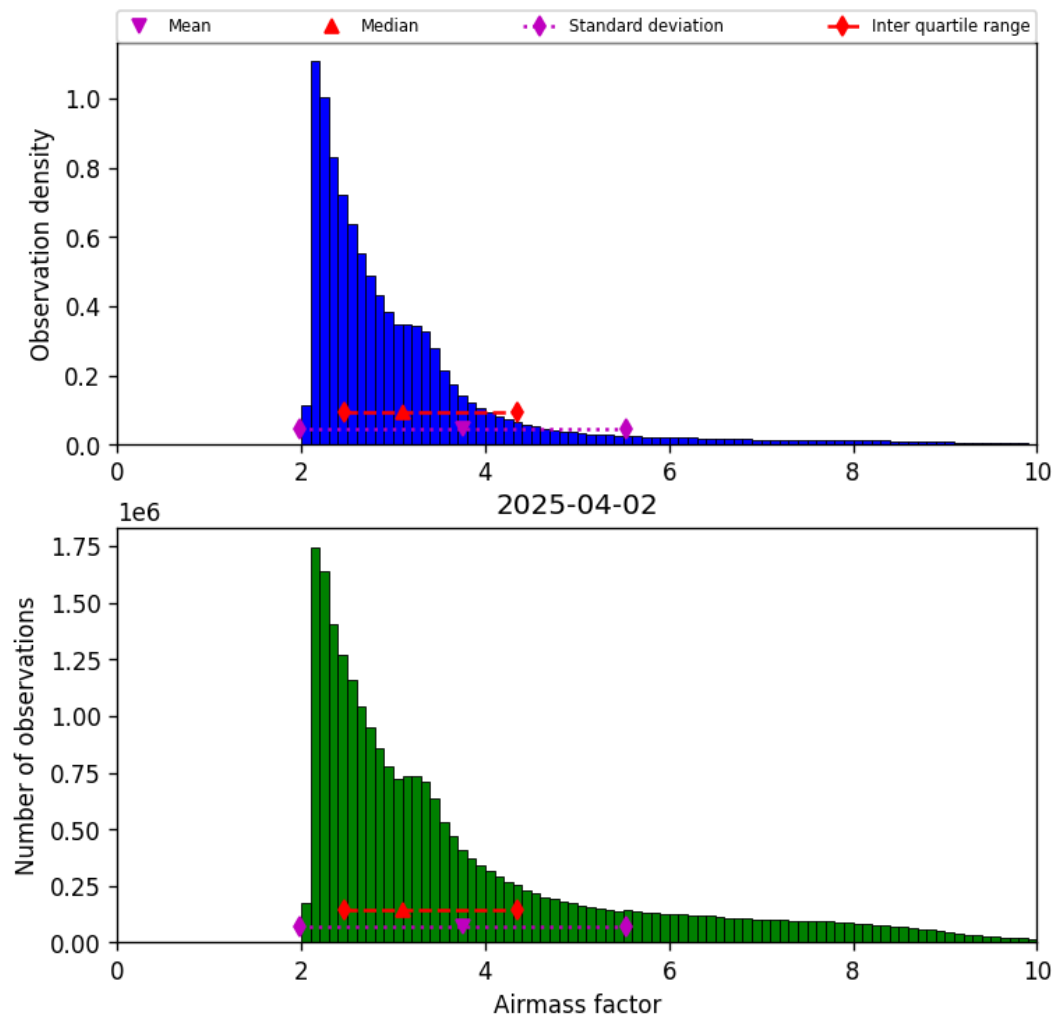
Figure 37: Histogram of “Airmass factor” for 2025-04-02 to 2025-04-03
