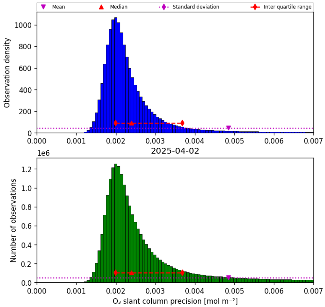
Figure 32: Histogram of “O 3 slant column precision” for 2025-04-02 to 2025-04-03
