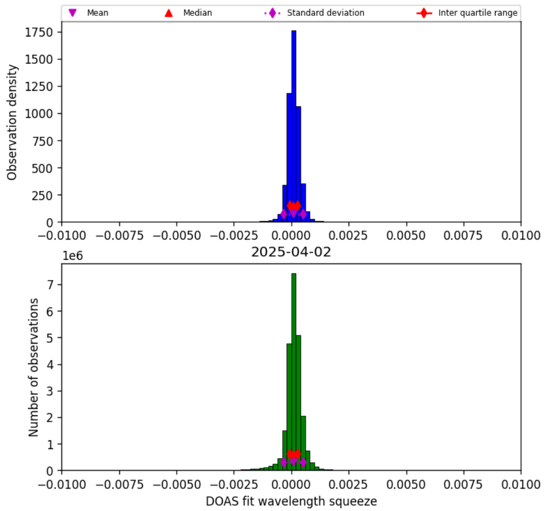
Figure 36: Histogram of “DOAS fit wavelength squeeze” for 2025-04-02 to 2025-04-03
