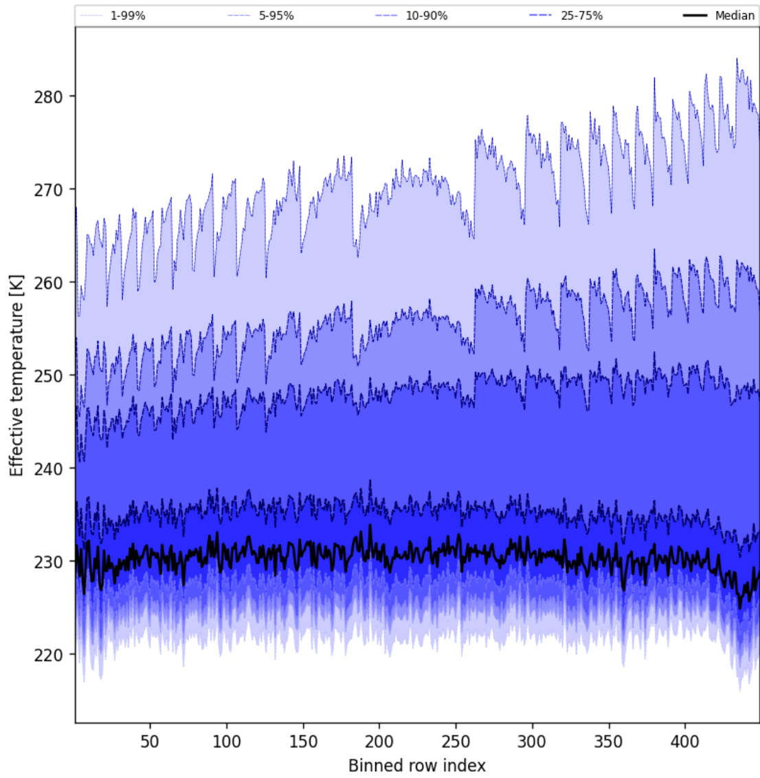
Figure 50: Along track statistics of “Effective temperature” for 2025-04-02 to 2025-04-03
