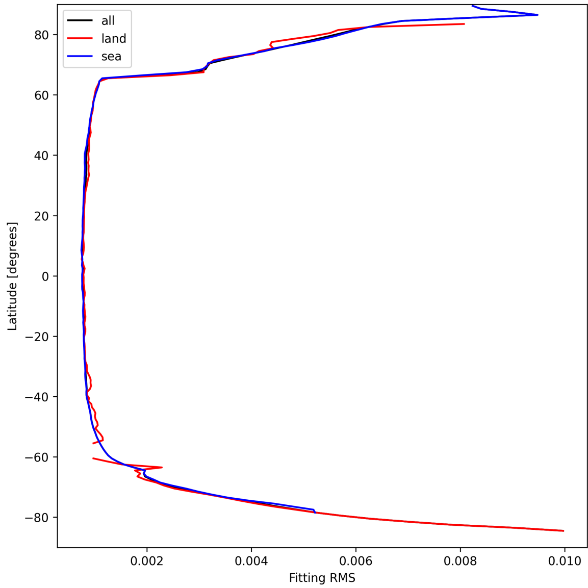
Figure 22: Zonal average of “Fitting RMS” for 2025-04-02 to 2025-04-03.
