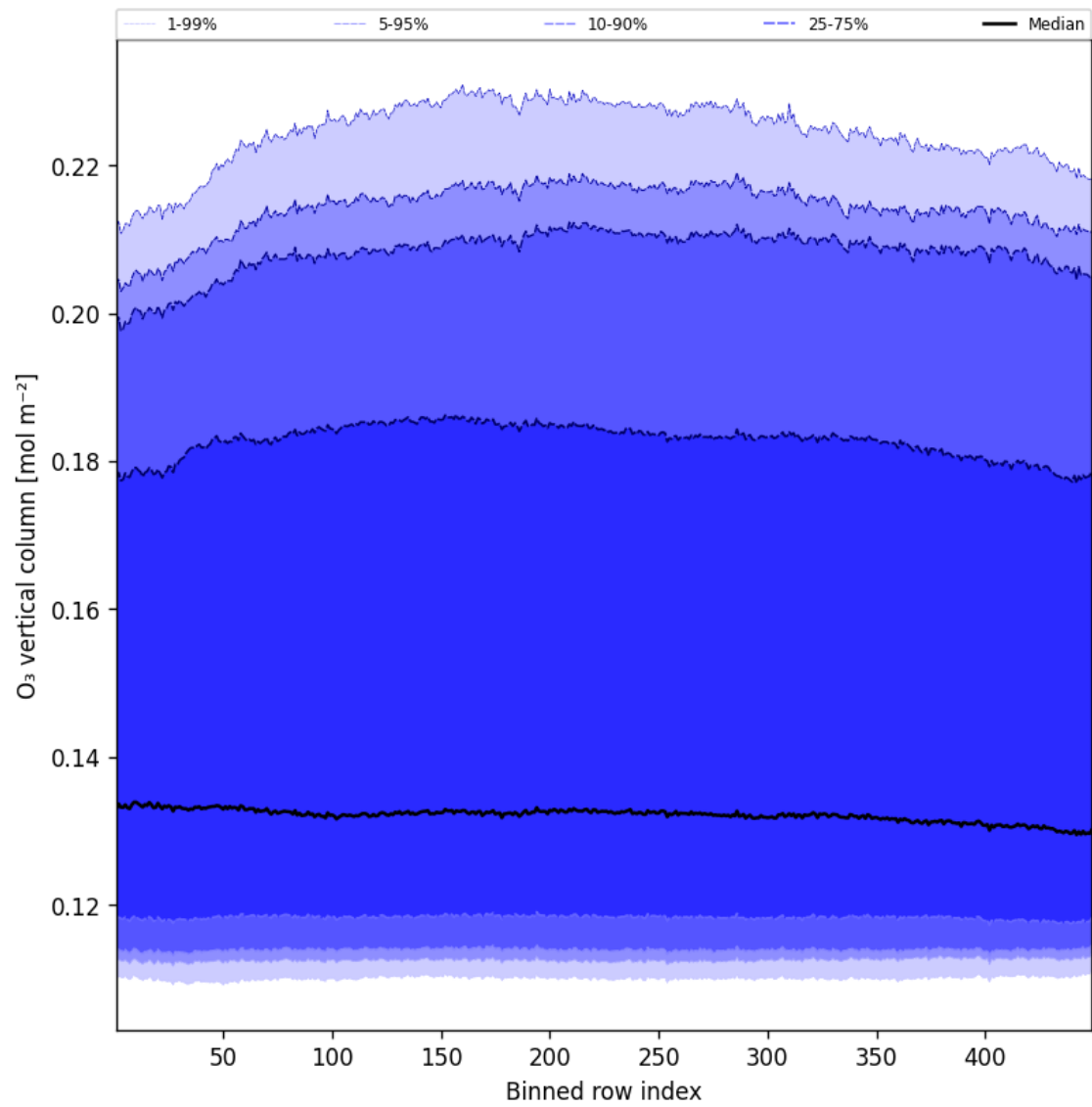
Figure 41: Along track statistics of “O 3 vertical column” for 2025-04-02 to 2025-04-03
