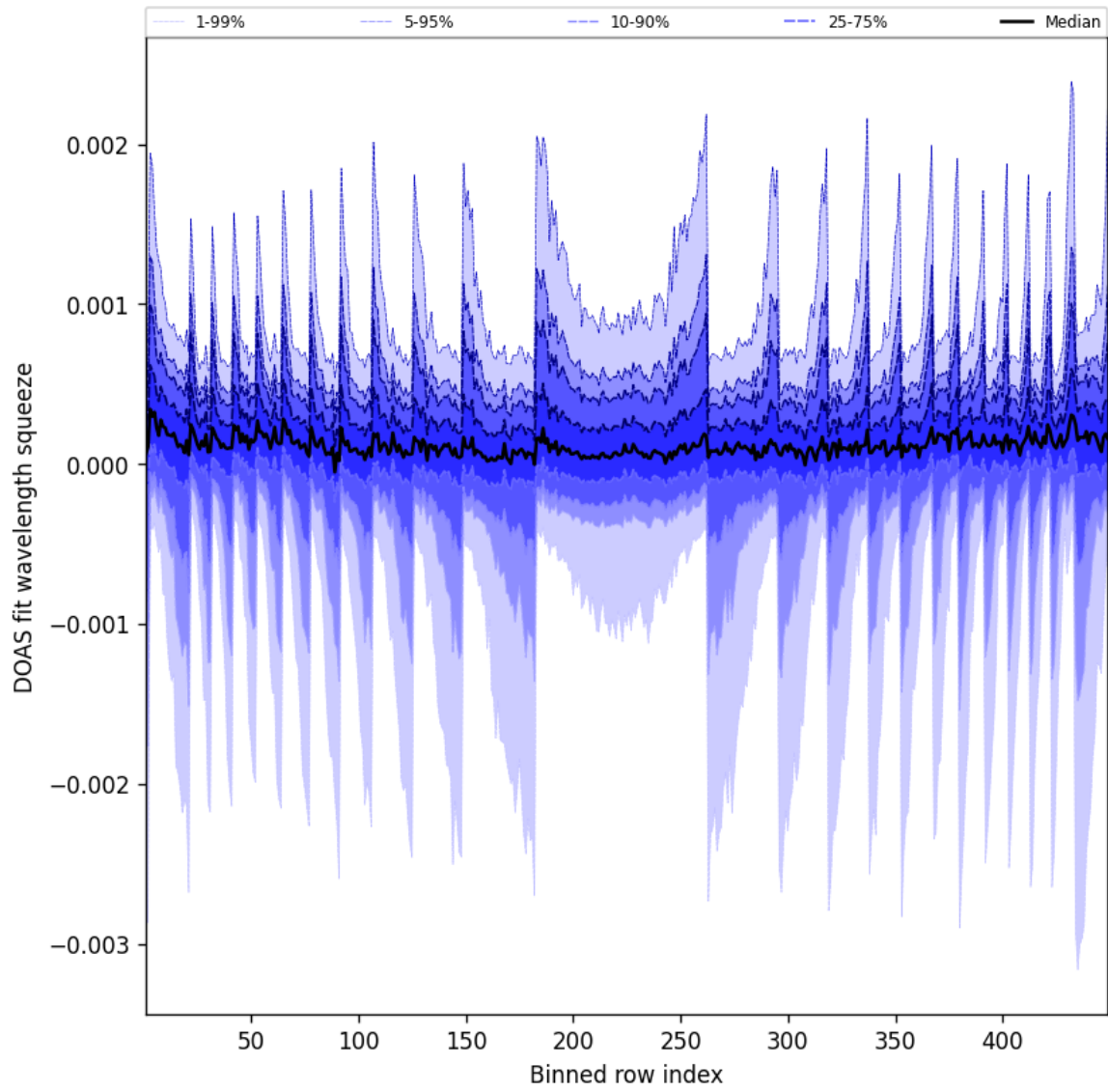
Figure 48: Along track statistics of “DOAS fit wavelength squeeze” for 2025-04-02 to 2025-04-03
