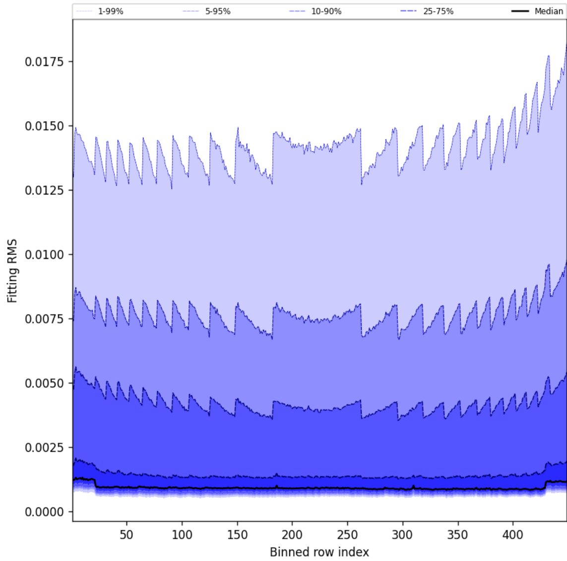
Figure 46: Along track statistics of “Fitting RMS” for 2025-04-02 to 2025-04-03
