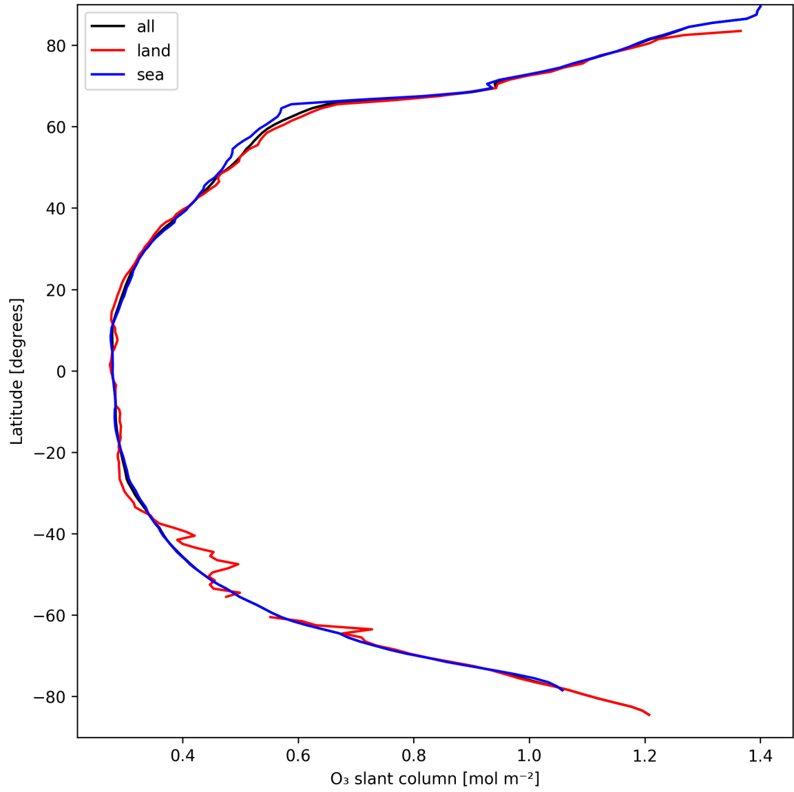
Figure 19: Zonal average of “O 3 slant column” for 2025-04-02 to 2025-04-03.
