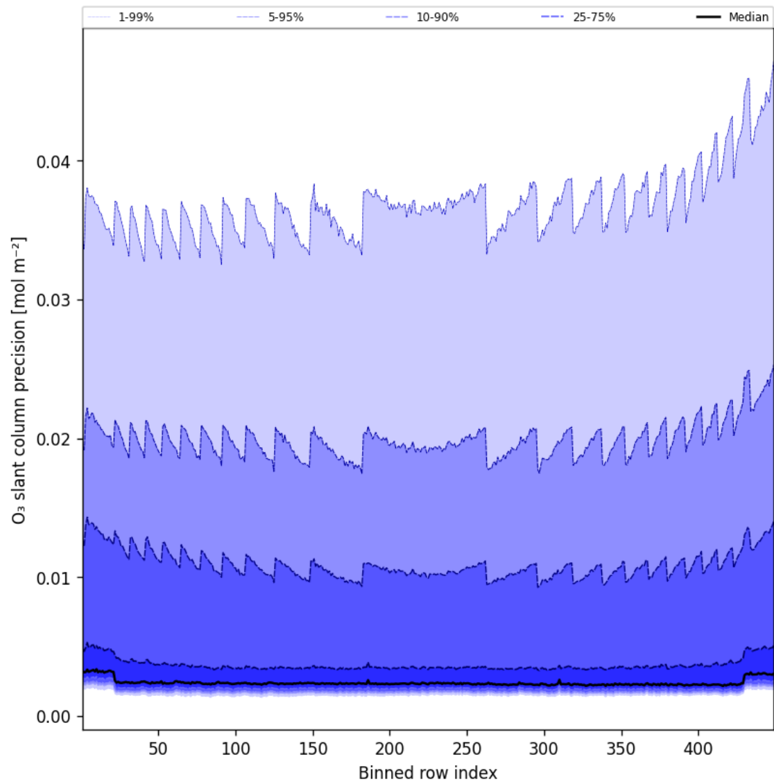
Figure 44: Along track statistics of “O 3 slant column precision” for 2025-04-02 to 2025-04-03
