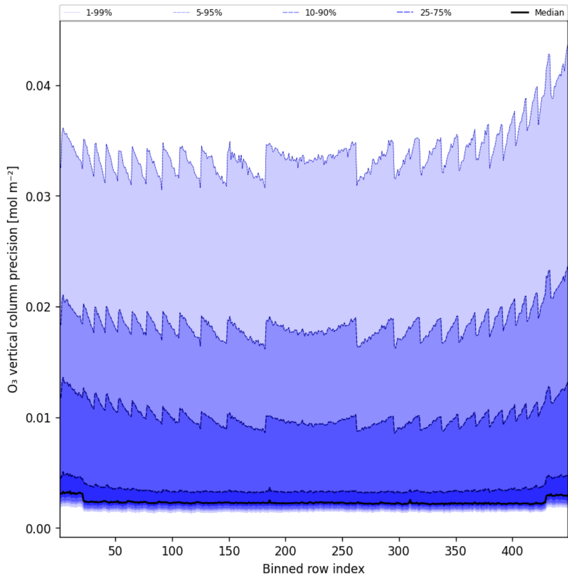
Figure 42: Along track statistics of “O 3 vertical column precision” for 2025-04-02 to 2025-04-03
