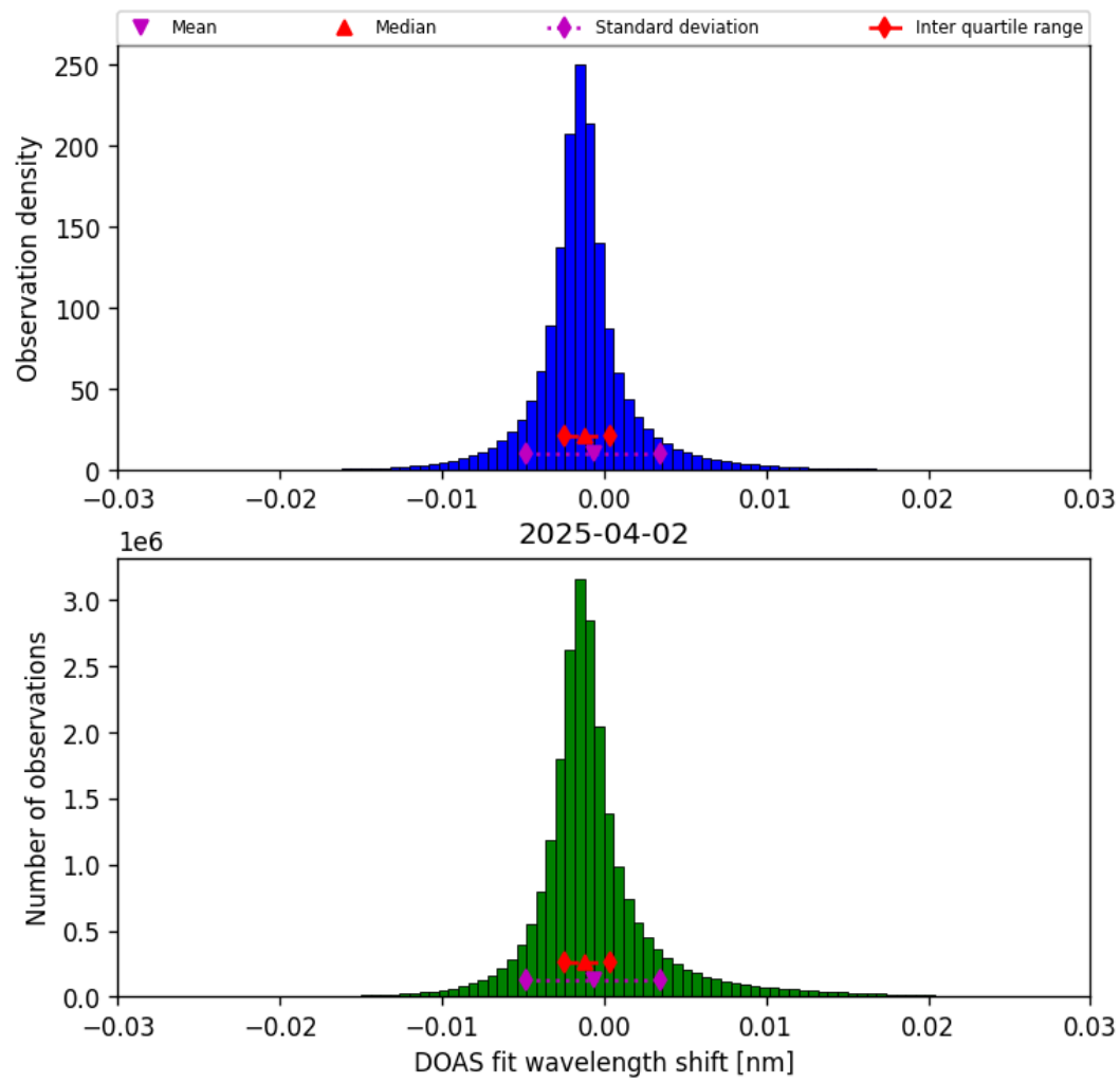
Figure 35: Histogram of “DOAS fit wavelength shift” for 2025-04-02 to 2025-04-03
