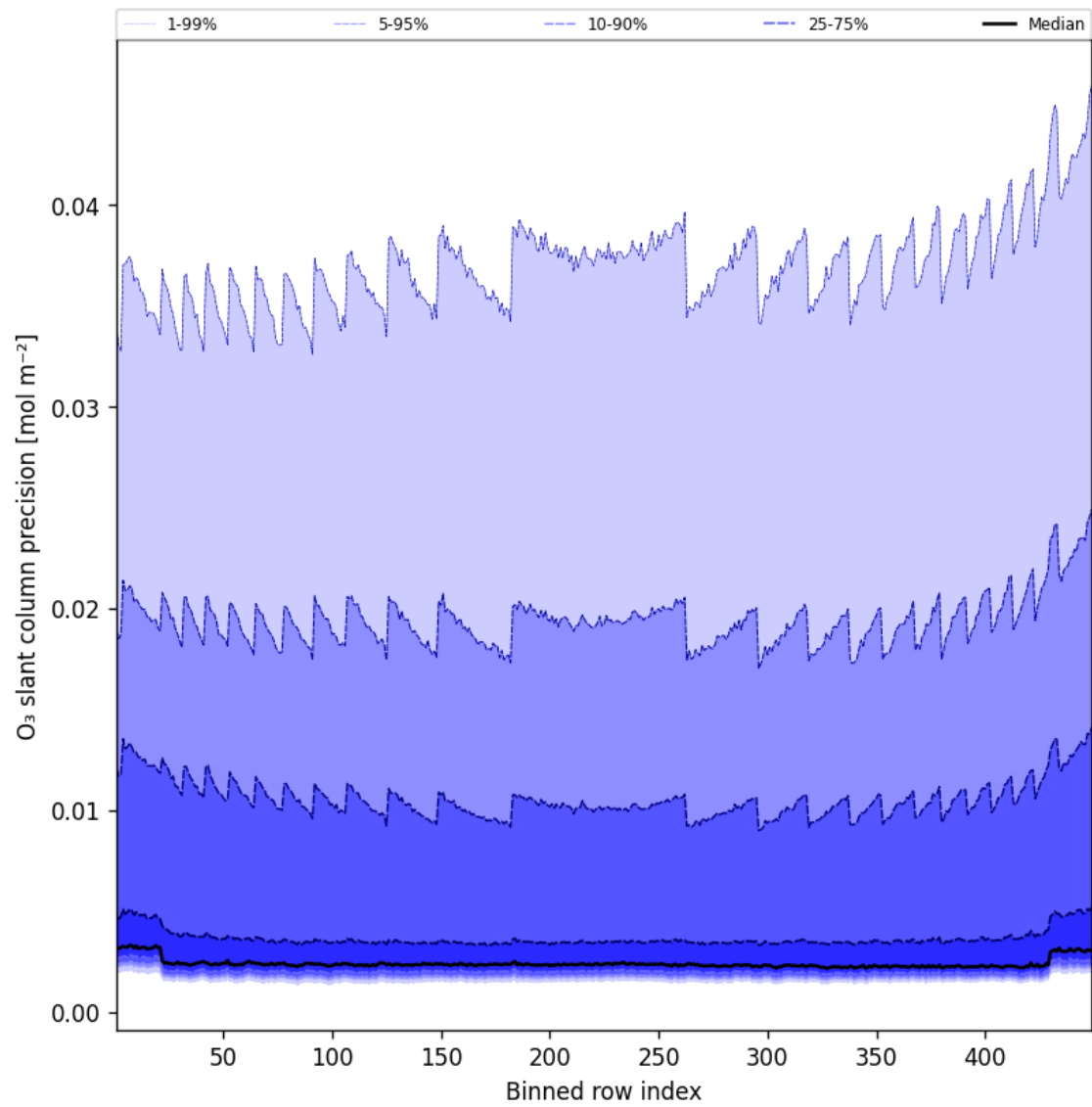
Figure 44: Along track statistics of “O 3 slant column precision” for 2025-04-03 to 2025-04-04
