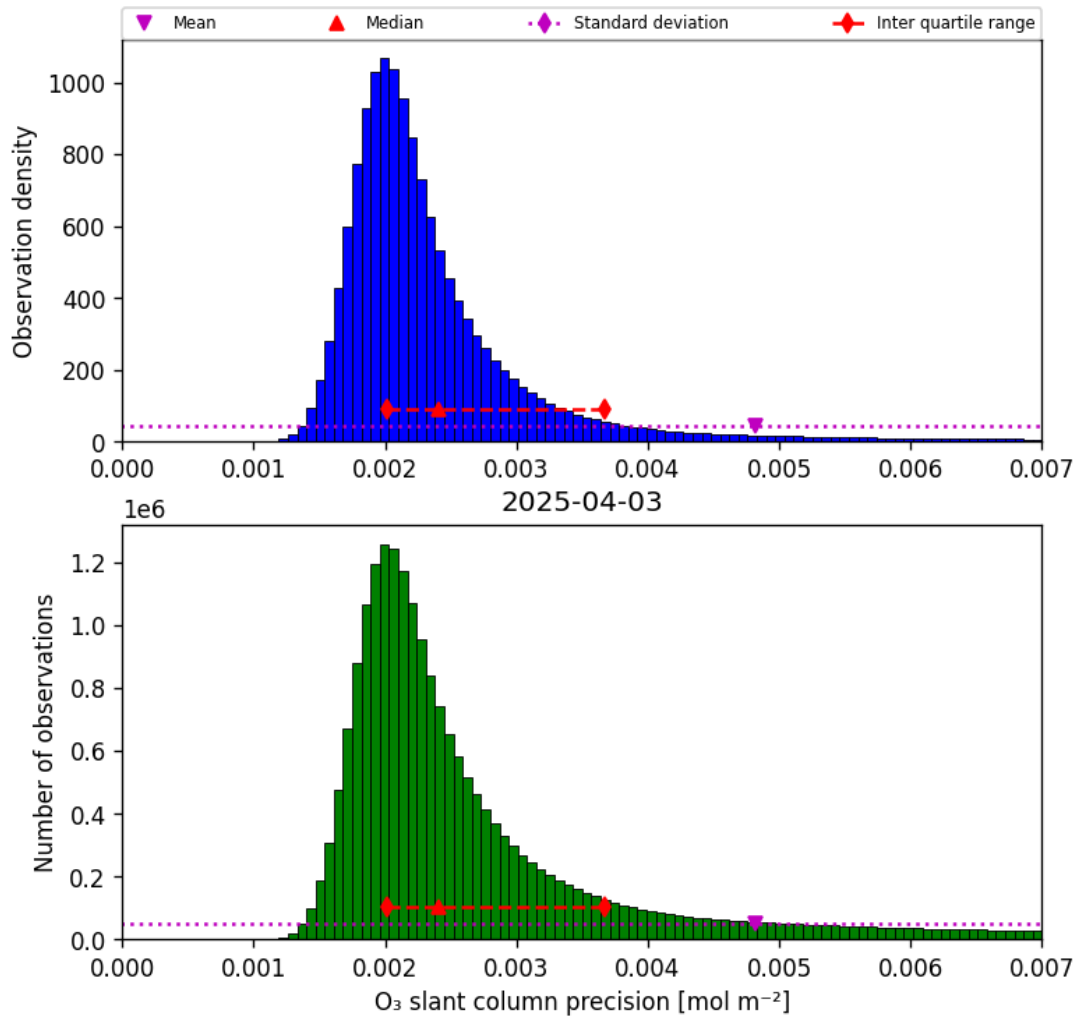
Figure 32: Histogram of “O 3 slant column precision” for 2025-04-03 to 2025-04-04
