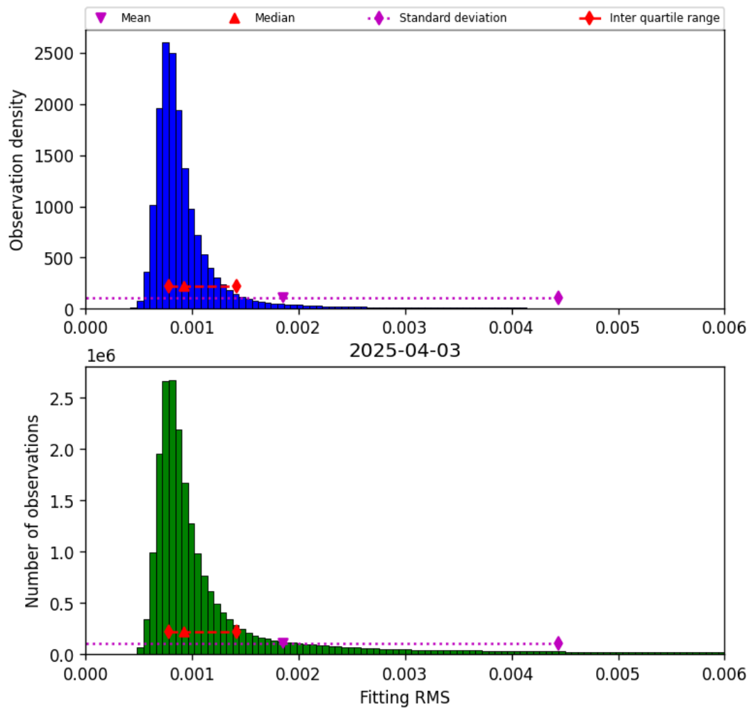
Figure 34: Histogram of “Fitting RMS” for 2025-04-03 to 2025-04-04
