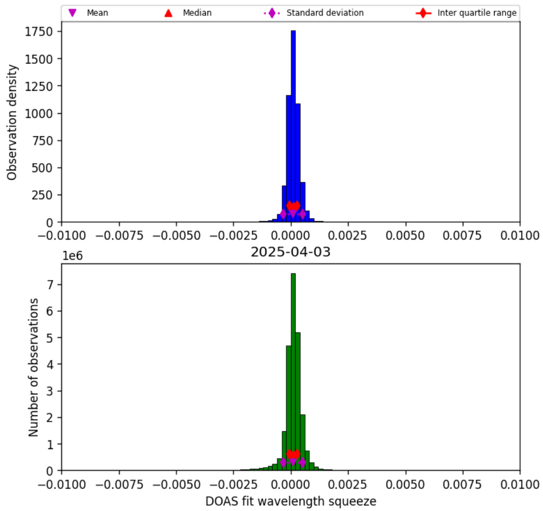
Figure 36: Histogram of “DOAS fit wavelength squeeze” for 2025-04-03 to 2025-04-04
