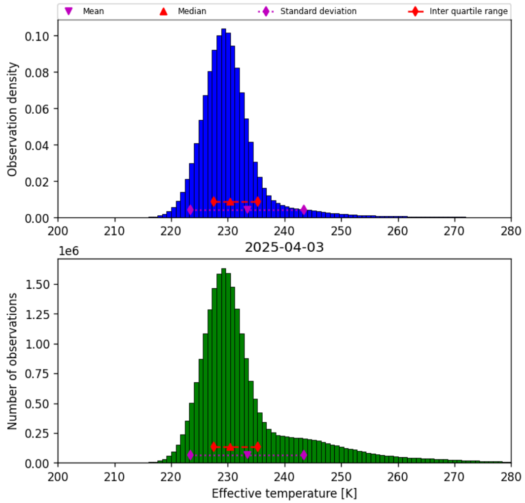
Figure 38: Histogram of “Effective temperature” for 2025-04-03 to 2025-04-04
