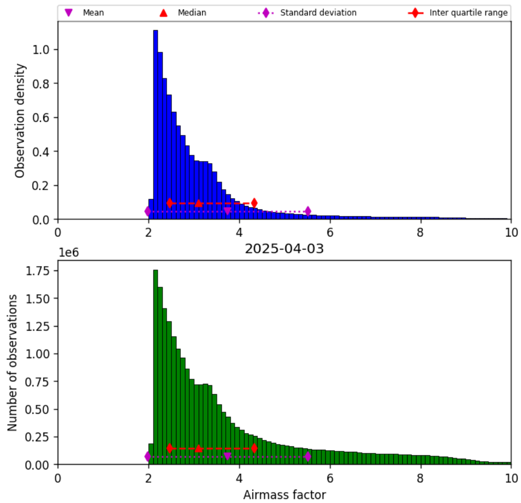
Figure 37: Histogram of “Airmass factor” for 2025-04-03 to 2025-04-04
