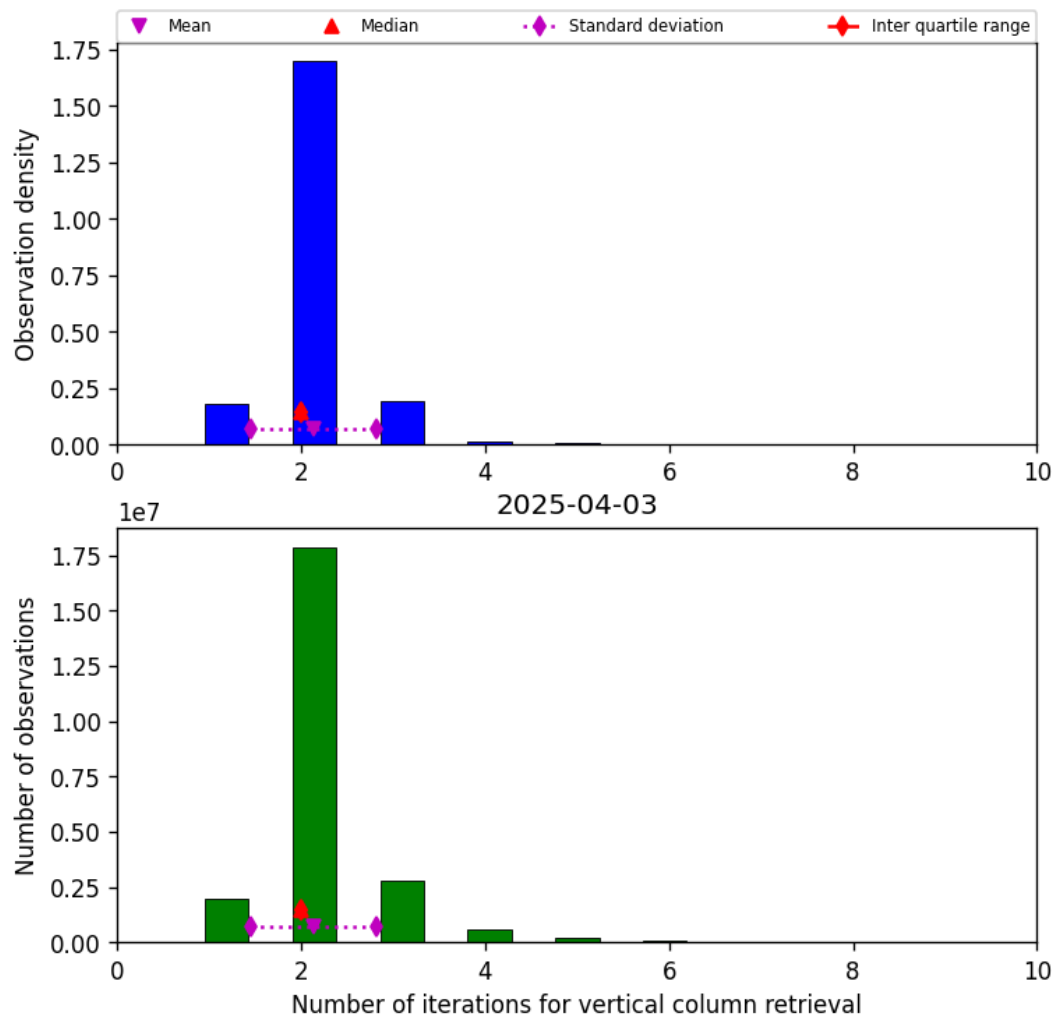
Figure 39: Histogram of “Number of iterations for vertical column retrieval” for 2025-04-03 to 2025-04-04
