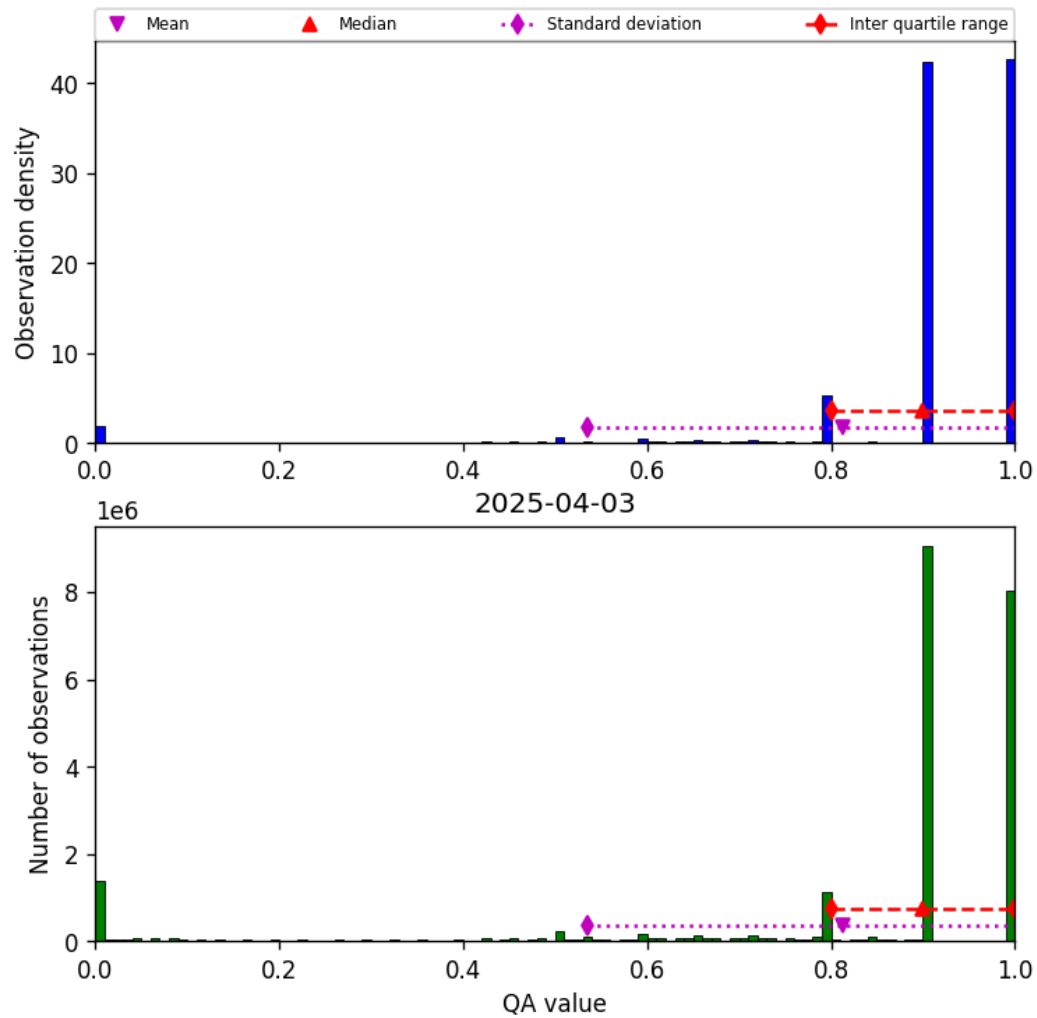
Figure 28: Histogram of “QA value” for 2025-04-03 to 2025-04-04
