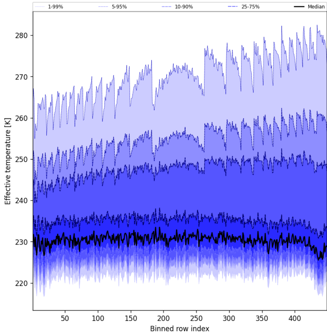
Figure 50: Along track statistics of “Effective temperature” for 2025-04-03 to 2025-04-04
