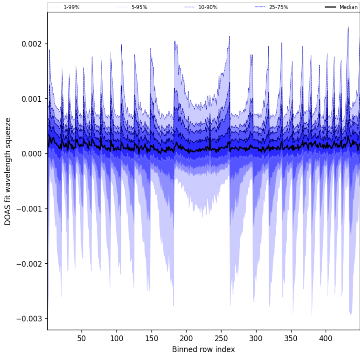
Figure 48: Along track statistics of “DOAS fit wavelength squeeze” for 2025-04-03 to 2025-04-04
