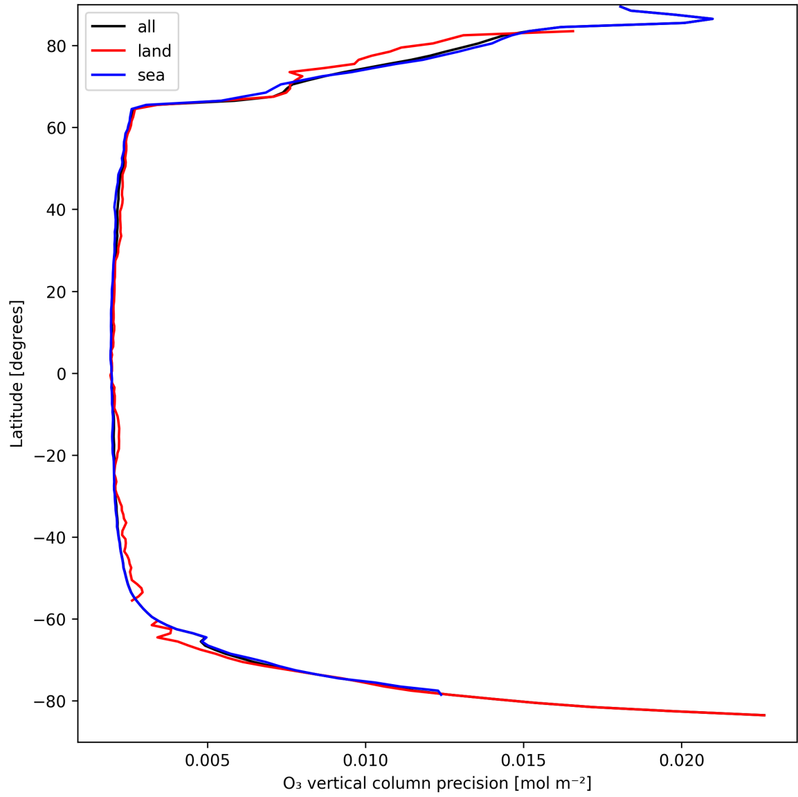
Figure 18: Zonal average of “O 3 vertical column precision” for 2025-04-03 to 2025-04-04.
