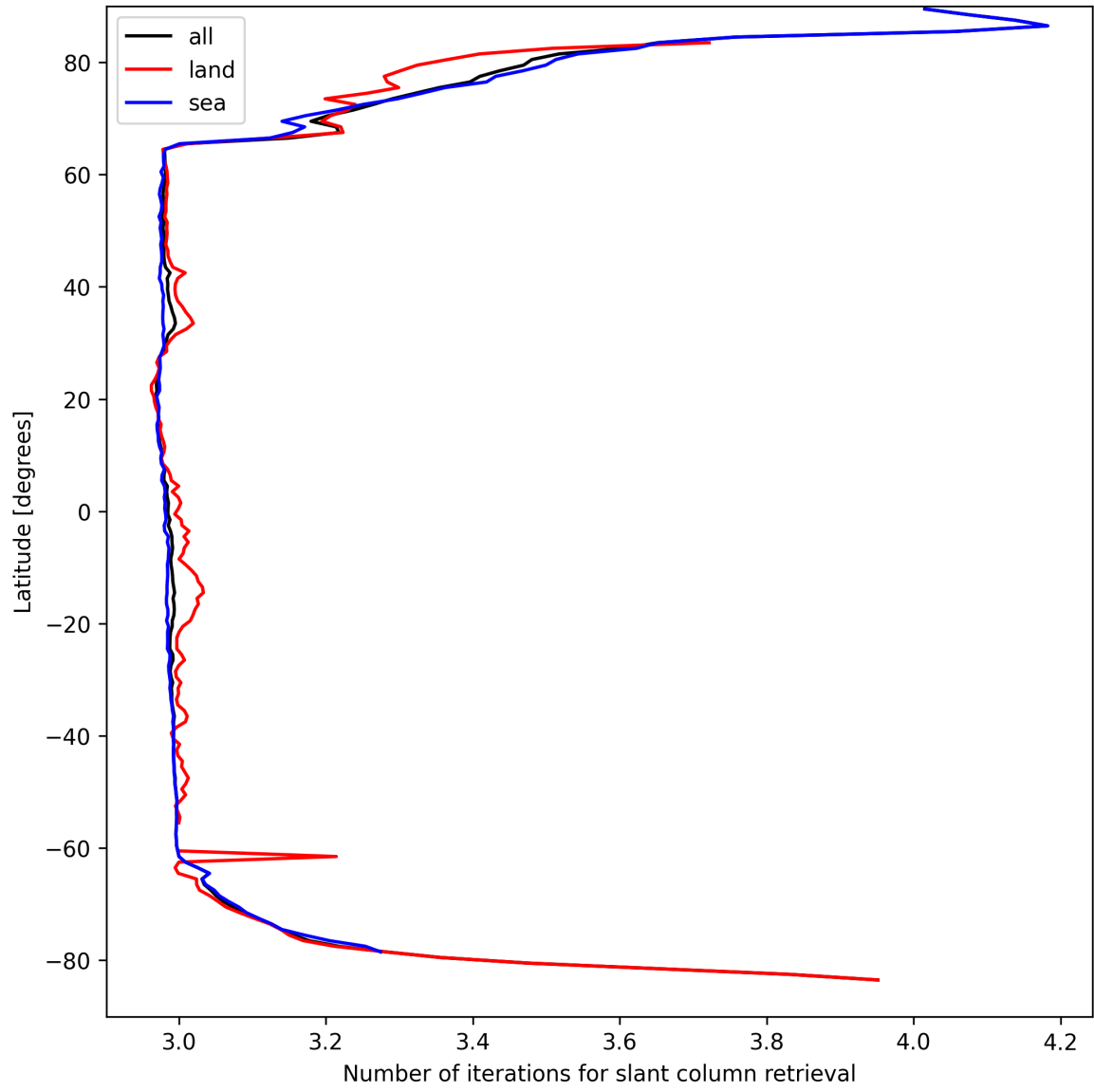
Figure 21: Zonal average of “Number of iterations for slant column retrieval” for 2025-04-03 to 2025-04-04.
