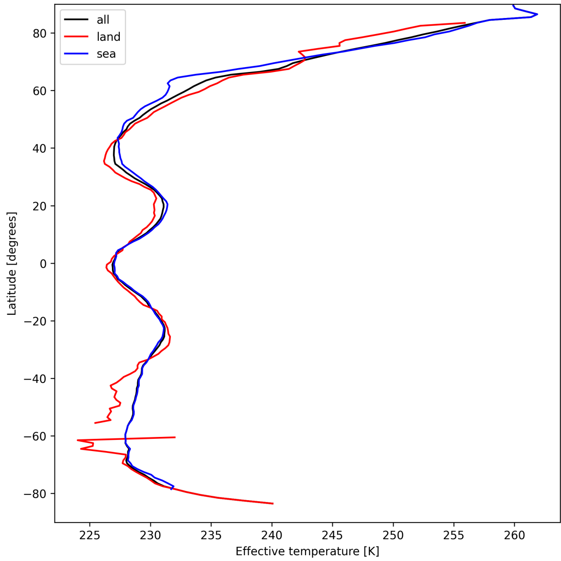
Figure 26: Zonal average of “Effective temperature” for 2025-04-03 to 2025-04-04.
