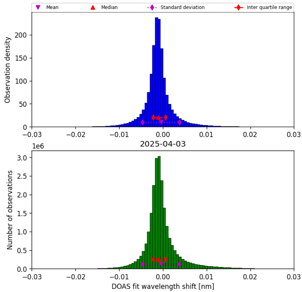
Figure 35: Histogram of “DOAS fit wavelength shift” for 2025-04-03 to 2025-04-04
