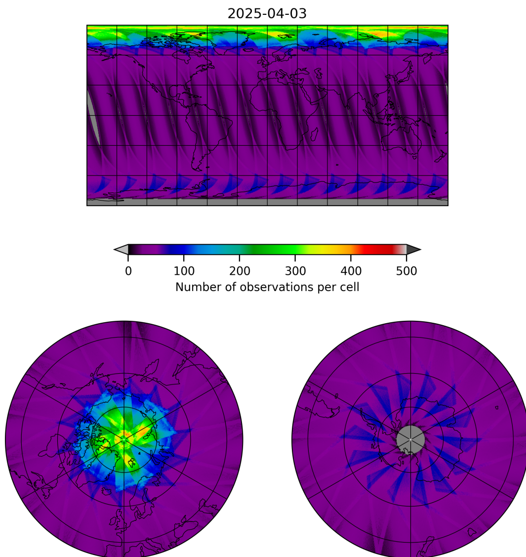
Figure 15: Map of the number of observations for 2025-04-03 to 2025-04-04
