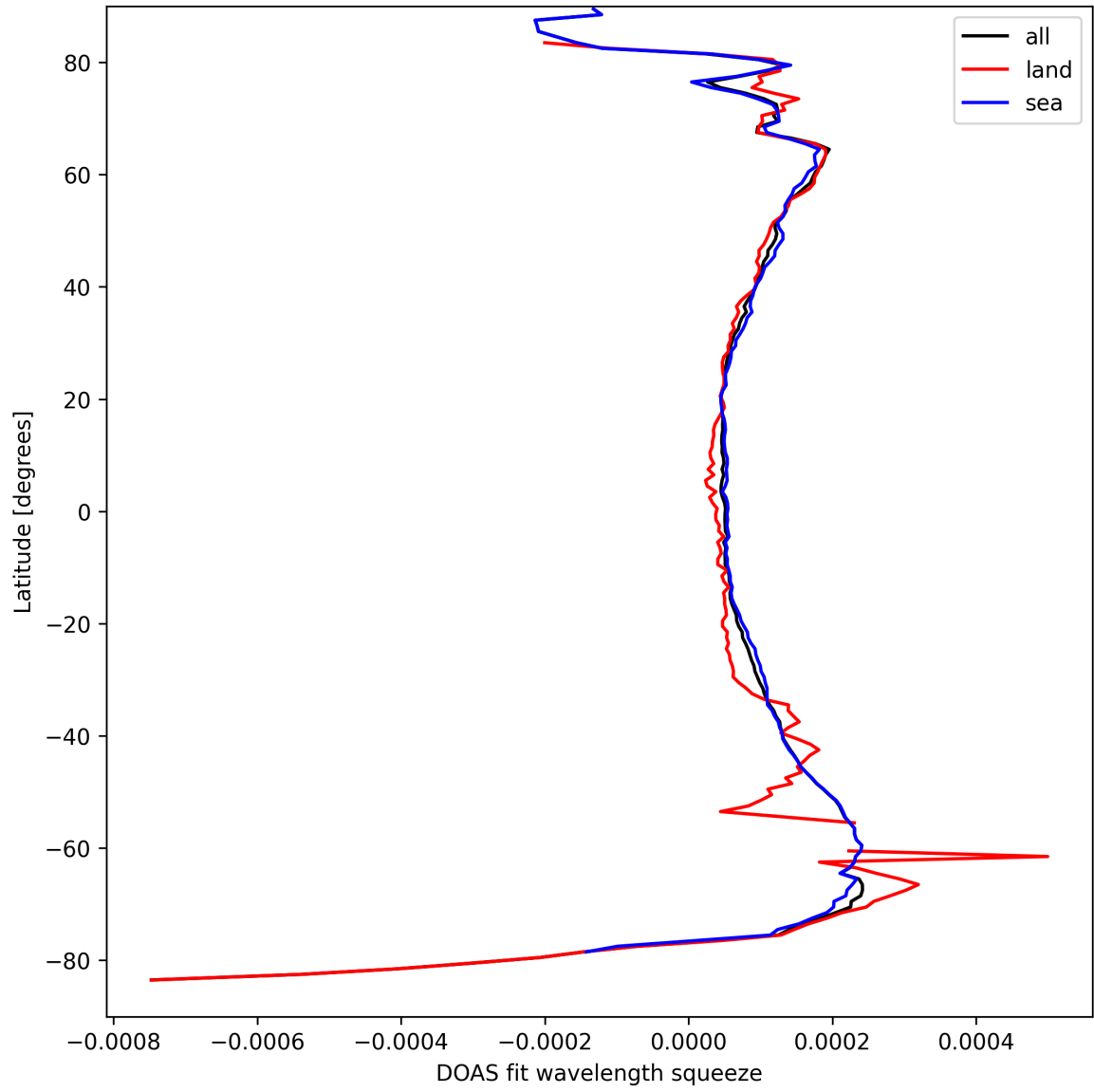
Figure 24: Zonal average of “DOAS fit wavelength squeeze” for 2025-04-03 to 2025-04-04.
