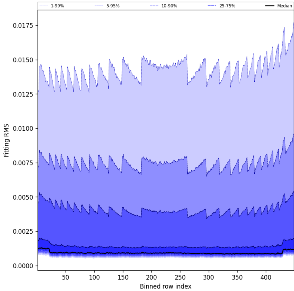
Figure 46: Along track statistics of “Fitting RMS” for 2025-04-03 to 2025-04-04
