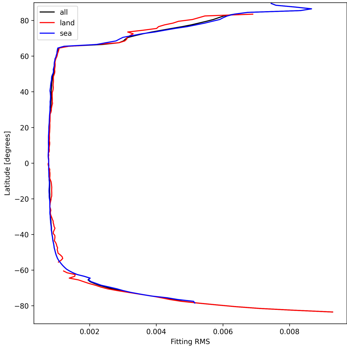
Figure 22: Zonal average of “Fitting RMS” for 2025-04-03 to 2025-04-04.
