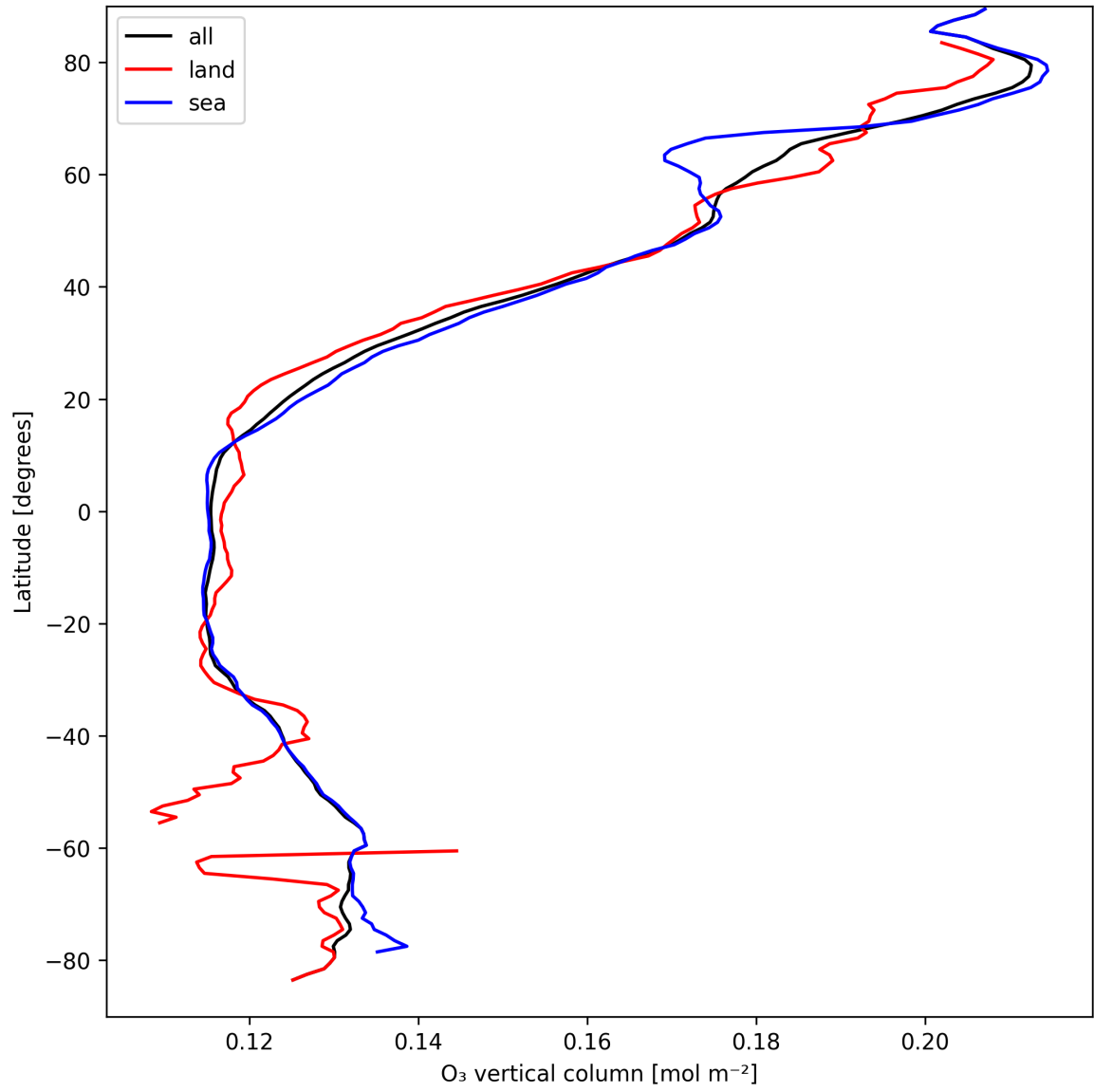
Figure 17: Zonal average of “O 3 vertical column” for 2025-04-03 to 2025-04-04.
