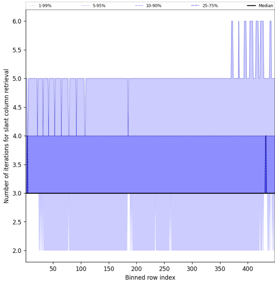
Figure 45: Along track statistics of “Number of iterations for slant column retrieval” for 2025-04-03 to 2025-04-04
