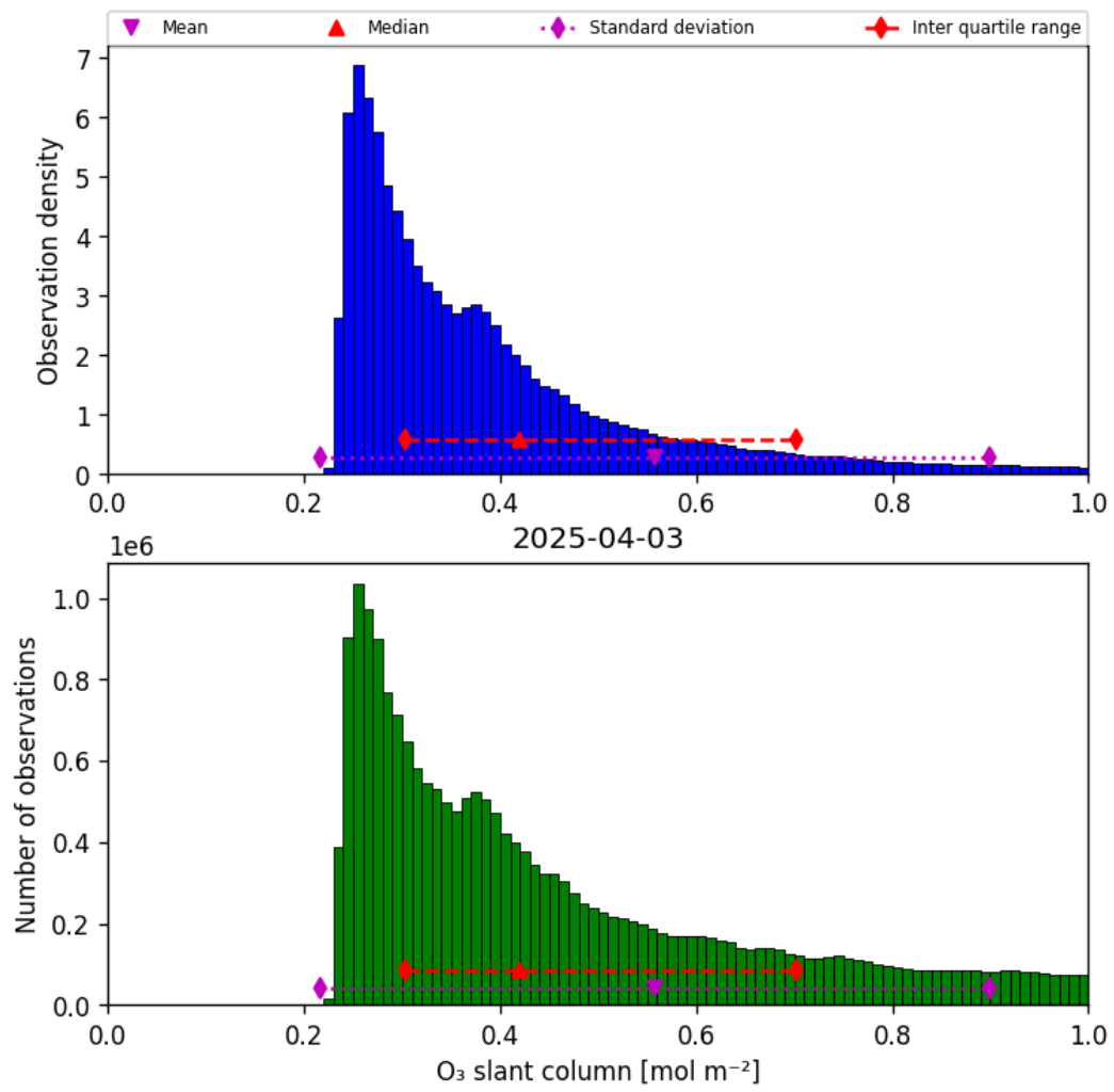
Figure 31: Histogram of “O 3 slant column” for 2025-04-03 to 2025-04-04
