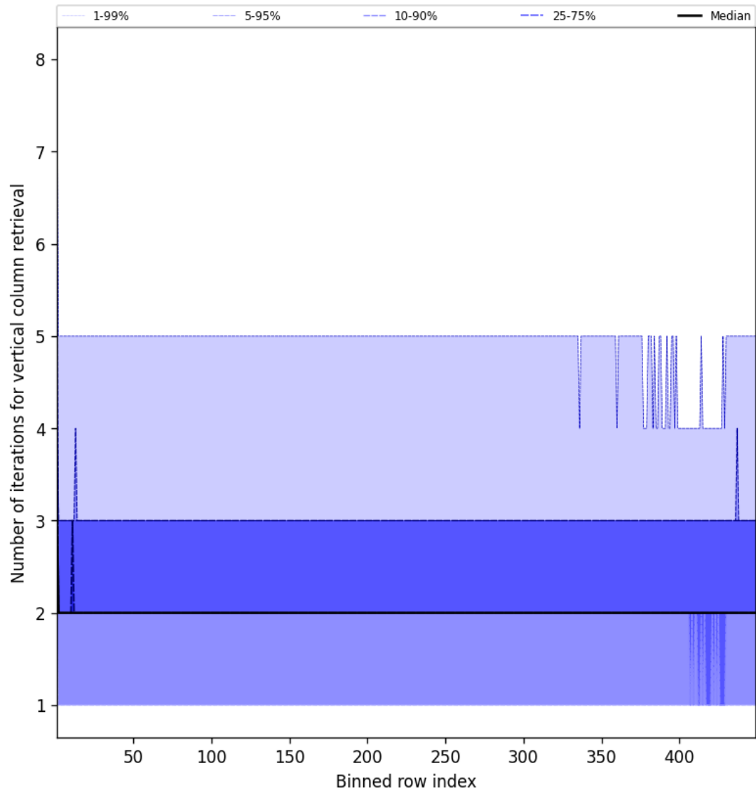
Figure 51: Along track statistics of “Number of iterations for vertical column retrieval” for 2025-04-03 to 2025-04-04
