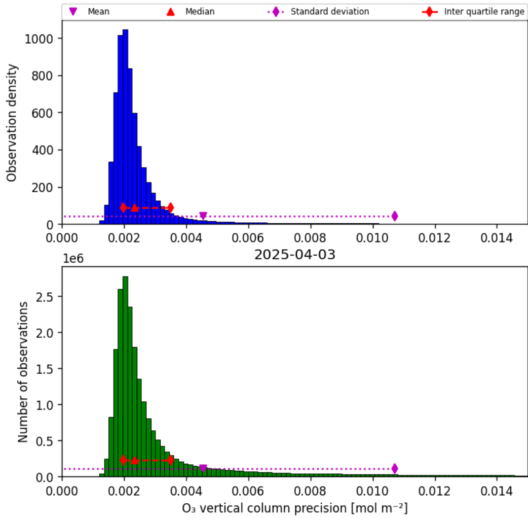
Figure 30: Histogram of “O 3 vertical column precision” for 2025-04-03 to 2025-04-04
