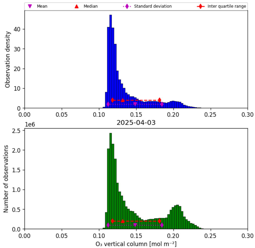
Figure 29: Histogram of “O 3 vertical column” for 2025-04-03 to 2025-04-04
