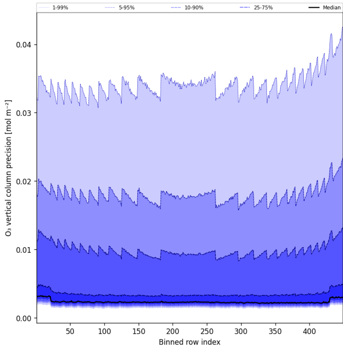
Figure 42: Along track statistics of “O 3 vertical column precision” for 2025-04-03 to 2025-04-04
