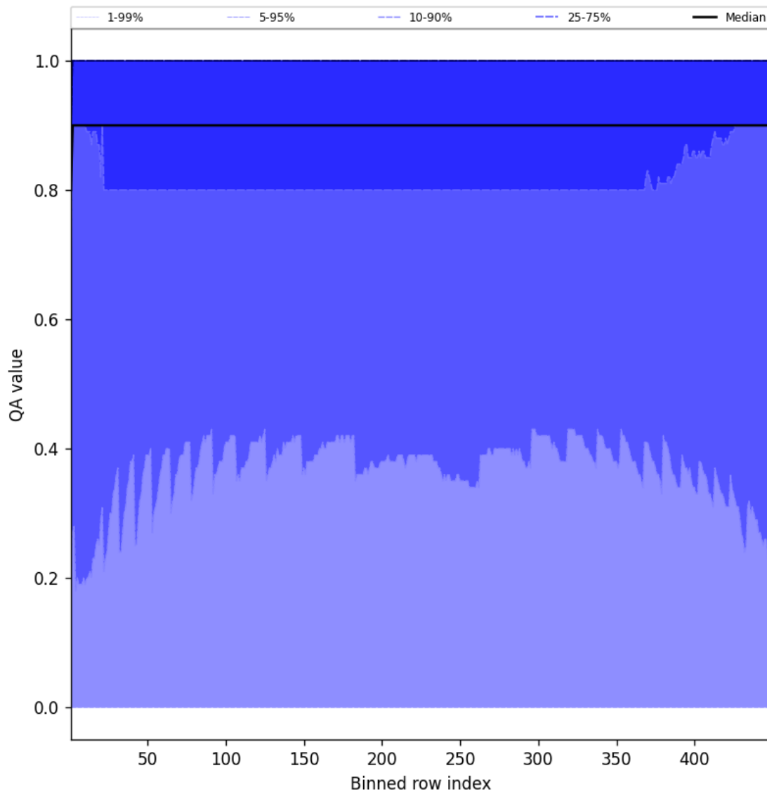
Figure 40: Along track statistics of “QA value” for 2025-04-03 to 2025-04-04
