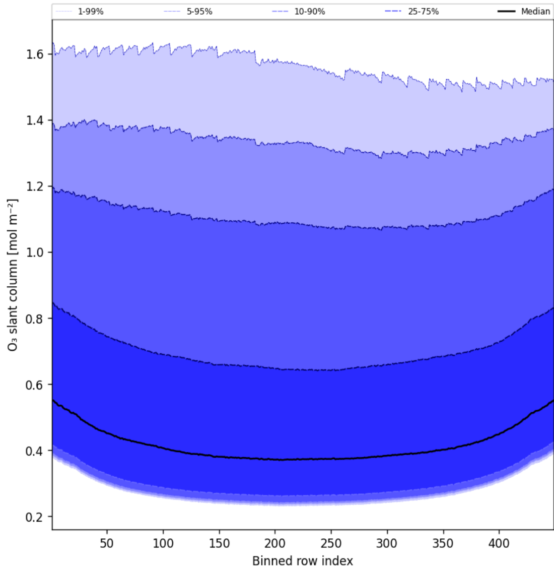
Figure 43: Along track statistics of “O 3 slant column” for 2025-04-03 to 2025-04-04
