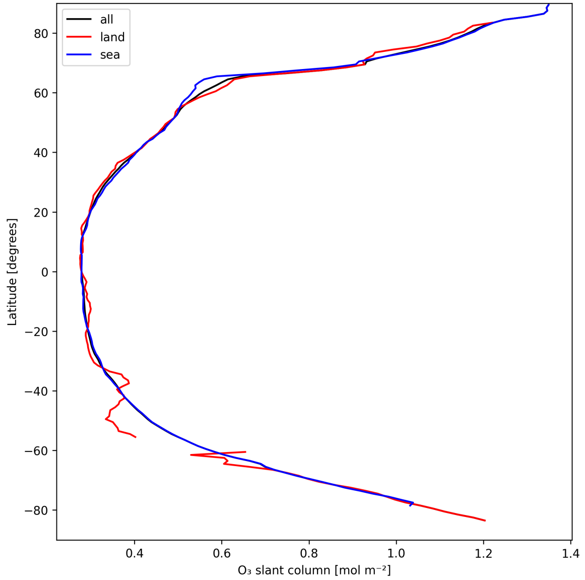
Figure 19: Zonal average of “O 3 slant column” for 2025-04-03 to 2025-04-04.
