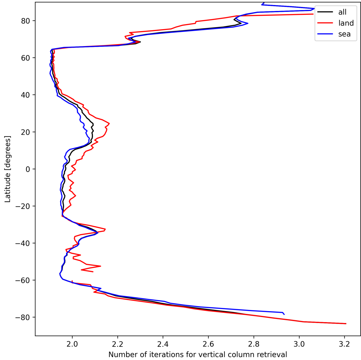
Figure 27: Zonal average of “Number of iterations for vertical column retrieval” for 2025-04-03 to 2025-04-04.
