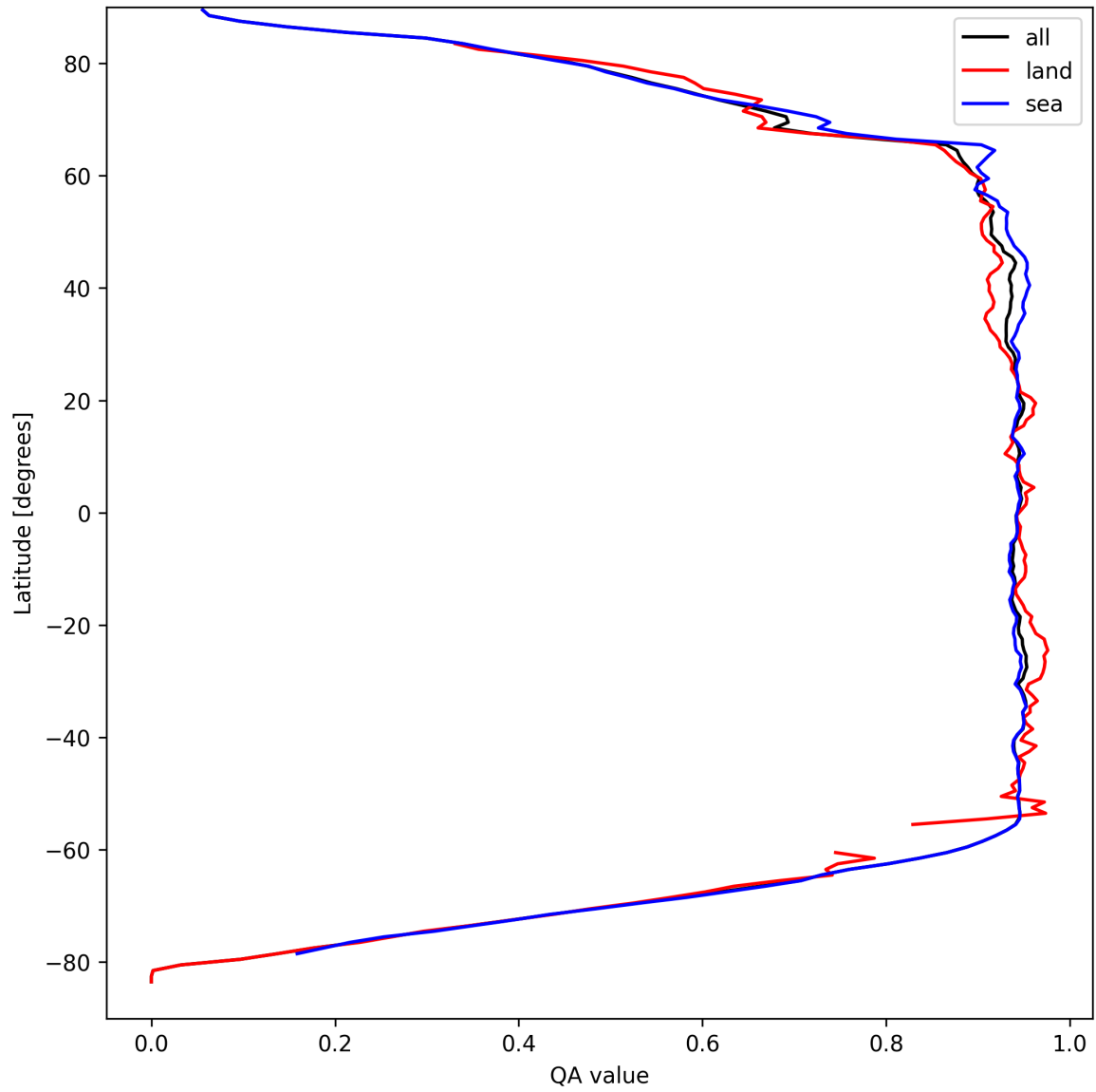
Figure 16: Zonal average of “QA value” for 2025-04-03 to 2025-04-04.
