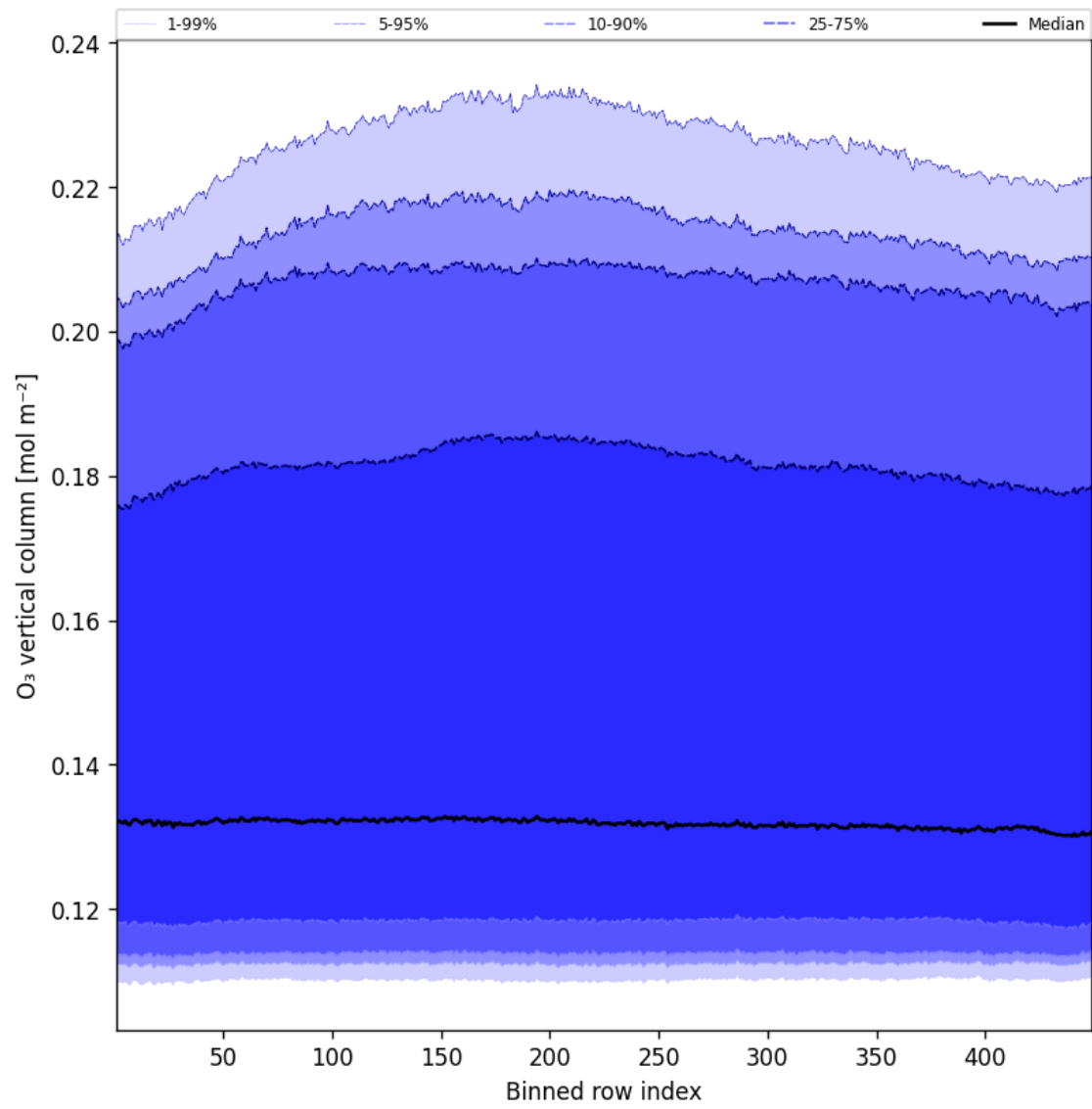
Figure 41: Along track statistics of “O 3 vertical column” for 2025-04-03 to 2025-04-04
