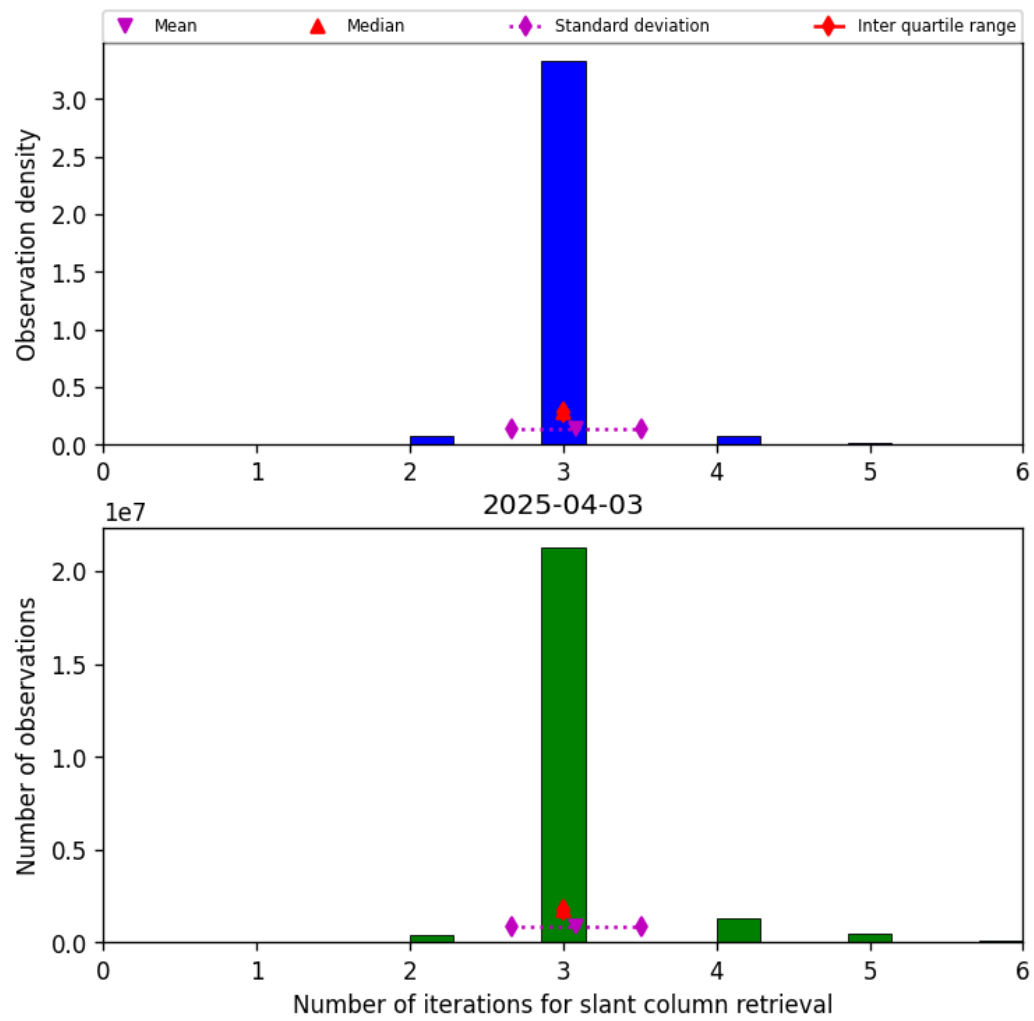
Figure 33: Histogram of “Number of iterations for slant column retrieval” for 2025-04-03 to 2025-04-04
