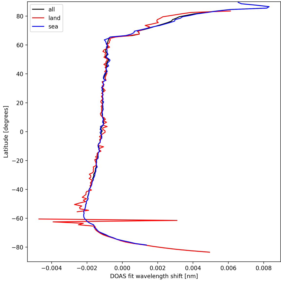
Figure 23: Zonal average of “DOAS fit wavelength shift” for 2025-04-03 to 2025-04-04.
