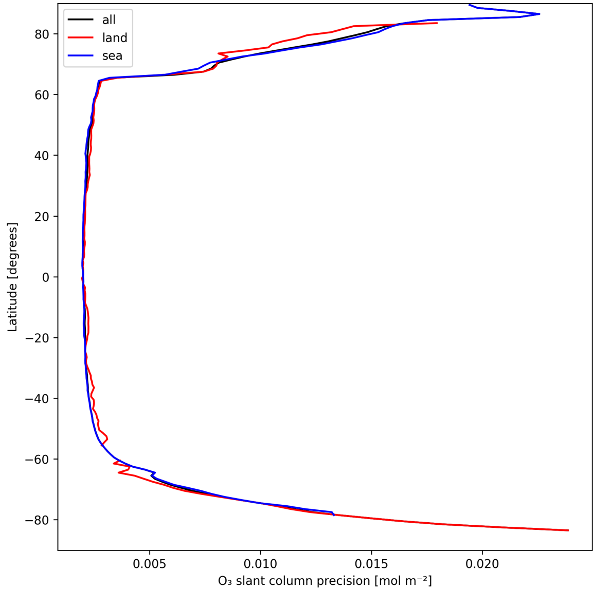
Figure 20: Zonal average of "O 3 slant column precision" for 2025-04-03 to 2025-04-04.
