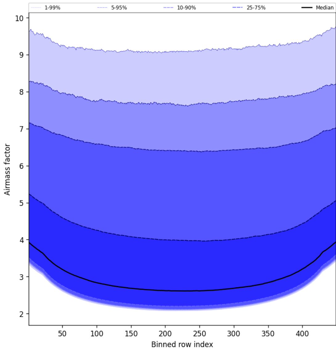
Figure 49: Along track statistics of “Airmass factor” for 2025-04-03 to 2025-04-04
