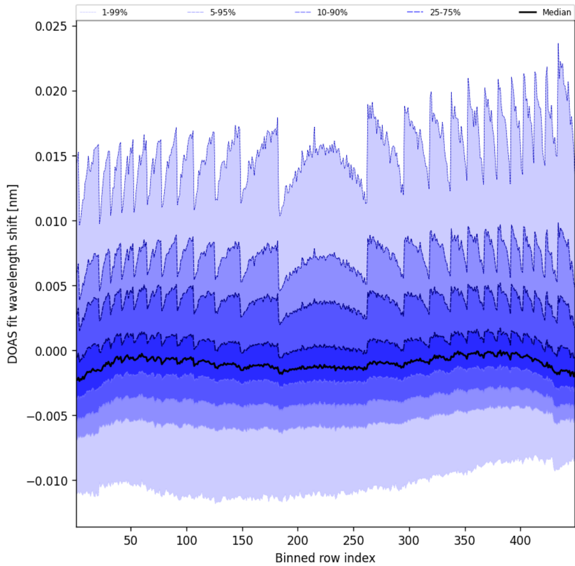
Figure 47: Along track statistics of “DOAS fit wavelength shift” for 2025-04-03 to 2025-04-04
