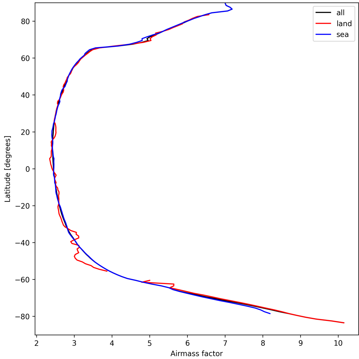
Figure 25: Zonal average of “Airmass factor” for 2025-04-03 to 2025-04-04.
