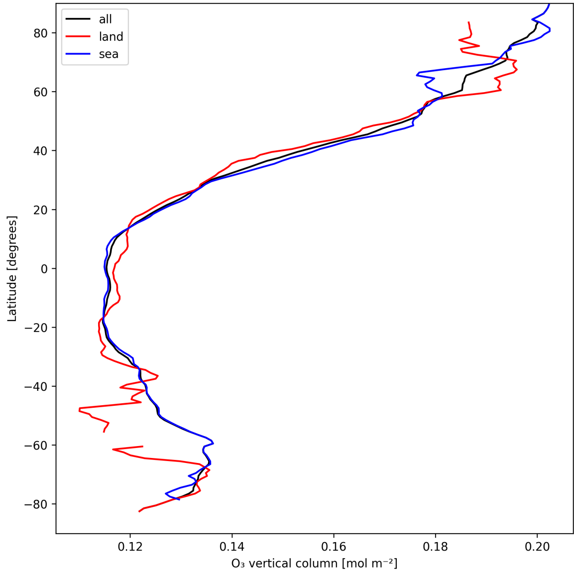
Figure 17: Zonal average of “O 3 vertical column” for 2025-04-06 to 2025-04-06.
