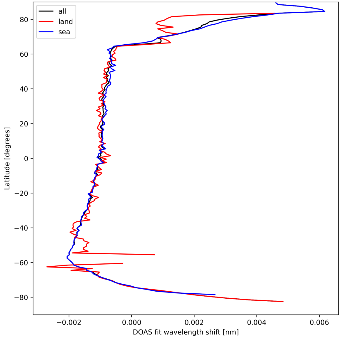
Figure 23: Zonal average of “DOAS fit wavelength shift” for 2025-04-06 to 2025-04-06.
