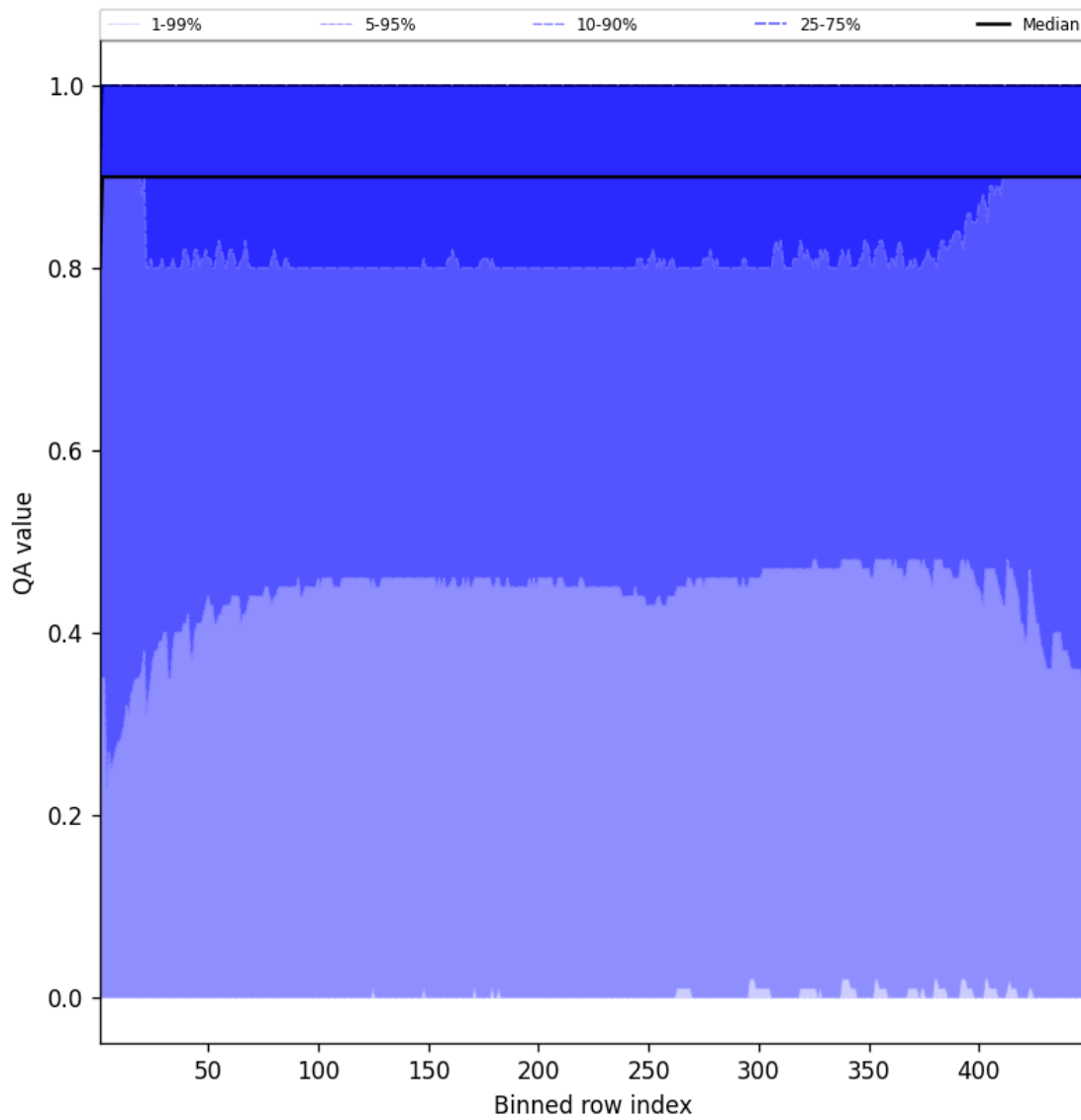
Figure 40: Along track statistics of “QA value” for 2025-04-06 to 2025-04-06
