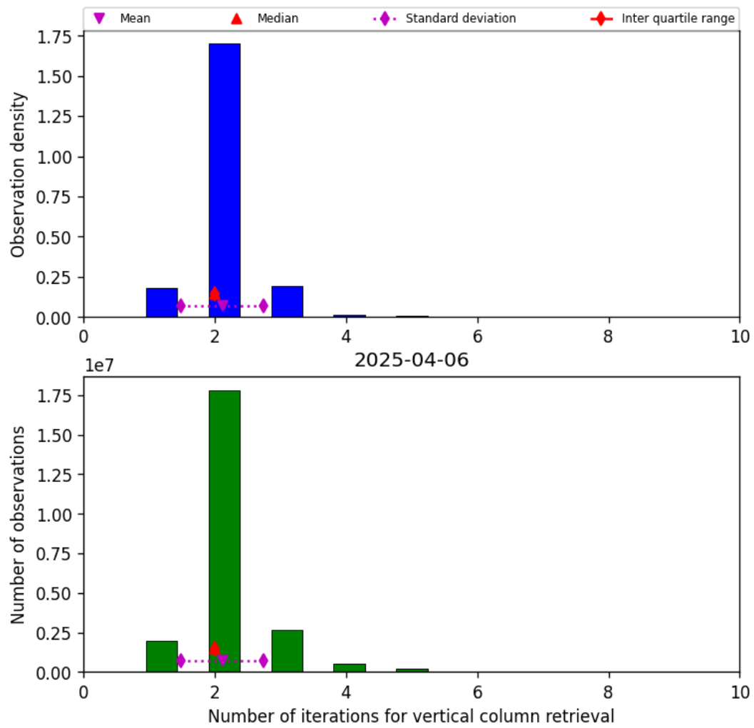
Figure 39: Histogram of “Number of iterations for vertical column retrieval” for 2025-04-06 to 2025-04-06
