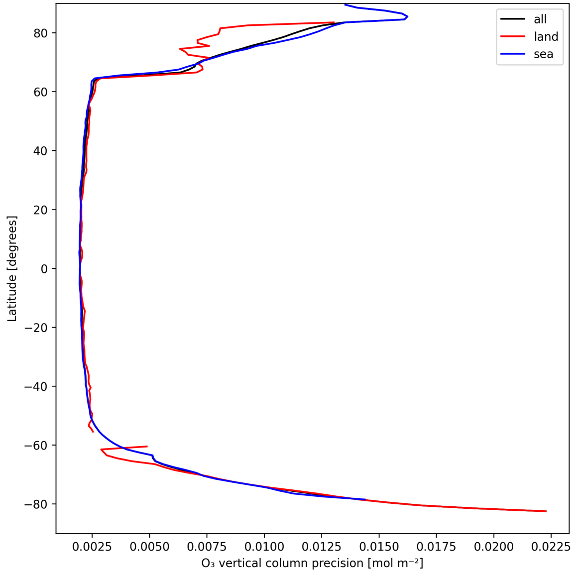
Figure 18: Zonal average of “O 3 vertical column precision” for 2025-04-06 to 2025-04-06.
