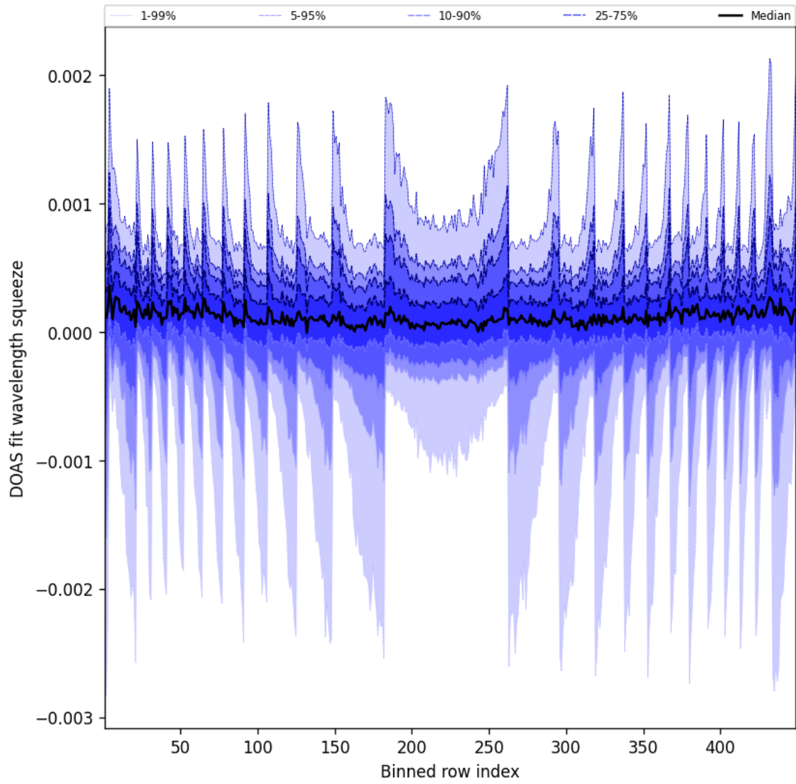
Figure 48: Along track statistics of “DOAS fit wavelength squeeze” for 2025-04-06 to 2025-04-06
