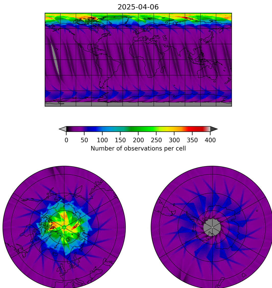
Figure 15: Map of the number of observations for 2025-04-06 to 2025-04-06
