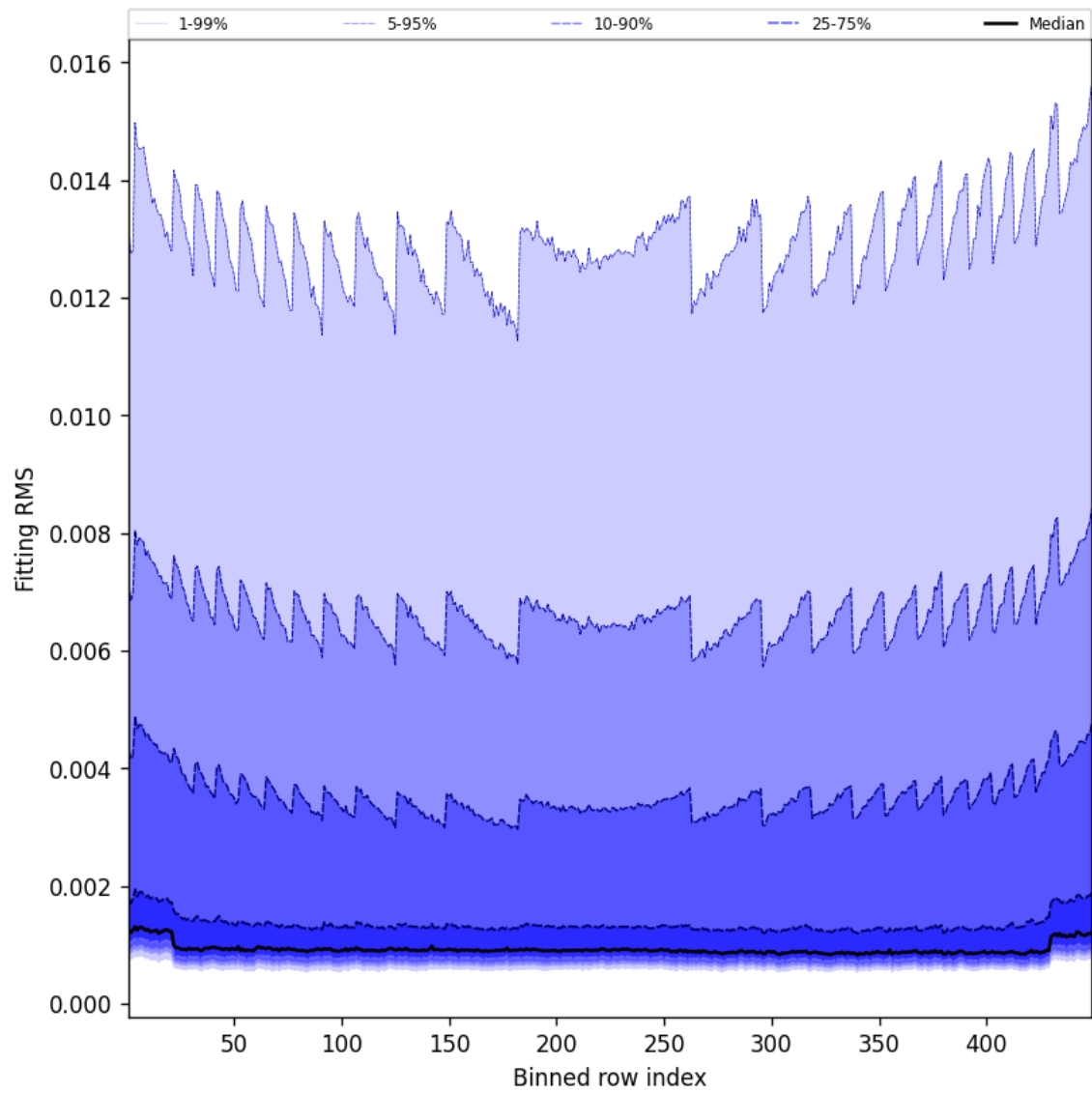
Figure 46: Along track statistics of “Fitting RMS” for 2025-04-06 to 2025-04-06
