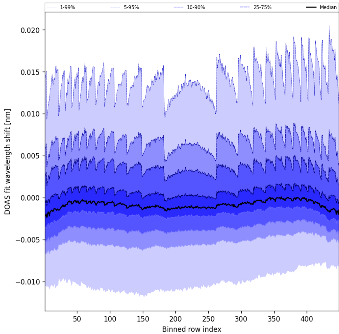
Figure 47: Along track statistics of "DOAS fit wavelength shift" for 2025-04-06 to 2025-04-06
