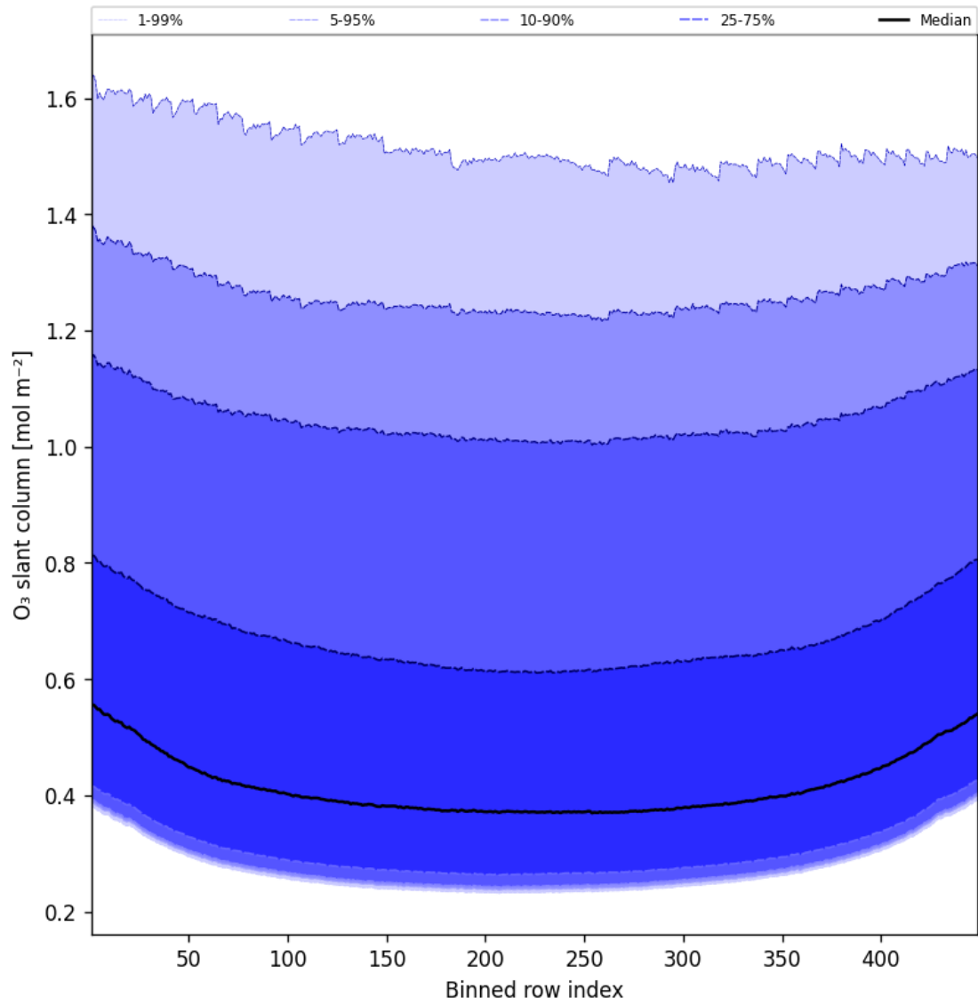
Figure 43: Along track statistics of “O 3 slant column” for 2025-04-06 to 2025-04-06
