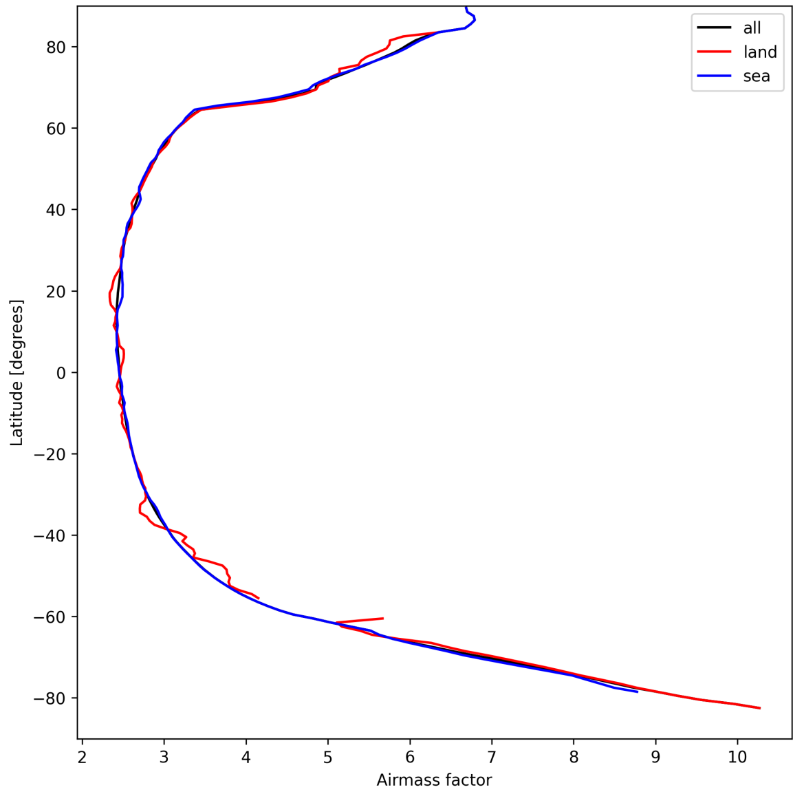
Figure 25: Zonal average of “Airmass factor” for 2025-04-06 to 2025-04-06.
