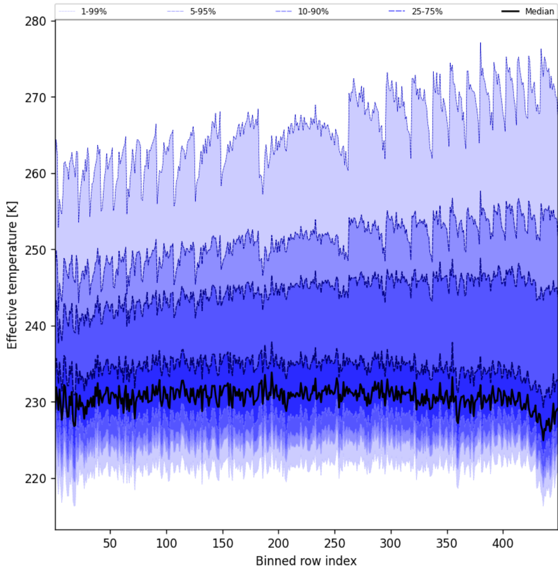
Figure 50: Along track statistics of “Effective temperature” for 2025-04-06 to 2025-04-06
