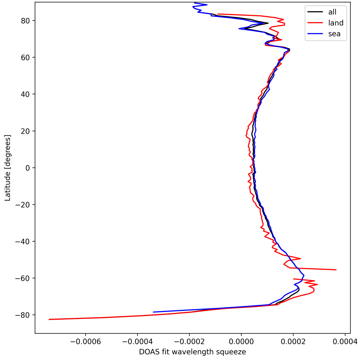
Figure 24: Zonal average of “DOAS fit wavelength squeeze” for 2025-04-06 to 2025-04-06.
