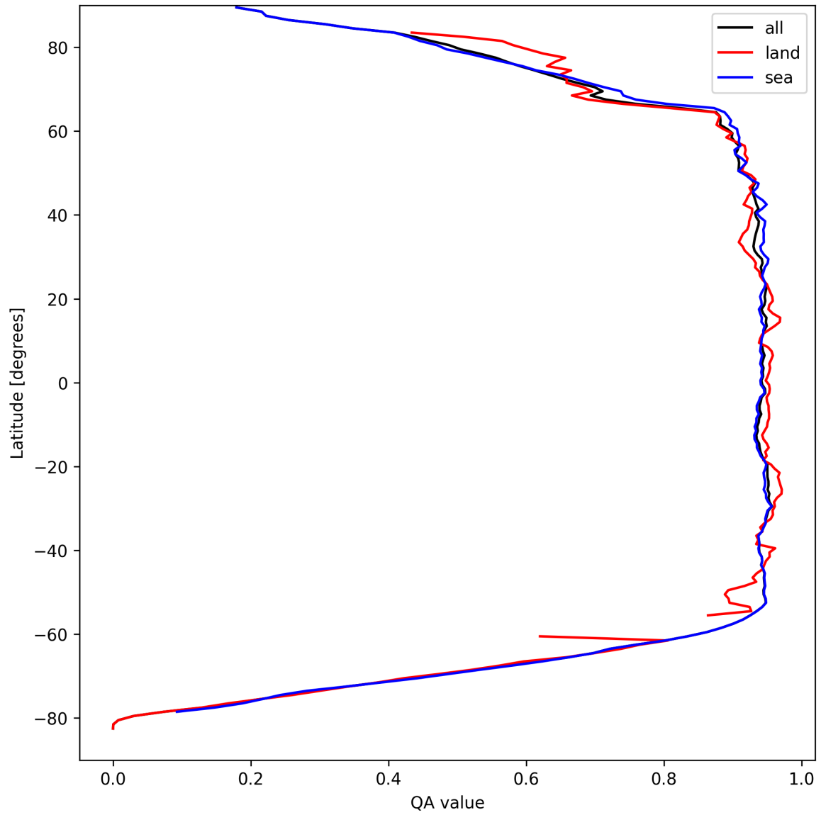
Figure 16: Zonal average of “QA value” for 2025-04-06 to 2025-04-06.
