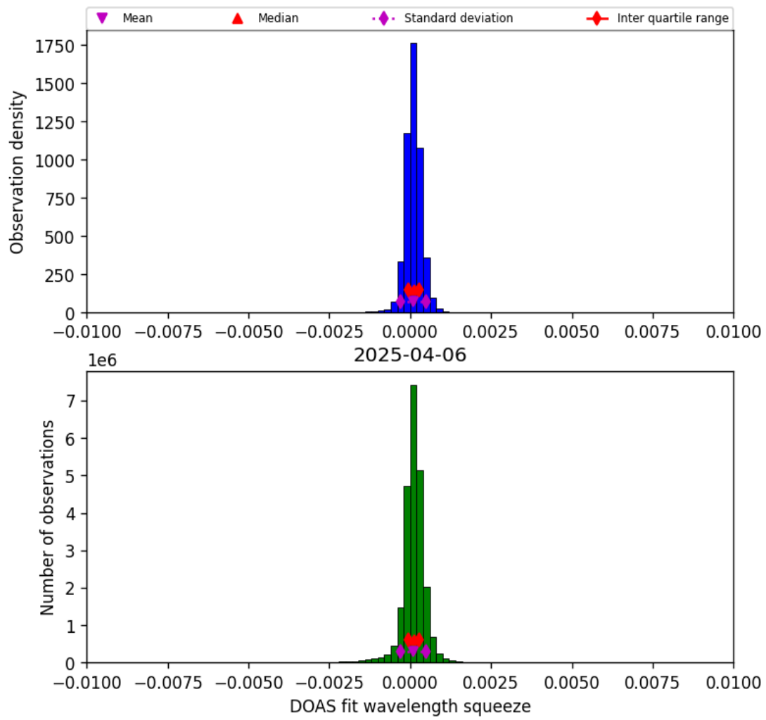
Figure 36: Histogram of “DOAS fit wavelength squeeze” for 2025-04-06 to 2025-04-06
