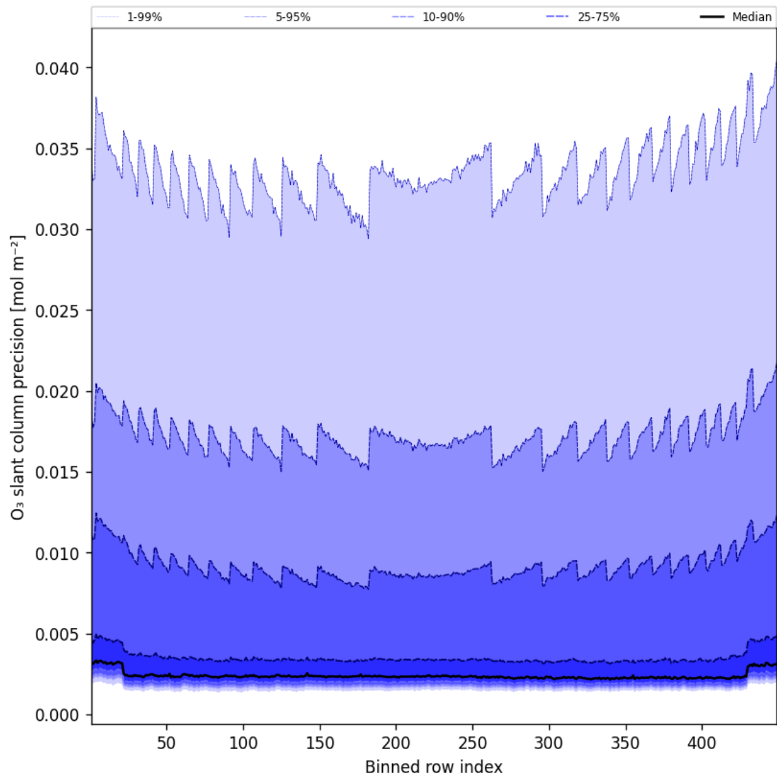
Figure 44: Along track statistics of “O 3 slant column precision” for 2025-04-06 to 2025-04-06
