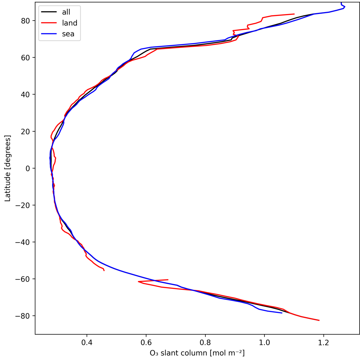
Figure 19: Zonal average of “O 3 slant column” for 2025-04-06 to 2025-04-06.
