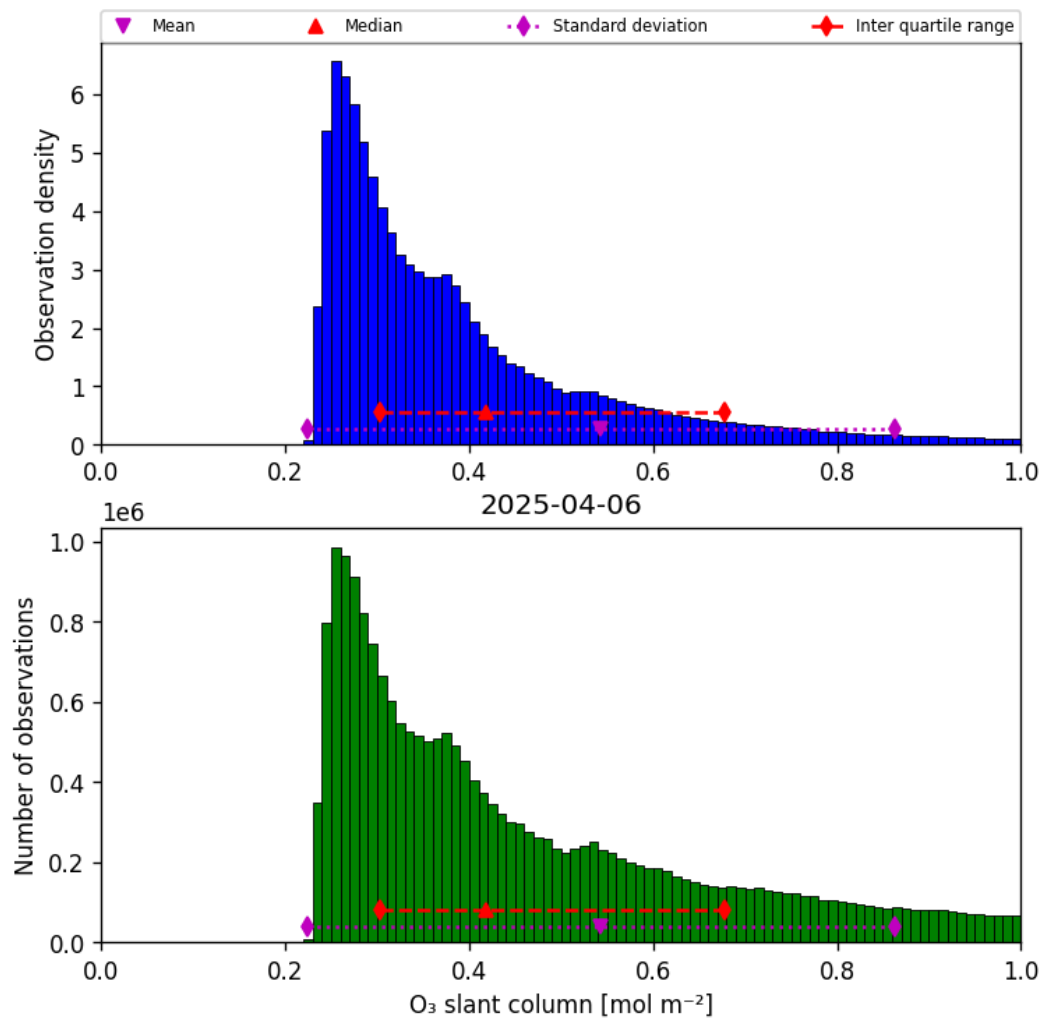
Figure 31: Histogram of “O 3 slant column” for 2025-04-06 to 2025-04-06
