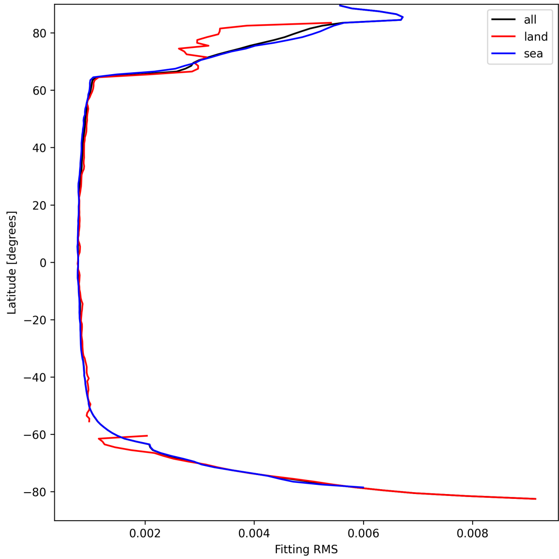
Figure 22: Zonal average of “Fitting RMS” for 2025-04-06 to 2025-04-06.
