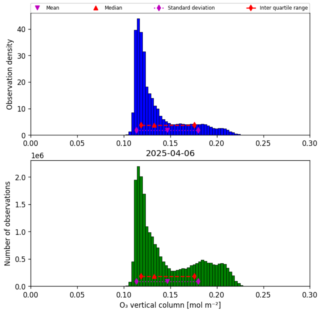
Figure 29: Histogram of “O 3 vertical column” for 2025-04-06 to 2025-04-06
