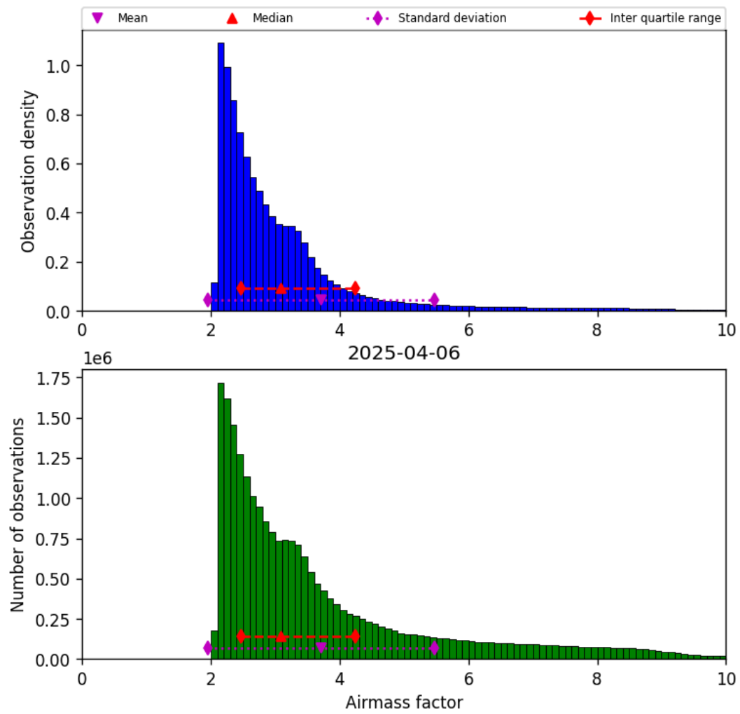
Figure 37: Histogram of “Airmass factor” for 2025-04-06 to 2025-04-06
