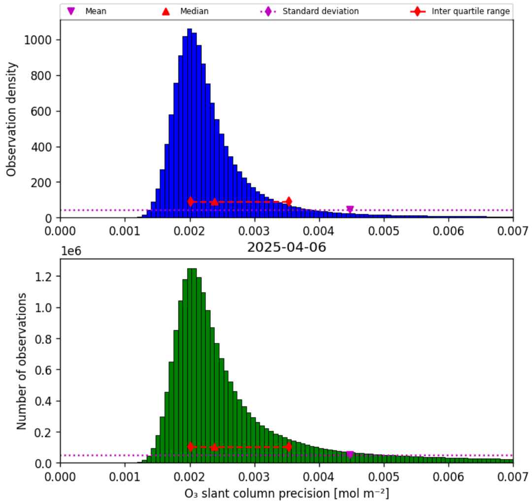
Figure 32: Histogram of “O 3 slant column precision” for 2025-04-06 to 2025-04-06
