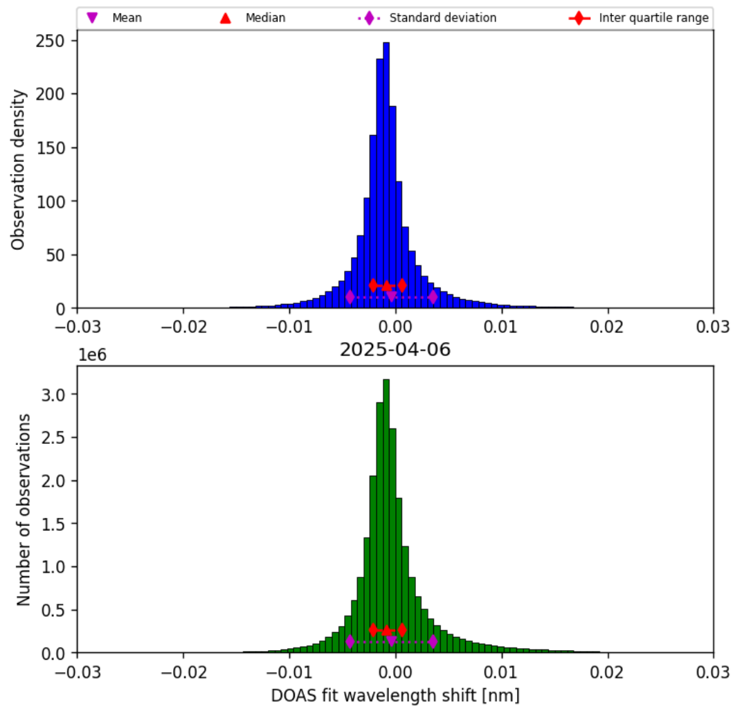
Figure 35: Histogram of “DOAS fit wavelength shift” for 2025-04-06 to 2025-04-06
