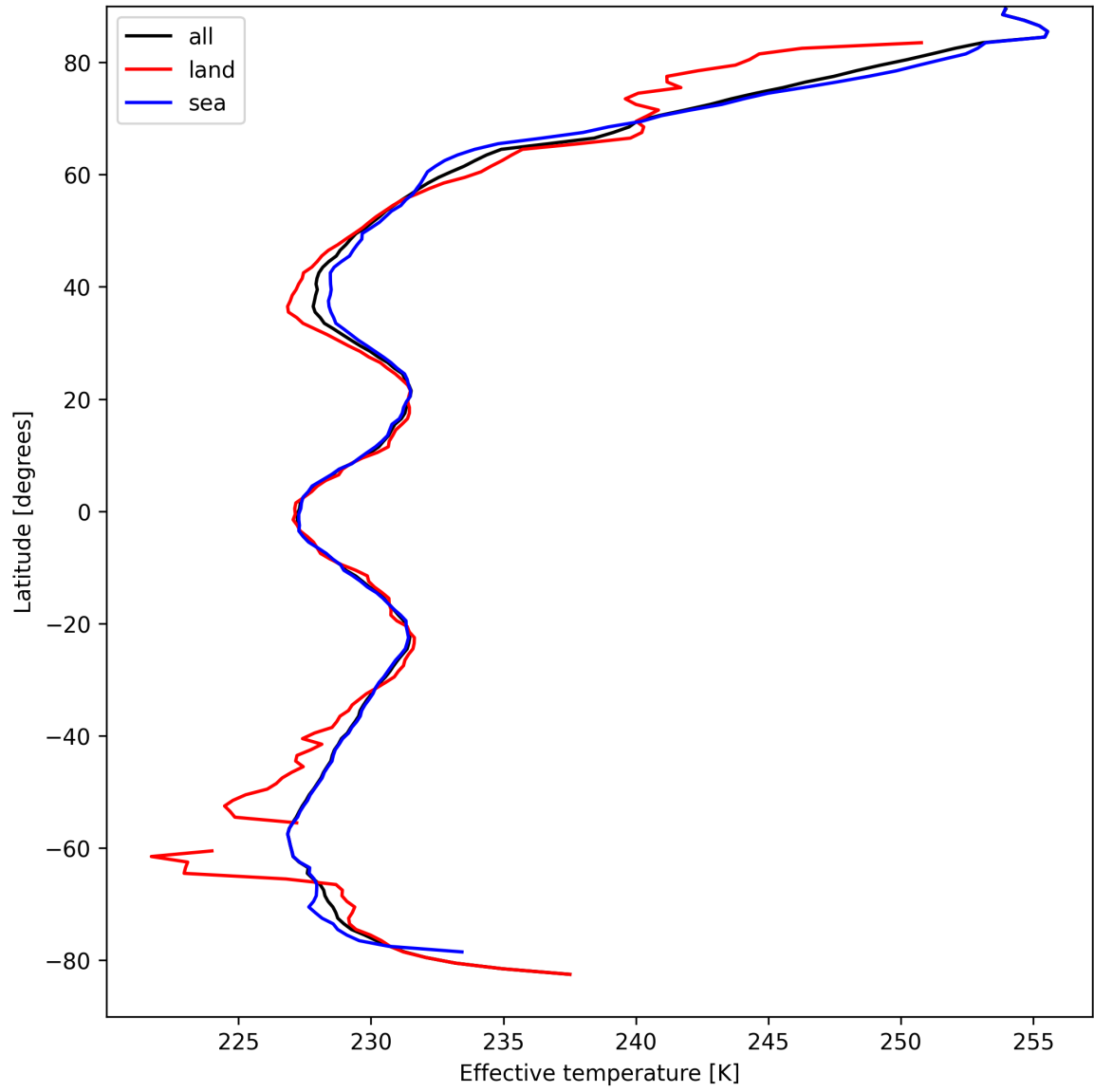
Figure 26: Zonal average of “Effective temperature” for 2025-04-06 to 2025-04-06.
