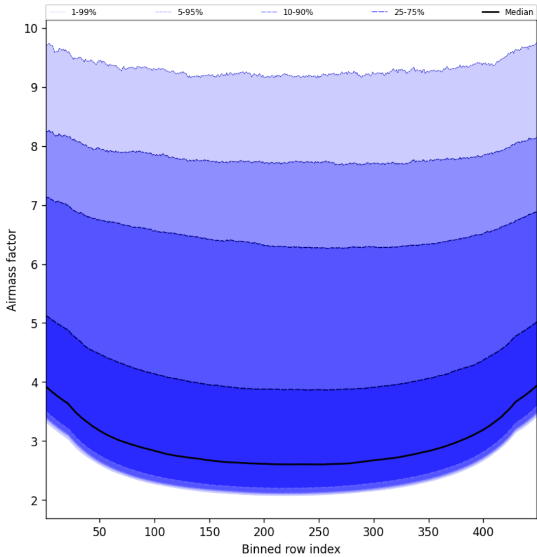
Figure 49: Along track statistics of “Airmass factor” for 2025-04-06 to 2025-04-06
