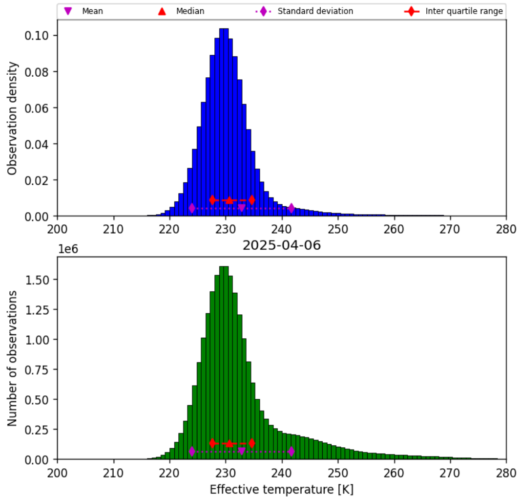
Figure 38: Histogram of “Effective temperature” for 2025-04-06 to 2025-04-06
