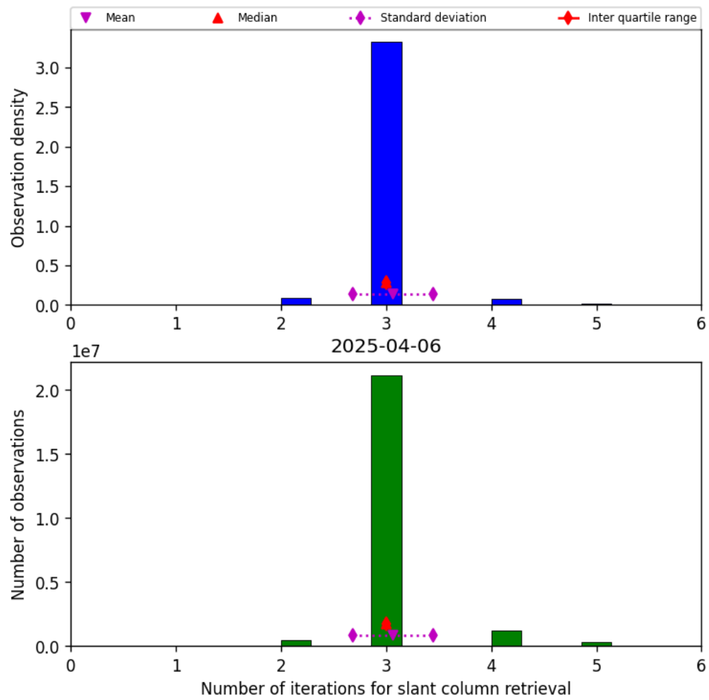
Figure 33: Histogram of “Number of iterations for slant column retrieval” for 2025-04-06 to 2025-04-06
