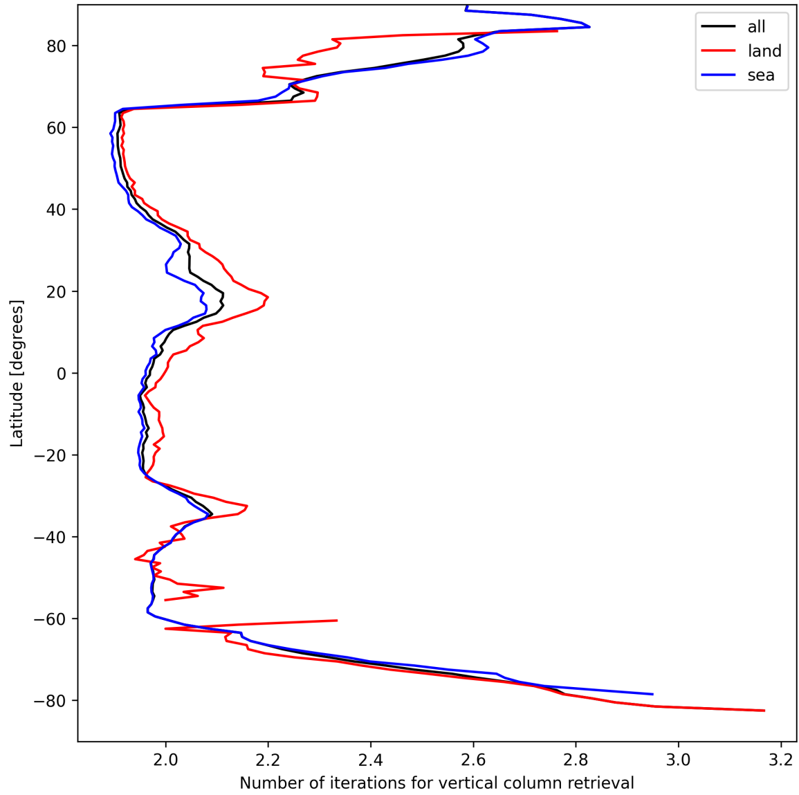
Figure 27: Zonal average of “Number of iterations for vertical column retrieval” for 2025-04-06 to 2025-04-06.
