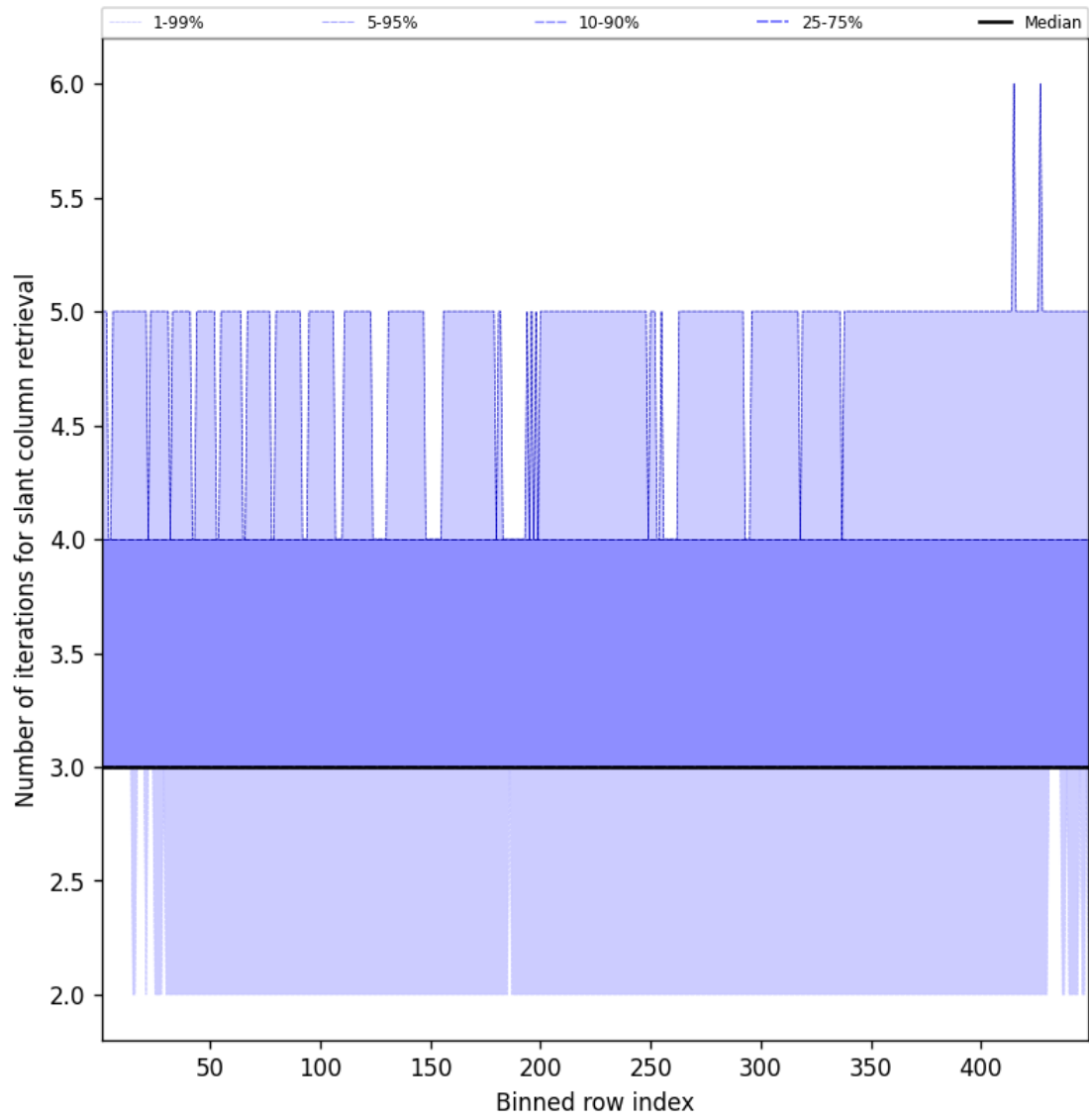
Figure 45: Along track statistics of “Number of iterations for slant column retrieval” for 2025-04-06 to 2025-04-06
