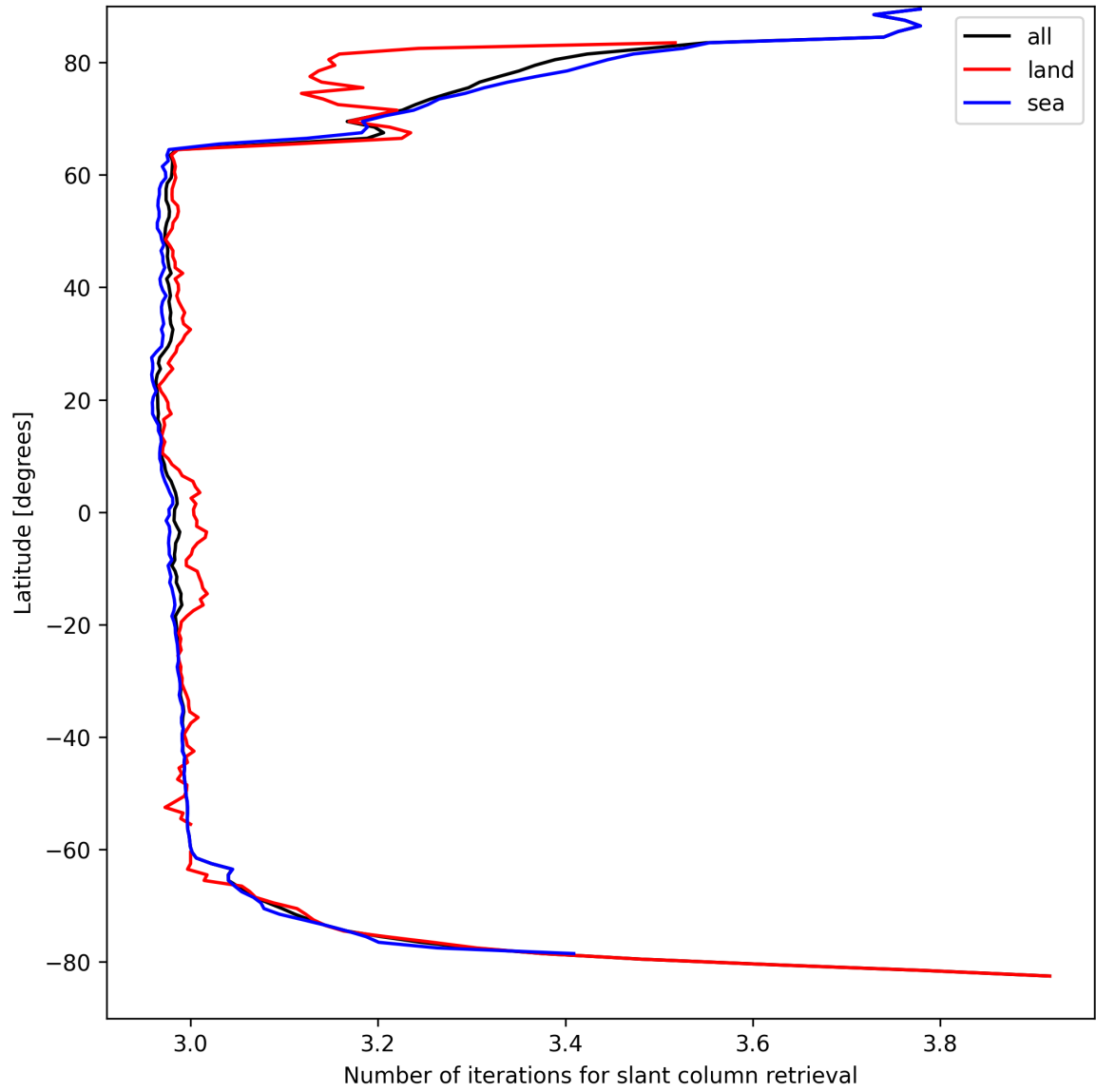
Figure 21: Zonal average of “Number of iterations for slant column retrieval” for 2025-04-06 to 2025-04-06.
