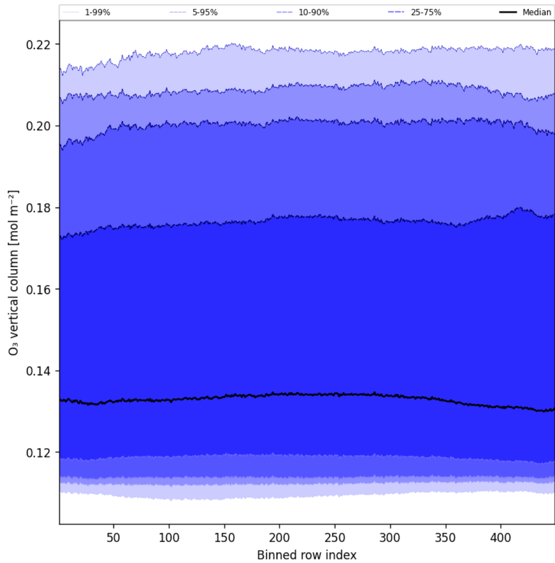
Figure 41: Along track statistics of “O 3 vertical column” for 2025-04-06 to 2025-04-06
