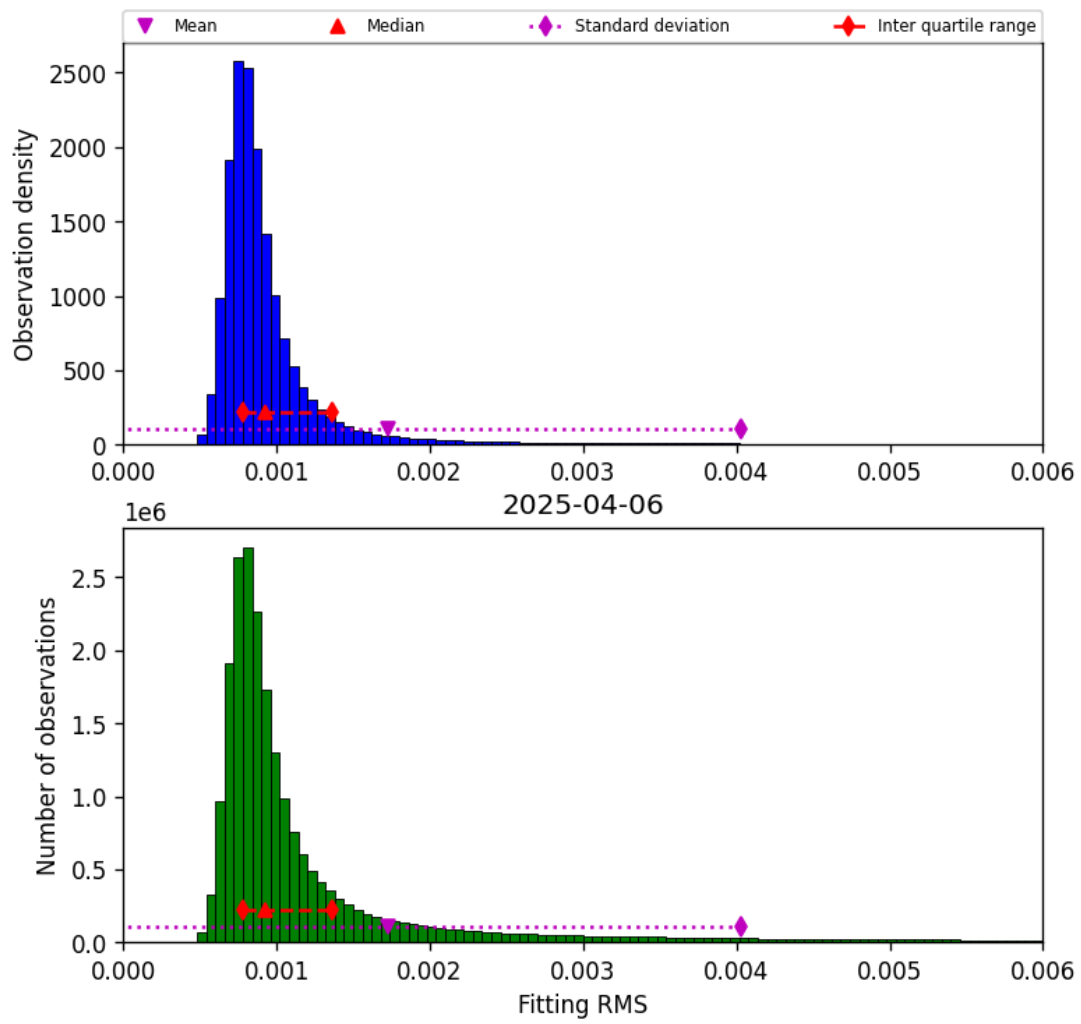
Figure 34: Histogram of “Fitting RMS” for 2025-04-06 to 2025-04-06
