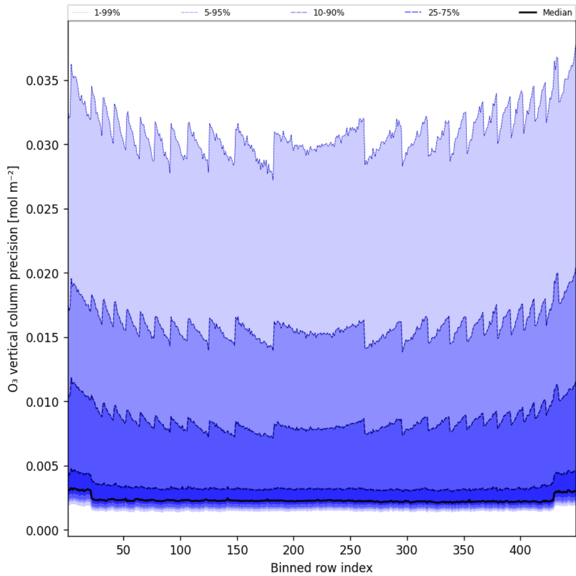
Figure 42: Along track statistics of “O 3 vertical column precision” for 2025-04-06 to 2025-04-06
