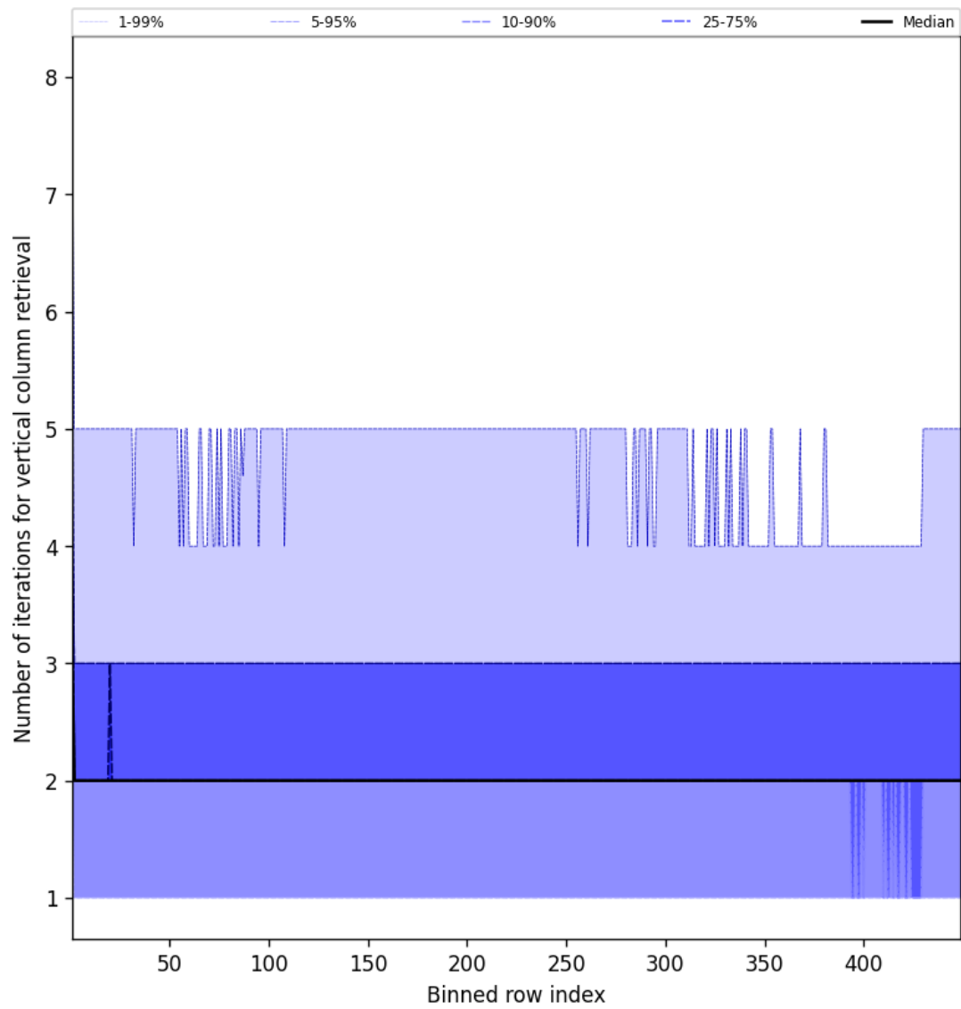
Figure 51: Along track statistics of “Number of iterations for vertical column retrieval” for 2025-04-06 to 2025-04-06
