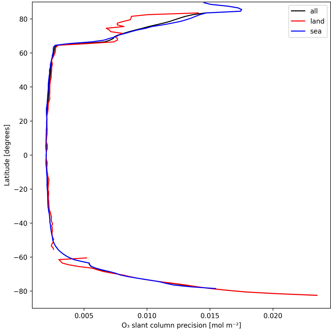
Figure 20: Zonal average of “O 3 slant column precision” for 2025-04-06 to 2025-04-06.
