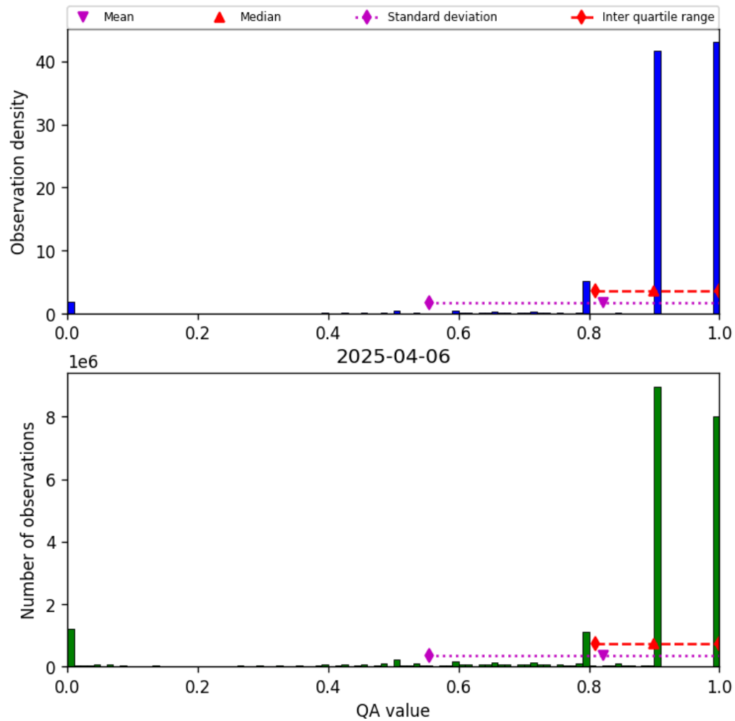
Figure 28: Histogram of “QA value” for 2025-04-06 to 2025-04-06
