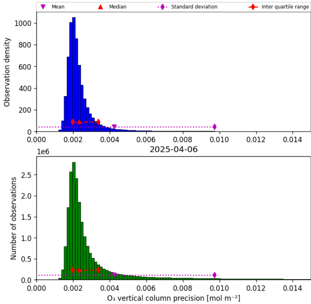
Figure 30: Histogram of "O 3 vertical column precision" for 2025-04-06 to 2025-04-06
