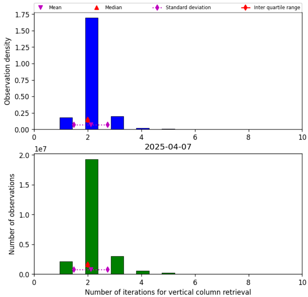
Figure 39: Histogram of “Number of iterations for vertical column retrieval” for 2025-04-07 to 2025-04-08
