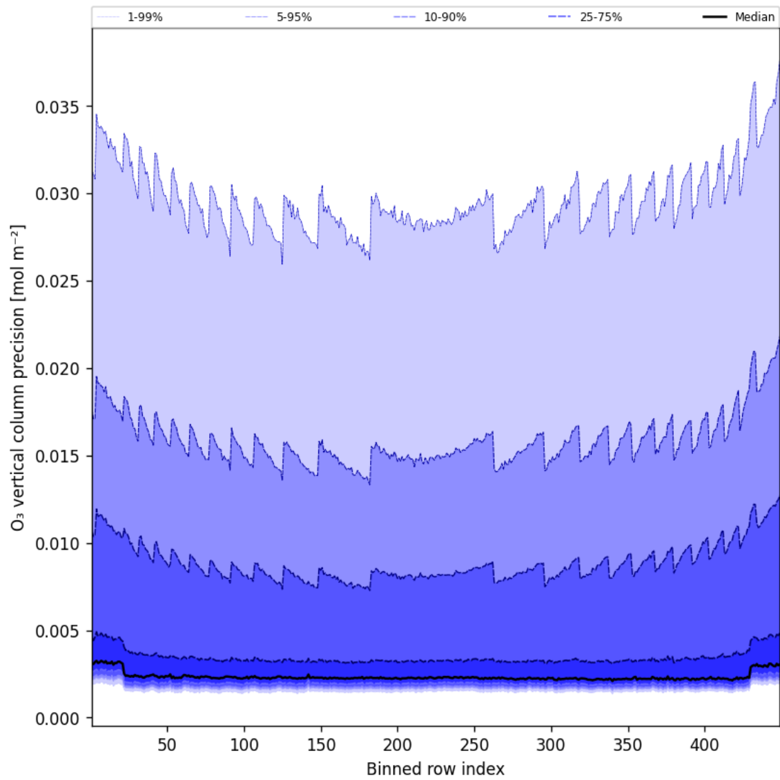
Figure 42: Along track statistics of “O 3 vertical column precision” for 2025-04-07 to 2025-04-08
