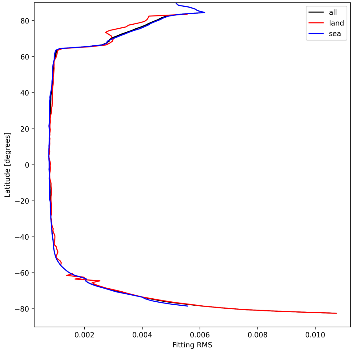
Figure 22: Zonal average of “Fitting RMS” for 2025-04-07 to 2025-04-08.
