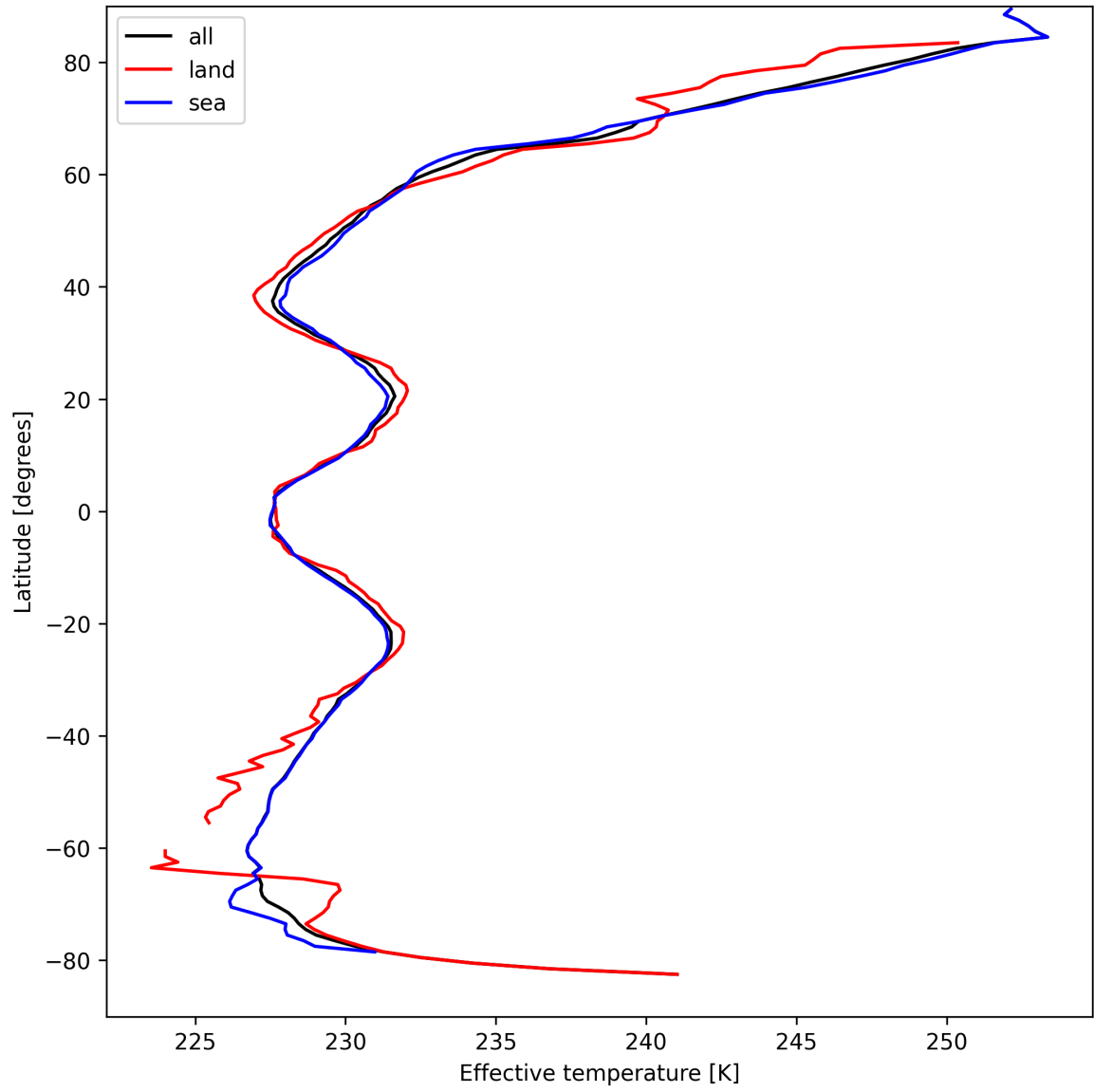
Figure 26: Zonal average of “Effective temperature” for 2025-04-07 to 2025-04-08.
