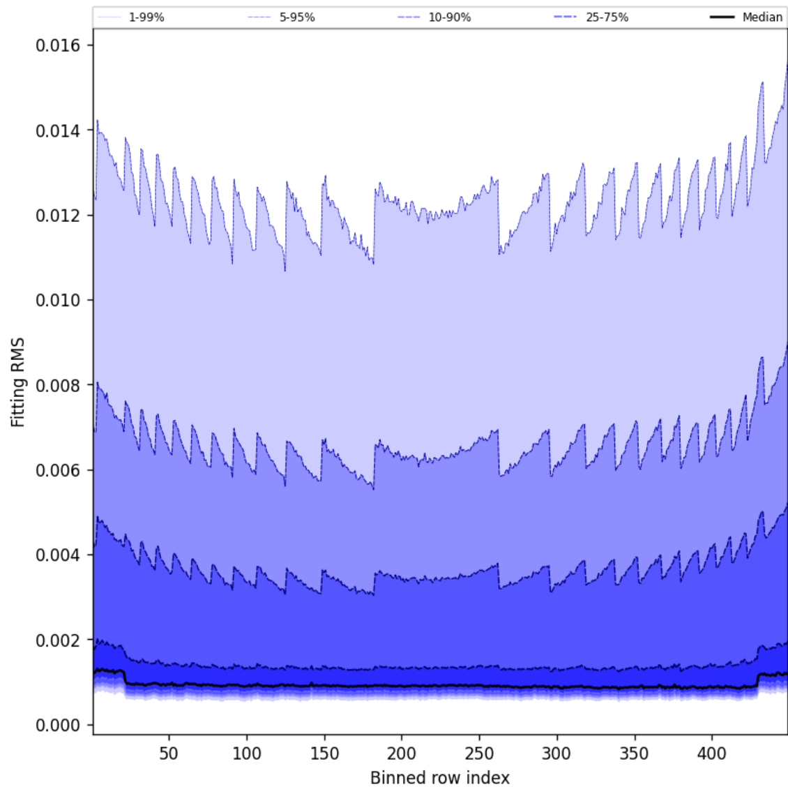
Figure 46: Along track statistics of “Fitting RMS” for 2025-04-07 to 2025-04-08
