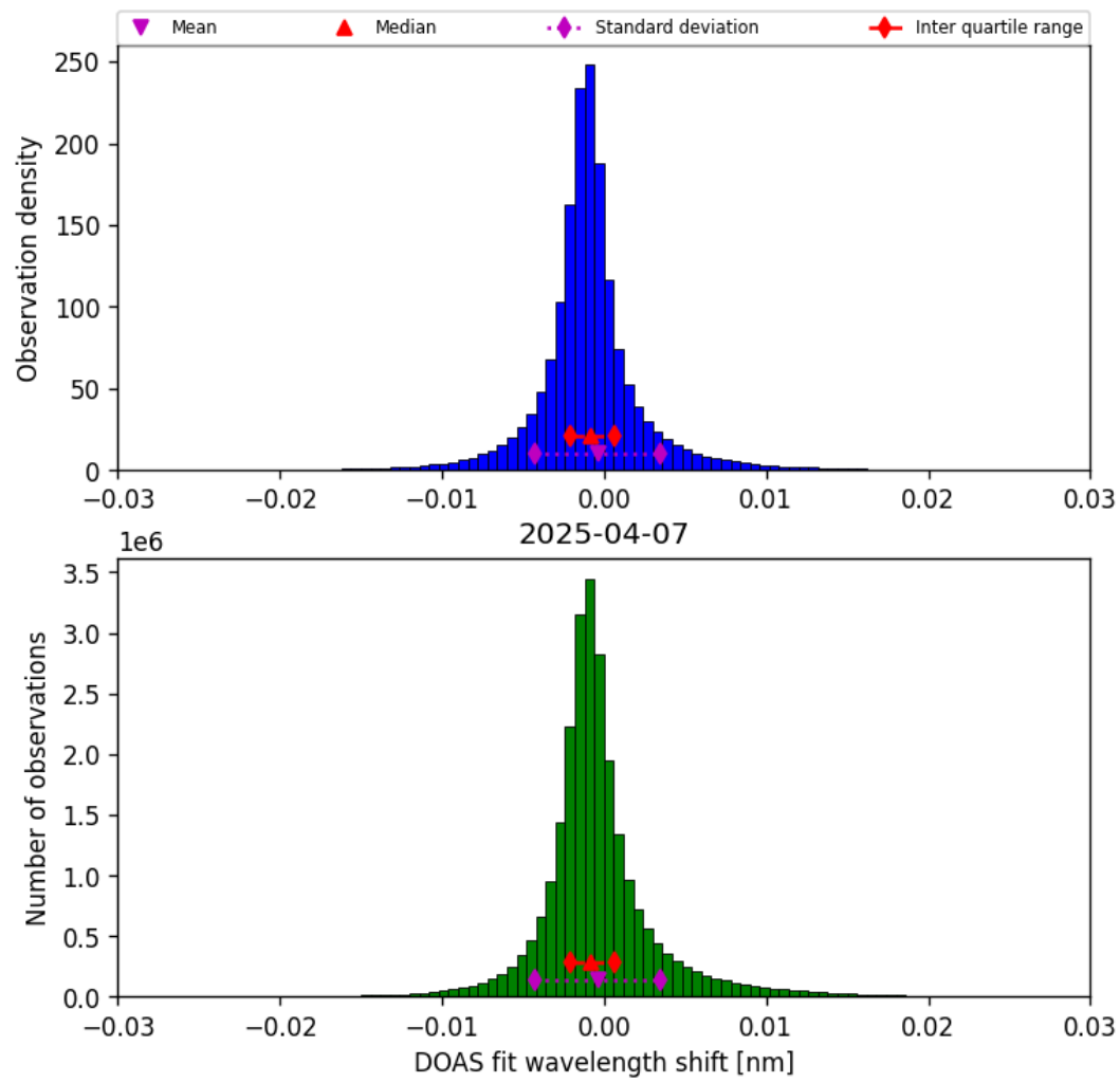
Figure 35: Histogram of “DOAS fit wavelength shift” for 2025-04-07 to 2025-04-08
