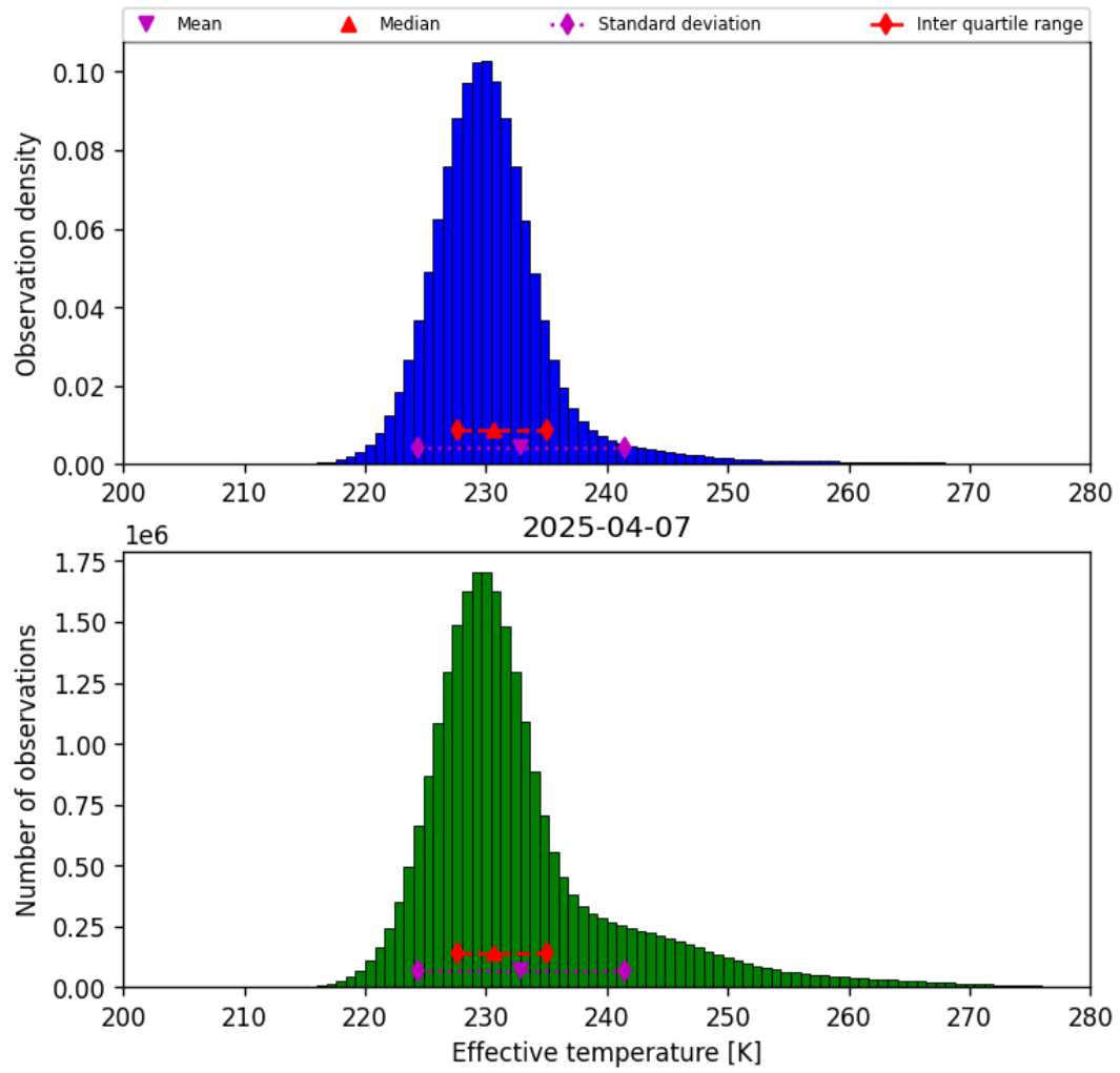
Figure 38: Histogram of “Effective temperature” for 2025-04-07 to 2025-04-08
