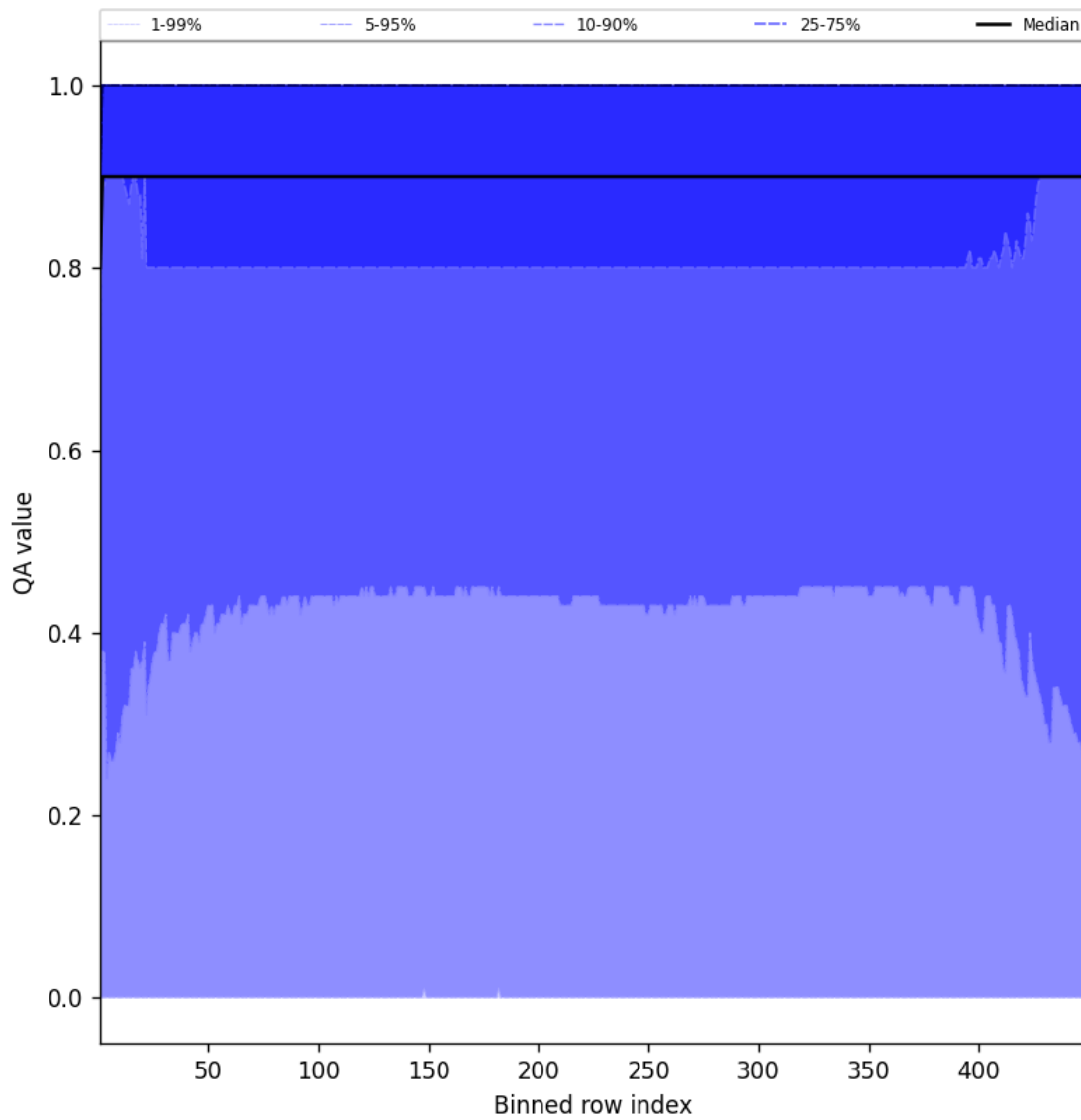
Figure 40: Along track statistics of “QA value” for 2025-04-07 to 2025-04-08
