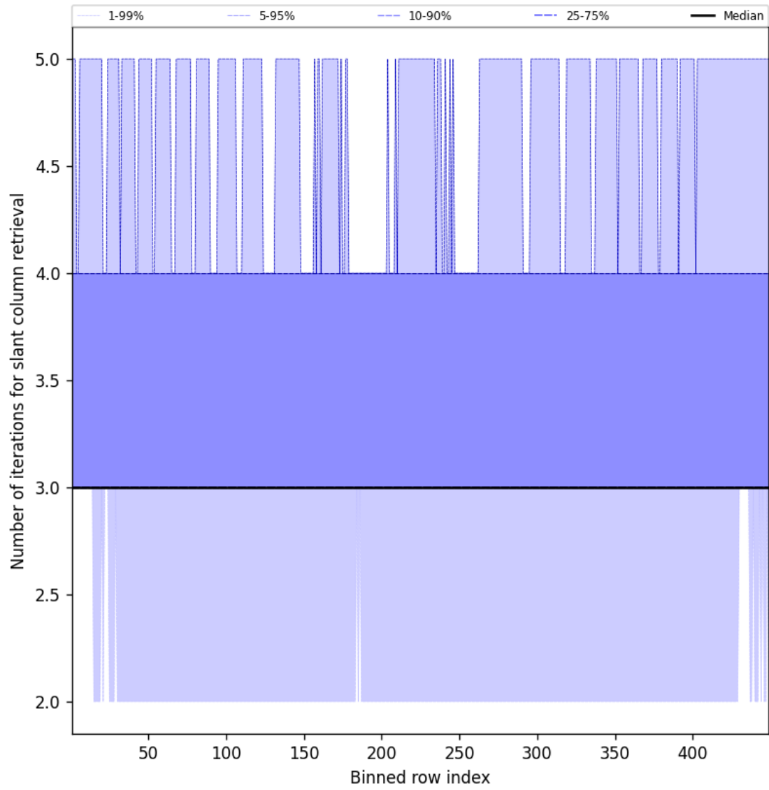
Figure 45: Along track statistics of “Number of iterations for slant column retrieval” for 2025-04-07 to 2025-04-08
