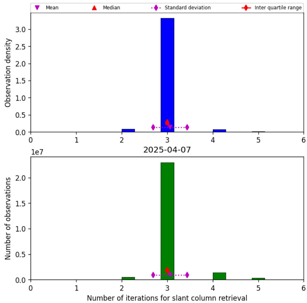
Figure 33: Histogram of "Number of iterations for slant column retrieval" for 2025-04-07 to 2025-04-08
