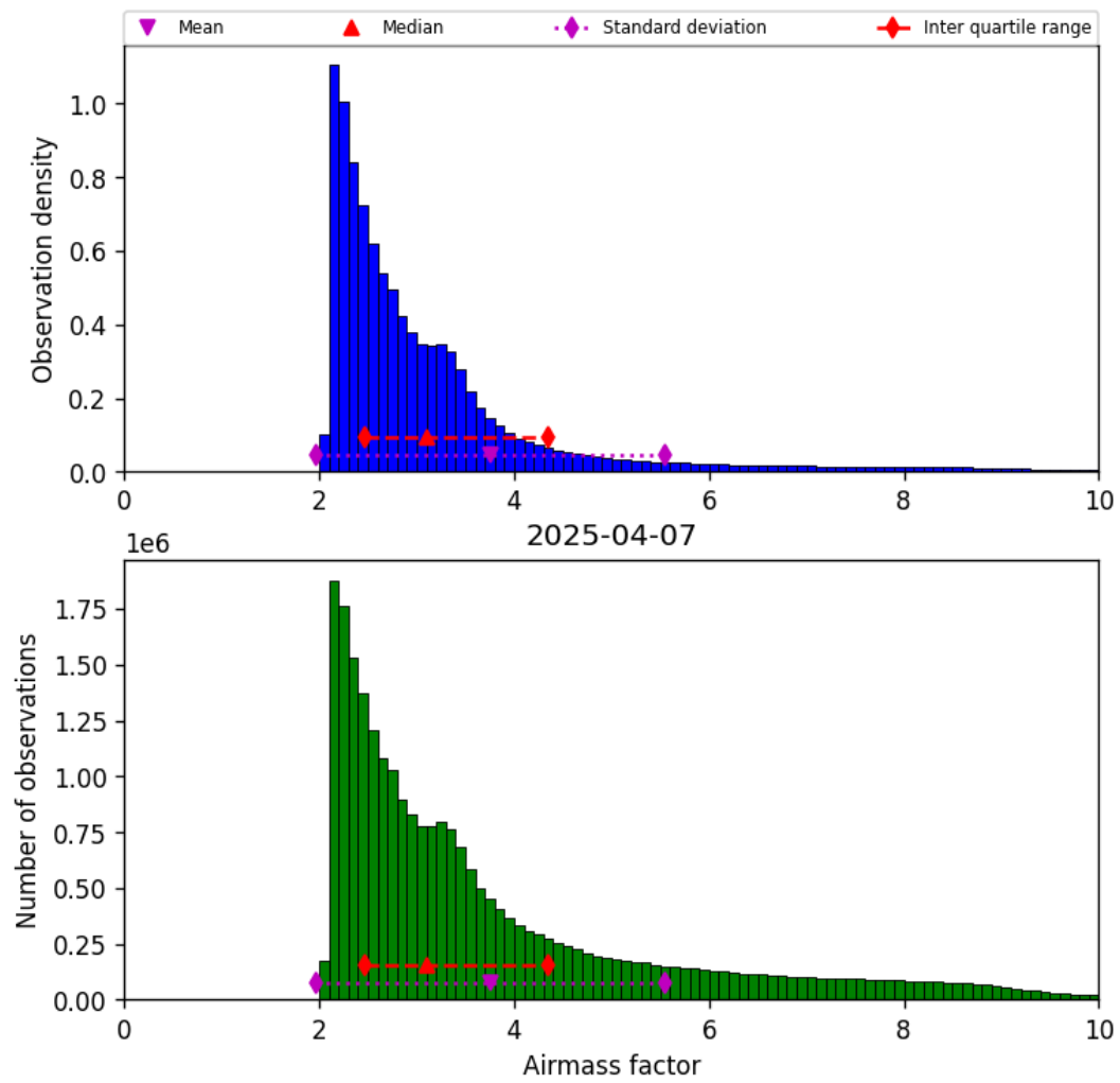
Figure 37: Histogram of “Airmass factor” for 2025-04-07 to 2025-04-08
