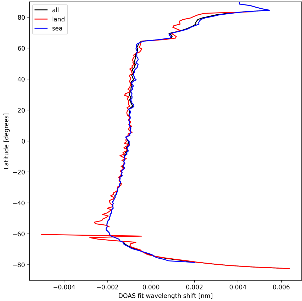
Figure 23: Zonal average of “DOAS fit wavelength shift” for 2025-04-07 to 2025-04-08.
