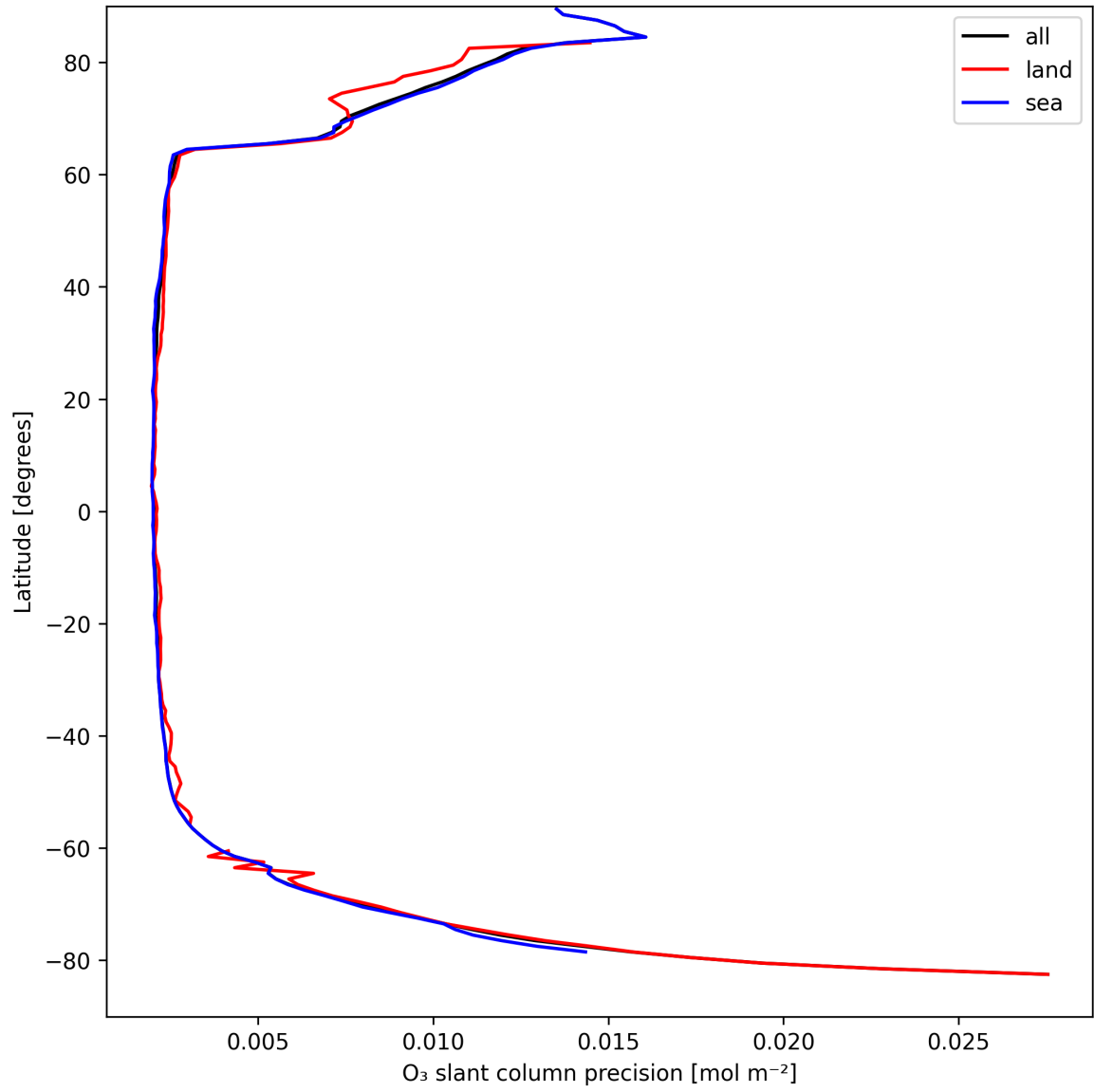
Figure 20: Zonal average of “O 3 slant column precision” for 2025-04-07 to 2025-04-08.
