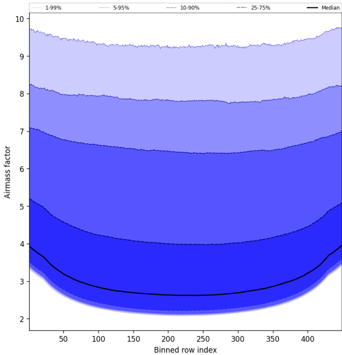
Figure 49: Along track statistics of “Airmass factor” for 2025-04-07 to 2025-04-08
