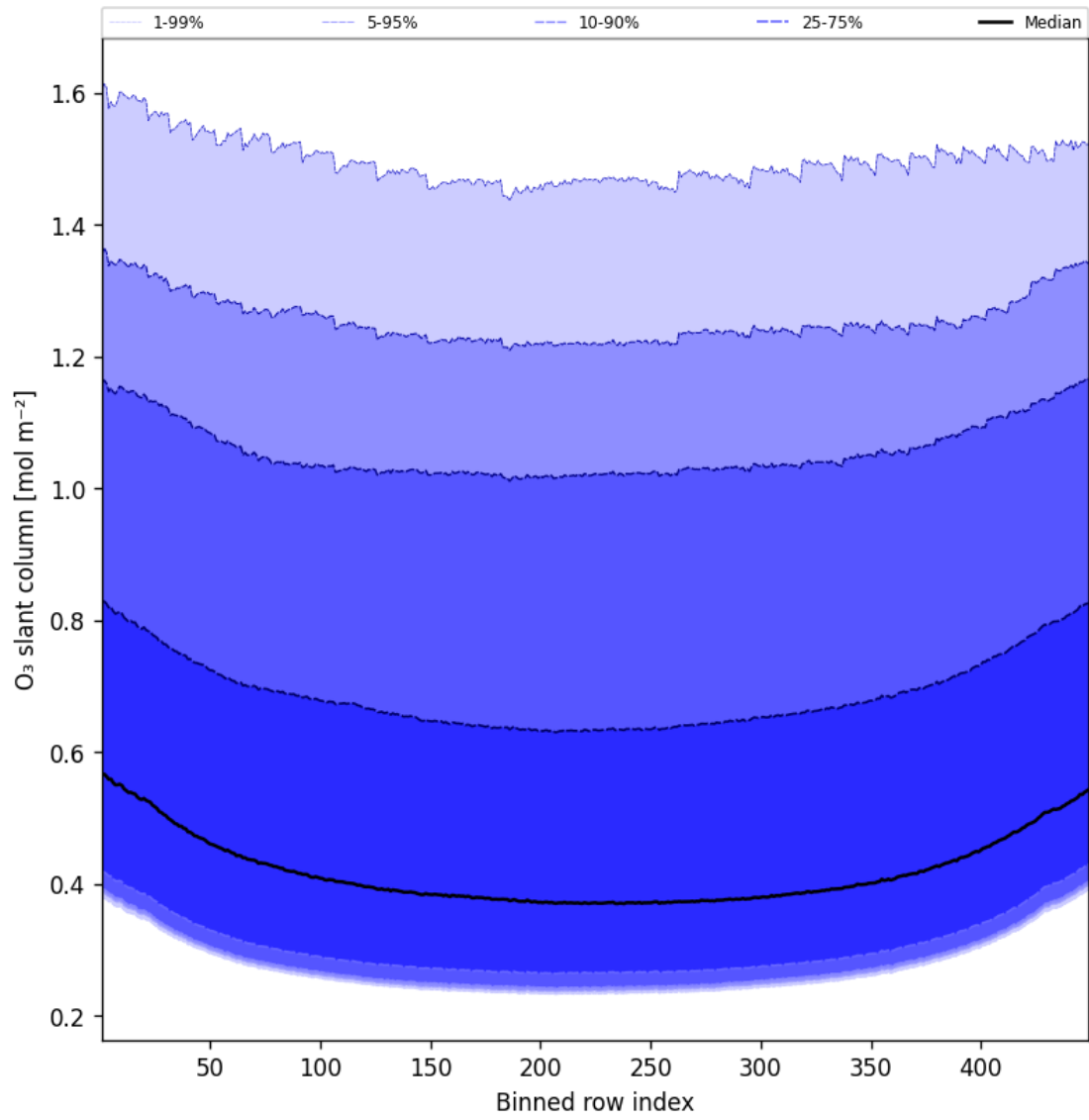
Figure 43: Along track statistics of “O 3 slant column” for 2025-04-07 to 2025-04-08
