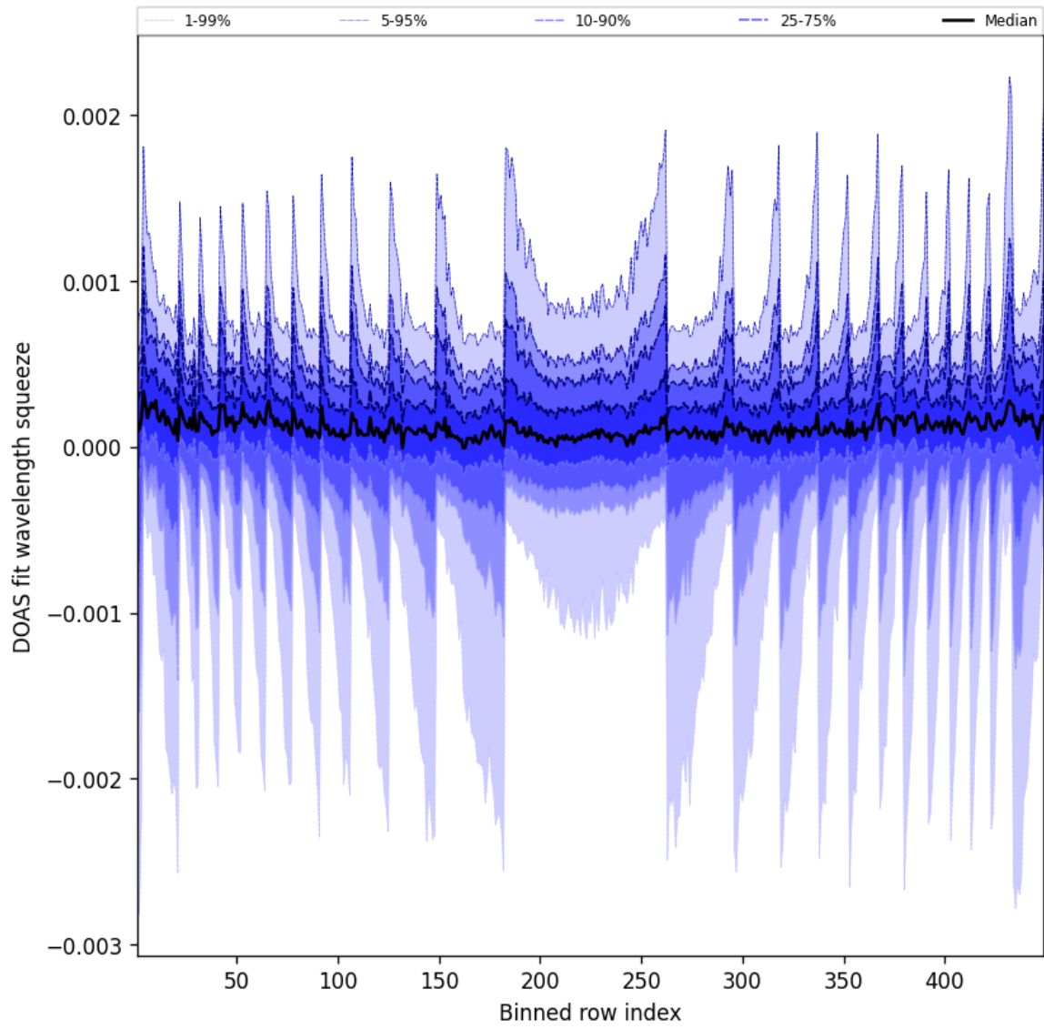
Figure 48: Along track statistics of “DOAS fit wavelength squeeze” for 2025-04-07 to 2025-04-08
