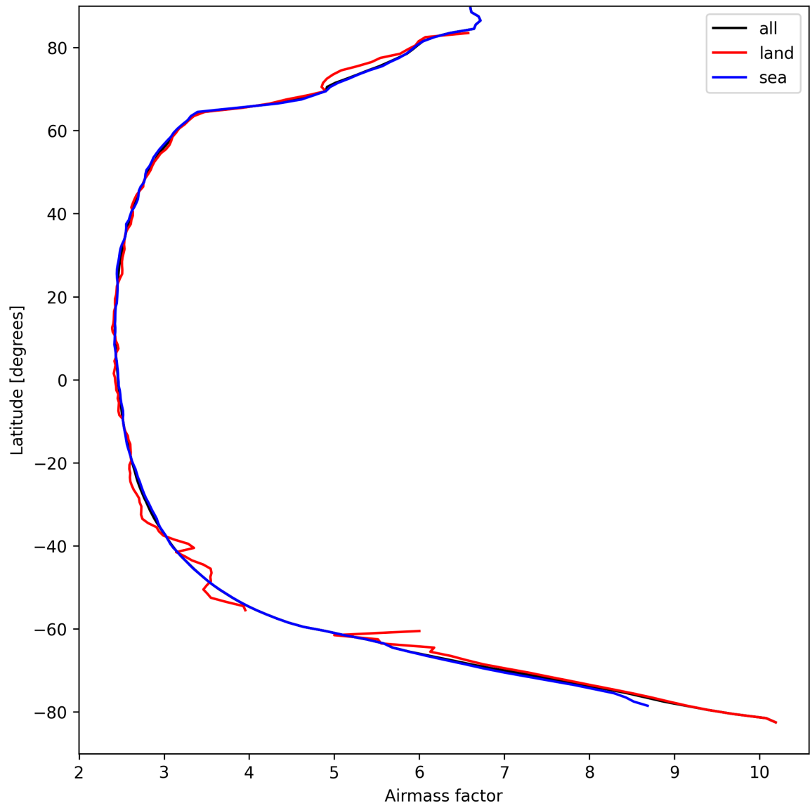
Figure 25: Zonal average of “Airmass factor” for 2025-04-07 to 2025-04-08.
