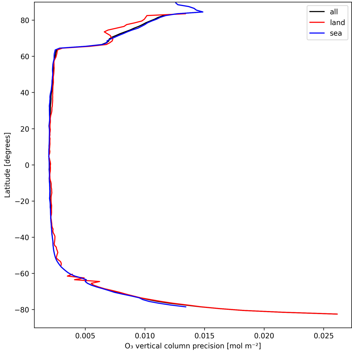
Figure 18: Zonal average of “O 3 vertical column precision” for 2025-04-07 to 2025-04-08.
