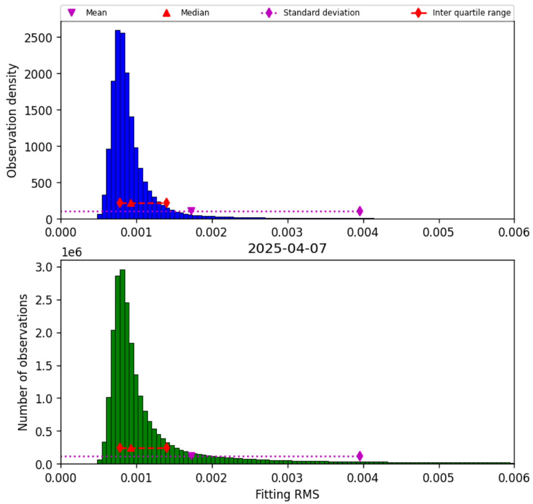
Figure 34: Histogram of “Fitting RMS” for 2025-04-07 to 2025-04-08
