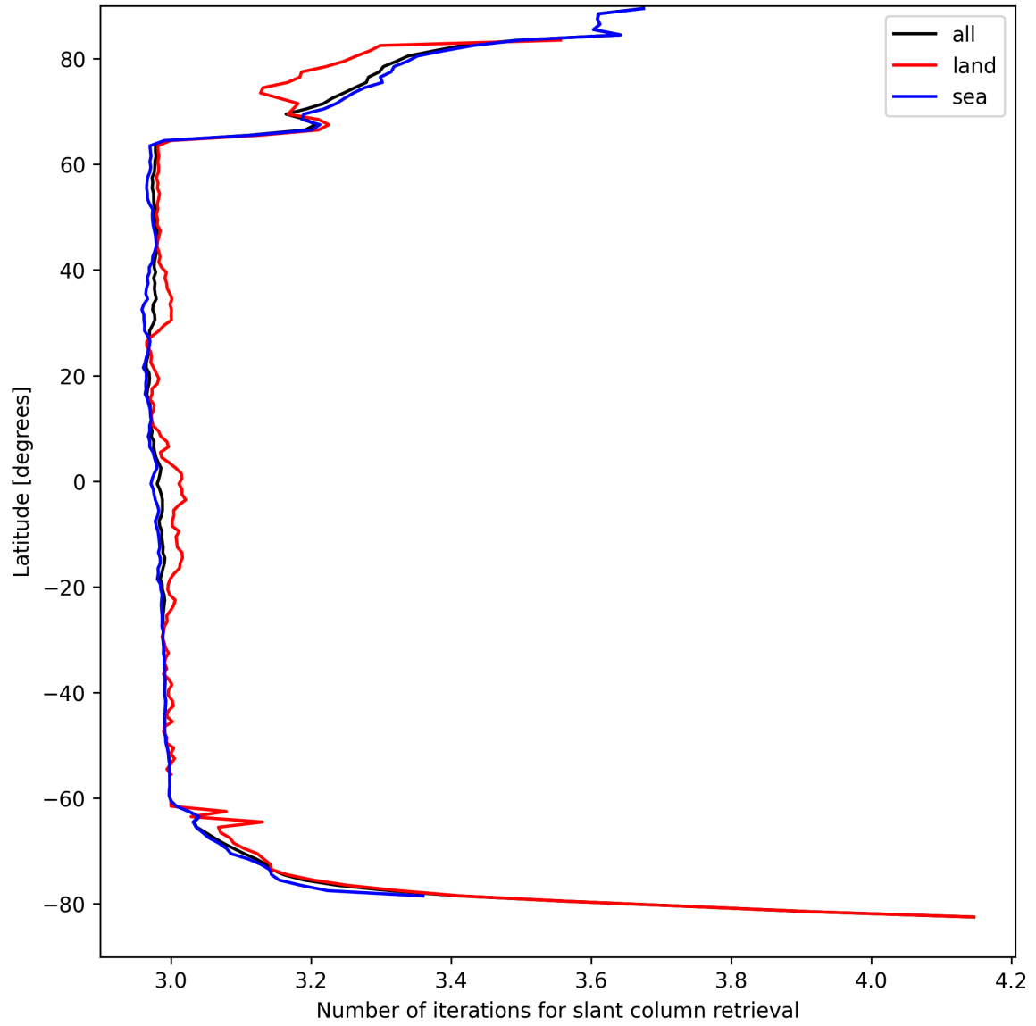
Figure 21: Zonal average of “Number of iterations for slant column retrieval” for 2025-04-07 to 2025-04-08.
