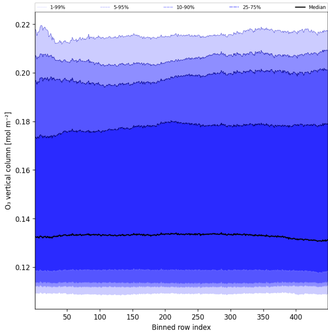
Figure 41: Along track statistics of “O 3 vertical column” for 2025-04-07 to 2025-04-08
