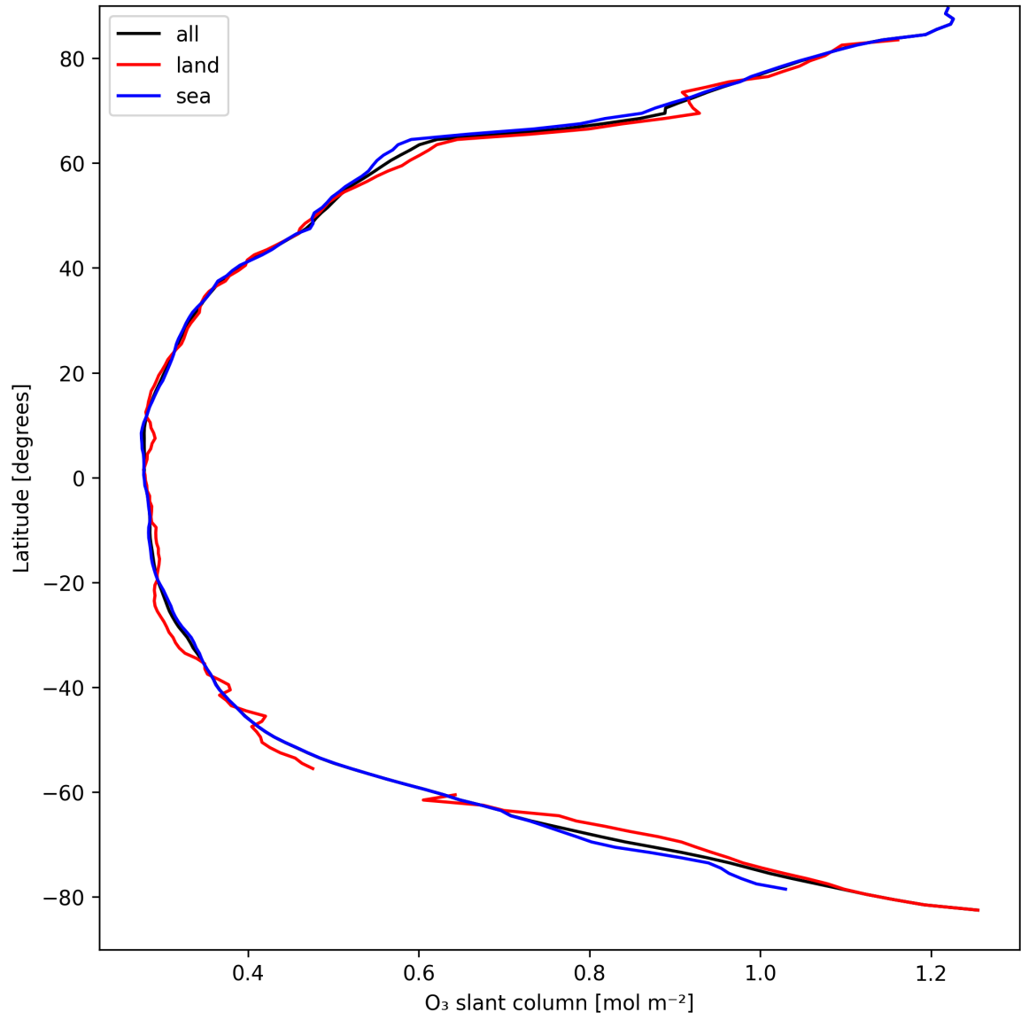
Figure 19: Zonal average of “O 3 slant column” for 2025-04-07 to 2025-04-08.
