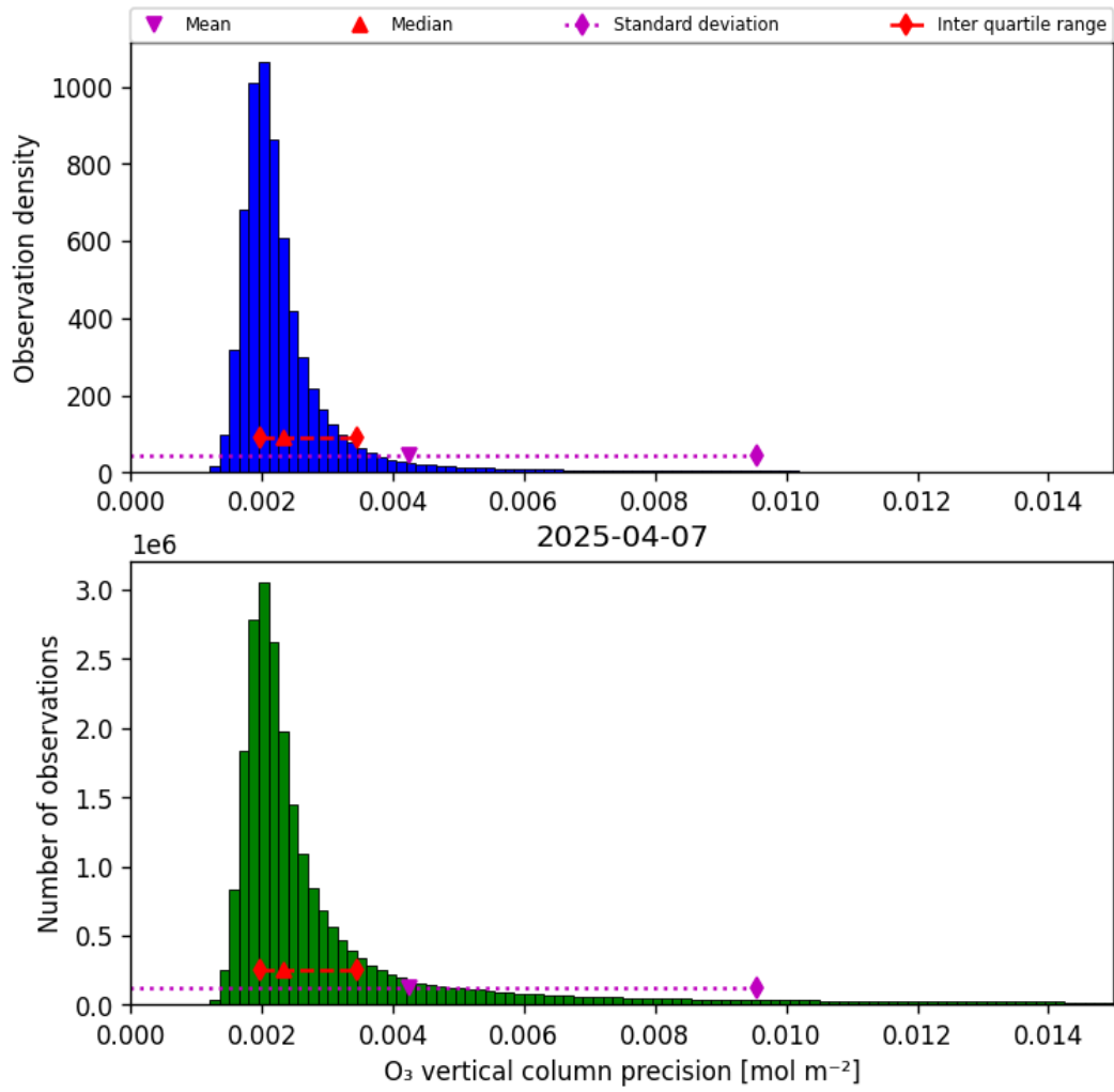
Figure 30: Histogram of “O 3 vertical column precision” for 2025-04-07 to 2025-04-08
