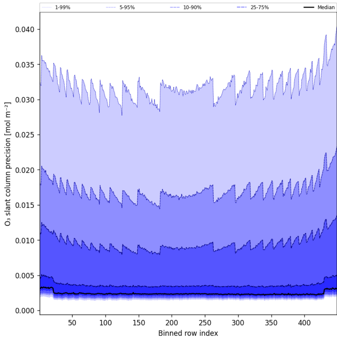
Figure 44: Along track statistics of “O 3 slant column precision” for 2025-04-07 to 2025-04-08
