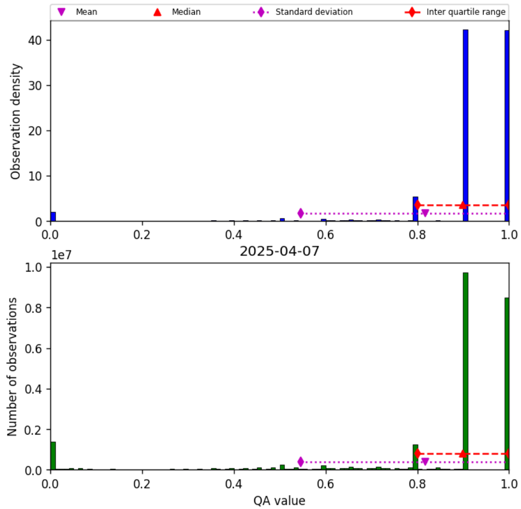
Figure 28: Histogram of “QA value” for 2025-04-07 to 2025-04-08
