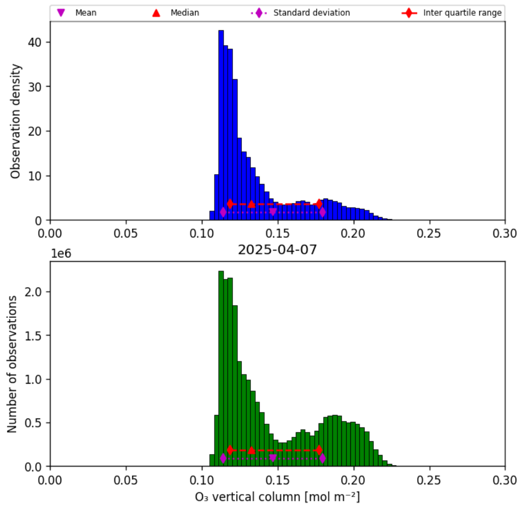
Figure 29: Histogram of “O 3 vertical column” for 2025-04-07 to 2025-04-08
