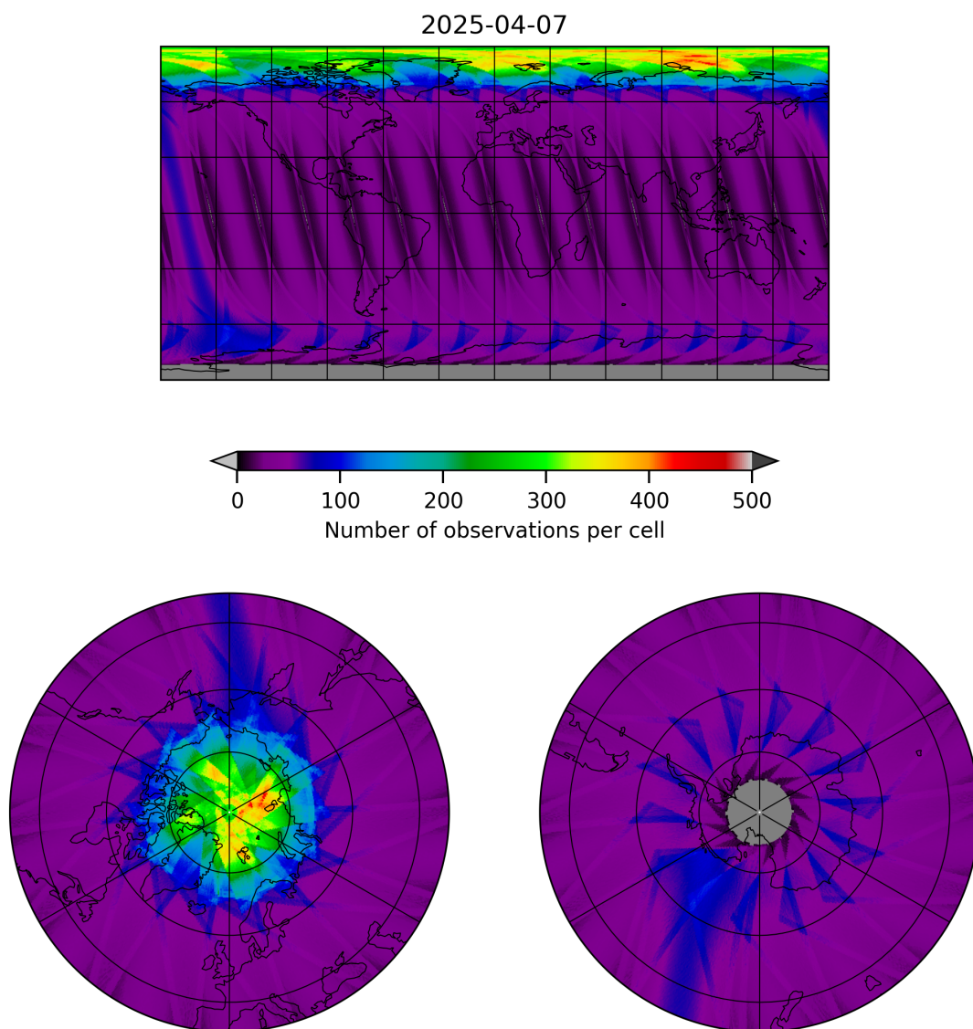
Figure 15: Map of the number of observations for 2025-04-07 to 2025-04-08
