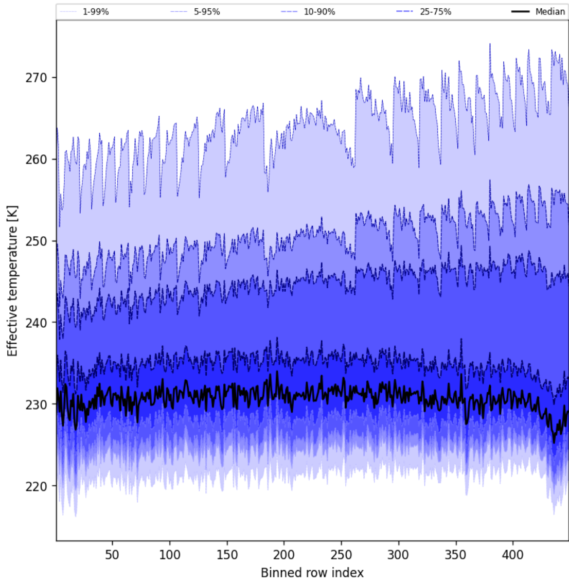
Figure 50: Along track statistics of “Effective temperature” for 2025-04-07 to 2025-04-08
