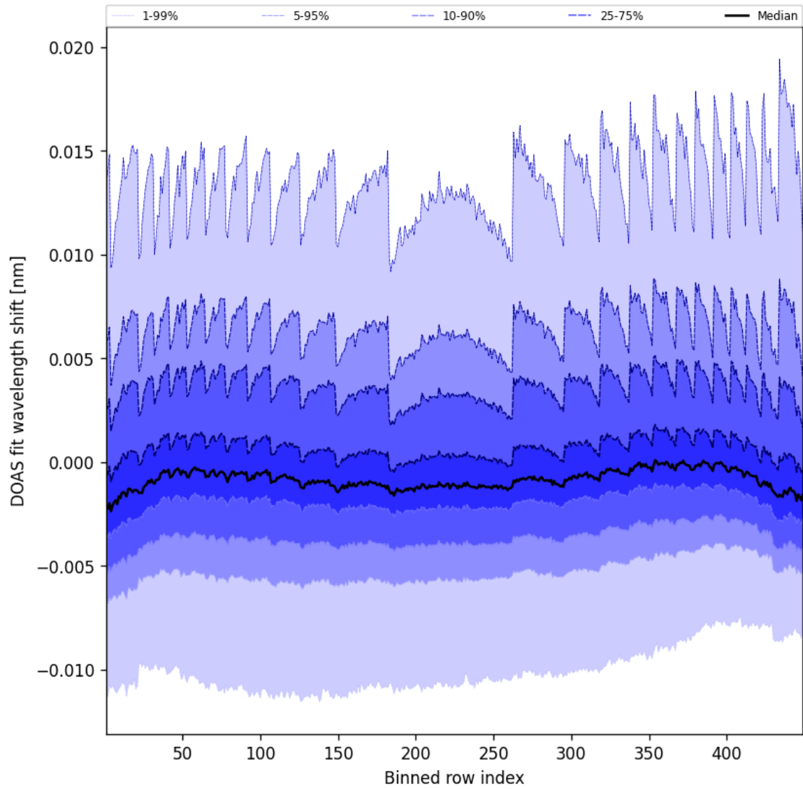
Figure 47: Along track statistics of "DOAS fit wavelength shift" for 2025-04-07 to 2025-04-08
