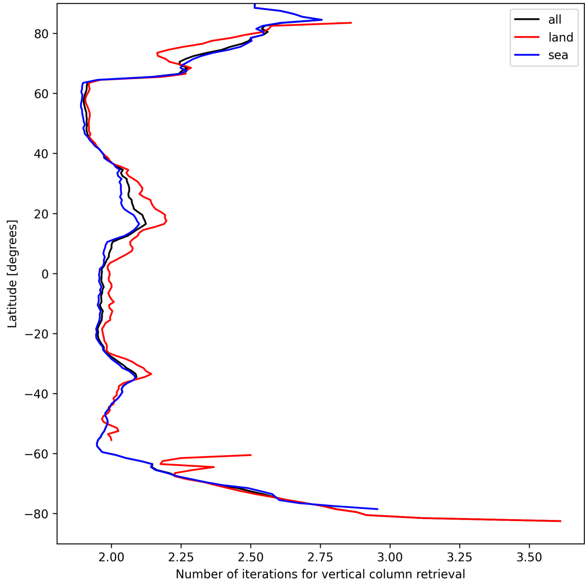
Figure 27: Zonal average of “Number of iterations for vertical column retrieval” for 2025-04-07 to 2025-04-08.
