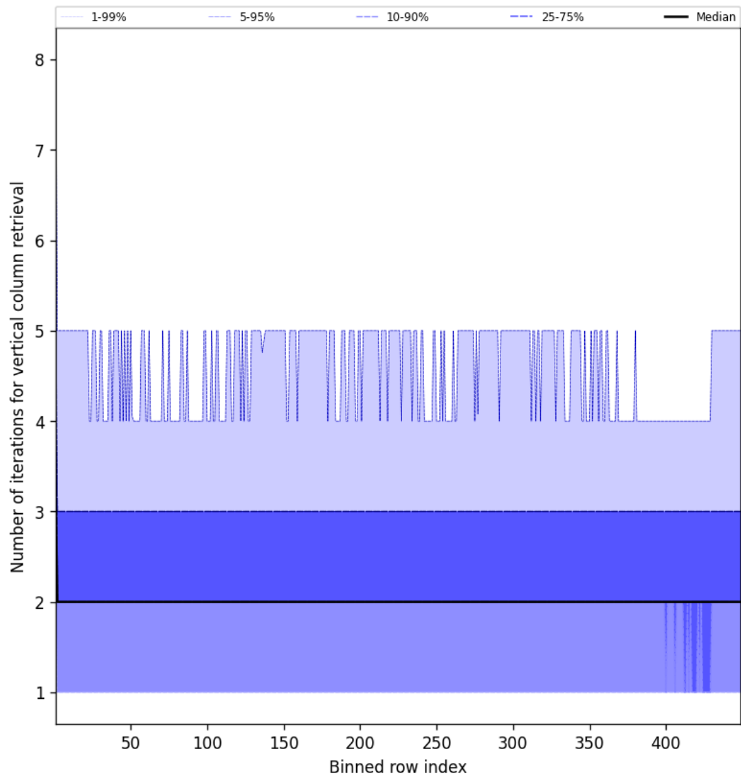
Figure 51: Along track statistics of “Number of iterations for vertical column retrieval” for 2025-04-07 to 2025-04-08
