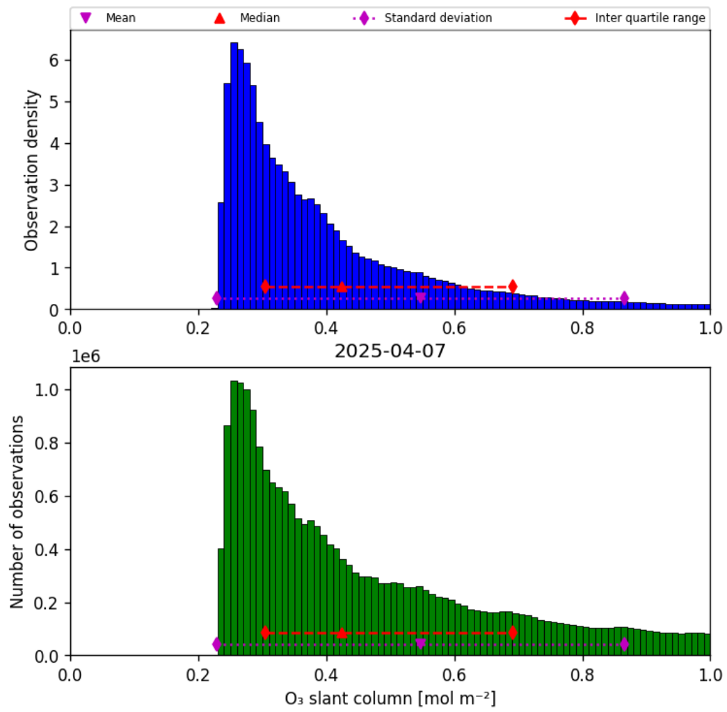
Figure 31: Histogram of “O 3 slant column” for 2025-04-07 to 2025-04-08
