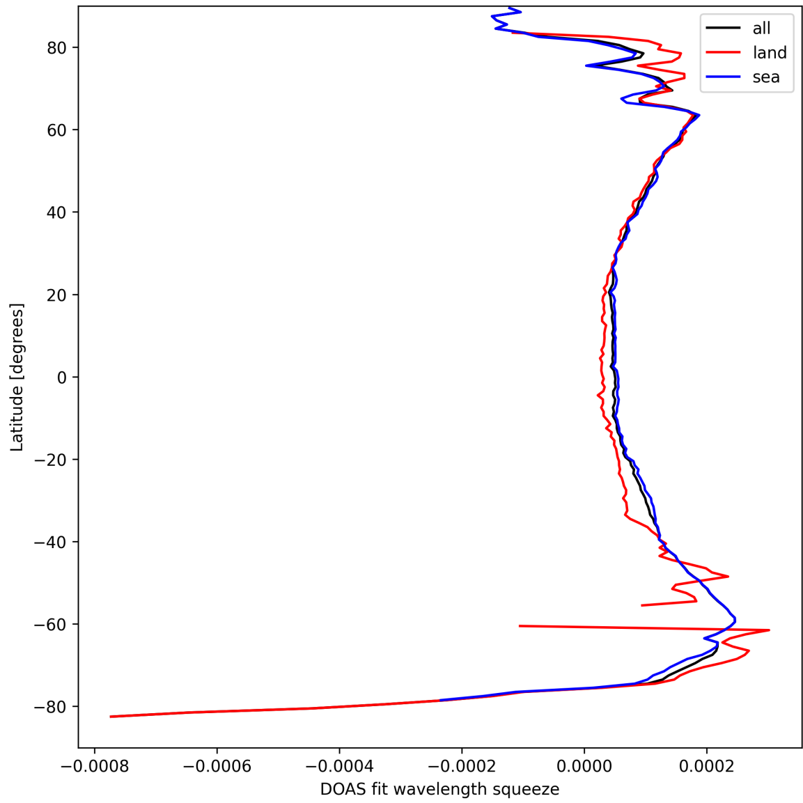
Figure 24: Zonal average of “DOAS fit wavelength squeeze” for 2025-04-07 to 2025-04-08.
