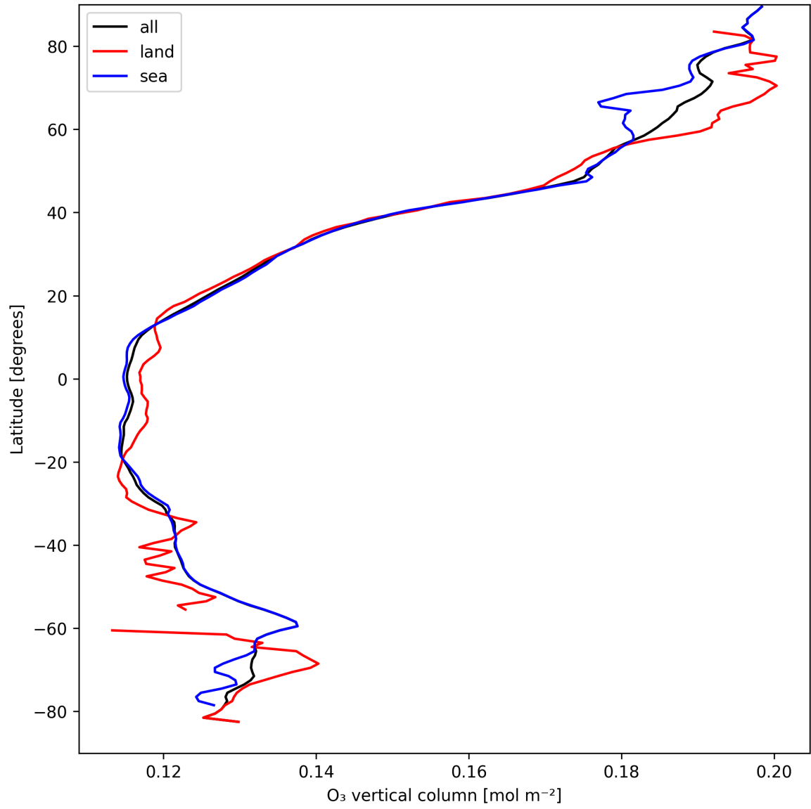
Figure 17: Zonal average of “O 3 vertical column” for 2025-04-07 to 2025-04-08.
