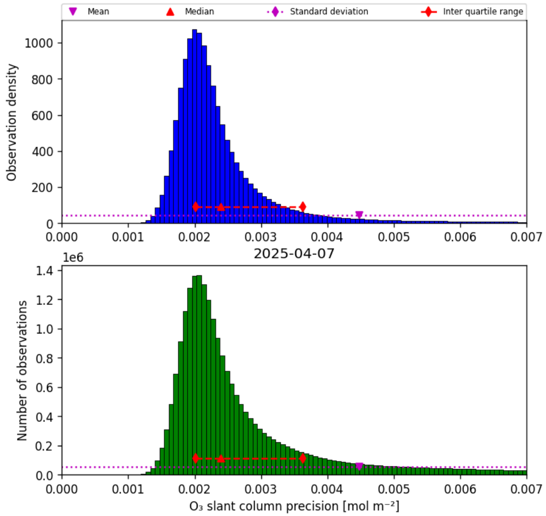
Figure 32: Histogram of “O 3 slant column precision” for 2025-04-07 to 2025-04-08
