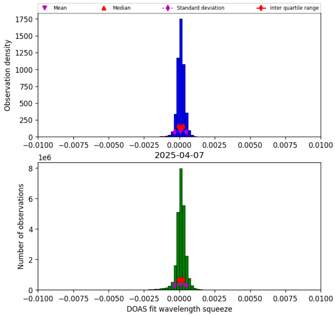
Figure 36: Histogram of “DOAS fit wavelength squeeze” for 2025-04-07 to 2025-04-08
