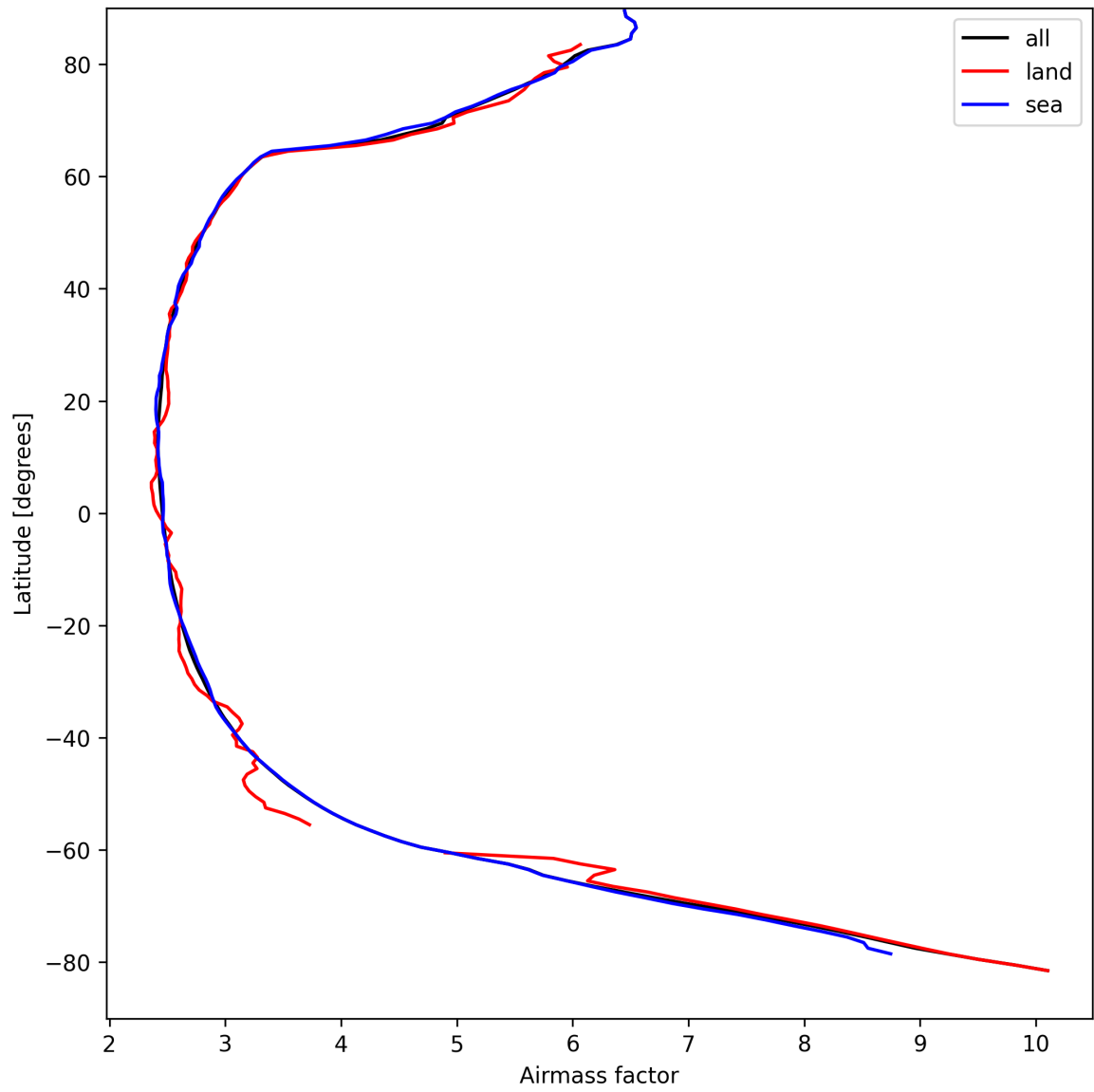
Figure 25: Zonal average of “Airmass factor” for 2025-04-08 to 2025-04-09.
