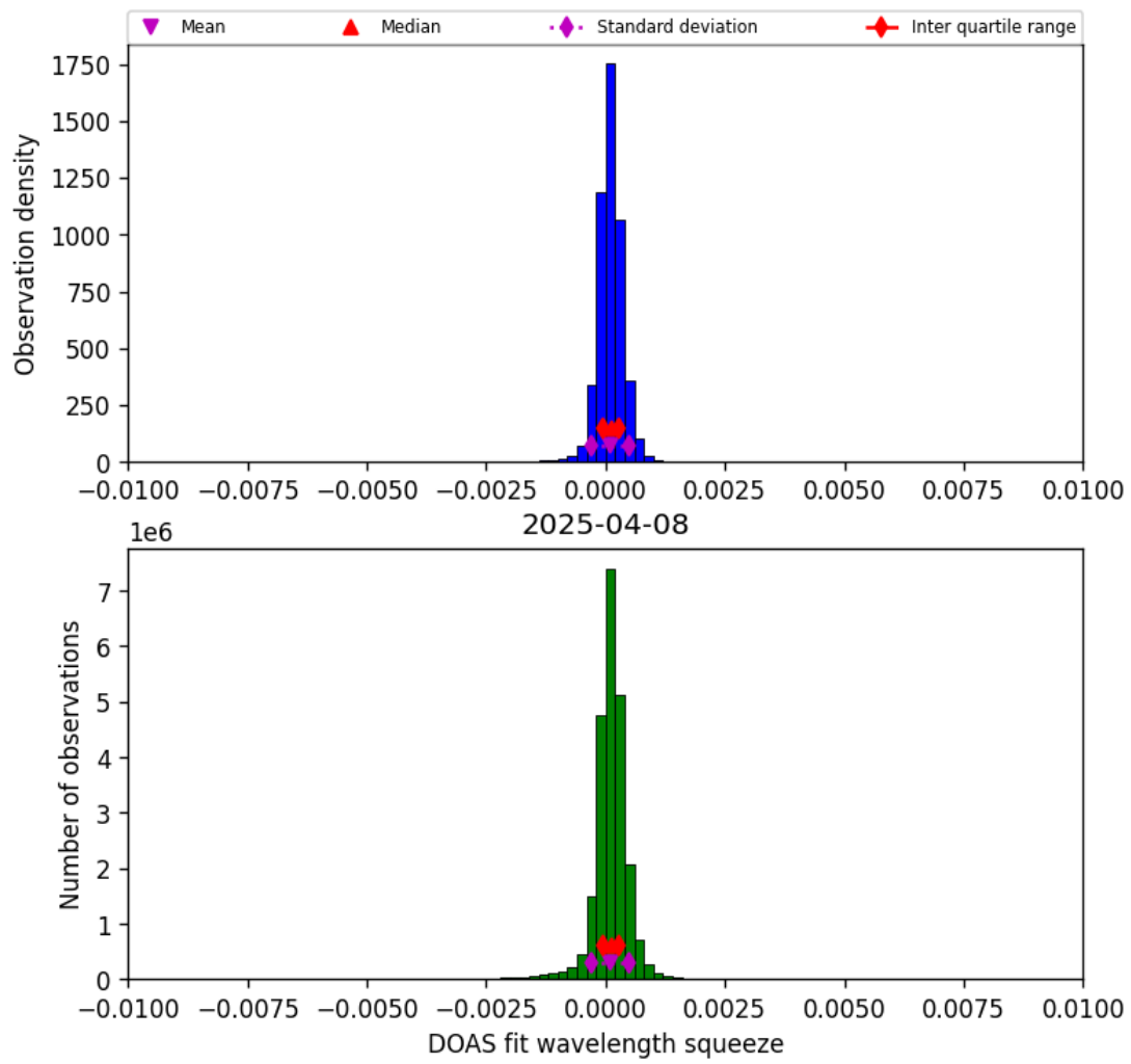
Figure 36: Histogram of “DOAS fit wavelength squeeze” for 2025-04-08 to 2025-04-09
