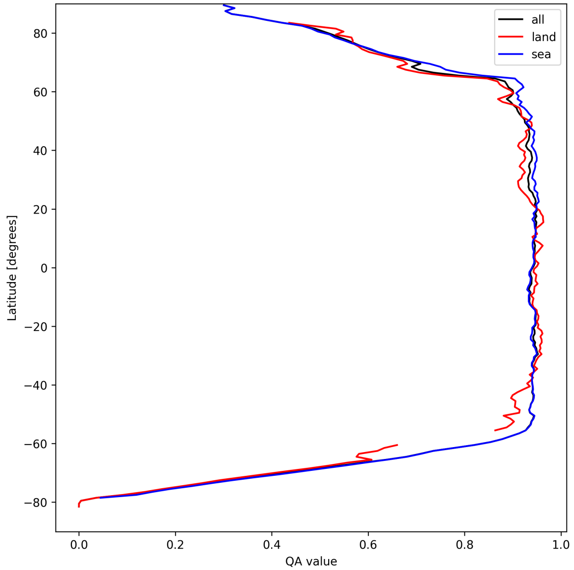
Figure 16: Zonal average of “QA value” for 2025-04-08 to 2025-04-09.
