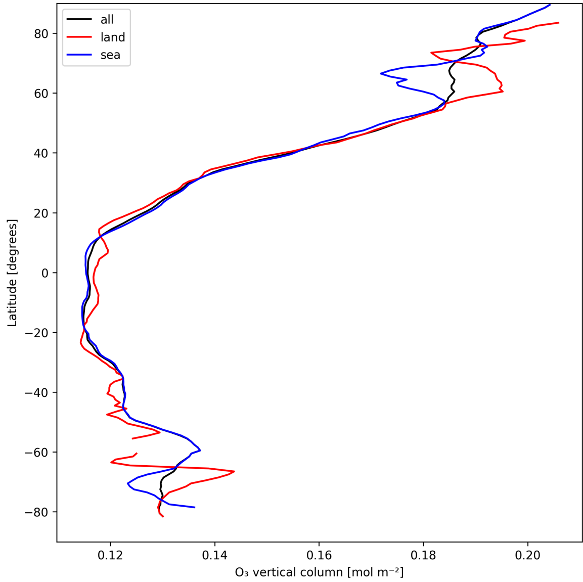
Figure 17: Zonal average of “O 3 vertical column” for 2025-04-08 to 2025-04-09.
