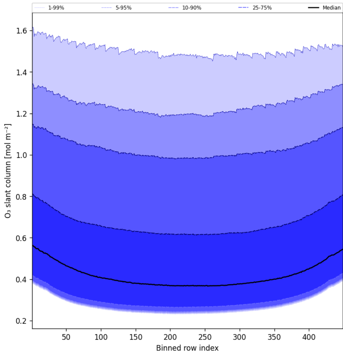
Figure 43: Along track statistics of “O 3 slant column” for 2025-04-08 to 2025-04-09
