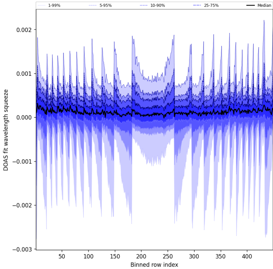
Figure 48: Along track statistics of “DOAS fit wavelength squeeze” for 2025-04-08 to 2025-04-09
