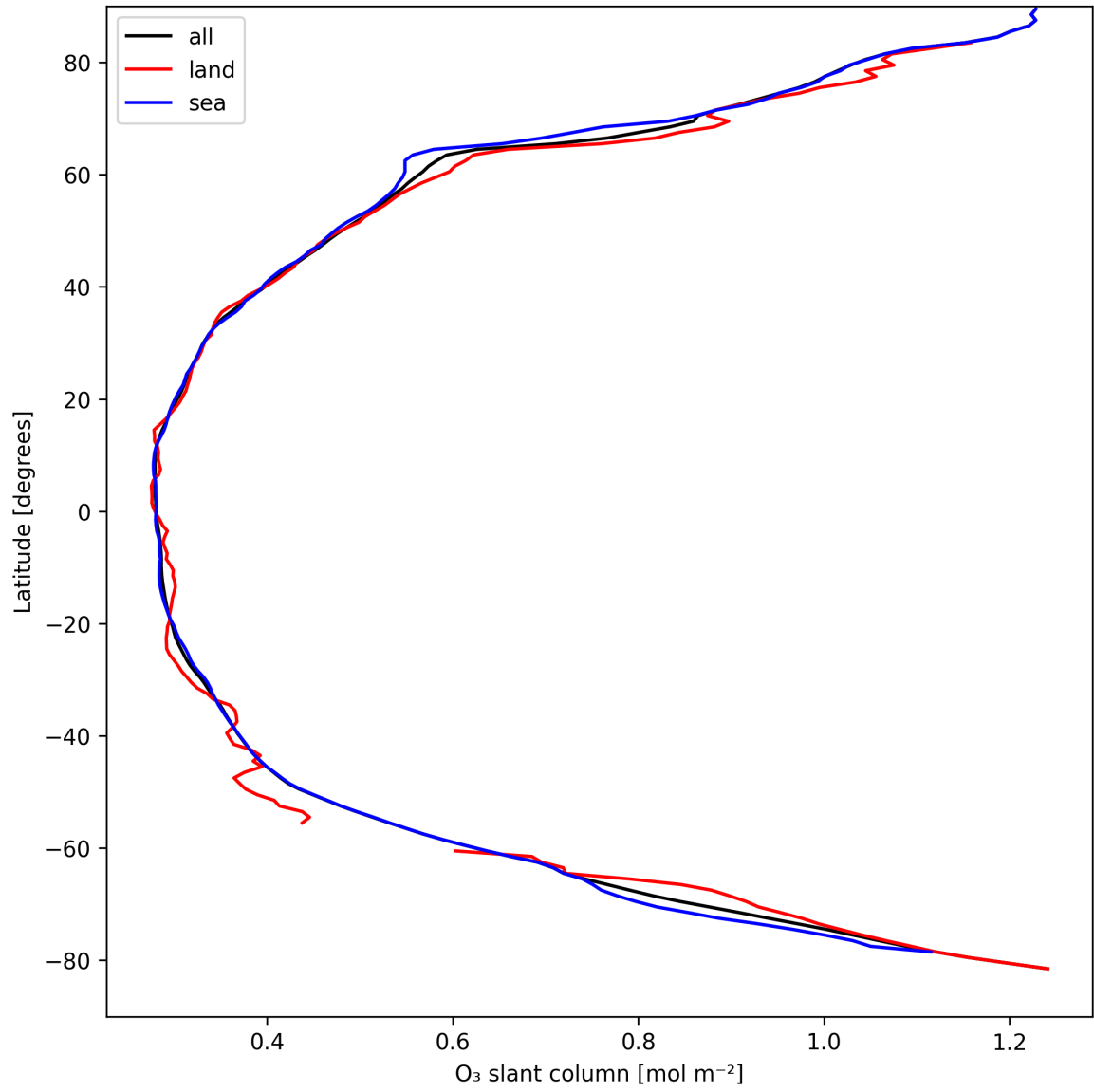
Figure 19: Zonal average of “O 3 slant column” for 2025-04-08 to 2025-04-09.
