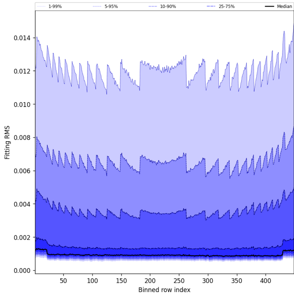
Figure 46: Along track statistics of “Fitting RMS” for 2025-04-09 to 2025-04-10
