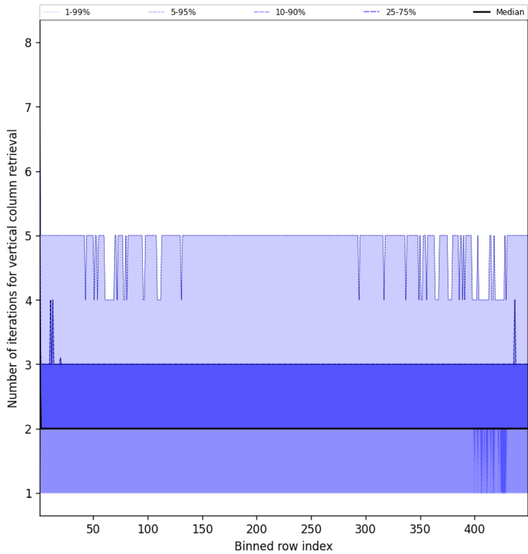
Figure 51: Along track statistics of “Number of iterations for vertical column retrieval” for 2025-04-09 to 2025-04-10
