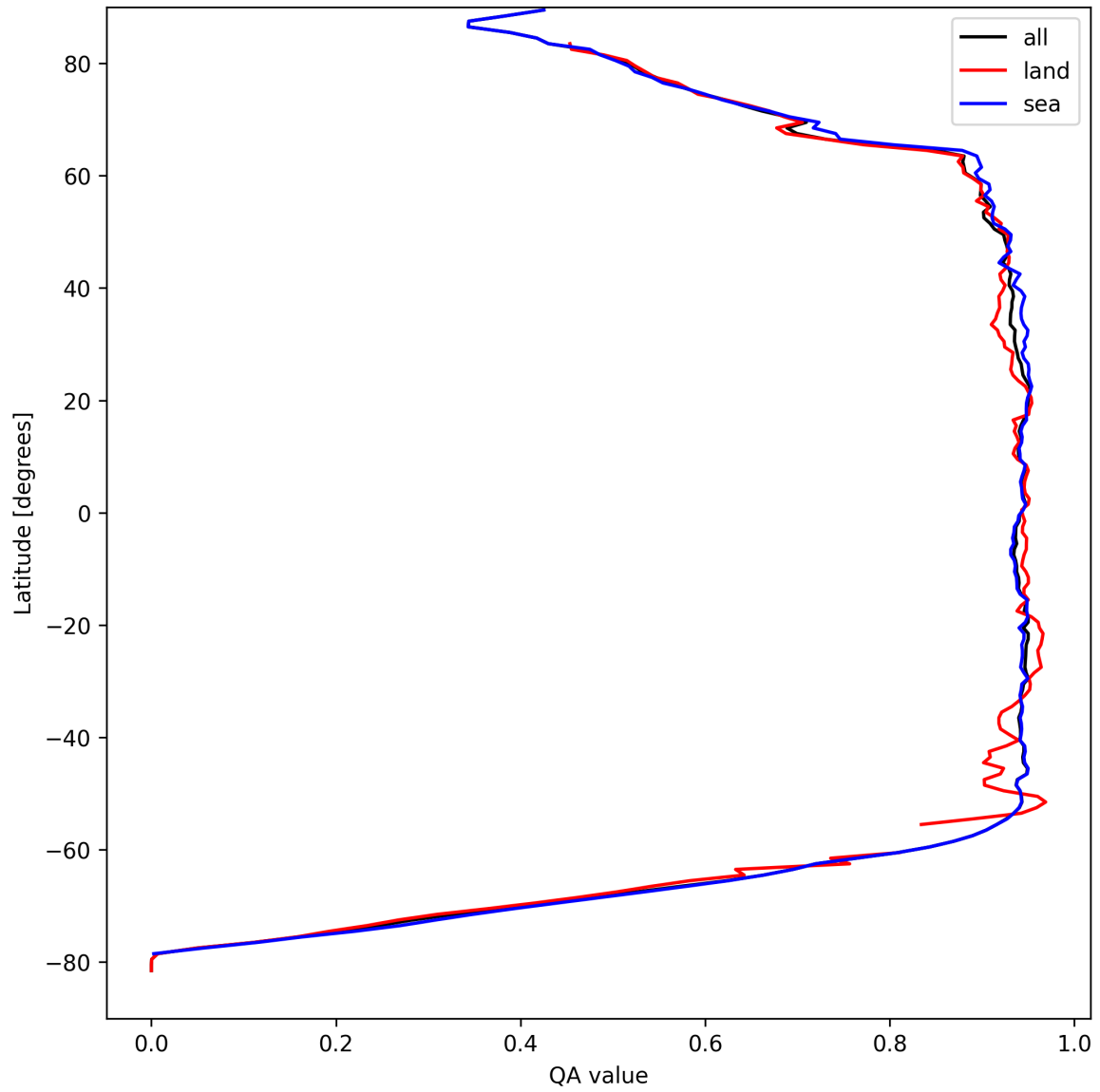
Figure 16: Zonal average of “QA value” for 2025-04-09 to 2025-04-10.
