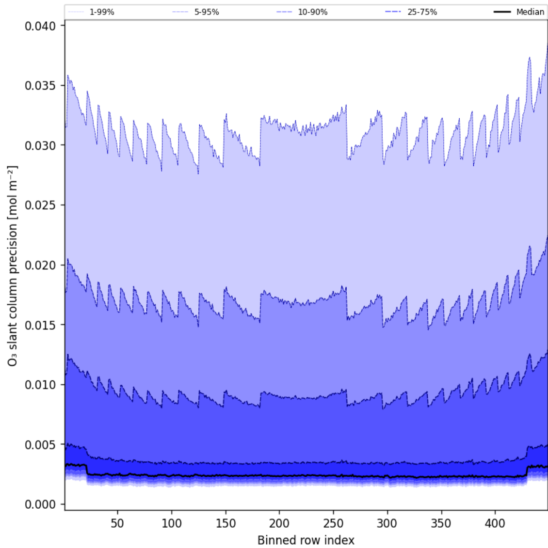
Figure 44: Along track statistics of “O 3 slant column precision” for 2025-04-09 to 2025-04-10
