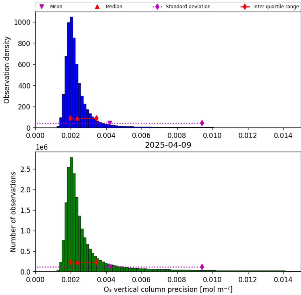
Figure 30: Histogram of “O 3 vertical column precision” for 2025-04-09 to 2025-04-10
