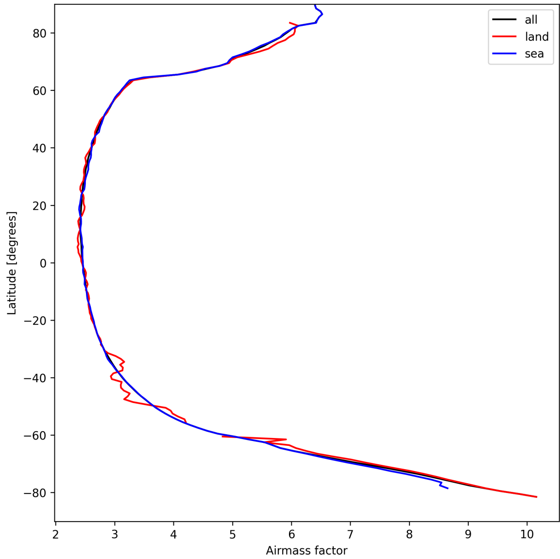
Figure 25: Zonal average of “Airmass factor” for 2025-04-09 to 2025-04-10.
