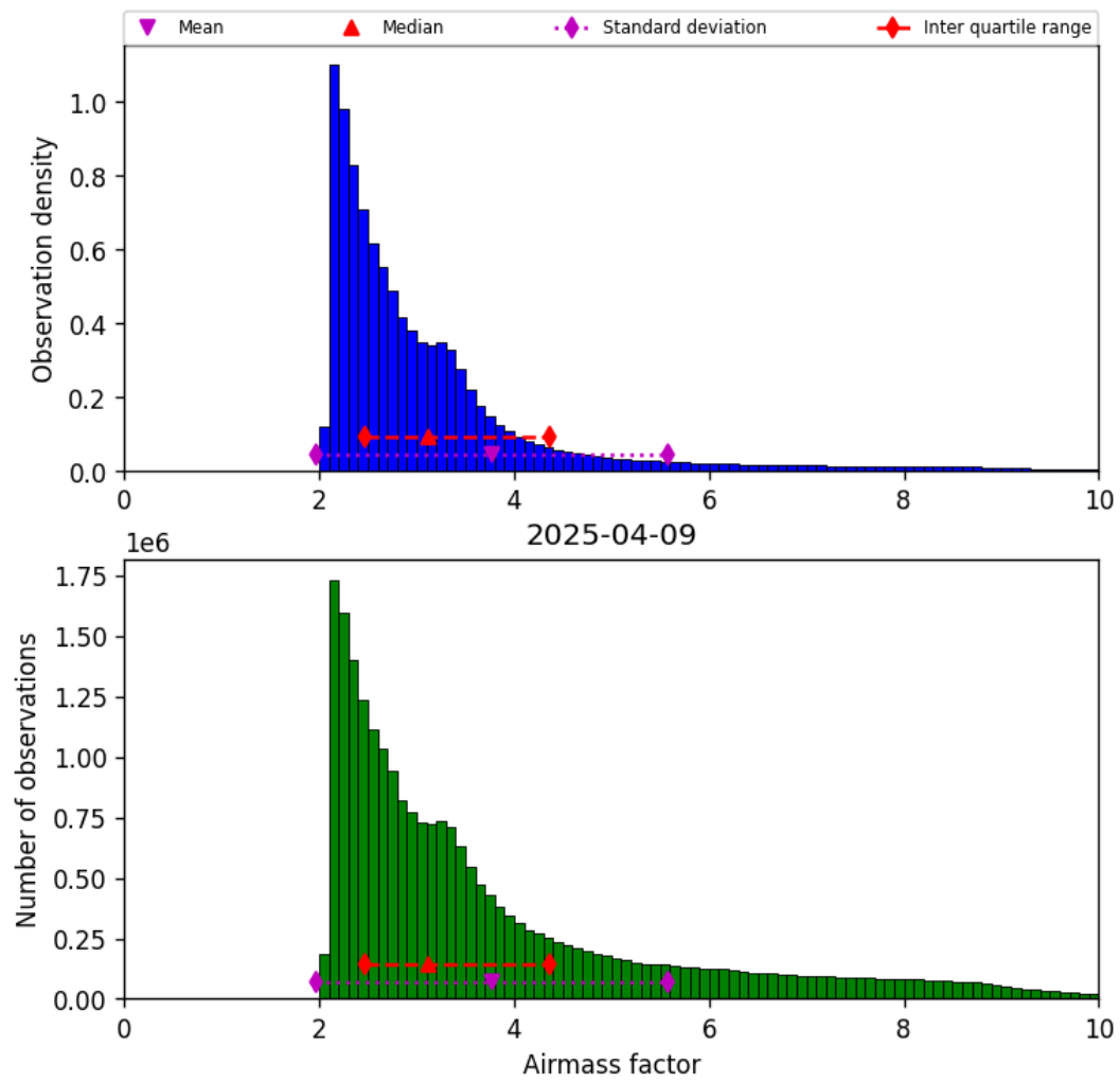
Figure 37: Histogram of “Airmass factor” for 2025-04-09 to 2025-04-10
