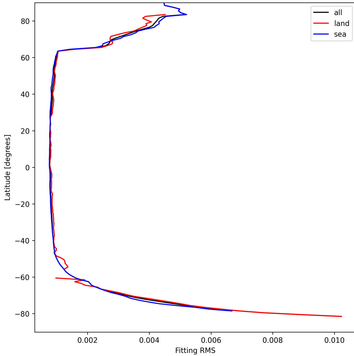
Figure 22: Zonal average of “Fitting RMS” for 2025-04-09 to 2025-04-10.
