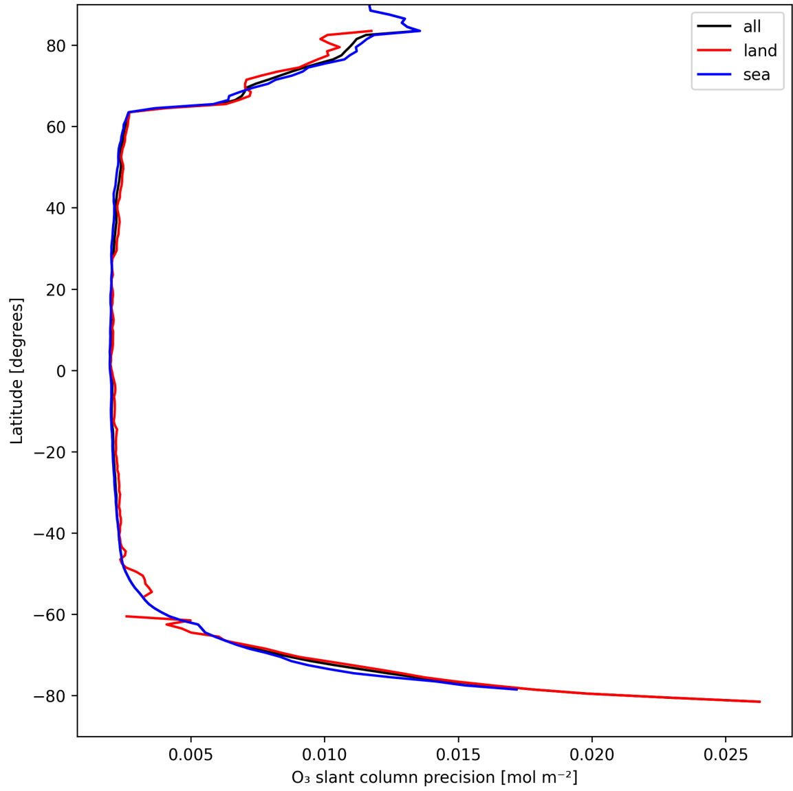
Figure 20: Zonal average of "O 3 slant column precision" for 2025-04-09 to 2025-04-10.
