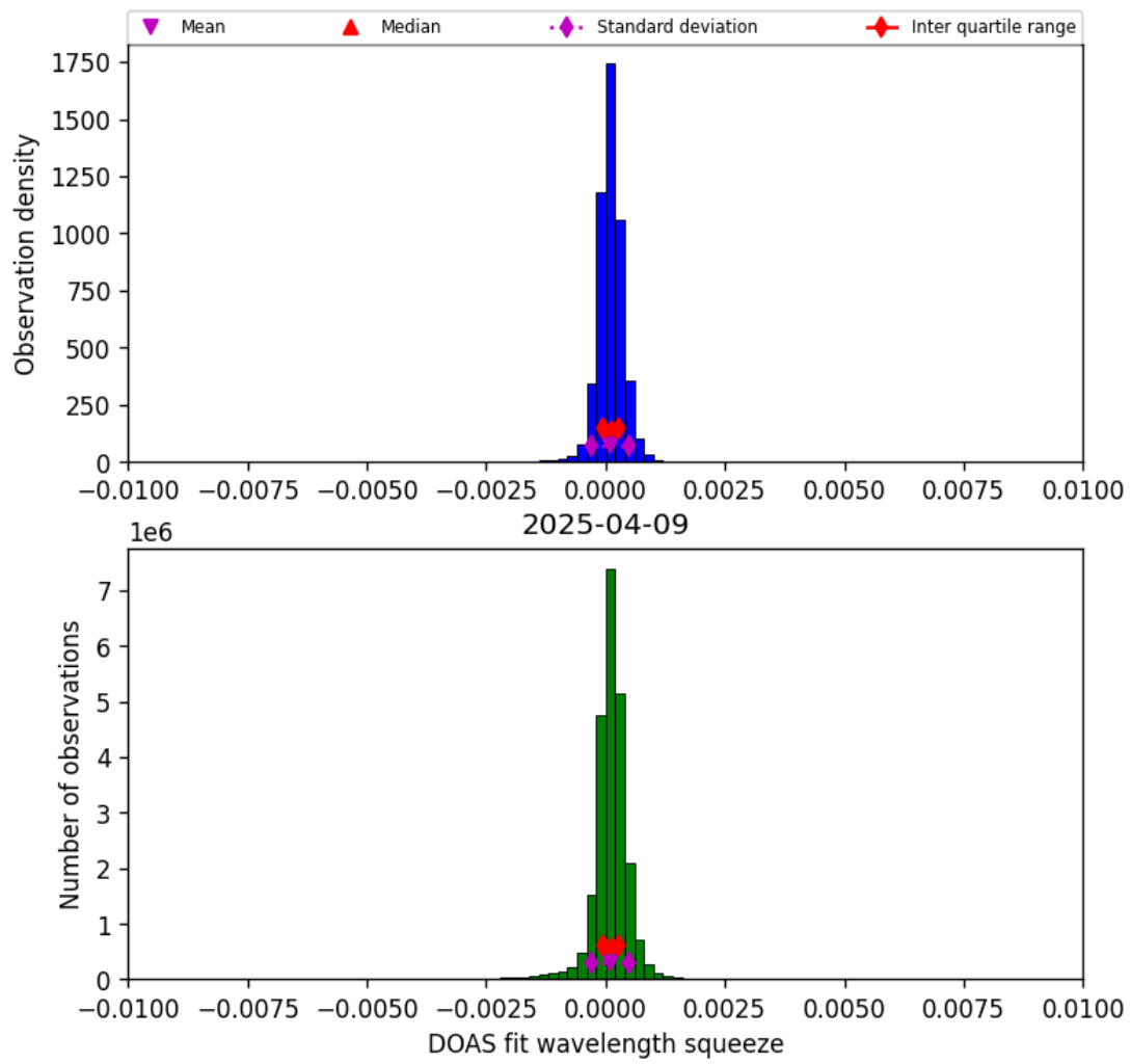
Figure 36: Histogram of “DOAS fit wavelength squeeze” for 2025-04-09 to 2025-04-10
