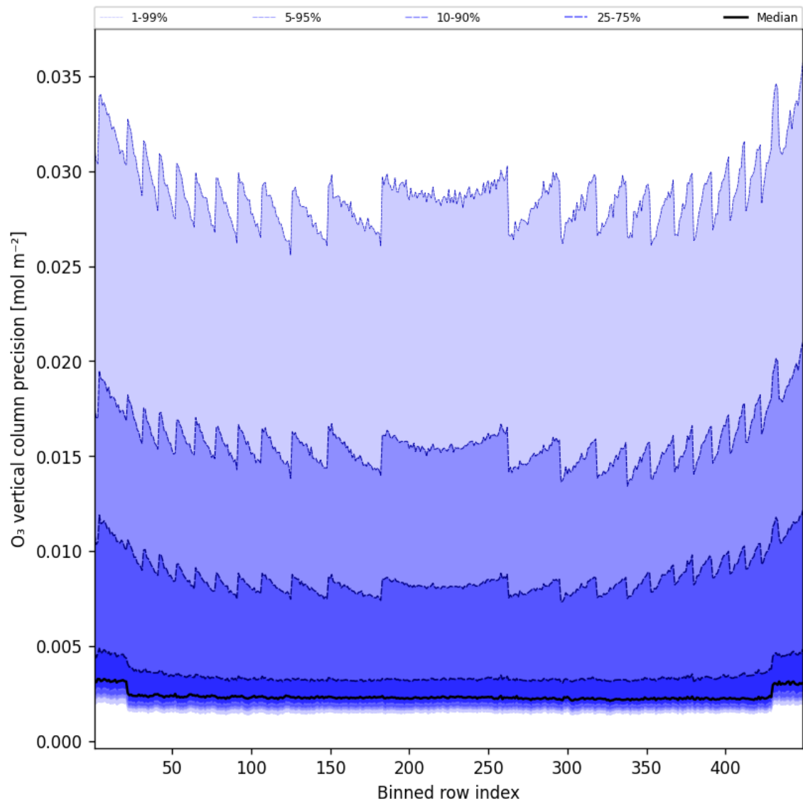
Figure 42: Along track statistics of “O 3 vertical column precision” for 2025-04-09 to 2025-04-10
