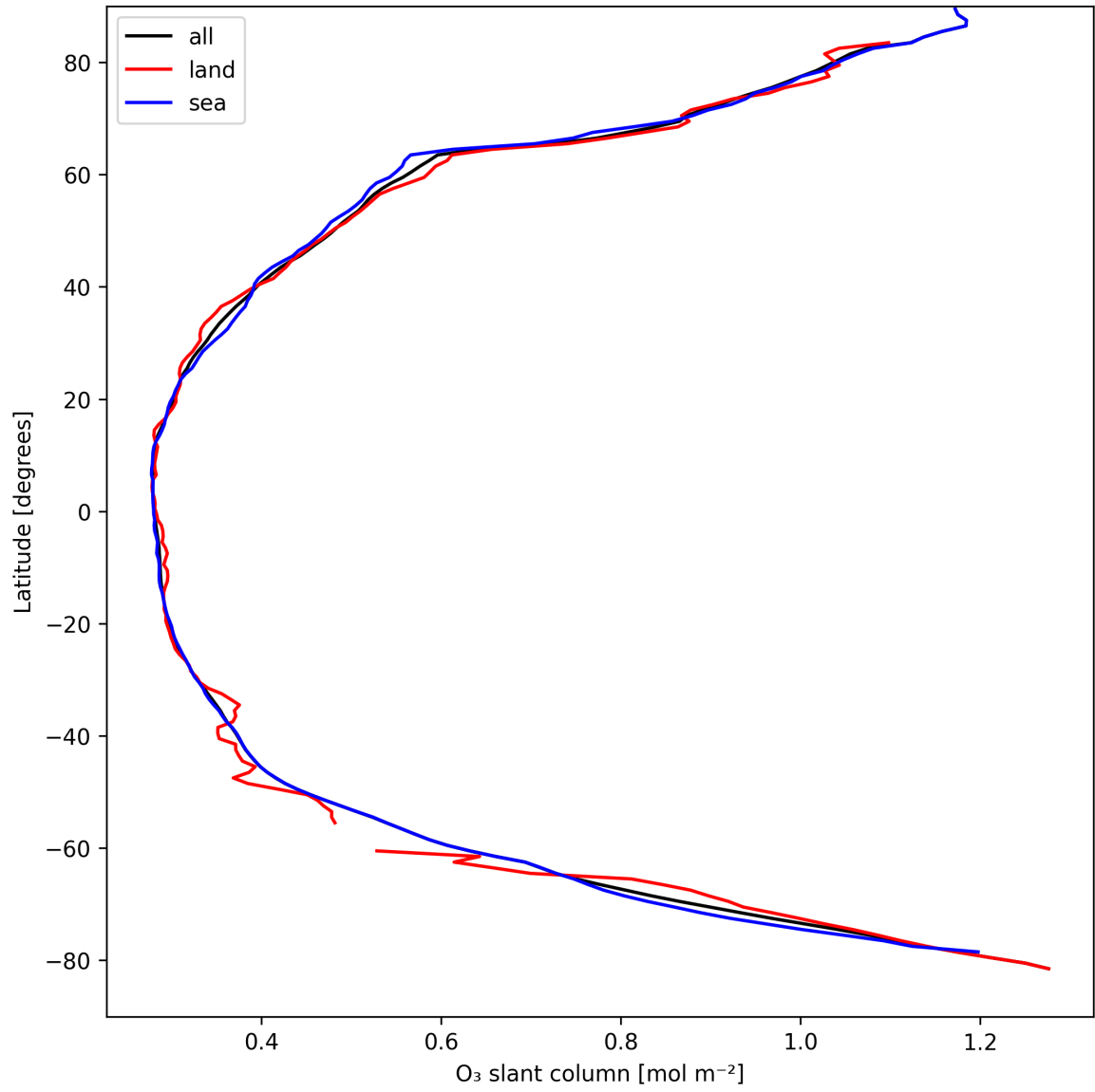
Figure 19: Zonal average of “O 3 slant column” for 2025-04-09 to 2025-04-10.
