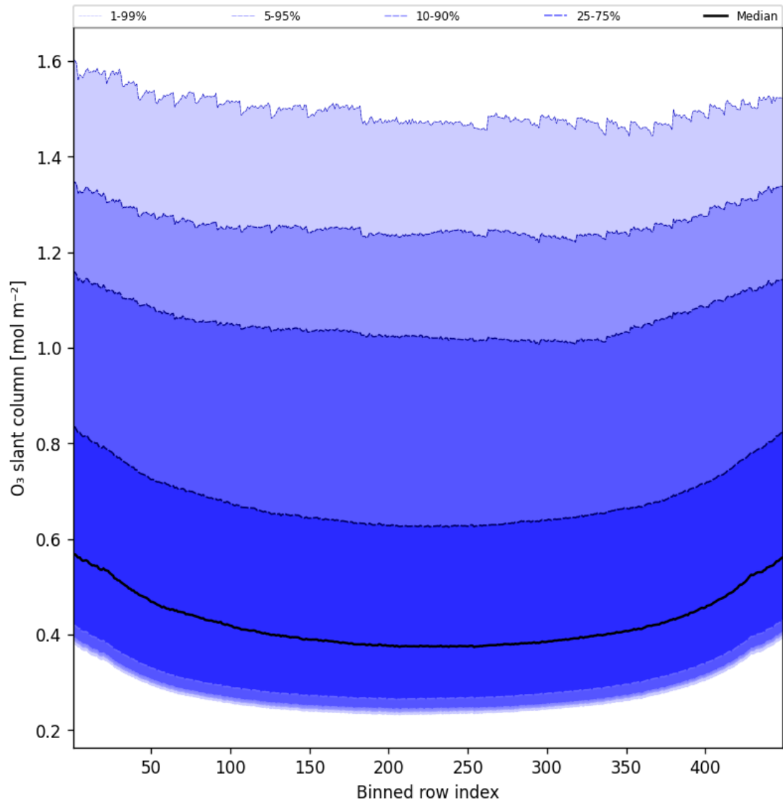
Figure 43: Along track statistics of “O 3 slant column” for 2025-04-09 to 2025-04-10
