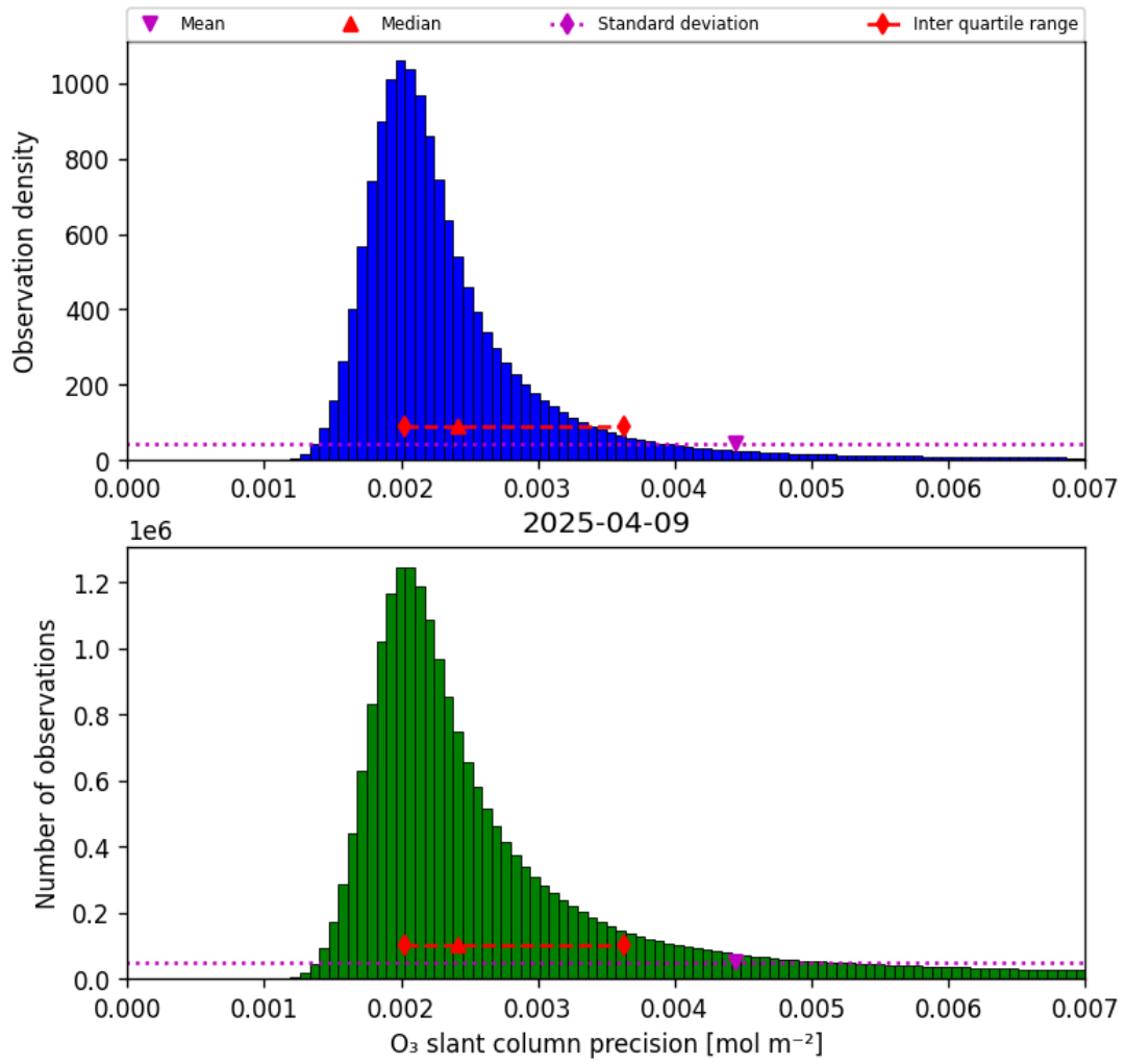
Figure 32: Histogram of “O 3 slant column precision” for 2025-04-09 to 2025-04-10
