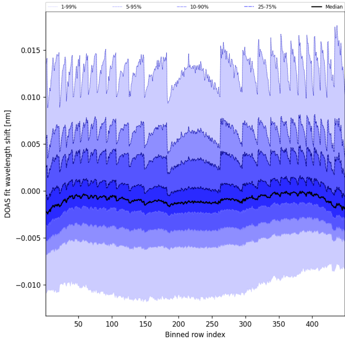
Figure 47: Along track statistics of “DOAS fit wavelength shift” for 2025-04-09 to 2025-04-10
