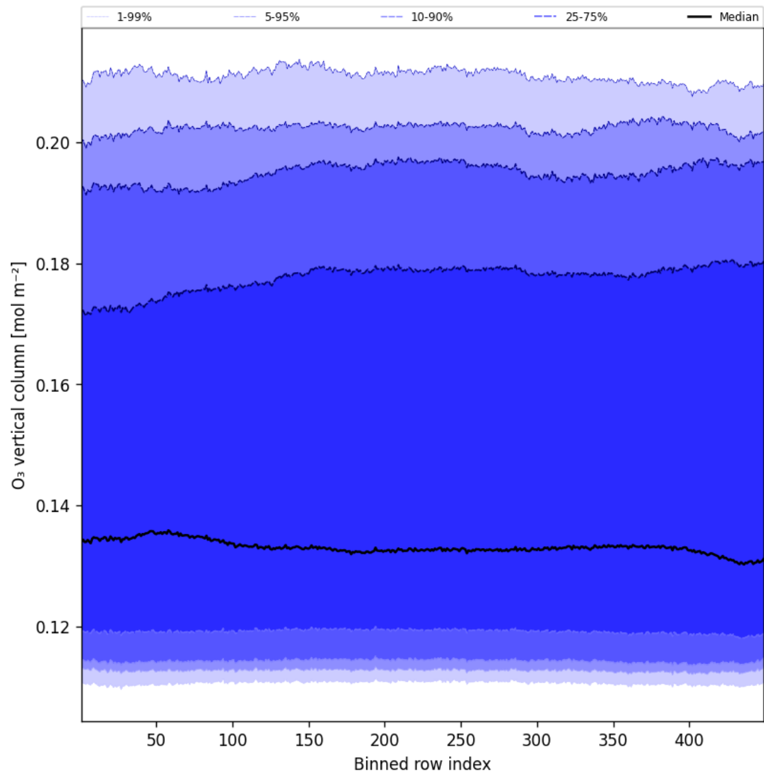
Figure 41: Along track statistics of “O 3 vertical column” for 2025-04-09 to 2025-04-10
