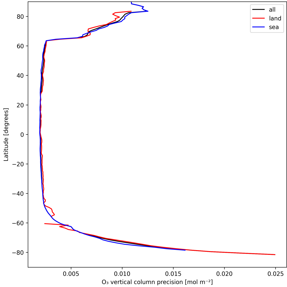
Figure 18: Zonal average of "O 3 vertical column precision" for 2025-04-09 to 2025-04-10.
