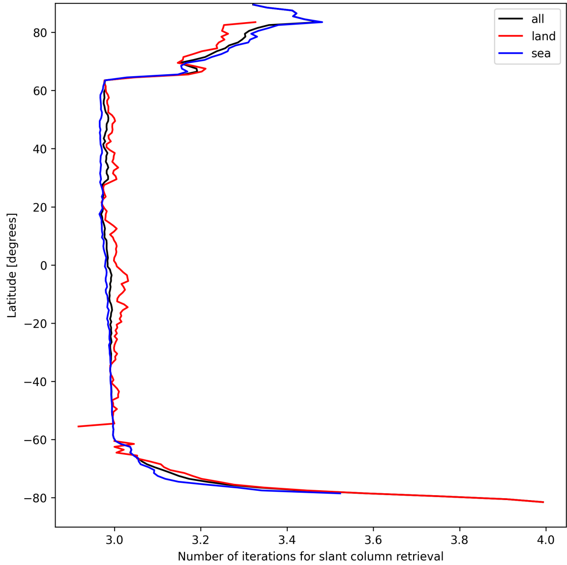
Figure 21: Zonal average of “Number of iterations for slant column retrieval” for 2025-04-09 to 2025-04-10.
