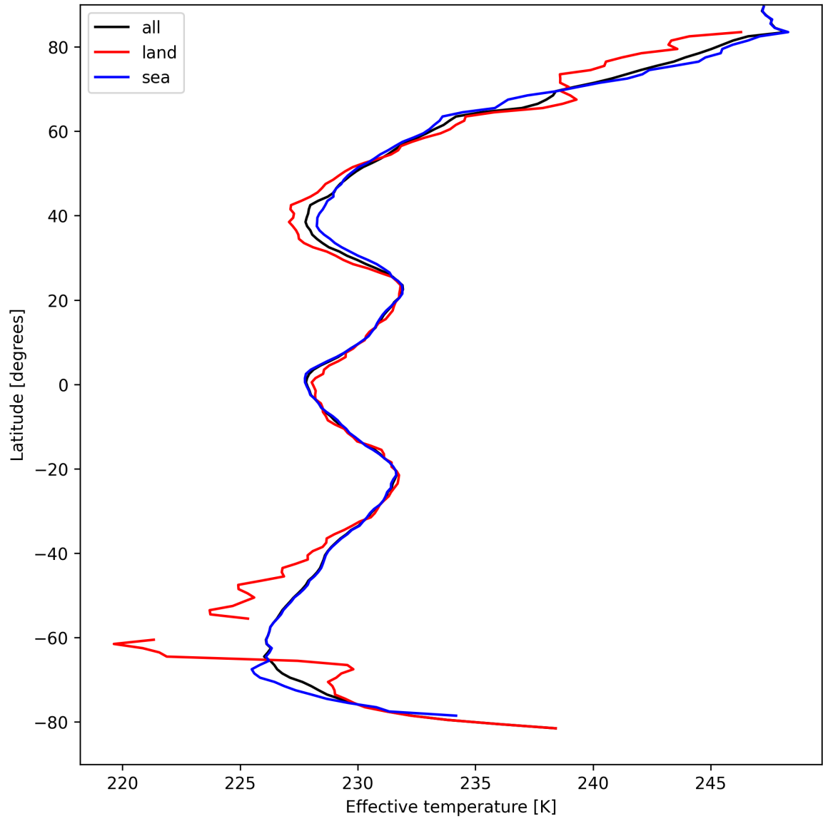
Figure 26: Zonal average of “Effective temperature” for 2025-04-09 to 2025-04-10.
