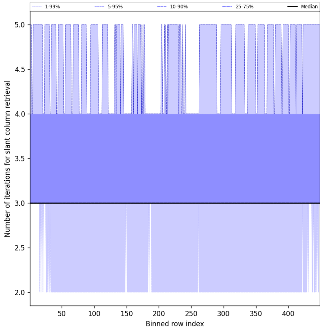
Figure 45: Along track statistics of “Number of iterations for slant column retrieval” for 2025-04-09 to 2025-04-10
