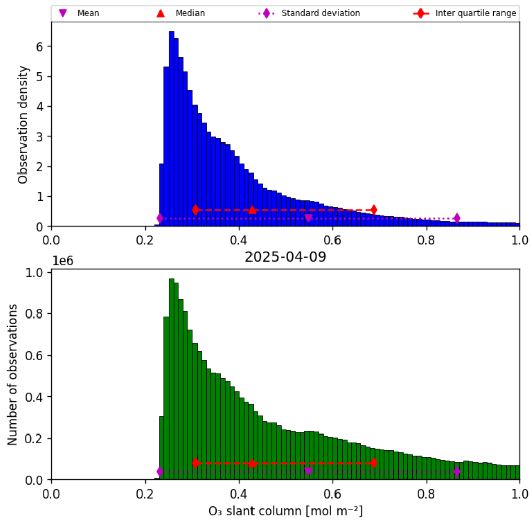
Figure 31: Histogram of “O 3 slant column” for 2025-04-09 to 2025-04-10
