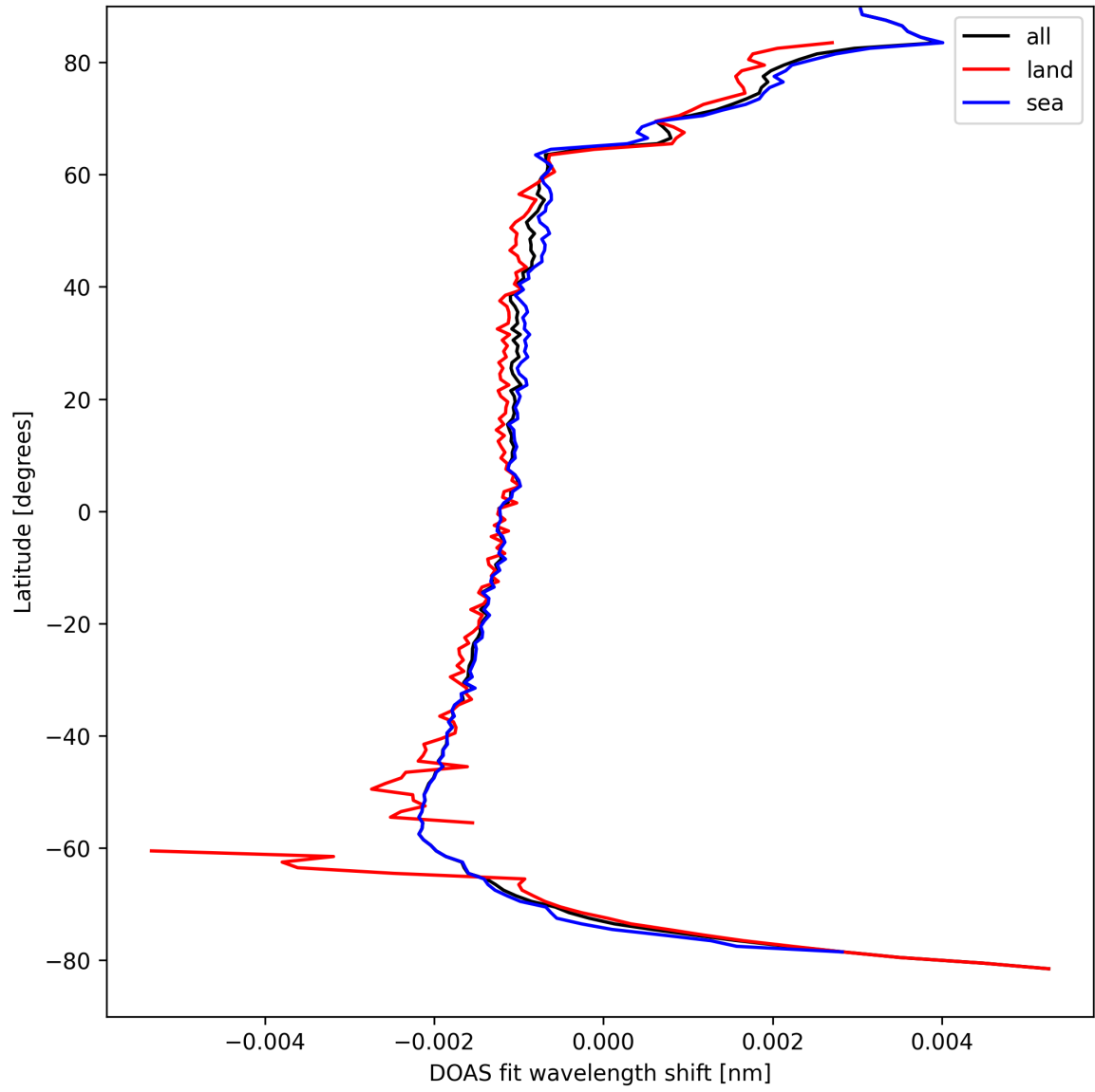
Figure 23: Zonal average of “DOAS fit wavelength shift” for 2025-04-09 to 2025-04-10.
