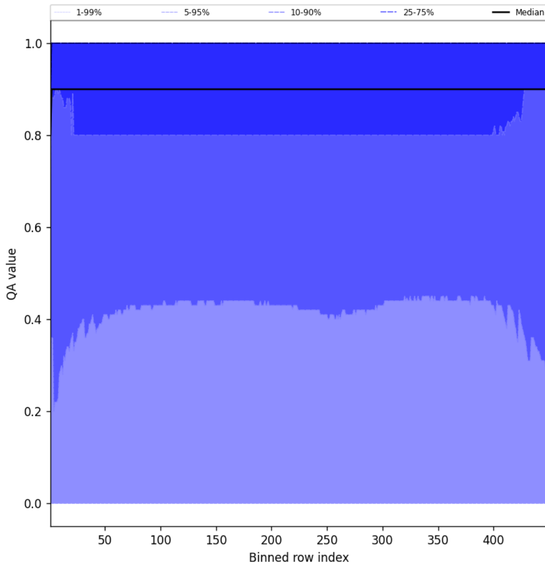
Figure 40: Along track statistics of “QA value” for 2025-04-09 to 2025-04-10
