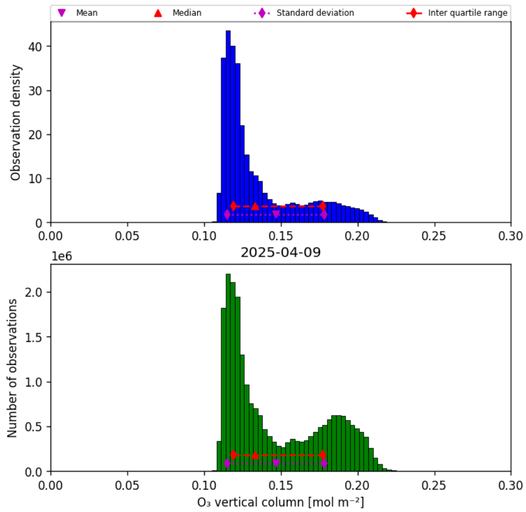
Figure 29: Histogram of “O 3 vertical column” for 2025-04-09 to 2025-04-10
