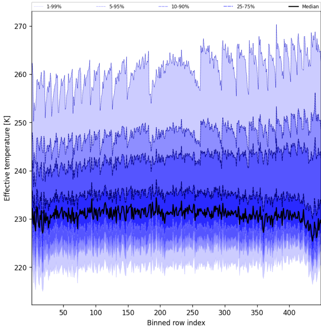
Figure 50: Along track statistics of “Effective temperature” for 2025-04-09 to 2025-04-10
