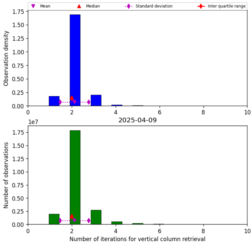
Figure 39: Histogram of “Number of iterations for vertical column retrieval” for 2025-04-09 to 2025-04-10
