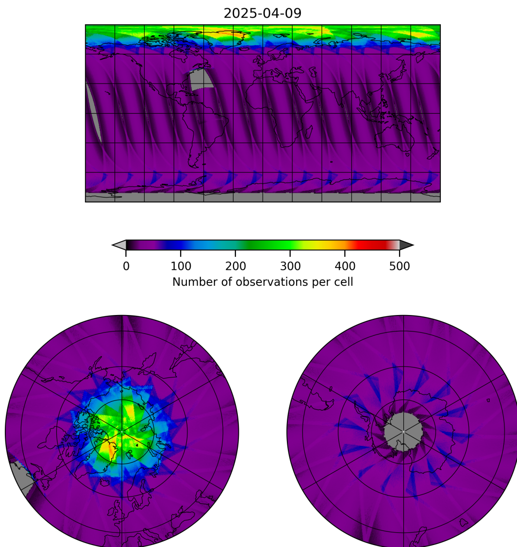
Figure 15: Map of the number of observations for 2025-04-09 to 2025-04-10
