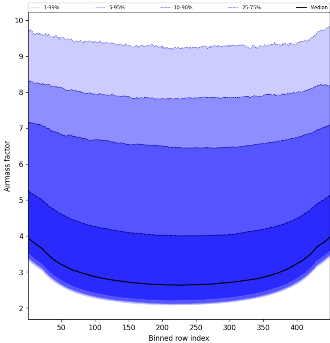
Figure 49: Along track statistics of “Airmass factor” for 2025-04-09 to 2025-04-10
