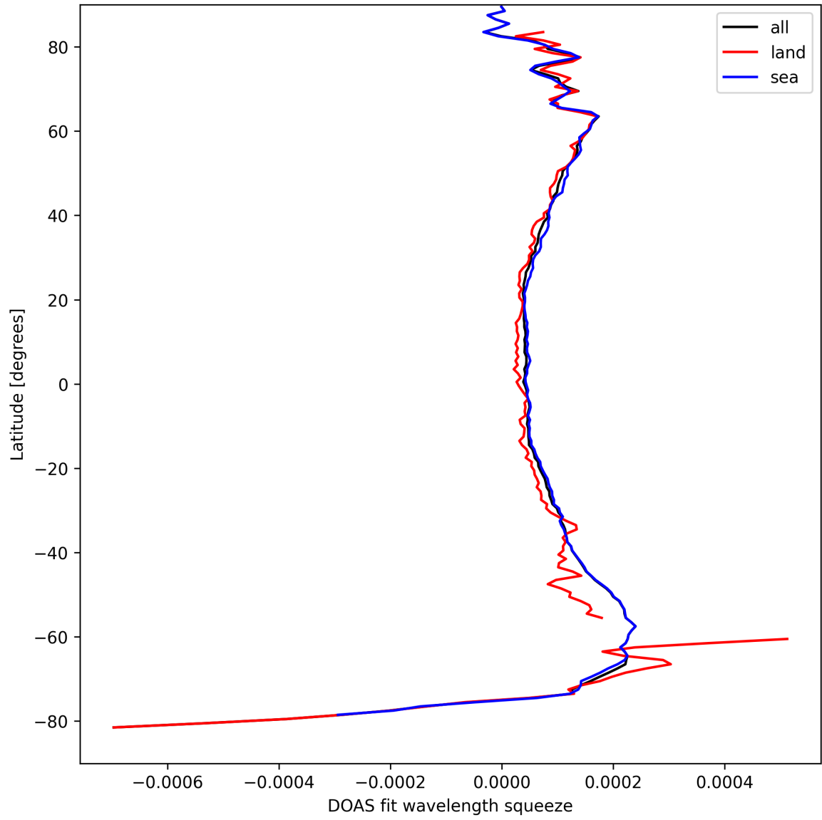
Figure 24: Zonal average of “DOAS fit wavelength squeeze” for 2025-04-09 to 2025-04-10.
