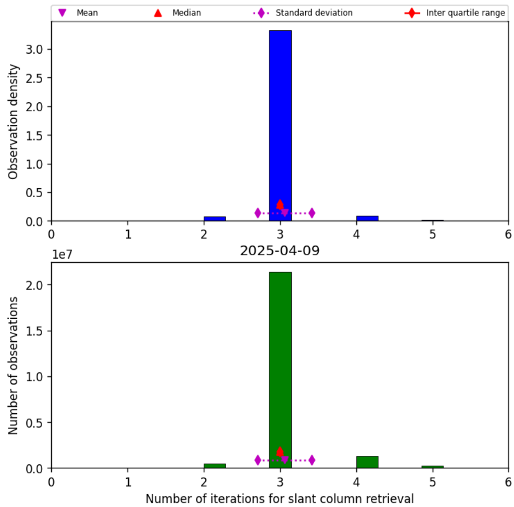
Figure 33: Histogram of “Number of iterations for slant column retrieval” for 2025-04-09 to 2025-04-10
