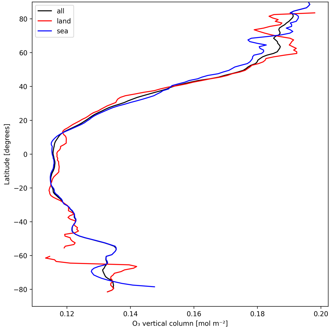
Figure 17: Zonal average of “O 3 vertical column” for 2025-04-09 to 2025-04-10.
