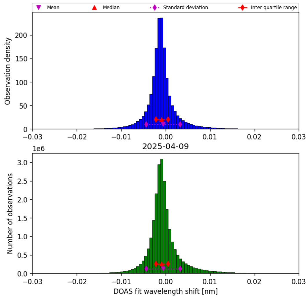
Figure 35: Histogram of “DOAS fit wavelength shift” for 2025-04-09 to 2025-04-10
