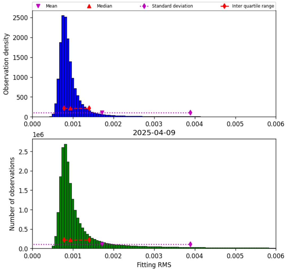
Figure 34: Histogram of “Fitting RMS” for 2025-04-09 to 2025-04-10
