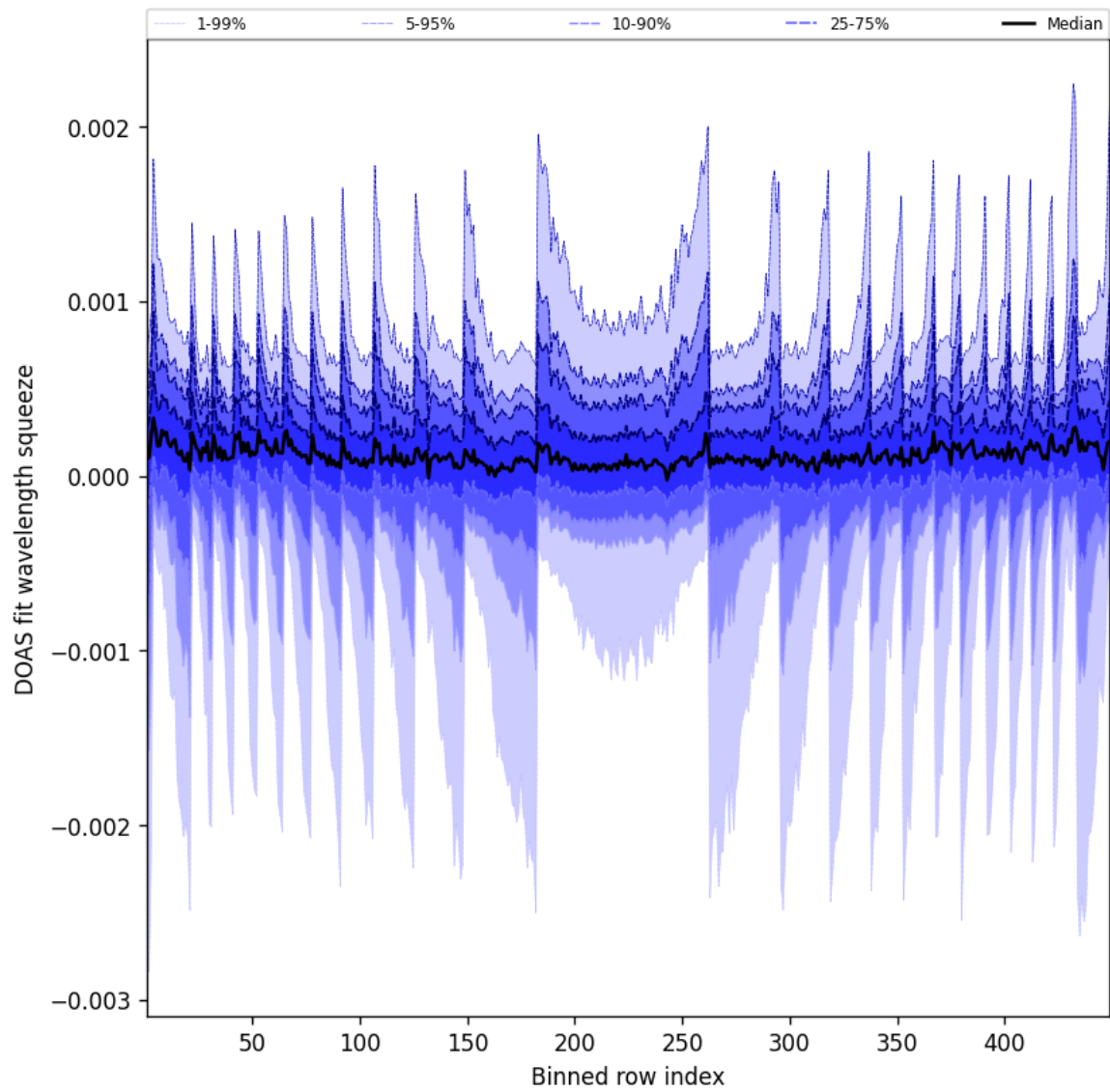
Figure 48: Along track statistics of “DOAS fit wavelength squeeze” for 2025-04-09 to 2025-04-10
