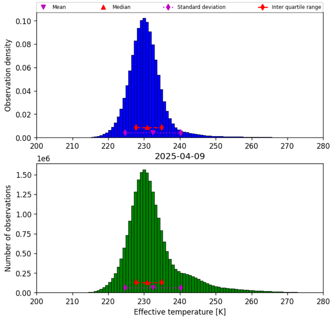
Figure 38: Histogram of “Effective temperature” for 2025-04-09 to 2025-04-10
