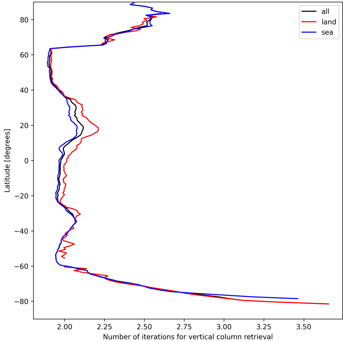
Figure 27: Zonal average of “Number of iterations for vertical column retrieval” for 2025-04-09 to 2025-04-10.
